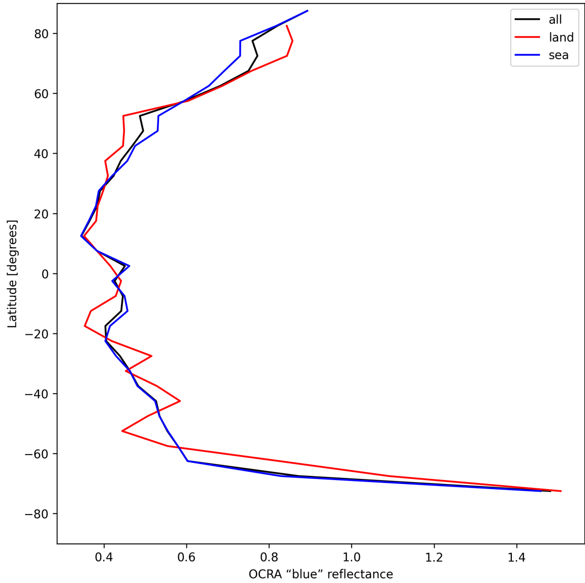
Figure 33: Zonal average of “OCRA “blue” reflectance” for 2025-05-09 to 2025-05-10.
