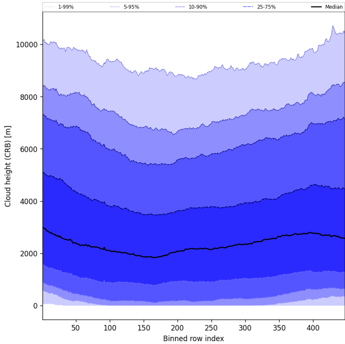
Figure 57: Along track statistics of “Cloud height (CRB)” for 2025-05-09 to 2025-05-10
