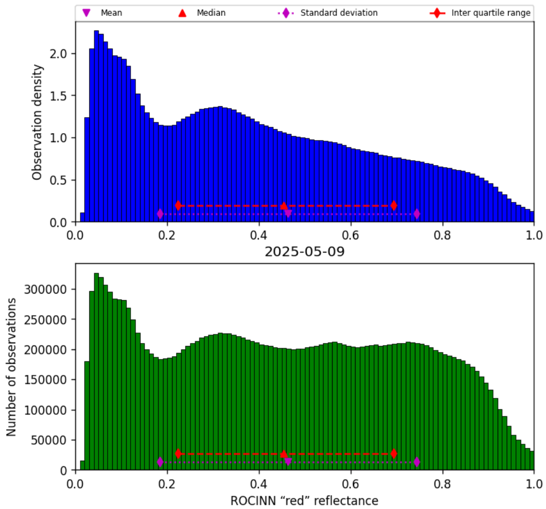
Figure 51: Histogram of “ROCINN “red” reflectance” for 2025-05-09 to 2025-05-10
