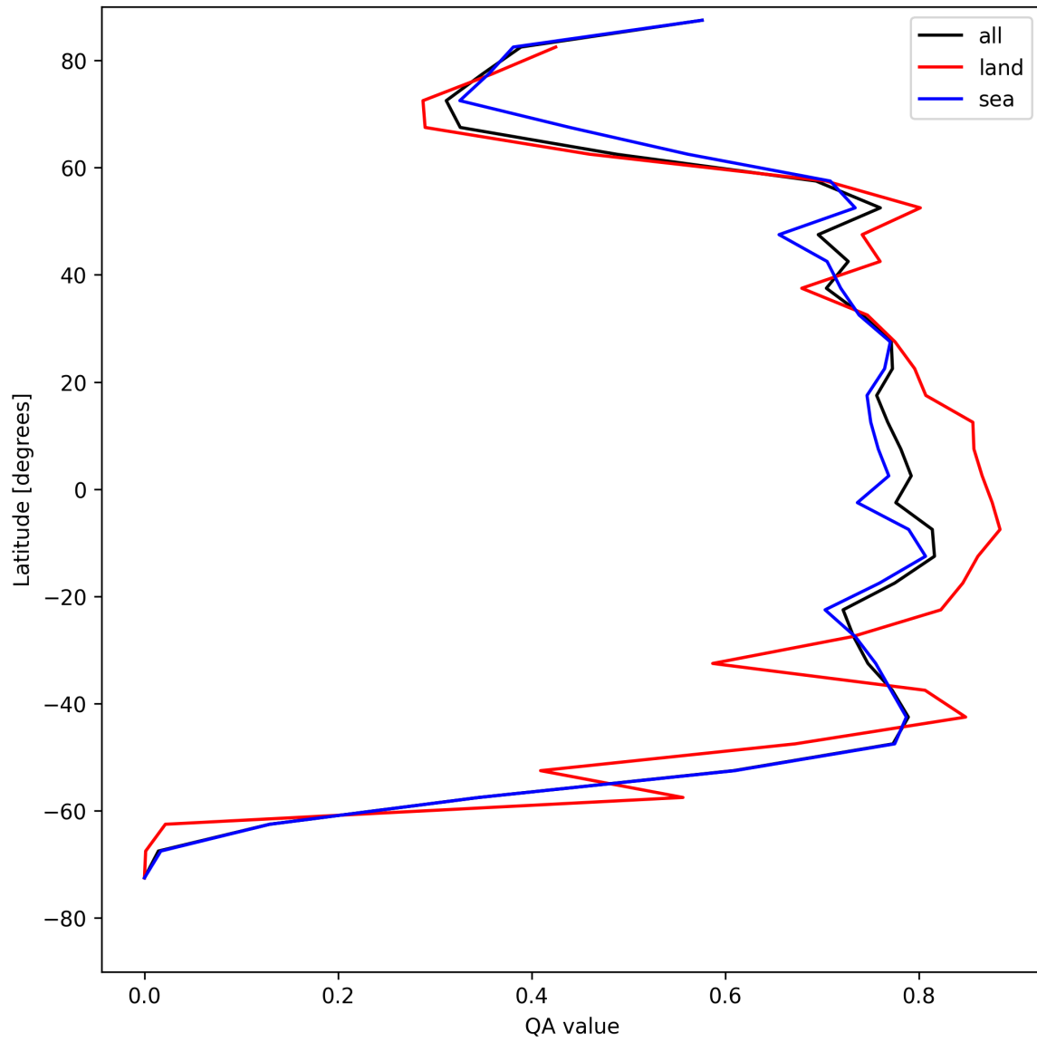
Figure 20: Zonal average of “QA value” for 2025-05-09 to 2025-05-10.
