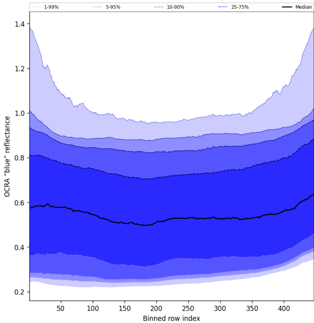
Figure 65: Along track statistics of “OCRA “blue” reflectance” for 2025-05-09 to 2025-05-10
