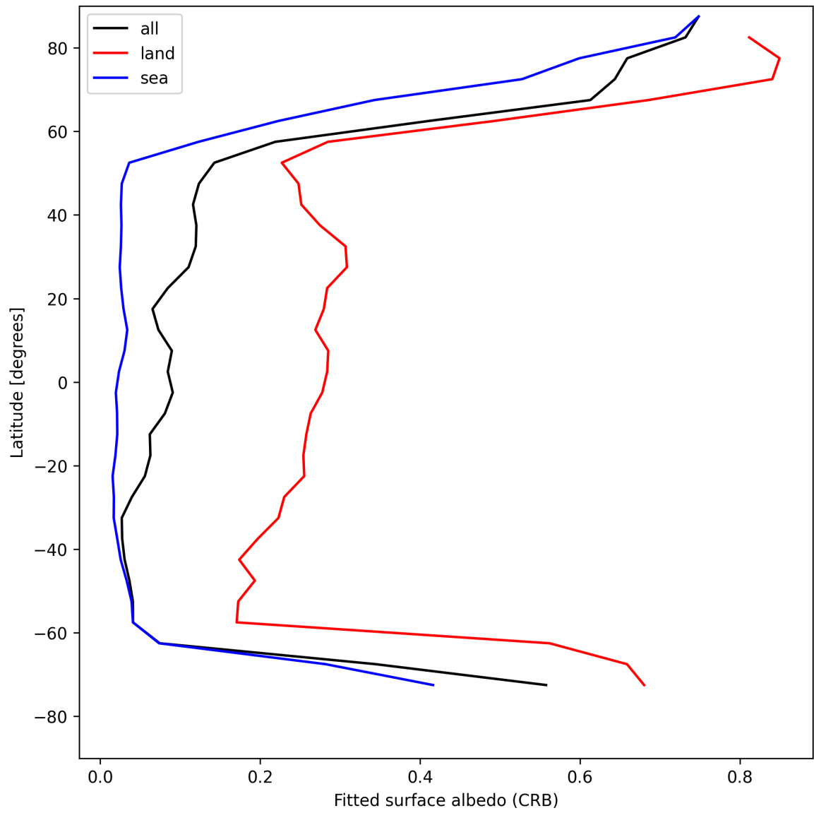
Figure 28: Zonal average of “Fitted surface albedo (CRB)” for 2025-05-09 to 2025-05-10.
