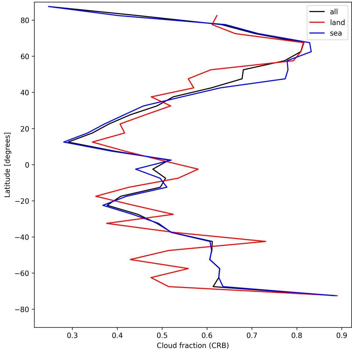
Figure 24: Zonal average of “Cloud fraction (CRB)” for 2025-05-09 to 2025-05-10.
