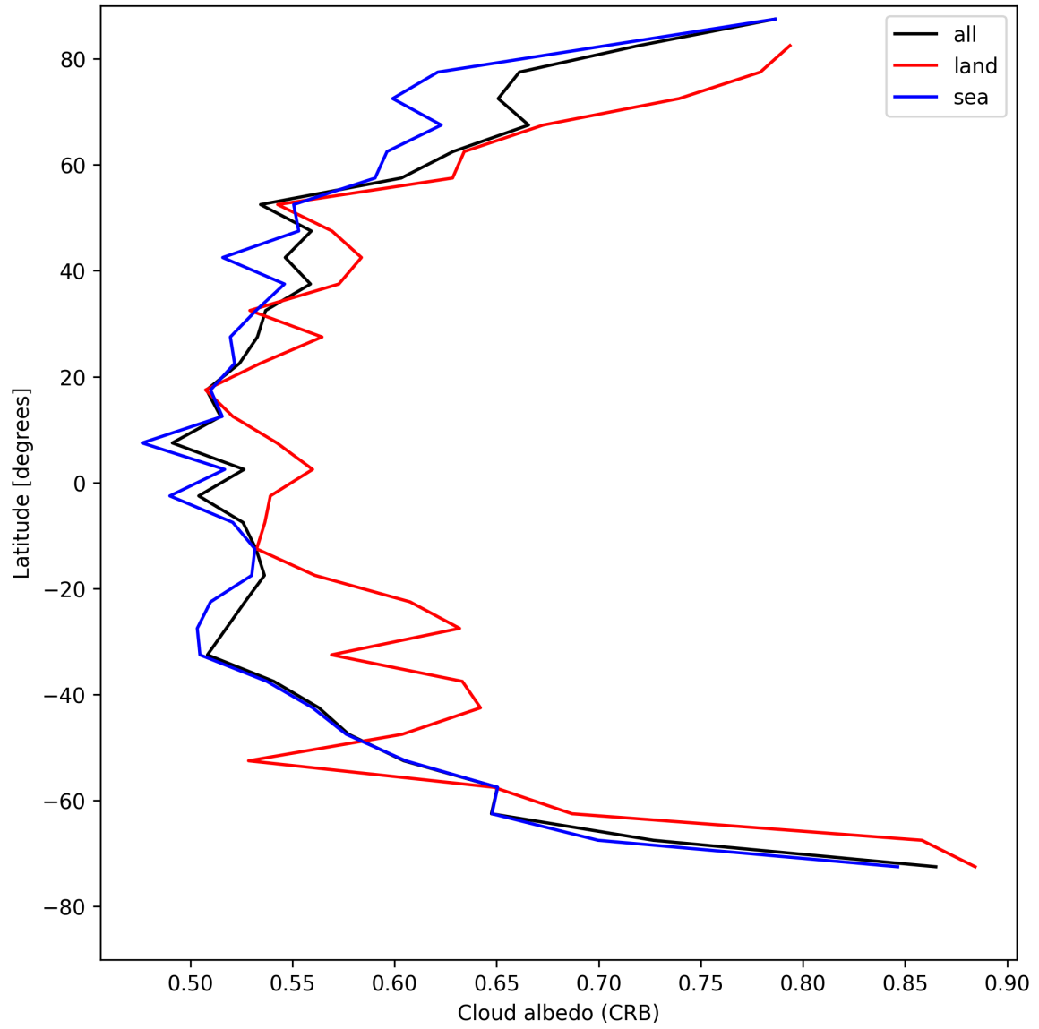
Figure 26: Zonal average of “Cloud albedo (CRB)” for 2025-05-09 to 2025-05-10.
