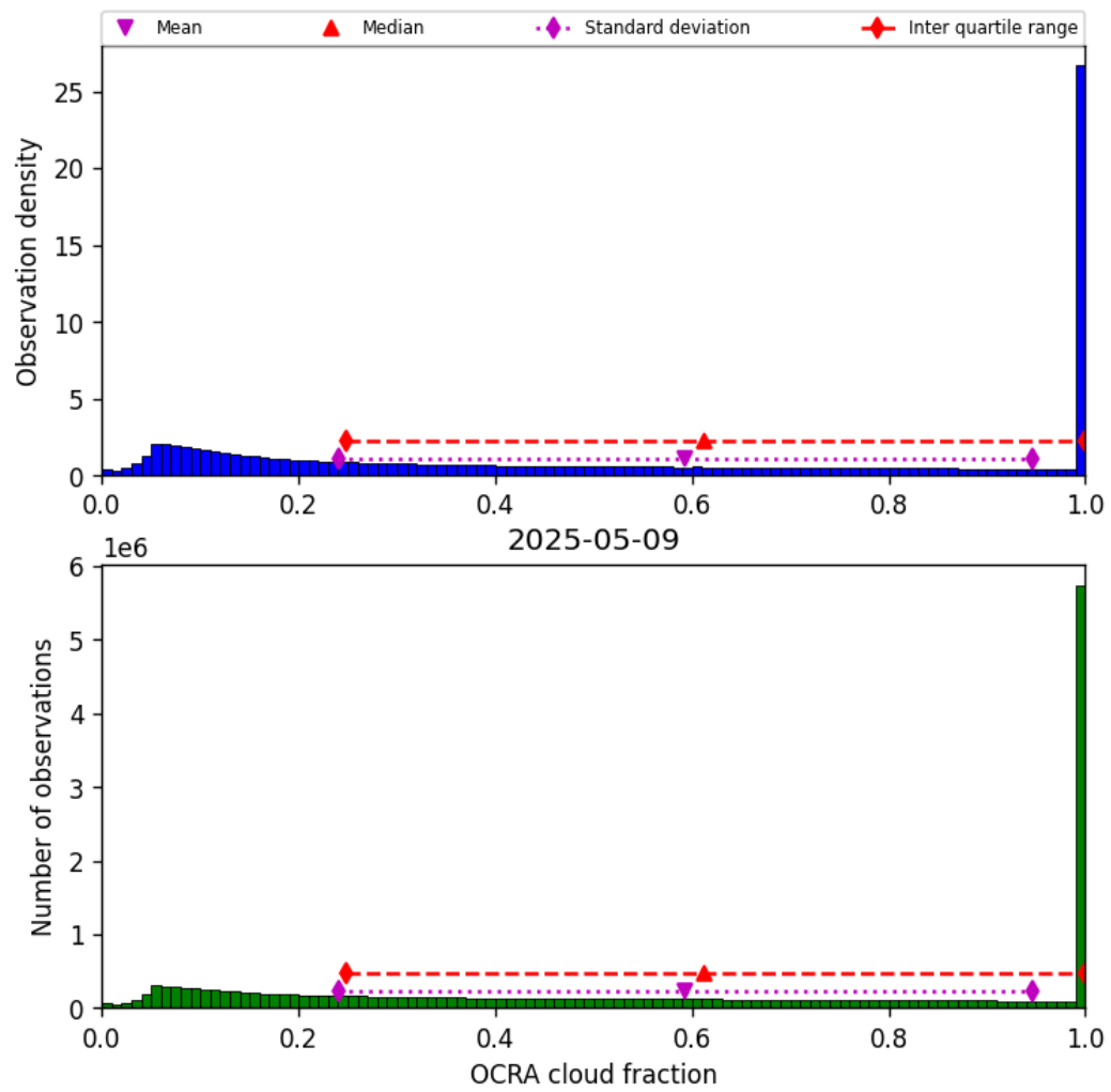
Figure 48: Histogram of “OCRA cloud fraction” for 2025-05-09 to 2025-05-10
