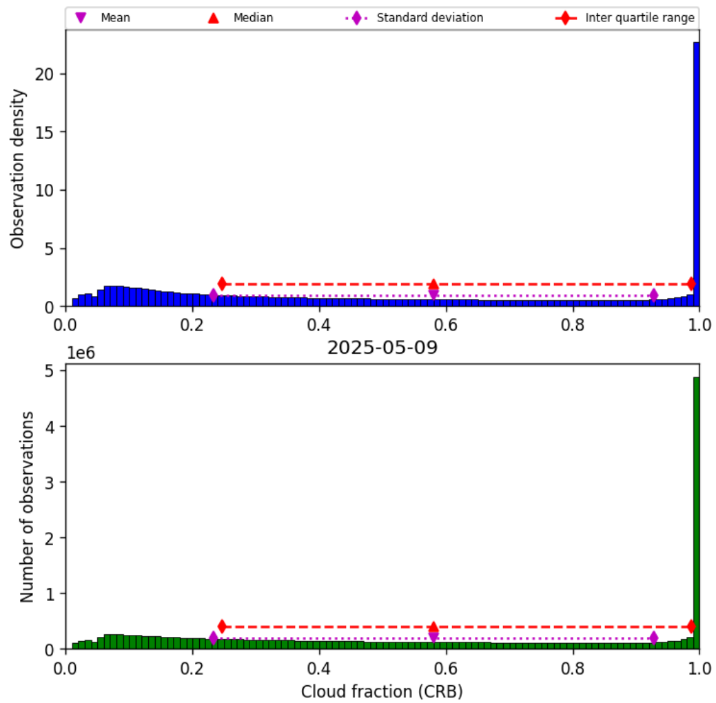
Figure 40: Histogram of “Cloud fraction (CRB)” for 2025-05-09 to 2025-05-10
