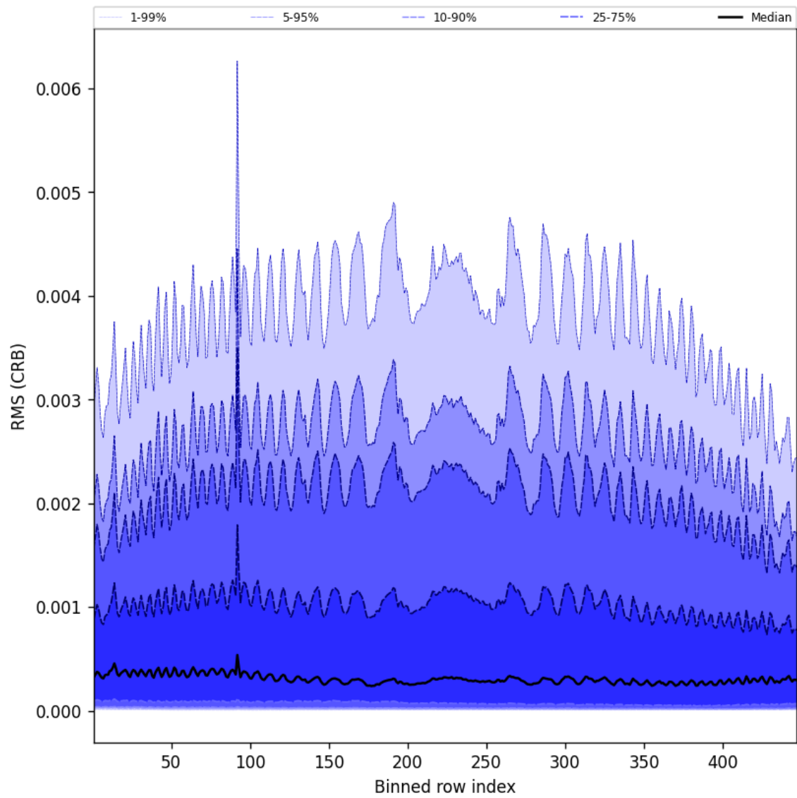
Figure 62: Along track statistics of “RMS (CRB)” for 2025-05-09 to 2025-05-10
