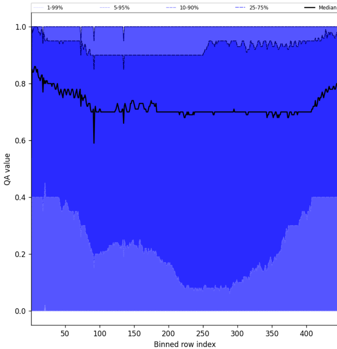
Figure 52: Along track statistics of “QA value” for 2025-05-09 to 2025-05-10
