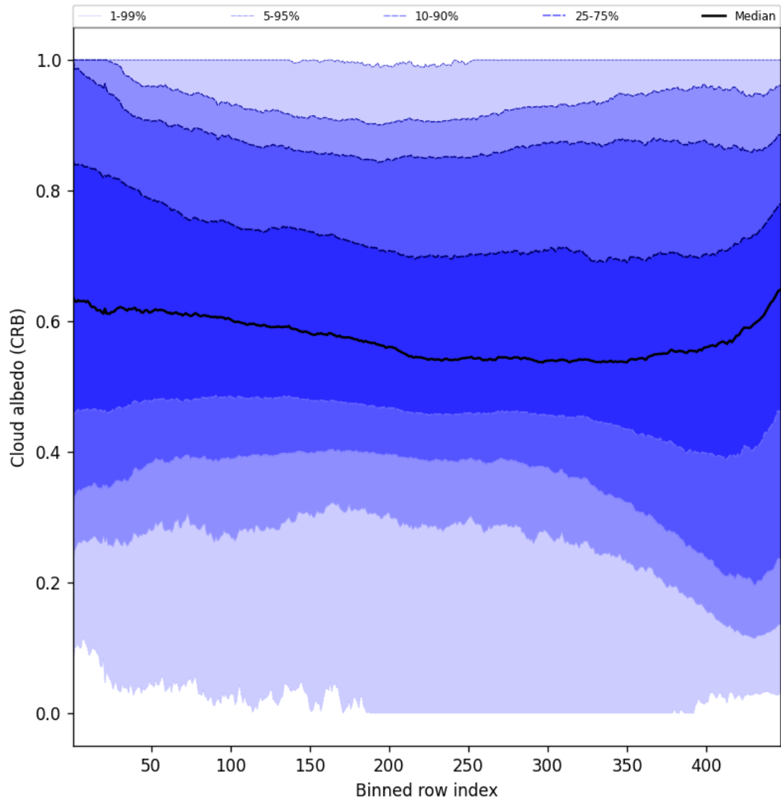
Figure 58: Along track statistics of “Cloud albedo (CRB)” for 2025-05-09 to 2025-05-10
