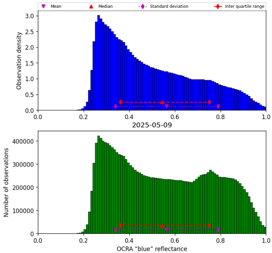
Figure 49: Histogram of “OCRA “blue” reflectance” for 2025-05-09 to 2025-05-10
