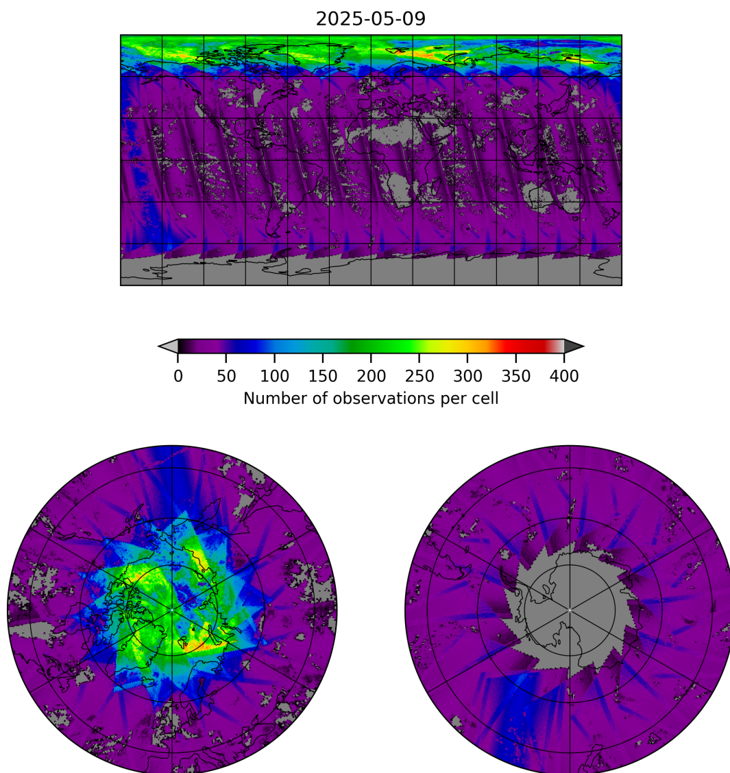
Figure 19: Map of the number of observations for 2025-05-09 to 2025-05-10
