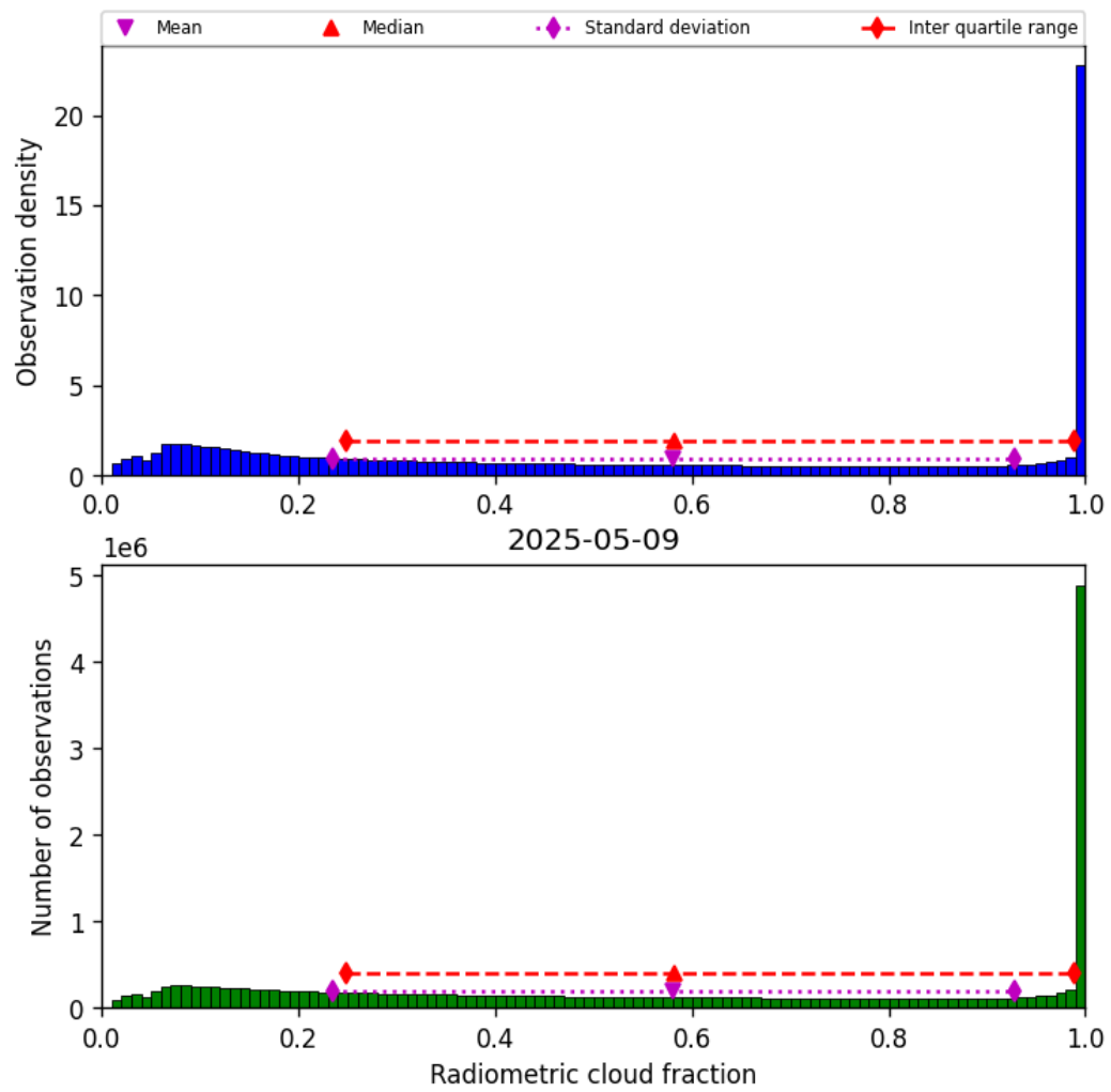
Figure 37: Histogram of “Radiometric cloud fraction” for 2025-05-09 to 2025-05-10
