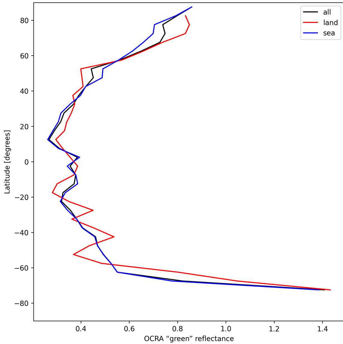
Figure 34: Zonal average of “OCRA “green” reflectance” for 2025-05-09 to 2025-05-10.
