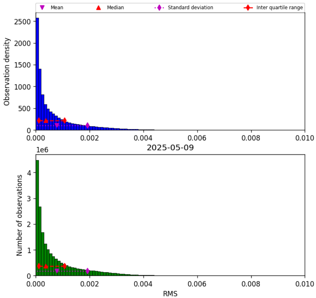
Figure 45: Histogram of “RMS” for 2025-05-09 to 2025-05-10
