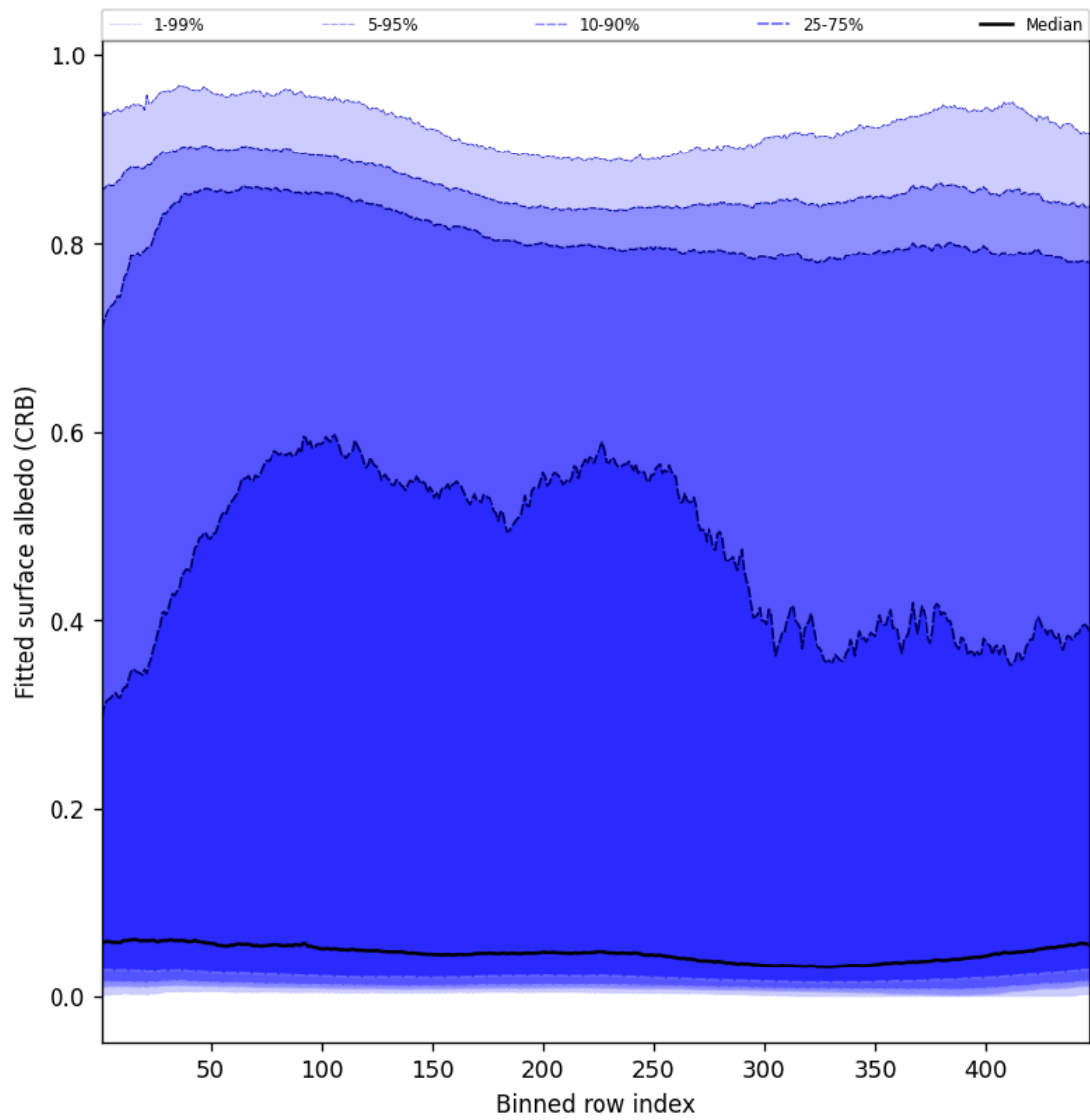
Figure 60: Along track statistics of “Fitted surface albedo (CRB)” for 2025-05-09 to 2025-05-10
