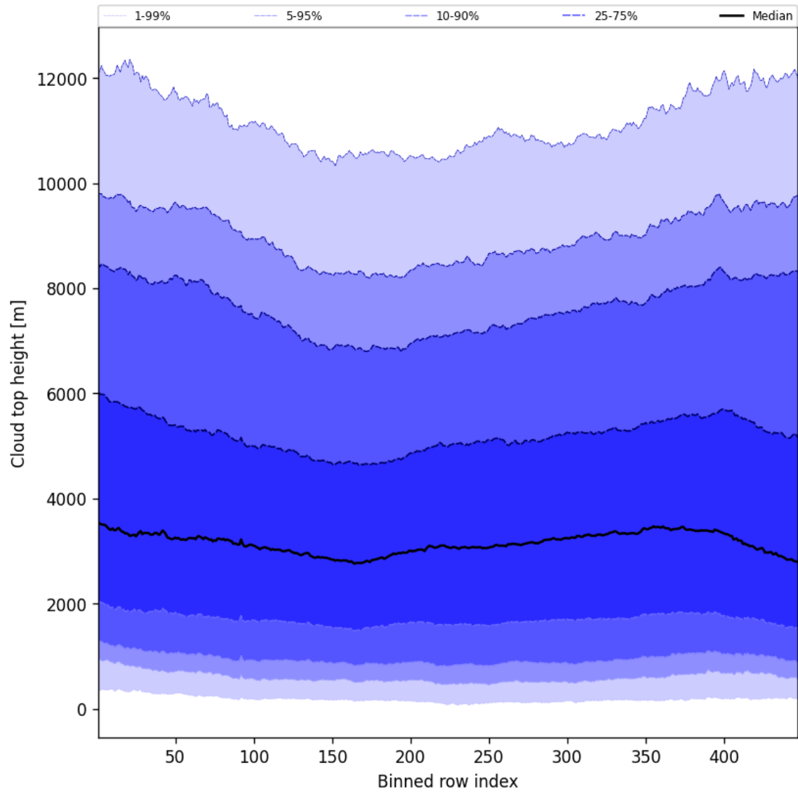
Figure 54: Along track statistics of “Cloud top height” for 2025-05-09 to 2025-05-10
