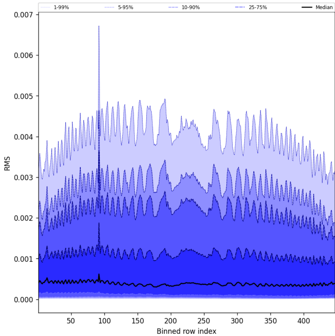
Figure 61: Along track statistics of “RMS” for 2025-05-09 to 2025-05-10
