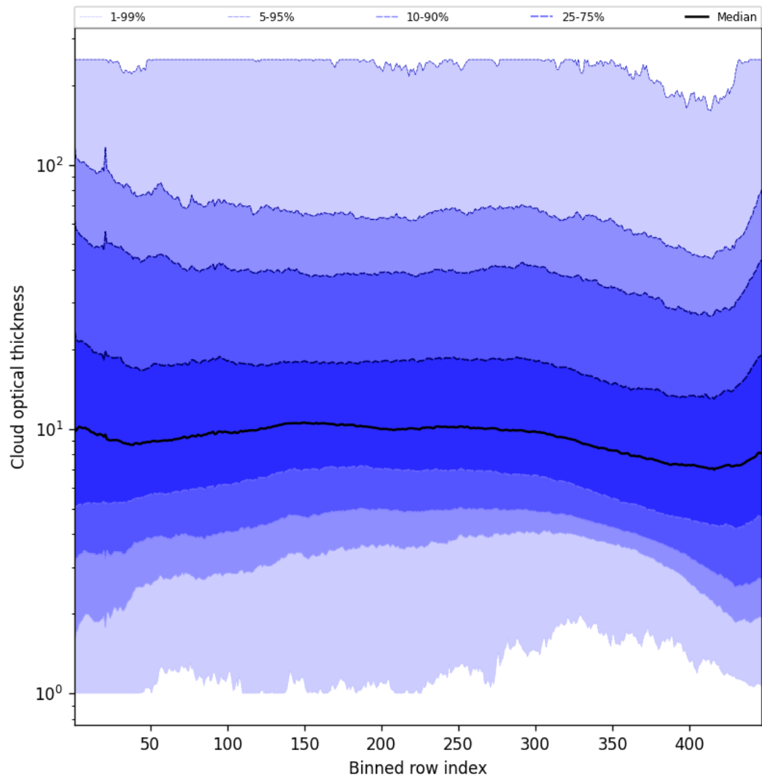
Figure 55: Along track statistics of “Cloud optical thickness” for 2025-05-09 to 2025-05-10
