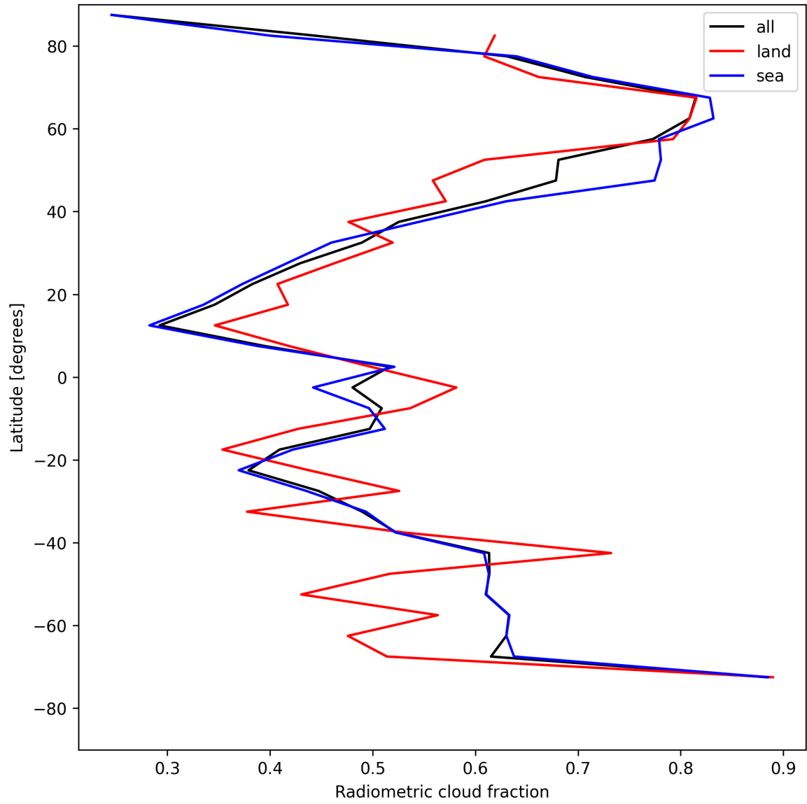
Figure 21: Zonal average of “Radiometric cloud fraction” for 2025-05-09 to 2025-05-10.
