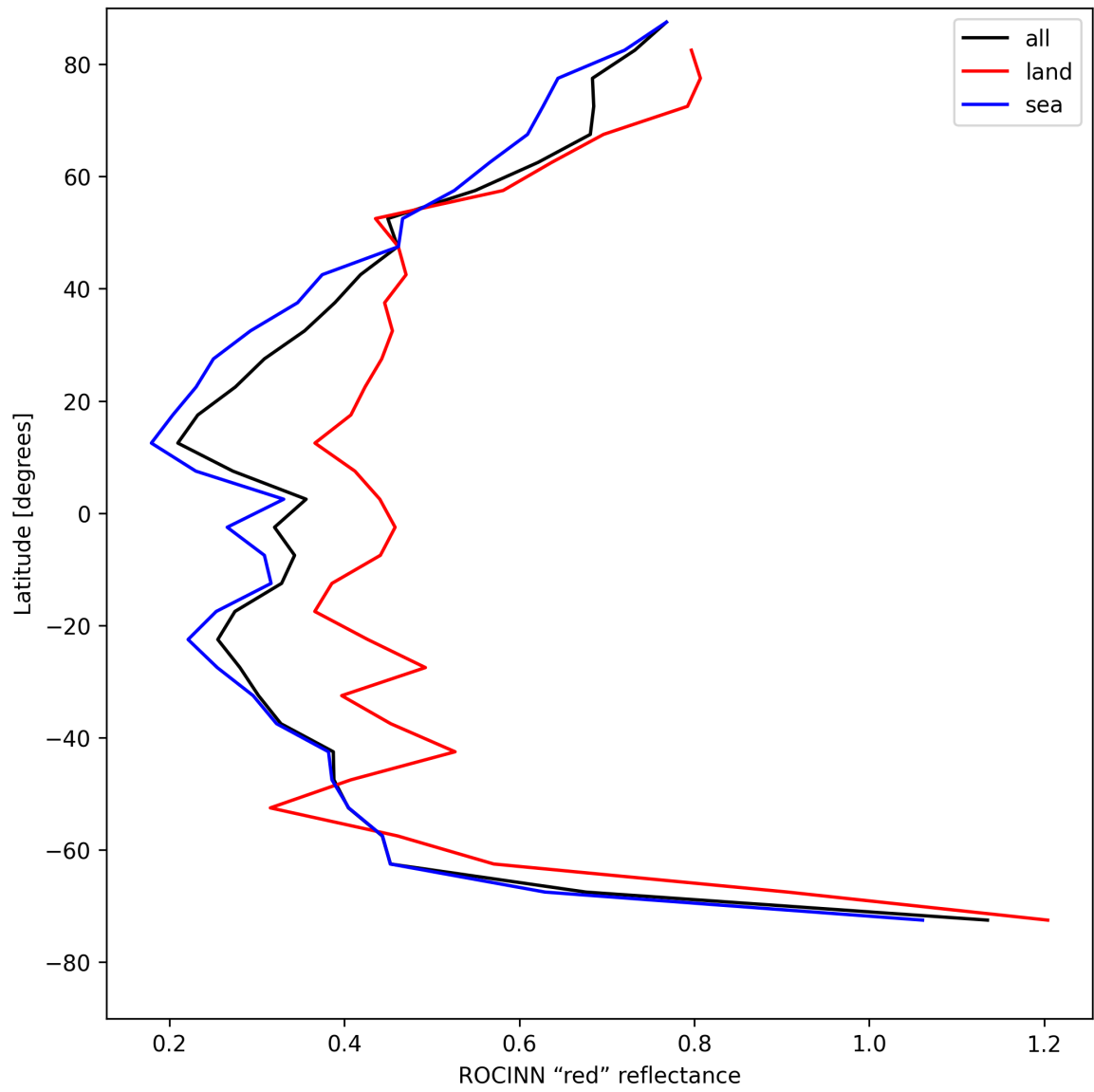
Figure 35: Zonal average of “ROCINN “red” reflectance” for 2025-05-09 to 2025-05-10.
