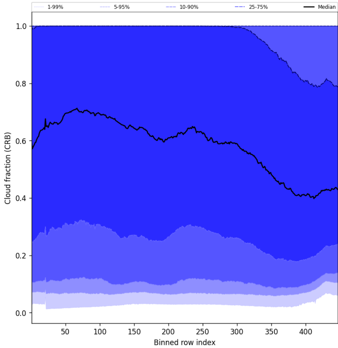
Figure 56: Along track statistics of “Cloud fraction (CRB)” for 2025-05-09 to 2025-05-10
