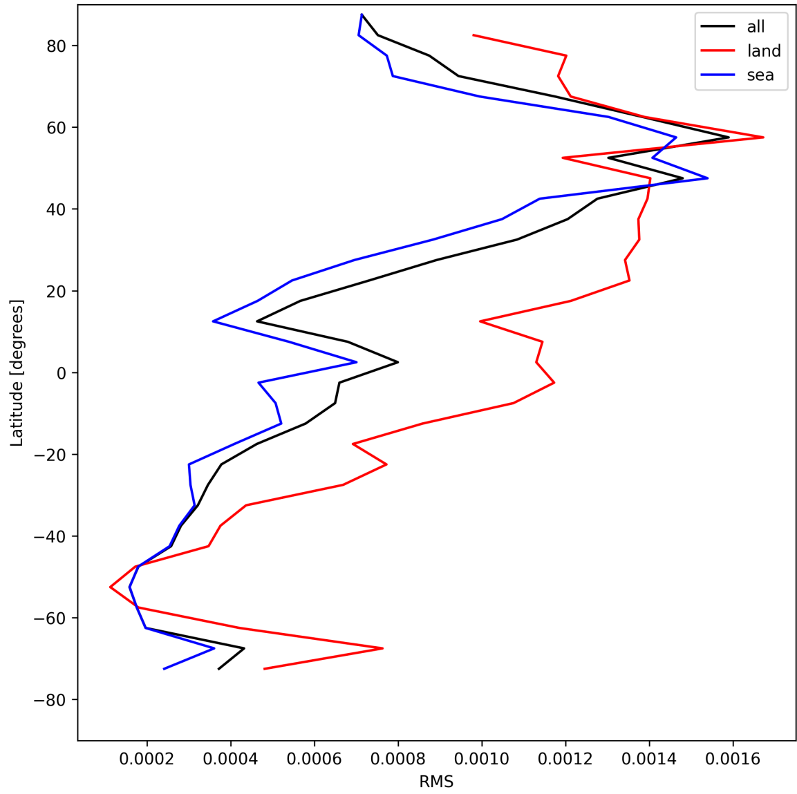
Figure 29: Zonal average of “RMS” for 2025-05-09 to 2025-05-10.
