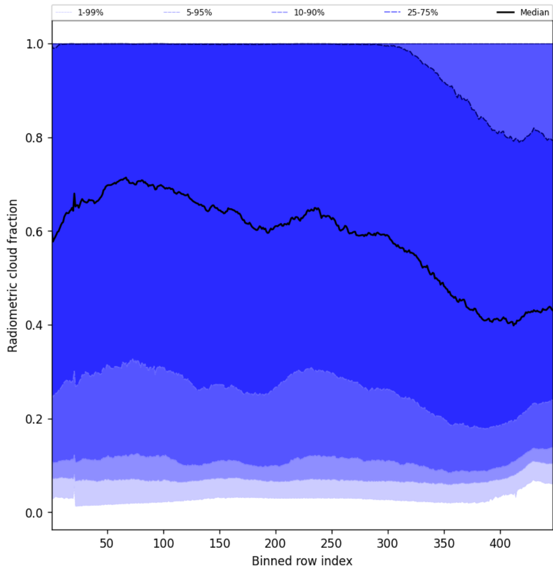
Figure 53: Along track statistics of “Radiometric cloud fraction” for 2025-05-09 to 2025-05-10
