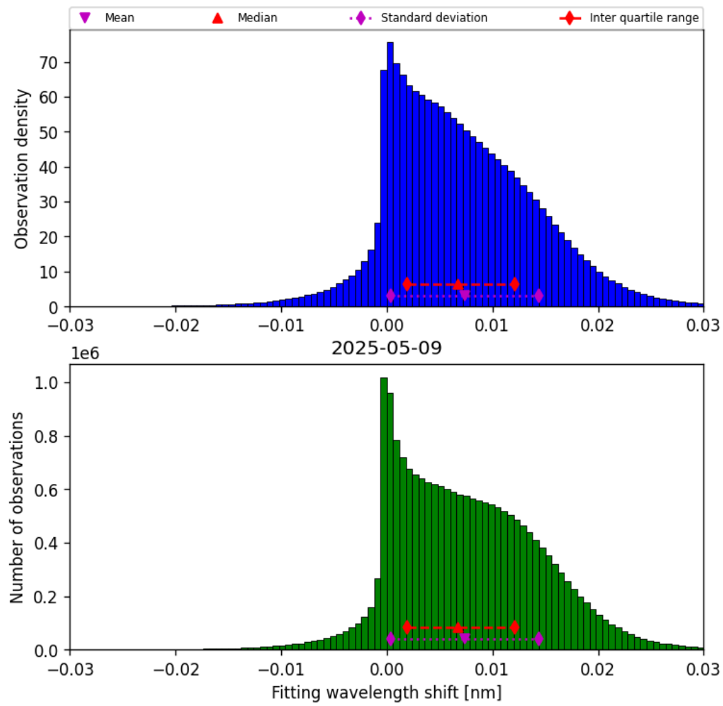
Figure 47: Histogram of “Fitting wavelength shift” for 2025-05-09 to 2025-05-10
