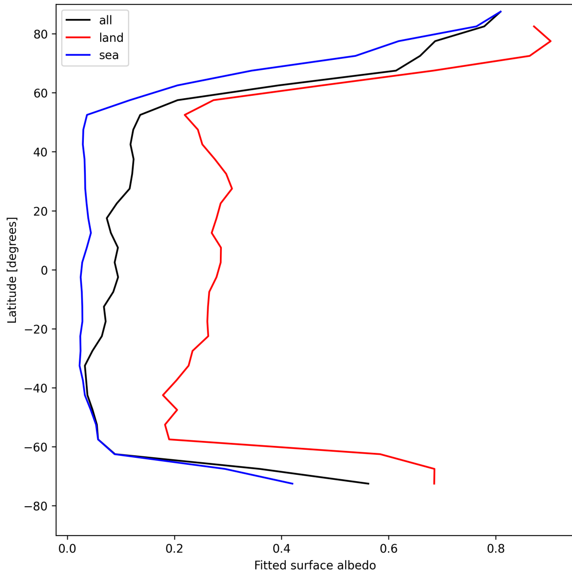
Figure 27: Zonal average of “Fitted surface albedo” for 2025-05-09 to 2025-05-10.
