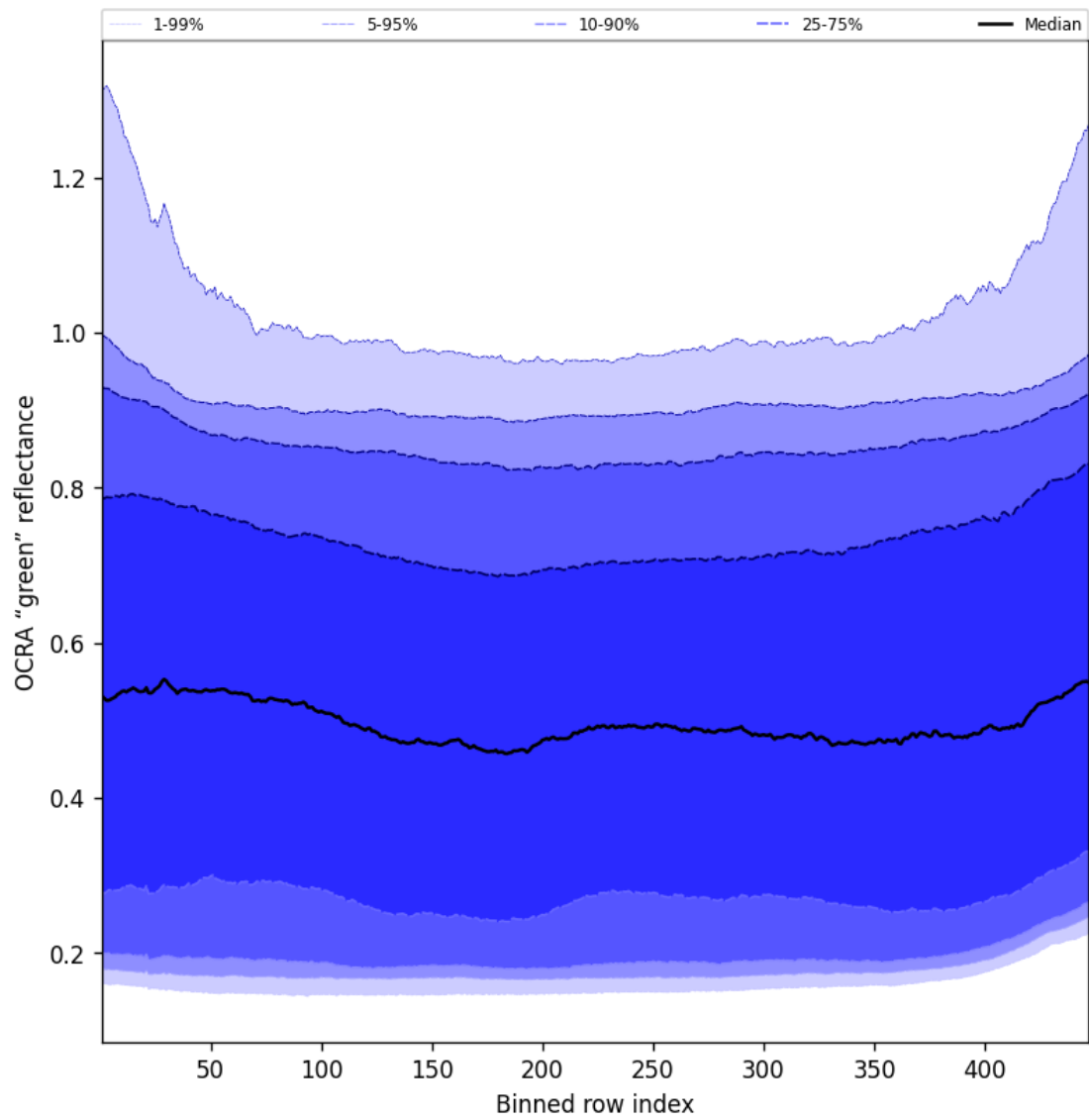
Figure 66: Along track statistics of “OCRA “green” reflectance” for 2025-05-09 to 2025-05-10
