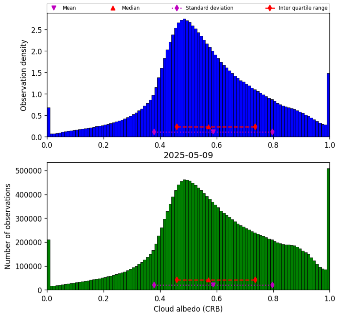
Figure 42: Histogram of “Cloud albedo (CRB)” for 2025-05-09 to 2025-05-10
