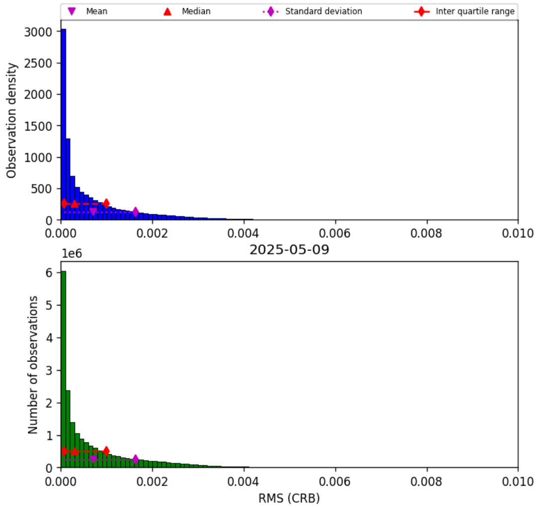
Figure 46: Histogram of “RMS (CRB)” for 2025-05-09 to 2025-05-10
