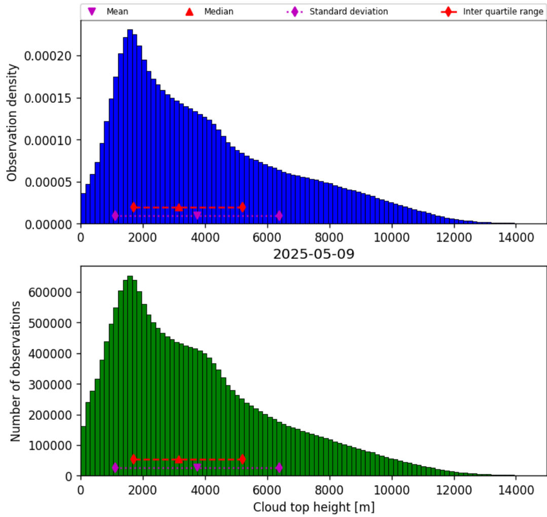
Figure 38: Histogram of “Cloud top height” for 2025-05-09 to 2025-05-10
