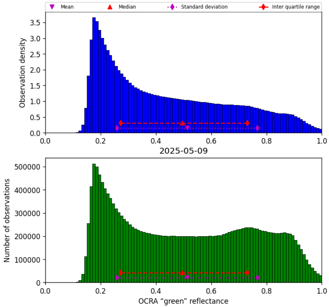
Figure 50: Histogram of “OCRA “green” reflectance” for 2025-05-09 to 2025-05-10
