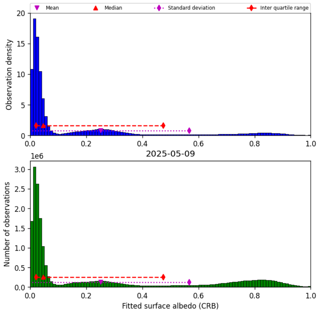
Figure 44: Histogram of “Fitted surface albedo (CRB)” for 2025-05-09 to 2025-05-10
