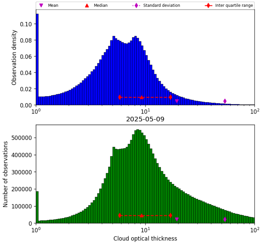
Figure 39: Histogram of “Cloud optical thickness” for 2025-05-09 to 2025-05-10
