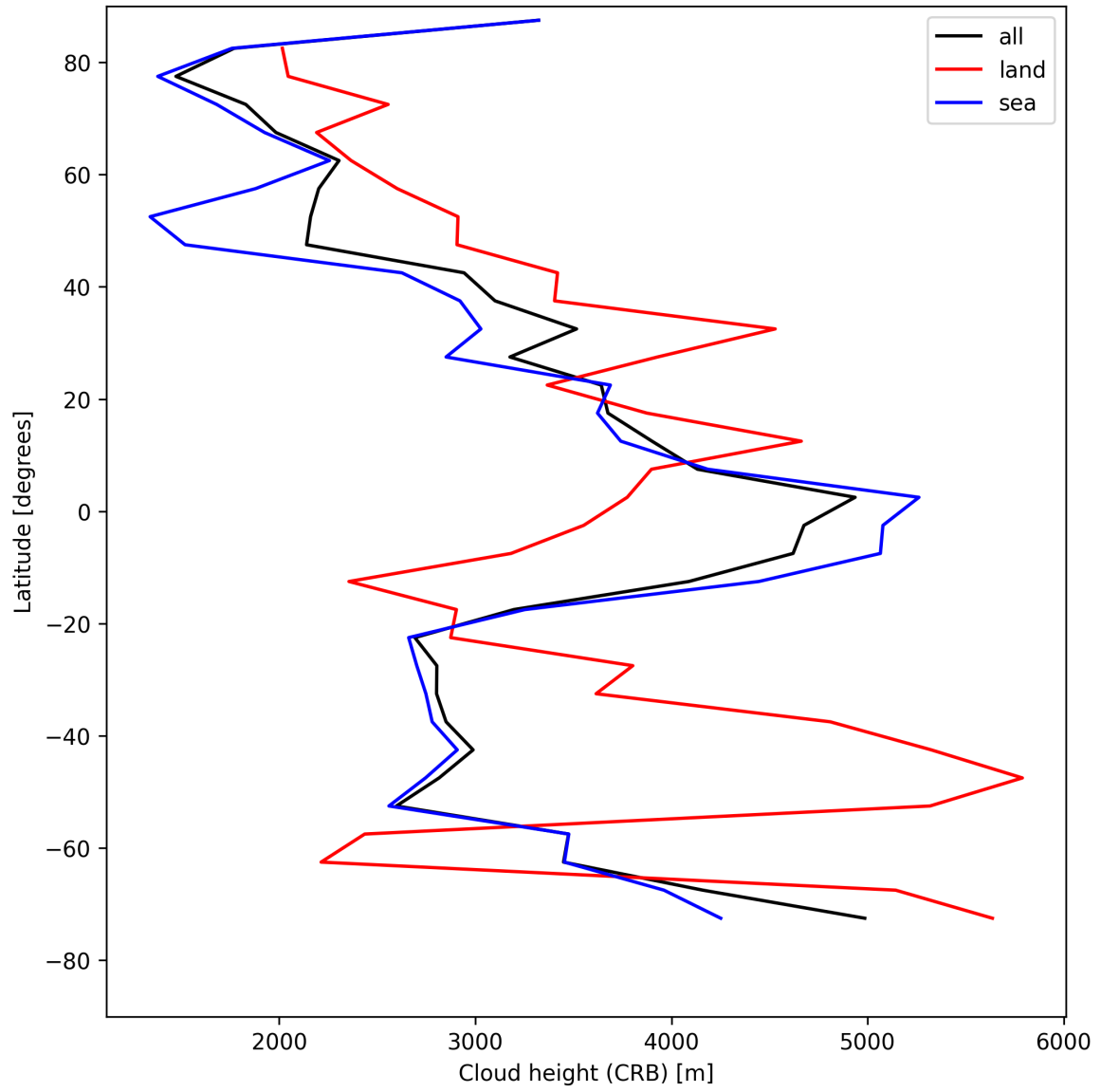
Figure 25: Zonal average of “Cloud height (CRB)” for 2025-05-09 to 2025-05-10.
