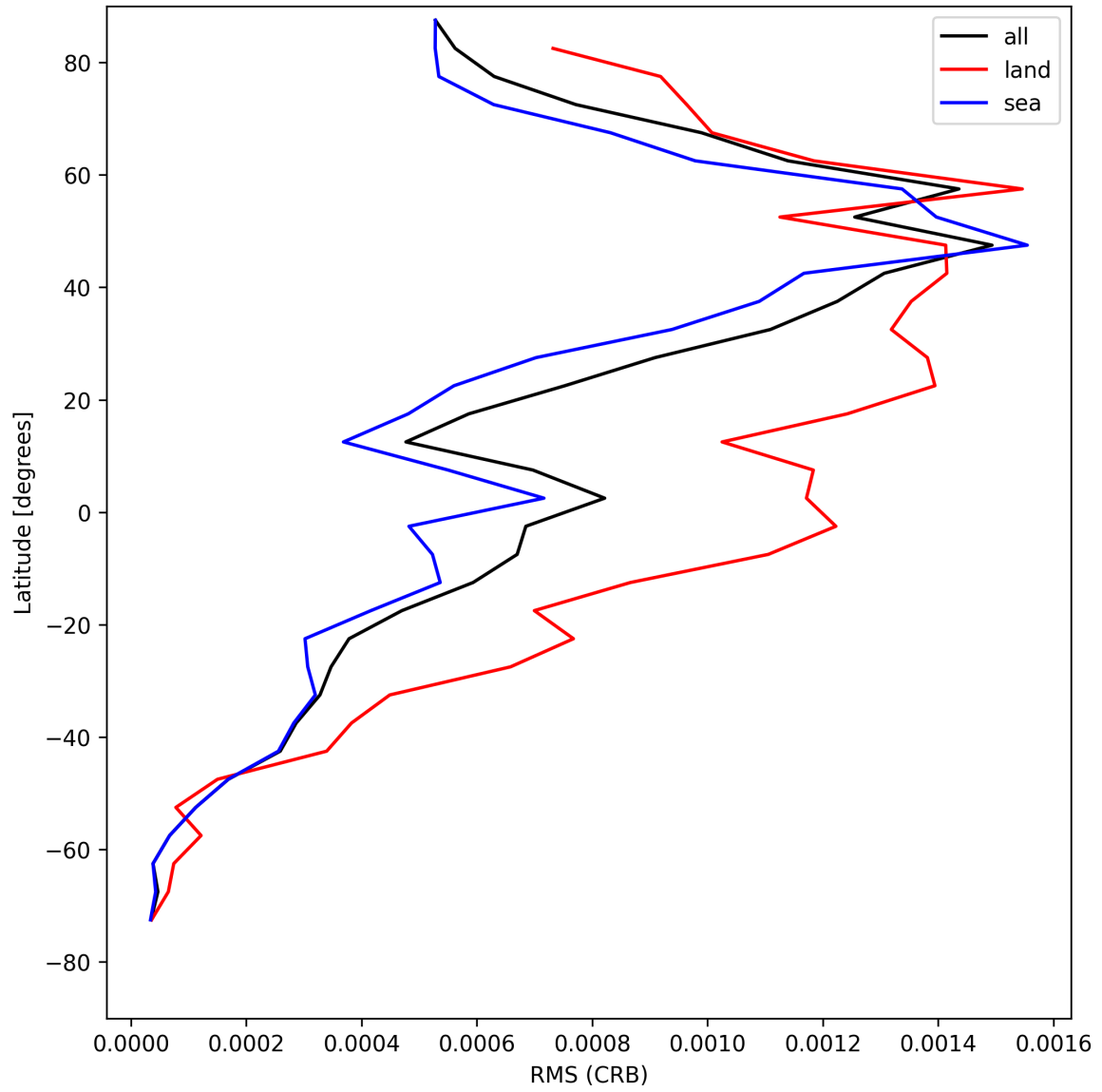
Figure 30: Zonal average of “RMS (CRB)” for 2025-05-09 to 2025-05-10.
