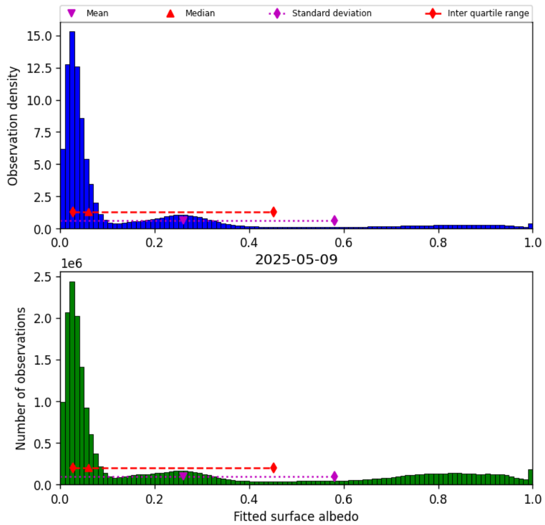
Figure 43: Histogram of “Fitted surface albedo” for 2025-05-09 to 2025-05-10
