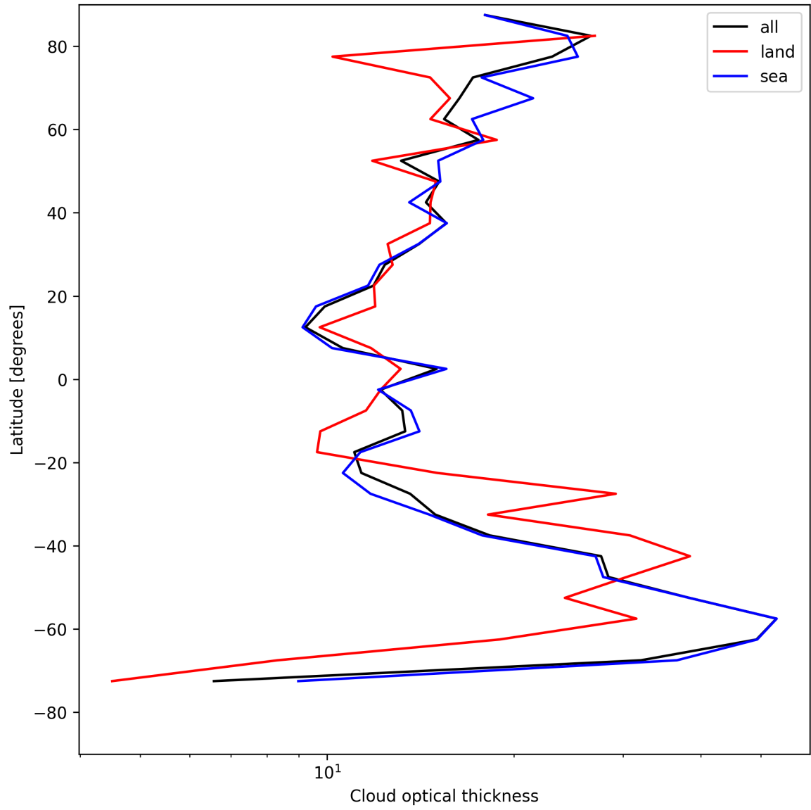
Figure 23: Zonal average of “Cloud optical thickness” for 2025-05-09 to 2025-05-10.
