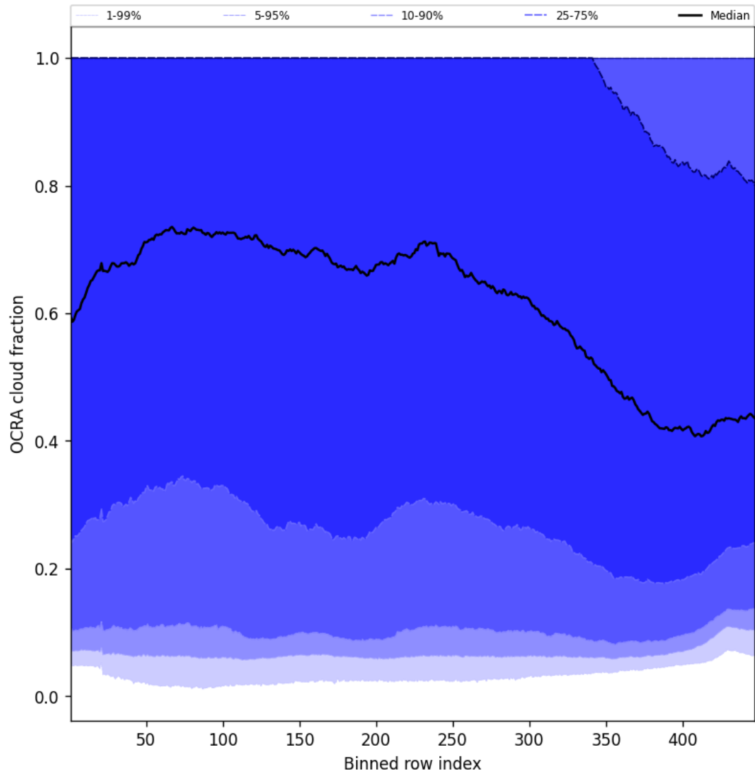
Figure 64: Along track statistics of “OCRA cloud fraction” for 2025-05-09 to 2025-05-10
