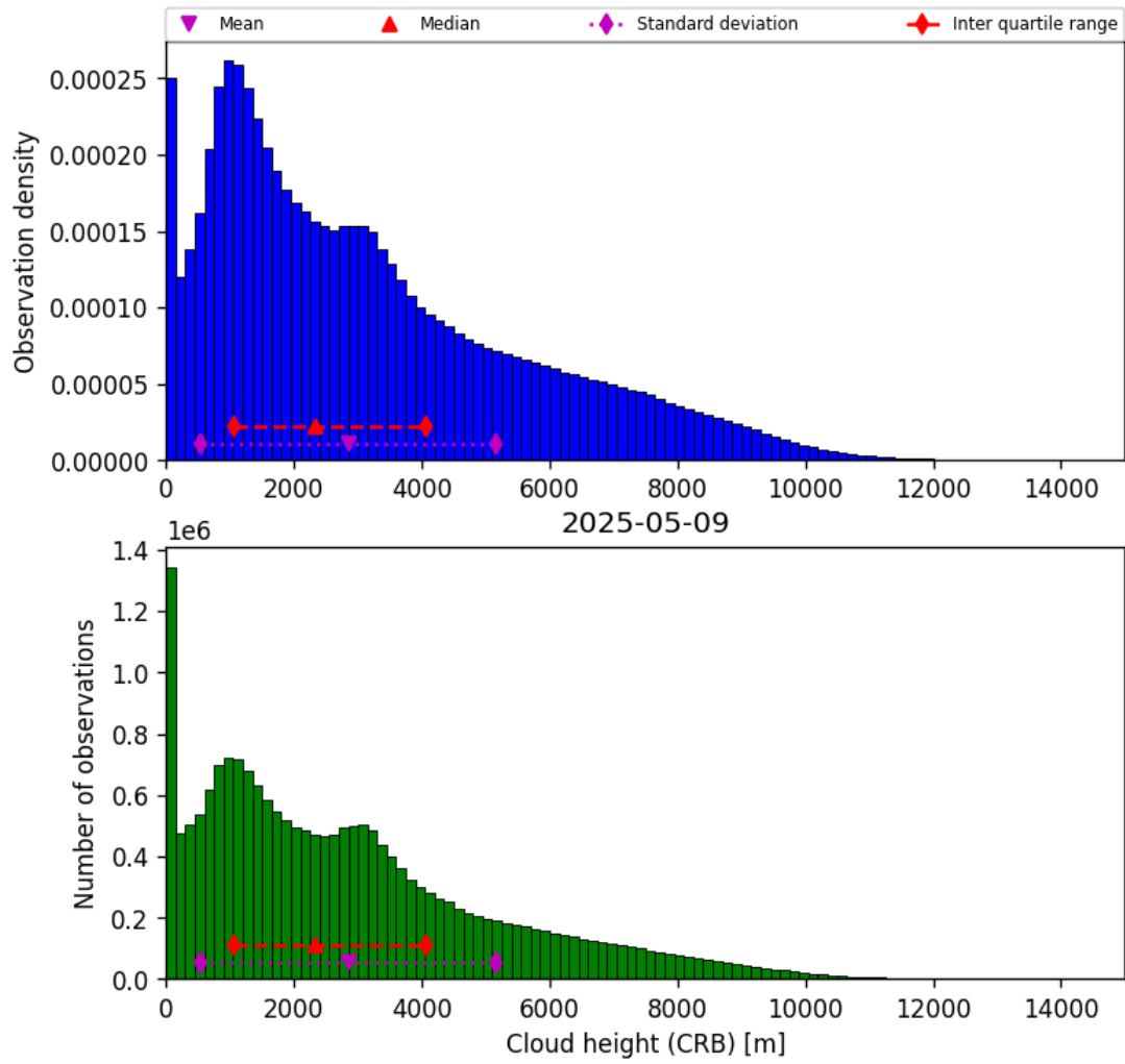
Figure 41: Histogram of “Cloud height (CRB)” for 2025-05-09 to 2025-05-10
