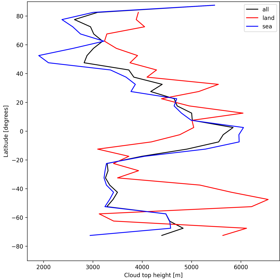
Figure 22: Zonal average of “Cloud top height” for 2025-05-09 to 2025-05-10.
