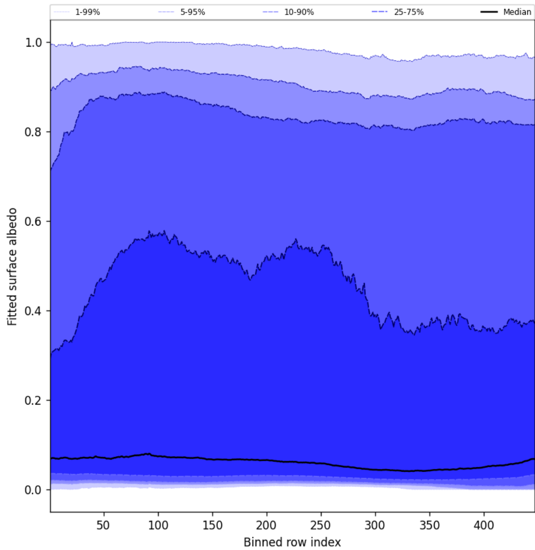
Figure 59: Along track statistics of “Fitted surface albedo” for 2025-05-09 to 2025-05-10
