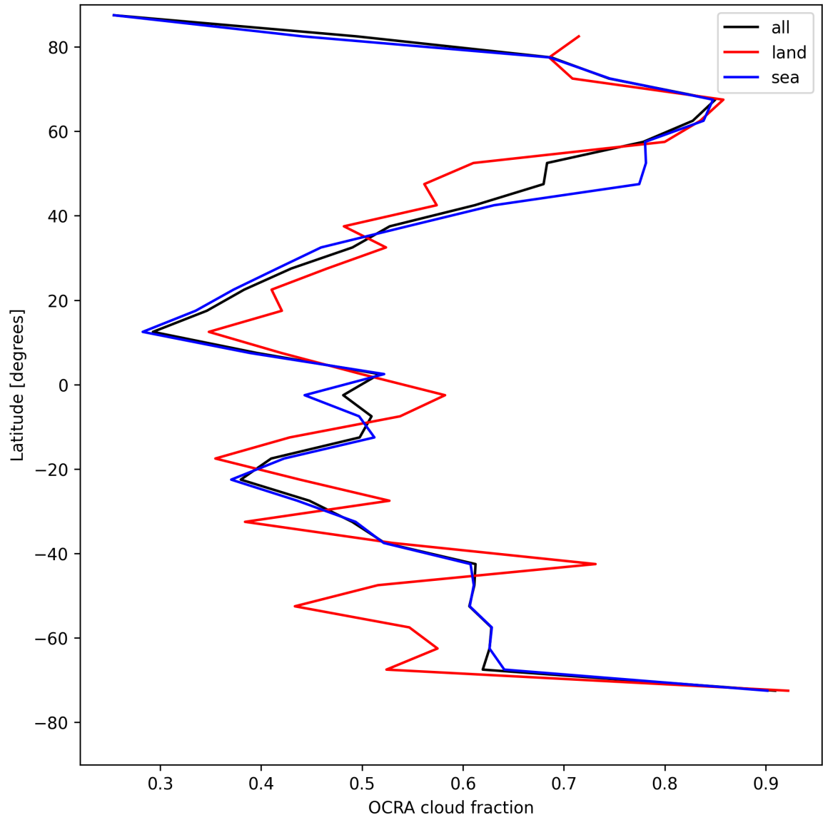
Figure 32: Zonal average of “OCRA cloud fraction” for 2025-05-09 to 2025-05-10.
