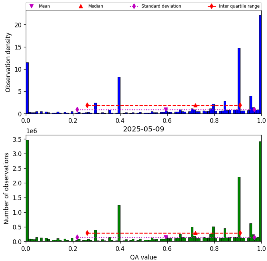
Figure 36: Histogram of “QA value” for 2025-05-09 to 2025-05-10
