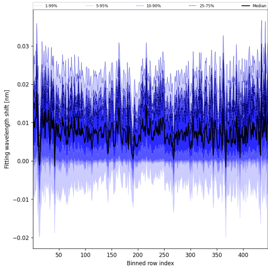
Figure 63: Along track statistics of “Fitting wavelength shift” for 2025-05-09 to 2025-05-10
