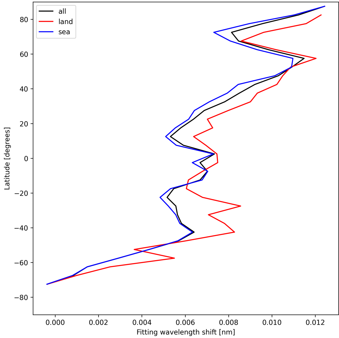
Figure 31: Zonal average of “Fitting wavelength shift” for 2025-05-09 to 2025-05-10.
