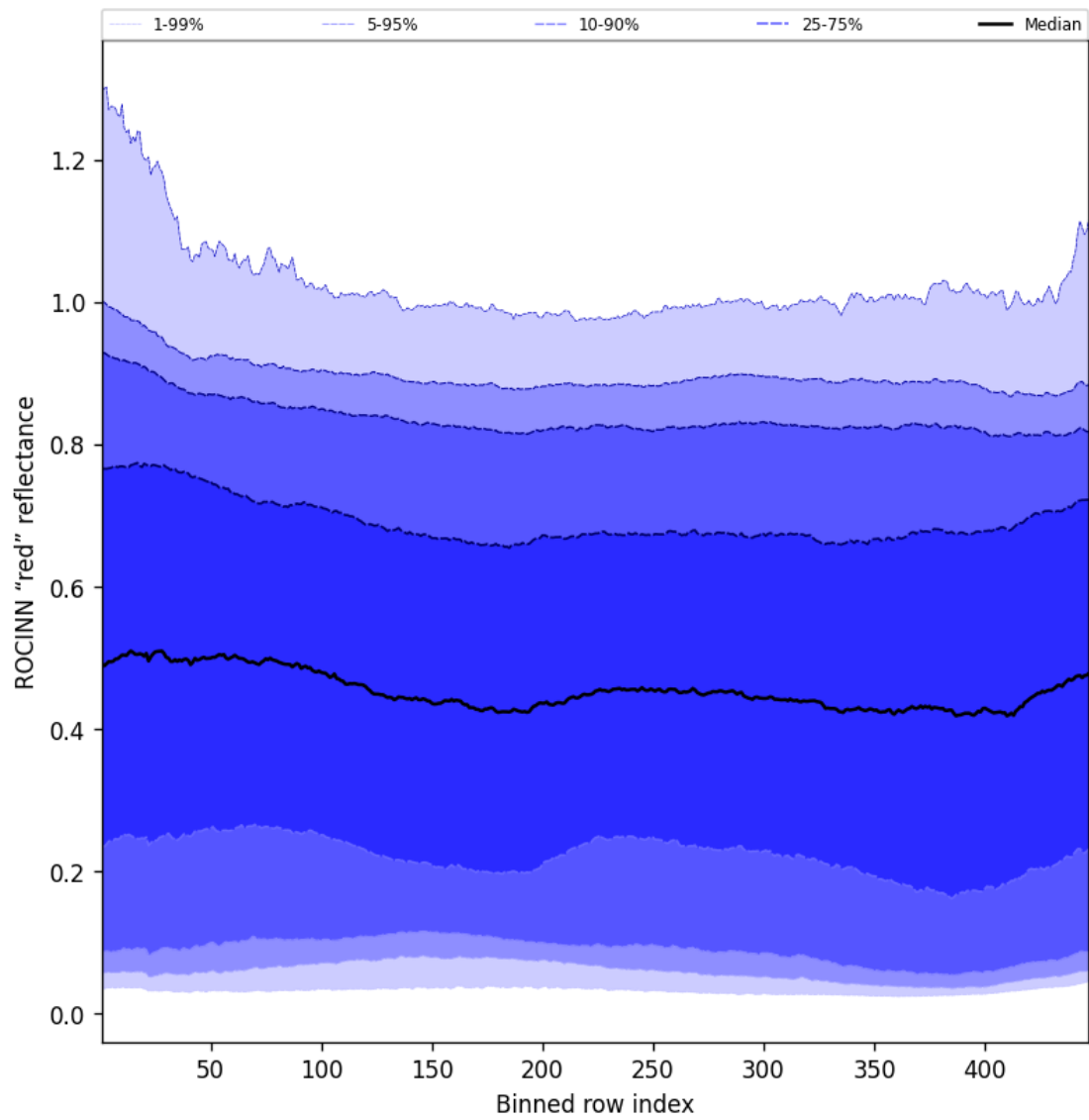
Figure 67: Along track statistics of "ROCINN "red" reflectance" for 2025-05-09 to 2025-05-10
