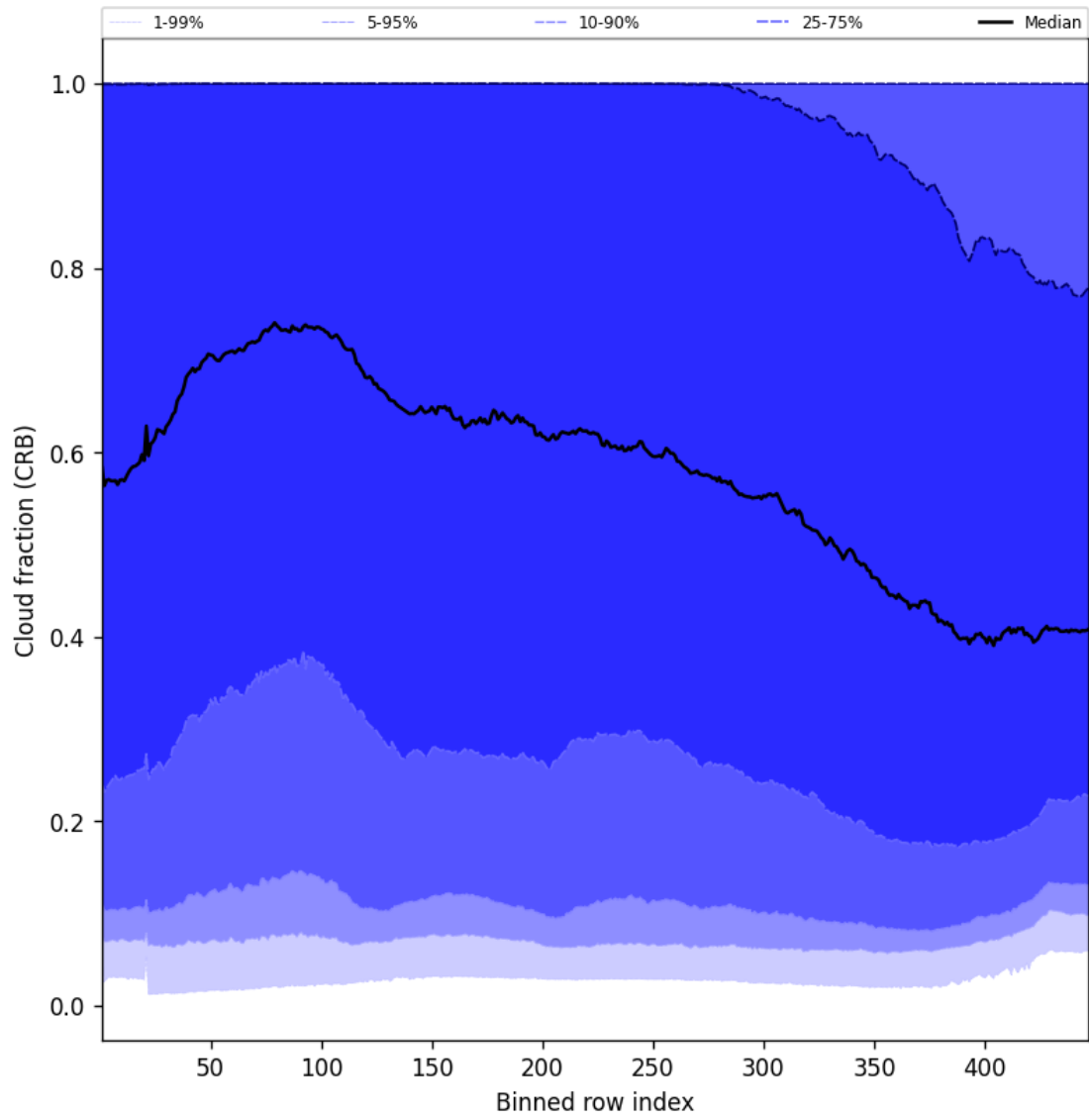
Figure 56: Along track statistics of “Cloud fraction (CRB)” for 2025-05-10 to 2025-05-11
