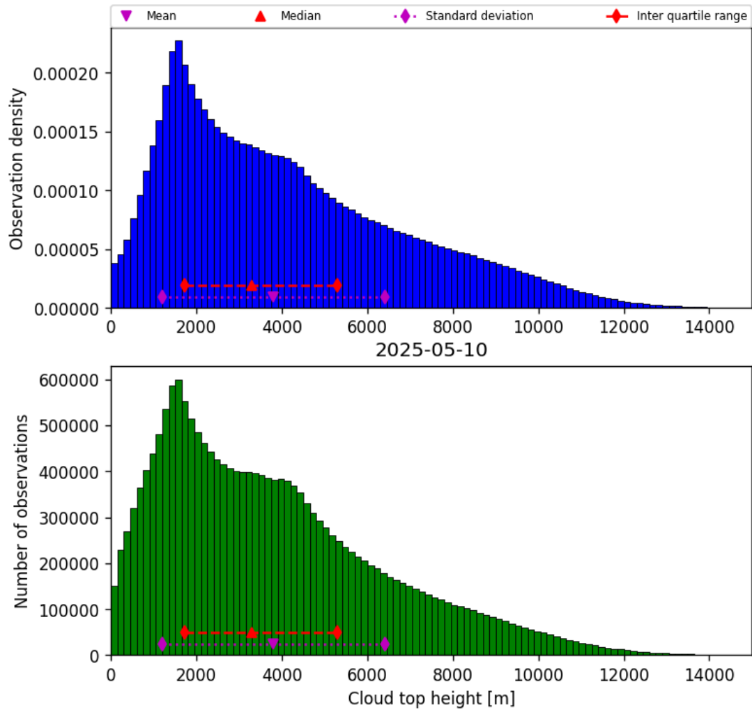
Figure 38: Histogram of “Cloud top height” for 2025-05-10 to 2025-05-11
