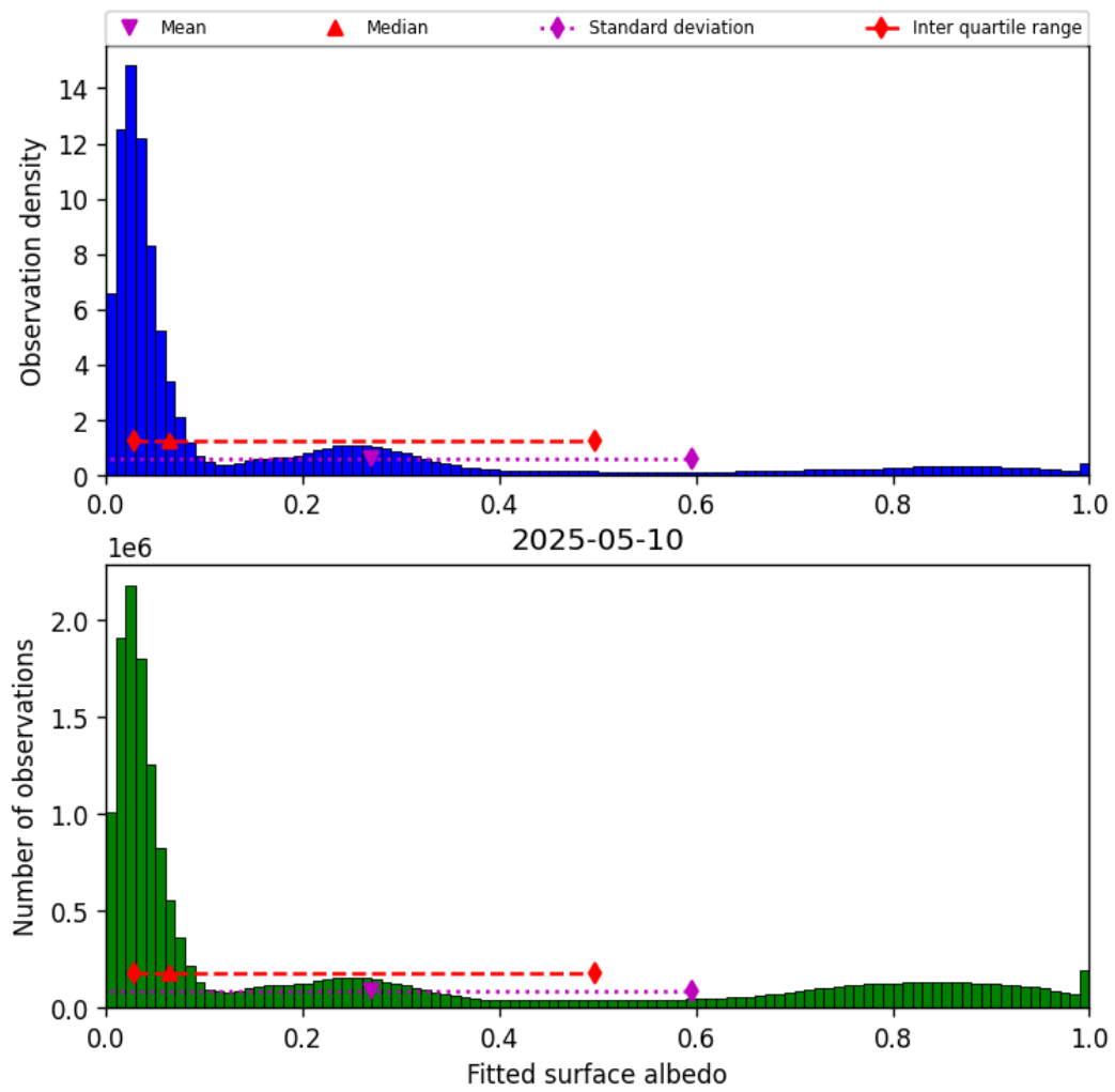
Figure 43: Histogram of “Fitted surface albedo” for 2025-05-10 to 2025-05-11
