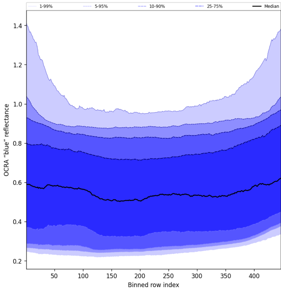
Figure 65: Along track statistics of “OCRA “blue” reflectance” for 2025-05-10 to 2025-05-11
