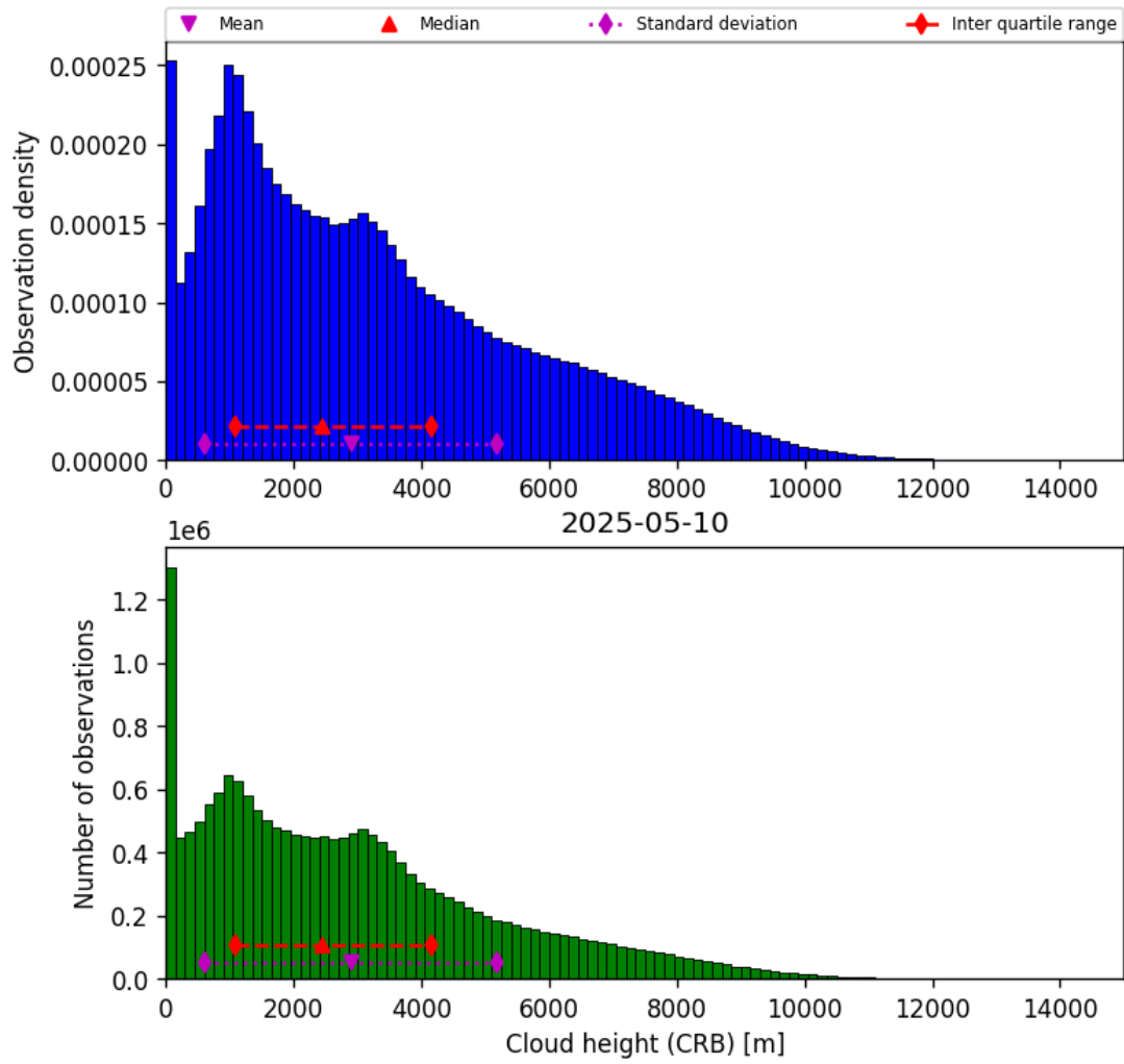
Figure 41: Histogram of “Cloud height (CRB)” for 2025-05-10 to 2025-05-11
