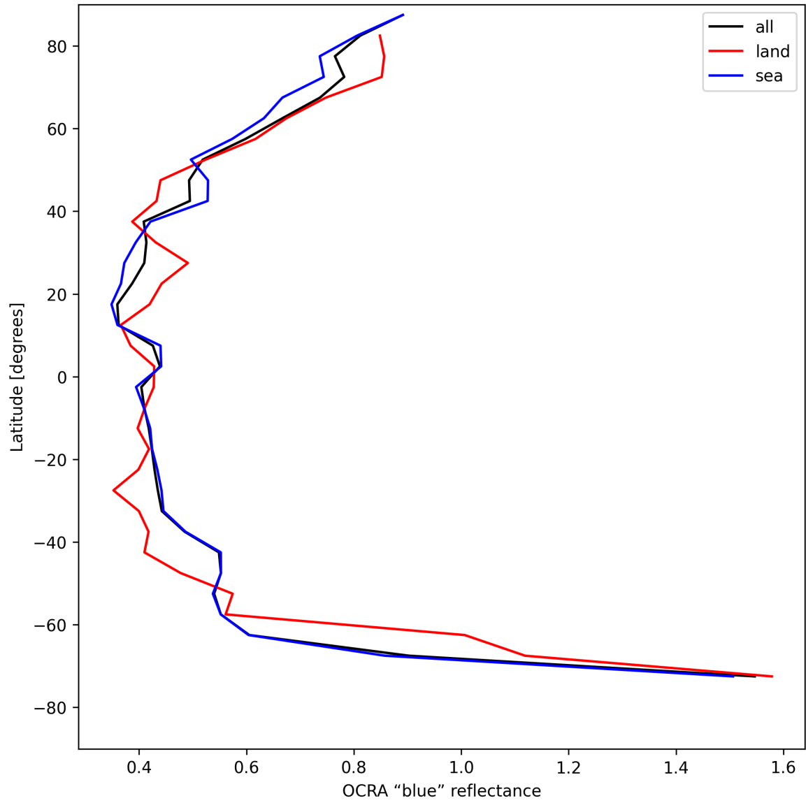
Figure 33: Zonal average of “OCRA “blue” reflectance” for 2025-05-10 to 2025-05-11.
