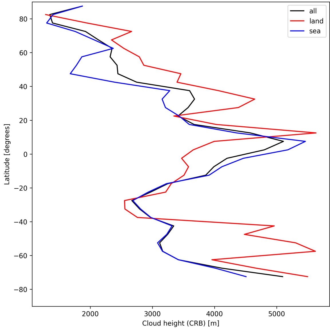
Figure 25: Zonal average of “Cloud height (CRB)” for 2025-05-10 to 2025-05-11.
