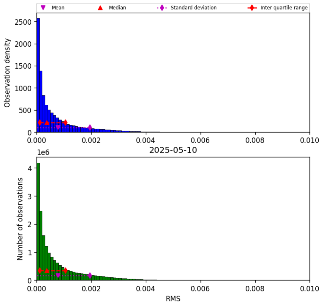
Figure 45: Histogram of “RMS” for 2025-05-10 to 2025-05-11
