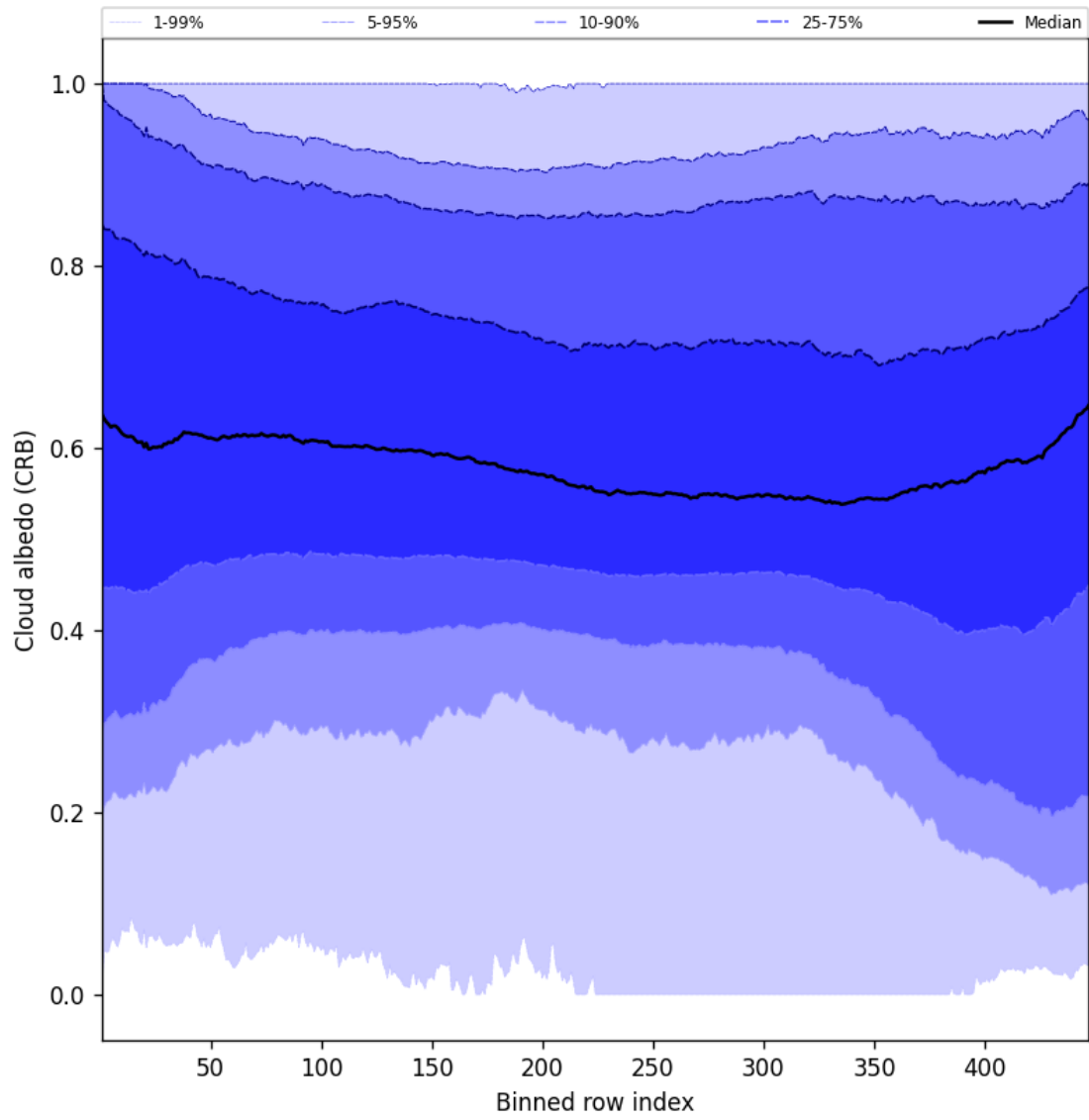
Figure 58: Along track statistics of “Cloud albedo (CRB)” for 2025-05-10 to 2025-05-11
