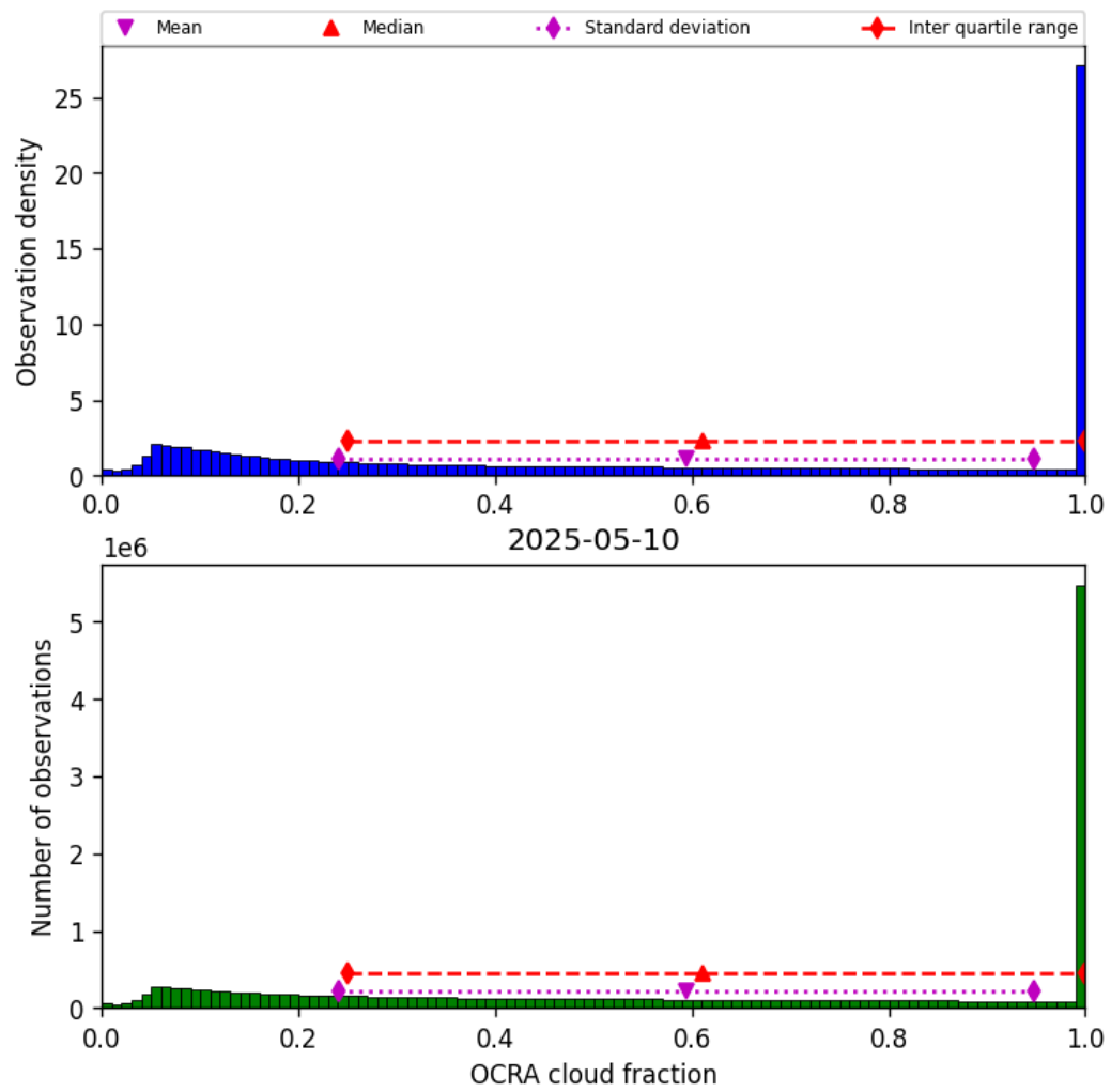
Figure 48: Histogram of “OCRA cloud fraction” for 2025-05-10 to 2025-05-11
