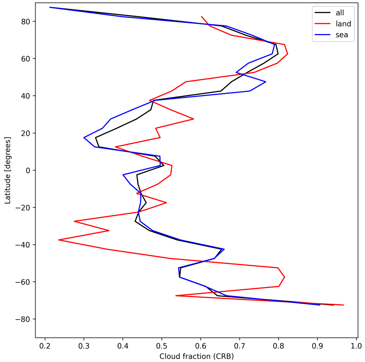
Figure 24: Zonal average of “Cloud fraction (CRB)” for 2025-05-10 to 2025-05-11.
