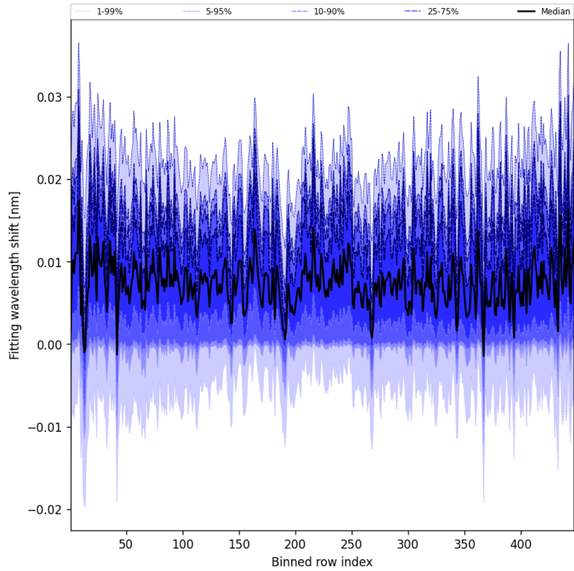
Figure 63: Along track statistics of “Fitting wavelength shift” for 2025-05-10 to 2025-05-11
