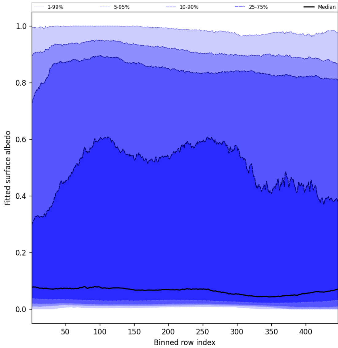
Figure 59: Along track statistics of “Fitted surface albedo” for 2025-05-10 to 2025-05-11
