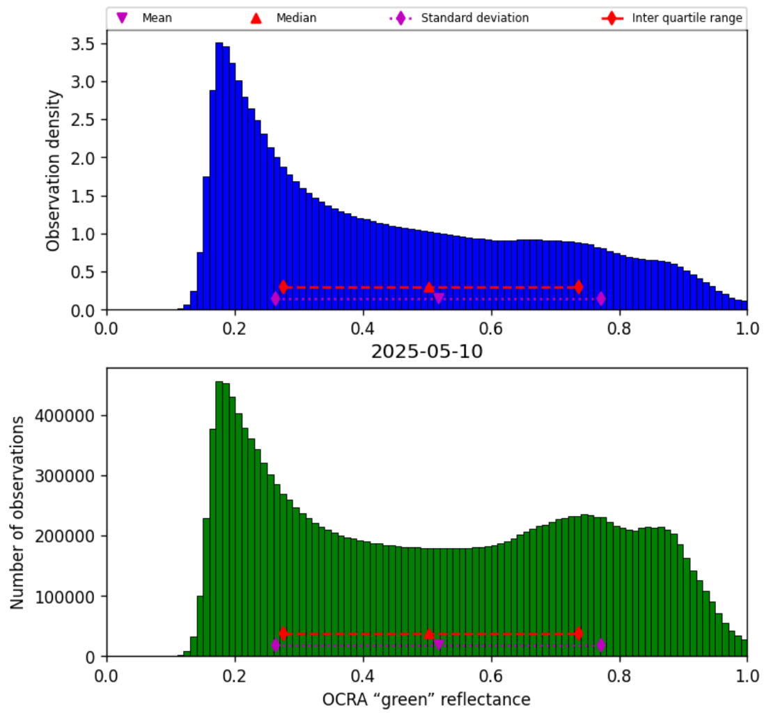
Figure 50: Histogram of “OCRA “green” reflectance” for 2025-05-10 to 2025-05-11
