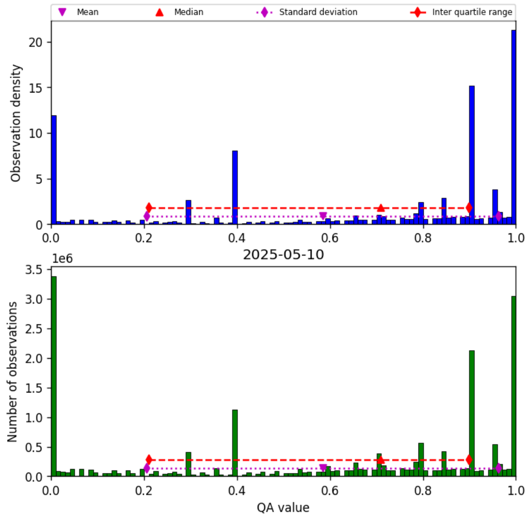
Figure 36: Histogram of “QA value” for 2025-05-10 to 2025-05-11
