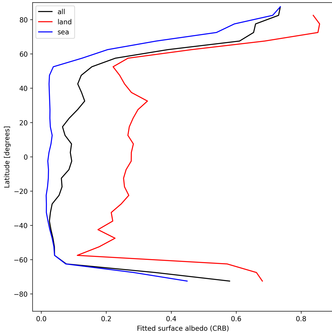
Figure 28: Zonal average of “Fitted surface albedo (CRB)” for 2025-05-10 to 2025-05-11.
