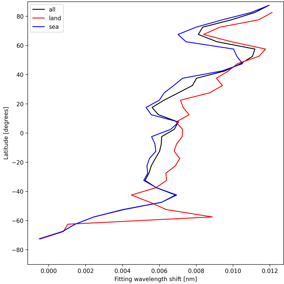
Figure 31: Zonal average of “Fitting wavelength shift” for 2025-05-10 to 2025-05-11.
