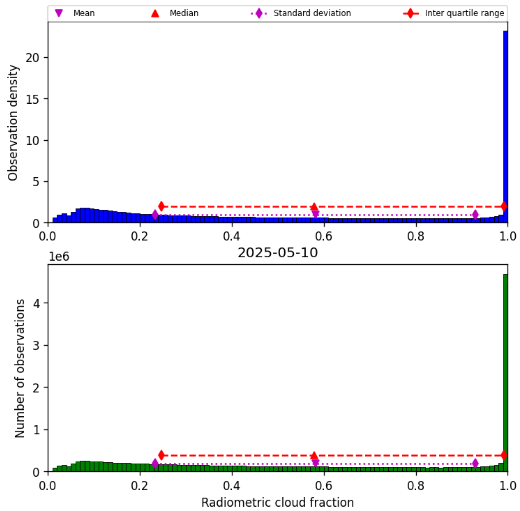
Figure 37: Histogram of “Radiometric cloud fraction” for 2025-05-10 to 2025-05-11
