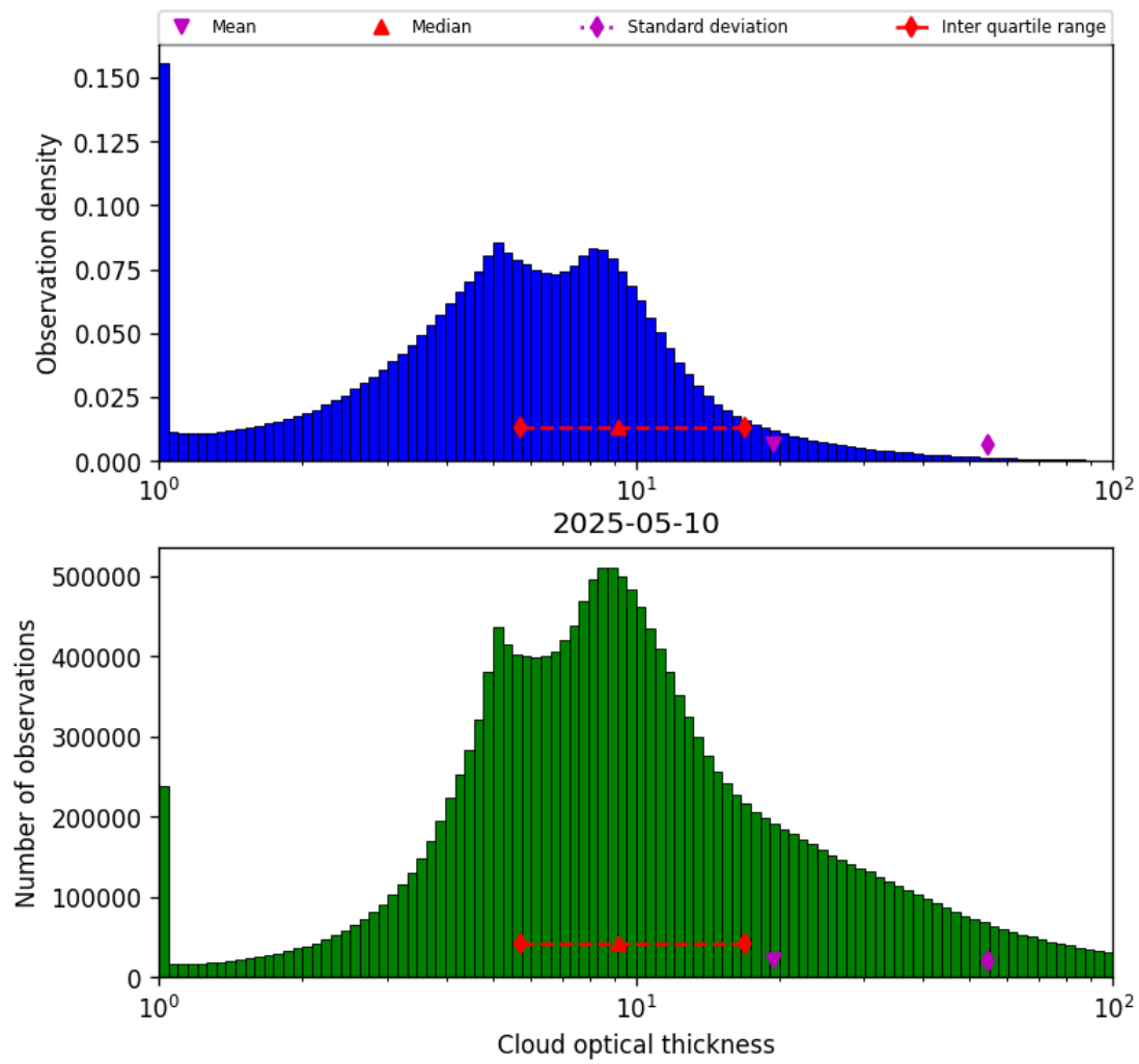
Figure 39: Histogram of “Cloud optical thickness” for 2025-05-10 to 2025-05-11
