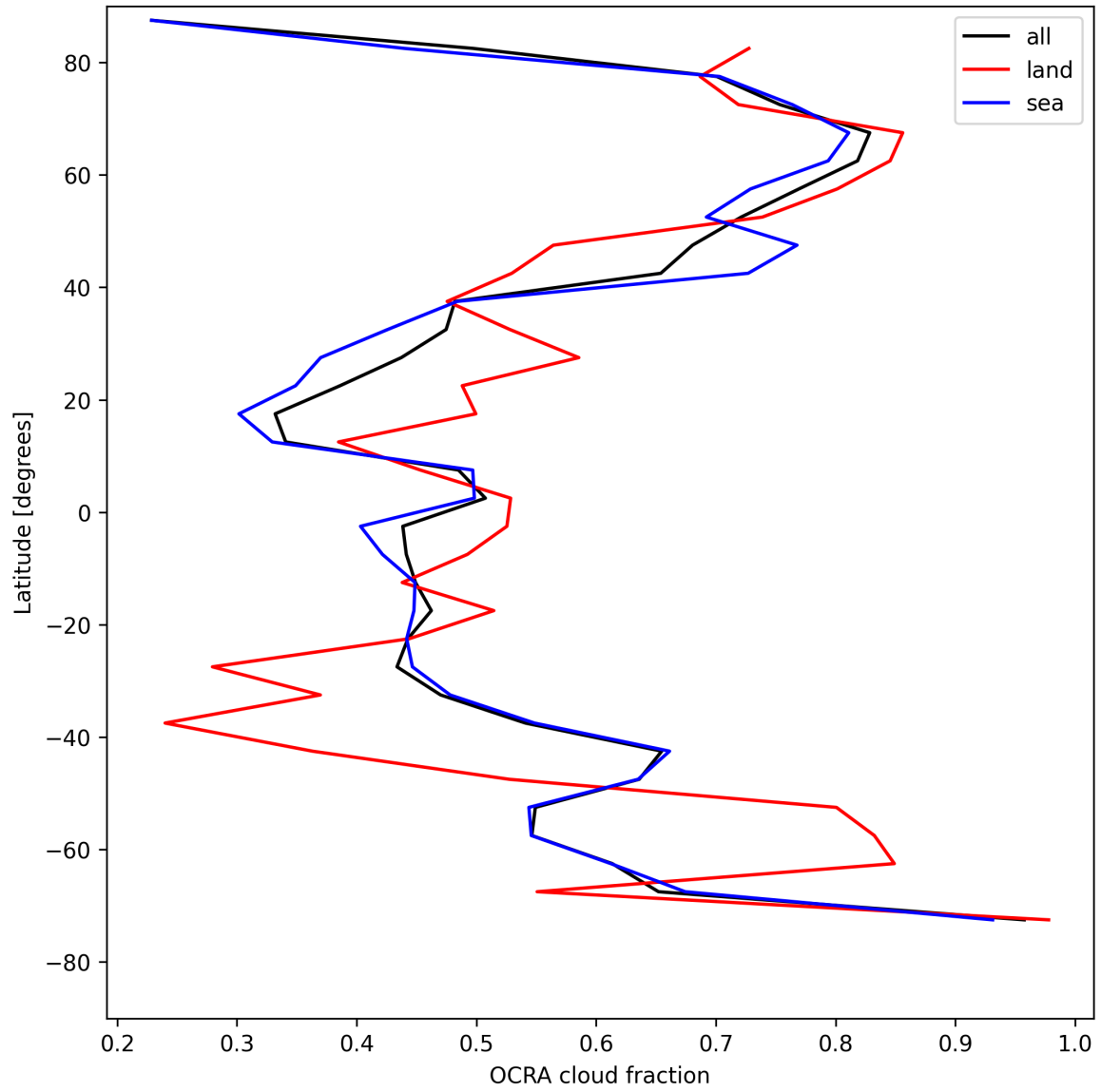
Figure 32: Zonal average of “OCRA cloud fraction” for 2025-05-10 to 2025-05-11.
