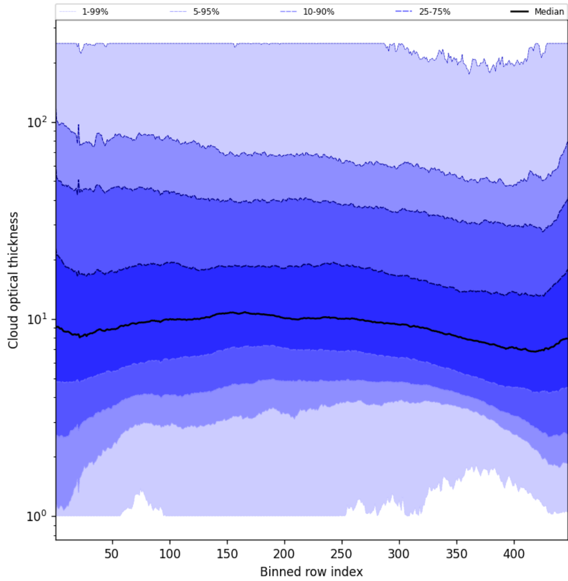
Figure 55: Along track statistics of “Cloud optical thickness” for 2025-05-10 to 2025-05-11
