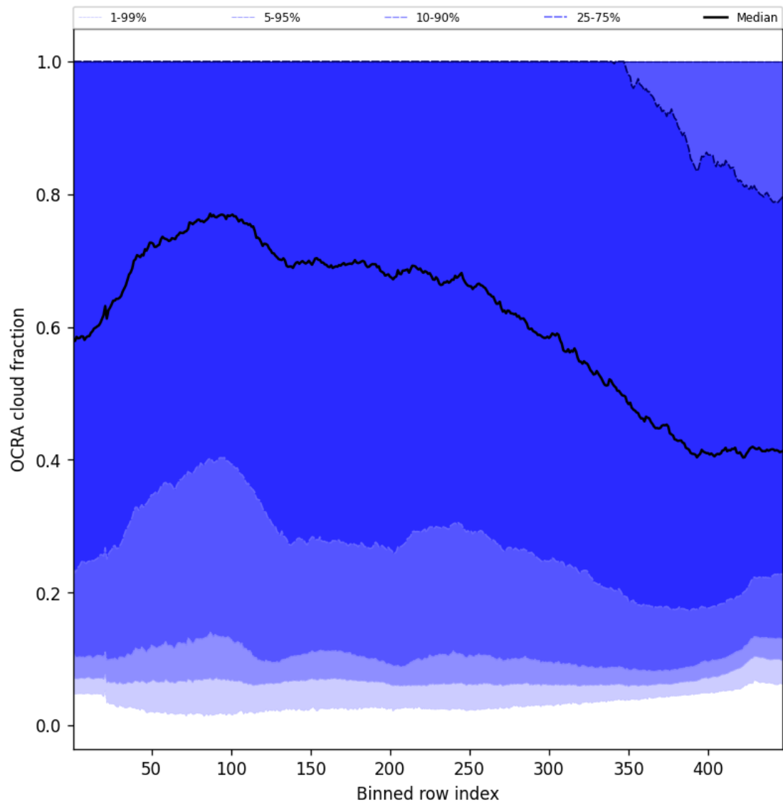
Figure 64: Along track statistics of “OCRA cloud fraction” for 2025-05-10 to 2025-05-11
