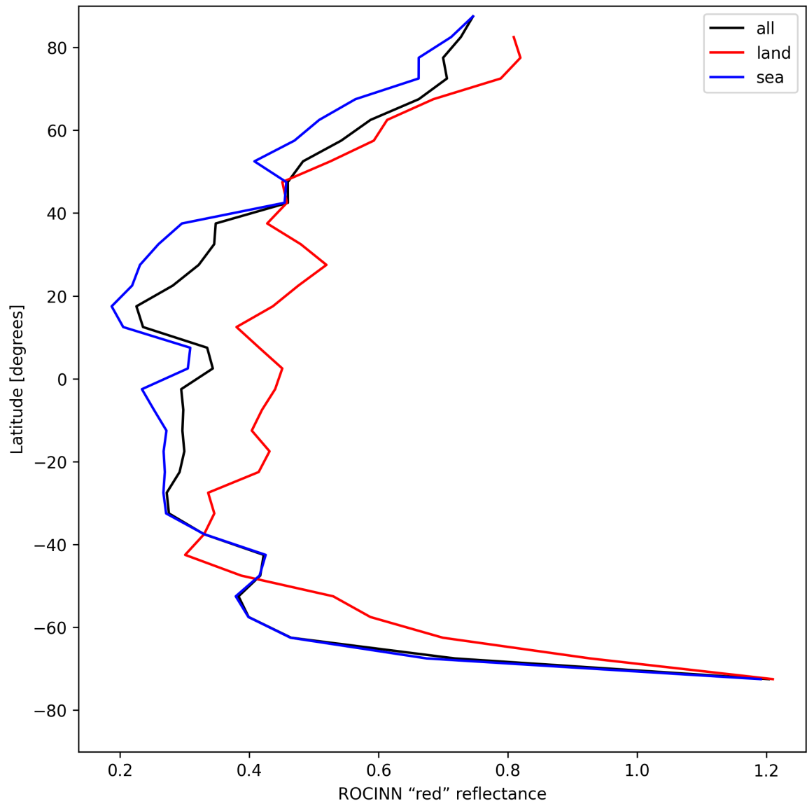
Figure 35: Zonal average of “ROCINN “red” reflectance” for 2025-05-10 to 2025-05-11.
