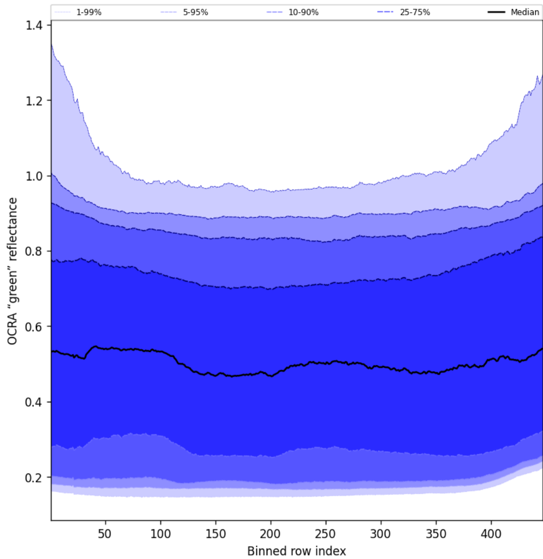
Figure 66: Along track statistics of “OCRA “green” reflectance” for 2025-05-10 to 2025-05-11
