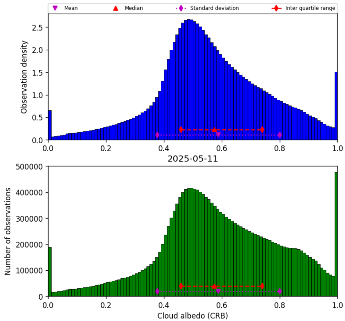
Figure 42: Histogram of “Cloud albedo (CRB)” for 2025-05-11 to 2025-05-12
