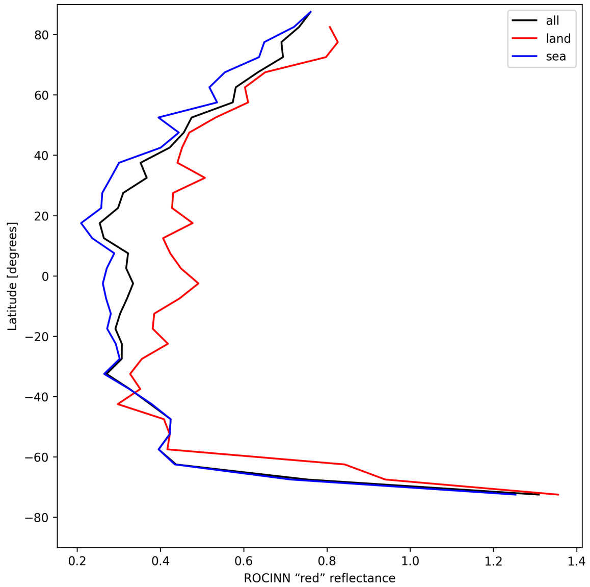
Figure 35: Zonal average of “ROCINN “red” reflectance” for 2025-05-11 to 2025-05-12.
