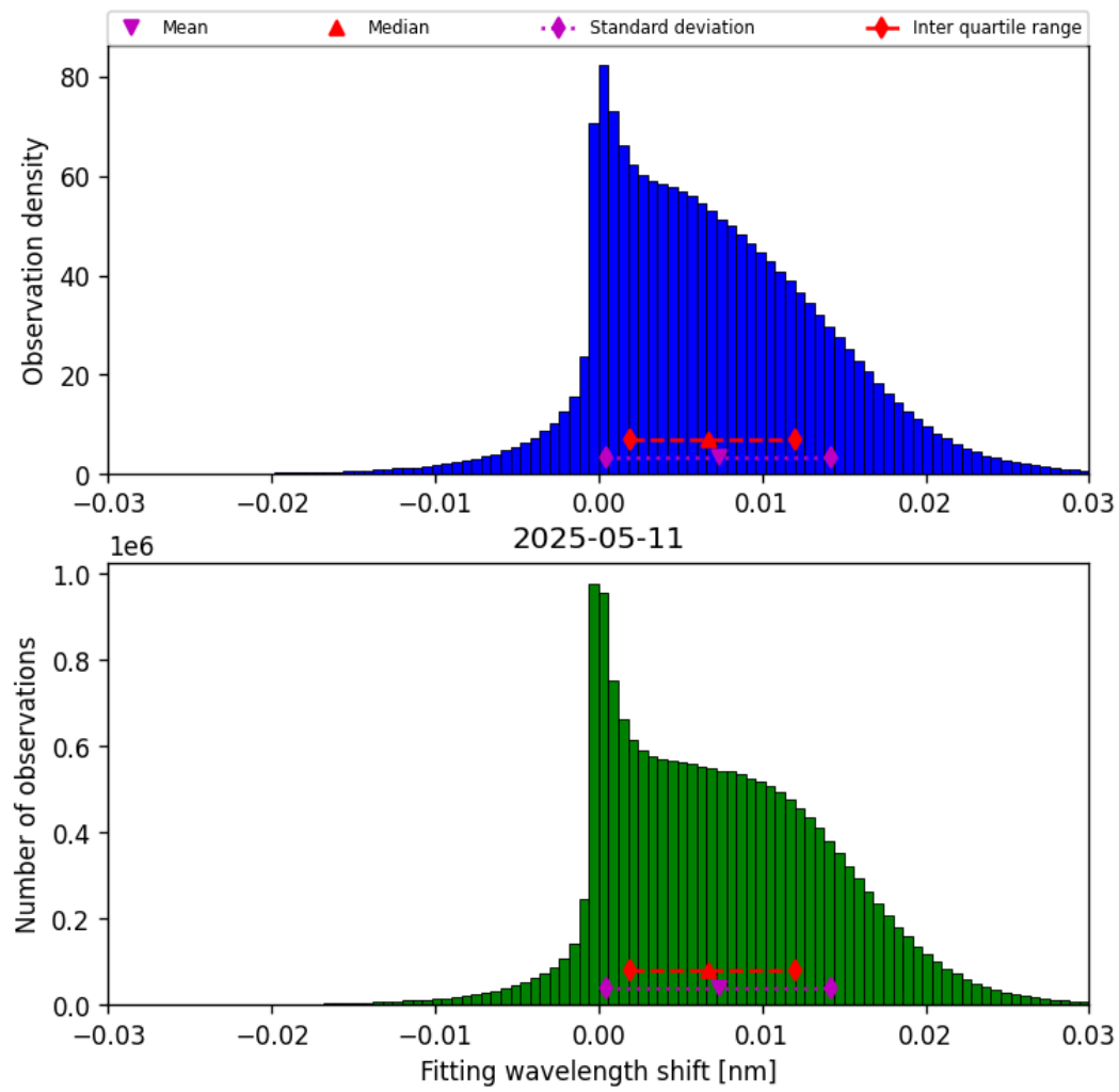
Figure 47: Histogram of “Fitting wavelength shift” for 2025-05-11 to 2025-05-12
