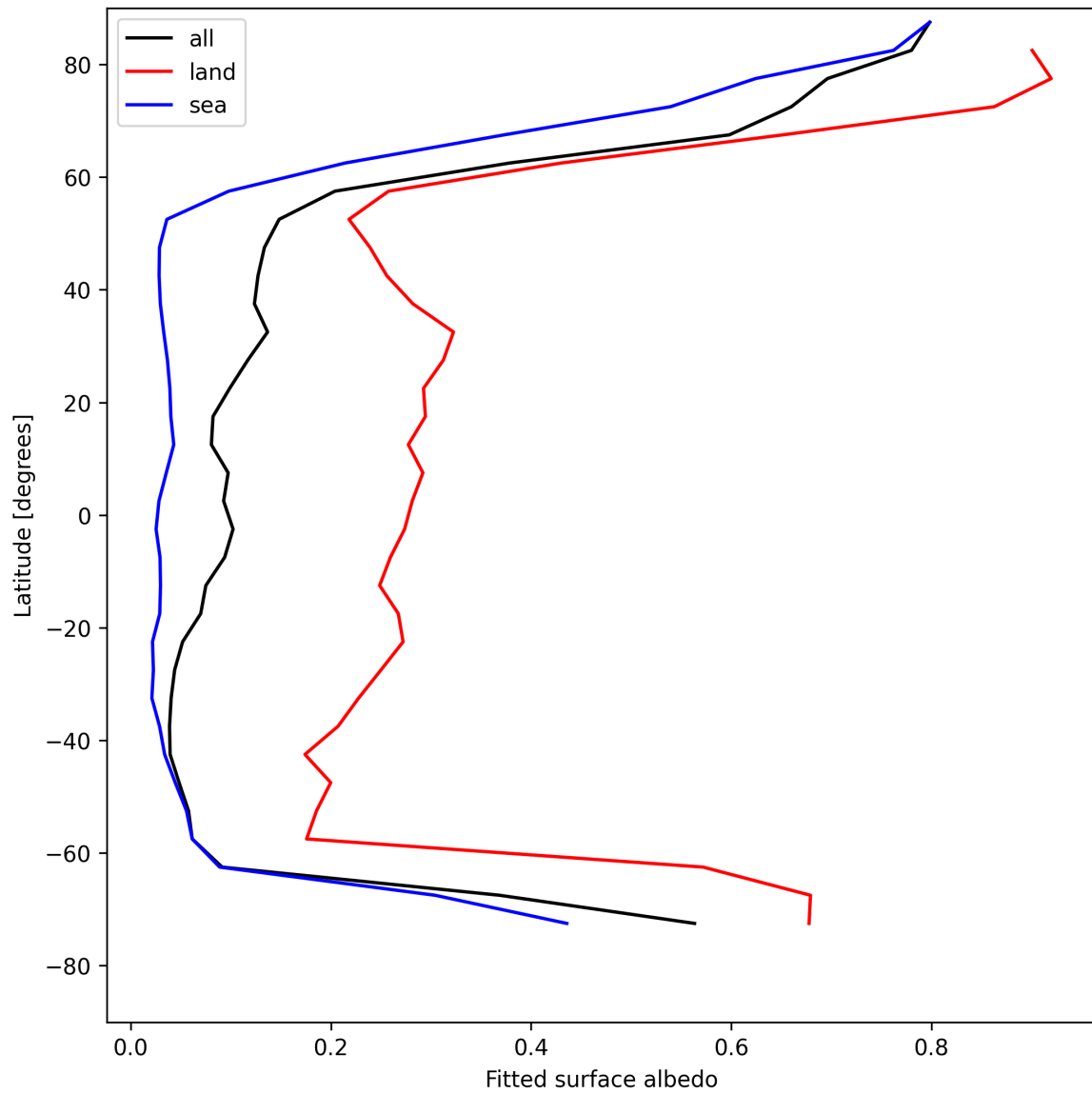
Figure 27: Zonal average of “Fitted surface albedo” for 2025-05-11 to 2025-05-12.
