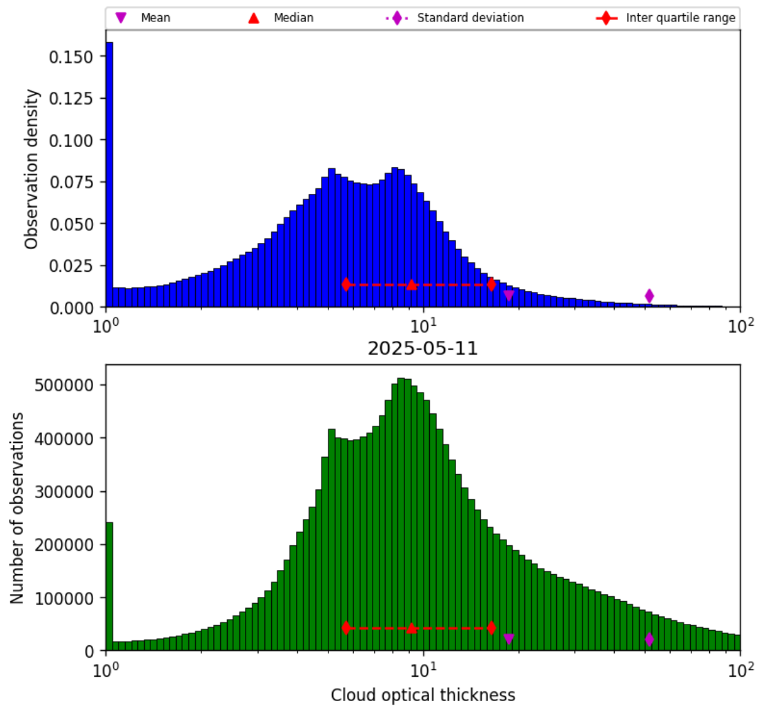
Figure 39: Histogram of “Cloud optical thickness” for 2025-05-11 to 2025-05-12
