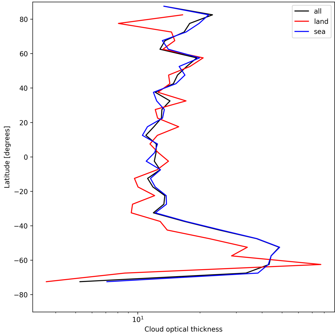
Figure 23: Zonal average of “Cloud optical thickness” for 2025-05-11 to 2025-05-12.
