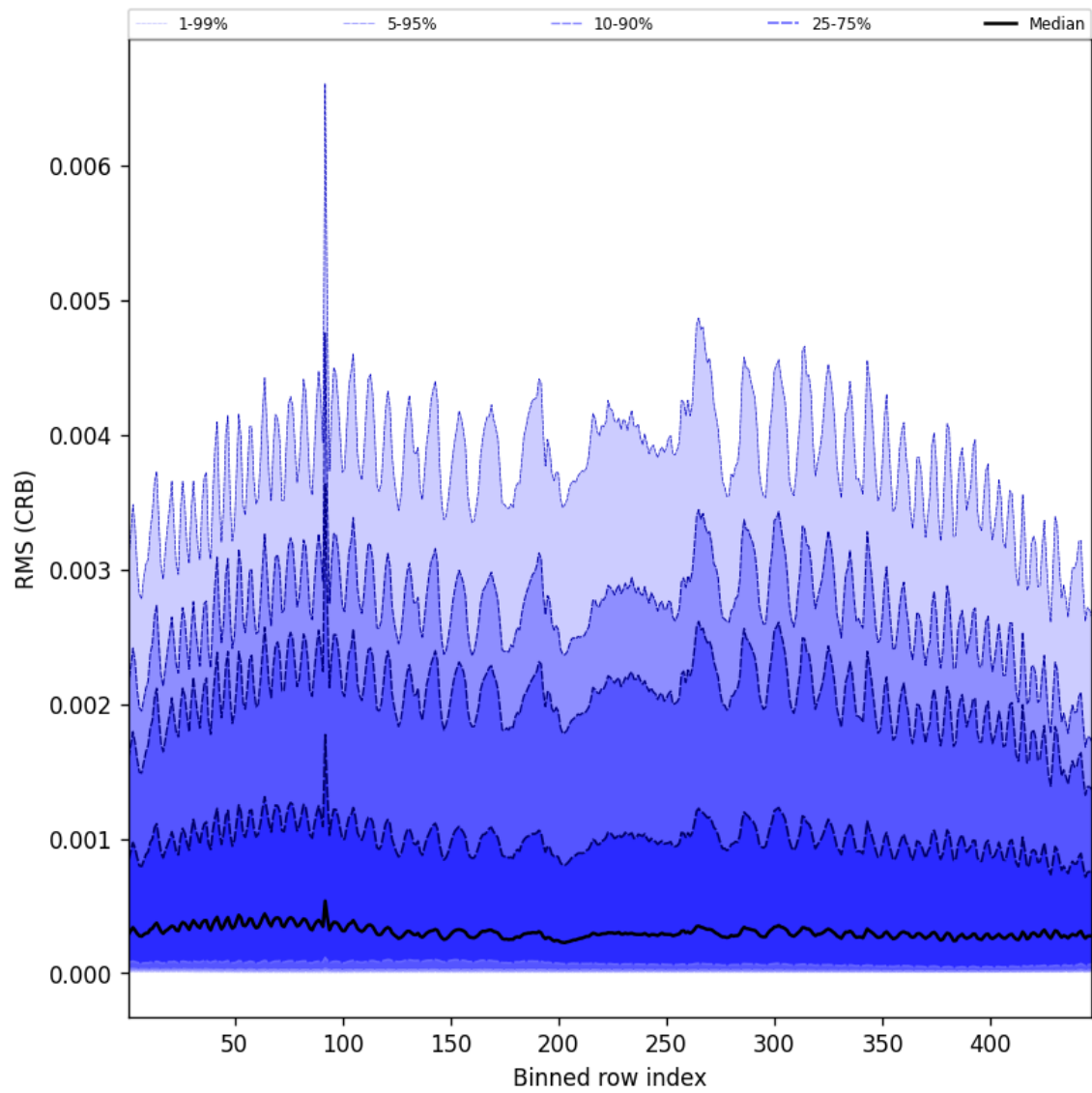
Figure 62: Along track statistics of “RMS (CRB)” for 2025-05-11 to 2025-05-12
