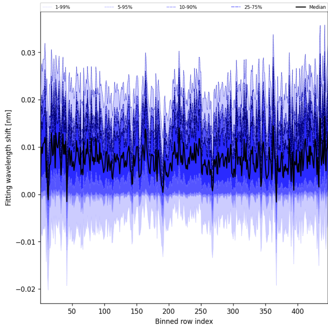
Figure 63: Along track statistics of “Fitting wavelength shift” for 2025-05-11 to 2025-05-12
