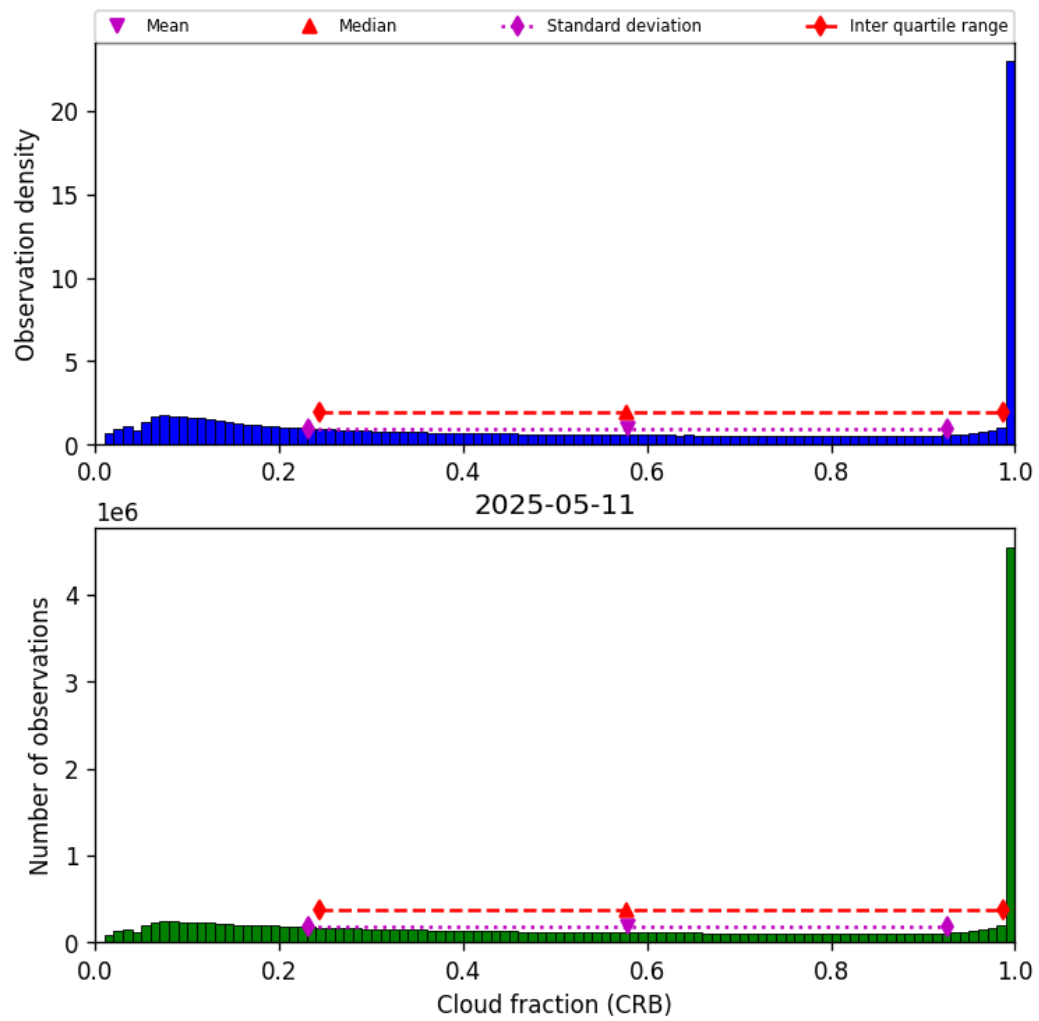
Figure 40: Histogram of “Cloud fraction (CRB)” for 2025-05-11 to 2025-05-12
