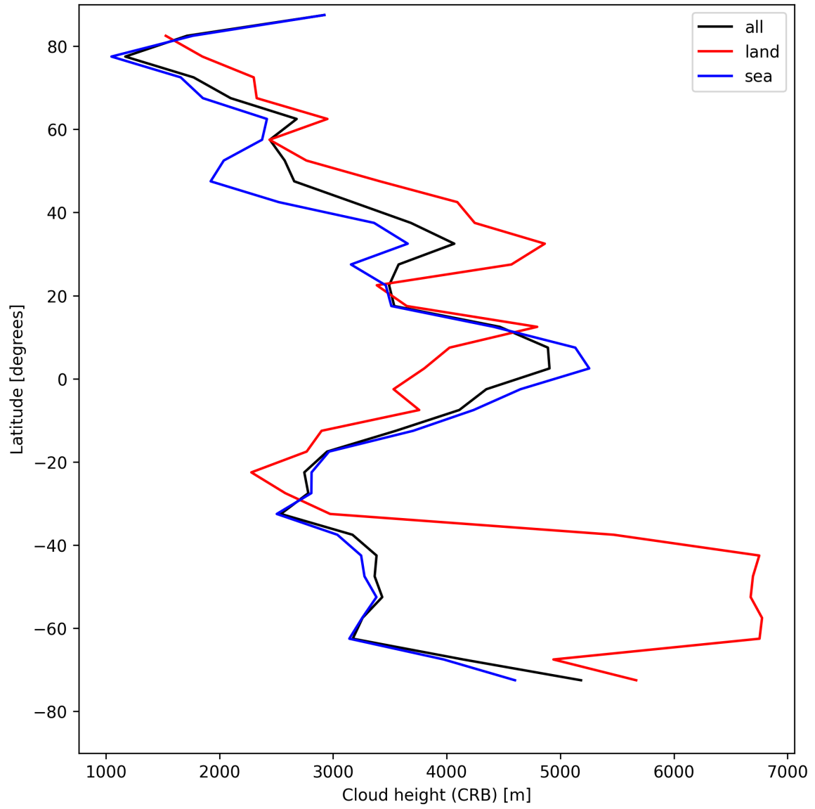
Figure 25: Zonal average of “Cloud height (CRB)” for 2025-05-11 to 2025-05-12.
