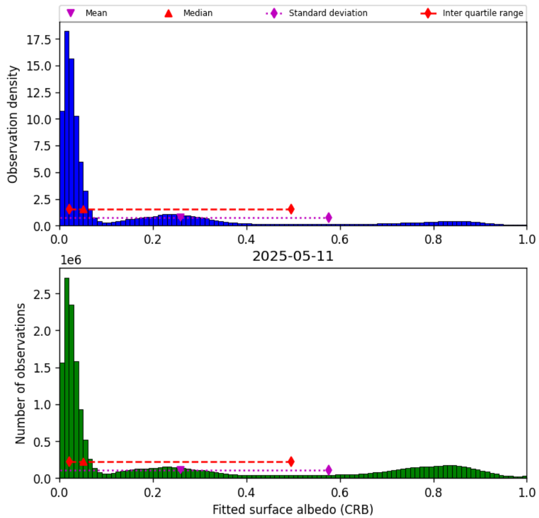
Figure 44: Histogram of “Fitted surface albedo (CRB)” for 2025-05-11 to 2025-05-12
