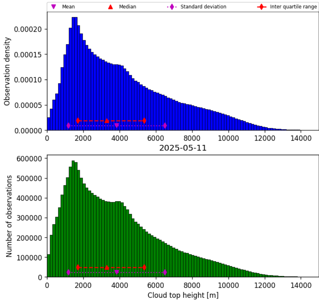
Figure 38: Histogram of “Cloud top height” for 2025-05-11 to 2025-05-12
