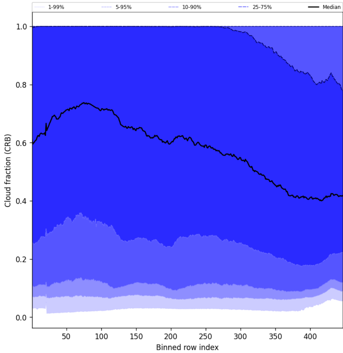
Figure 56: Along track statistics of “Cloud fraction (CRB)” for 2025-05-11 to 2025-05-12
