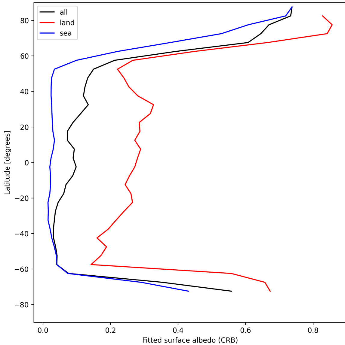
Figure 28: Zonal average of “Fitted surface albedo (CRB)” for 2025-05-11 to 2025-05-12.
