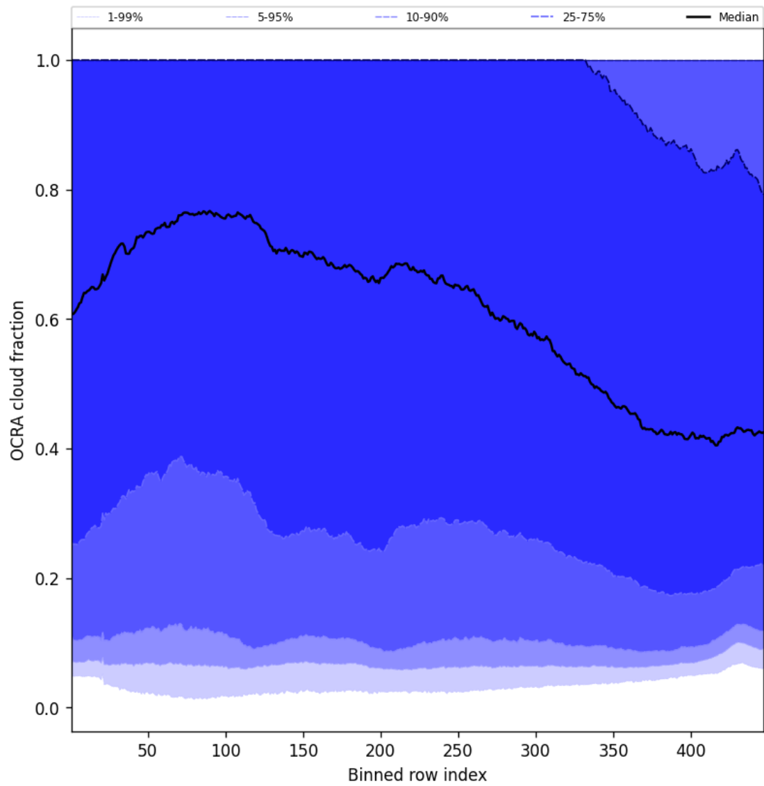
Figure 64: Along track statistics of “OCRA cloud fraction” for 2025-05-11 to 2025-05-12
