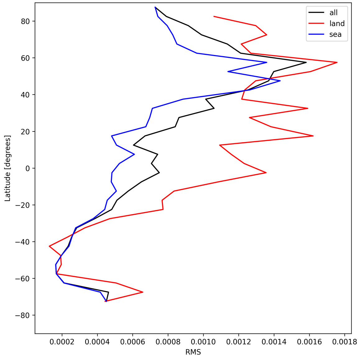
Figure 29: Zonal average of “RMS” for 2025-05-11 to 2025-05-12.
