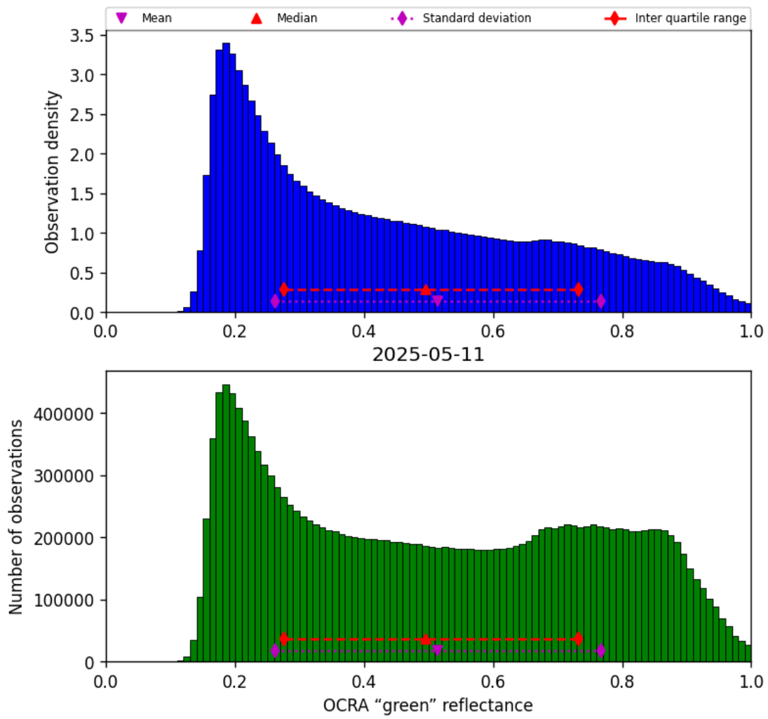
Figure 50: Histogram of “OCRA “green” reflectance” for 2025-05-11 to 2025-05-12
