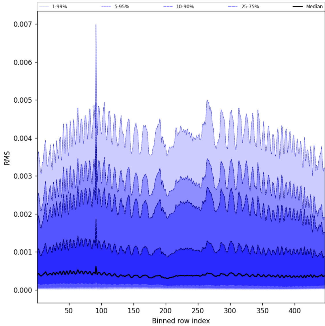
Figure 61: Along track statistics of “RMS” for 2025-05-11 to 2025-05-12
