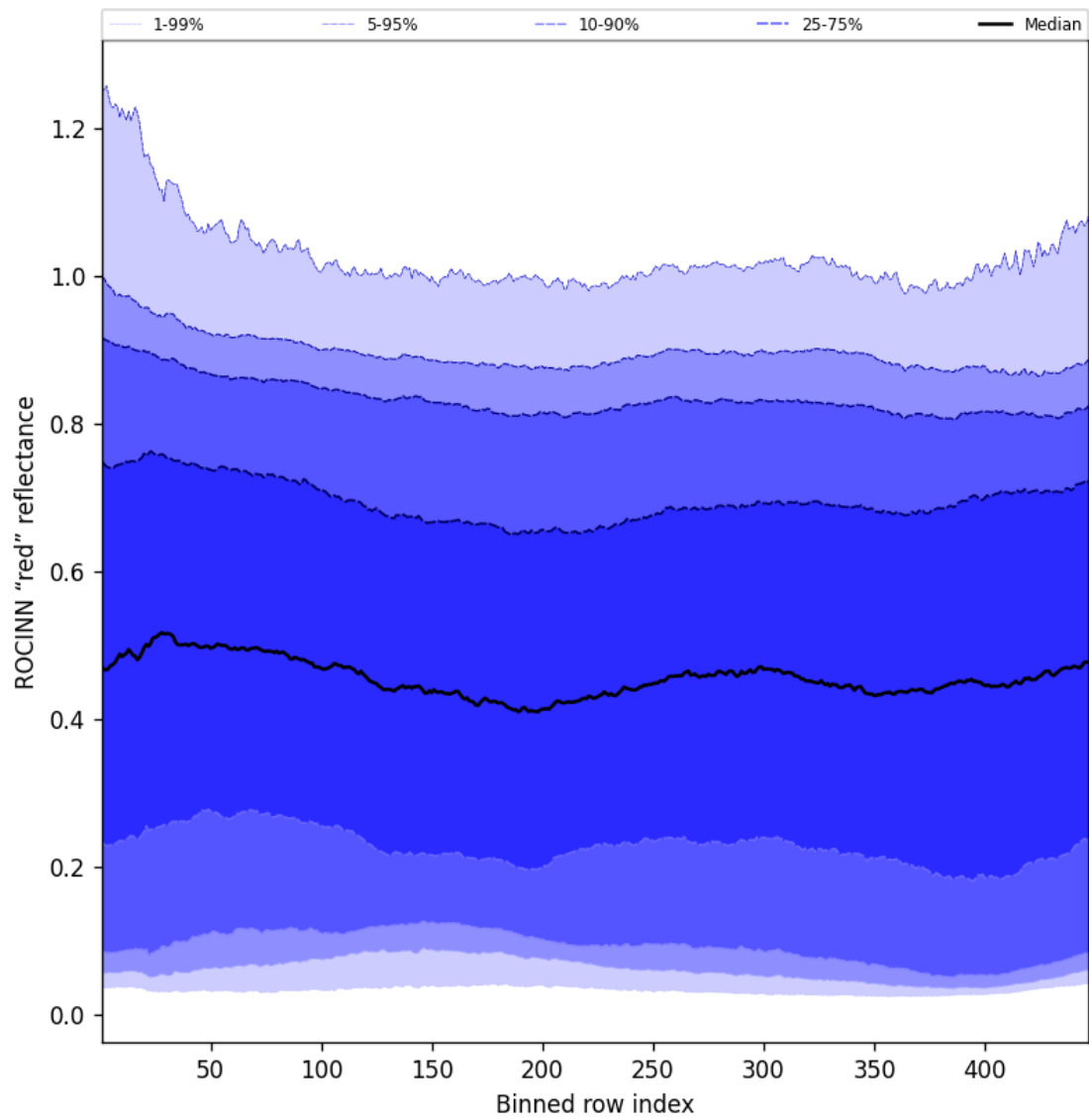
Figure 67: Along track statistics of “ROCINN “red” reflectance” for 2025-05-11 to 2025-05-12
