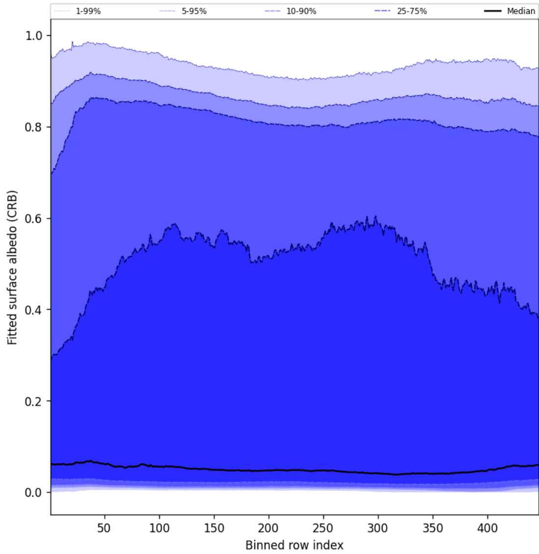
Figure 60: Along track statistics of “Fitted surface albedo (CRB)” for 2025-05-11 to 2025-05-12
