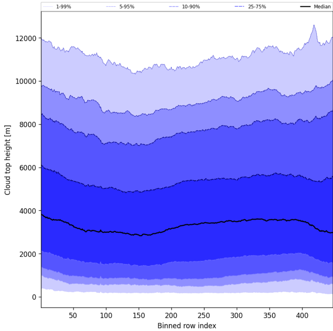
Figure 54: Along track statistics of “Cloud top height” for 2025-05-11 to 2025-05-12
