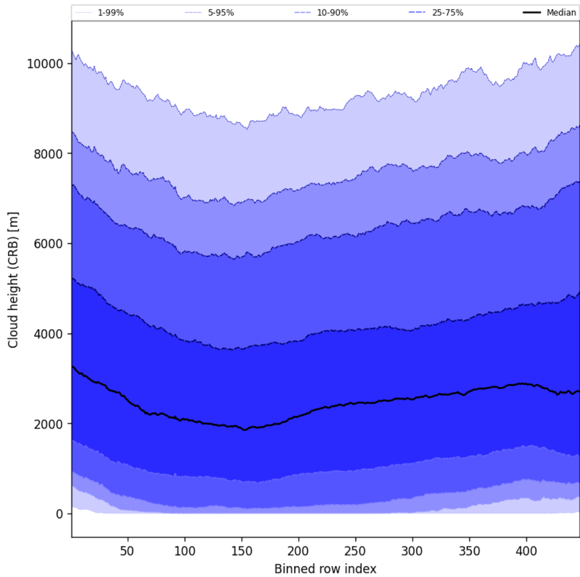
Figure 57: Along track statistics of “Cloud height (CRB)” for 2025-05-11 to 2025-05-12
