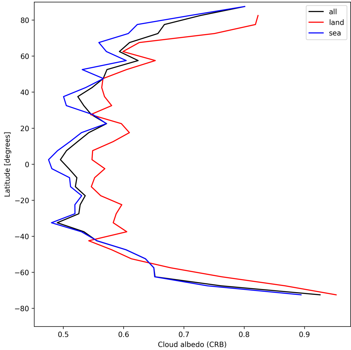
Figure 26: Zonal average of “Cloud albedo (CRB)” for 2025-05-11 to 2025-05-12.
