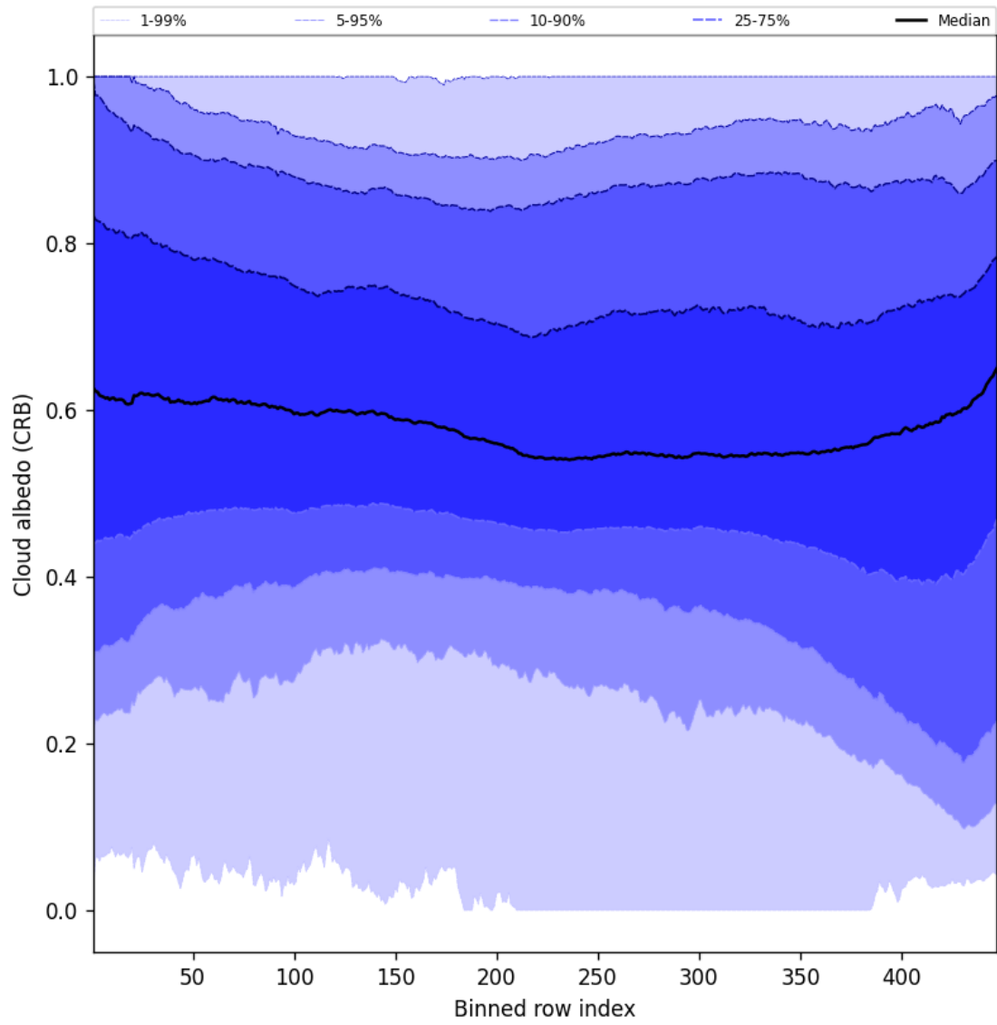
Figure 58: Along track statistics of “Cloud albedo (CRB)” for 2025-05-11 to 2025-05-12
