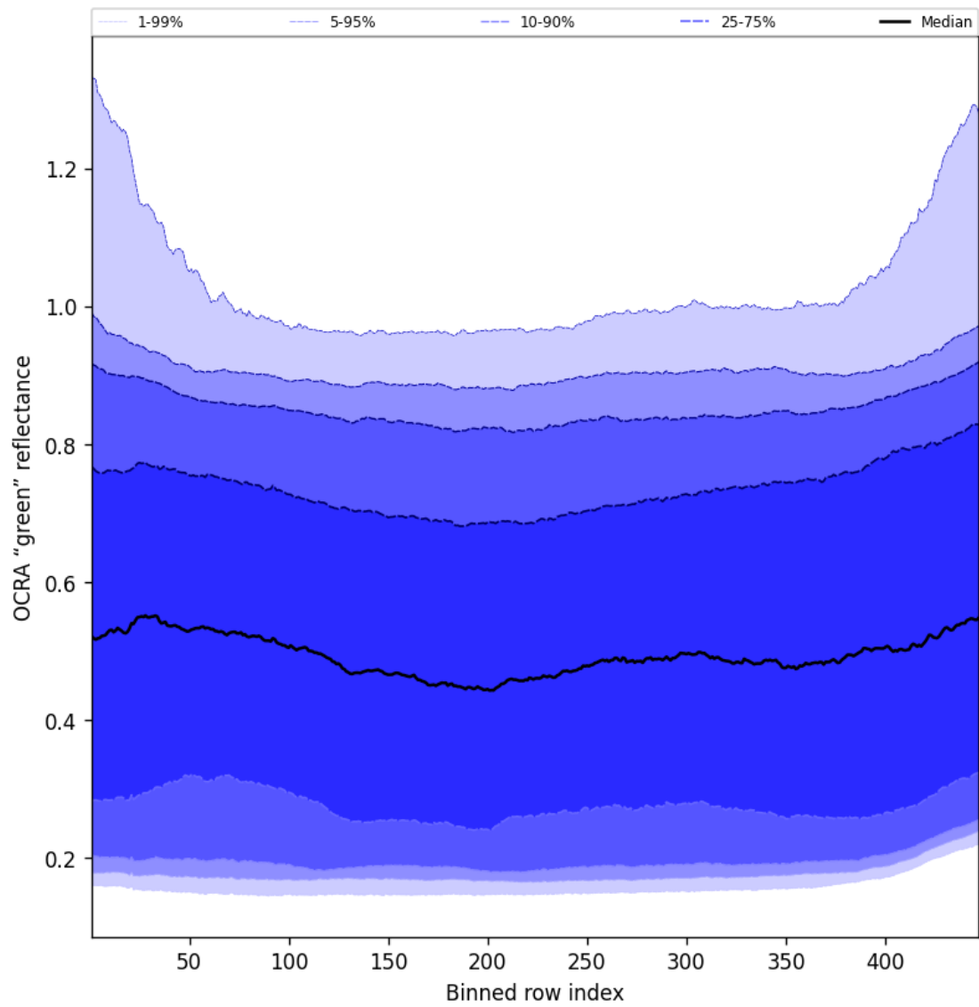
Figure 66: Along track statistics of “OCRA “green” reflectance” for 2025-05-11 to 2025-05-12
