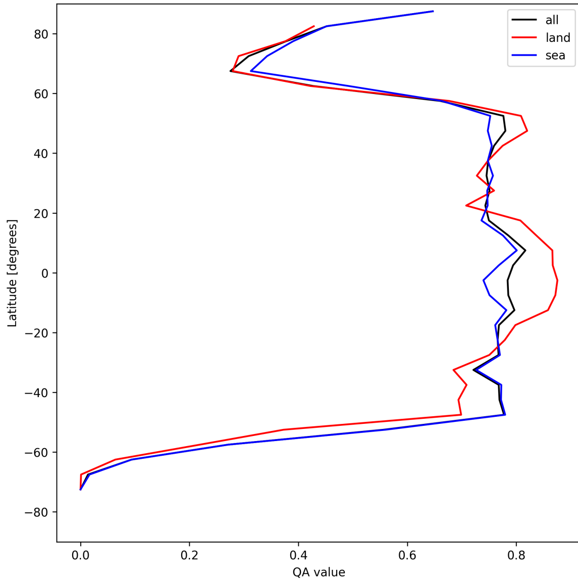
Figure 20: Zonal average of “QA value” for 2025-05-11 to 2025-05-12.
