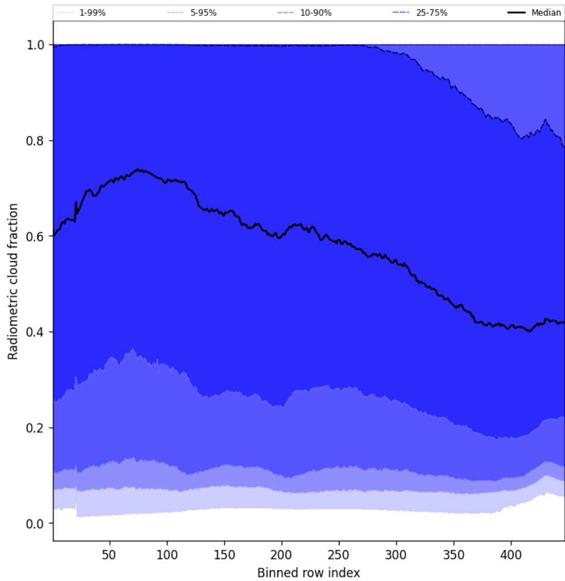
Figure 53: Along track statistics of “Radiometric cloud fraction” for 2025-05-11 to 2025-05-12
