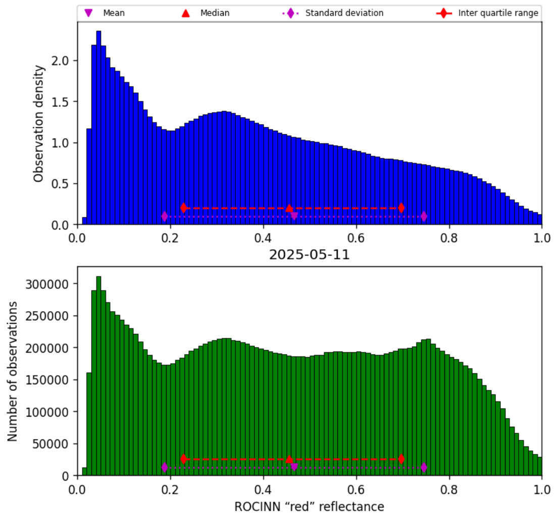
Figure 51: Histogram of “ROCINN “red” reflectance” for 2025-05-11 to 2025-05-12
