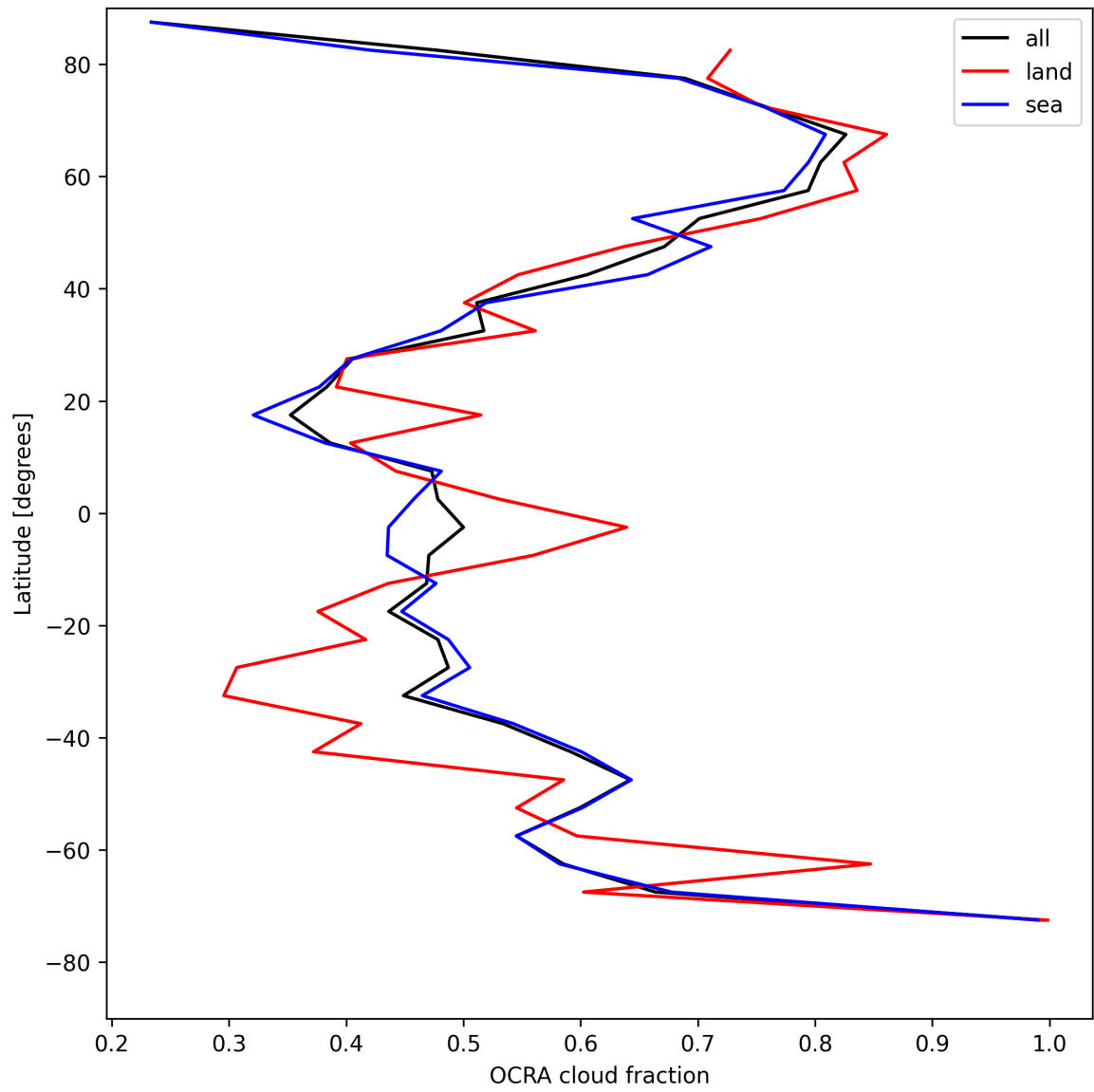
Figure 32: Zonal average of “OCRA cloud fraction” for 2025-05-11 to 2025-05-12.
