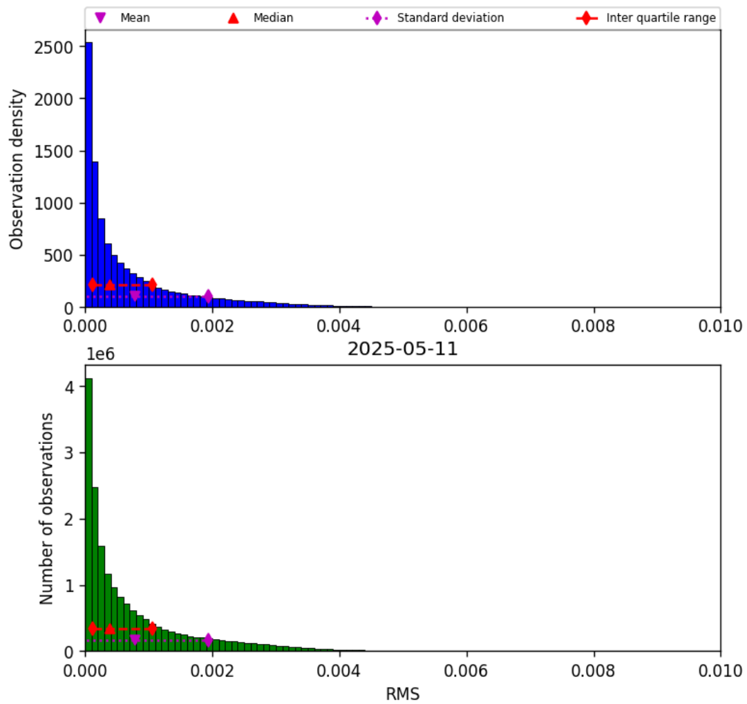
Figure 45: Histogram of “RMS” for 2025-05-11 to 2025-05-12
