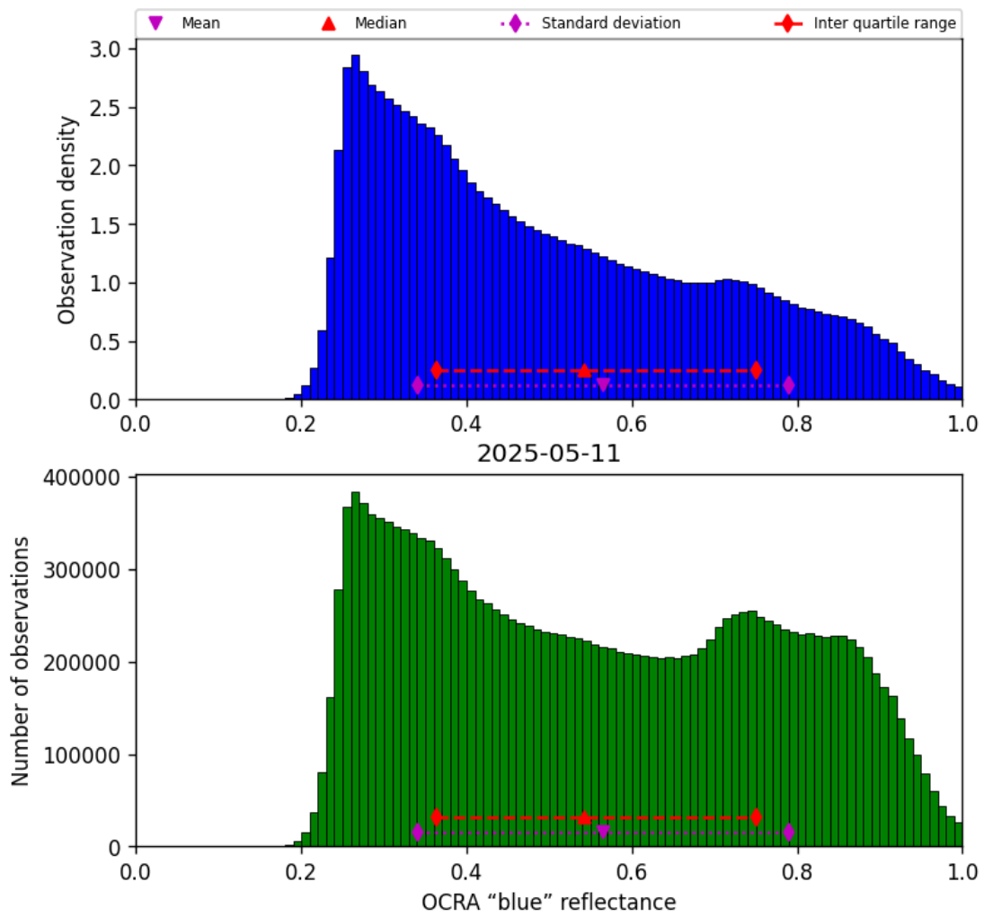
Figure 49: Histogram of “OCRA “blue” reflectance” for 2025-05-11 to 2025-05-12
