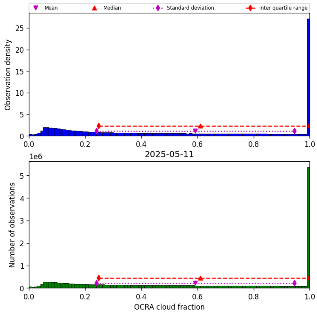
Figure 48: Histogram of “OCRA cloud fraction” for 2025-05-11 to 2025-05-12
