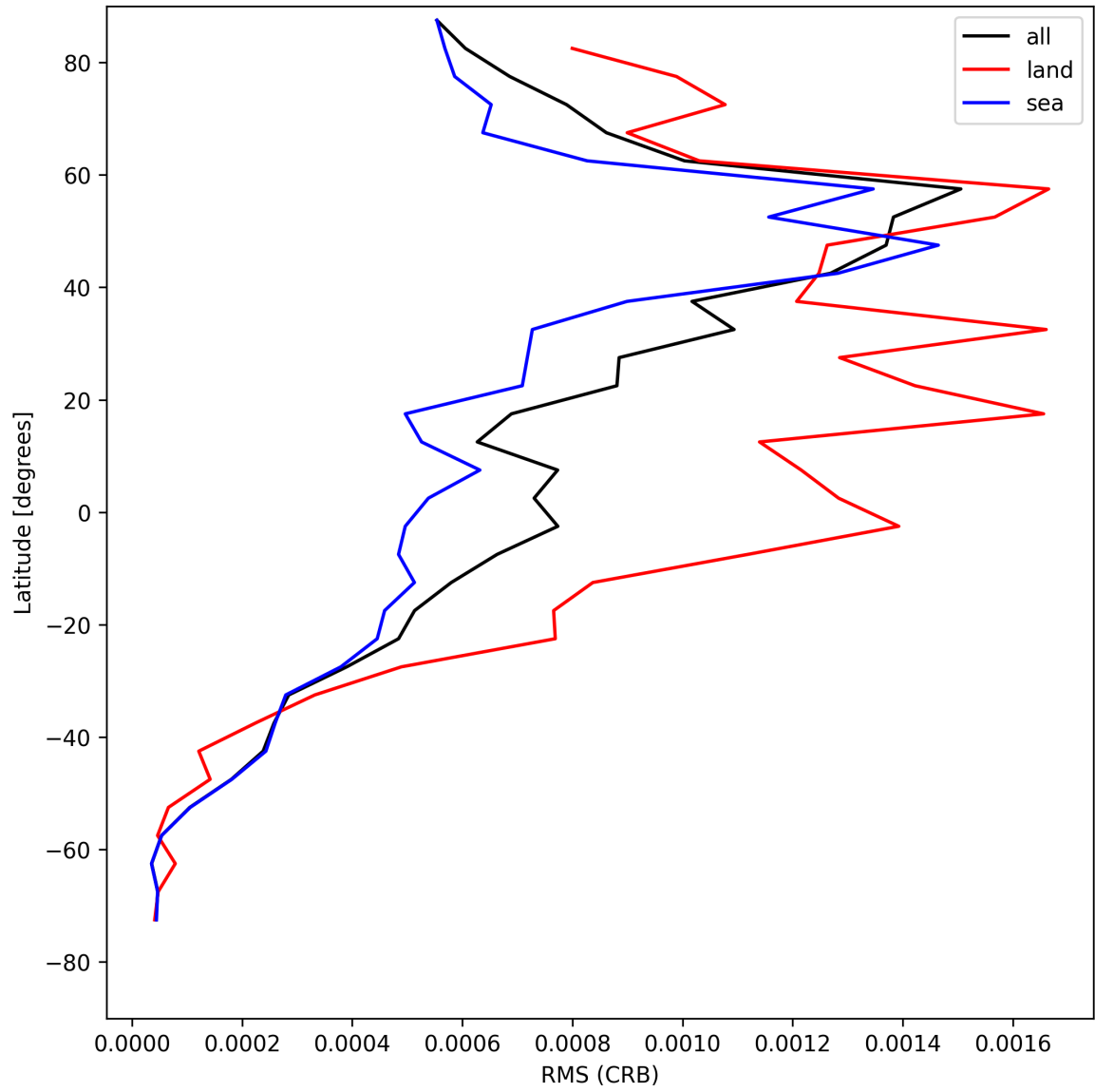
Figure 30: Zonal average of “RMS (CRB)” for 2025-05-11 to 2025-05-12.
