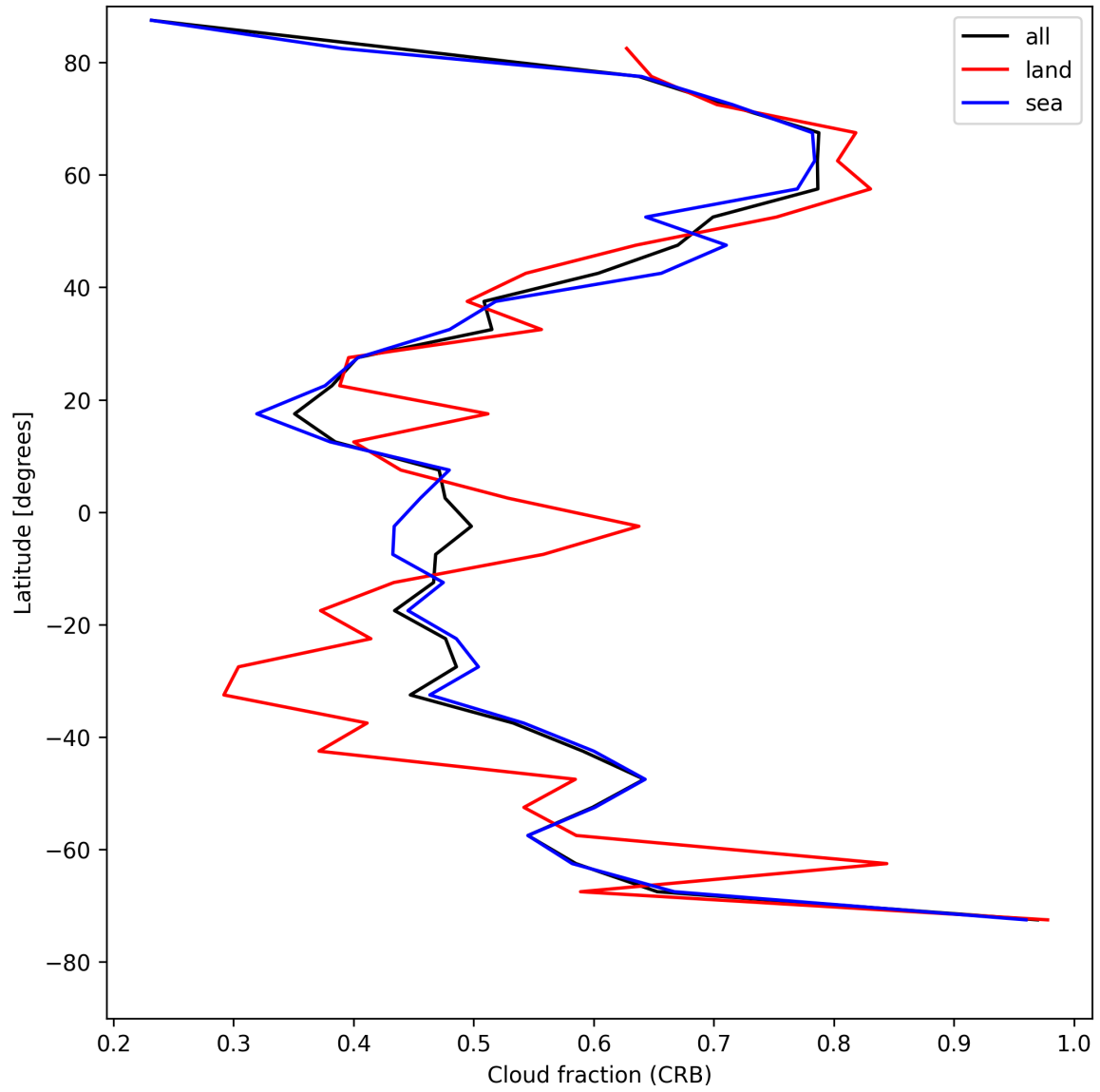
Figure 24: Zonal average of “Cloud fraction (CRB)” for 2025-05-11 to 2025-05-12.
