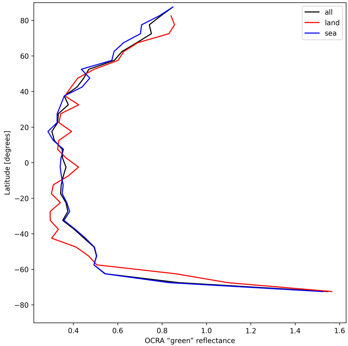
Figure 34: Zonal average of “OCRA “green” reflectance” for 2025-05-11 to 2025-05-12.
