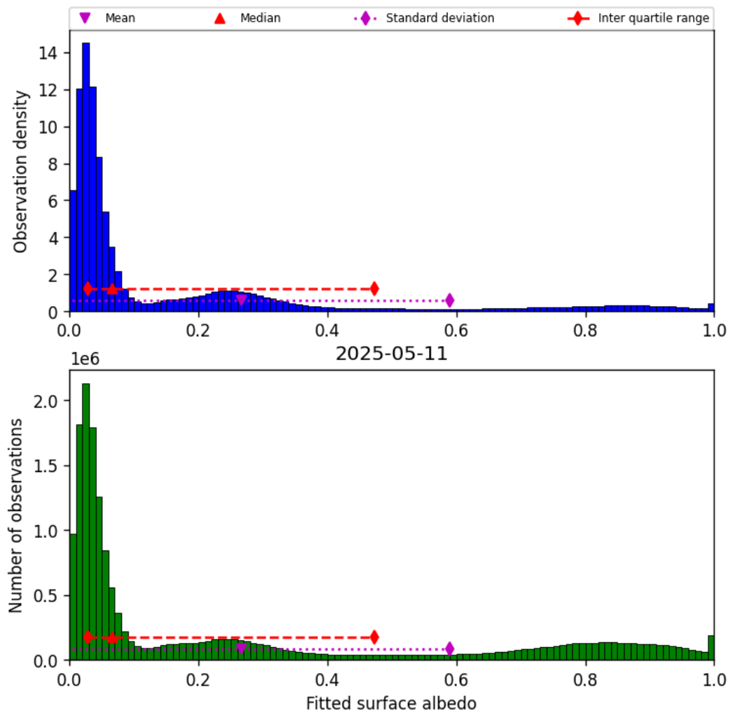
Figure 43: Histogram of “Fitted surface albedo” for 2025-05-11 to 2025-05-12
