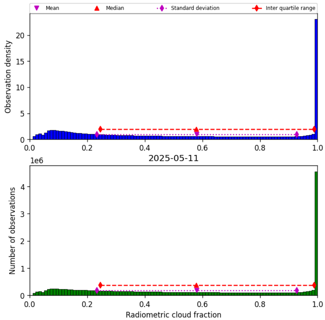
Figure 37: Histogram of “Radiometric cloud fraction” for 2025-05-11 to 2025-05-12
