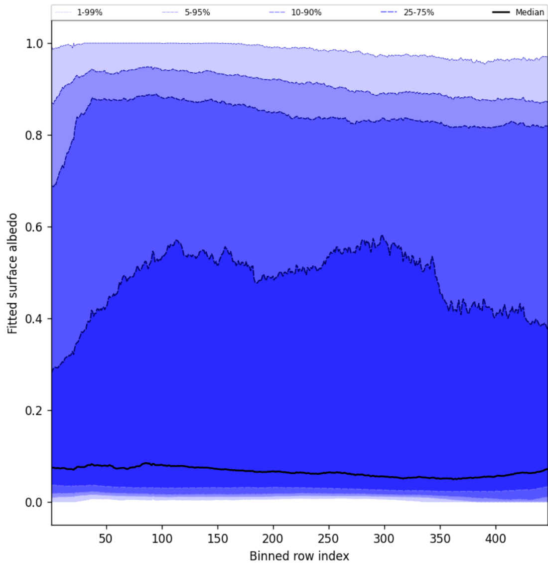
Figure 59: Along track statistics of “Fitted surface albedo” for 2025-05-11 to 2025-05-12
