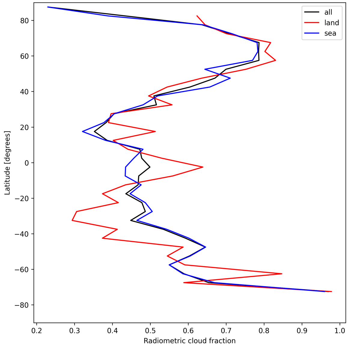
Figure 21: Zonal average of “Radiometric cloud fraction” for 2025-05-11 to 2025-05-12.
