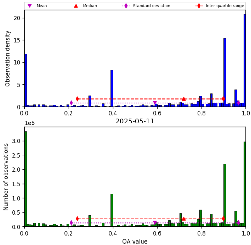
Figure 36: Histogram of “QA value” for 2025-05-11 to 2025-05-12
