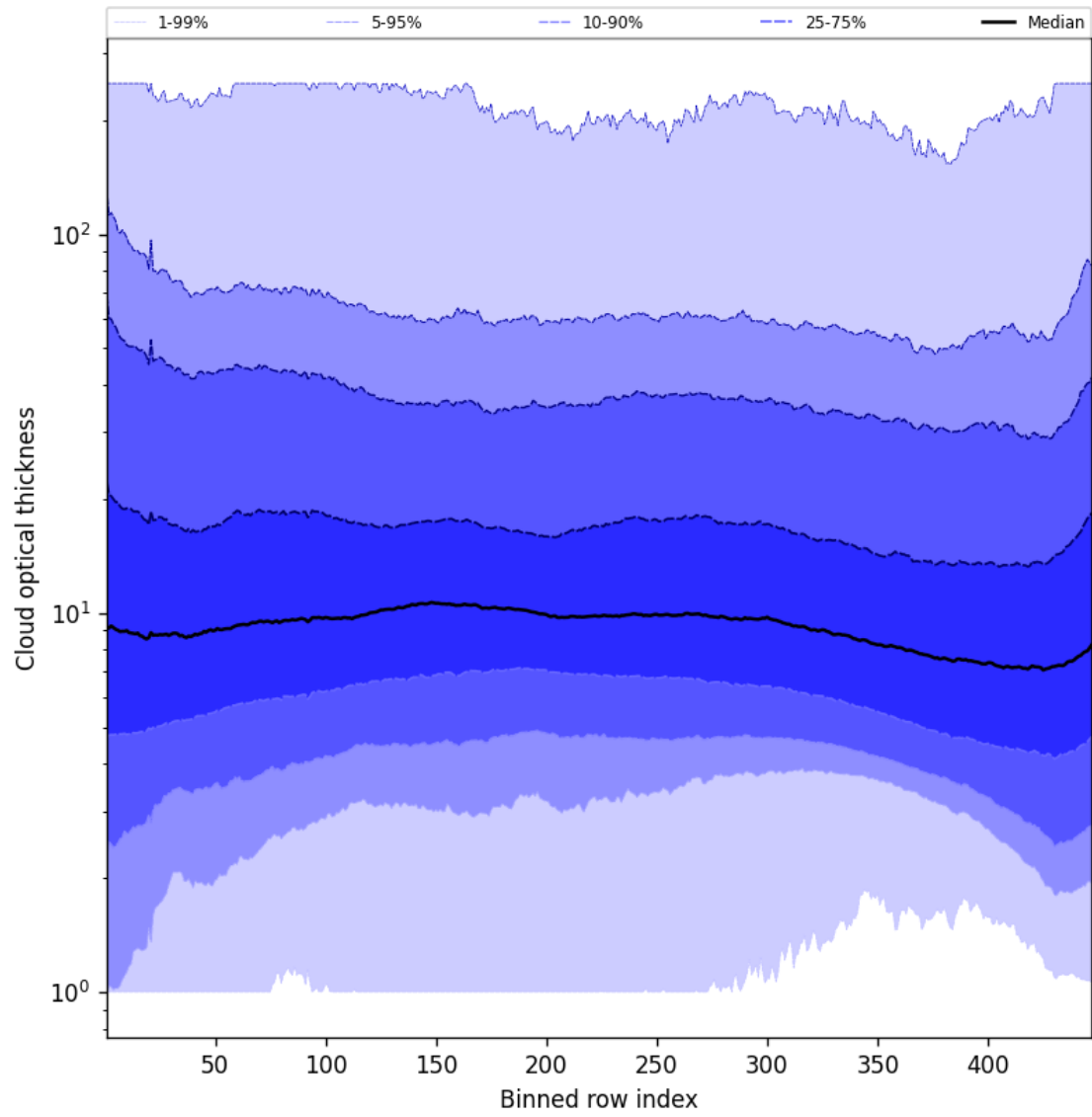
Figure 55: Along track statistics of “Cloud optical thickness” for 2025-05-11 to 2025-05-12
