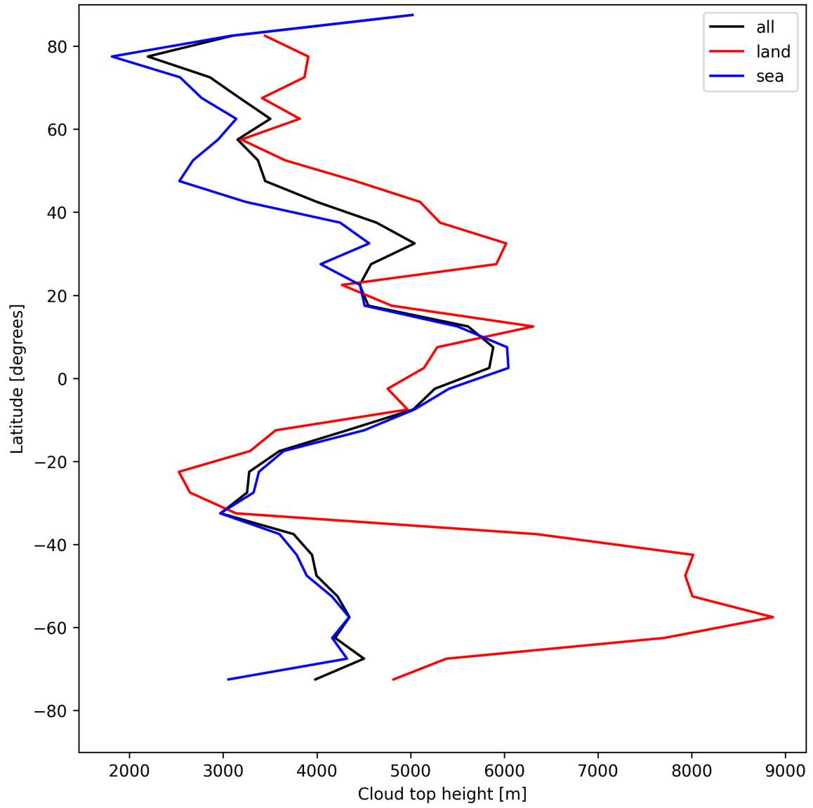
Figure 22: Zonal average of “Cloud top height” for 2025-05-11 to 2025-05-12.
