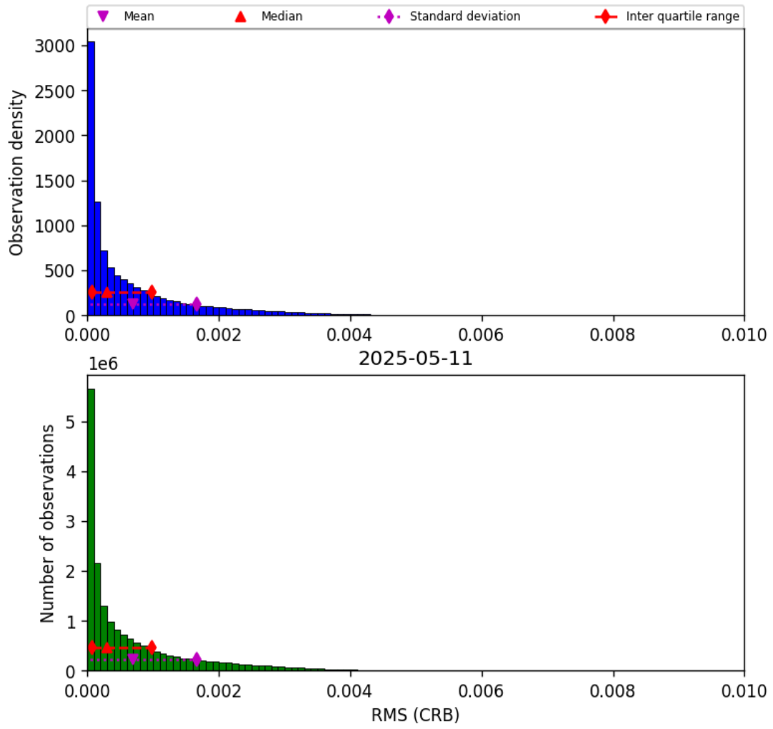
Figure 46: Histogram of “RMS (CRB)” for 2025-05-11 to 2025-05-12
