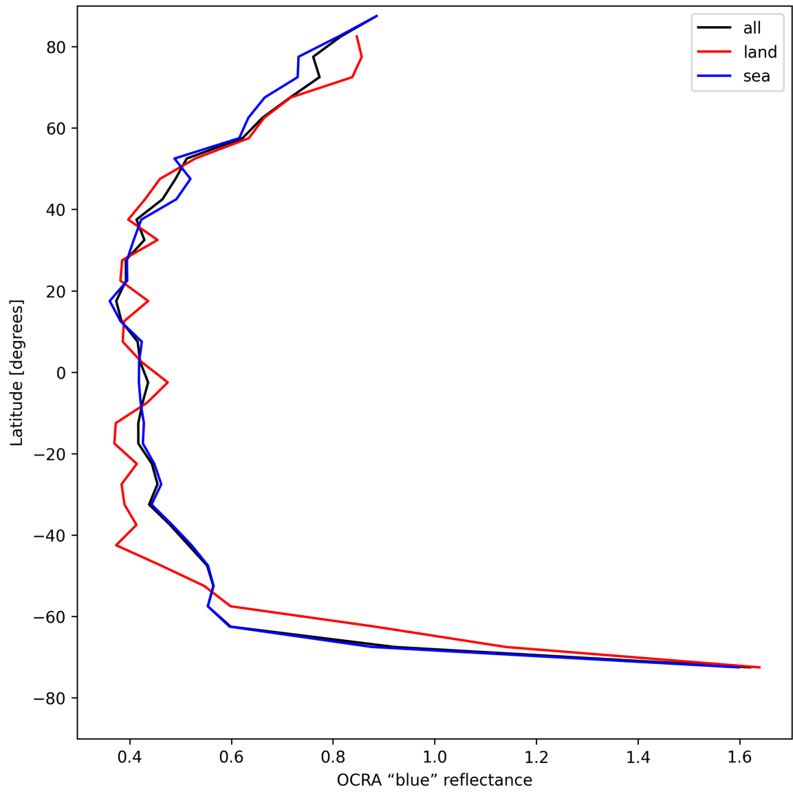
Figure 33: Zonal average of “OCRA “blue” reflectance” for 2025-05-11 to 2025-05-12.
