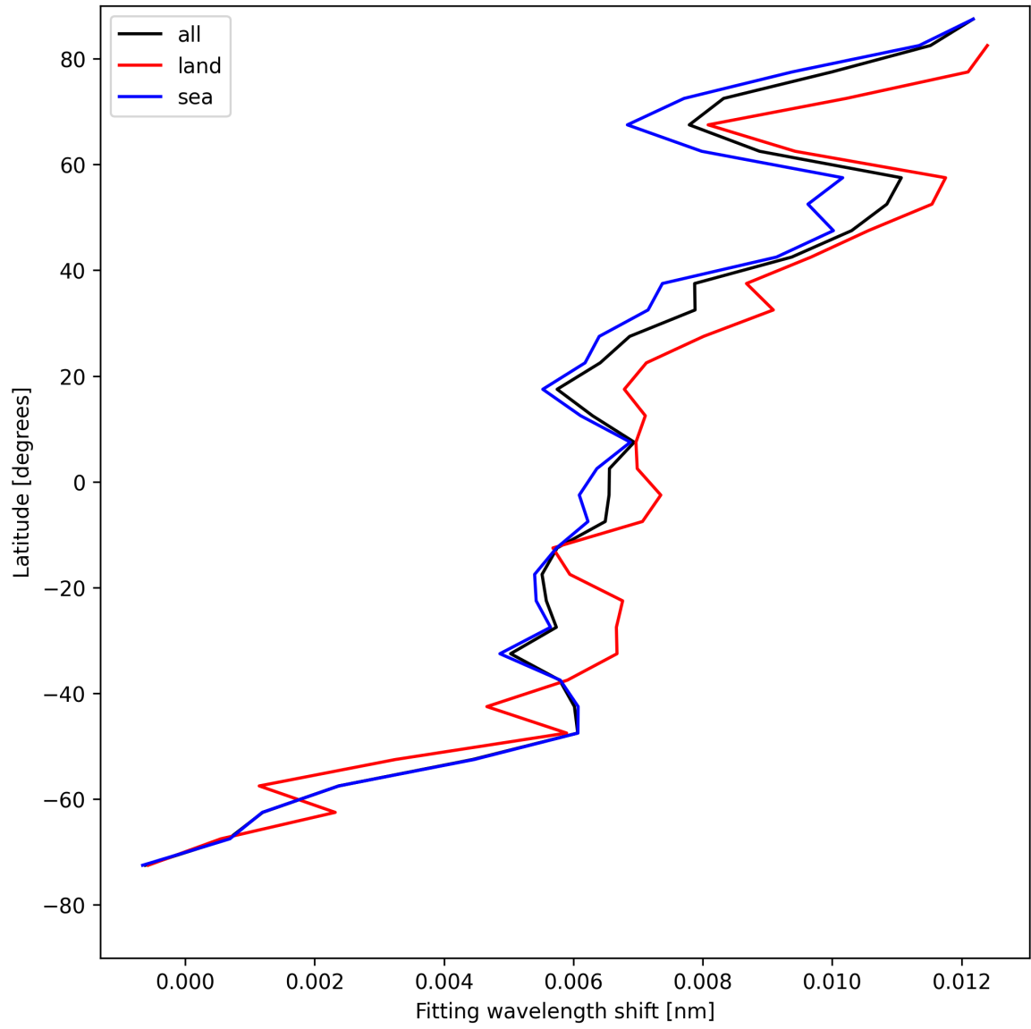
Figure 31: Zonal average of “Fitting wavelength shift” for 2025-05-11 to 2025-05-12.
