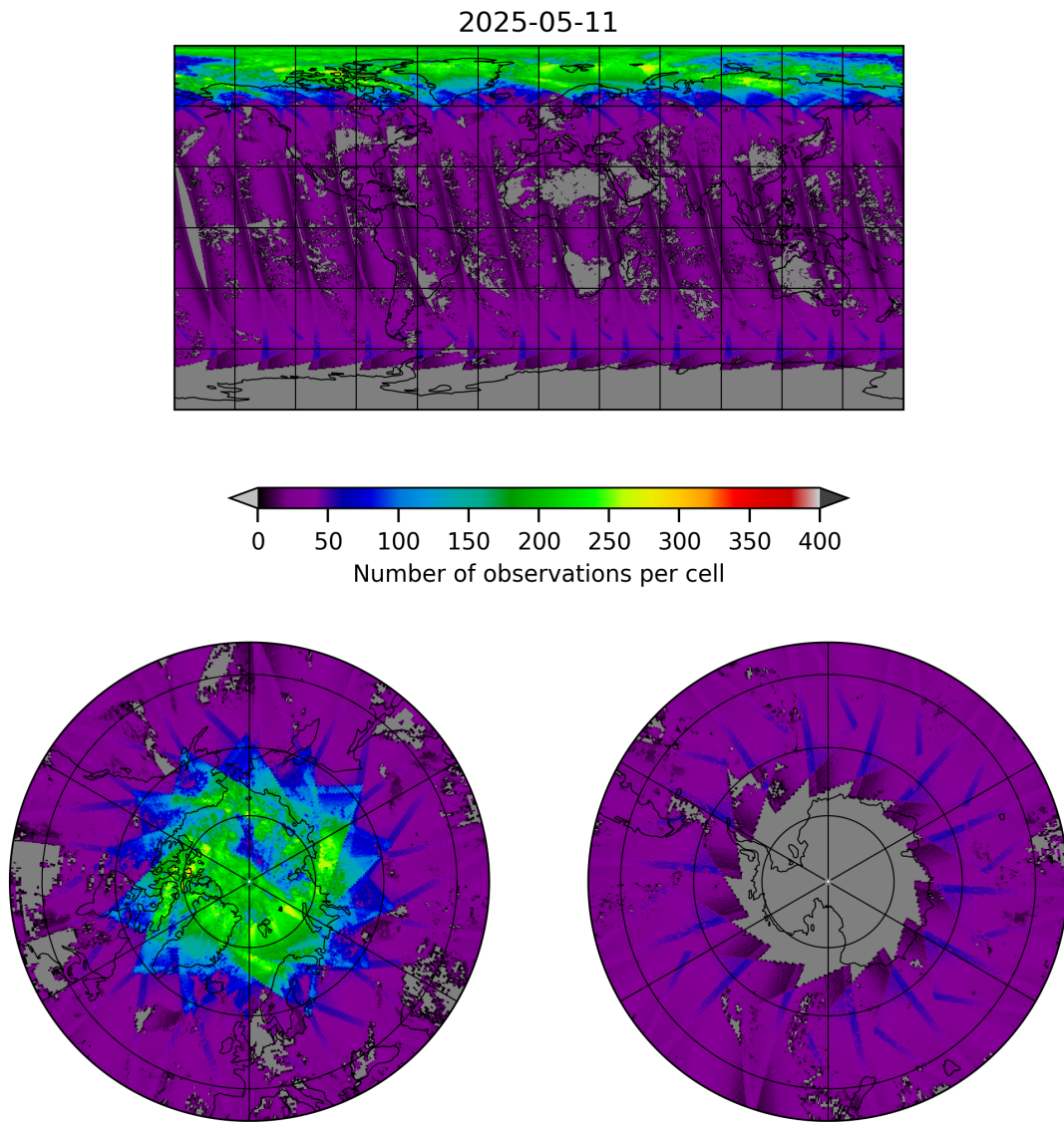
Figure 19: Map of the number of observations for 2025-05-11 to 2025-05-12
