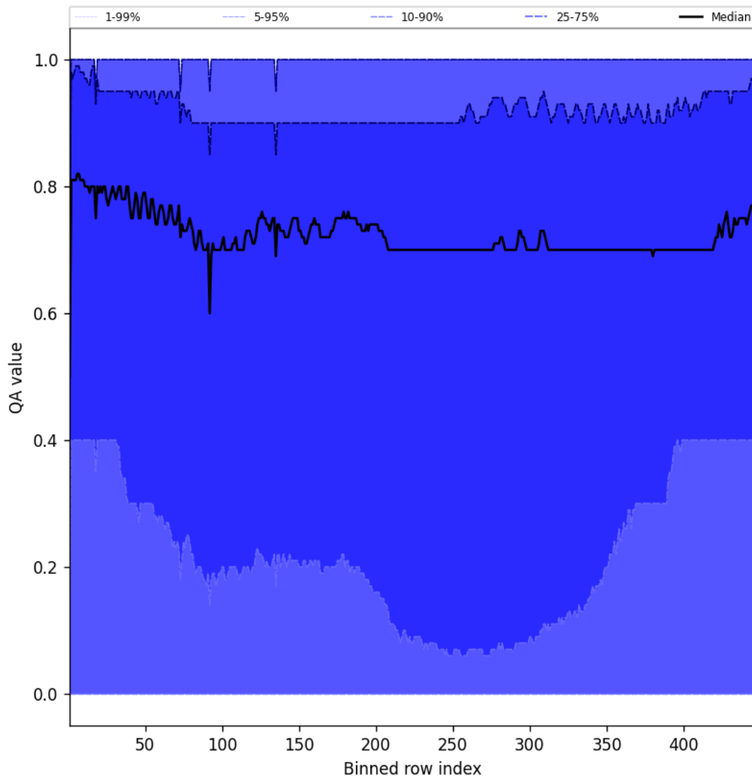
Figure 52: Along track statistics of “QA value” for 2025-05-11 to 2025-05-12
