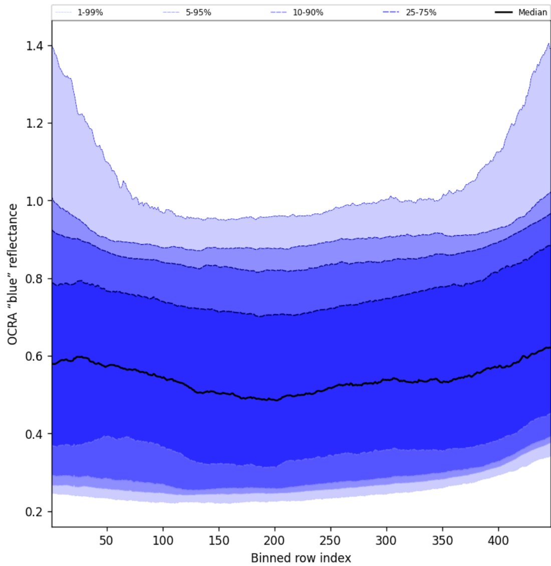
Figure 65: Along track statistics of "OCRA "blue" reflectance" for 2025-05-11 to 2025-05-12
