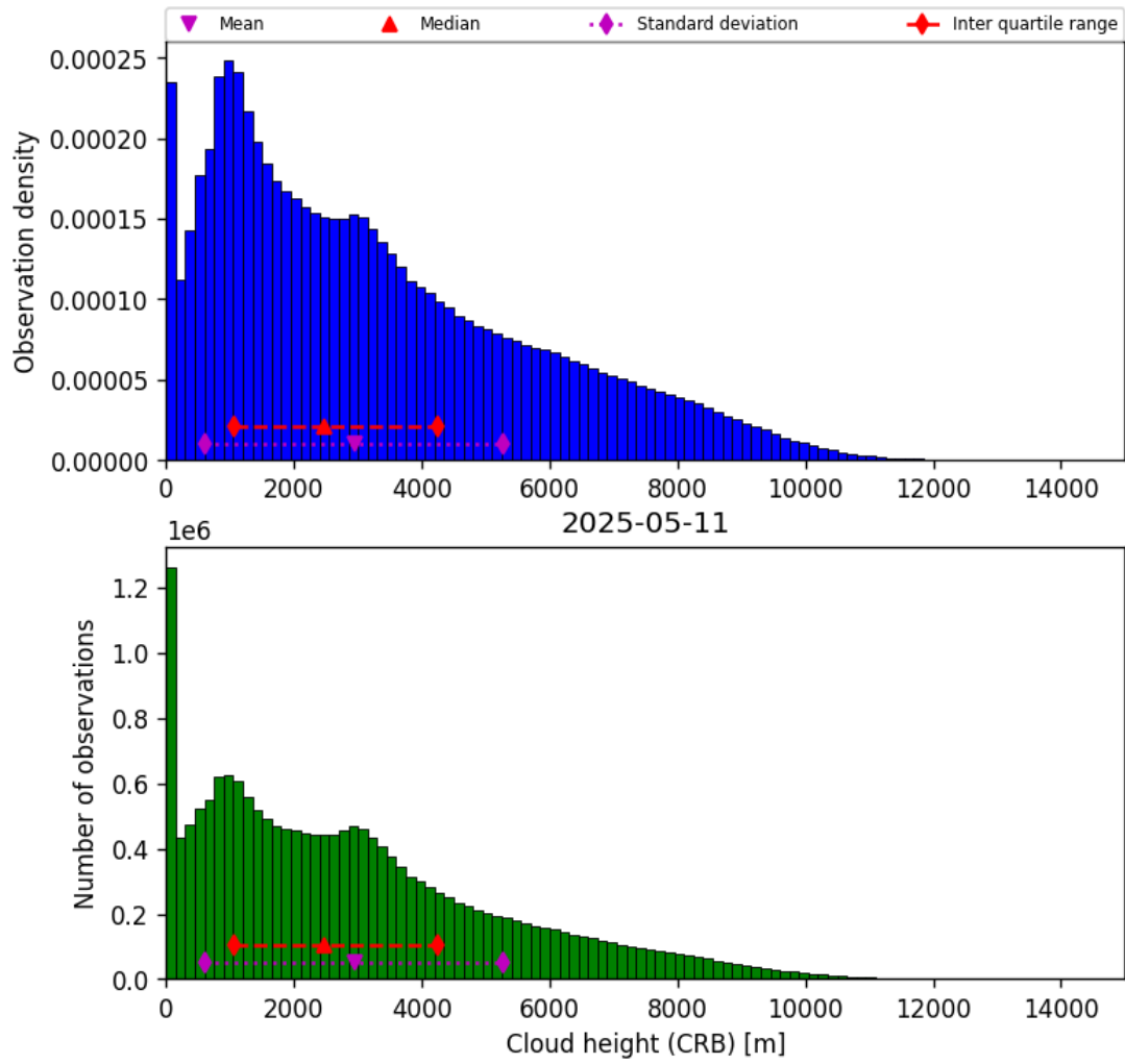
Figure 41: Histogram of “Cloud height (CRB)” for 2025-05-11 to 2025-05-12
