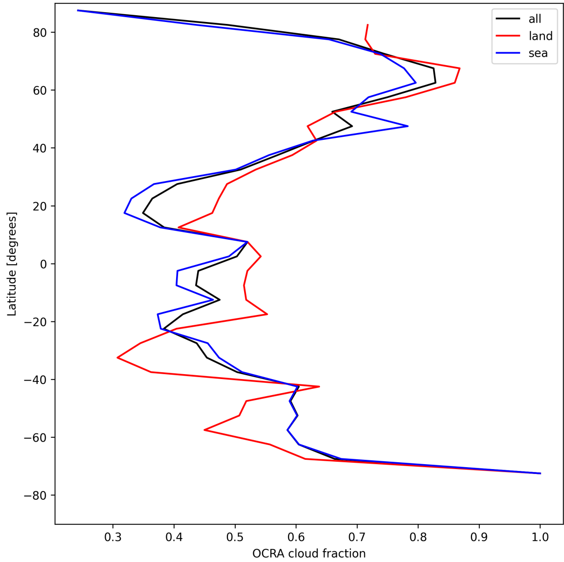
Figure 32: Zonal average of “OCRA cloud fraction” for 2025-05-13 to 2025-05-13.
