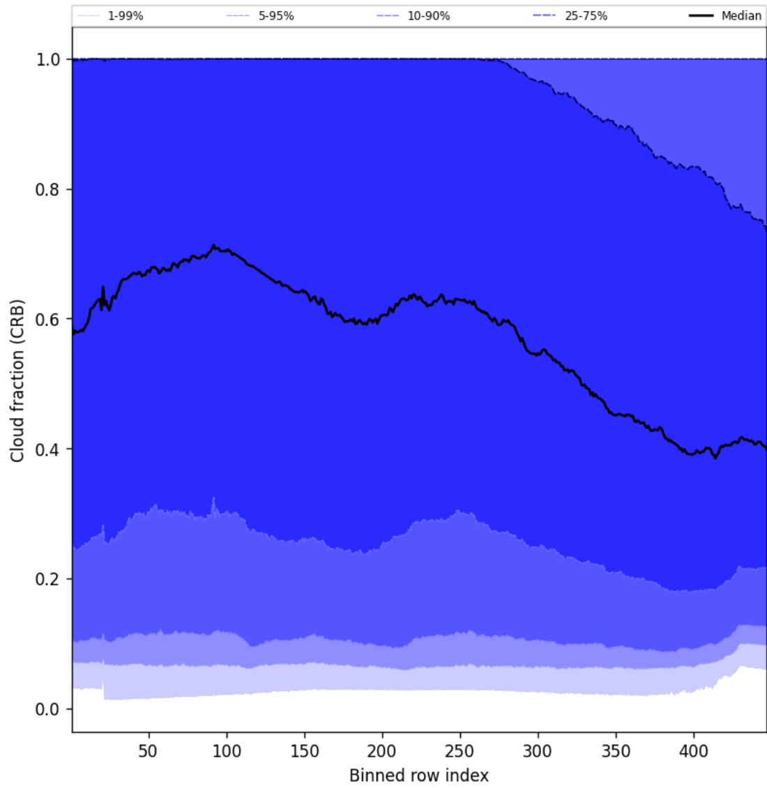
Figure 56: Along track statistics of “Cloud fraction (CRB)” for 2025-05-13 to 2025-05-13
