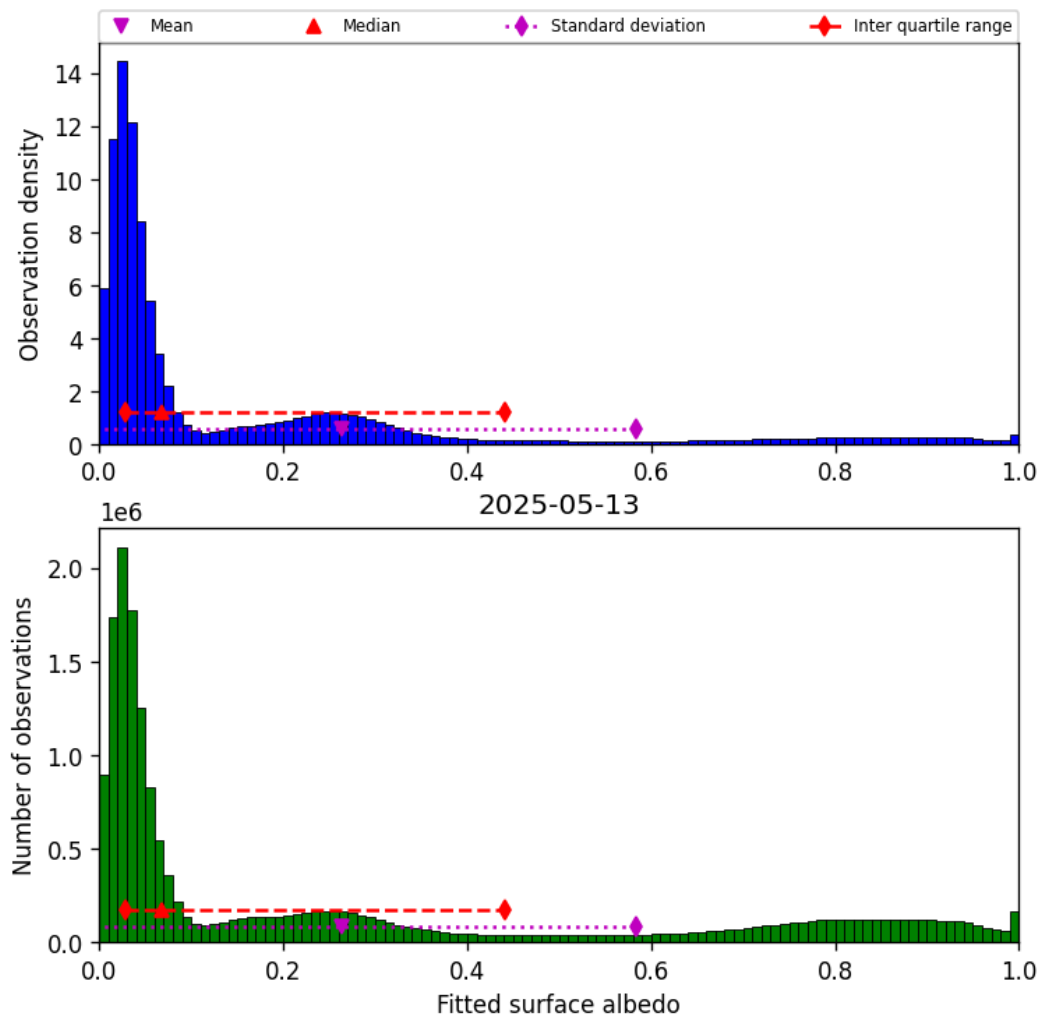
Figure 43: Histogram of “Fitted surface albedo” for 2025-05-13 to 2025-05-13
