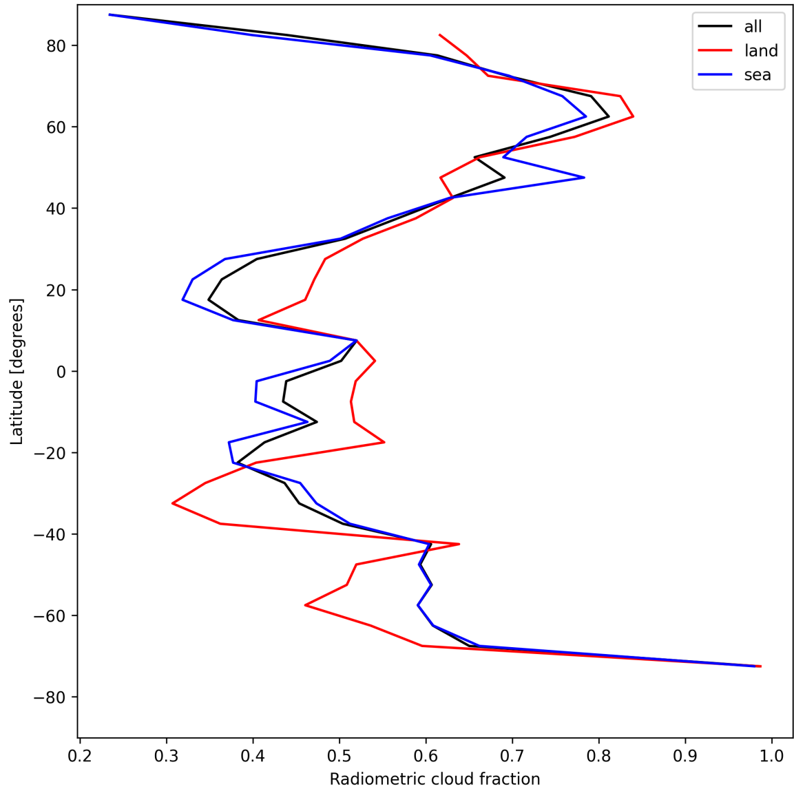
Figure 21: Zonal average of “Radiometric cloud fraction” for 2025-05-13 to 2025-05-13.
