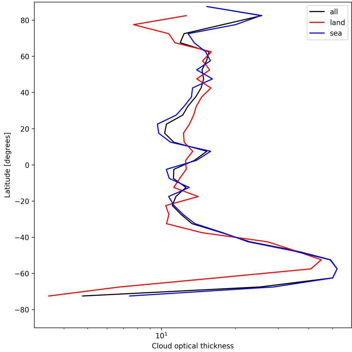
Figure 23: Zonal average of “Cloud optical thickness” for 2025-05-13 to 2025-05-13.
