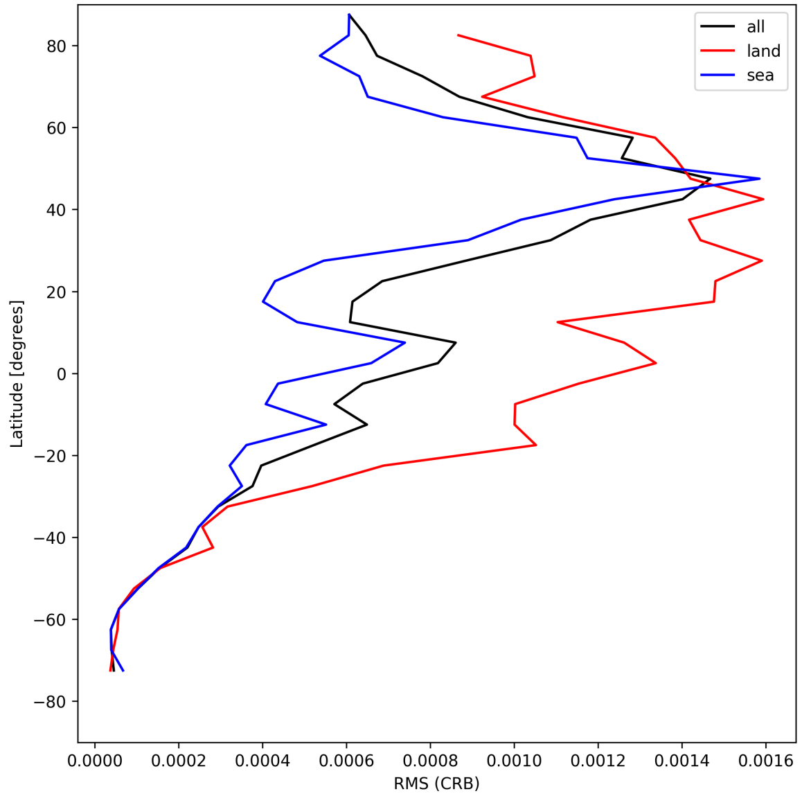
Figure 30: Zonal average of “RMS (CRB)” for 2025-05-13 to 2025-05-13.
