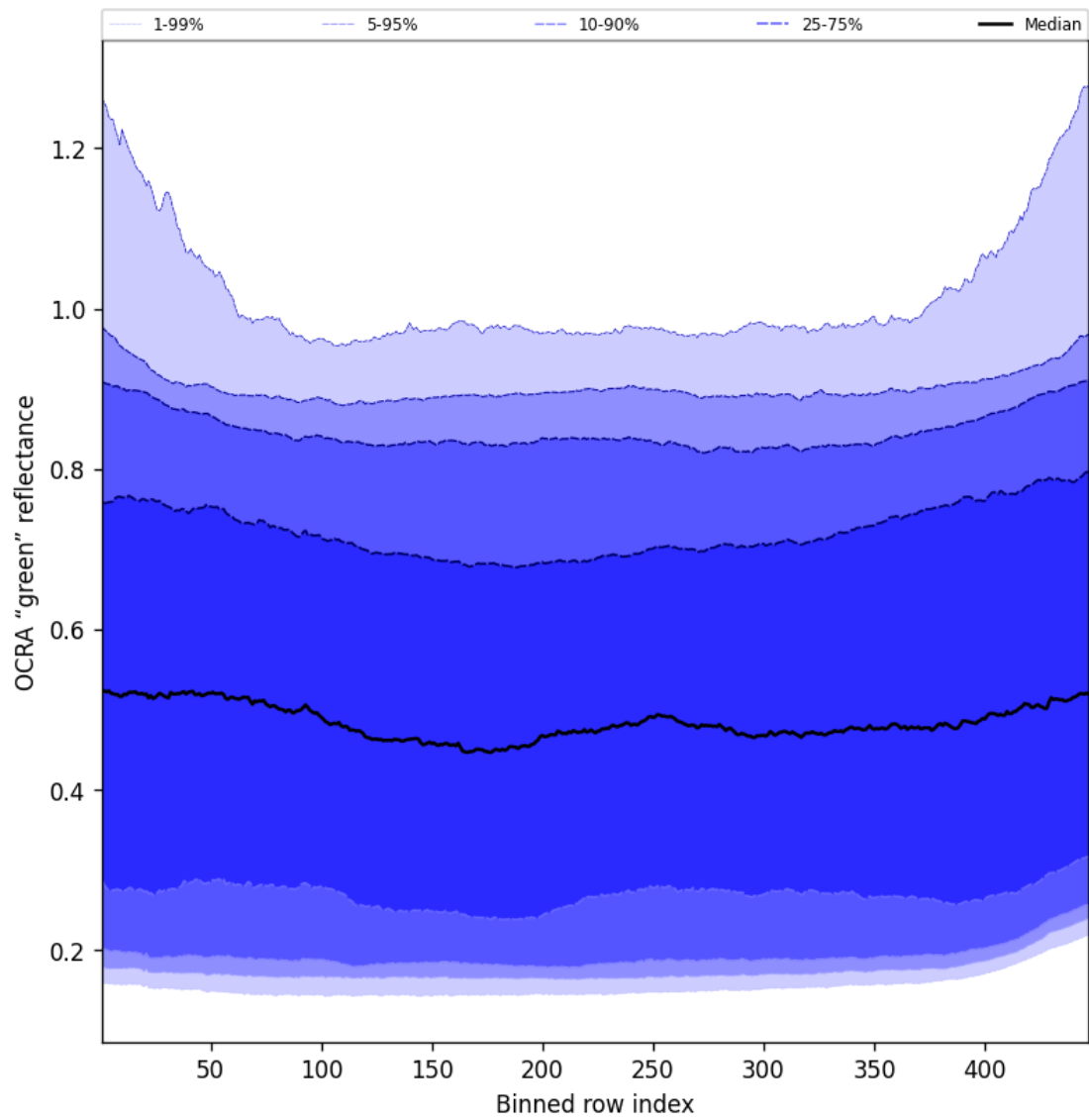
Figure 66: Along track statistics of “OCRA “green” reflectance” for 2025-05-13 to 2025-05-13
