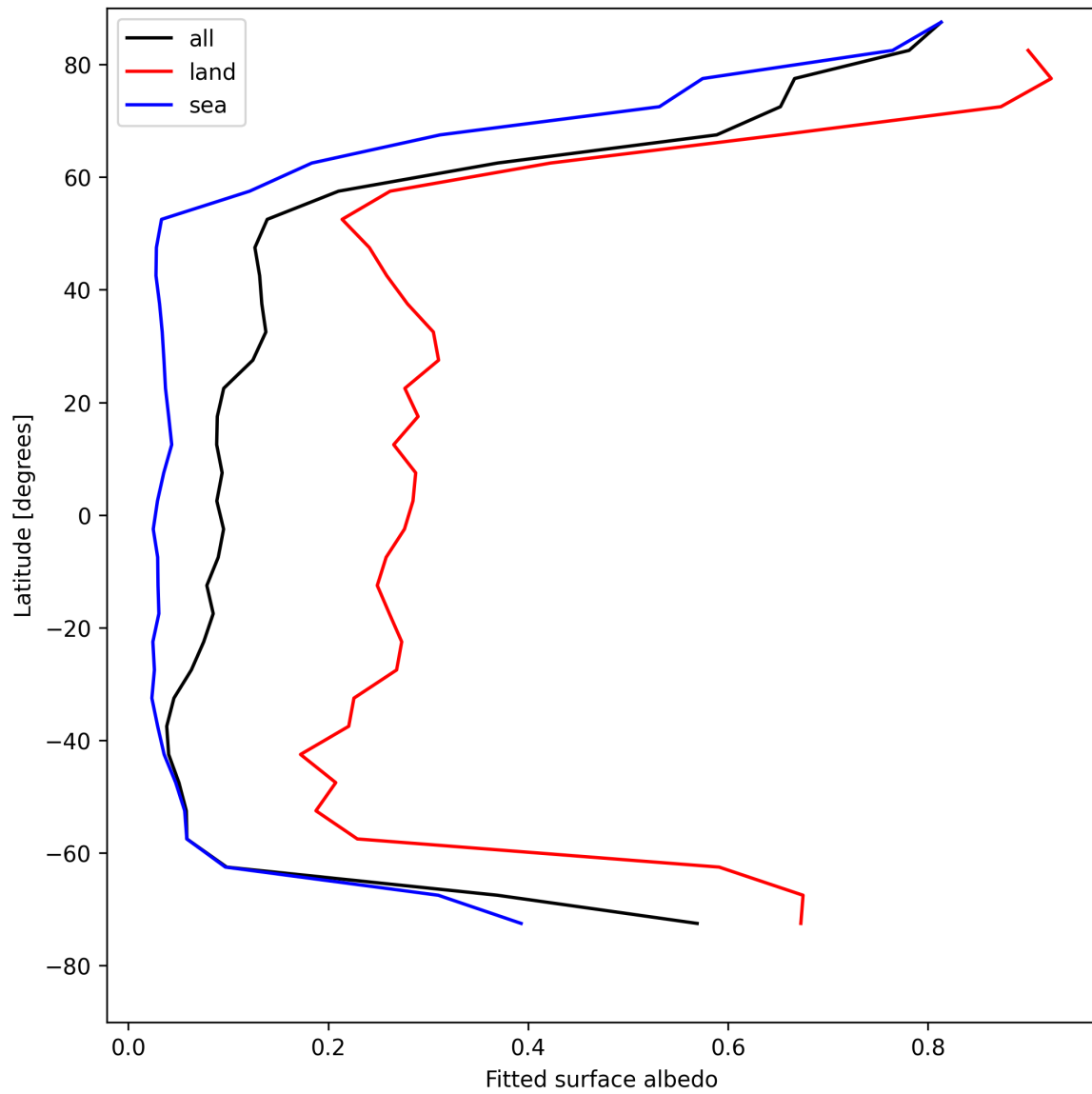
Figure 27: Zonal average of “Fitted surface albedo” for 2025-05-13 to 2025-05-13.
