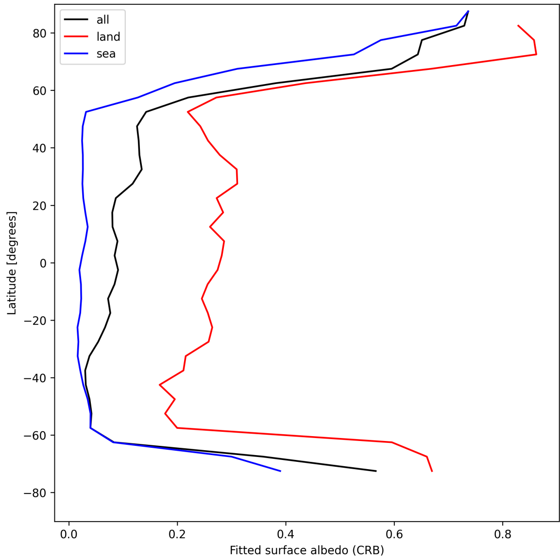
Figure 28: Zonal average of “Fitted surface albedo (CRB)” for 2025-05-13 to 2025-05-13.
