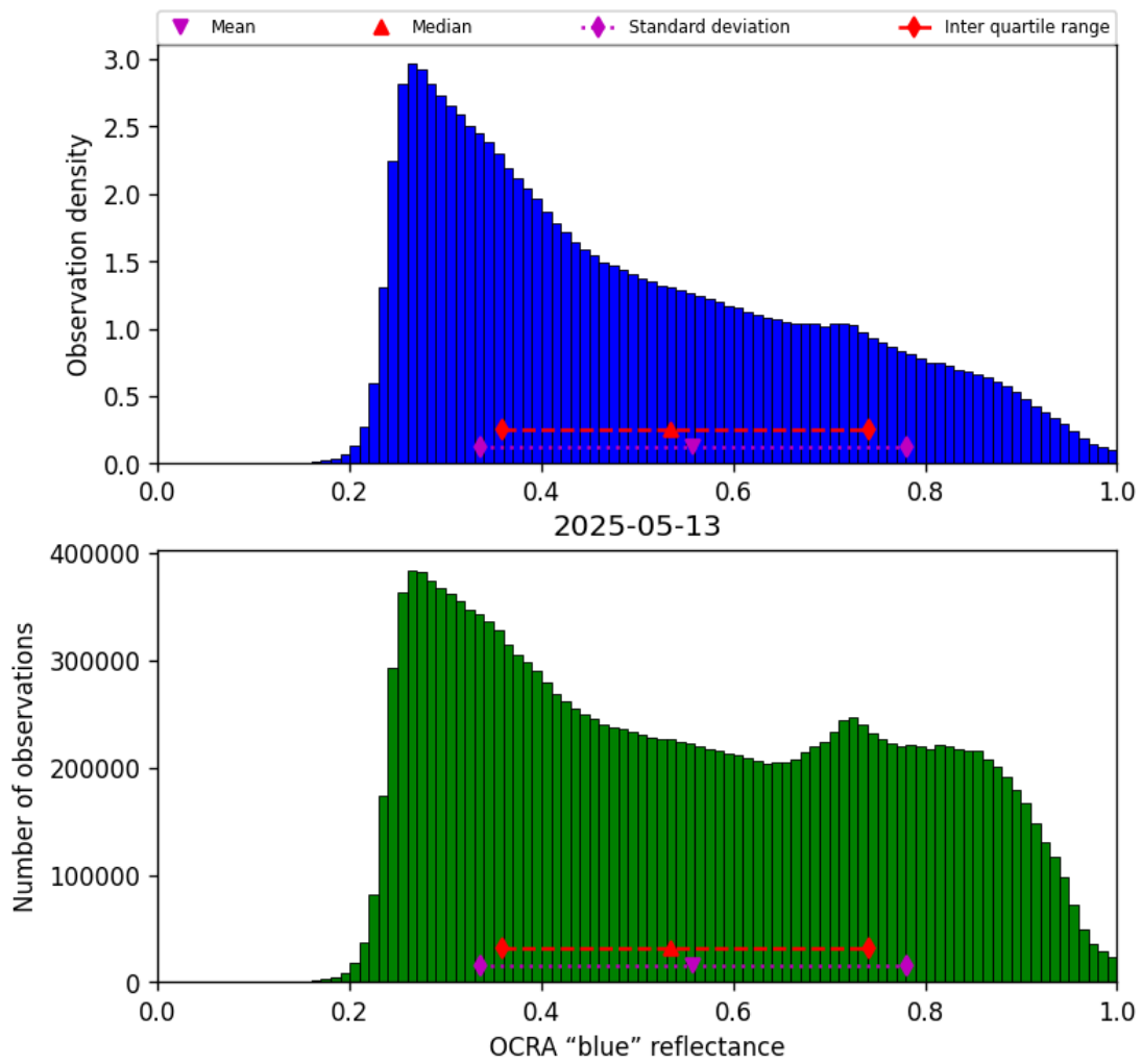
Figure 49: Histogram of “OCRA “blue” reflectance” for 2025-05-13 to 2025-05-13
