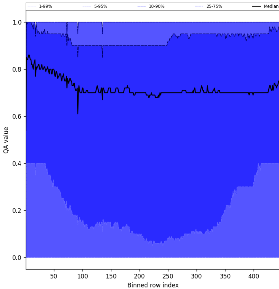
Figure 52: Along track statistics of “QA value” for 2025-05-13 to 2025-05-13
