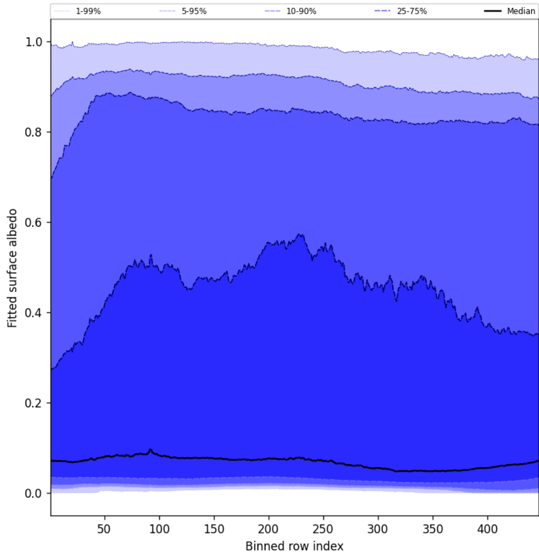
Figure 59: Along track statistics of “Fitted surface albedo” for 2025-05-13 to 2025-05-13
