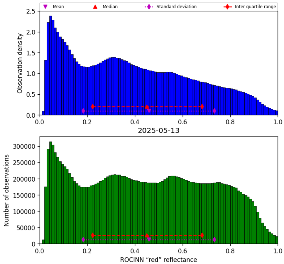
Figure 51: Histogram of “ROCINN “red” reflectance” for 2025-05-13 to 2025-05-13
