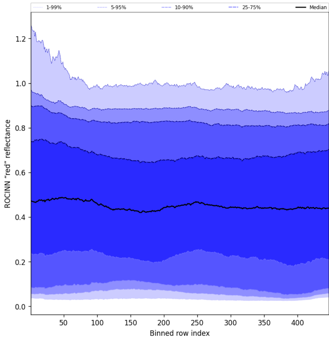
Figure 67: Along track statistics of "ROCINN "red" reflectance" for 2025-05-13 to 2025-05-13
