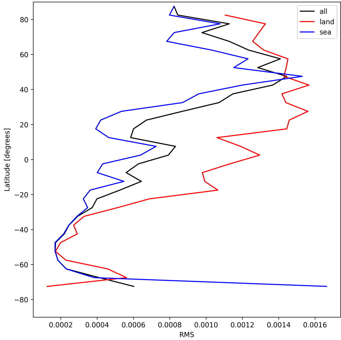
Figure 29: Zonal average of “RMS” for 2025-05-13 to 2025-05-13.
