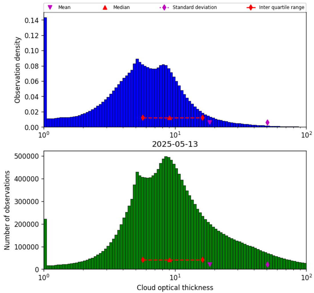
Figure 39: Histogram of “Cloud optical thickness” for 2025-05-13 to 2025-05-13
