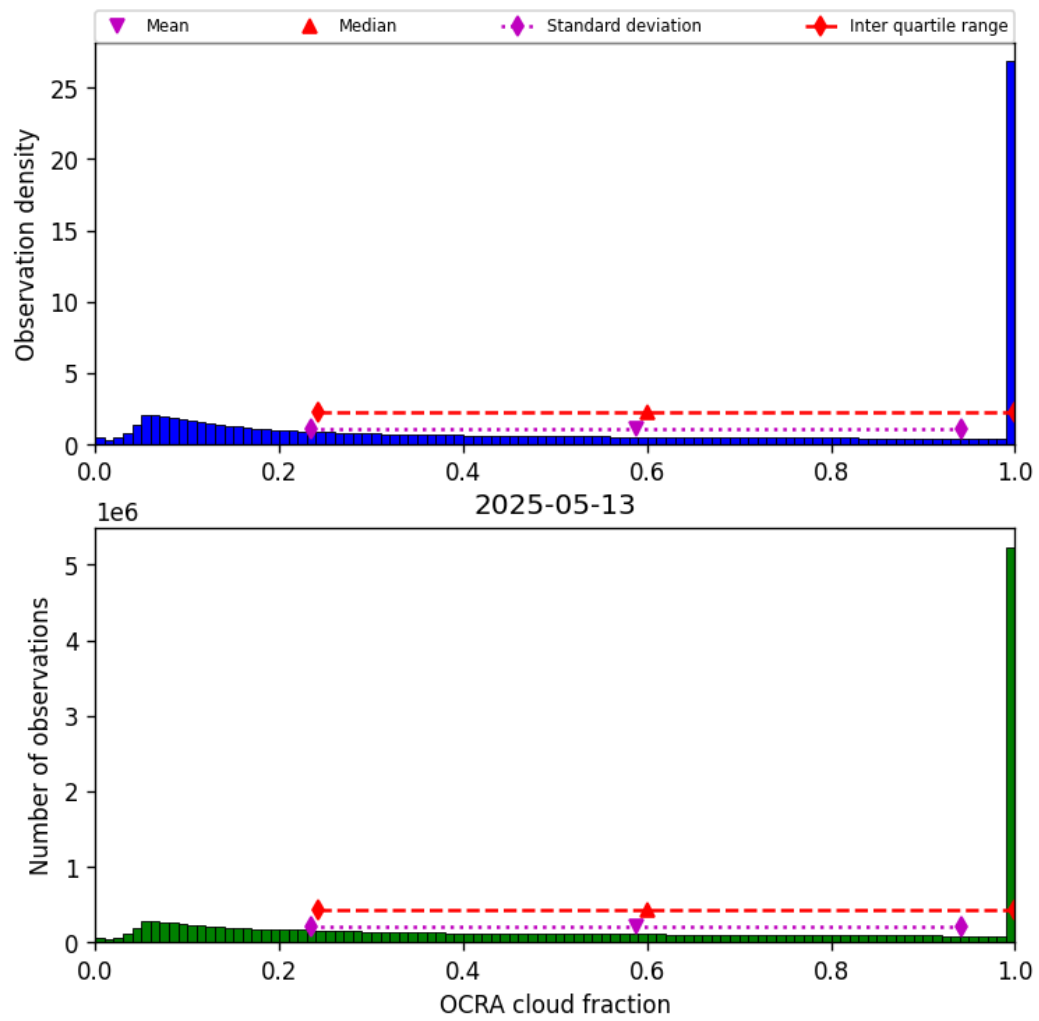
Figure 48: Histogram of “OCRA cloud fraction” for 2025-05-13 to 2025-05-13
