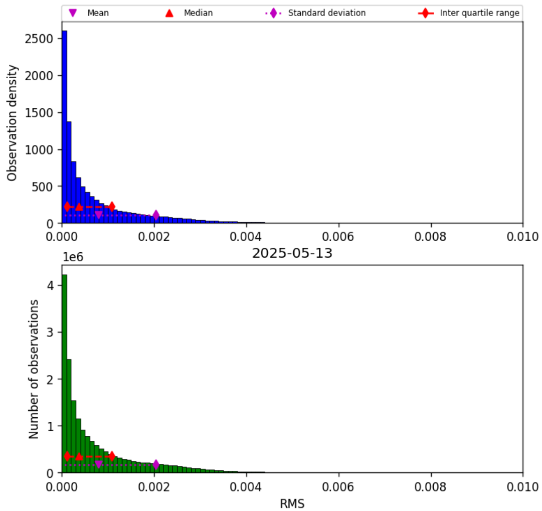
Figure 45: Histogram of “RMS” for 2025-05-13 to 2025-05-13
