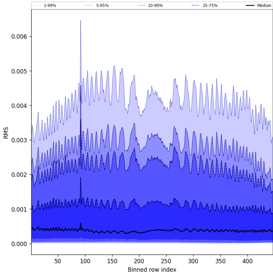
Figure 61: Along track statistics of “RMS” for 2025-05-13 to 2025-05-13
