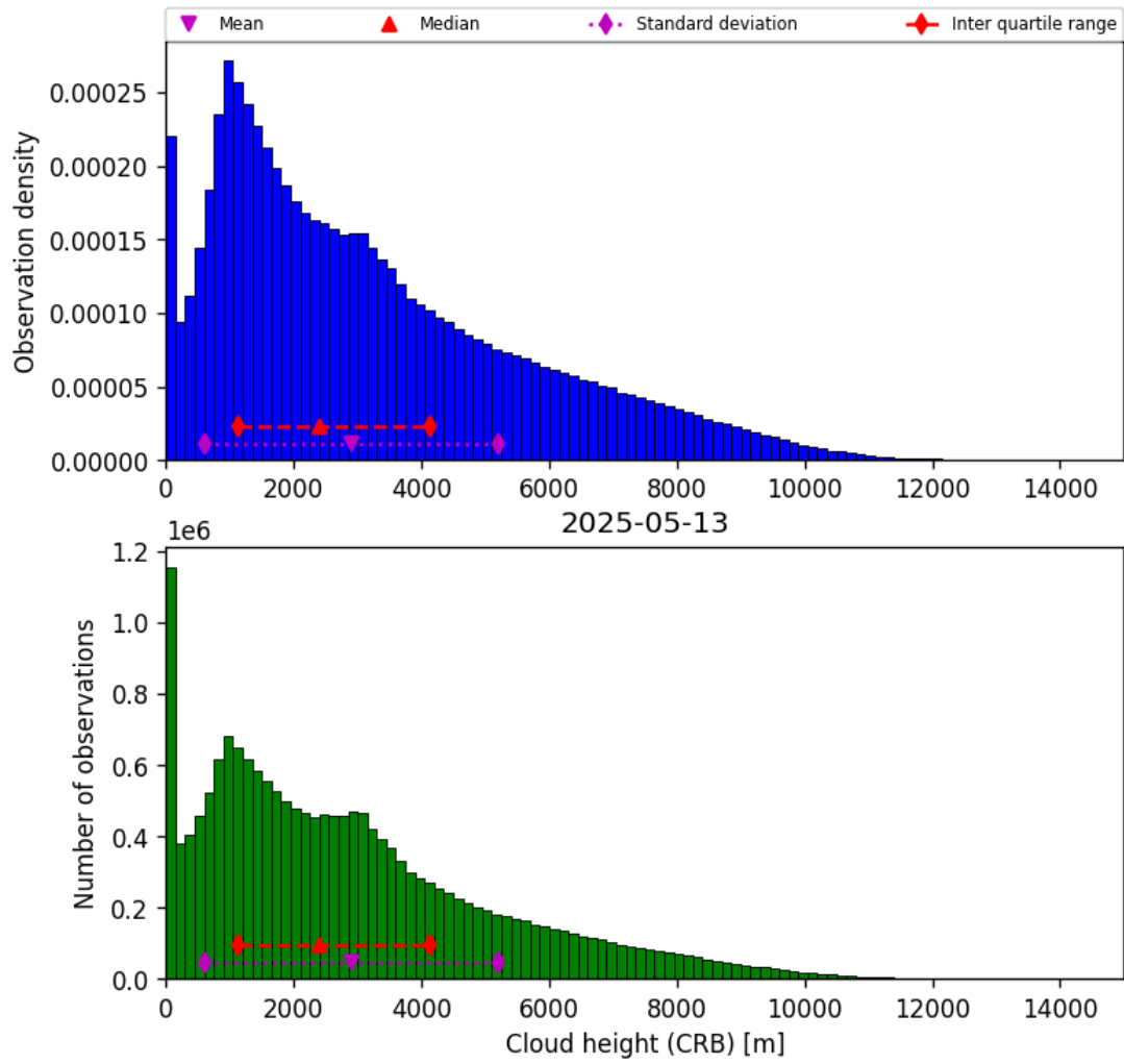
Figure 41: Histogram of “Cloud height (CRB)” for 2025-05-13 to 2025-05-13
