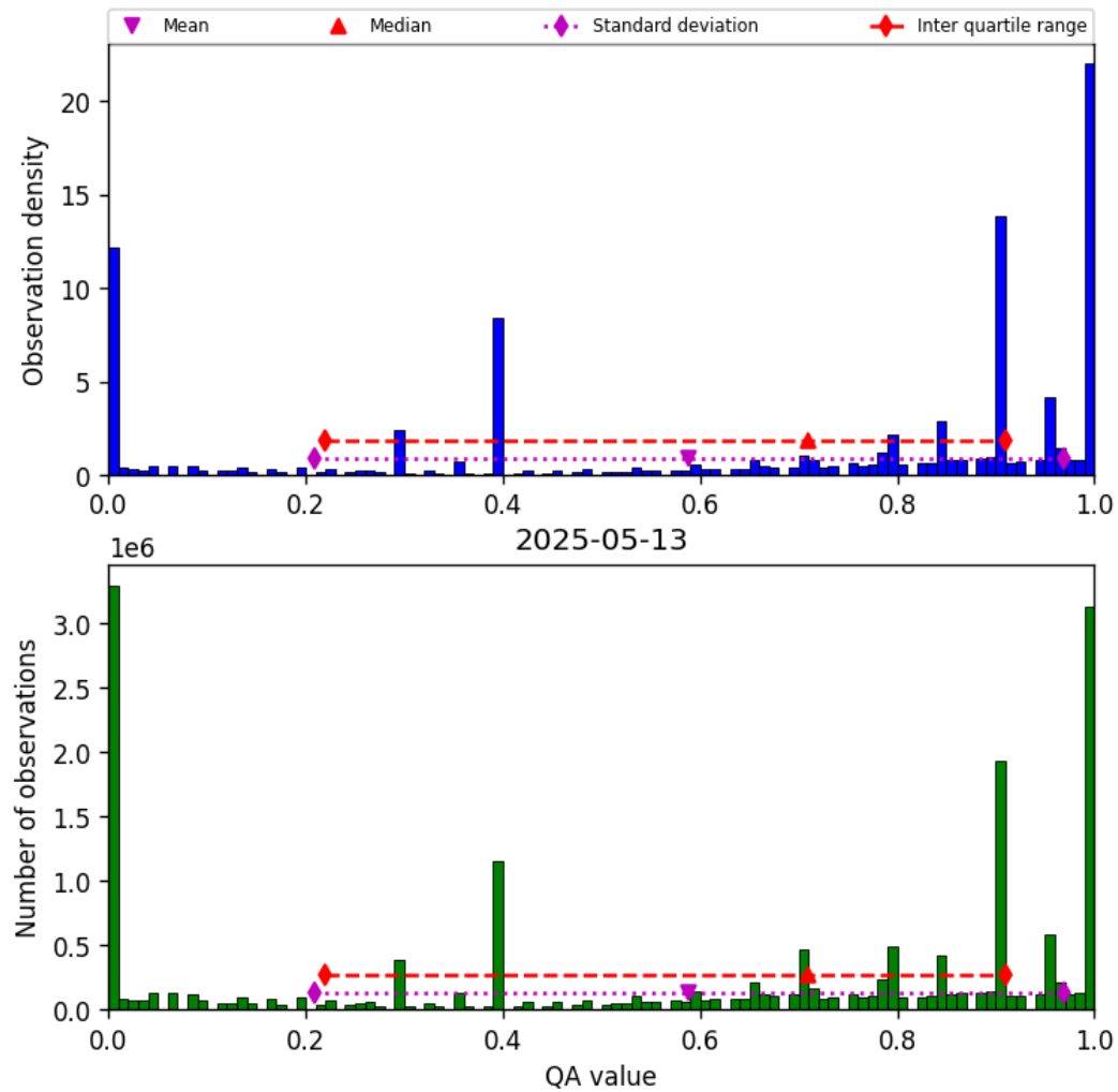
Figure 36: Histogram of “QA value” for 2025-05-13 to 2025-05-13
