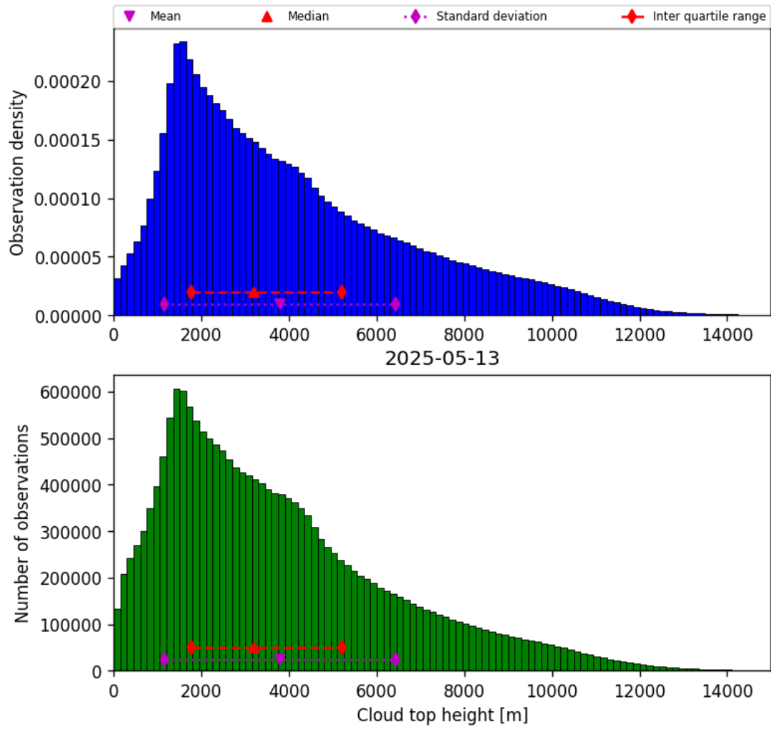
Figure 38: Histogram of “Cloud top height” for 2025-05-13 to 2025-05-13
