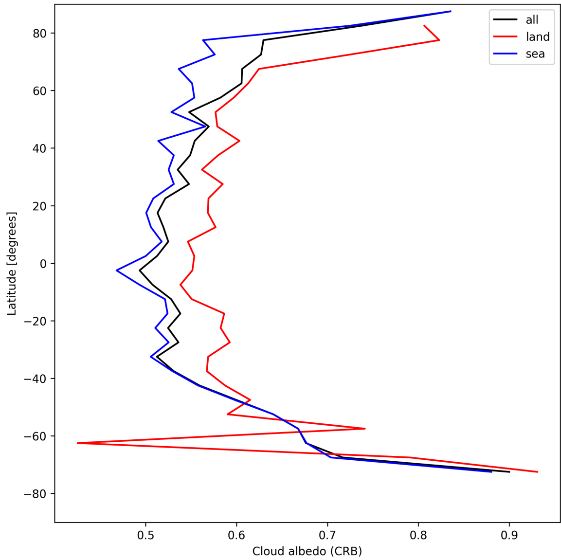
Figure 26: Zonal average of “Cloud albedo (CRB)” for 2025-05-13 to 2025-05-13.
