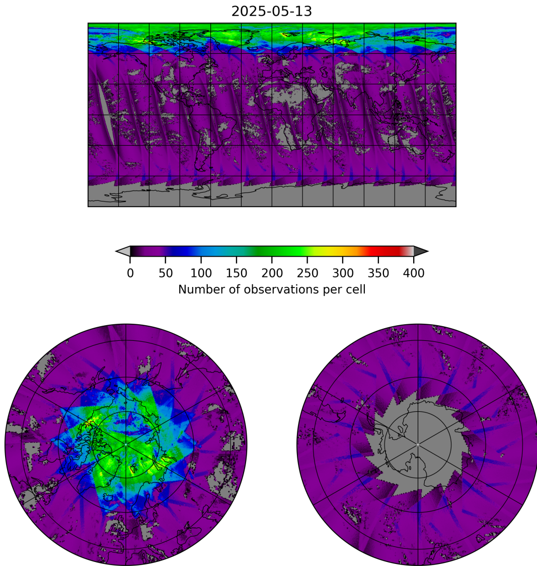
Figure 19: Map of the number of observations for 2025-05-13 to 2025-05-13
