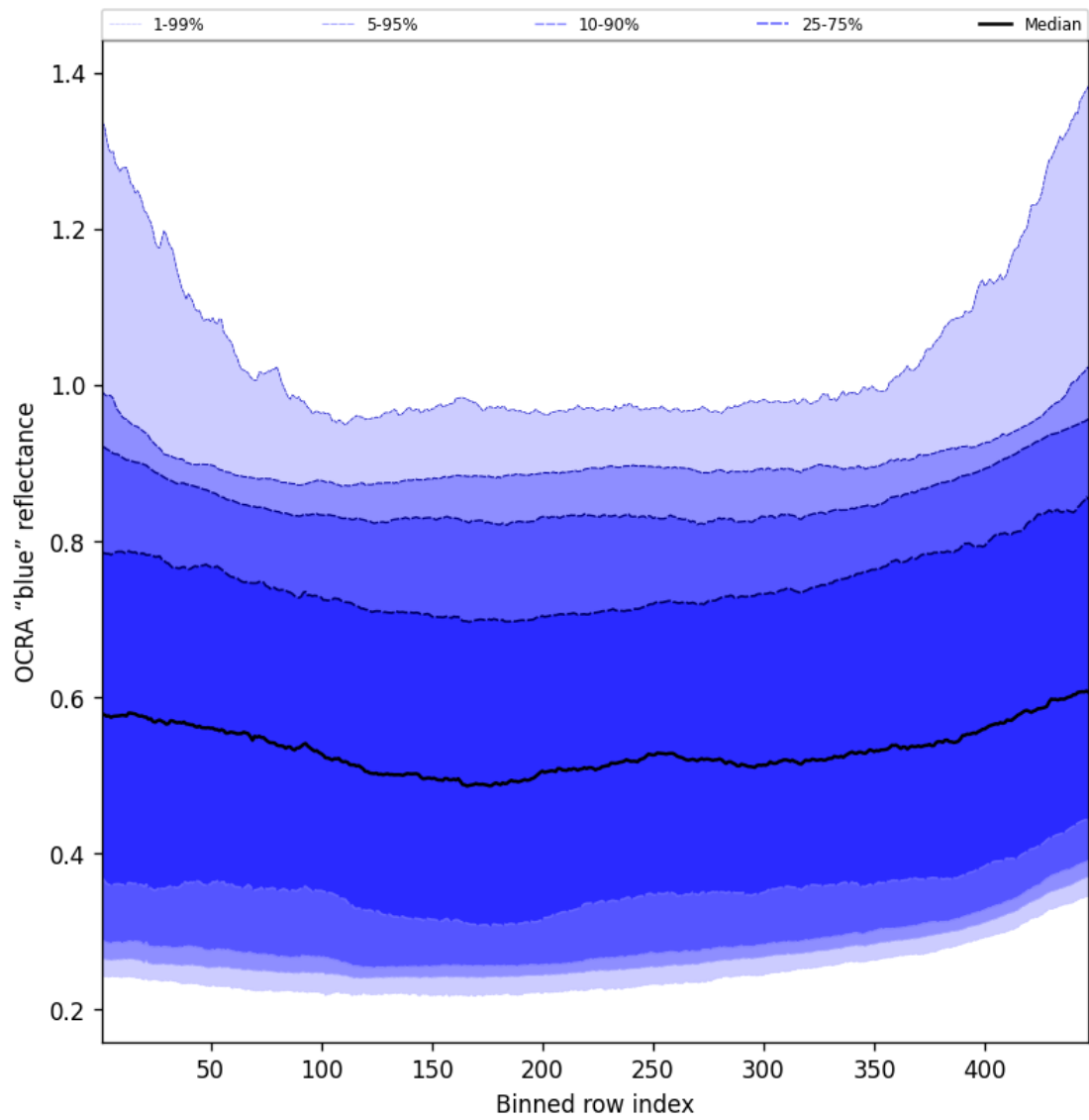
Figure 65: Along track statistics of “OCRA “blue” reflectance” for 2025-05-13 to 2025-05-13
