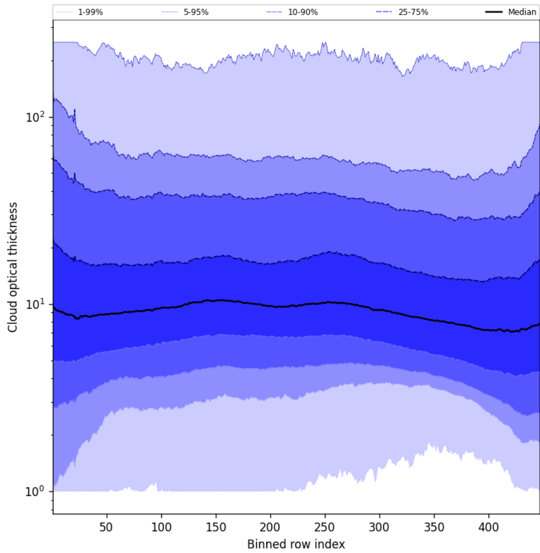
Figure 55: Along track statistics of “Cloud optical thickness” for 2025-05-13 to 2025-05-13
