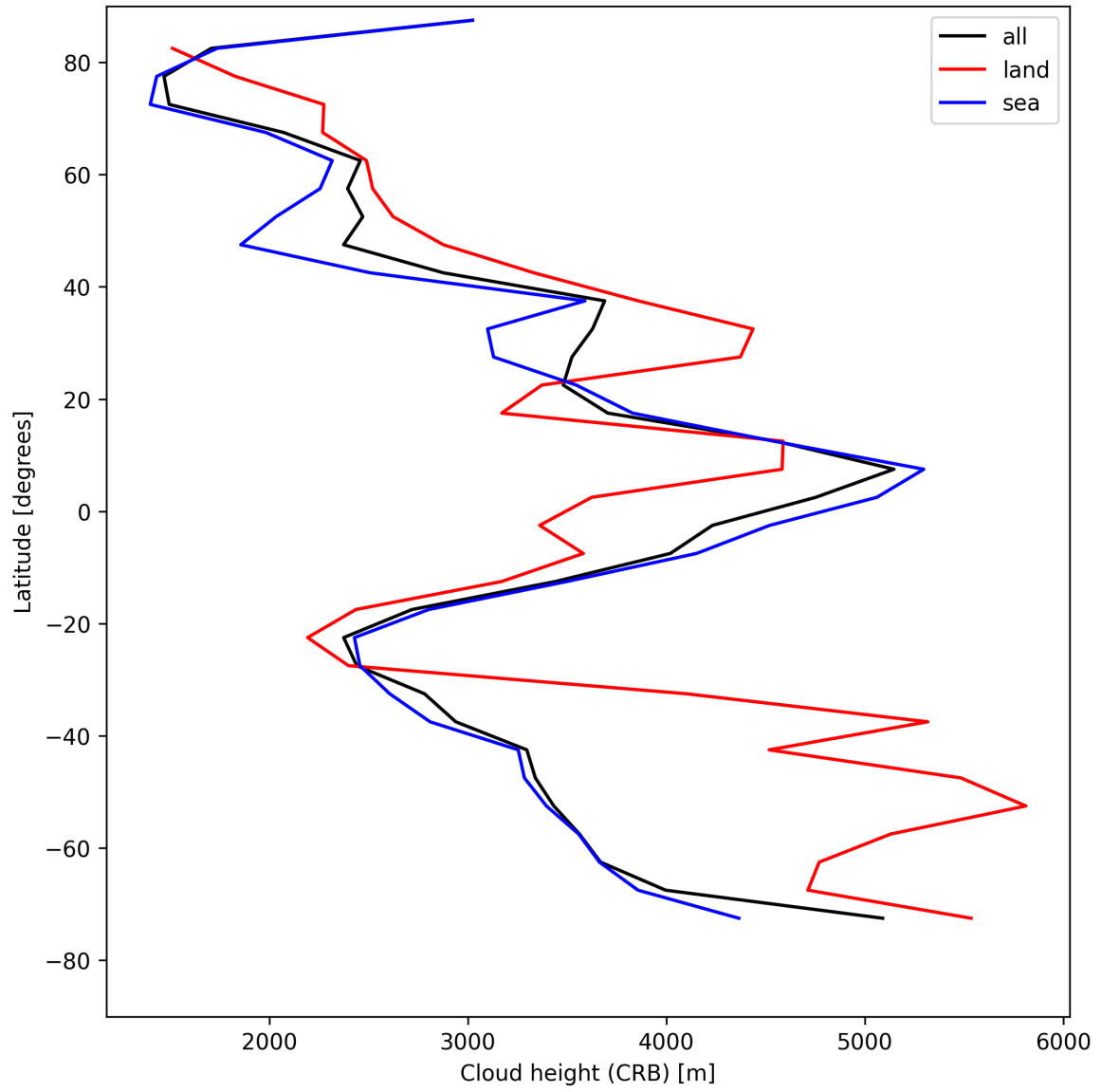
Figure 25: Zonal average of “Cloud height (CRB)” for 2025-05-13 to 2025-05-13.
