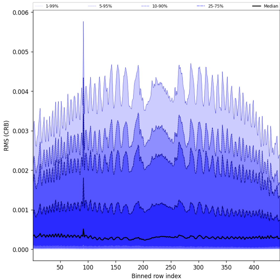
Figure 62: Along track statistics of “RMS (CRB)” for 2025-05-13 to 2025-05-13
