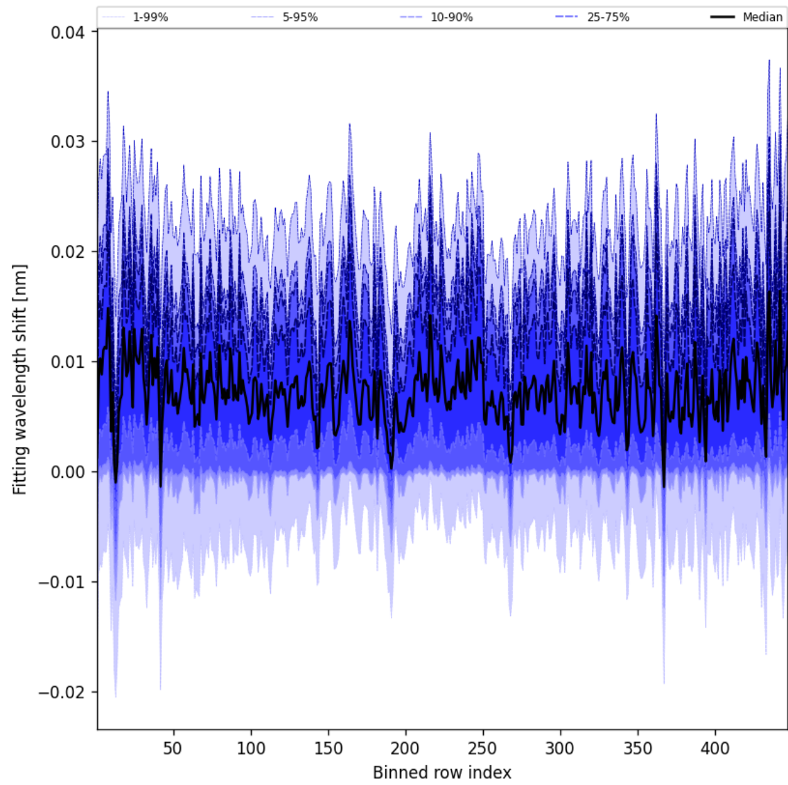
Figure 63: Along track statistics of “Fitting wavelength shift” for 2025-05-13 to 2025-05-13
