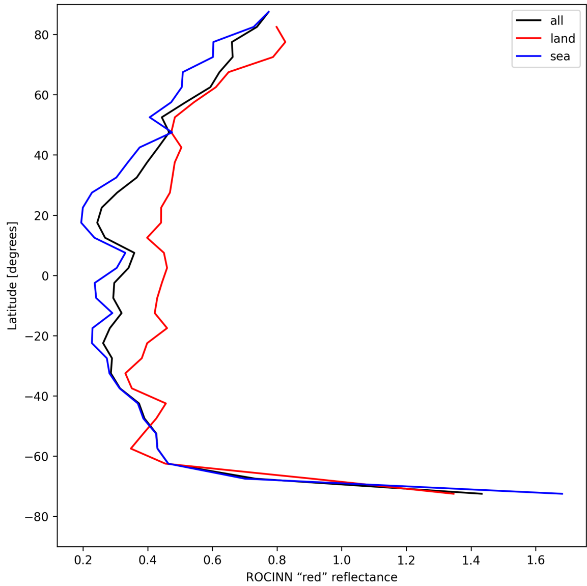
Figure 35: Zonal average of “ROCINN “red” reflectance” for 2025-05-13 to 2025-05-13.
