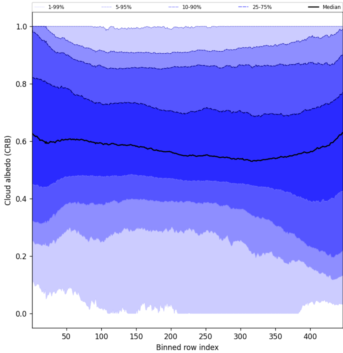
Figure 58: Along track statistics of “Cloud albedo (CRB)” for 2025-05-13 to 2025-05-13
