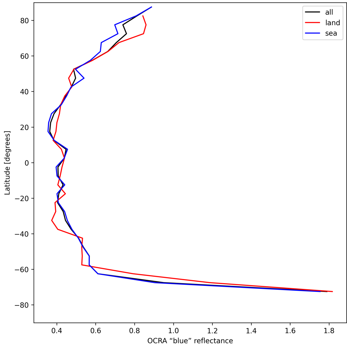
Figure 33: Zonal average of “OCRA “blue” reflectance” for 2025-05-13 to 2025-05-13.
