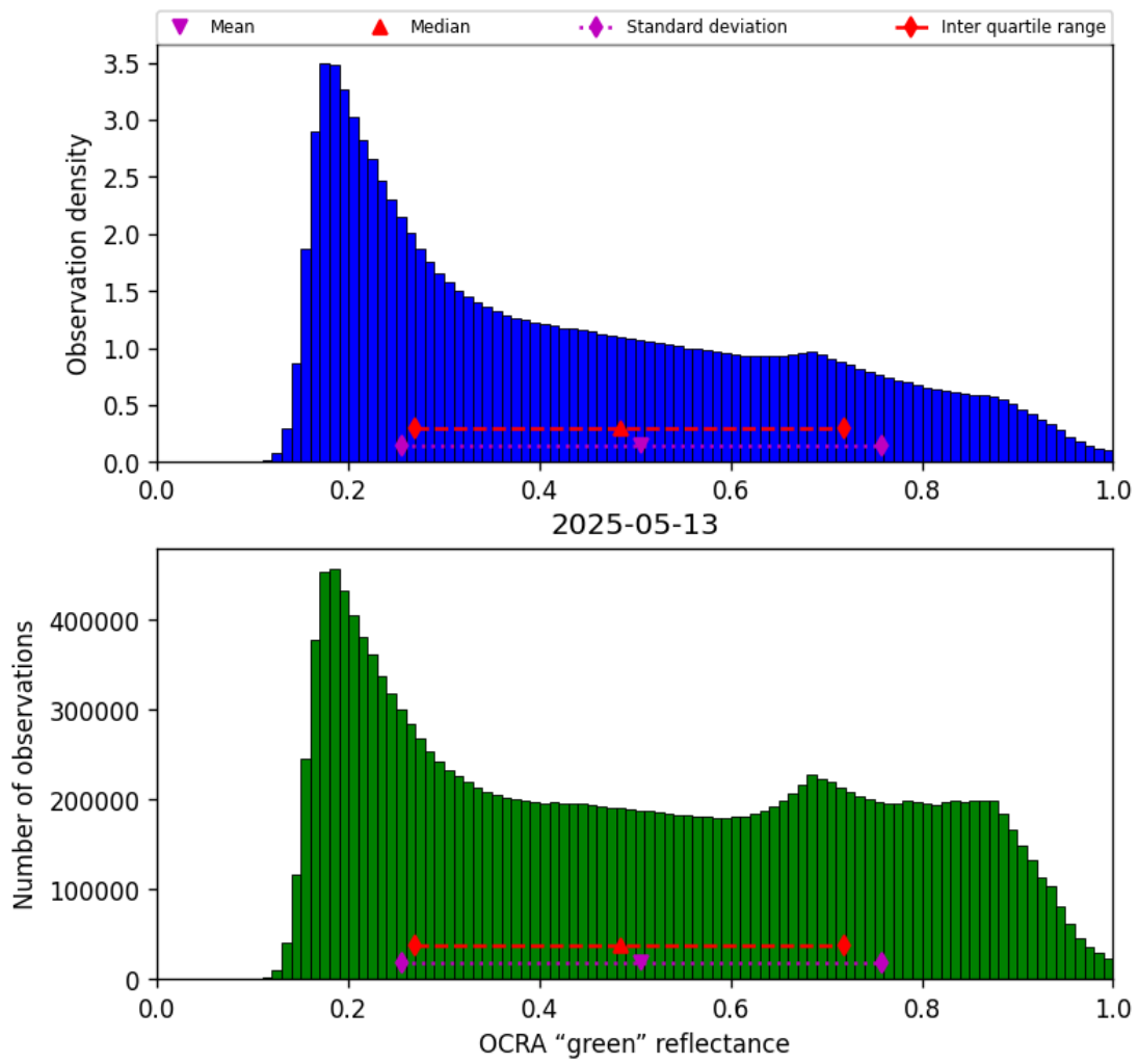
Figure 50: Histogram of “OCRA “green” reflectance” for 2025-05-13 to 2025-05-13
