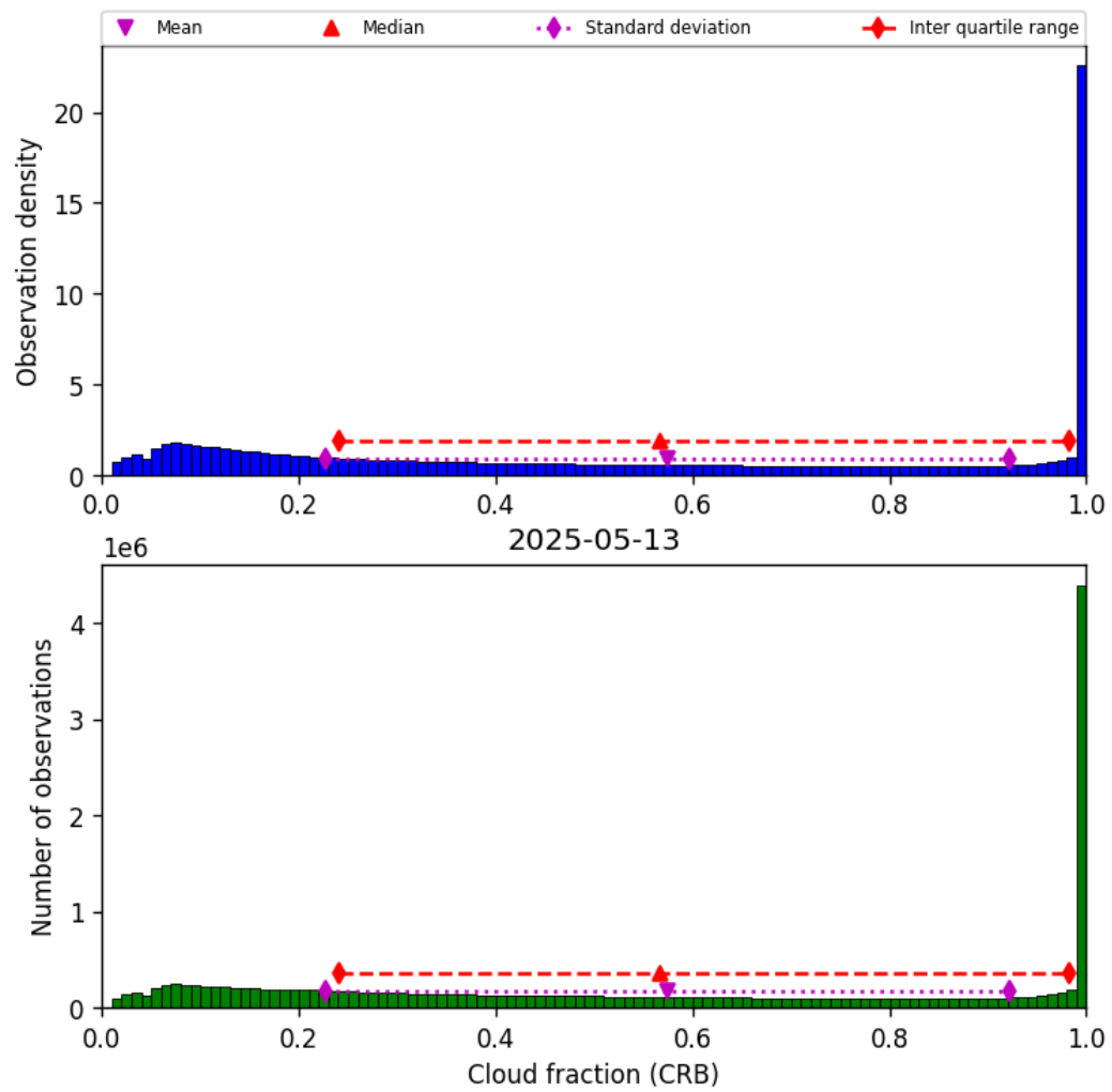
Figure 40: Histogram of “Cloud fraction (CRB)” for 2025-05-13 to 2025-05-13
