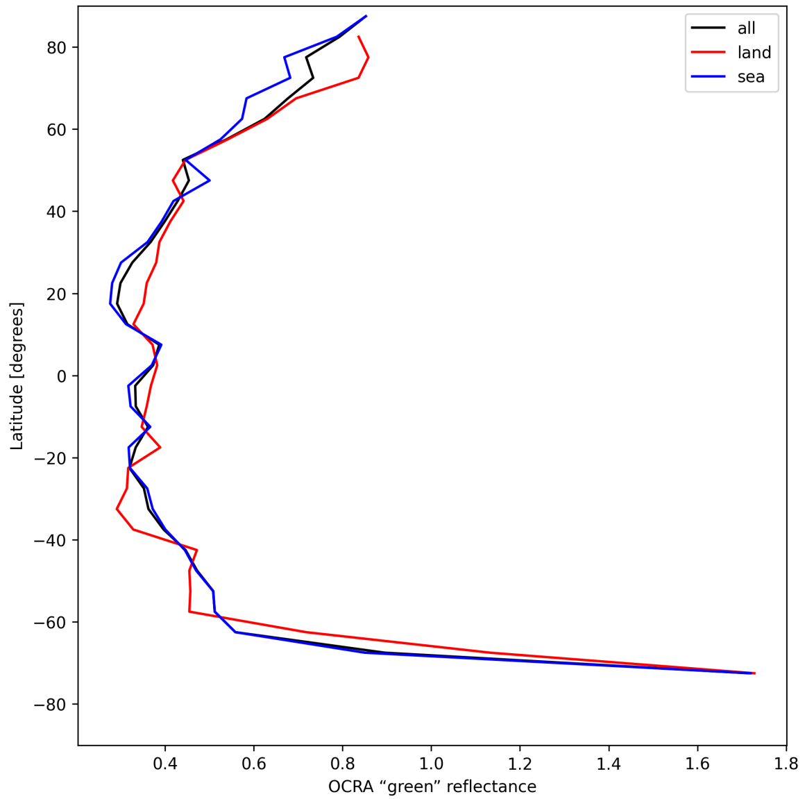
Figure 34: Zonal average of “OCRA “green” reflectance” for 2025-05-13 to 2025-05-13.
