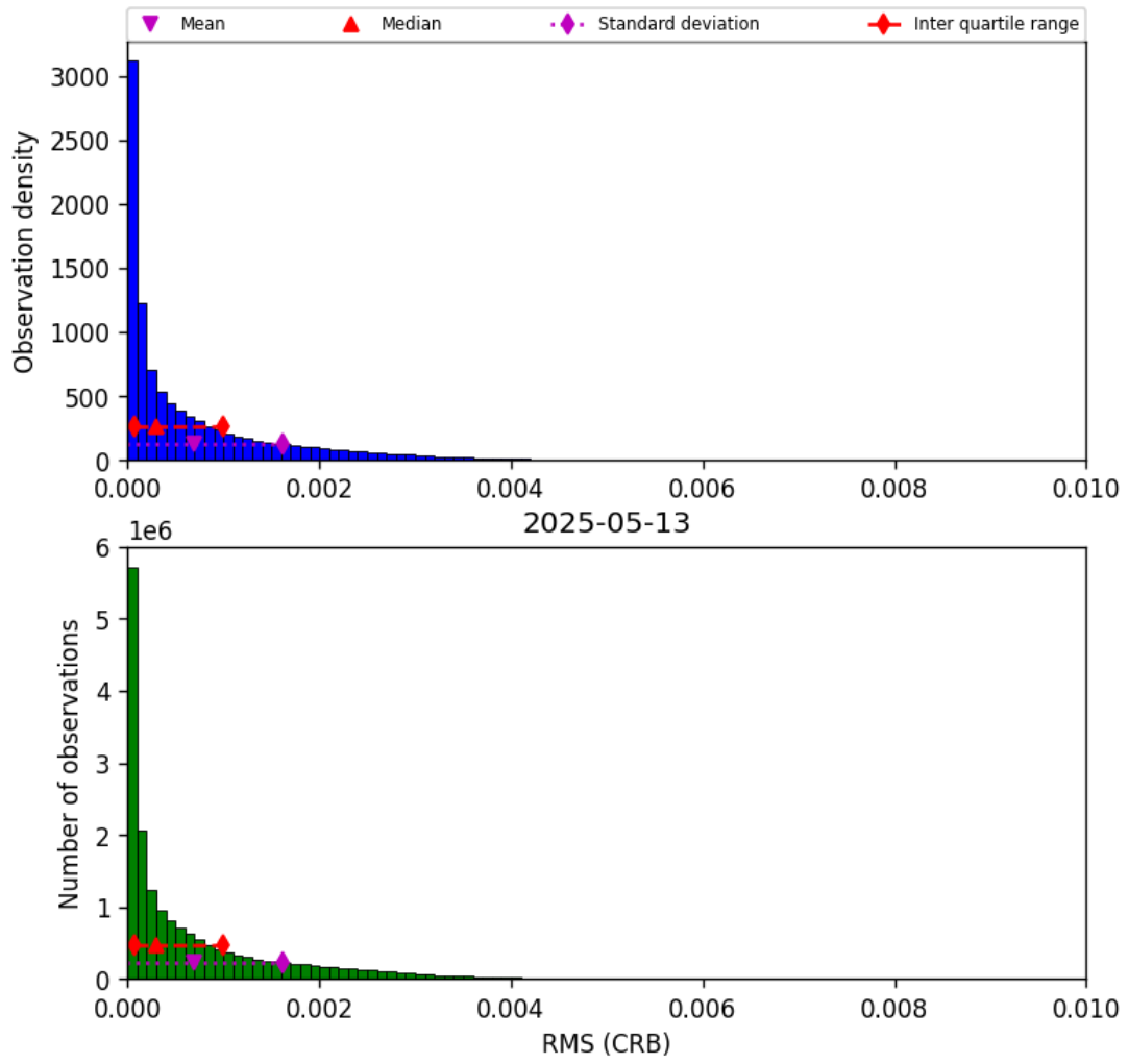
Figure 46: Histogram of “RMS (CRB)” for 2025-05-13 to 2025-05-13
