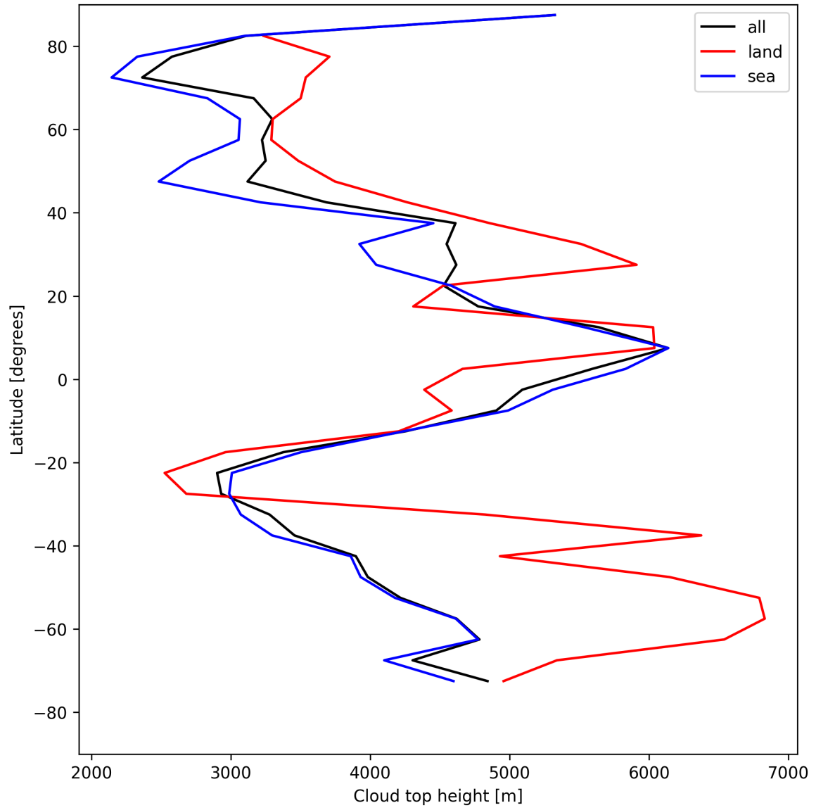
Figure 22: Zonal average of “Cloud top height” for 2025-05-13 to 2025-05-13.
