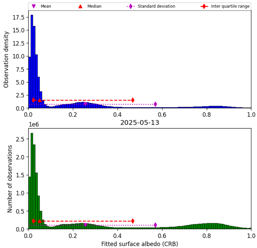
Figure 44: Histogram of “Fitted surface albedo (CRB)” for 2025-05-13 to 2025-05-13
