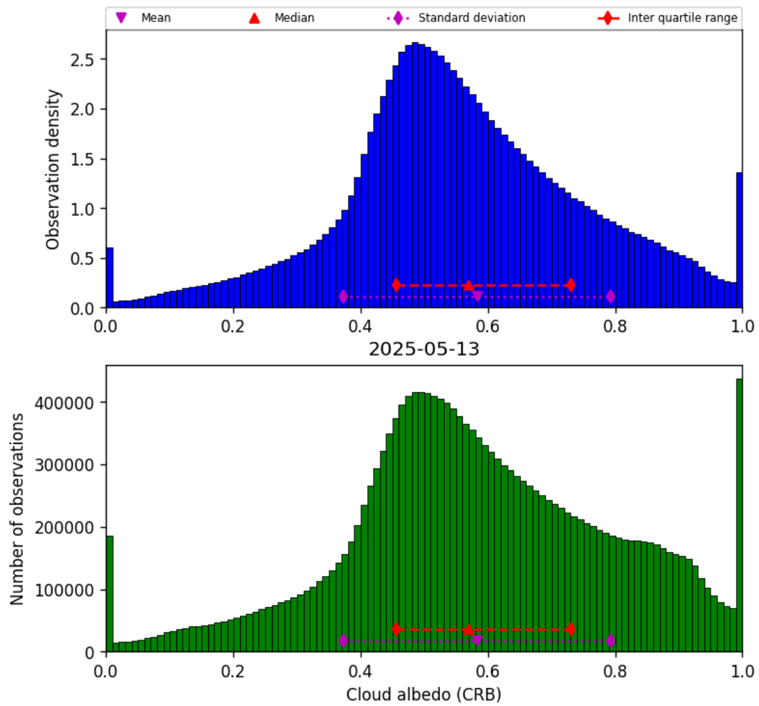
Figure 42: Histogram of “Cloud albedo (CRB)” for 2025-05-13 to 2025-05-13
