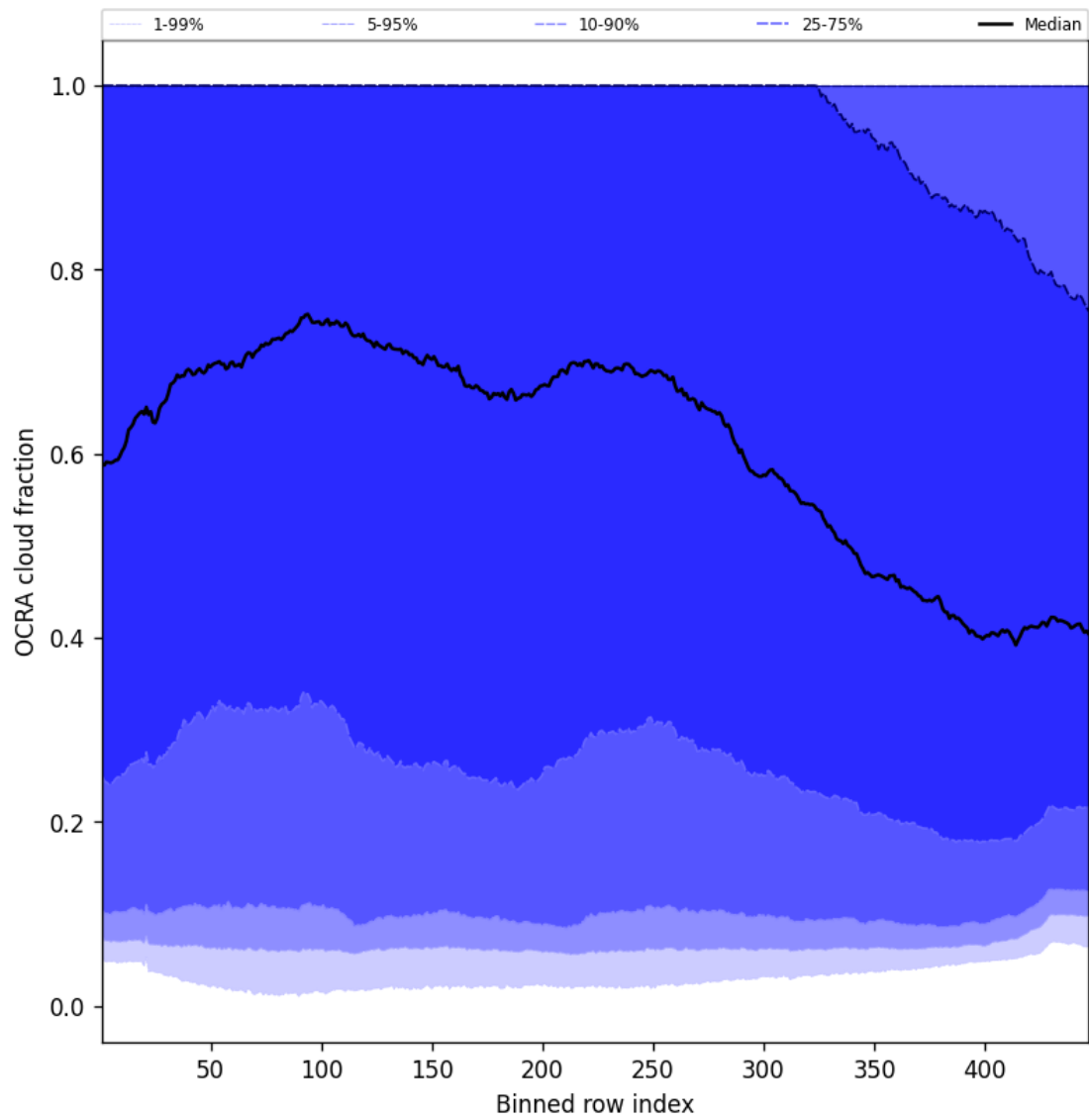
Figure 64: Along track statistics of “OCRA cloud fraction” for 2025-05-13 to 2025-05-13
