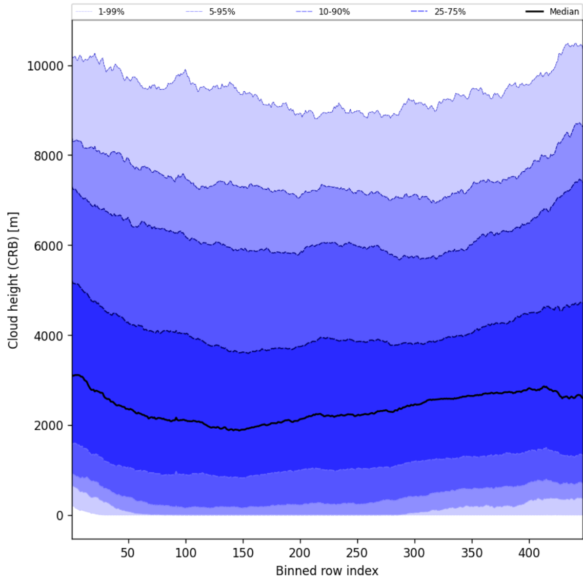
Figure 57: Along track statistics of “Cloud height (CRB)” for 2025-05-13 to 2025-05-13
