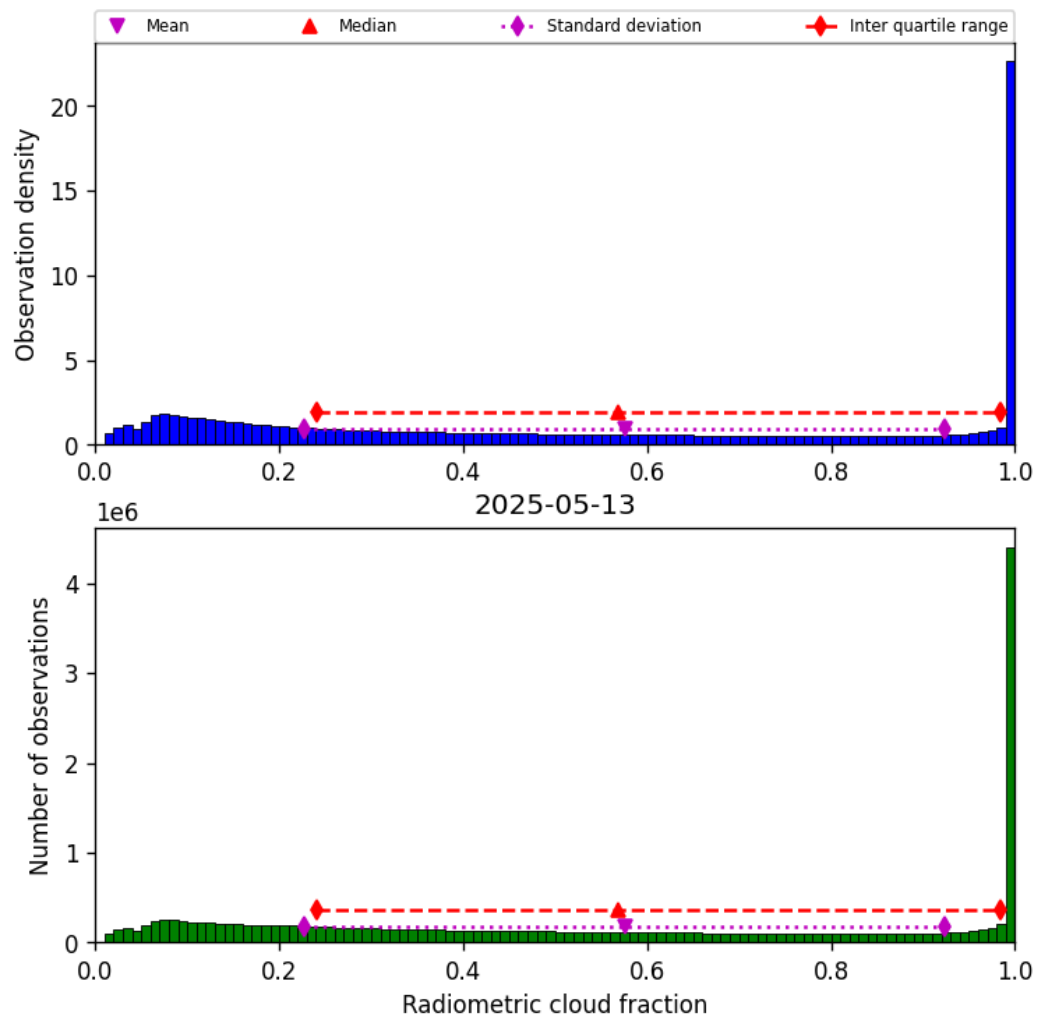
Figure 37: Histogram of “Radiometric cloud fraction” for 2025-05-13 to 2025-05-13
