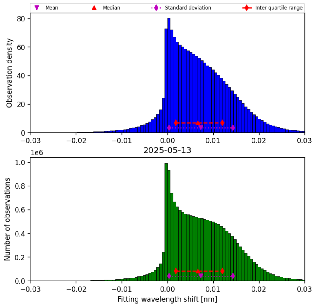
Figure 47: Histogram of “Fitting wavelength shift” for 2025-05-13 to 2025-05-13
