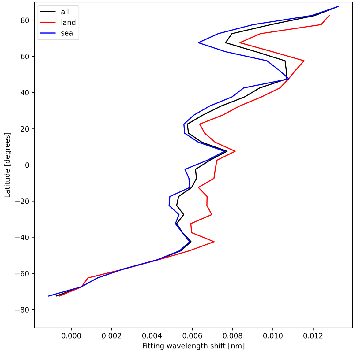
Figure 31: Zonal average of “Fitting wavelength shift” for 2025-05-13 to 2025-05-13.
