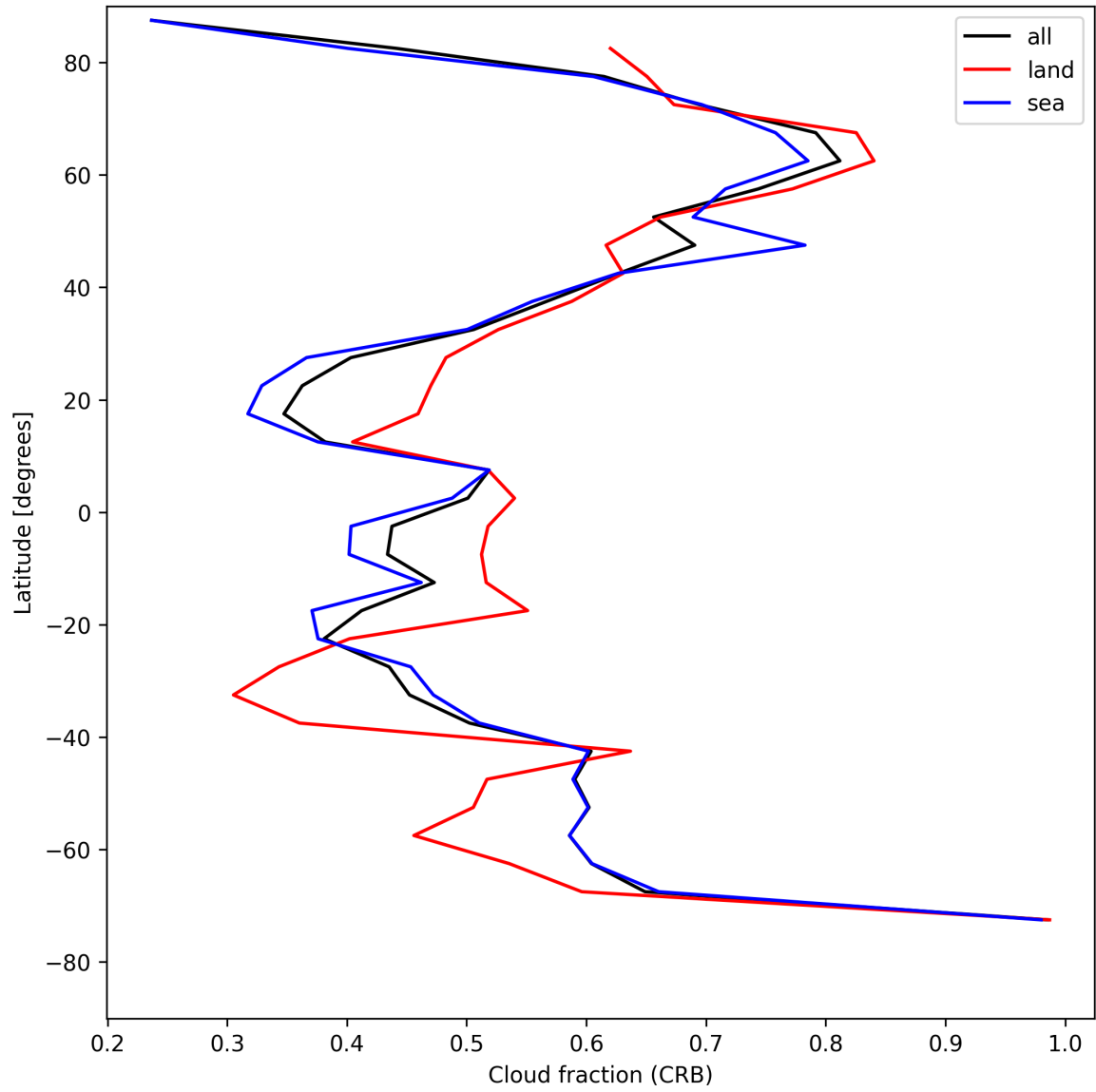
Figure 24: Zonal average of “Cloud fraction (CRB)” for 2025-05-13 to 2025-05-13.
