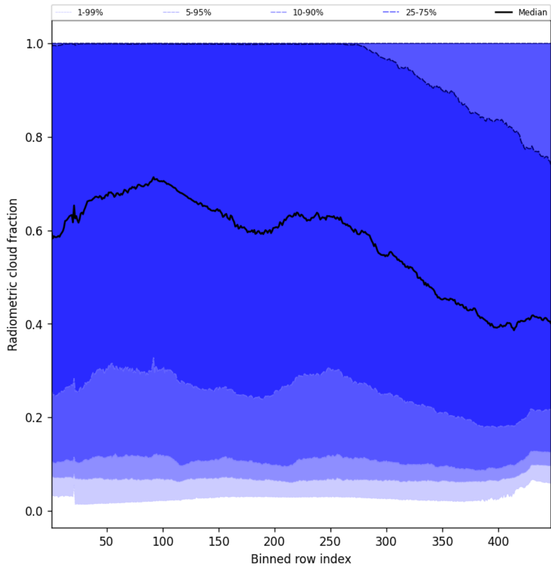
Figure 53: Along track statistics of “Radiometric cloud fraction” for 2025-05-13 to 2025-05-13
