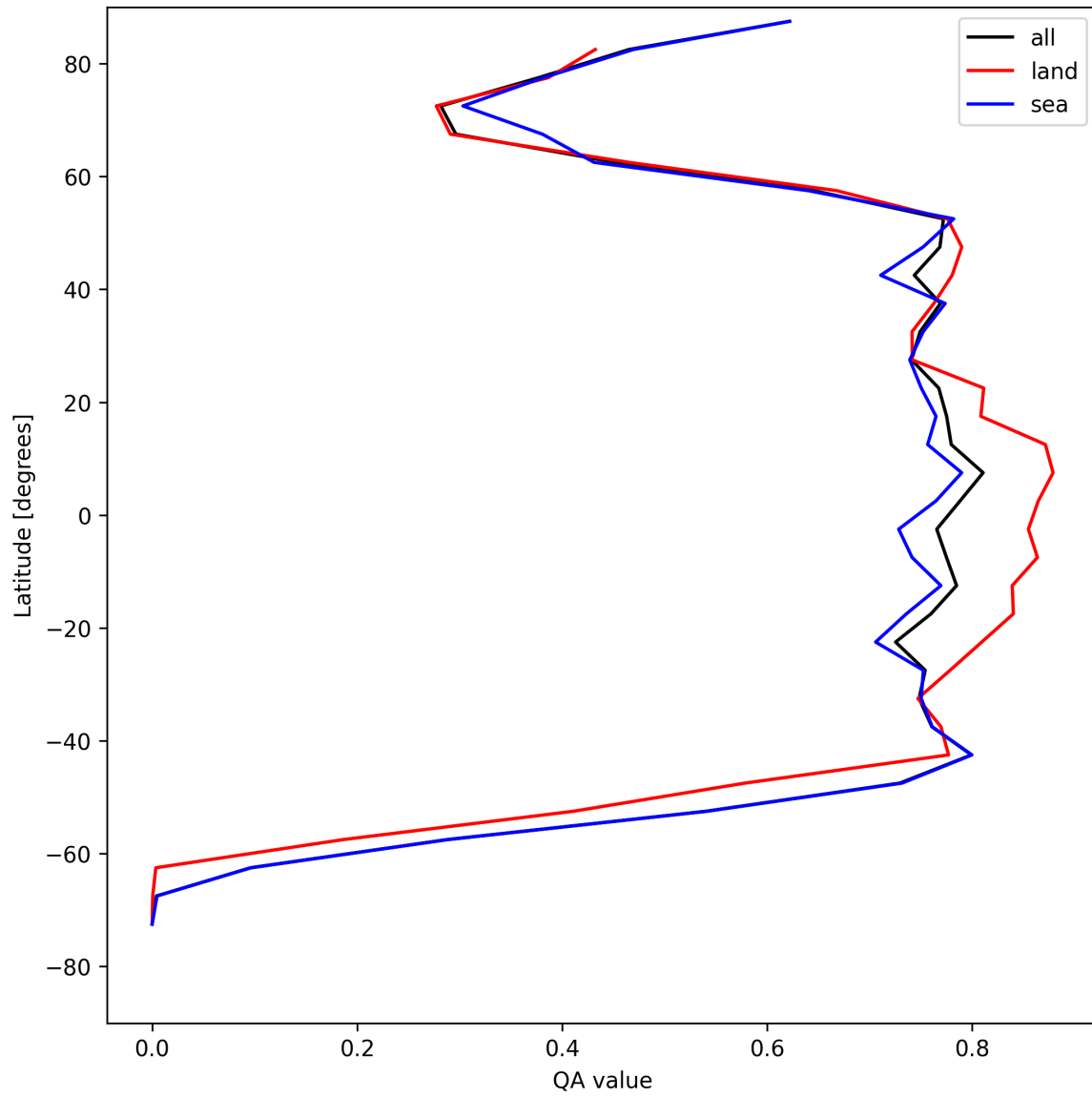
Figure 20: Zonal average of “QA value” for 2025-05-13 to 2025-05-13.
