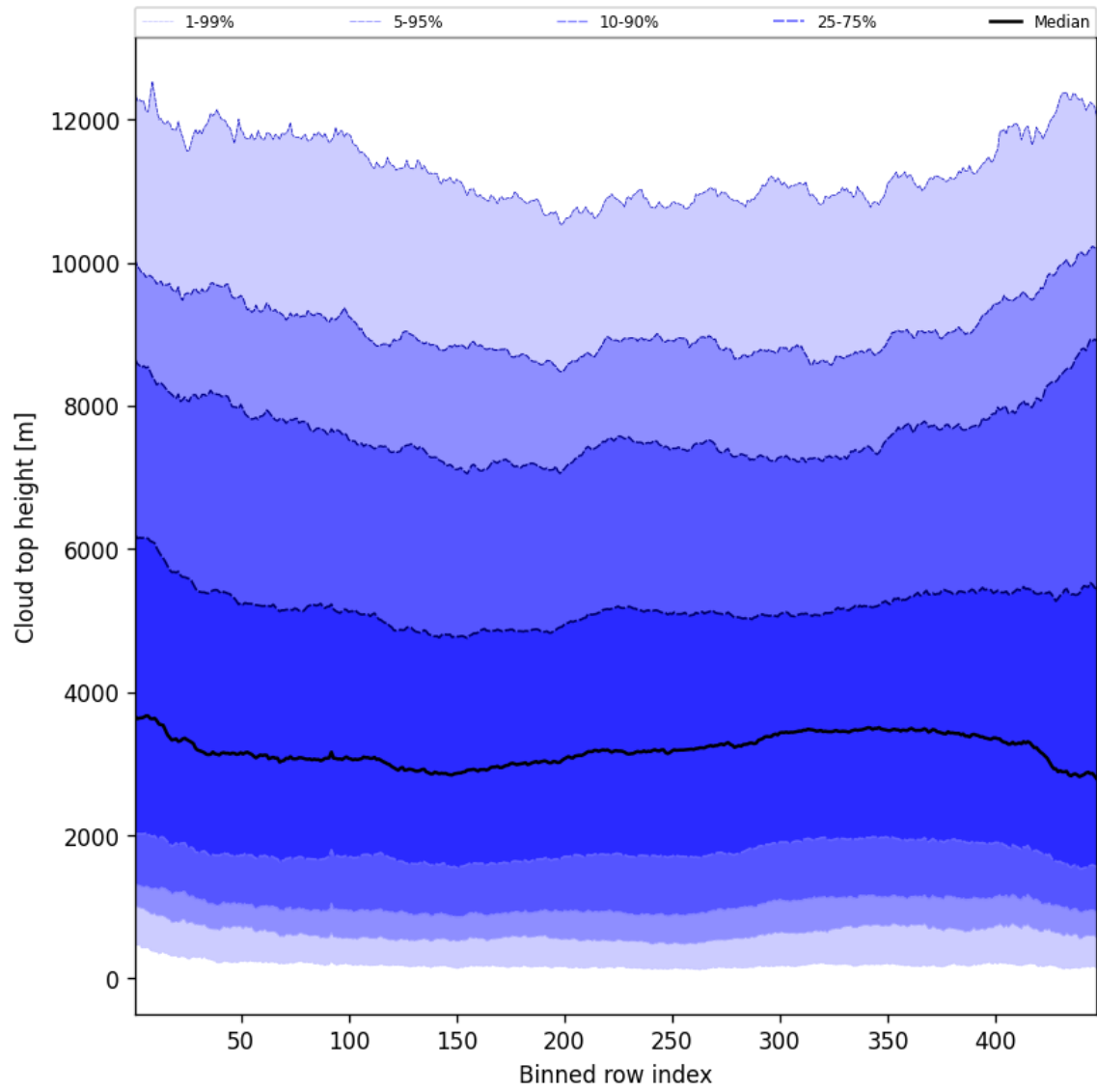
Figure 54: Along track statistics of “Cloud top height” for 2025-05-13 to 2025-05-13
