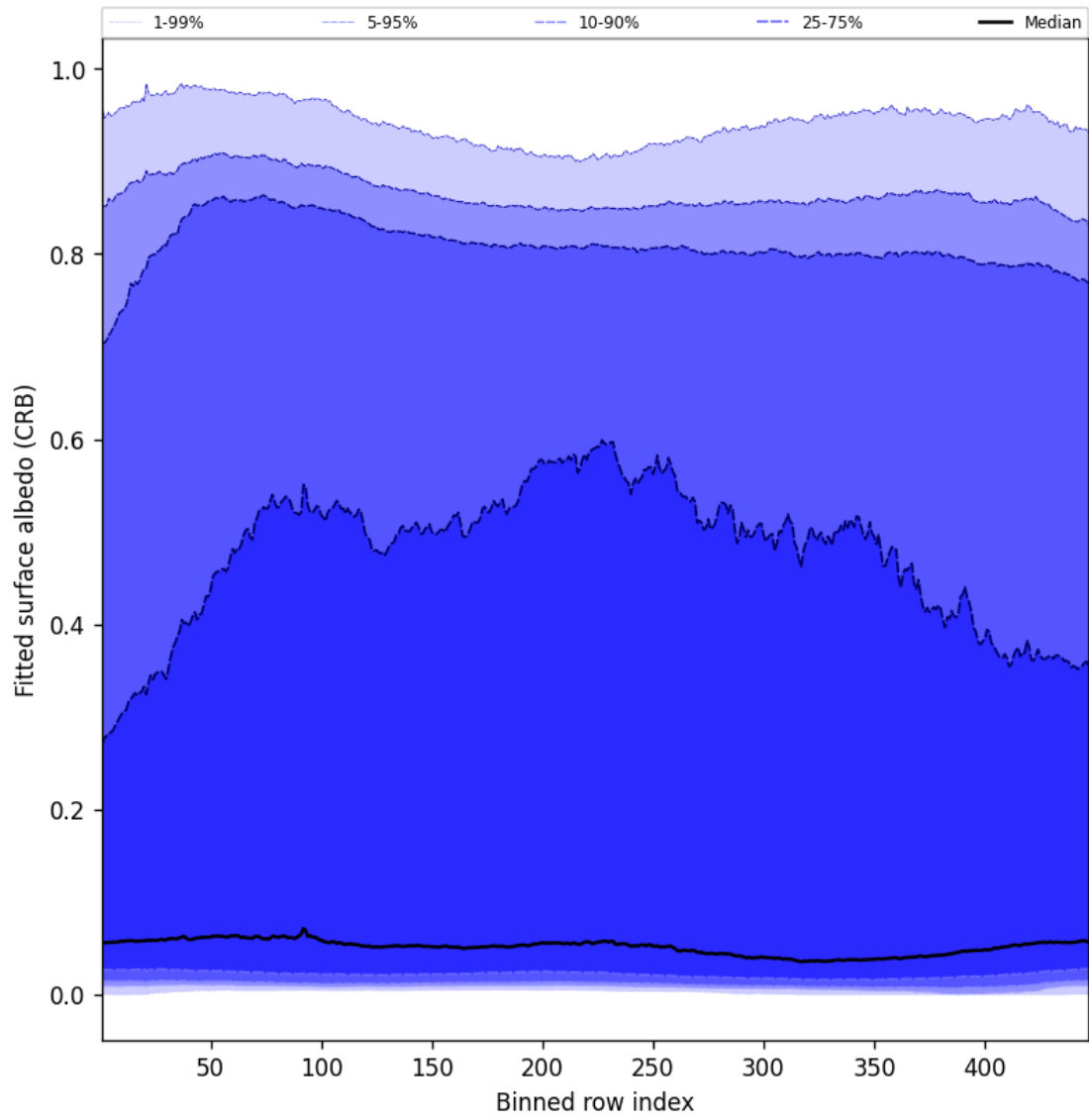
Figure 60: Along track statistics of “Fitted surface albedo (CRB)” for 2025-05-13 to 2025-05-13
