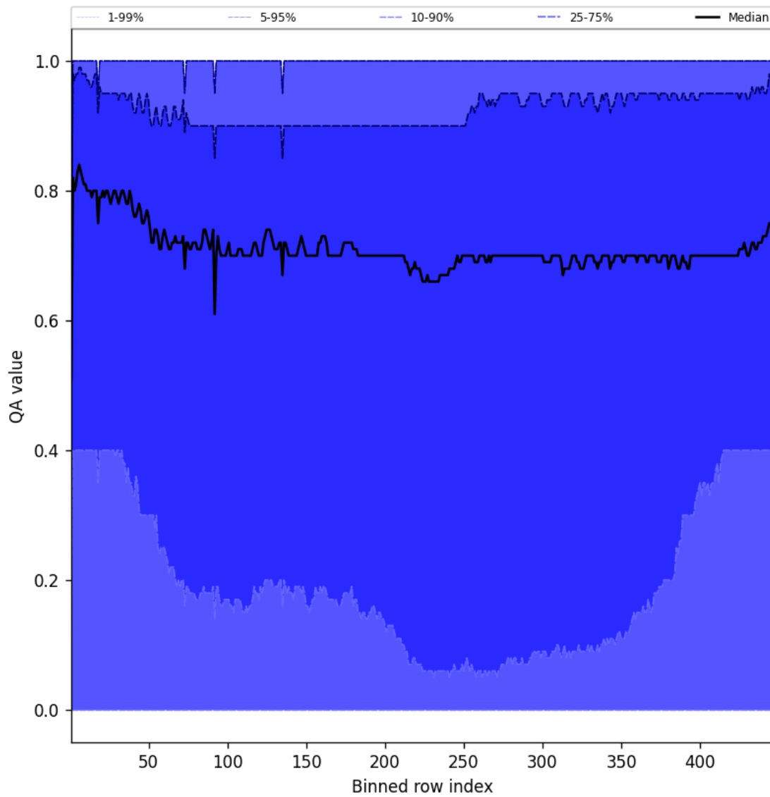
Figure 52: Along track statistics of “QA value” for 2025-05-14 to 2025-05-15
