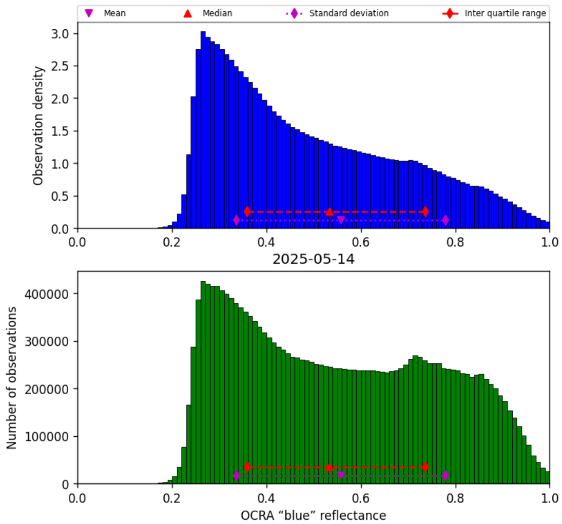
Figure 49: Histogram of “OCRA “blue” reflectance” for 2025-05-14 to 2025-05-15
