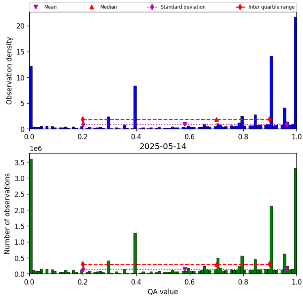
Figure 36: Histogram of “QA value” for 2025-05-14 to 2025-05-15
