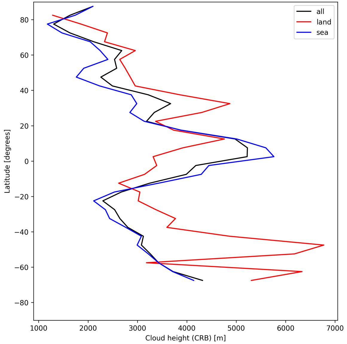
Figure 25: Zonal average of “Cloud height (CRB)” for 2025-05-14 to 2025-05-15.
