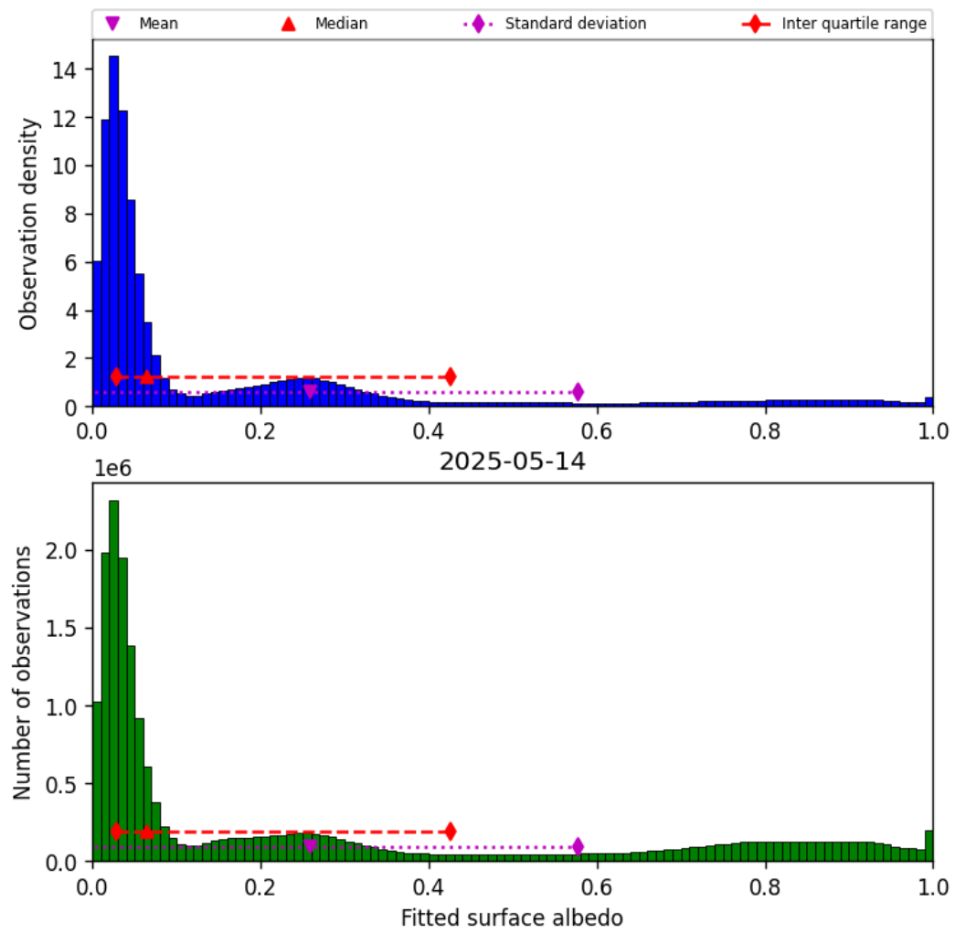
Figure 43: Histogram of “Fitted surface albedo” for 2025-05-14 to 2025-05-15
