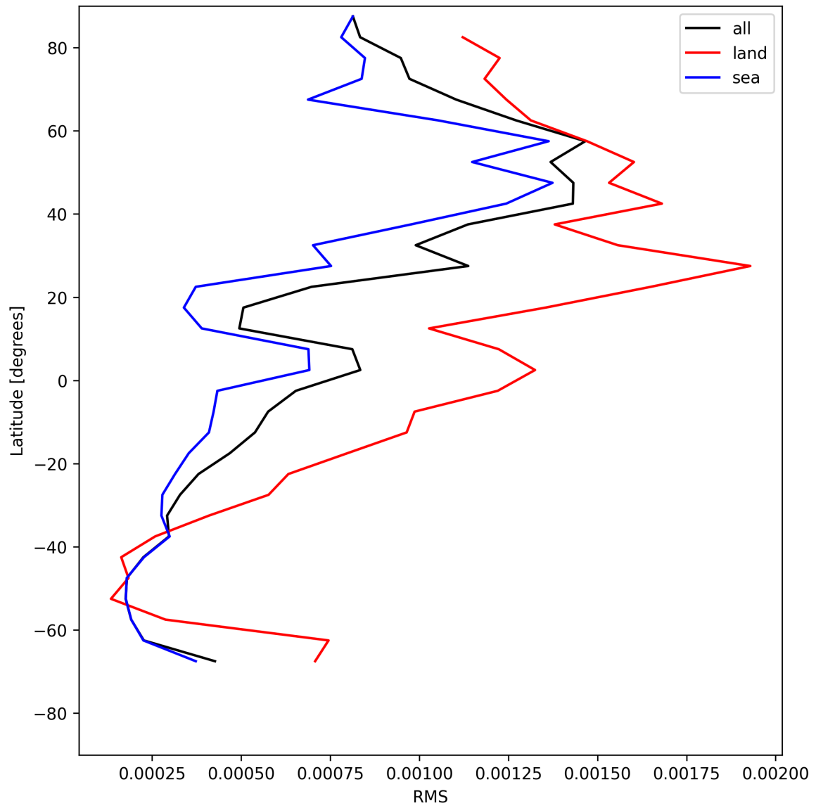
Figure 29: Zonal average of “RMS” for 2025-05-14 to 2025-05-15.
