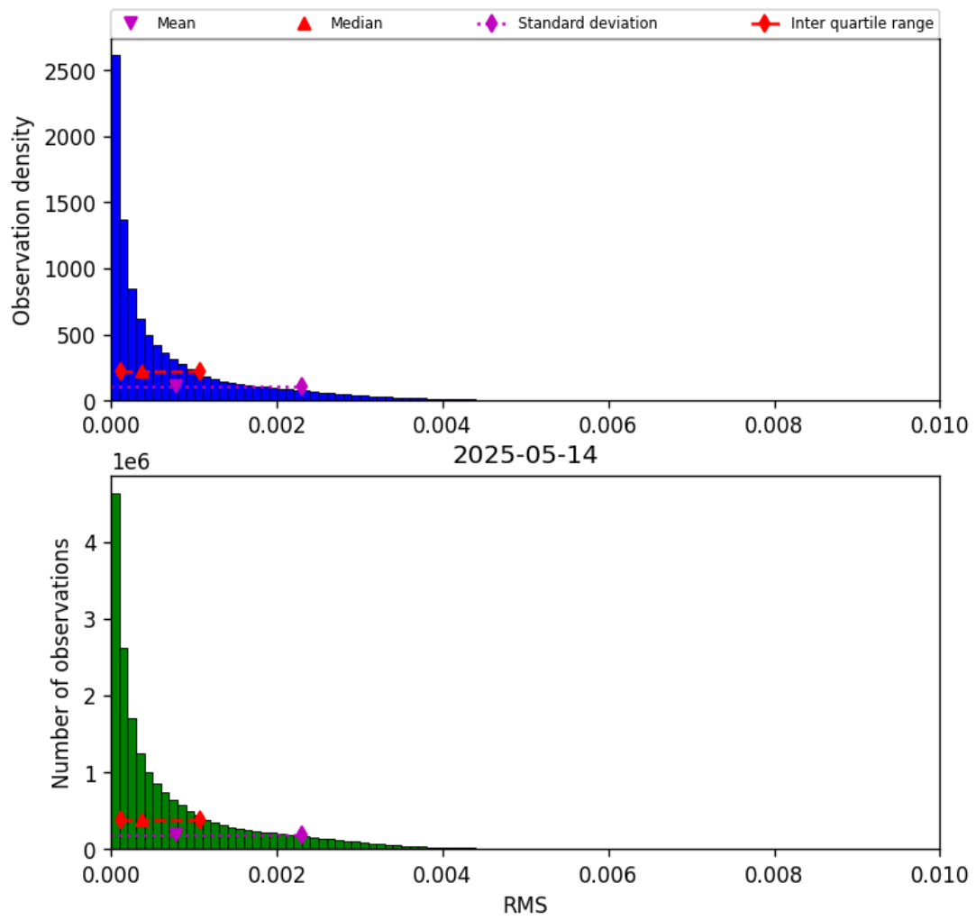
Figure 45: Histogram of “RMS” for 2025-05-14 to 2025-05-15
