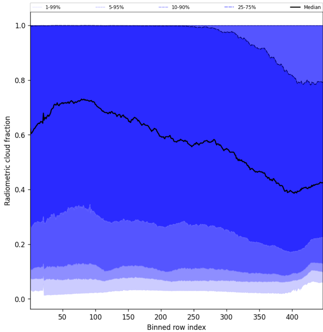
Figure 53: Along track statistics of “Radiometric cloud fraction” for 2025-05-14 to 2025-05-15
