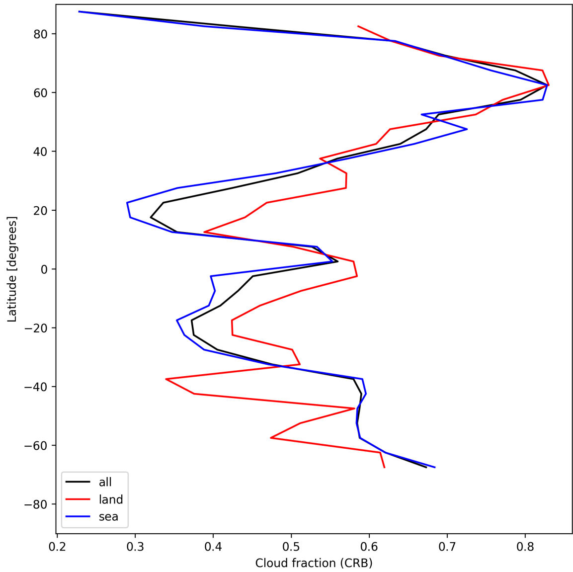
Figure 24: Zonal average of “Cloud fraction (CRB)” for 2025-05-14 to 2025-05-15.
