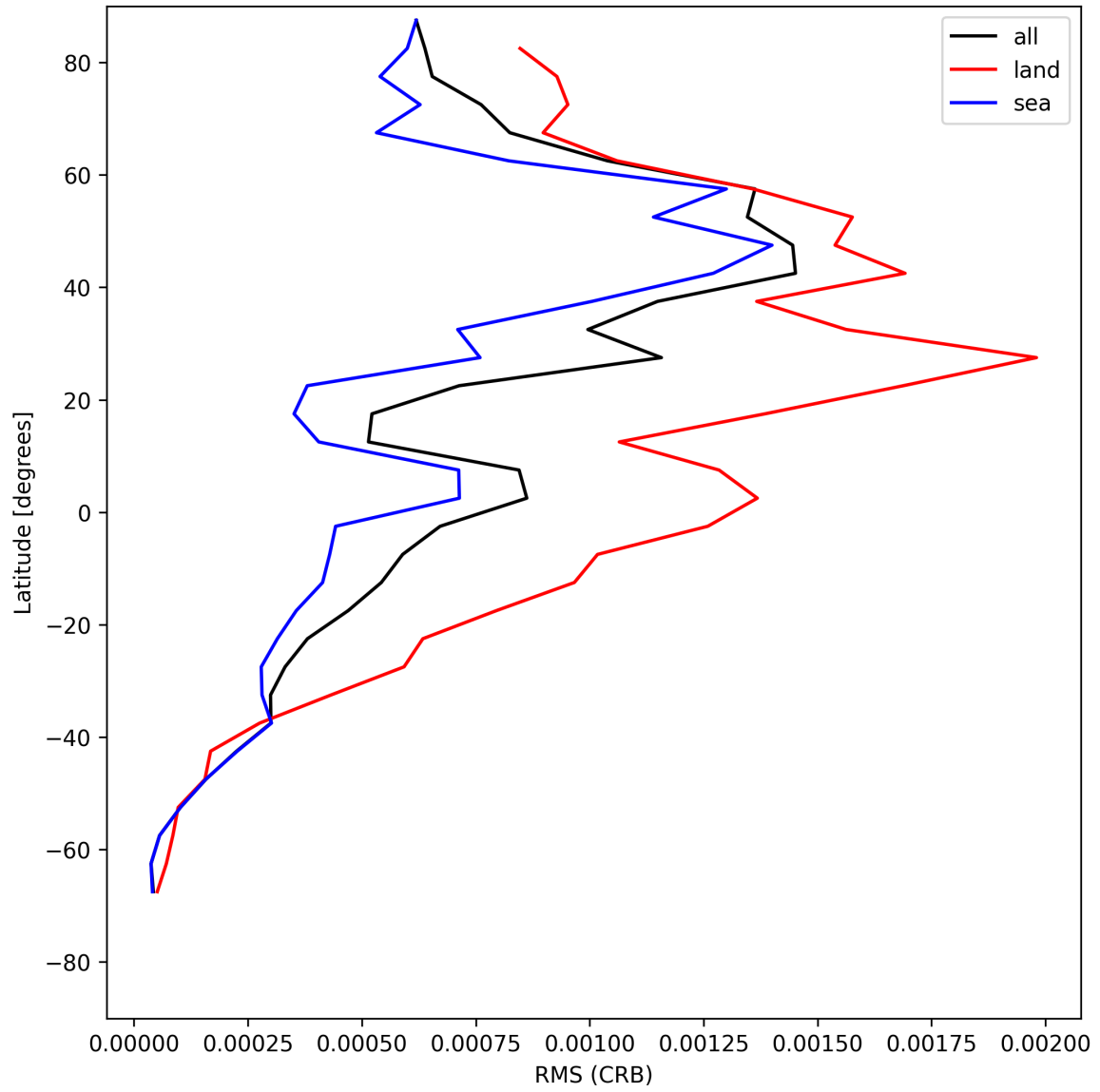
Figure 30: Zonal average of “RMS (CRB)” for 2025-05-14 to 2025-05-15.
