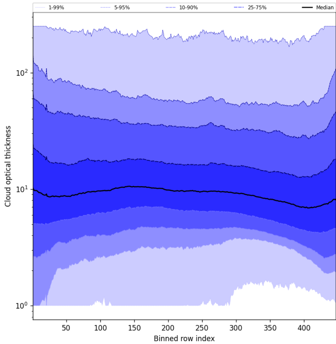
Figure 55: Along track statistics of “Cloud optical thickness” for 2025-05-14 to 2025-05-15
