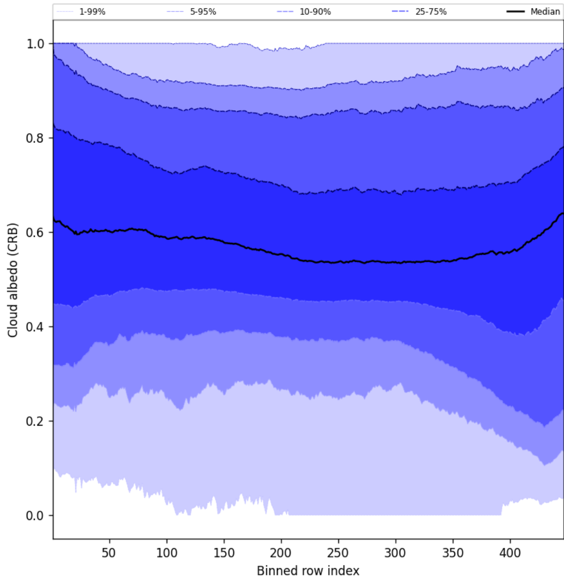
Figure 58: Along track statistics of “Cloud albedo (CRB)” for 2025-05-14 to 2025-05-15
