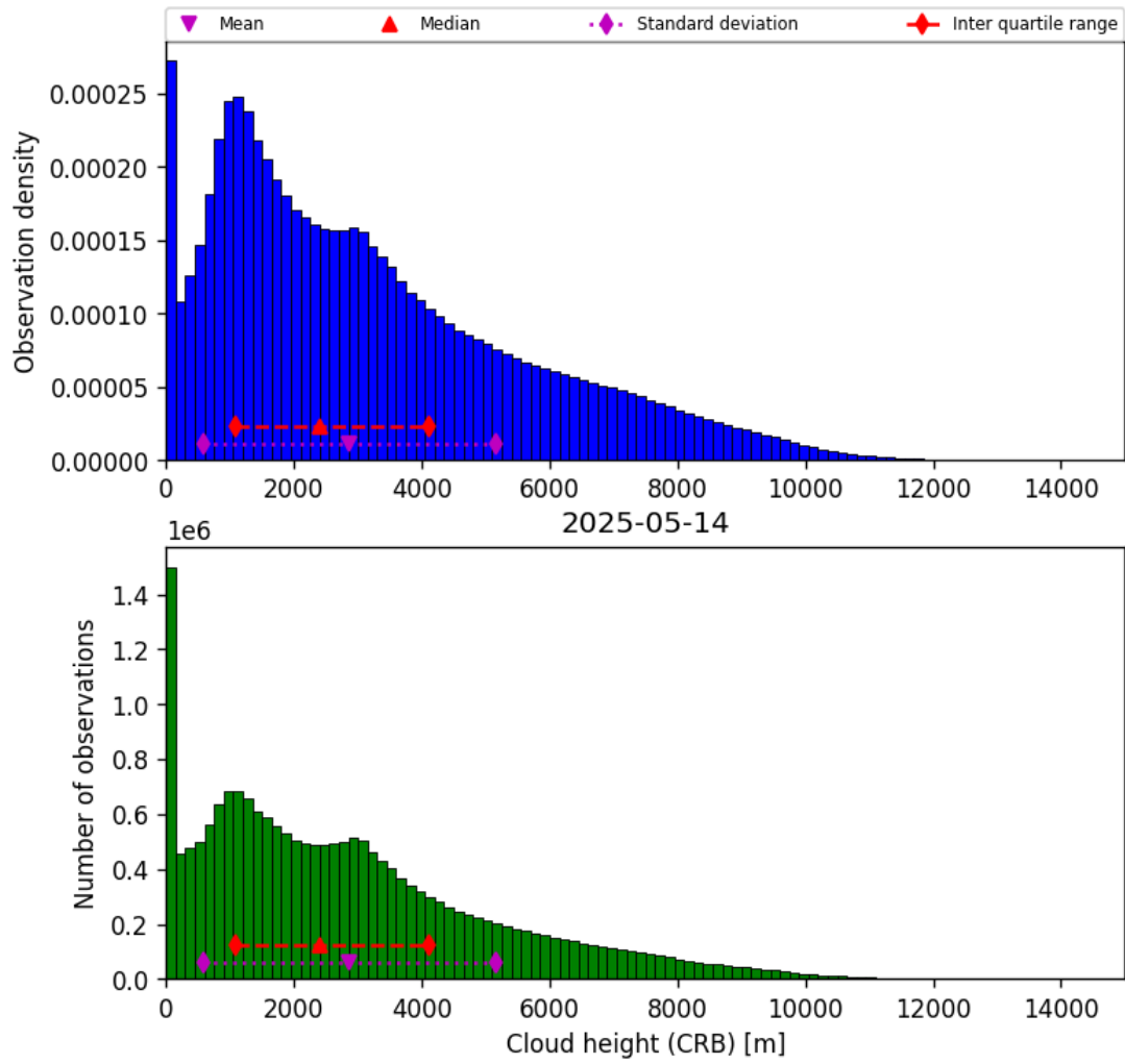
Figure 41: Histogram of “Cloud height (CRB)” for 2025-05-14 to 2025-05-15
