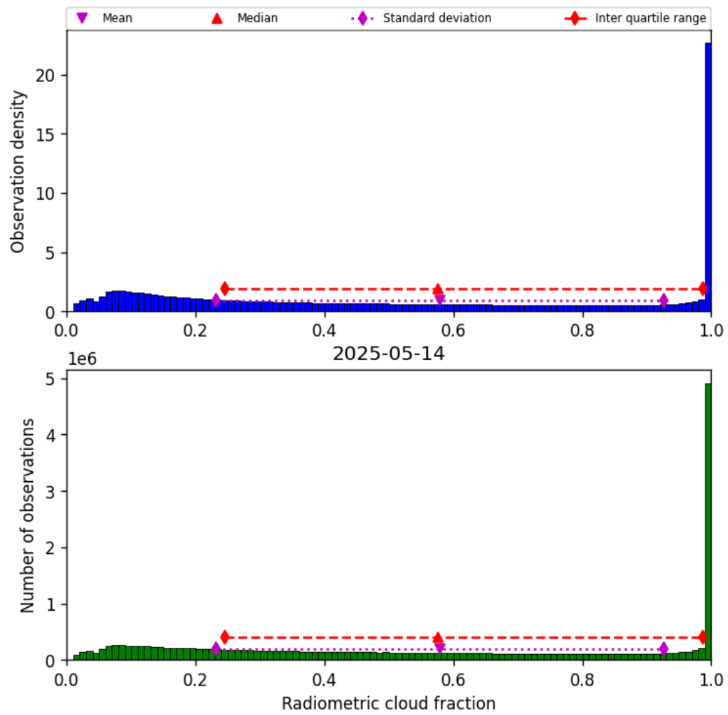
Figure 37: Histogram of “Radiometric cloud fraction” for 2025-05-14 to 2025-05-15
