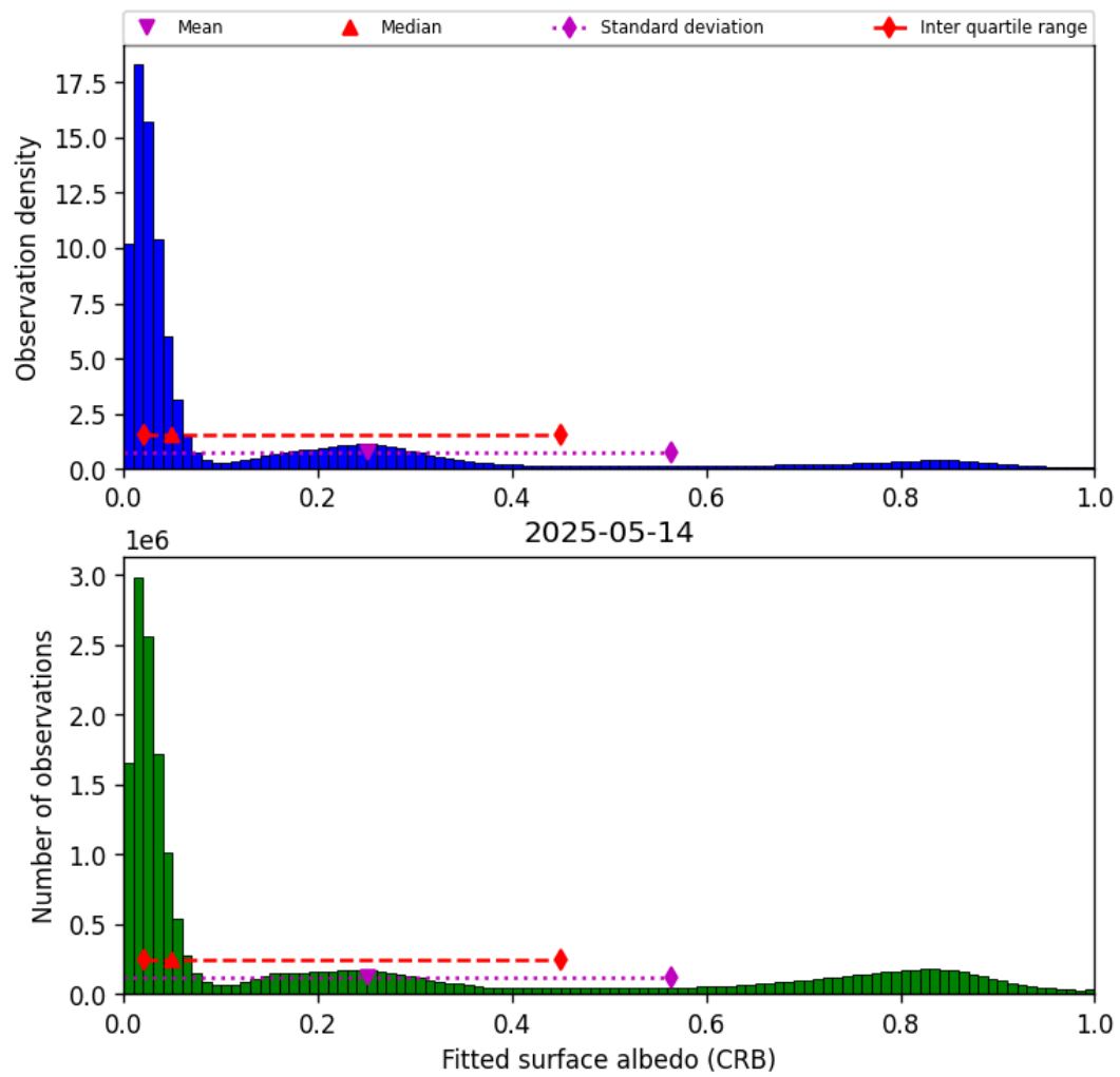
Figure 44: Histogram of “Fitted surface albedo (CRB)” for 2025-05-14 to 2025-05-15
