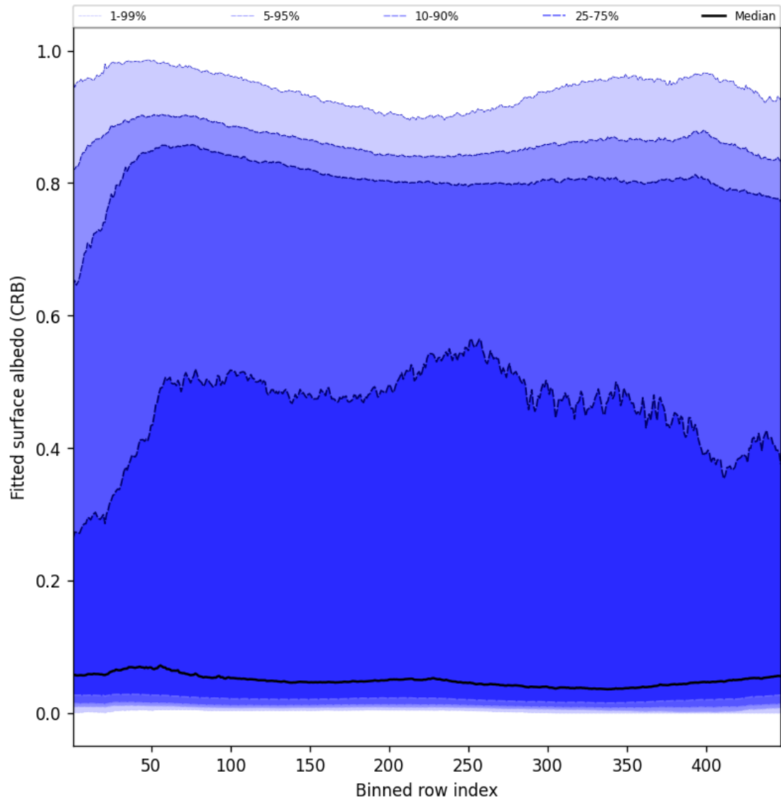
Figure 60: Along track statistics of “Fitted surface albedo (CRB)” for 2025-05-14 to 2025-05-15
