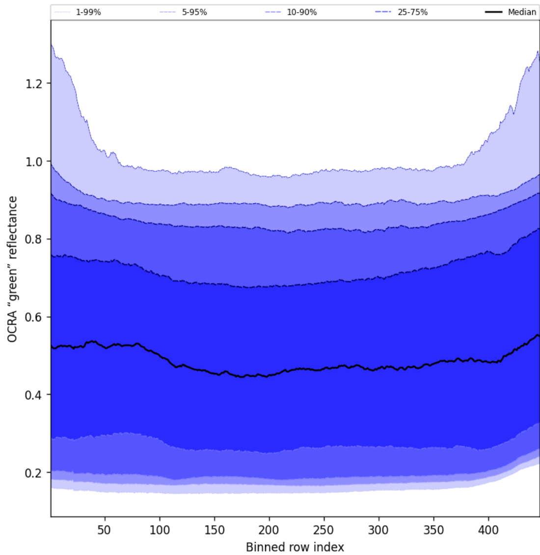
Figure 66: Along track statistics of "OCRA "green" reflectance" for 2025-05-14 to 2025-05-15
