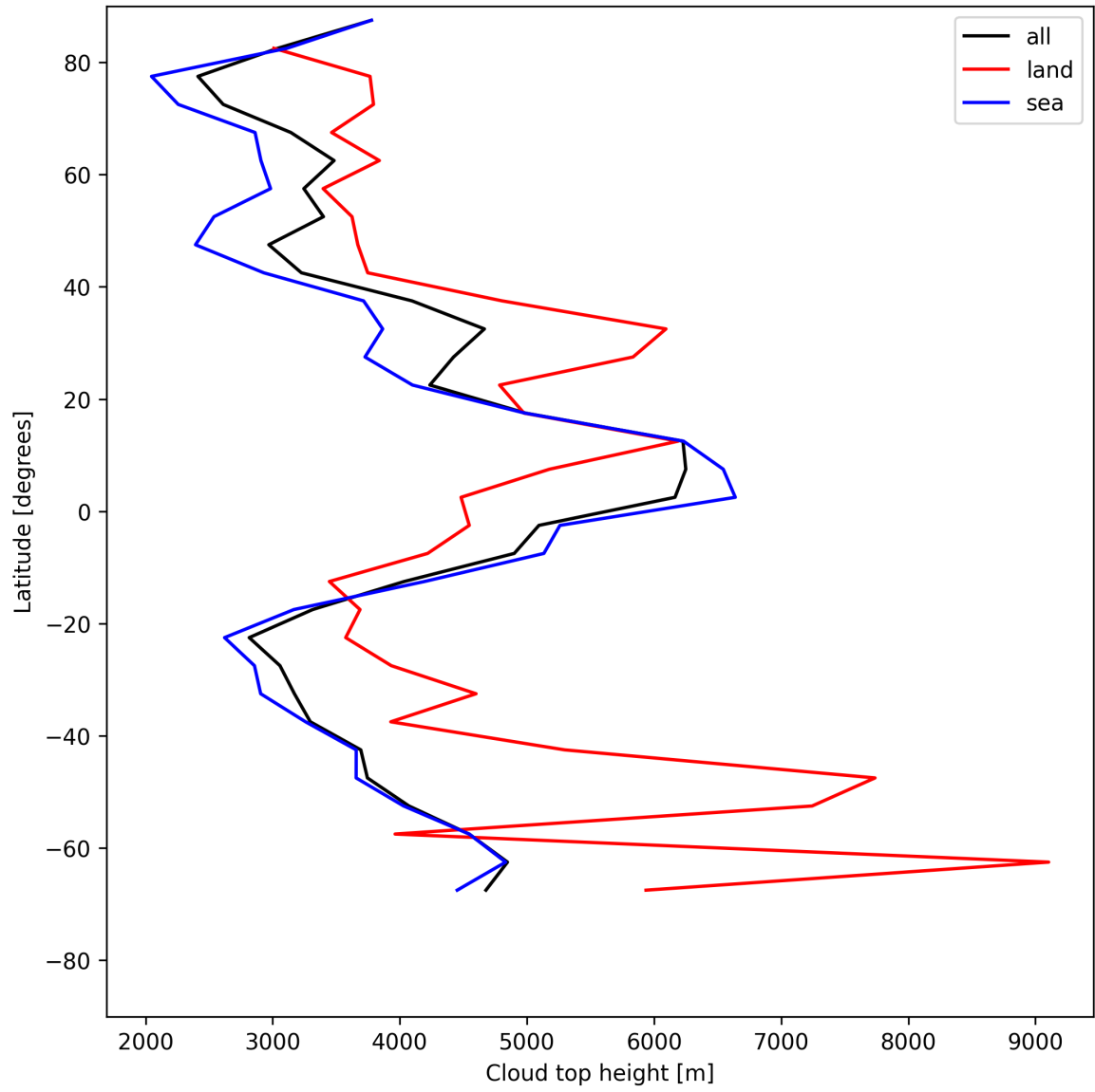
Figure 22: Zonal average of “Cloud top height” for 2025-05-14 to 2025-05-15.
