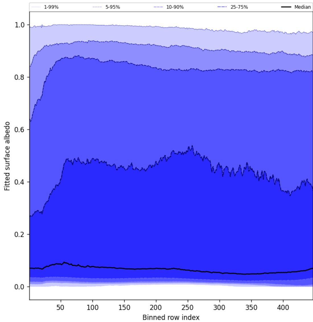
Figure 59: Along track statistics of “Fitted surface albedo” for 2025-05-14 to 2025-05-15
