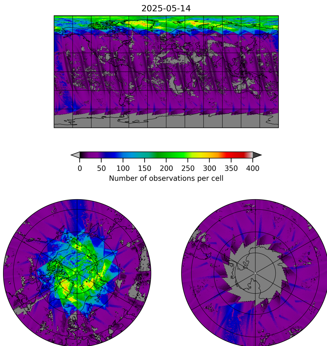
Figure 19: Map of the number of observations for 2025-05-14 to 2025-05-15
