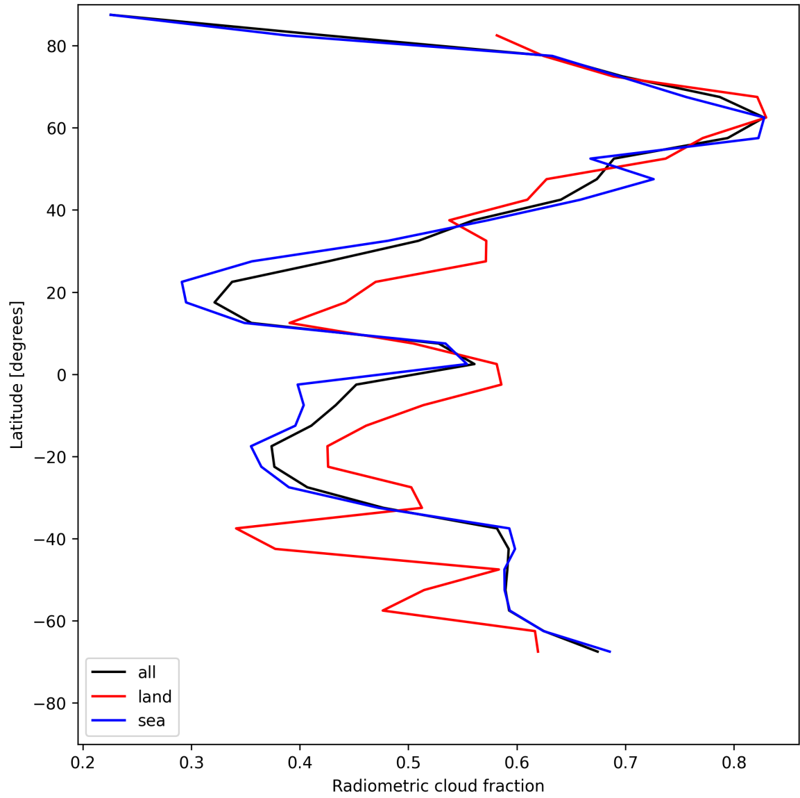
Figure 21: Zonal average of “Radiometric cloud fraction” for 2025-05-14 to 2025-05-15.
