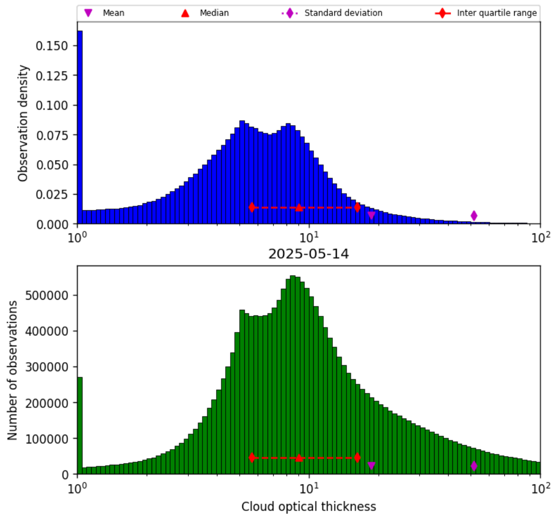
Figure 39: Histogram of “Cloud optical thickness” for 2025-05-14 to 2025-05-15
