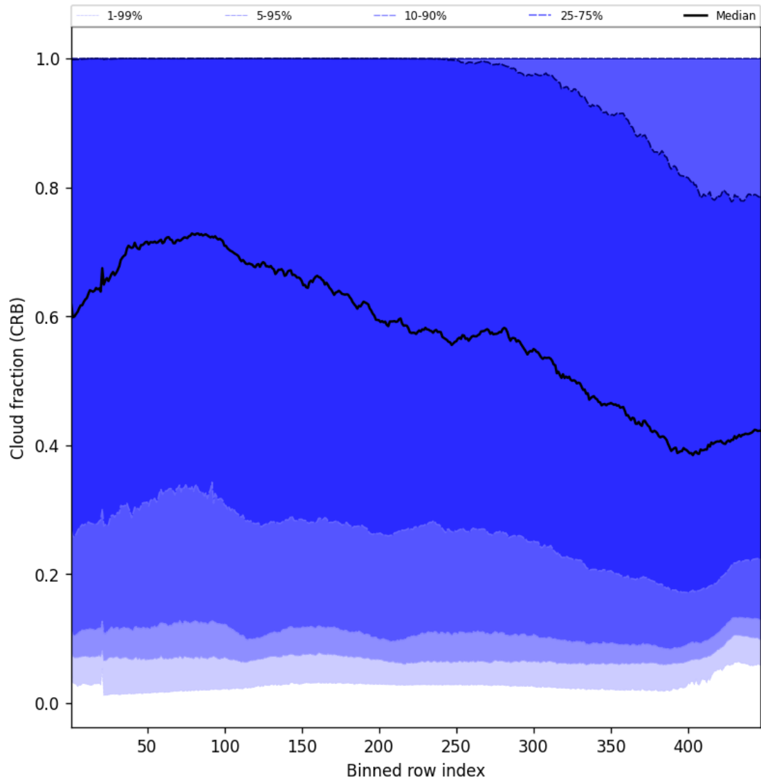
Figure 56: Along track statistics of “Cloud fraction (CRB)” for 2025-05-14 to 2025-05-15
