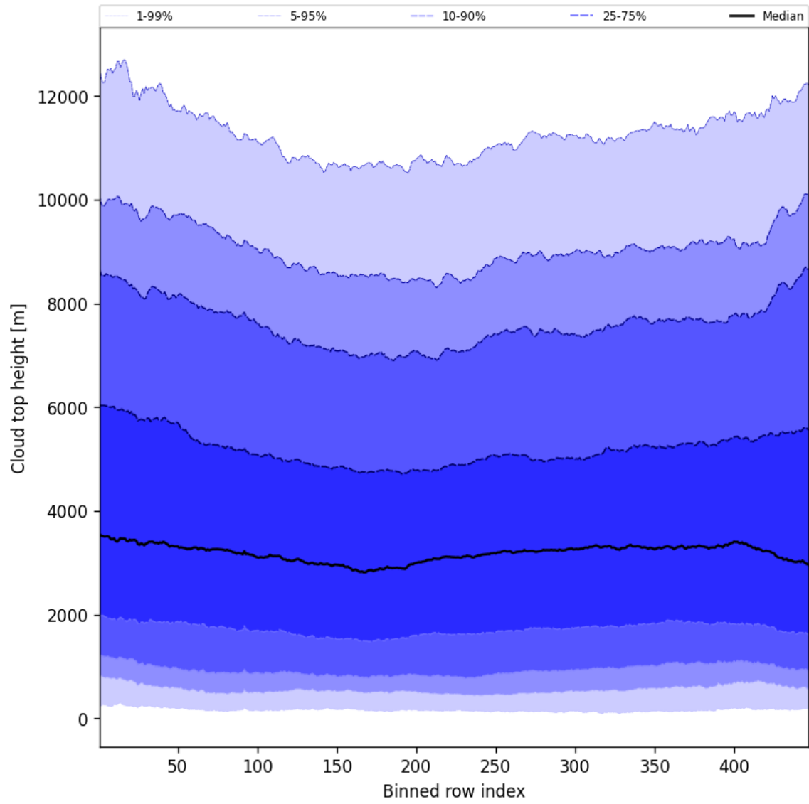
Figure 54: Along track statistics of “Cloud top height” for 2025-05-14 to 2025-05-15
