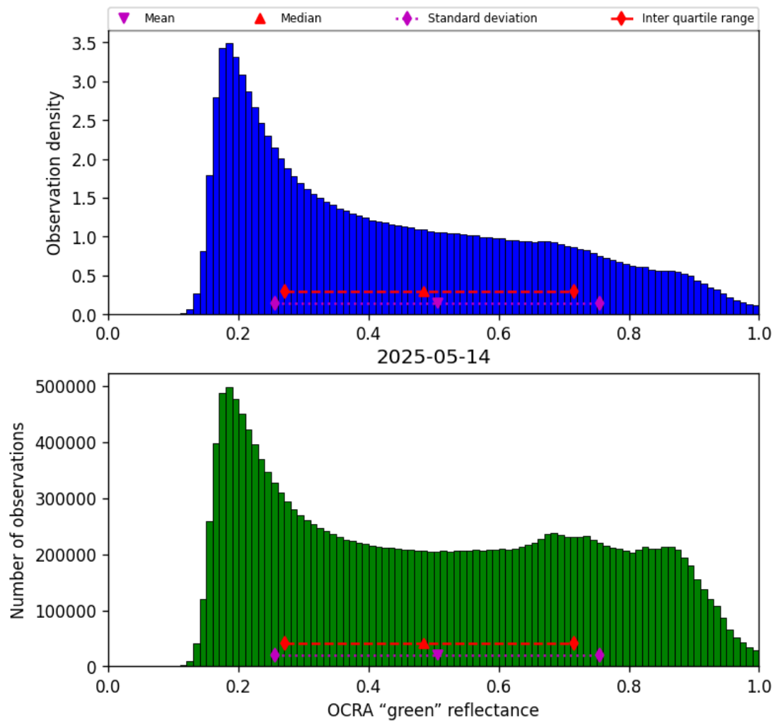
Figure 50: Histogram of “OCRA “green” reflectance” for 2025-05-14 to 2025-05-15
