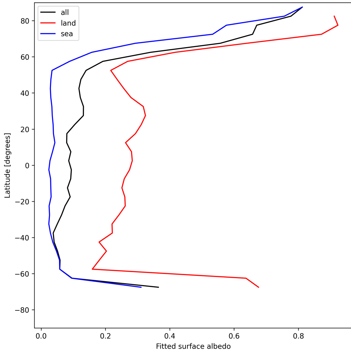
Figure 27: Zonal average of “Fitted surface albedo” for 2025-05-14 to 2025-05-15.
