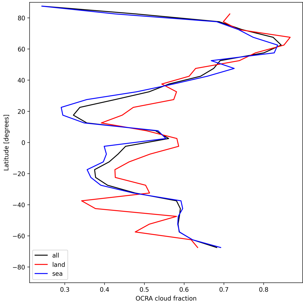
Figure 32: Zonal average of “OCRA cloud fraction” for 2025-05-14 to 2025-05-15.
