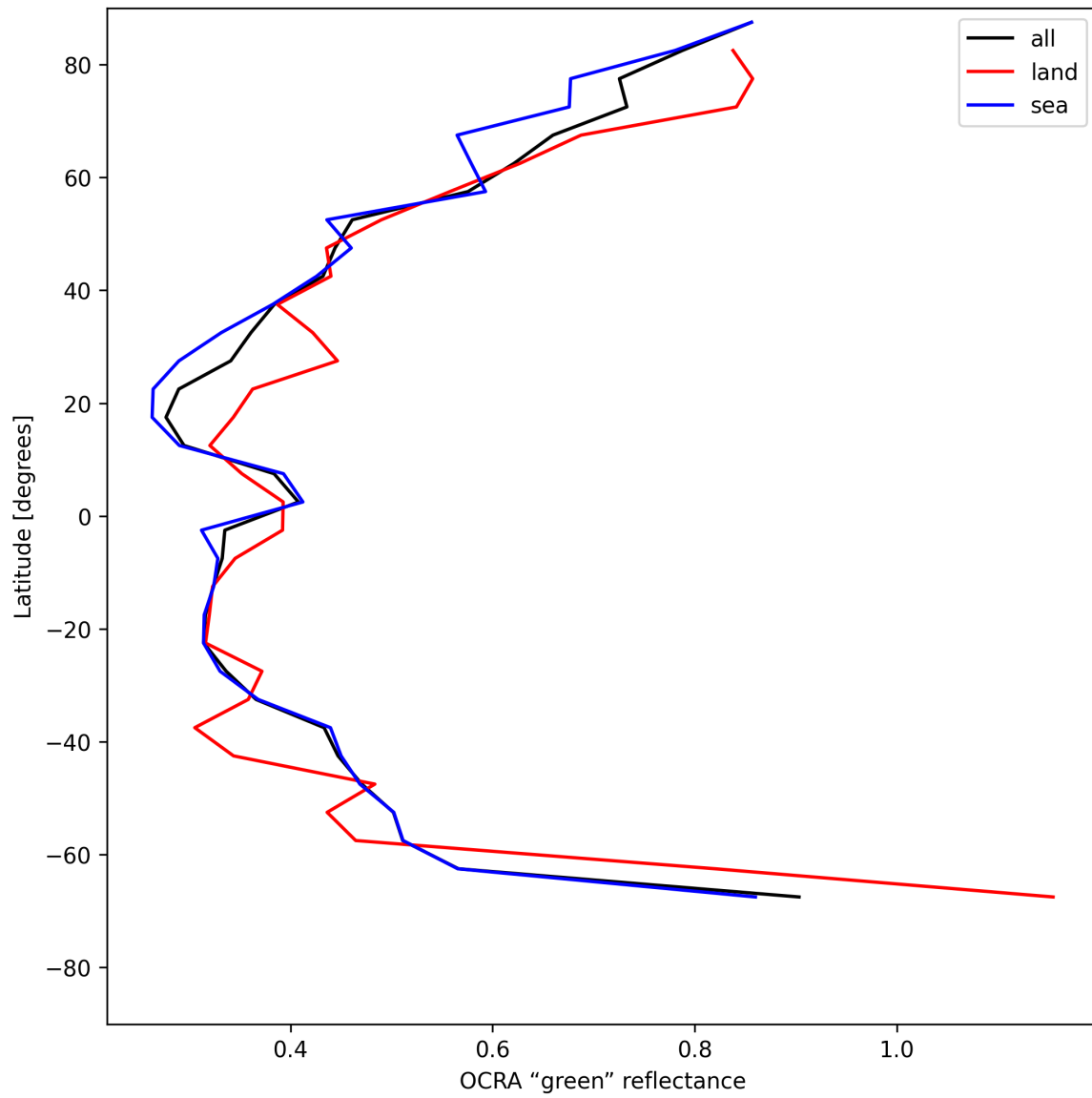
Figure 34: Zonal average of “OCRA “green” reflectance” for 2025-05-14 to 2025-05-15.
