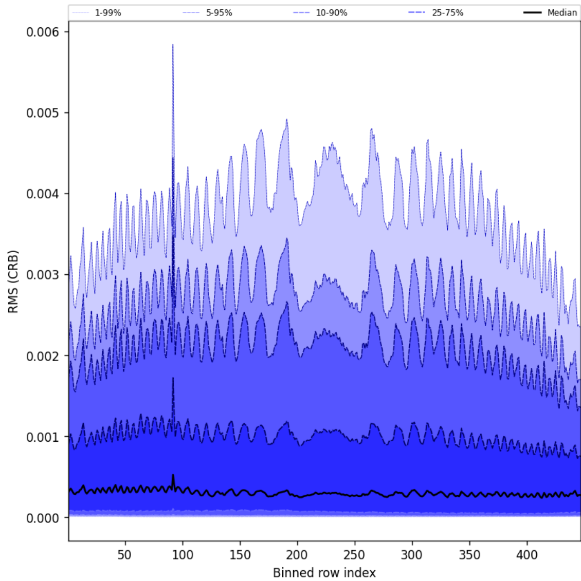
Figure 62: Along track statistics of “RMS (CRB)” for 2025-05-14 to 2025-05-15
