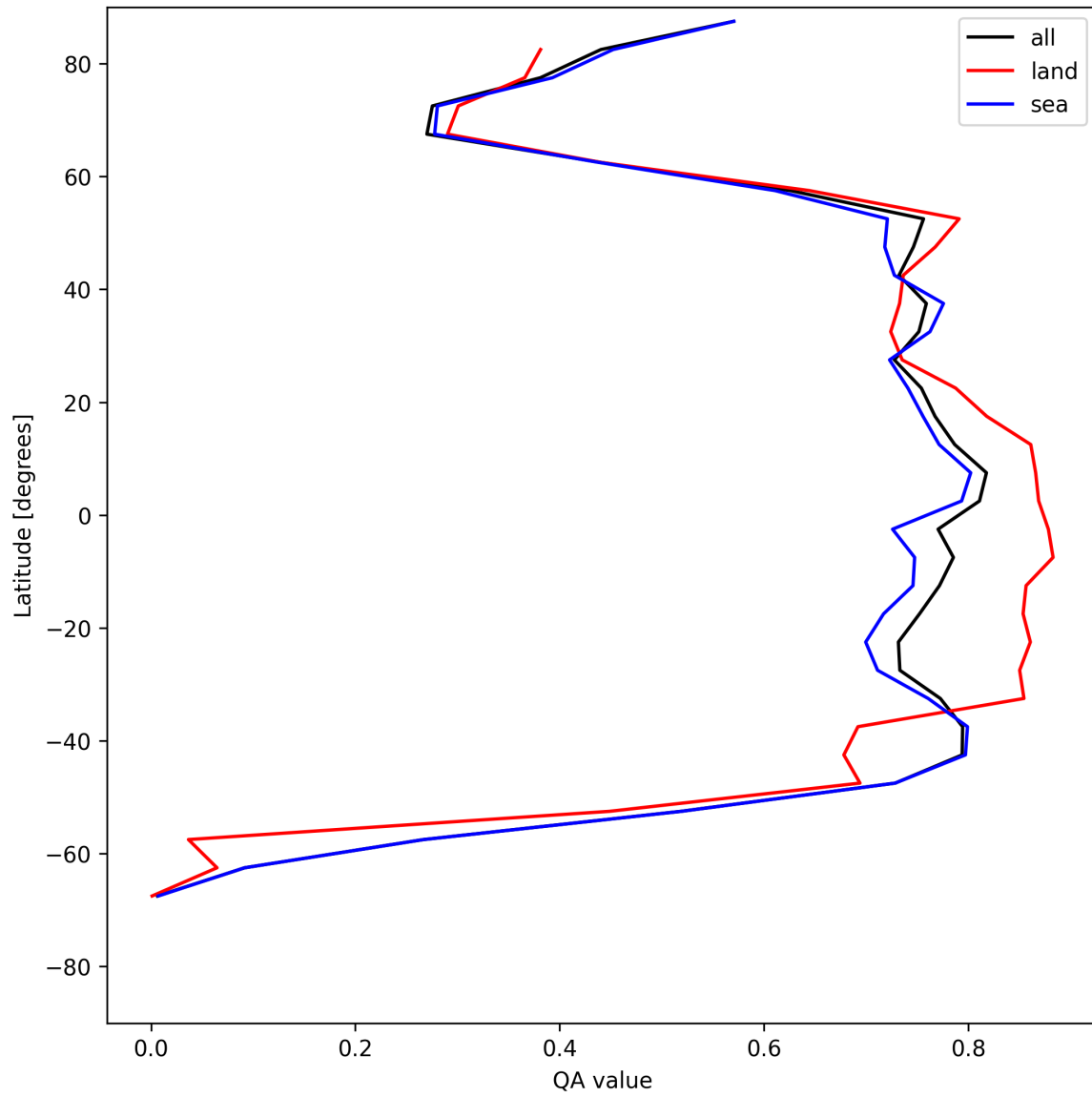
Figure 20: Zonal average of “QA value” for 2025-05-14 to 2025-05-15.
