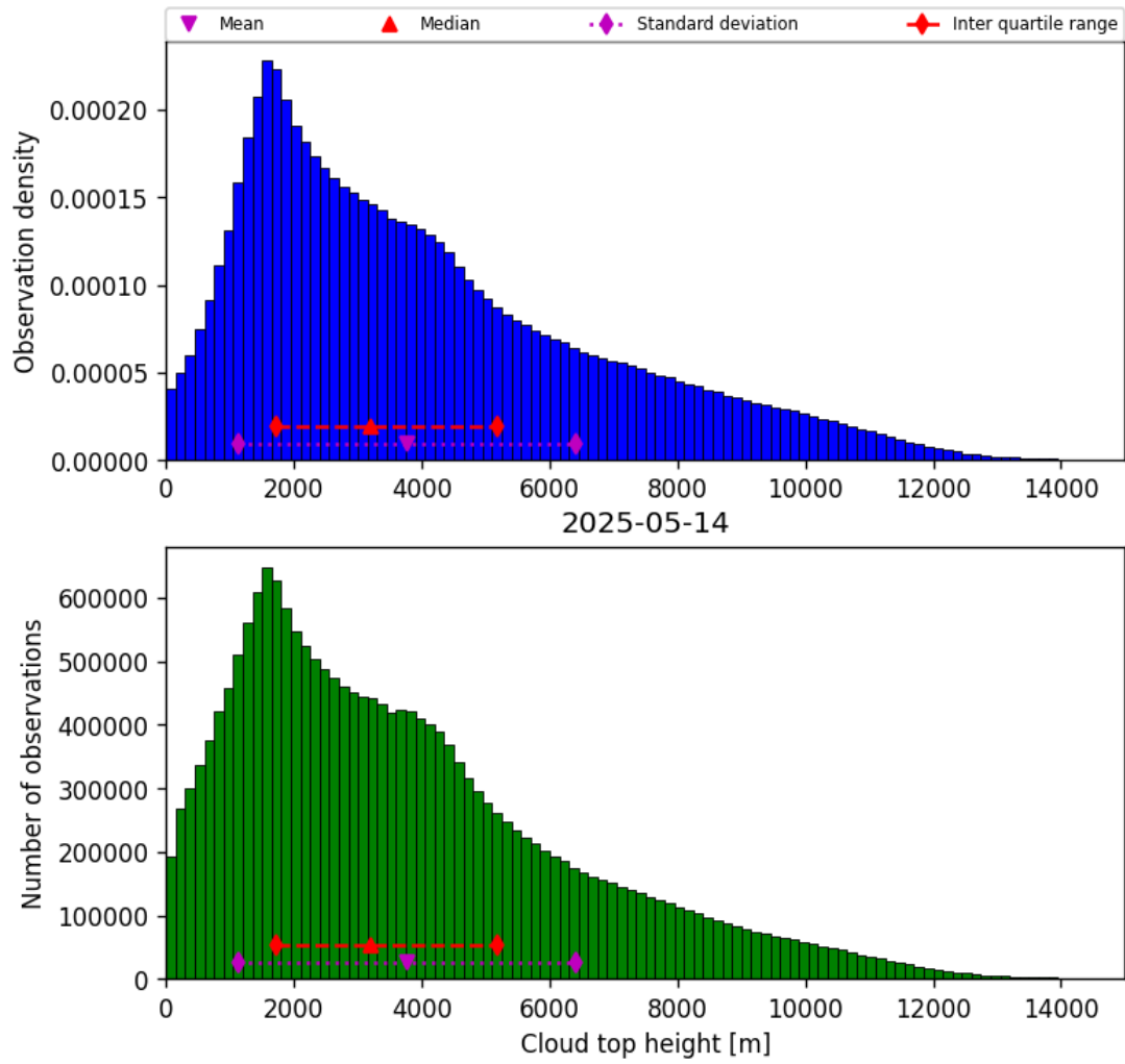
Figure 38: Histogram of “Cloud top height” for 2025-05-14 to 2025-05-15
