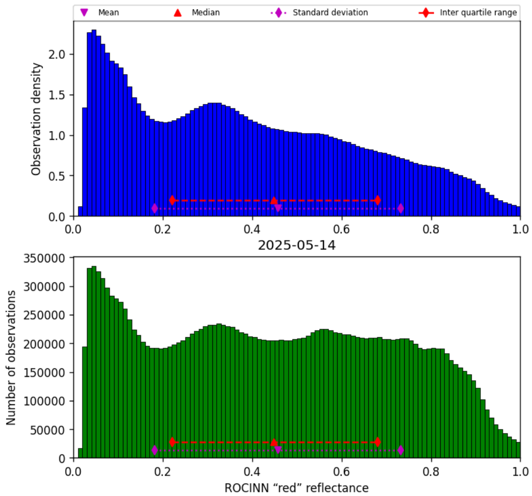
Figure 51: Histogram of “ROCINN “red” reflectance” for 2025-05-14 to 2025-05-15
