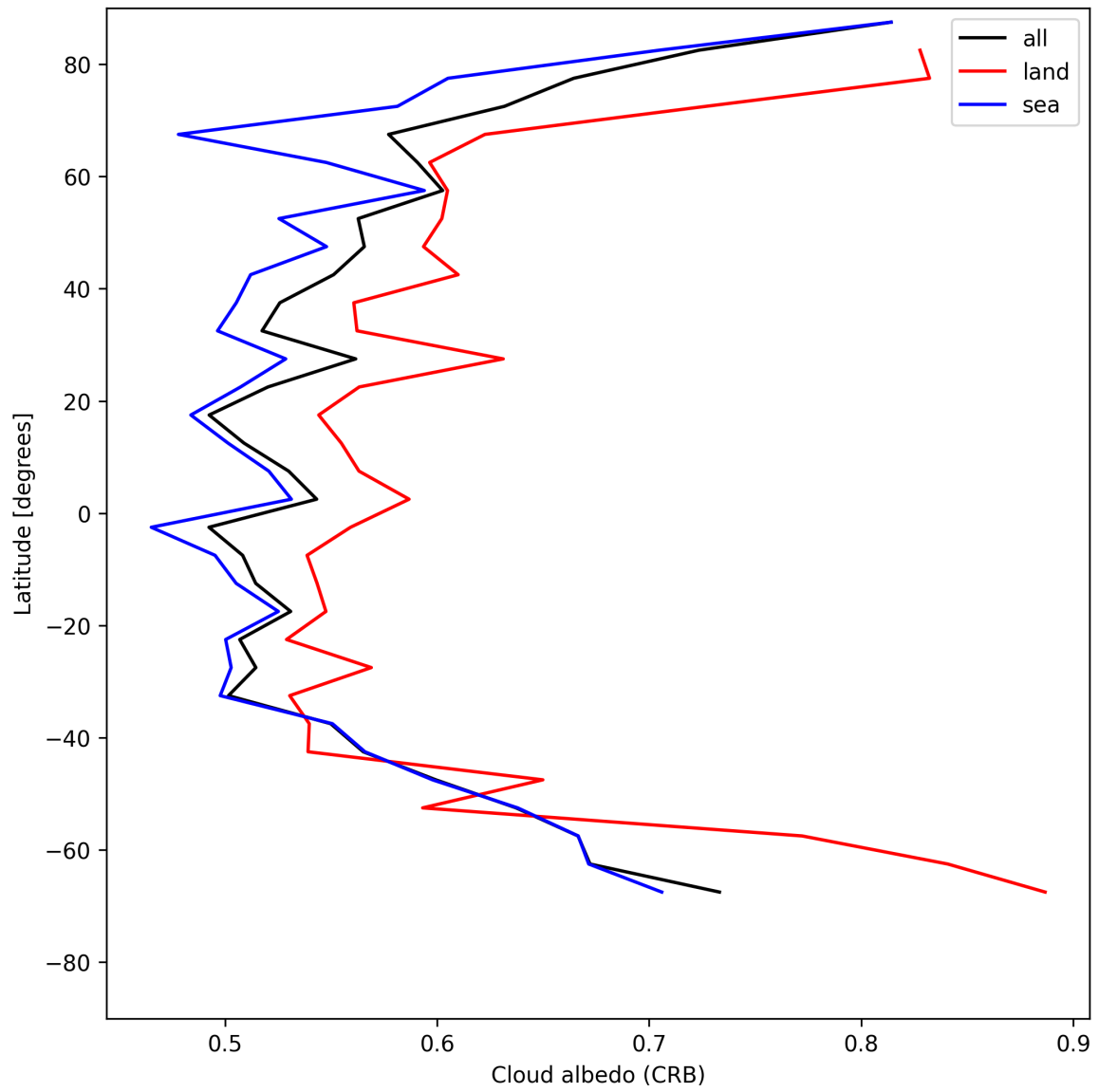
Figure 26: Zonal average of “Cloud albedo (CRB)” for 2025-05-14 to 2025-05-15.
