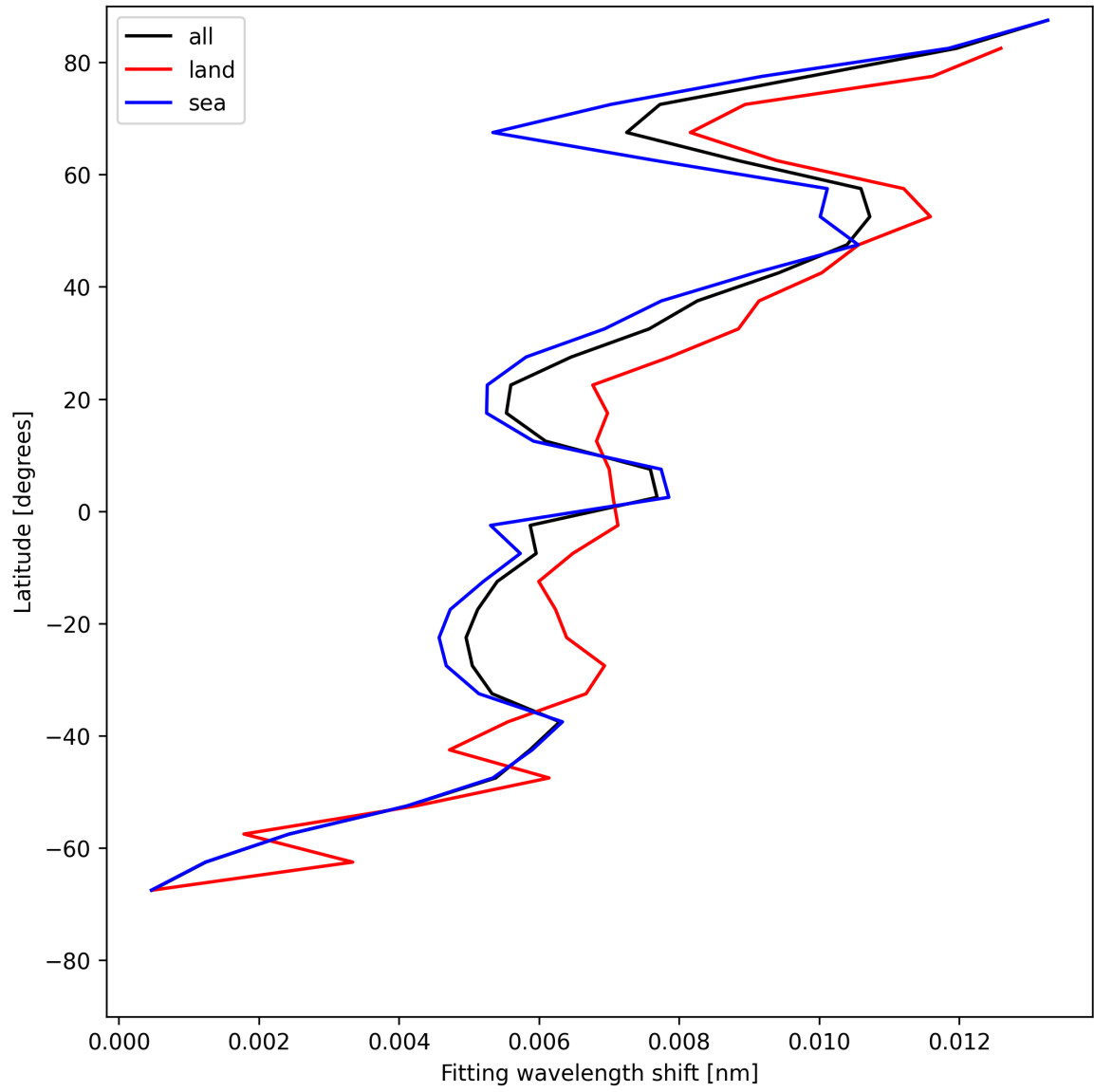
Figure 31: Zonal average of “Fitting wavelength shift” for 2025-05-14 to 2025-05-15.
