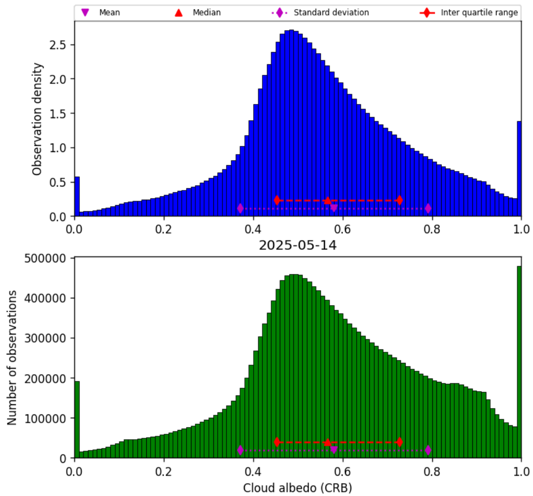
Figure 42: Histogram of “Cloud albedo (CRB)” for 2025-05-14 to 2025-05-15
