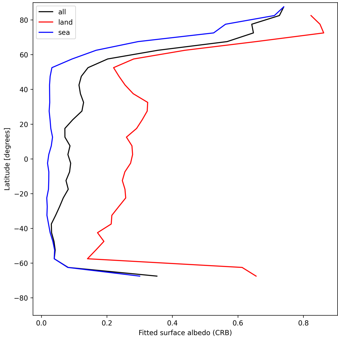
Figure 28: Zonal average of “Fitted surface albedo (CRB)” for 2025-05-14 to 2025-05-15.
