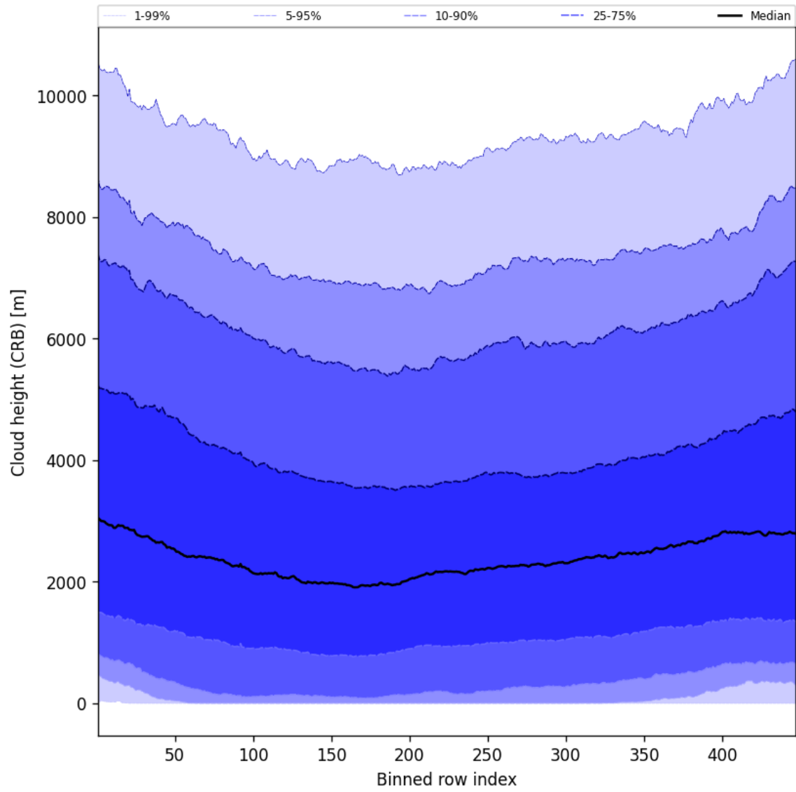
Figure 57: Along track statistics of “Cloud height (CRB)” for 2025-05-14 to 2025-05-15
