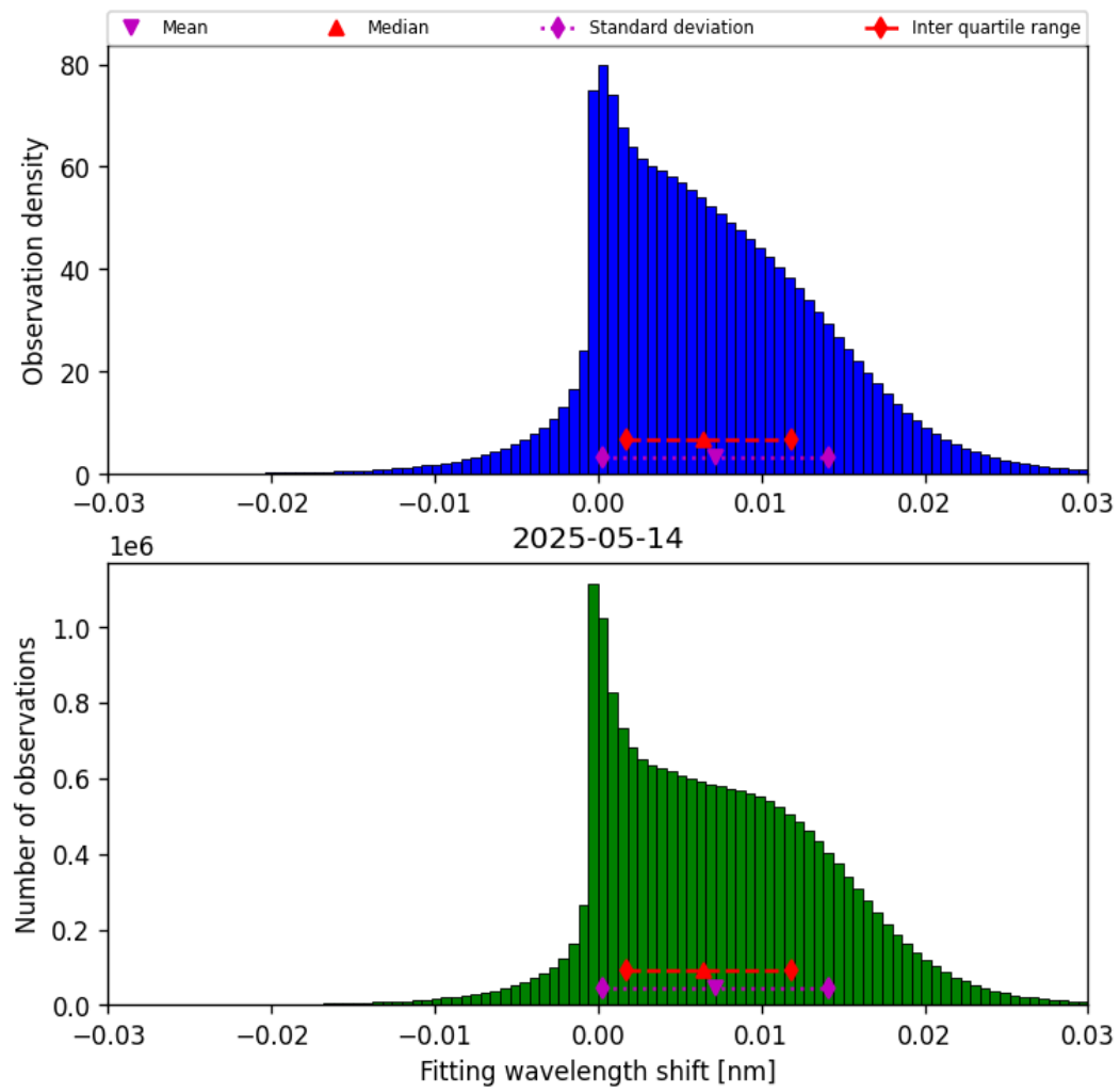
Figure 47: Histogram of “Fitting wavelength shift” for 2025-05-14 to 2025-05-15
