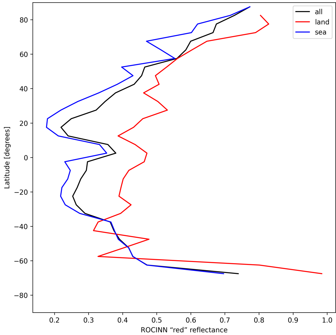
Figure 35: Zonal average of “ROCINN “red” reflectance” for 2025-05-14 to 2025-05-15.
