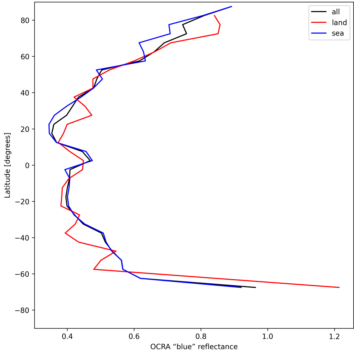
Figure 33: Zonal average of “OCRA “blue” reflectance” for 2025-05-14 to 2025-05-15.
