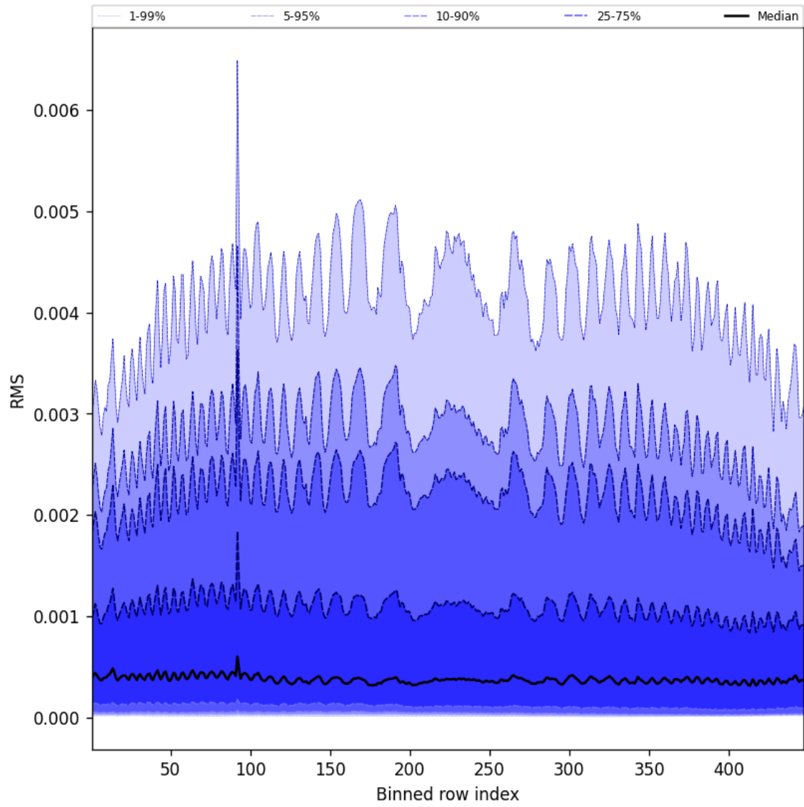
Figure 61: Along track statistics of “RMS” for 2025-05-14 to 2025-05-15
