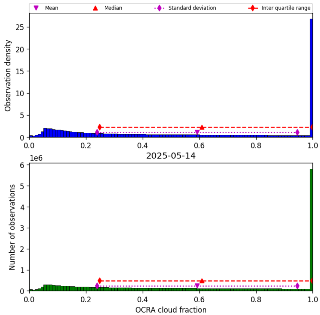
Figure 48: Histogram of “OCRA cloud fraction” for 2025-05-14 to 2025-05-15
