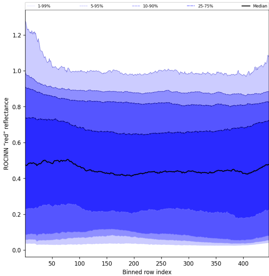
Figure 67: Along track statistics of "ROCINN "red" reflectance" for 2025-05-14 to 2025-05-15
