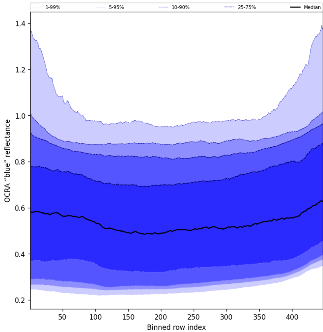
Figure 65: Along track statistics of “OCRA “blue” reflectance” for 2025-05-14 to 2025-05-15
