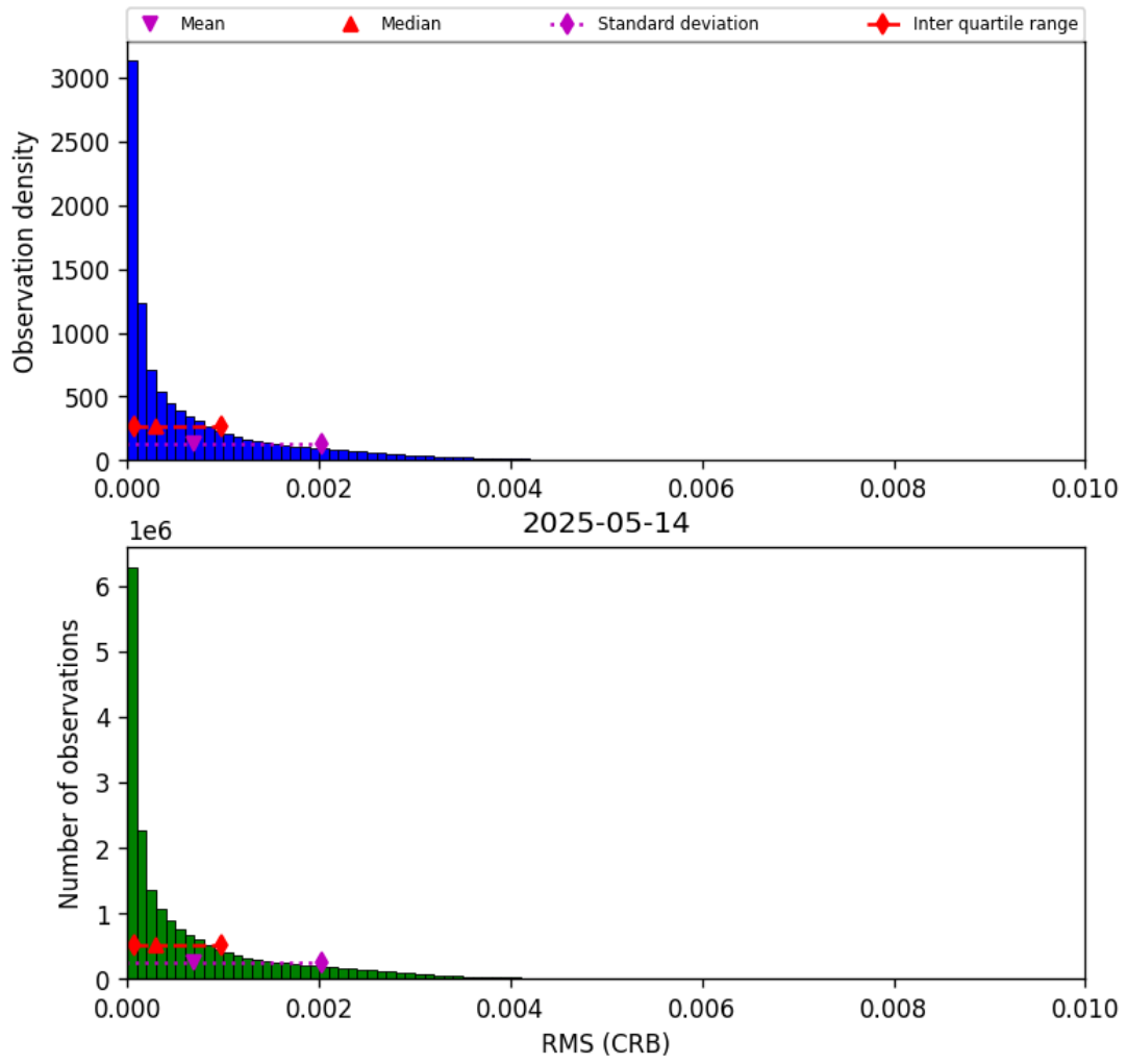
Figure 46: Histogram of "RMS (CRB)" for 2025-05-14 to 2025-05-15
