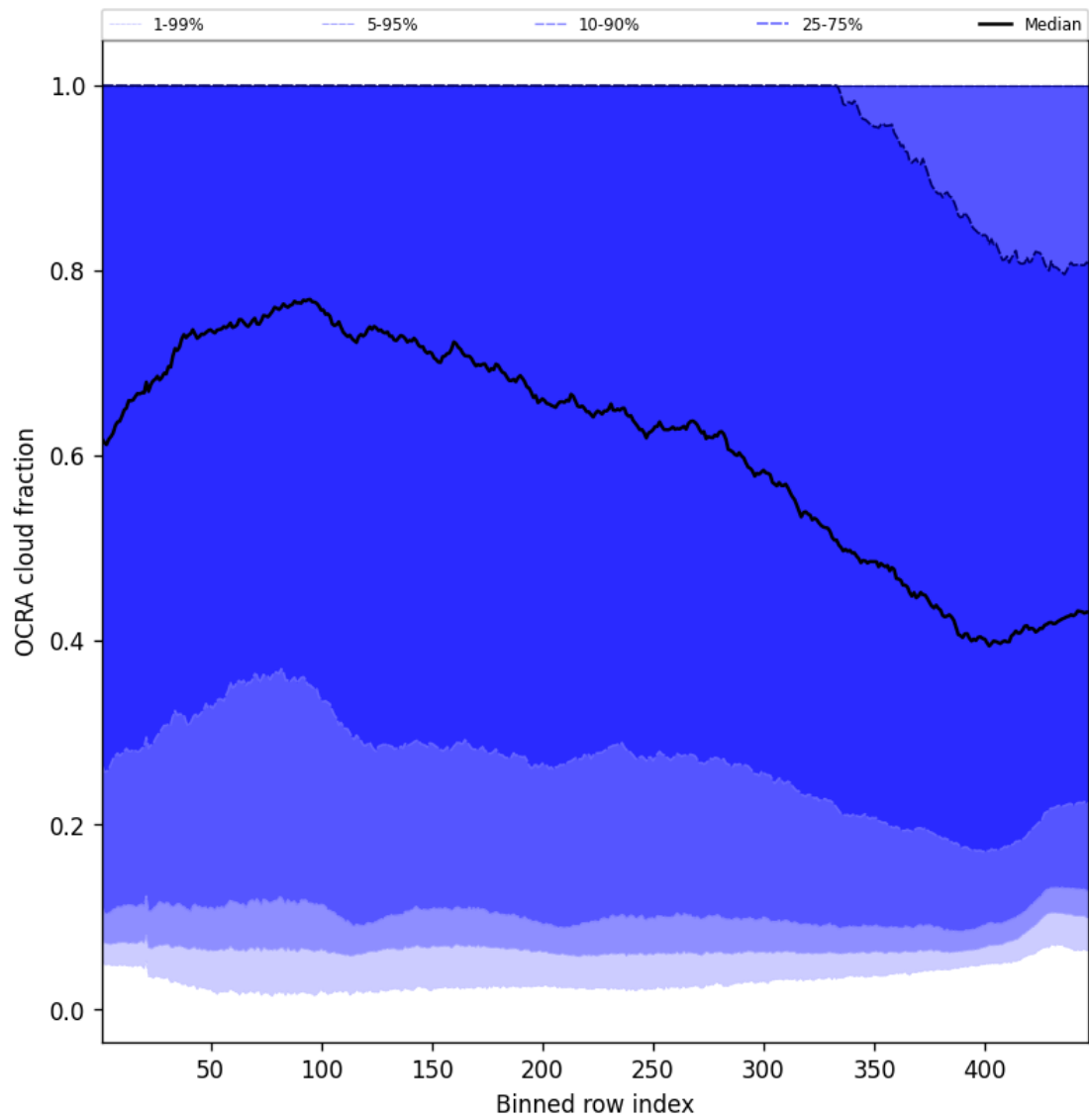
Figure 64: Along track statistics of “OCRA cloud fraction” for 2025-05-14 to 2025-05-15
