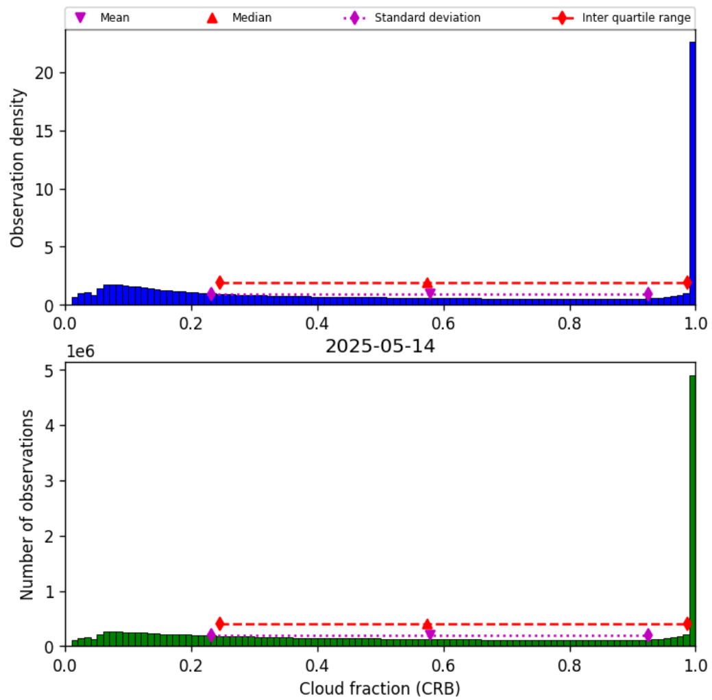
Figure 40: Histogram of “Cloud fraction (CRB)” for 2025-05-14 to 2025-05-15
