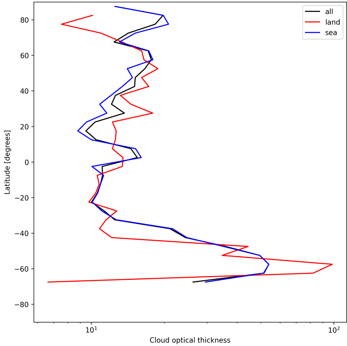
Figure 23: Zonal average of “Cloud optical thickness” for 2025-05-14 to 2025-05-15.
