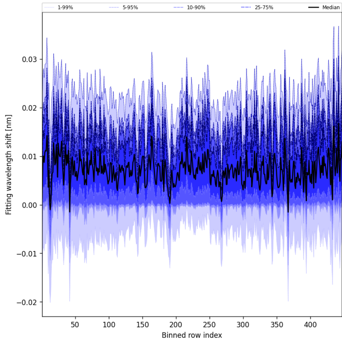
Figure 63: Along track statistics of “Fitting wavelength shift” for 2025-05-14 to 2025-05-15
