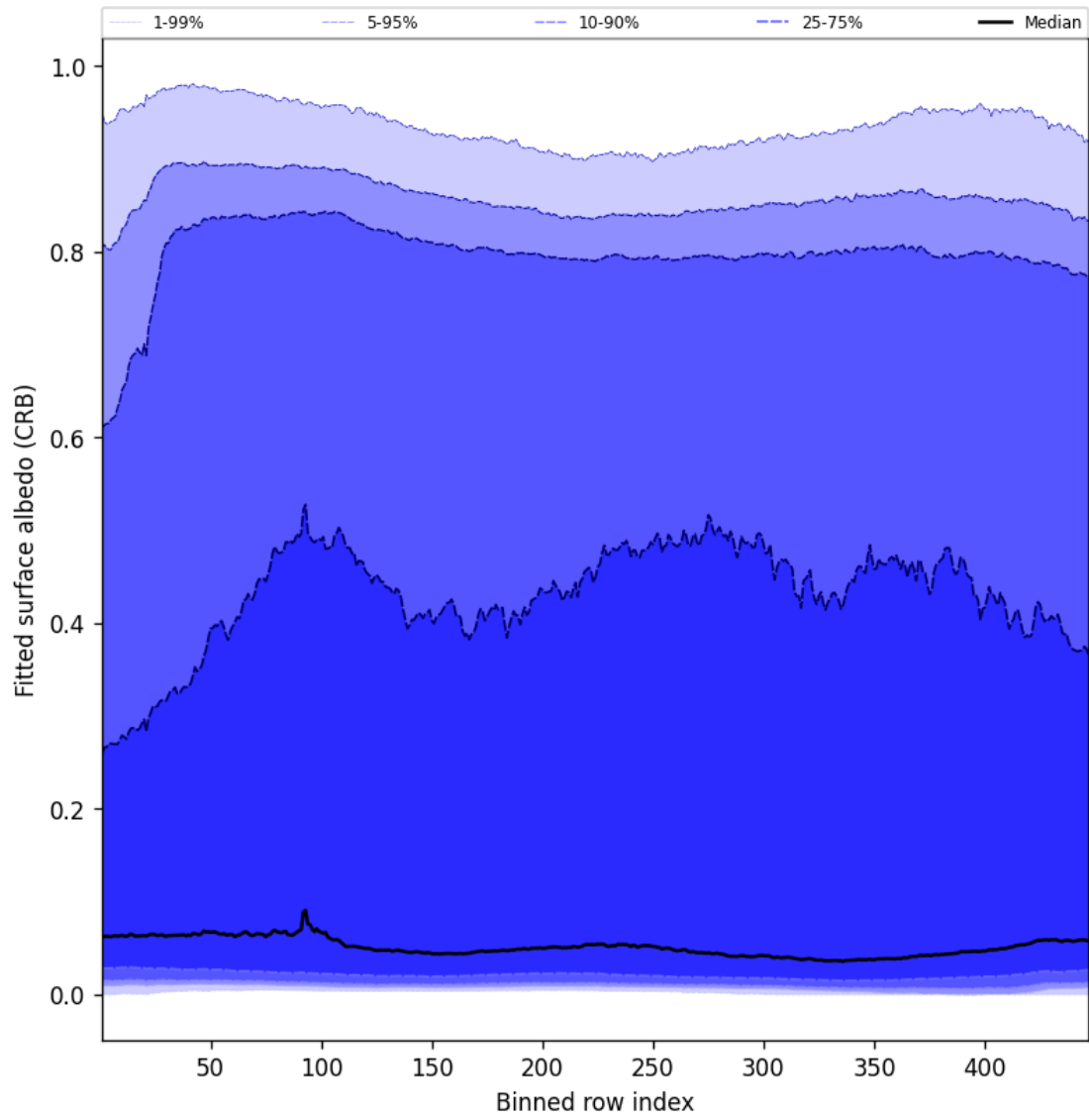
Figure 60: Along track statistics of “Fitted surface albedo (CRB)” for 2025-05-15 to 2025-05-16
