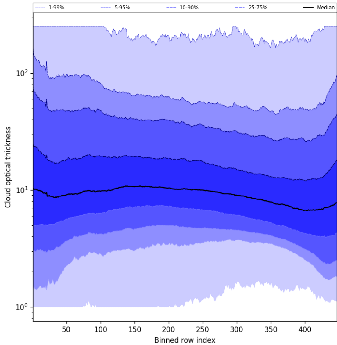
Figure 55: Along track statistics of “Cloud optical thickness” for 2025-05-15 to 2025-05-16
