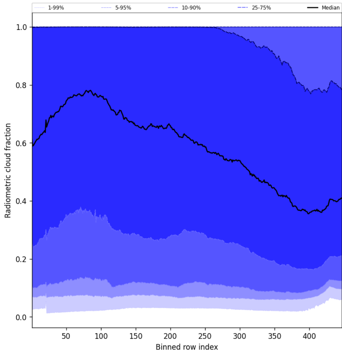
Figure 53: Along track statistics of “Radiometric cloud fraction” for 2025-05-15 to 2025-05-16
