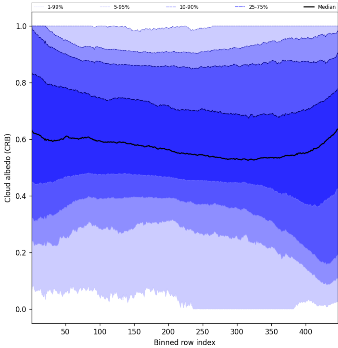
Figure 58: Along track statistics of “Cloud albedo (CRB)” for 2025-05-15 to 2025-05-16
