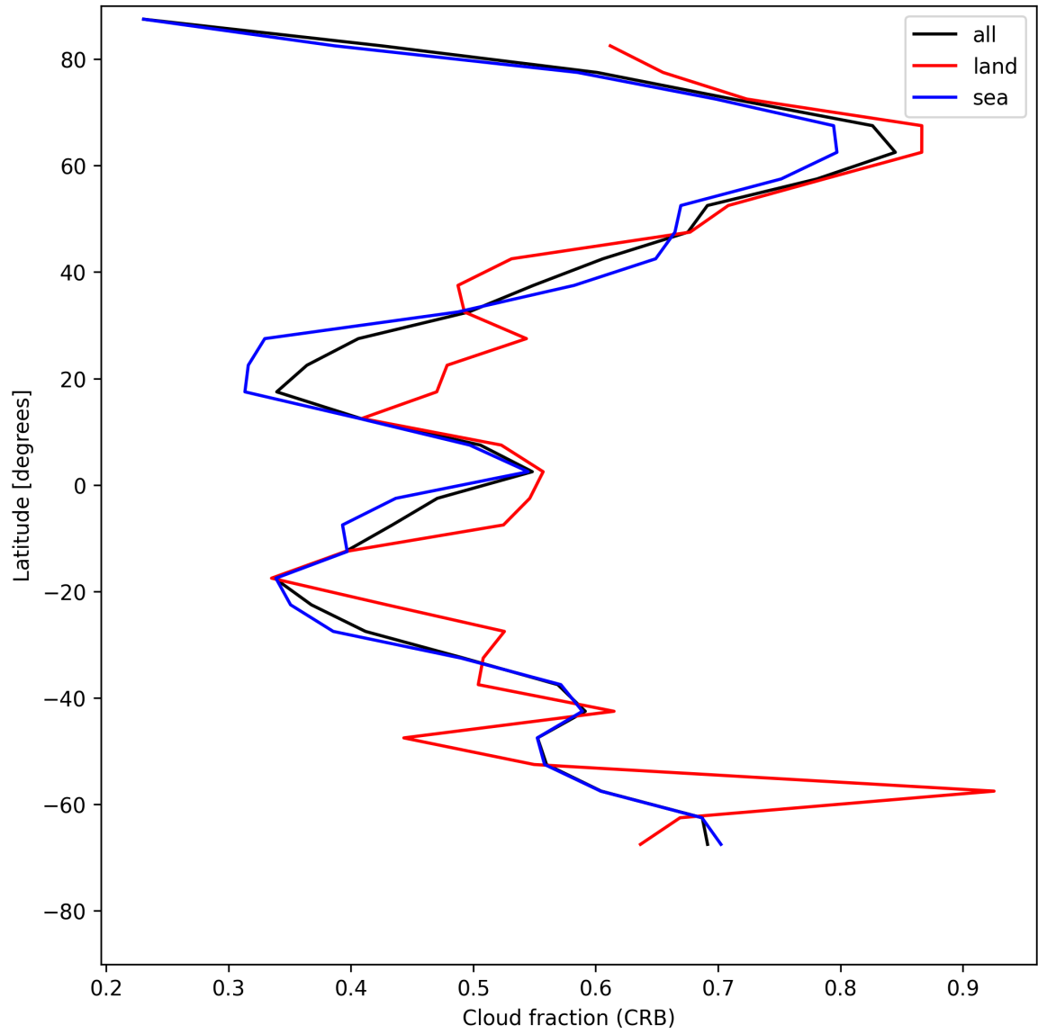
Figure 24: Zonal average of “Cloud fraction (CRB)” for 2025-05-15 to 2025-05-16.
