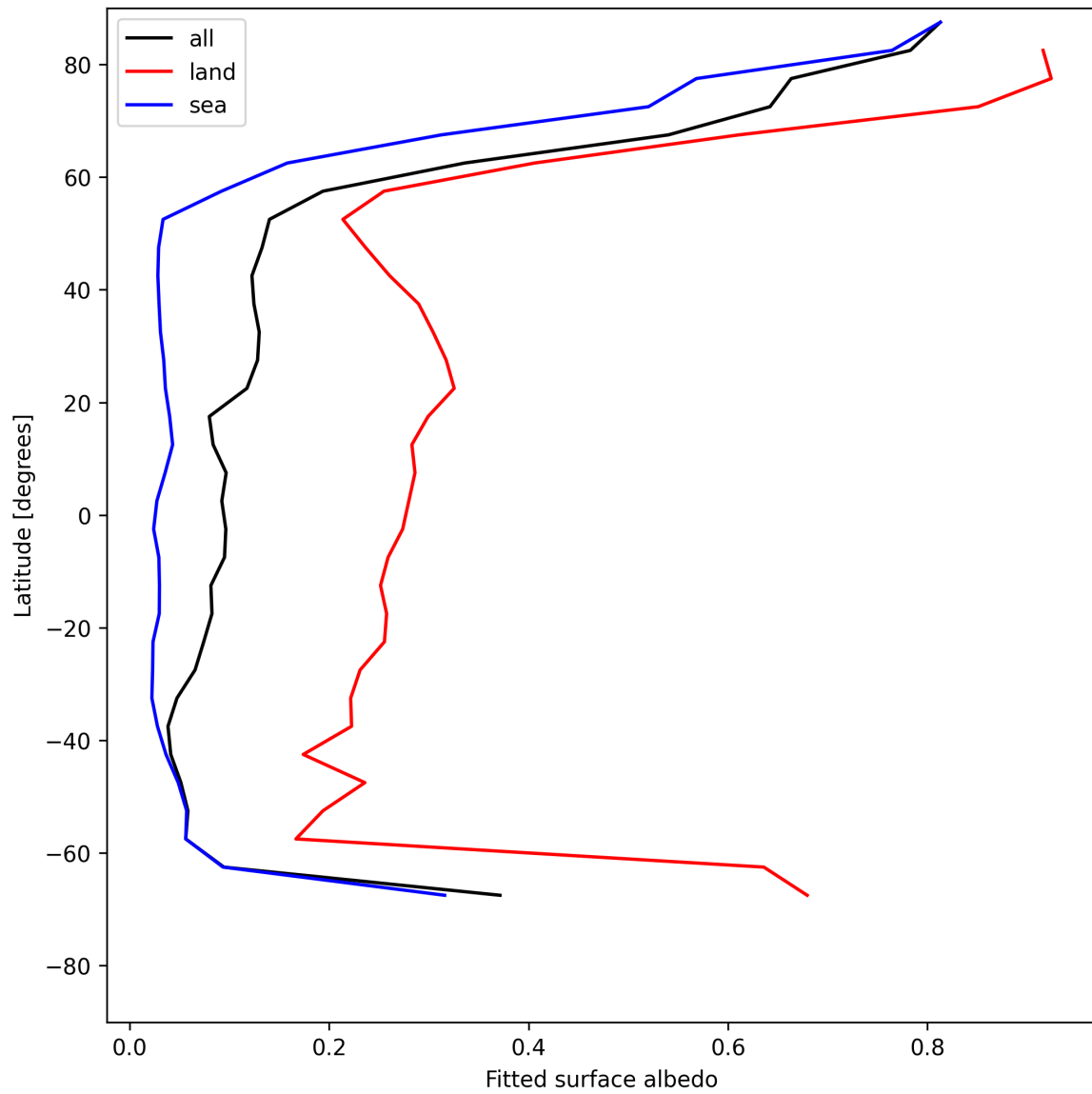
Figure 27: Zonal average of “Fitted surface albedo” for 2025-05-15 to 2025-05-16.
