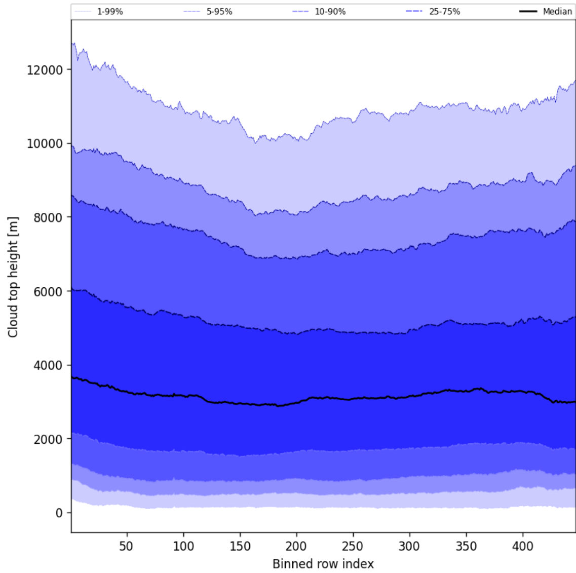
Figure 54: Along track statistics of “Cloud top height” for 2025-05-15 to 2025-05-16
