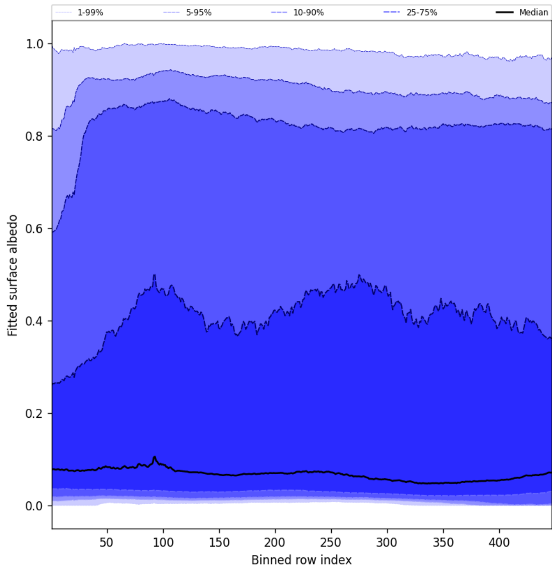
Figure 59: Along track statistics of “Fitted surface albedo” for 2025-05-15 to 2025-05-16
