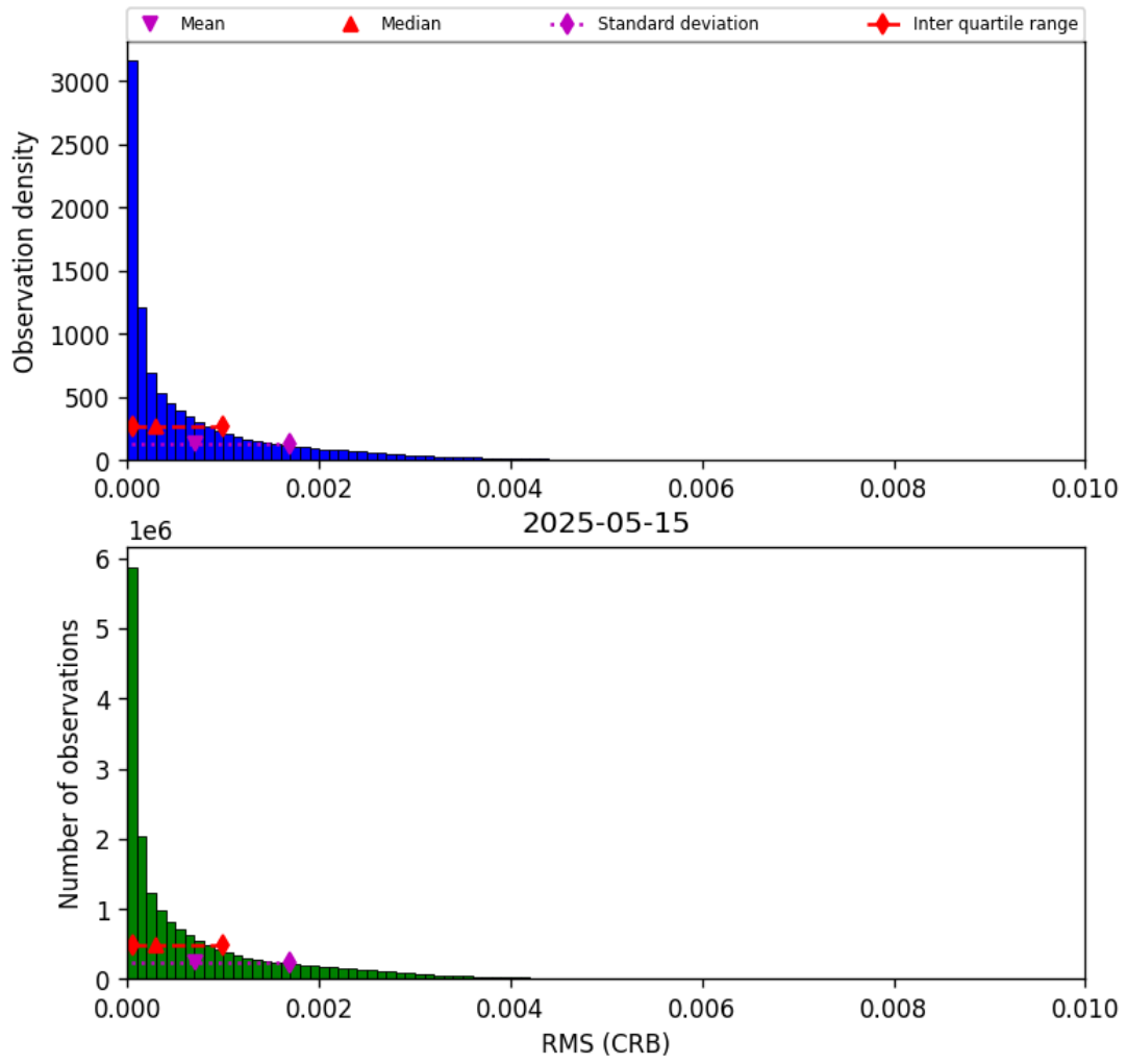
Figure 46: Histogram of “RMS (CRB)” for 2025-05-15 to 2025-05-16
