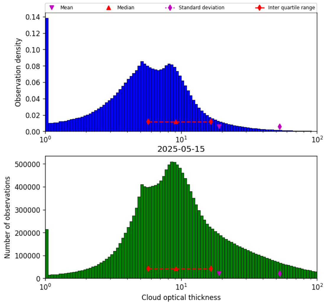
Figure 39: Histogram of “Cloud optical thickness” for 2025-05-15 to 2025-05-16
