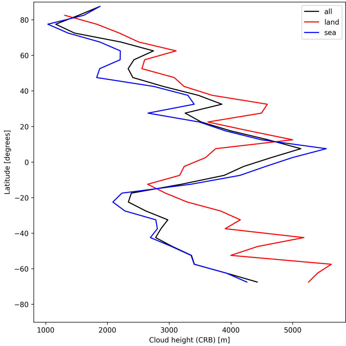
Figure 25: Zonal average of “Cloud height (CRB)” for 2025-05-15 to 2025-05-16.
