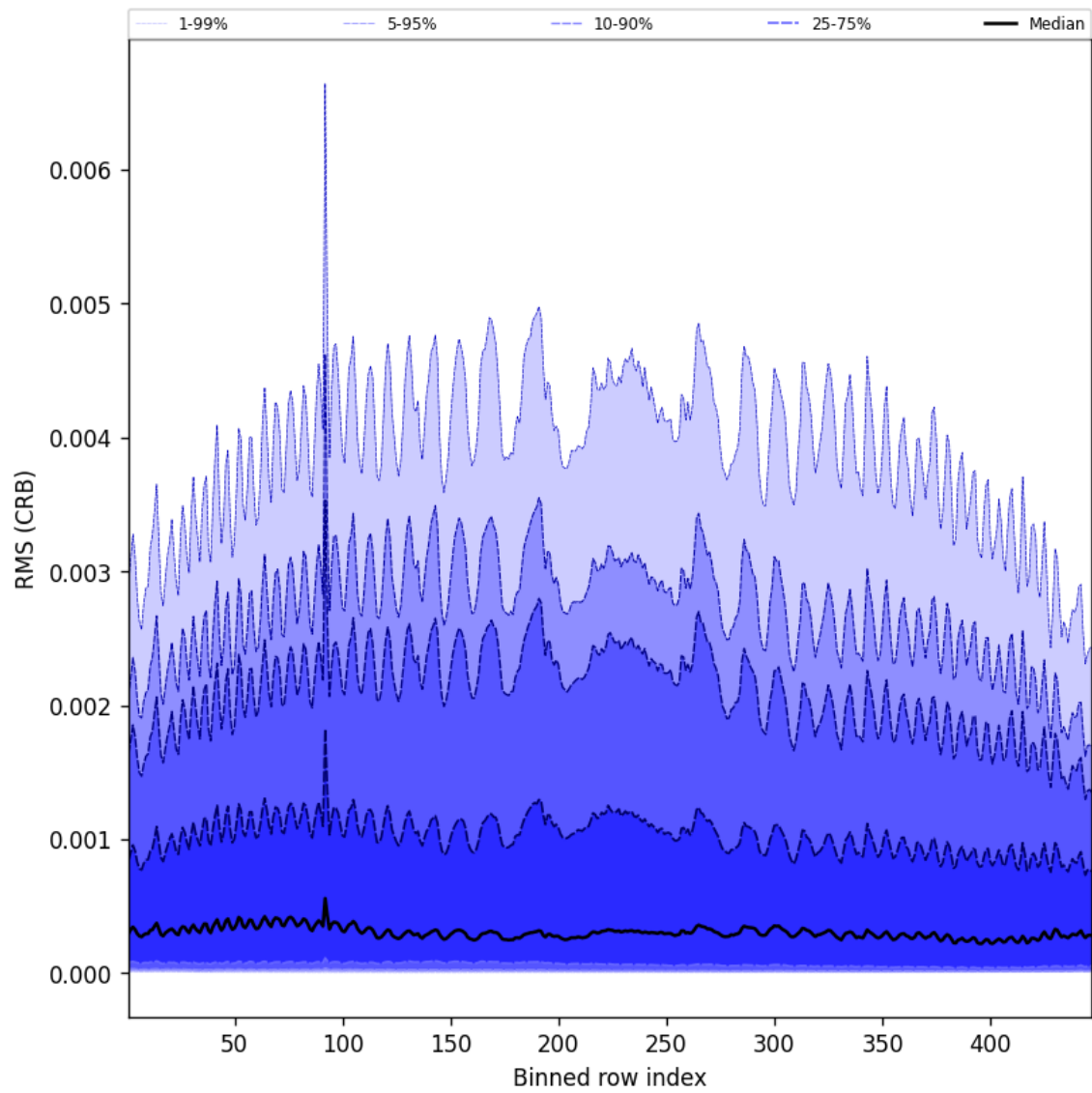
Figure 62: Along track statistics of “RMS (CRB)” for 2025-05-15 to 2025-05-16
