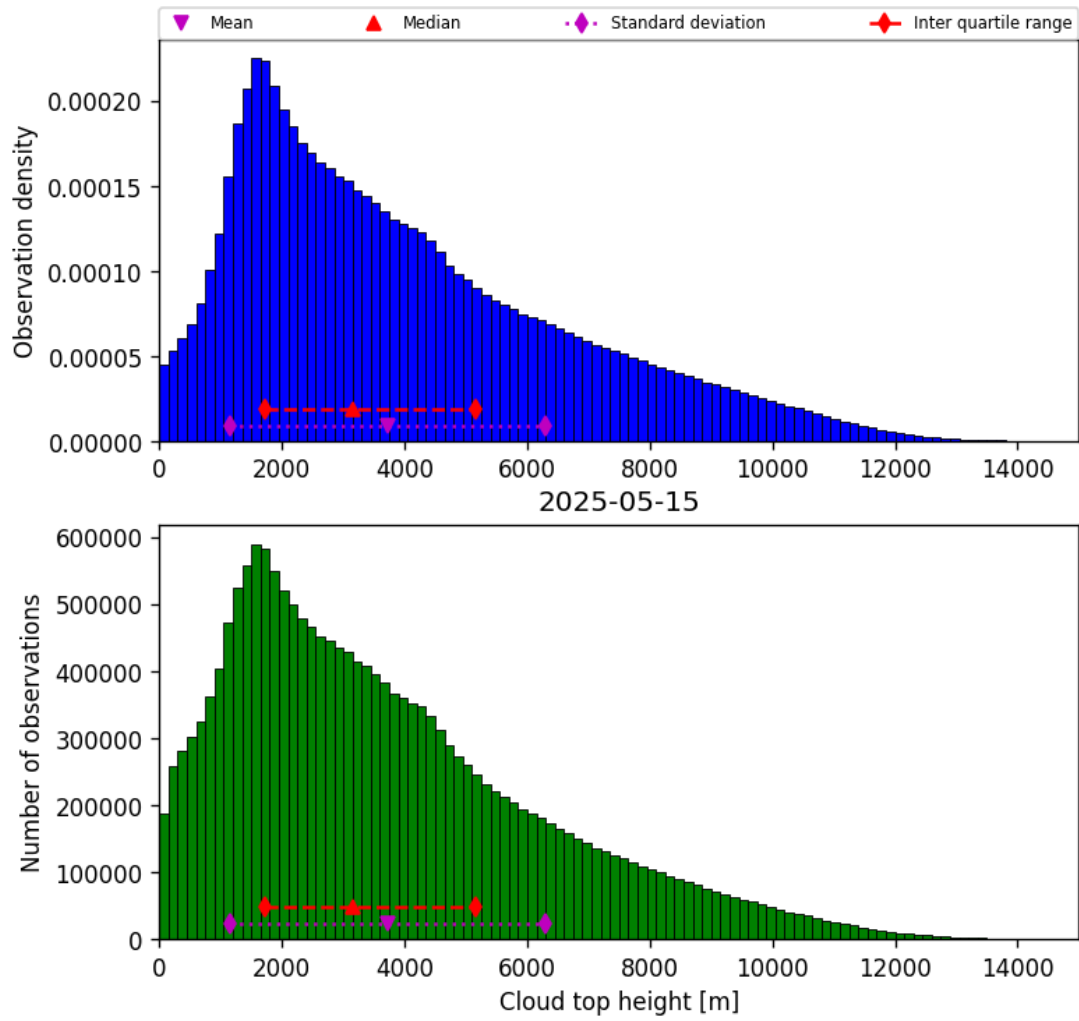
Figure 38: Histogram of “Cloud top height” for 2025-05-15 to 2025-05-16
