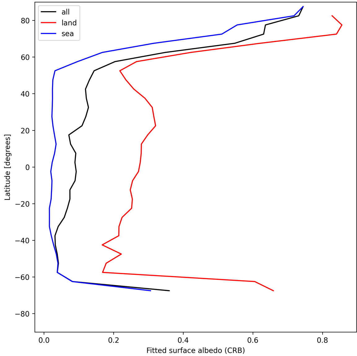
Figure 28: Zonal average of “Fitted surface albedo (CRB)” for 2025-05-15 to 2025-05-16.
