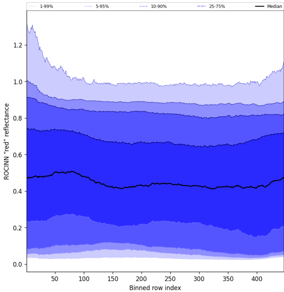
Figure 67: Along track statistics of "ROCINN "red" reflectance" for 2025-05-15 to 2025-05-16
