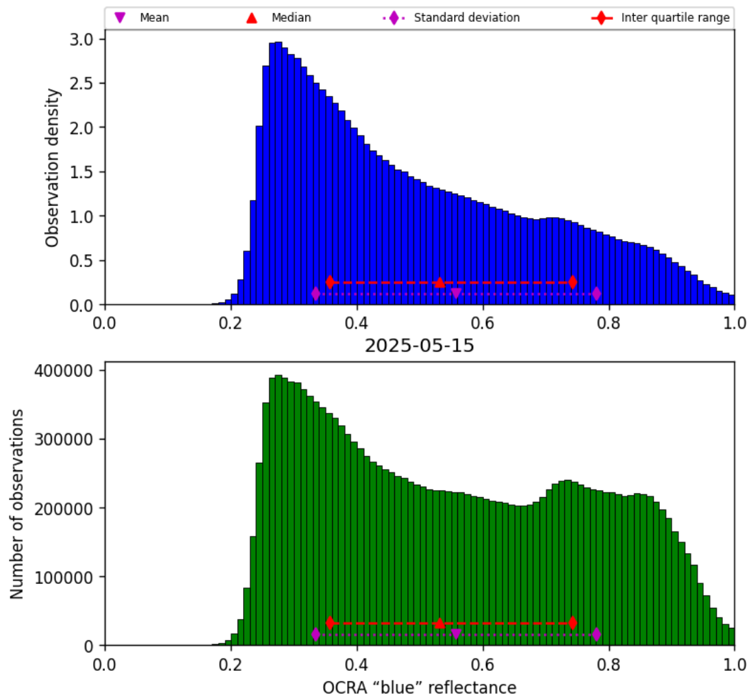
Figure 49: Histogram of “OCRA “blue” reflectance” for 2025-05-15 to 2025-05-16
