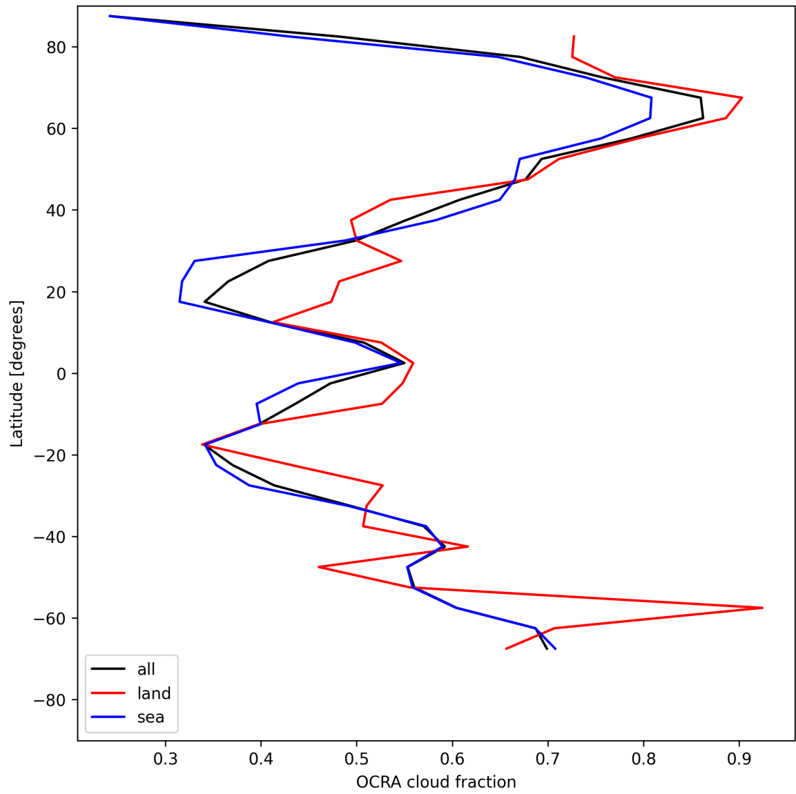
Figure 32: Zonal average of “OCRA cloud fraction” for 2025-05-15 to 2025-05-16.
