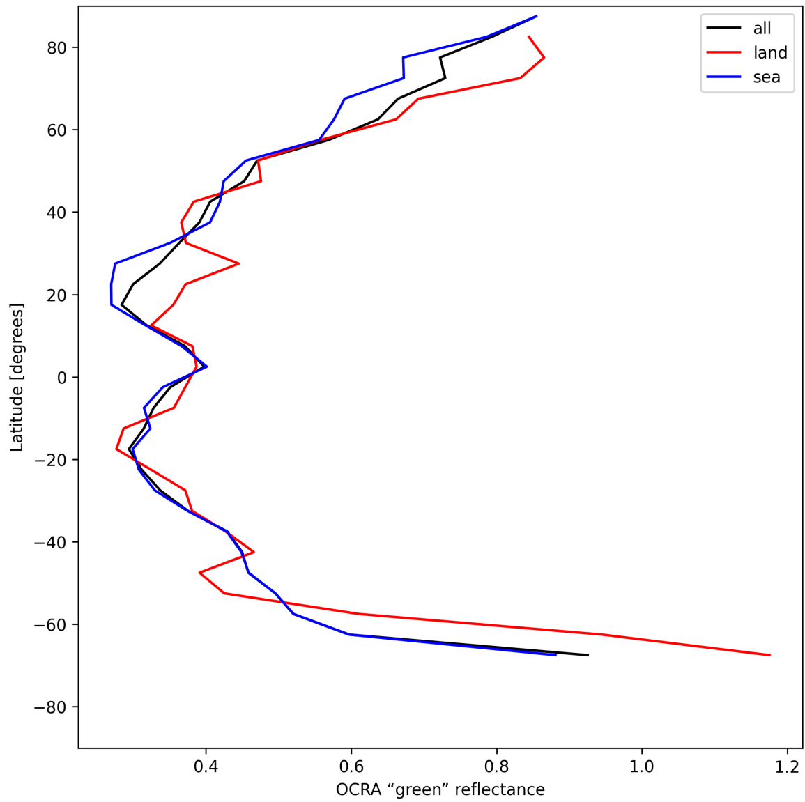
Figure 34: Zonal average of “OCRA “green” reflectance” for 2025-05-15 to 2025-05-16.
