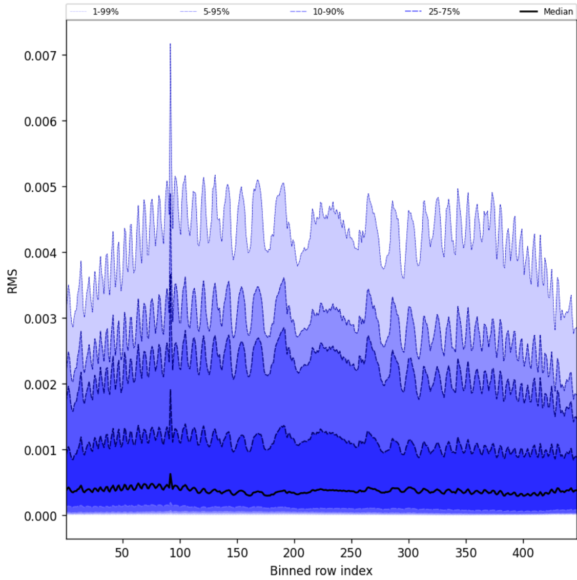
Figure 61: Along track statistics of “RMS” for 2025-05-15 to 2025-05-16
