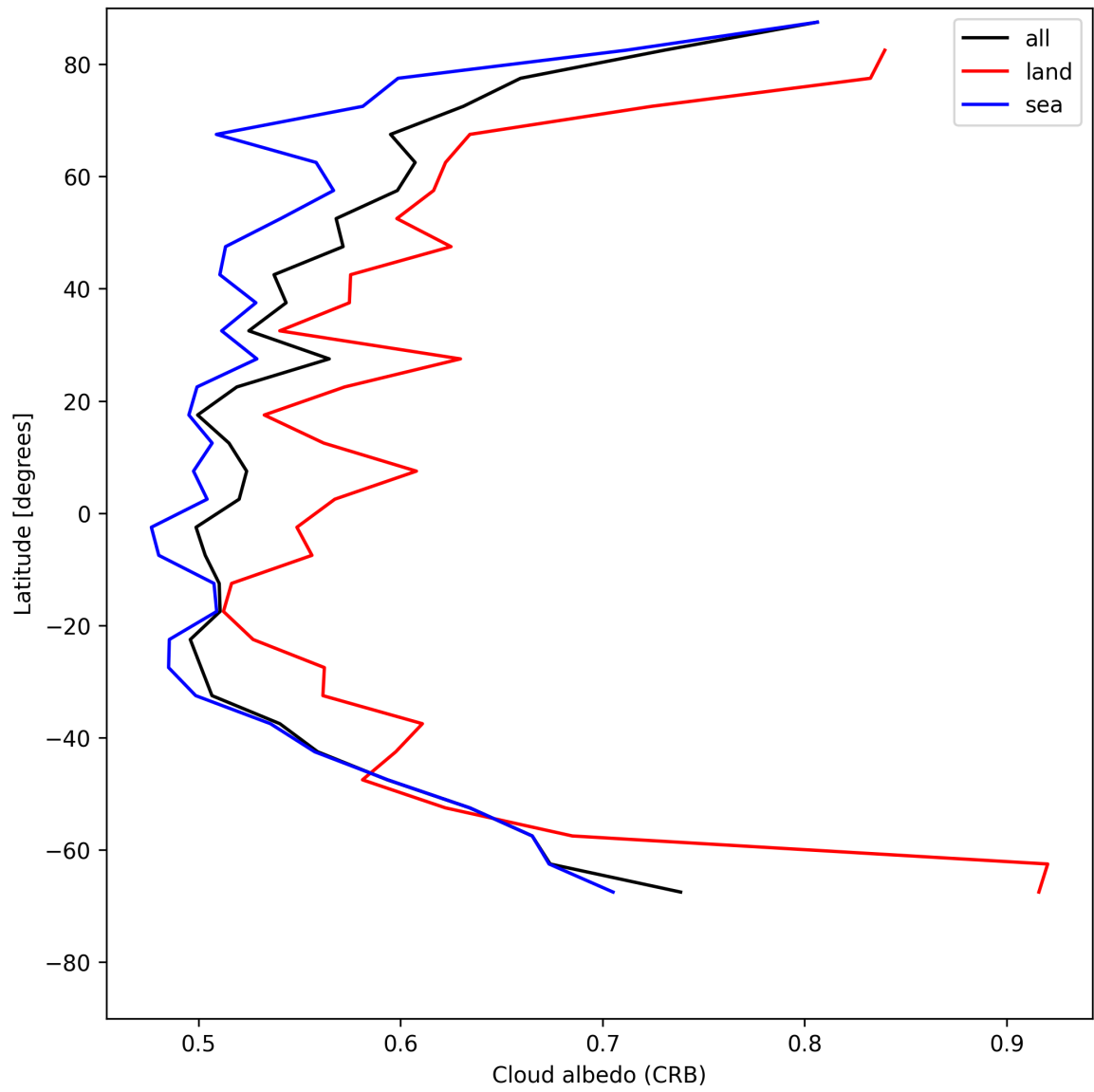
Figure 26: Zonal average of “Cloud albedo (CRB)” for 2025-05-15 to 2025-05-16.
