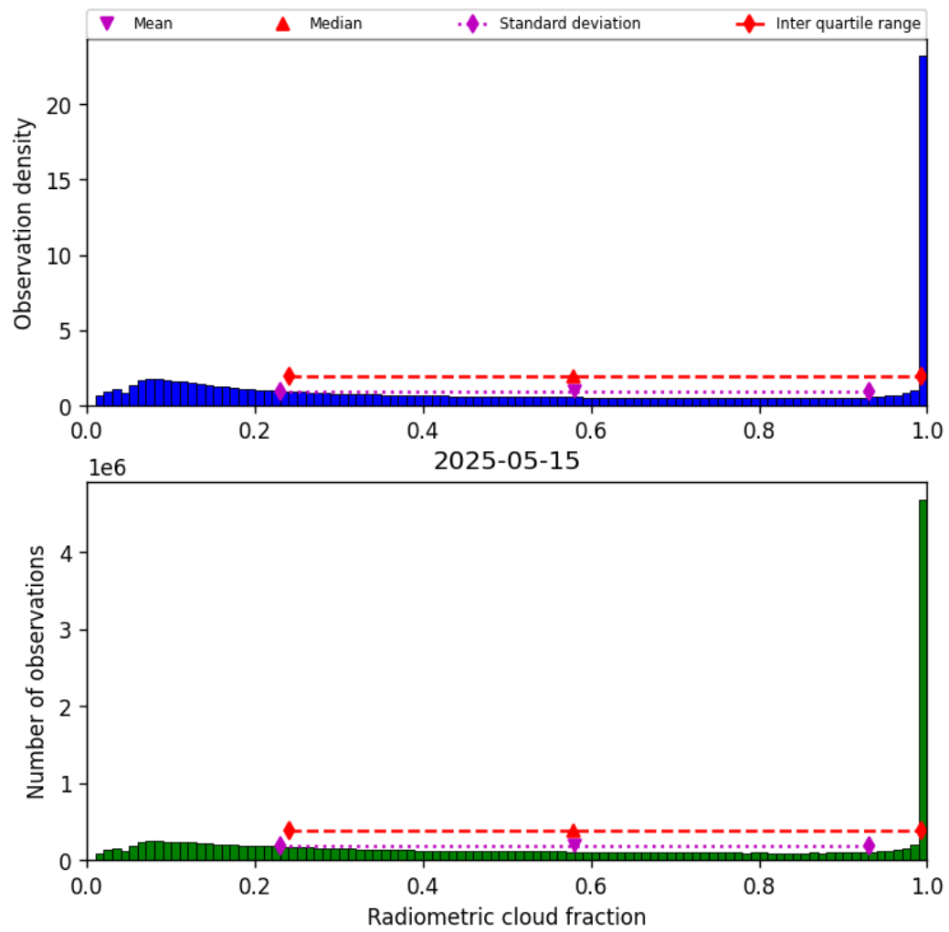
Figure 37: Histogram of “Radiometric cloud fraction” for 2025-05-15 to 2025-05-16
