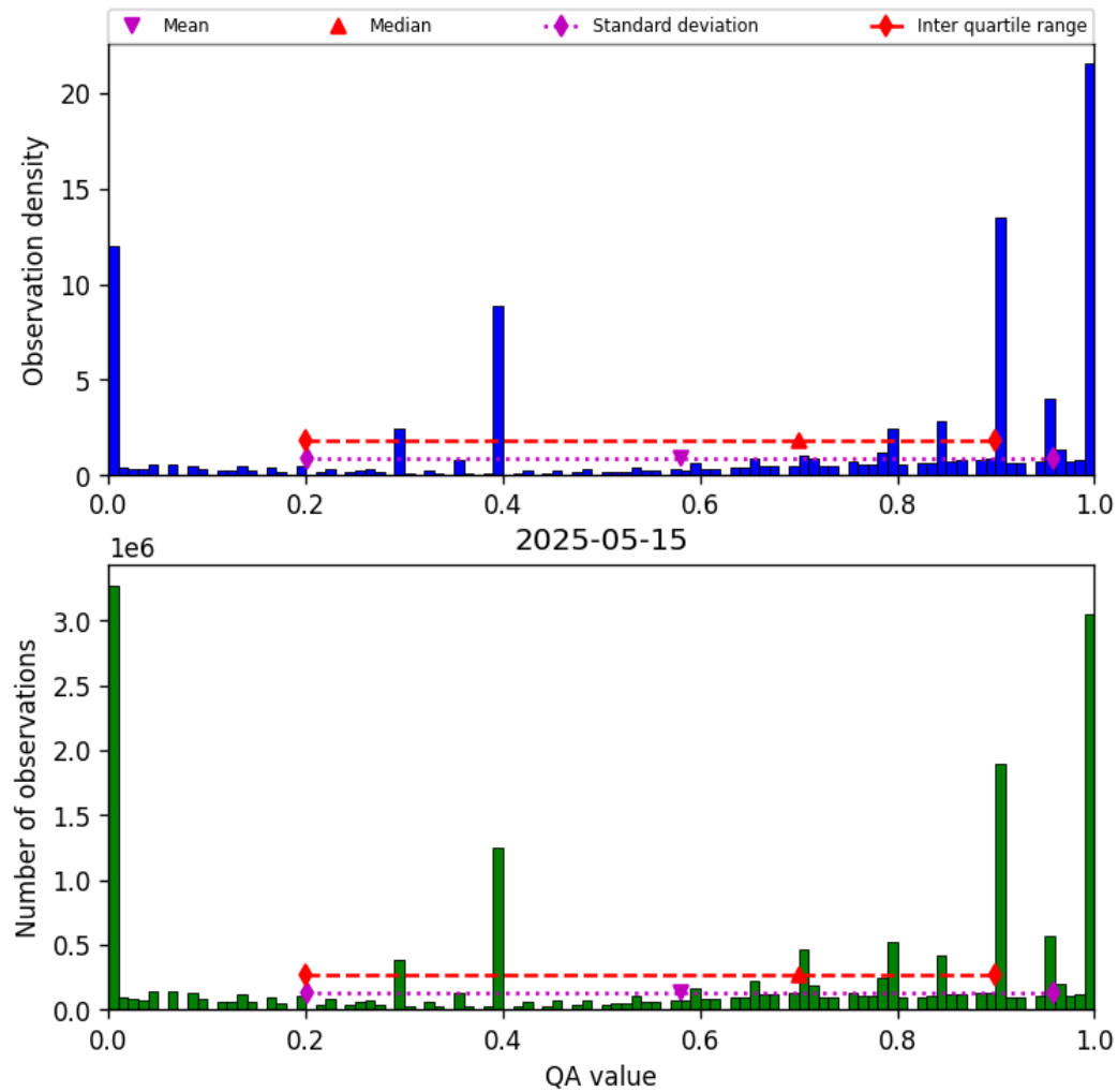
Figure 36: Histogram of “QA value” for 2025-05-15 to 2025-05-16
