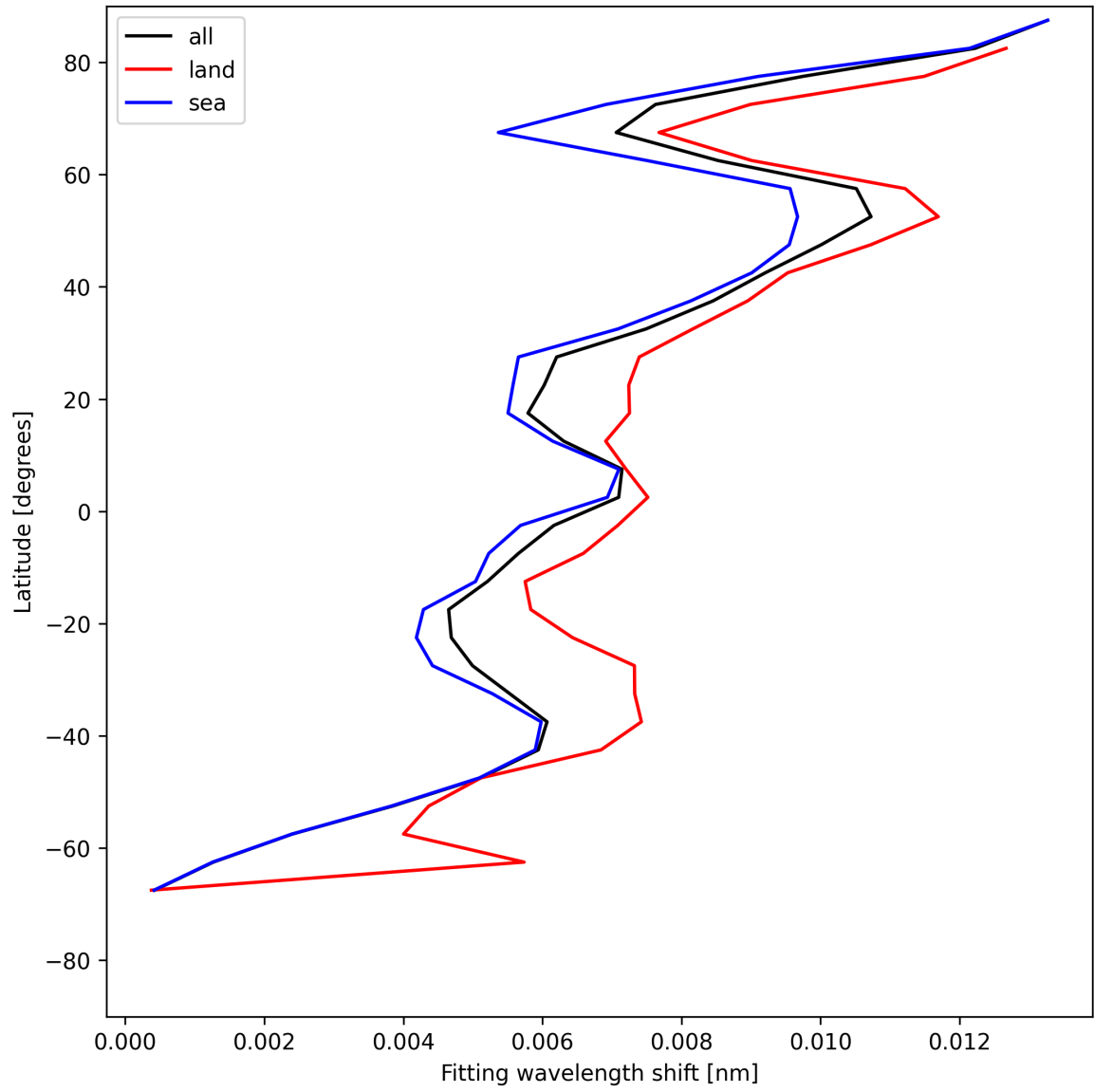
Figure 31: Zonal average of “Fitting wavelength shift” for 2025-05-15 to 2025-05-16.
