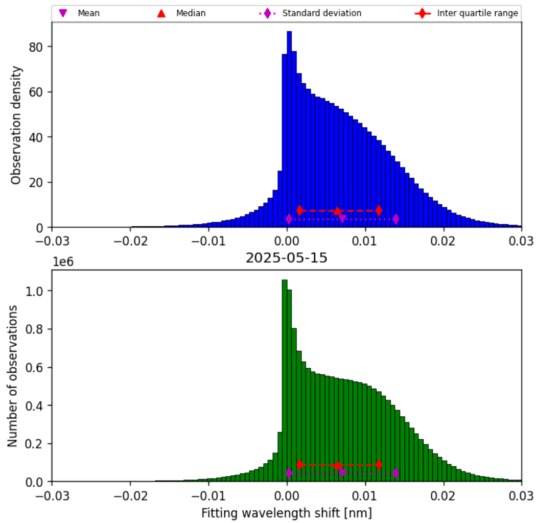
Figure 47: Histogram of “Fitting wavelength shift” for 2025-05-15 to 2025-05-16
