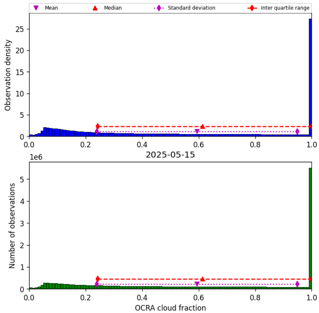
Figure 48: Histogram of “OCRA cloud fraction” for 2025-05-15 to 2025-05-16
