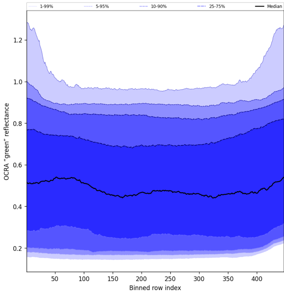
Figure 66: Along track statistics of “OCRA “green” reflectance” for 2025-05-15 to 2025-05-16
