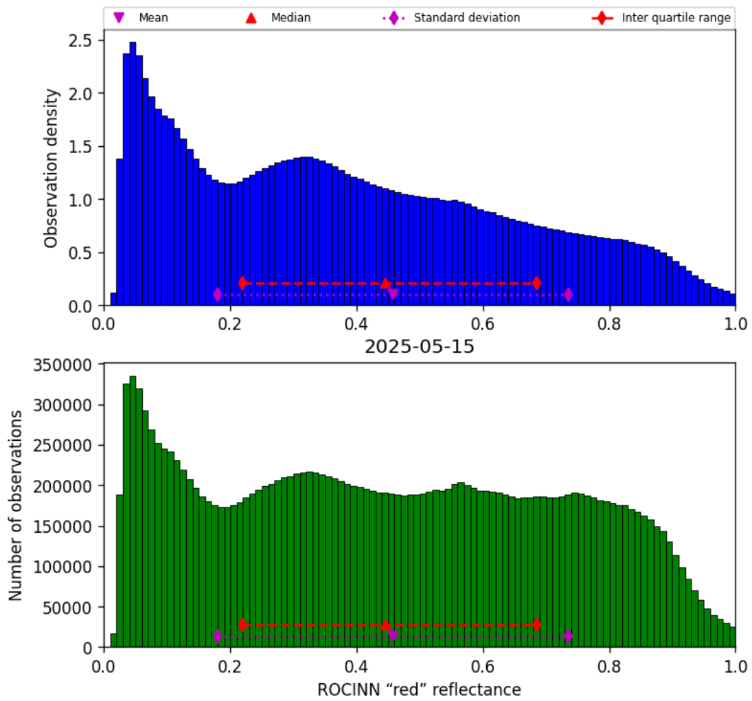
Figure 51: Histogram of “ROCINN “red” reflectance” for 2025-05-15 to 2025-05-16
