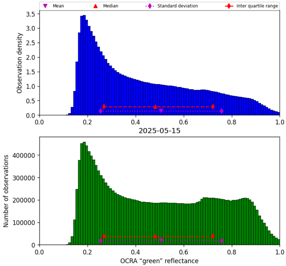
Figure 50: Histogram of “OCRA “green” reflectance” for 2025-05-15 to 2025-05-16
