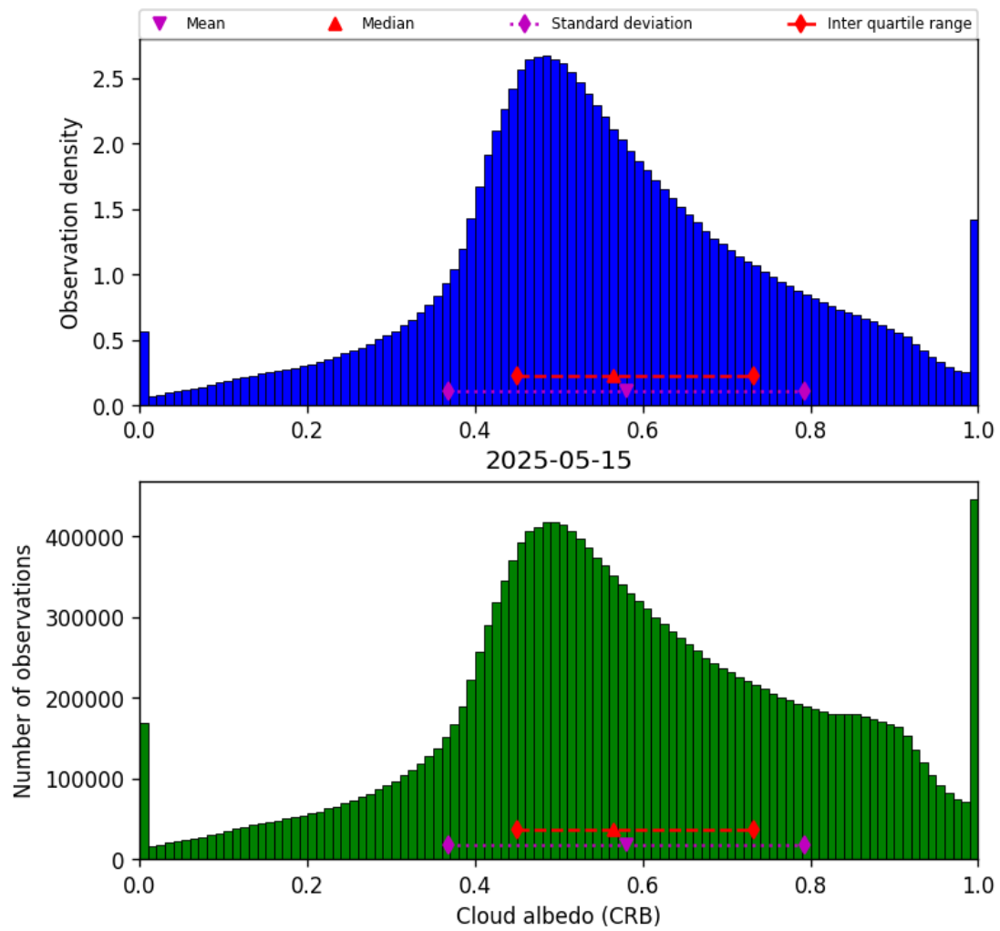
Figure 42: Histogram of “Cloud albedo (CRB)” for 2025-05-15 to 2025-05-16
