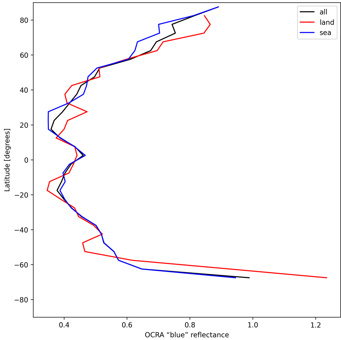
Figure 33: Zonal average of "OCRA "blue" reflectance" for 2025-05-15 to 2025-05-16.
