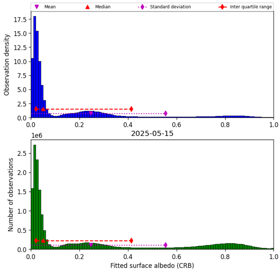
Figure 44: Histogram of “Fitted surface albedo (CRB)” for 2025-05-15 to 2025-05-16
