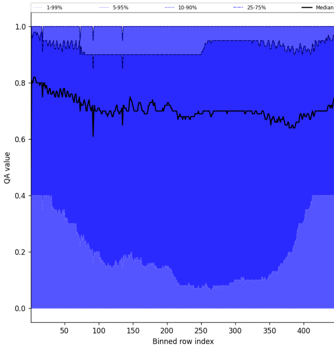
Figure 52: Along track statistics of “QA value” for 2025-05-15 to 2025-05-16
