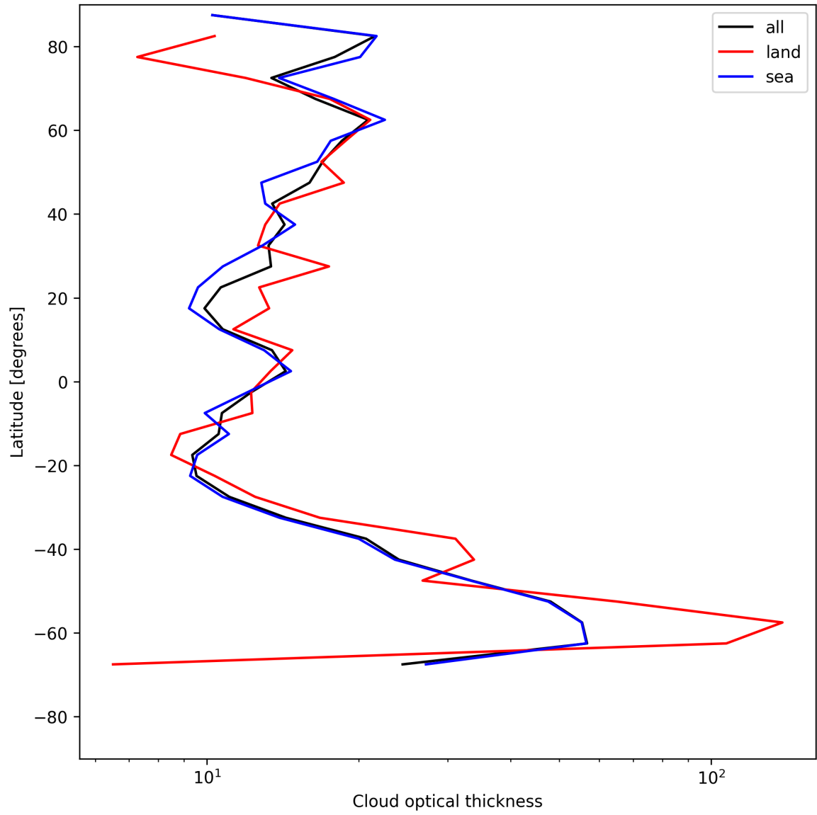
Figure 23: Zonal average of “Cloud optical thickness” for 2025-05-15 to 2025-05-16.
