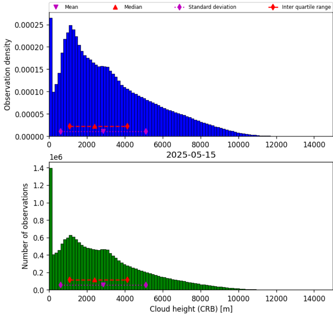
Figure 41: Histogram of “Cloud height (CRB)” for 2025-05-15 to 2025-05-16
