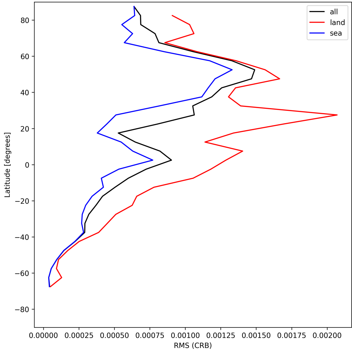
Figure 30: Zonal average of “RMS (CRB)” for 2025-05-15 to 2025-05-16.
