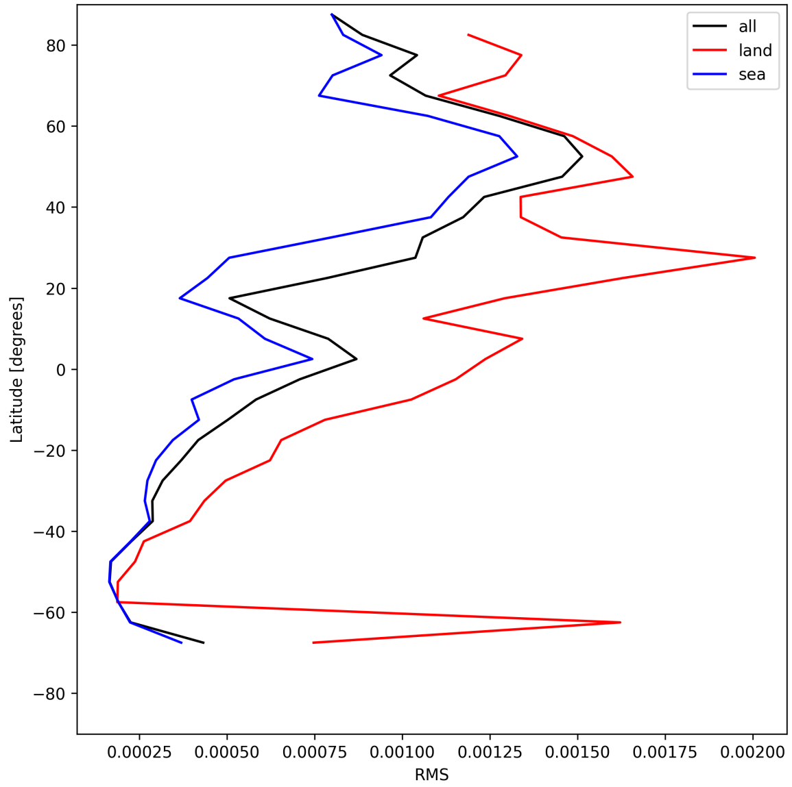
Figure 29: Zonal average of “RMS” for 2025-05-15 to 2025-05-16.
