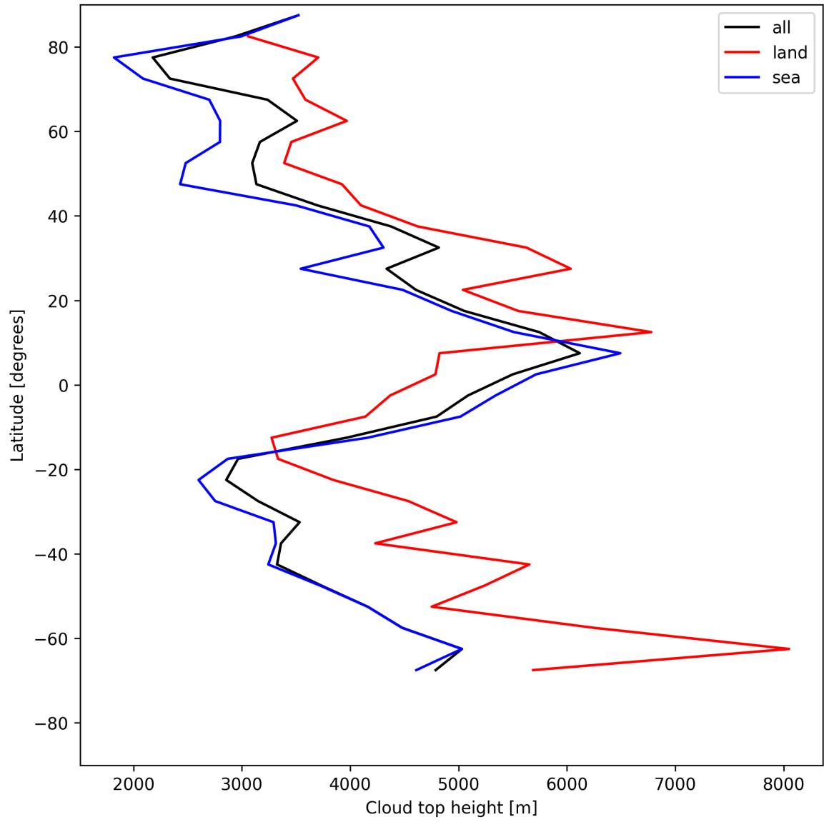
Figure 22: Zonal average of “Cloud top height” for 2025-05-15 to 2025-05-16.
