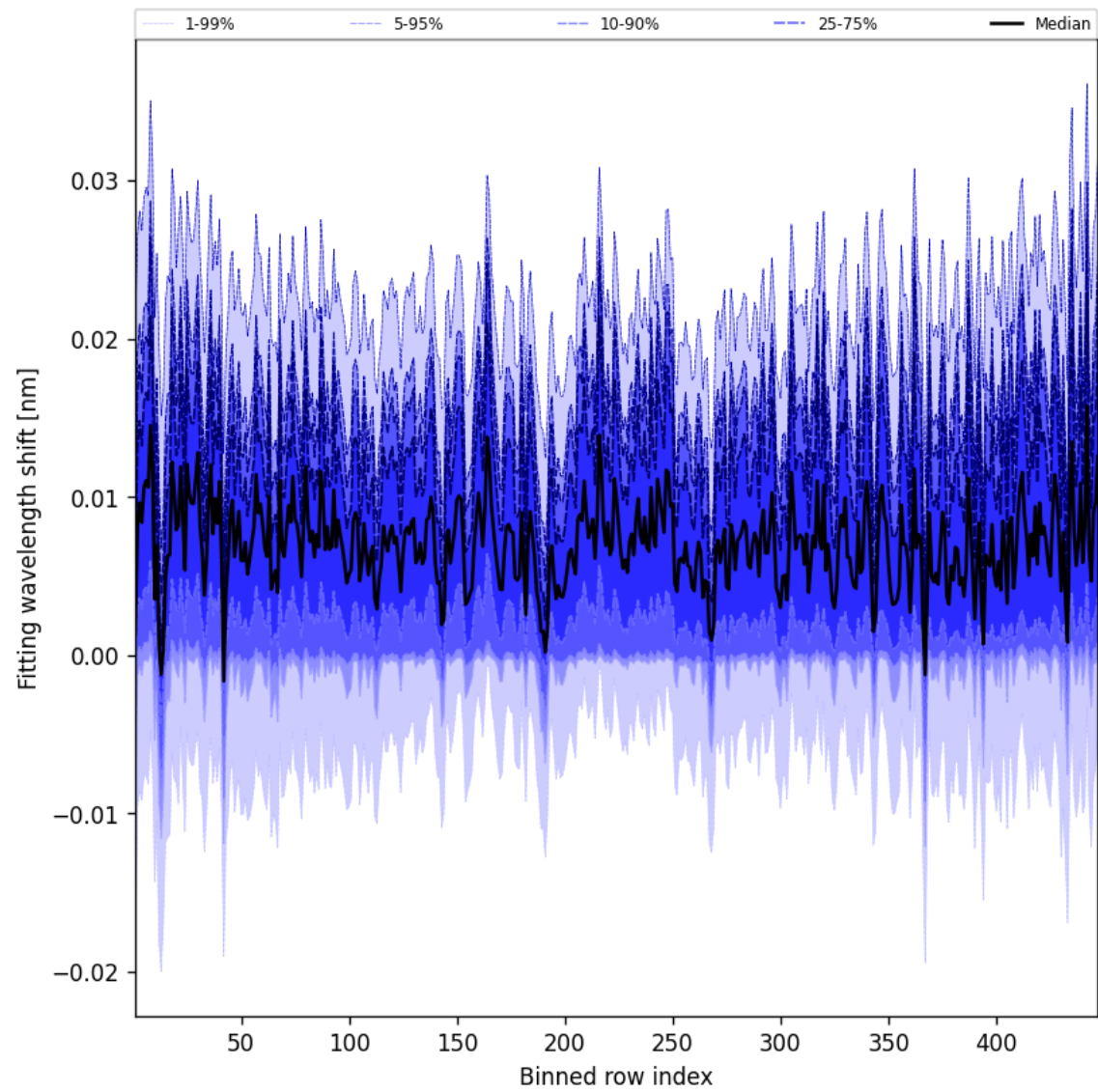
Figure 63: Along track statistics of “Fitting wavelength shift” for 2025-05-15 to 2025-05-16
