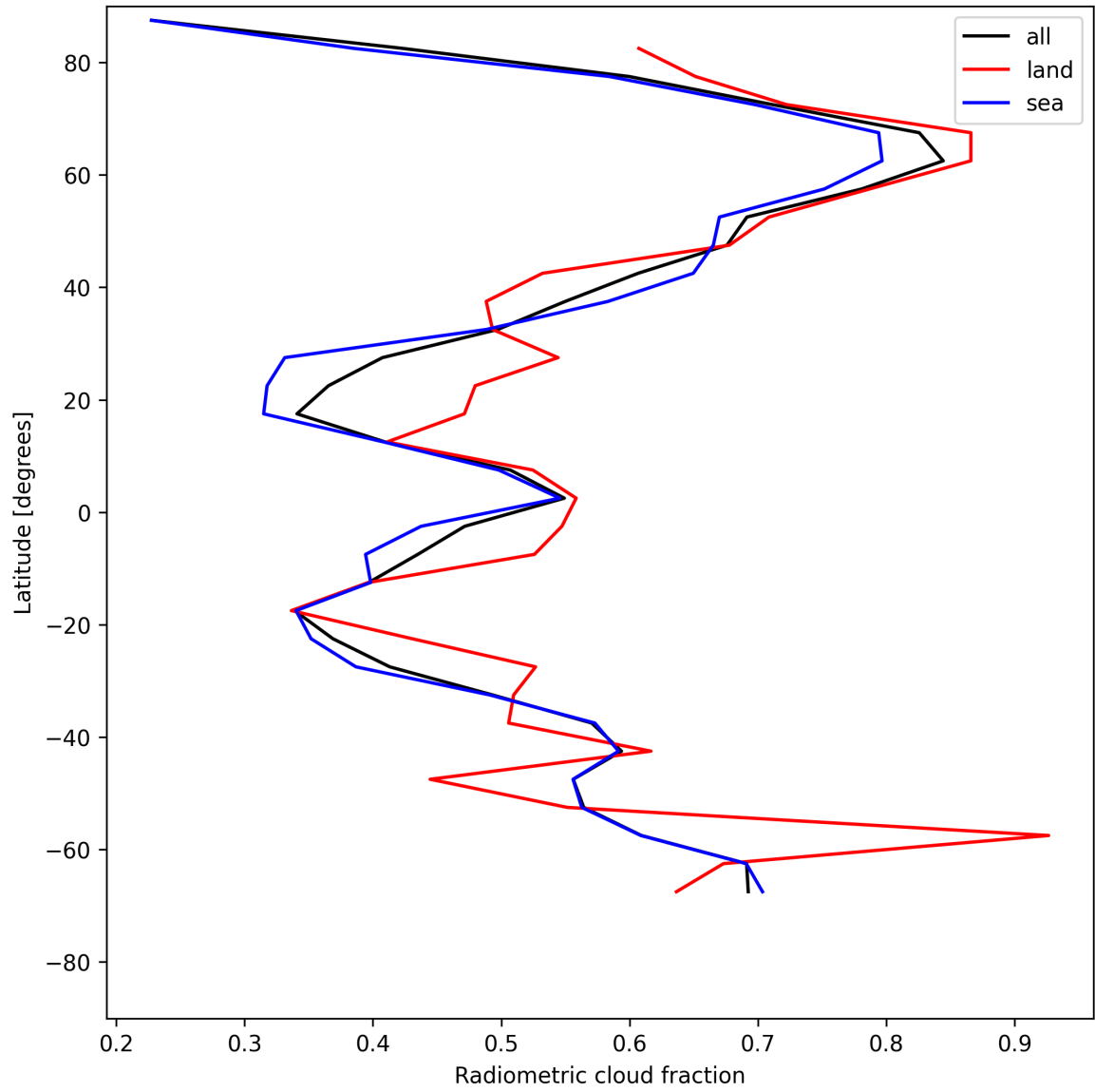
Figure 21: Zonal average of “Radiometric cloud fraction” for 2025-05-15 to 2025-05-16.
