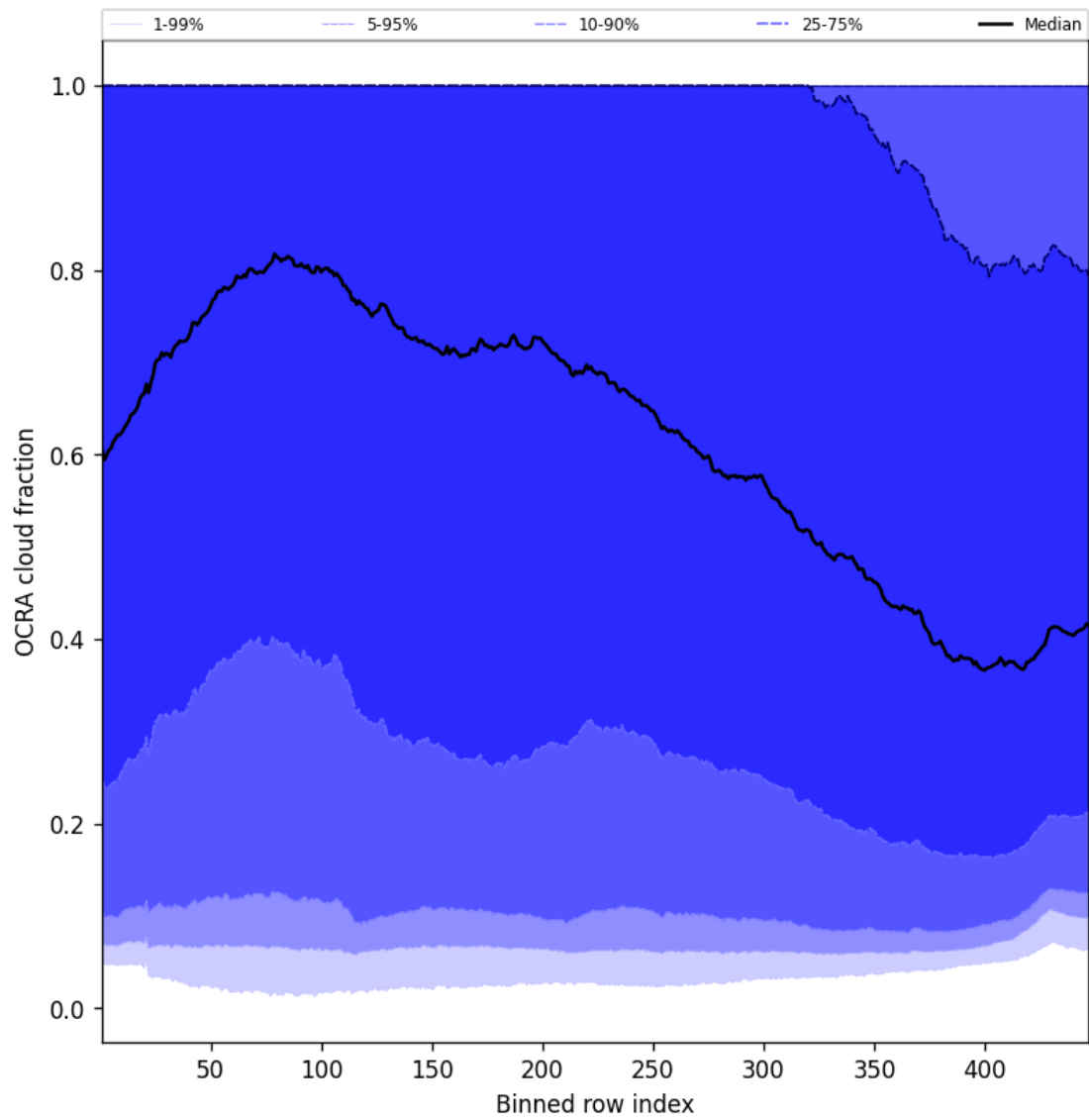
Figure 64: Along track statistics of “OCRA cloud fraction” for 2025-05-15 to 2025-05-16
