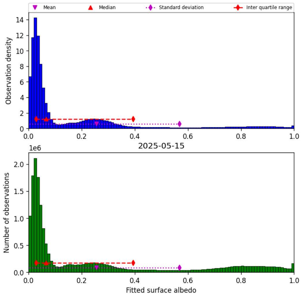
Figure 43: Histogram of “Fitted surface albedo” for 2025-05-15 to 2025-05-16
