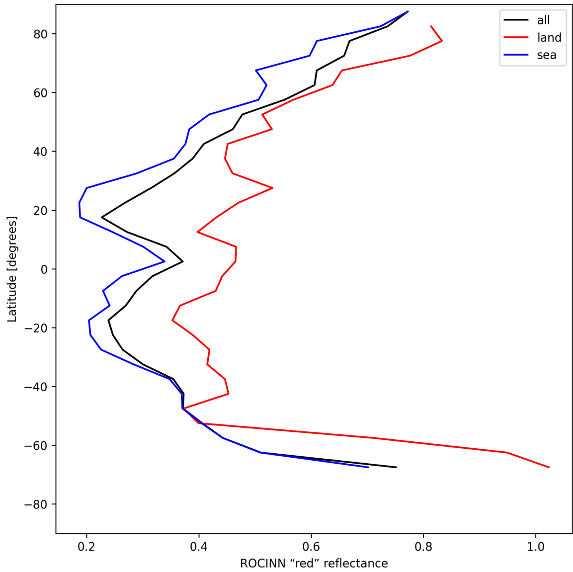
Figure 35: Zonal average of “ROCINN “red” reflectance” for 2025-05-15 to 2025-05-16.
