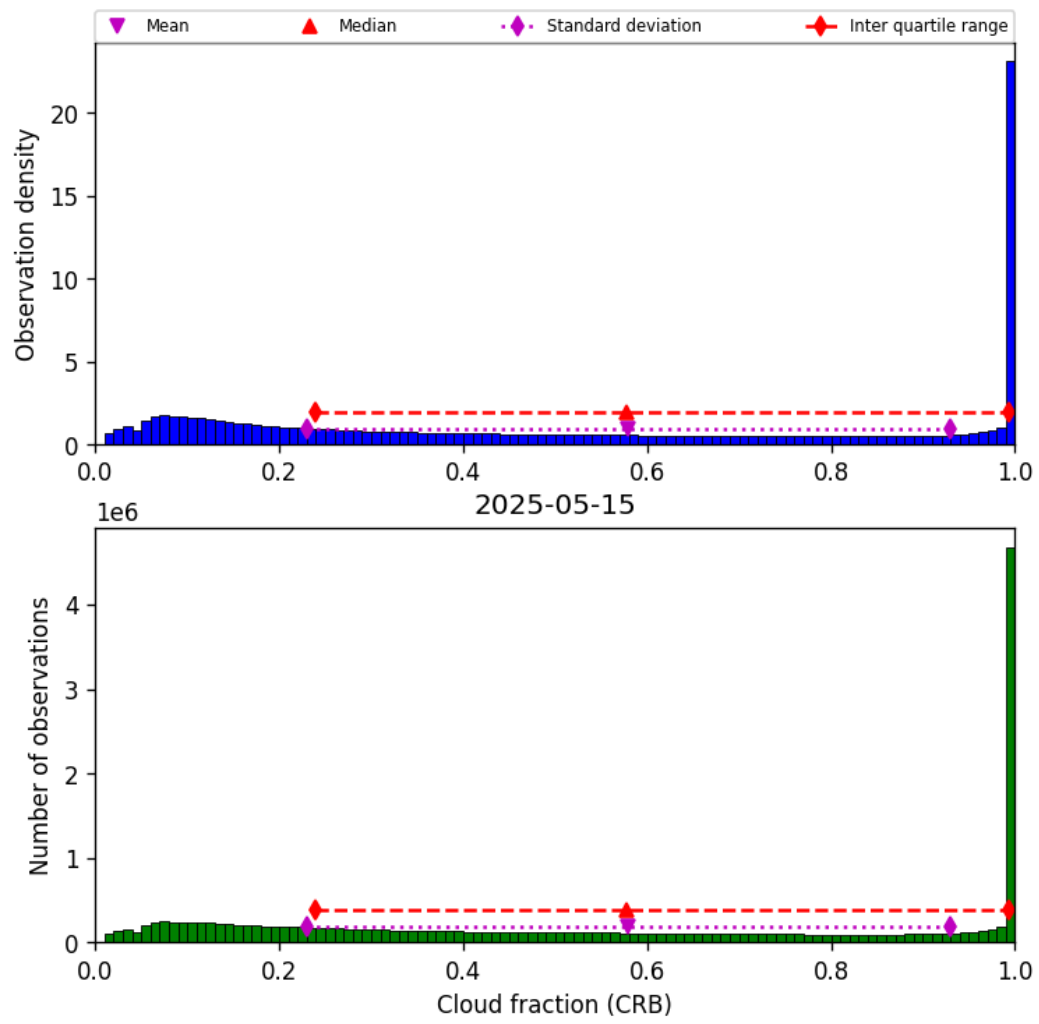
Figure 40: Histogram of “Cloud fraction (CRB)” for 2025-05-15 to 2025-05-16
