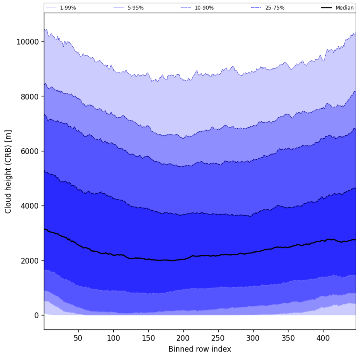
Figure 57: Along track statistics of “Cloud height (CRB)” for 2025-05-15 to 2025-05-16
