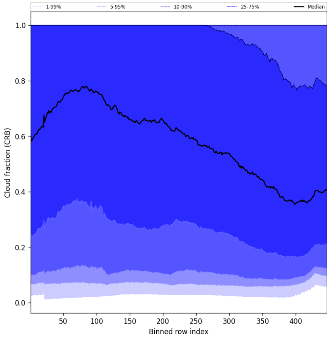
Figure 56: Along track statistics of “Cloud fraction (CRB)” for 2025-05-15 to 2025-05-16
