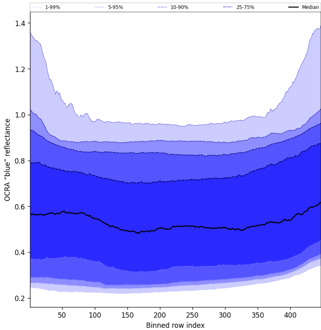
Figure 65: Along track statistics of “OCRA “blue” reflectance” for 2025-05-15 to 2025-05-16
