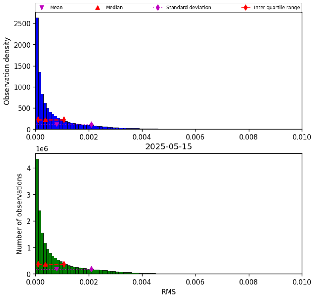
Figure 45: Histogram of “RMS” for 2025-05-15 to 2025-05-16
