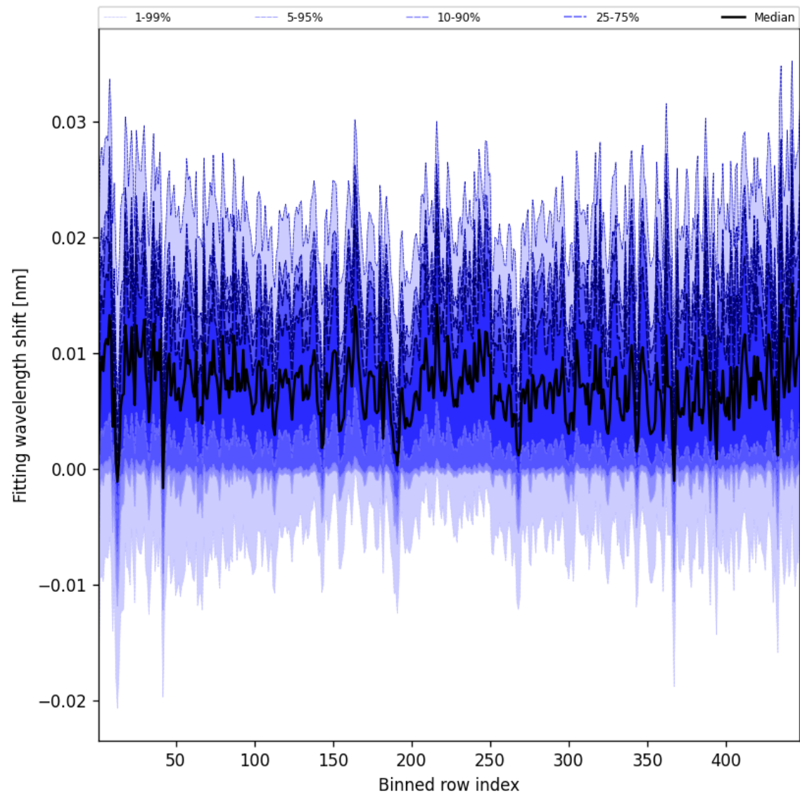
Figure 63: Along track statistics of “Fitting wavelength shift” for 2025-05-16 to 2025-05-17
