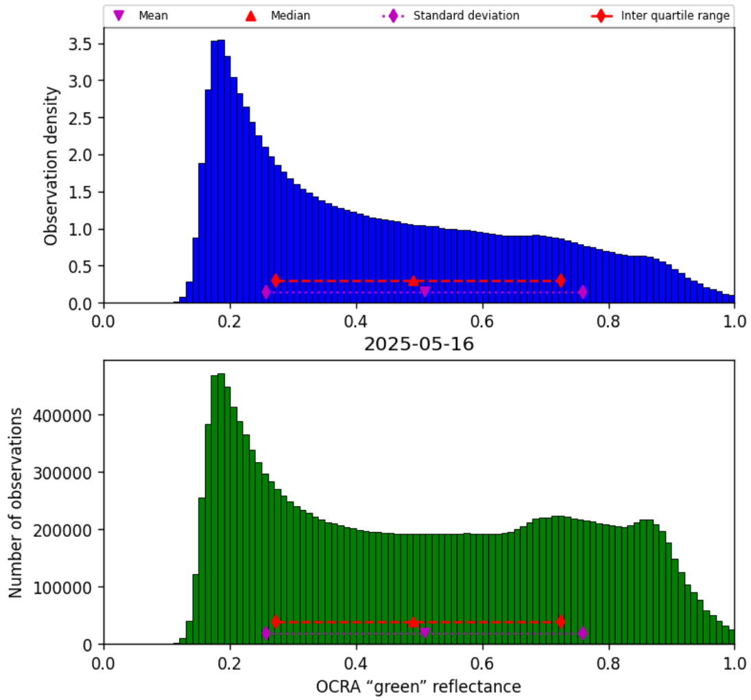
Figure 50: Histogram of “OCRA “green” reflectance” for 2025-05-16 to 2025-05-17
