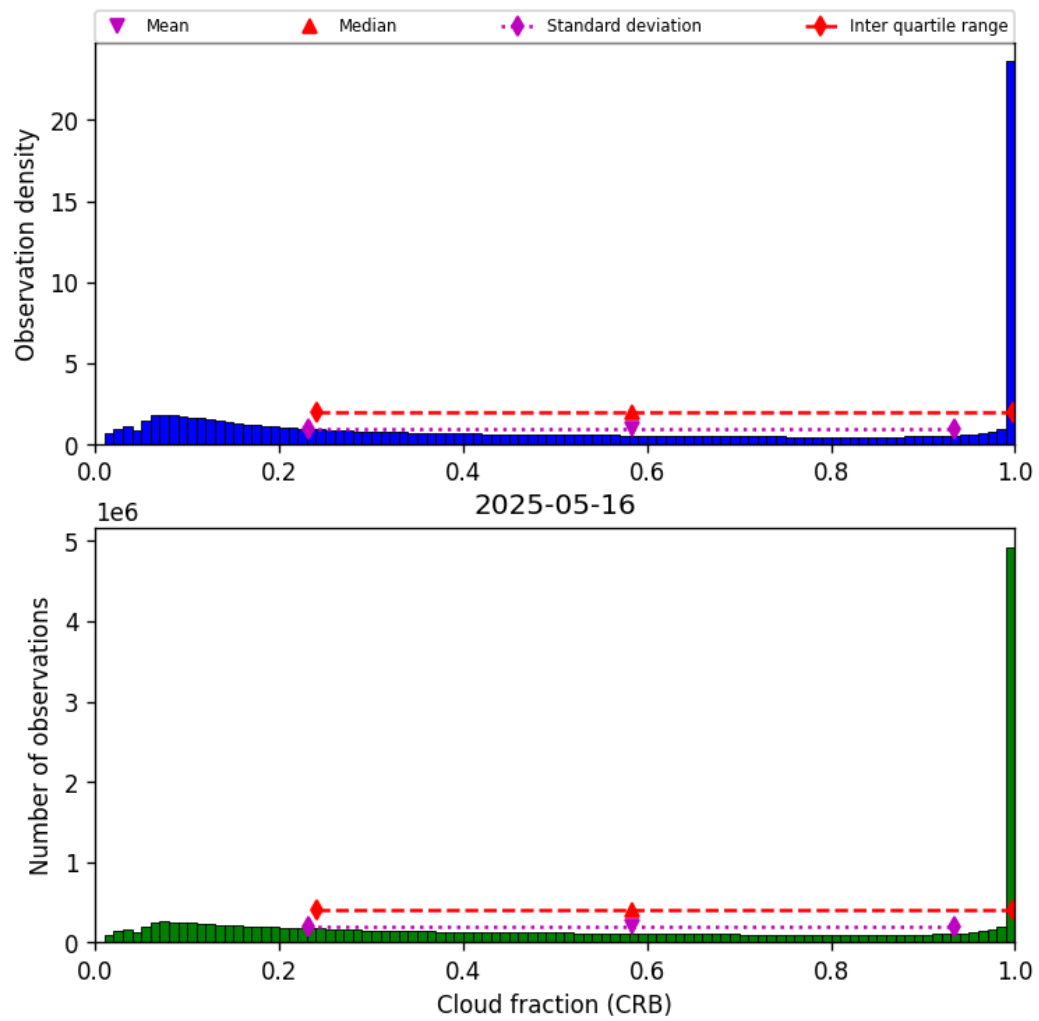
Figure 40: Histogram of “Cloud fraction (CRB)” for 2025-05-16 to 2025-05-17
