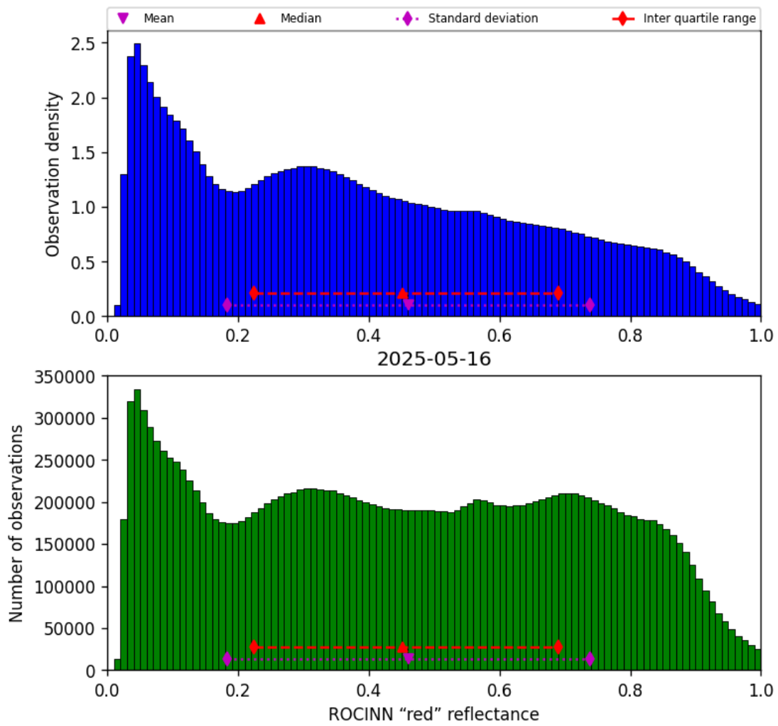
Figure 51: Histogram of “ROCINN “red” reflectance” for 2025-05-16 to 2025-05-17
