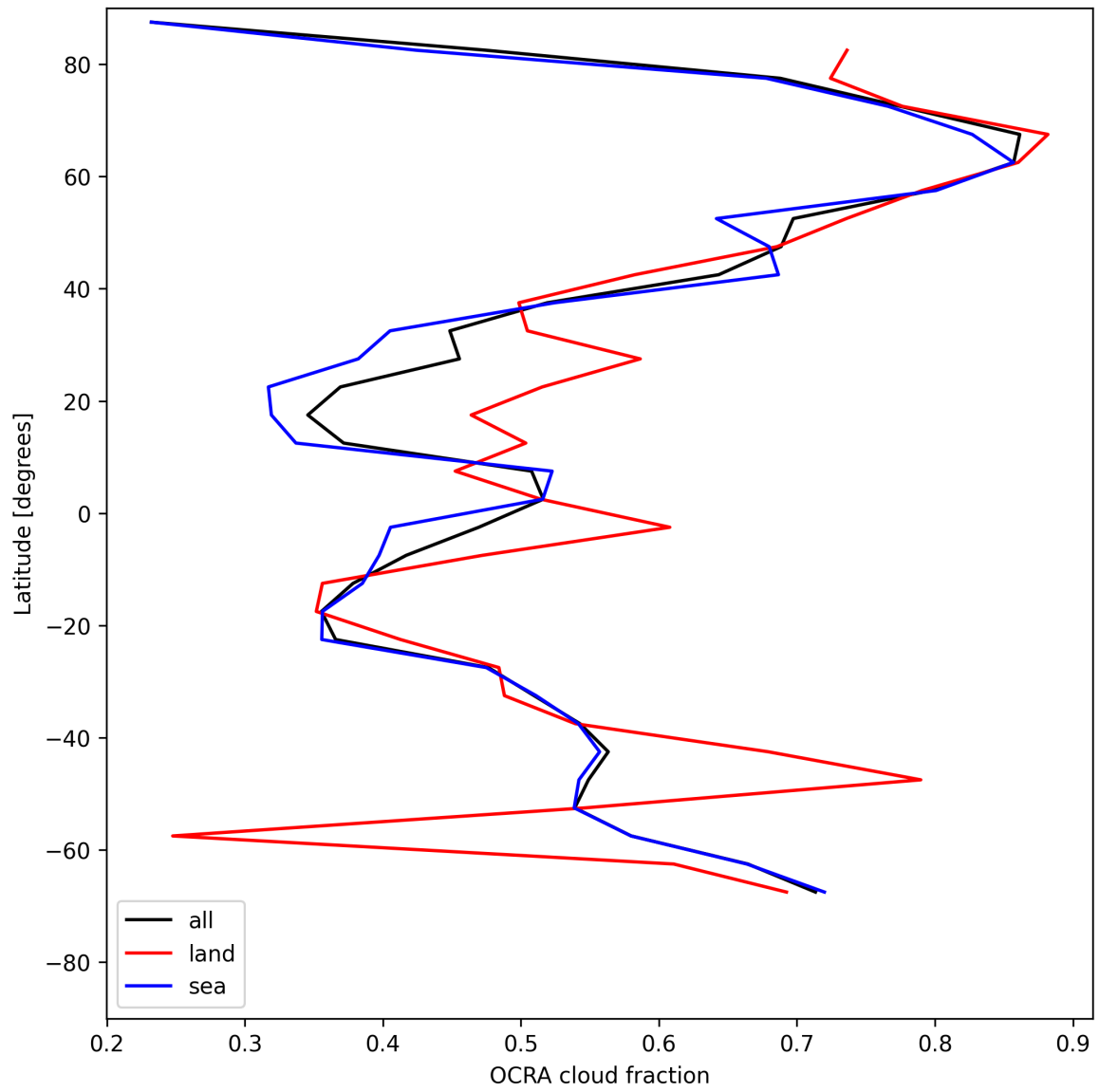
Figure 32: Zonal average of “OCRA cloud fraction” for 2025-05-16 to 2025-05-17.
