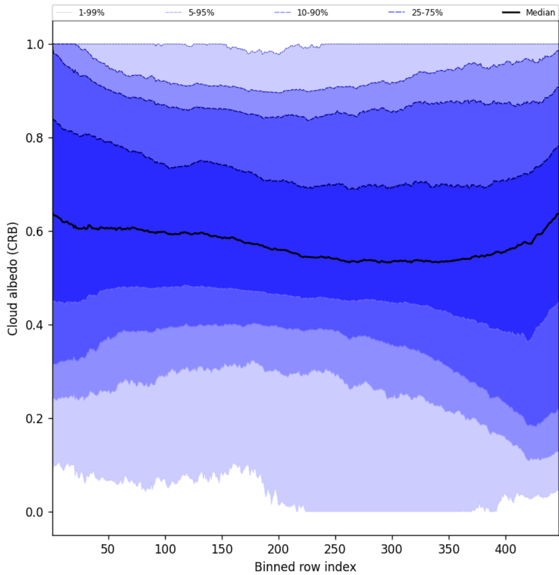
Figure 58: Along track statistics of “Cloud albedo (CRB)” for 2025-05-16 to 2025-05-17
