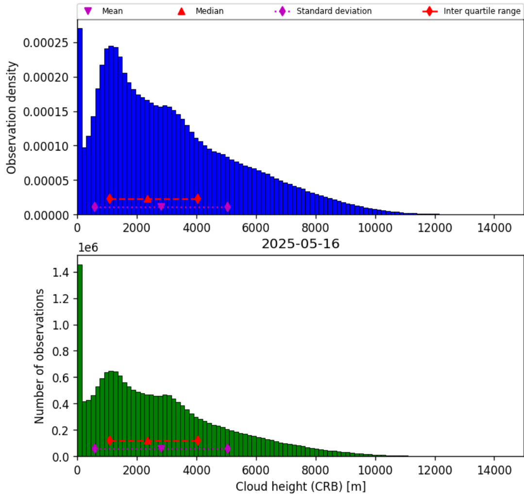
Figure 41: Histogram of “Cloud height (CRB)” for 2025-05-16 to 2025-05-17
