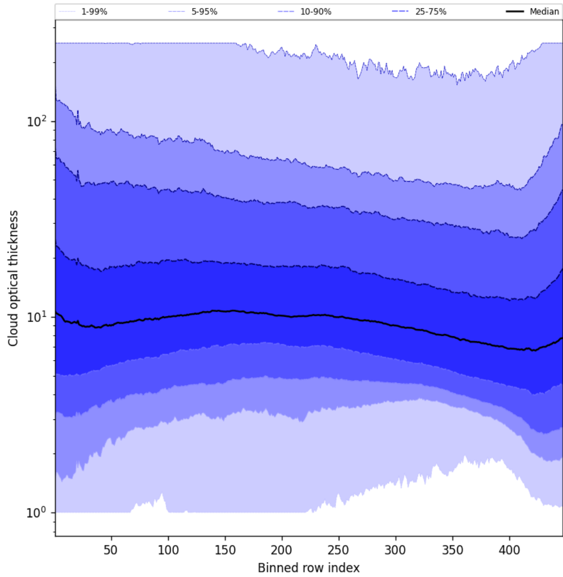
Figure 55: Along track statistics of “Cloud optical thickness” for 2025-05-16 to 2025-05-17
