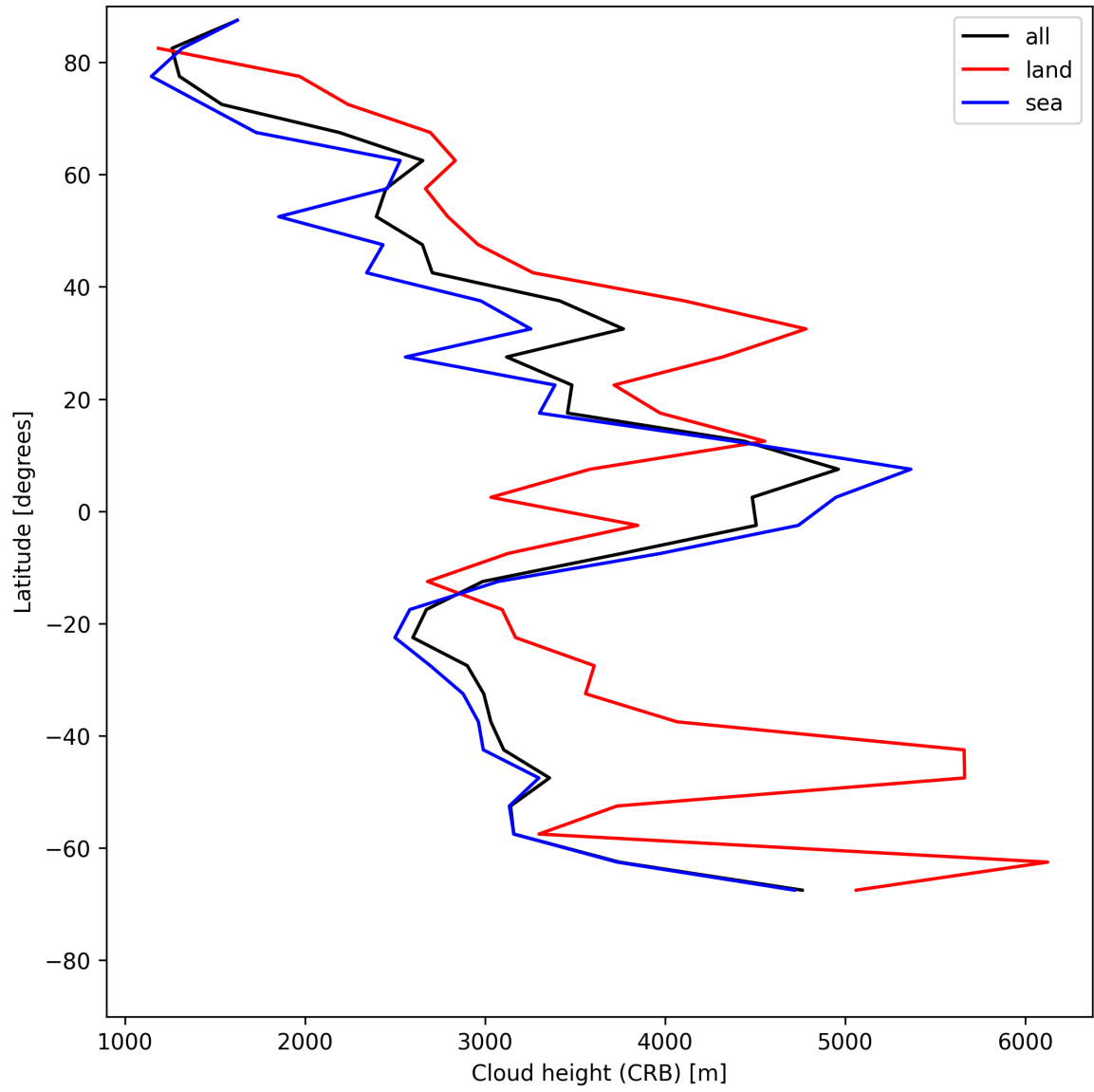
Figure 25: Zonal average of “Cloud height (CRB)” for 2025-05-16 to 2025-05-17.
