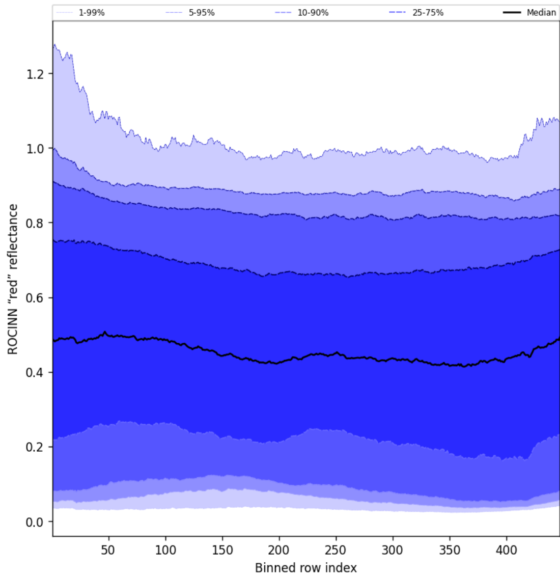
Figure 67: Along track statistics of "ROCINN "red" reflectance" for 2025-05-16 to 2025-05-17
