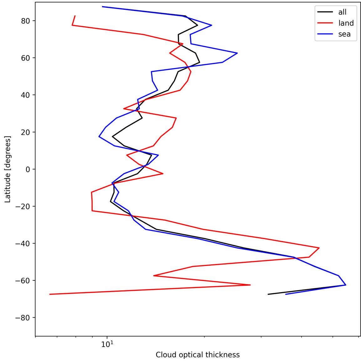
Figure 23: Zonal average of “Cloud optical thickness” for 2025-05-16 to 2025-05-17.
