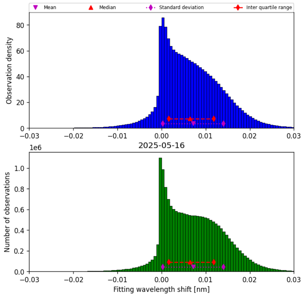
Figure 47: Histogram of “Fitting wavelength shift” for 2025-05-16 to 2025-05-17
