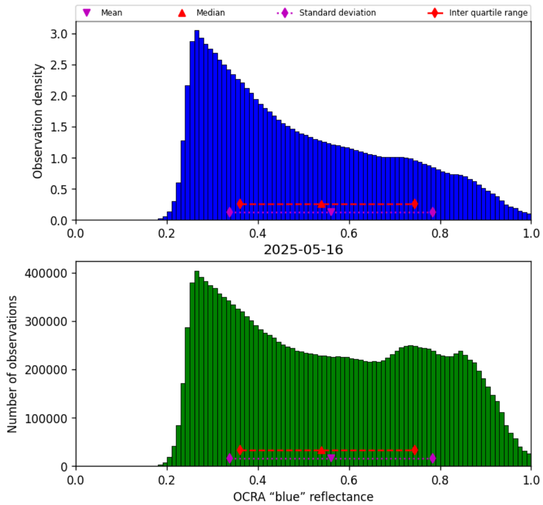
Figure 49: Histogram of “OCRA “blue” reflectance” for 2025-05-16 to 2025-05-17
