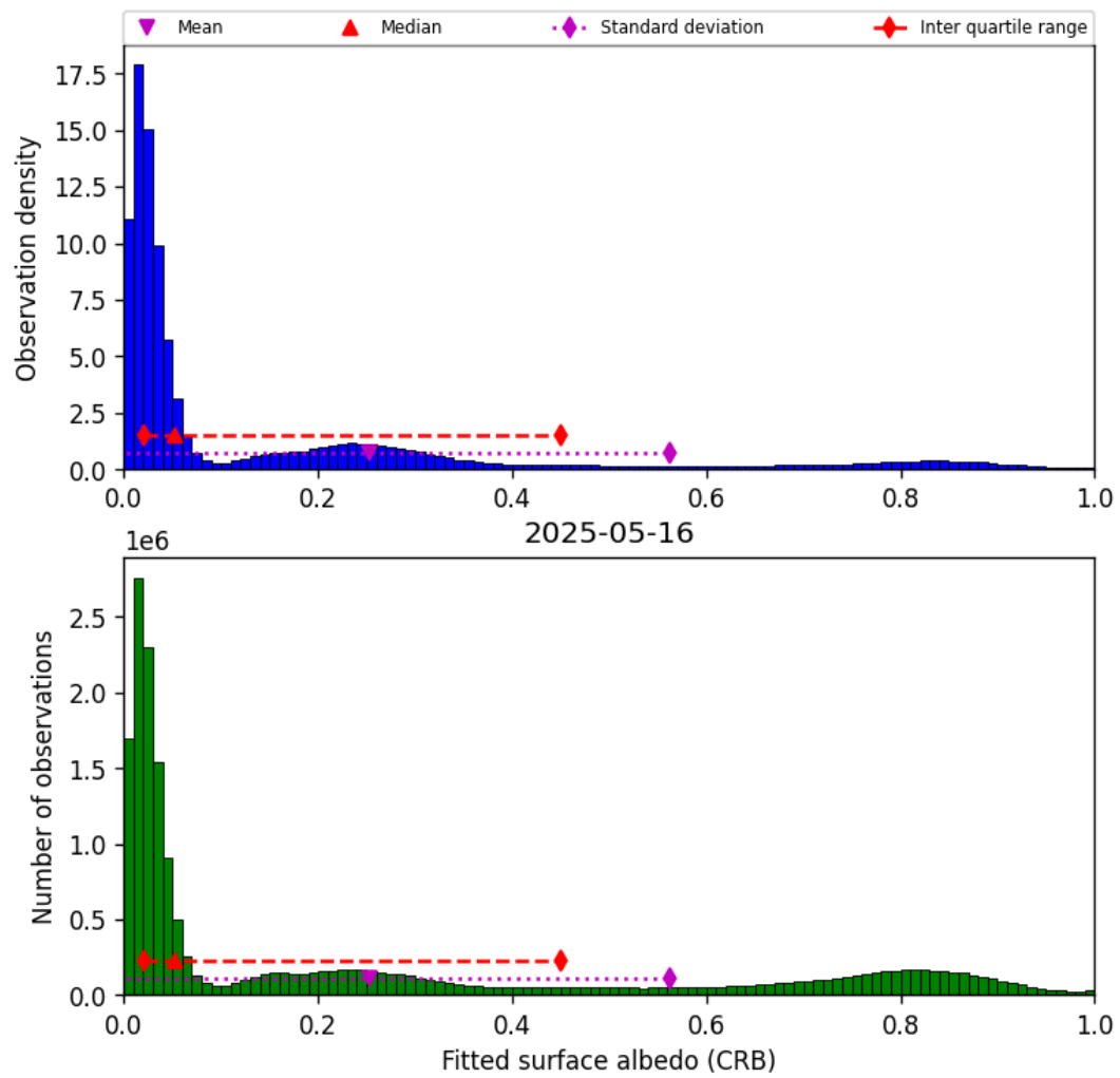
Figure 44: Histogram of “Fitted surface albedo (CRB)” for 2025-05-16 to 2025-05-17
