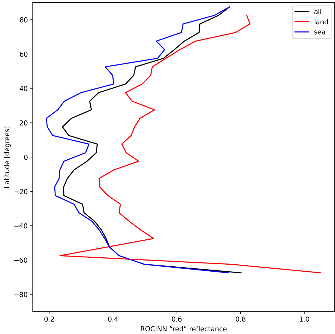
Figure 35: Zonal average of “ROCINN “red” reflectance” for 2025-05-16 to 2025-05-17.
