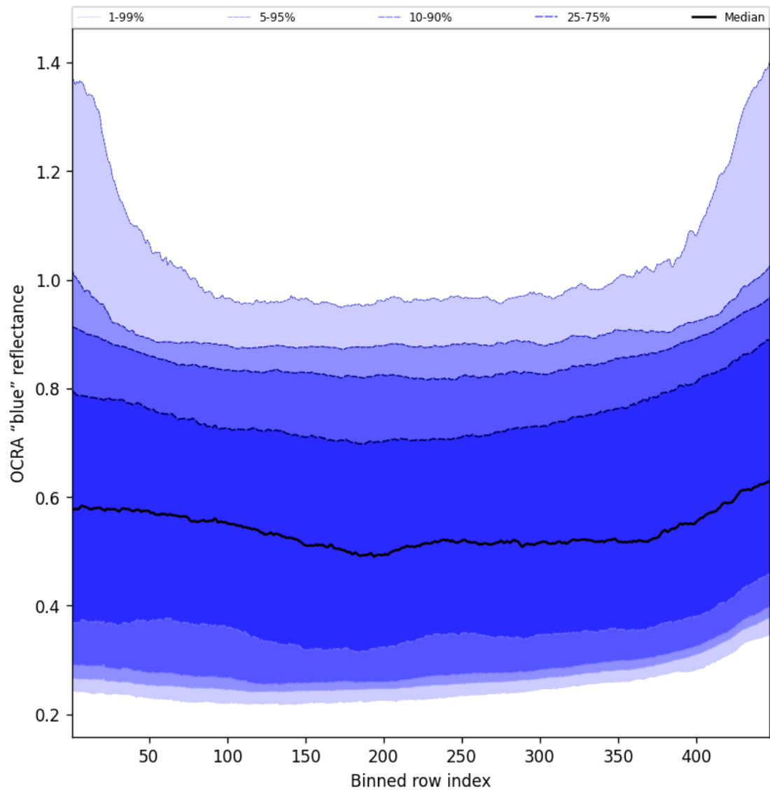
Figure 65: Along track statistics of “OCRA “blue” reflectance” for 2025-05-16 to 2025-05-17
