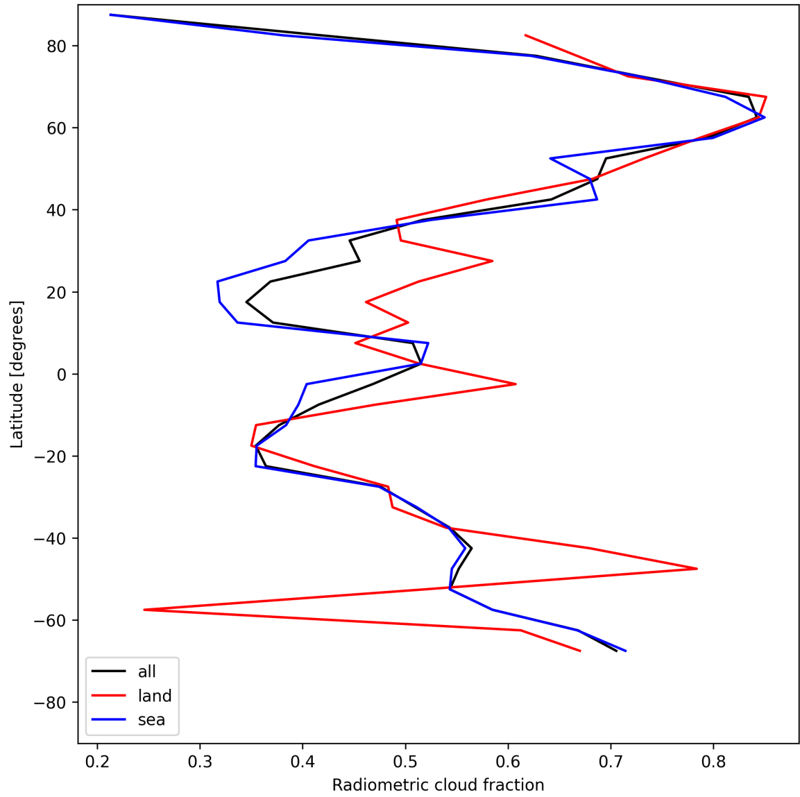
Figure 21: Zonal average of “Radiometric cloud fraction” for 2025-05-16 to 2025-05-17.
