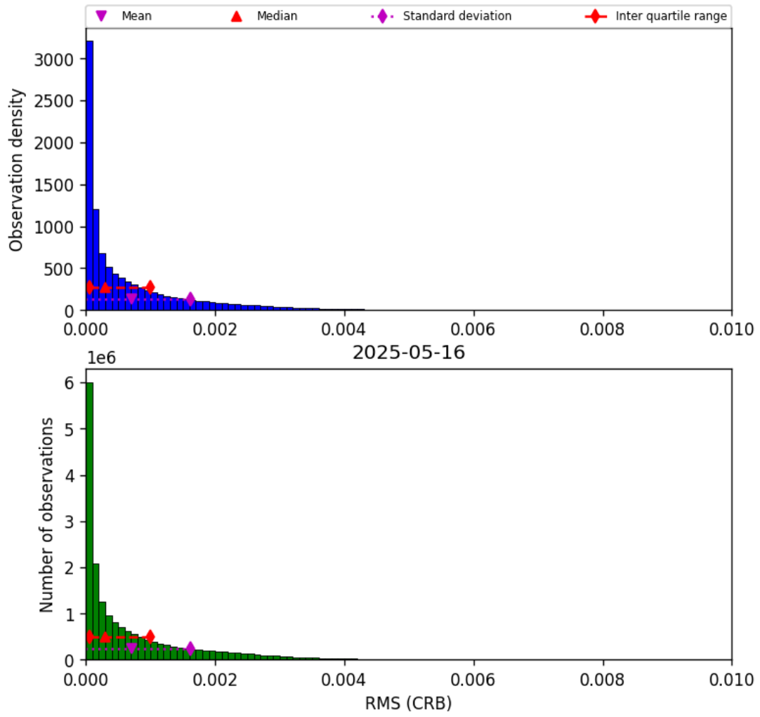
Figure 46: Histogram of "RMS (CRB)" for 2025-05-16 to 2025-05-17
