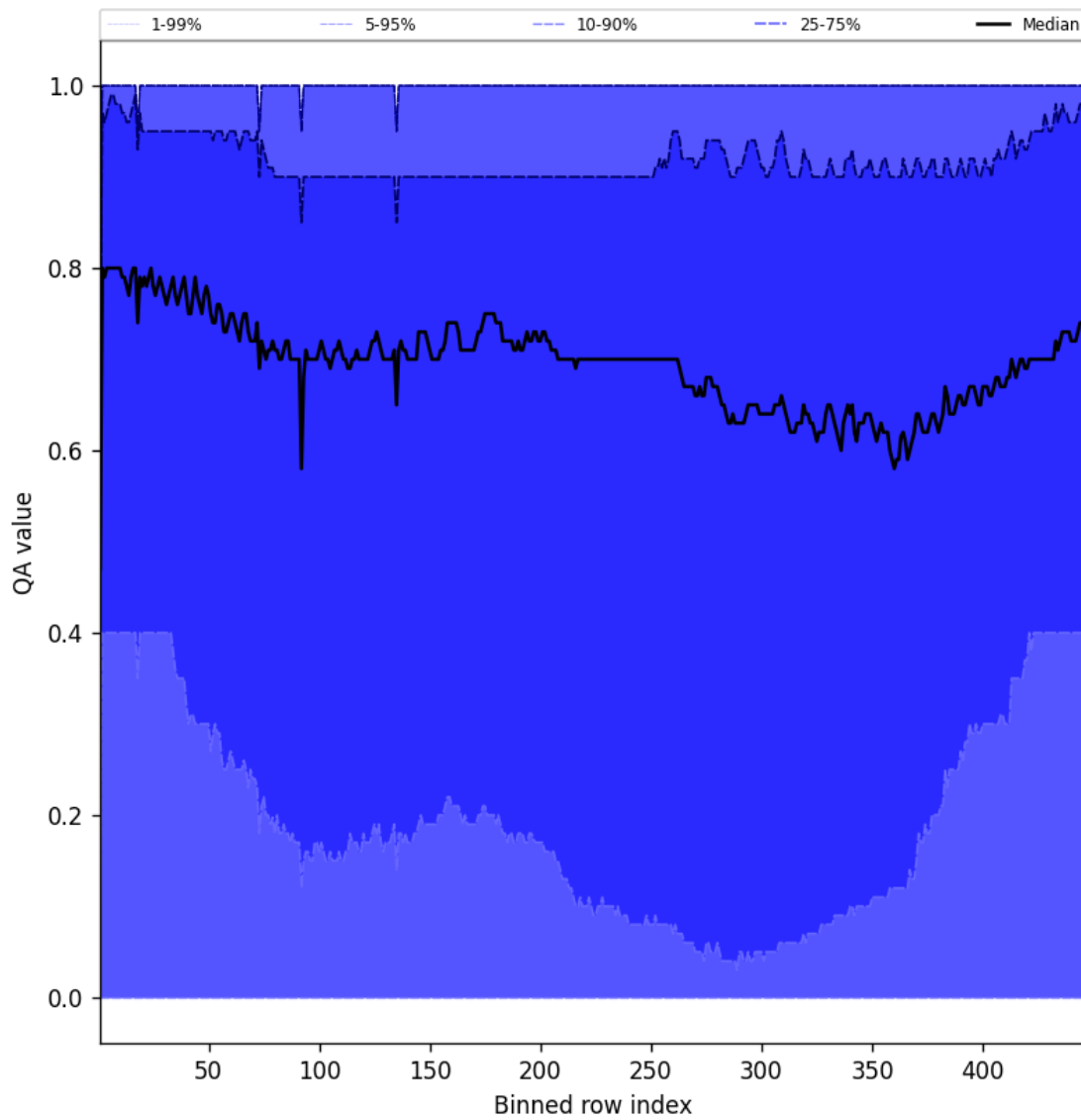
Figure 52: Along track statistics of “QA value” for 2025-05-16 to 2025-05-17
