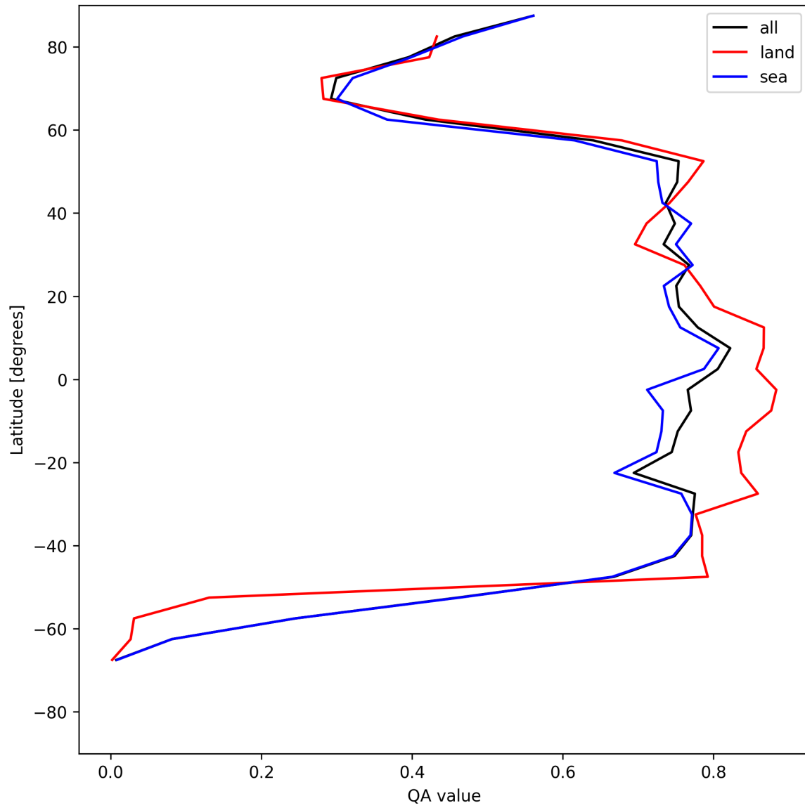
Figure 20: Zonal average of “QA value” for 2025-05-16 to 2025-05-17.
