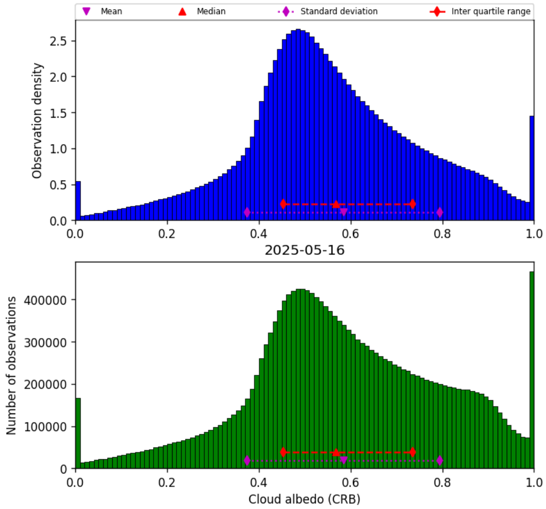
Figure 42: Histogram of “Cloud albedo (CRB)” for 2025-05-16 to 2025-05-17
