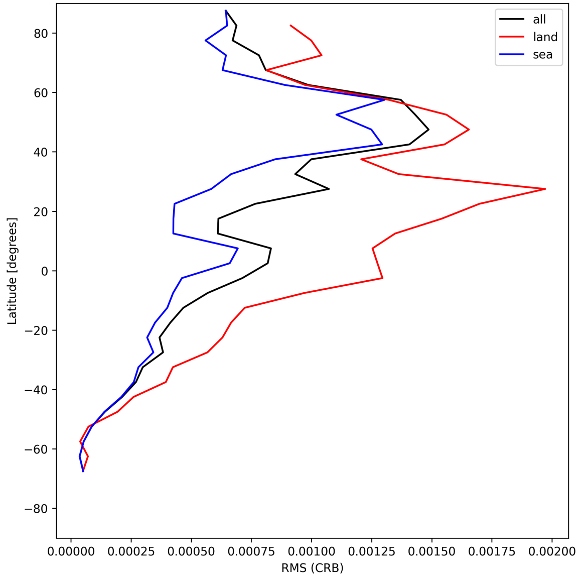
Figure 30: Zonal average of “RMS (CRB)” for 2025-05-16 to 2025-05-17.
