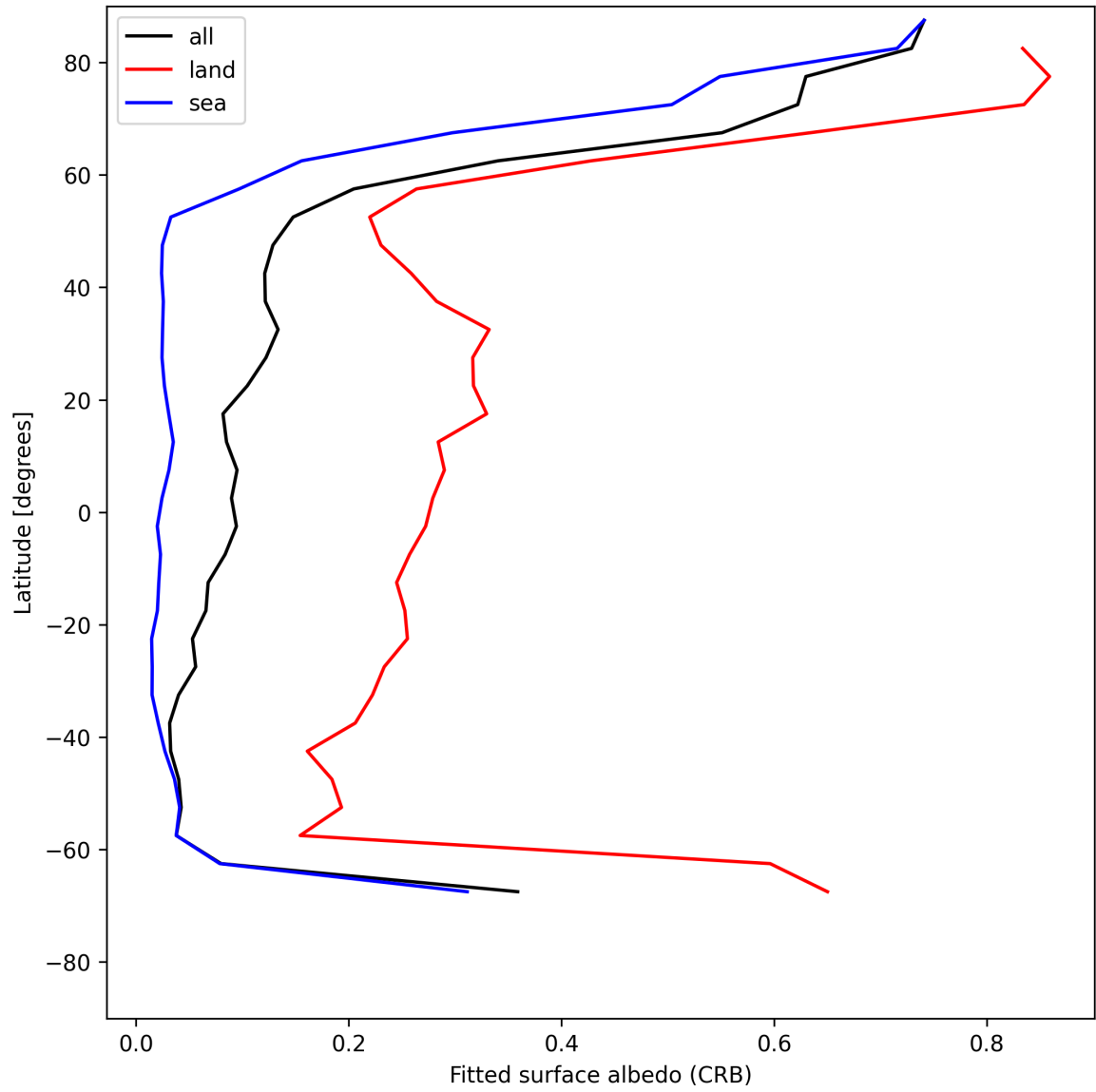
Figure 28: Zonal average of “Fitted surface albedo (CRB)” for 2025-05-16 to 2025-05-17.
