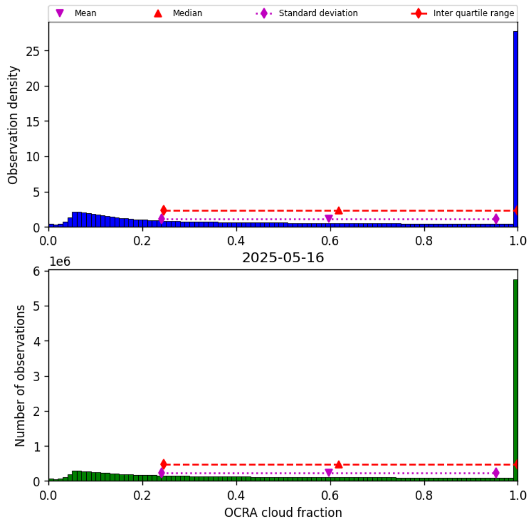
Figure 48: Histogram of “OCRA cloud fraction” for 2025-05-16 to 2025-05-17
