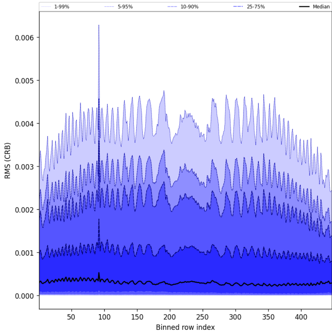
Figure 62: Along track statistics of “RMS (CRB)” for 2025-05-16 to 2025-05-17
