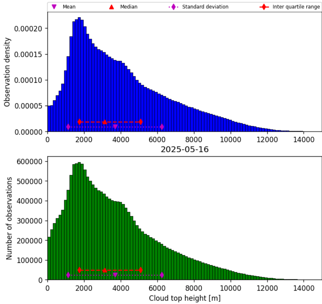
Figure 38: Histogram of “Cloud top height” for 2025-05-16 to 2025-05-17
