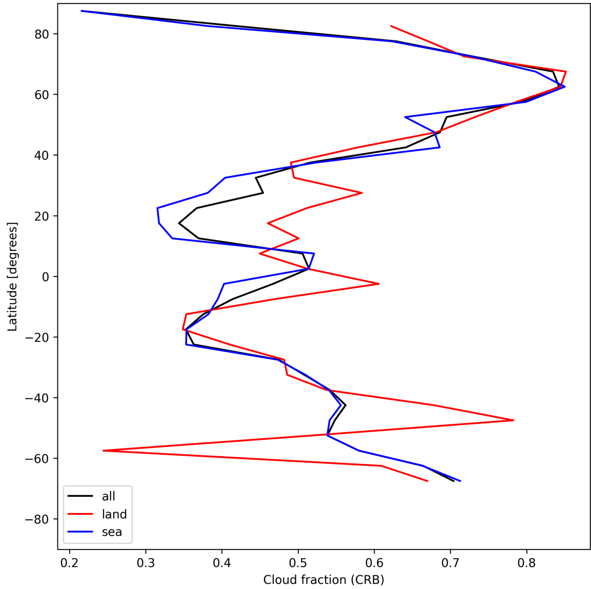
Figure 24: Zonal average of “Cloud fraction (CRB)” for 2025-05-16 to 2025-05-17.
