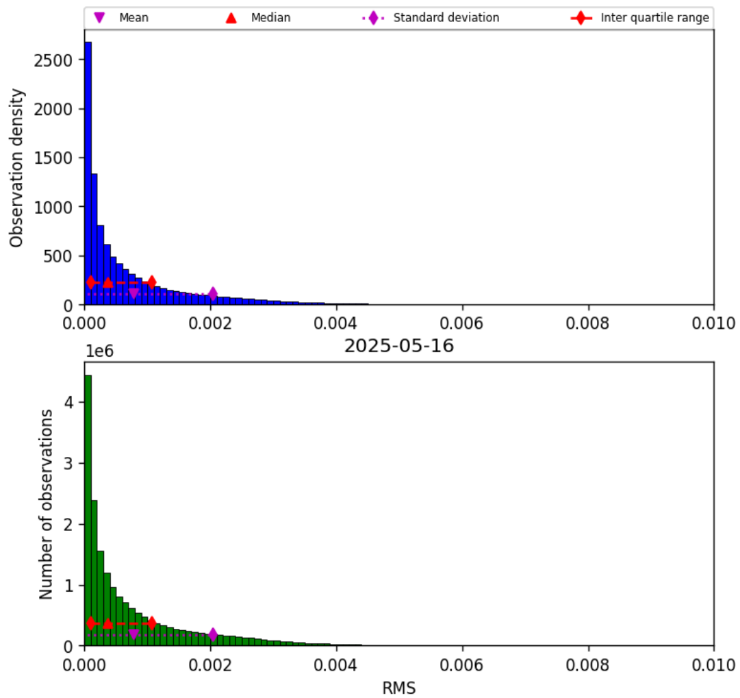
Figure 45: Histogram of “RMS” for 2025-05-16 to 2025-05-17
