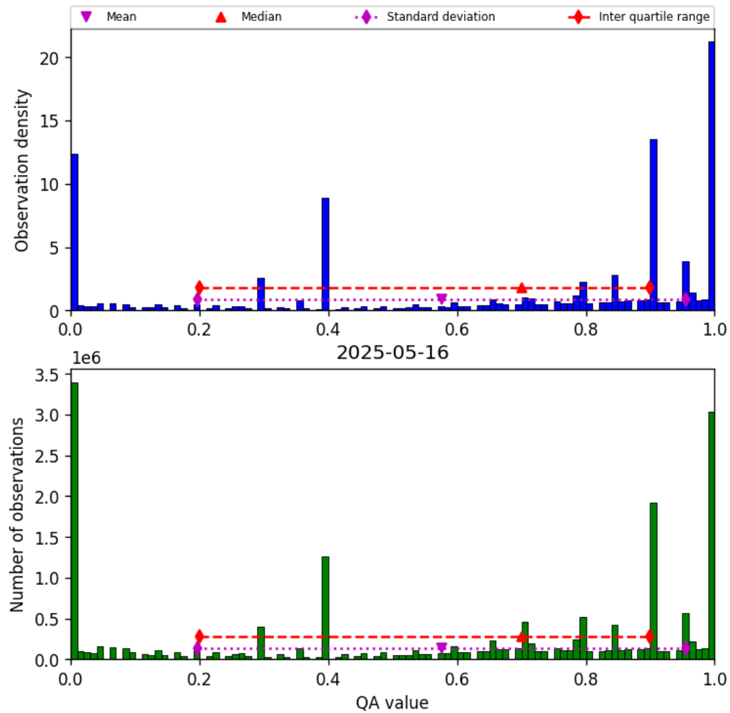
Figure 36: Histogram of “QA value” for 2025-05-16 to 2025-05-17
