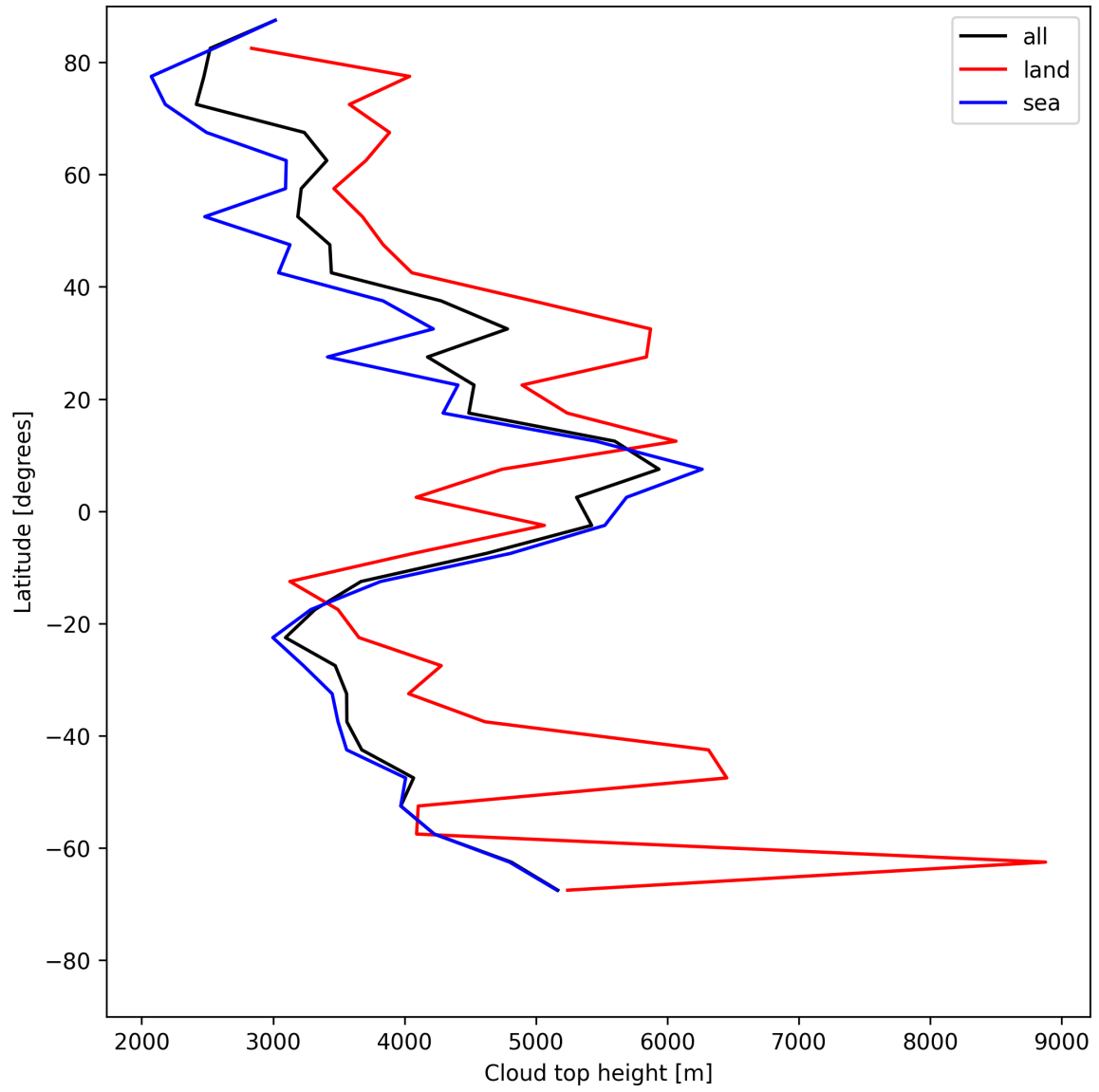
Figure 22: Zonal average of “Cloud top height” for 2025-05-16 to 2025-05-17.
