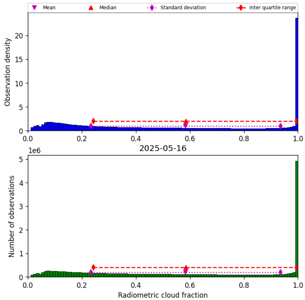
Figure 37: Histogram of “Radiometric cloud fraction” for 2025-05-16 to 2025-05-17
