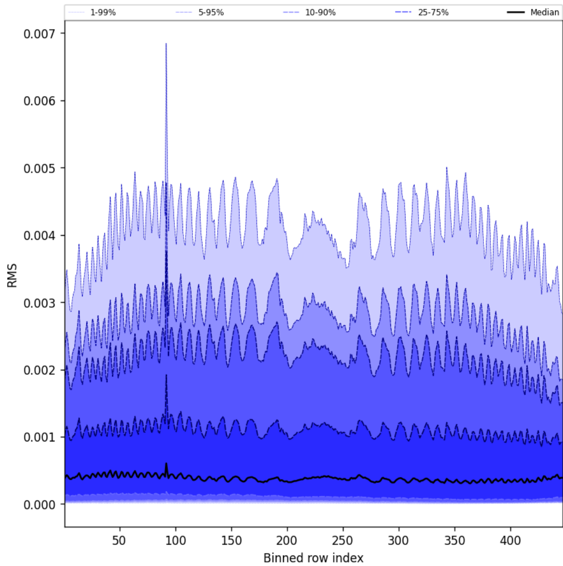
Figure 61: Along track statistics of “RMS” for 2025-05-16 to 2025-05-17
