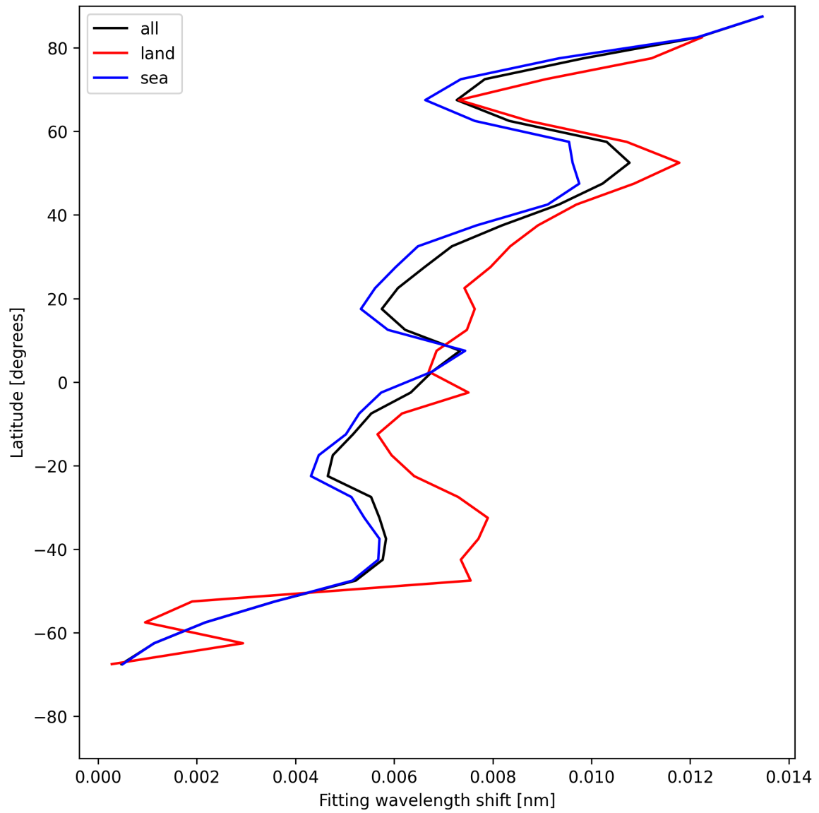
Figure 31: Zonal average of “Fitting wavelength shift” for 2025-05-16 to 2025-05-17.
