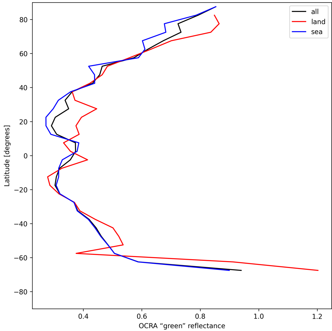
Figure 34: Zonal average of “OCRA “green” reflectance” for 2025-05-16 to 2025-05-17.
