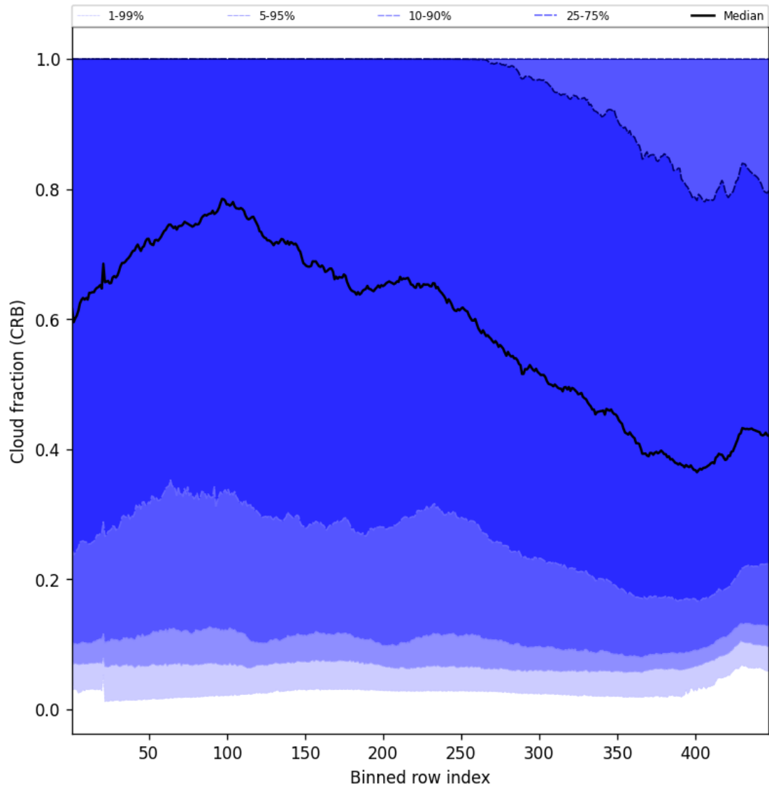
Figure 56: Along track statistics of “Cloud fraction (CRB)” for 2025-05-16 to 2025-05-17
