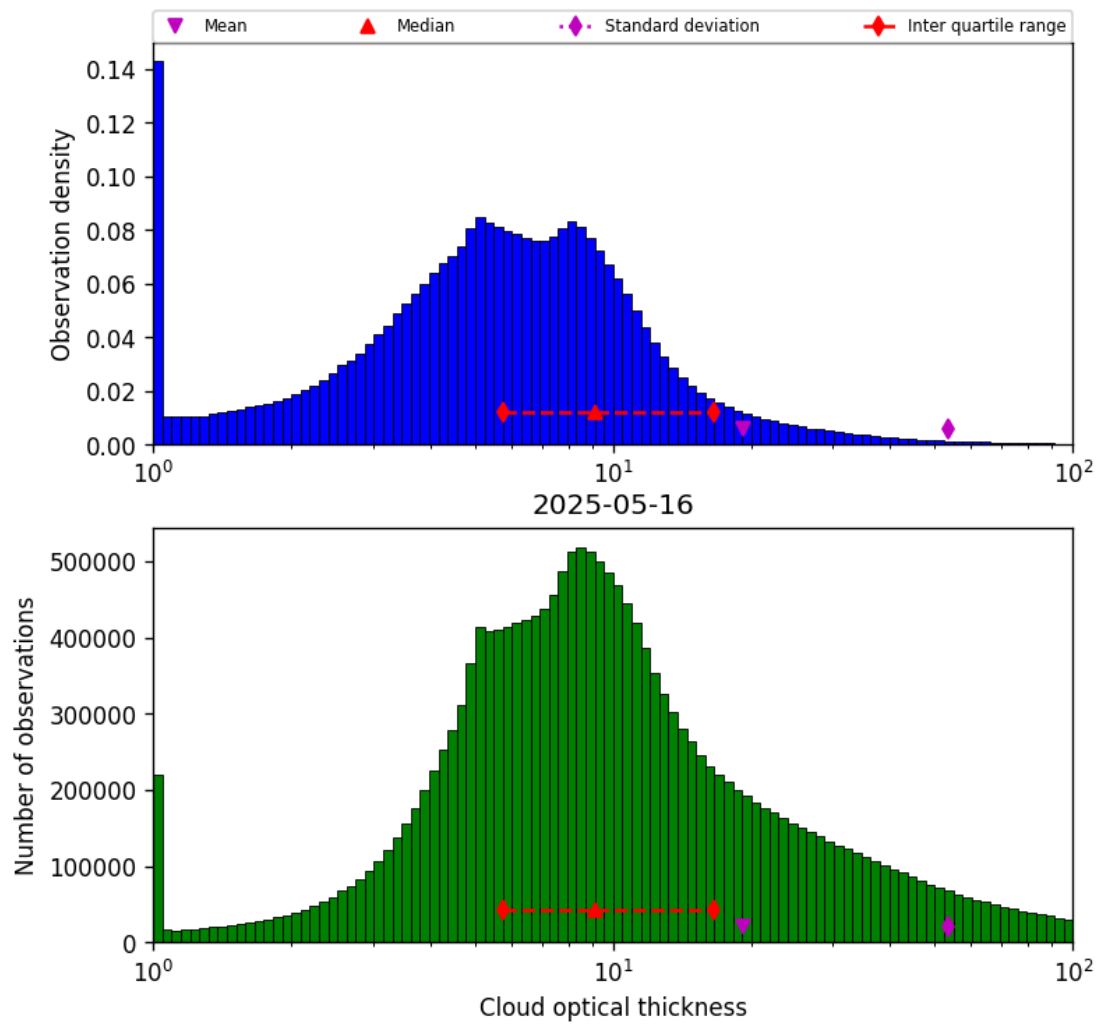
Figure 39: Histogram of “Cloud optical thickness” for 2025-05-16 to 2025-05-17
