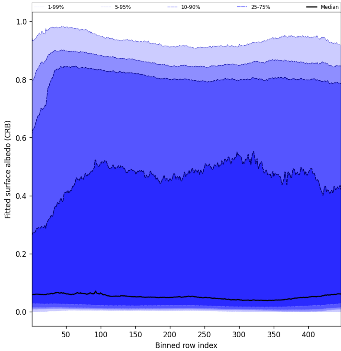
Figure 60: Along track statistics of “Fitted surface albedo (CRB)” for 2025-05-16 to 2025-05-17
