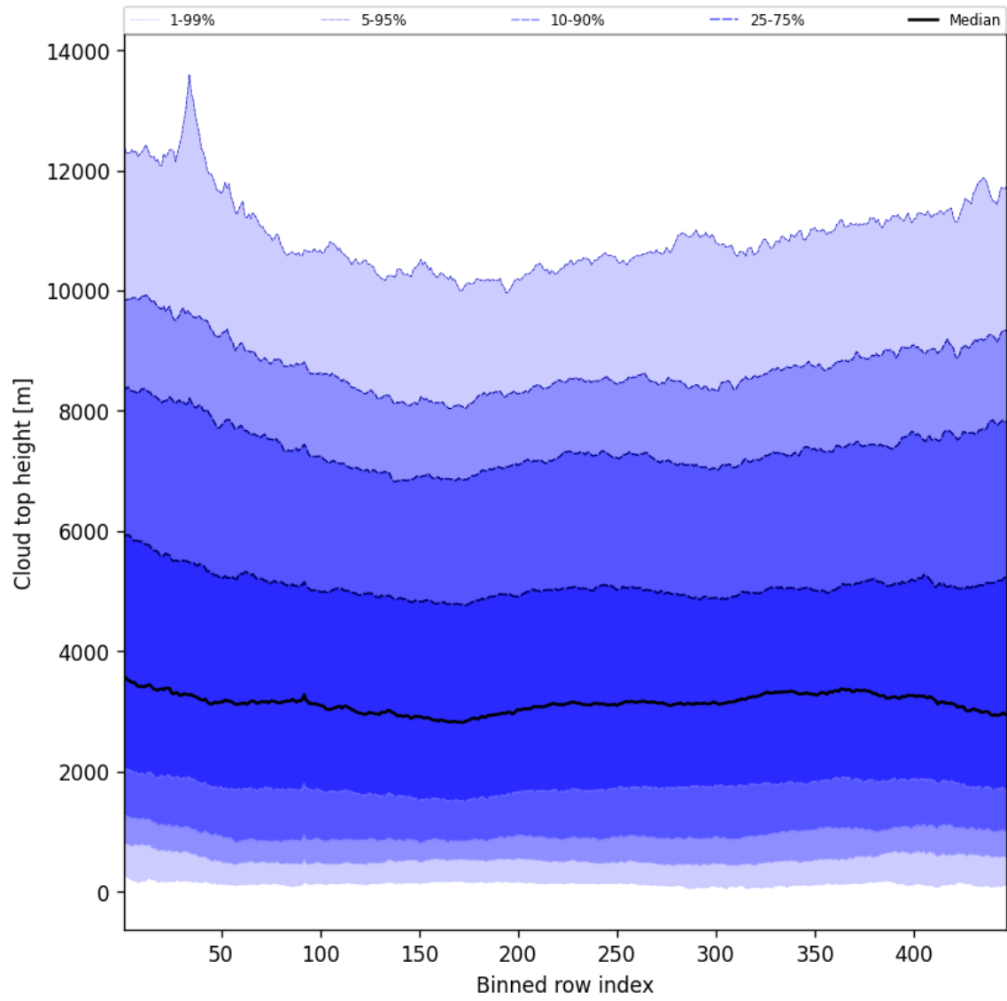
Figure 54: Along track statistics of “Cloud top height” for 2025-05-16 to 2025-05-17
