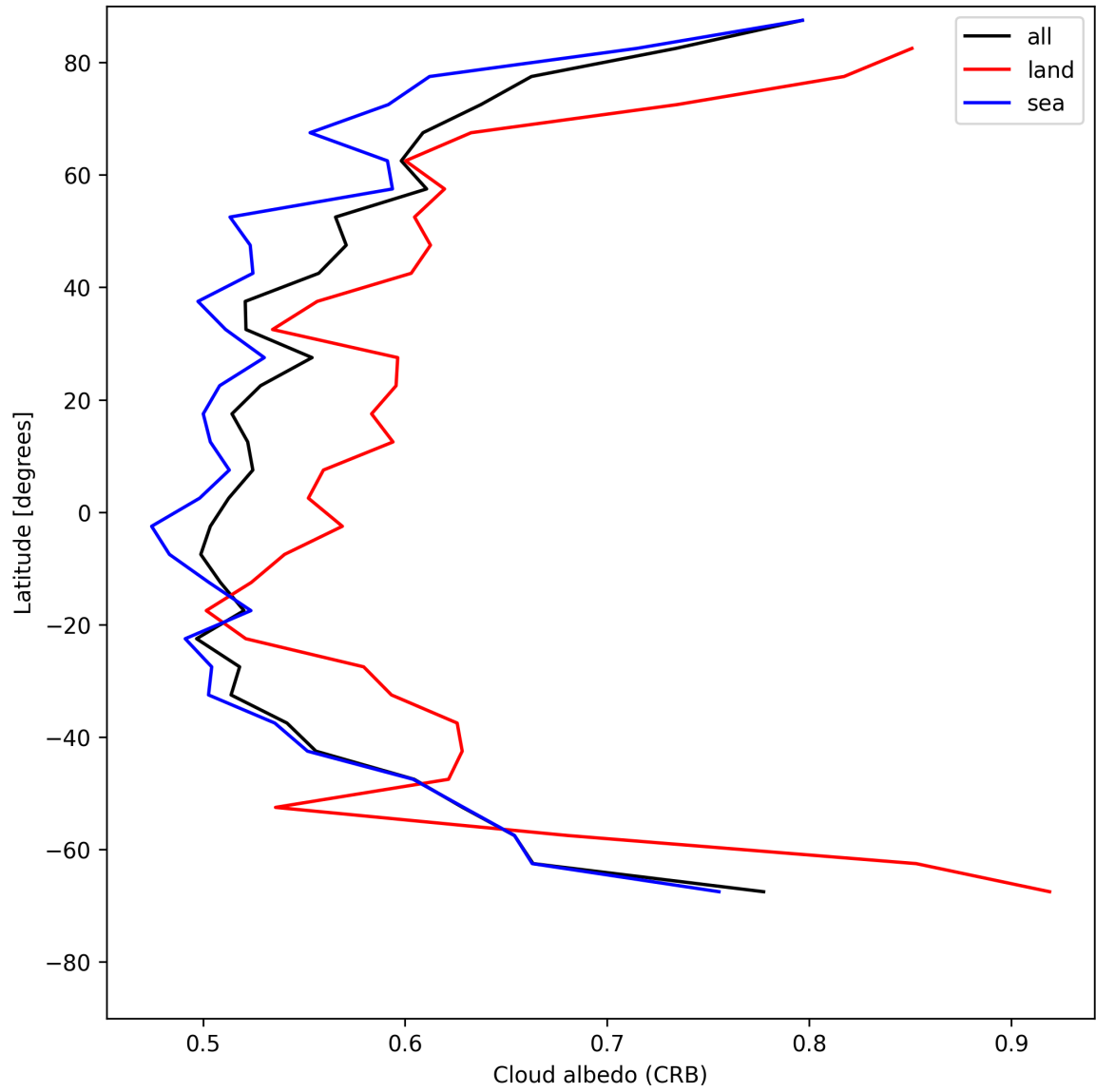
Figure 26: Zonal average of “Cloud albedo (CRB)” for 2025-05-16 to 2025-05-17.
