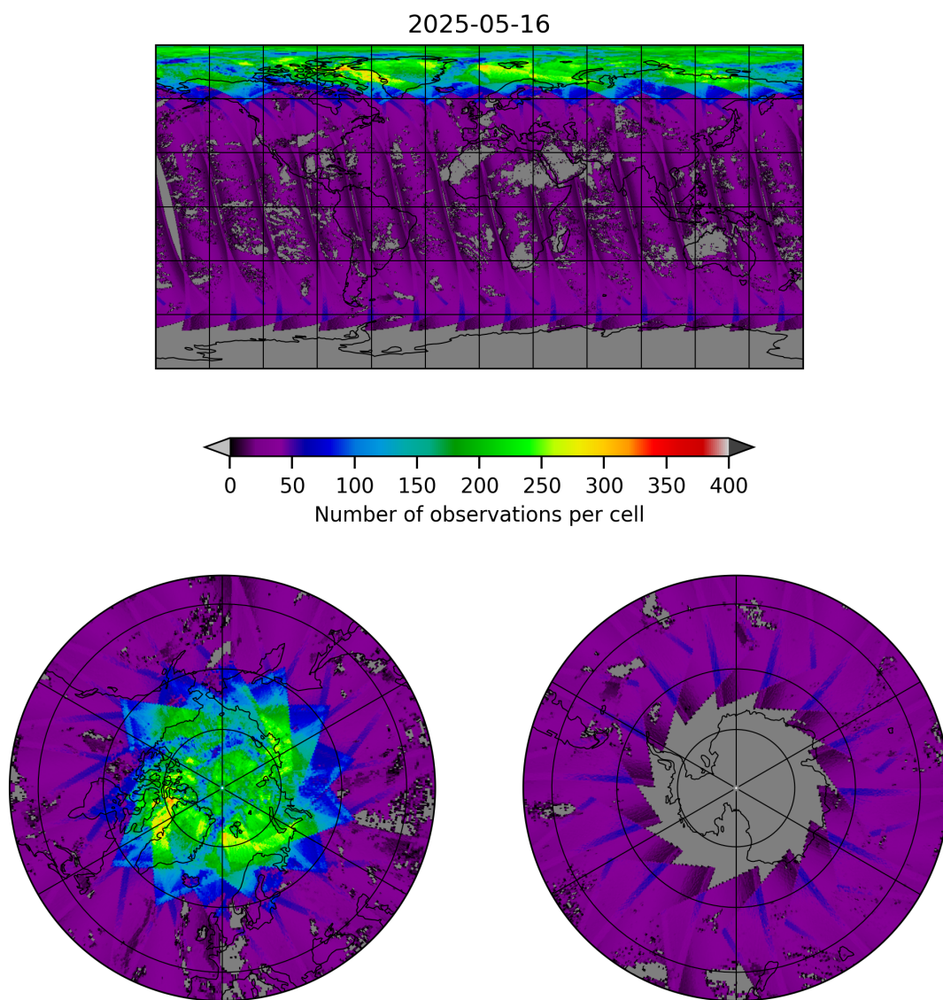
Figure 19: Map of the number of observations for 2025-05-16 to 2025-05-17
