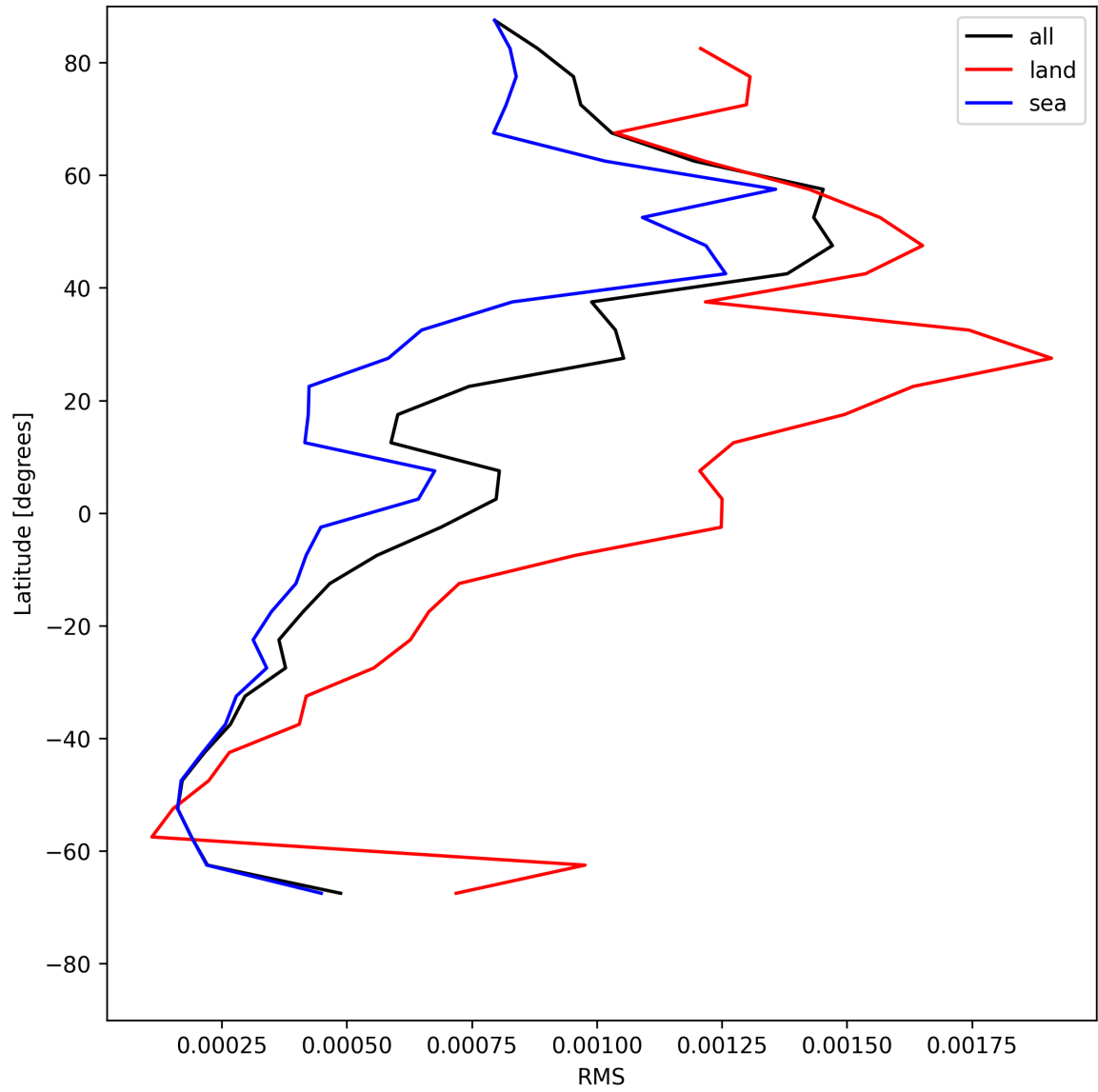
Figure 29: Zonal average of “RMS” for 2025-05-16 to 2025-05-17.
