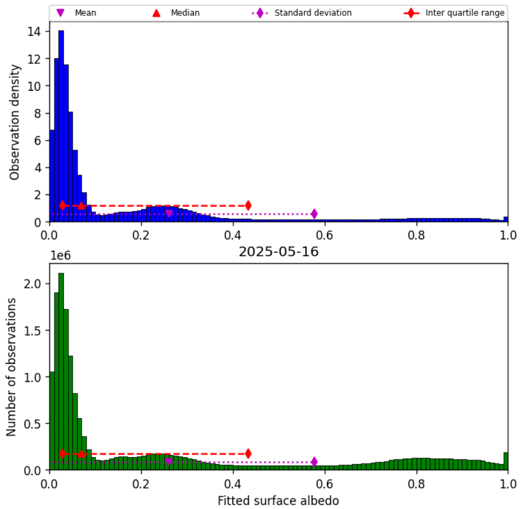
Figure 43: Histogram of “Fitted surface albedo” for 2025-05-16 to 2025-05-17
