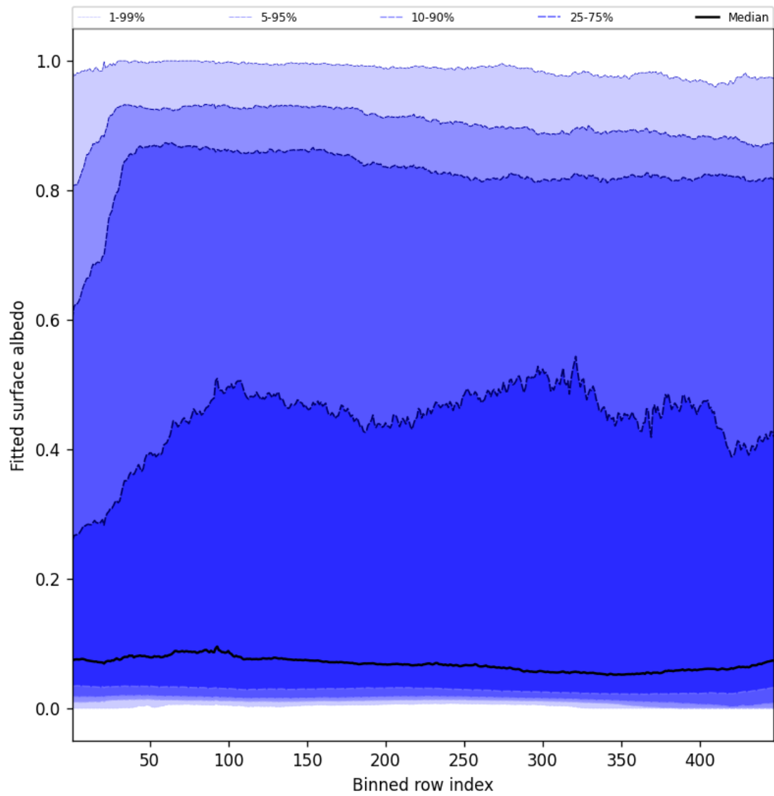
Figure 59: Along track statistics of “Fitted surface albedo” for 2025-05-16 to 2025-05-17
