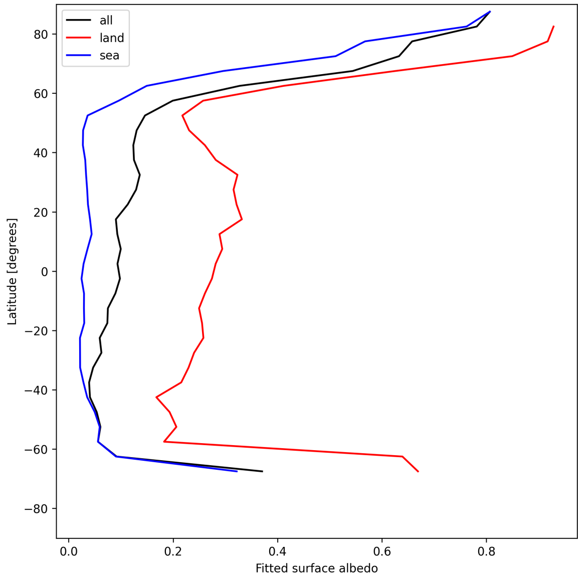
Figure 27: Zonal average of “Fitted surface albedo” for 2025-05-16 to 2025-05-17.
