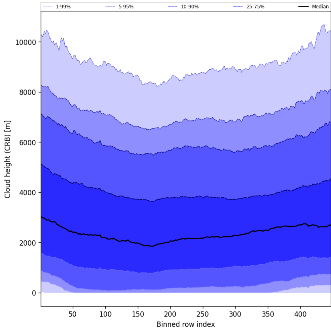
Figure 57: Along track statistics of “Cloud height (CRB)” for 2025-05-16 to 2025-05-17
