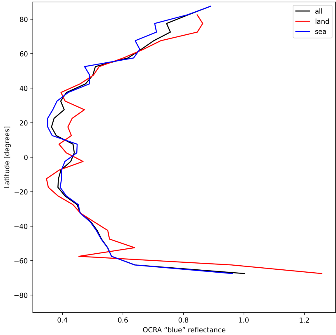
Figure 33: Zonal average of “OCRA “blue” reflectance” for 2025-05-16 to 2025-05-17.
