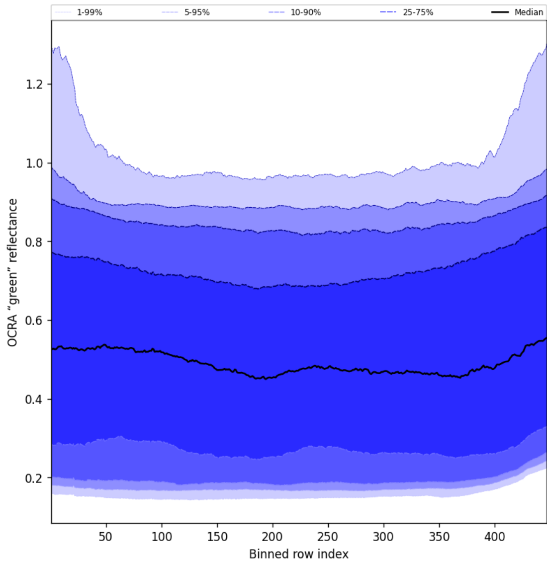
Figure 66: Along track statistics of “OCRA “green” reflectance” for 2025-05-16 to 2025-05-17
