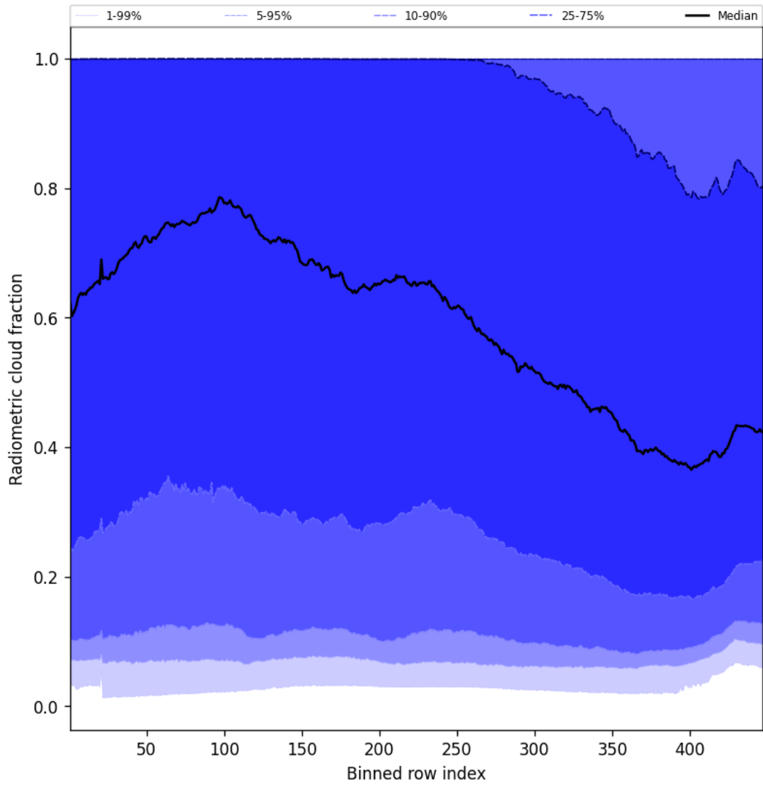
Figure 53: Along track statistics of “Radiometric cloud fraction” for 2025-05-16 to 2025-05-17
