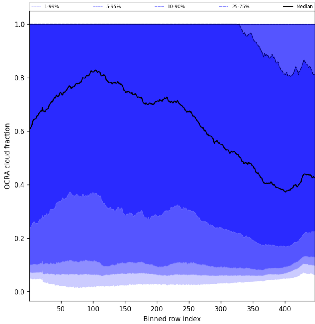
Figure 64: Along track statistics of “OCRA cloud fraction” for 2025-05-16 to 2025-05-17
