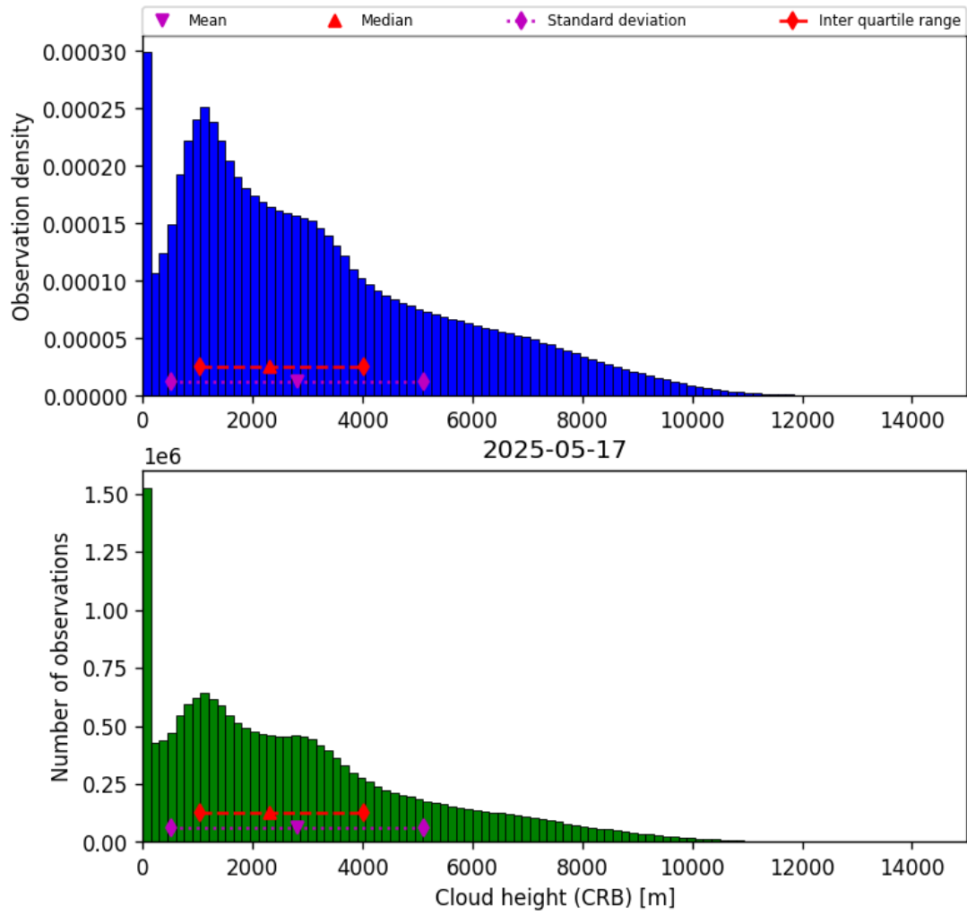
Figure 41: Histogram of “Cloud height (CRB)” for 2025-05-17 to 2025-05-18
