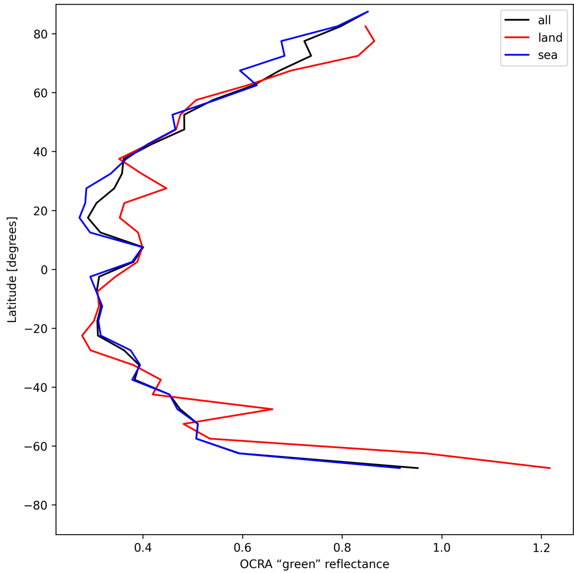
Figure 34: Zonal average of “OCRA “green” reflectance” for 2025-05-17 to 2025-05-18.
