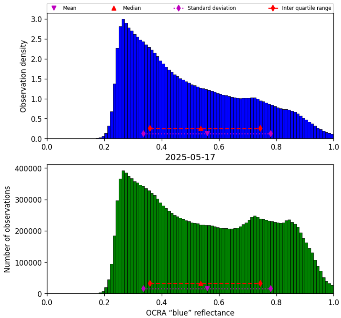
Figure 49: Histogram of “OCRA “blue” reflectance” for 2025-05-17 to 2025-05-18
