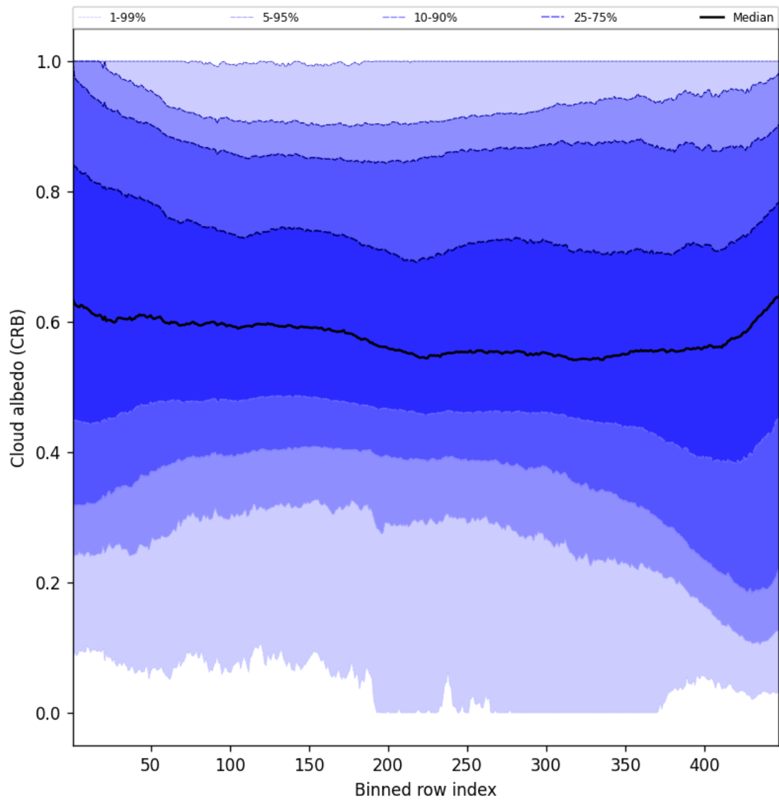
Figure 58: Along track statistics of “Cloud albedo (CRB)” for 2025-05-17 to 2025-05-18
