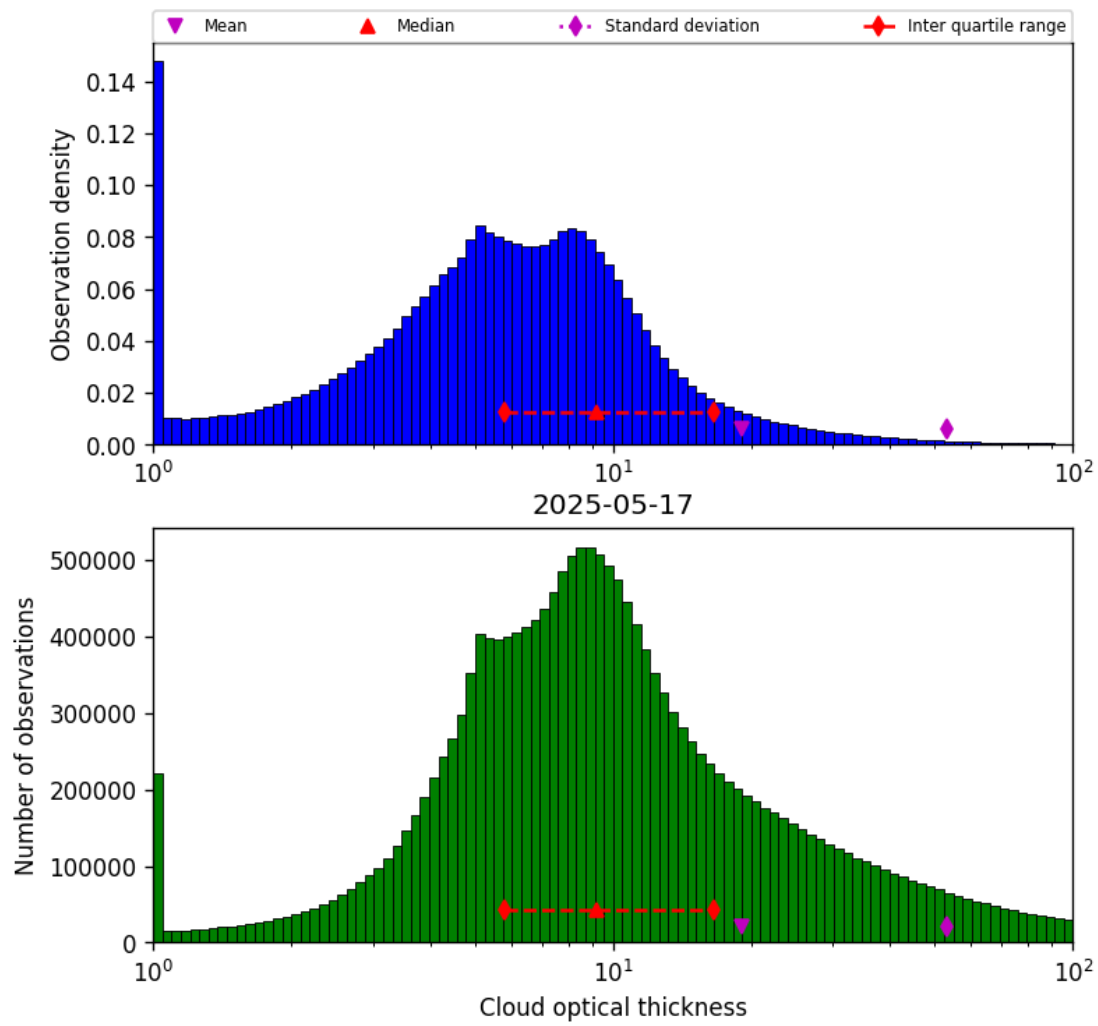
Figure 39: Histogram of “Cloud optical thickness” for 2025-05-17 to 2025-05-18
