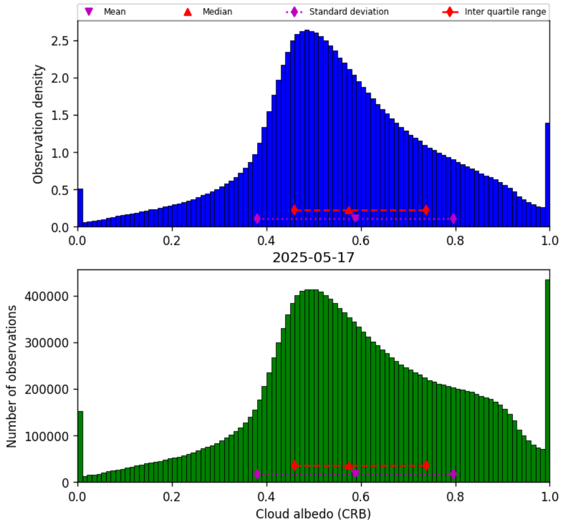
Figure 42: Histogram of “Cloud albedo (CRB)” for 2025-05-17 to 2025-05-18
