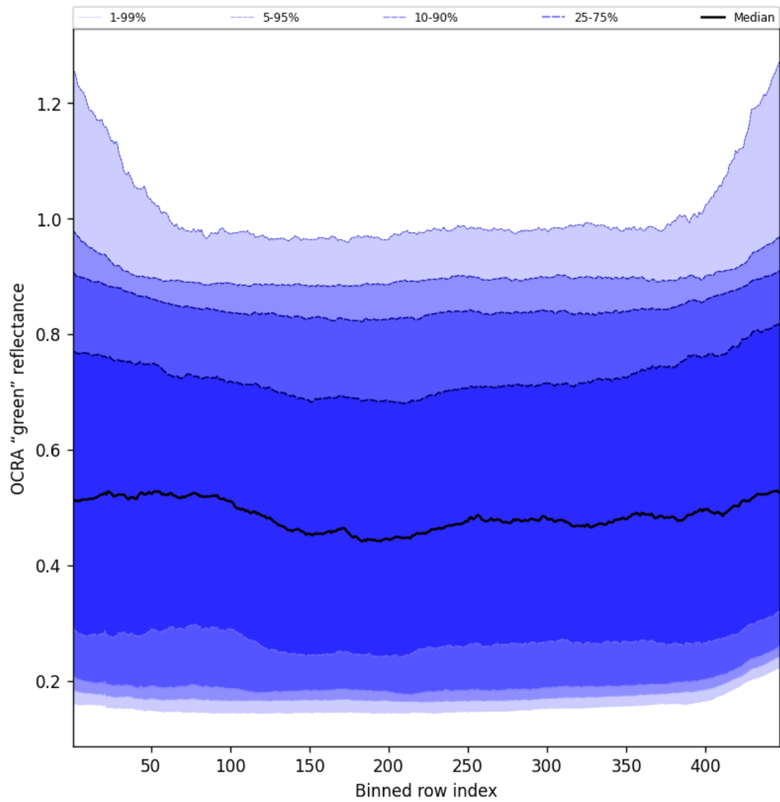
Figure 66: Along track statistics of “OCRA “green” reflectance” for 2025-05-17 to 2025-05-18
