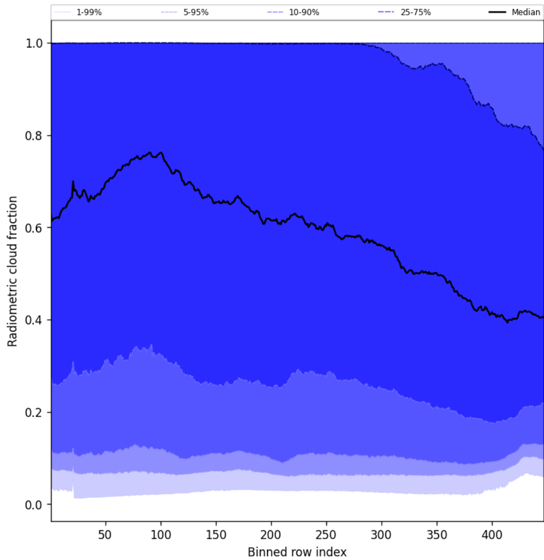
Figure 53: Along track statistics of “Radiometric cloud fraction” for 2025-05-17 to 2025-05-18
