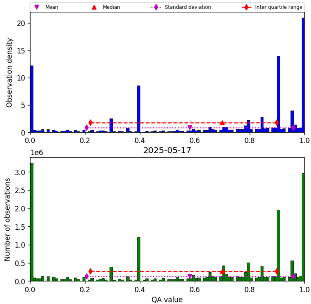
Figure 36: Histogram of “QA value” for 2025-05-17 to 2025-05-18
