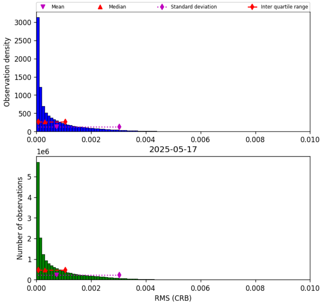
Figure 46: Histogram of “RMS (CRB)” for 2025-05-17 to 2025-05-18
