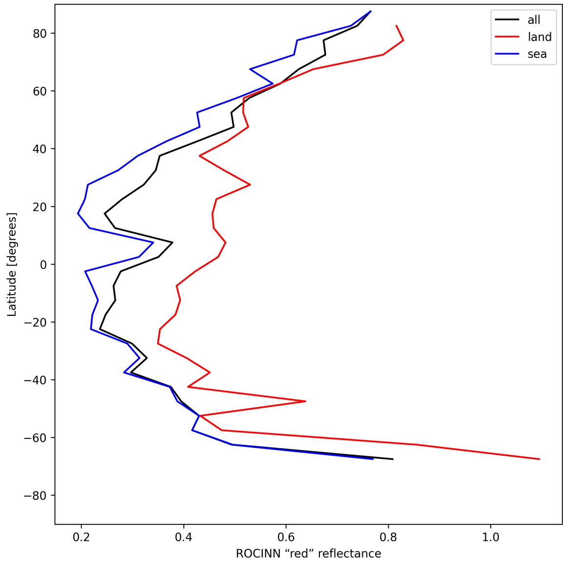
Figure 35: Zonal average of “ROCINN “red” reflectance” for 2025-05-17 to 2025-05-18.
