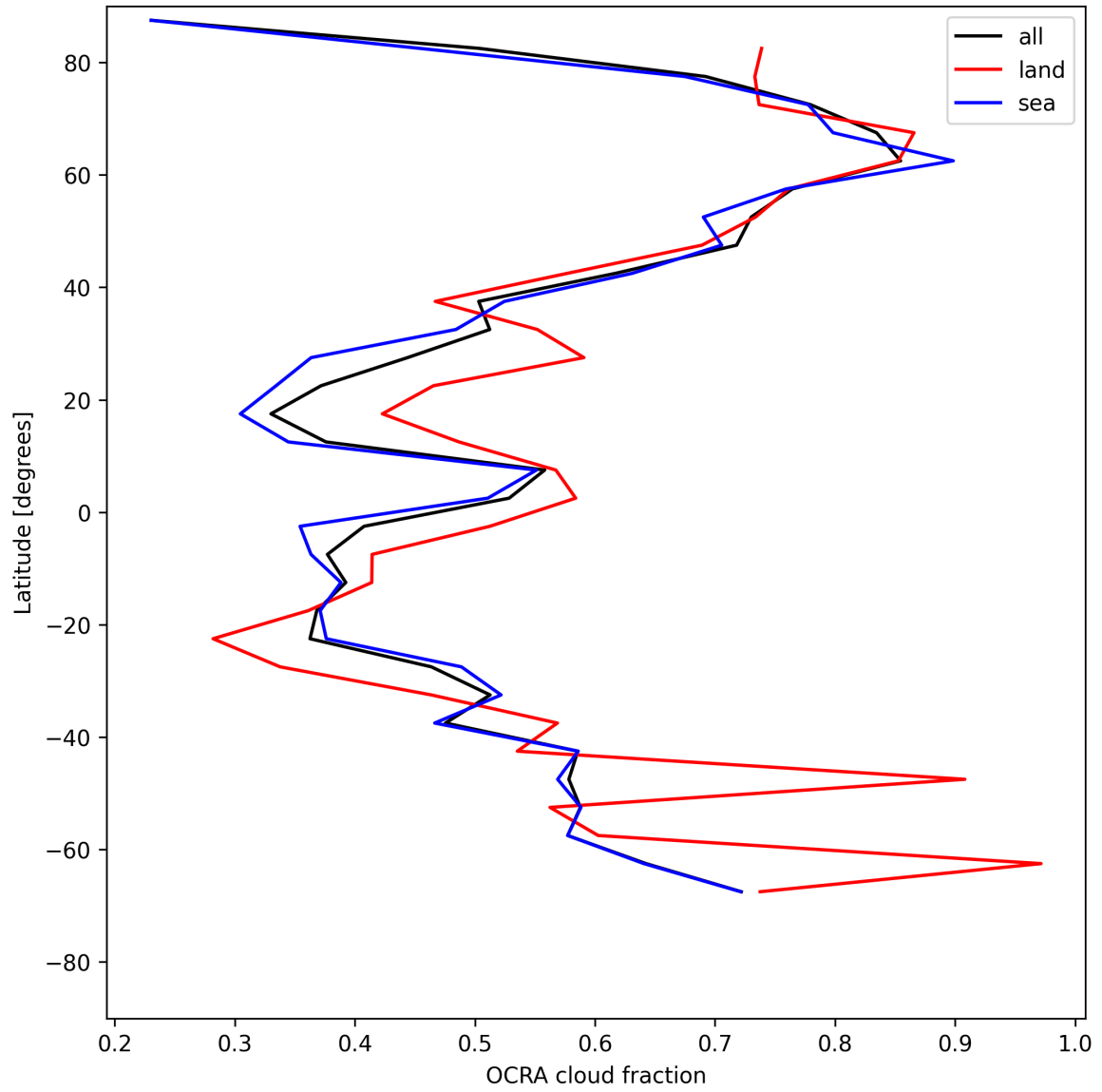
Figure 32: Zonal average of “OCRA cloud fraction” for 2025-05-17 to 2025-05-18.
