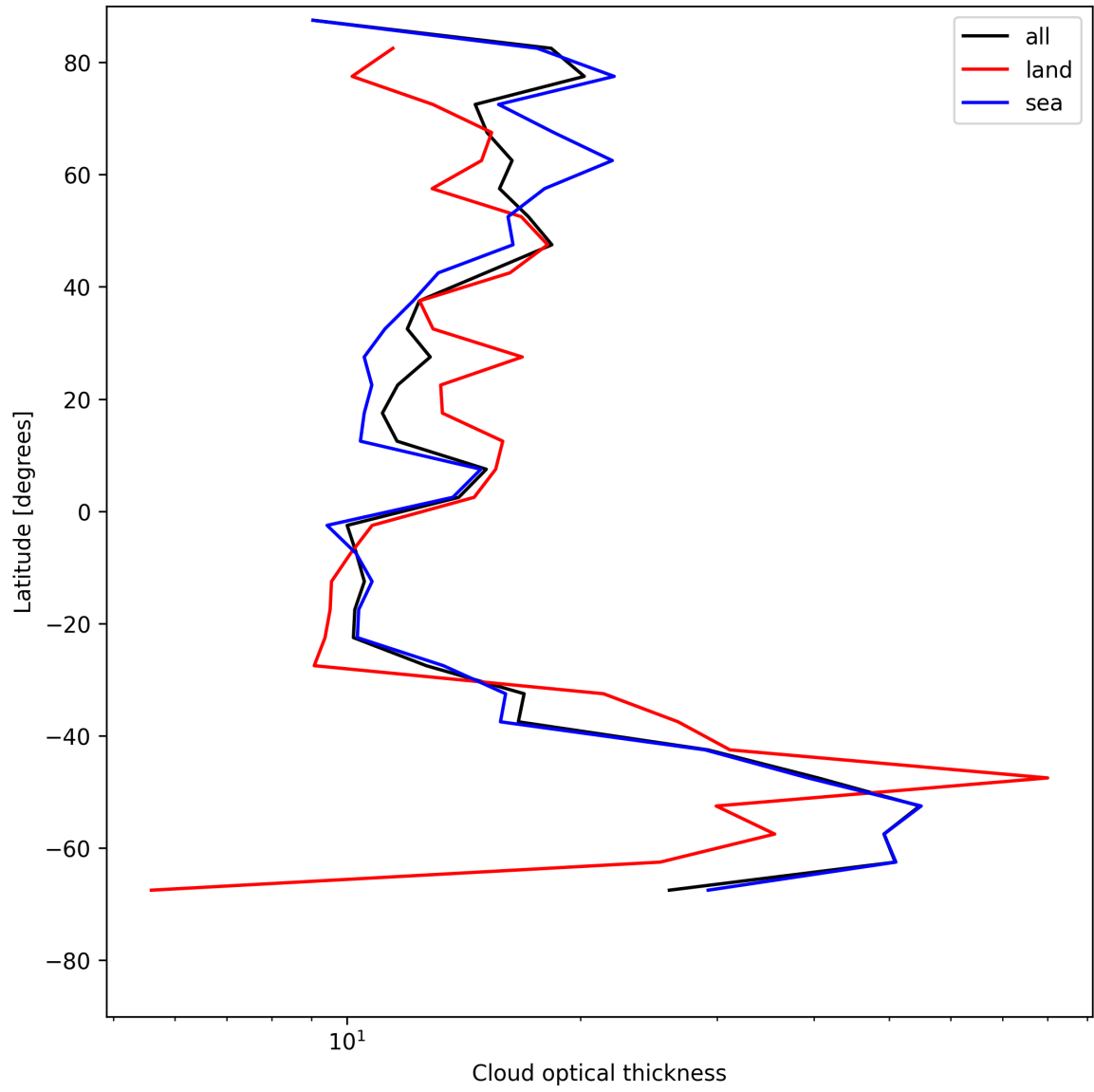
Figure 23: Zonal average of “Cloud optical thickness” for 2025-05-17 to 2025-05-18.
