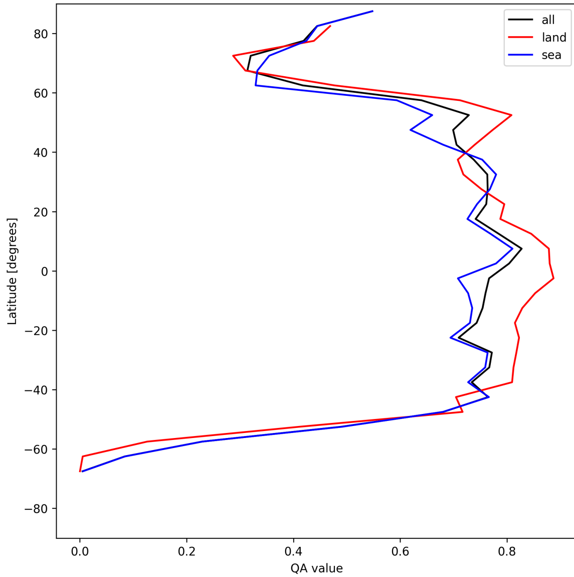
Figure 20: Zonal average of “QA value” for 2025-05-17 to 2025-05-18.
