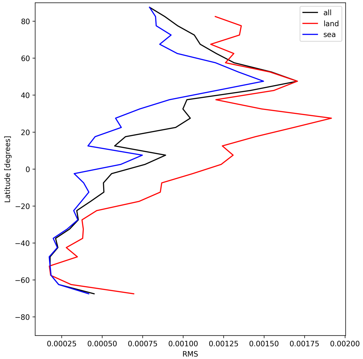
Figure 29: Zonal average of “RMS” for 2025-05-17 to 2025-05-18.
