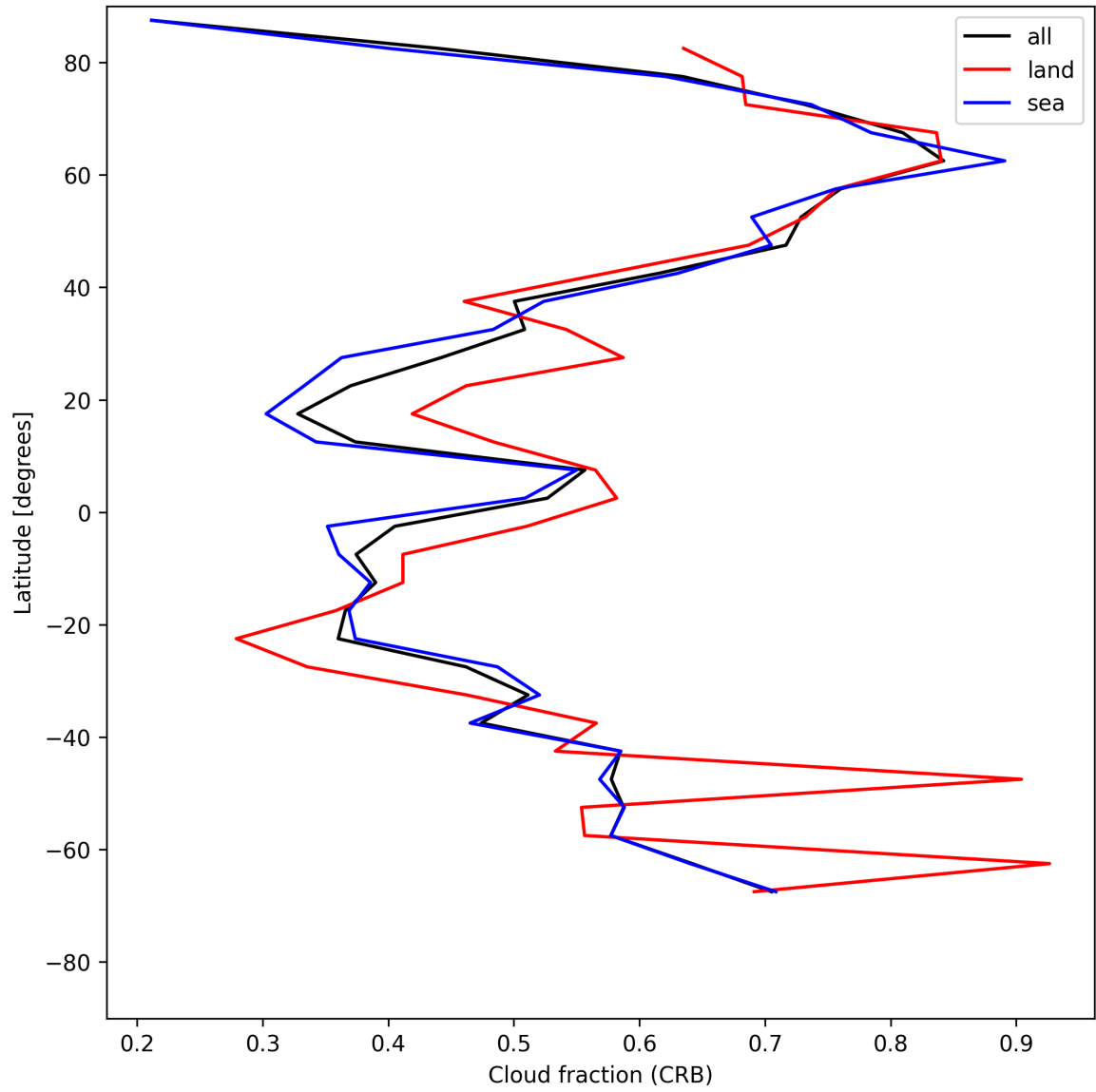
Figure 24: Zonal average of “Cloud fraction (CRB)” for 2025-05-17 to 2025-05-18.
