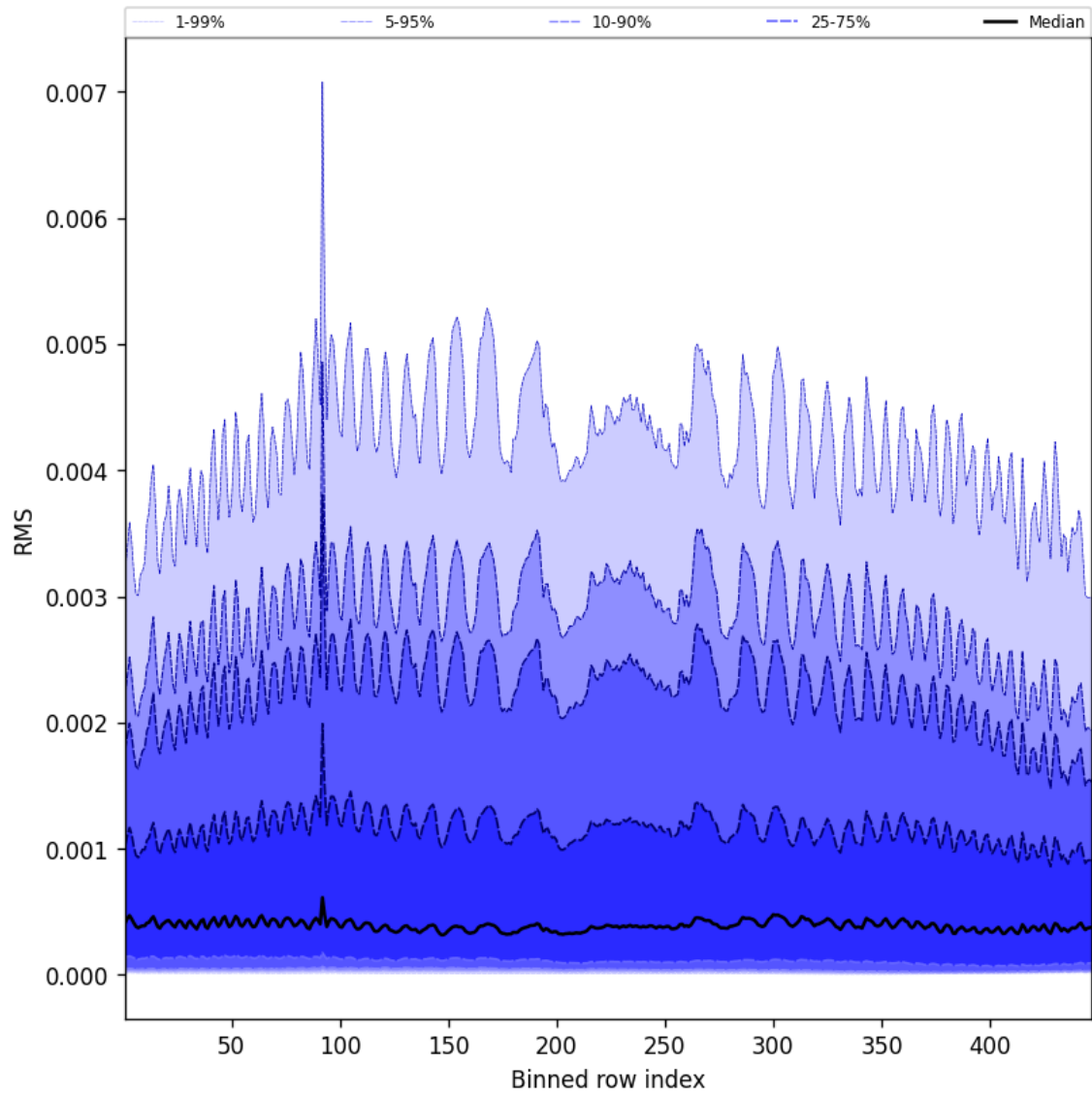
Figure 61: Along track statistics of “RMS” for 2025-05-17 to 2025-05-18
