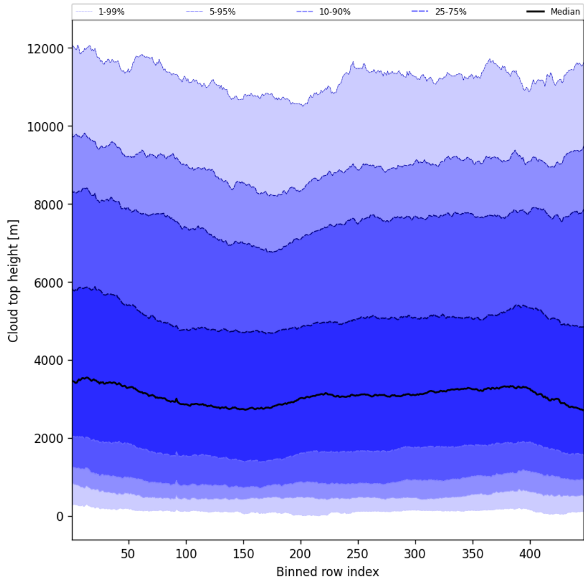
Figure 54: Along track statistics of “Cloud top height” for 2025-05-17 to 2025-05-18
