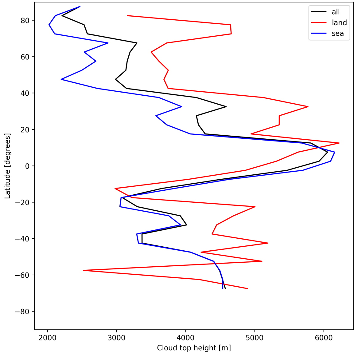
Figure 22: Zonal average of “Cloud top height” for 2025-05-17 to 2025-05-18.
