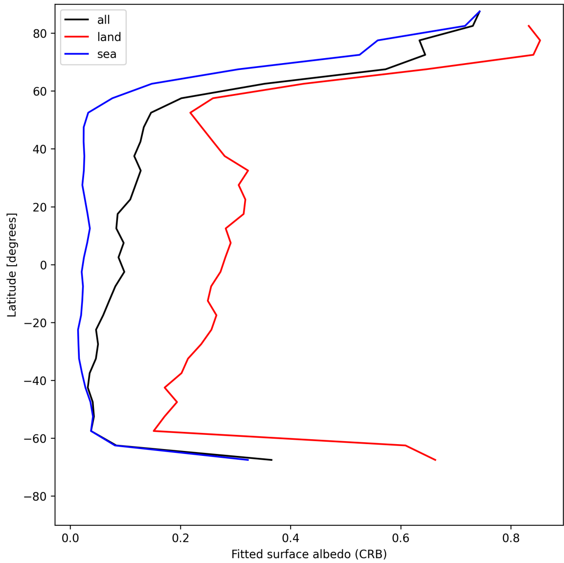
Figure 28: Zonal average of “Fitted surface albedo (CRB)” for 2025-05-17 to 2025-05-18.
