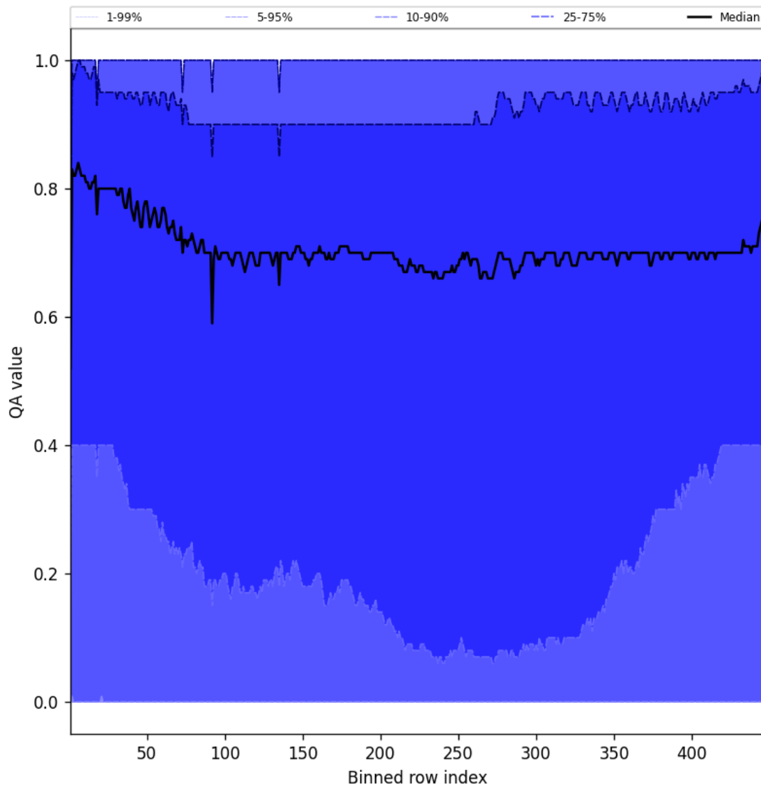
Figure 52: Along track statistics of “QA value” for 2025-05-17 to 2025-05-18
