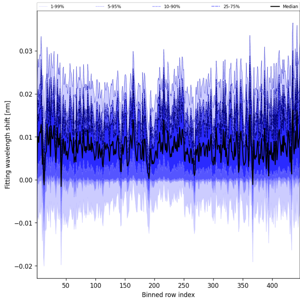
Figure 63: Along track statistics of “Fitting wavelength shift” for 2025-05-17 to 2025-05-18
