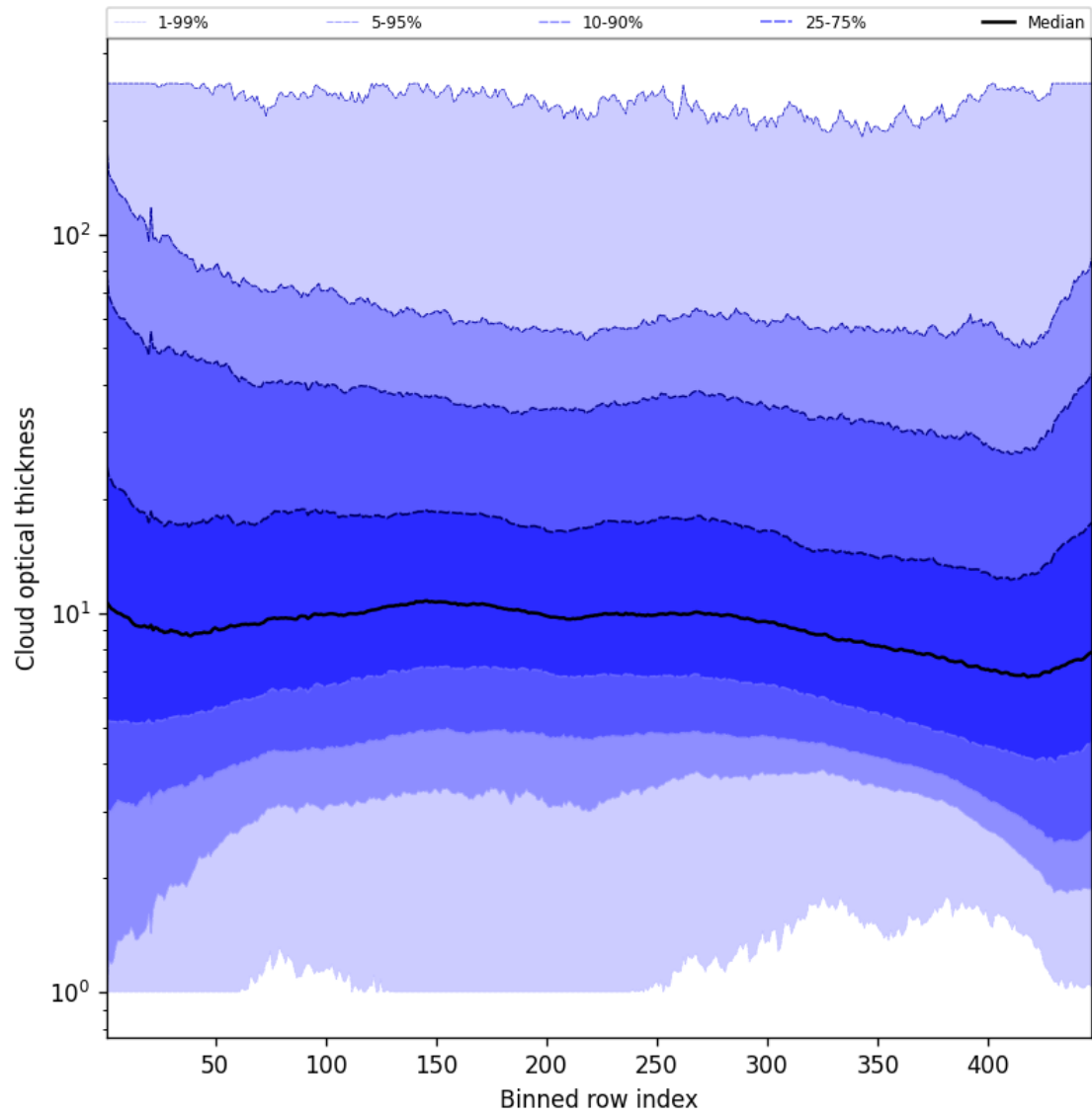
Figure 55: Along track statistics of “Cloud optical thickness” for 2025-05-17 to 2025-05-18
