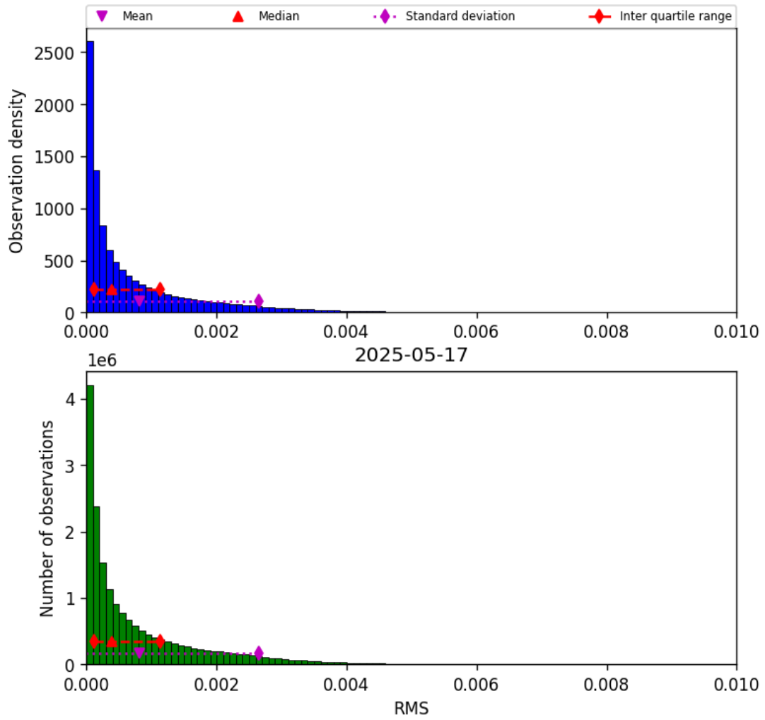
Figure 45: Histogram of “RMS” for 2025-05-17 to 2025-05-18
