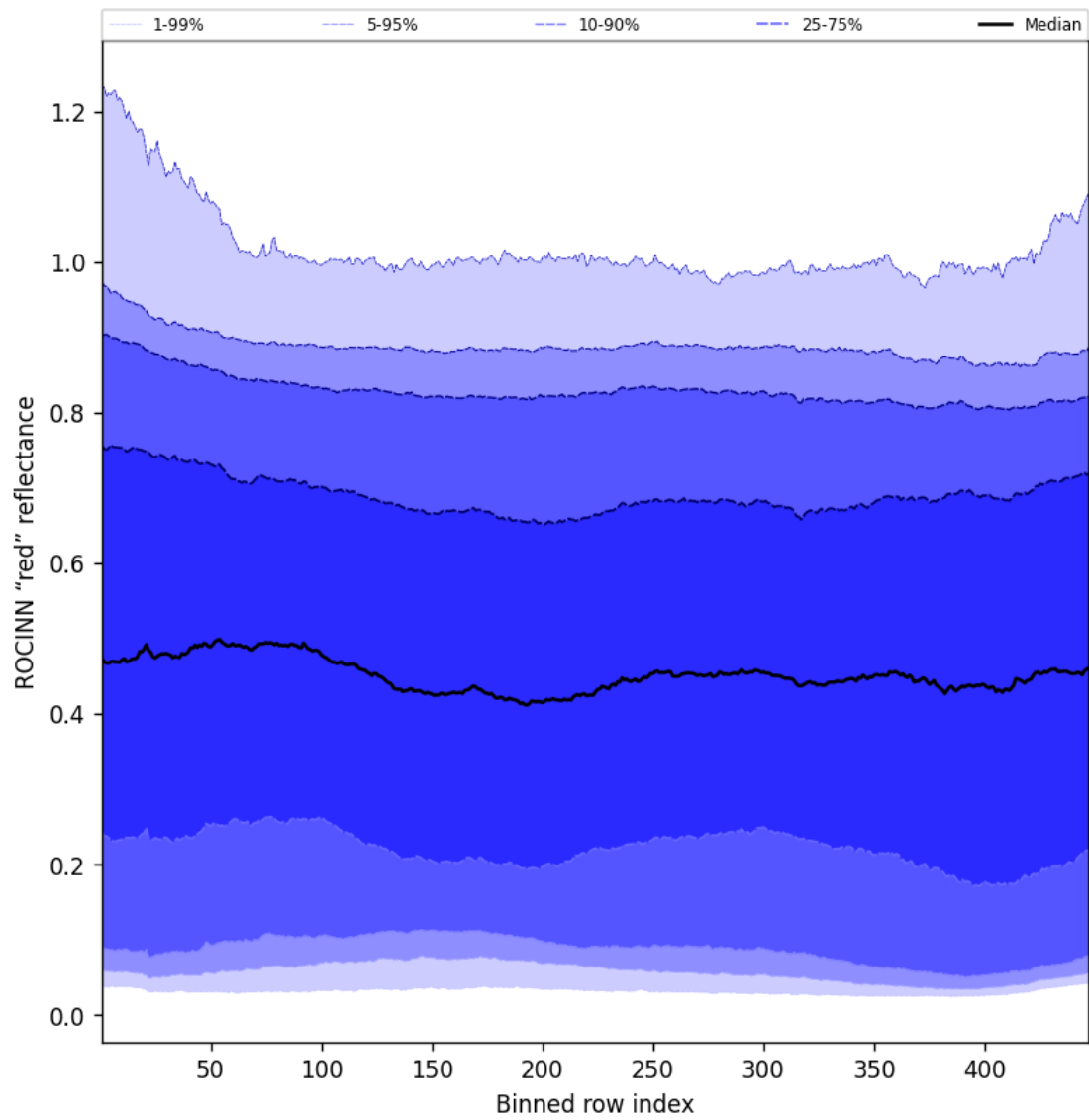
Figure 67: Along track statistics of "ROCINN "red" reflectance" for 2025-05-17 to 2025-05-18
