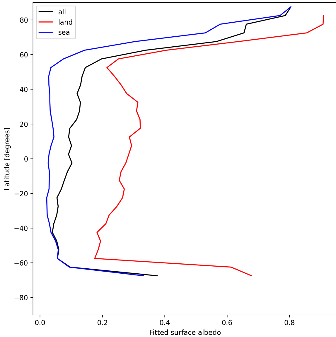
Figure 27: Zonal average of “Fitted surface albedo” for 2025-05-17 to 2025-05-18.
