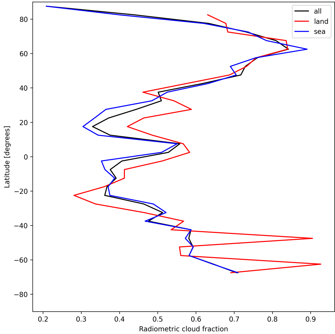
Figure 21: Zonal average of “Radiometric cloud fraction” for 2025-05-17 to 2025-05-18.
