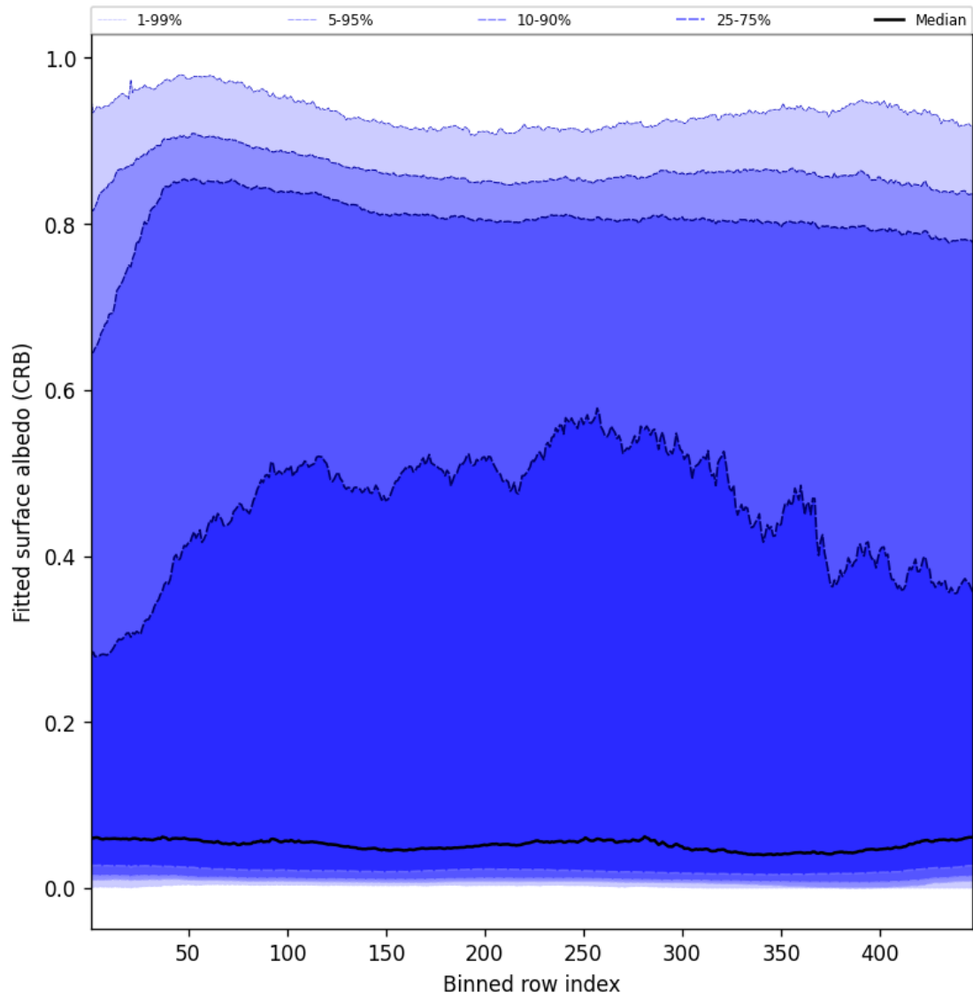
Figure 60: Along track statistics of “Fitted surface albedo (CRB)” for 2025-05-17 to 2025-05-18
