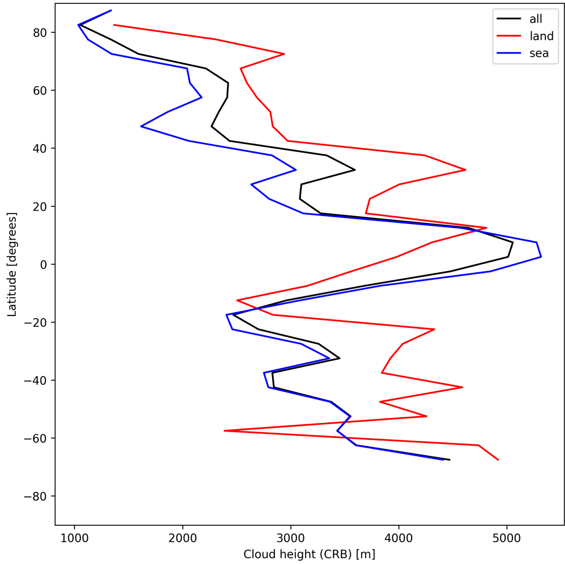
Figure 25: Zonal average of “Cloud height (CRB)” for 2025-05-17 to 2025-05-18.
