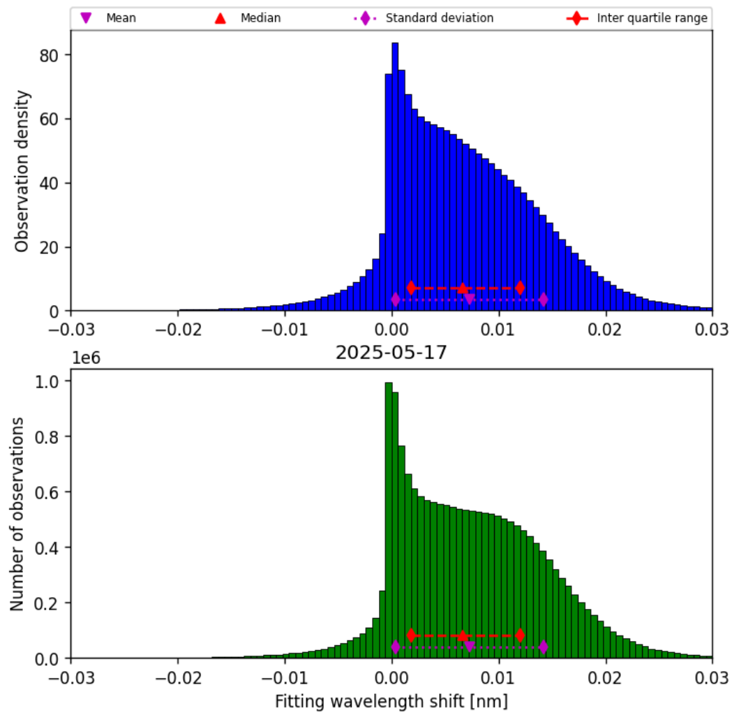
Figure 47: Histogram of “Fitting wavelength shift” for 2025-05-17 to 2025-05-18
