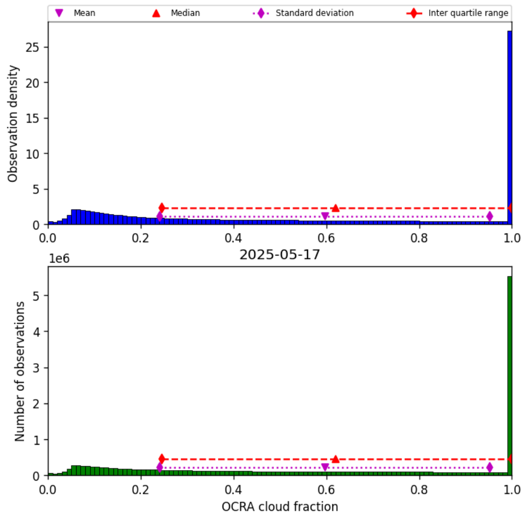
Figure 48: Histogram of “OCRA cloud fraction” for 2025-05-17 to 2025-05-18
