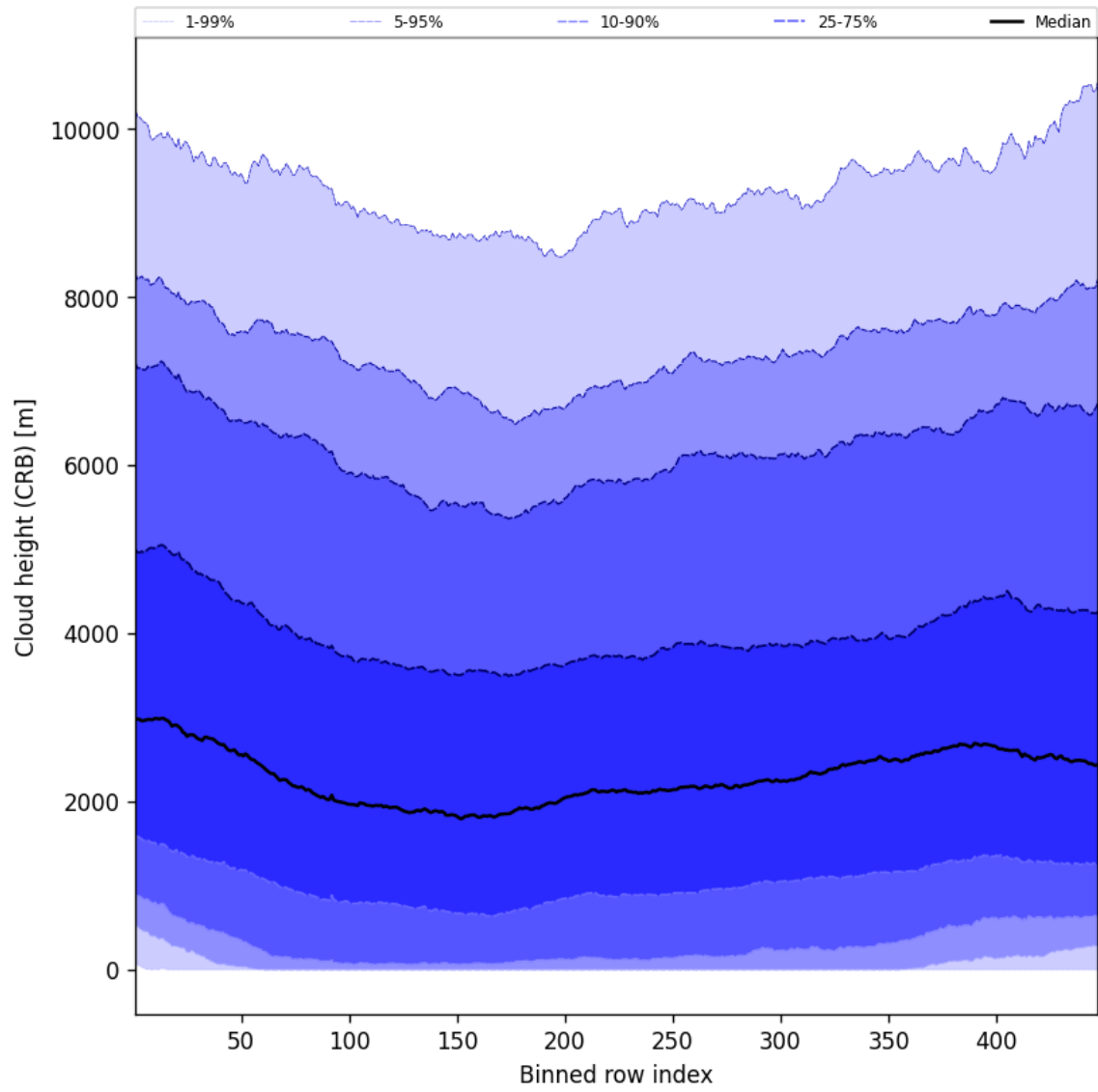
Figure 57: Along track statistics of “Cloud height (CRB)” for 2025-05-17 to 2025-05-18
