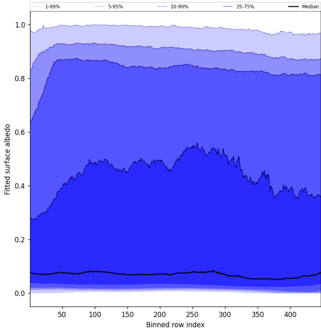
Figure 59: Along track statistics of “Fitted surface albedo” for 2025-05-17 to 2025-05-18
