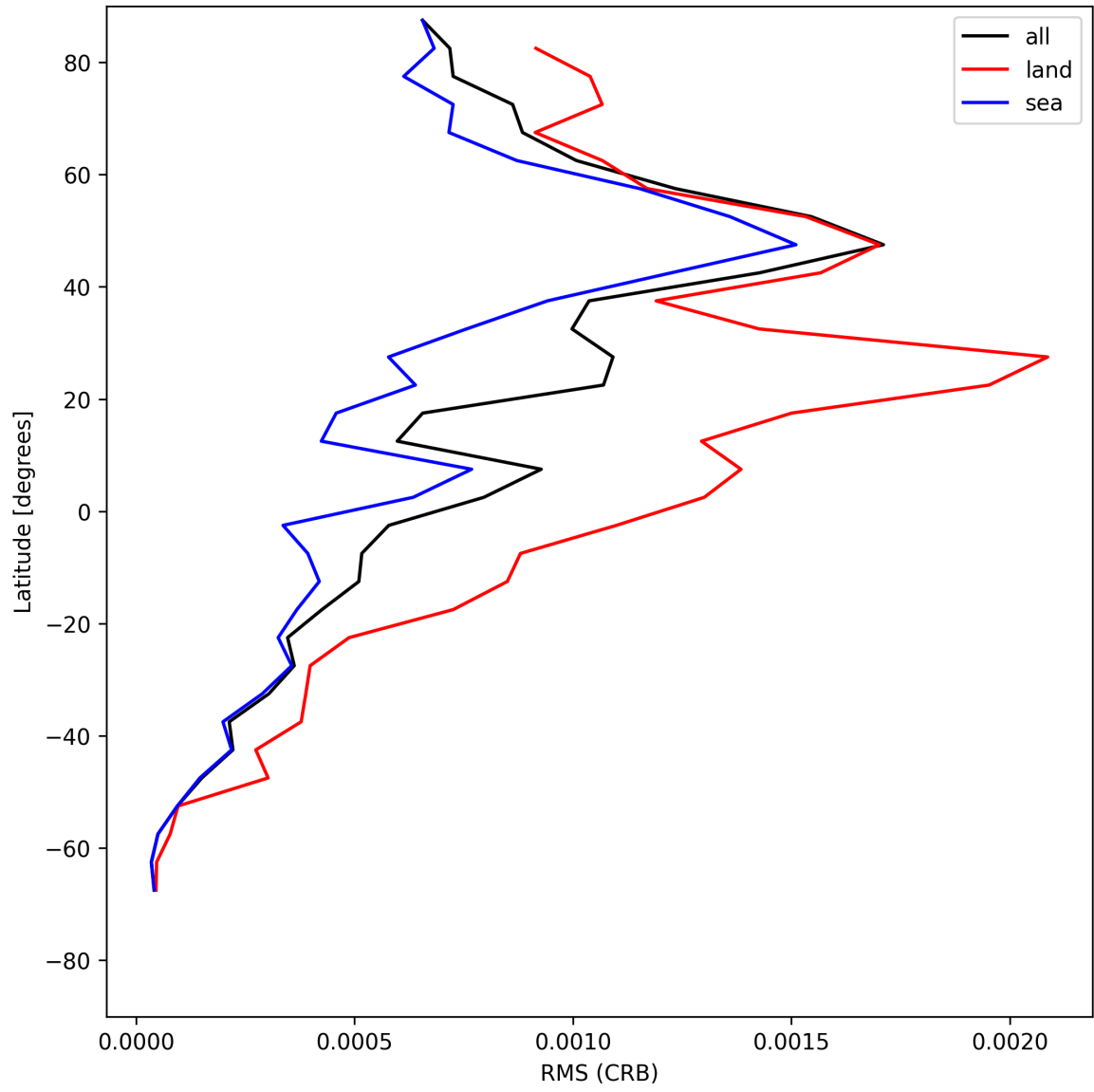
Figure 30: Zonal average of “RMS (CRB)” for 2025-05-17 to 2025-05-18.
