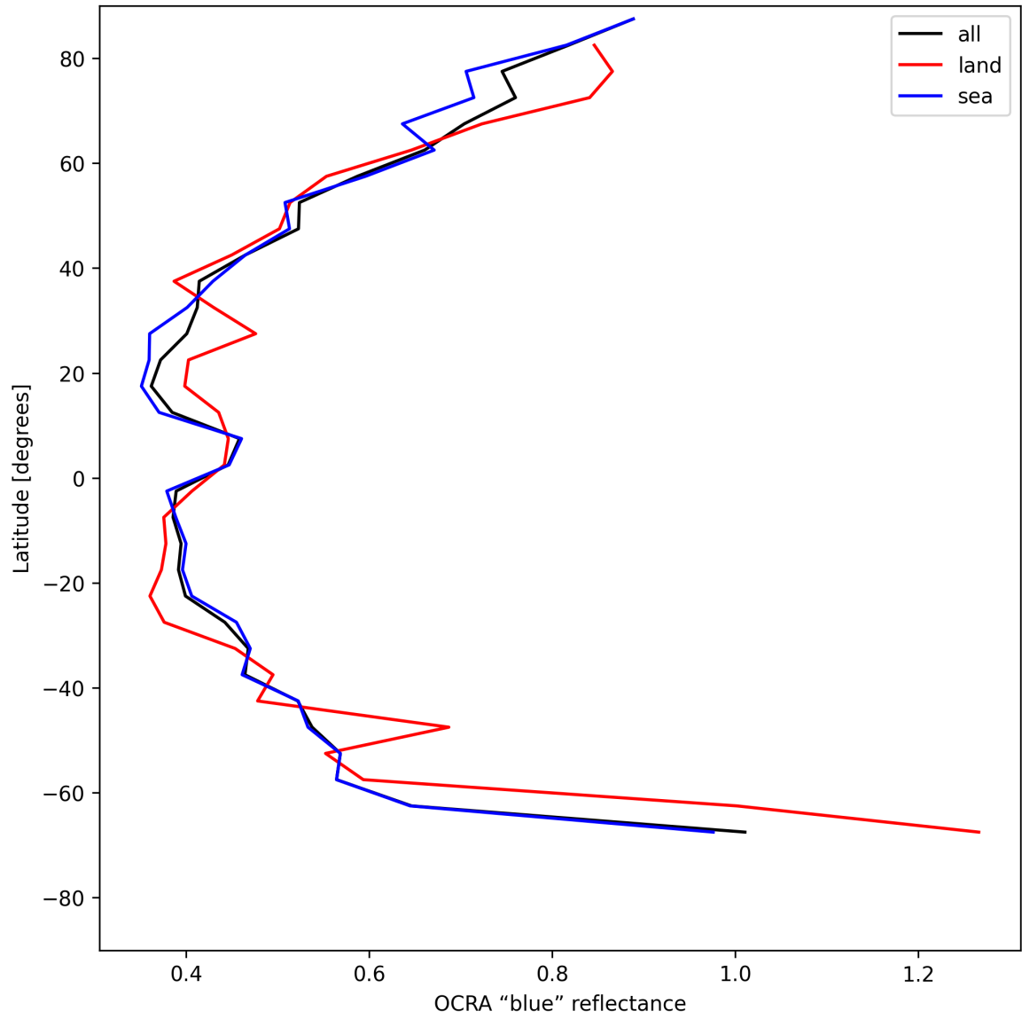
Figure 33: Zonal average of "OCRA "blue" reflectance" for 2025-05-17 to 2025-05-18.
