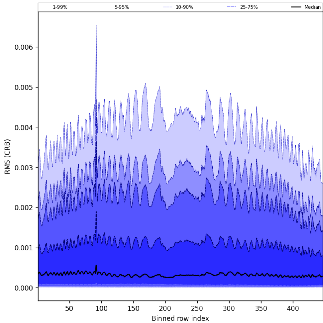
Figure 62: Along track statistics of “RMS (CRB)” for 2025-05-17 to 2025-05-18
