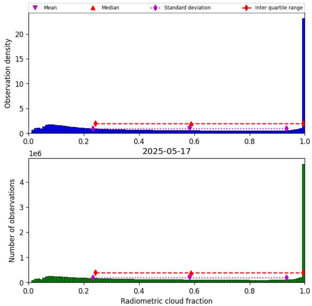
Figure 37: Histogram of “Radiometric cloud fraction” for 2025-05-17 to 2025-05-18
