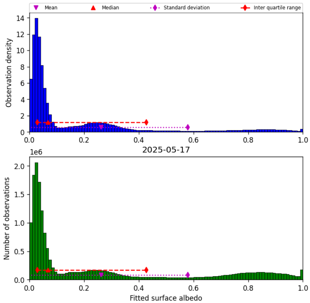
Figure 43: Histogram of “Fitted surface albedo” for 2025-05-17 to 2025-05-18
