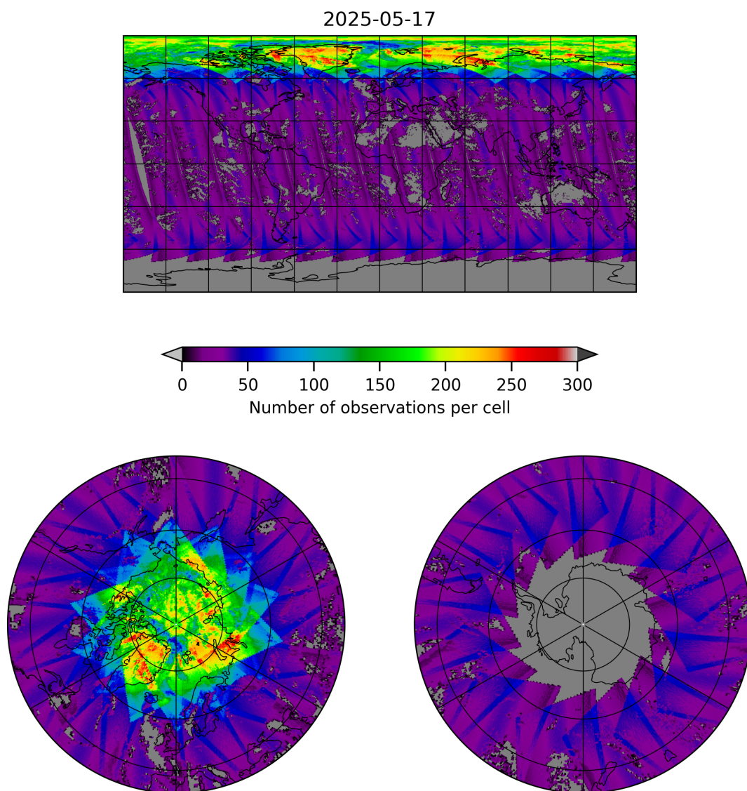
Figure 19: Map of the number of observations for 2025-05-17 to 2025-05-18
