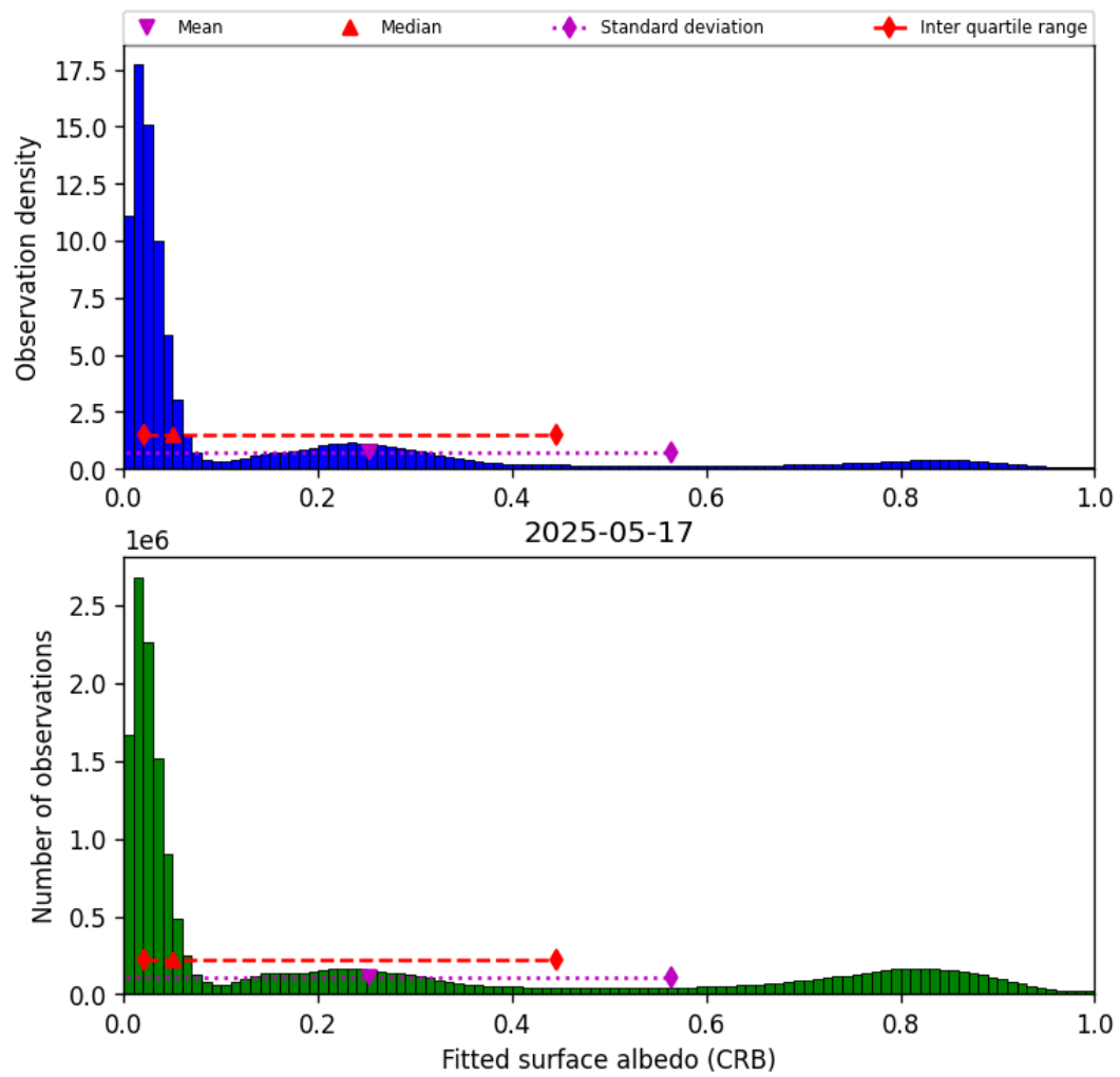
Figure 44: Histogram of “Fitted surface albedo (CRB)” for 2025-05-17 to 2025-05-18
