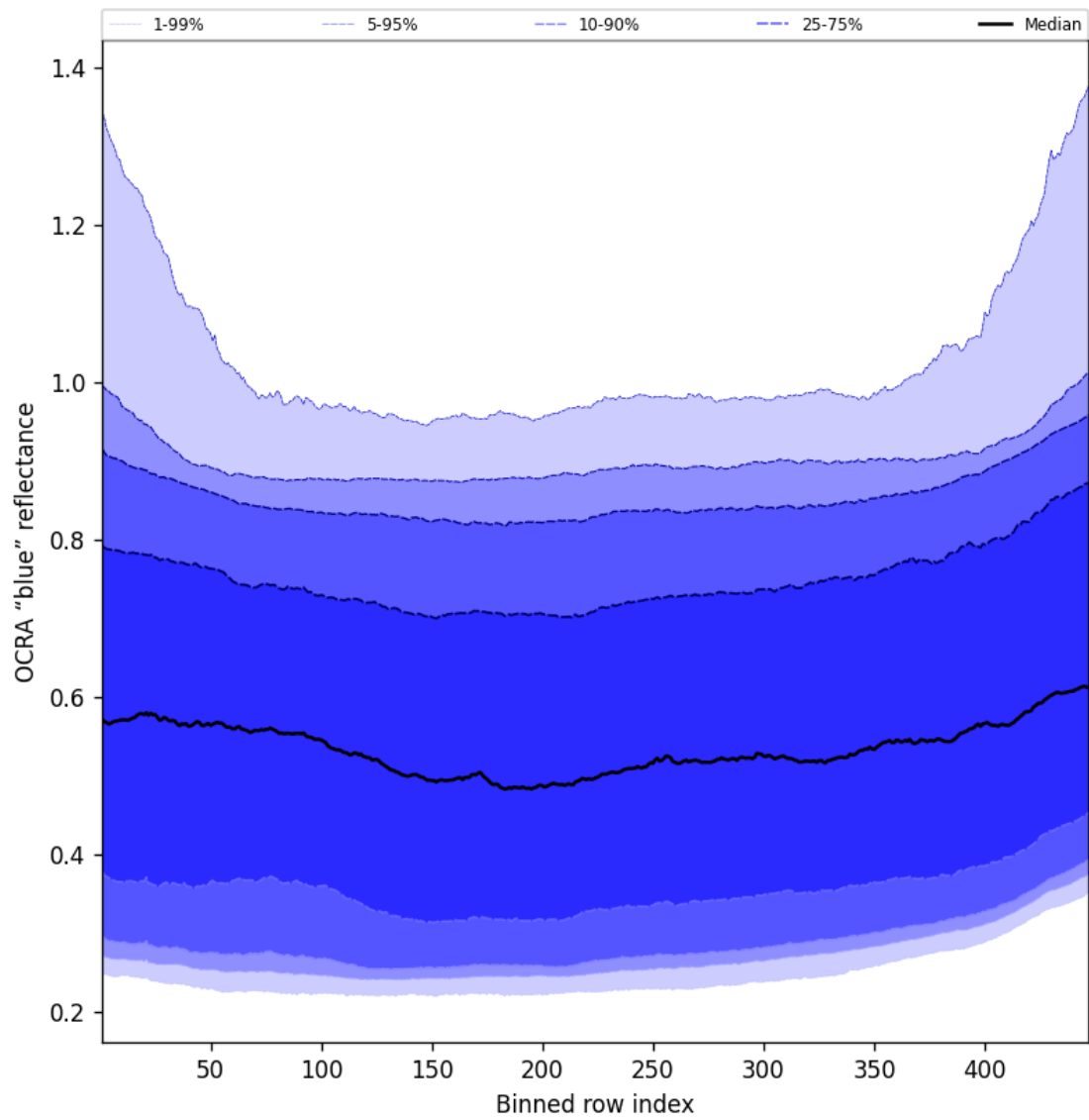
Figure 65: Along track statistics of “OCRA “blue” reflectance” for 2025-05-17 to 2025-05-18
