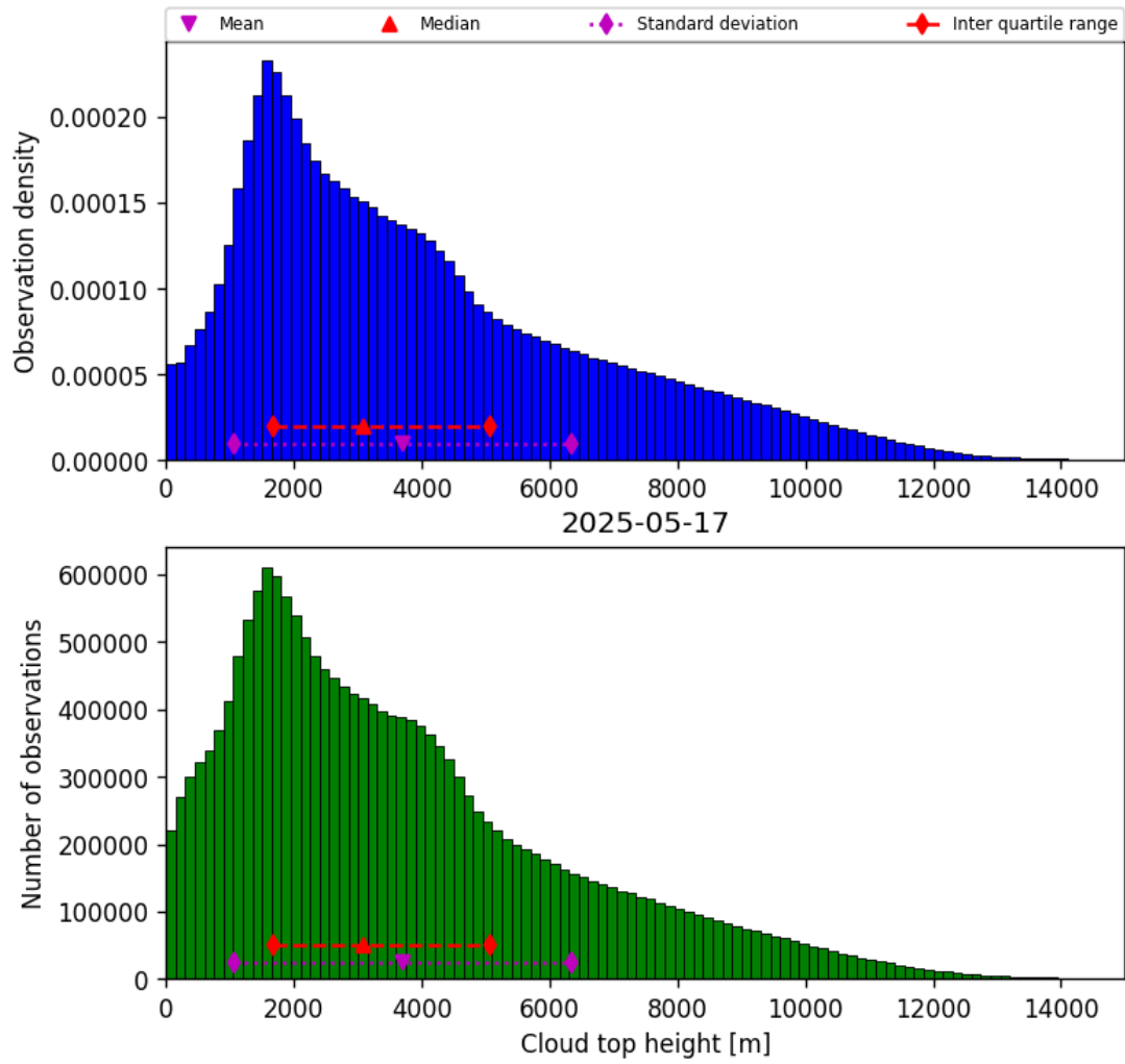
Figure 38: Histogram of “Cloud top height” for 2025-05-17 to 2025-05-18
