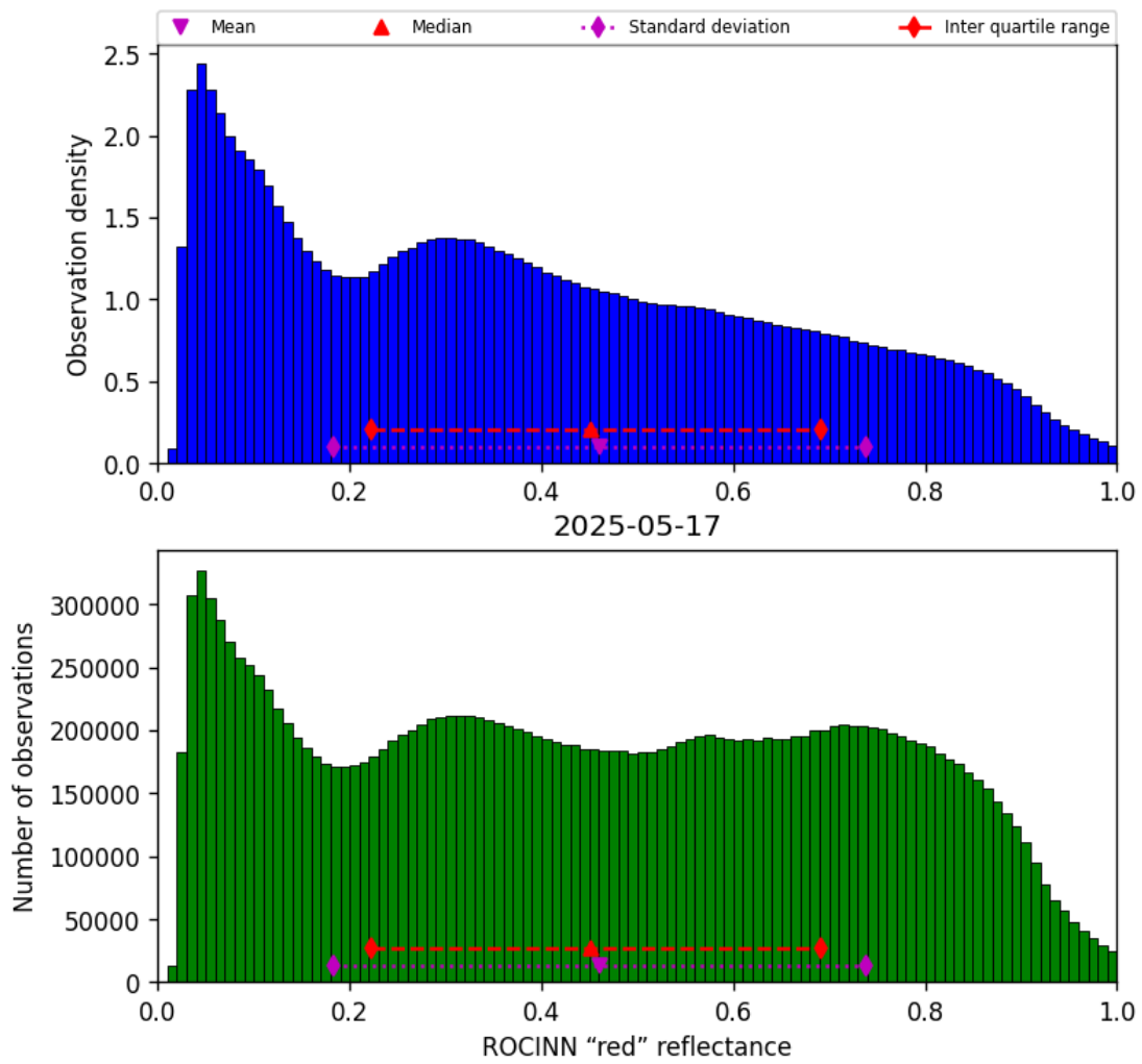
Figure 51: Histogram of “ROCINN “red” reflectance” for 2025-05-17 to 2025-05-18
