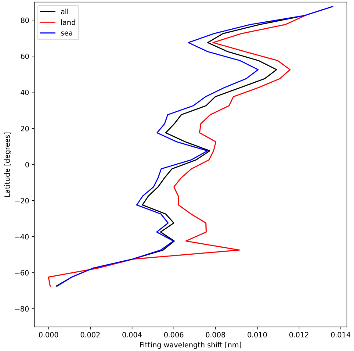
Figure 31: Zonal average of “Fitting wavelength shift” for 2025-05-17 to 2025-05-18.
