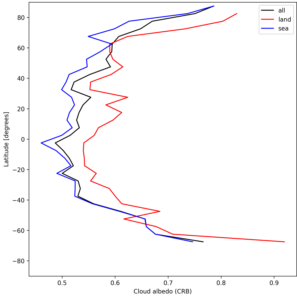
Figure 26: Zonal average of “Cloud albedo (CRB)” for 2025-05-17 to 2025-05-18.
