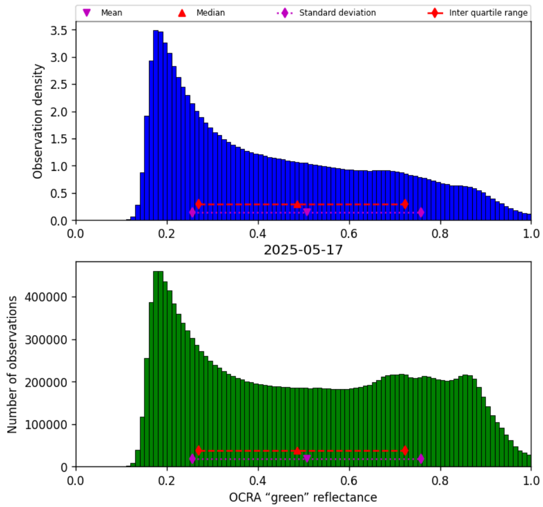
Figure 50: Histogram of “OCRA “green” reflectance” for 2025-05-17 to 2025-05-18
