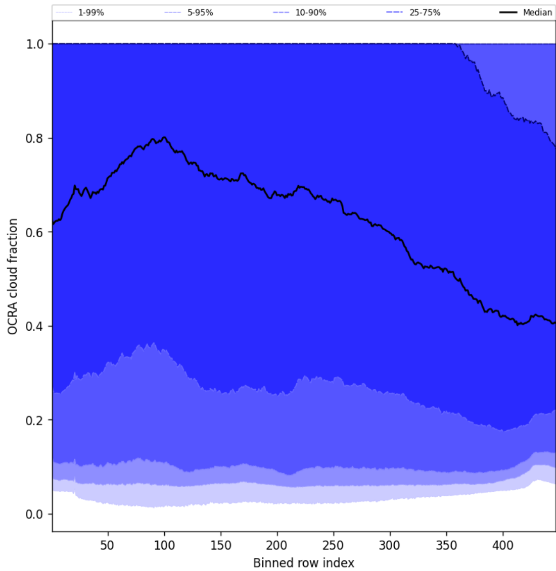
Figure 64: Along track statistics of “OCRA cloud fraction” for 2025-05-17 to 2025-05-18
