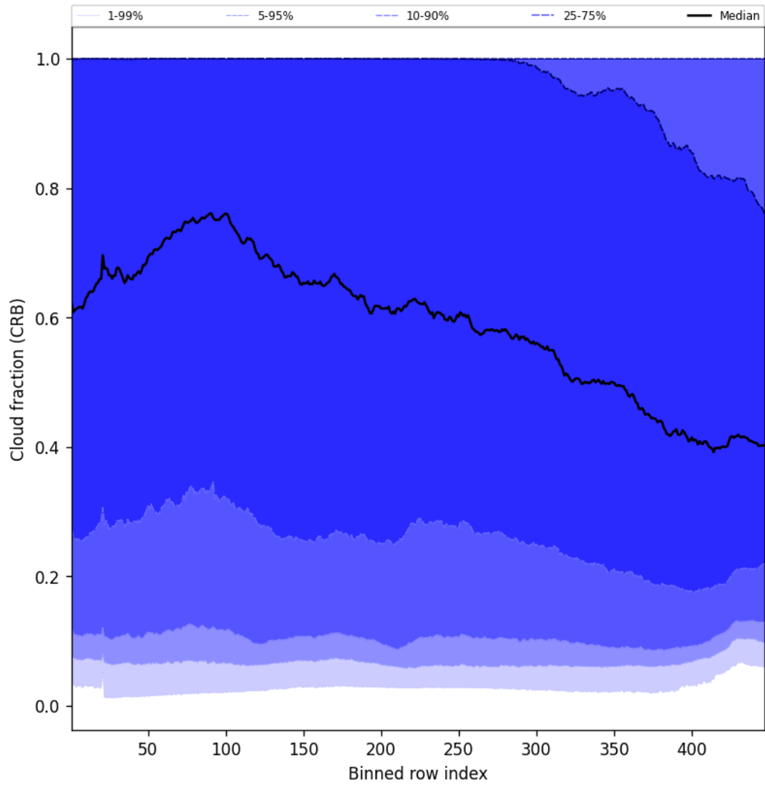
Figure 56: Along track statistics of “Cloud fraction (CRB)” for 2025-05-17 to 2025-05-18
