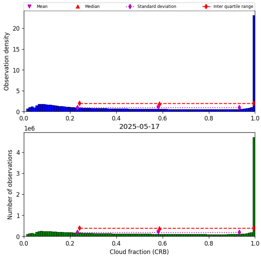
Figure 40: Histogram of “Cloud fraction (CRB)” for 2025-05-17 to 2025-05-18
