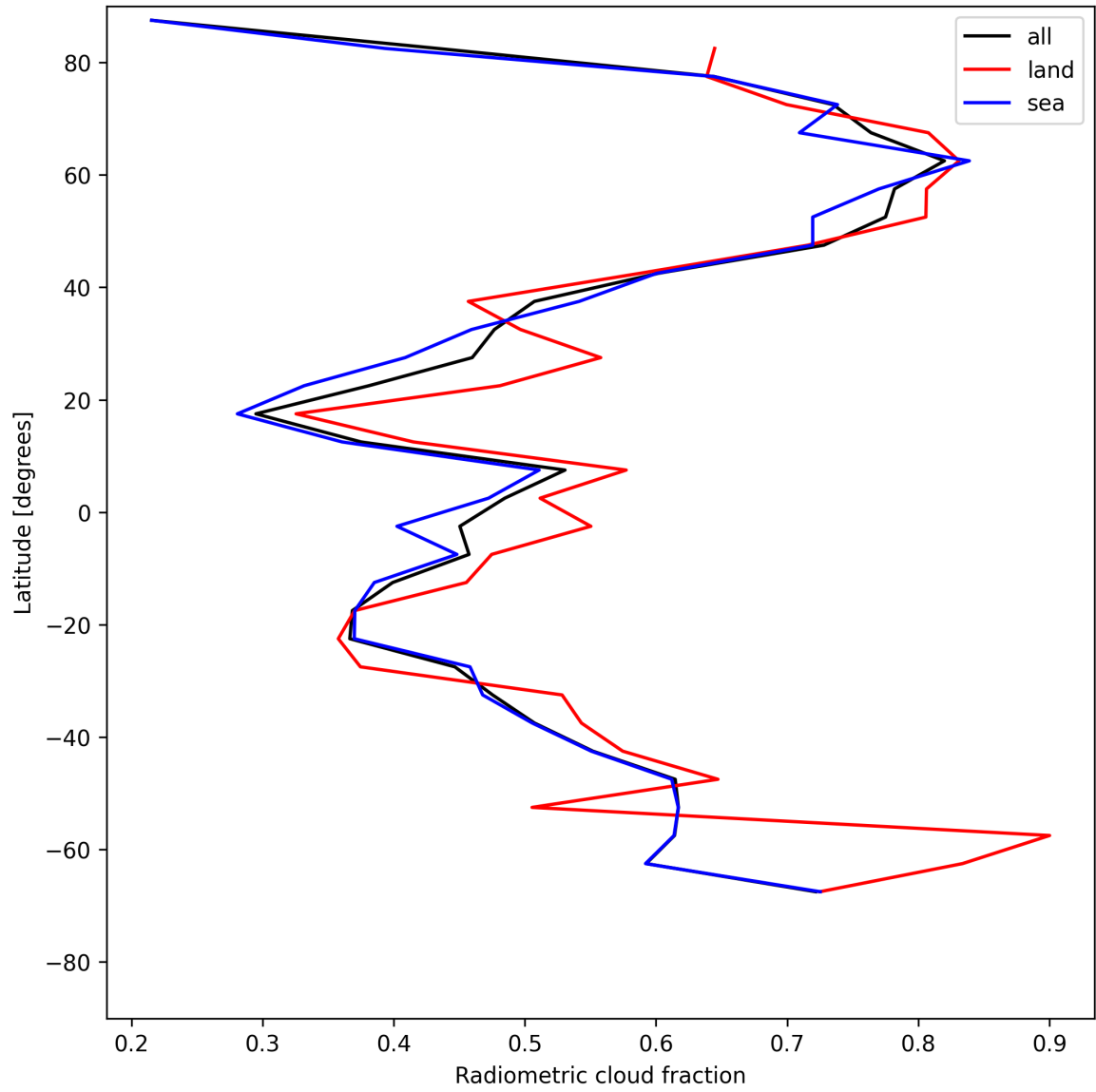
Figure 21: Zonal average of “Radiometric cloud fraction” for 2025-05-18 to 2025-05-19.
