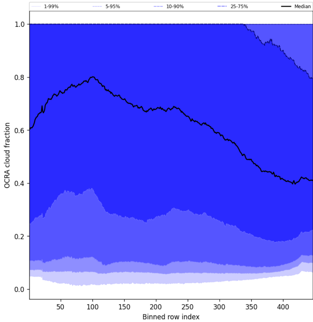
Figure 64: Along track statistics of “OCRA cloud fraction” for 2025-05-18 to 2025-05-19
