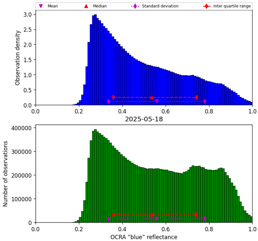
Figure 49: Histogram of “OCRA “blue” reflectance” for 2025-05-18 to 2025-05-19
