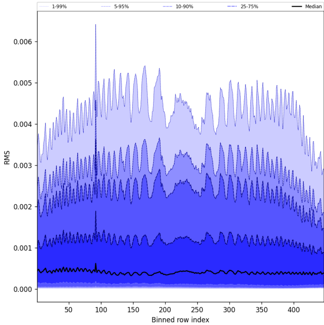
Figure 61: Along track statistics of “RMS” for 2025-05-18 to 2025-05-19
