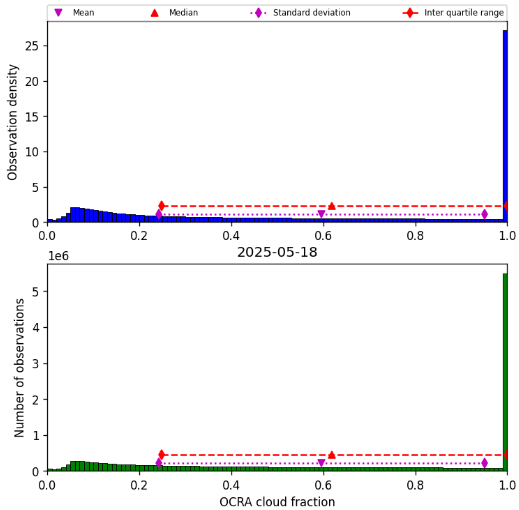
Figure 48: Histogram of “OCRA cloud fraction” for 2025-05-18 to 2025-05-19
