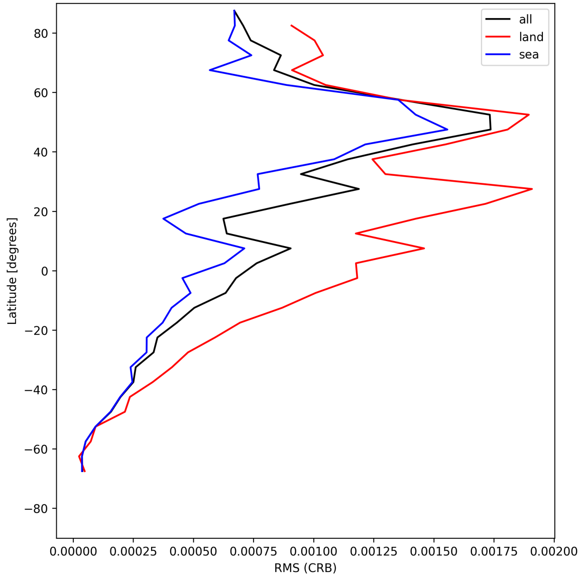
Figure 30: Zonal average of “RMS (CRB)” for 2025-05-18 to 2025-05-19.
