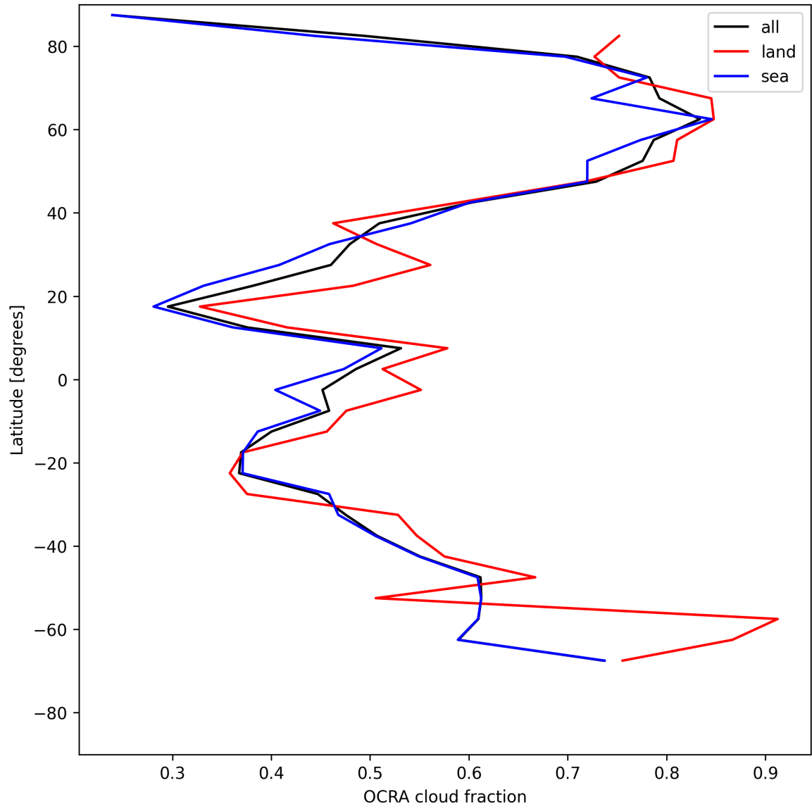
Figure 32: Zonal average of “OCRA cloud fraction” for 2025-05-18 to 2025-05-19.
