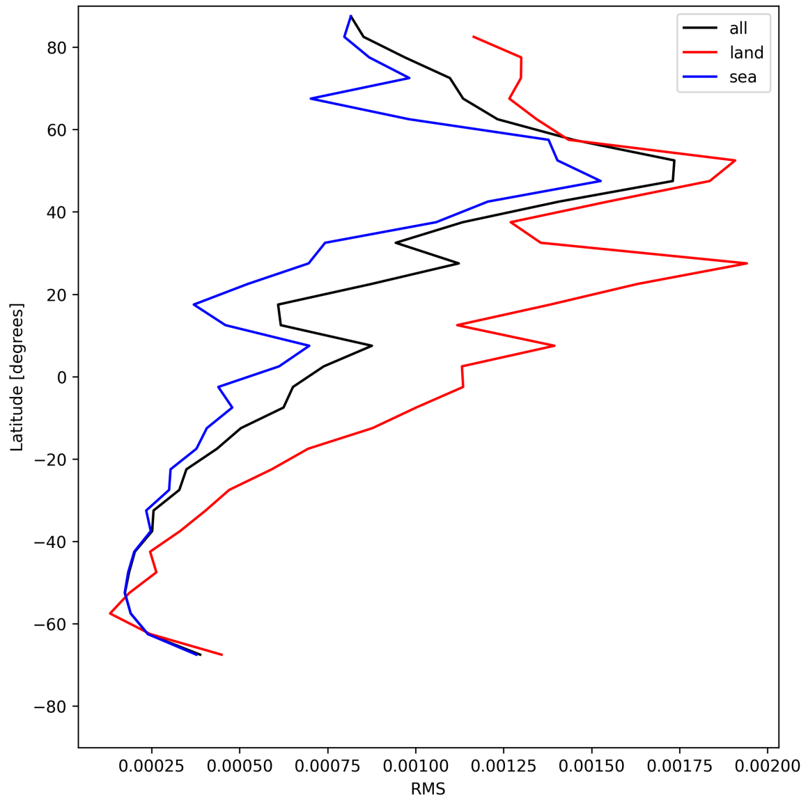
Figure 29: Zonal average of “RMS” for 2025-05-18 to 2025-05-19.
