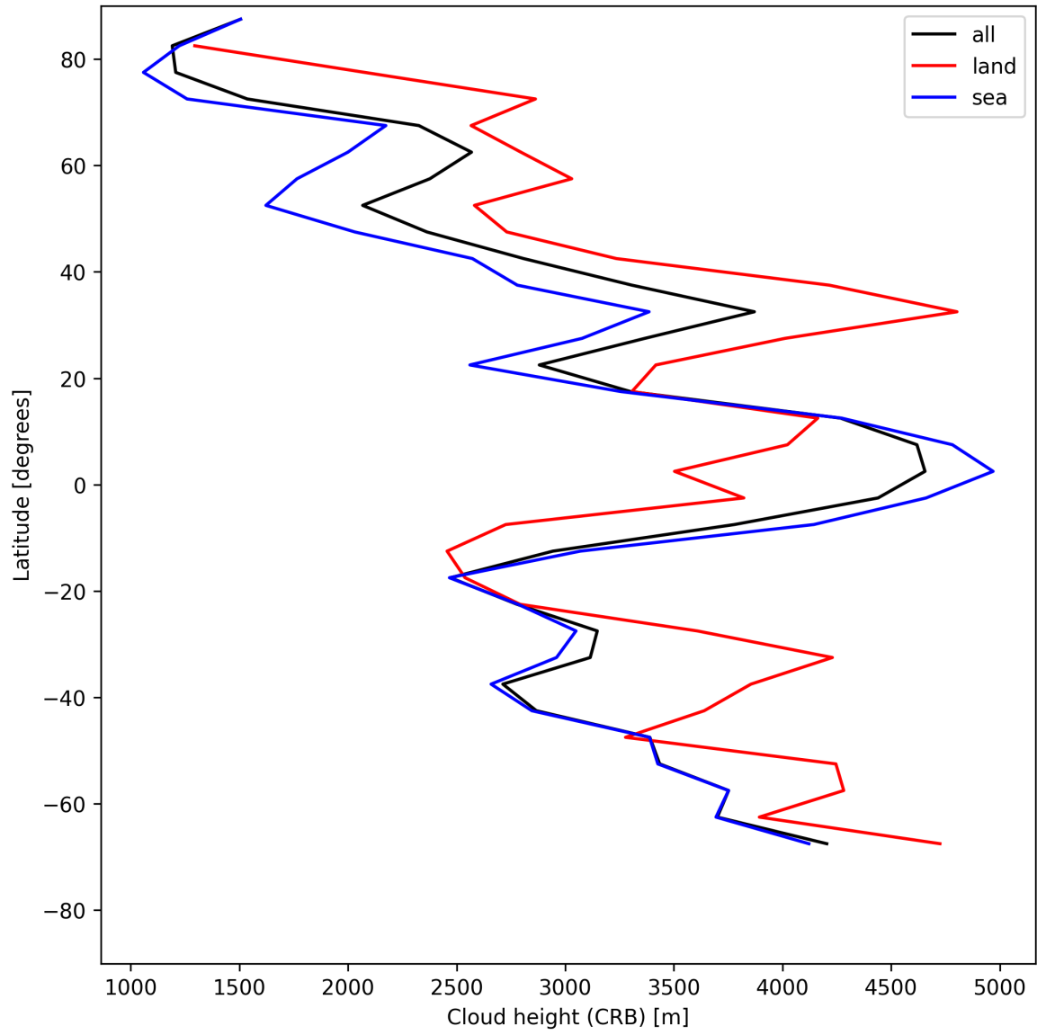
Figure 25: Zonal average of “Cloud height (CRB)” for 2025-05-18 to 2025-05-19.
