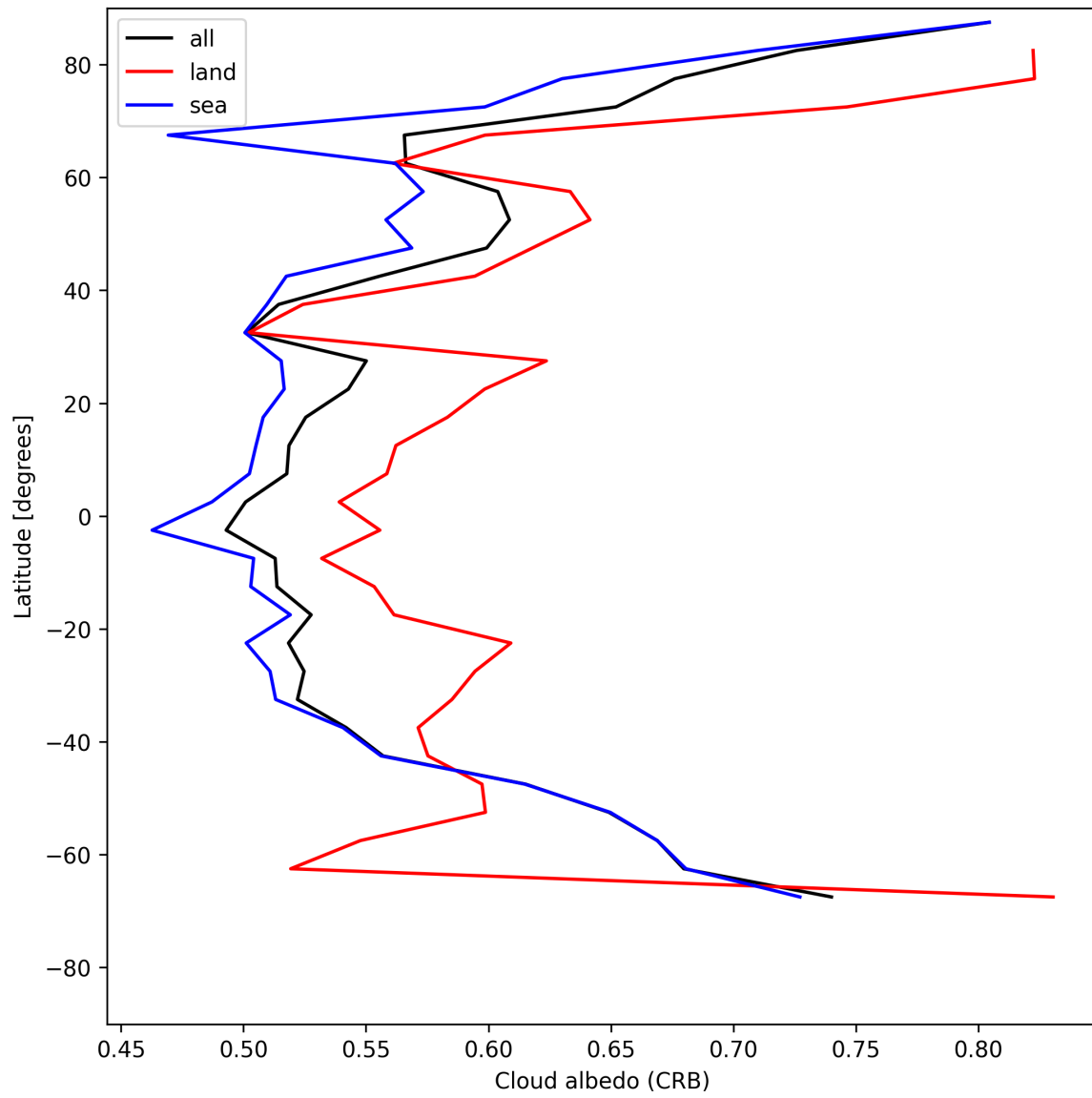
Figure 26: Zonal average of “Cloud albedo (CRB)” for 2025-05-18 to 2025-05-19.
