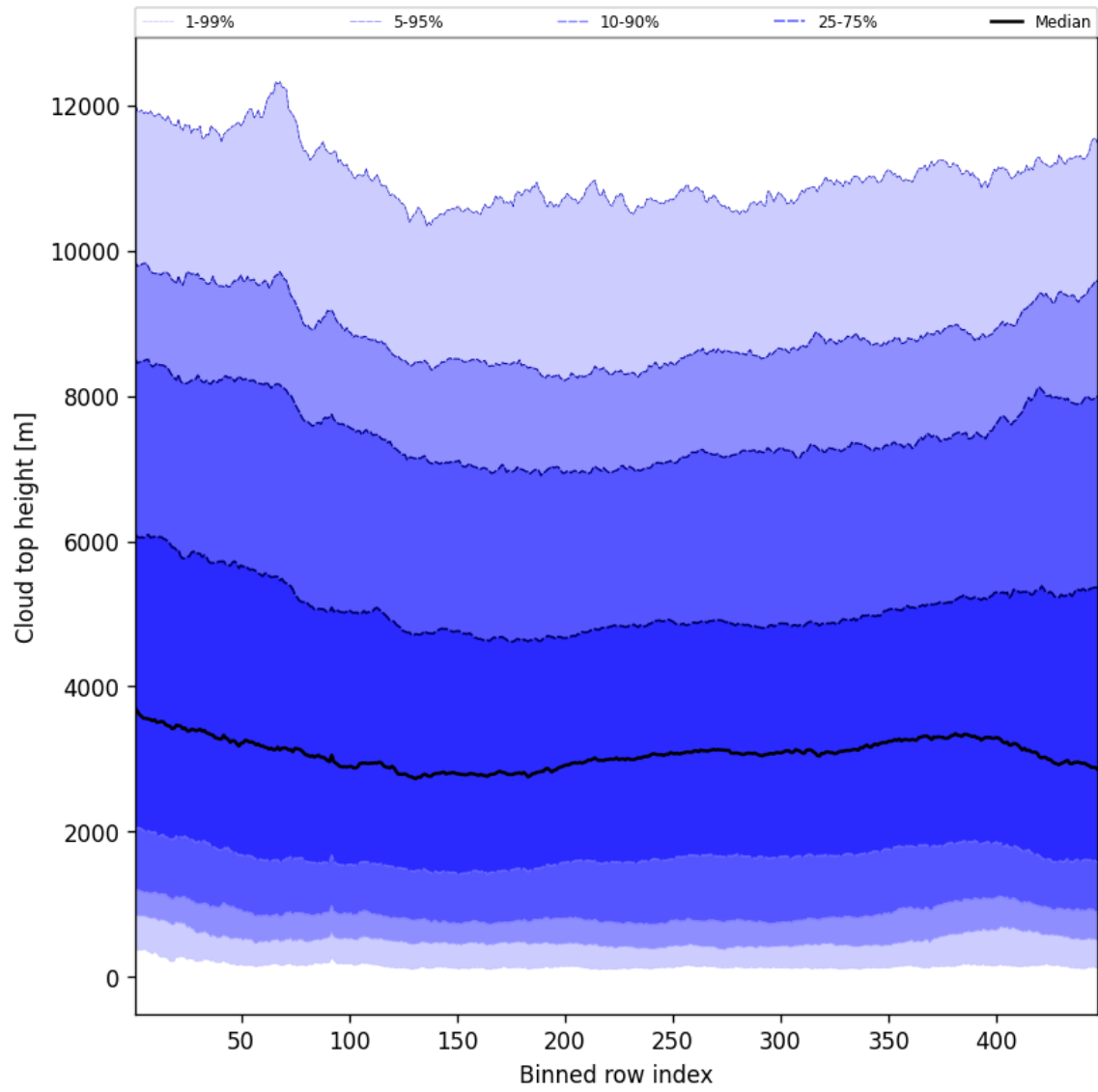
Figure 54: Along track statistics of “Cloud top height” for 2025-05-18 to 2025-05-19
