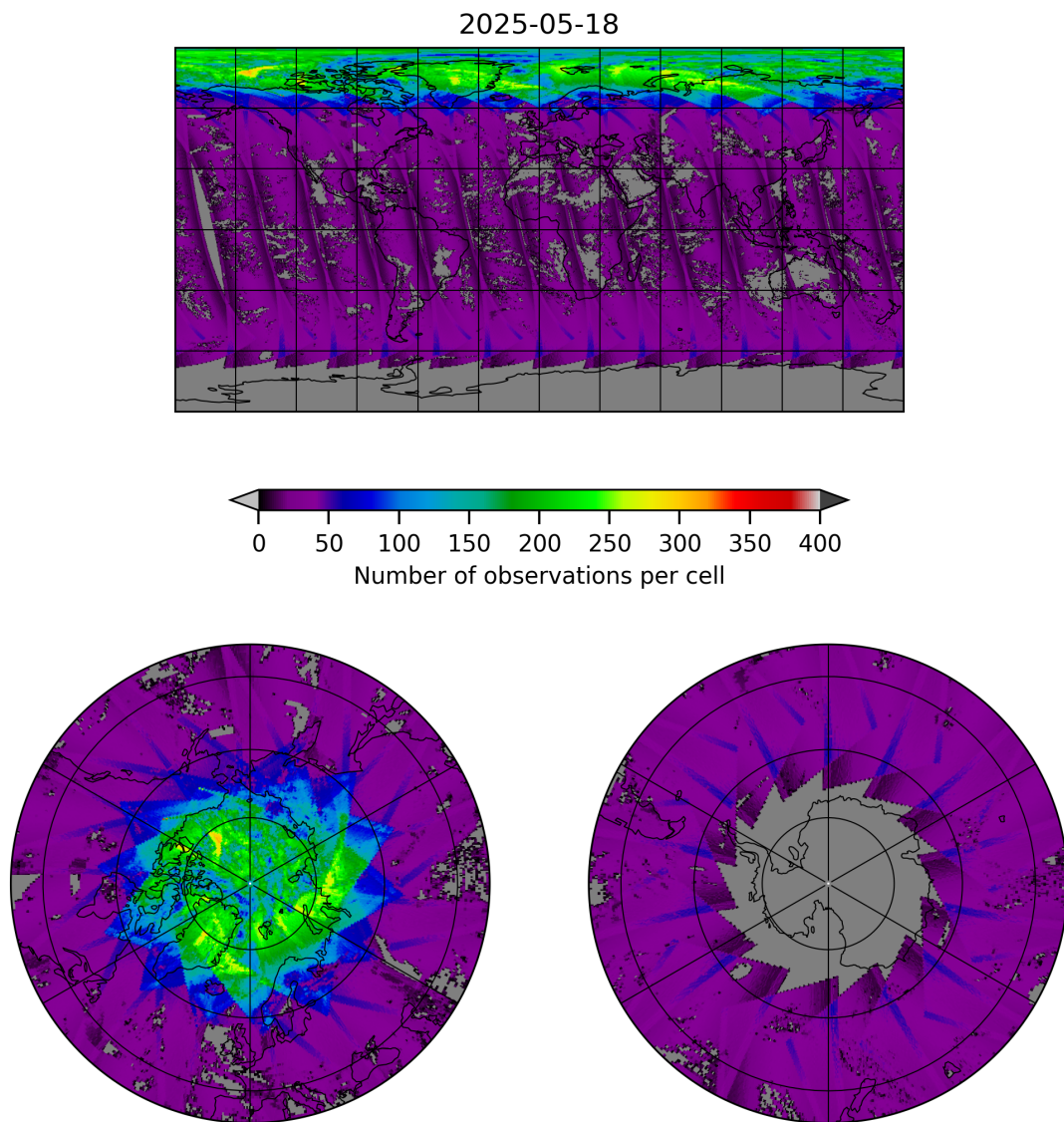
Figure 19: Map of the number of observations for 2025-05-18 to 2025-05-19
