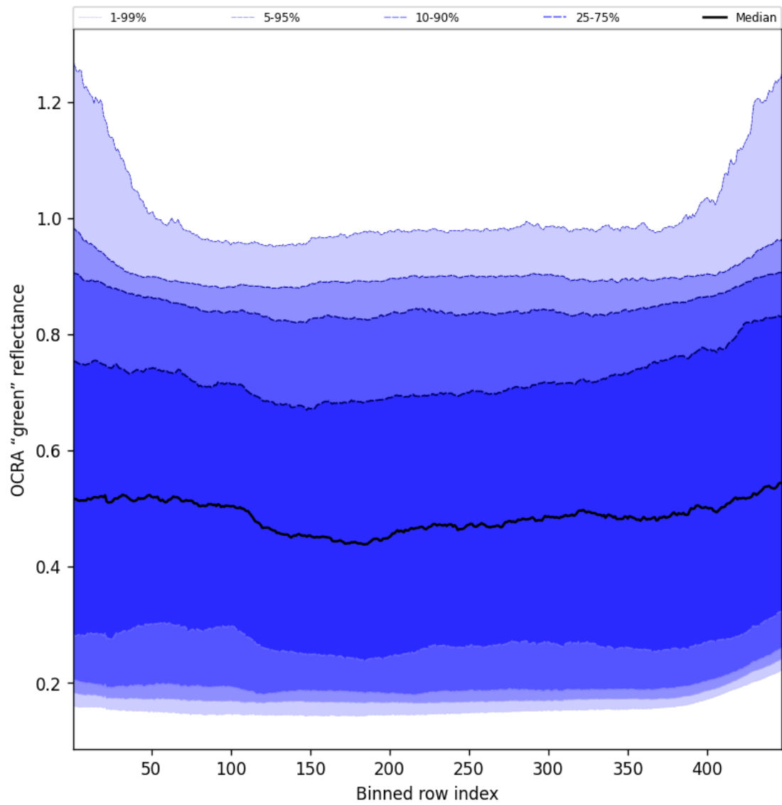
Figure 66: Along track statistics of “OCRA “green” reflectance” for 2025-05-18 to 2025-05-19
