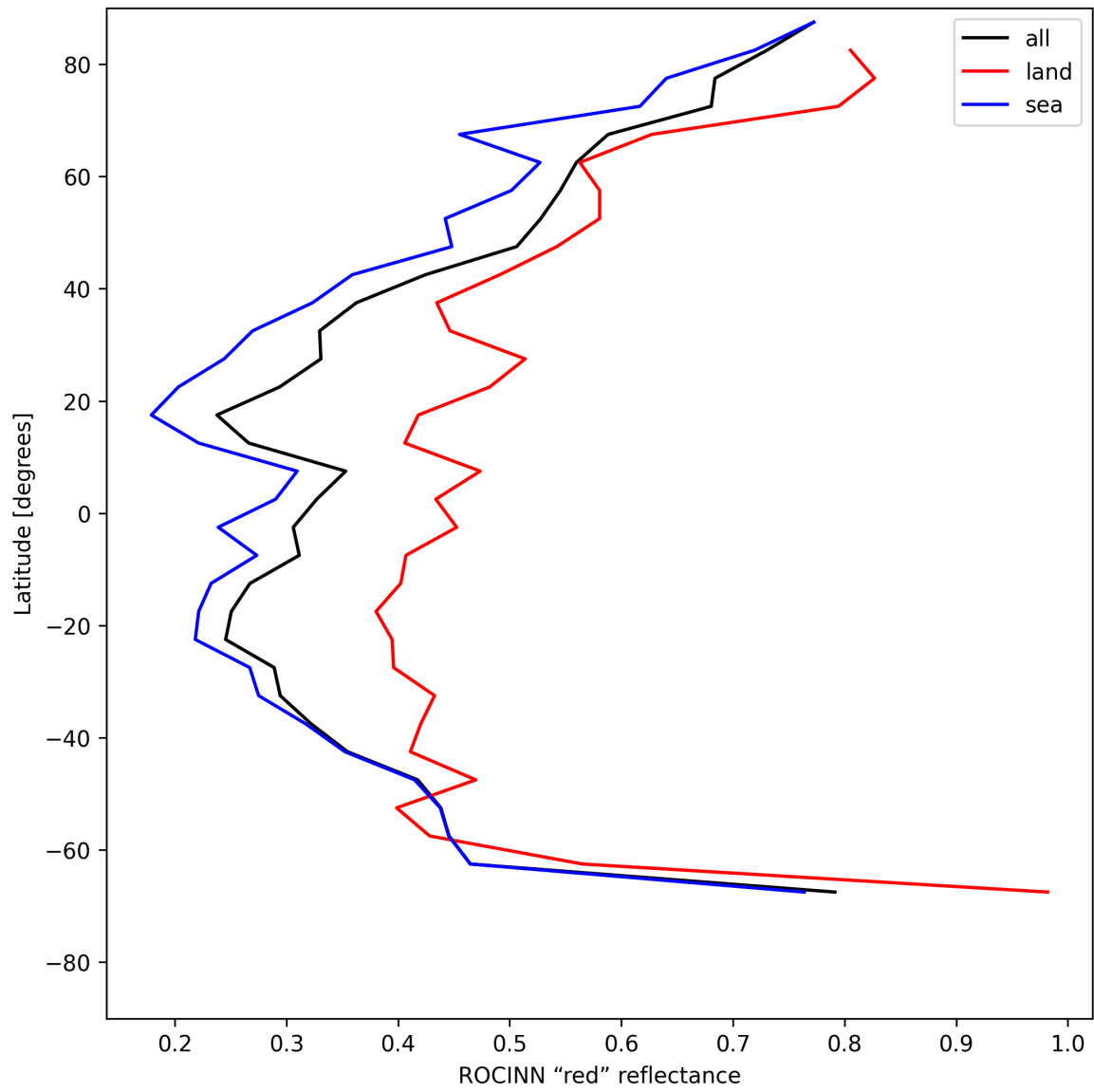
Figure 35: Zonal average of “ROCINN “red” reflectance” for 2025-05-18 to 2025-05-19.
