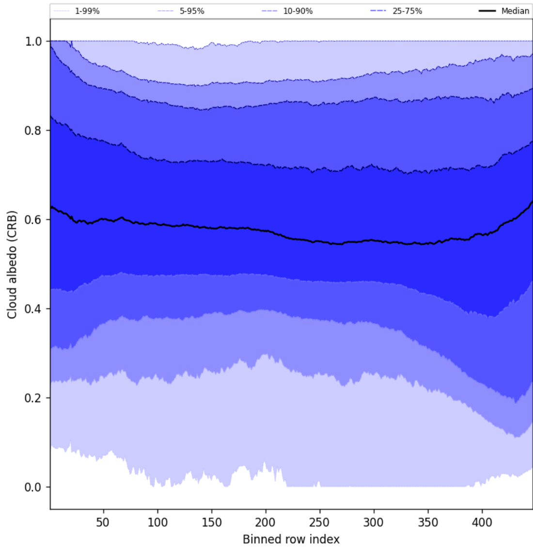
Figure 58: Along track statistics of “Cloud albedo (CRB)” for 2025-05-18 to 2025-05-19
