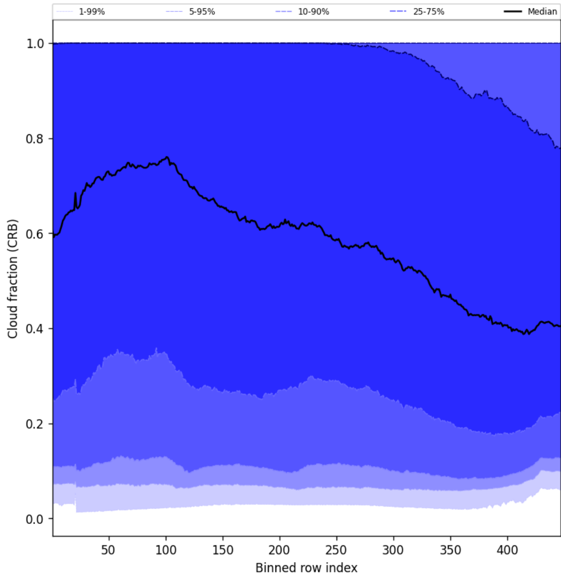
Figure 56: Along track statistics of “Cloud fraction (CRB)” for 2025-05-18 to 2025-05-19
