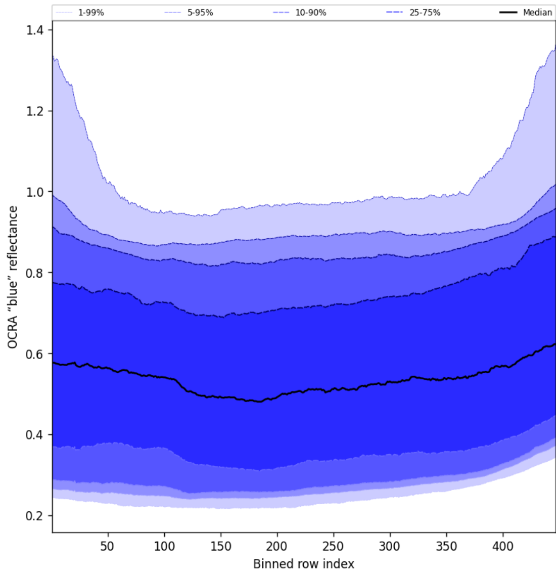
Figure 65: Along track statistics of “OCRA “blue” reflectance” for 2025-05-18 to 2025-05-19
