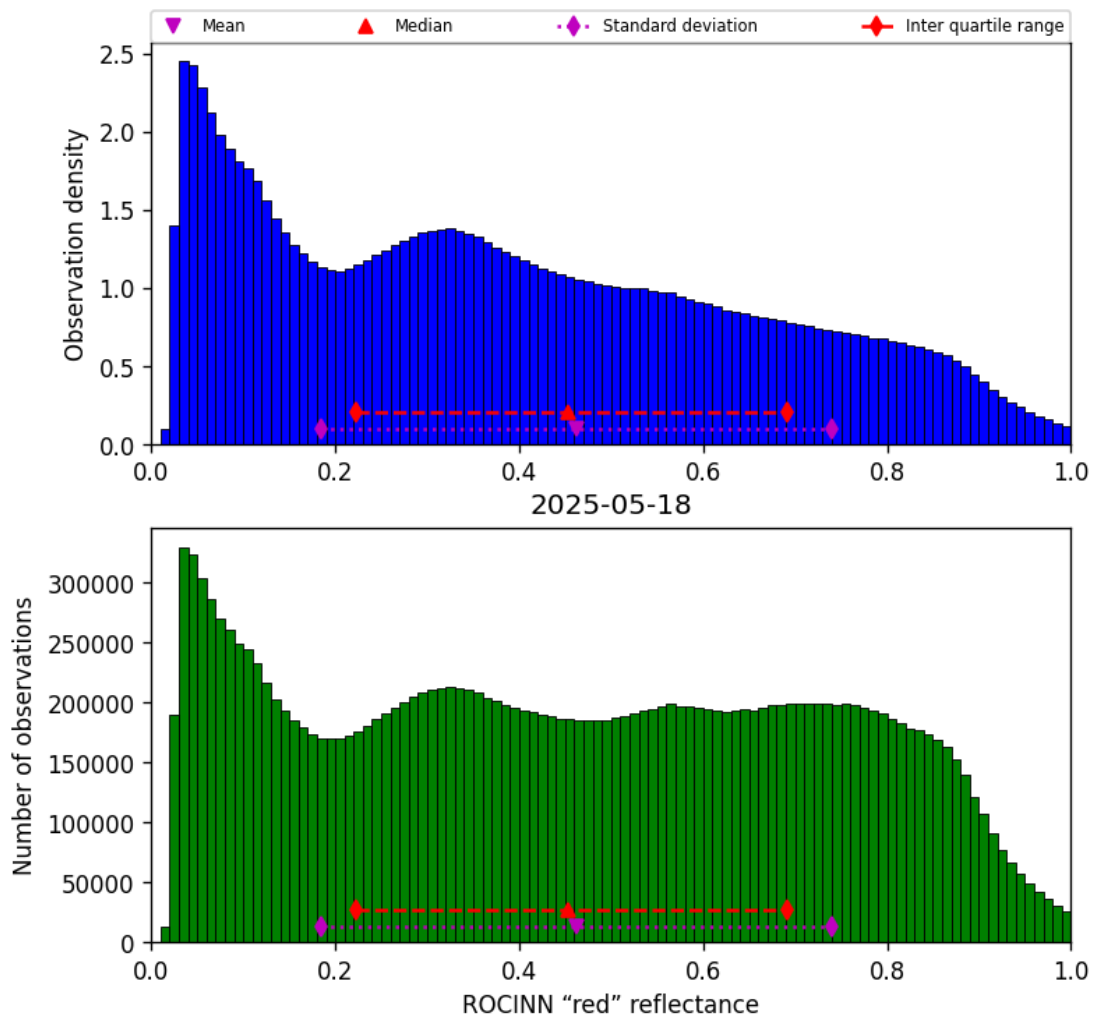
Figure 51: Histogram of “ROCINN “red” reflectance” for 2025-05-18 to 2025-05-19
