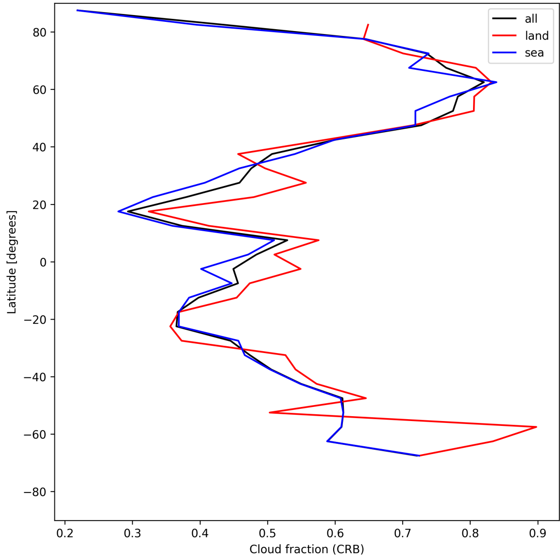
Figure 24: Zonal average of “Cloud fraction (CRB)” for 2025-05-18 to 2025-05-19.
