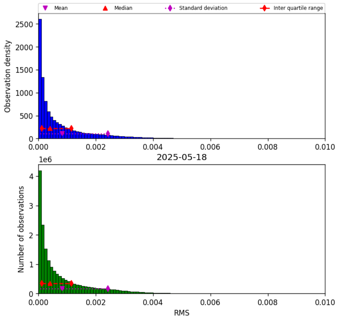
Figure 45: Histogram of “RMS” for 2025-05-18 to 2025-05-19
