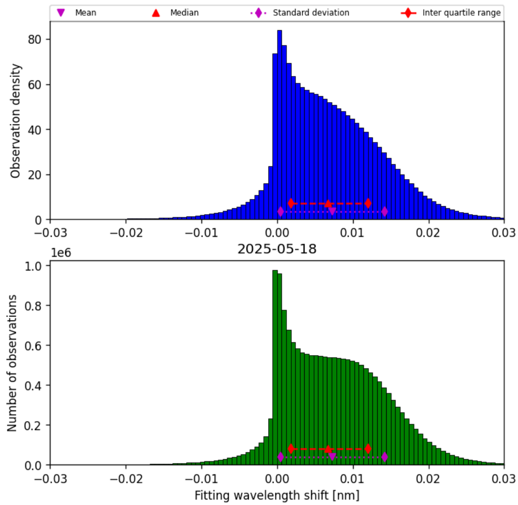
Figure 47: Histogram of “Fitting wavelength shift” for 2025-05-18 to 2025-05-19
