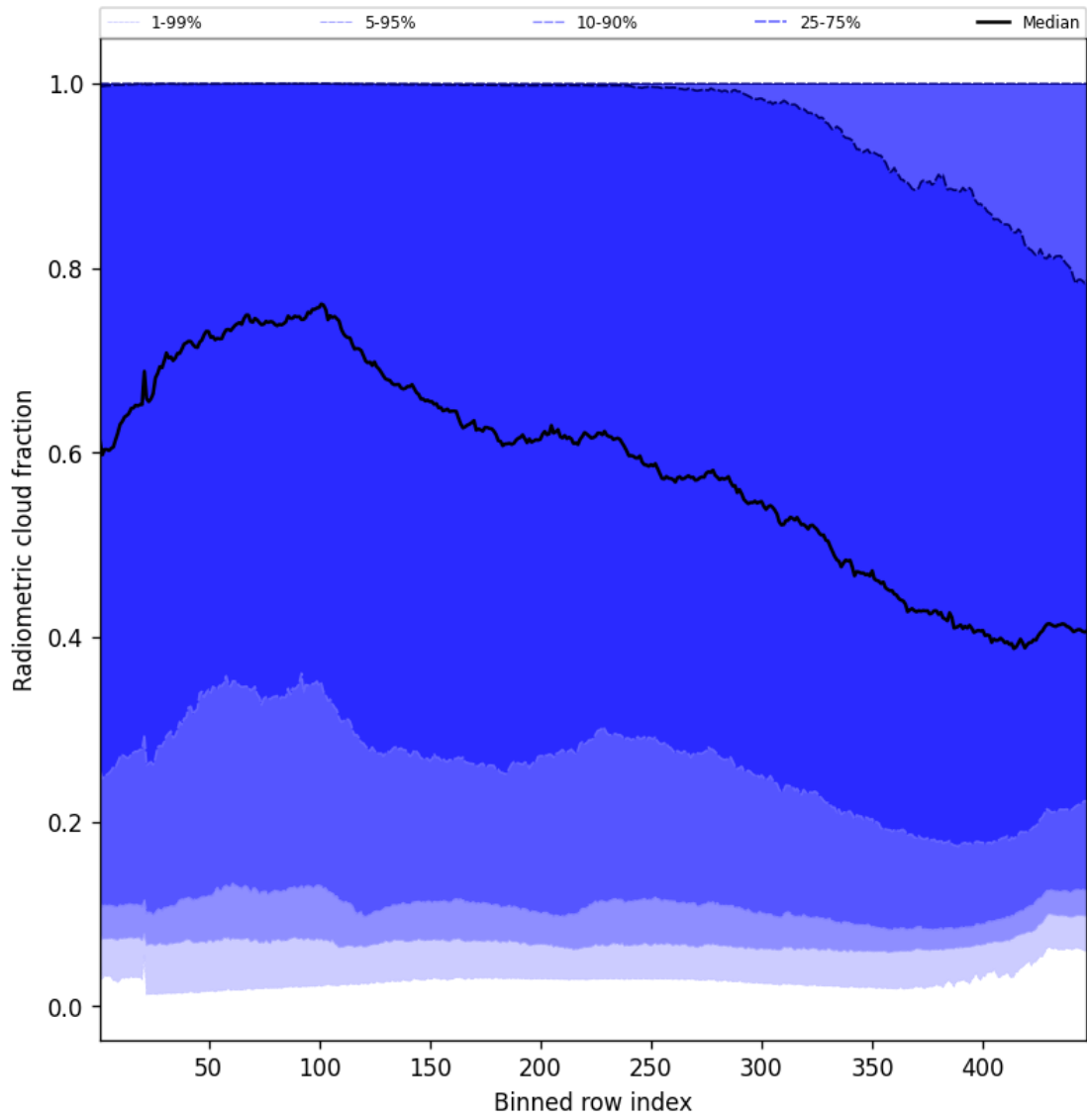
Figure 53: Along track statistics of “Radiometric cloud fraction” for 2025-05-18 to 2025-05-19
