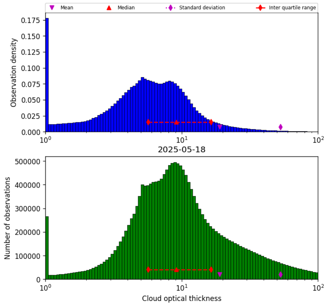
Figure 39: Histogram of “Cloud optical thickness” for 2025-05-18 to 2025-05-19
