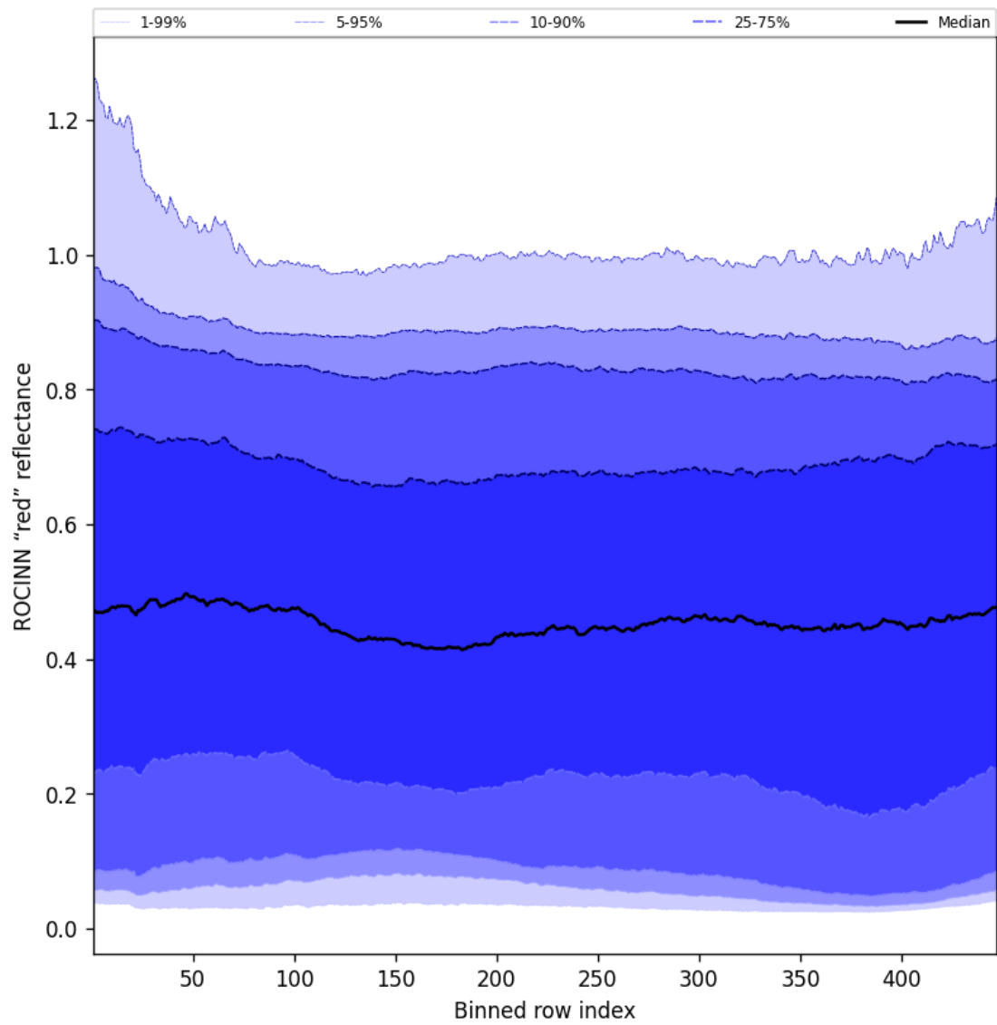
Figure 67: Along track statistics of "ROCINN "red" reflectance" for 2025-05-18 to 2025-05-19
