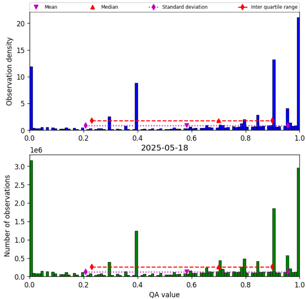
Figure 36: Histogram of “QA value” for 2025-05-18 to 2025-05-19
