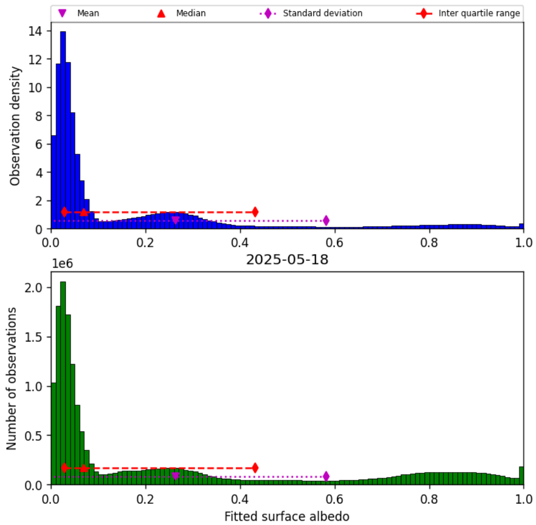
Figure 43: Histogram of “Fitted surface albedo” for 2025-05-18 to 2025-05-19
