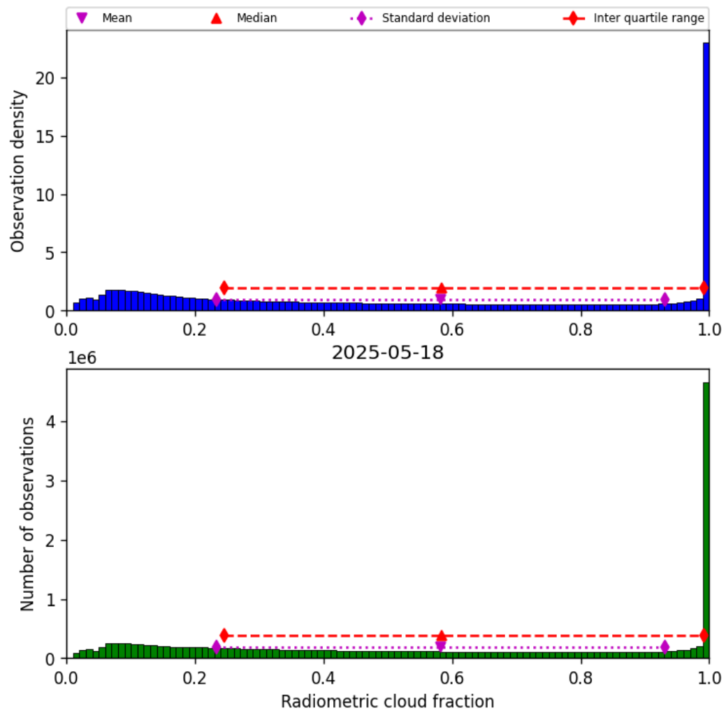
Figure 37: Histogram of “Radiometric cloud fraction” for 2025-05-18 to 2025-05-19
