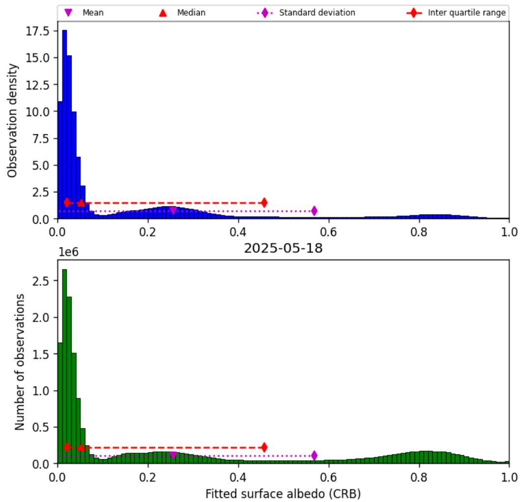
Figure 44: Histogram of “Fitted surface albedo (CRB)” for 2025-05-18 to 2025-05-19
