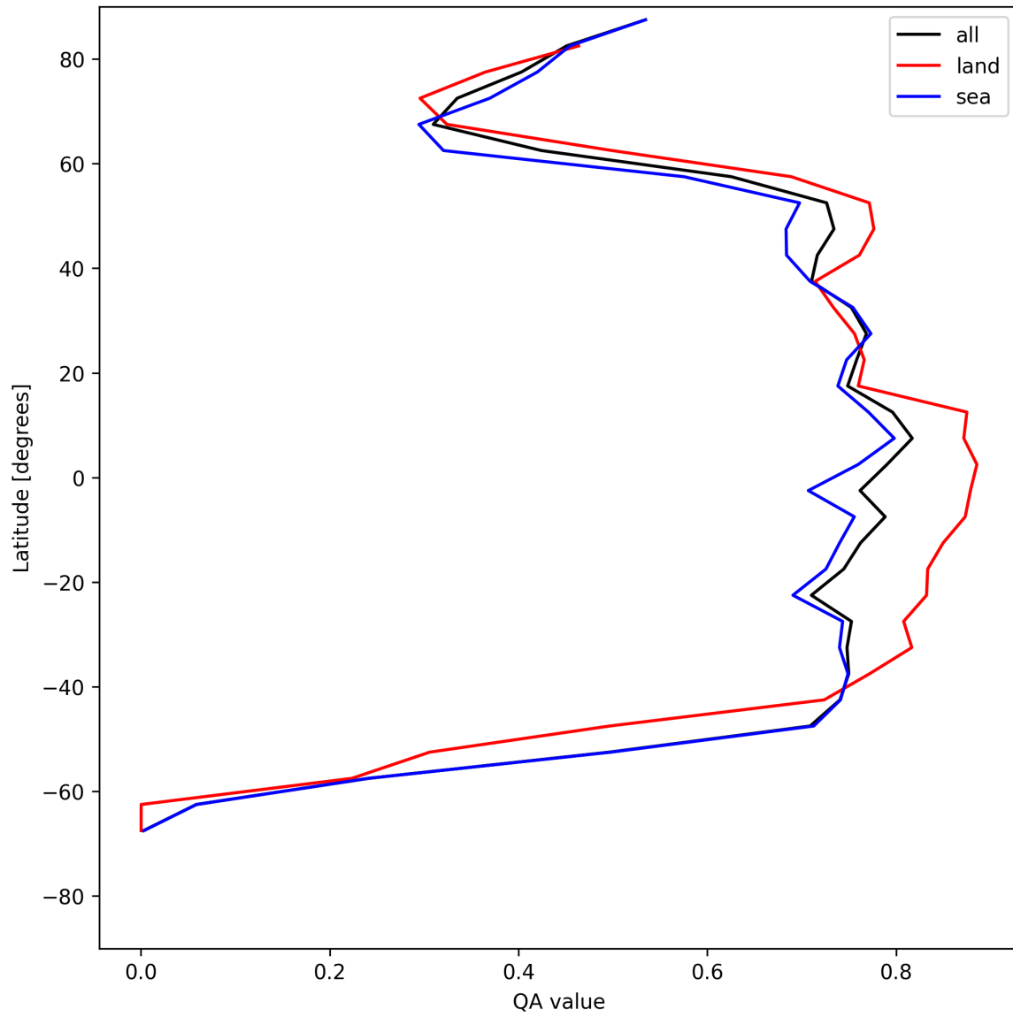
Figure 20: Zonal average of “QA value” for 2025-05-18 to 2025-05-19.
