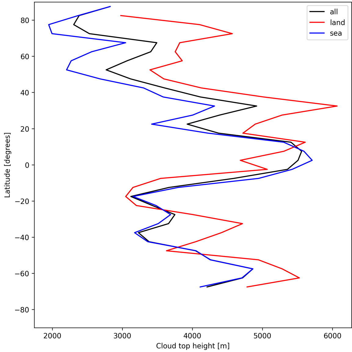
Figure 22: Zonal average of “Cloud top height” for 2025-05-18 to 2025-05-19.
