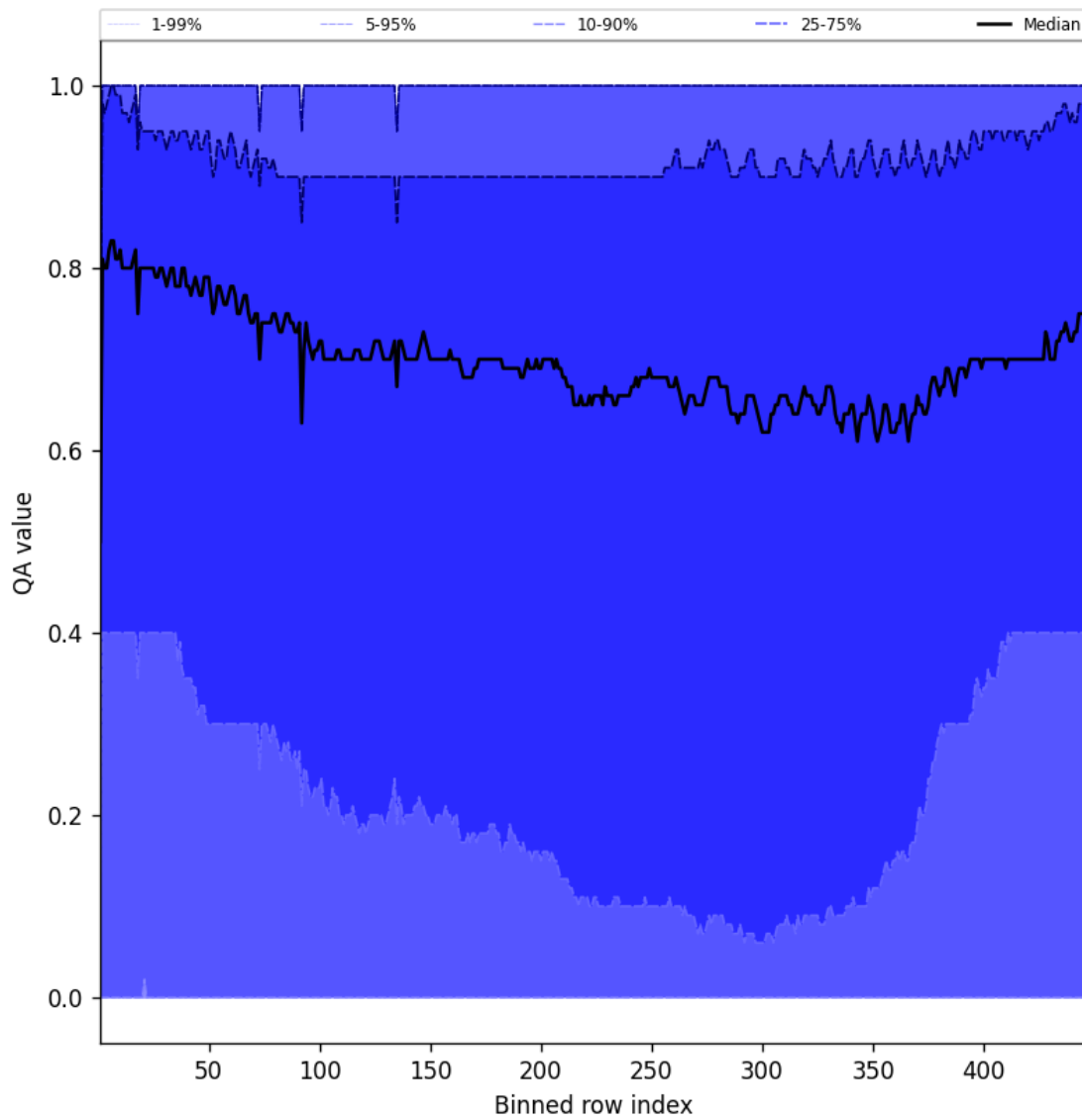
Figure 52: Along track statistics of “QA value” for 2025-05-18 to 2025-05-19
