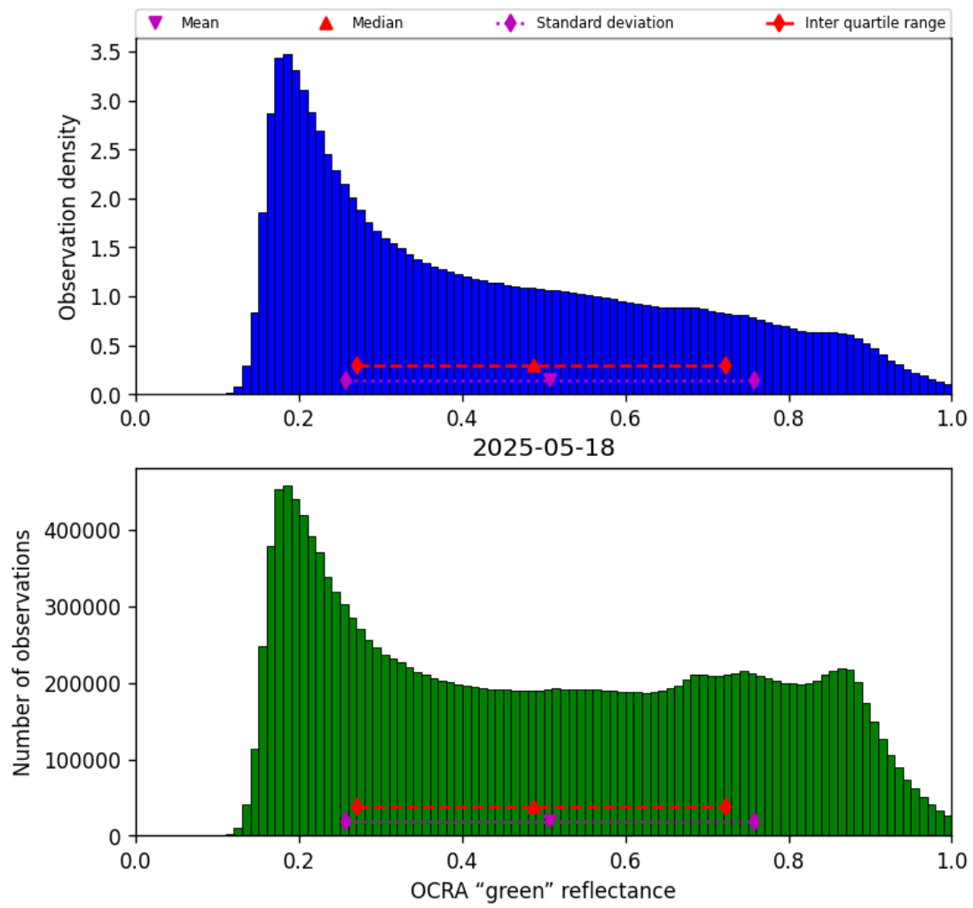
Figure 50: Histogram of “OCRA “green” reflectance” for 2025-05-18 to 2025-05-19
