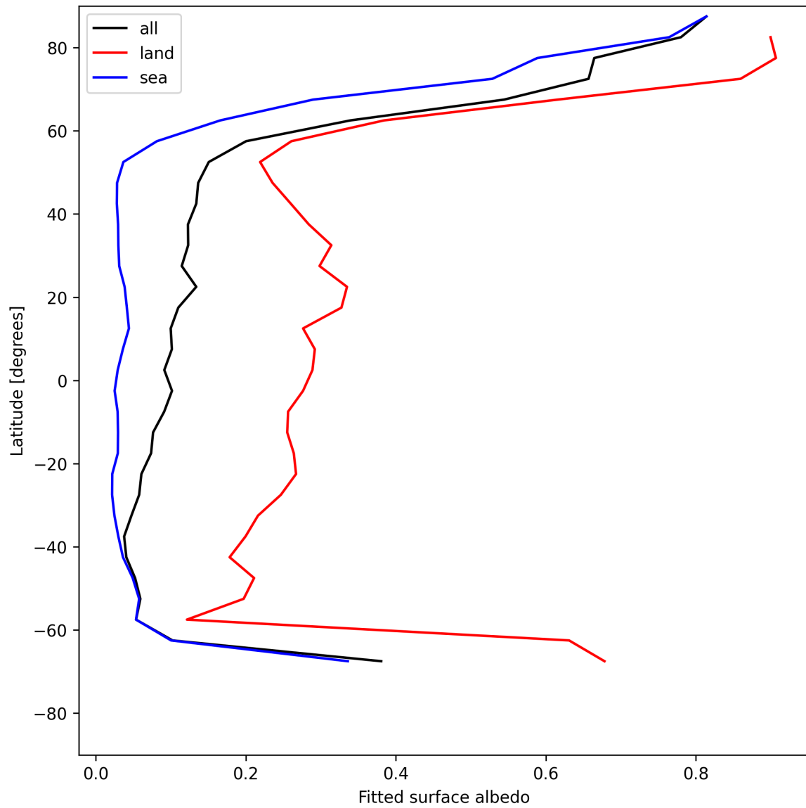
Figure 27: Zonal average of “Fitted surface albedo” for 2025-05-18 to 2025-05-19.
