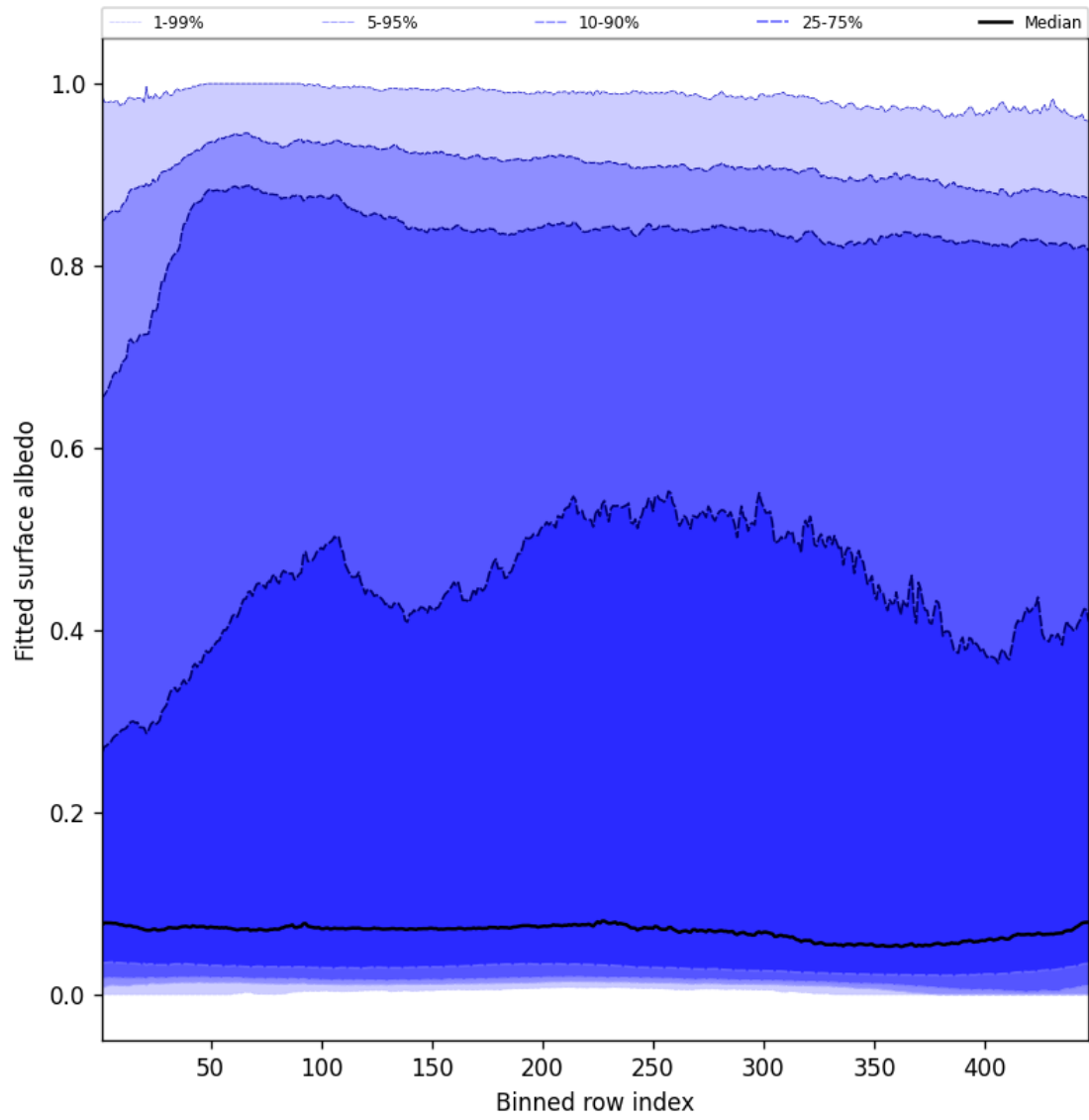
Figure 59: Along track statistics of “Fitted surface albedo” for 2025-05-18 to 2025-05-19
