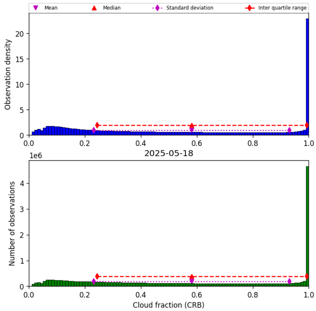
Figure 40: Histogram of “Cloud fraction (CRB)” for 2025-05-18 to 2025-05-19
