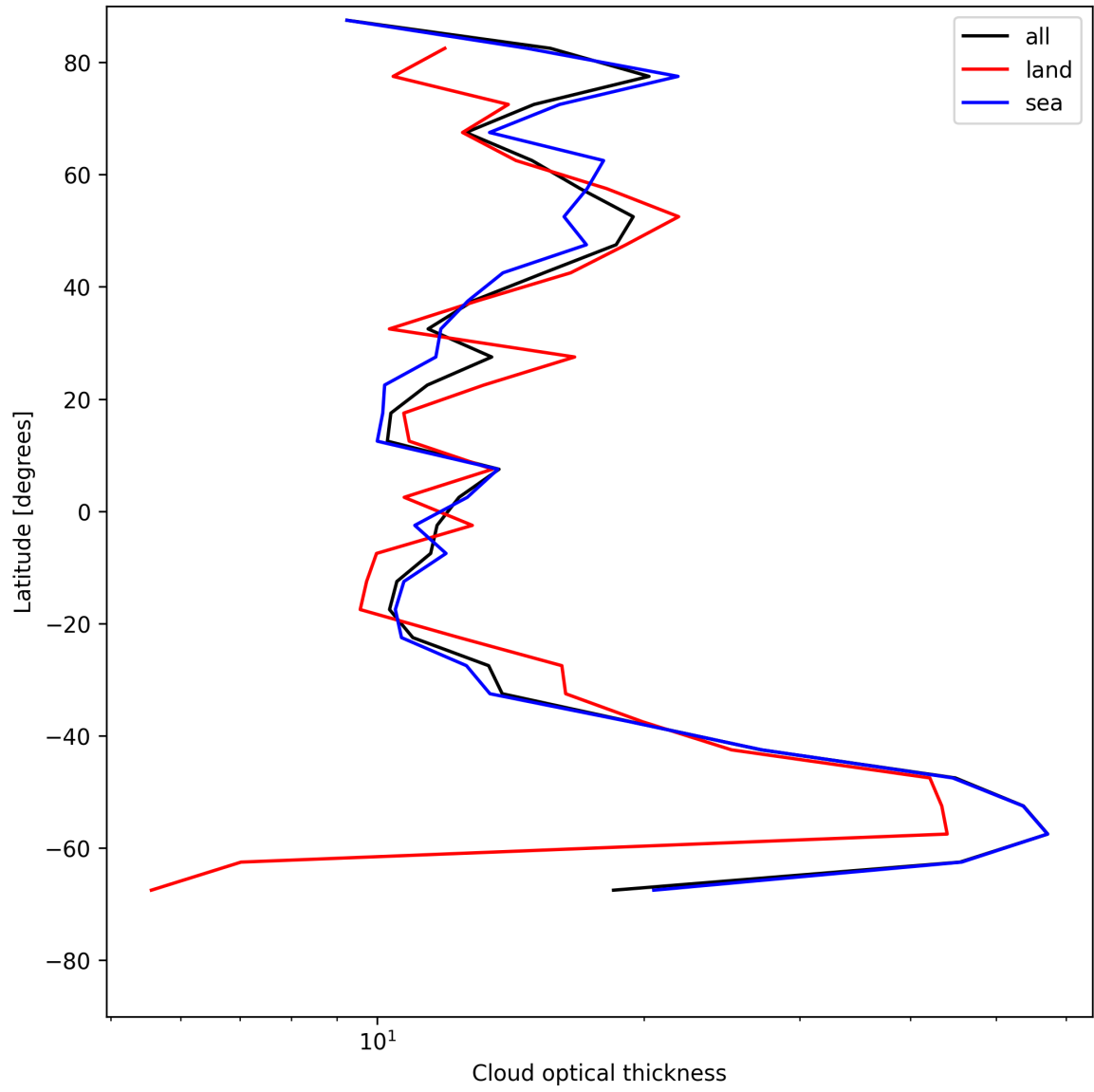
Figure 23: Zonal average of “Cloud optical thickness” for 2025-05-18 to 2025-05-19.
