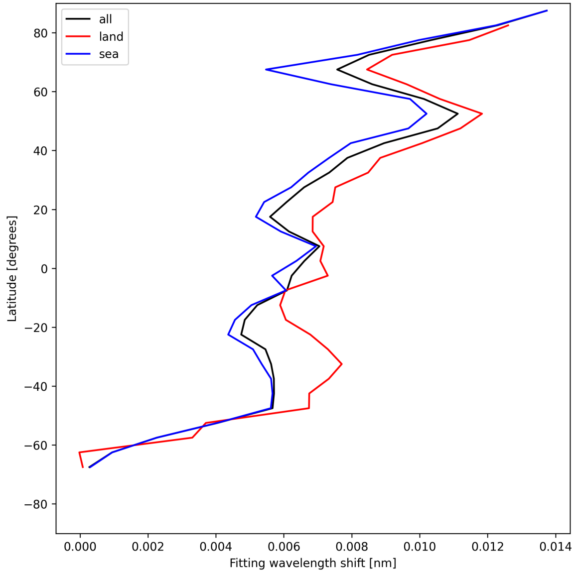
Figure 31: Zonal average of “Fitting wavelength shift” for 2025-05-18 to 2025-05-19.
