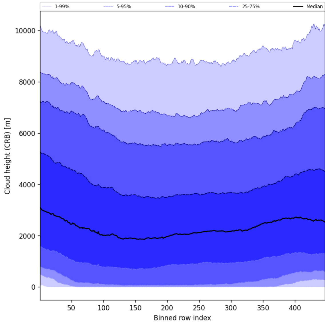
Figure 57: Along track statistics of “Cloud height (CRB)” for 2025-05-18 to 2025-05-19
