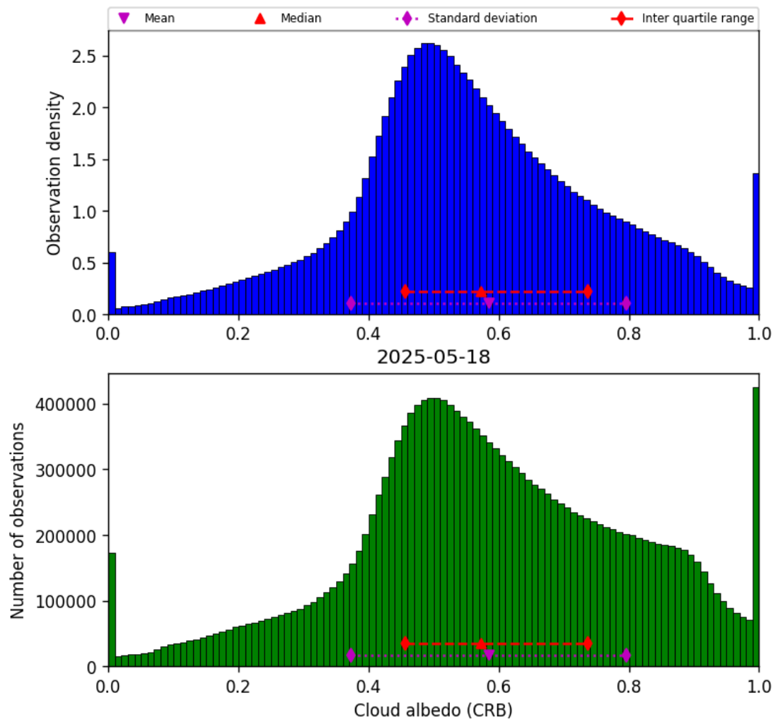
Figure 42: Histogram of “Cloud albedo (CRB)” for 2025-05-18 to 2025-05-19
