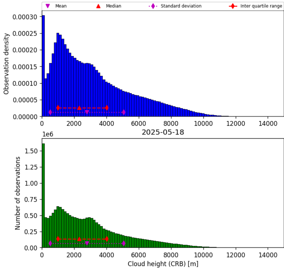
Figure 41: Histogram of “Cloud height (CRB)” for 2025-05-18 to 2025-05-19
