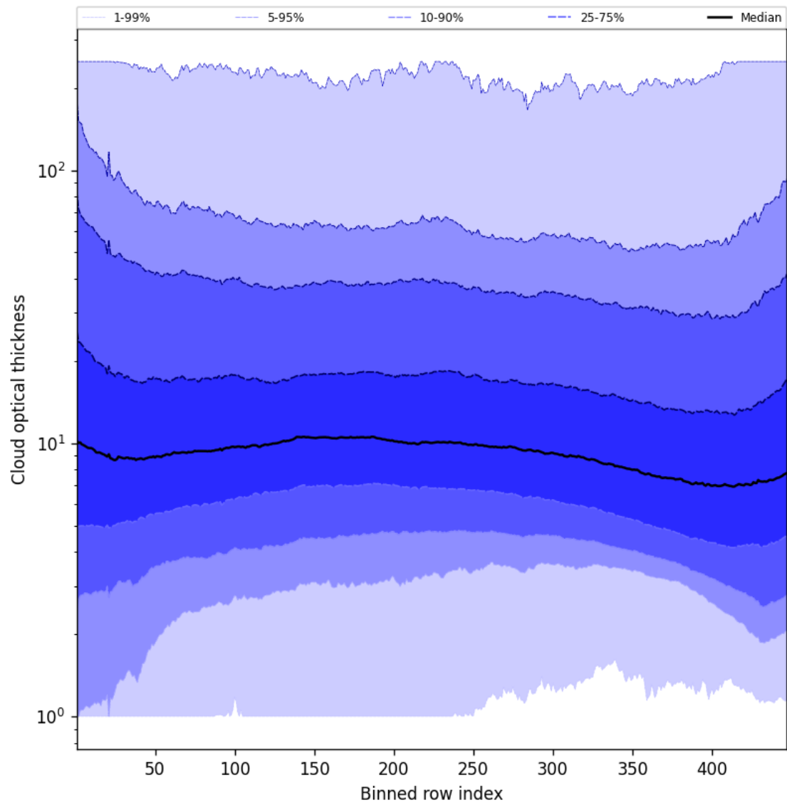
Figure 55: Along track statistics of “Cloud optical thickness” for 2025-05-18 to 2025-05-19
