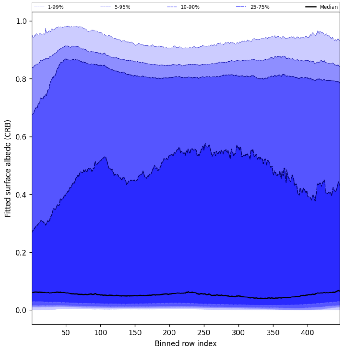
Figure 60: Along track statistics of “Fitted surface albedo (CRB)” for 2025-05-18 to 2025-05-19
