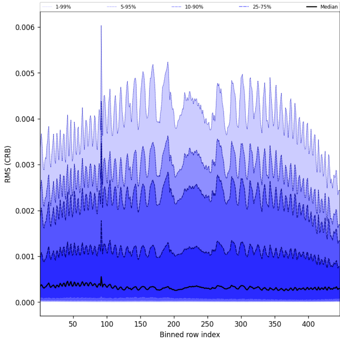
Figure 62: Along track statistics of “RMS (CRB)” for 2025-05-18 to 2025-05-19
