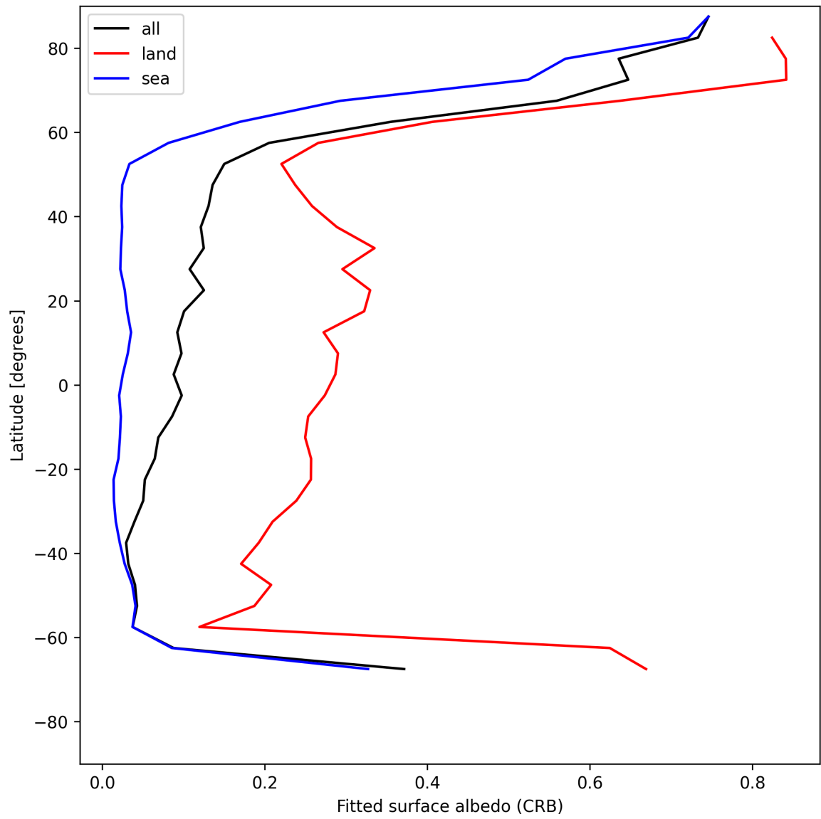
Figure 28: Zonal average of “Fitted surface albedo (CRB)” for 2025-05-18 to 2025-05-19.
