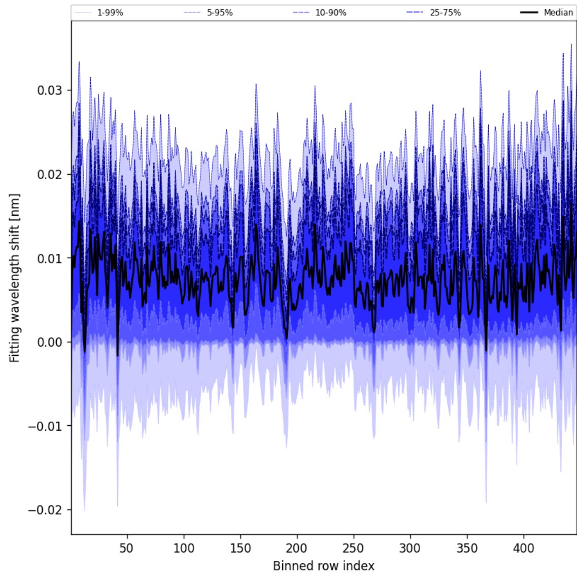
Figure 63: Along track statistics of “Fitting wavelength shift” for 2025-05-18 to 2025-05-19
