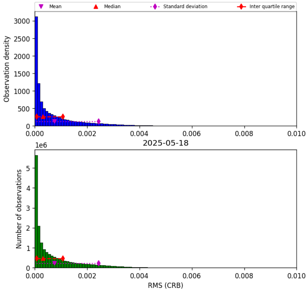
Figure 46: Histogram of “RMS (CRB)” for 2025-05-18 to 2025-05-19
