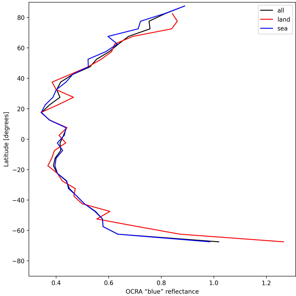
Figure 33: Zonal average of “OCRA “blue” reflectance” for 2025-05-18 to 2025-05-19.
