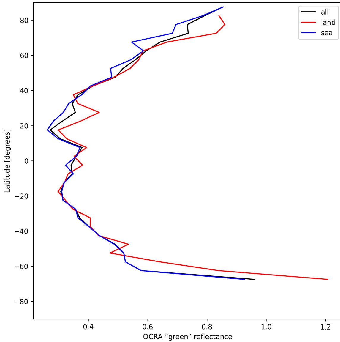
Figure 34: Zonal average of "OCRA "green" reflectance" for 2025-05-18 to 2025-05-19.
