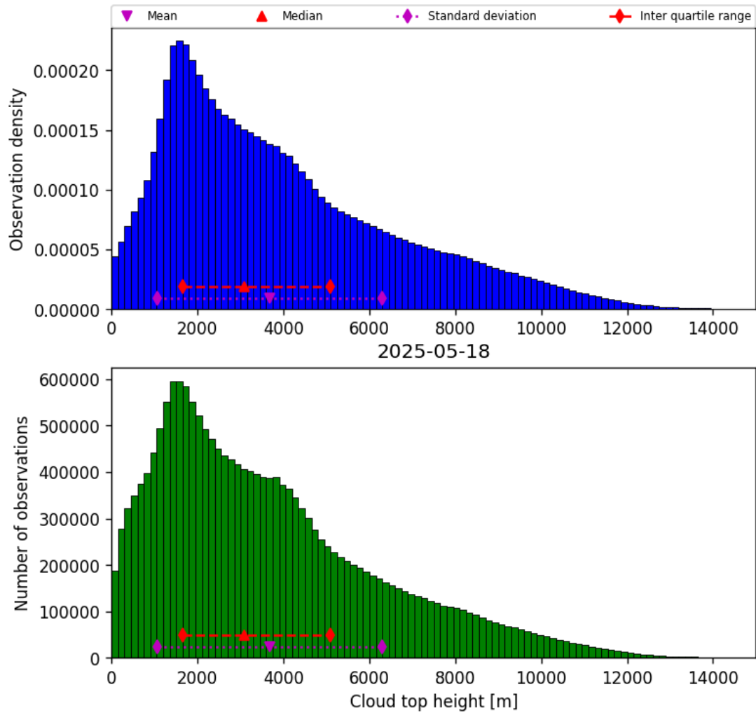
Figure 38: Histogram of “Cloud top height” for 2025-05-18 to 2025-05-19
