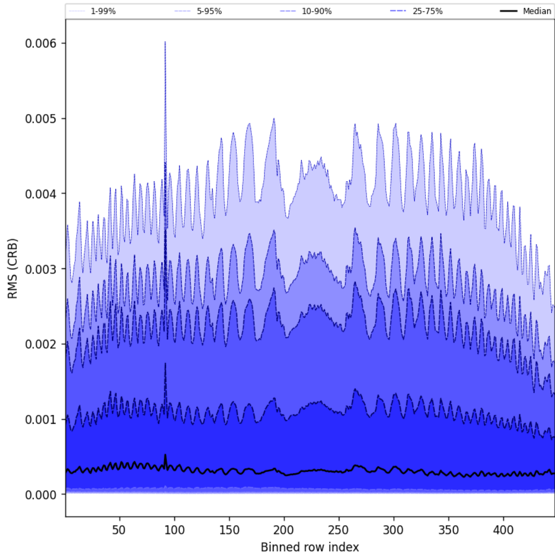
Figure 62: Along track statistics of “RMS (CRB)” for 2025-05-19 to 2025-05-19
