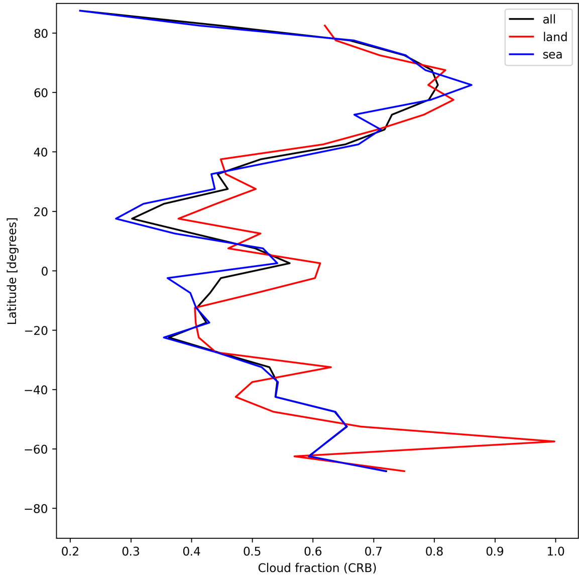
Figure 24: Zonal average of “Cloud fraction (CRB)” for 2025-05-19 to 2025-05-19.
