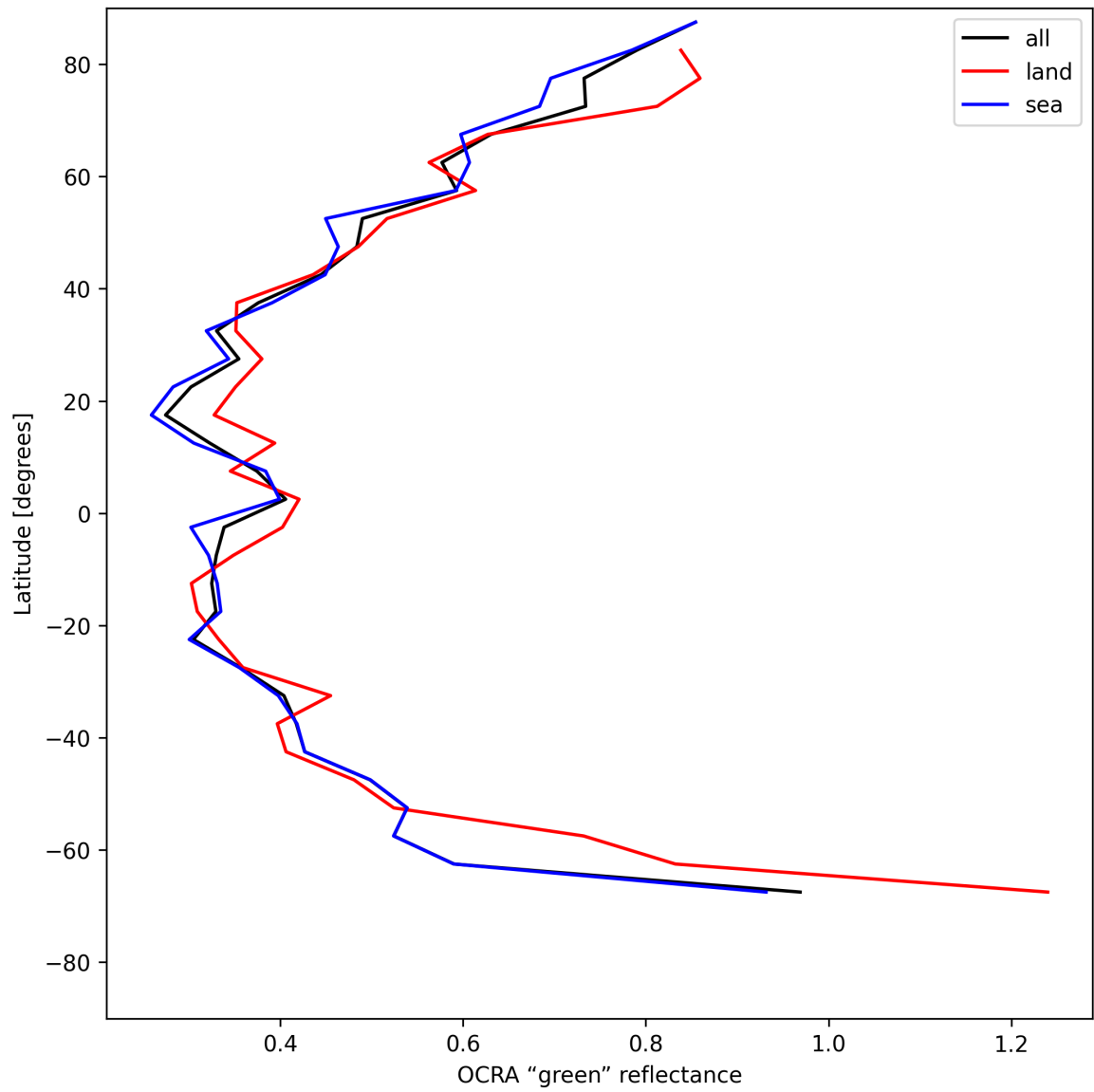
Figure 34: Zonal average of “OCRA “green” reflectance” for 2025-05-19 to 2025-05-19.
