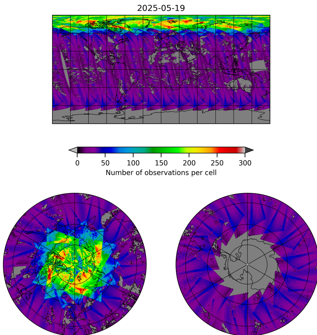
Figure 19: Map of the number of observations for 2025-05-19 to 2025-05-19
