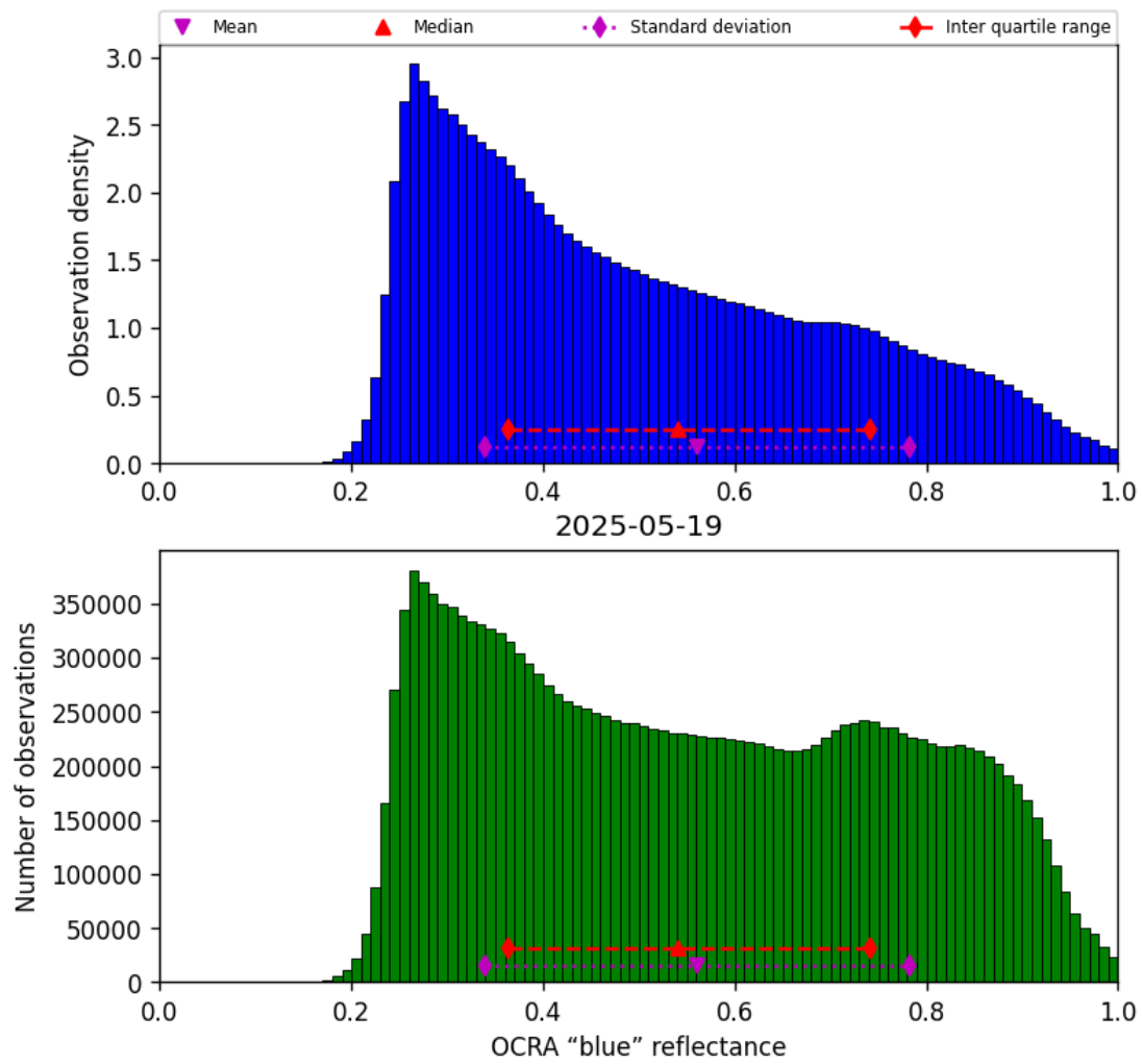
Figure 49: Histogram of “OCRA “blue” reflectance” for 2025-05-19 to 2025-05-19
