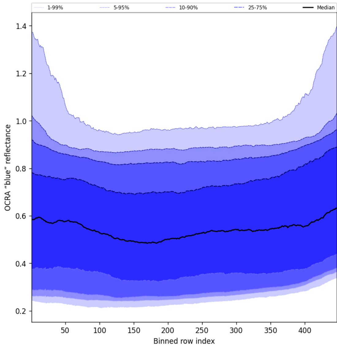
Figure 65: Along track statistics of “OCRA “blue” reflectance” for 2025-05-19 to 2025-05-19
