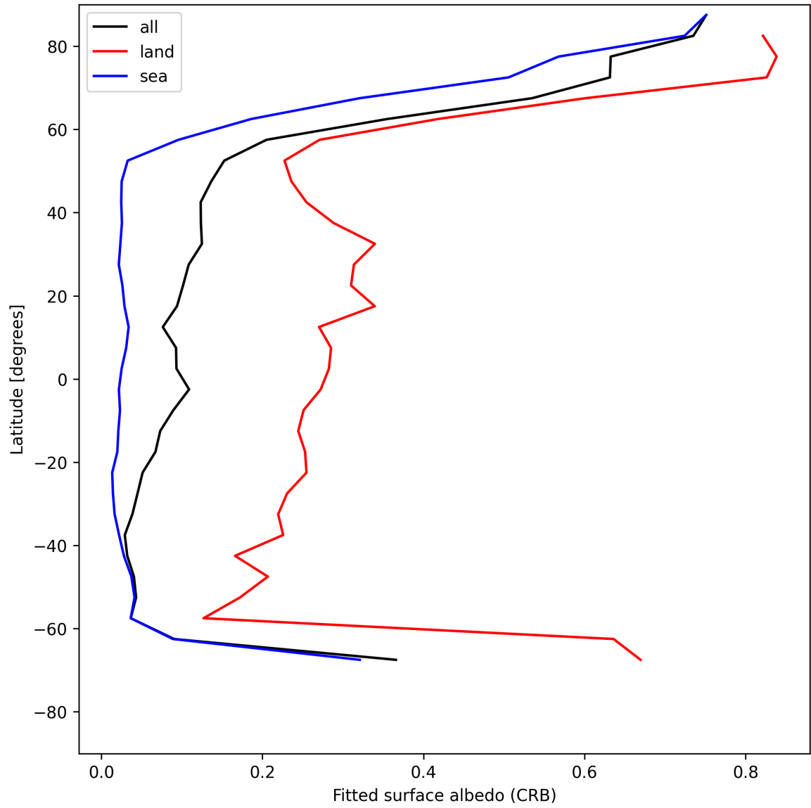
Figure 28: Zonal average of “Fitted surface albedo (CRB)” for 2025-05-19 to 2025-05-19.
