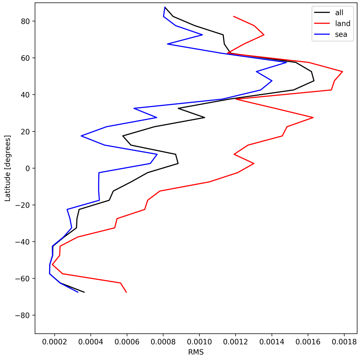
Figure 29: Zonal average of “RMS” for 2025-05-19 to 2025-05-19.
