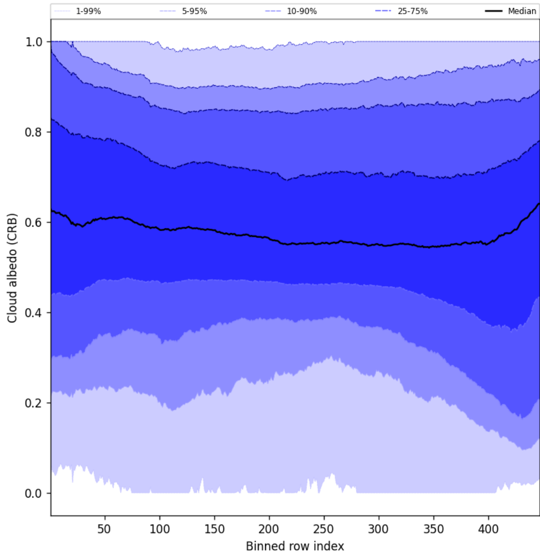
Figure 58: Along track statistics of “Cloud albedo (CRB)” for 2025-05-19 to 2025-05-19
