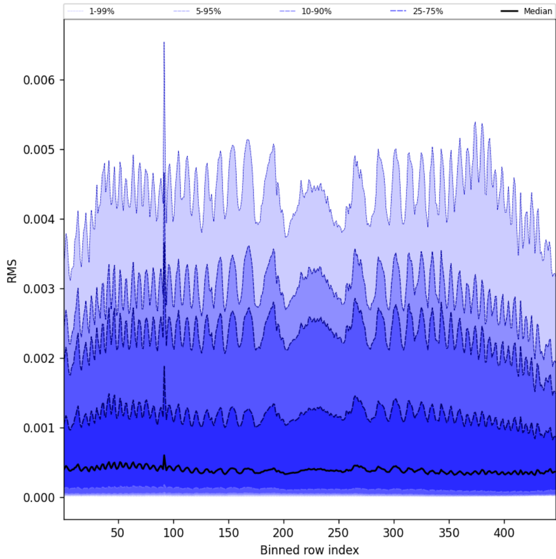
Figure 61: Along track statistics of “RMS” for 2025-05-19 to 2025-05-19
