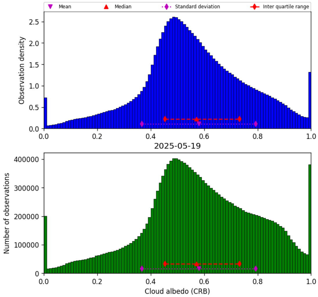
Figure 42: Histogram of “Cloud albedo (CRB)” for 2025-05-19 to 2025-05-19
