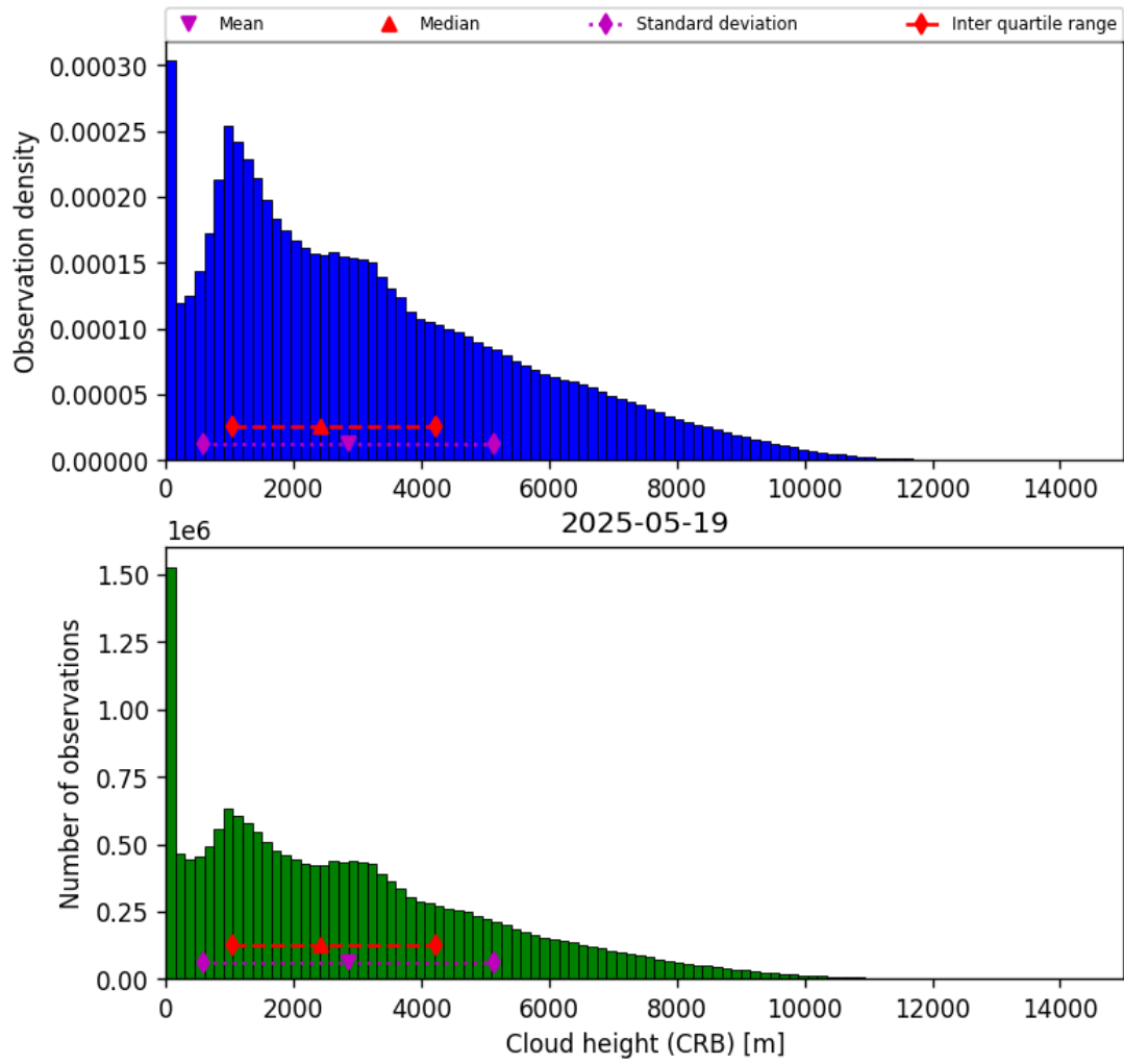
Figure 41: Histogram of “Cloud height (CRB)” for 2025-05-19 to 2025-05-19
