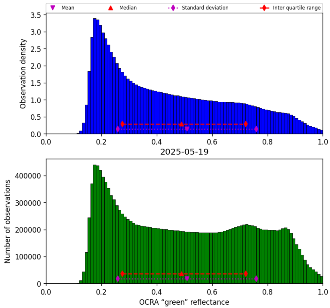
Figure 50: Histogram of “OCRA “green” reflectance” for 2025-05-19 to 2025-05-19
