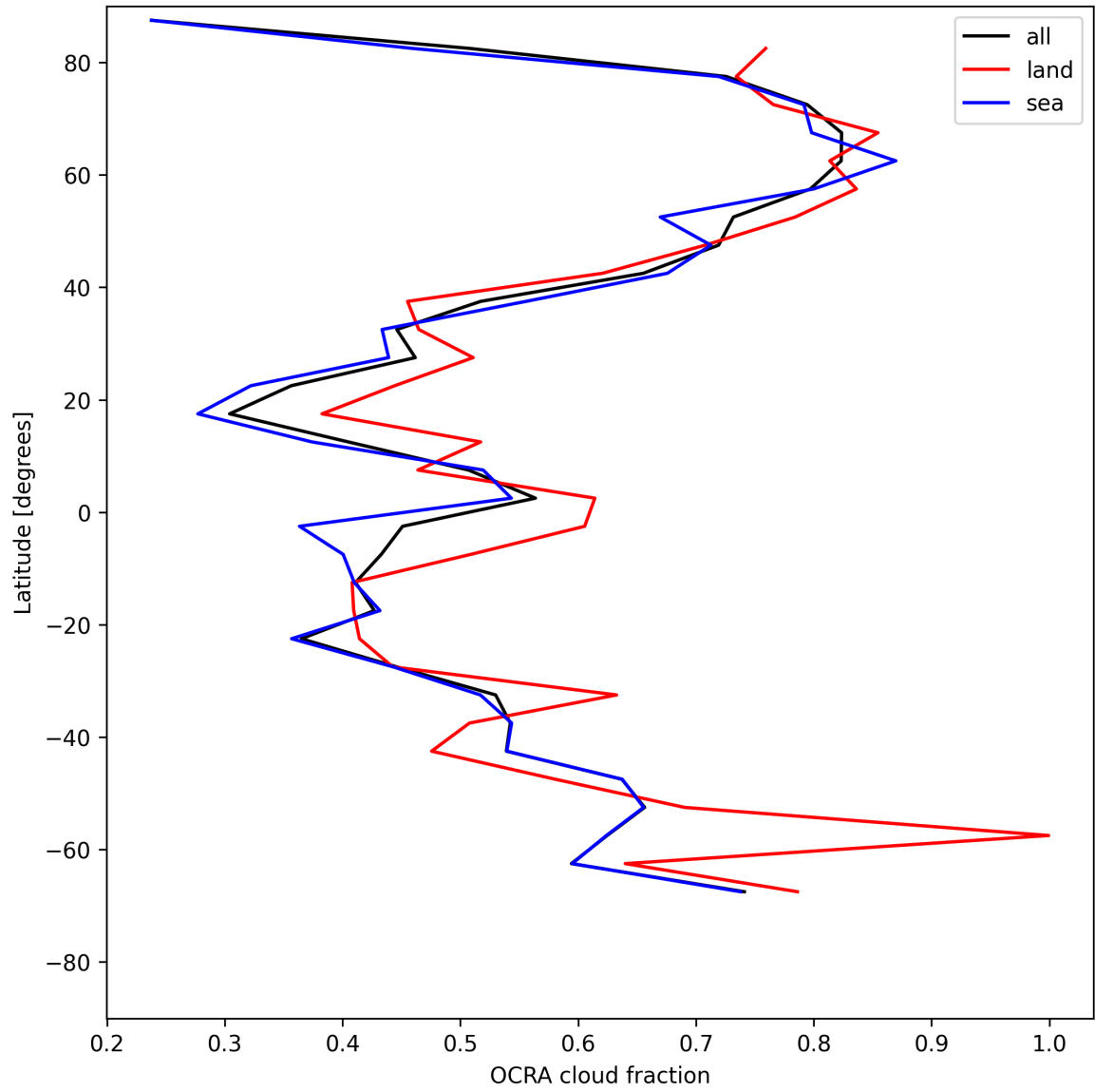
Figure 32: Zonal average of “OCRA cloud fraction” for 2025-05-19 to 2025-05-19.
