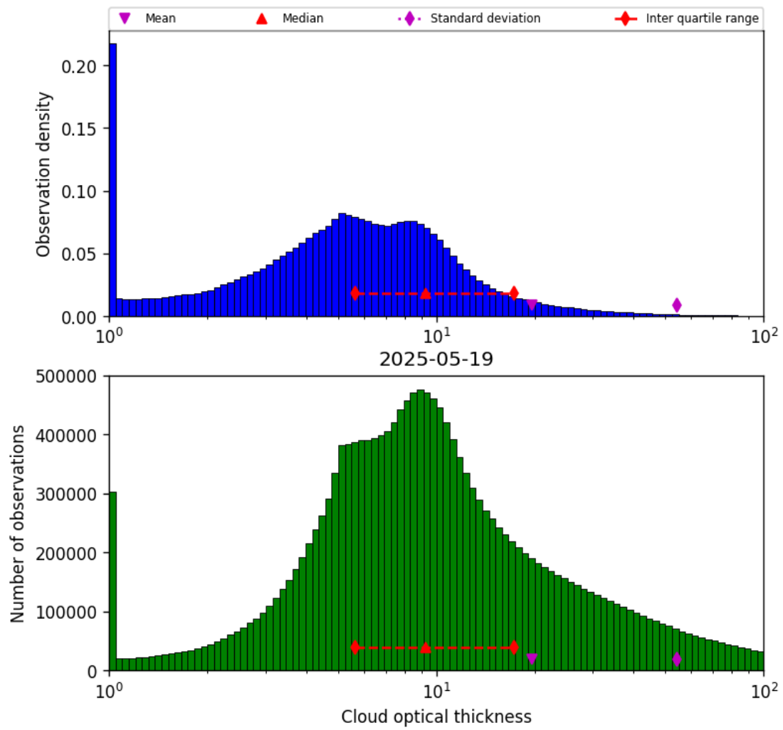
Figure 39: Histogram of “Cloud optical thickness” for 2025-05-19 to 2025-05-19
