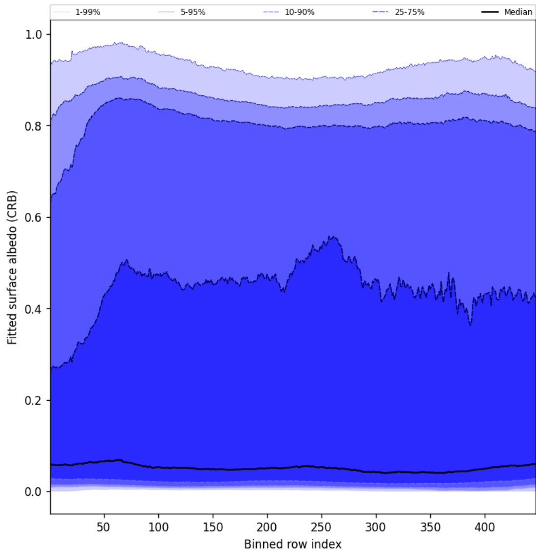
Figure 60: Along track statistics of “Fitted surface albedo (CRB)” for 2025-05-19 to 2025-05-19
