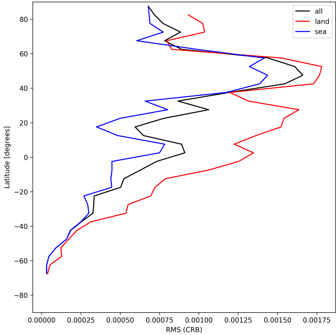
Figure 30: Zonal average of “RMS (CRB)” for 2025-05-19 to 2025-05-19.
