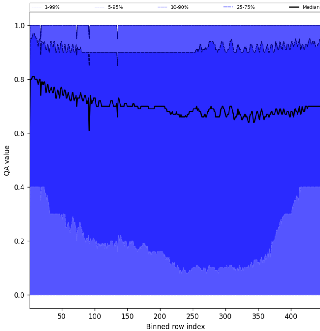
Figure 52: Along track statistics of “QA value” for 2025-05-19 to 2025-05-19
