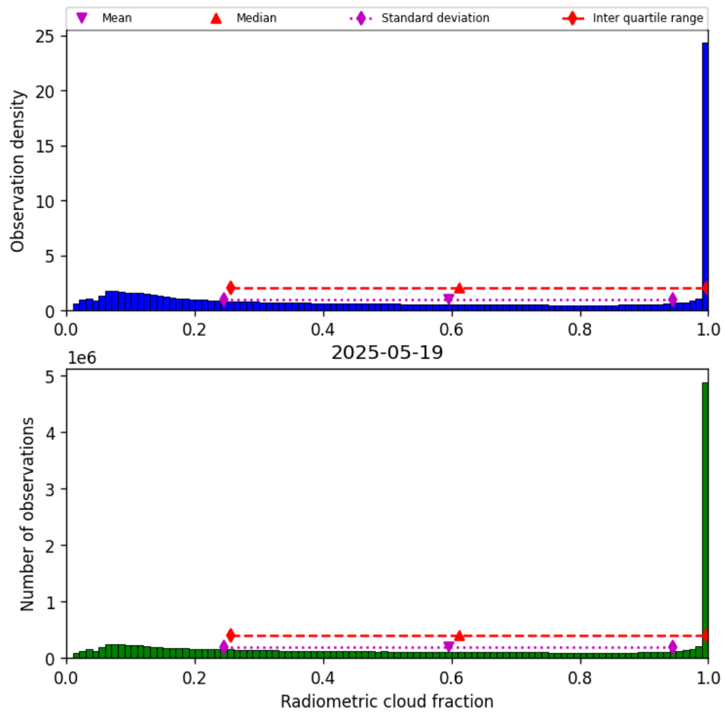
Figure 37: Histogram of “Radiometric cloud fraction” for 2025-05-19 to 2025-05-19
