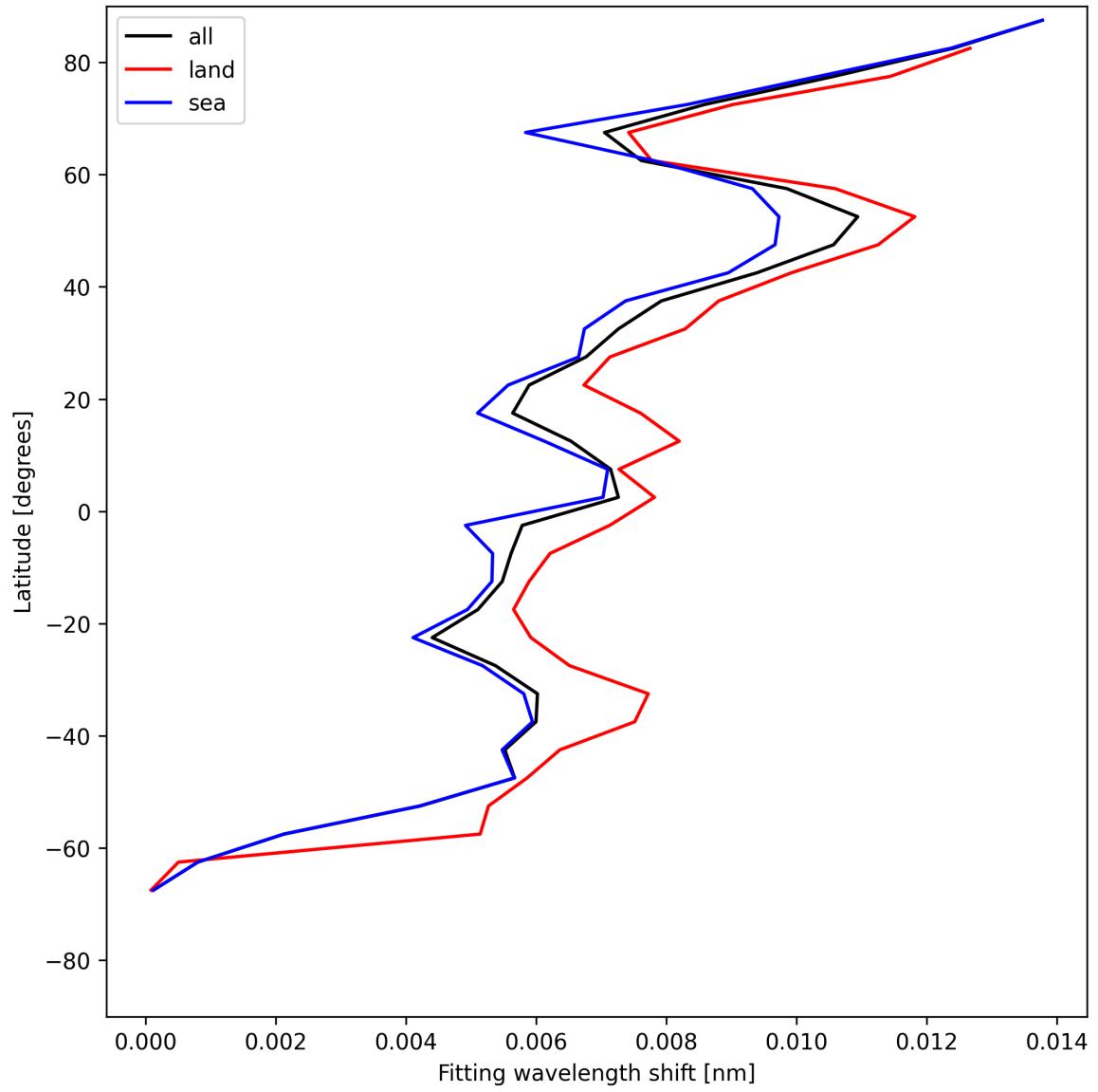
Figure 31: Zonal average of “Fitting wavelength shift” for 2025-05-19 to 2025-05-19.
