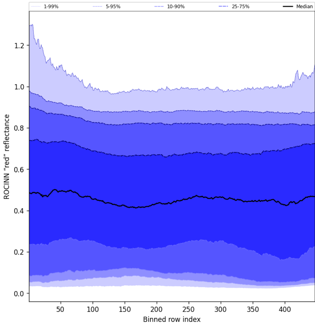
Figure 67: Along track statistics of "ROCINN "red" reflectance" for 2025-05-19 to 2025-05-19
