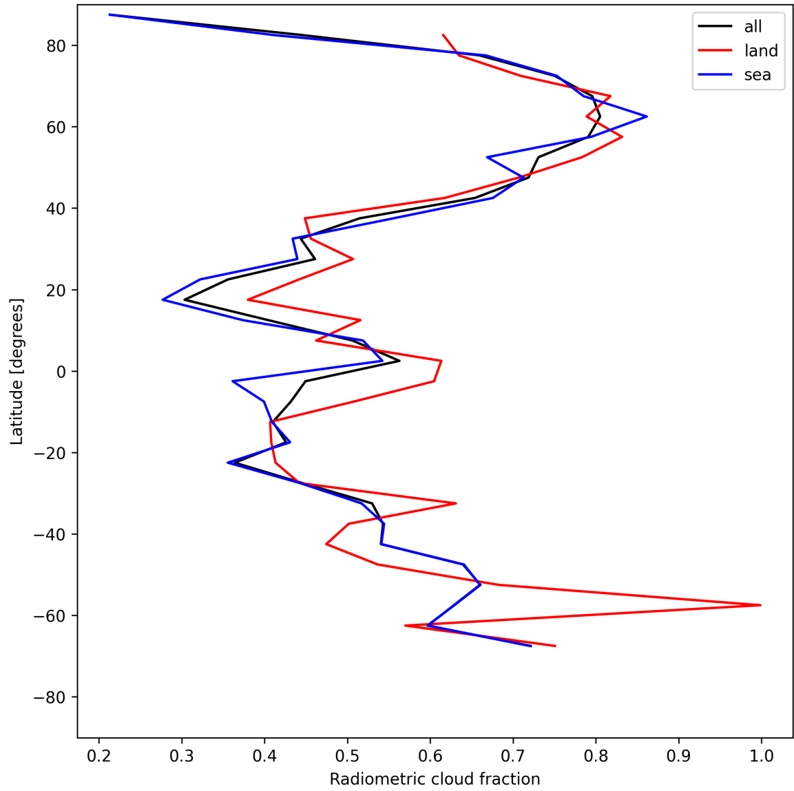
Figure 21: Zonal average of “Radiometric cloud fraction” for 2025-05-19 to 2025-05-19.
