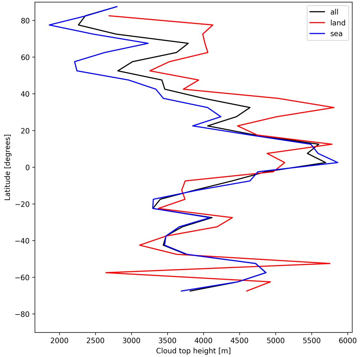
Figure 22: Zonal average of “Cloud top height” for 2025-05-19 to 2025-05-19.
