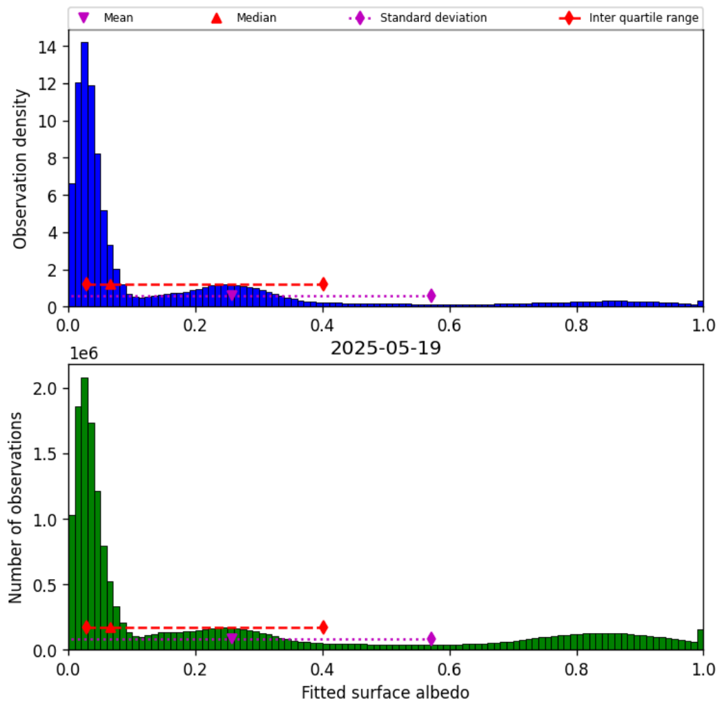
Figure 43: Histogram of “Fitted surface albedo” for 2025-05-19 to 2025-05-19
