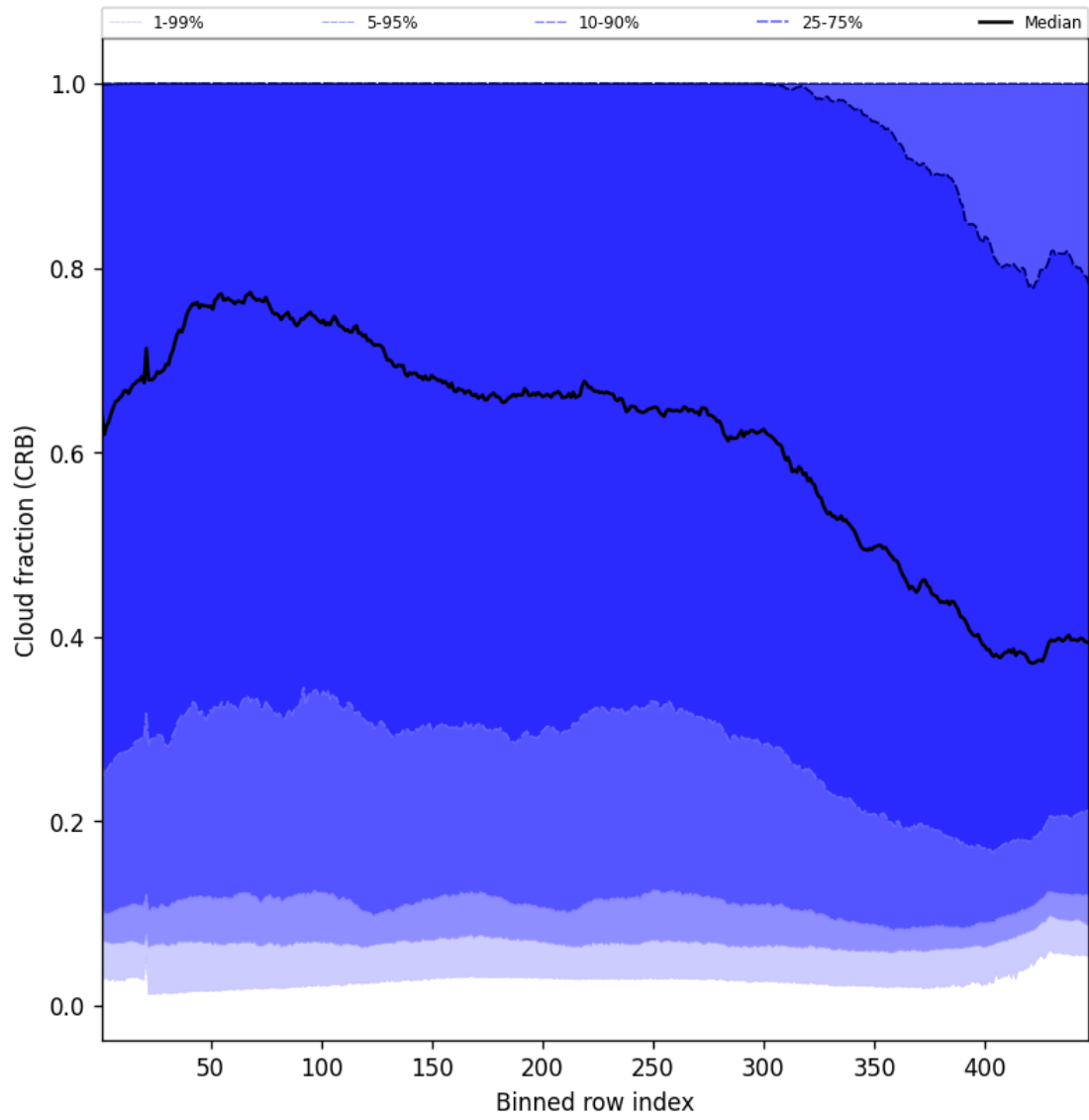
Figure 56: Along track statistics of “Cloud fraction (CRB)” for 2025-05-19 to 2025-05-19
