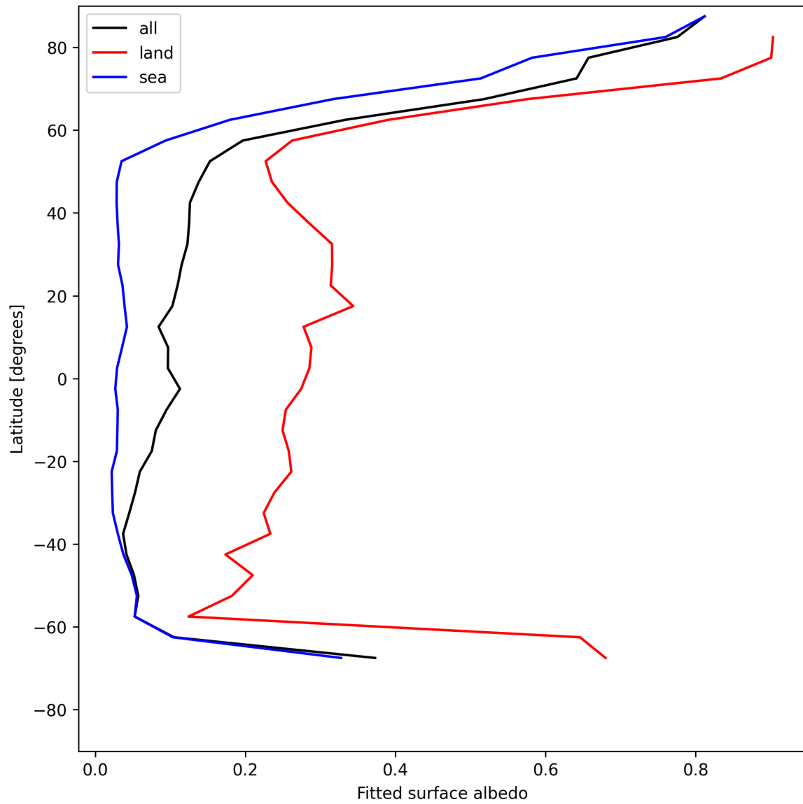
Figure 27: Zonal average of “Fitted surface albedo” for 2025-05-19 to 2025-05-19.
