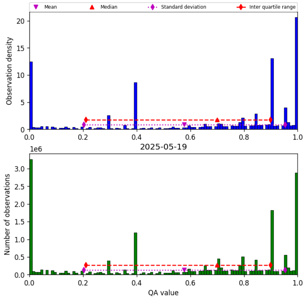
Figure 36: Histogram of “QA value” for 2025-05-19 to 2025-05-19
