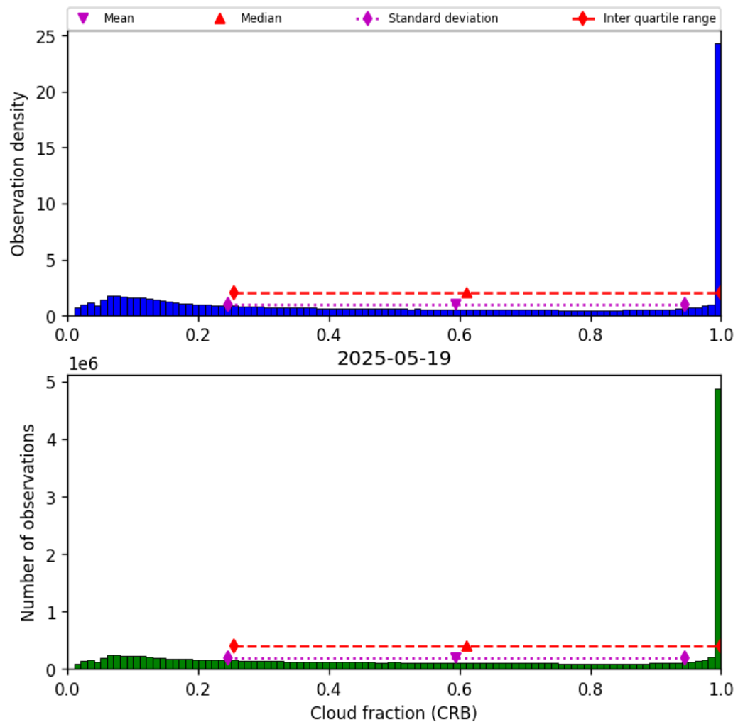
Figure 40: Histogram of “Cloud fraction (CRB)” for 2025-05-19 to 2025-05-19
