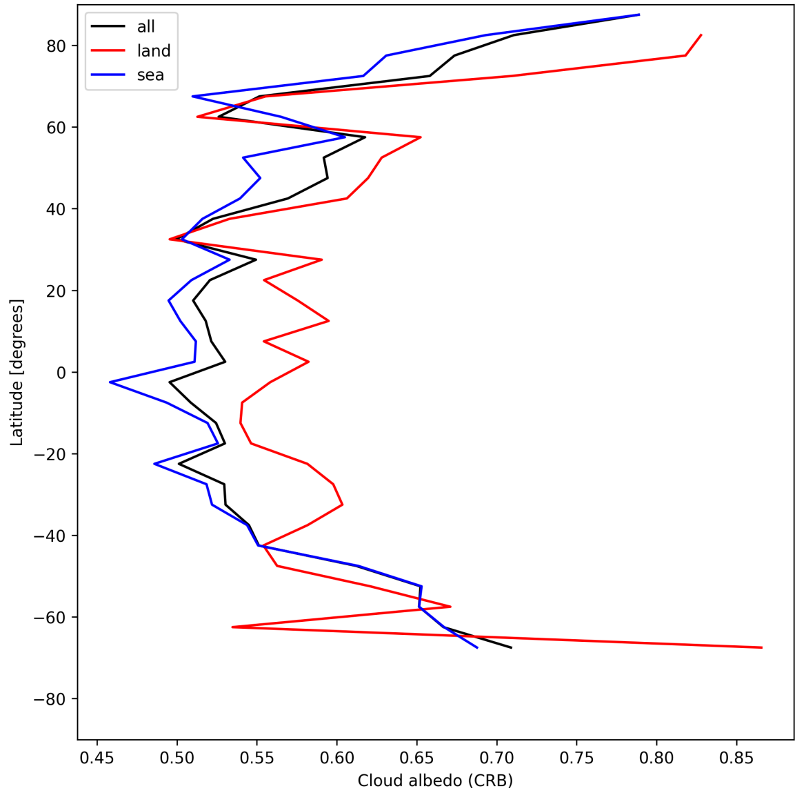
Figure 26: Zonal average of “Cloud albedo (CRB)” for 2025-05-19 to 2025-05-19.
