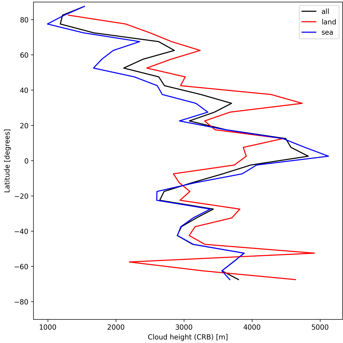
Figure 25: Zonal average of “Cloud height (CRB)” for 2025-05-19 to 2025-05-19.
