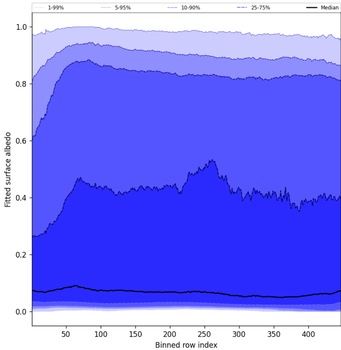
Figure 59: Along track statistics of “Fitted surface albedo” for 2025-05-19 to 2025-05-19
