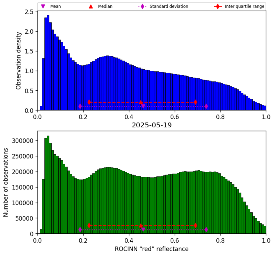
Figure 51: Histogram of “ROCINN “red” reflectance” for 2025-05-19 to 2025-05-19
