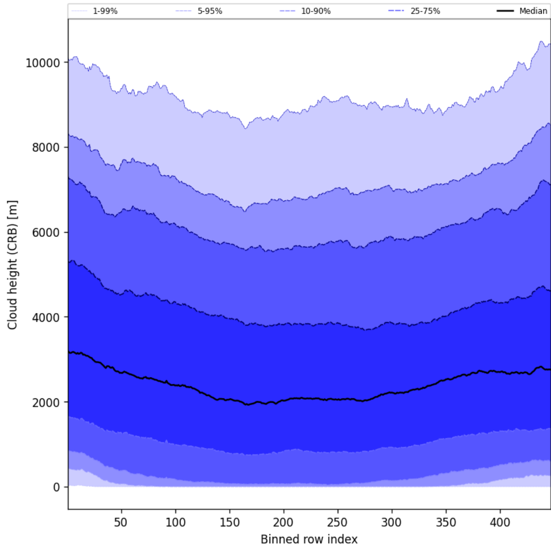
Figure 57: Along track statistics of “Cloud height (CRB)” for 2025-05-19 to 2025-05-19
