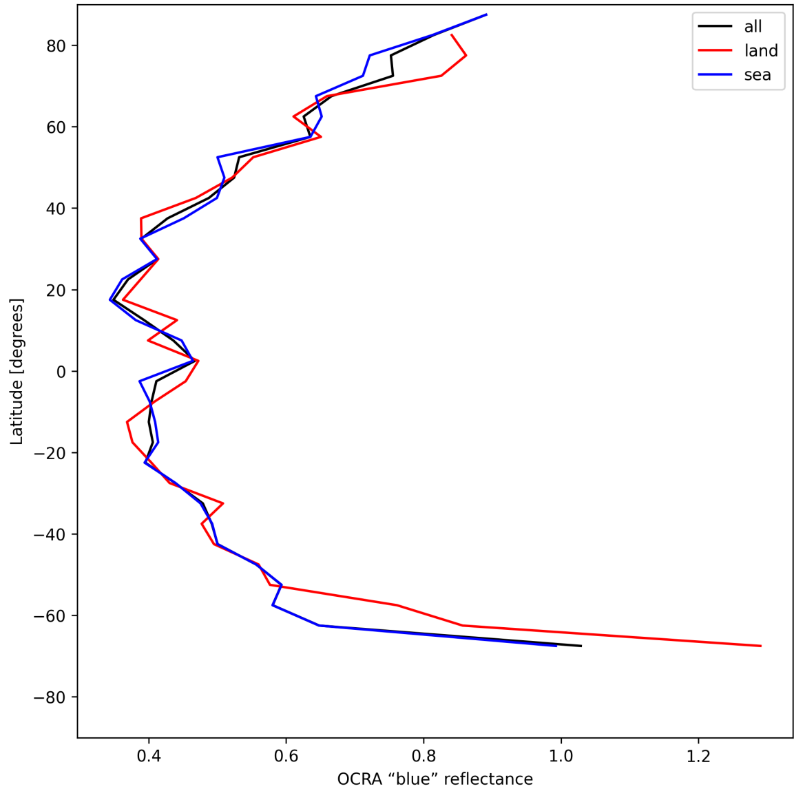
Figure 33: Zonal average of “OCRA “blue” reflectance” for 2025-05-19 to 2025-05-19.
