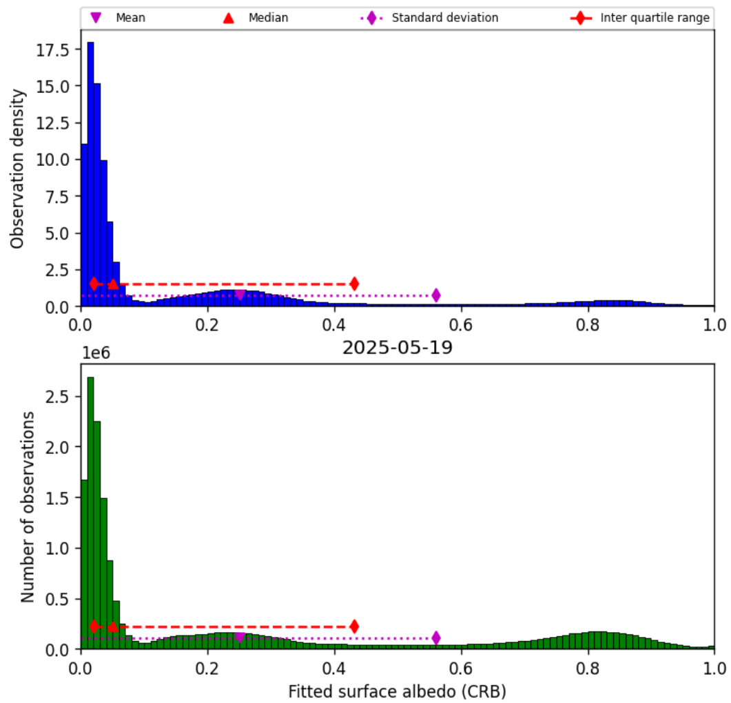
Figure 44: Histogram of “Fitted surface albedo (CRB)” for 2025-05-19 to 2025-05-19
