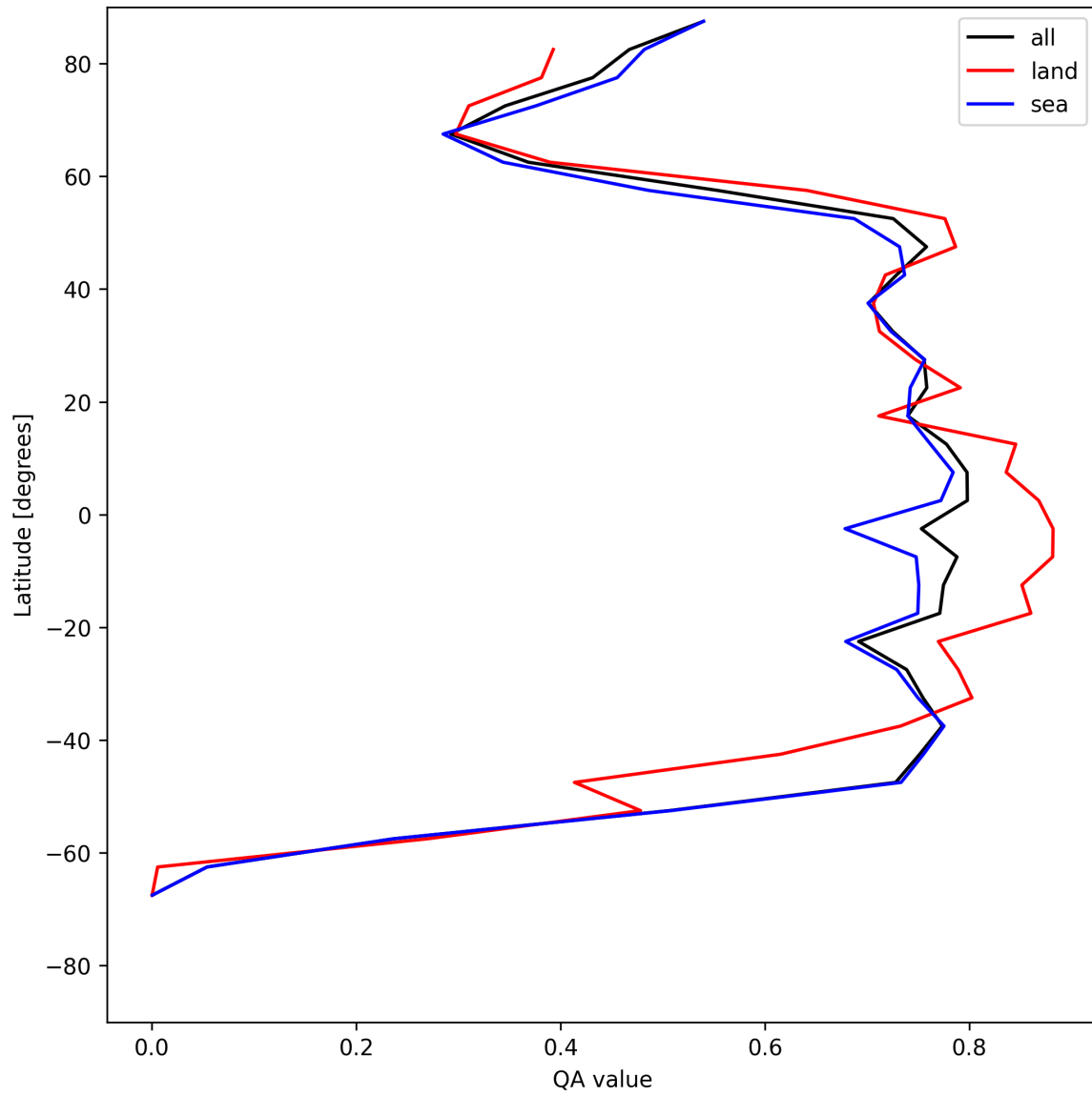
Figure 20: Zonal average of “QA value” for 2025-05-19 to 2025-05-19.
