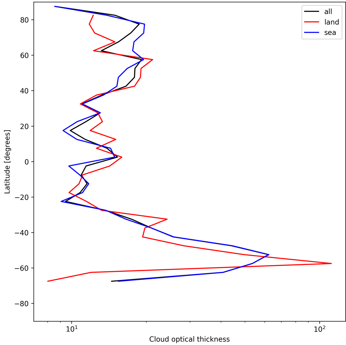
Figure 23: Zonal average of “Cloud optical thickness” for 2025-05-19 to 2025-05-19.
