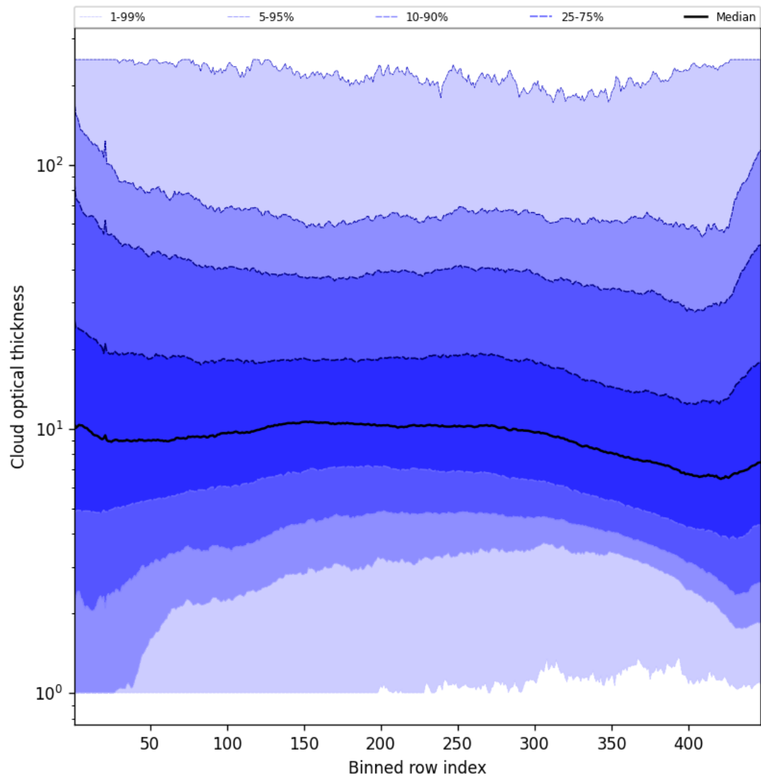
Figure 55: Along track statistics of “Cloud optical thickness” for 2025-05-19 to 2025-05-19
