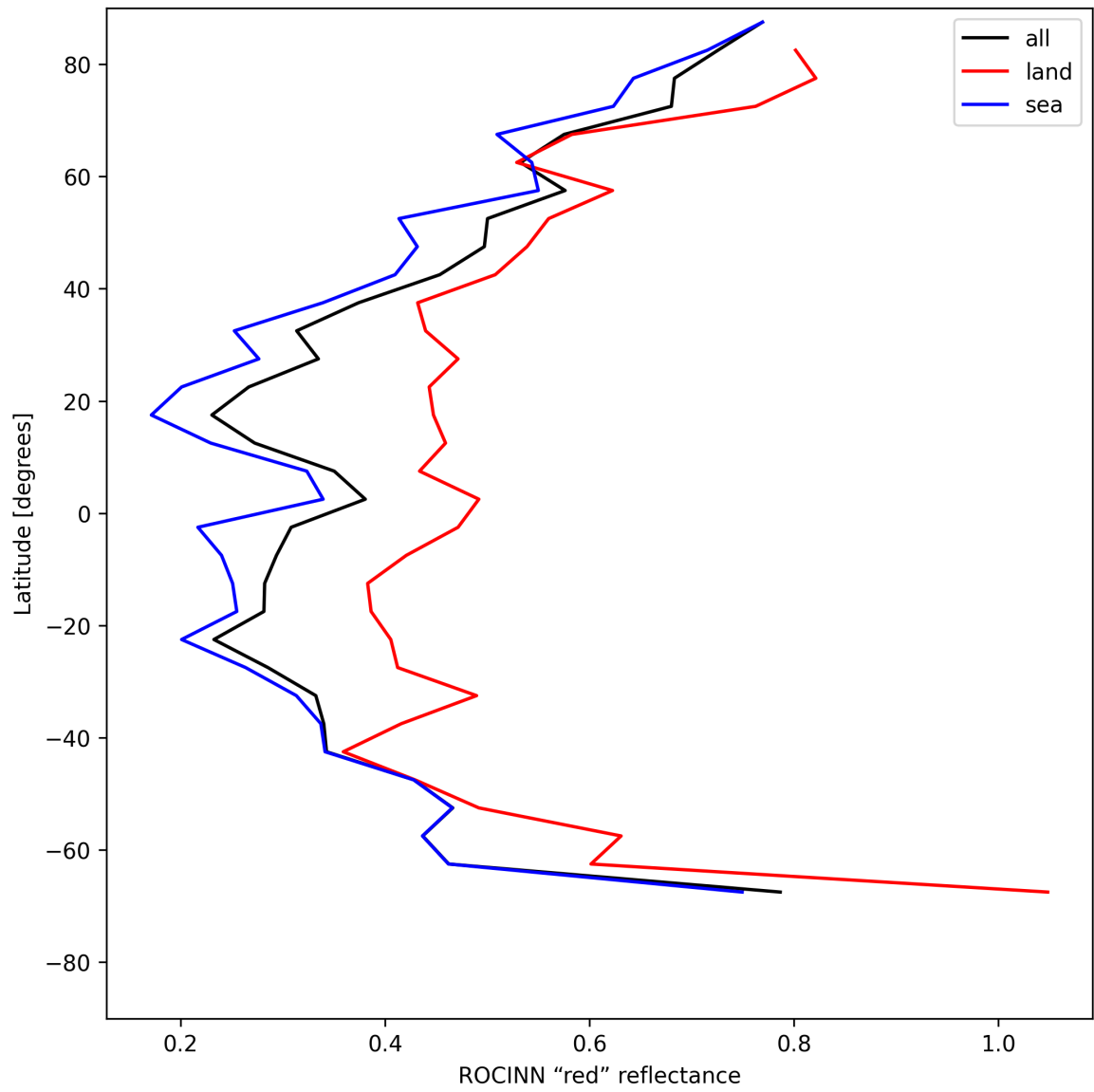
Figure 35: Zonal average of “ROCINN “red” reflectance” for 2025-05-19 to 2025-05-19.
