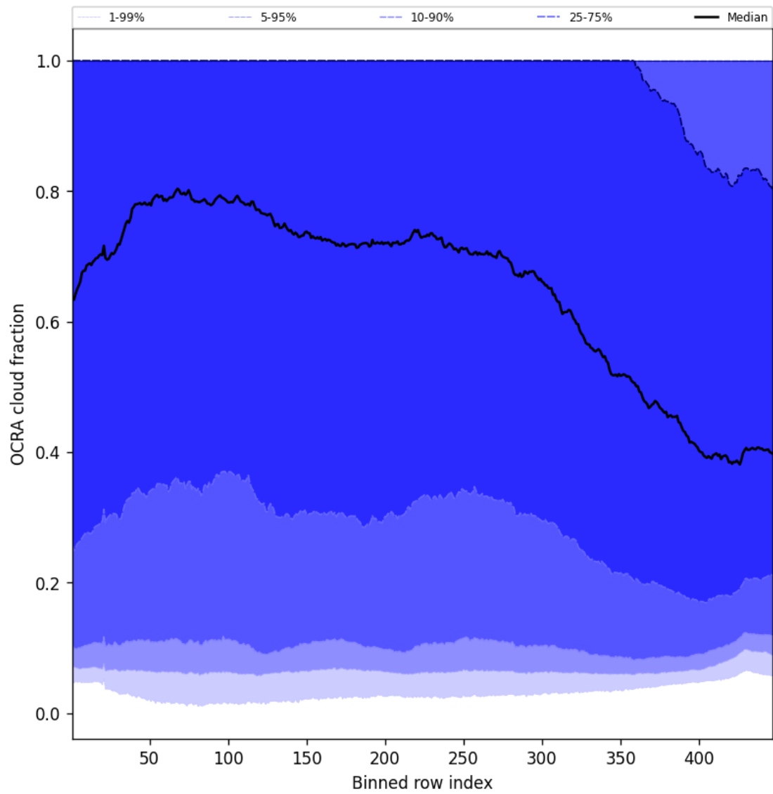
Figure 64: Along track statistics of “OCRA cloud fraction” for 2025-05-19 to 2025-05-19
