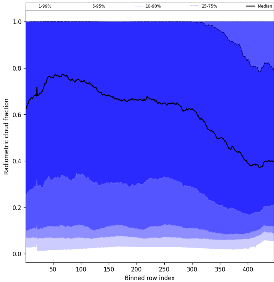
Figure 53: Along track statistics of “Radiometric cloud fraction” for 2025-05-19 to 2025-05-19
