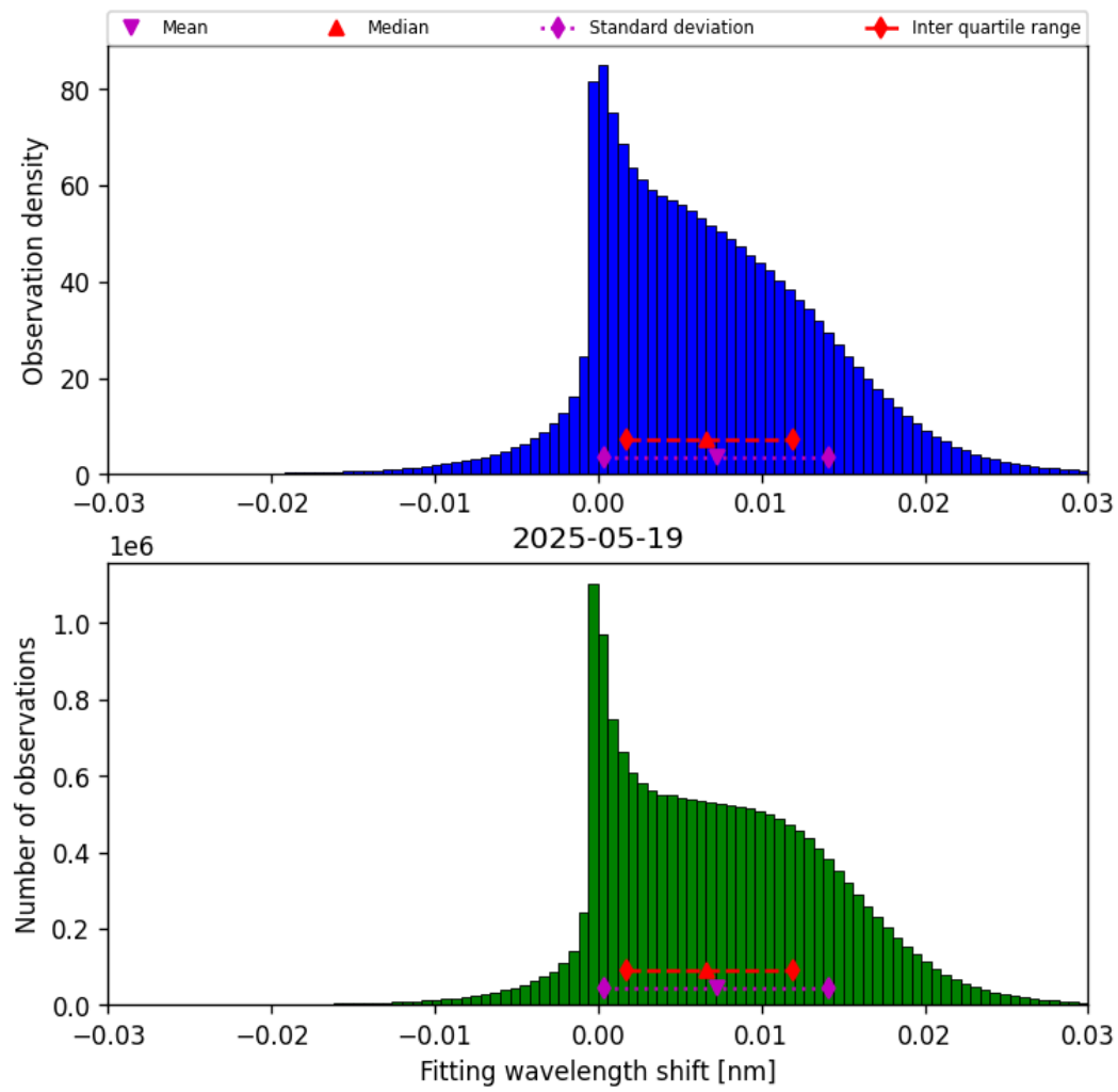
Figure 47: Histogram of “Fitting wavelength shift” for 2025-05-19 to 2025-05-19
