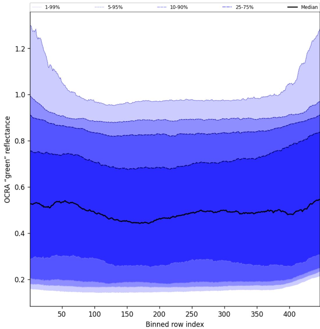
Figure 66: Along track statistics of "OCRA "green" reflectance" for 2025-05-19 to 2025-05-19
