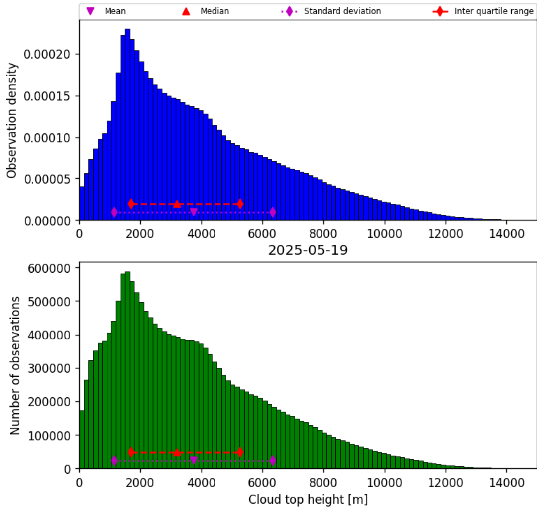
Figure 38: Histogram of “Cloud top height” for 2025-05-19 to 2025-05-19
