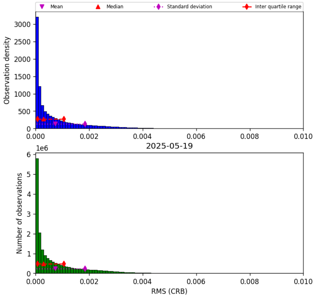
Figure 46: Histogram of “RMS (CRB)” for 2025-05-19 to 2025-05-19
