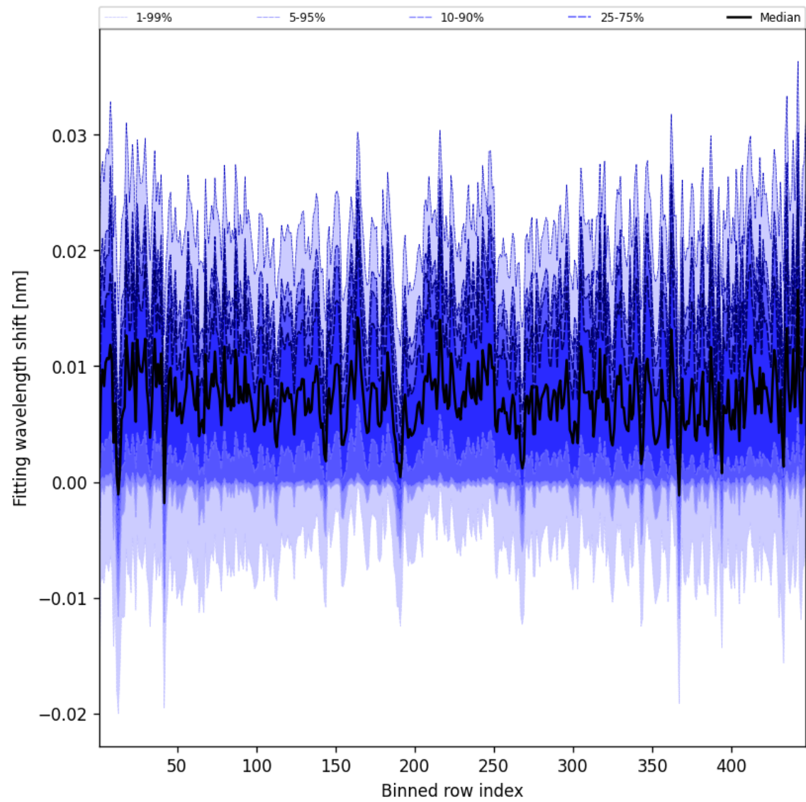
Figure 63: Along track statistics of “Fitting wavelength shift” for 2025-05-19 to 2025-05-19
