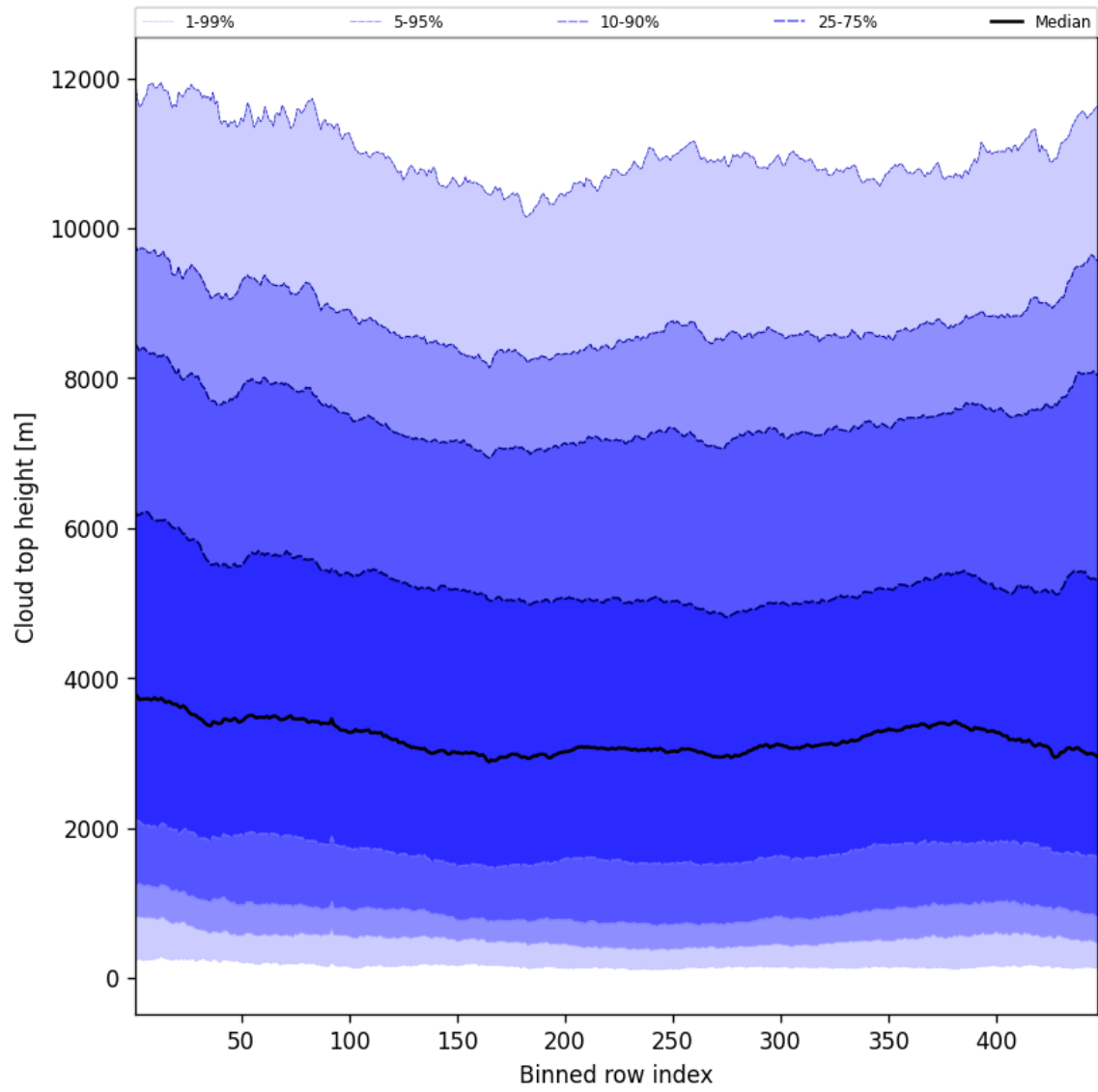
Figure 54: Along track statistics of “Cloud top height” for 2025-05-19 to 2025-05-19
