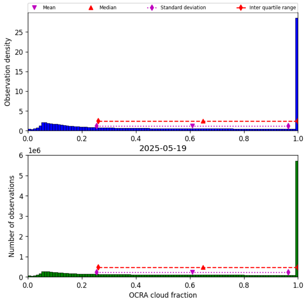
Figure 48: Histogram of “OCRA cloud fraction” for 2025-05-19 to 2025-05-19
