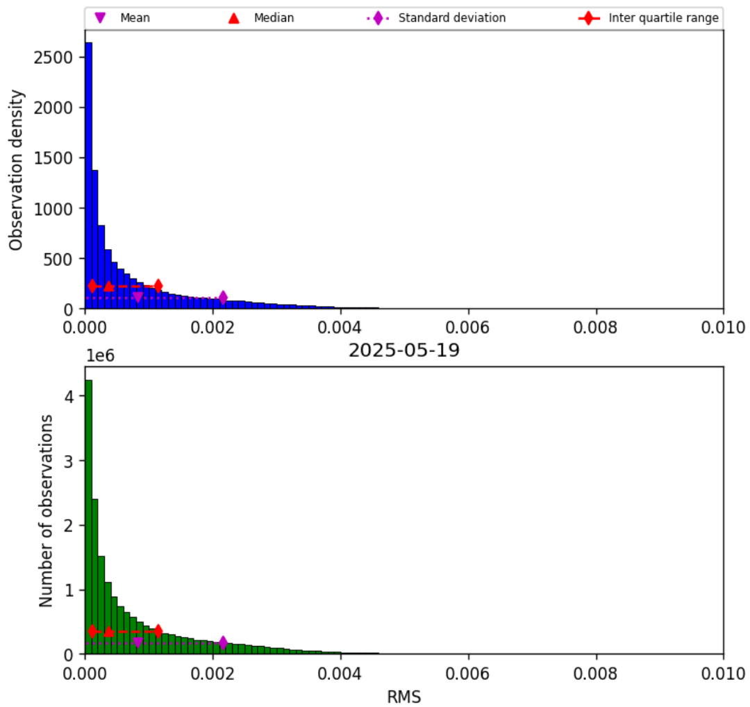
Figure 45: Histogram of “RMS” for 2025-05-19 to 2025-05-19
