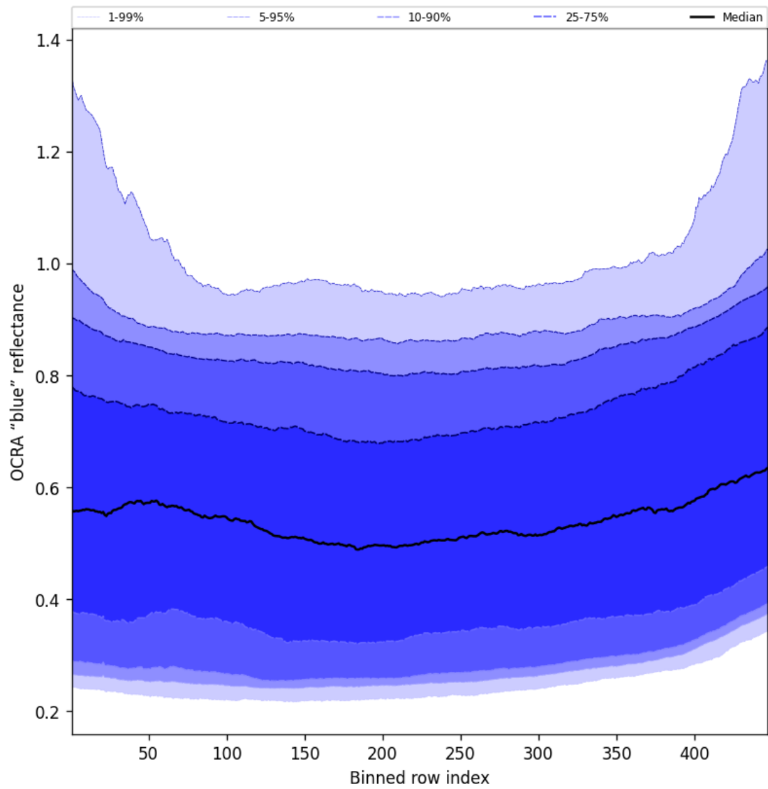
Figure 65: Along track statistics of “OCRA “blue” reflectance” for 2025-05-21 to 2025-05-22
