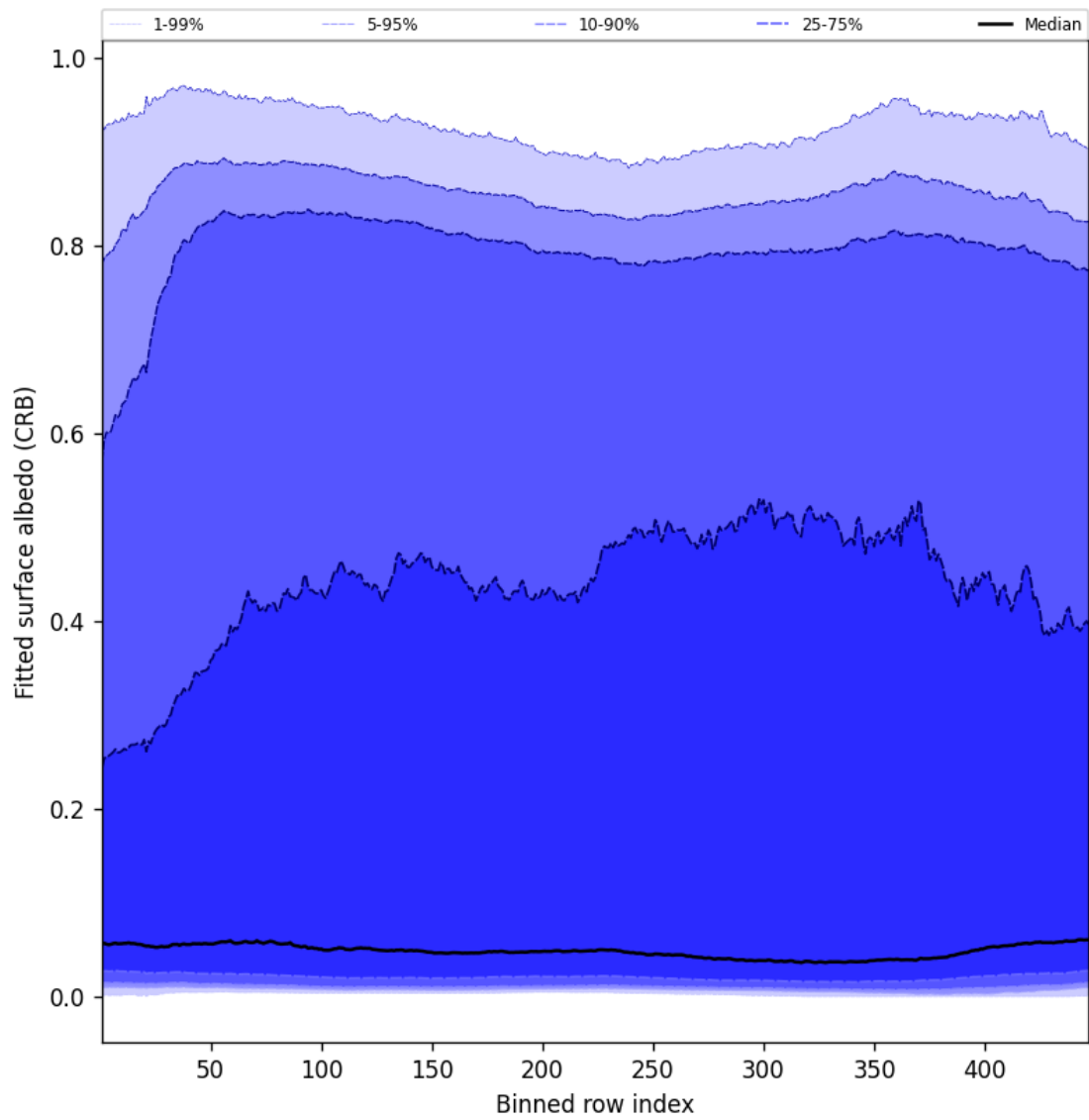
Figure 60: Along track statistics of “Fitted surface albedo (CRB)” for 2025-05-21 to 2025-05-22
