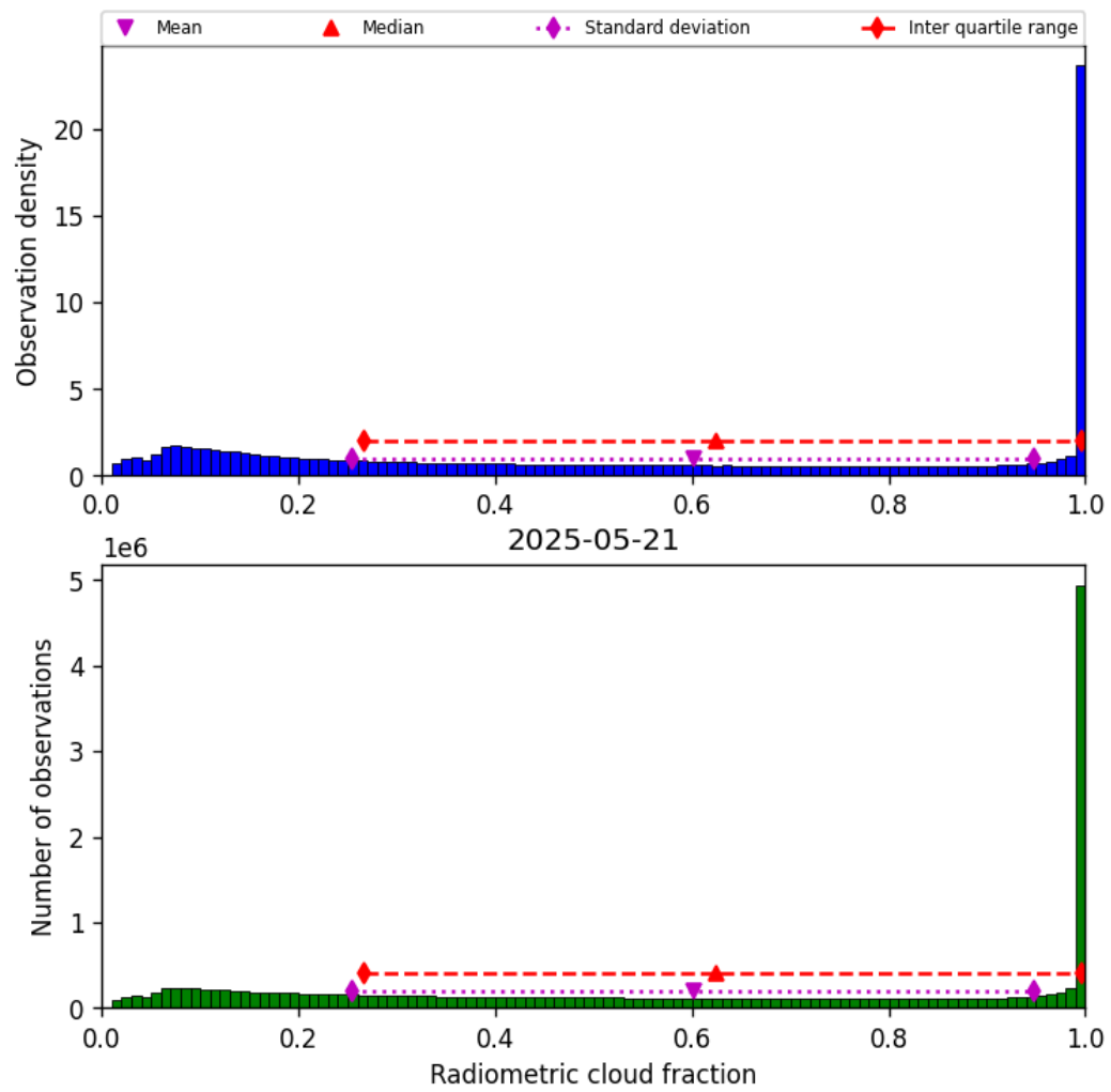
Figure 37: Histogram of “Radiometric cloud fraction” for 2025-05-21 to 2025-05-22
