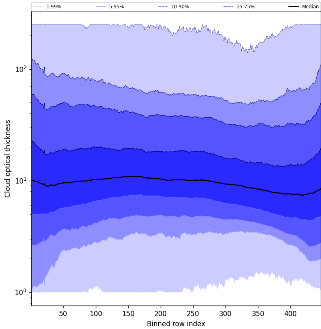
Figure 55: Along track statistics of “Cloud optical thickness” for 2025-05-21 to 2025-05-22
