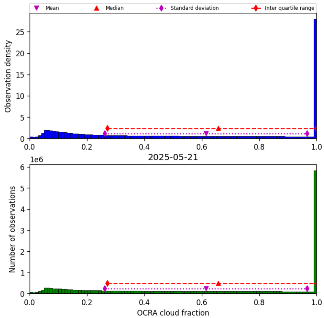
Figure 48: Histogram of “OCRA cloud fraction” for 2025-05-21 to 2025-05-22
