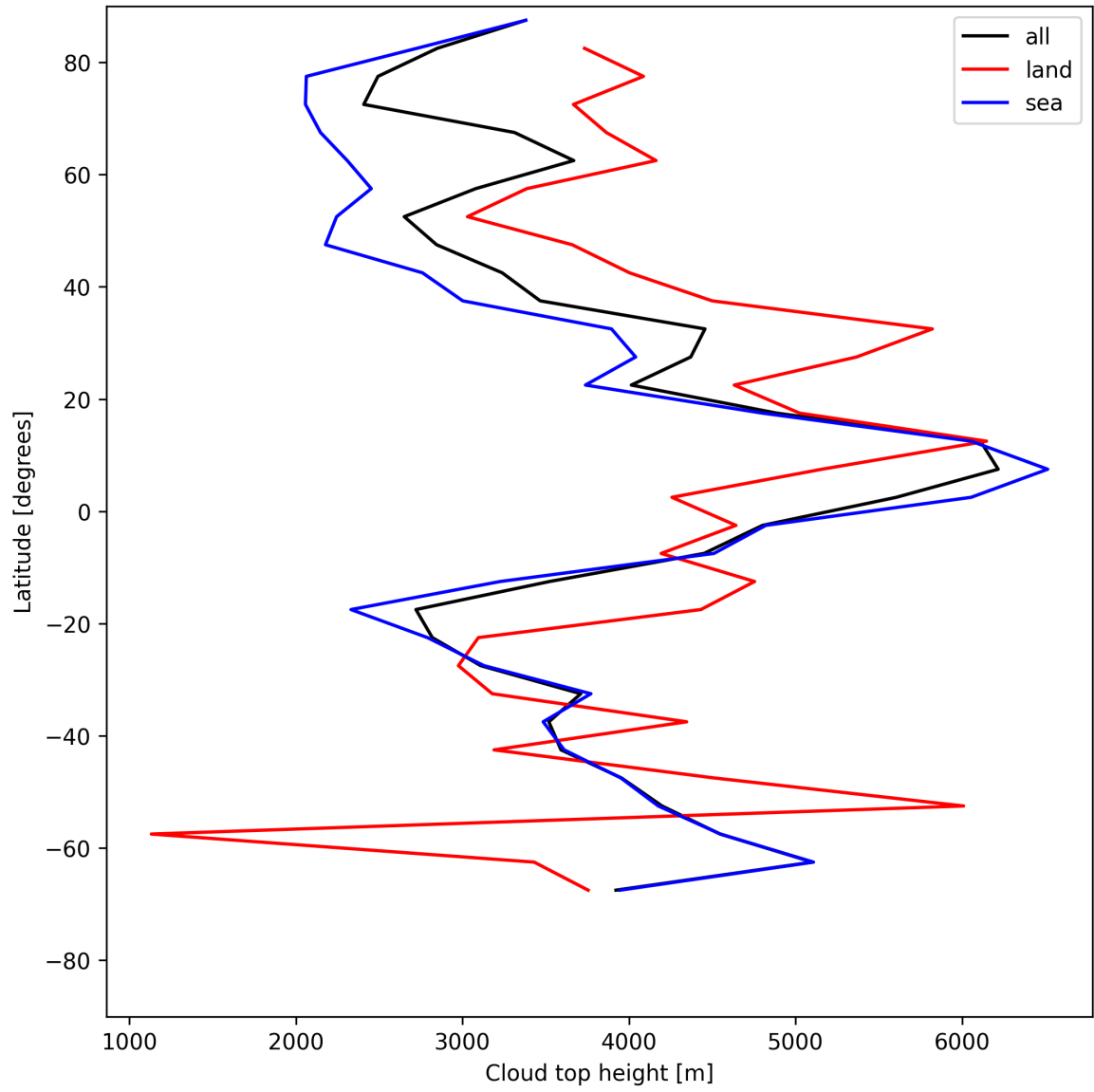
Figure 22: Zonal average of “Cloud top height” for 2025-05-21 to 2025-05-22.
