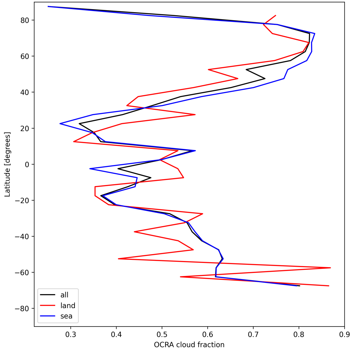
Figure 32: Zonal average of “OCRA cloud fraction” for 2025-05-21 to 2025-05-22.
