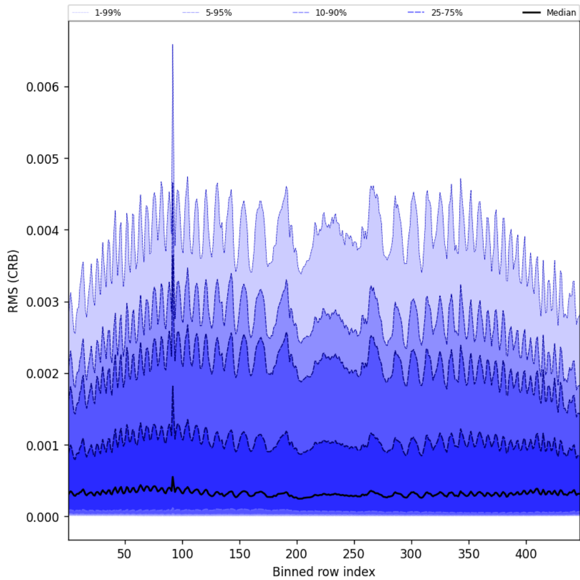
Figure 62: Along track statistics of “RMS (CRB)” for 2025-05-21 to 2025-05-22
