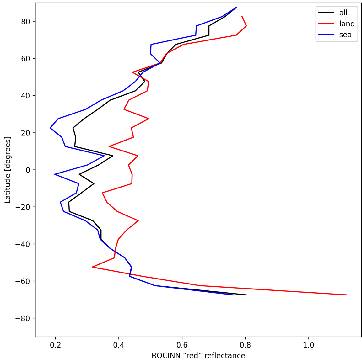
Figure 35: Zonal average of “ROCINN “red” reflectance” for 2025-05-21 to 2025-05-22.
