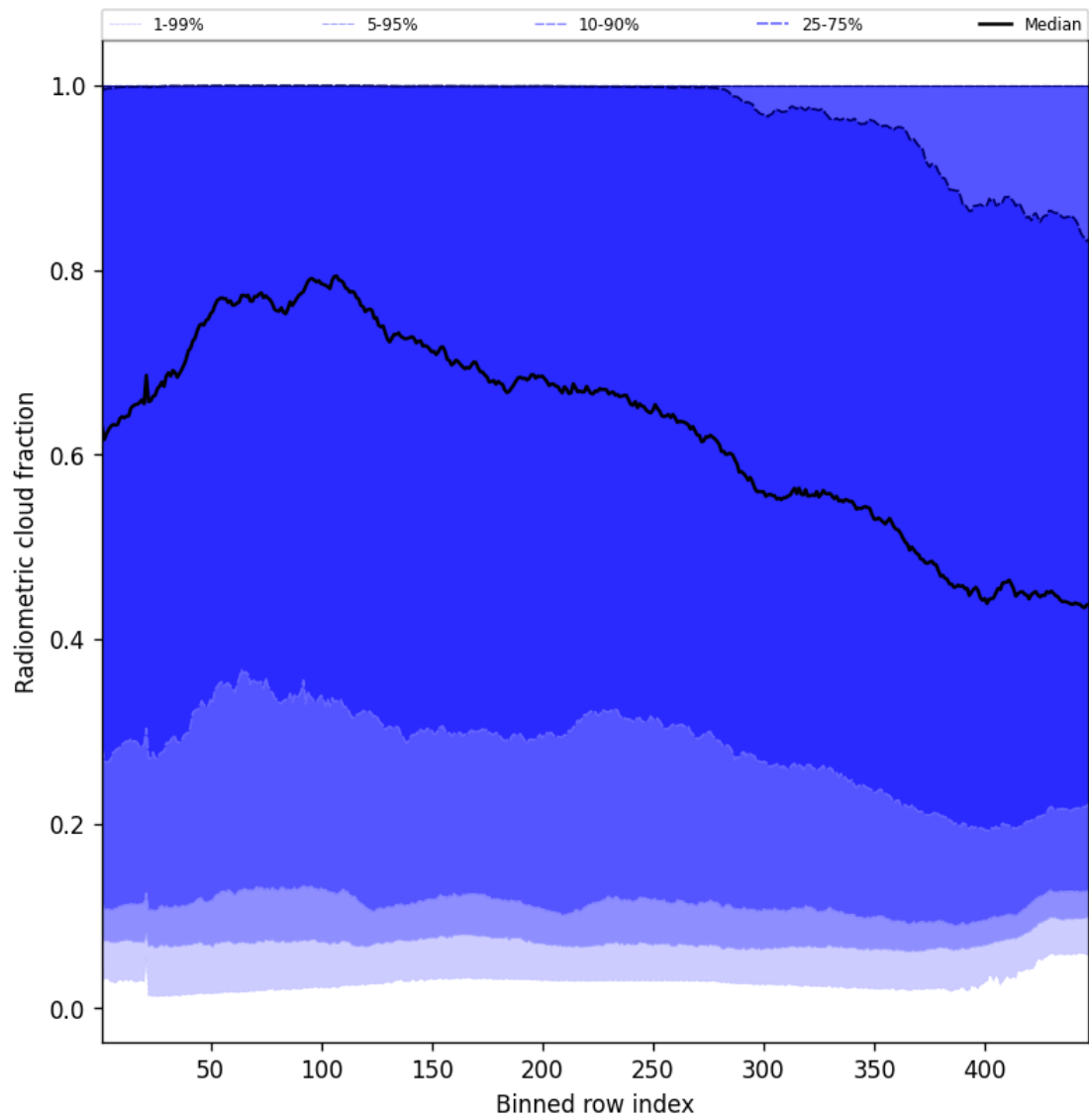
Figure 53: Along track statistics of “Radiometric cloud fraction” for 2025-05-21 to 2025-05-22
