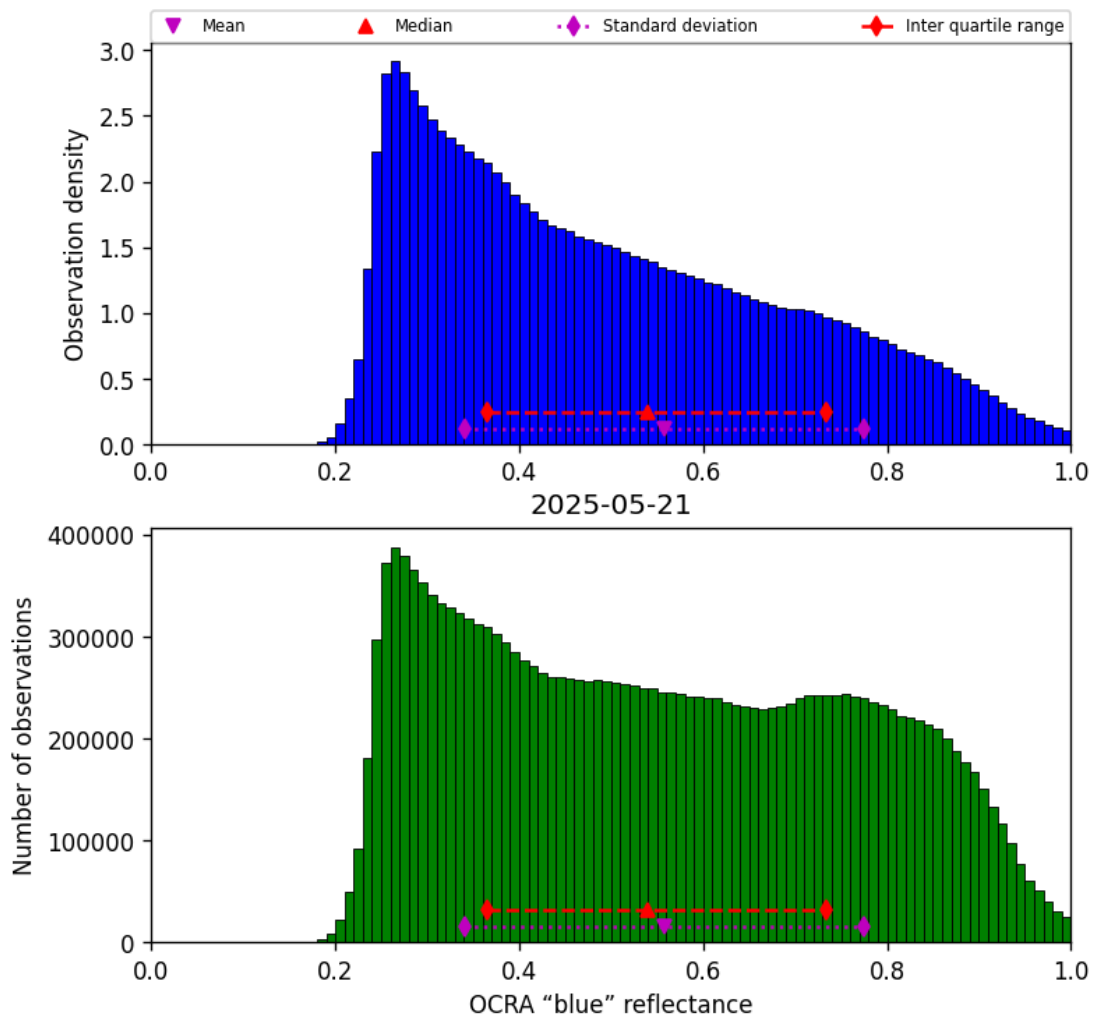
Figure 49: Histogram of “OCRA “blue” reflectance” for 2025-05-21 to 2025-05-22
