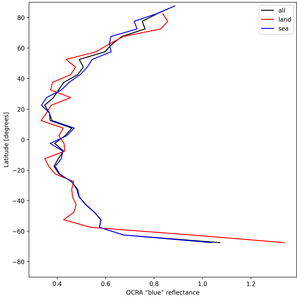
Figure 33: Zonal average of “OCRA “blue” reflectance” for 2025-05-21 to 2025-05-22.
