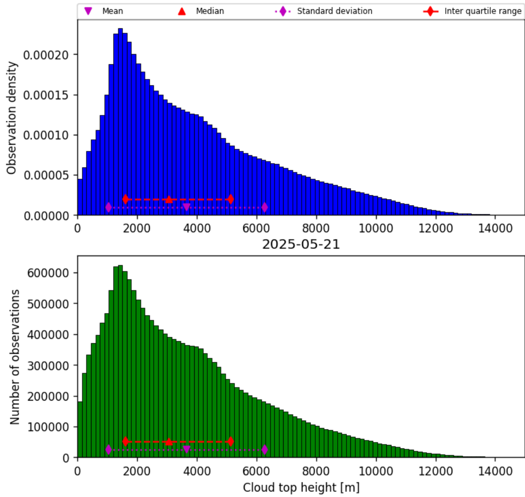
Figure 38: Histogram of “Cloud top height” for 2025-05-21 to 2025-05-22
