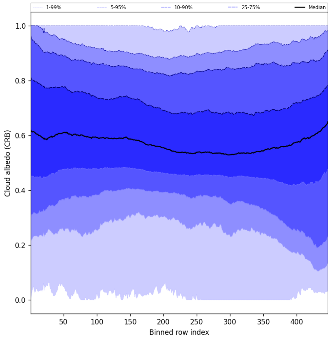
Figure 58: Along track statistics of “Cloud albedo (CRB)” for 2025-05-21 to 2025-05-22
