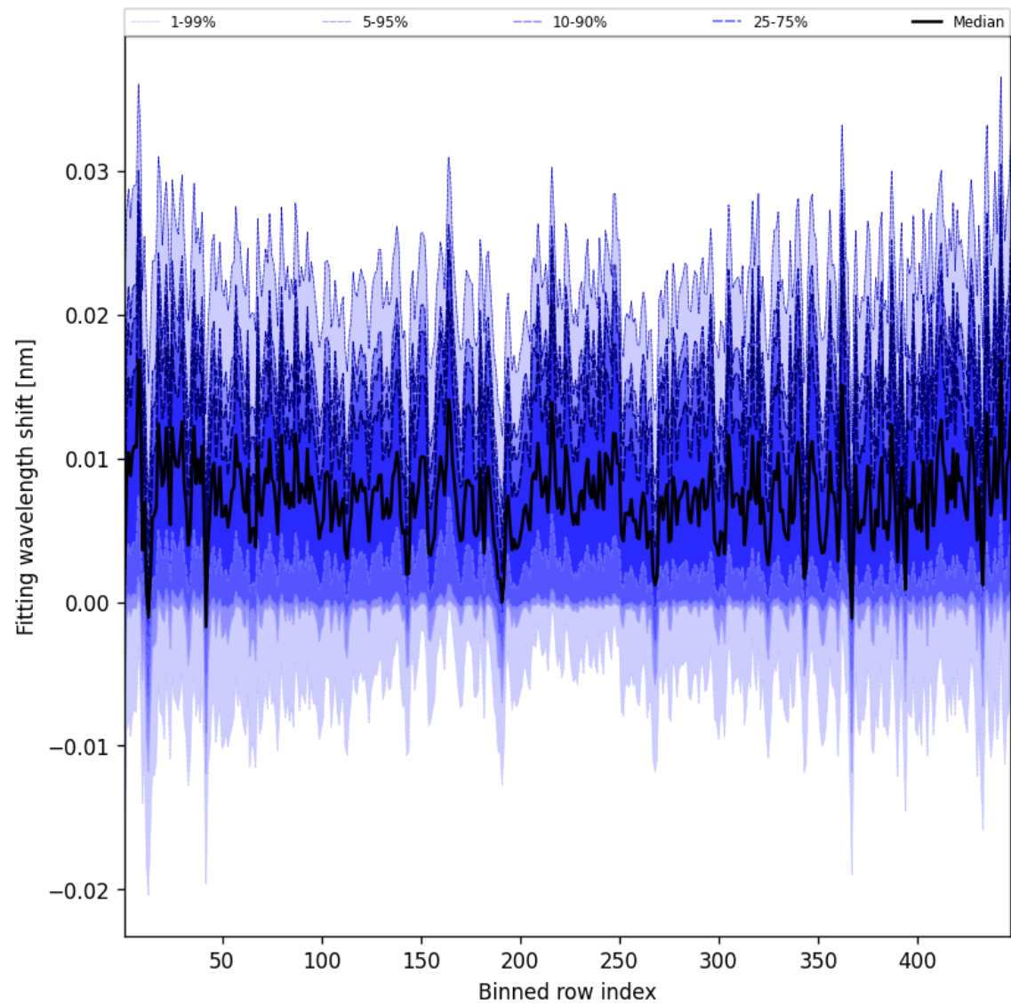
Figure 63: Along track statistics of “Fitting wavelength shift” for 2025-05-21 to 2025-05-22
