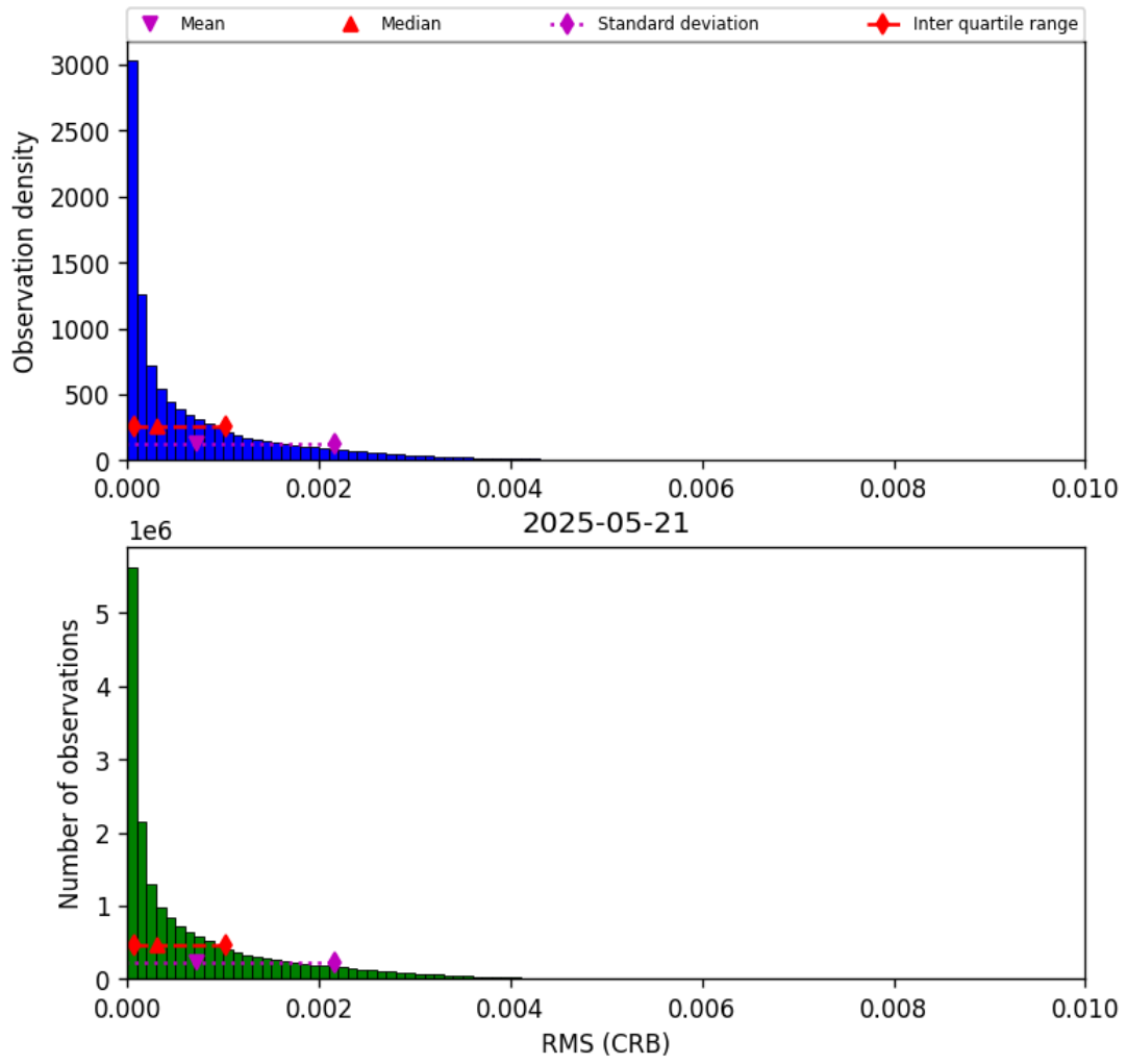
Figure 46: Histogram of "RMS (CRB)" for 2025-05-21 to 2025-05-22
