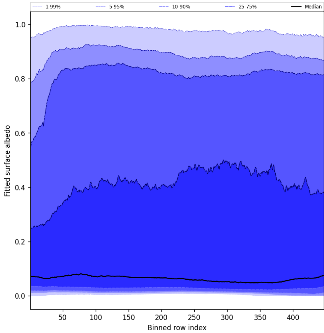
Figure 59: Along track statistics of “Fitted surface albedo” for 2025-05-21 to 2025-05-22
