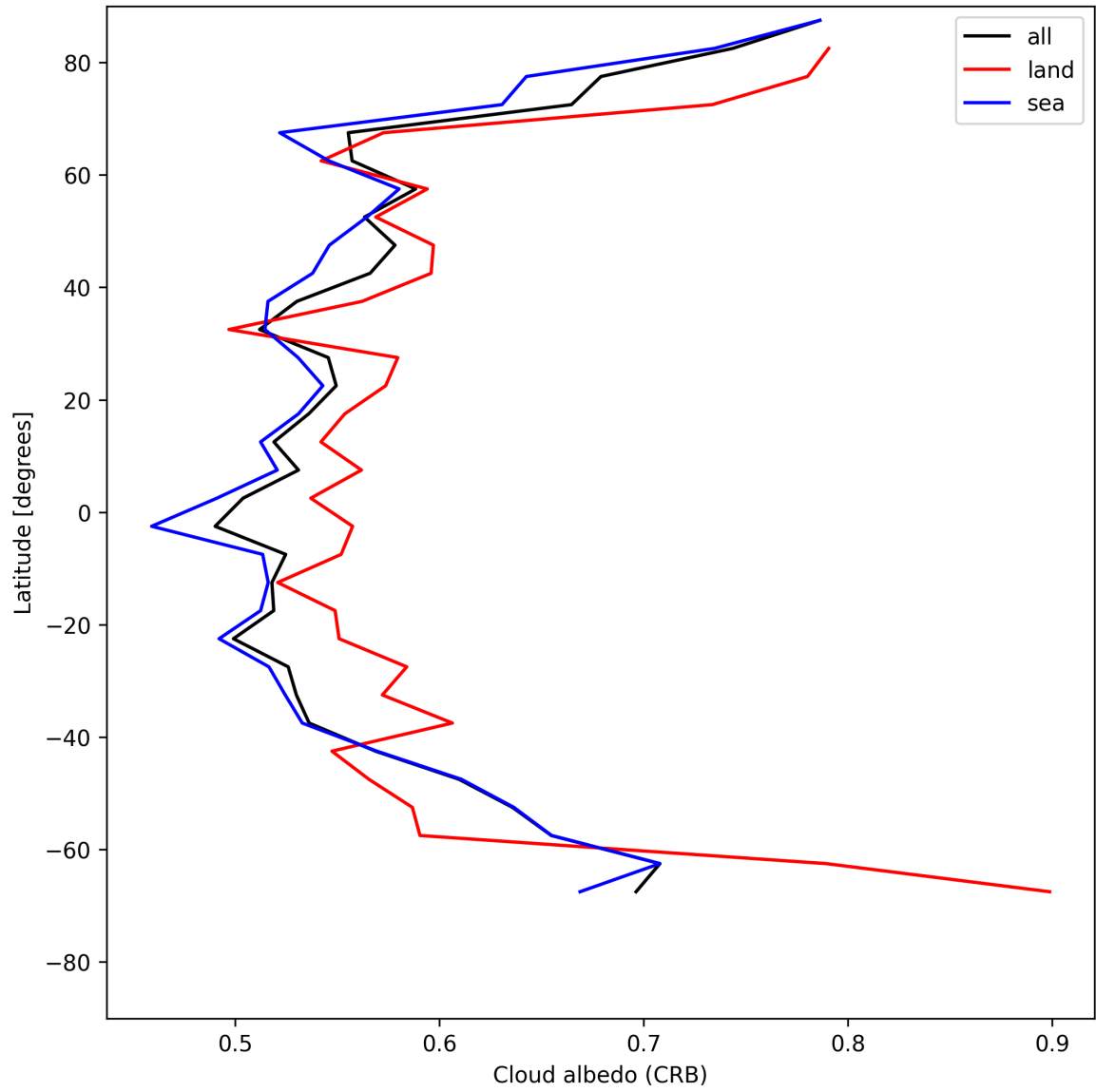
Figure 26: Zonal average of “Cloud albedo (CRB)” for 2025-05-21 to 2025-05-22.
