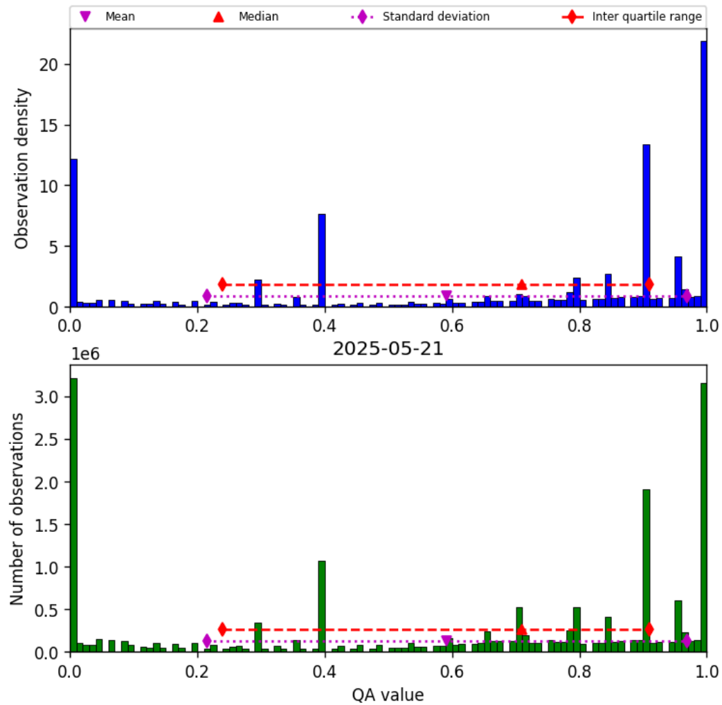
Figure 36: Histogram of “QA value” for 2025-05-21 to 2025-05-22
