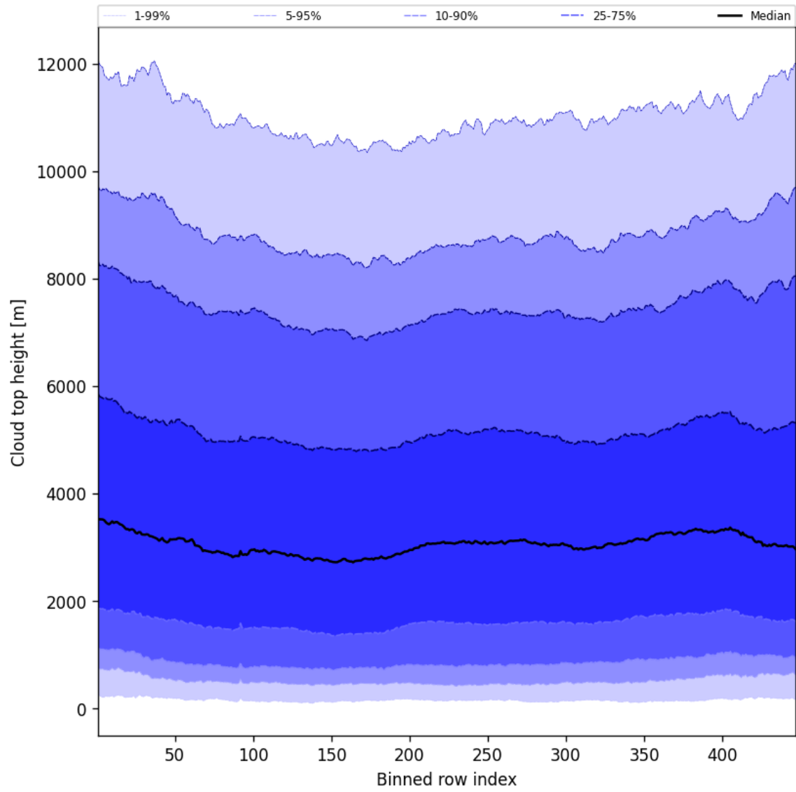
Figure 54: Along track statistics of “Cloud top height” for 2025-05-21 to 2025-05-22
