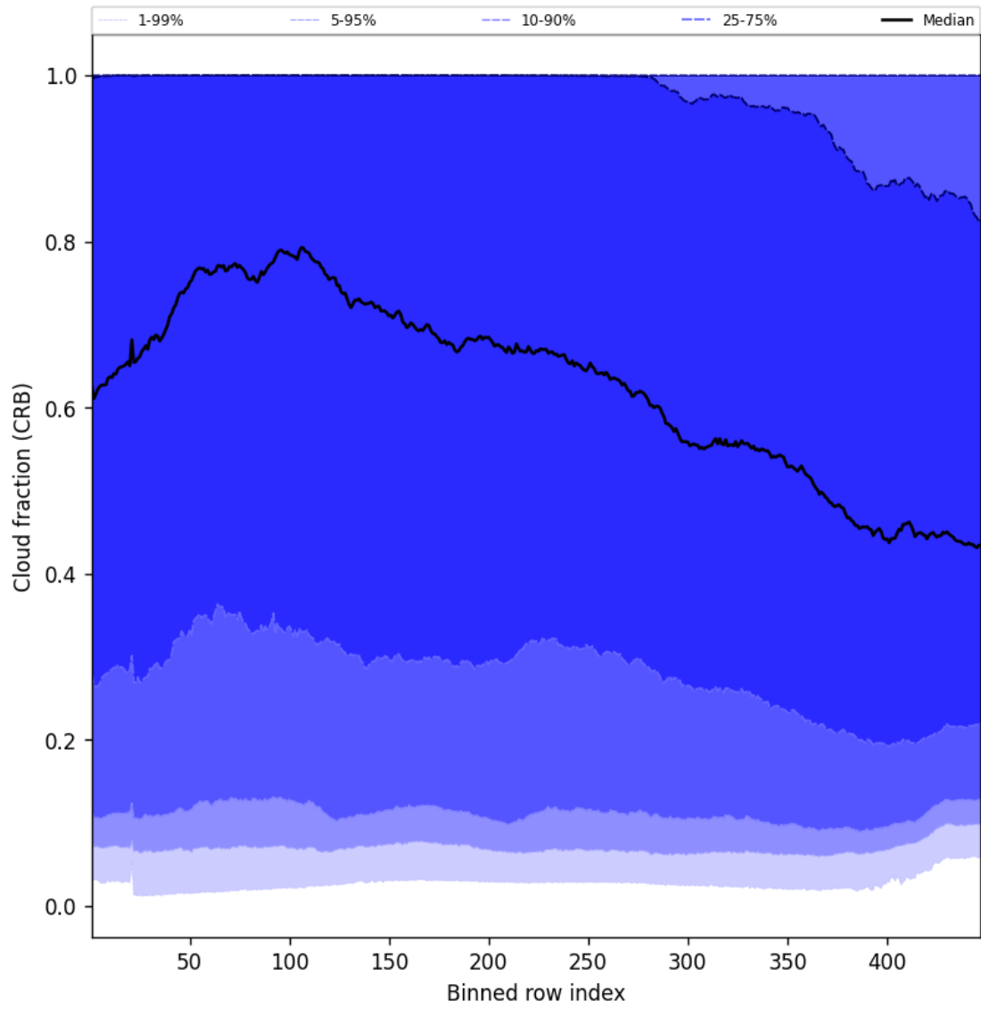
Figure 56: Along track statistics of “Cloud fraction (CRB)” for 2025-05-21 to 2025-05-22
