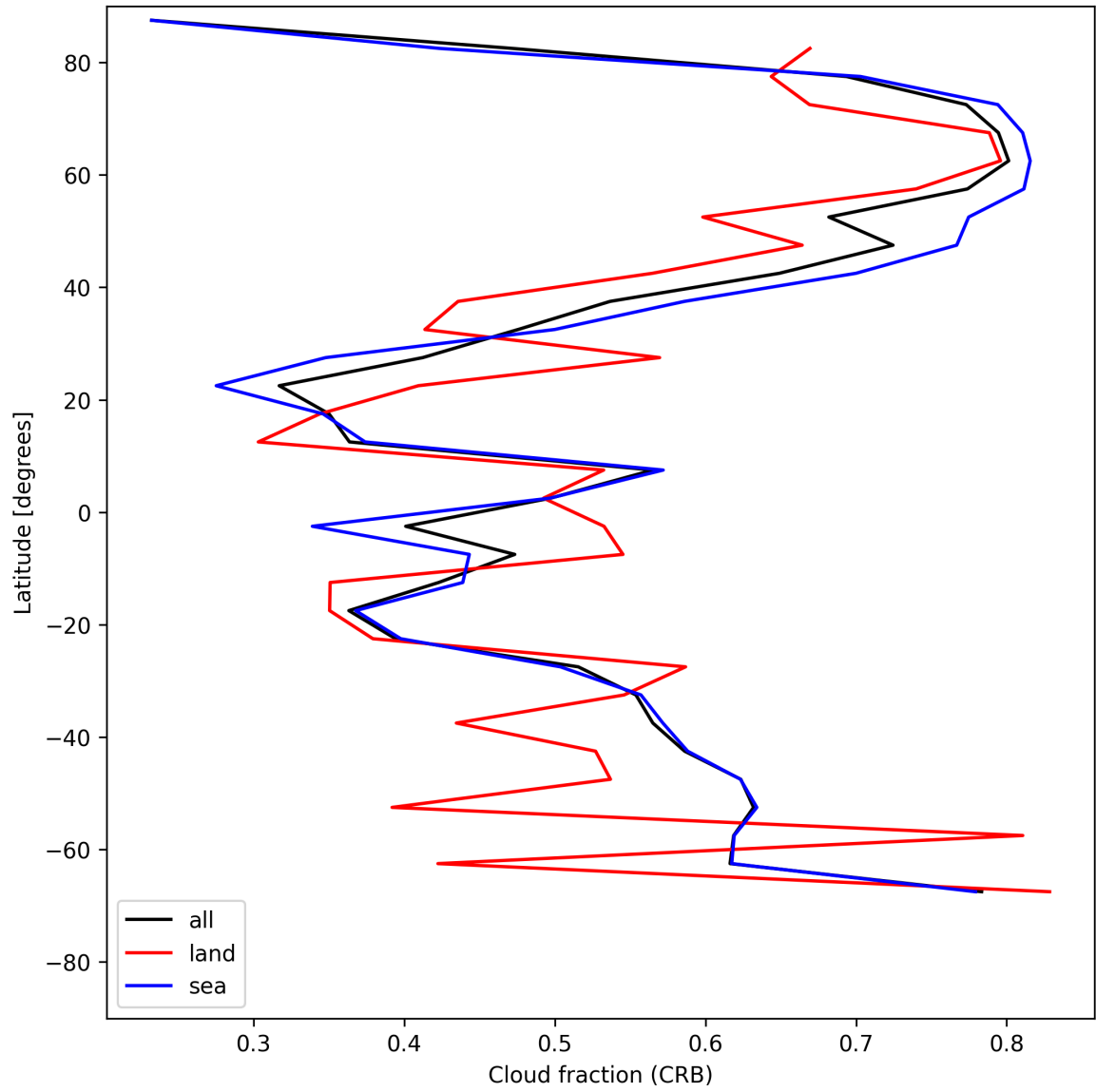
Figure 24: Zonal average of “Cloud fraction (CRB)” for 2025-05-21 to 2025-05-22.
