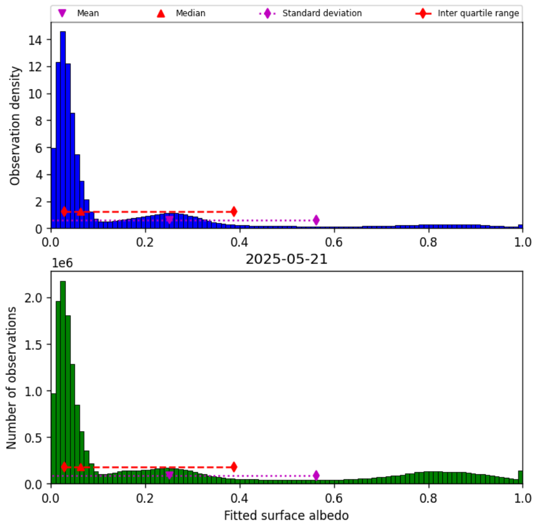
Figure 43: Histogram of “Fitted surface albedo” for 2025-05-21 to 2025-05-22
