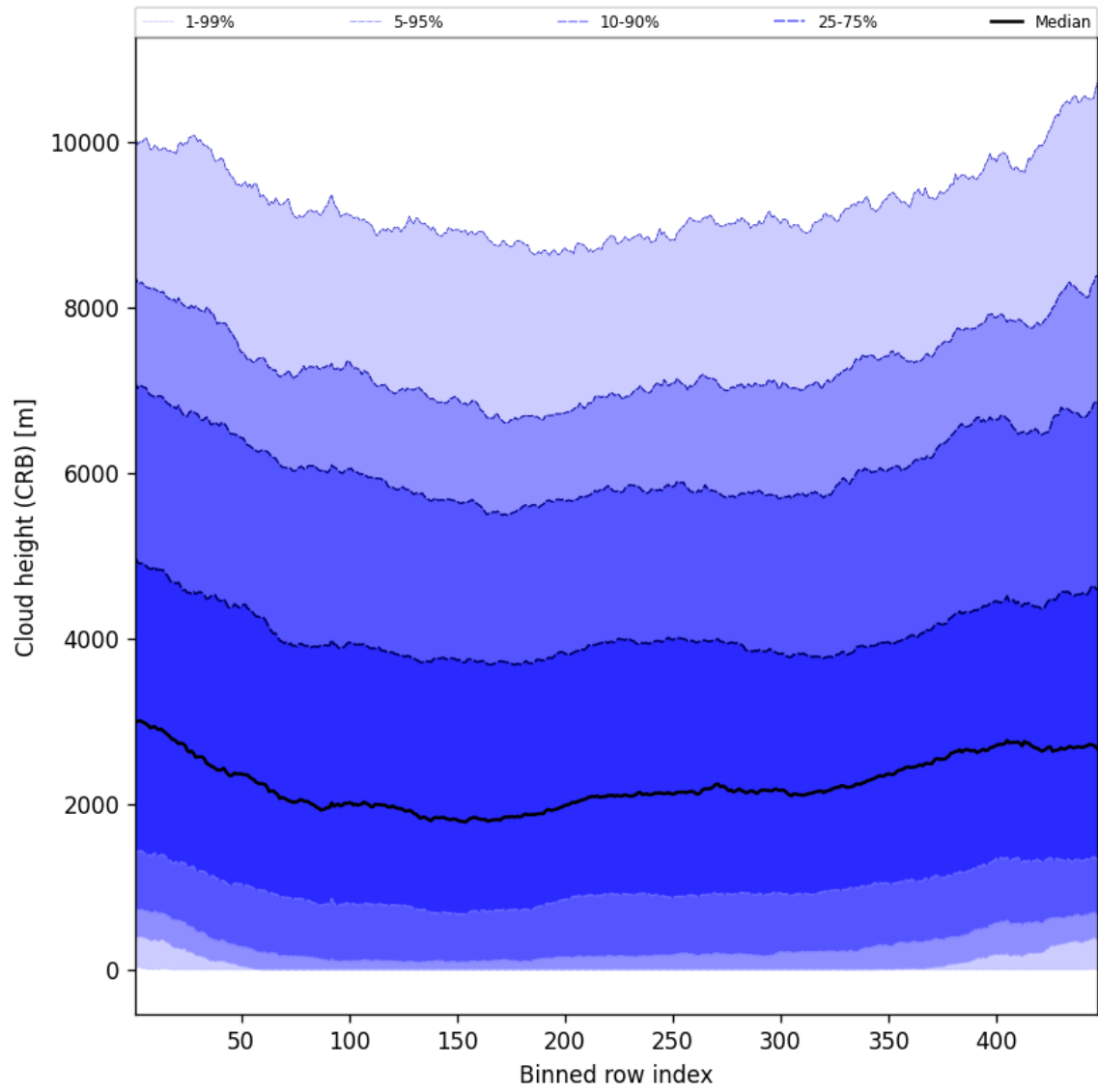
Figure 57: Along track statistics of “Cloud height (CRB)” for 2025-05-21 to 2025-05-22
