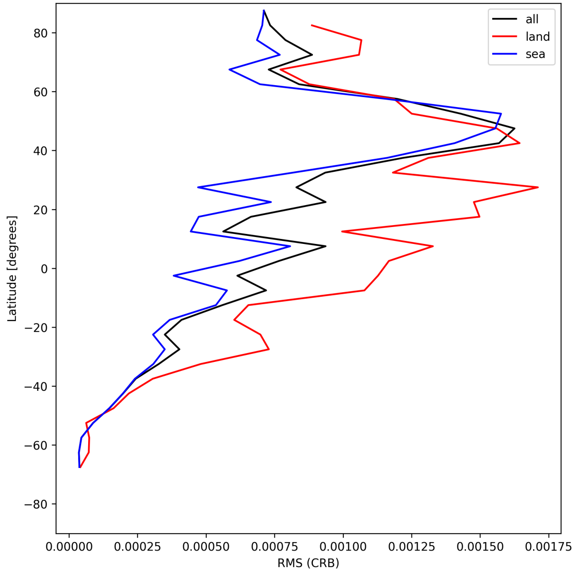
Figure 30: Zonal average of “RMS (CRB)” for 2025-05-21 to 2025-05-22.
