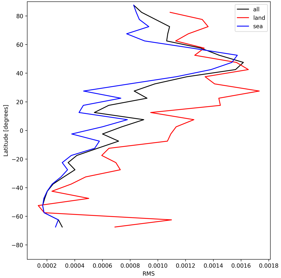
Figure 29: Zonal average of “RMS” for 2025-05-21 to 2025-05-22.
