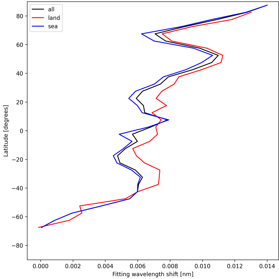
Figure 31: Zonal average of “Fitting wavelength shift” for 2025-05-21 to 2025-05-22.
