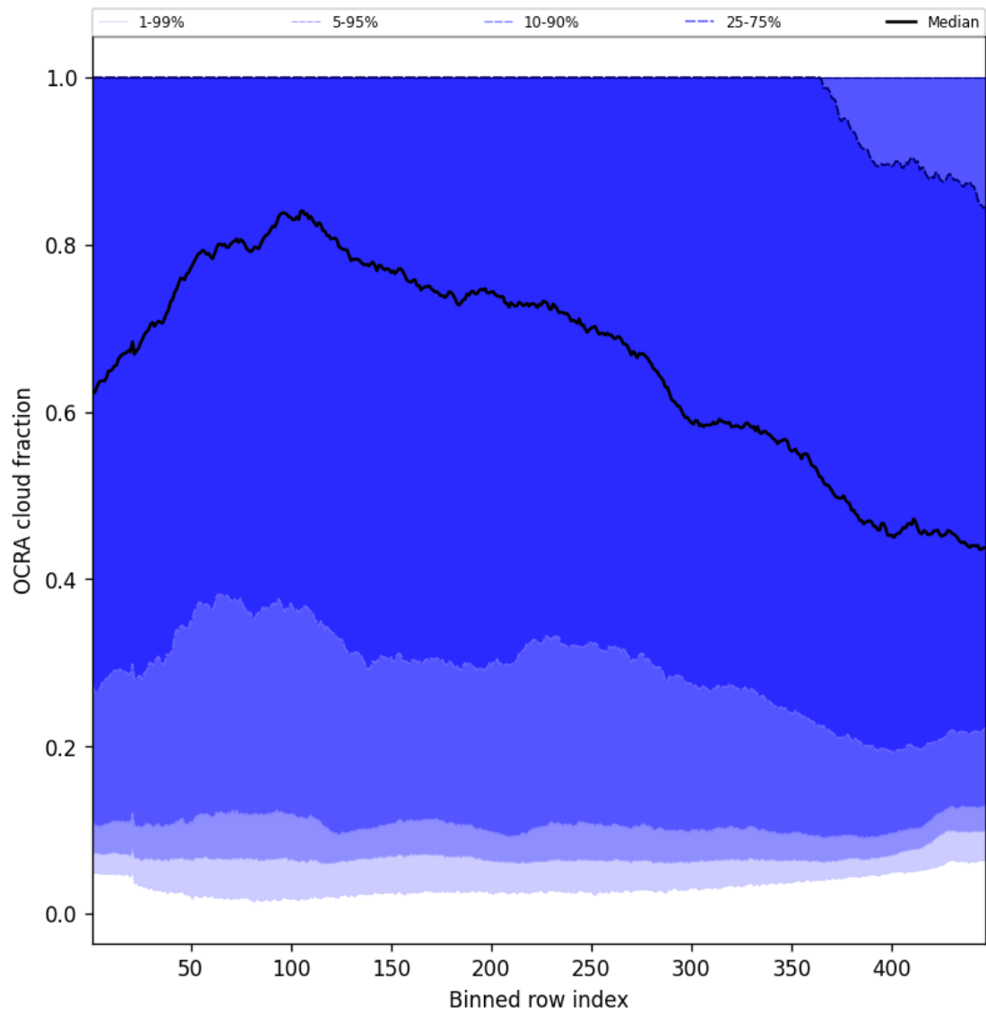
Figure 64: Along track statistics of “OCRA cloud fraction” for 2025-05-21 to 2025-05-22
