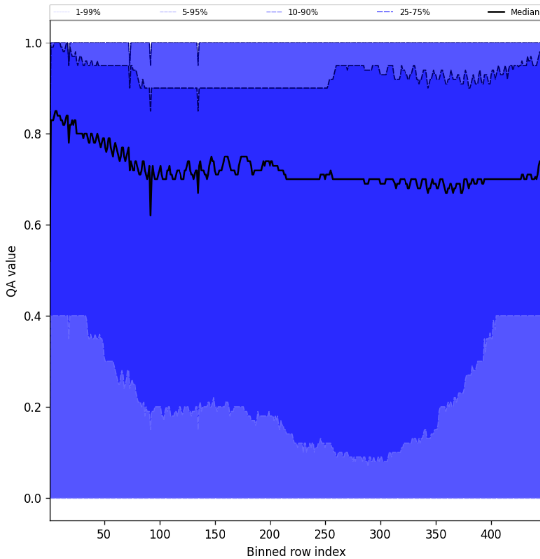
Figure 52: Along track statistics of “QA value” for 2025-05-21 to 2025-05-22
