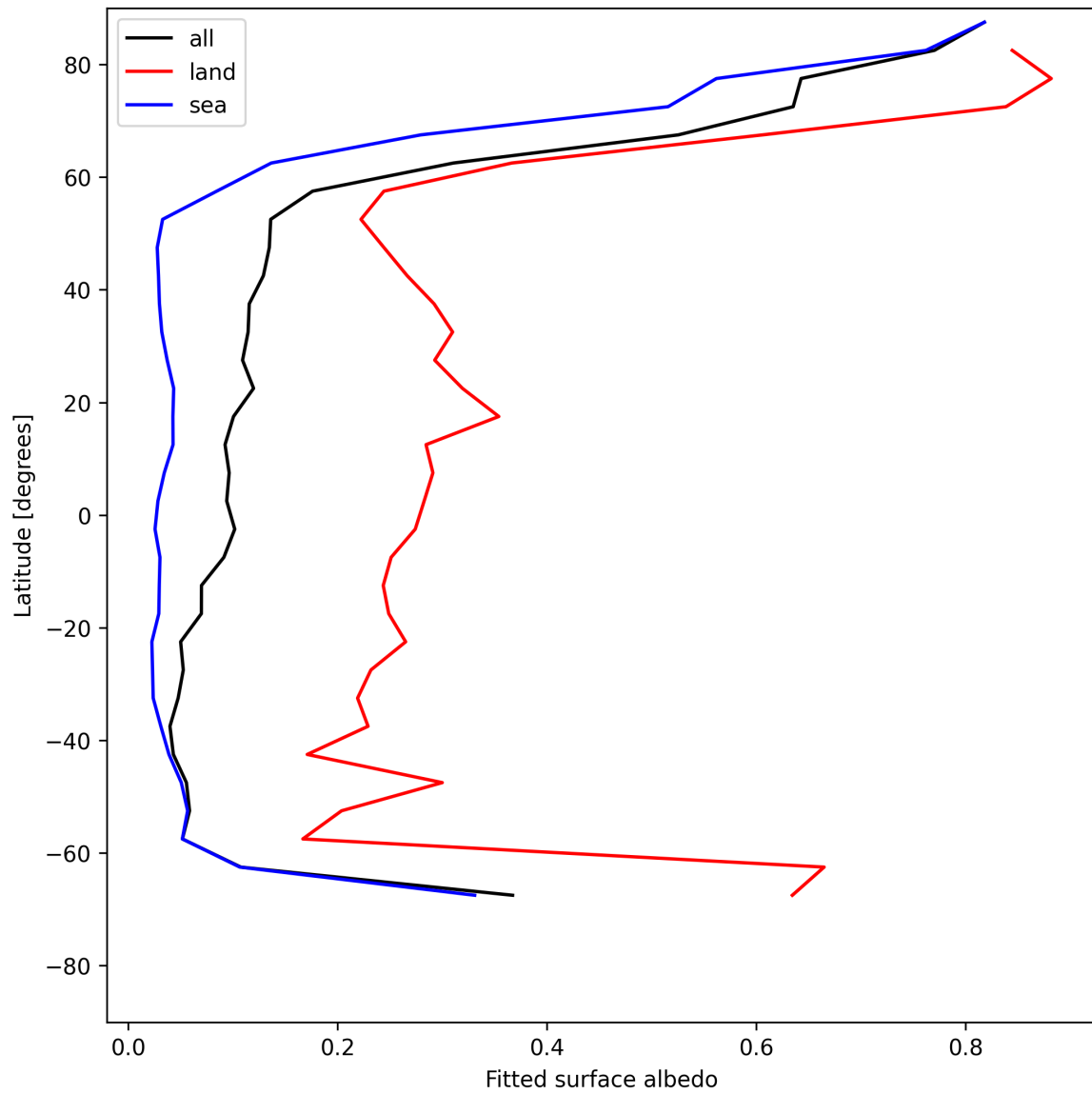
Figure 27: Zonal average of “Fitted surface albedo” for 2025-05-21 to 2025-05-22.
