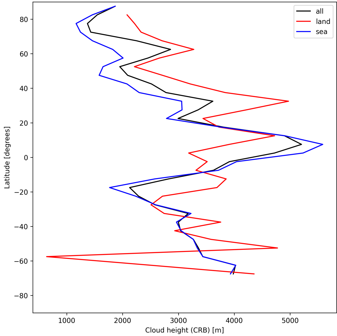
Figure 25: Zonal average of “Cloud height (CRB)” for 2025-05-21 to 2025-05-22.
