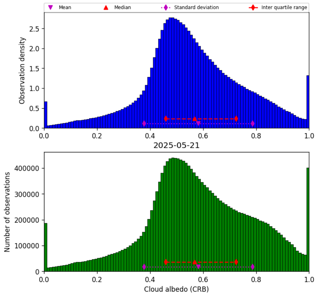
Figure 42: Histogram of “Cloud albedo (CRB)” for 2025-05-21 to 2025-05-22
