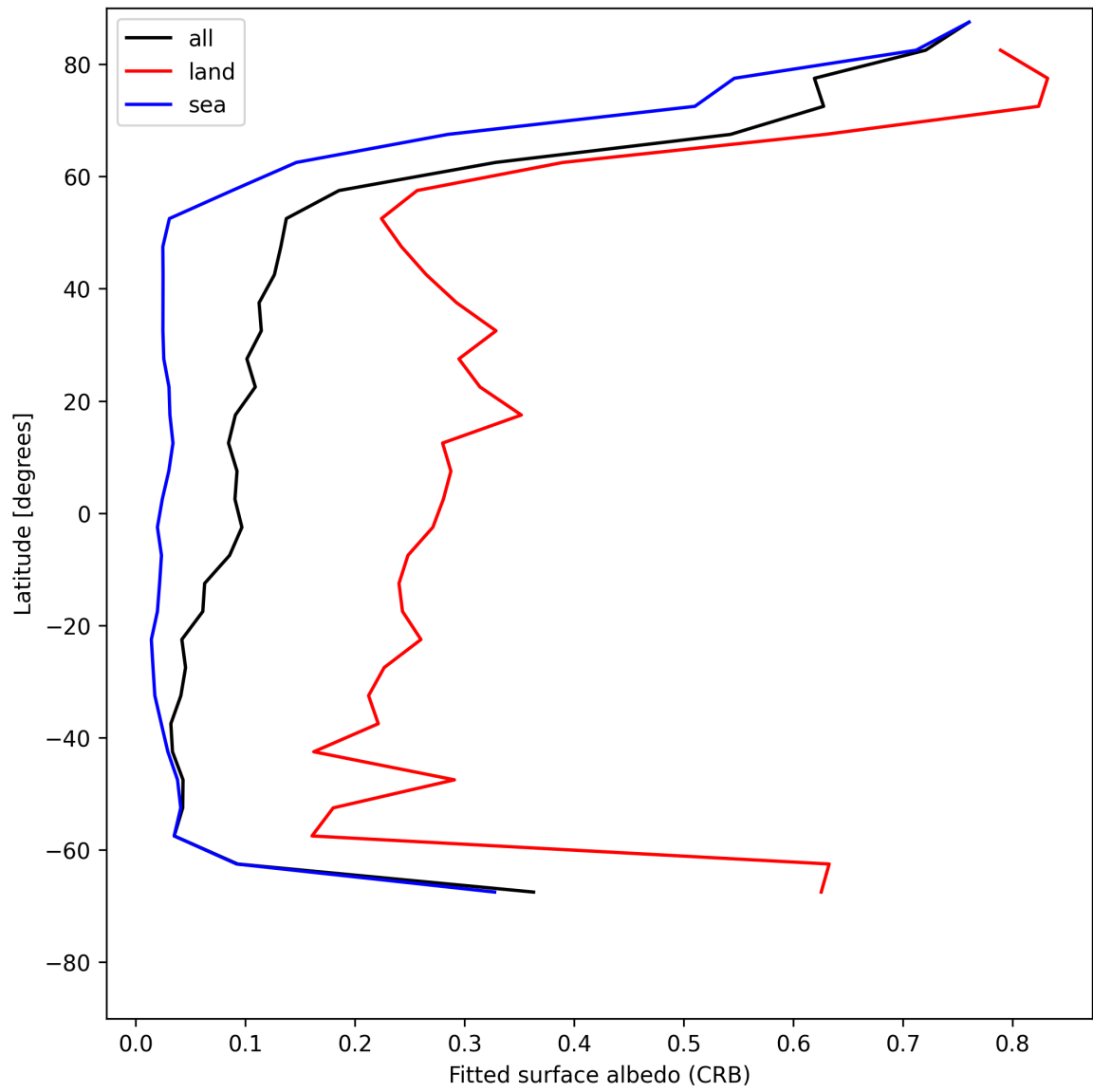
Figure 28: Zonal average of “Fitted surface albedo (CRB)” for 2025-05-21 to 2025-05-22.
