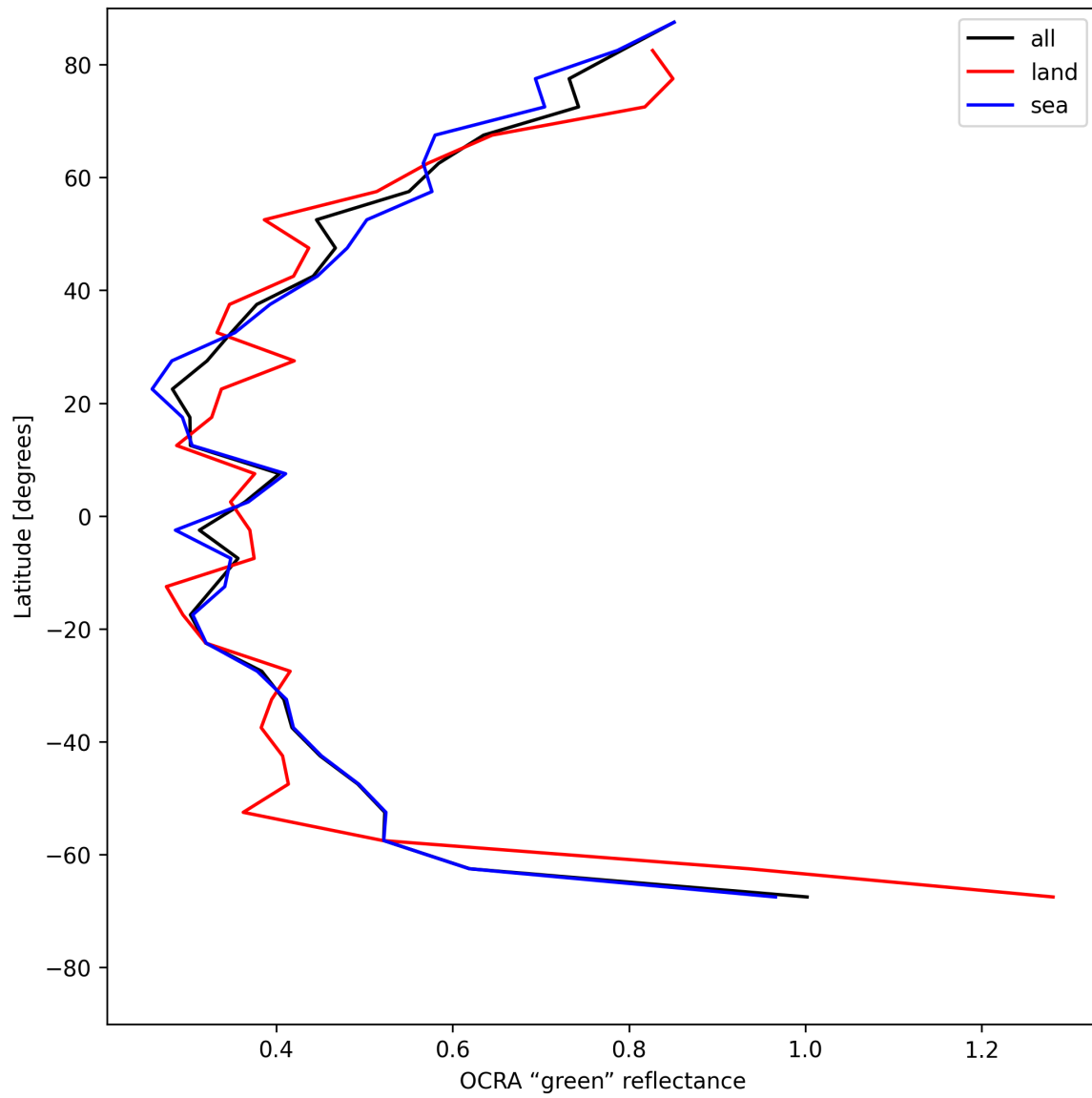
Figure 34: Zonal average of "OCRA "green" reflectance" for 2025-05-21 to 2025-05-22.
