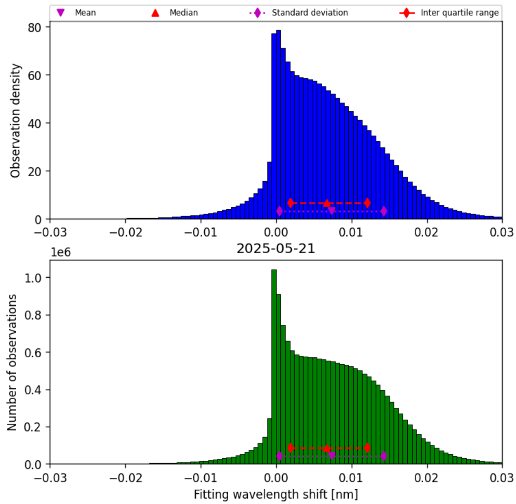
Figure 47: Histogram of “Fitting wavelength shift” for 2025-05-21 to 2025-05-22
