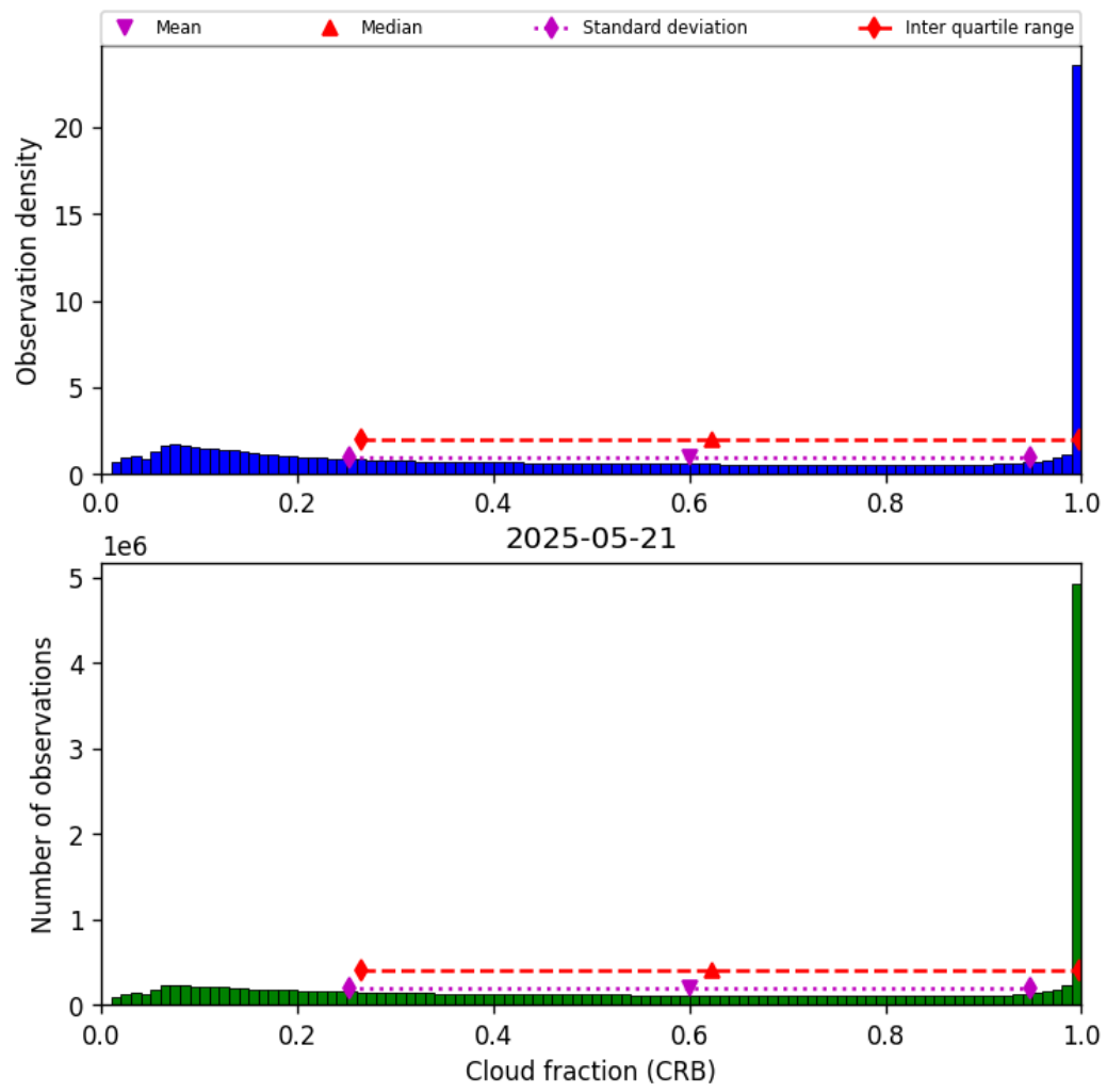
Figure 40: Histogram of “Cloud fraction (CRB)” for 2025-05-21 to 2025-05-22
