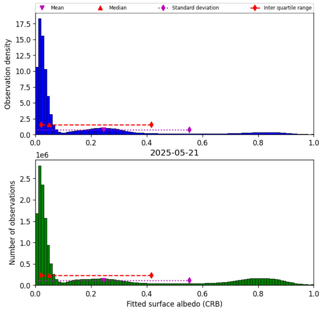
Figure 44: Histogram of “Fitted surface albedo (CRB)” for 2025-05-21 to 2025-05-22
