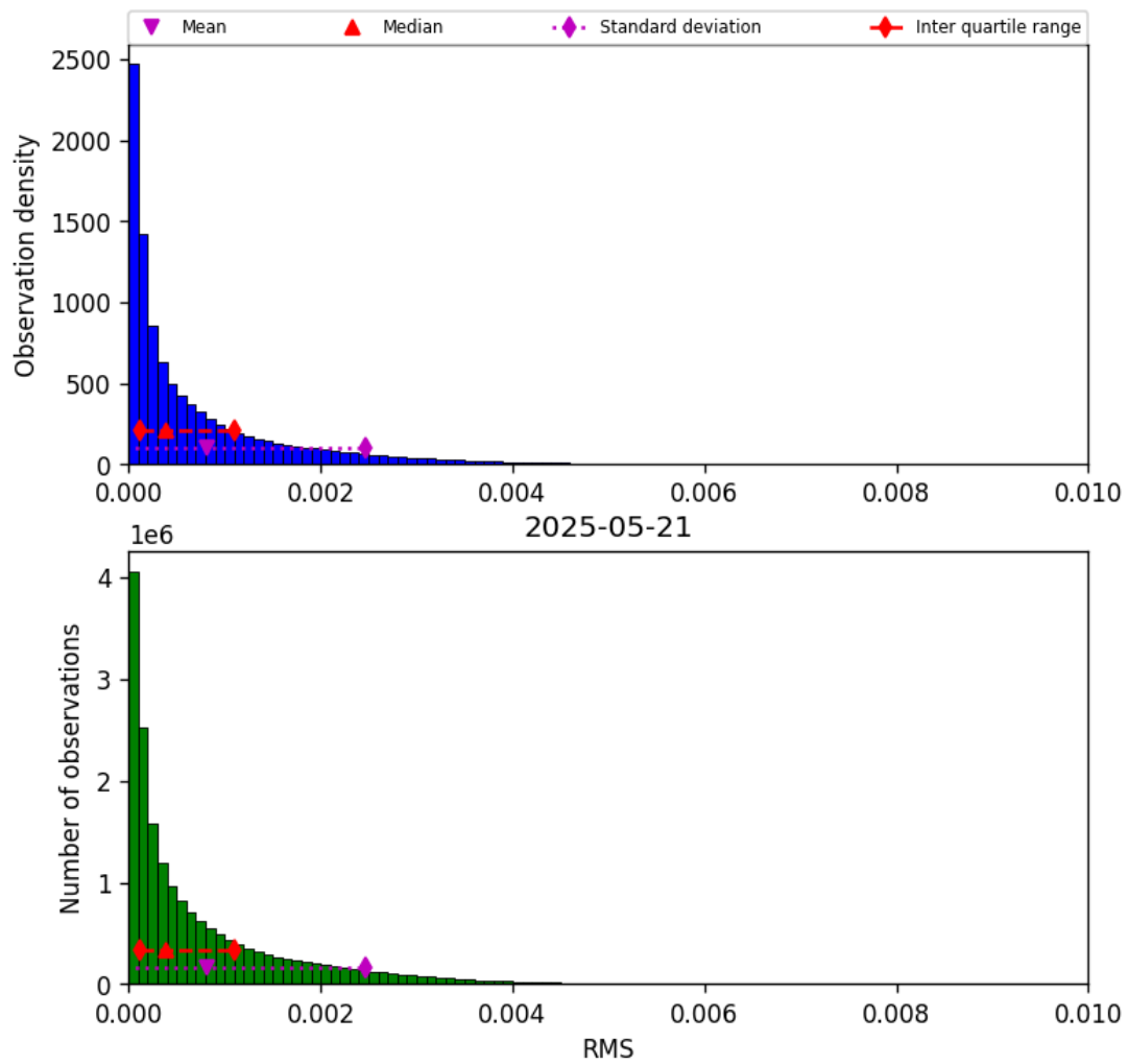
Figure 45: Histogram of “RMS” for 2025-05-21 to 2025-05-22
