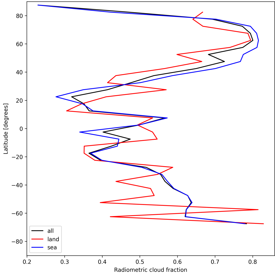
Figure 21: Zonal average of “Radiometric cloud fraction” for 2025-05-21 to 2025-05-22.
