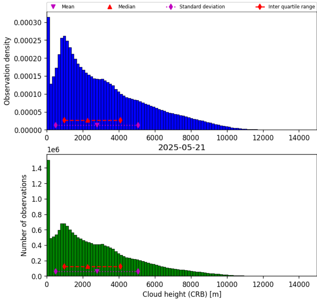
Figure 41: Histogram of “Cloud height (CRB)” for 2025-05-21 to 2025-05-22
