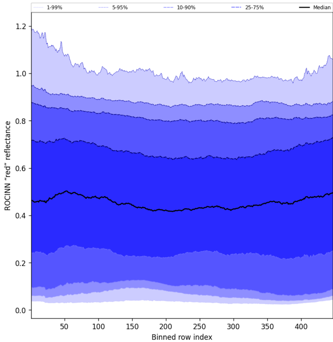
Figure 67: Along track statistics of "ROCINN "red" reflectance" for 2025-05-21 to 2025-05-22
