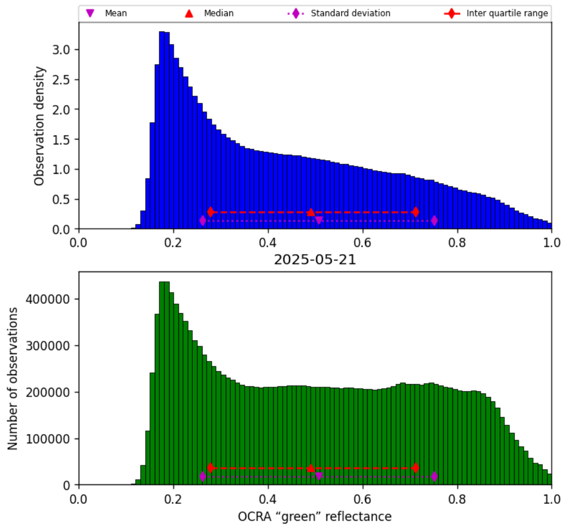
Figure 50: Histogram of “OCRA “green” reflectance” for 2025-05-21 to 2025-05-22
