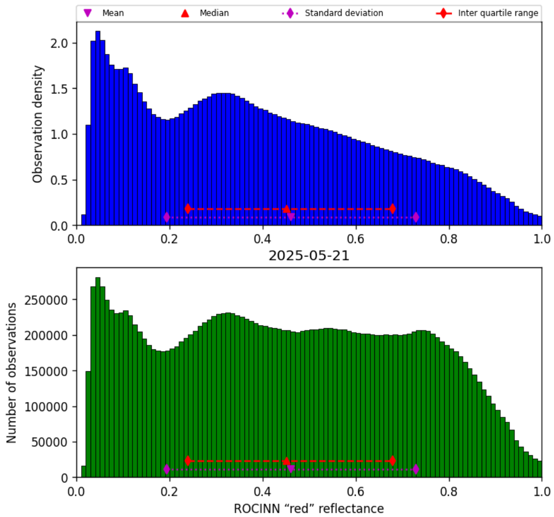
Figure 51: Histogram of "ROCINN "red" reflectance" for 2025-05-21 to 2025-05-22
