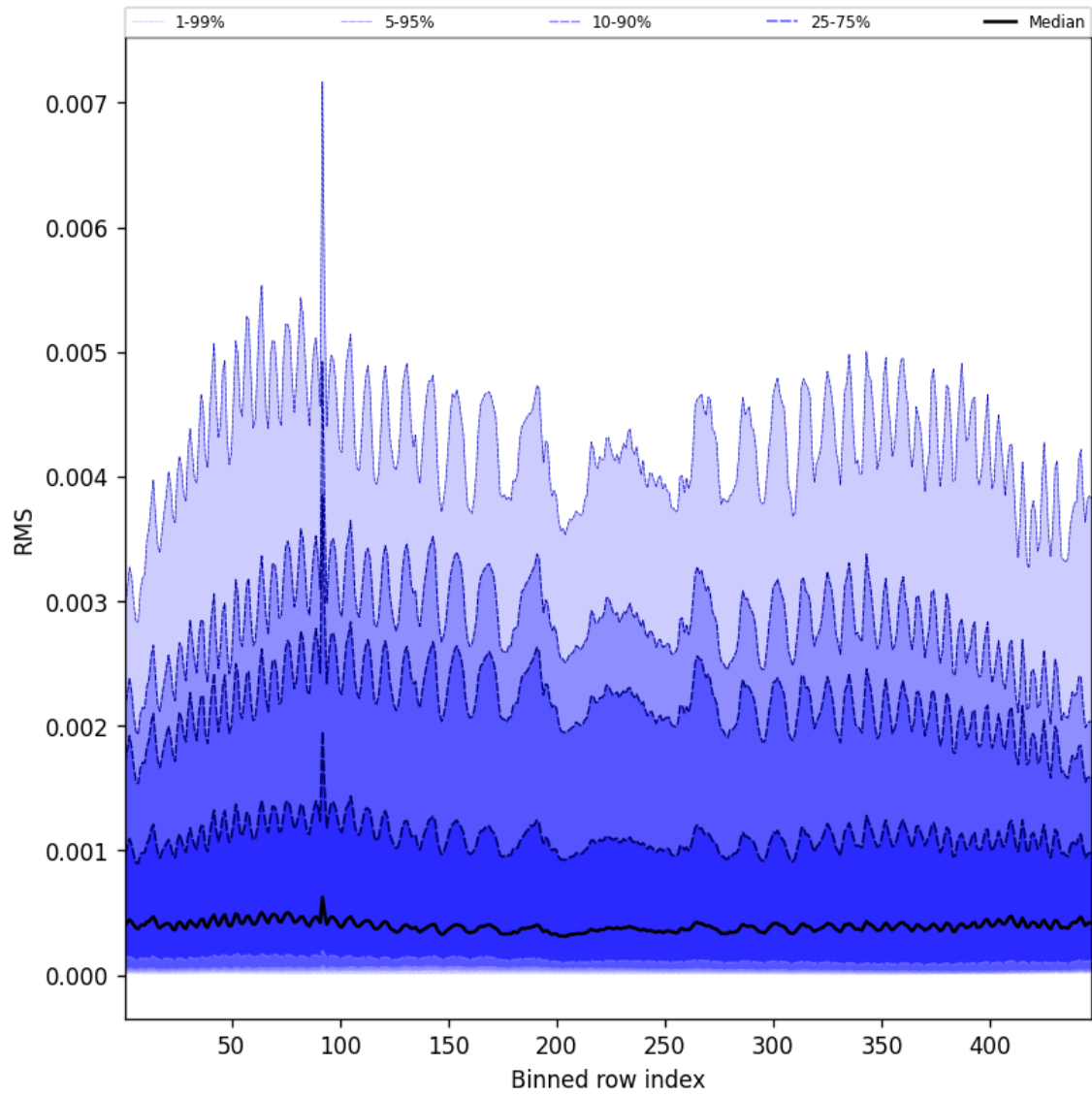
Figure 61: Along track statistics of “RMS” for 2025-05-21 to 2025-05-22
