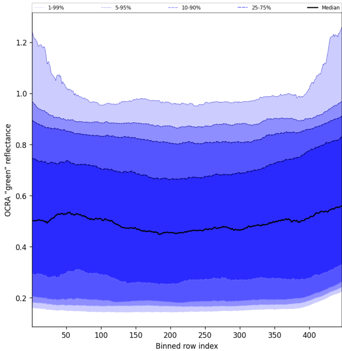
Figure 66: Along track statistics of “OCRA “green” reflectance” for 2025-05-21 to 2025-05-22
