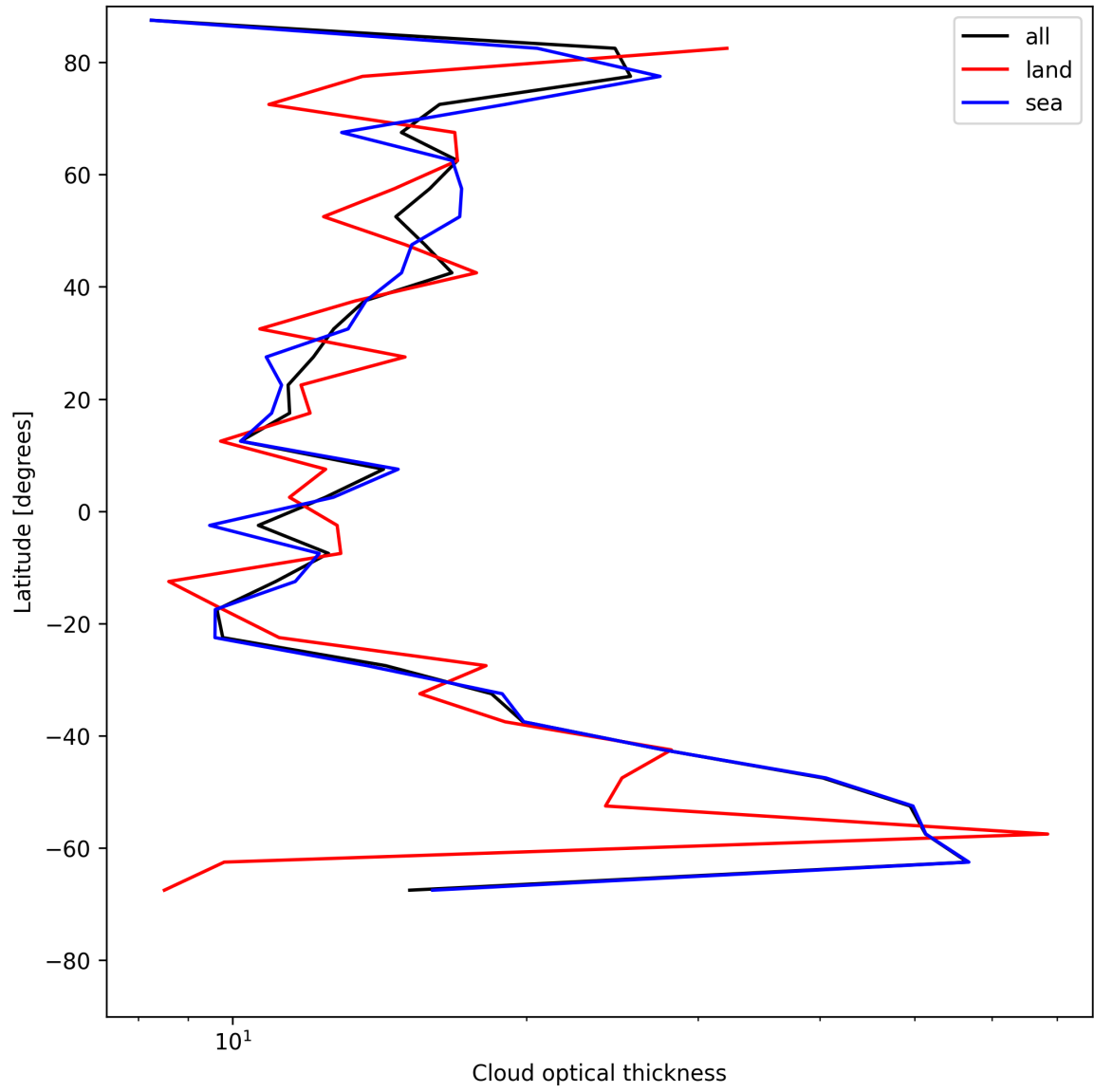
Figure 23: Zonal average of “Cloud optical thickness” for 2025-05-21 to 2025-05-22.
