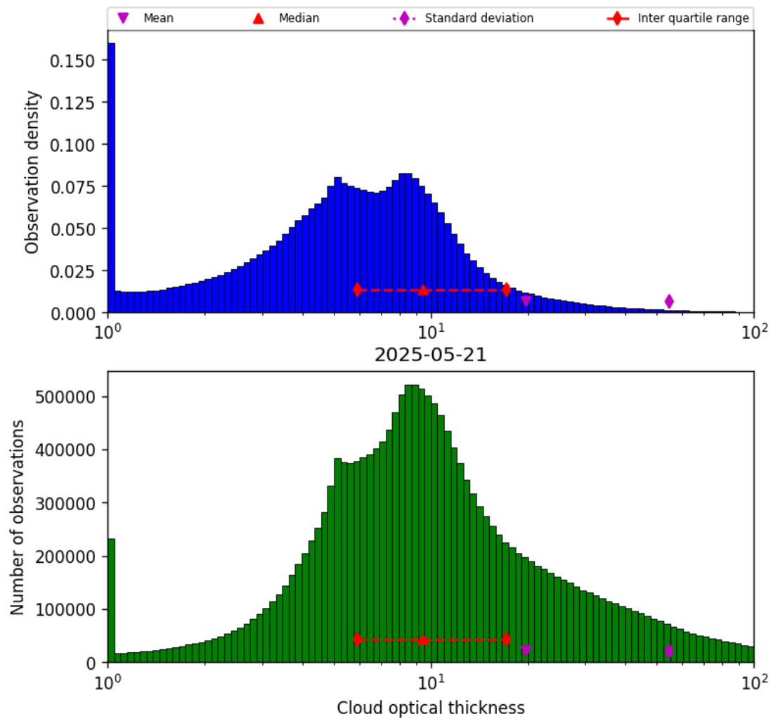
Figure 39: Histogram of “Cloud optical thickness” for 2025-05-21 to 2025-05-22
