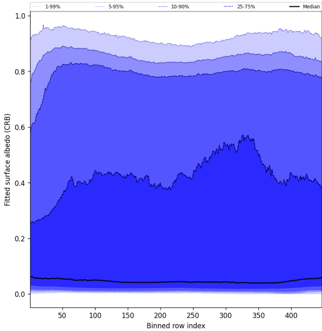
Figure 60: Along track statistics of “Fitted surface albedo (CRB)” for 2025-05-22 to 2025-05-23
