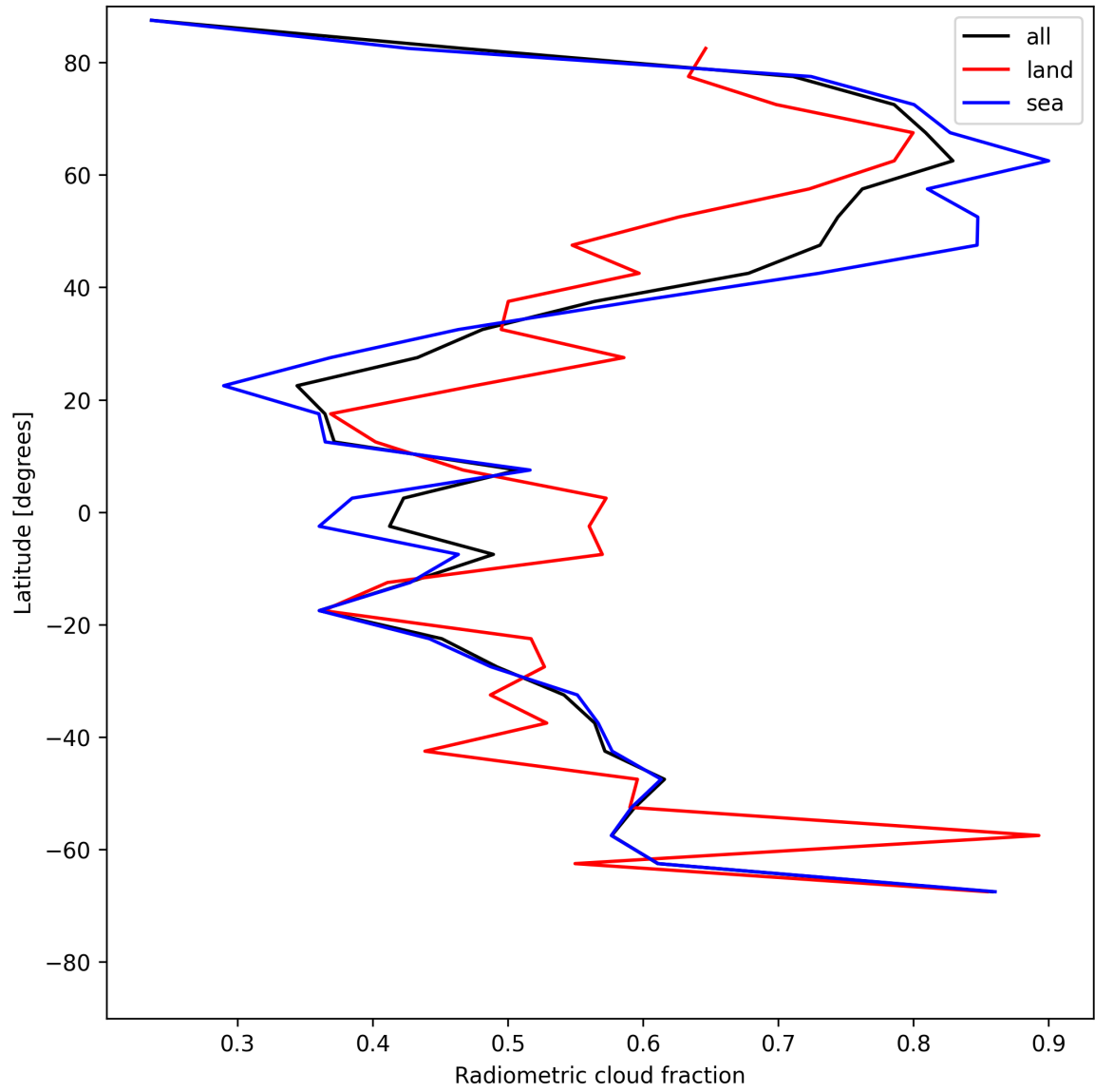
Figure 21: Zonal average of “Radiometric cloud fraction” for 2025-05-22 to 2025-05-23.
