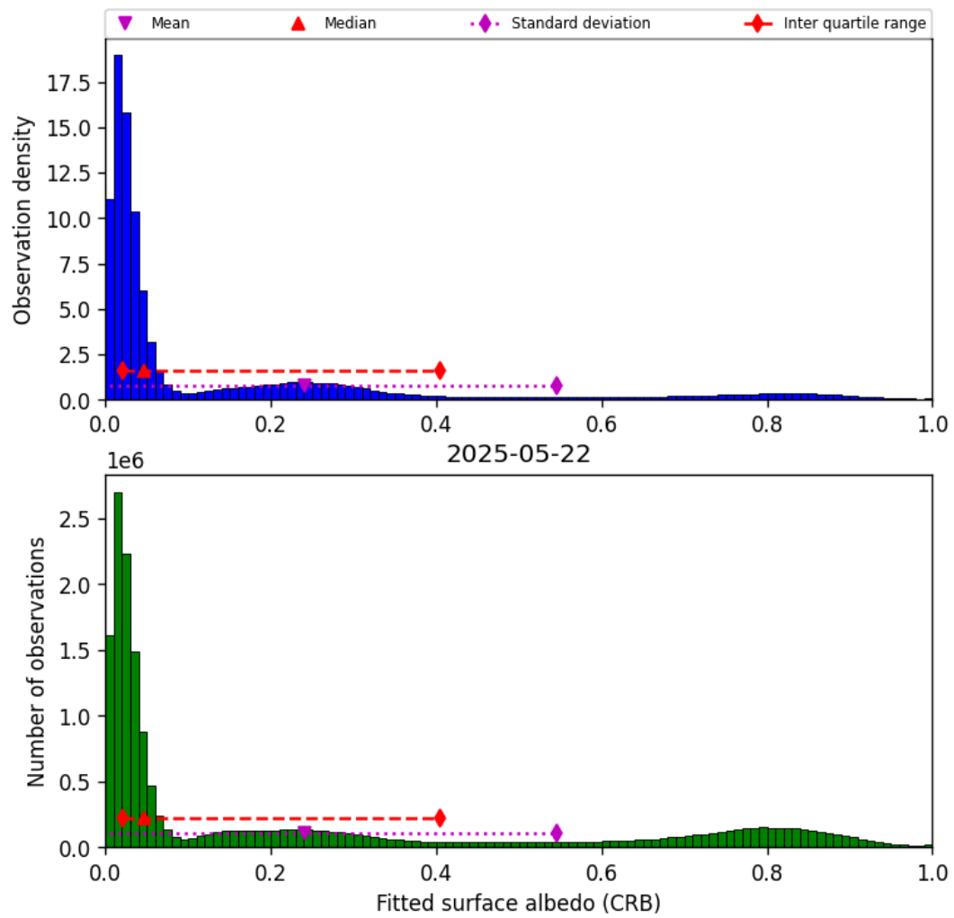
Figure 44: Histogram of “Fitted surface albedo (CRB)” for 2025-05-22 to 2025-05-23
