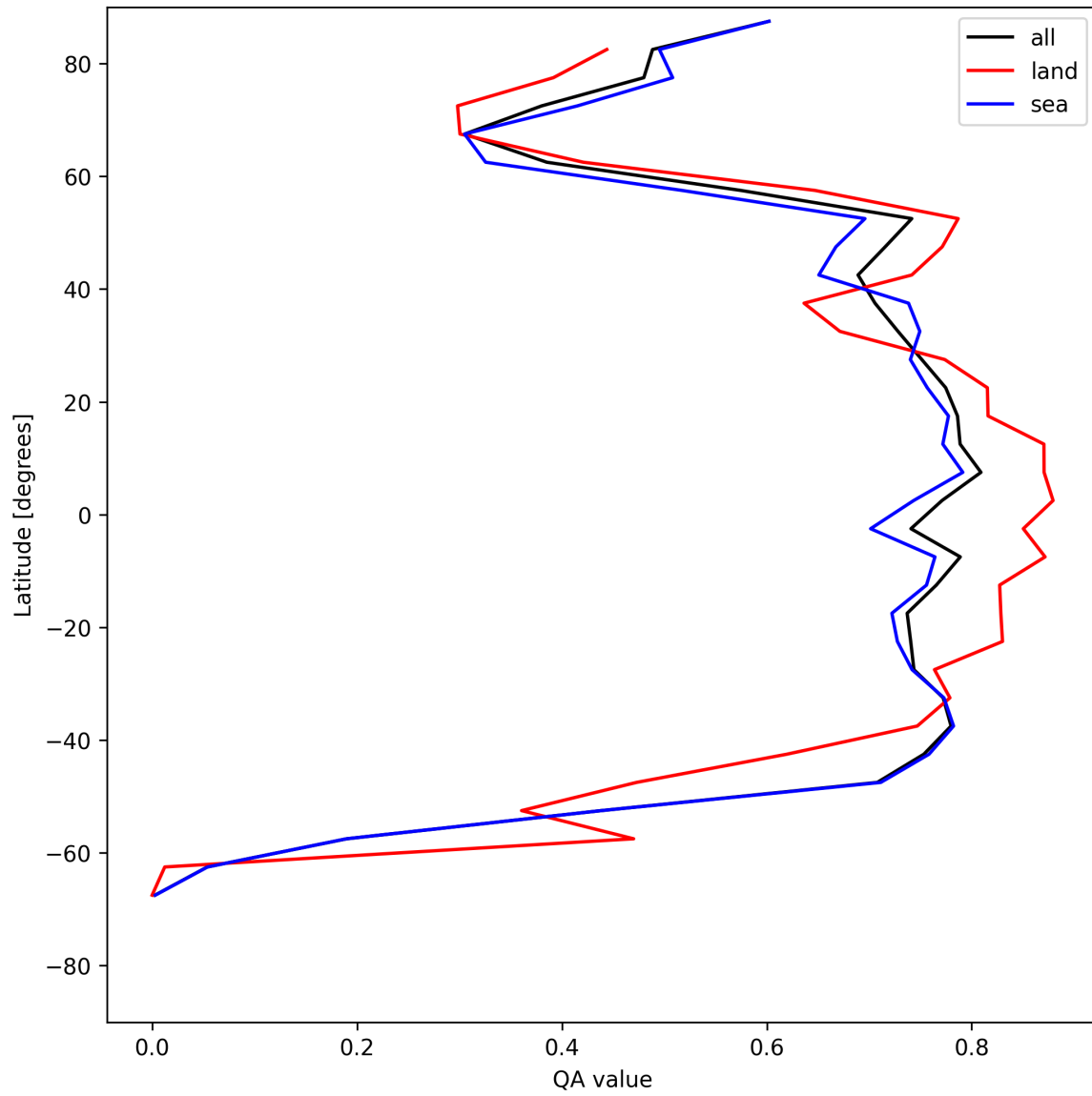
Figure 20: Zonal average of “QA value” for 2025-05-22 to 2025-05-23.
