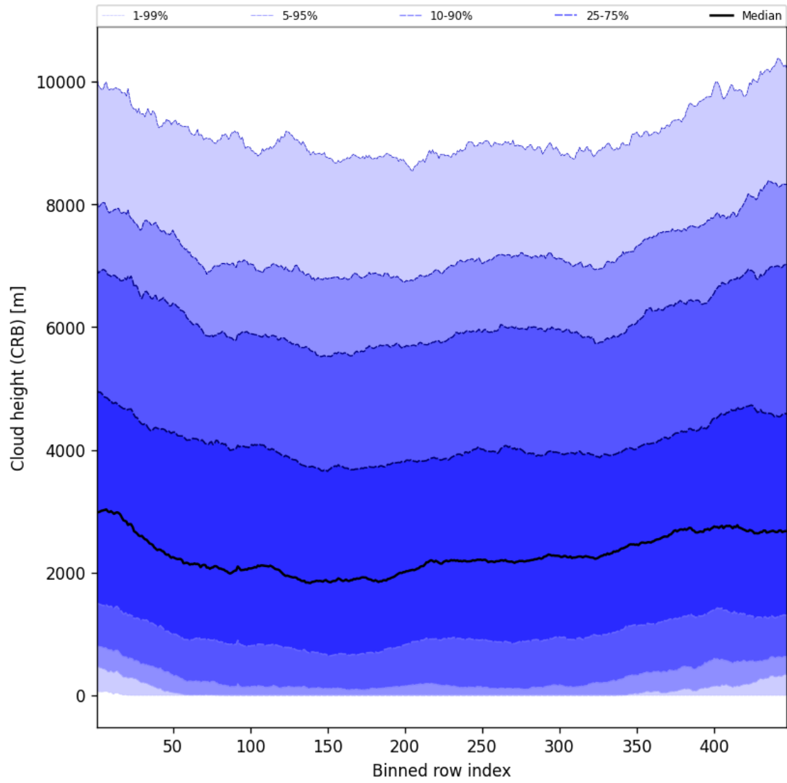
Figure 57: Along track statistics of “Cloud height (CRB)” for 2025-05-22 to 2025-05-23
