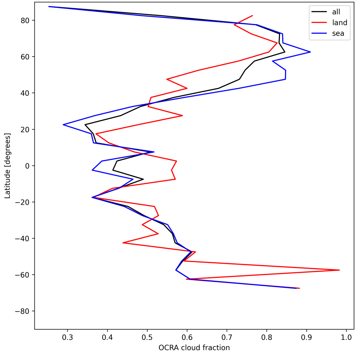
Figure 32: Zonal average of “OCRA cloud fraction” for 2025-05-22 to 2025-05-23.
