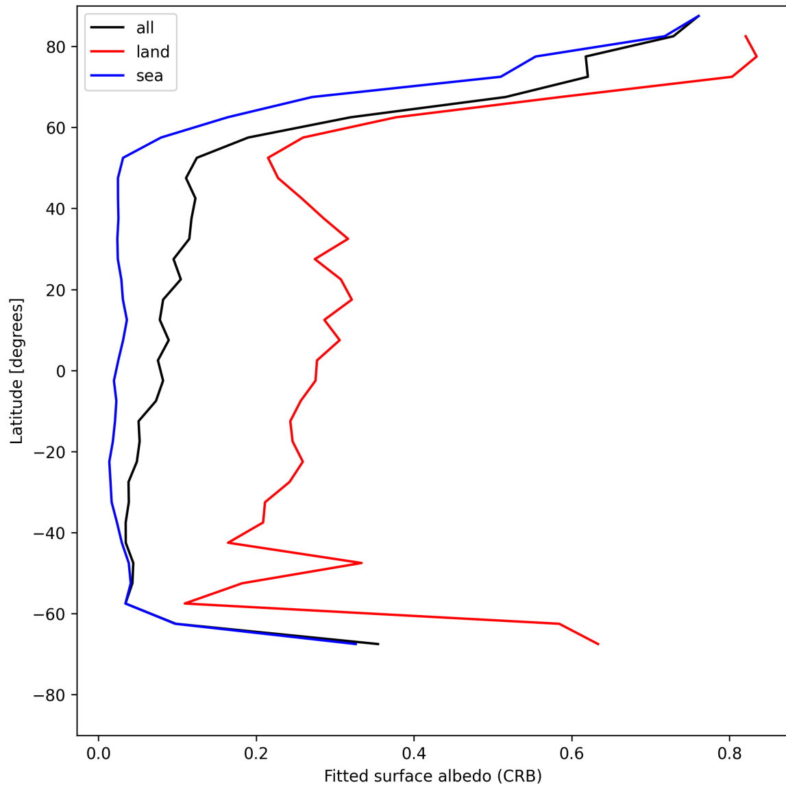
Figure 28: Zonal average of “Fitted surface albedo (CRB)” for 2025-05-22 to 2025-05-23.
