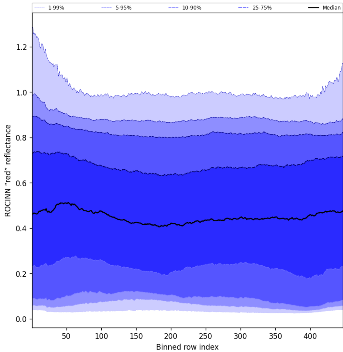
Figure 67: Along track statistics of "ROCINN "red" reflectance" for 2025-05-22 to 2025-05-23
