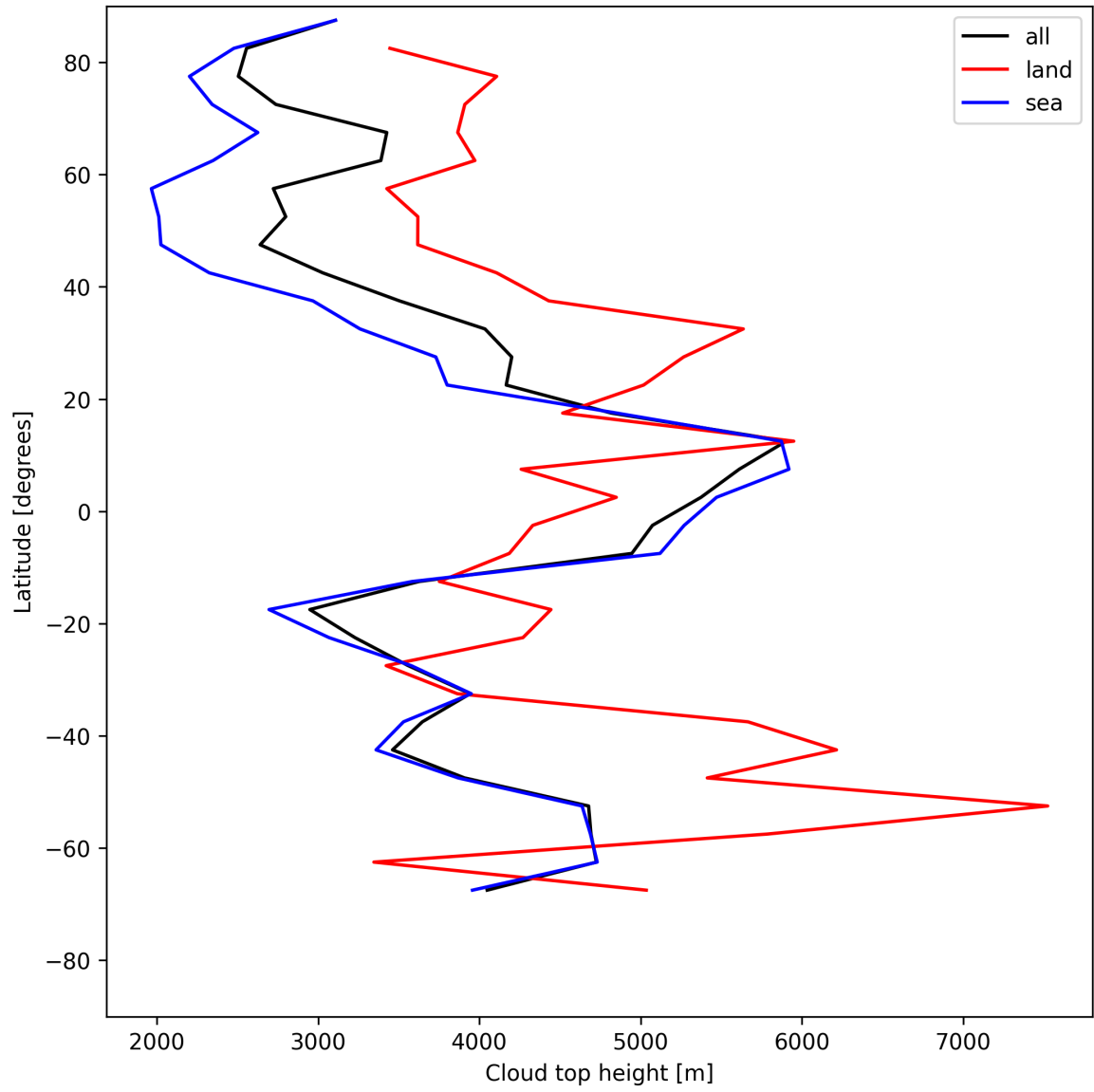
Figure 22: Zonal average of “Cloud top height” for 2025-05-22 to 2025-05-23.
