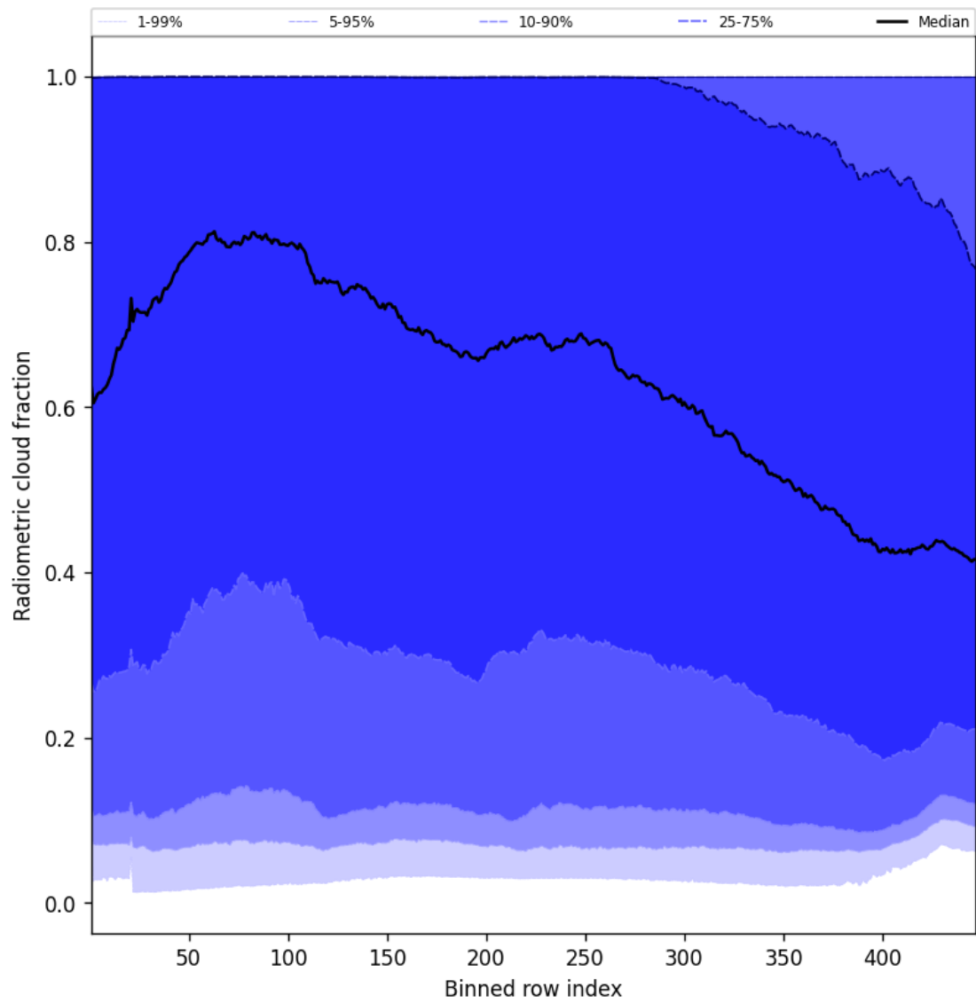
Figure 53: Along track statistics of “Radiometric cloud fraction” for 2025-05-22 to 2025-05-23
