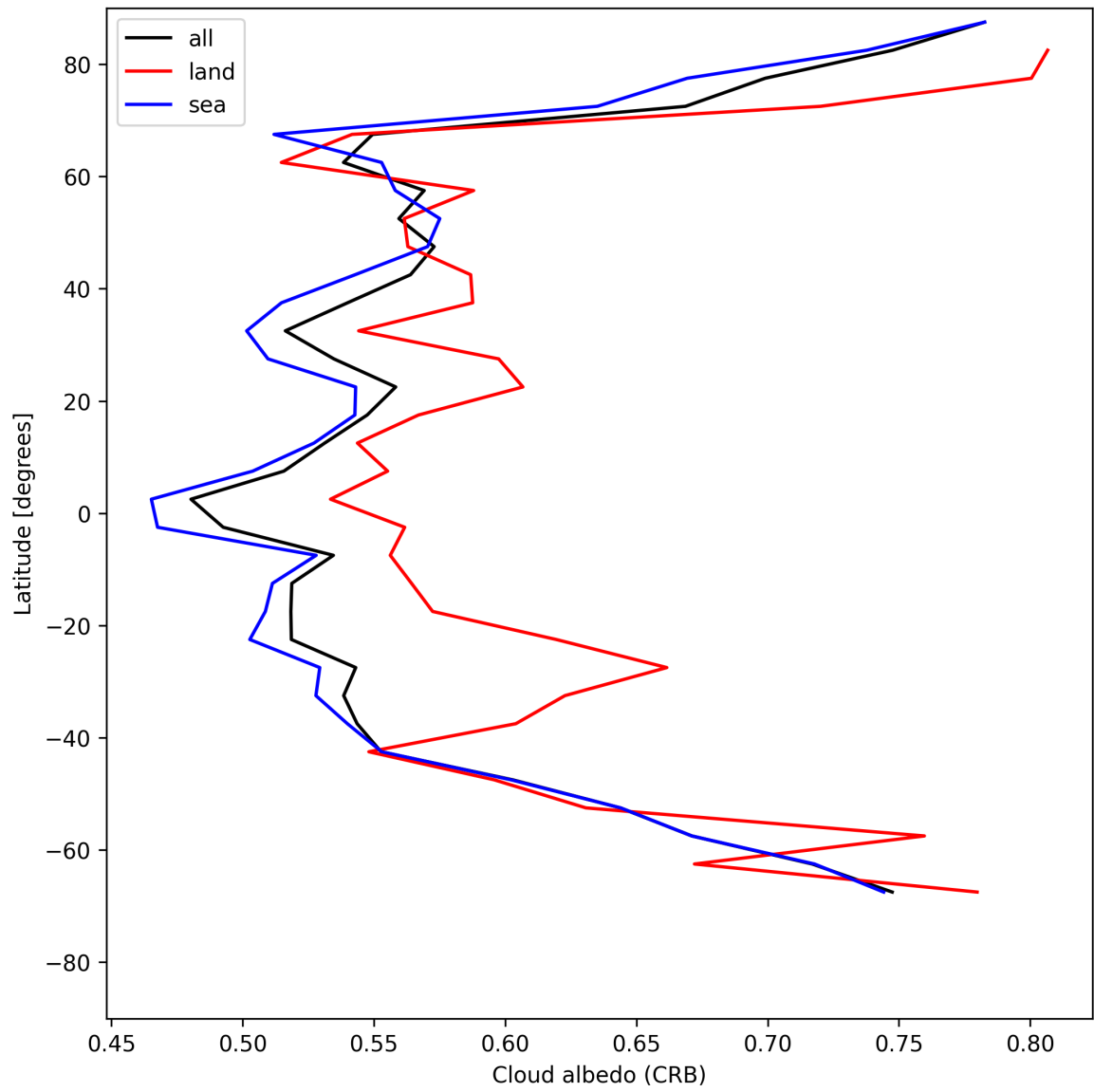
Figure 26: Zonal average of “Cloud albedo (CRB)” for 2025-05-22 to 2025-05-23.
