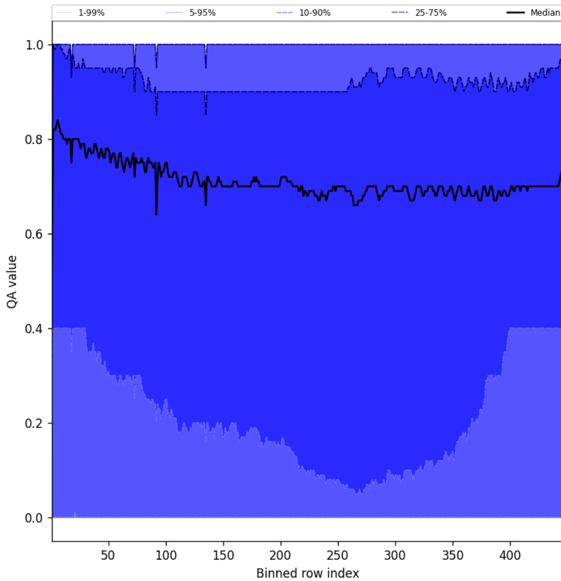
Figure 52: Along track statistics of "QA value" for 2025-05-22 to 2025-05-23
