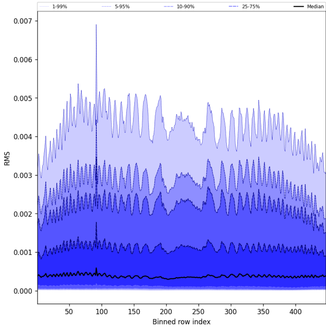
Figure 61: Along track statistics of “RMS” for 2025-05-22 to 2025-05-23
