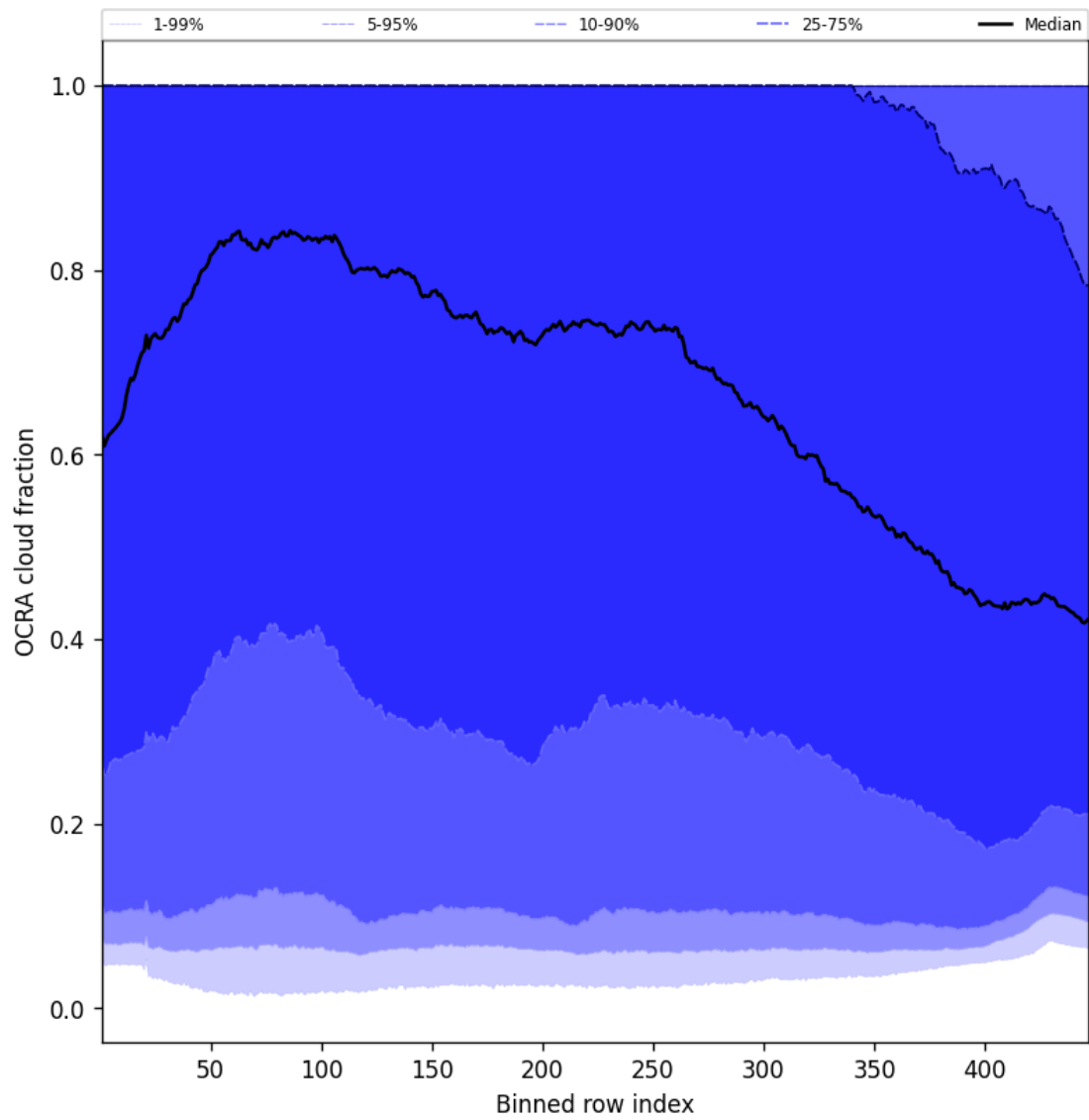
Figure 64: Along track statistics of “OCRA cloud fraction” for 2025-05-22 to 2025-05-23
