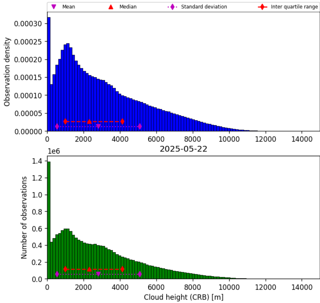
Figure 41: Histogram of “Cloud height (CRB)” for 2025-05-22 to 2025-05-23
