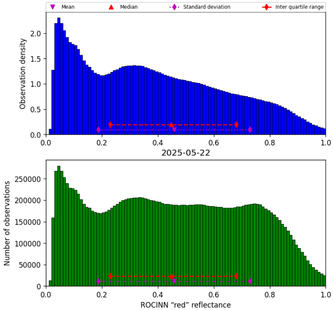
Figure 51: Histogram of “ROCINN “red” reflectance” for 2025-05-22 to 2025-05-23
