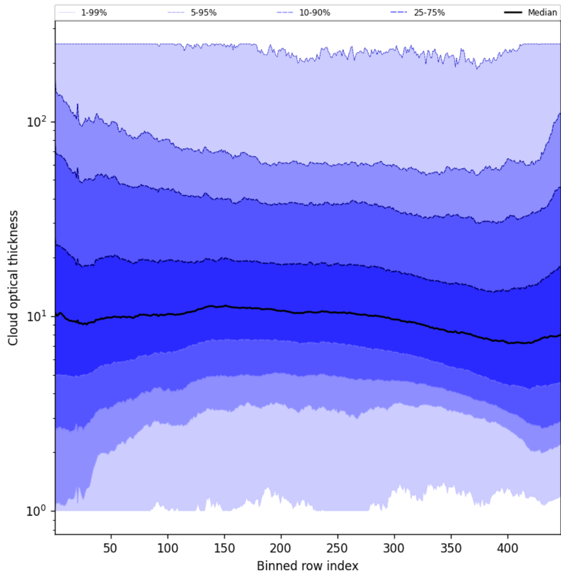
Figure 55: Along track statistics of “Cloud optical thickness” for 2025-05-22 to 2025-05-23
