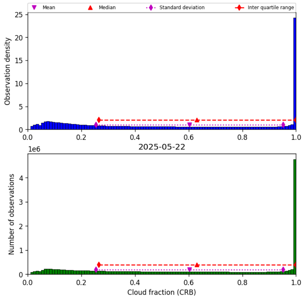
Figure 40: Histogram of “Cloud fraction (CRB)” for 2025-05-22 to 2025-05-23
