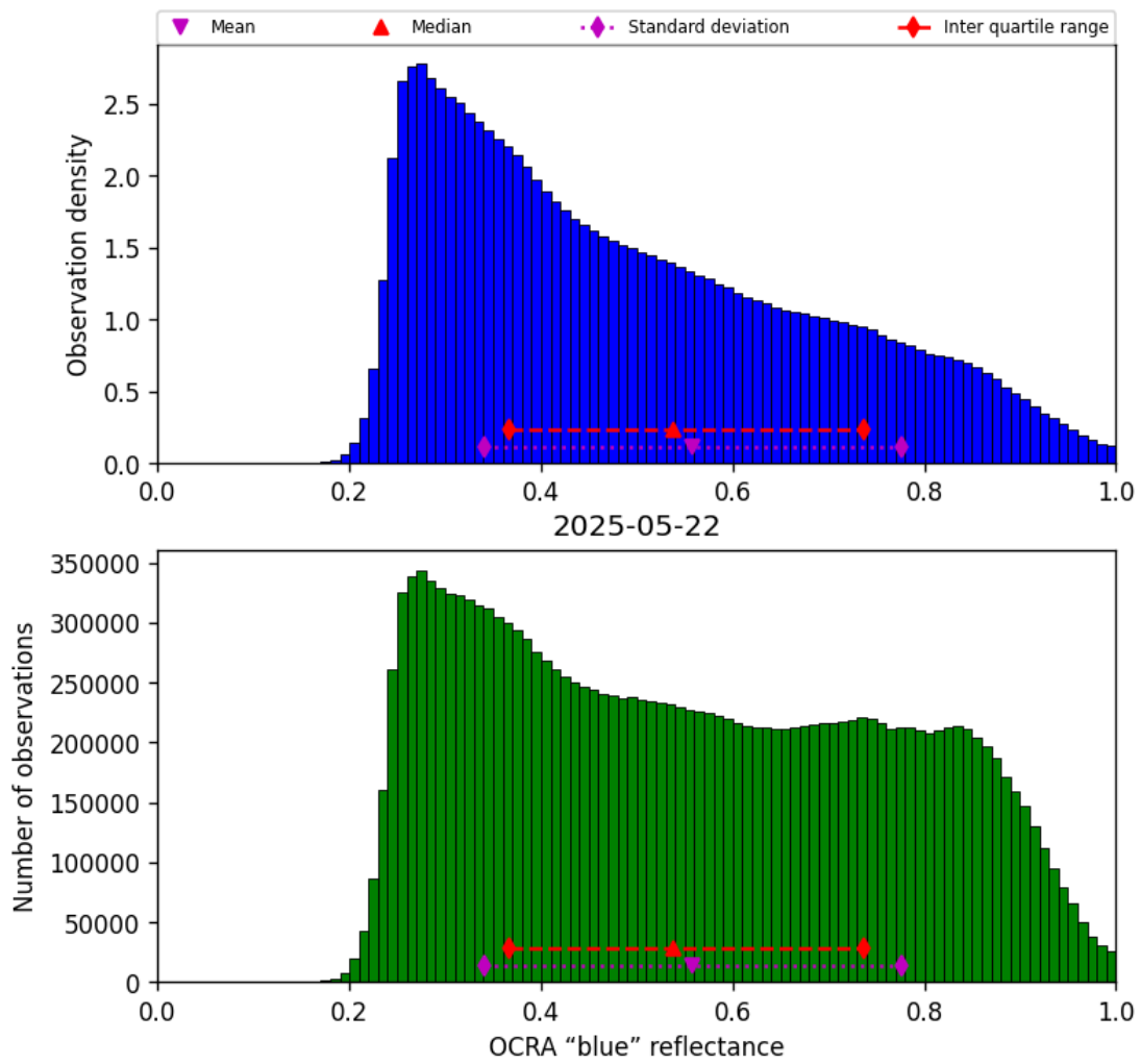
Figure 49: Histogram of “OCRA “blue” reflectance” for 2025-05-22 to 2025-05-23
