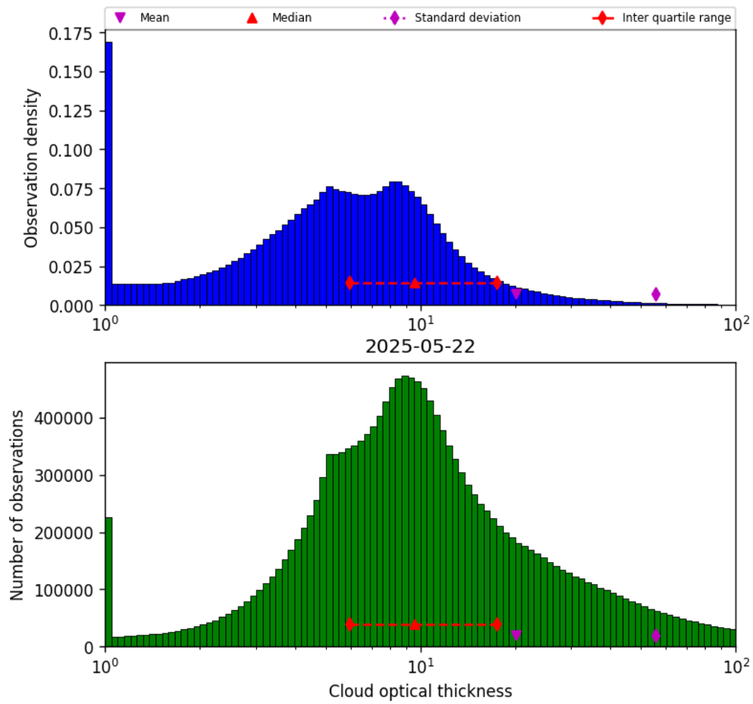
Figure 39: Histogram of “Cloud optical thickness” for 2025-05-22 to 2025-05-23
