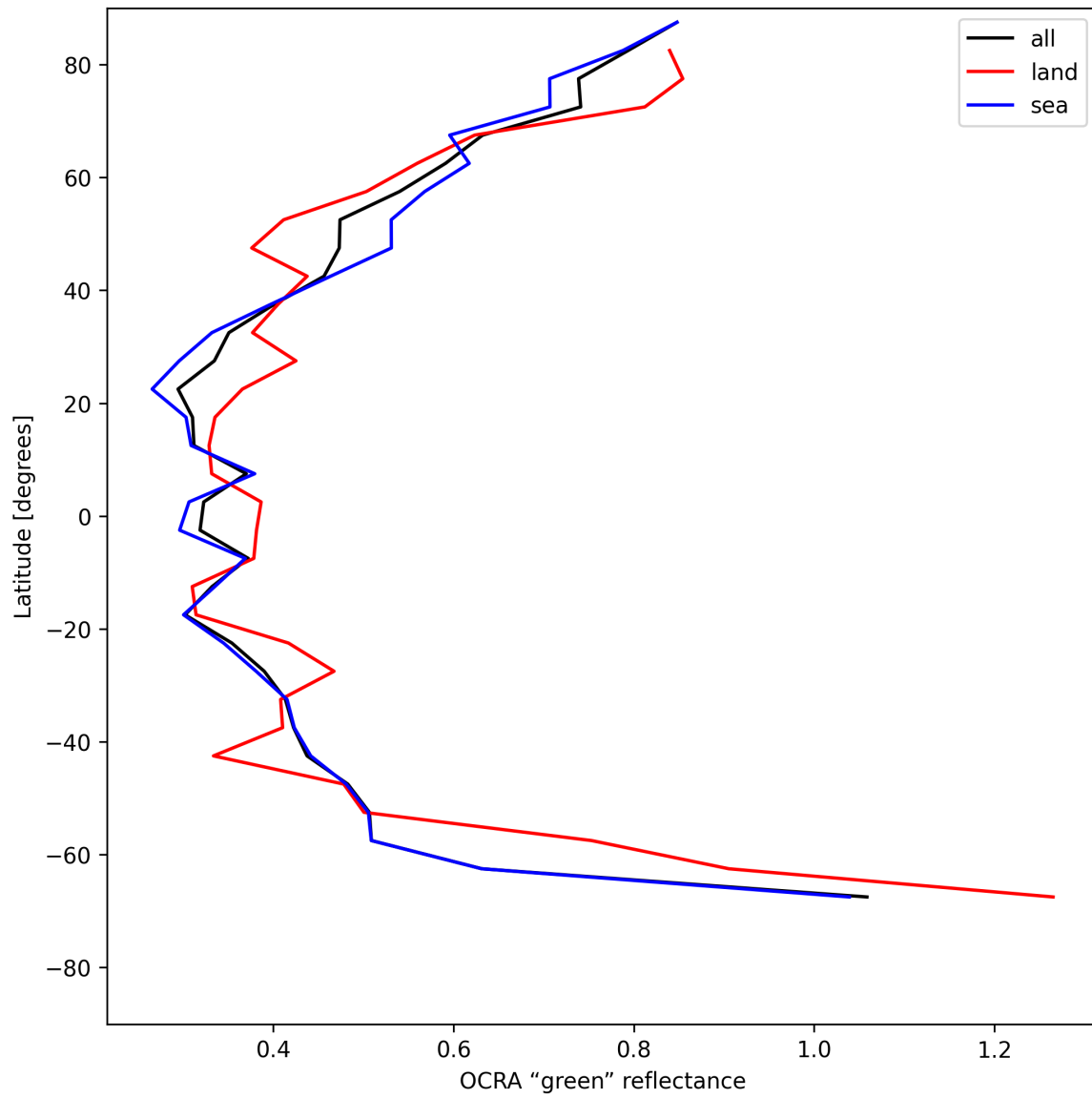
Figure 34: Zonal average of “OCRA “green” reflectance” for 2025-05-22 to 2025-05-23.
