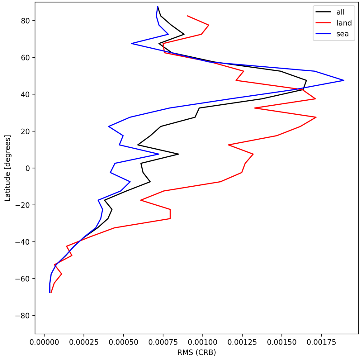
Figure 30: Zonal average of “RMS (CRB)” for 2025-05-22 to 2025-05-23.
