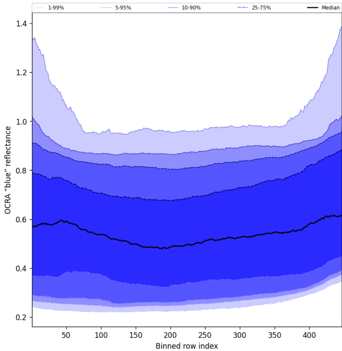
Figure 65: Along track statistics of “OCRA “blue” reflectance” for 2025-05-22 to 2025-05-23
