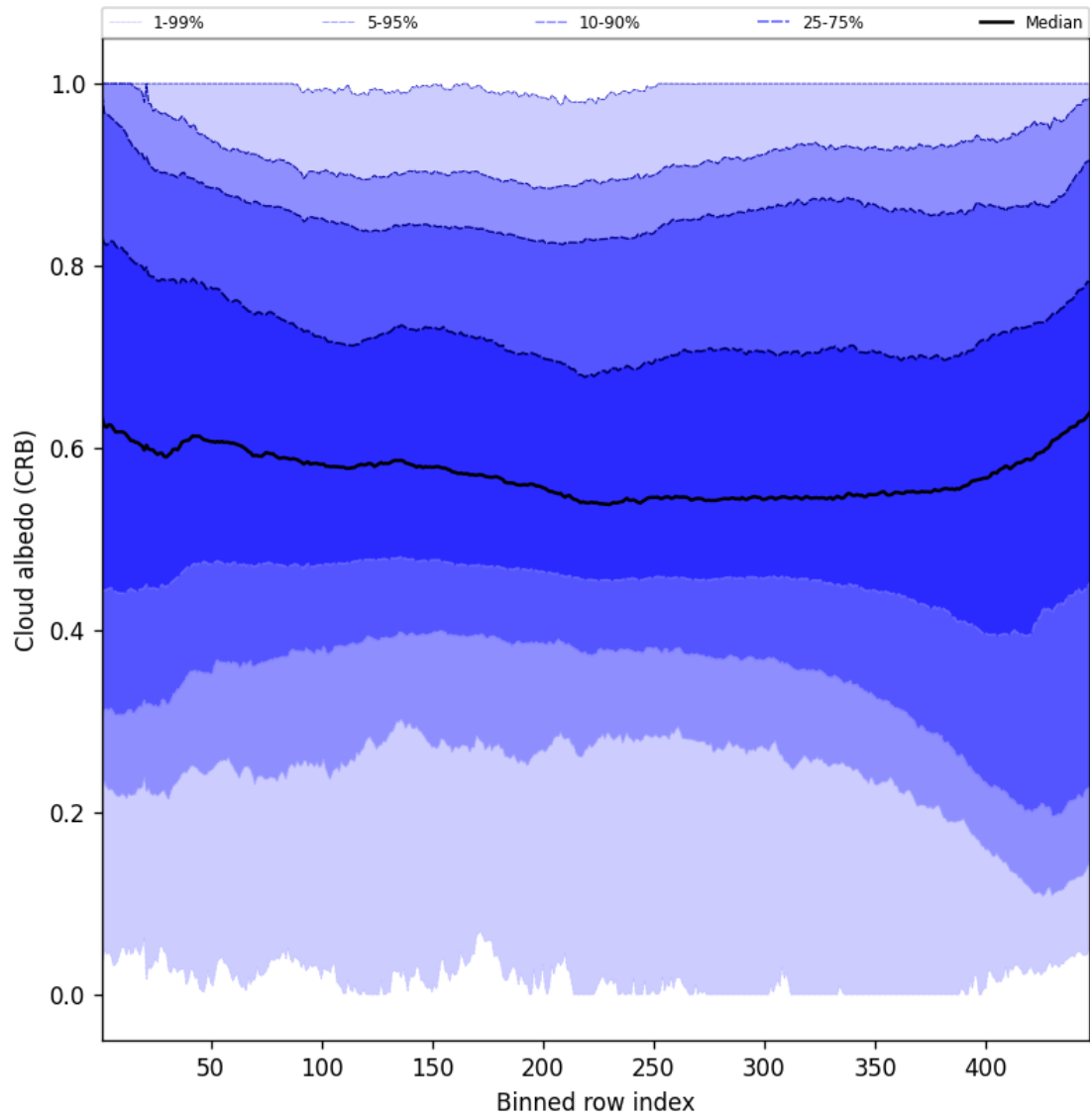
Figure 58: Along track statistics of “Cloud albedo (CRB)” for 2025-05-22 to 2025-05-23
