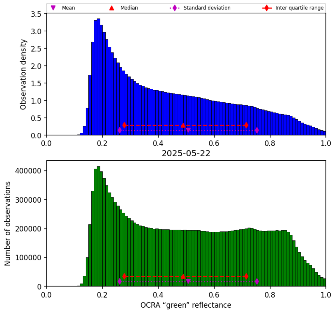
Figure 50: Histogram of “OCRA “green” reflectance” for 2025-05-22 to 2025-05-23
