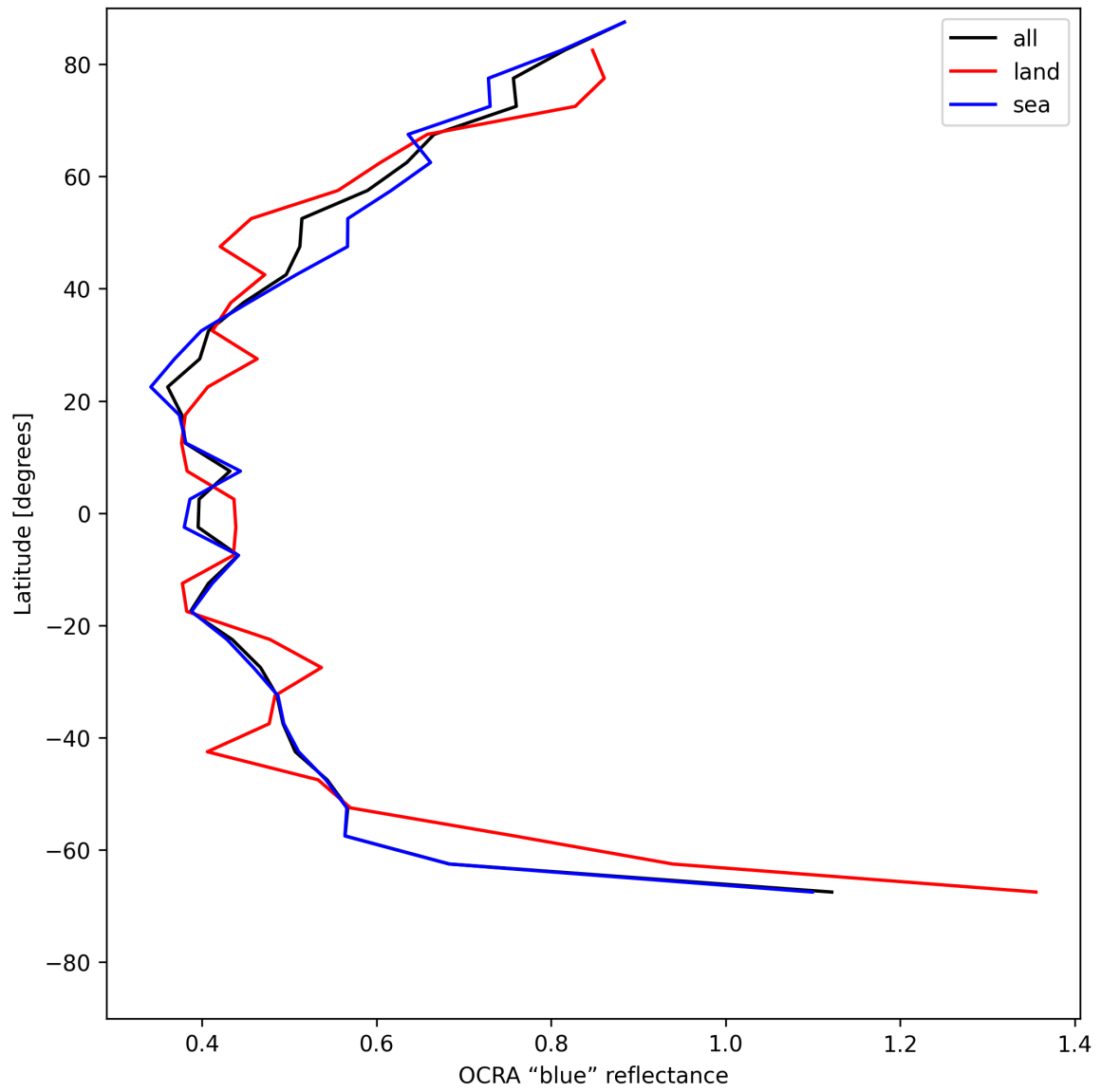
Figure 33: Zonal average of “OCRA “blue” reflectance” for 2025-05-22 to 2025-05-23.
