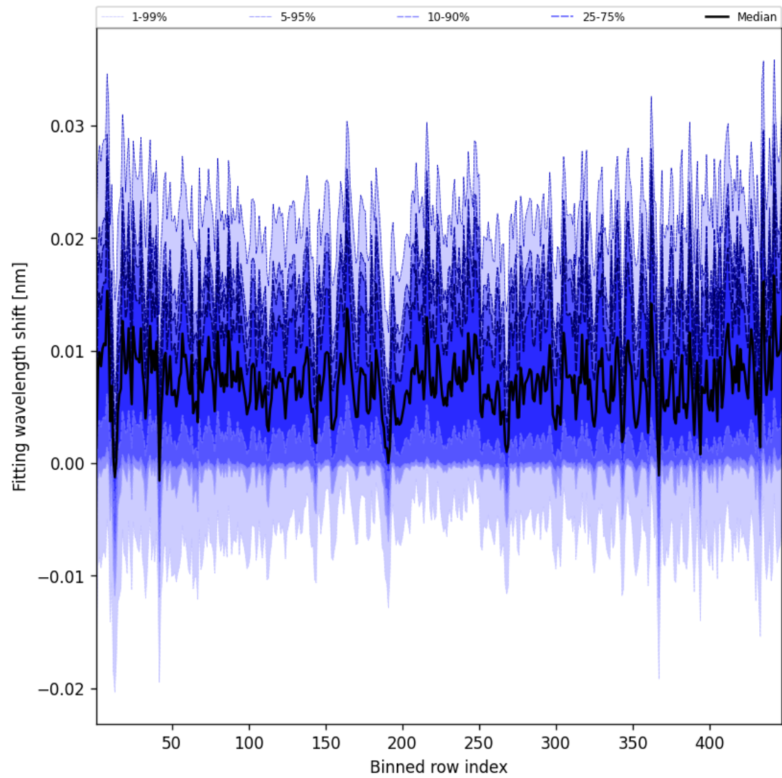
Figure 63: Along track statistics of “Fitting wavelength shift” for 2025-05-22 to 2025-05-23
