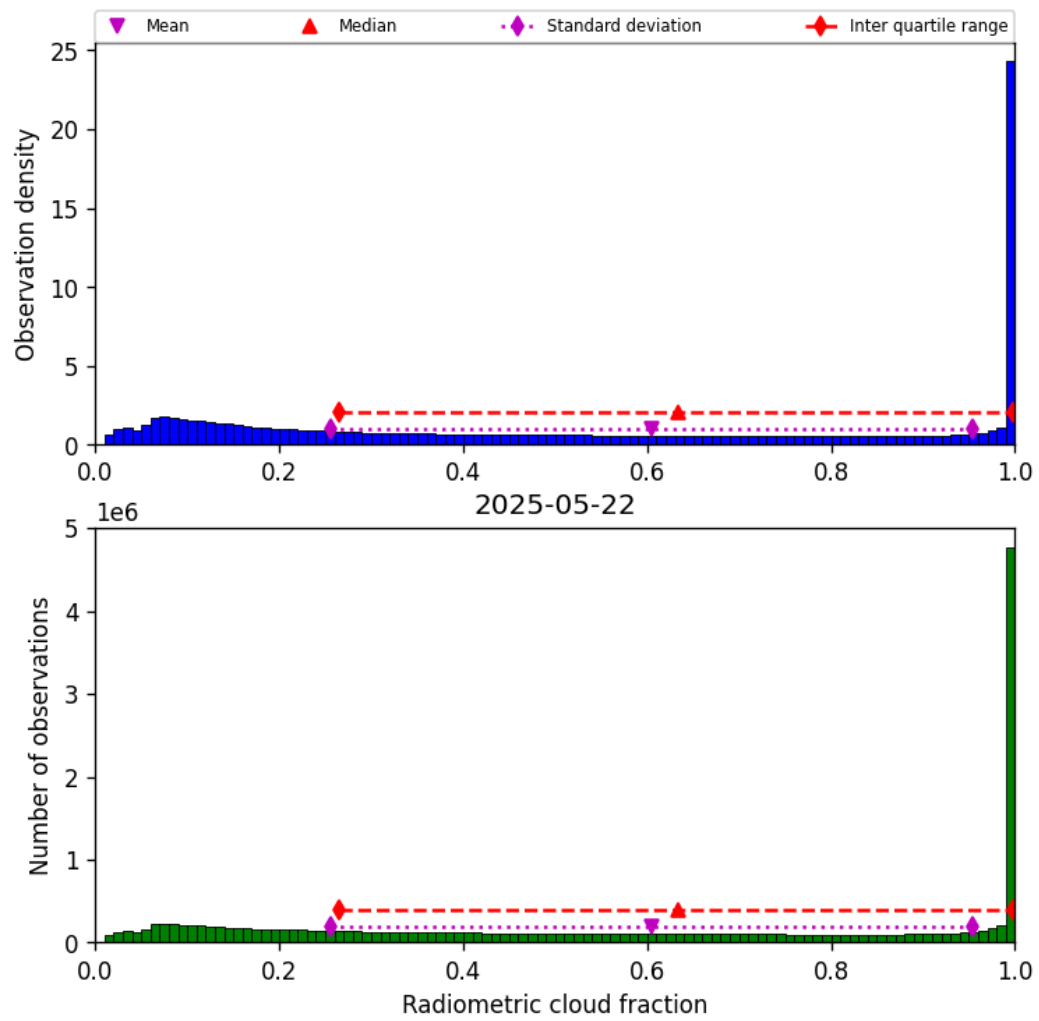
Figure 37: Histogram of “Radiometric cloud fraction” for 2025-05-22 to 2025-05-23
