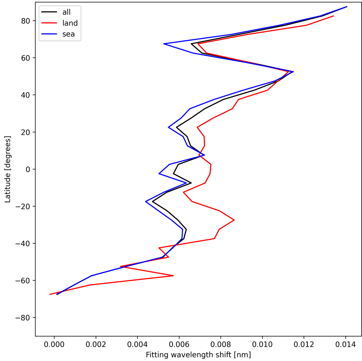
Figure 31: Zonal average of “Fitting wavelength shift” for 2025-05-22 to 2025-05-23.
