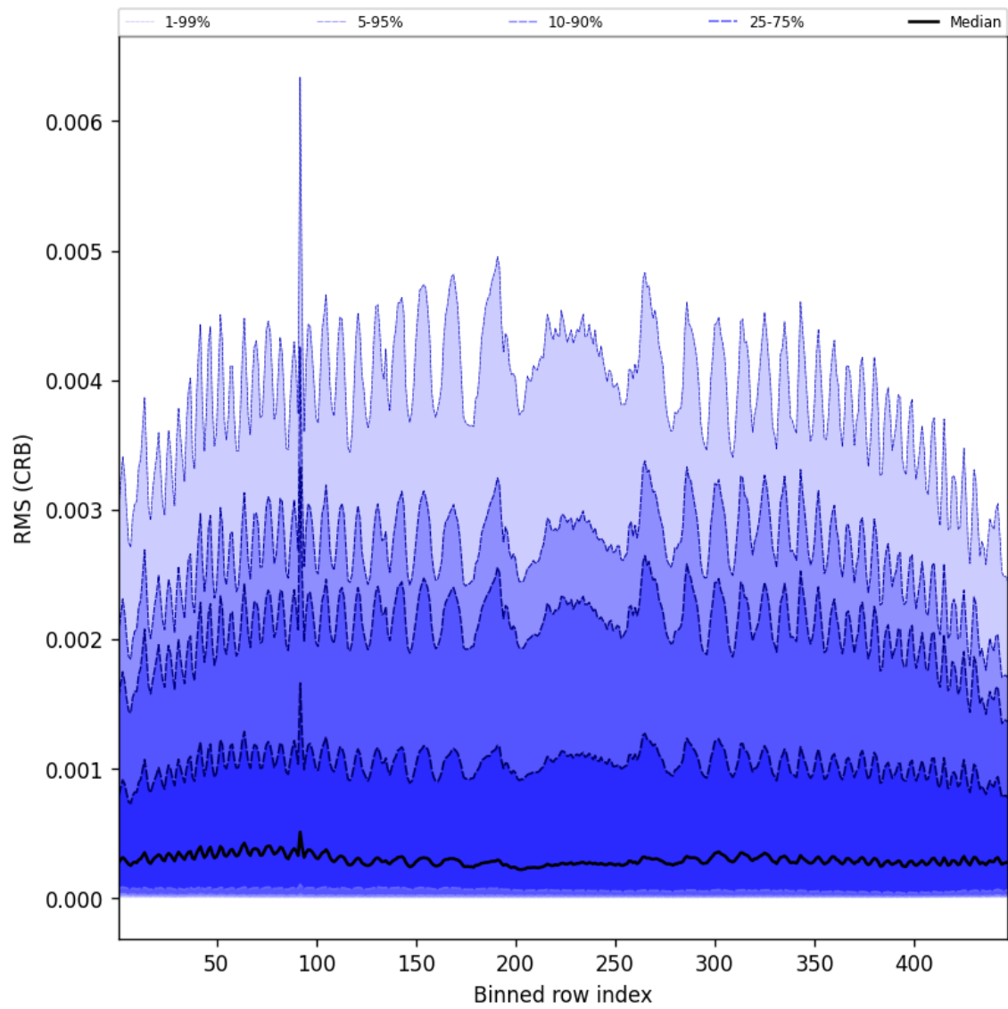
Figure 62: Along track statistics of “RMS (CRB)” for 2025-05-22 to 2025-05-23
