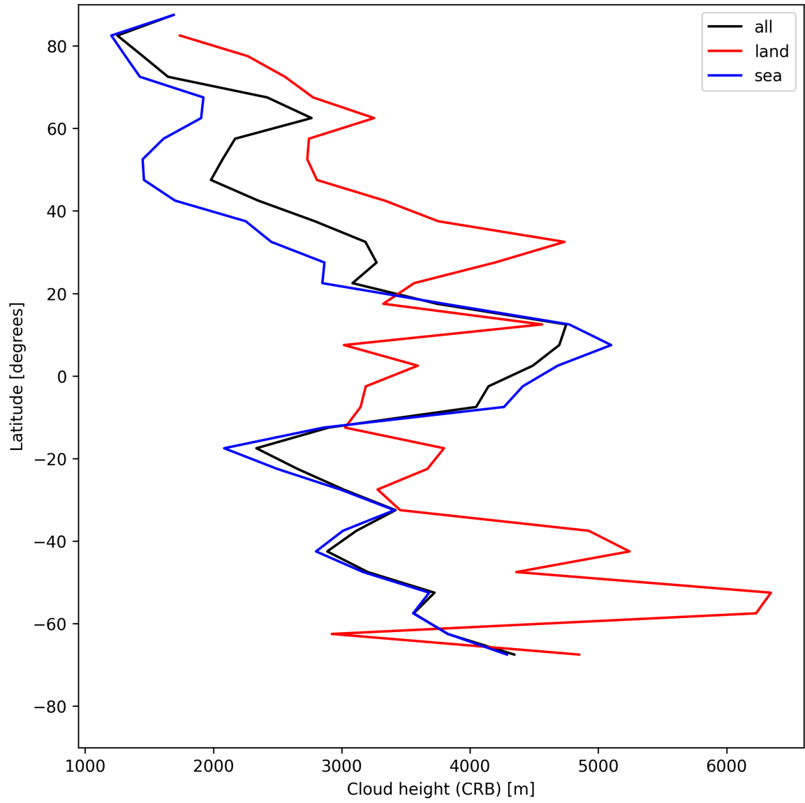
Figure 25: Zonal average of “Cloud height (CRB)” for 2025-05-22 to 2025-05-23.
