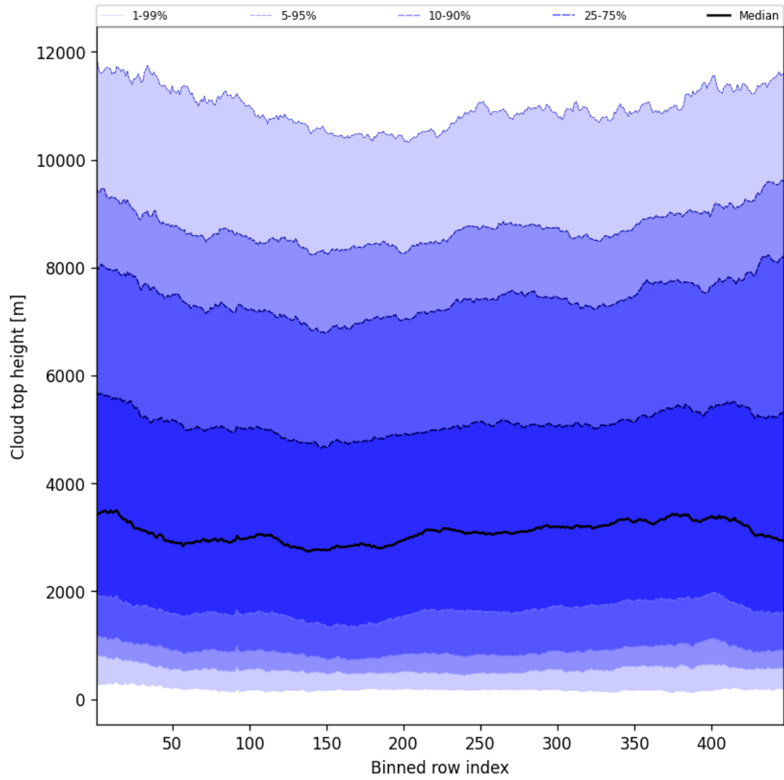
Figure 54: Along track statistics of “Cloud top height” for 2025-05-22 to 2025-05-23
