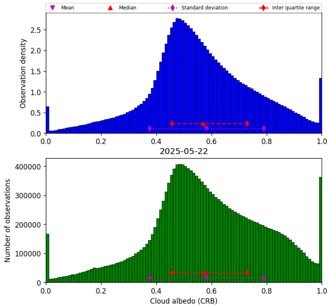
Figure 42: Histogram of “Cloud albedo (CRB)” for 2025-05-22 to 2025-05-23
