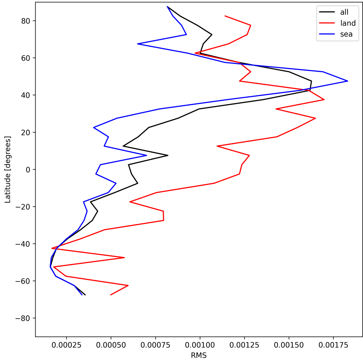
Figure 29: Zonal average of “RMS” for 2025-05-22 to 2025-05-23.
