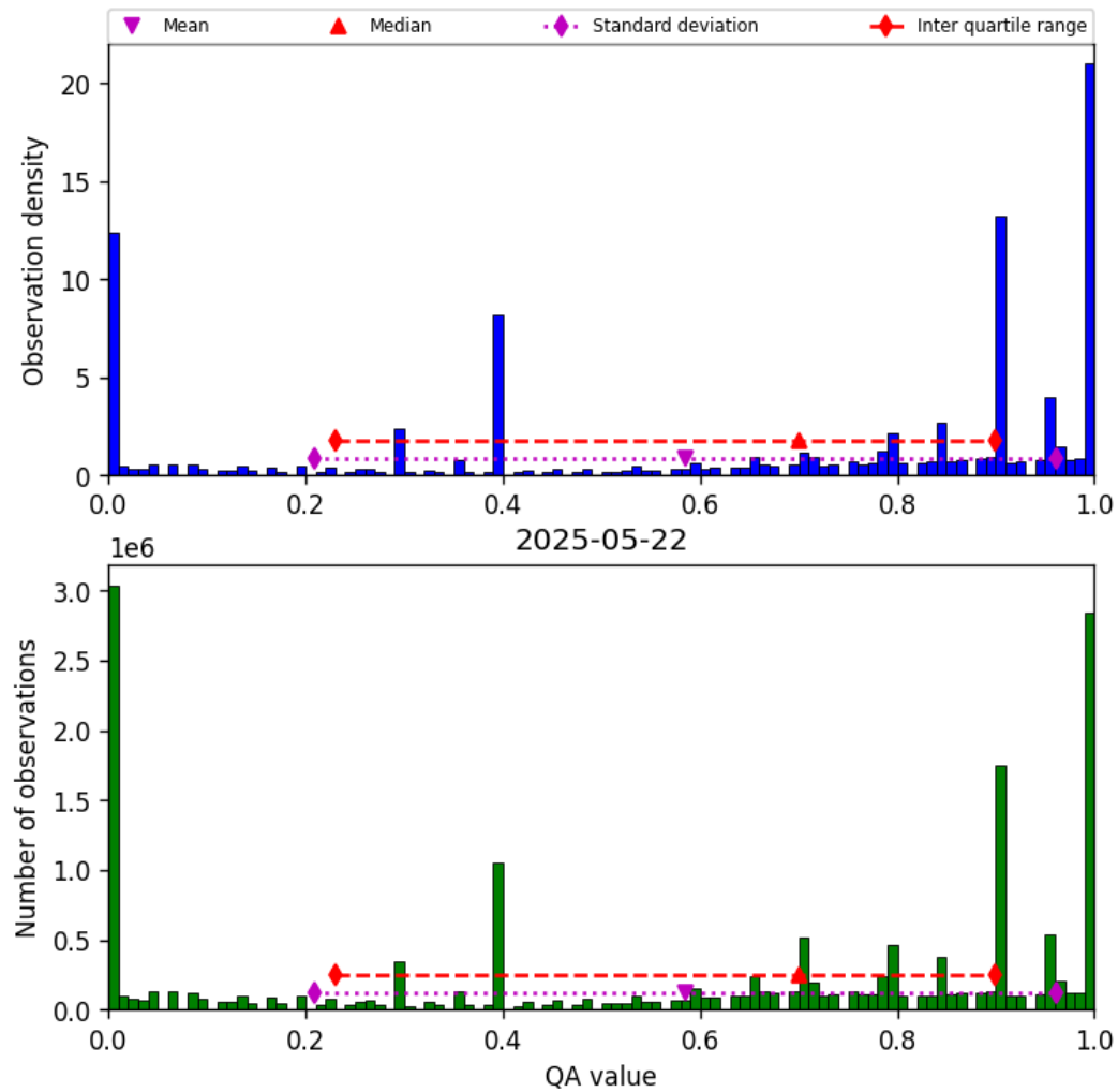
Figure 36: Histogram of “QA value” for 2025-05-22 to 2025-05-23
