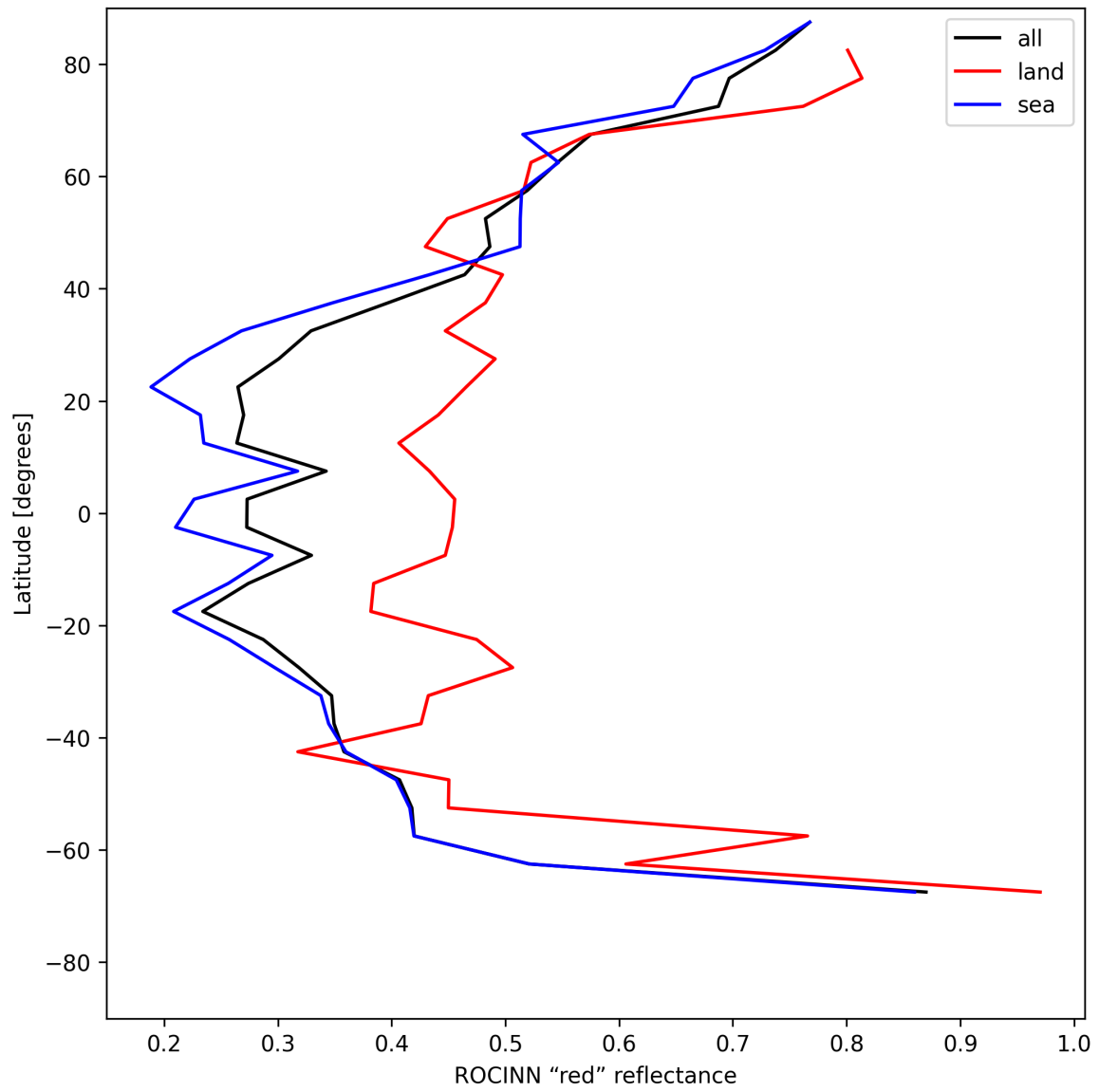
Figure 35: Zonal average of “ROCINN “red” reflectance” for 2025-05-22 to 2025-05-23.
