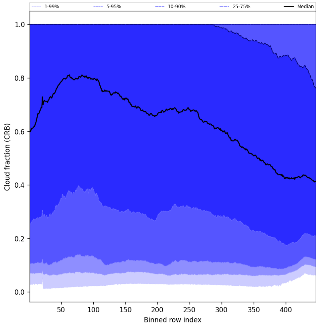
Figure 56: Along track statistics of “Cloud fraction (CRB)” for 2025-05-22 to 2025-05-23
