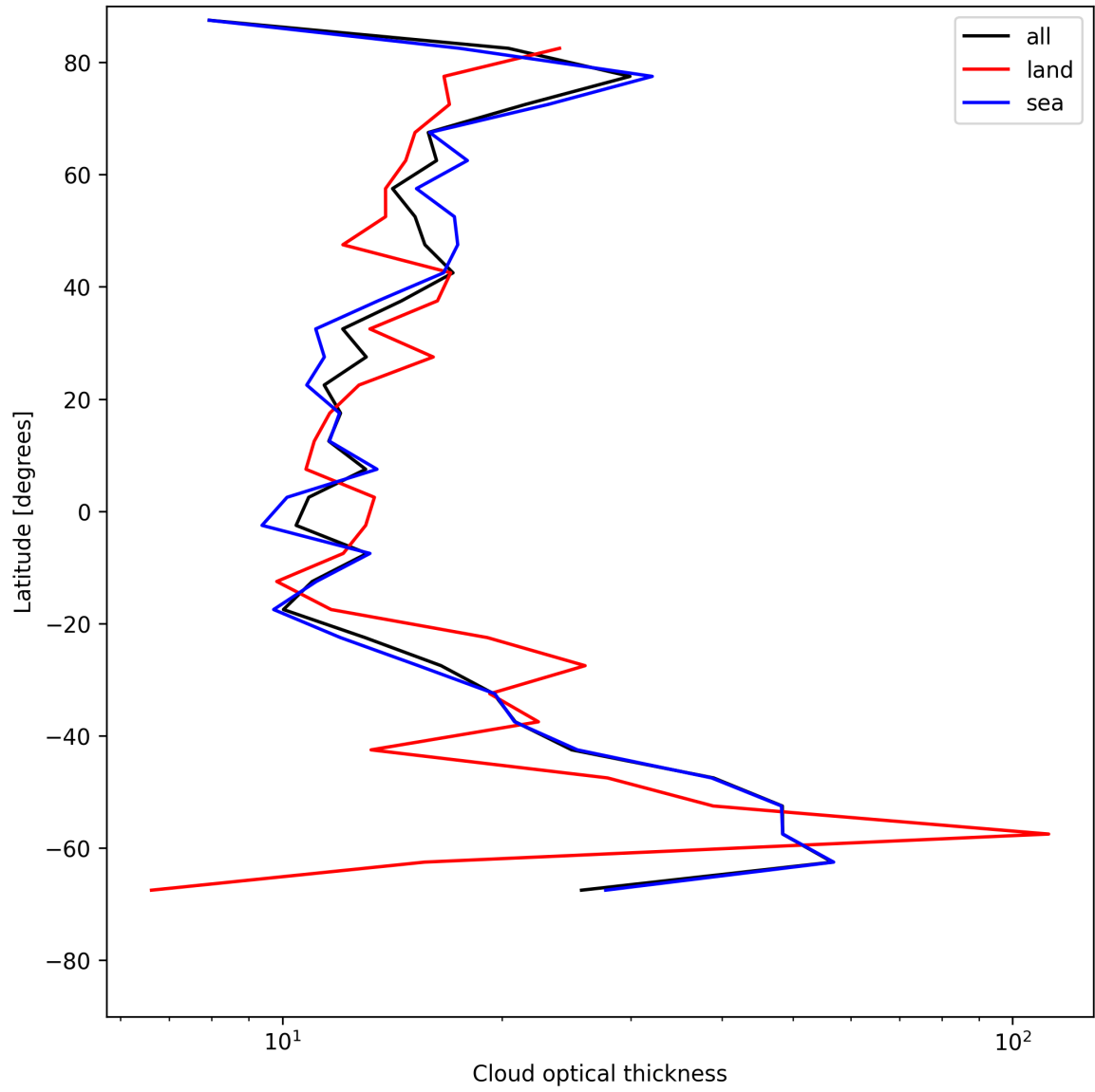
Figure 23: Zonal average of “Cloud optical thickness” for 2025-05-22 to 2025-05-23.
