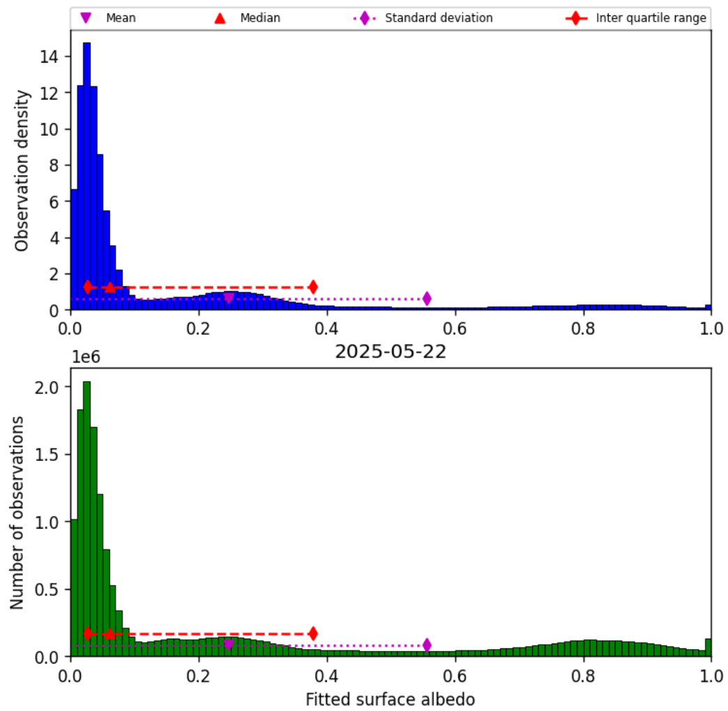
Figure 43: Histogram of “Fitted surface albedo” for 2025-05-22 to 2025-05-23
