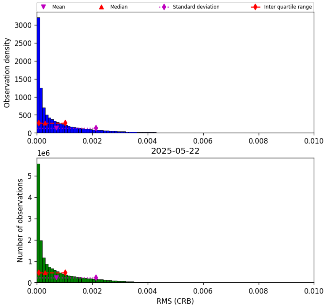
Figure 46: Histogram of “RMS (CRB)” for 2025-05-22 to 2025-05-23
