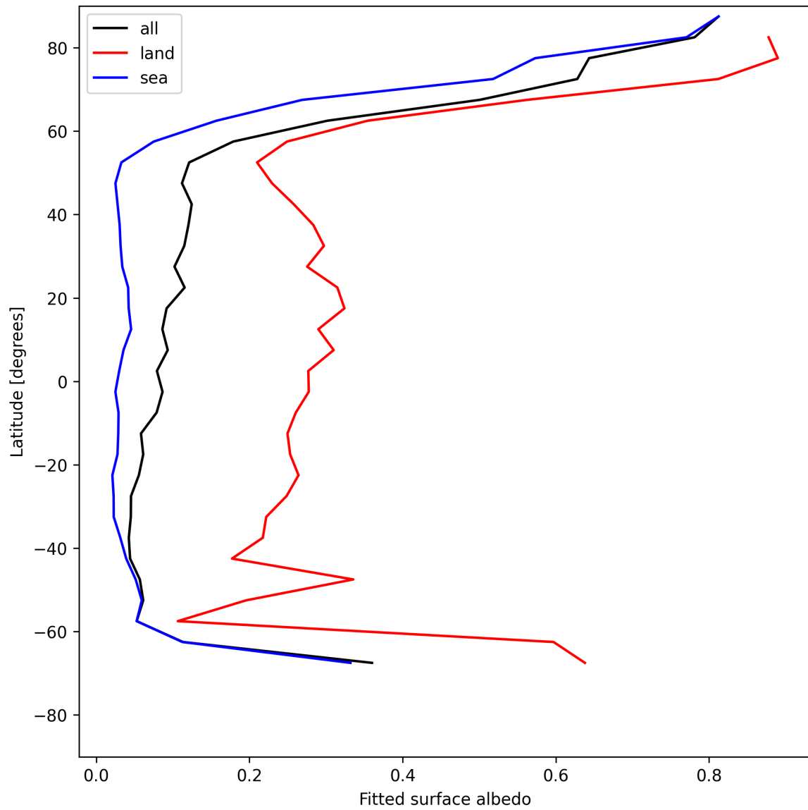
Figure 27: Zonal average of “Fitted surface albedo” for 2025-05-22 to 2025-05-23.
