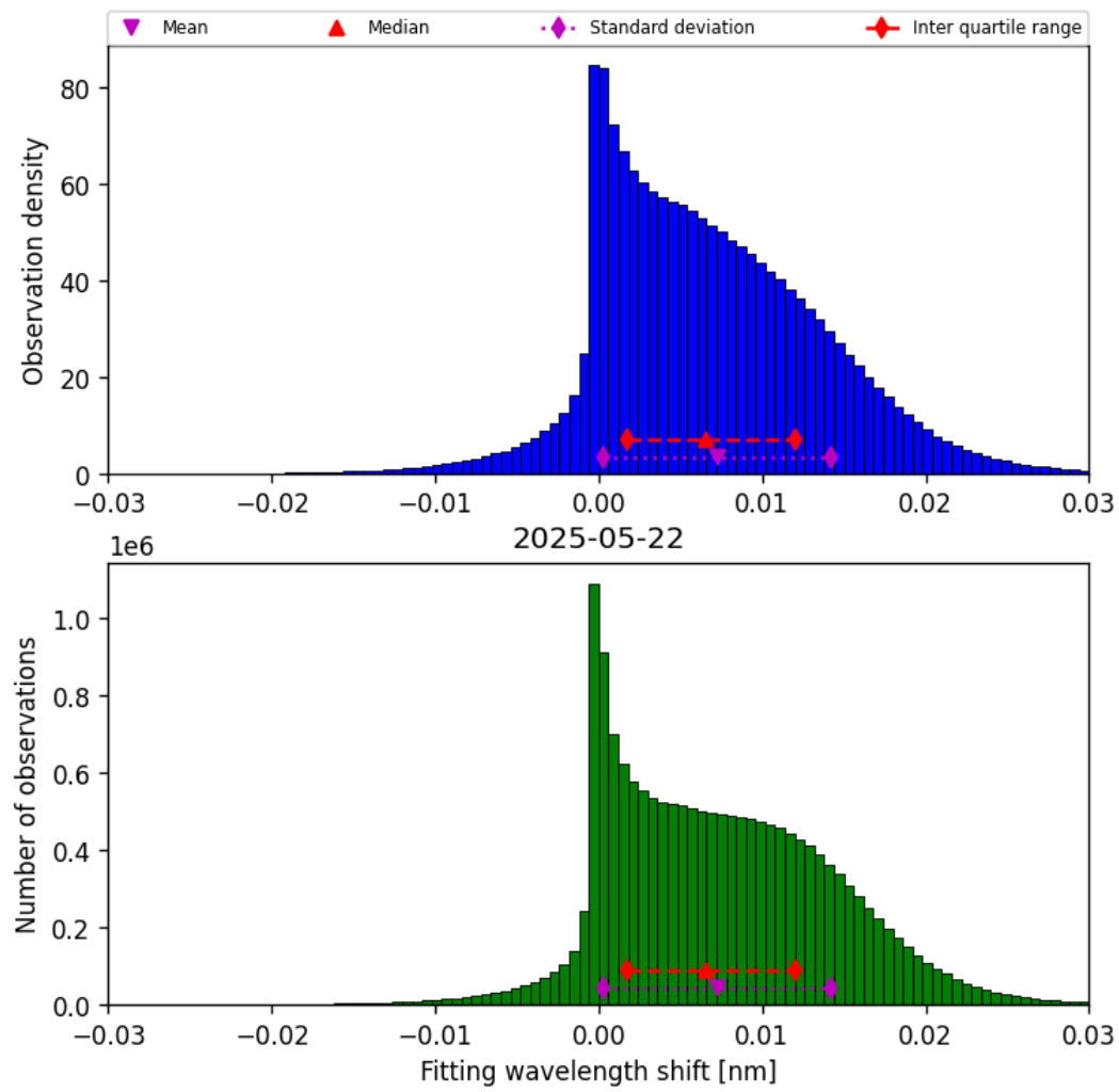
Figure 47: Histogram of “Fitting wavelength shift” for 2025-05-22 to 2025-05-23
