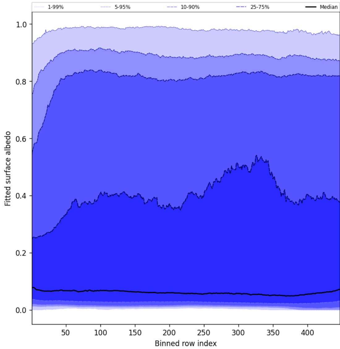
Figure 59: Along track statistics of “Fitted surface albedo” for 2025-05-22 to 2025-05-23
