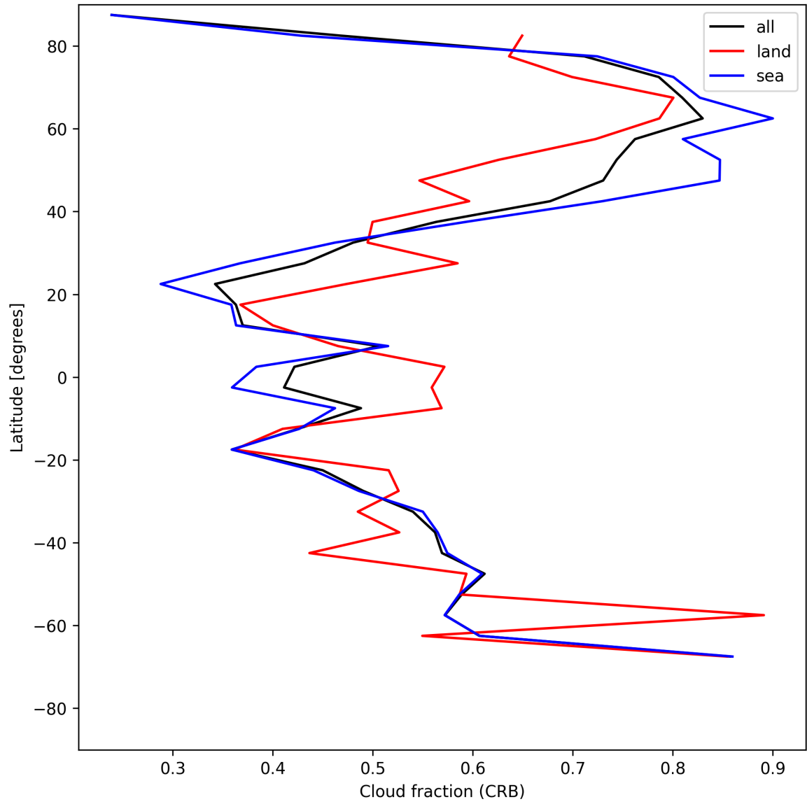
Figure 24: Zonal average of “Cloud fraction (CRB)” for 2025-05-22 to 2025-05-23.
