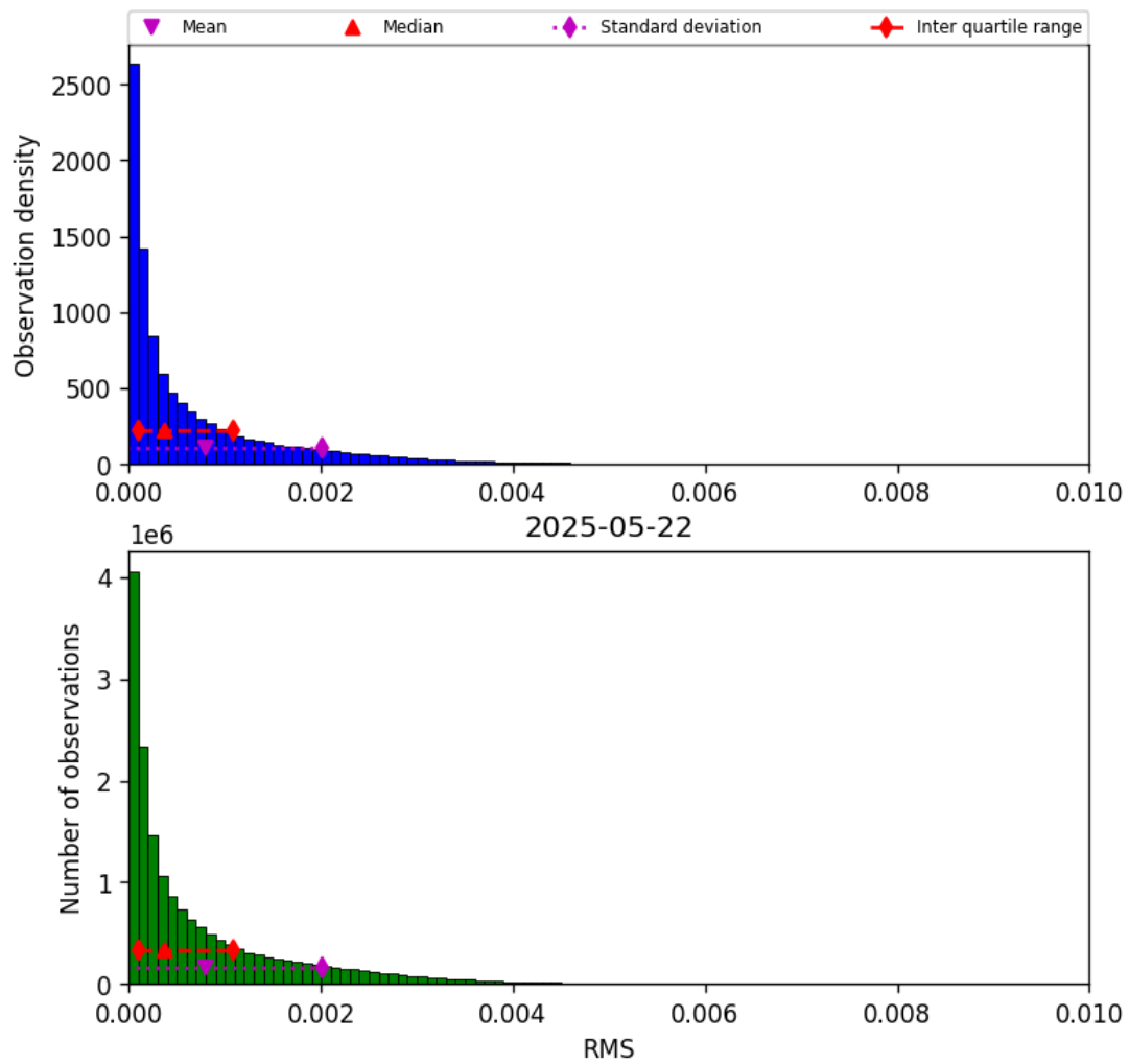
Figure 45: Histogram of “RMS” for 2025-05-22 to 2025-05-23
