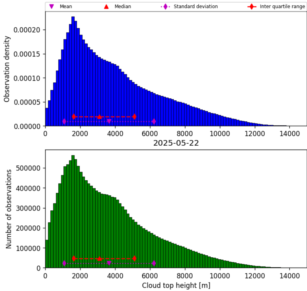
Figure 38: Histogram of “Cloud top height” for 2025-05-22 to 2025-05-23
