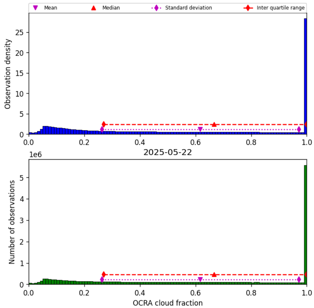
Figure 48: Histogram of “OCRA cloud fraction” for 2025-05-22 to 2025-05-23
