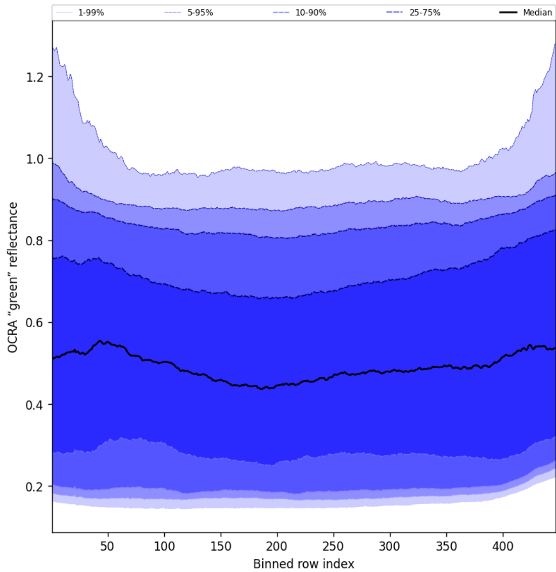
Figure 66: Along track statistics of “OCRA “green” reflectance” for 2025-05-22 to 2025-05-23
