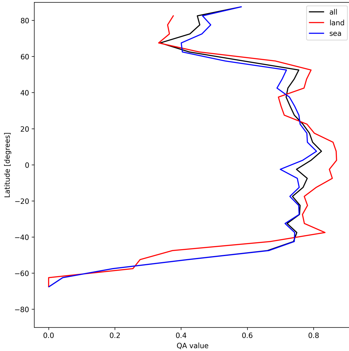
Figure 20: Zonal average of “QA value” for 2025-05-23 to 2025-05-24.
