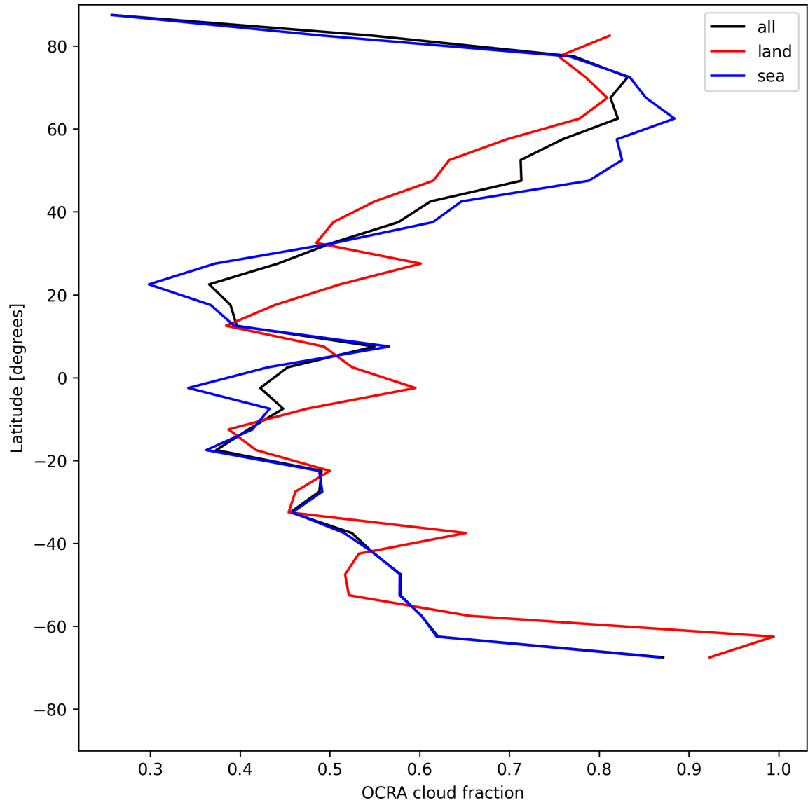
Figure 32: Zonal average of “OCRA cloud fraction” for 2025-05-23 to 2025-05-24.
