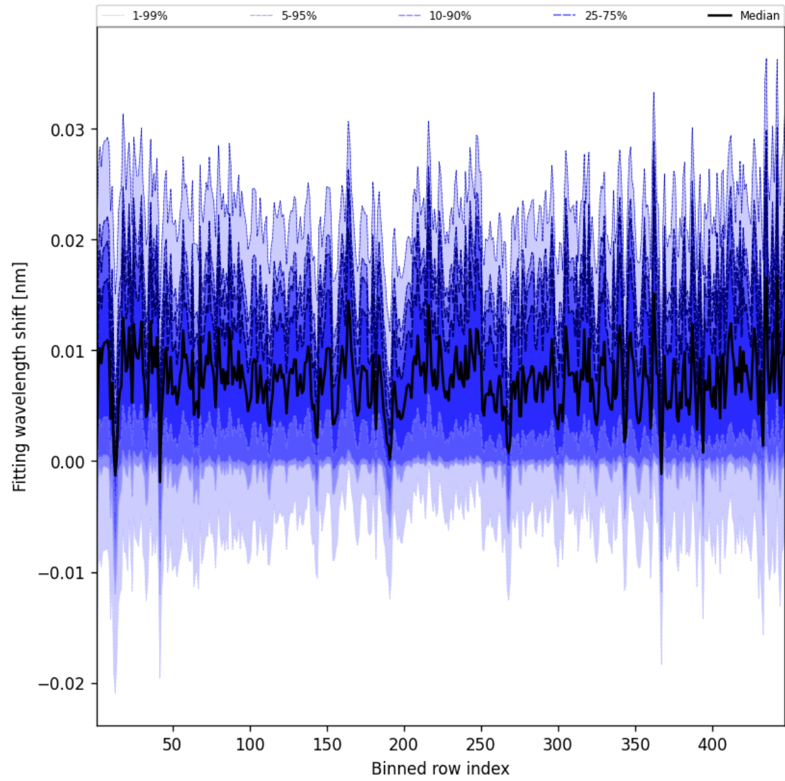
Figure 63: Along track statistics of “Fitting wavelength shift” for 2025-05-23 to 2025-05-24
