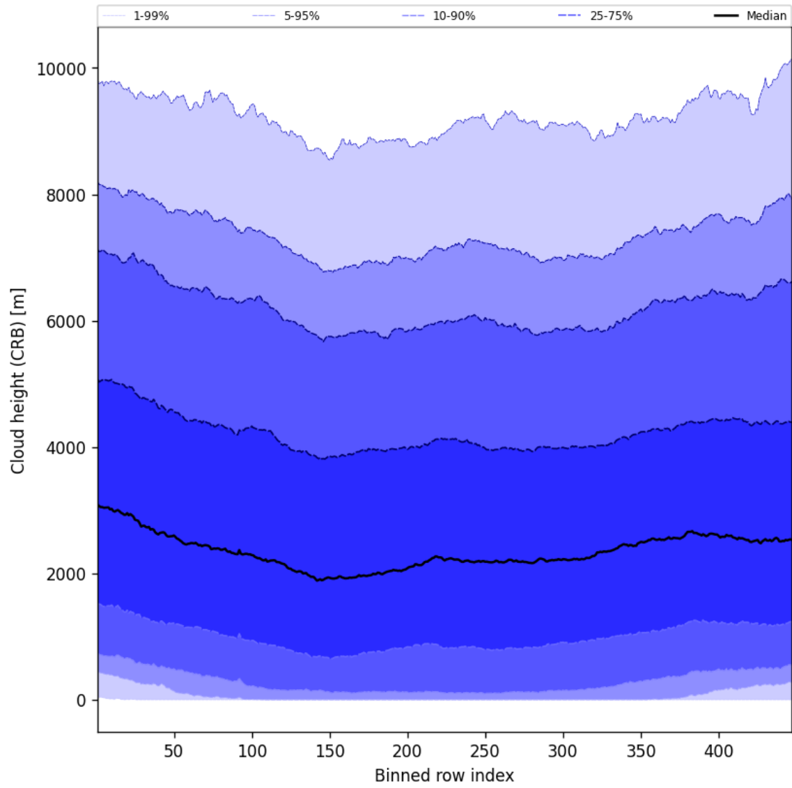
Figure 57: Along track statistics of “Cloud height (CRB)” for 2025-05-23 to 2025-05-24
