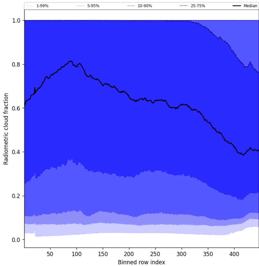
Figure 53: Along track statistics of “Radiometric cloud fraction” for 2025-05-23 to 2025-05-24
