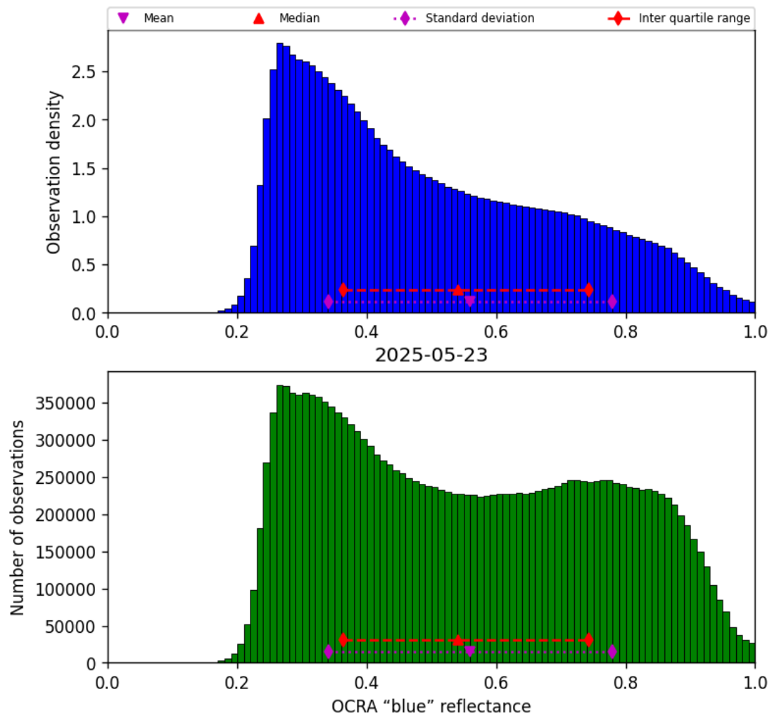
Figure 49: Histogram of “OCRA “blue” reflectance” for 2025-05-23 to 2025-05-24
