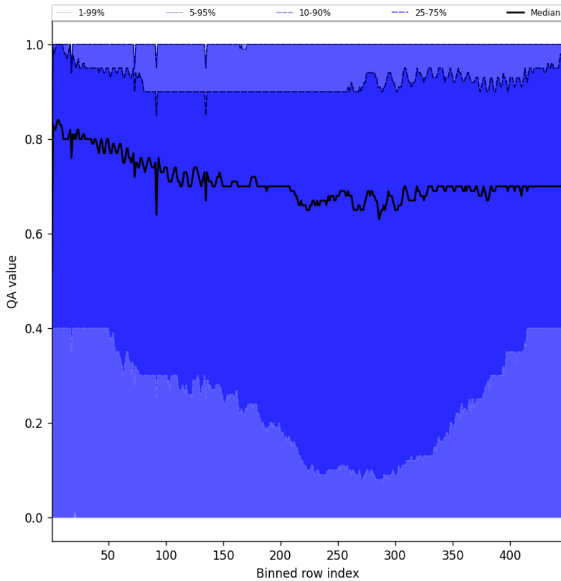
Figure 52: Along track statistics of "QA value" for 2025-05-23 to 2025-05-24
