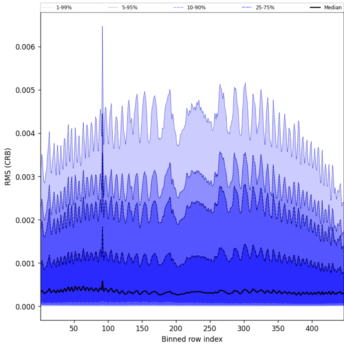
Figure 62: Along track statistics of “RMS (CRB)” for 2025-05-23 to 2025-05-24
