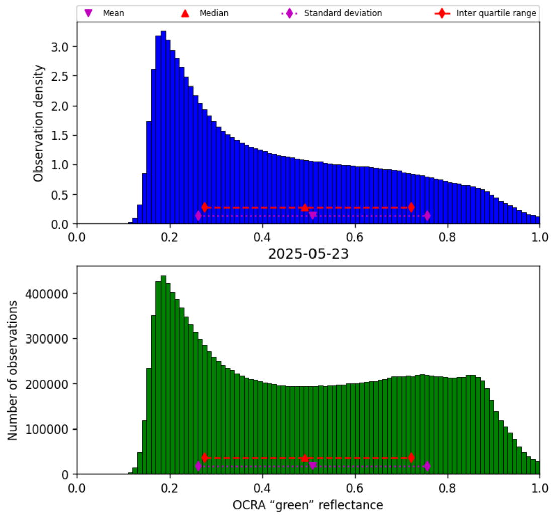
Figure 50: Histogram of “OCRA “green” reflectance” for 2025-05-23 to 2025-05-24
