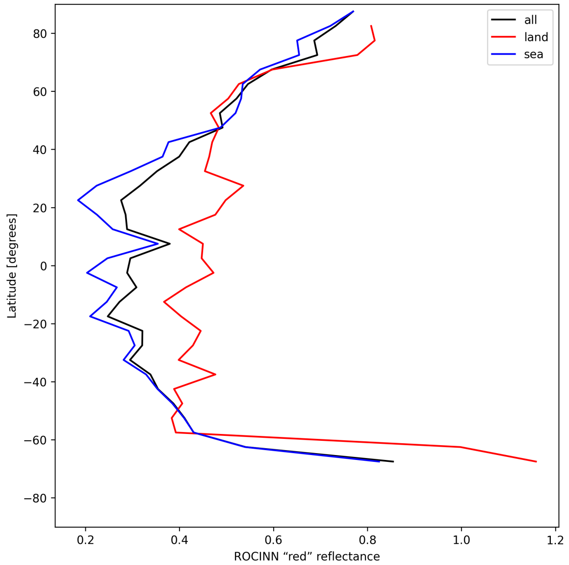
Figure 35: Zonal average of “ROCINN “red” reflectance” for 2025-05-23 to 2025-05-24.
