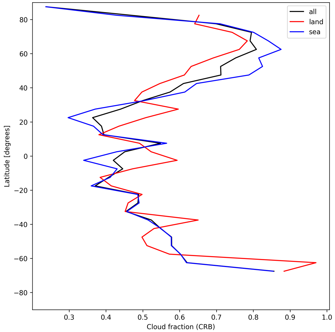
Figure 24: Zonal average of “Cloud fraction (CRB)” for 2025-05-23 to 2025-05-24.
