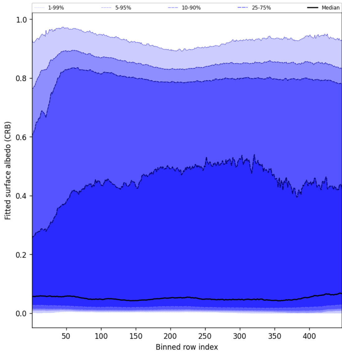
Figure 60: Along track statistics of “Fitted surface albedo (CRB)” for 2025-05-23 to 2025-05-24
