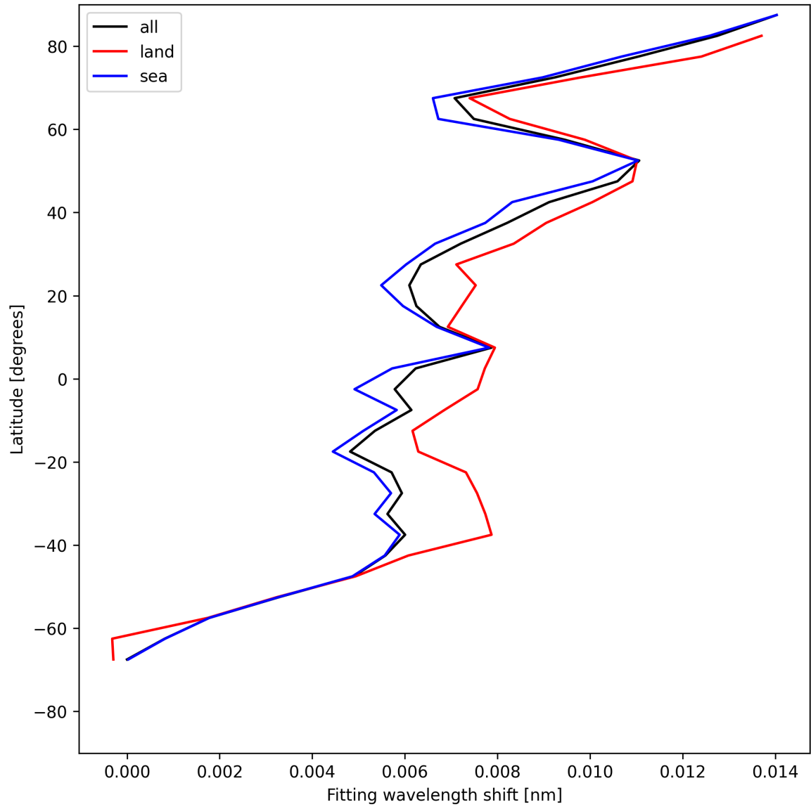
Figure 31: Zonal average of “Fitting wavelength shift” for 2025-05-23 to 2025-05-24.
