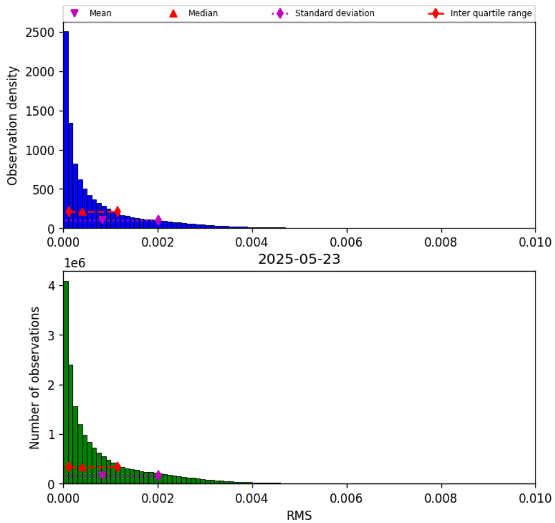
Figure 45: Histogram of “RMS” for 2025-05-23 to 2025-05-24
