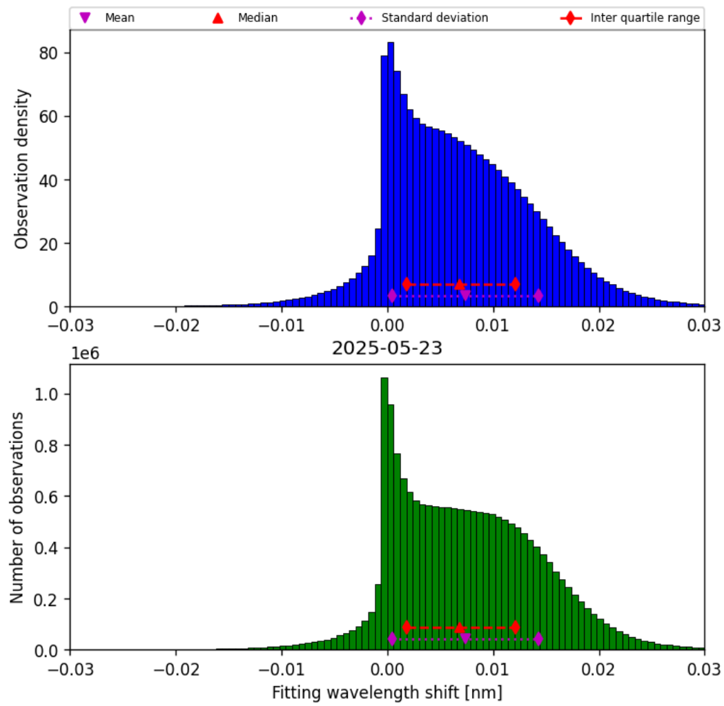
Figure 47: Histogram of “Fitting wavelength shift” for 2025-05-23 to 2025-05-24
