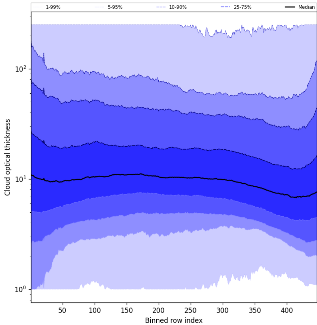
Figure 55: Along track statistics of “Cloud optical thickness” for 2025-05-23 to 2025-05-24
