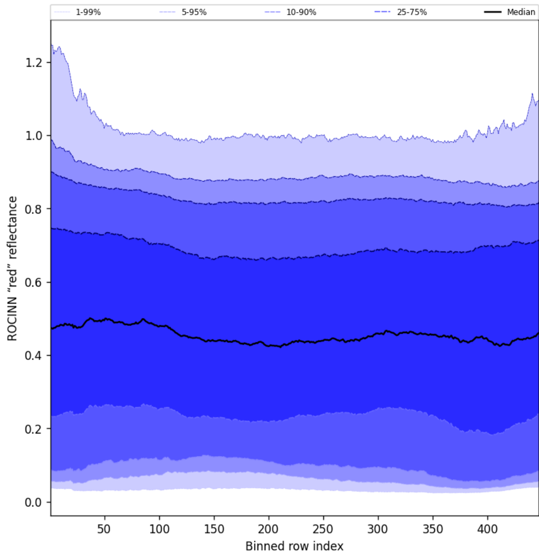
Figure 67: Along track statistics of “ROCINN “red” reflectance” for 2025-05-23 to 2025-05-24
