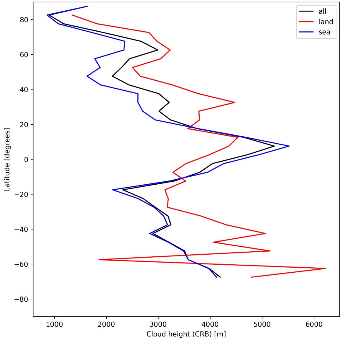
Figure 25: Zonal average of “Cloud height (CRB)” for 2025-05-23 to 2025-05-24.
