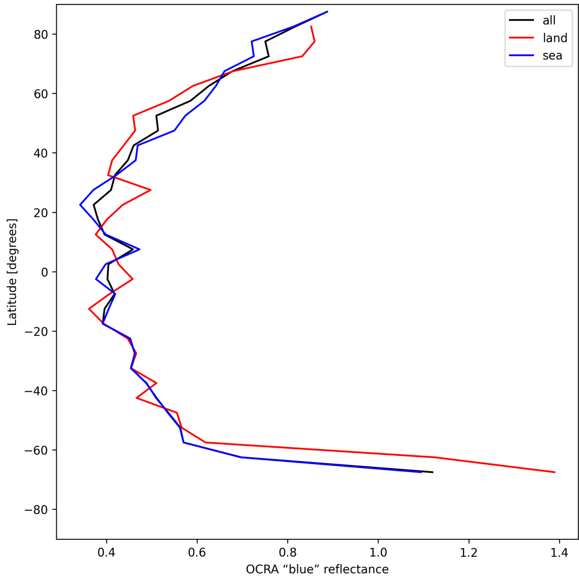
Figure 33: Zonal average of “OCRA “blue” reflectance” for 2025-05-23 to 2025-05-24.
