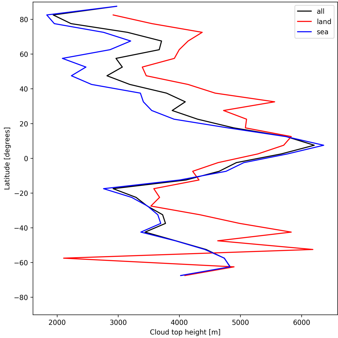
Figure 22: Zonal average of “Cloud top height” for 2025-05-23 to 2025-05-24.
