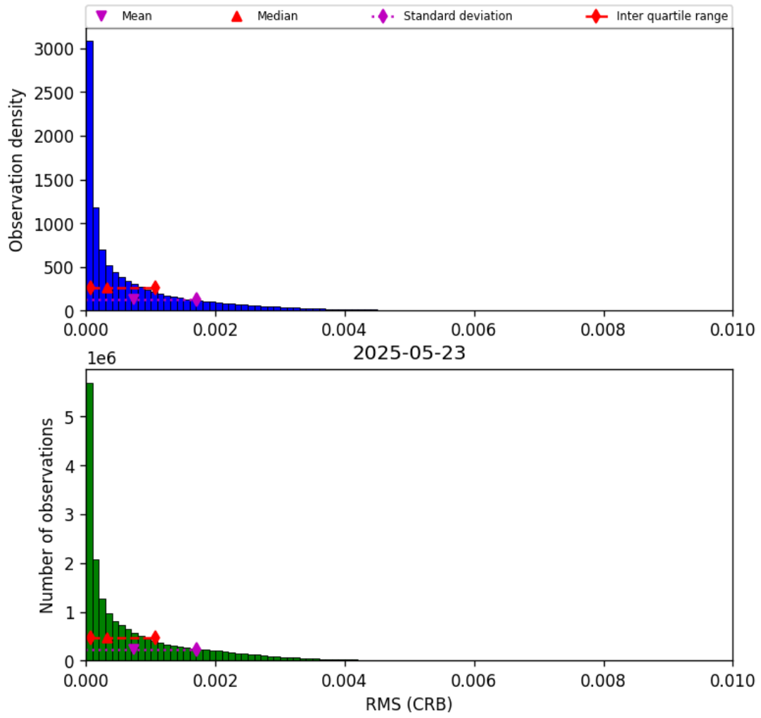
Figure 46: Histogram of “RMS (CRB)” for 2025-05-23 to 2025-05-24
