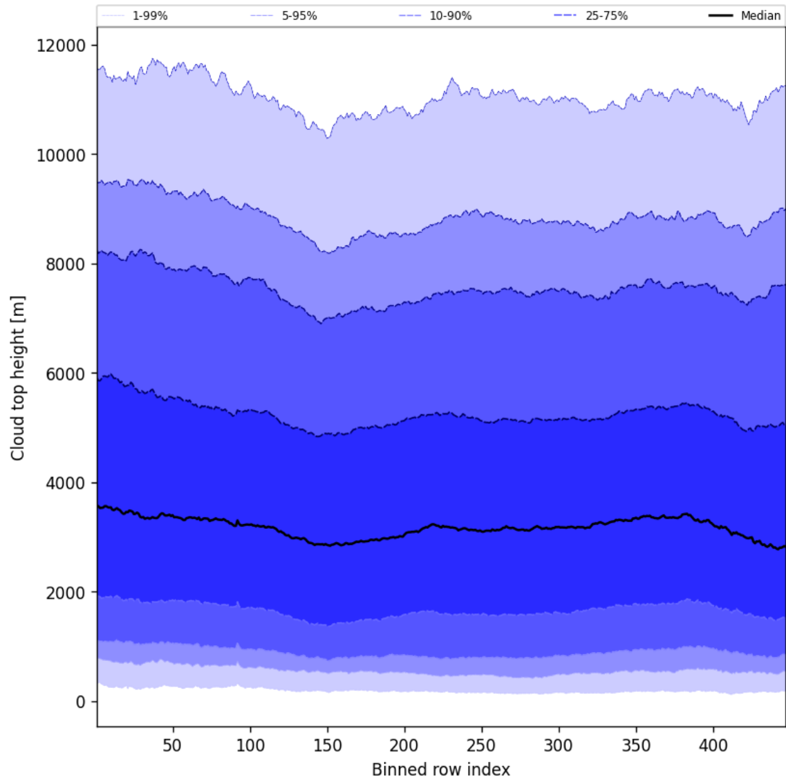
Figure 54: Along track statistics of “Cloud top height” for 2025-05-23 to 2025-05-24
