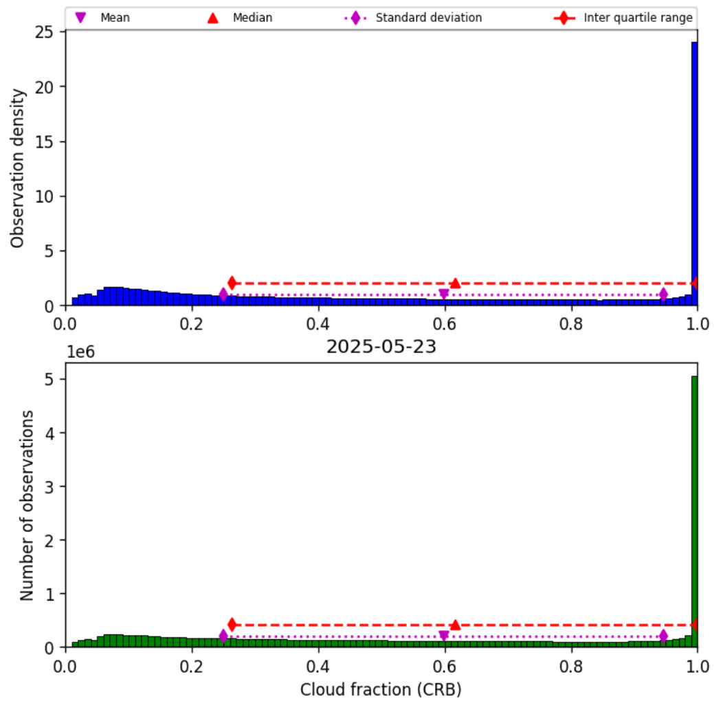
Figure 40: Histogram of “Cloud fraction (CRB)” for 2025-05-23 to 2025-05-24
