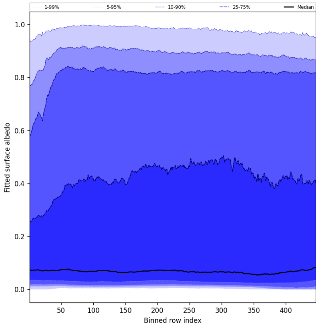
Figure 59: Along track statistics of “Fitted surface albedo” for 2025-05-23 to 2025-05-24
