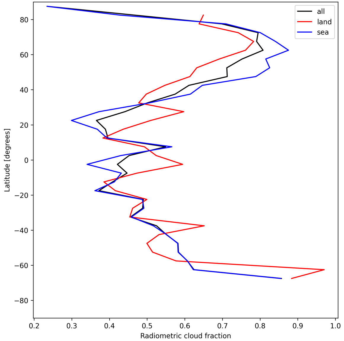
Figure 21: Zonal average of “Radiometric cloud fraction” for 2025-05-23 to 2025-05-24.
