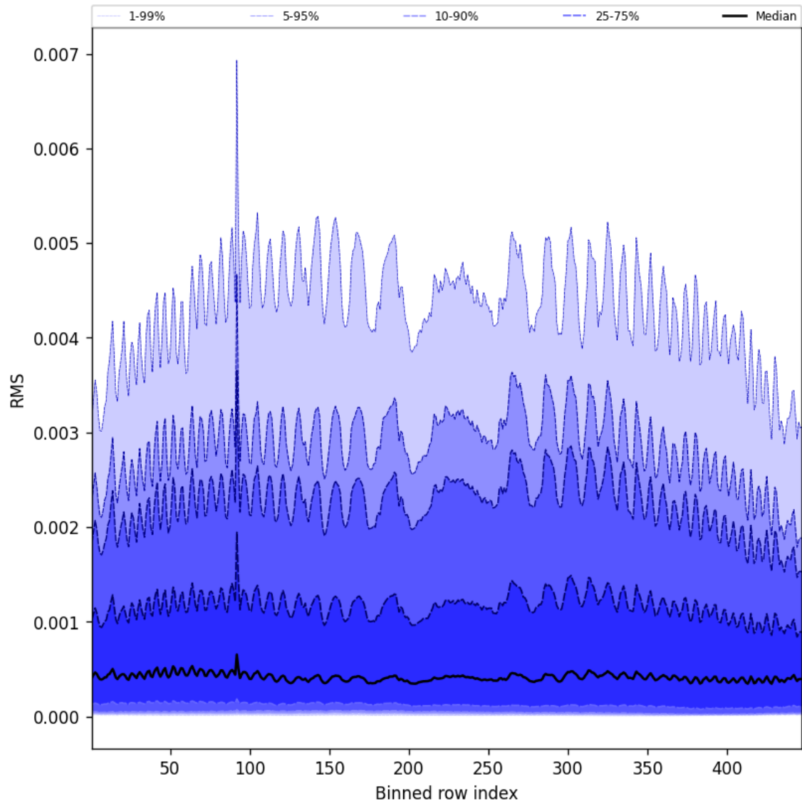
Figure 61: Along track statistics of “RMS” for 2025-05-23 to 2025-05-24
