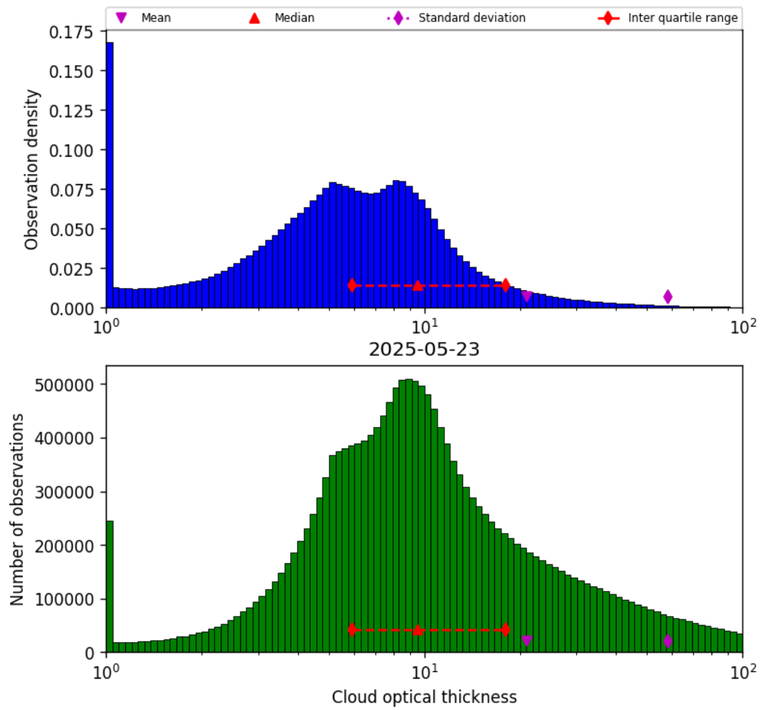
Figure 39: Histogram of “Cloud optical thickness” for 2025-05-23 to 2025-05-24
