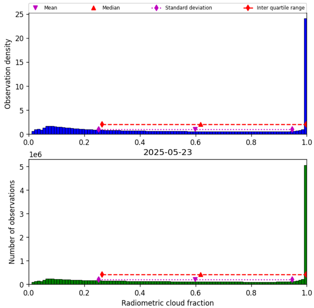
Figure 37: Histogram of “Radiometric cloud fraction” for 2025-05-23 to 2025-05-24
