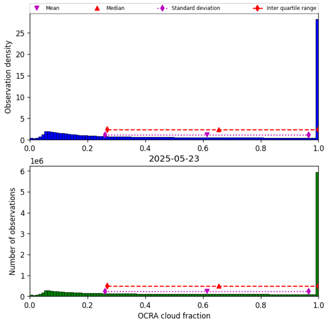
Figure 48: Histogram of “OCRA cloud fraction” for 2025-05-23 to 2025-05-24
