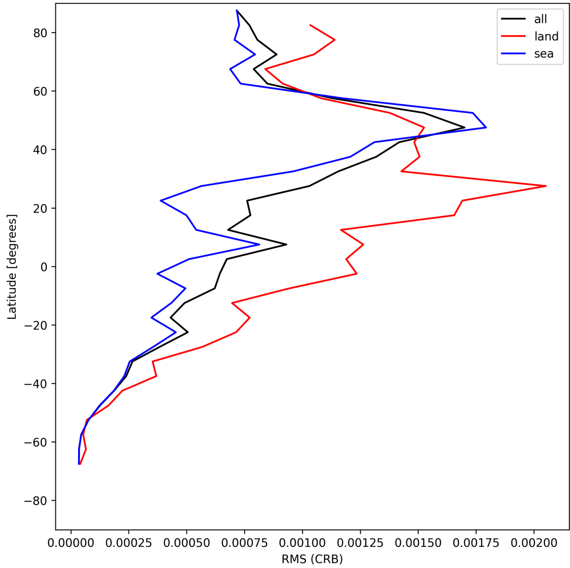
Figure 30: Zonal average of “RMS (CRB)” for 2025-05-23 to 2025-05-24.
