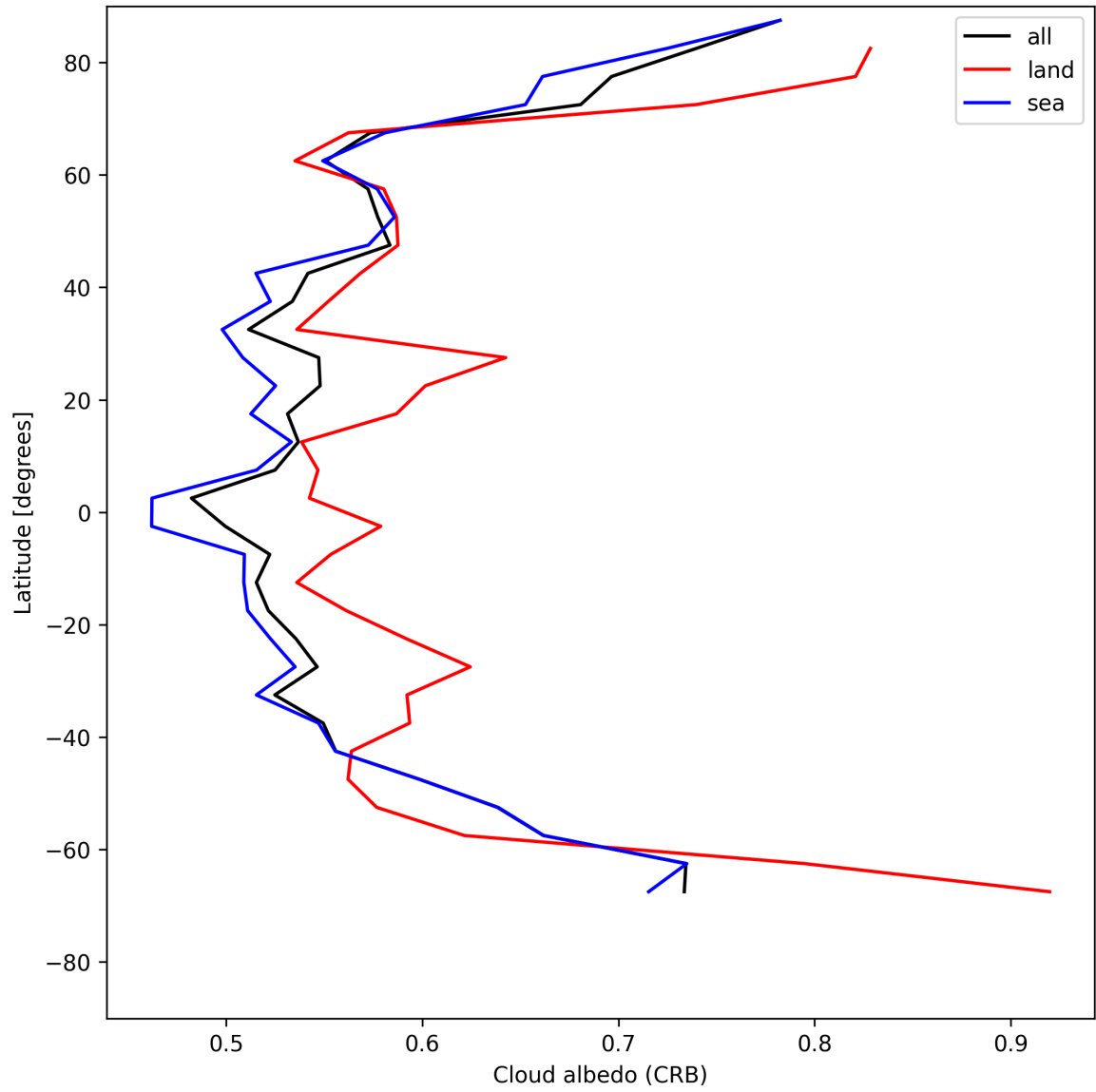
Figure 26: Zonal average of “Cloud albedo (CRB)” for 2025-05-23 to 2025-05-24.
