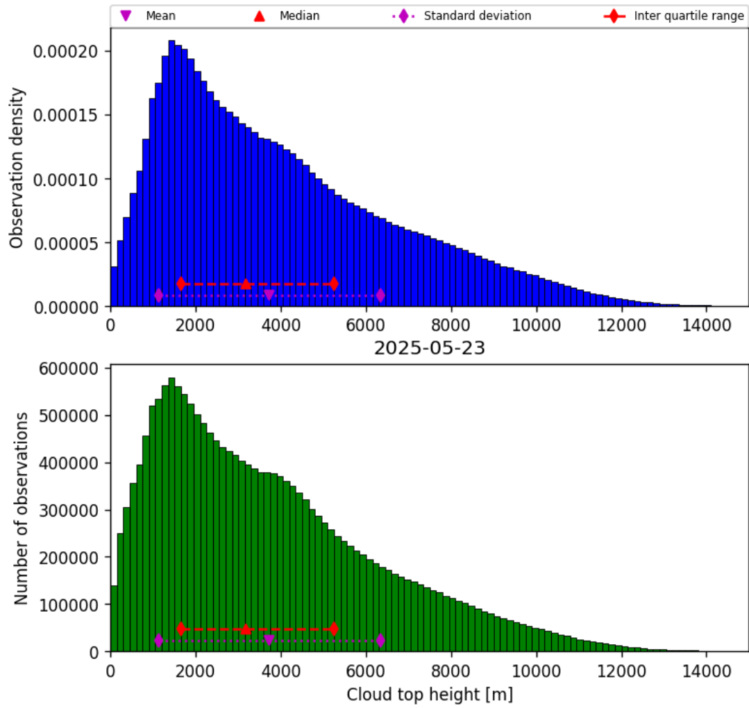
Figure 38: Histogram of “Cloud top height” for 2025-05-23 to 2025-05-24
