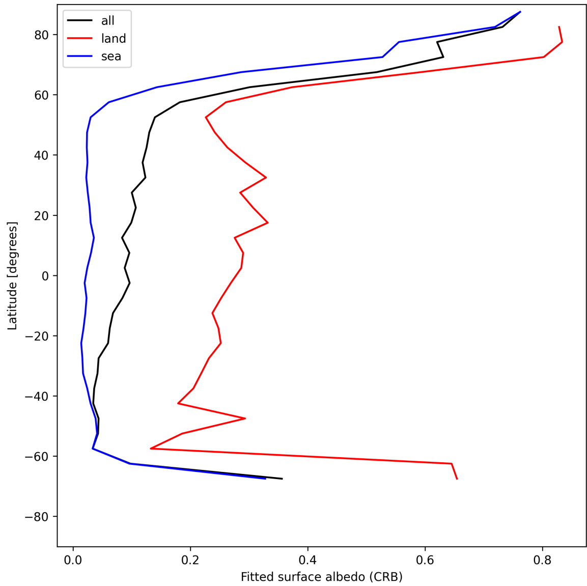
Figure 28: Zonal average of “Fitted surface albedo (CRB)” for 2025-05-23 to 2025-05-24.
