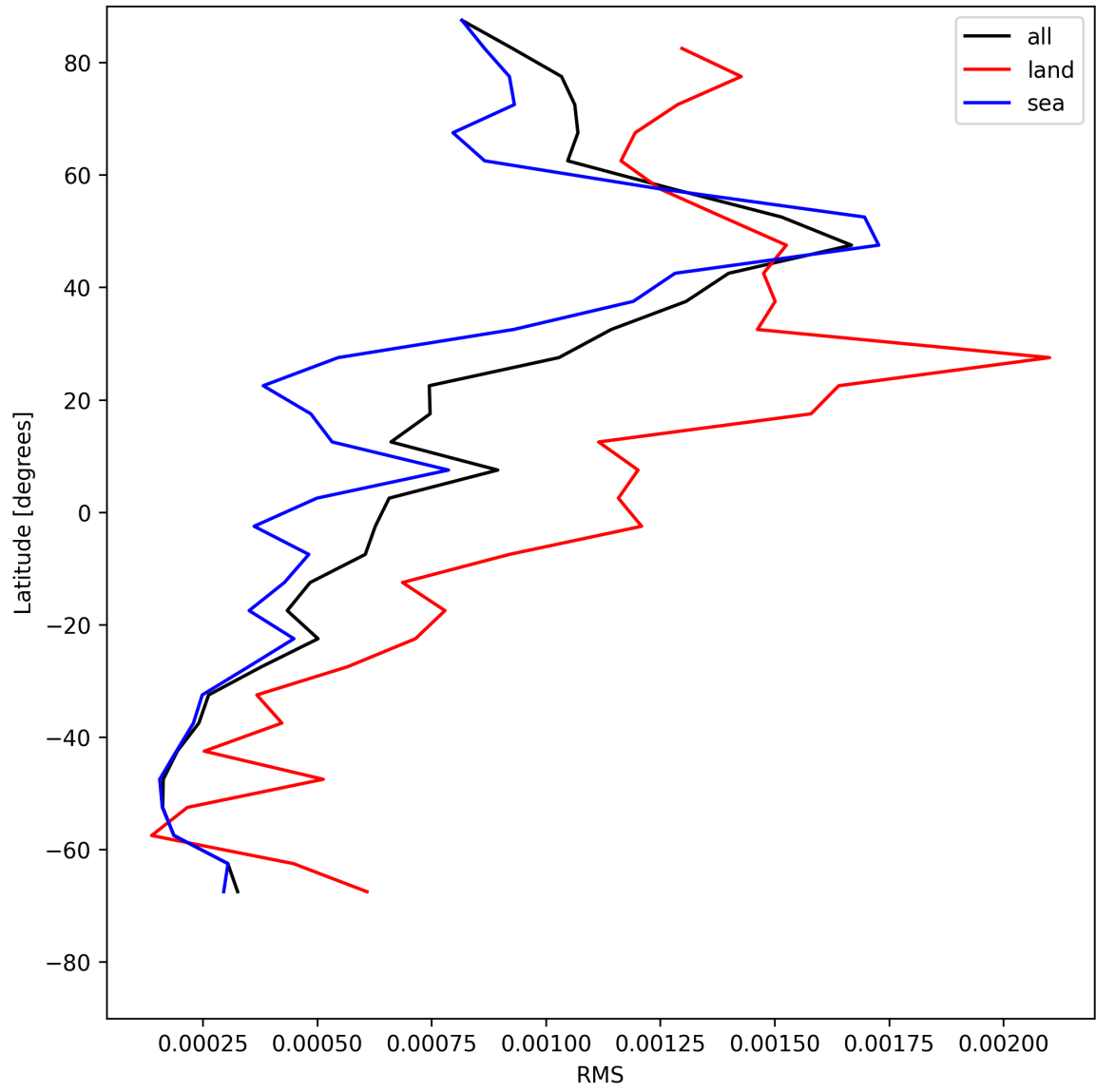
Figure 29: Zonal average of “RMS” for 2025-05-23 to 2025-05-24.
