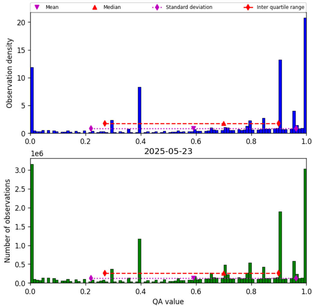
Figure 36: Histogram of “QA value” for 2025-05-23 to 2025-05-24
