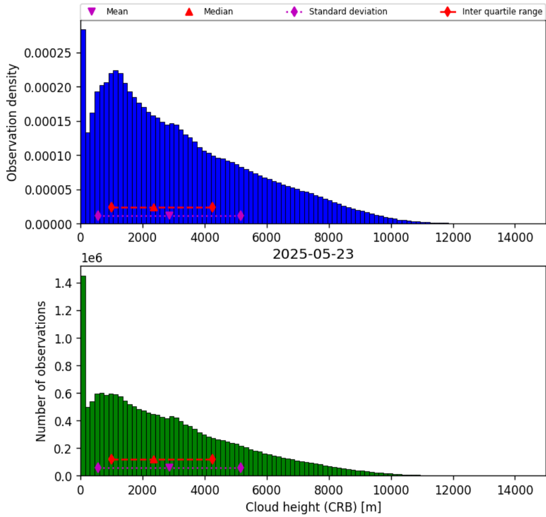
Figure 41: Histogram of “Cloud height (CRB)” for 2025-05-23 to 2025-05-24
