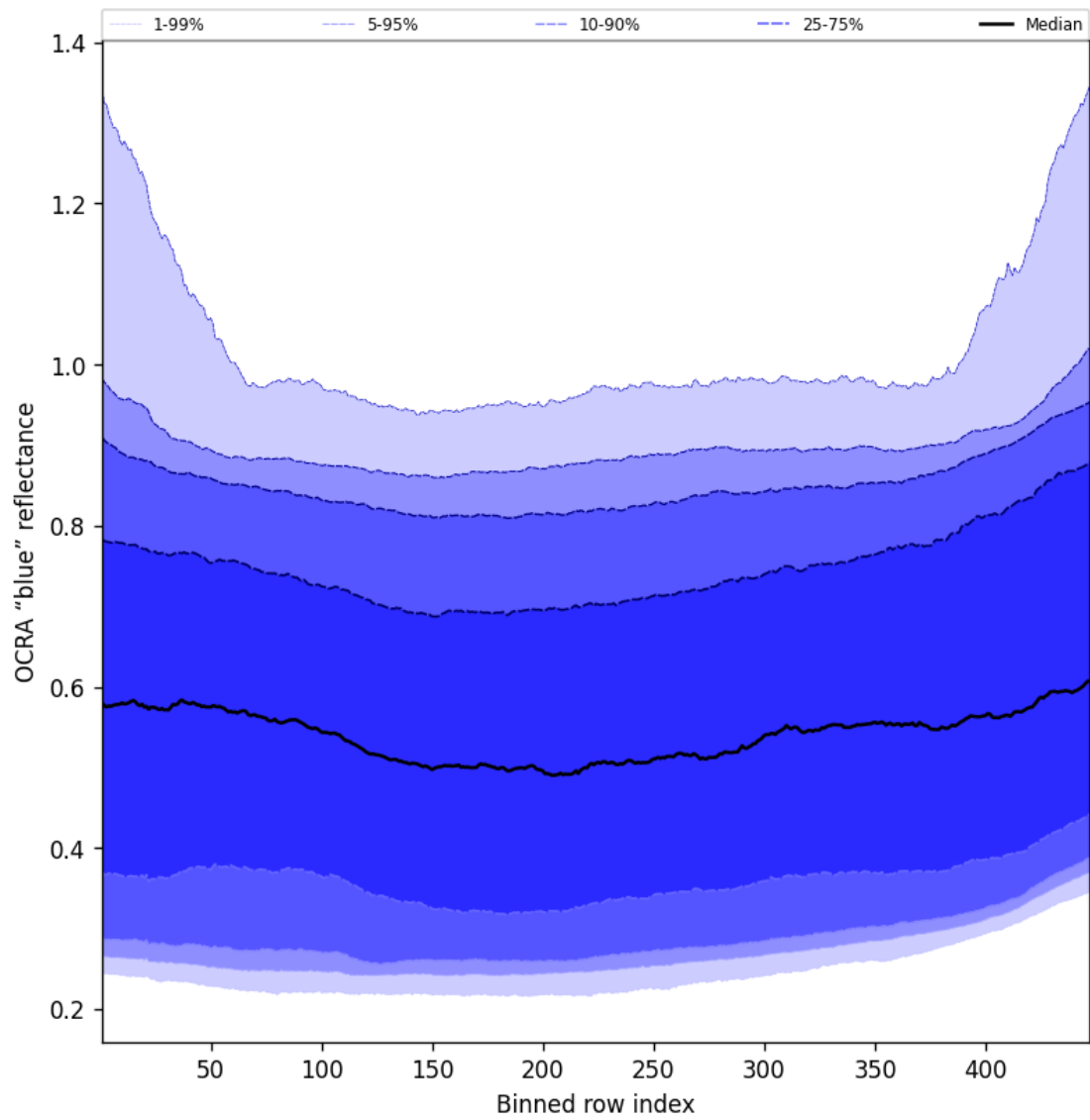
Figure 65: Along track statistics of "OCRA "blue" reflectance" for 2025-05-23 to 2025-05-24
