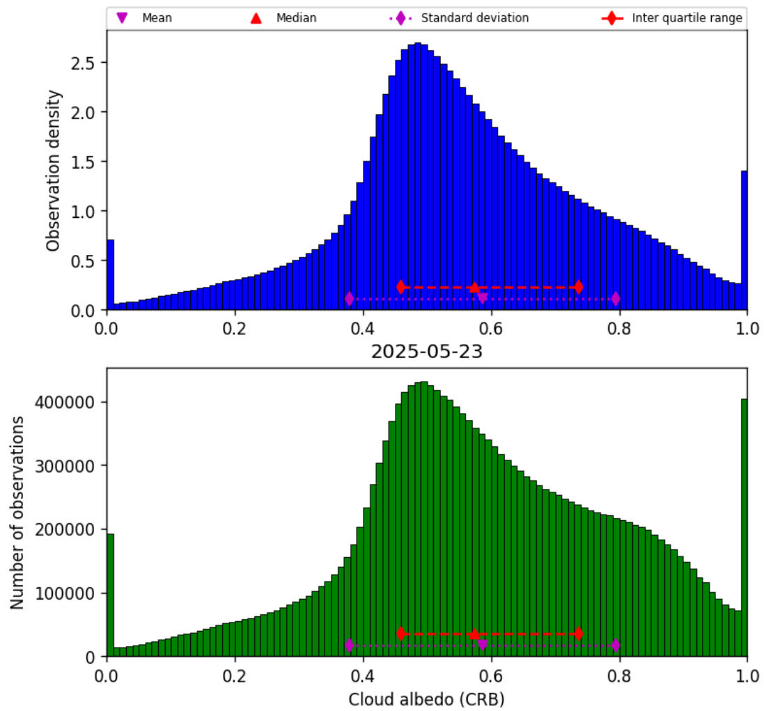
Figure 42: Histogram of “Cloud albedo (CRB)” for 2025-05-23 to 2025-05-24
