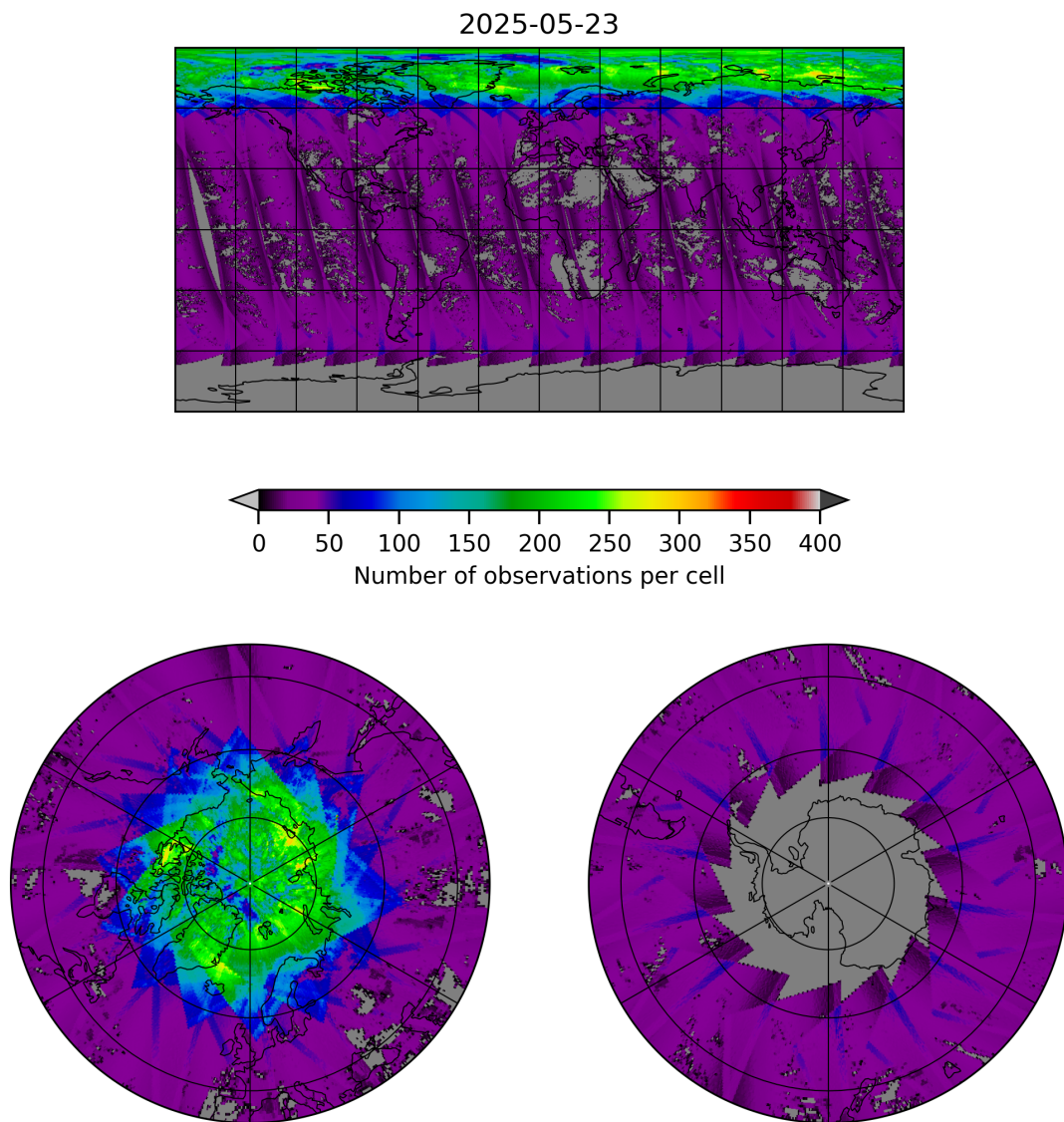
Figure 19: Map of the number of observations for 2025-05-23 to 2025-05-24
