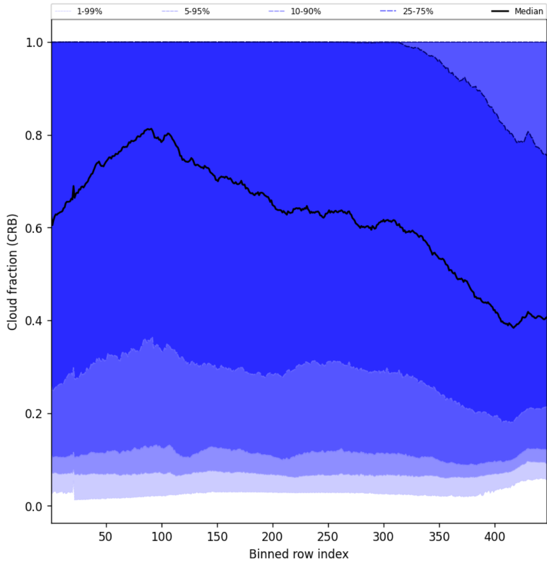
Figure 56: Along track statistics of “Cloud fraction (CRB)” for 2025-05-23 to 2025-05-24
