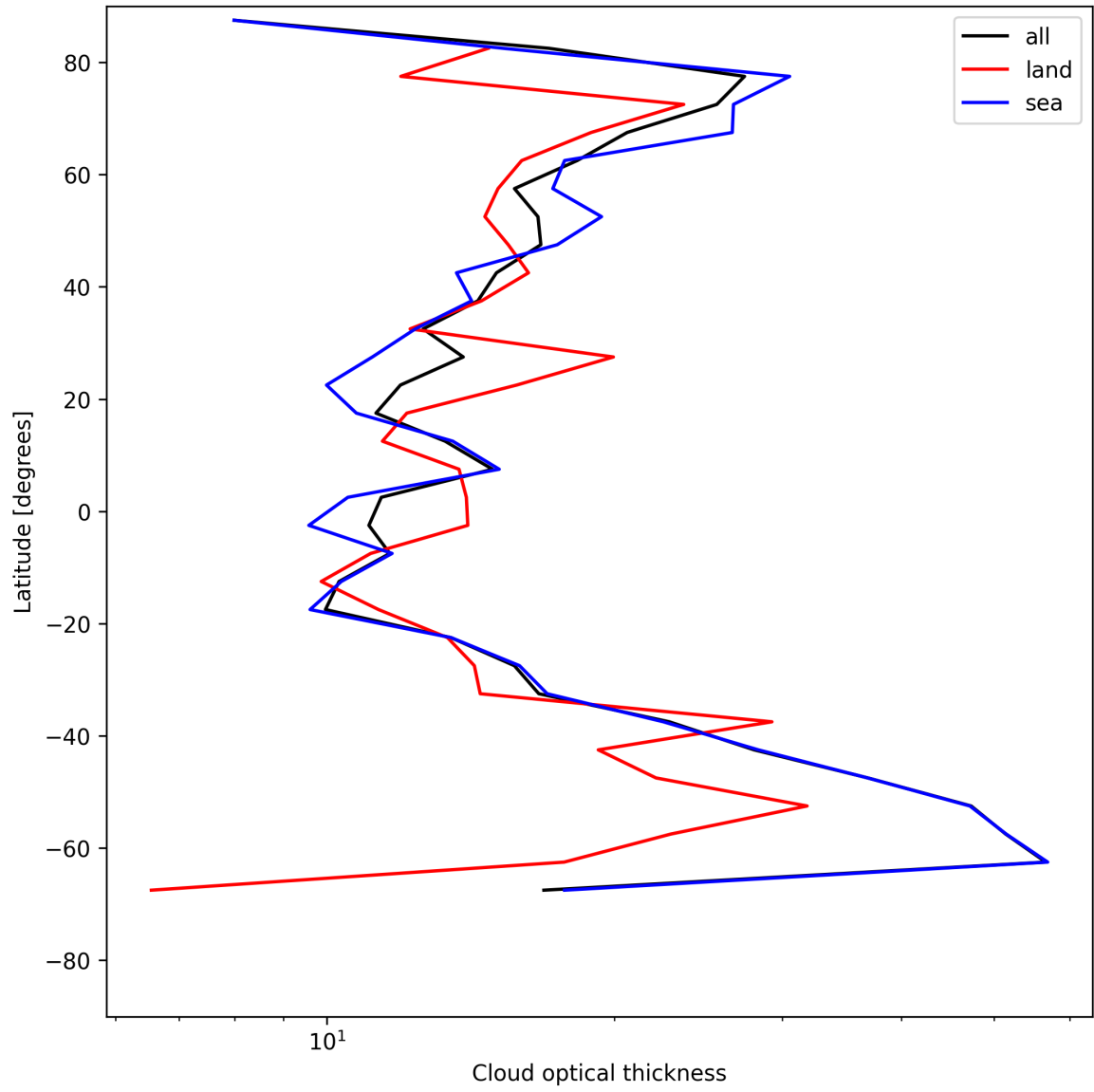
Figure 23: Zonal average of “Cloud optical thickness” for 2025-05-23 to 2025-05-24.
