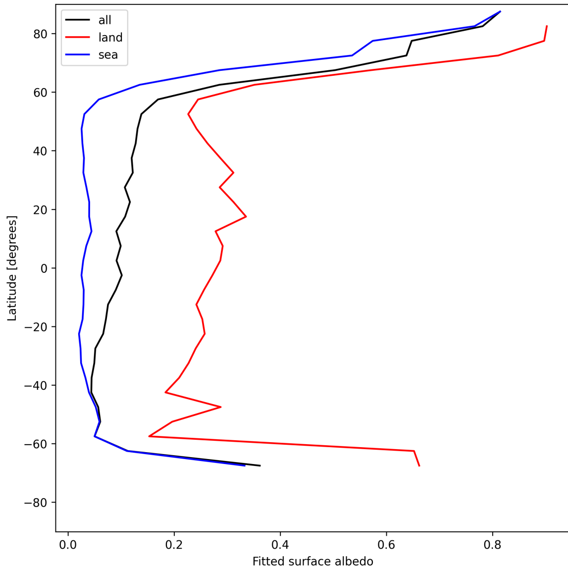
Figure 27: Zonal average of “Fitted surface albedo” for 2025-05-23 to 2025-05-24.
