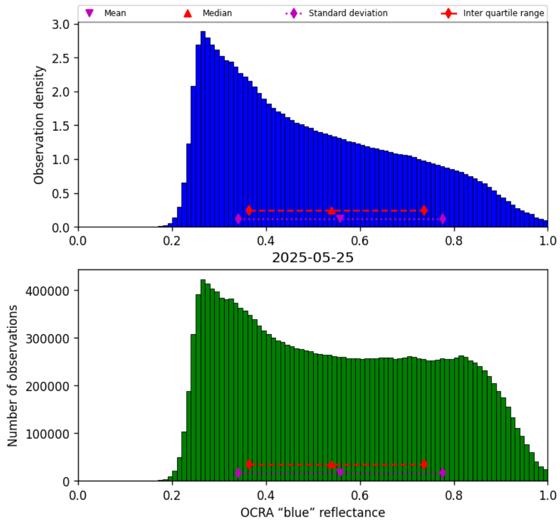
Figure 49: Histogram of “OCRA “blue” reflectance” for 2025-05-25 to 2025-05-26
