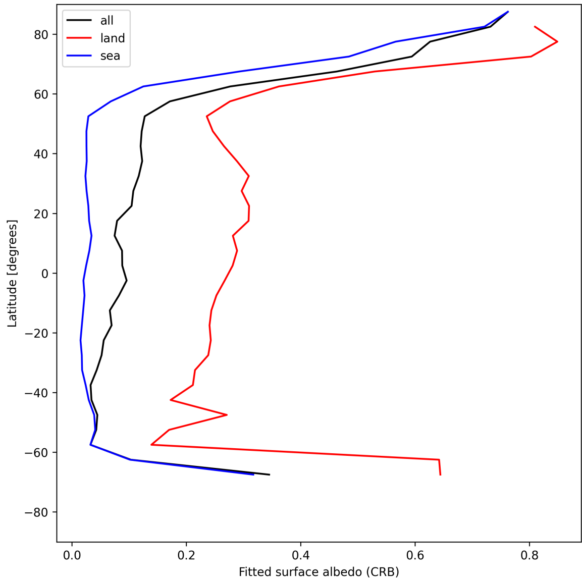
Figure 28: Zonal average of “Fitted surface albedo (CRB)” for 2025-05-25 to 2025-05-26.
