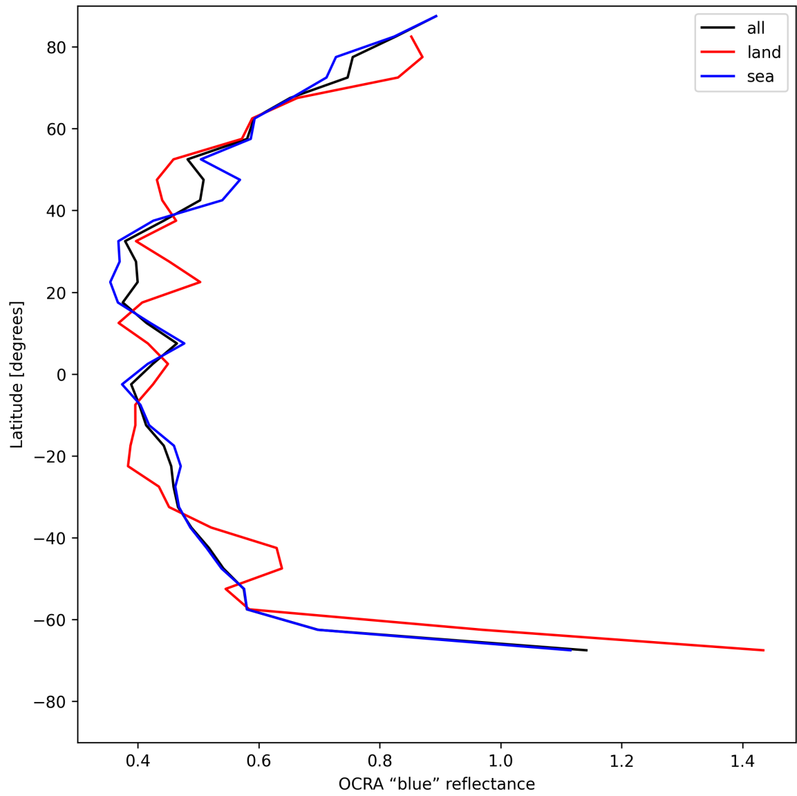
Figure 33: Zonal average of “OCRA “blue” reflectance” for 2025-05-25 to 2025-05-26.
