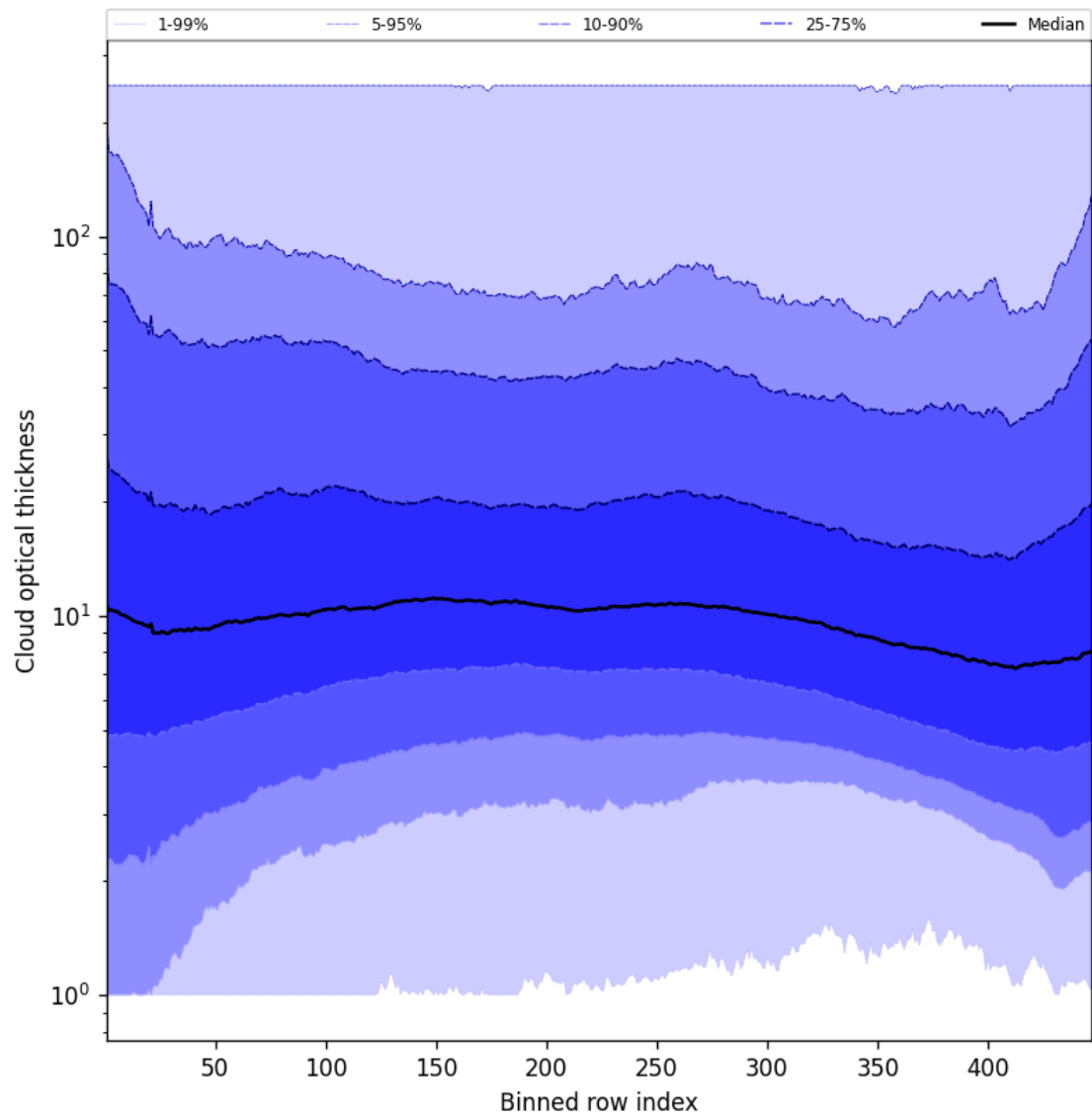
Figure 55: Along track statistics of “Cloud optical thickness” for 2025-05-25 to 2025-05-26
