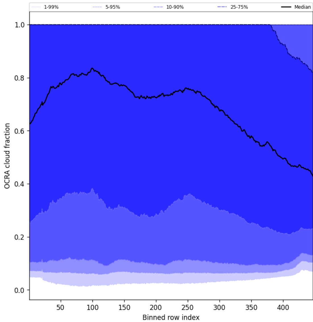
Figure 64: Along track statistics of “OCRA cloud fraction” for 2025-05-25 to 2025-05-26
