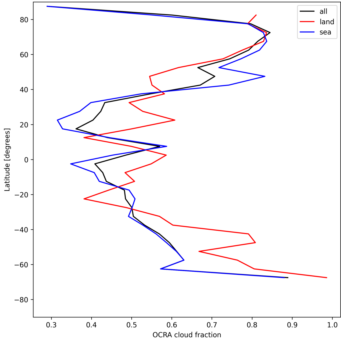
Figure 32: Zonal average of “OCRA cloud fraction” for 2025-05-25 to 2025-05-26.
