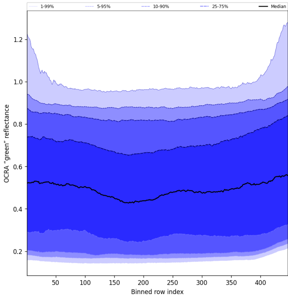
Figure 66: Along track statistics of “OCRA “green” reflectance” for 2025-05-25 to 2025-05-26
