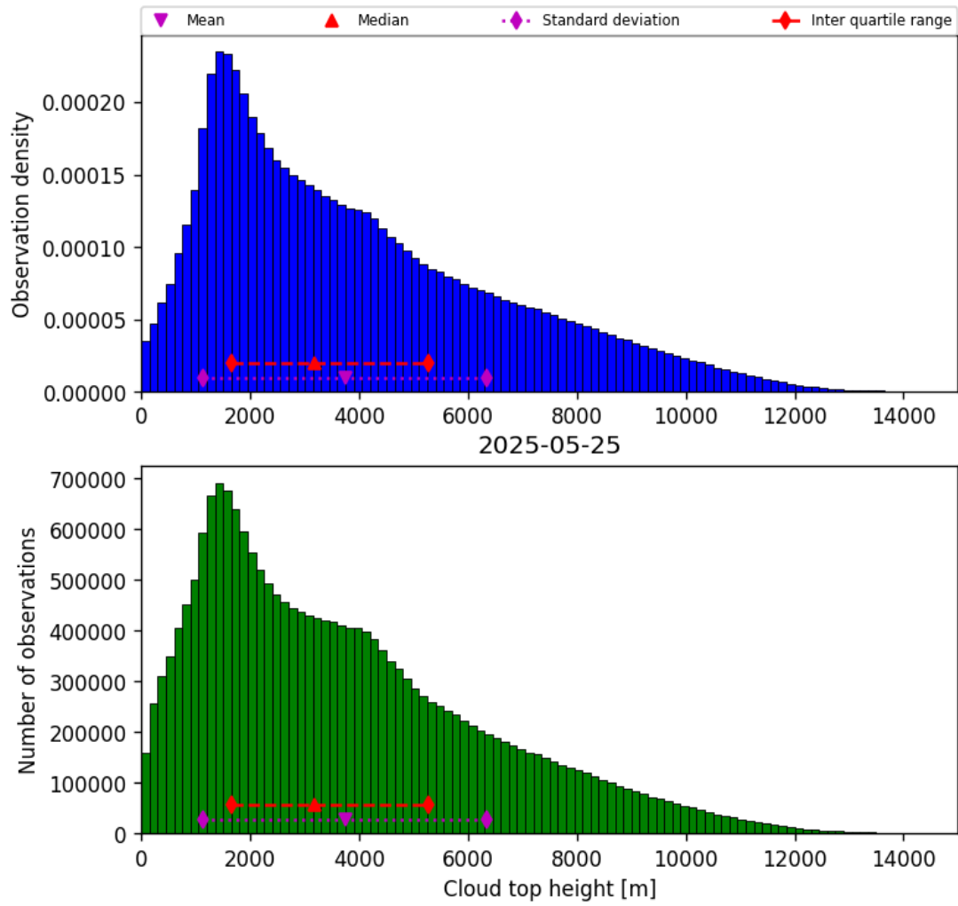
Figure 38: Histogram of “Cloud top height” for 2025-05-25 to 2025-05-26
