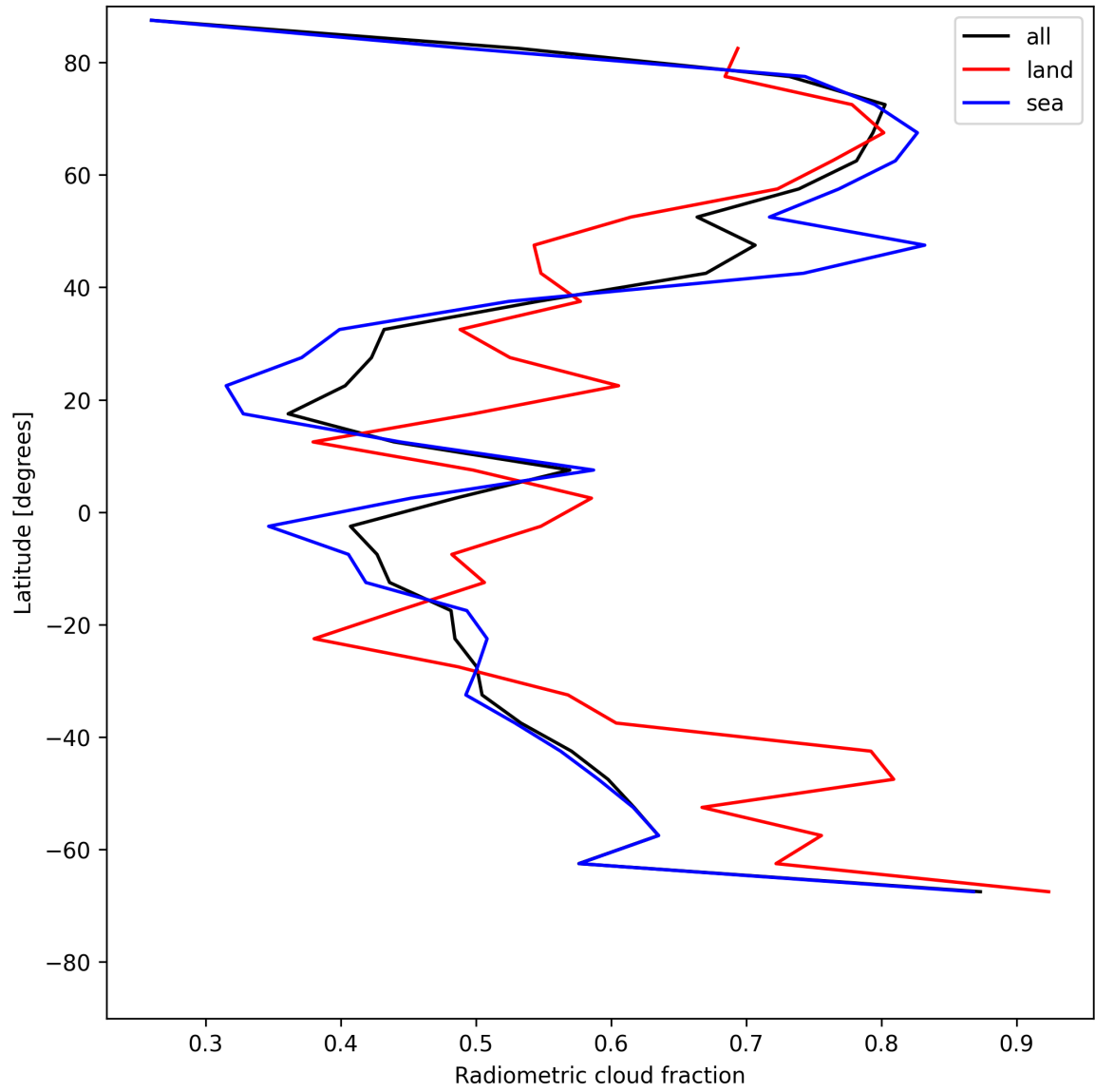
Figure 21: Zonal average of “Radiometric cloud fraction” for 2025-05-25 to 2025-05-26.
