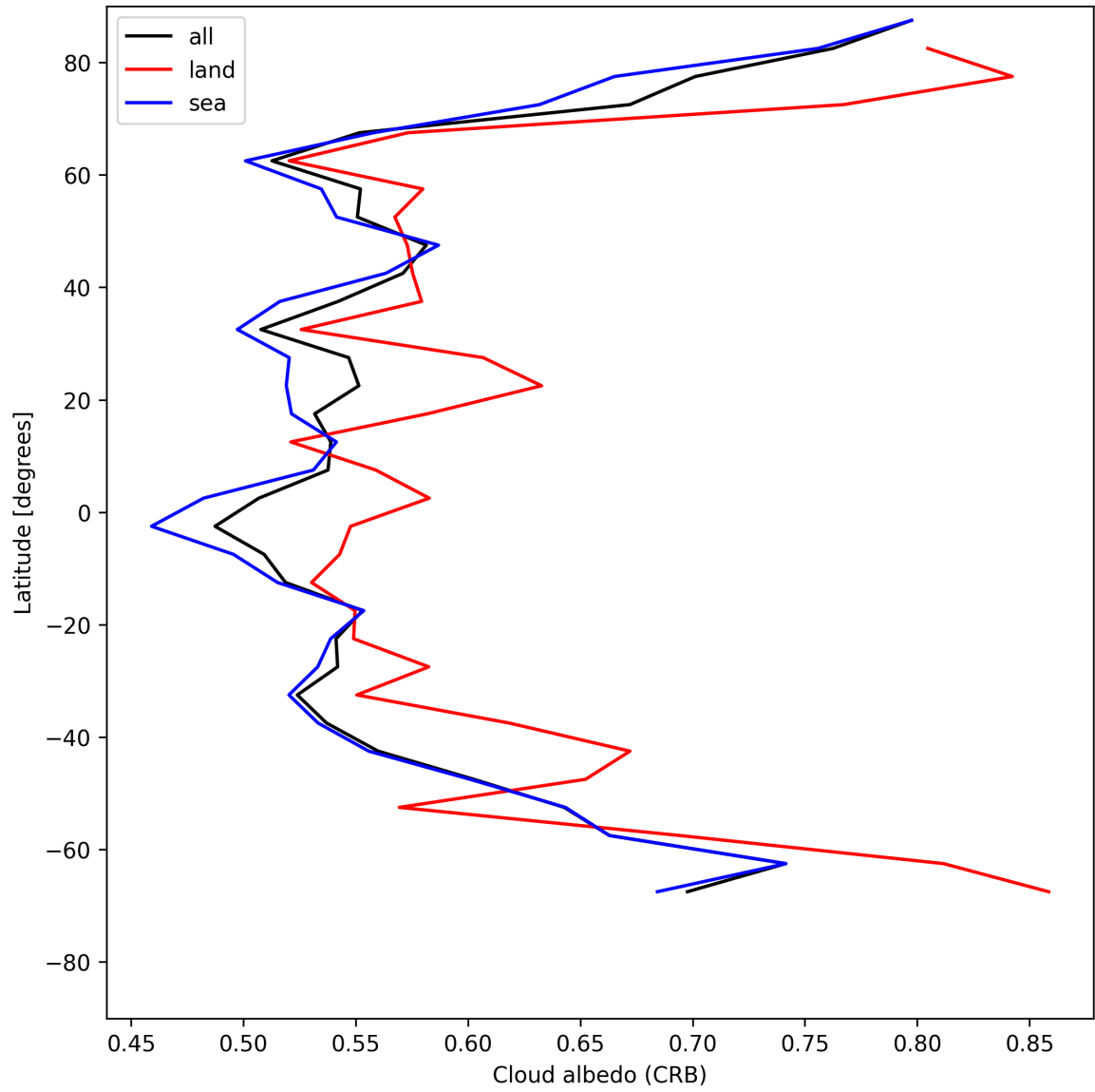
Figure 26: Zonal average of “Cloud albedo (CRB)” for 2025-05-25 to 2025-05-26.
