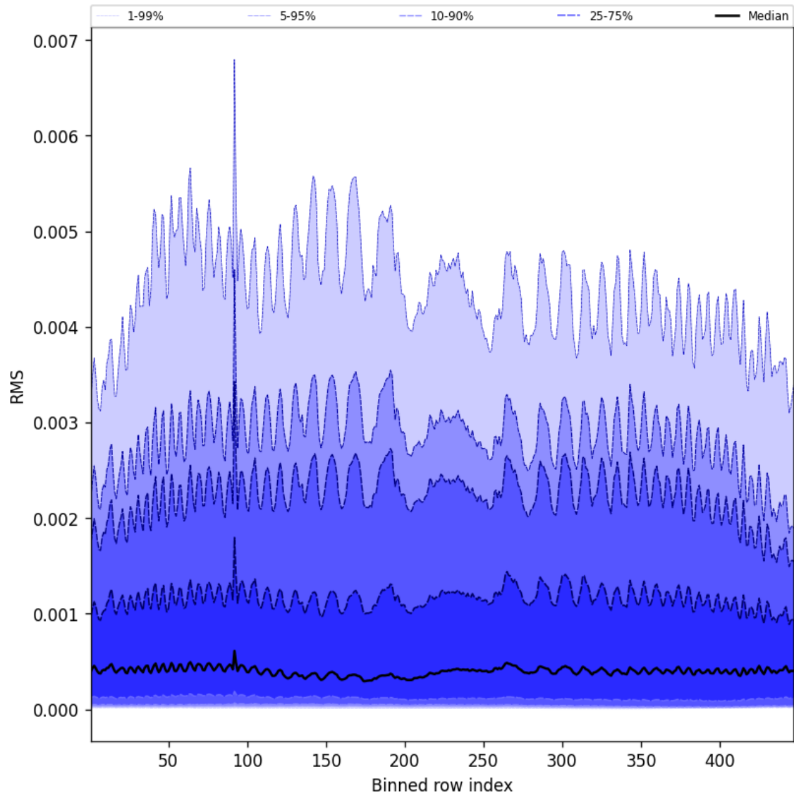
Figure 61: Along track statistics of “RMS” for 2025-05-25 to 2025-05-26
