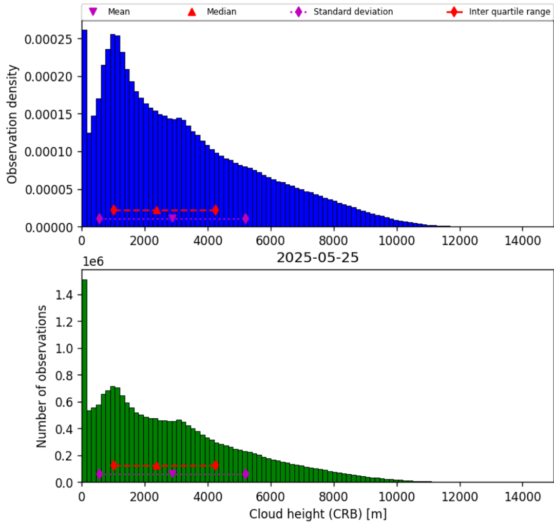
Figure 41: Histogram of “Cloud height (CRB)” for 2025-05-25 to 2025-05-26
