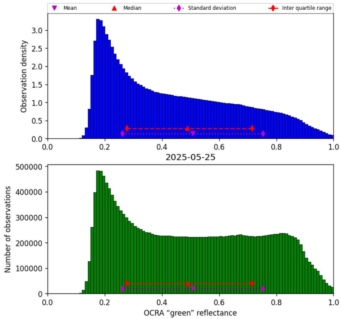
Figure 50: Histogram of “OCRA “green” reflectance” for 2025-05-25 to 2025-05-26
