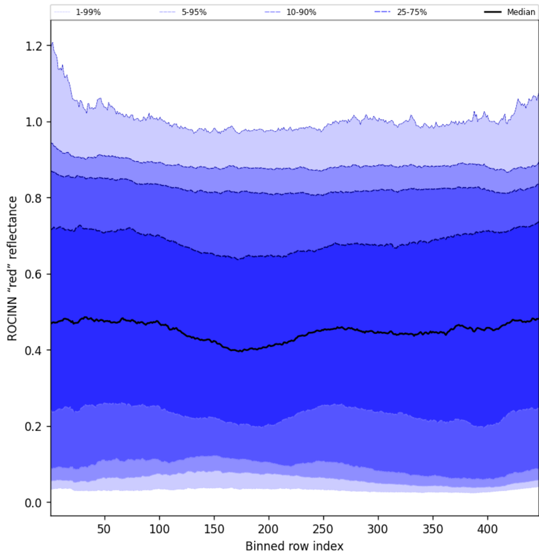
Figure 67: Along track statistics of "ROCINN "red" reflectance" for 2025-05-25 to 2025-05-26
