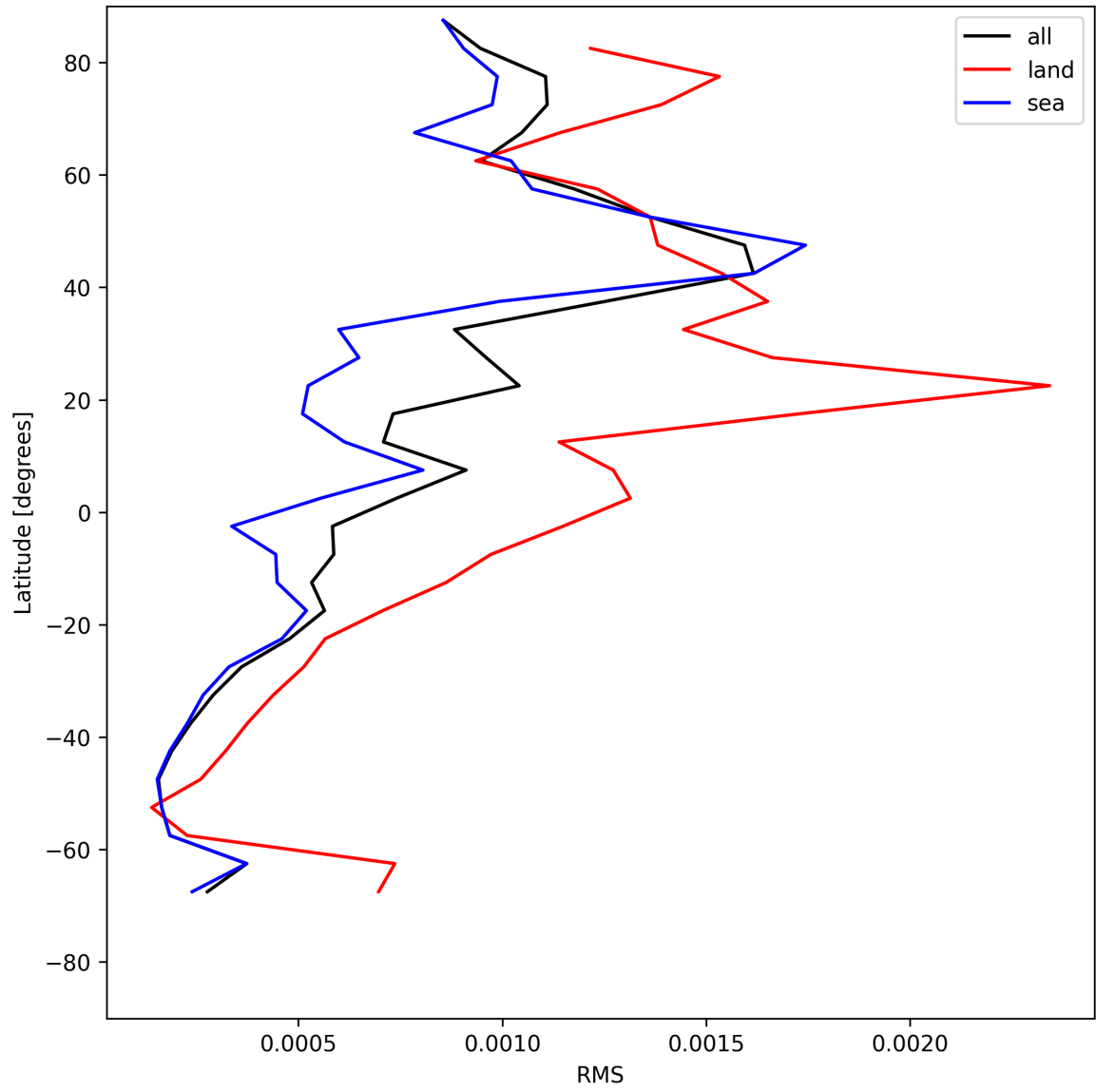
Figure 29: Zonal average of “RMS” for 2025-05-25 to 2025-05-26.
