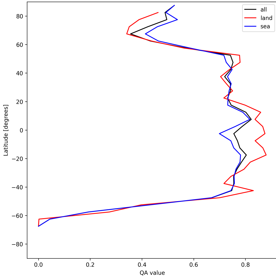
Figure 20: Zonal average of “QA value” for 2025-05-25 to 2025-05-26.
