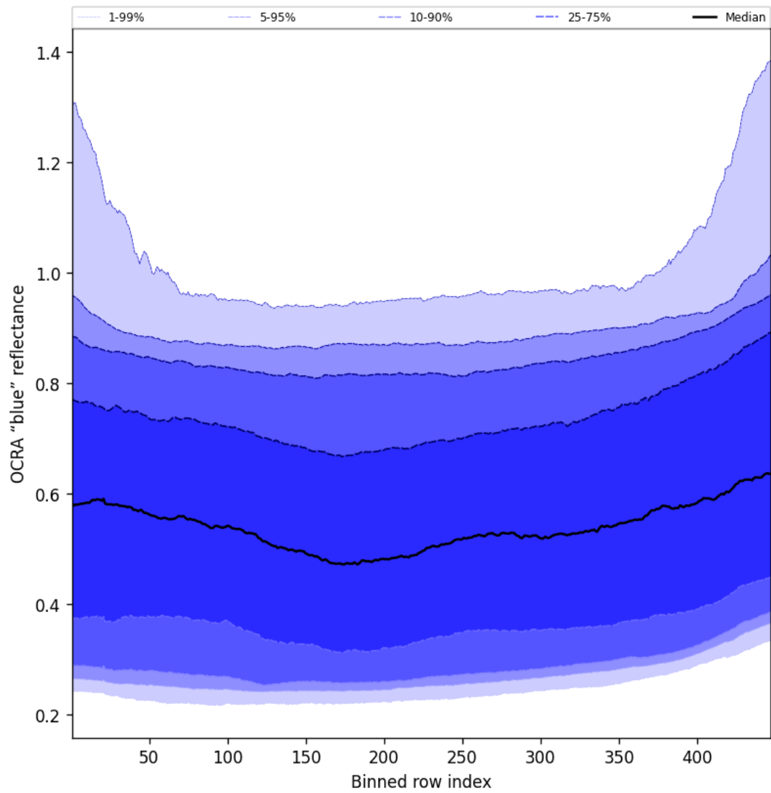
Figure 65: Along track statistics of “OCRA “blue” reflectance” for 2025-05-25 to 2025-05-26
