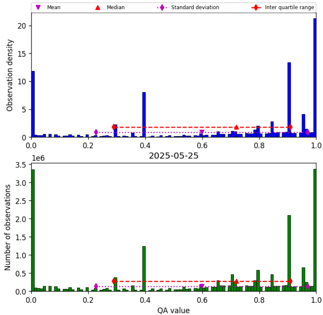
Figure 36: Histogram of “QA value” for 2025-05-25 to 2025-05-26
