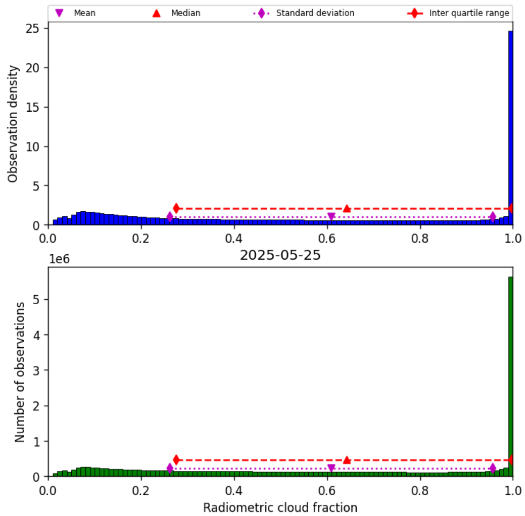
Figure 37: Histogram of “Radiometric cloud fraction” for 2025-05-25 to 2025-05-26
