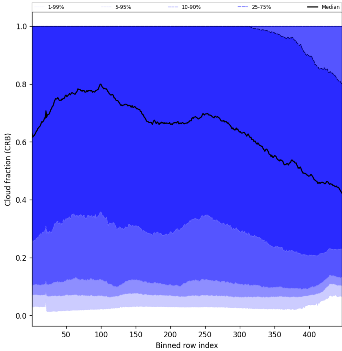
Figure 56: Along track statistics of “Cloud fraction (CRB)” for 2025-05-25 to 2025-05-26
