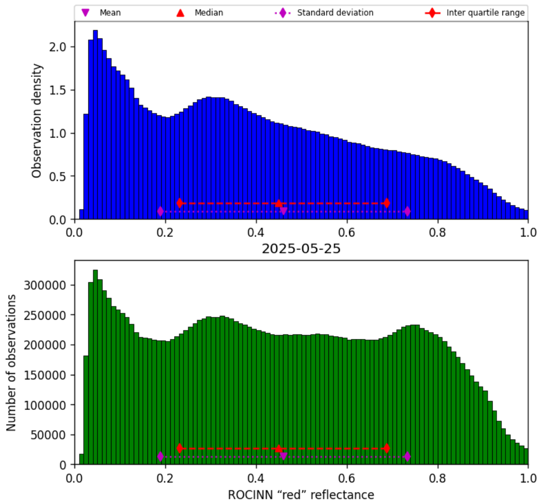
Figure 51: Histogram of “ROCINN “red” reflectance” for 2025-05-25 to 2025-05-26
