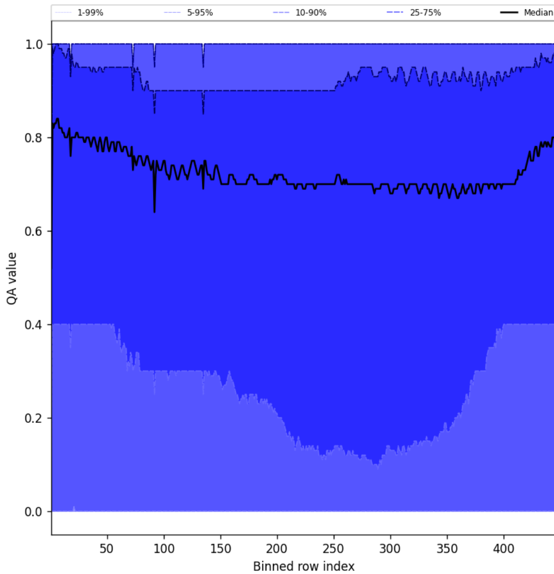
Figure 52: Along track statistics of “QA value” for 2025-05-25 to 2025-05-26
