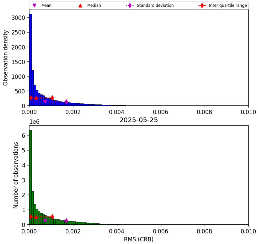
Figure 46: Histogram of "RMS (CRB)" for 2025-05-25 to 2025-05-26
