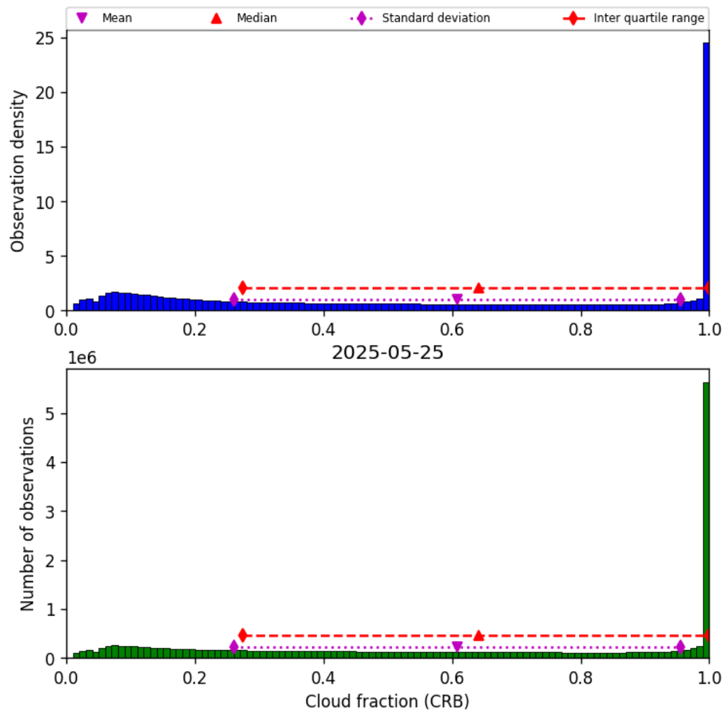
Figure 40: Histogram of “Cloud fraction (CRB)” for 2025-05-25 to 2025-05-26
