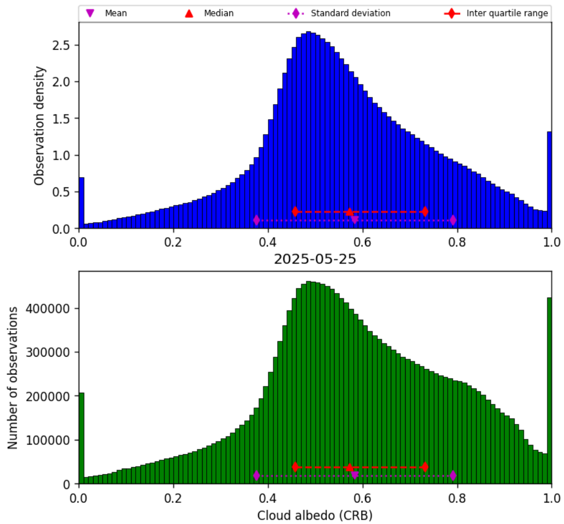
Figure 42: Histogram of “Cloud albedo (CRB)” for 2025-05-25 to 2025-05-26
