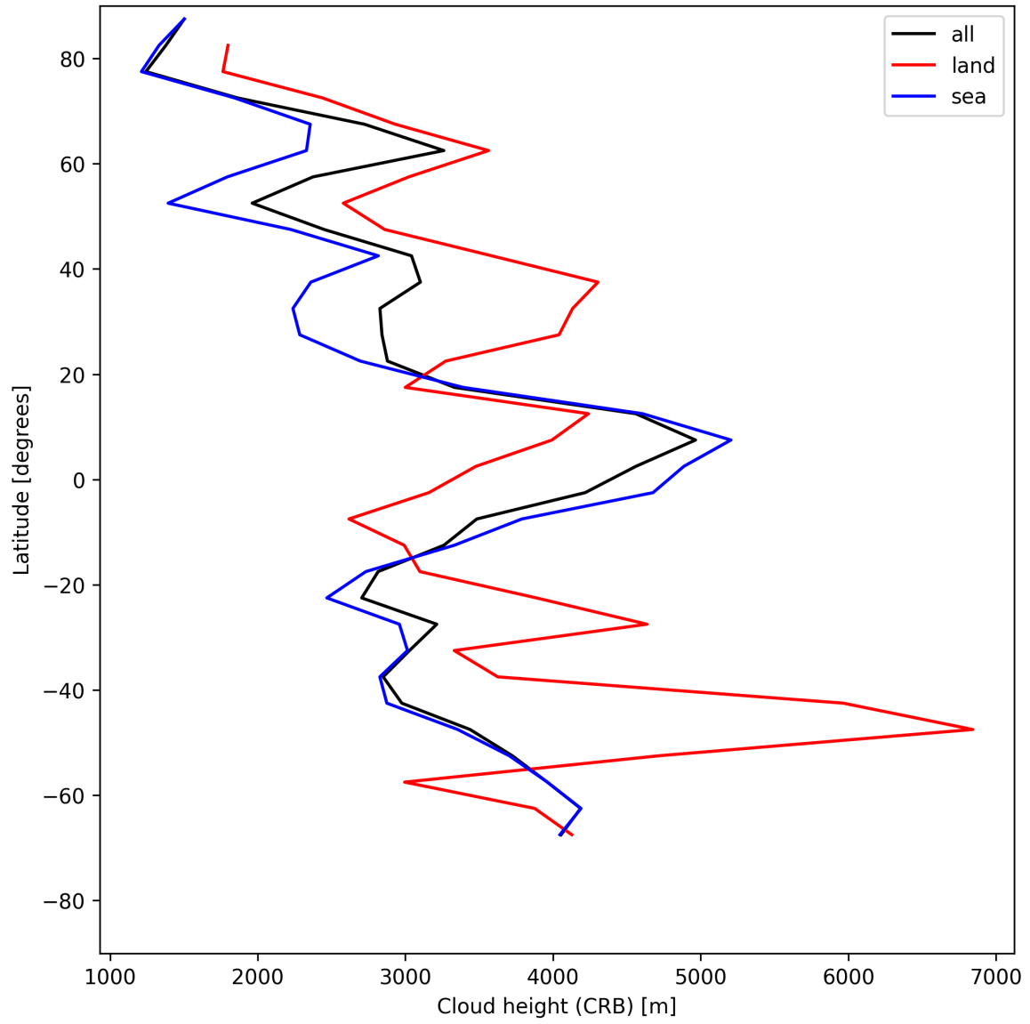
Figure 25: Zonal average of “Cloud height (CRB)” for 2025-05-25 to 2025-05-26.
