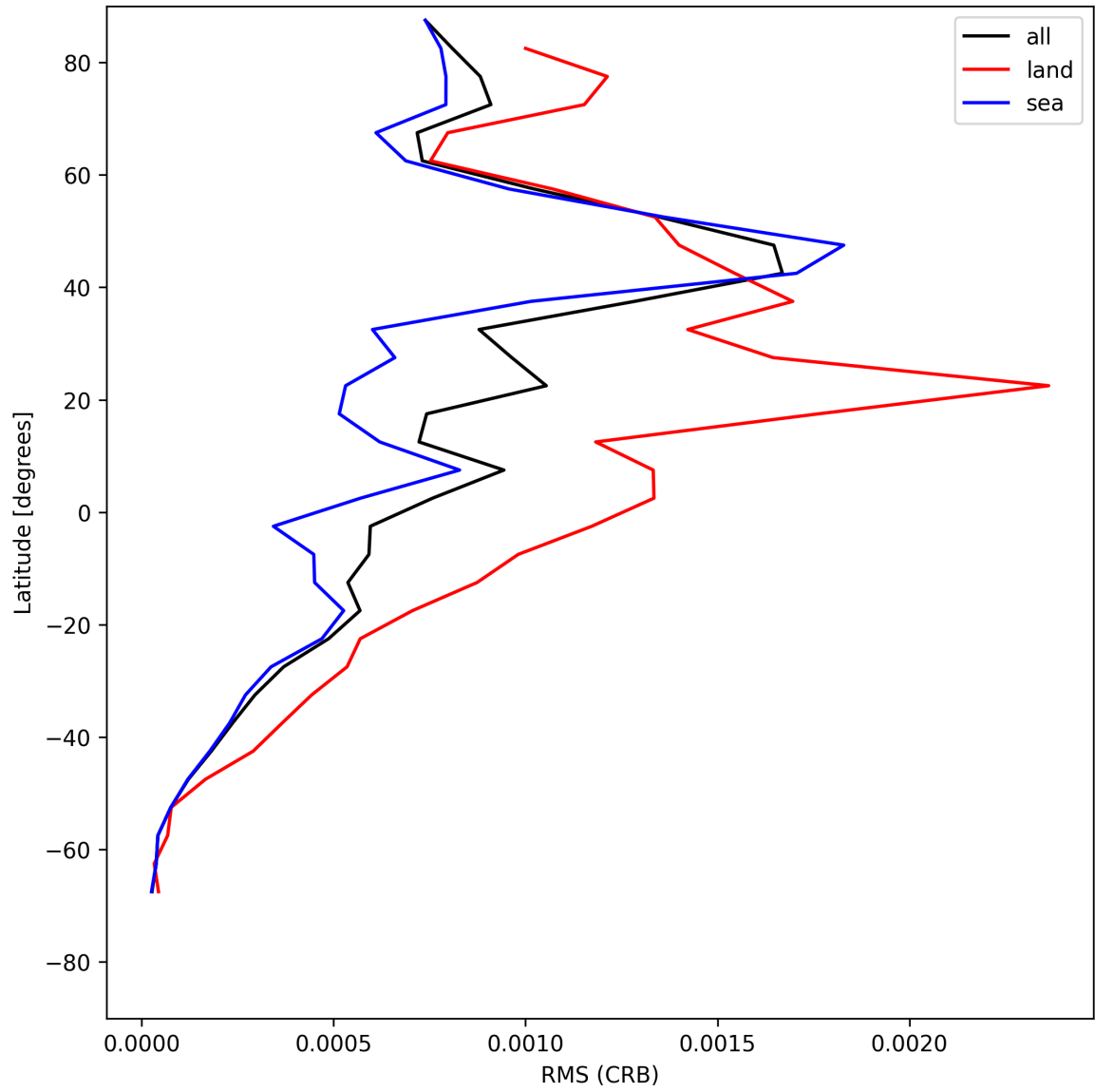
Figure 30: Zonal average of “RMS (CRB)” for 2025-05-25 to 2025-05-26.
