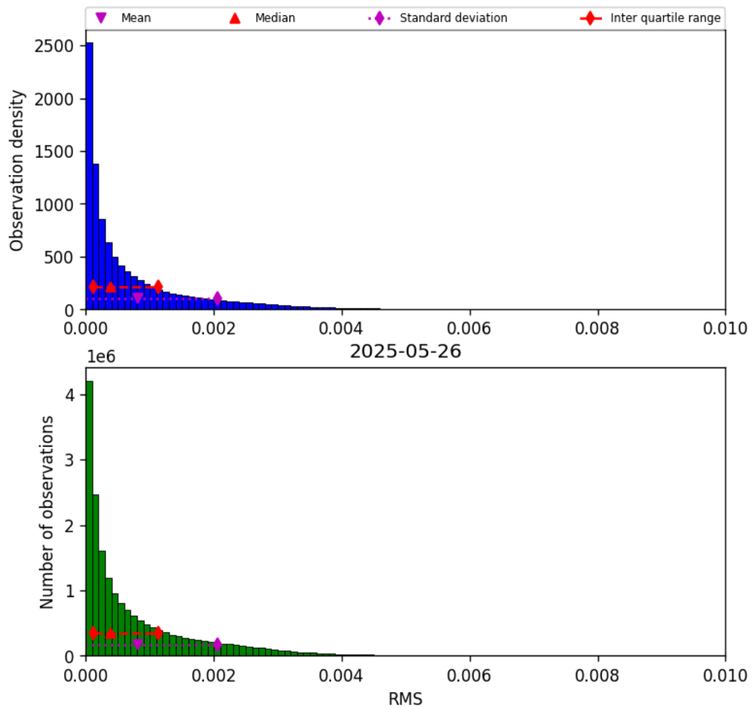
Figure 45: Histogram of “RMS” for 2025-05-26 to 2025-05-27
