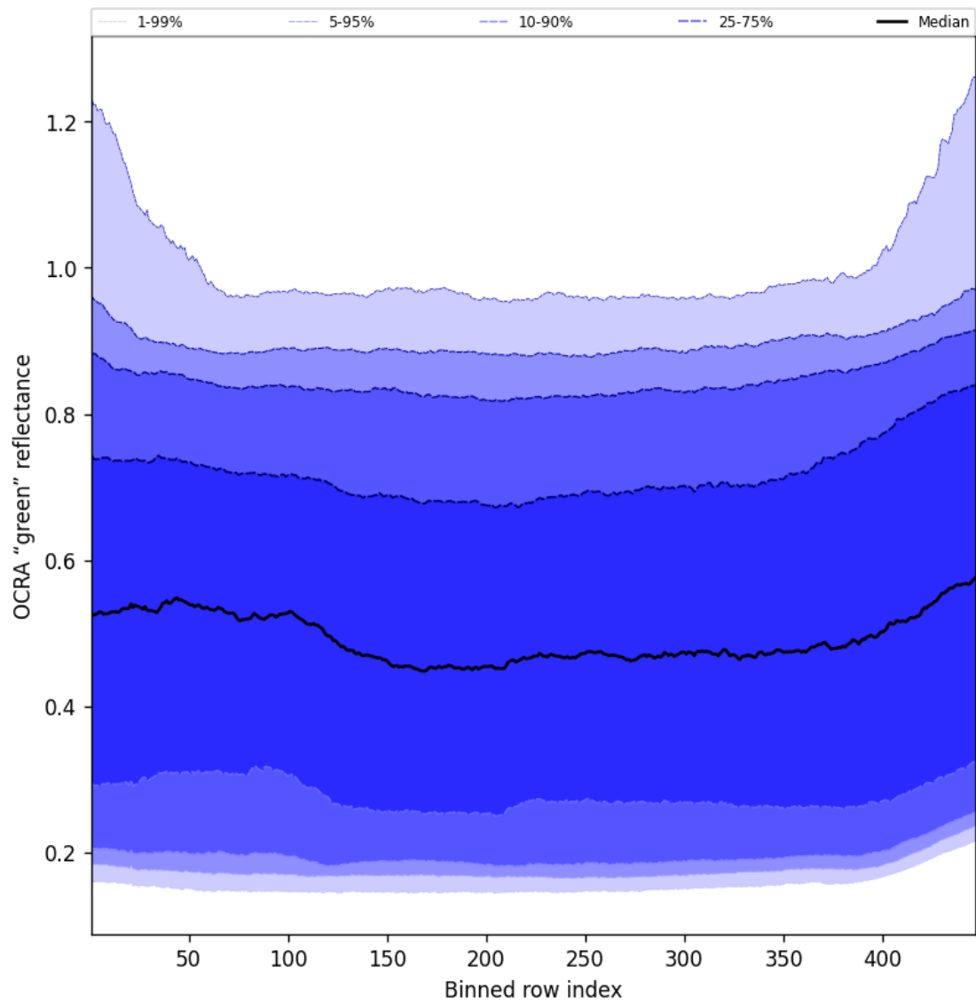
Figure 66: Along track statistics of “OCRA “green” reflectance” for 2025-05-26 to 2025-05-27
