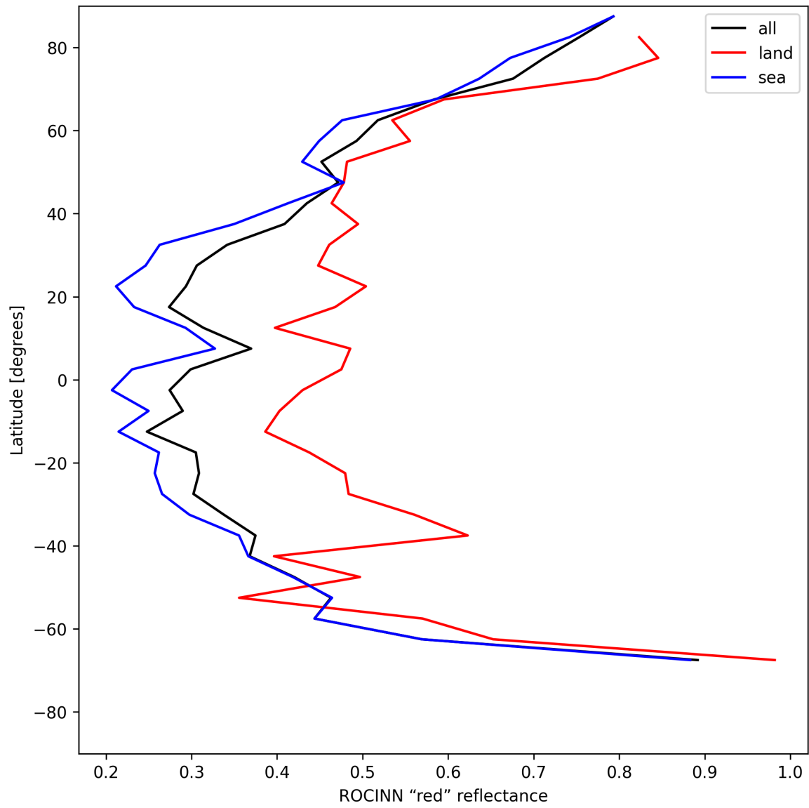
Figure 35: Zonal average of "ROCINN "red" reflectance" for 2025-05-26 to 2025-05-27.
