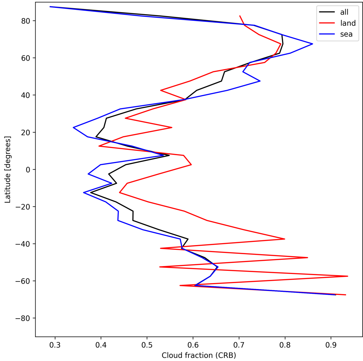
Figure 24: Zonal average of “Cloud fraction (CRB)” for 2025-05-26 to 2025-05-27.
