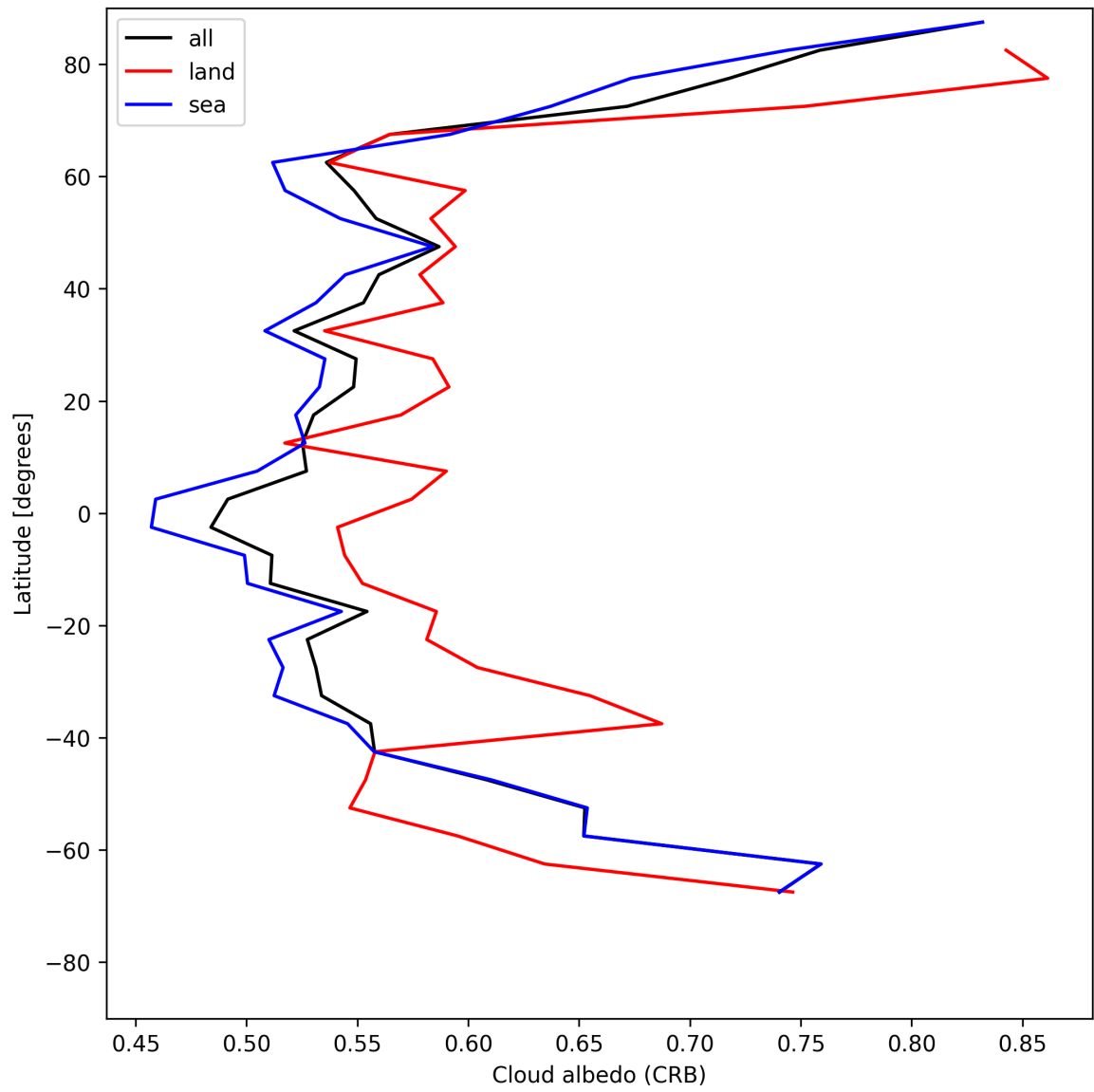
Figure 26: Zonal average of “Cloud albedo (CRB)” for 2025-05-26 to 2025-05-27.
