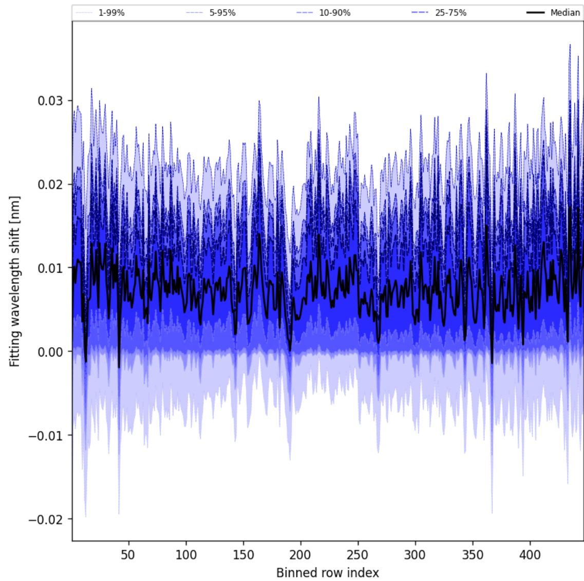
Figure 63: Along track statistics of “Fitting wavelength shift” for 2025-05-26 to 2025-05-27
