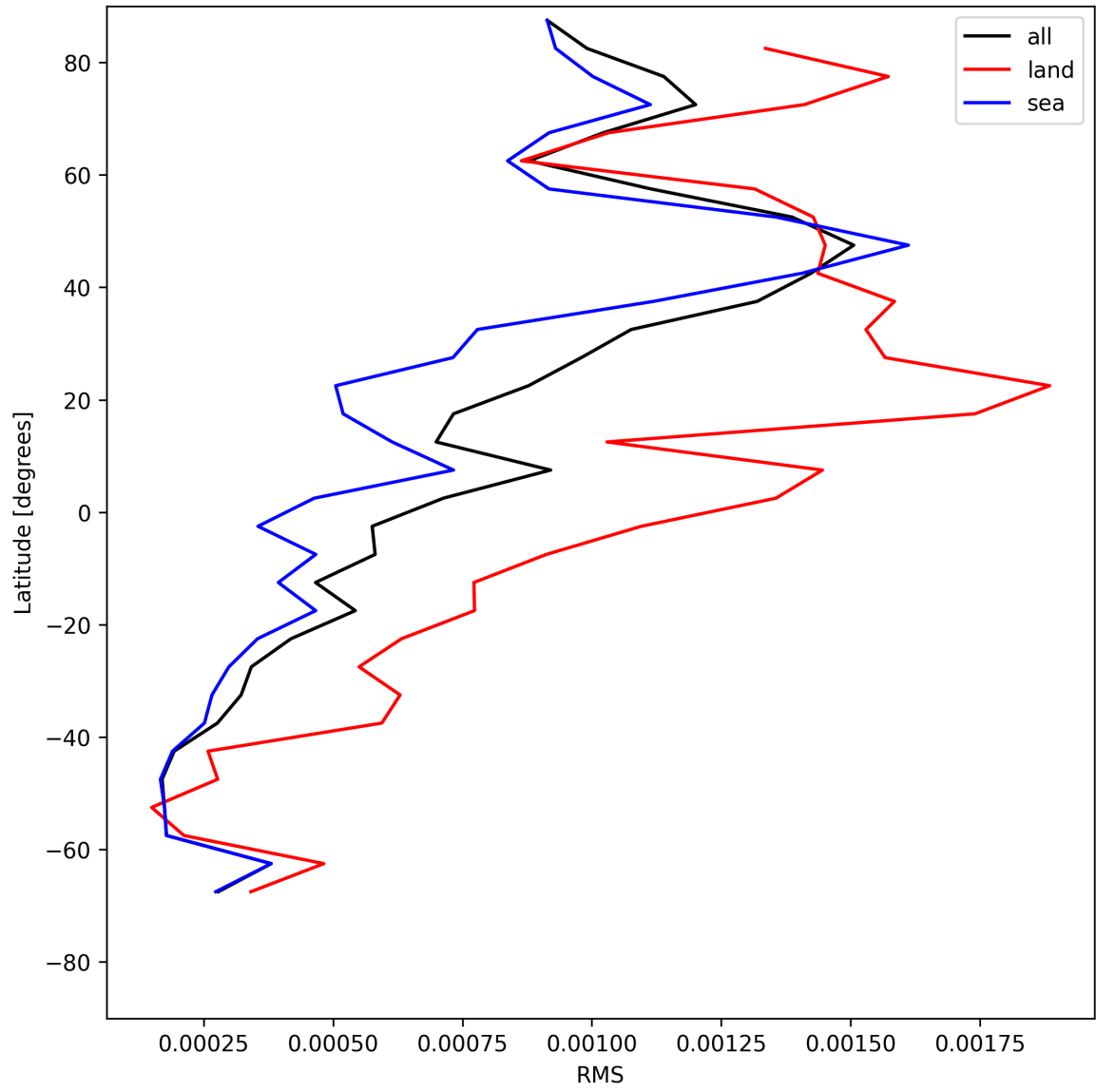
Figure 29: Zonal average of “RMS” for 2025-05-26 to 2025-05-27.
