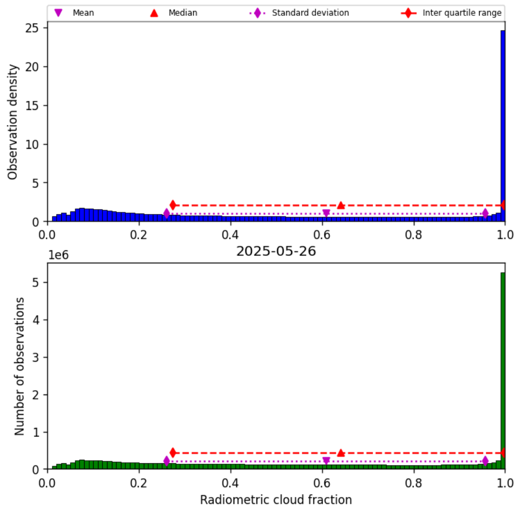
Figure 37: Histogram of “Radiometric cloud fraction” for 2025-05-26 to 2025-05-27
