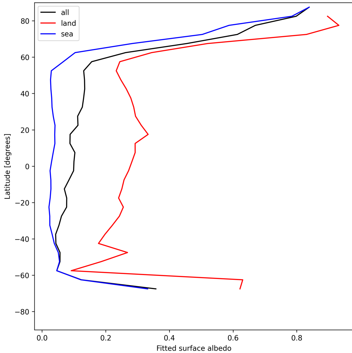
Figure 27: Zonal average of “Fitted surface albedo” for 2025-05-26 to 2025-05-27.
