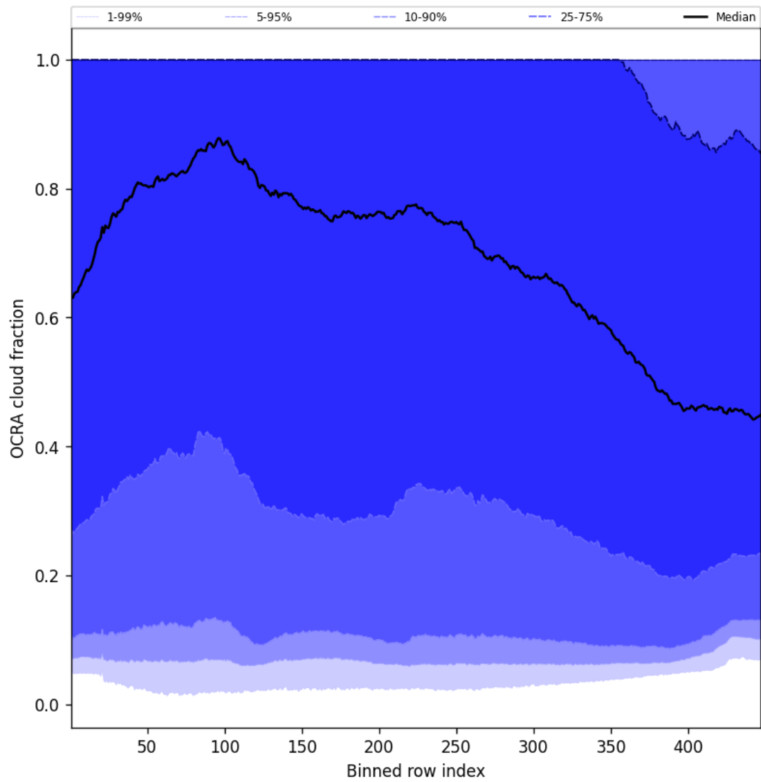
Figure 64: Along track statistics of “OCRA cloud fraction” for 2025-05-26 to 2025-05-27
