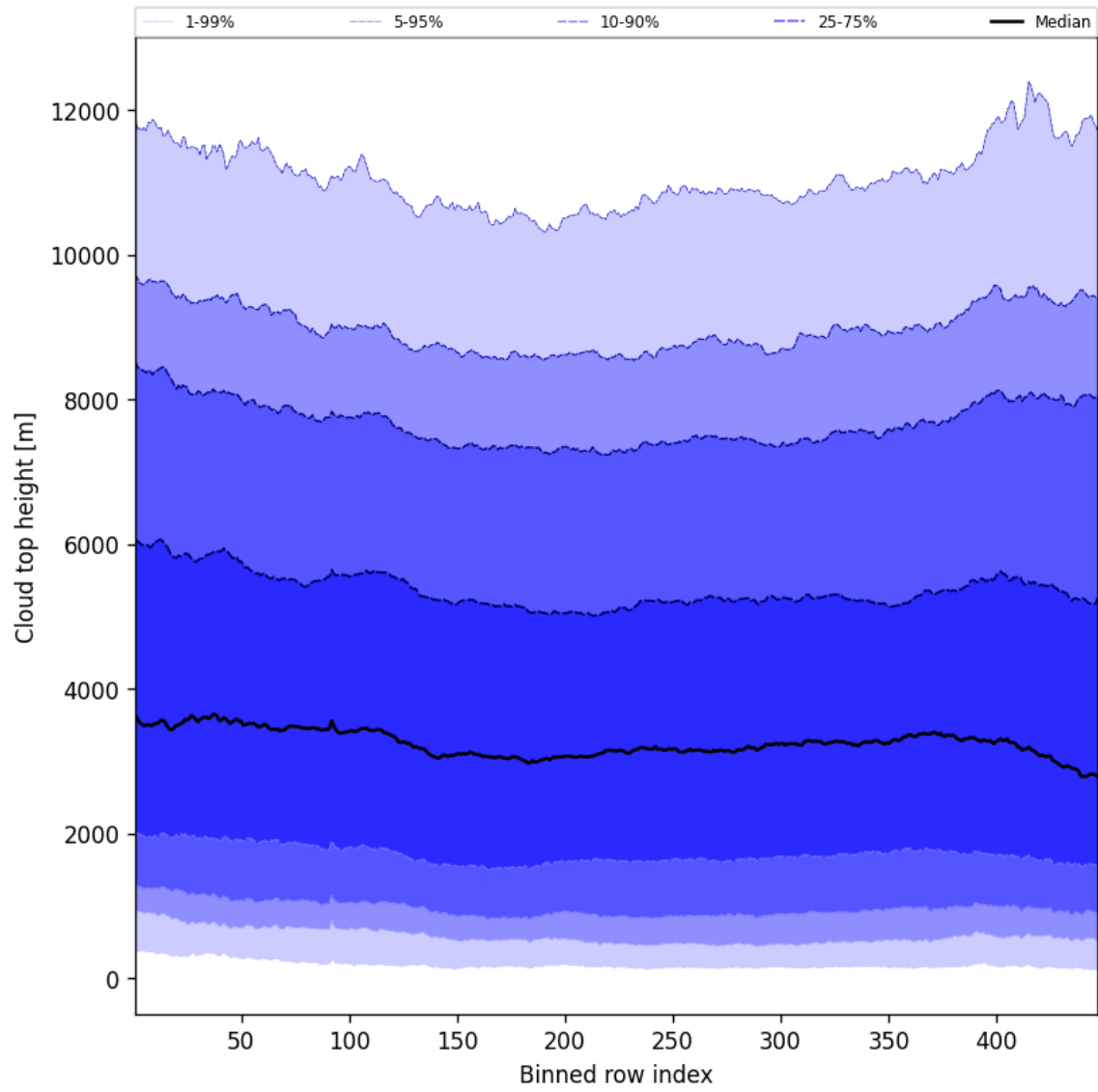
Figure 54: Along track statistics of “Cloud top height” for 2025-05-26 to 2025-05-27
