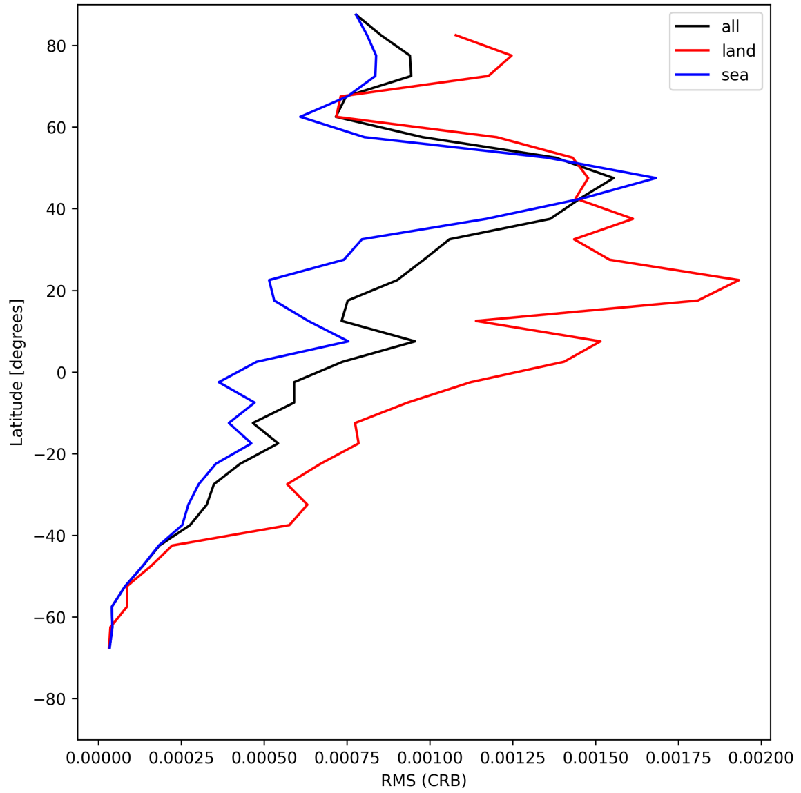
Figure 30: Zonal average of “RMS (CRB)” for 2025-05-26 to 2025-05-27.
