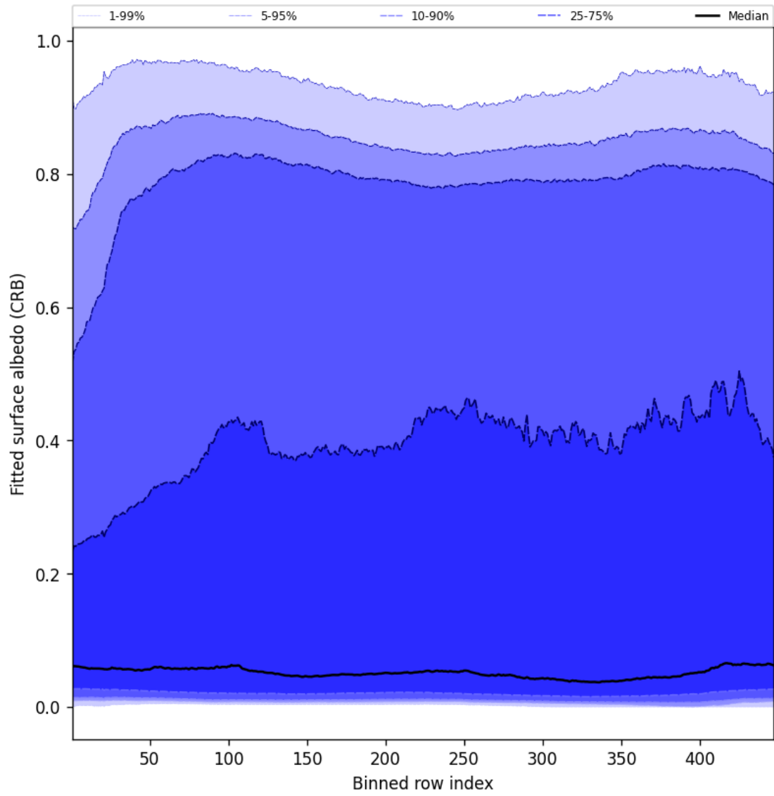
Figure 60: Along track statistics of “Fitted surface albedo (CRB)” for 2025-05-26 to 2025-05-27
