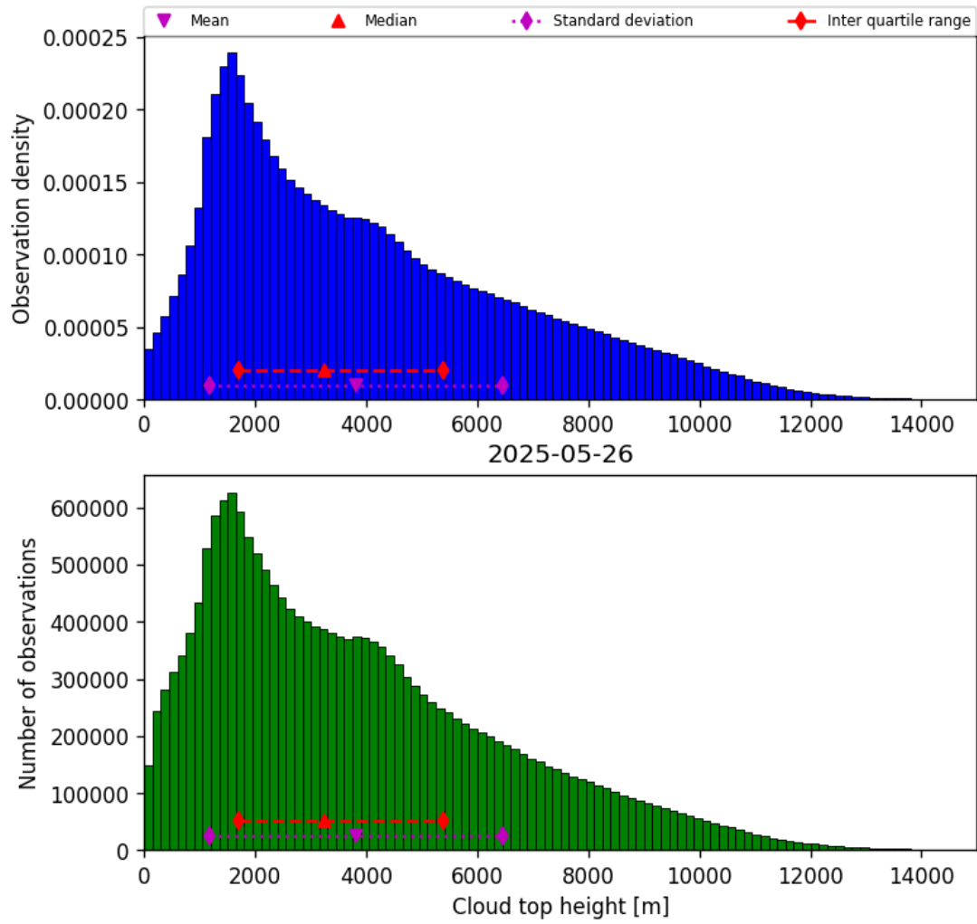
Figure 38: Histogram of “Cloud top height” for 2025-05-26 to 2025-05-27
