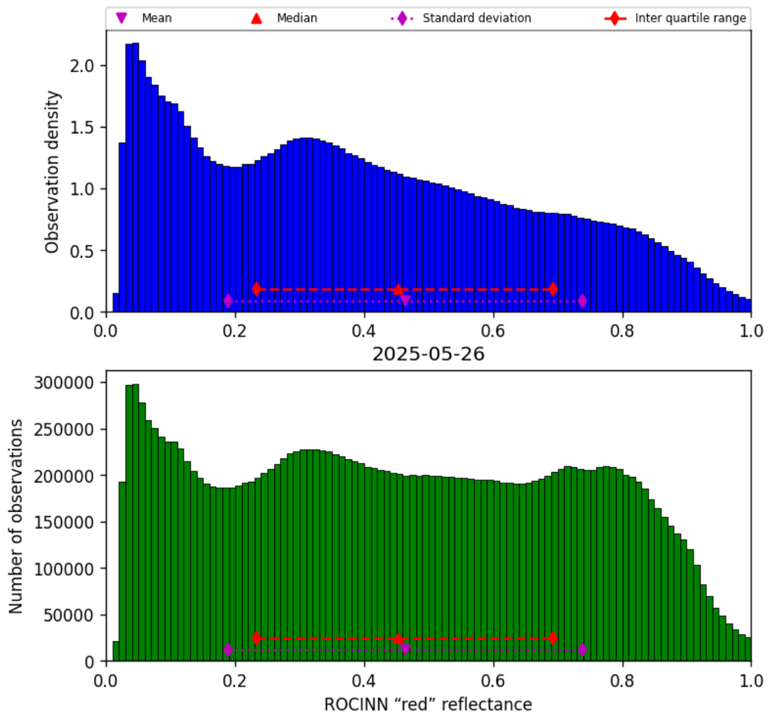
Figure 51: Histogram of “ROCINN “red” reflectance” for 2025-05-26 to 2025-05-27
