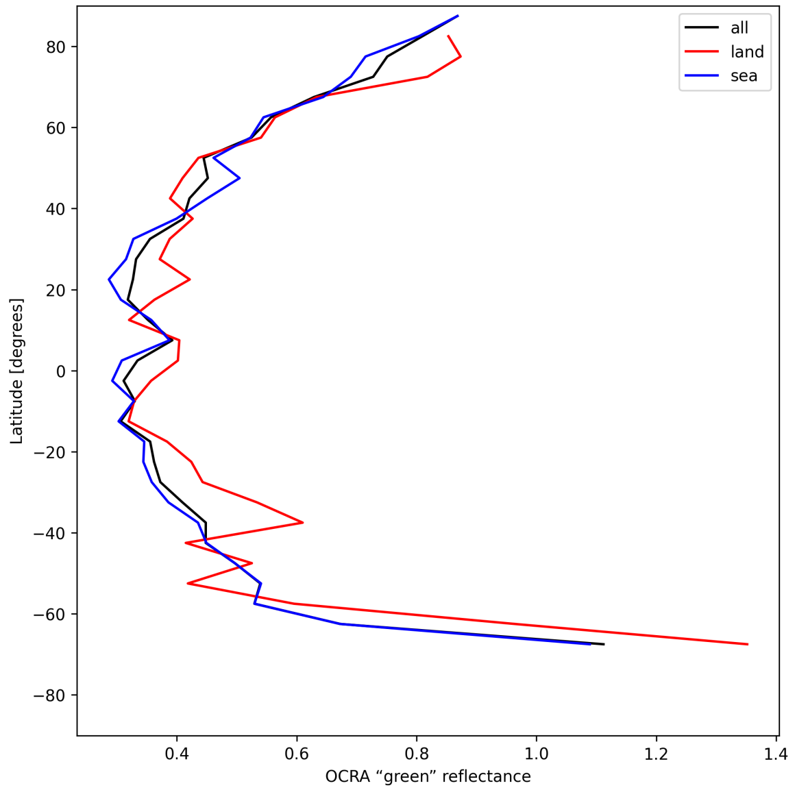
Figure 34: Zonal average of “OCRA “green” reflectance” for 2025-05-26 to 2025-05-27.
