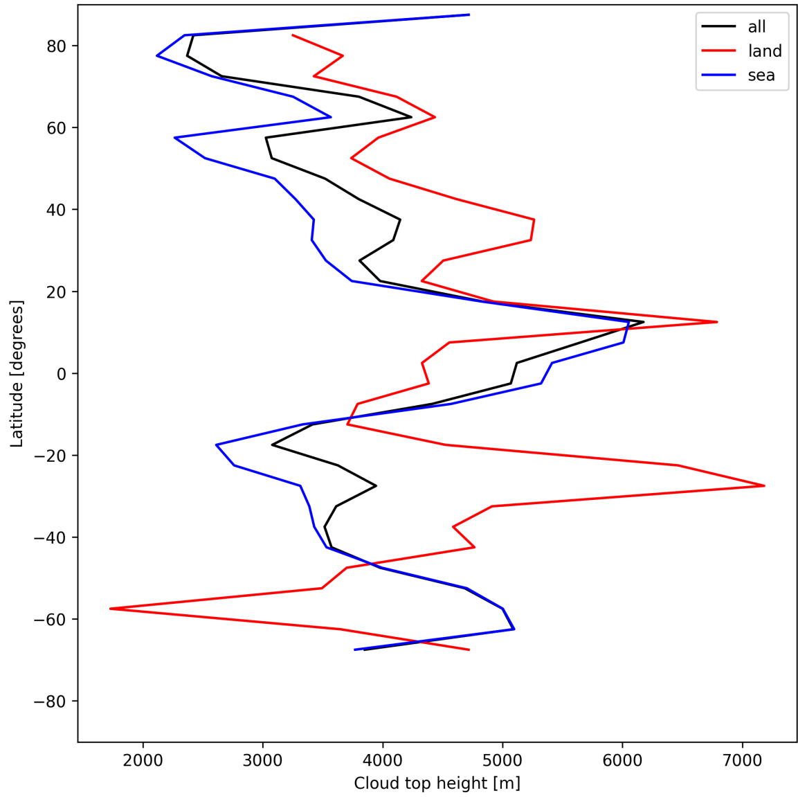
Figure 22: Zonal average of “Cloud top height” for 2025-05-26 to 2025-05-27.
