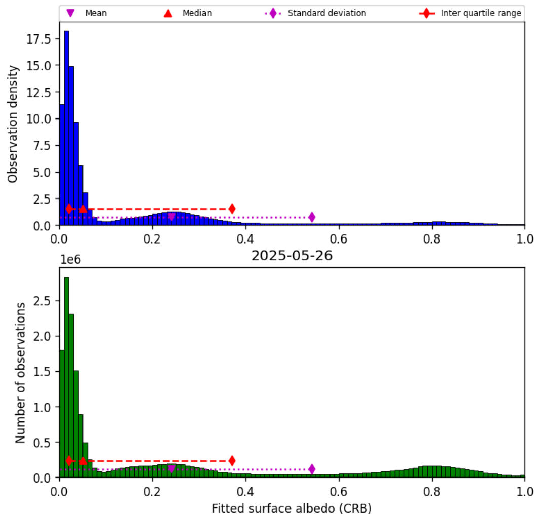
Figure 44: Histogram of “Fitted surface albedo (CRB)” for 2025-05-26 to 2025-05-27
