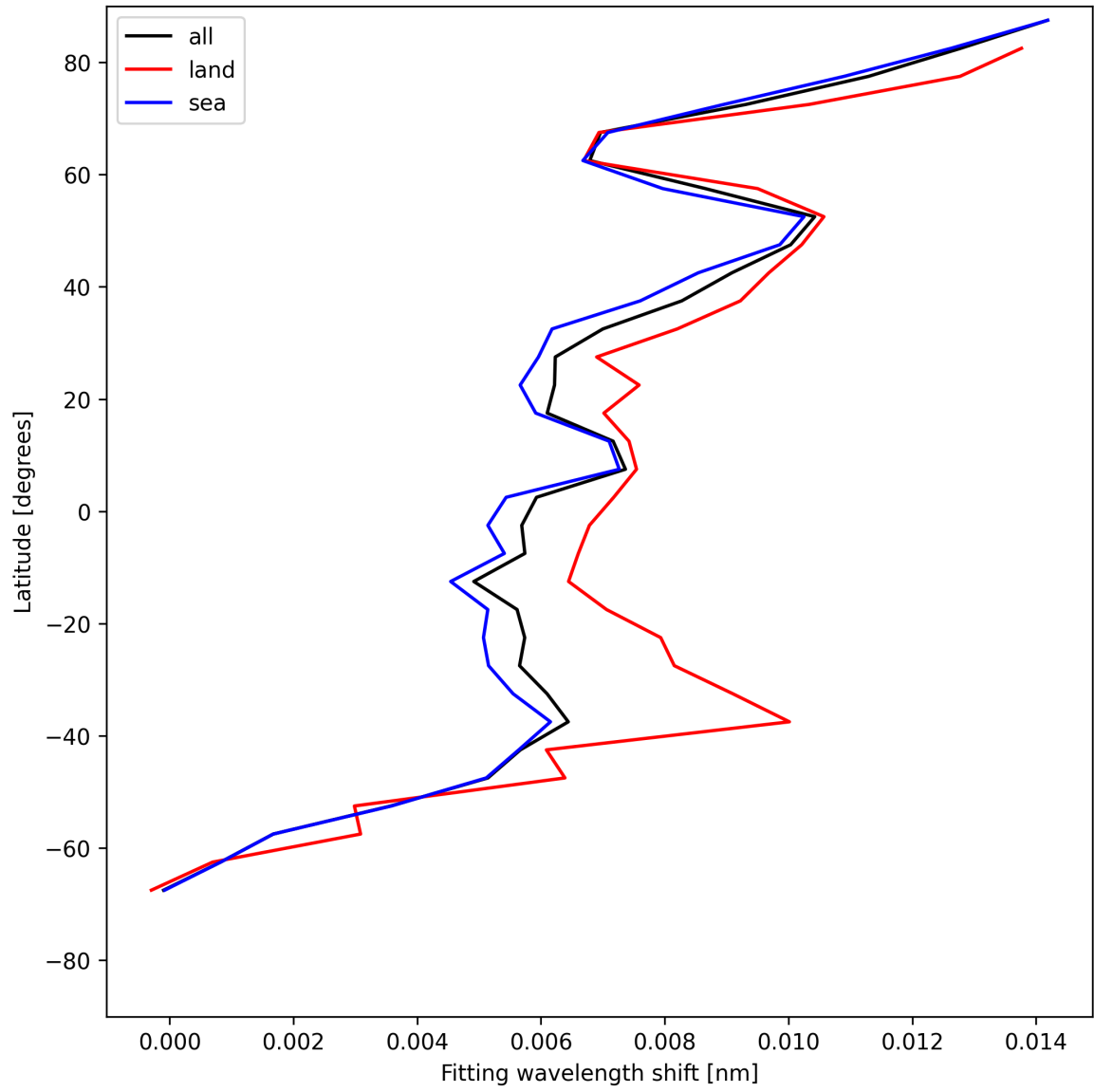
Figure 31: Zonal average of “Fitting wavelength shift” for 2025-05-26 to 2025-05-27.
