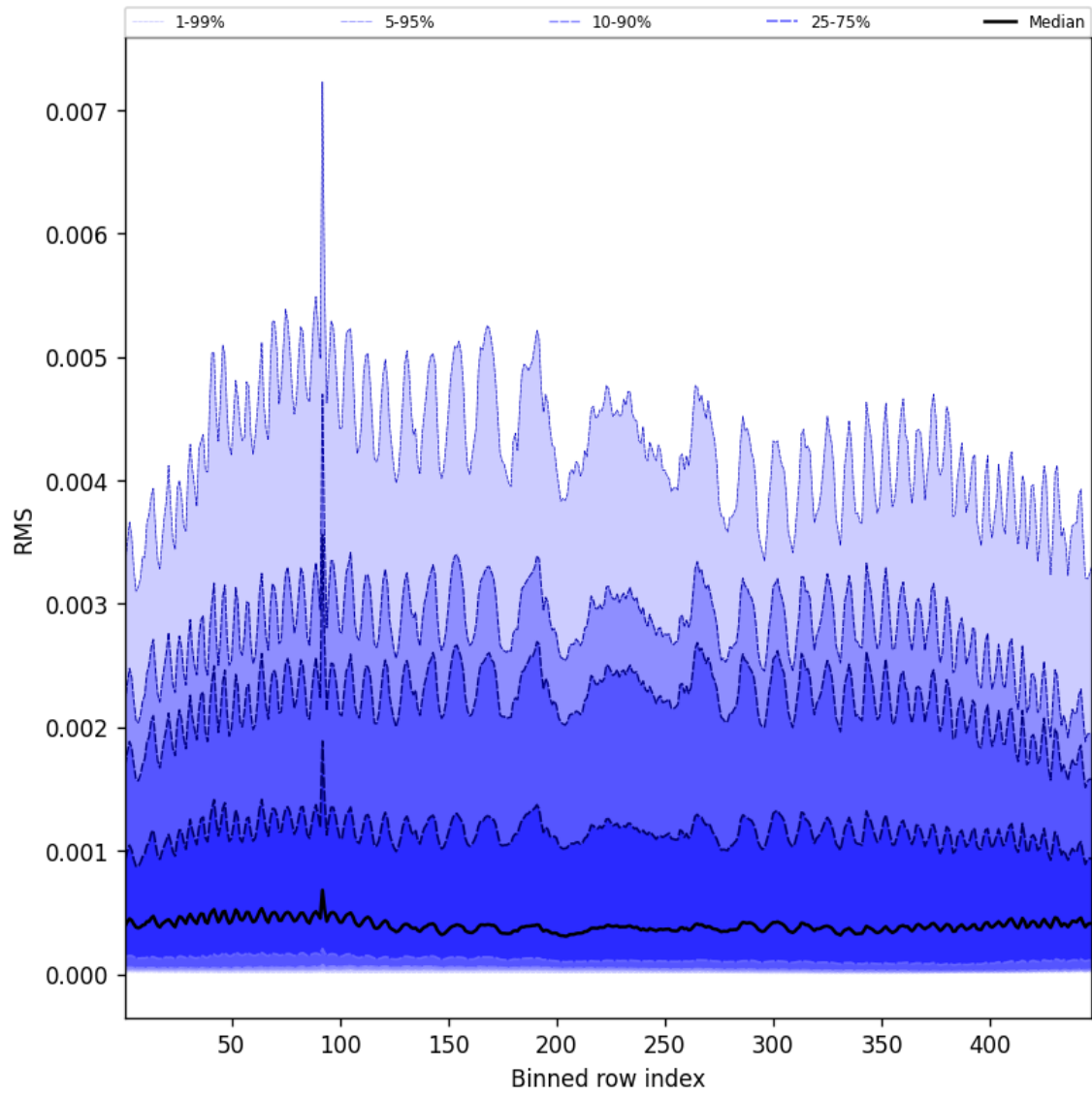
Figure 61: Along track statistics of “RMS” for 2025-05-26 to 2025-05-27
