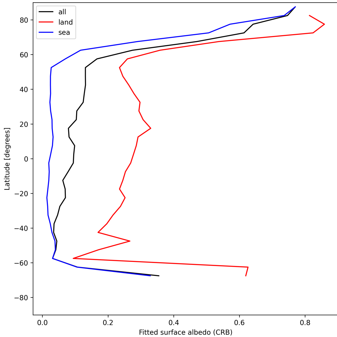
Figure 28: Zonal average of “Fitted surface albedo (CRB)” for 2025-05-26 to 2025-05-27.
