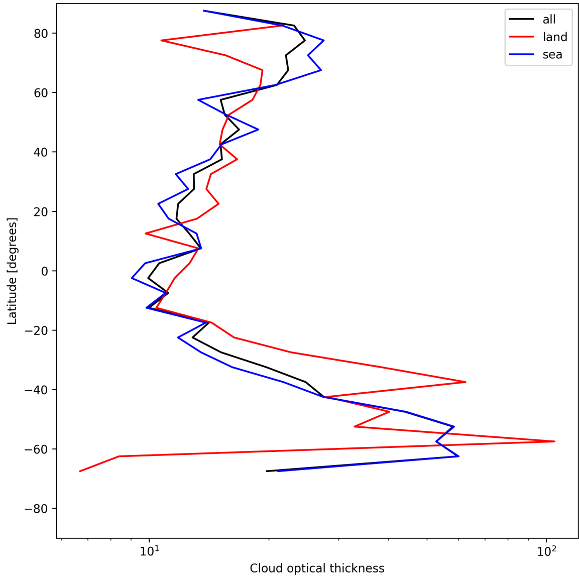
Figure 23: Zonal average of “Cloud optical thickness” for 2025-05-26 to 2025-05-27.
