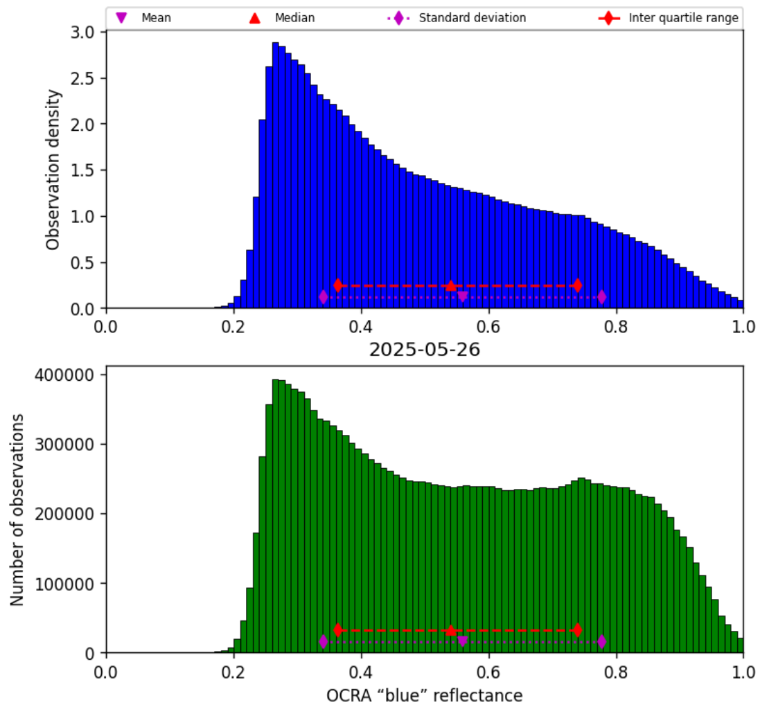
Figure 49: Histogram of “OCRA “blue” reflectance” for 2025-05-26 to 2025-05-27
