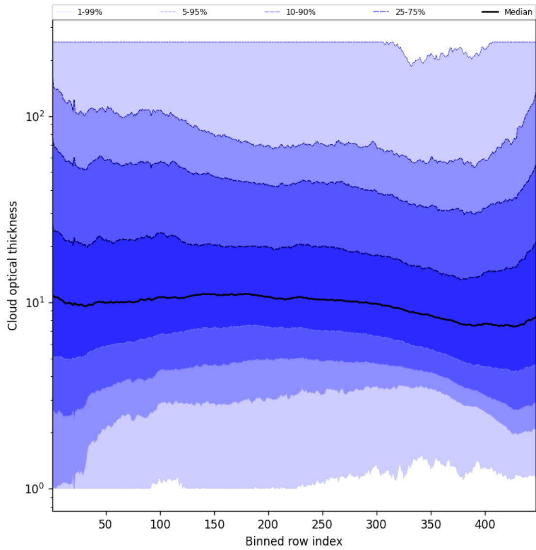
Figure 55: Along track statistics of “Cloud optical thickness” for 2025-05-26 to 2025-05-27
