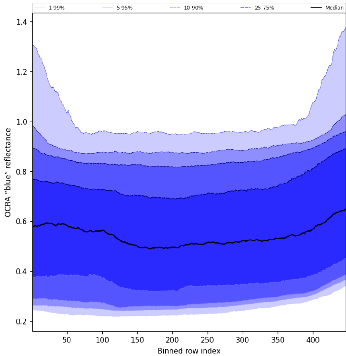
Figure 65: Along track statistics of “OCRA “blue” reflectance” for 2025-05-26 to 2025-05-27
