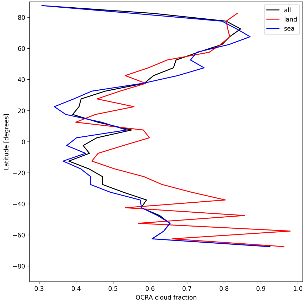
Figure 32: Zonal average of “OCRA cloud fraction” for 2025-05-26 to 2025-05-27.
