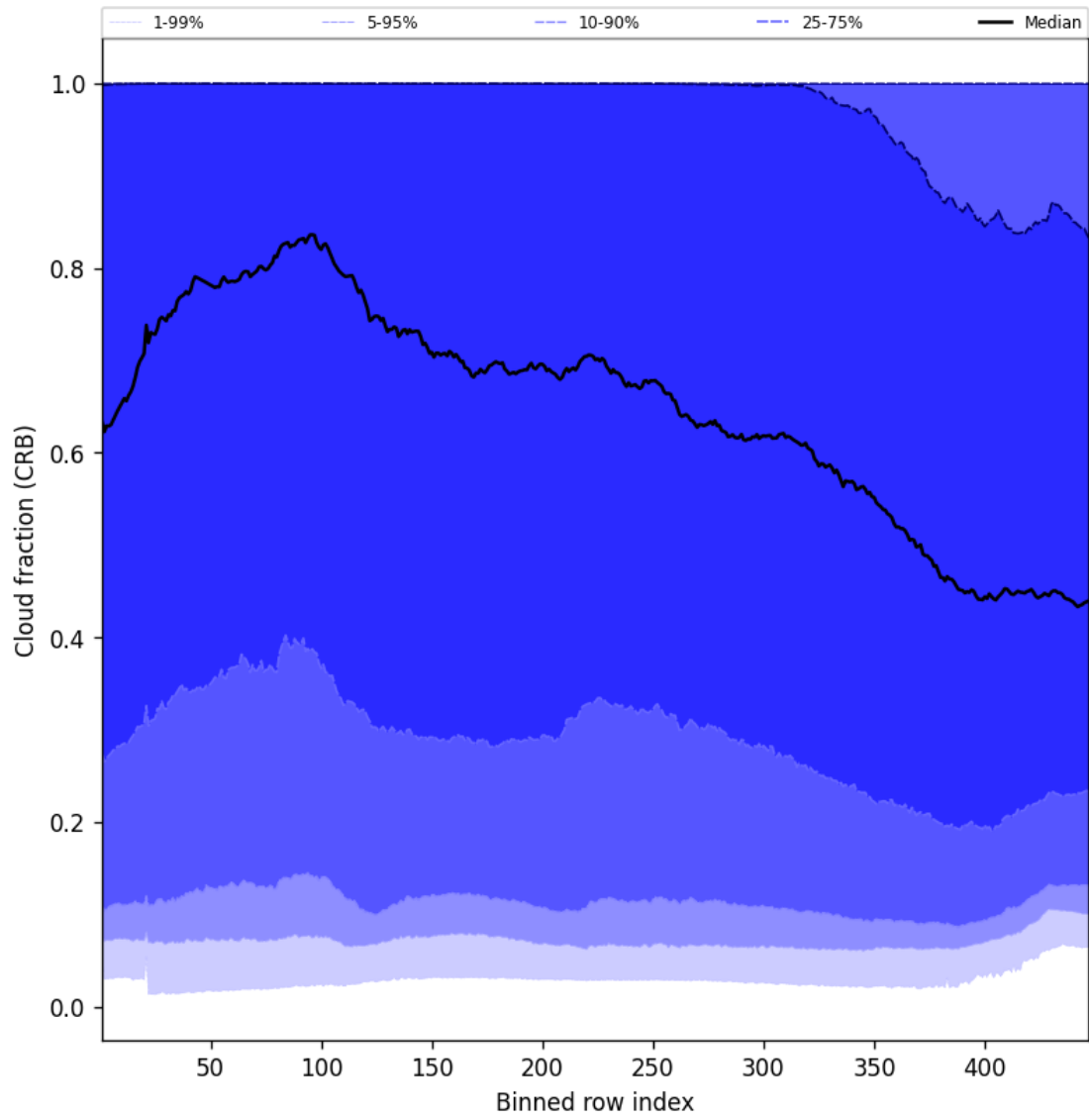
Figure 56: Along track statistics of “Cloud fraction (CRB)” for 2025-05-26 to 2025-05-27
