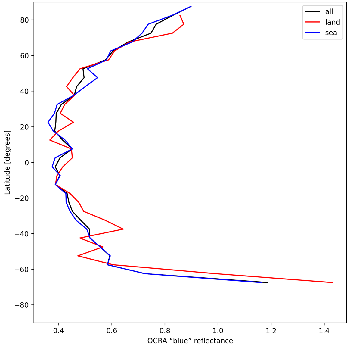
Figure 33: Zonal average of “OCRA “blue” reflectance” for 2025-05-26 to 2025-05-27.
