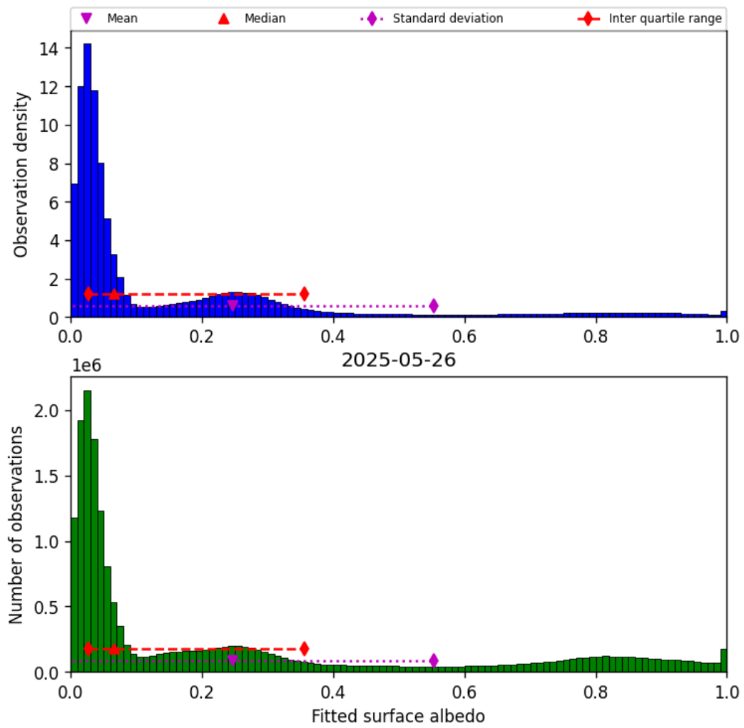
Figure 43: Histogram of “Fitted surface albedo” for 2025-05-26 to 2025-05-27
