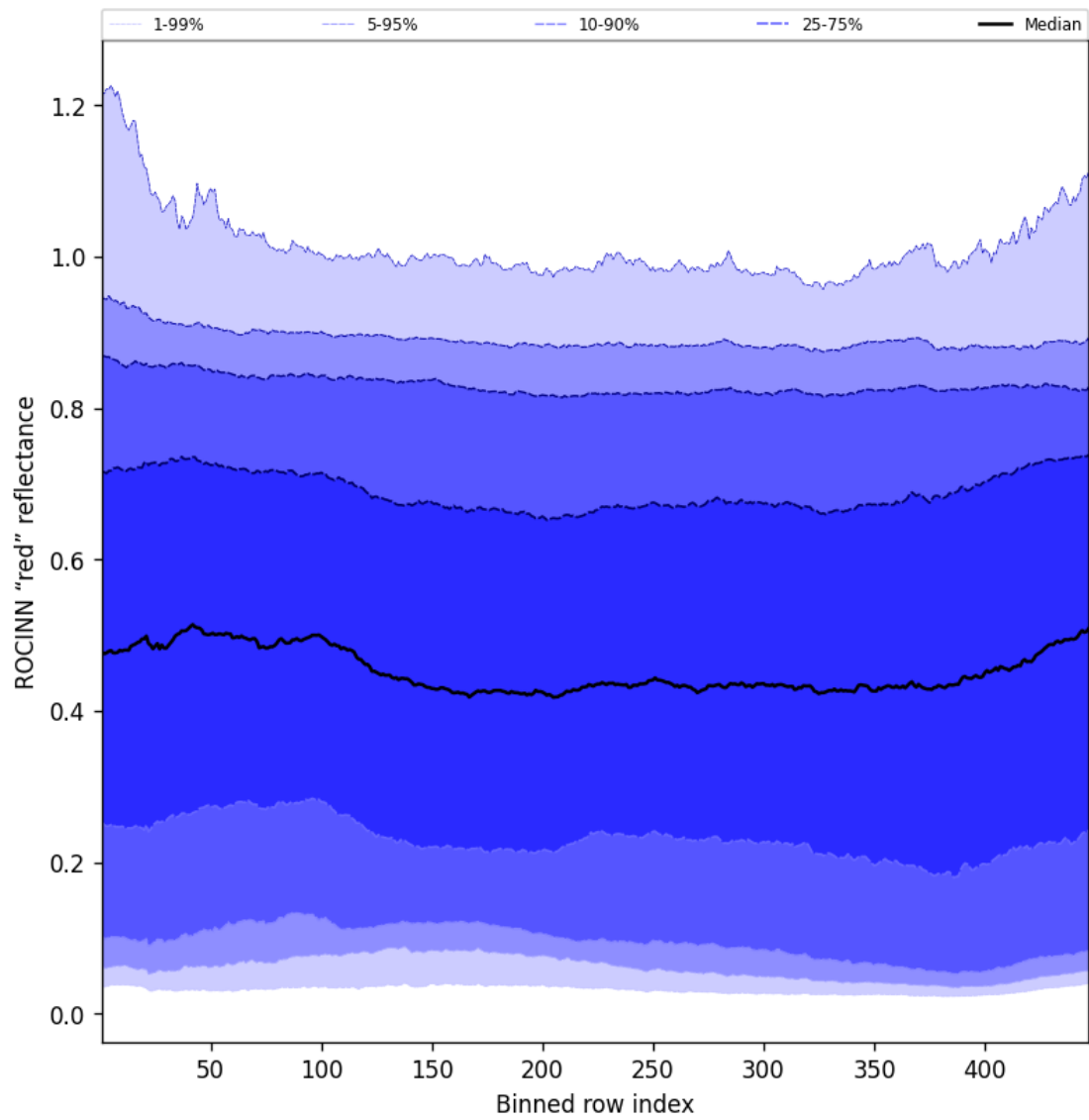
Figure 67: Along track statistics of "ROCINN "red" reflectance" for 2025-05-26 to 2025-05-27
