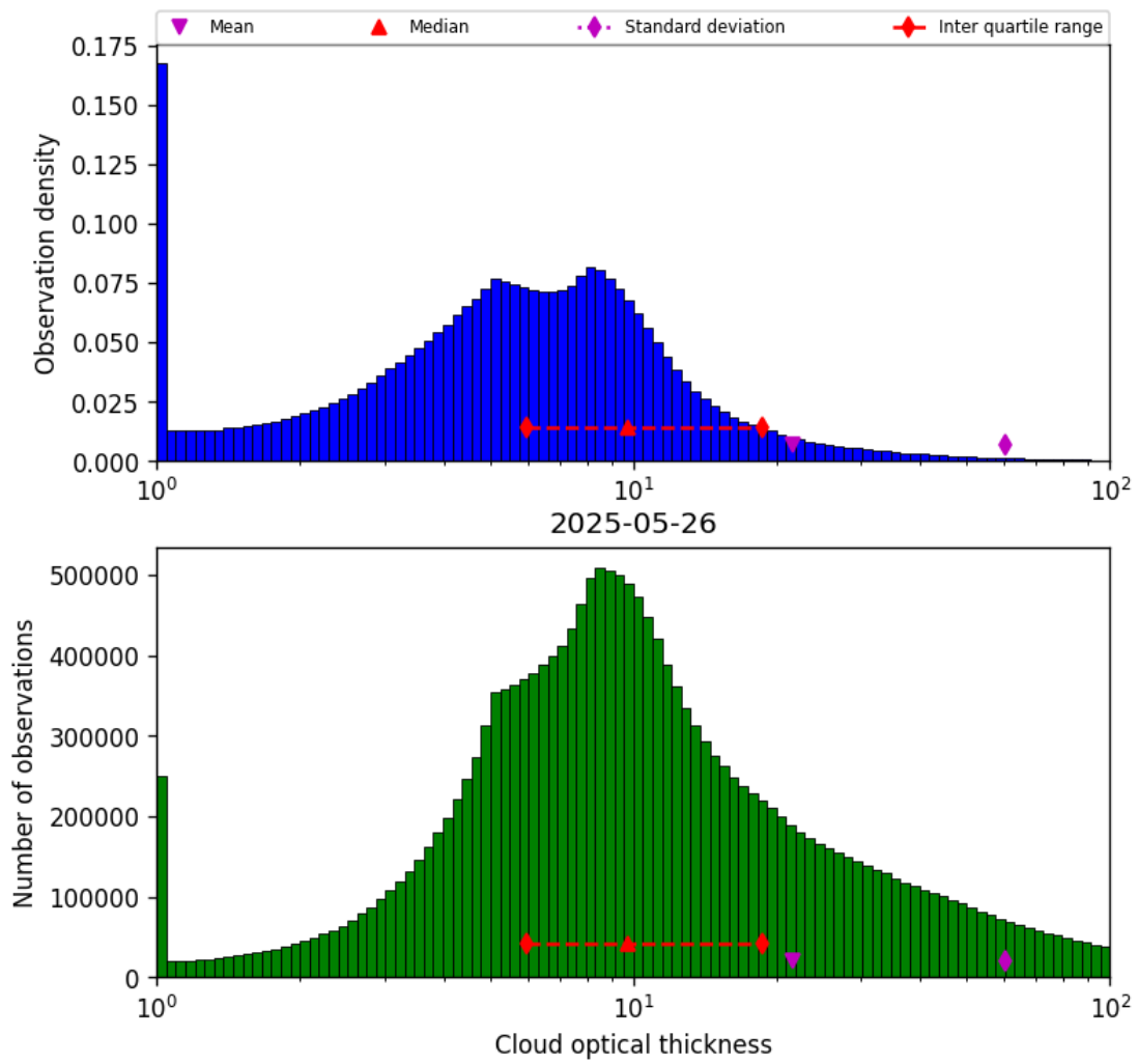
Figure 39: Histogram of “Cloud optical thickness” for 2025-05-26 to 2025-05-27
