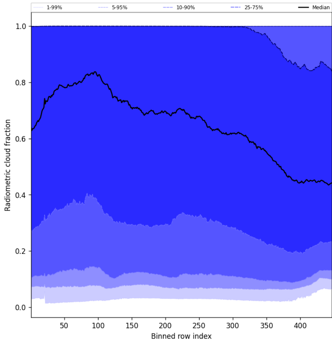
Figure 53: Along track statistics of “Radiometric cloud fraction” for 2025-05-26 to 2025-05-27
