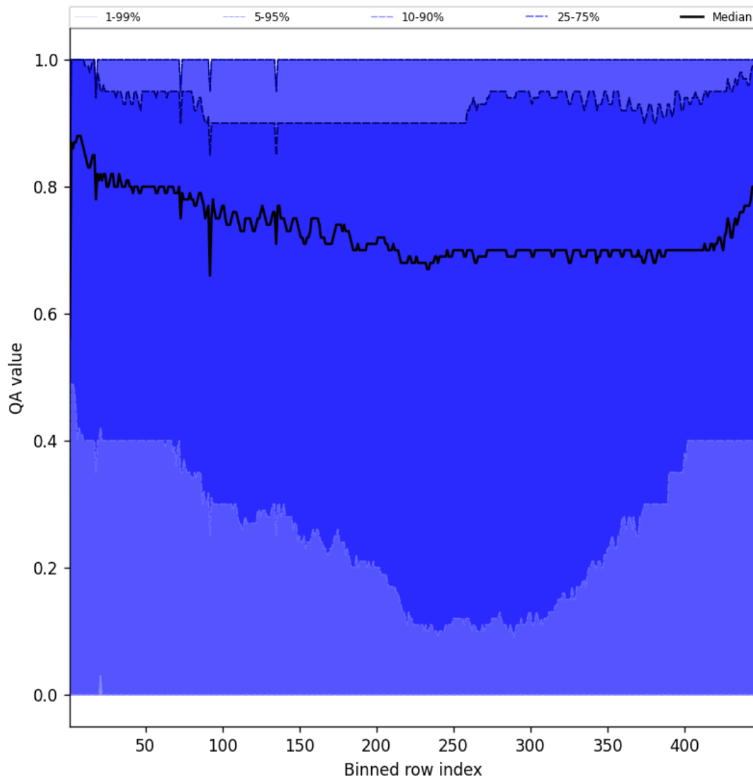
Figure 52: Along track statistics of “QA value” for 2025-05-26 to 2025-05-27
