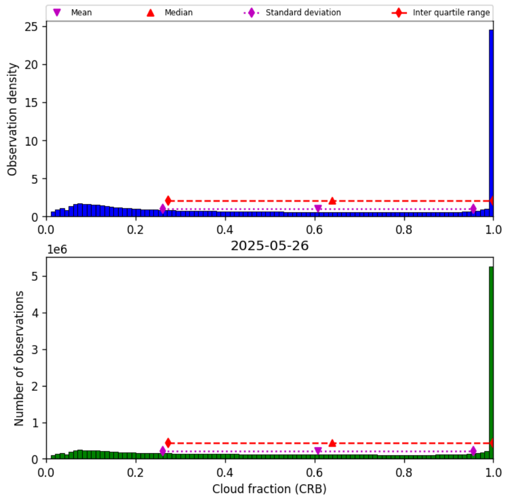
Figure 40: Histogram of “Cloud fraction (CRB)” for 2025-05-26 to 2025-05-27
