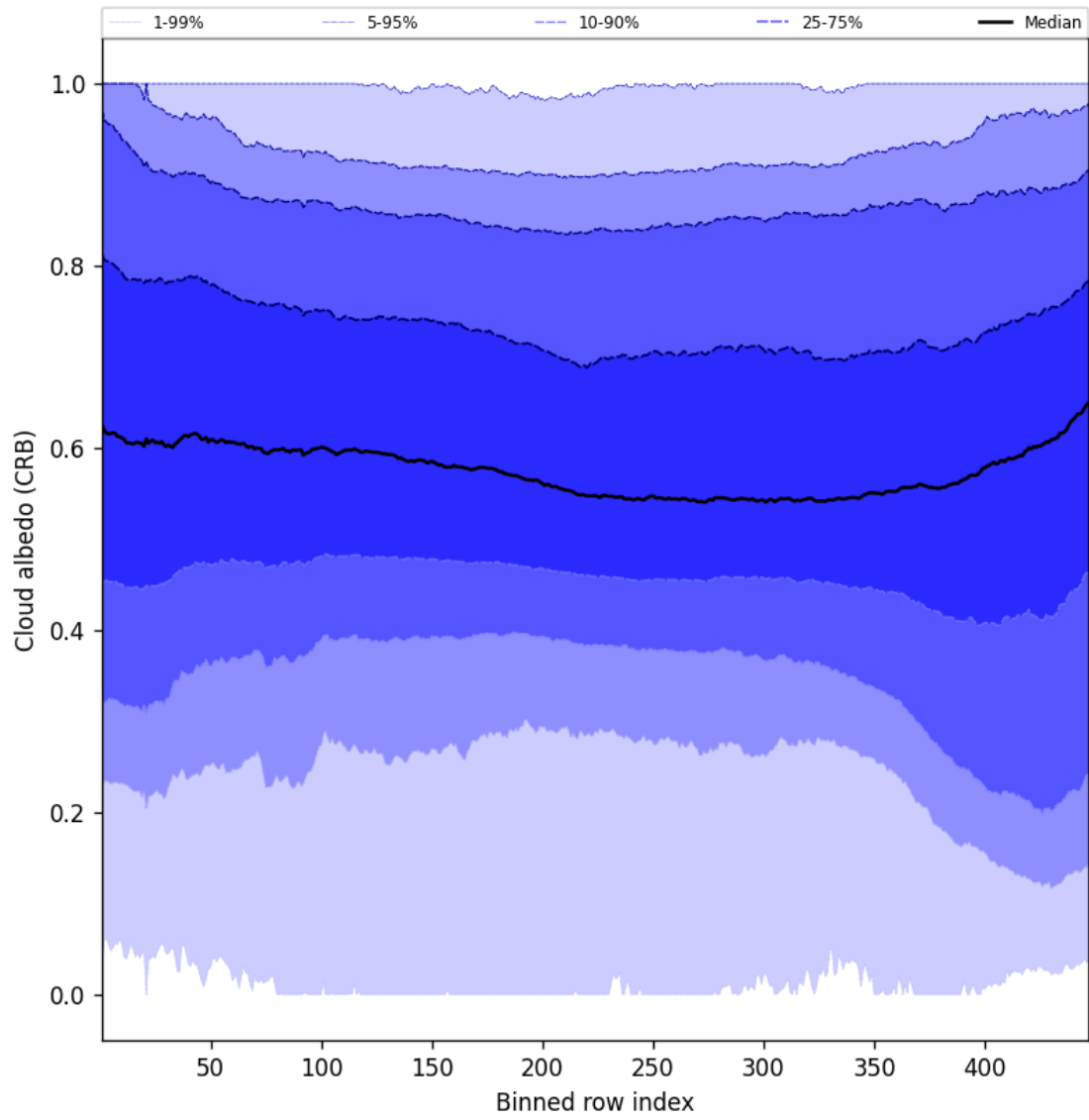
Figure 58: Along track statistics of “Cloud albedo (CRB)” for 2025-05-26 to 2025-05-27
