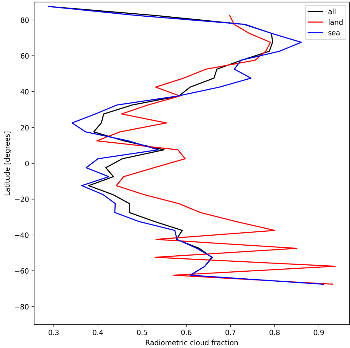
Figure 21: Zonal average of “Radiometric cloud fraction” for 2025-05-26 to 2025-05-27.
