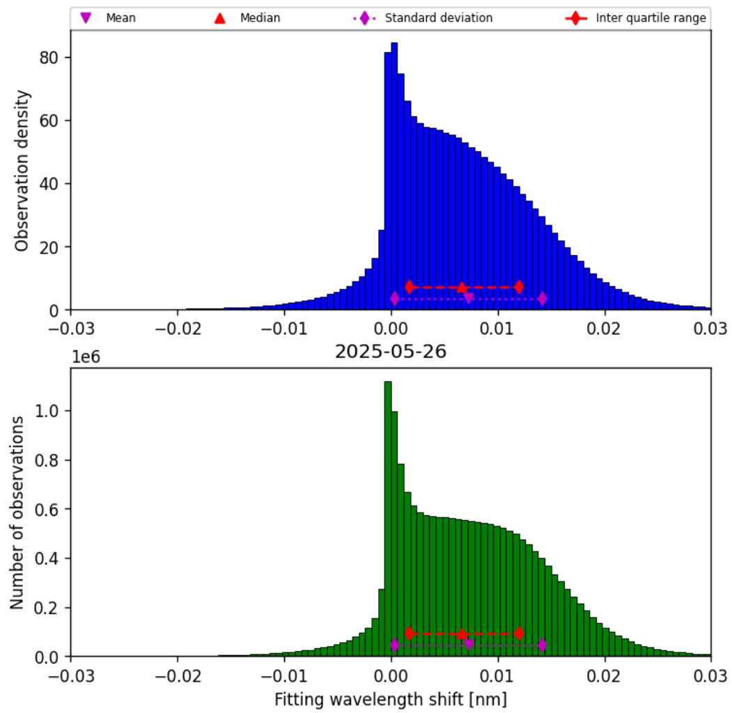
Figure 47: Histogram of “Fitting wavelength shift” for 2025-05-26 to 2025-05-27
