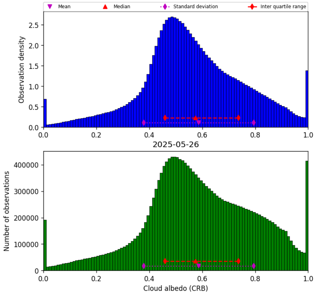
Figure 42: Histogram of “Cloud albedo (CRB)” for 2025-05-26 to 2025-05-27
