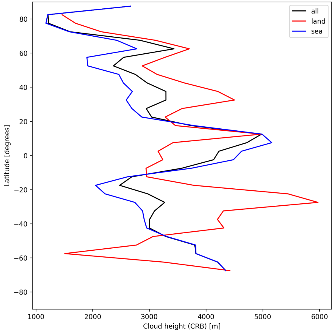
Figure 25: Zonal average of “Cloud height (CRB)” for 2025-05-26 to 2025-05-27.
