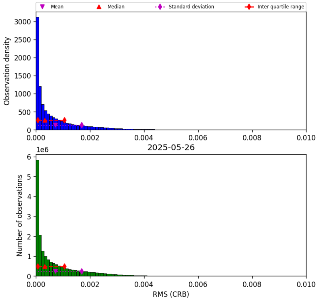
Figure 46: Histogram of “RMS (CRB)” for 2025-05-26 to 2025-05-27
