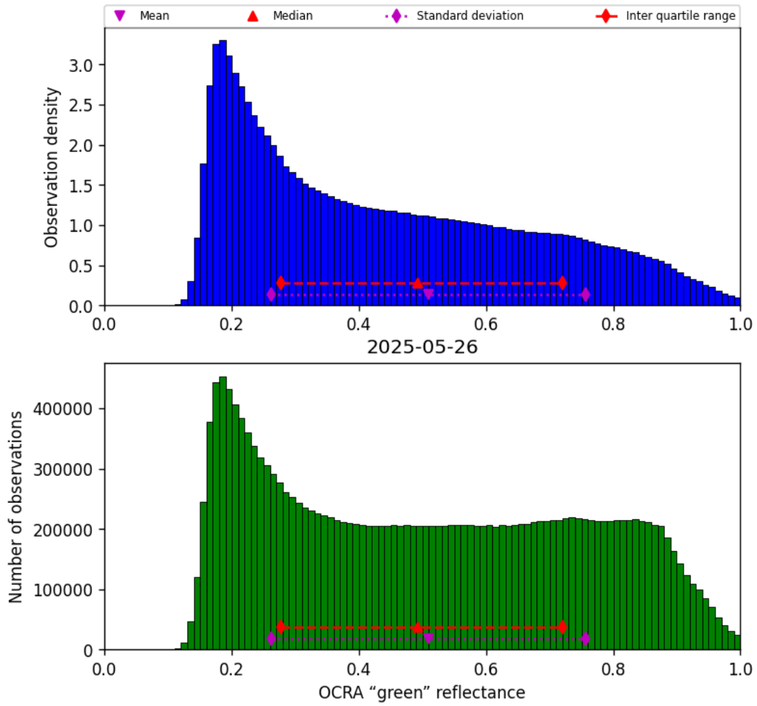
Figure 50: Histogram of “OCRA “green” reflectance” for 2025-05-26 to 2025-05-27
