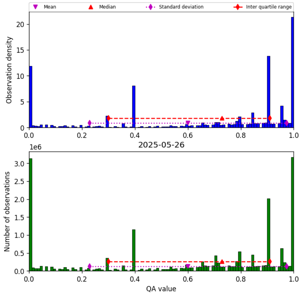
Figure 36: Histogram of “QA value” for 2025-05-26 to 2025-05-27
