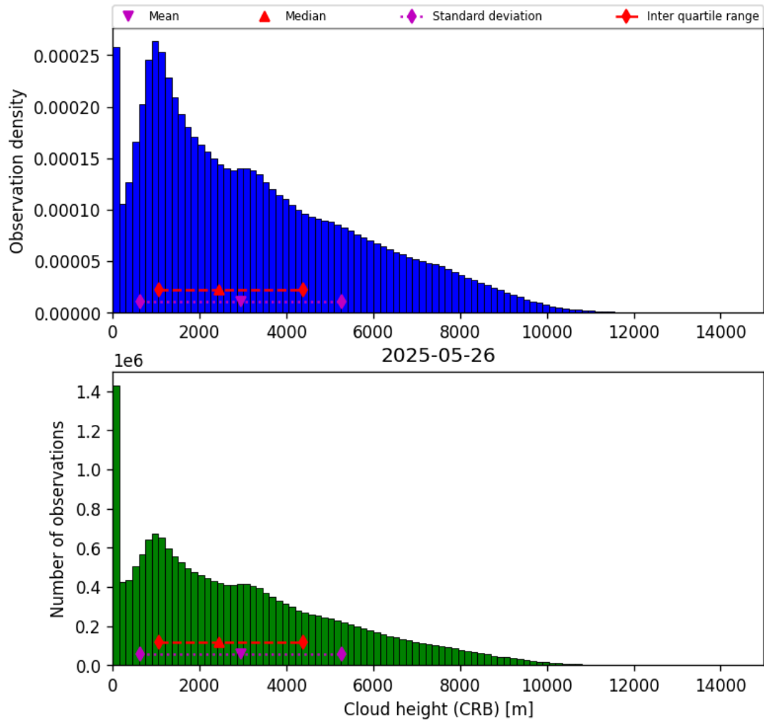
Figure 41: Histogram of “Cloud height (CRB)” for 2025-05-26 to 2025-05-27
