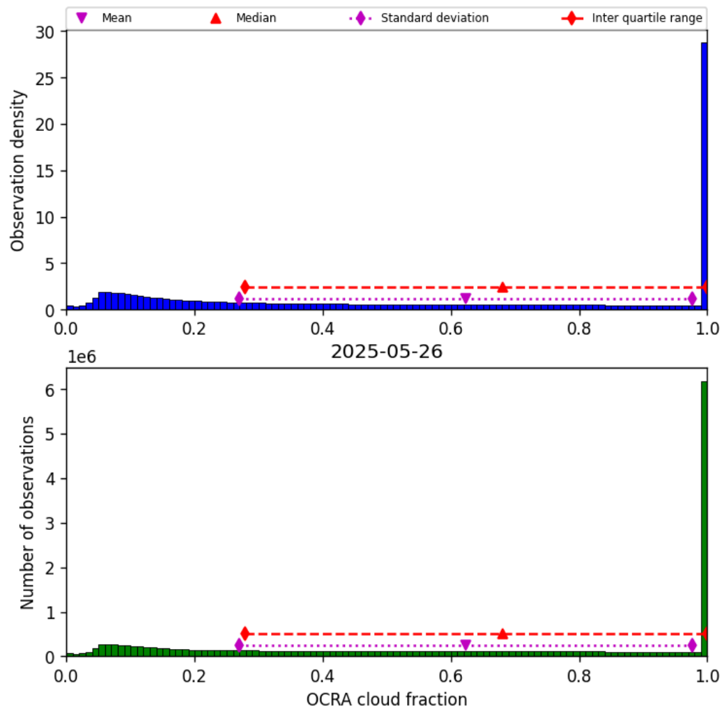
Figure 48: Histogram of “OCRA cloud fraction” for 2025-05-26 to 2025-05-27
