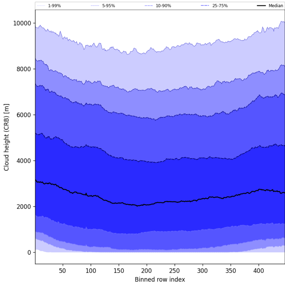
Figure 57: Along track statistics of “Cloud height (CRB)” for 2025-05-26 to 2025-05-27
