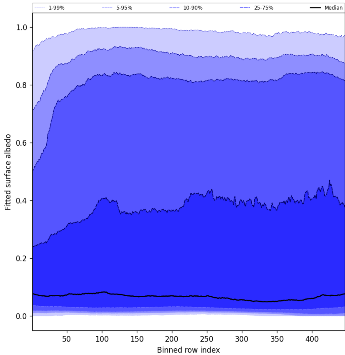
Figure 59: Along track statistics of “Fitted surface albedo” for 2025-05-26 to 2025-05-27
