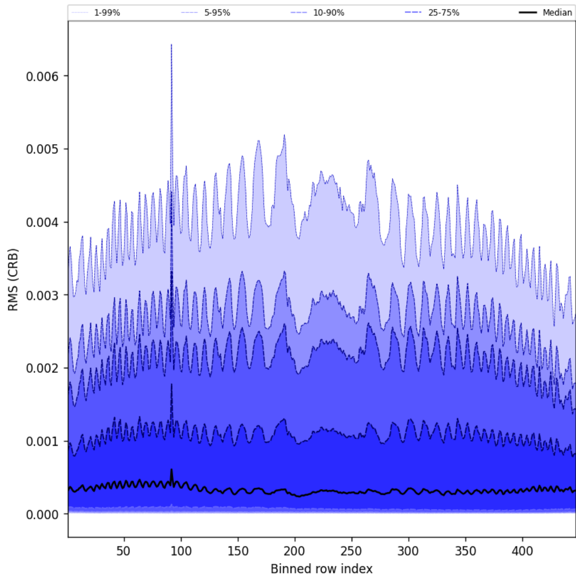
Figure 62: Along track statistics of “RMS (CRB)” for 2025-05-26 to 2025-05-27
