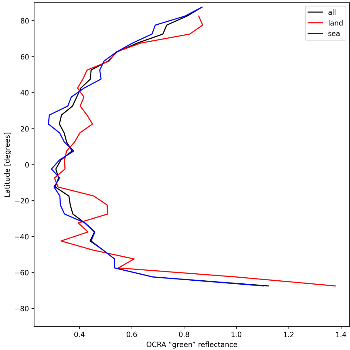
Figure 34: Zonal average of “OCRA “green” reflectance” for 2025-05-27 to 2025-05-28.
