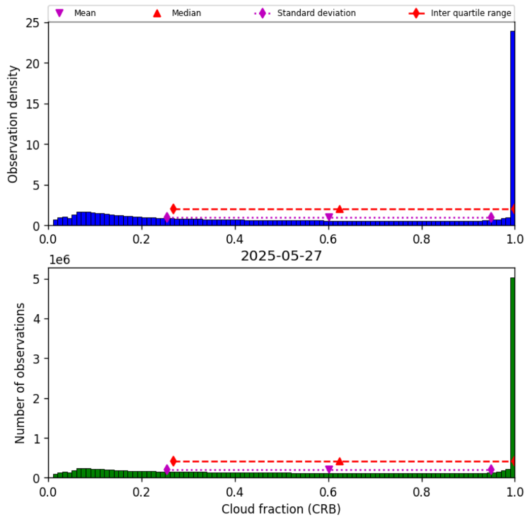
Figure 40: Histogram of “Cloud fraction (CRB)” for 2025-05-27 to 2025-05-28
