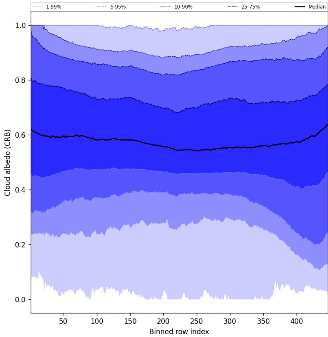
Figure 58: Along track statistics of “Cloud albedo (CRB)” for 2025-05-27 to 2025-05-28
