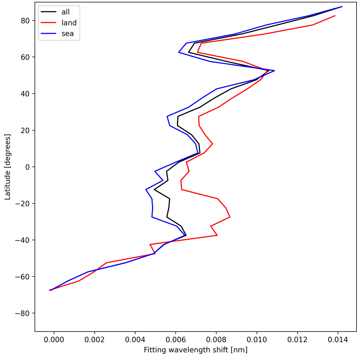
Figure 31: Zonal average of “Fitting wavelength shift” for 2025-05-27 to 2025-05-28.
