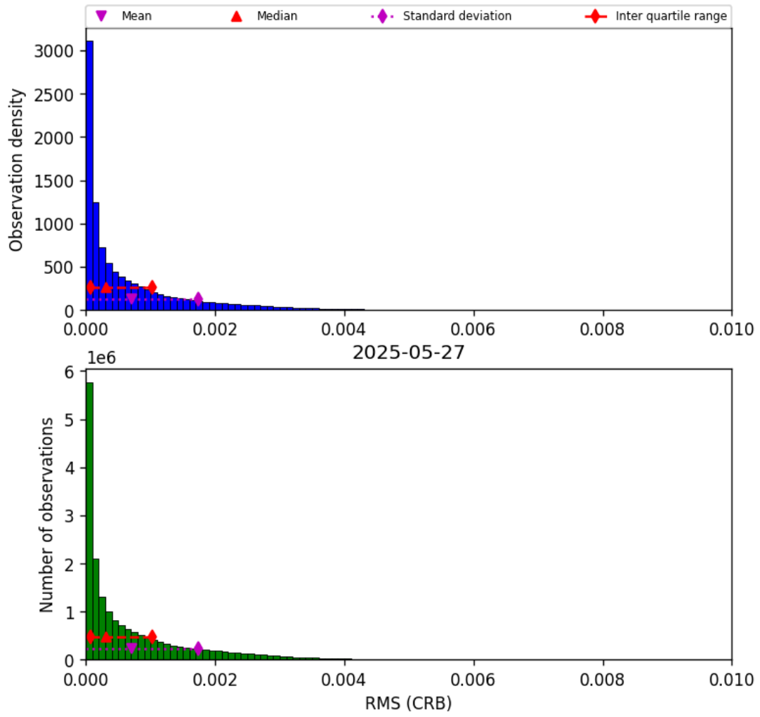
Figure 46: Histogram of “RMS (CRB)” for 2025-05-27 to 2025-05-28
