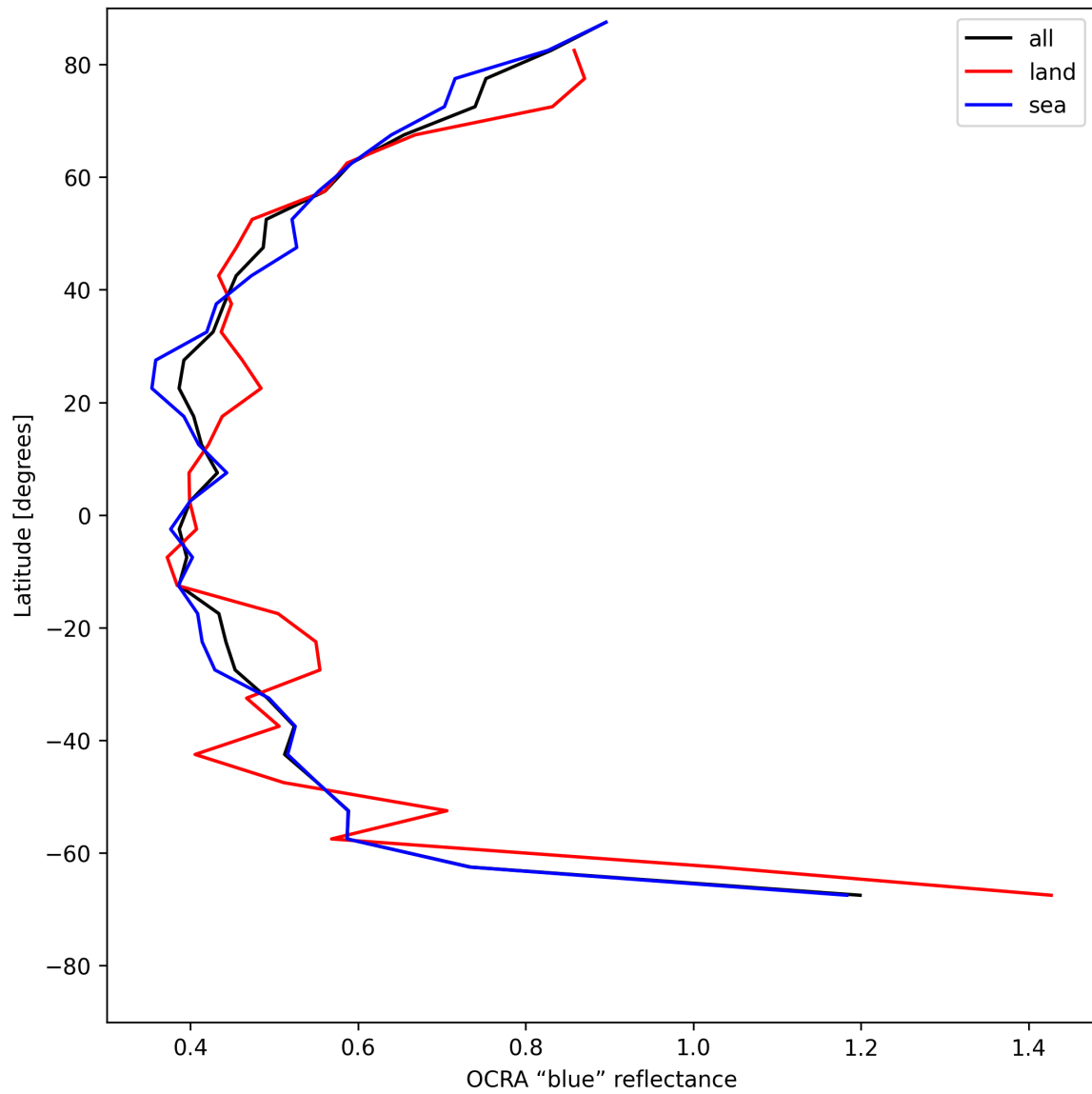
Figure 33: Zonal average of “OCRA “blue” reflectance” for 2025-05-27 to 2025-05-28.
