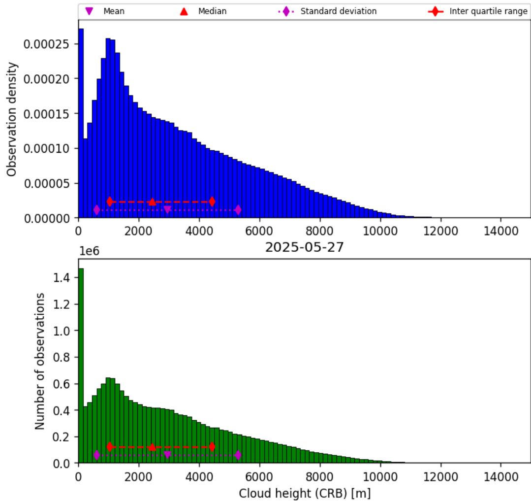
Figure 41: Histogram of “Cloud height (CRB)” for 2025-05-27 to 2025-05-28
