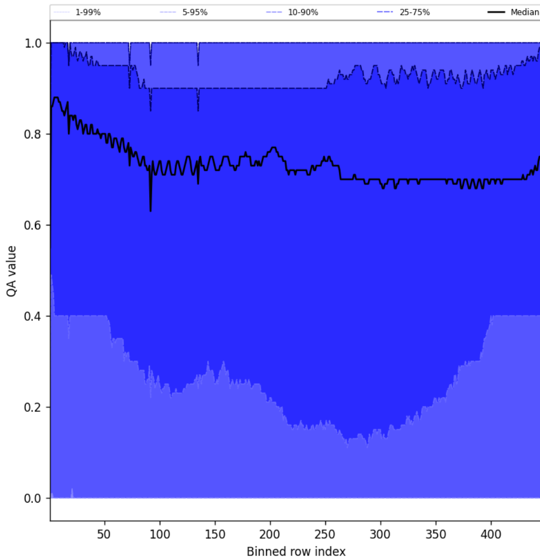
Figure 52: Along track statistics of “QA value” for 2025-05-27 to 2025-05-28
