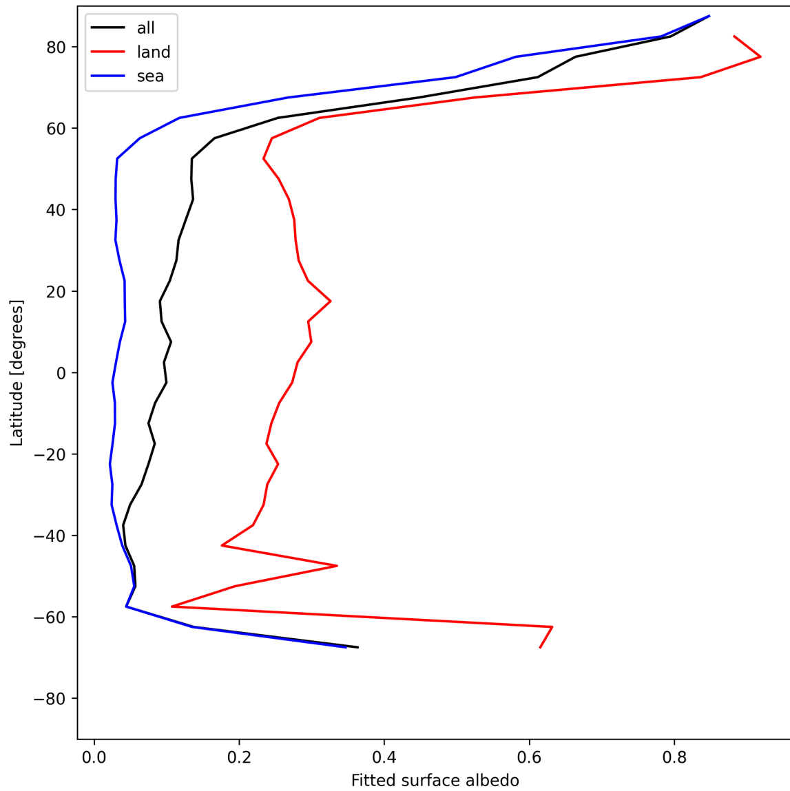
Figure 27: Zonal average of “Fitted surface albedo” for 2025-05-27 to 2025-05-28.
