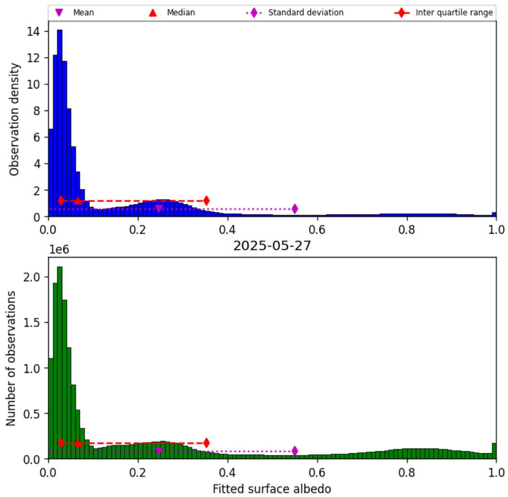
Figure 43: Histogram of “Fitted surface albedo” for 2025-05-27 to 2025-05-28
