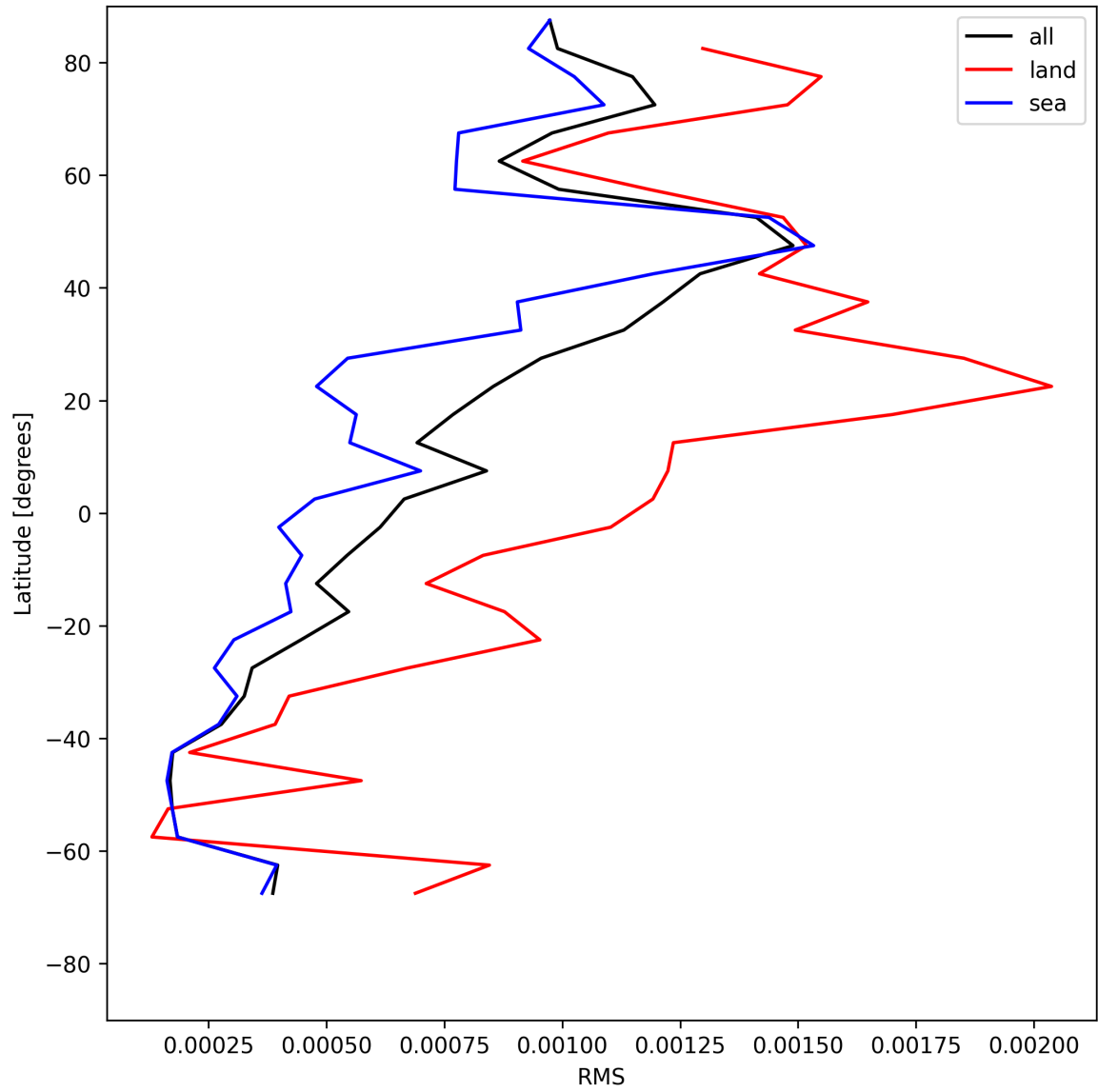
Figure 29: Zonal average of “RMS” for 2025-05-27 to 2025-05-28.
