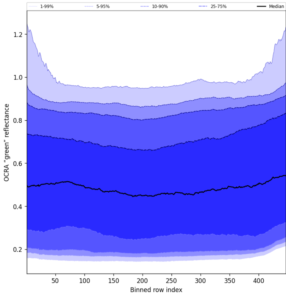
Figure 66: Along track statistics of “OCRA “green” reflectance” for 2025-05-27 to 2025-05-28
