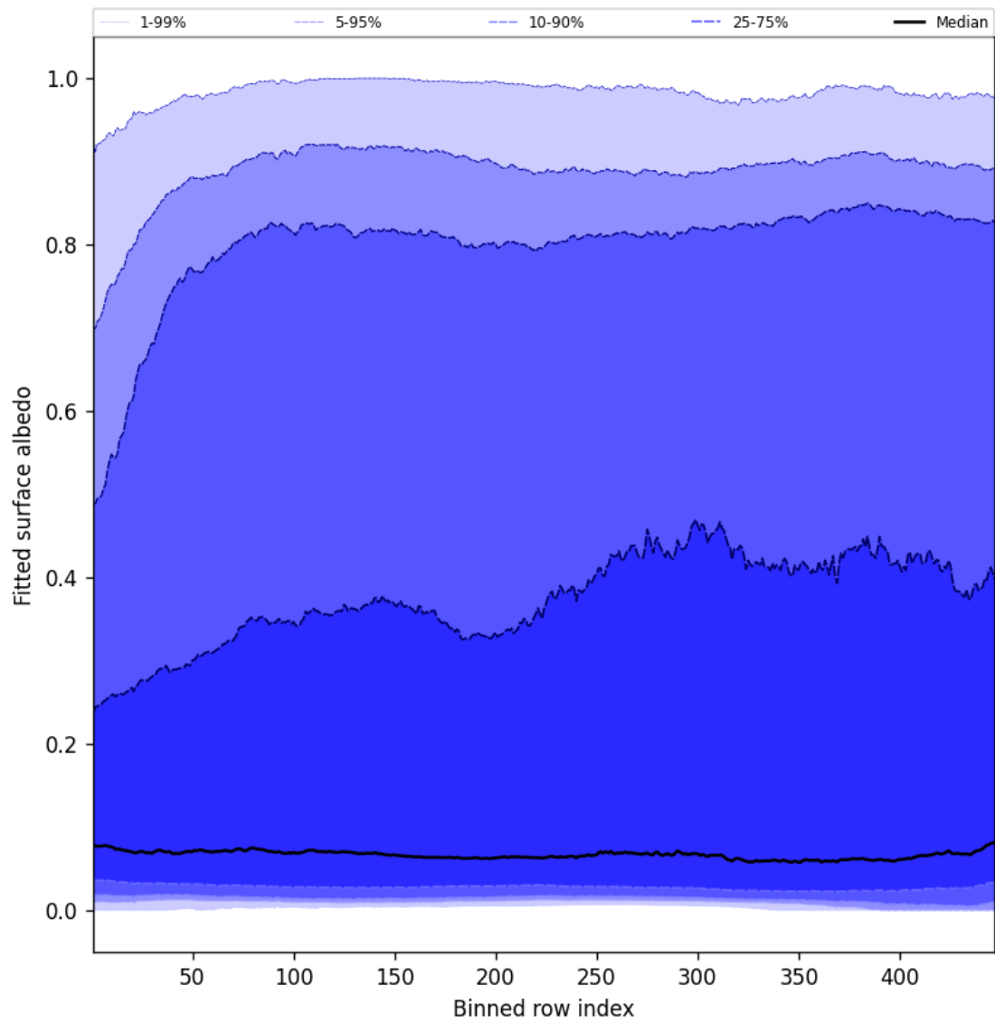
Figure 59: Along track statistics of “Fitted surface albedo” for 2025-05-27 to 2025-05-28
