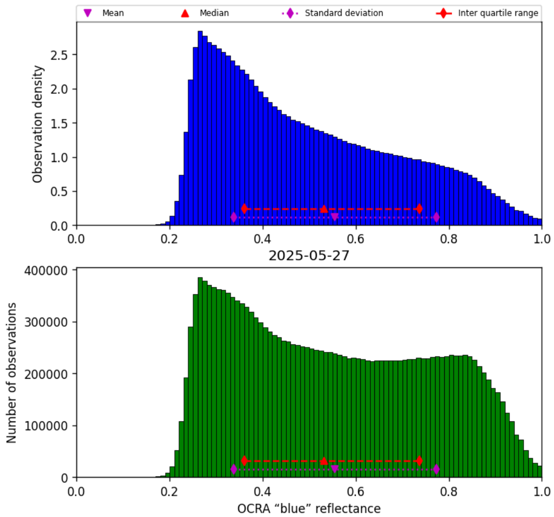
Figure 49: Histogram of “OCRA “blue” reflectance” for 2025-05-27 to 2025-05-28
