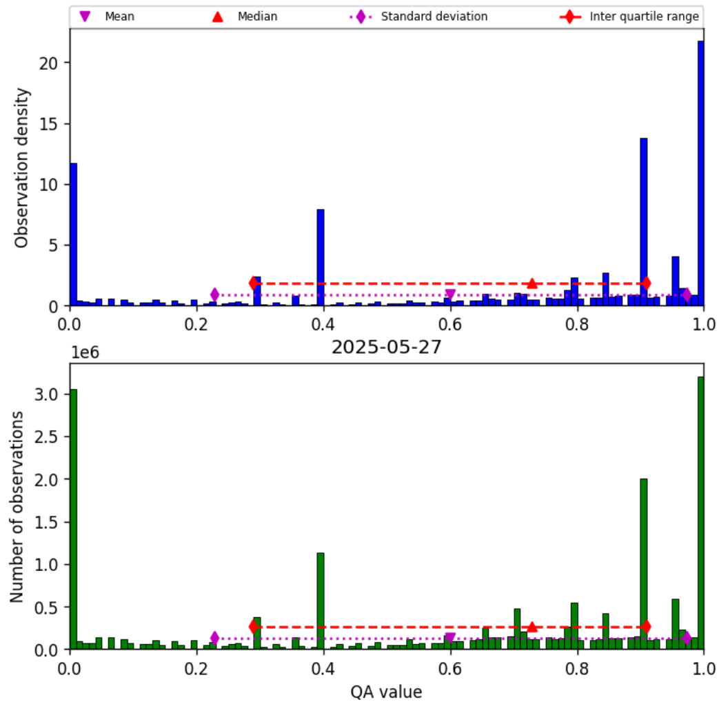
Figure 36: Histogram of “QA value” for 2025-05-27 to 2025-05-28
