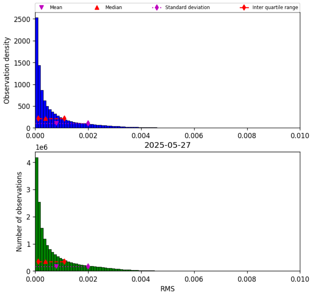
Figure 45: Histogram of “RMS” for 2025-05-27 to 2025-05-28
