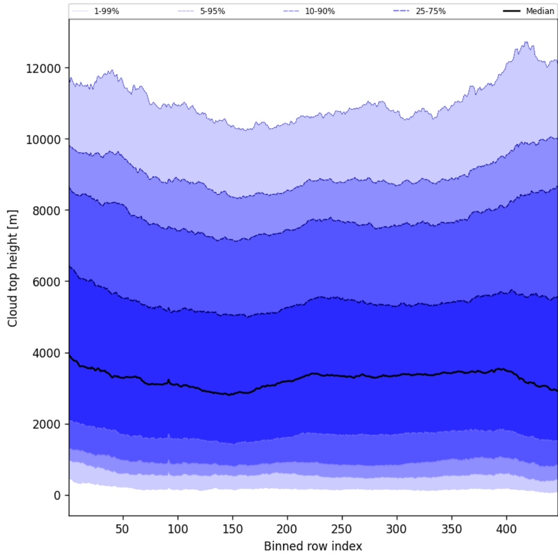
Figure 54: Along track statistics of “Cloud top height” for 2025-05-27 to 2025-05-28
