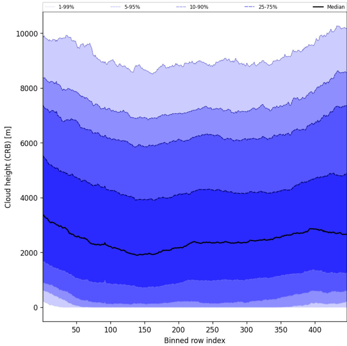
Figure 57: Along track statistics of “Cloud height (CRB)” for 2025-05-27 to 2025-05-28
