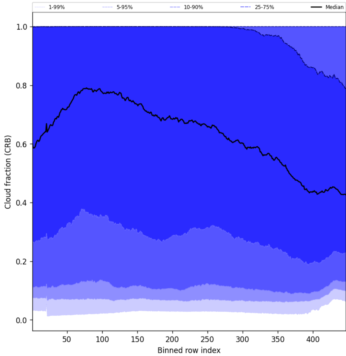
Figure 56: Along track statistics of “Cloud fraction (CRB)” for 2025-05-27 to 2025-05-28
