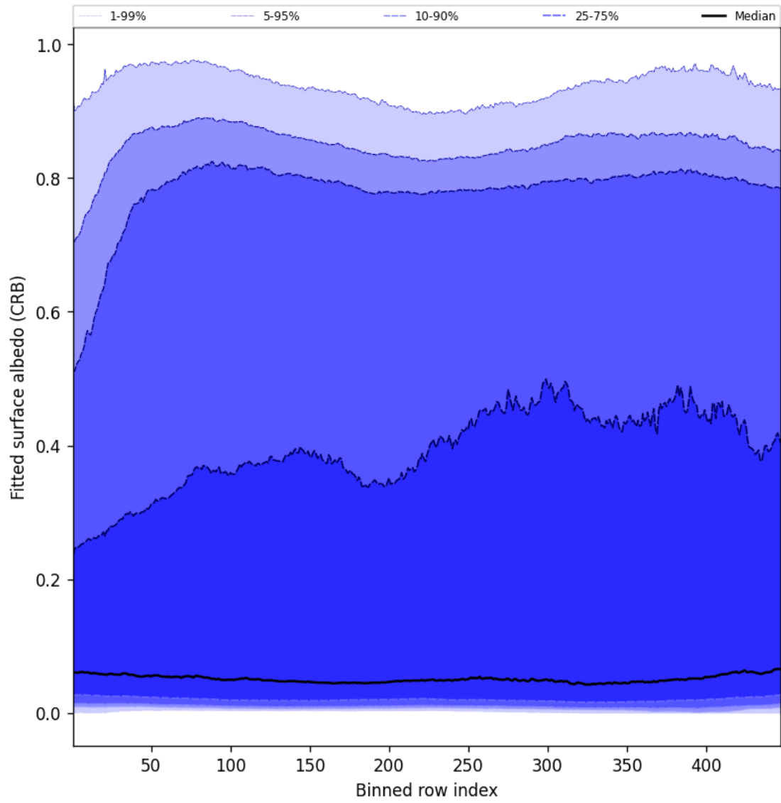
Figure 60: Along track statistics of “Fitted surface albedo (CRB)” for 2025-05-27 to 2025-05-28
