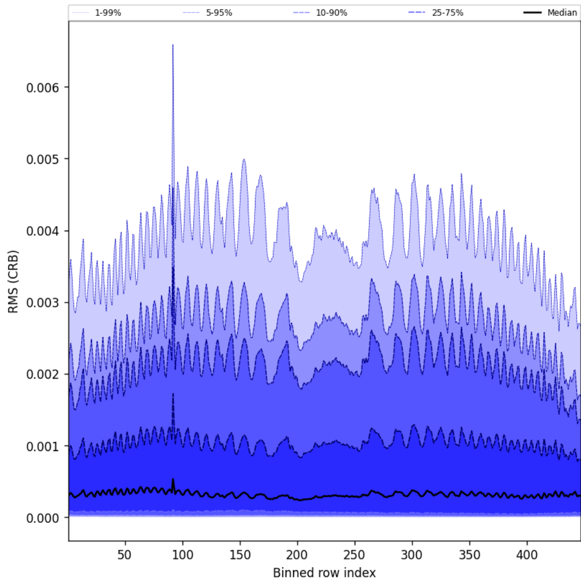
Figure 62: Along track statistics of “RMS (CRB)” for 2025-05-27 to 2025-05-28
