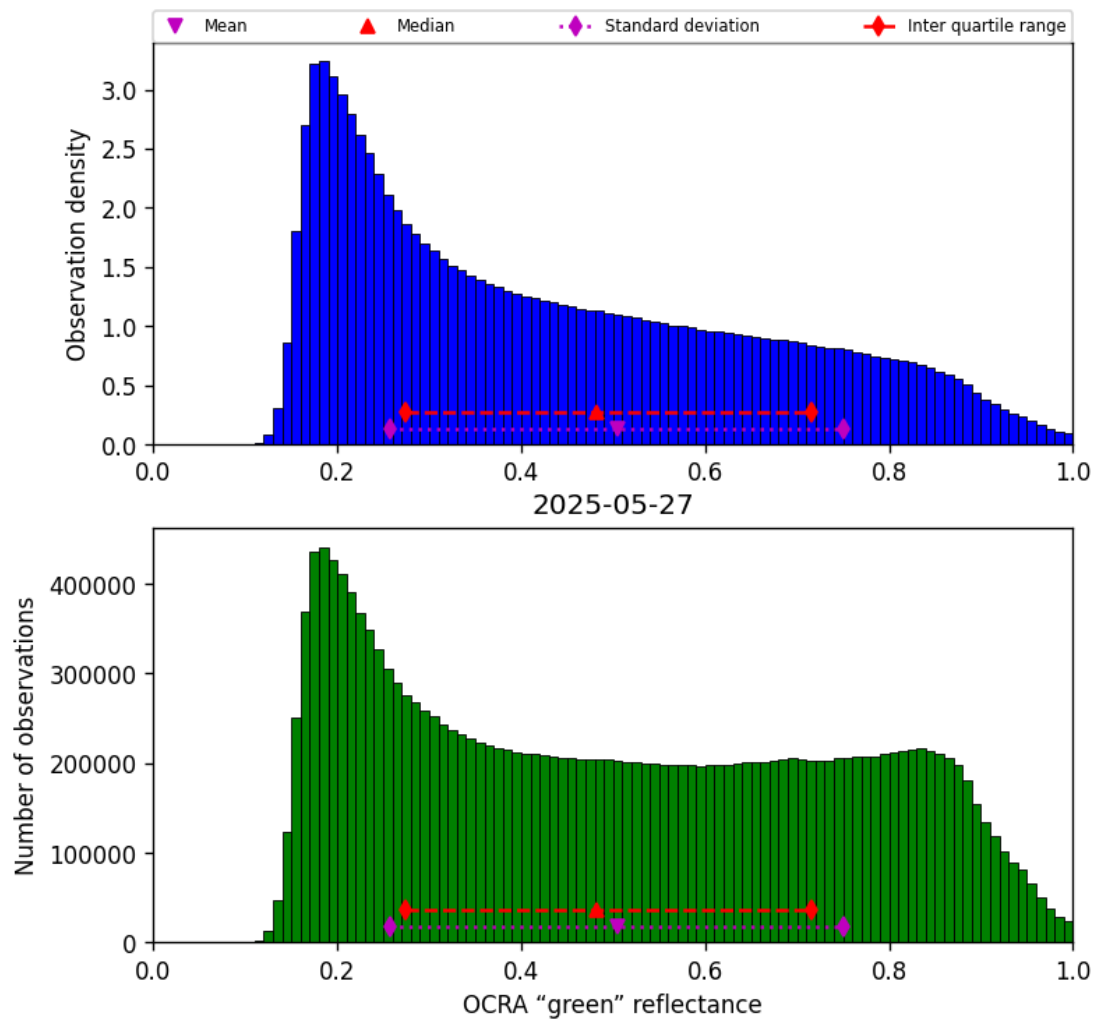
Figure 50: Histogram of “OCRA “green” reflectance” for 2025-05-27 to 2025-05-28
