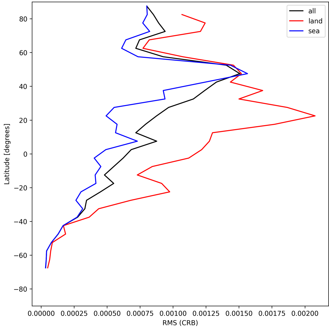
Figure 30: Zonal average of “RMS (CRB)” for 2025-05-27 to 2025-05-28.
