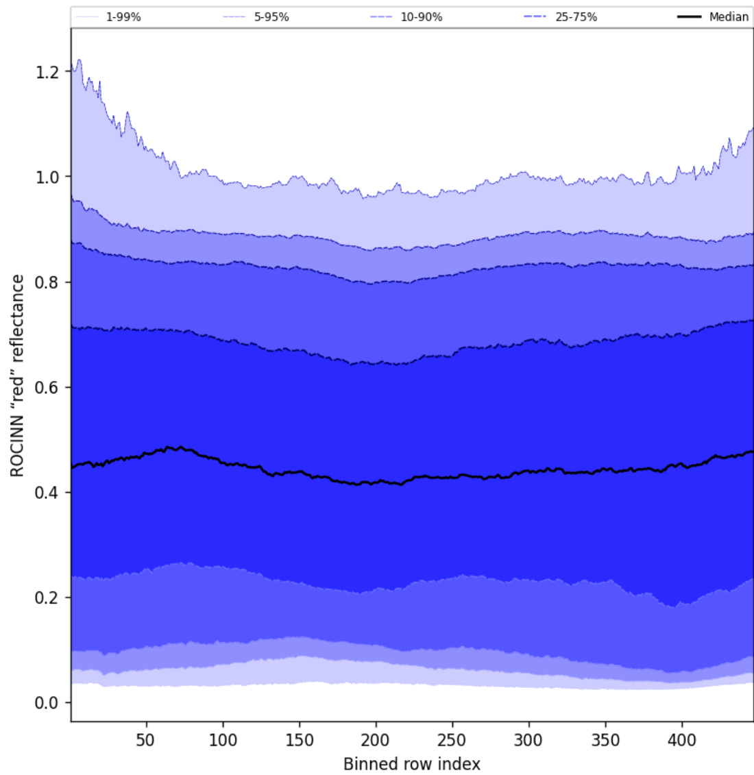
Figure 67: Along track statistics of “ROCINN “red” reflectance” for 2025-05-27 to 2025-05-28
