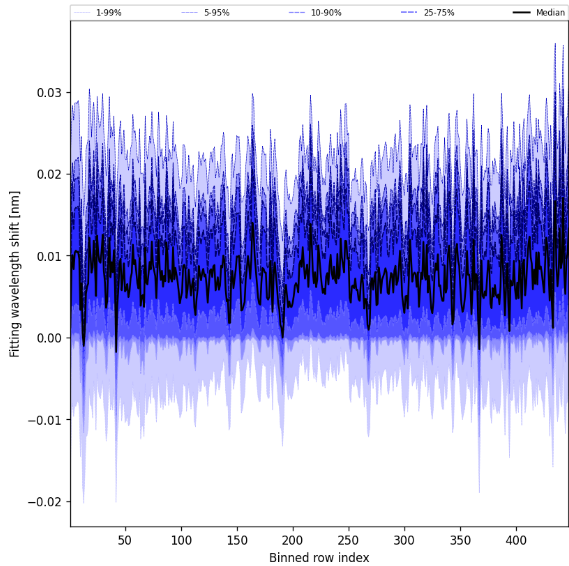
Figure 63: Along track statistics of “Fitting wavelength shift” for 2025-05-27 to 2025-05-28
