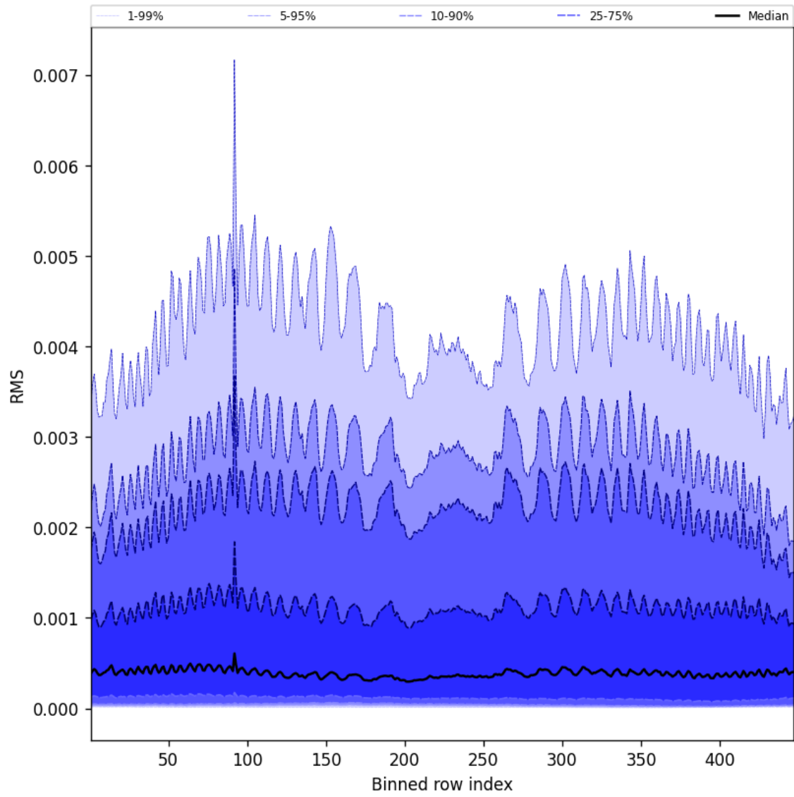
Figure 61: Along track statistics of “RMS” for 2025-05-27 to 2025-05-28
