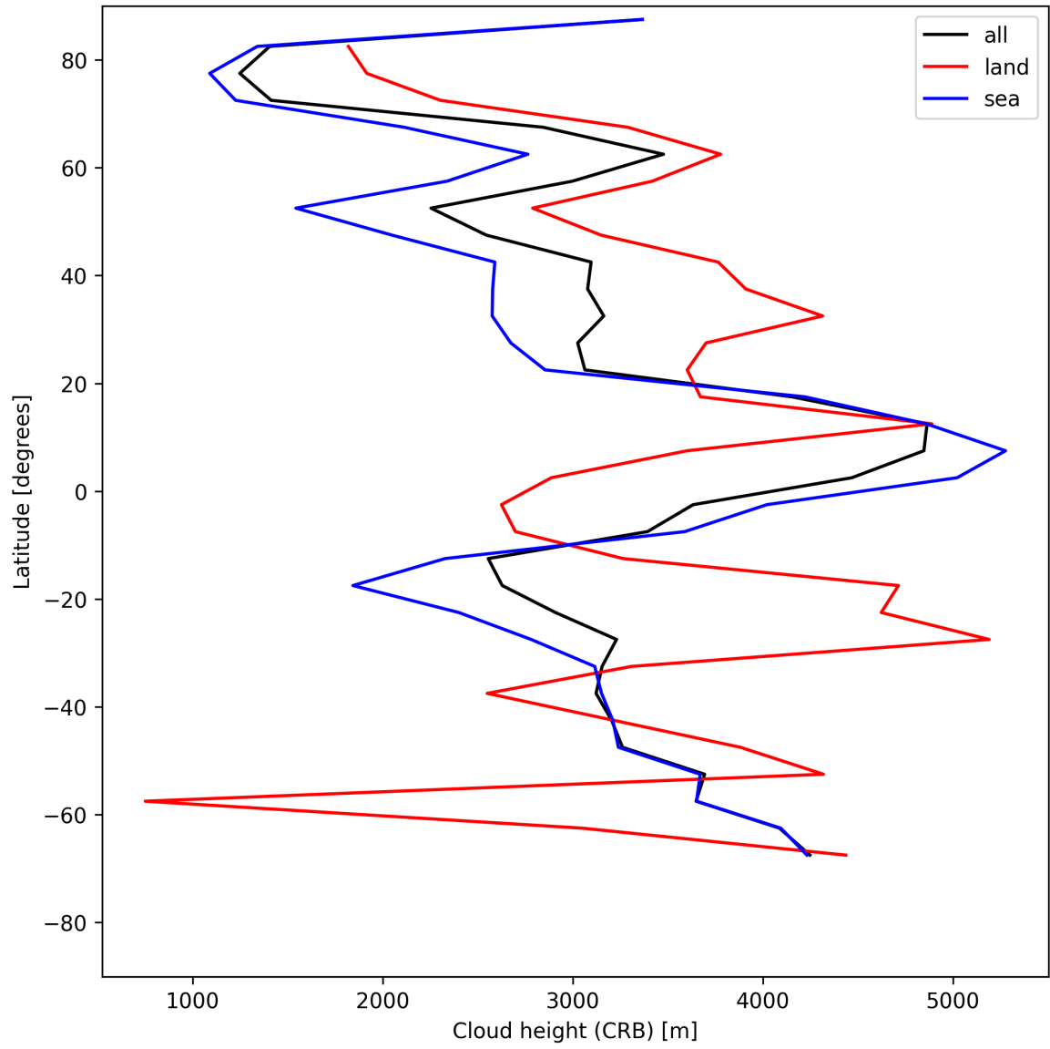
Figure 25: Zonal average of “Cloud height (CRB)” for 2025-05-27 to 2025-05-28.
