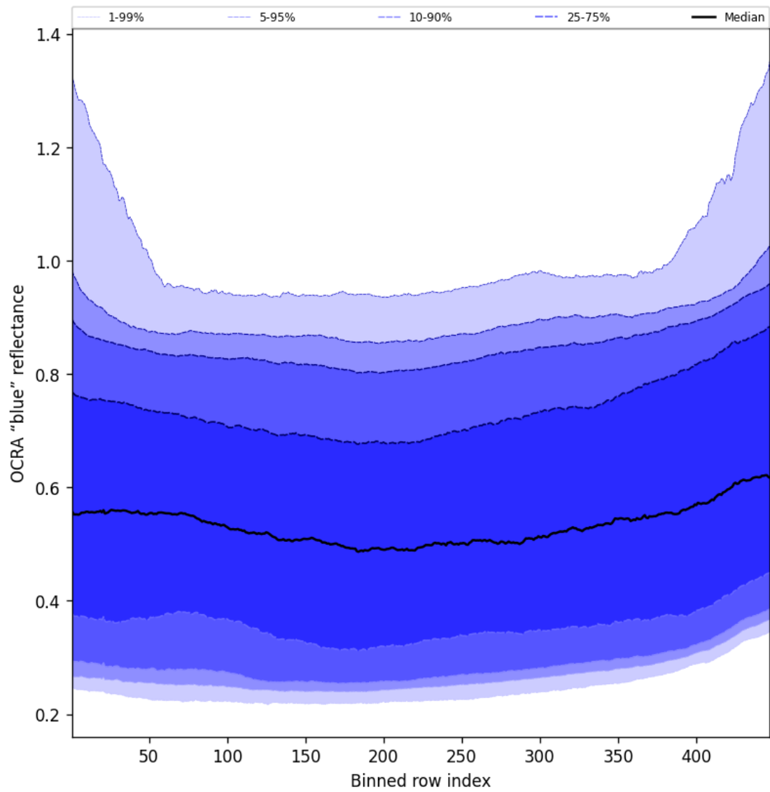
Figure 65: Along track statistics of “OCRA “blue” reflectance” for 2025-05-27 to 2025-05-28
