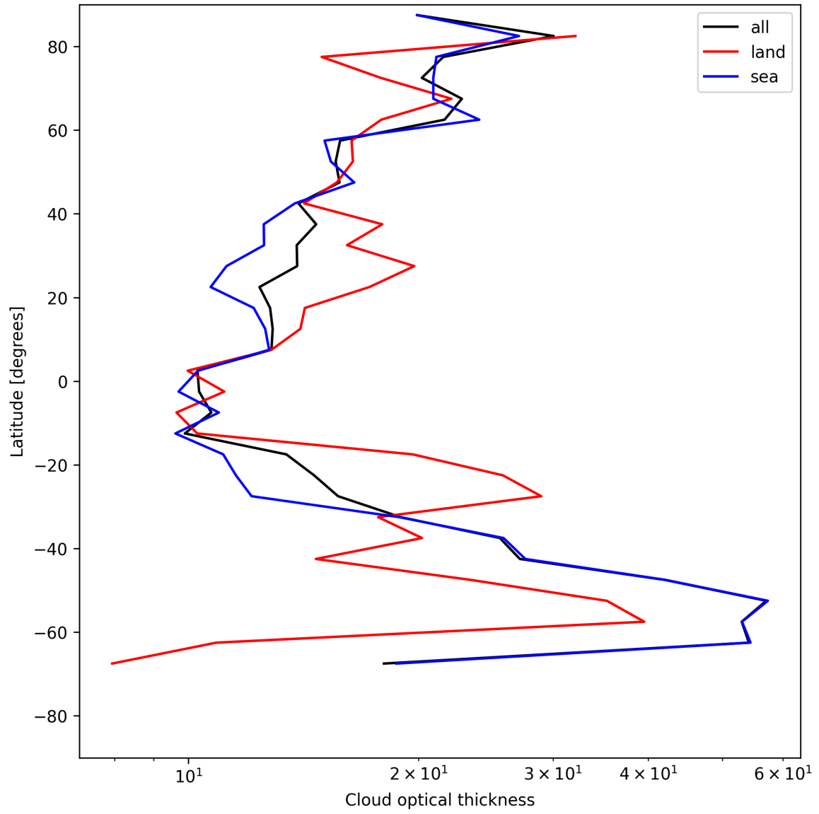
Figure 23: Zonal average of “Cloud optical thickness” for 2025-05-27 to 2025-05-28.
