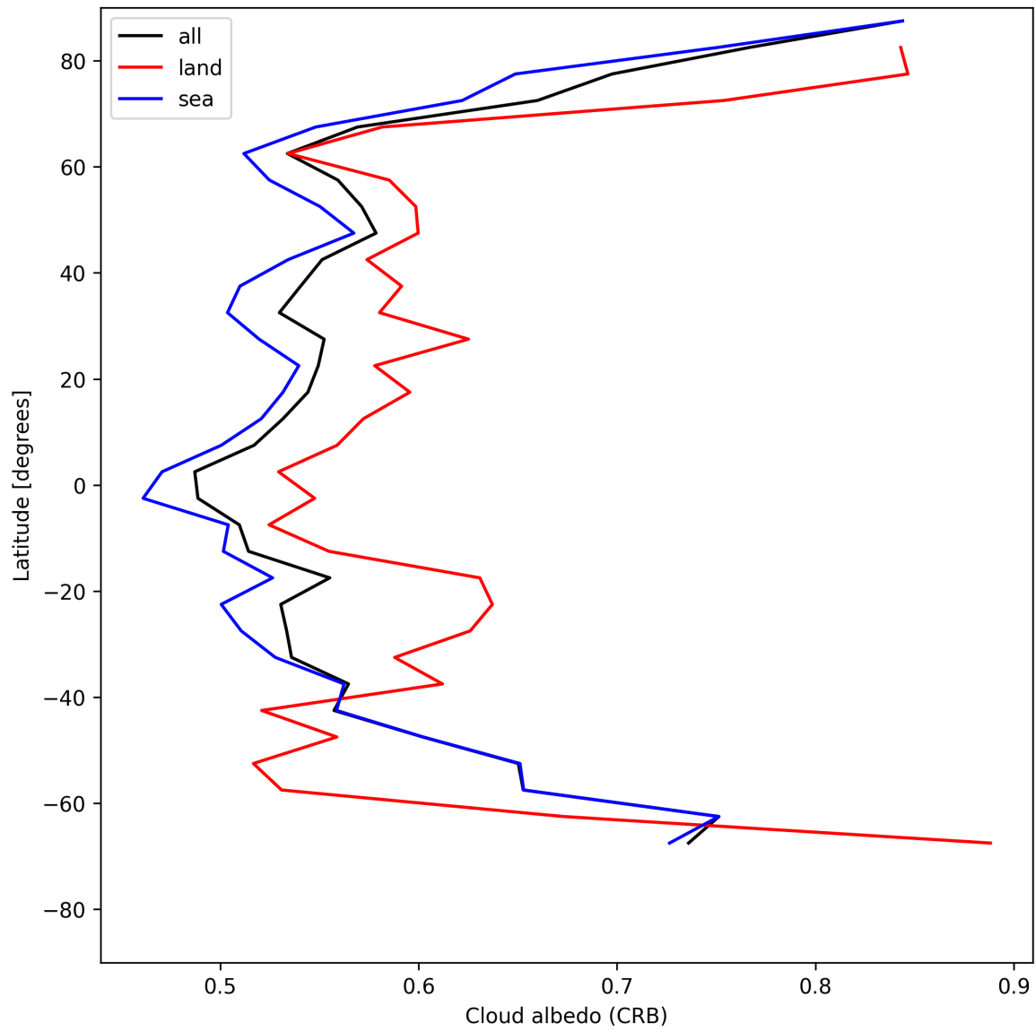
Figure 26: Zonal average of “Cloud albedo (CRB)” for 2025-05-27 to 2025-05-28.
