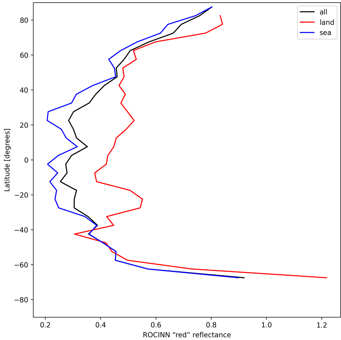
Figure 35: Zonal average of “ROCINN “red” reflectance” for 2025-05-27 to 2025-05-28.
