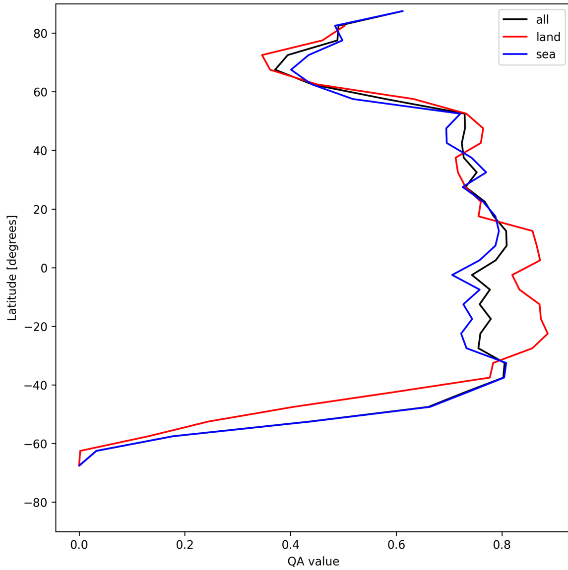
Figure 20: Zonal average of “QA value” for 2025-05-27 to 2025-05-28.
