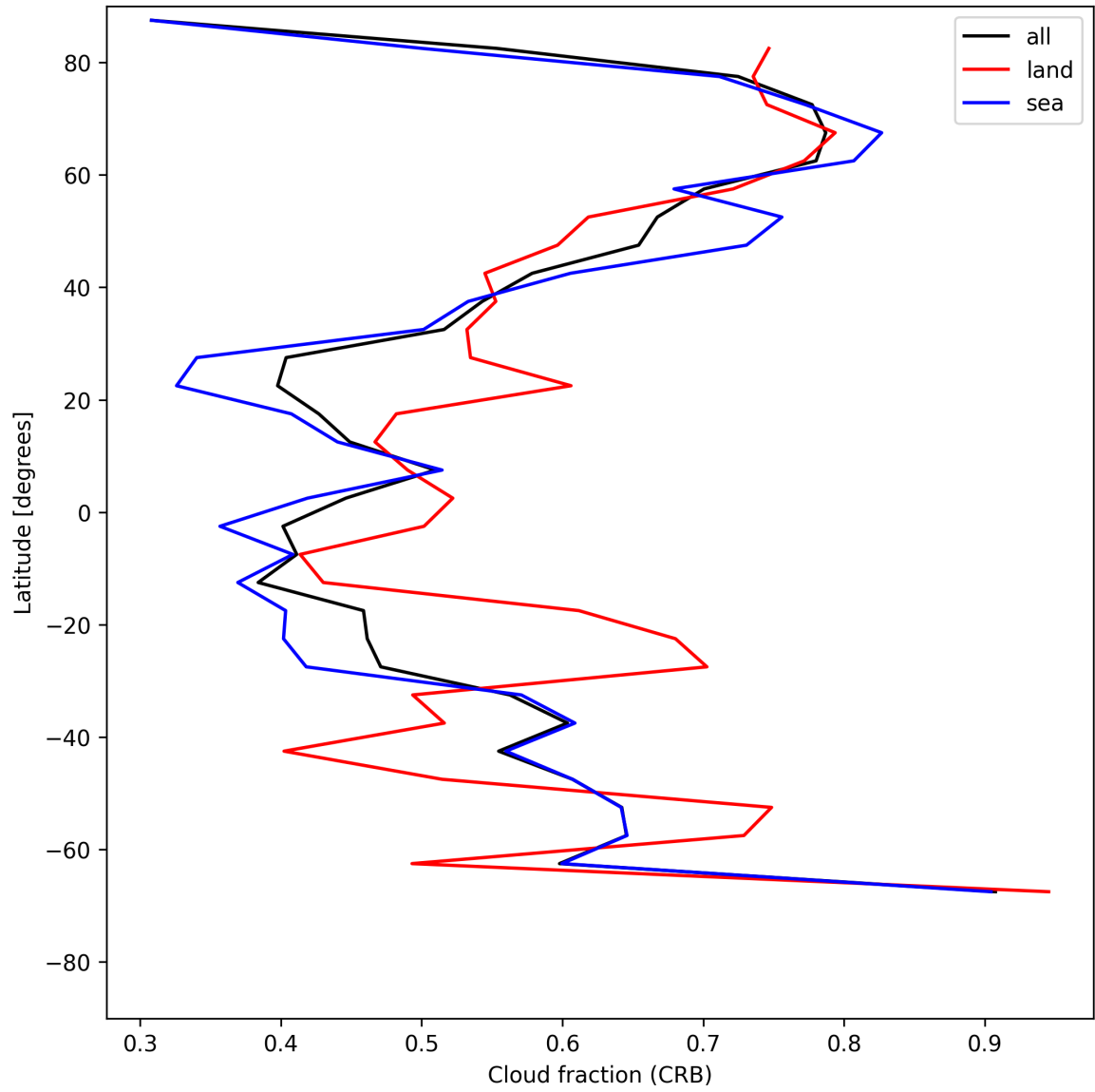
Figure 24: Zonal average of “Cloud fraction (CRB)” for 2025-05-27 to 2025-05-28.
