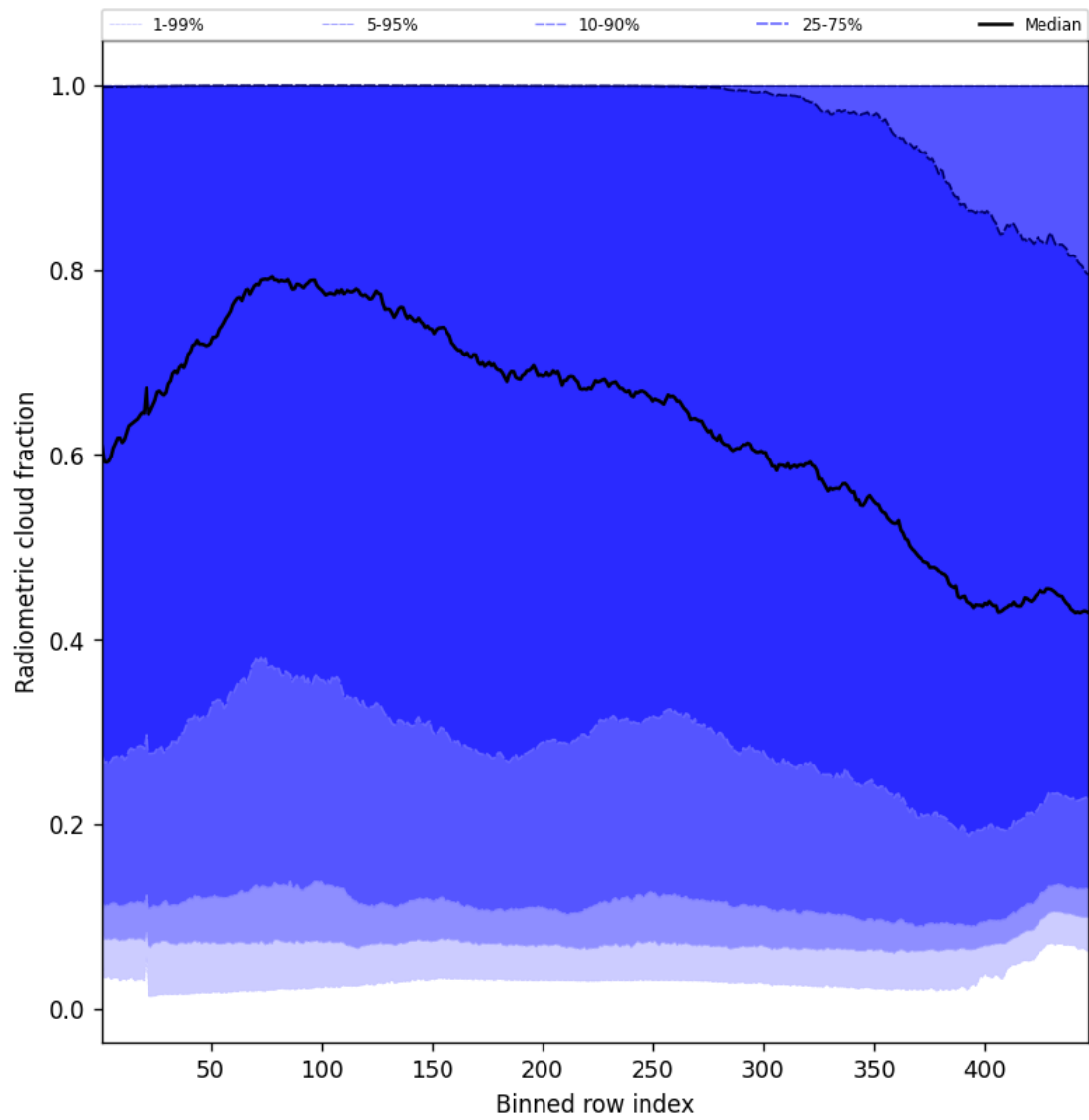
Figure 53: Along track statistics of “Radiometric cloud fraction” for 2025-05-27 to 2025-05-28
