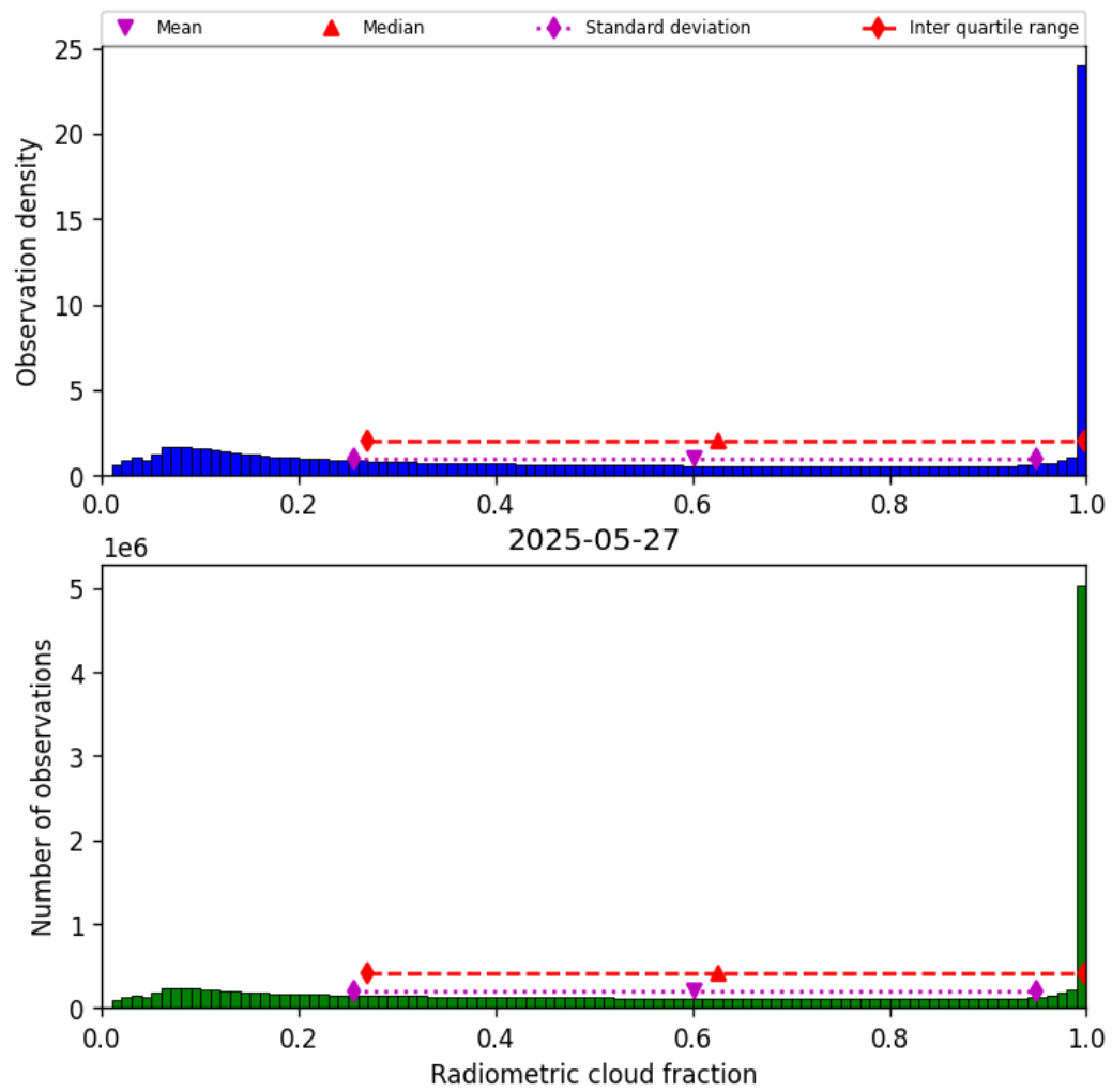
Figure 37: Histogram of “Radiometric cloud fraction” for 2025-05-27 to 2025-05-28
