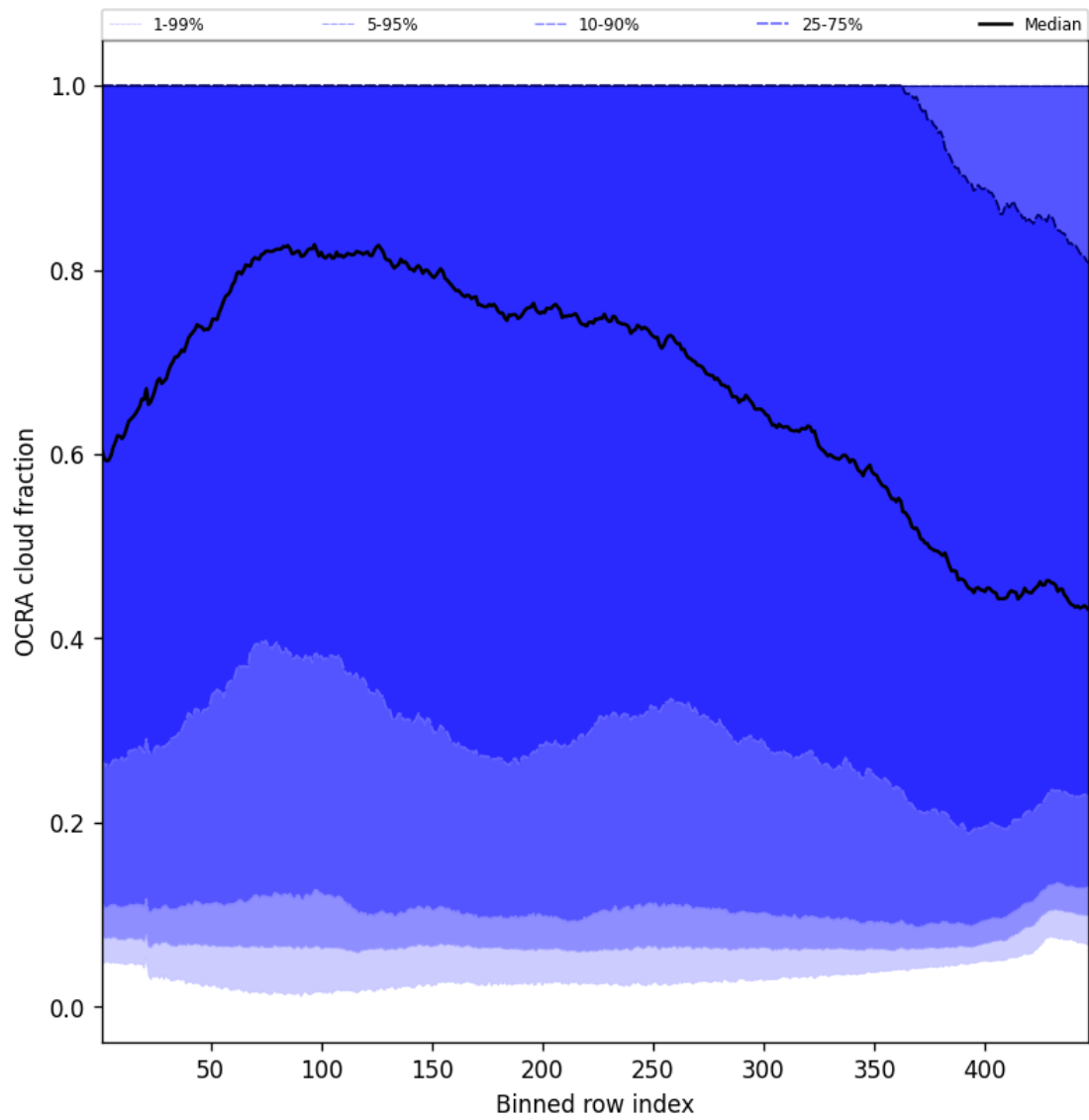
Figure 64: Along track statistics of “OCRA cloud fraction” for 2025-05-27 to 2025-05-28
