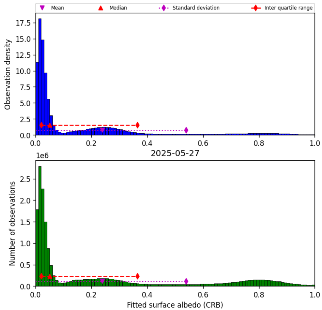
Figure 44: Histogram of “Fitted surface albedo (CRB)” for 2025-05-27 to 2025-05-28
