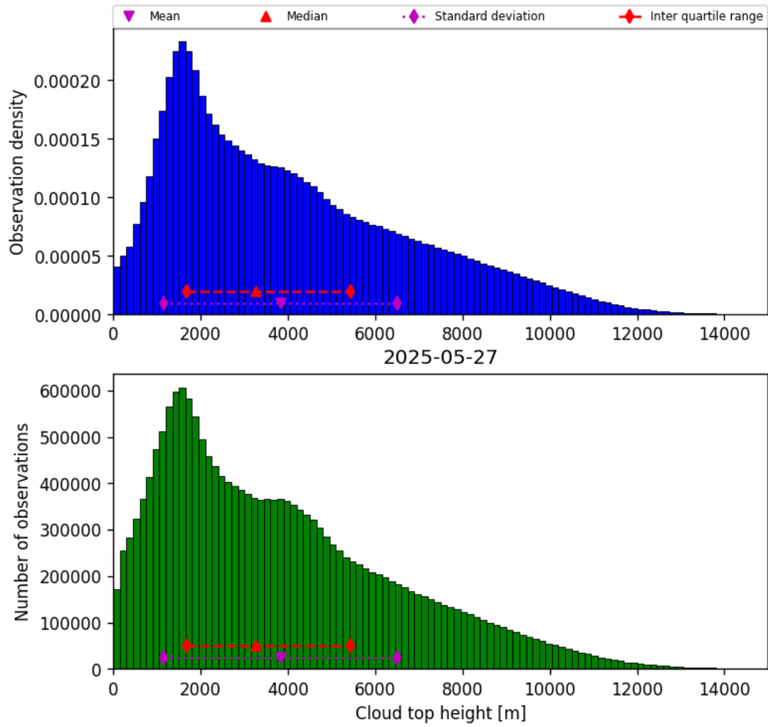
Figure 38: Histogram of “Cloud top height” for 2025-05-27 to 2025-05-28
