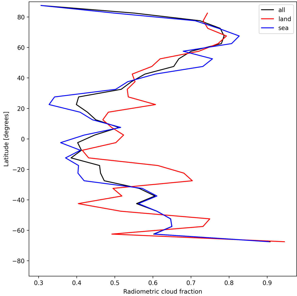
Figure 21: Zonal average of “Radiometric cloud fraction” for 2025-05-27 to 2025-05-28.
