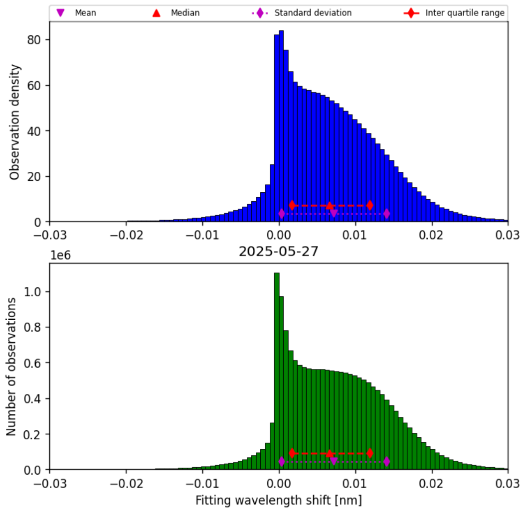
Figure 47: Histogram of “Fitting wavelength shift” for 2025-05-27 to 2025-05-28
