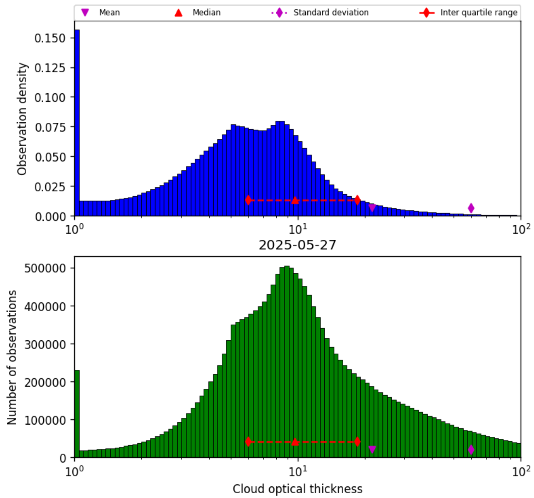
Figure 39: Histogram of “Cloud optical thickness” for 2025-05-27 to 2025-05-28
