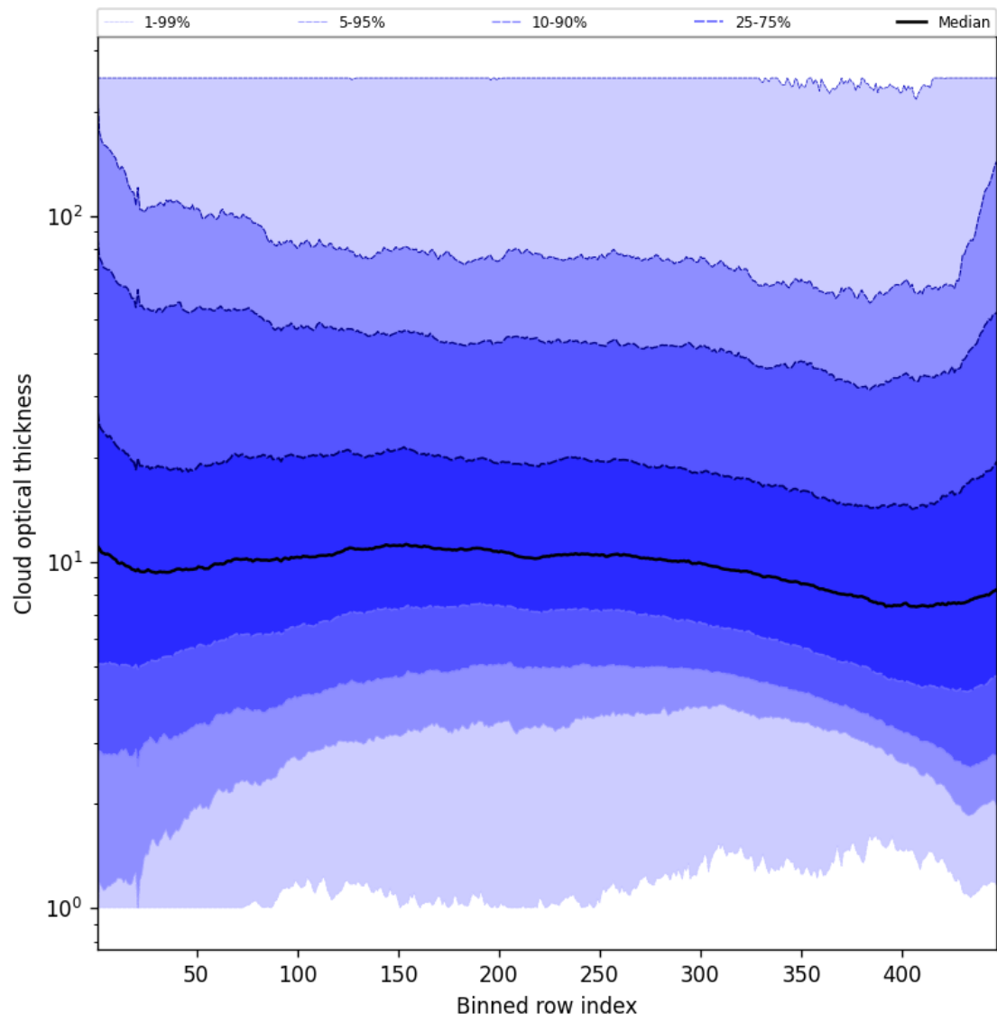
Figure 55: Along track statistics of “Cloud optical thickness” for 2025-05-27 to 2025-05-28
