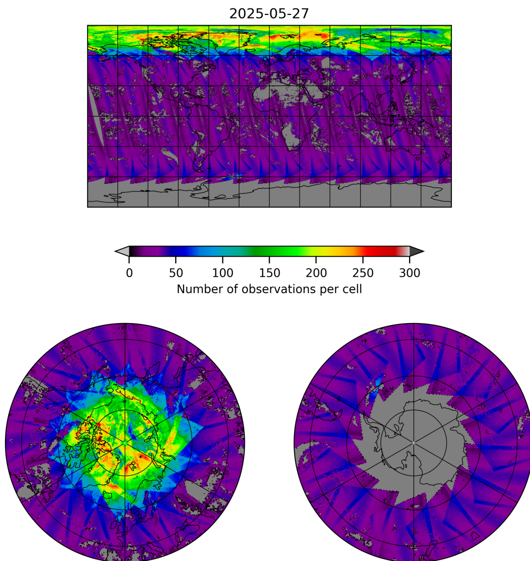
Figure 19: Map of the number of observations for 2025-05-27 to 2025-05-28
