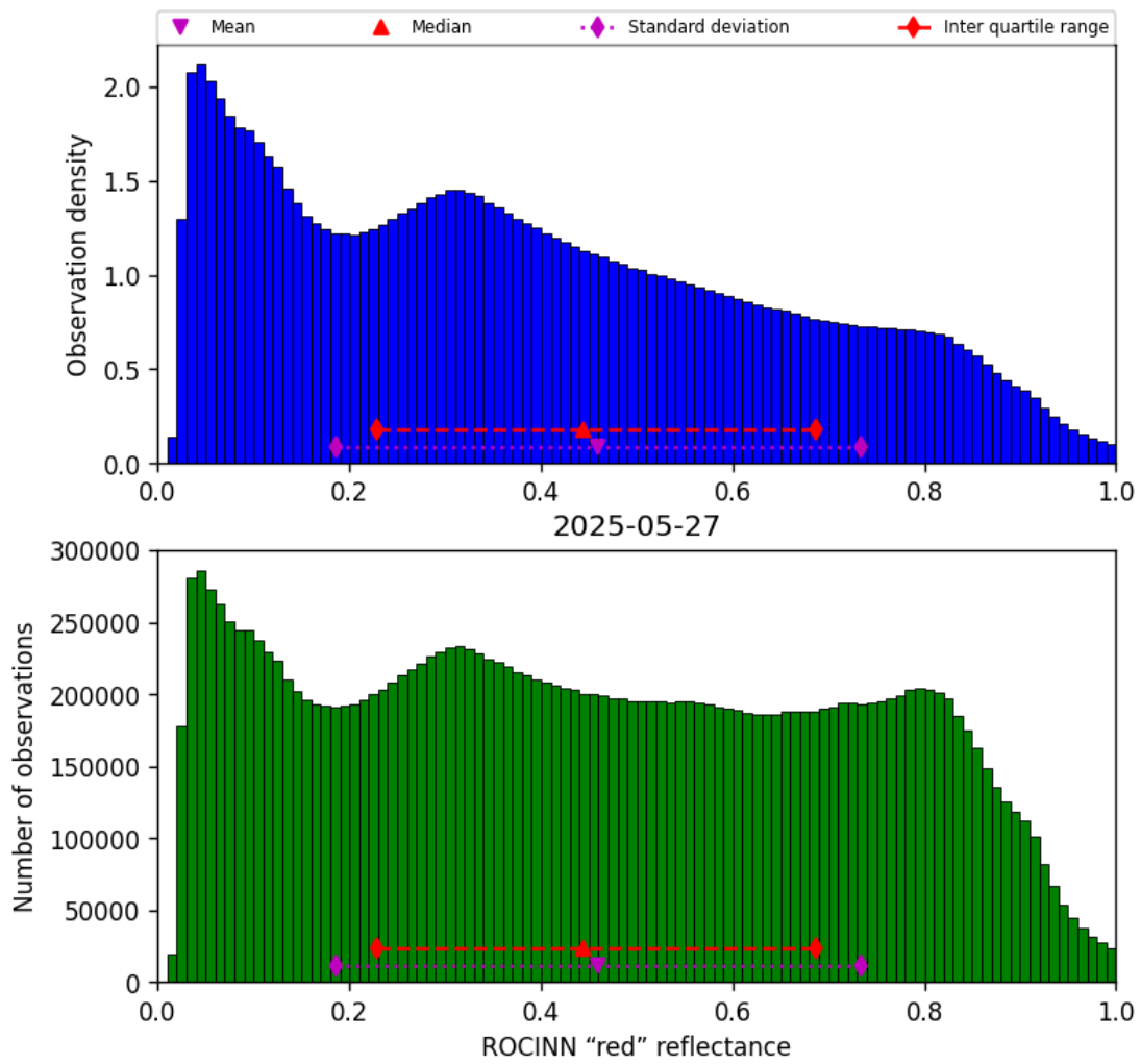
Figure 51: Histogram of “ROCINN “red” reflectance” for 2025-05-27 to 2025-05-28
