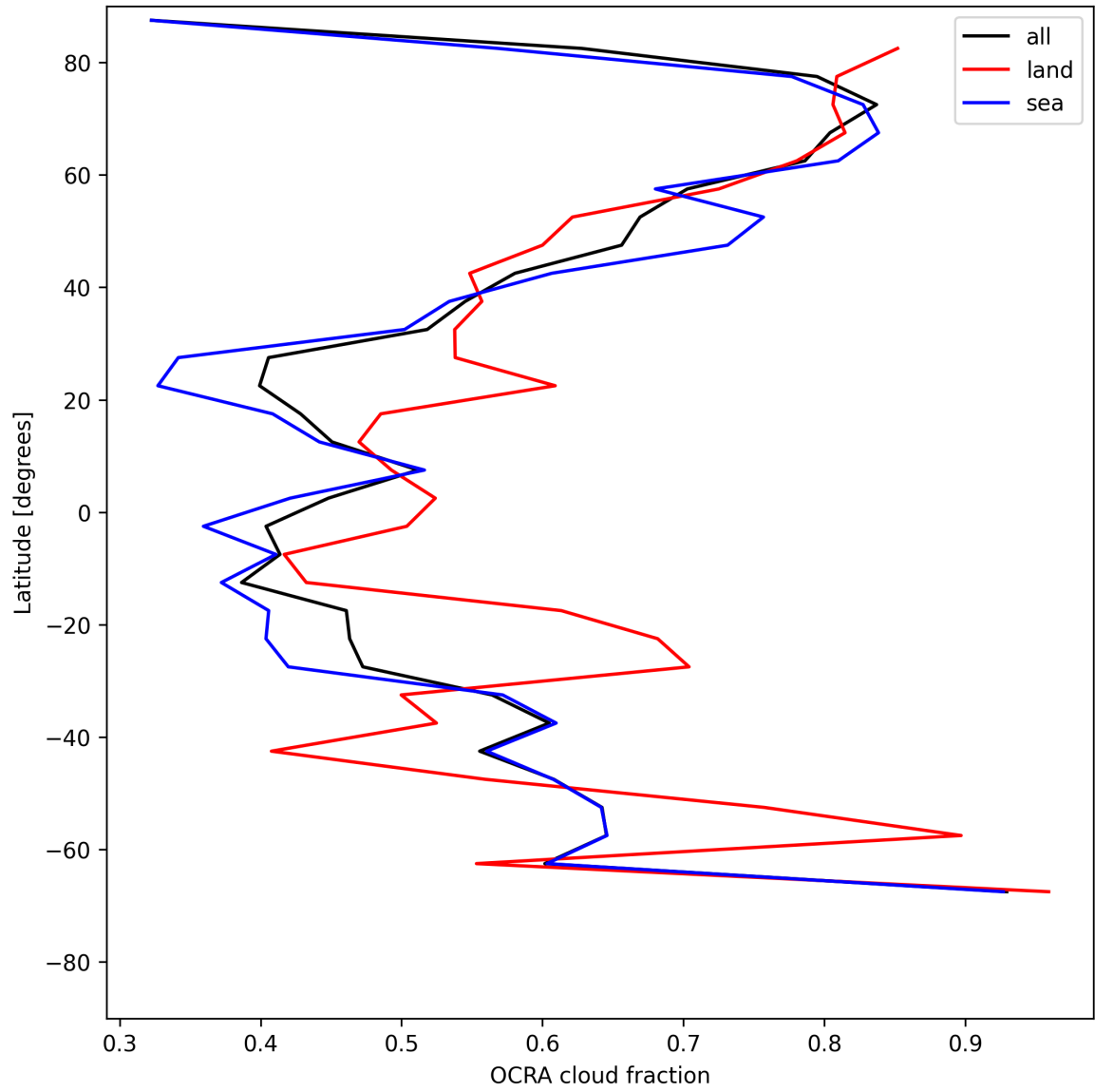
Figure 32: Zonal average of “OCRA cloud fraction” for 2025-05-27 to 2025-05-28.
