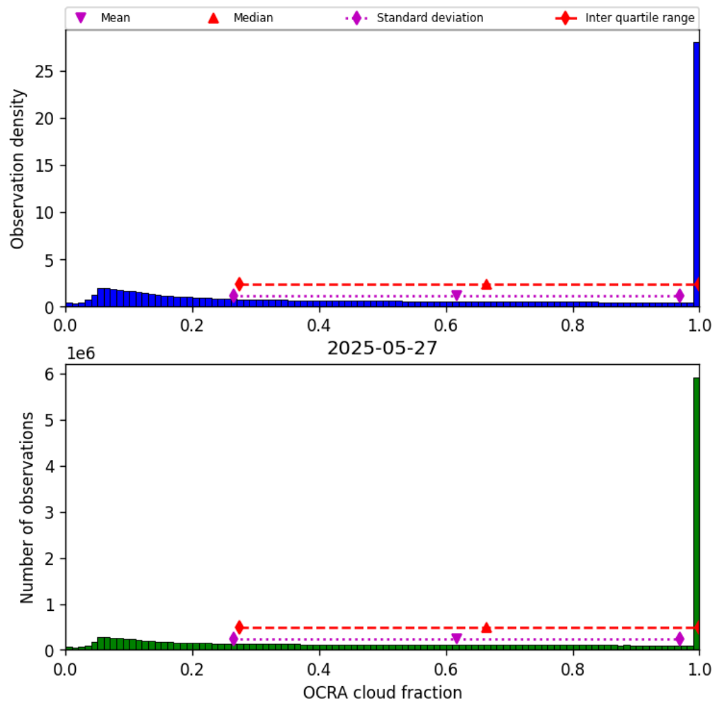
Figure 48: Histogram of “OCRA cloud fraction” for 2025-05-27 to 2025-05-28
