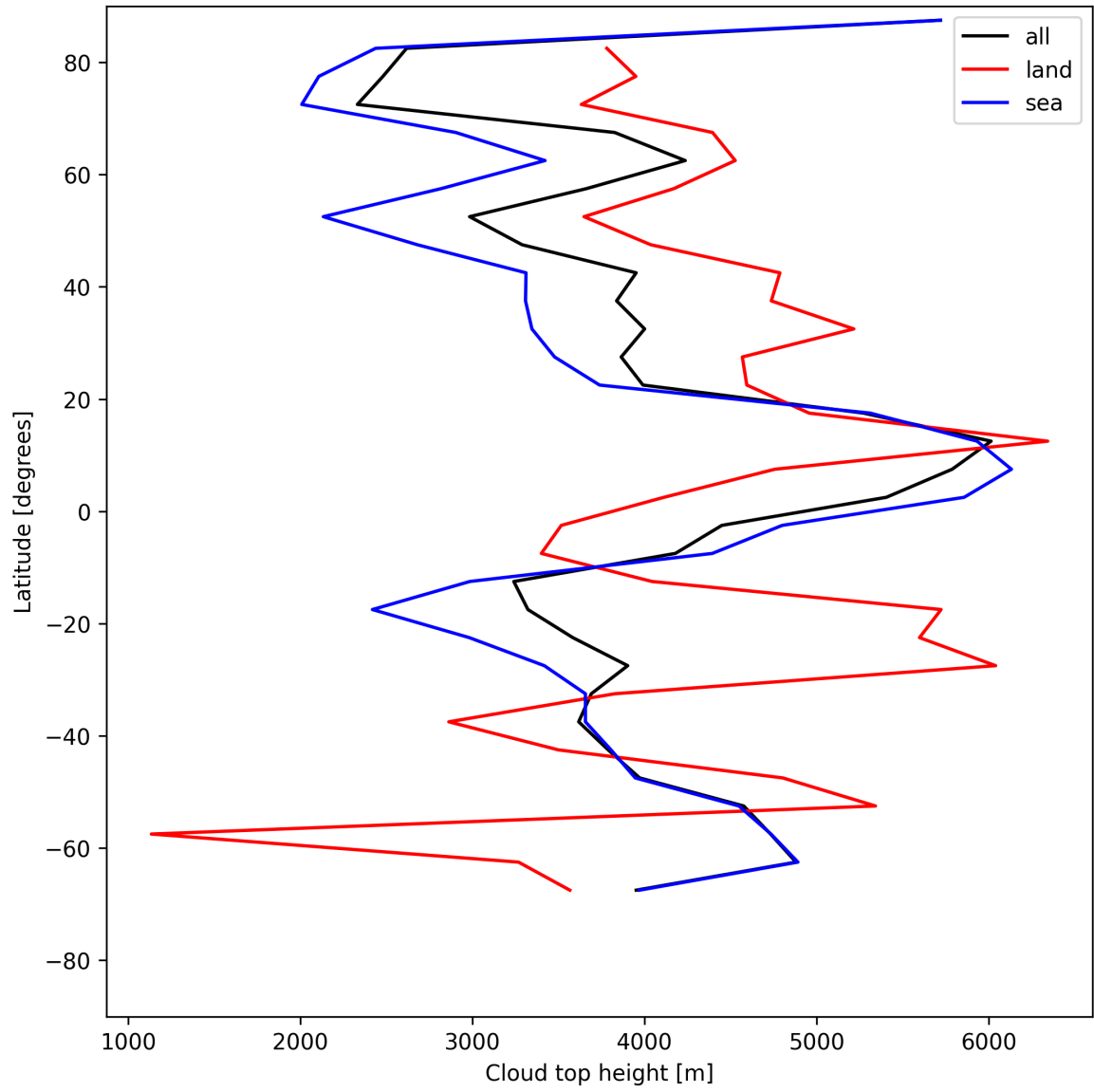
Figure 22: Zonal average of “Cloud top height” for 2025-05-27 to 2025-05-28.
