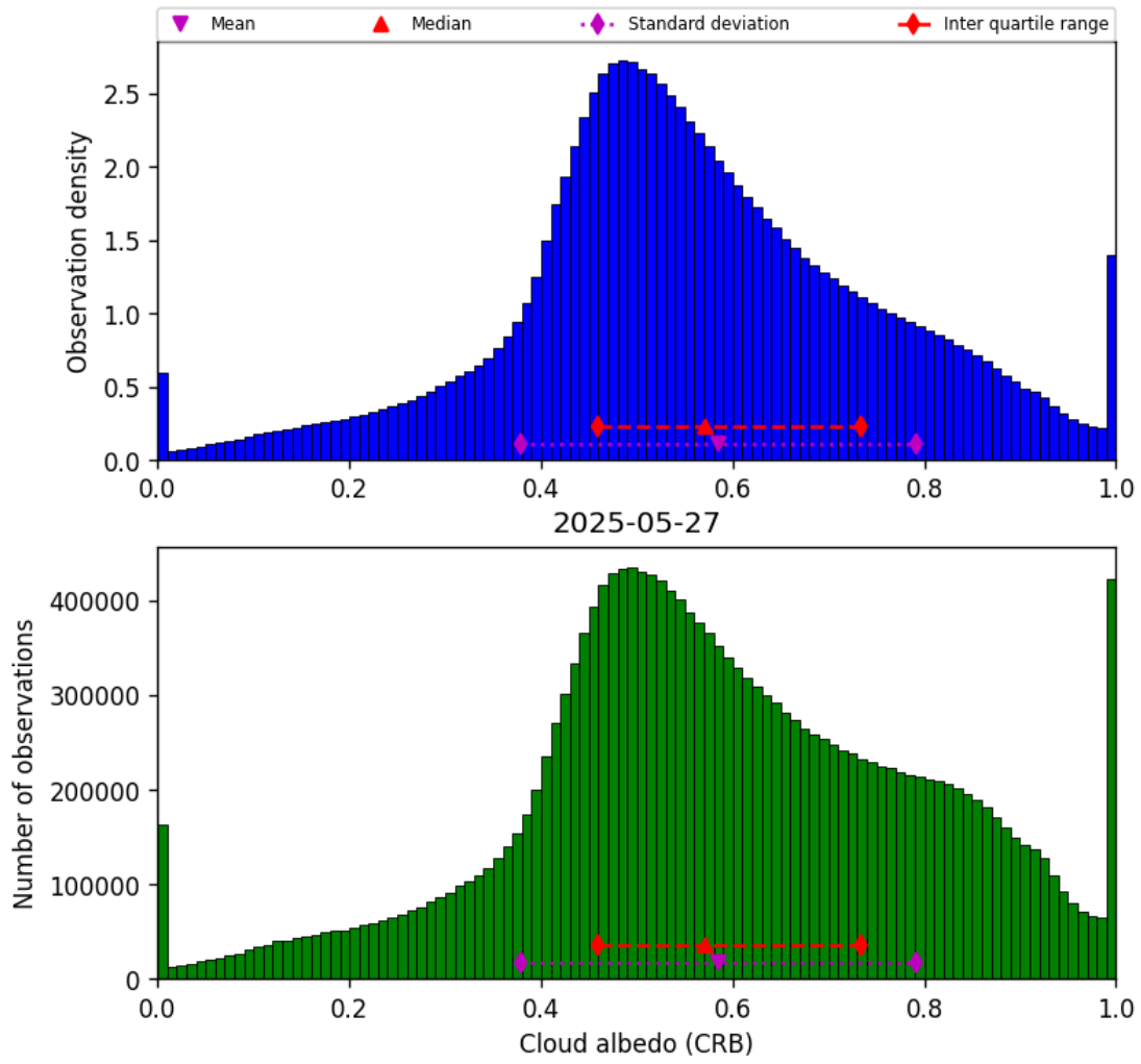
Figure 42: Histogram of “Cloud albedo (CRB)” for 2025-05-27 to 2025-05-28
