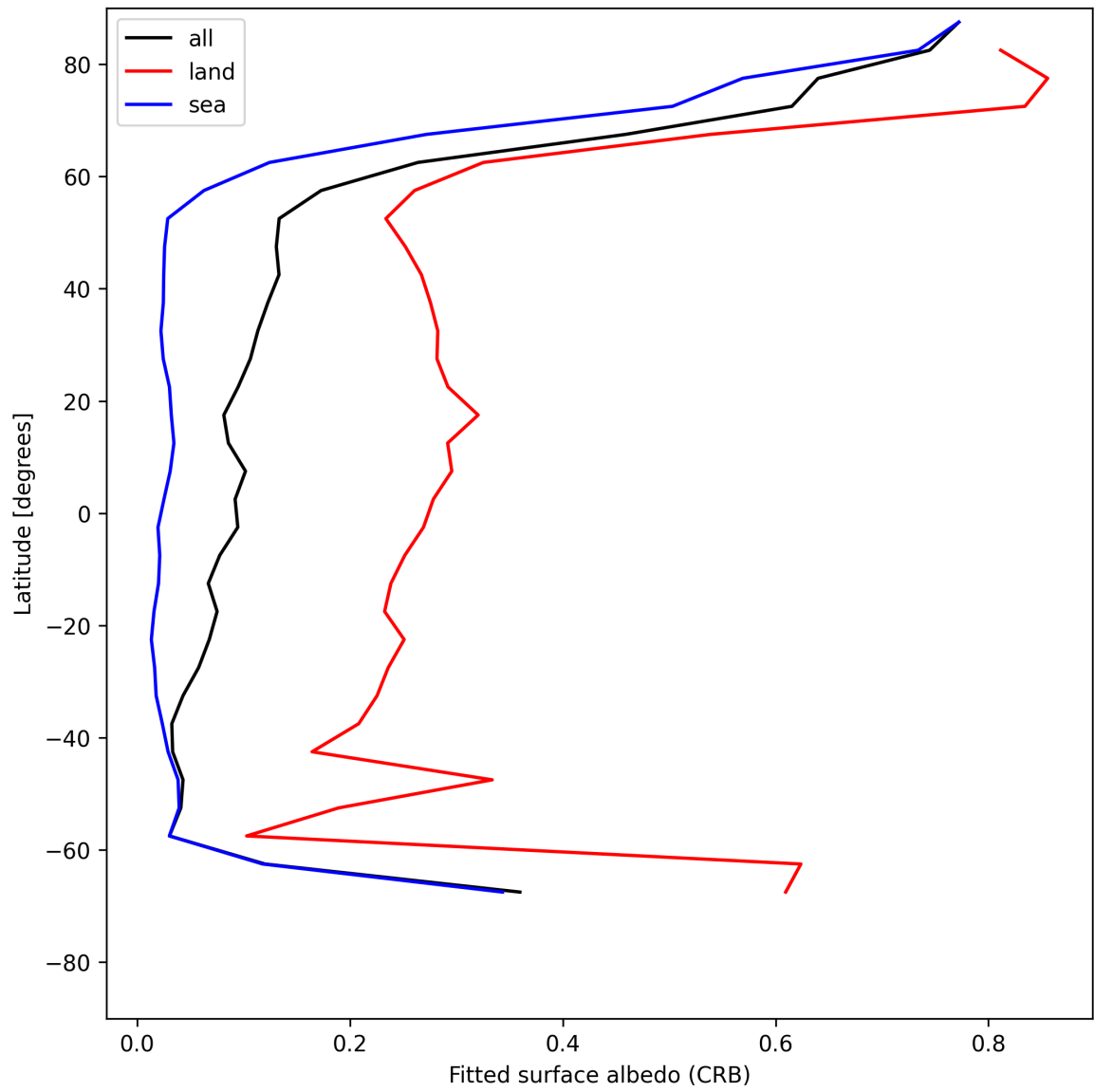
Figure 28: Zonal average of “Fitted surface albedo (CRB)” for 2025-05-27 to 2025-05-28.
