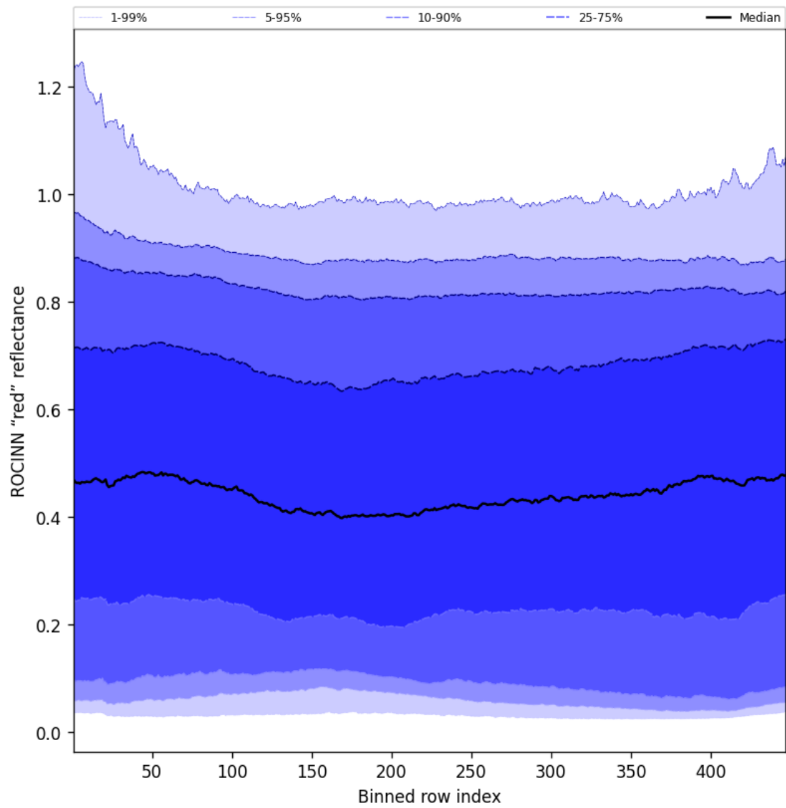
Figure 67: Along track statistics of "ROCINN "red" reflectance" for 2025-05-28 to 2025-05-29
