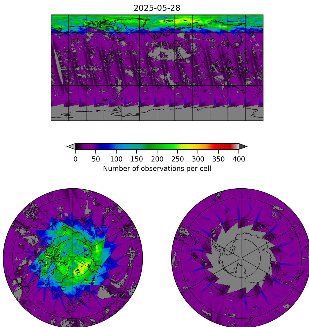
Figure 19: Map of the number of observations for 2025-05-28 to 2025-05-29
