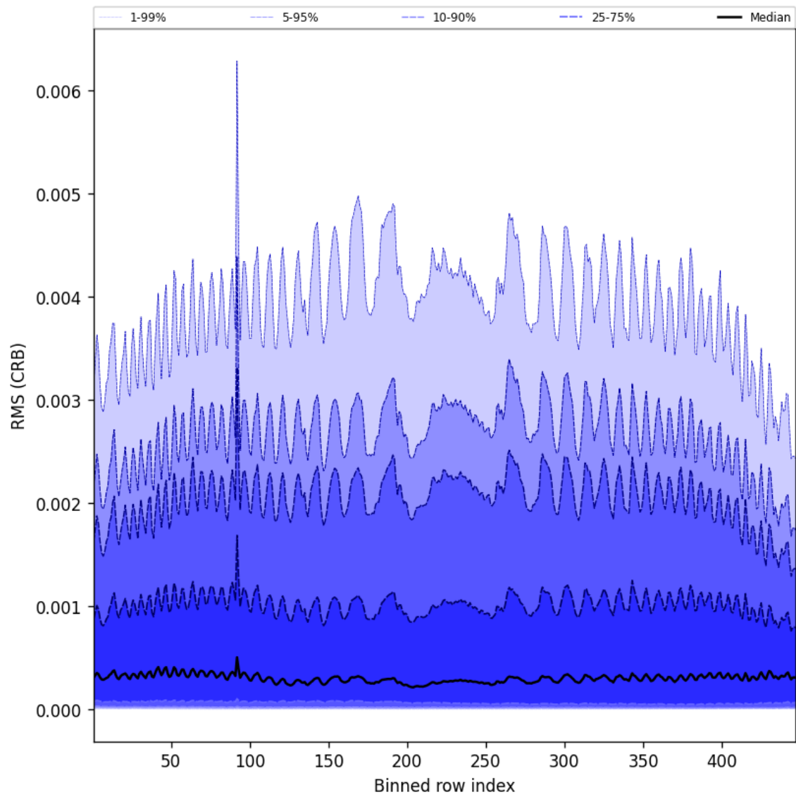
Figure 62: Along track statistics of “RMS (CRB)” for 2025-05-28 to 2025-05-29
