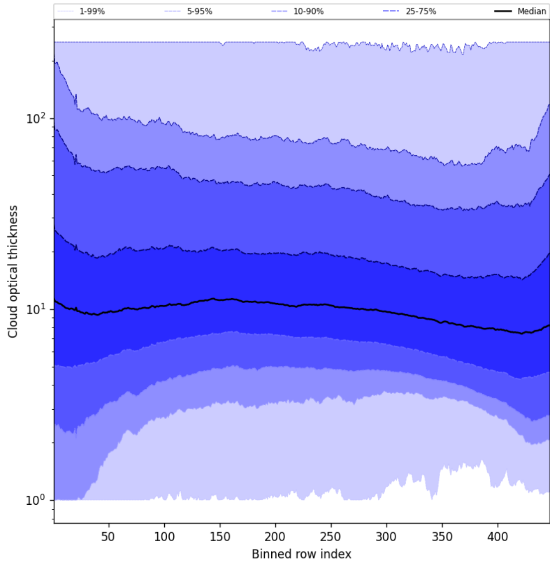
Figure 55: Along track statistics of “Cloud optical thickness” for 2025-05-28 to 2025-05-29
