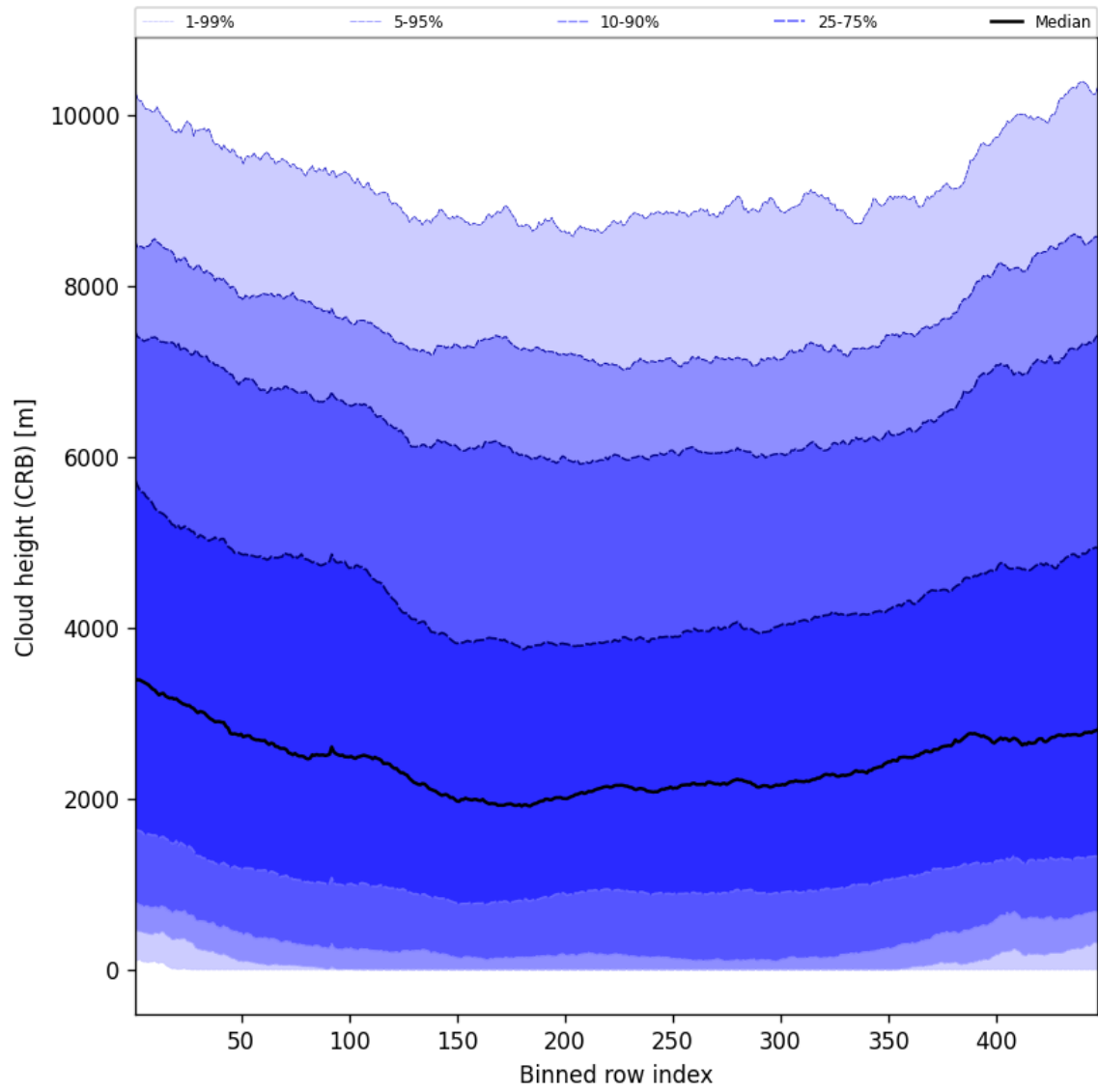
Figure 57: Along track statistics of “Cloud height (CRB)” for 2025-05-28 to 2025-05-29
