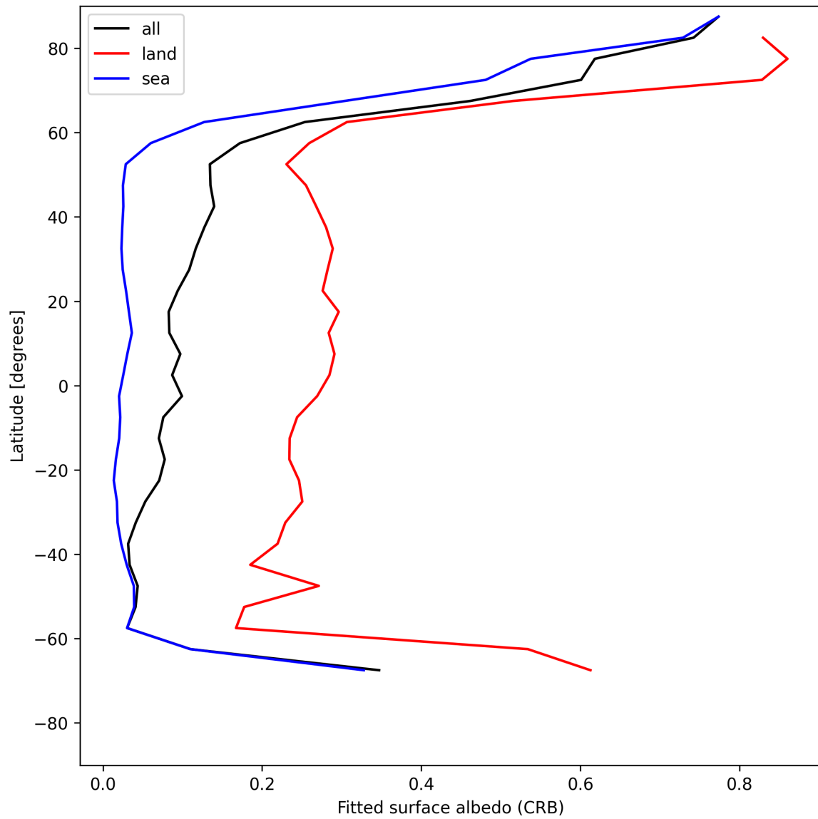
Figure 28: Zonal average of “Fitted surface albedo (CRB)” for 2025-05-28 to 2025-05-29.
