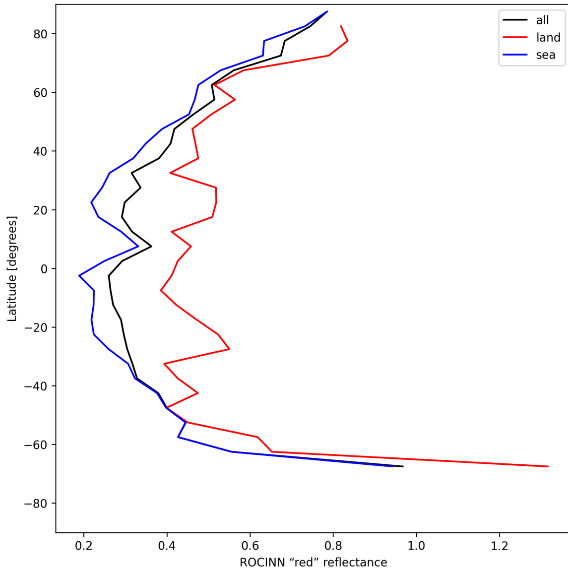
Figure 35: Zonal average of “ROCINN “red” reflectance” for 2025-05-28 to 2025-05-29.
