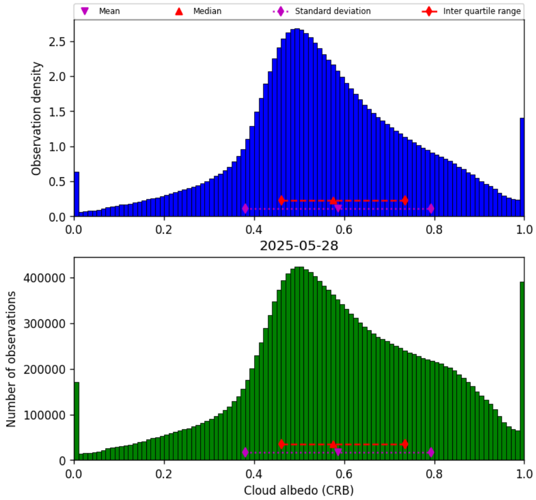
Figure 42: Histogram of “Cloud albedo (CRB)” for 2025-05-28 to 2025-05-29
