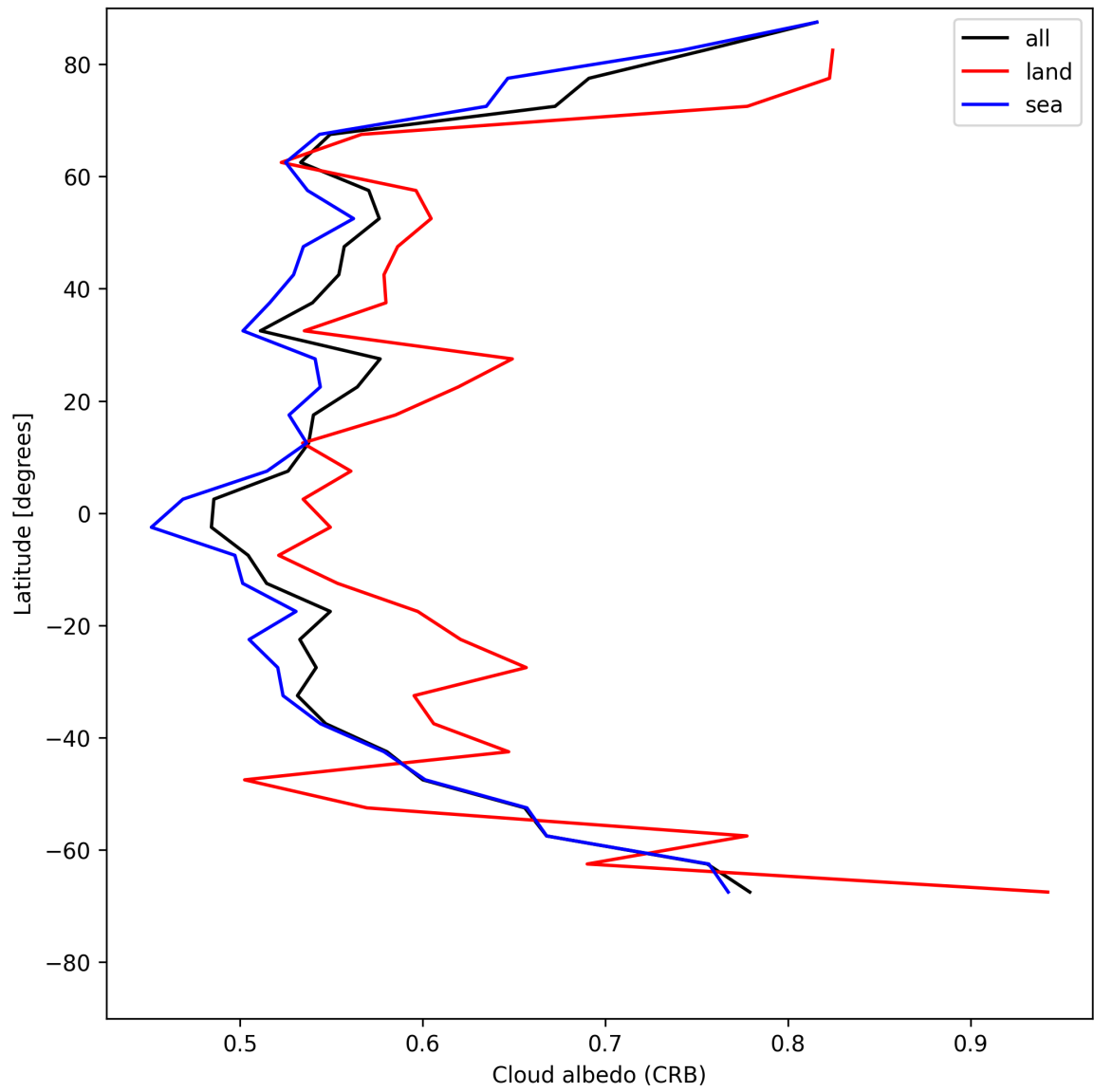
Figure 26: Zonal average of “Cloud albedo (CRB)” for 2025-05-28 to 2025-05-29.
