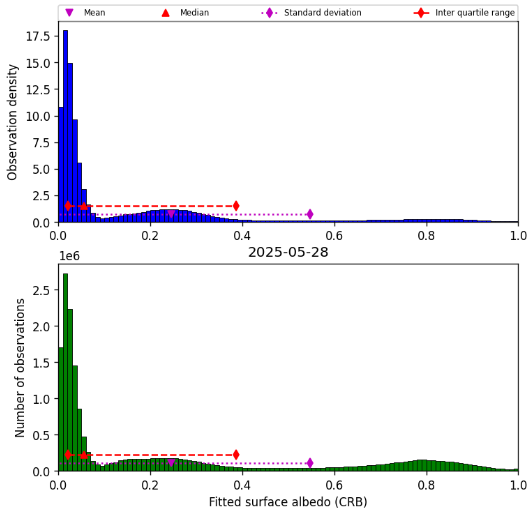
Figure 44: Histogram of “Fitted surface albedo (CRB)” for 2025-05-28 to 2025-05-29
