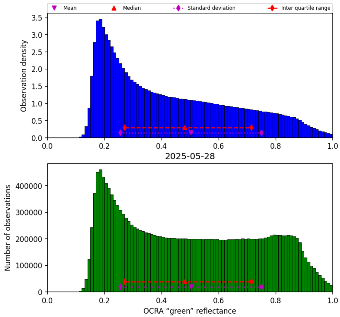
Figure 50: Histogram of “OCRA “green” reflectance” for 2025-05-28 to 2025-05-29
