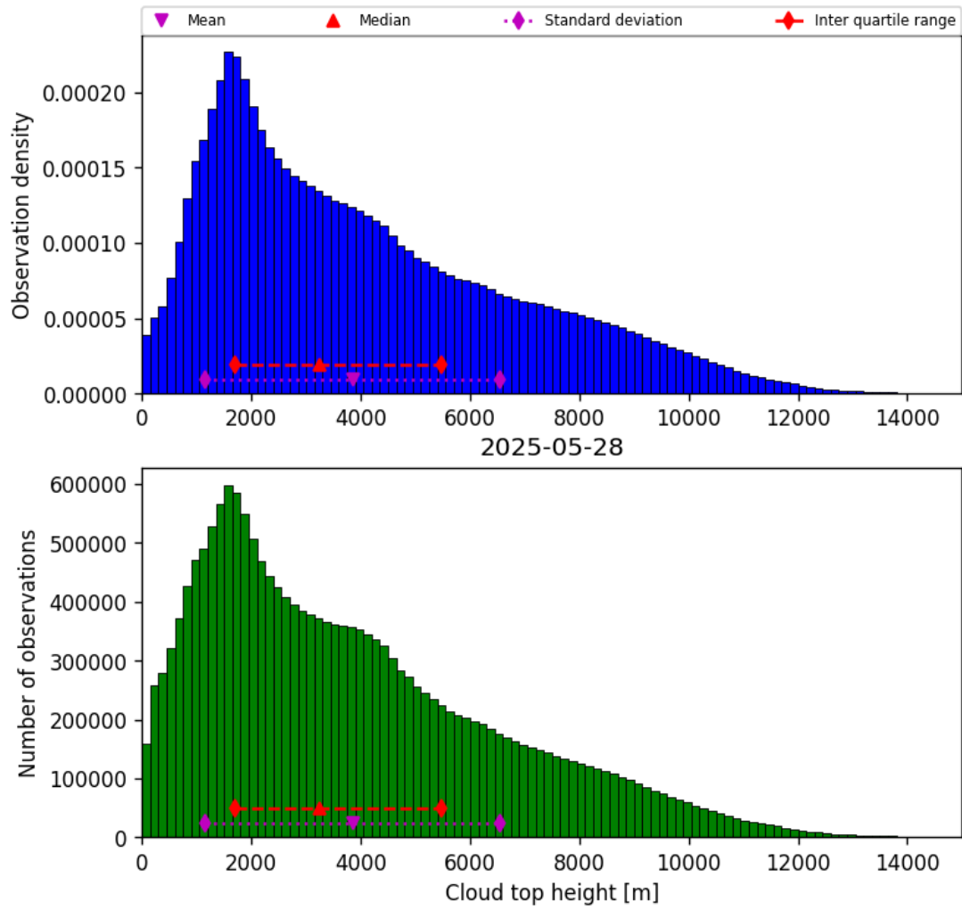
Figure 38: Histogram of “Cloud top height” for 2025-05-28 to 2025-05-29
