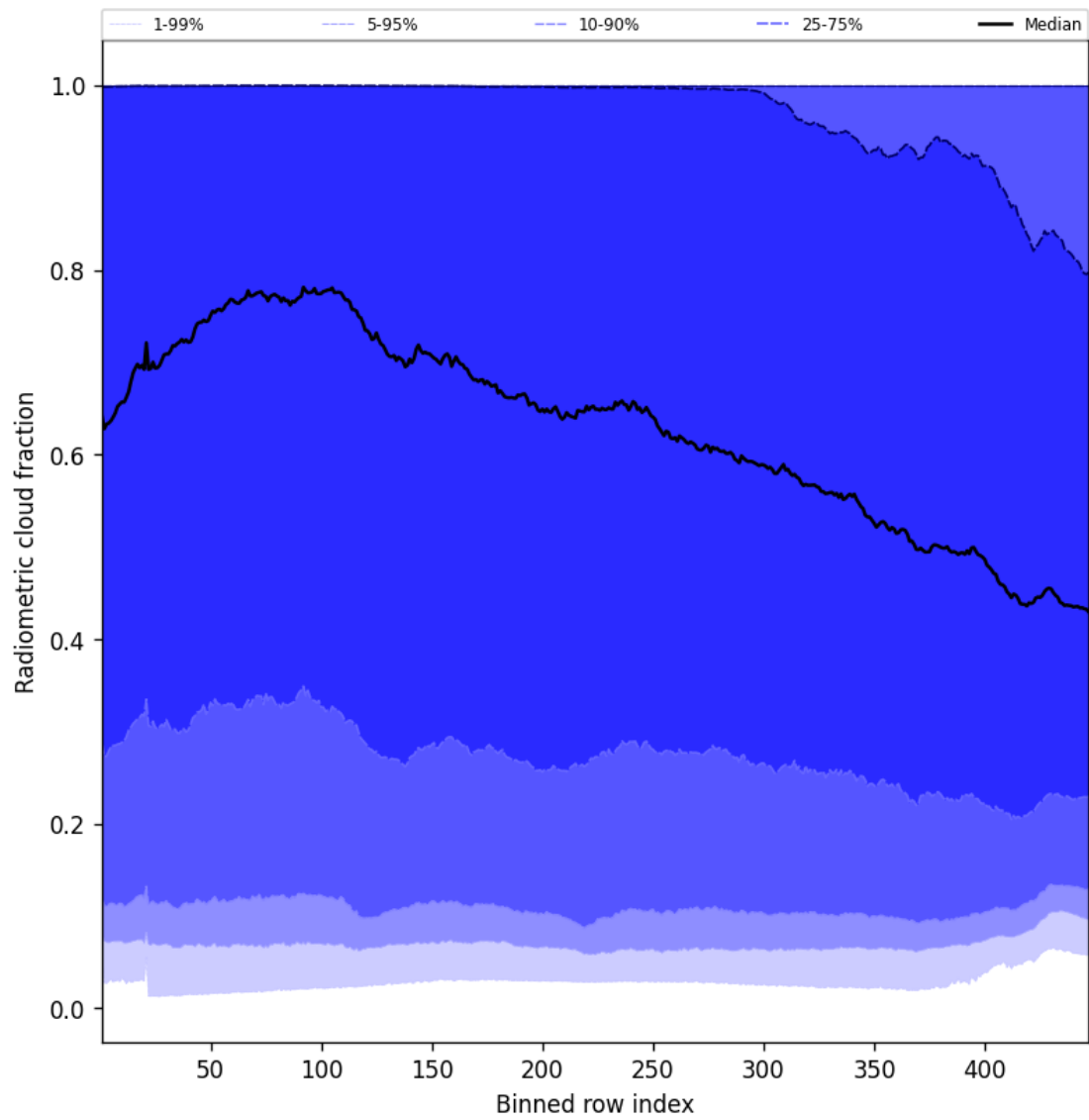
Figure 53: Along track statistics of “Radiometric cloud fraction” for 2025-05-28 to 2025-05-29
