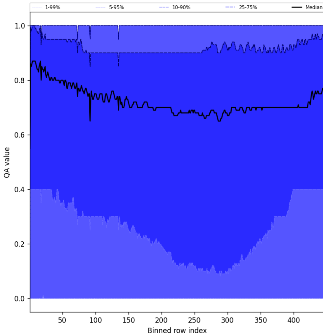
Figure 52: Along track statistics of “QA value” for 2025-05-28 to 2025-05-29
