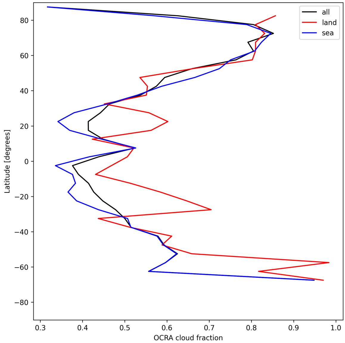
Figure 32: Zonal average of “OCRA cloud fraction” for 2025-05-28 to 2025-05-29.
