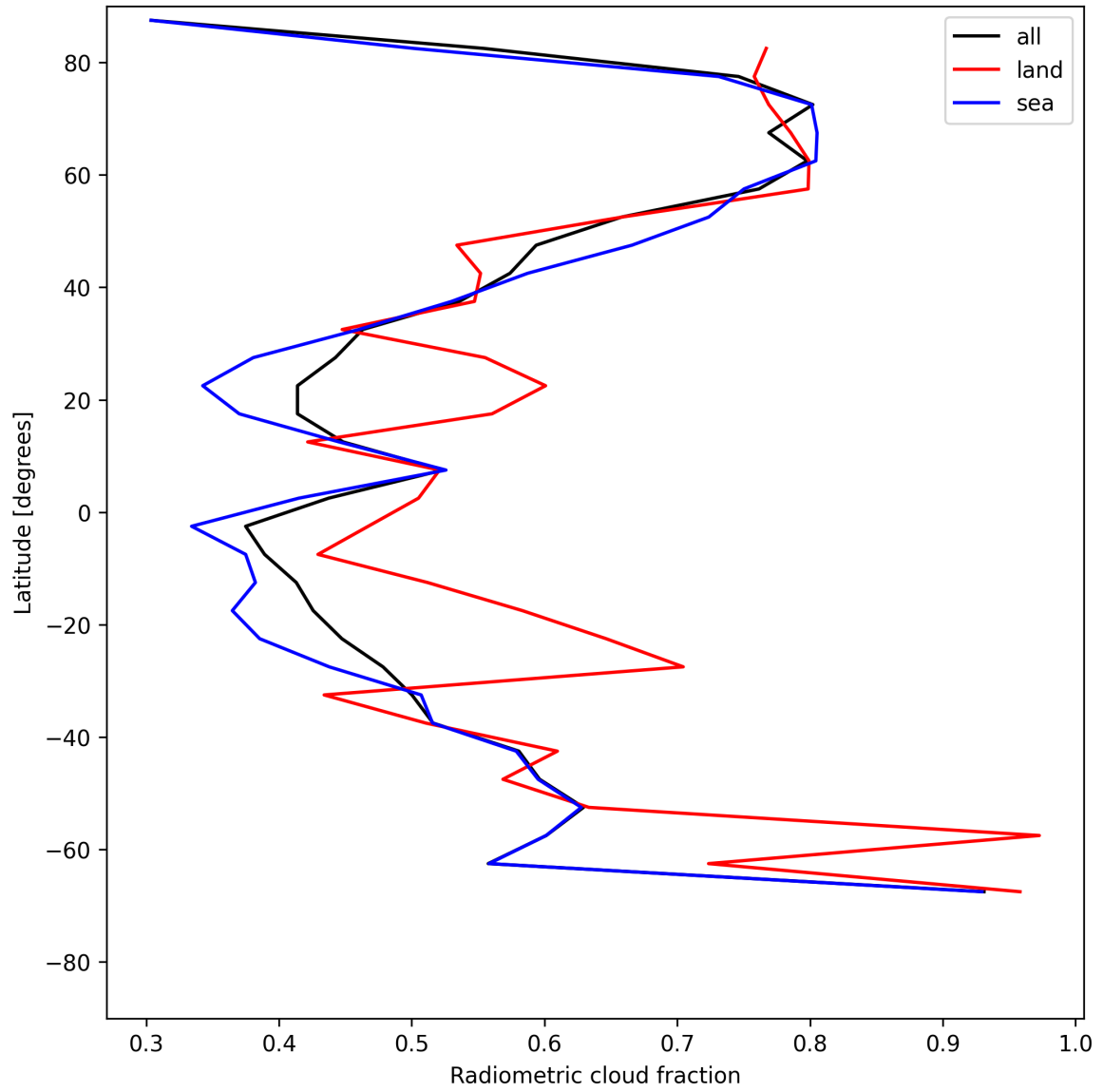
Figure 21: Zonal average of “Radiometric cloud fraction” for 2025-05-28 to 2025-05-29.
