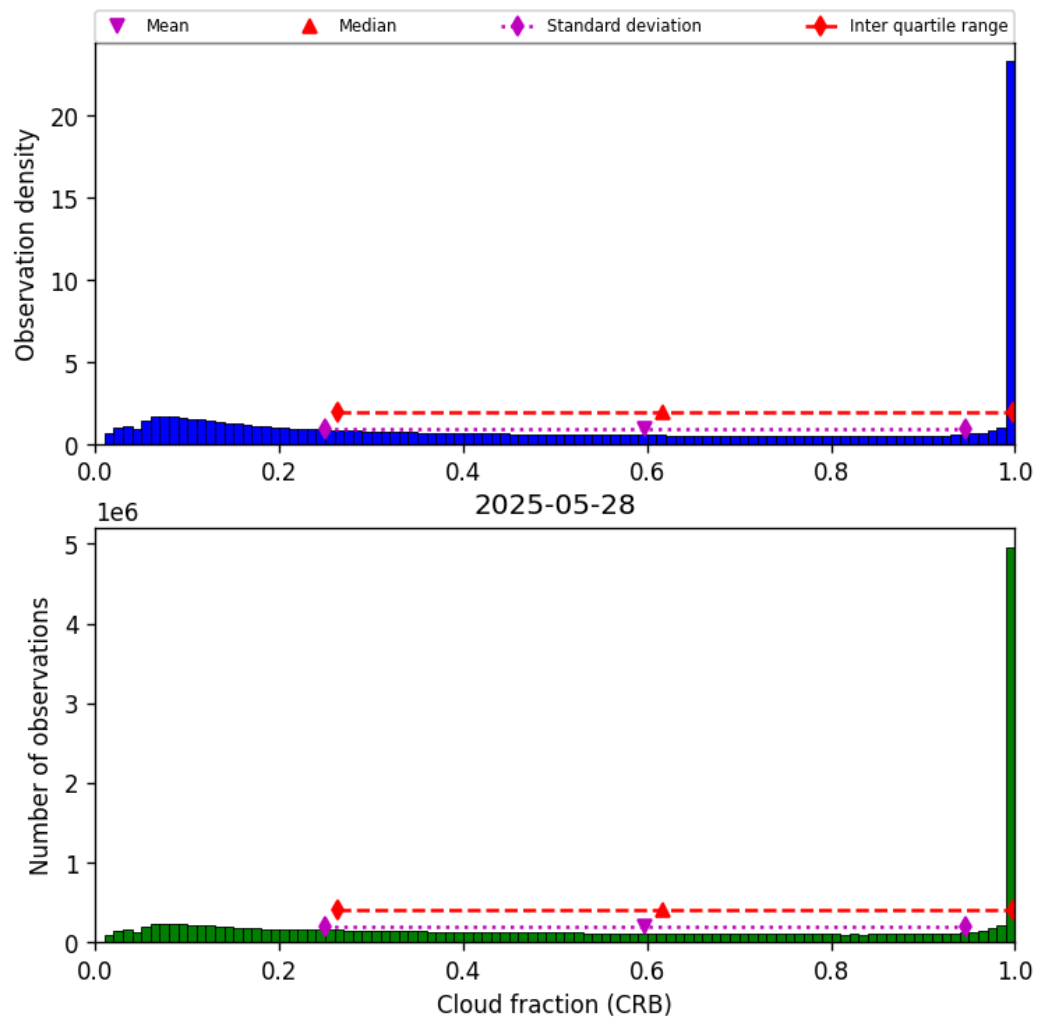
Figure 40: Histogram of “Cloud fraction (CRB)” for 2025-05-28 to 2025-05-29
