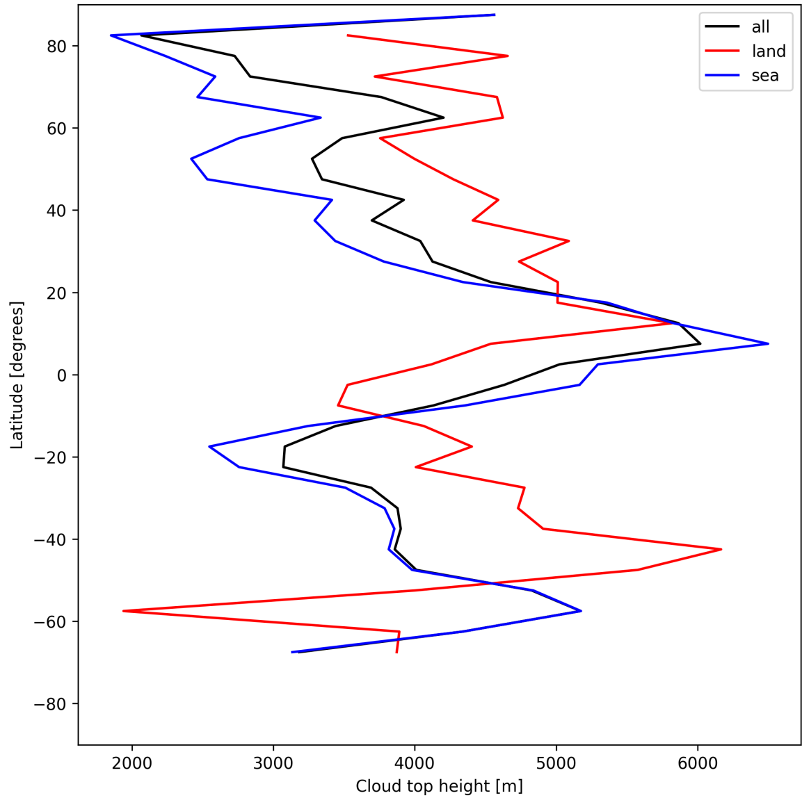
Figure 22: Zonal average of “Cloud top height” for 2025-05-28 to 2025-05-29.
