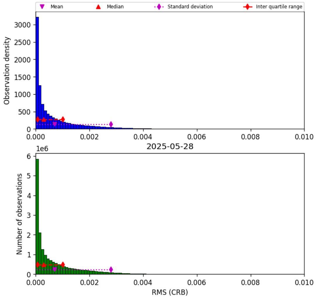
Figure 46: Histogram of “RMS (CRB)” for 2025-05-28 to 2025-05-29
