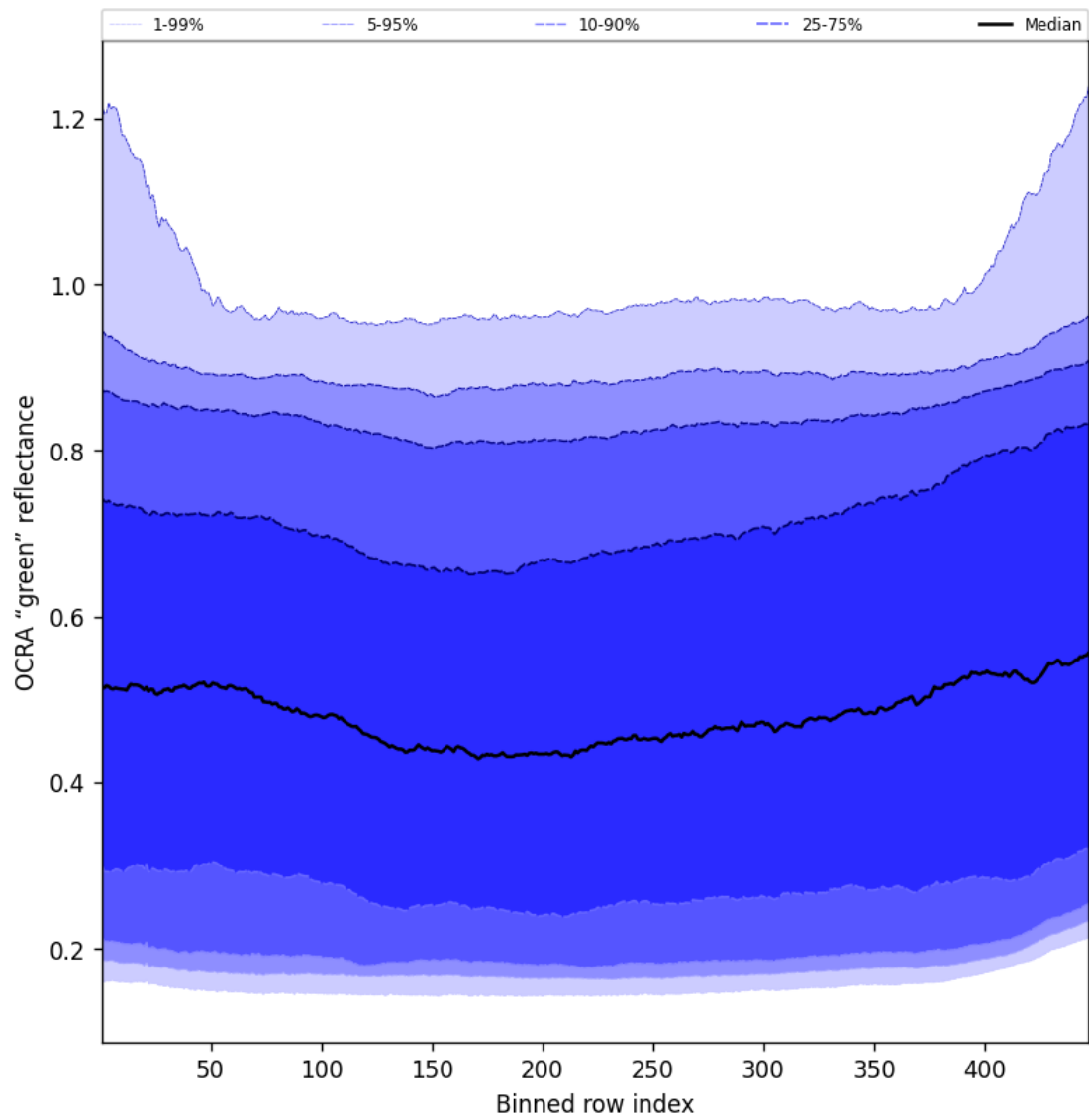
Figure 66: Along track statistics of “OCRA “green” reflectance” for 2025-05-28 to 2025-05-29
