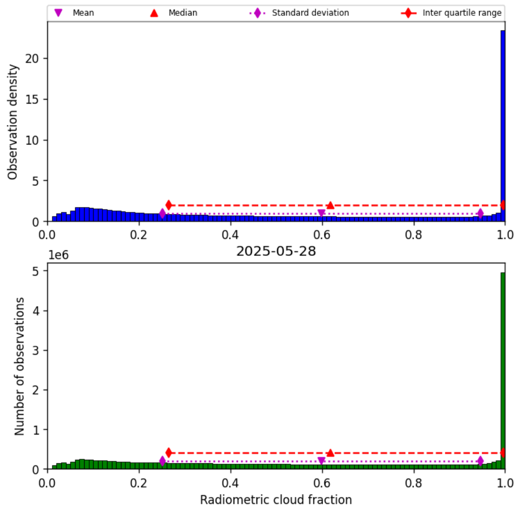
Figure 37: Histogram of “Radiometric cloud fraction” for 2025-05-28 to 2025-05-29
