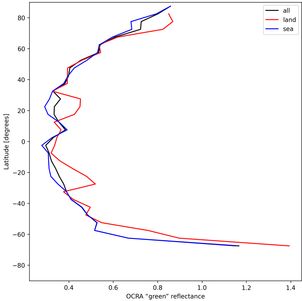
Figure 34: Zonal average of “OCRA “green” reflectance” for 2025-05-28 to 2025-05-29.
