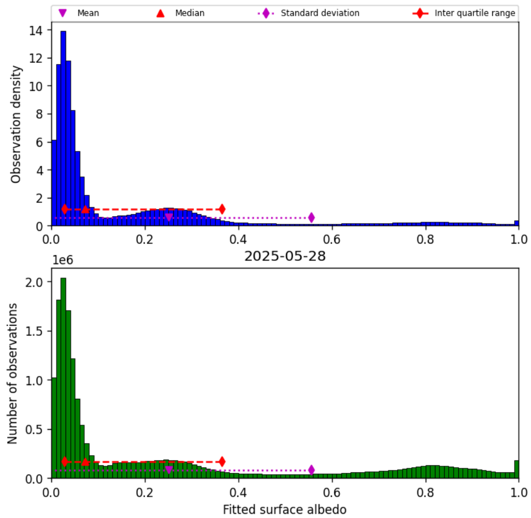
Figure 43: Histogram of “Fitted surface albedo” for 2025-05-28 to 2025-05-29
