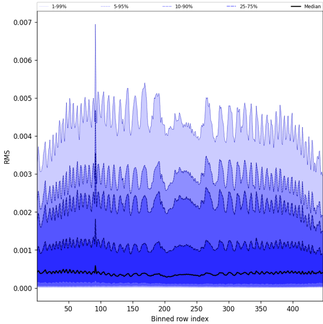
Figure 61: Along track statistics of “RMS” for 2025-05-28 to 2025-05-29
