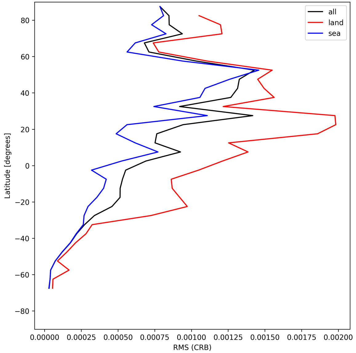
Figure 30: Zonal average of “RMS (CRB)” for 2025-05-28 to 2025-05-29.
