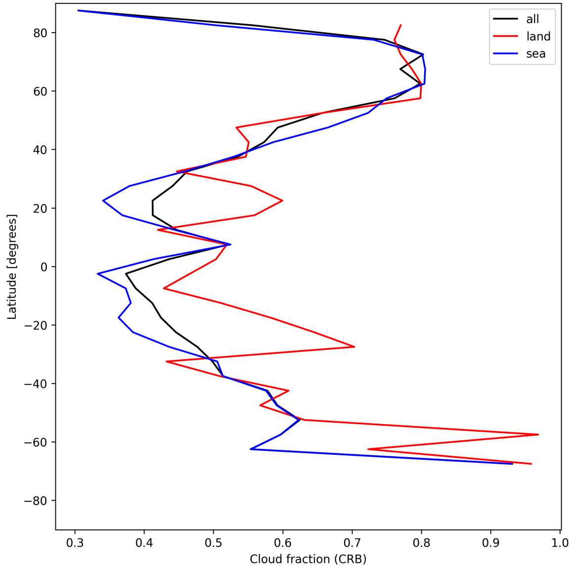
Figure 24: Zonal average of “Cloud fraction (CRB)” for 2025-05-28 to 2025-05-29.
