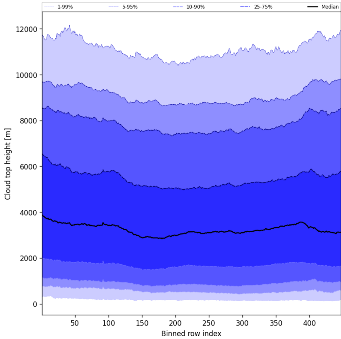
Figure 54: Along track statistics of “Cloud top height” for 2025-05-28 to 2025-05-29
