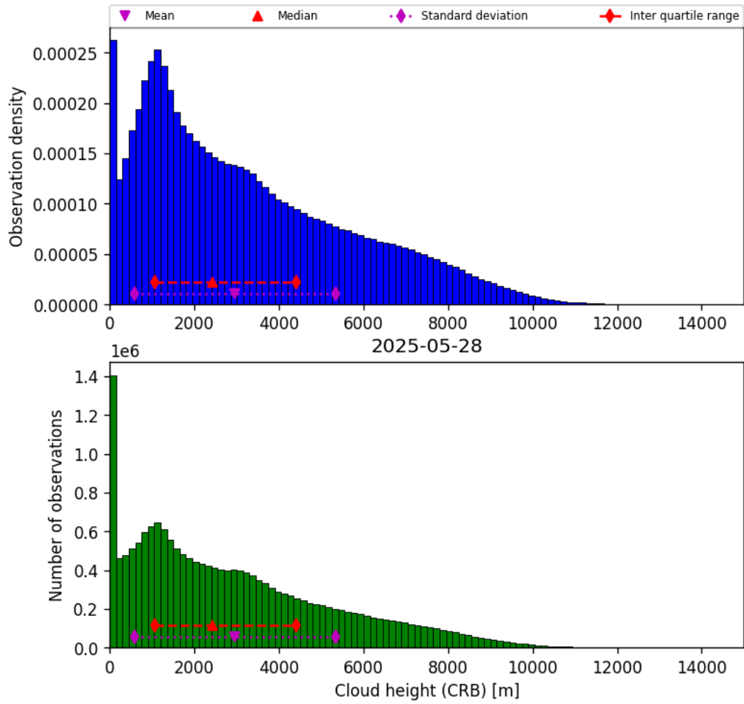
Figure 41: Histogram of “Cloud height (CRB)” for 2025-05-28 to 2025-05-29
