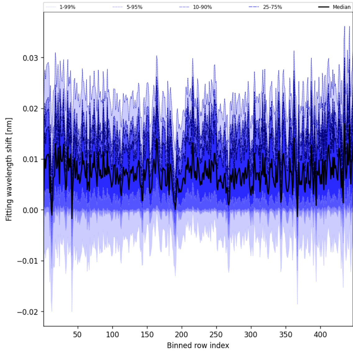
Figure 63: Along track statistics of “Fitting wavelength shift” for 2025-05-28 to 2025-05-29
