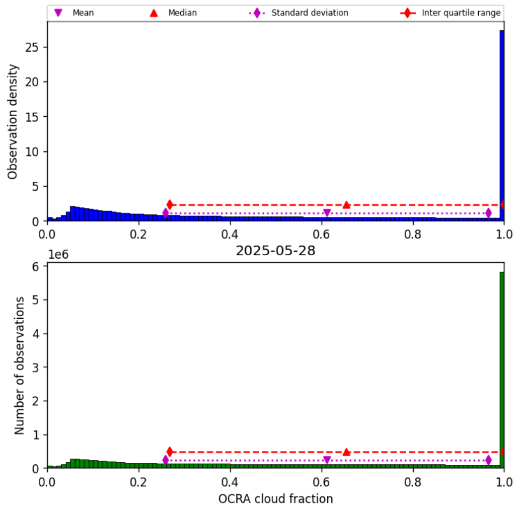
Figure 48: Histogram of “OCRA cloud fraction” for 2025-05-28 to 2025-05-29
