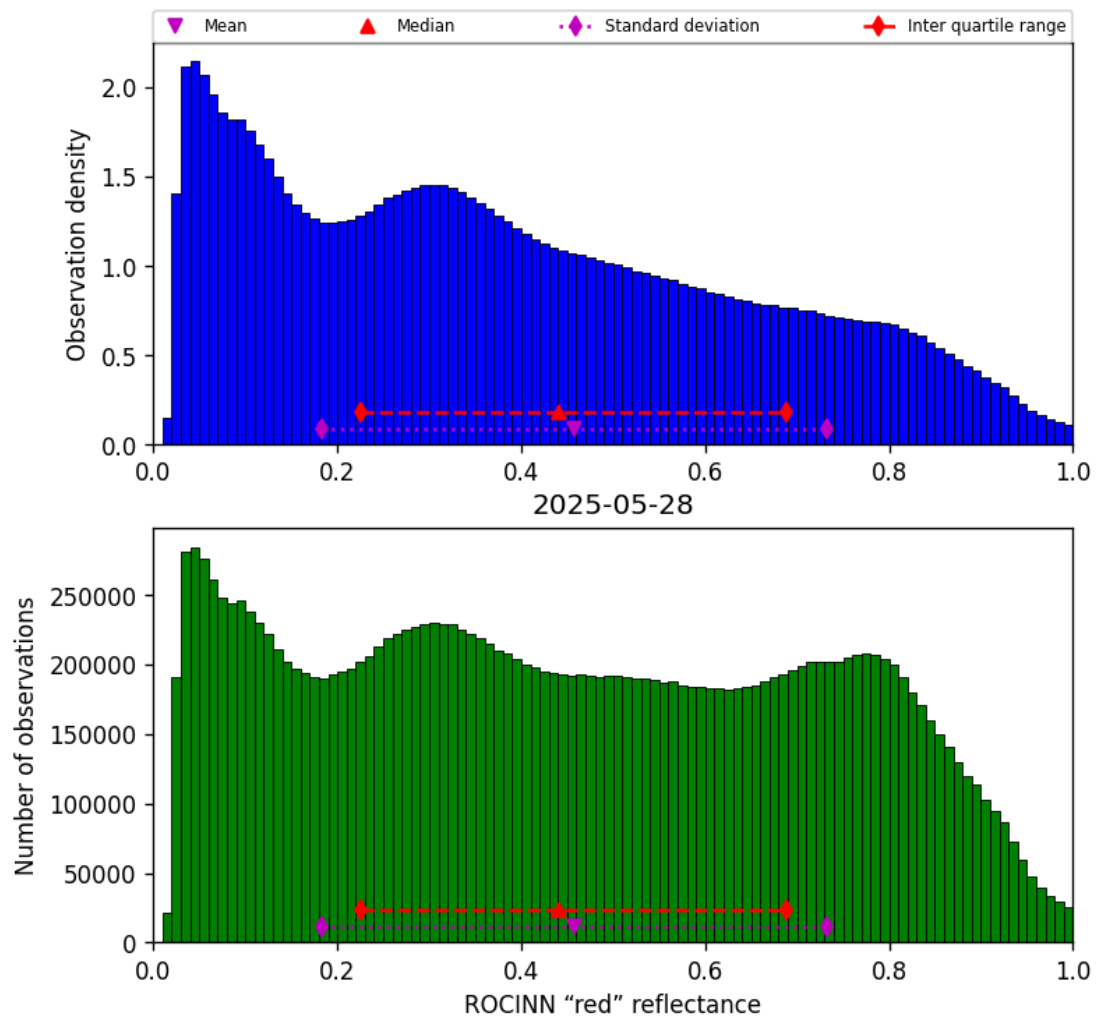
Figure 51: Histogram of “ROCINN “red” reflectance” for 2025-05-28 to 2025-05-29
