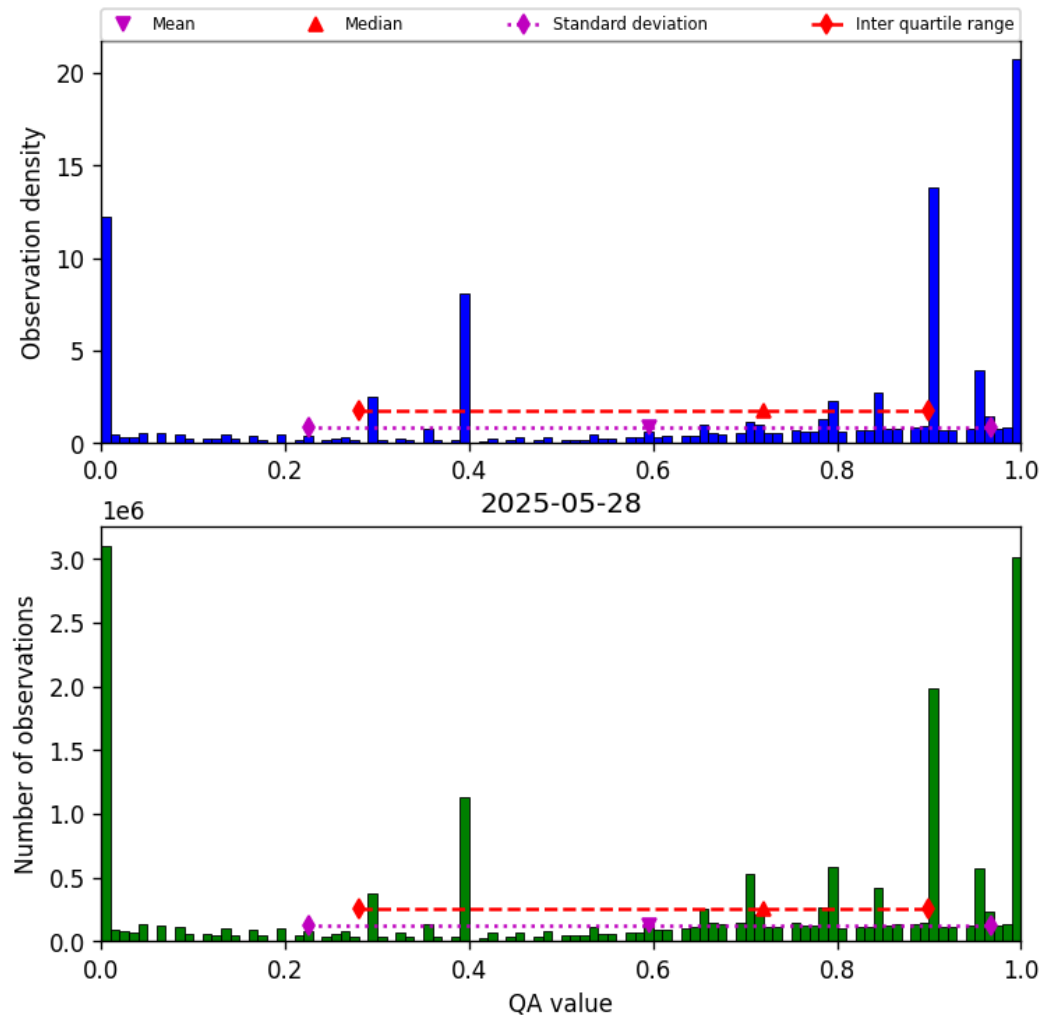
Figure 36: Histogram of “QA value” for 2025-05-28 to 2025-05-29
