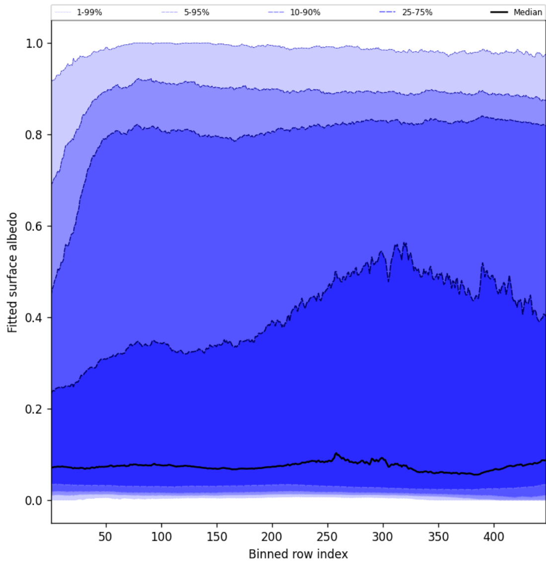
Figure 59: Along track statistics of “Fitted surface albedo” for 2025-05-28 to 2025-05-29
