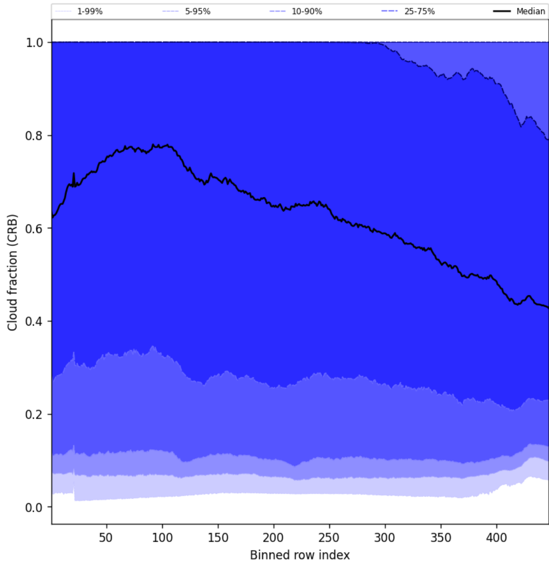
Figure 56: Along track statistics of “Cloud fraction (CRB)” for 2025-05-28 to 2025-05-29
