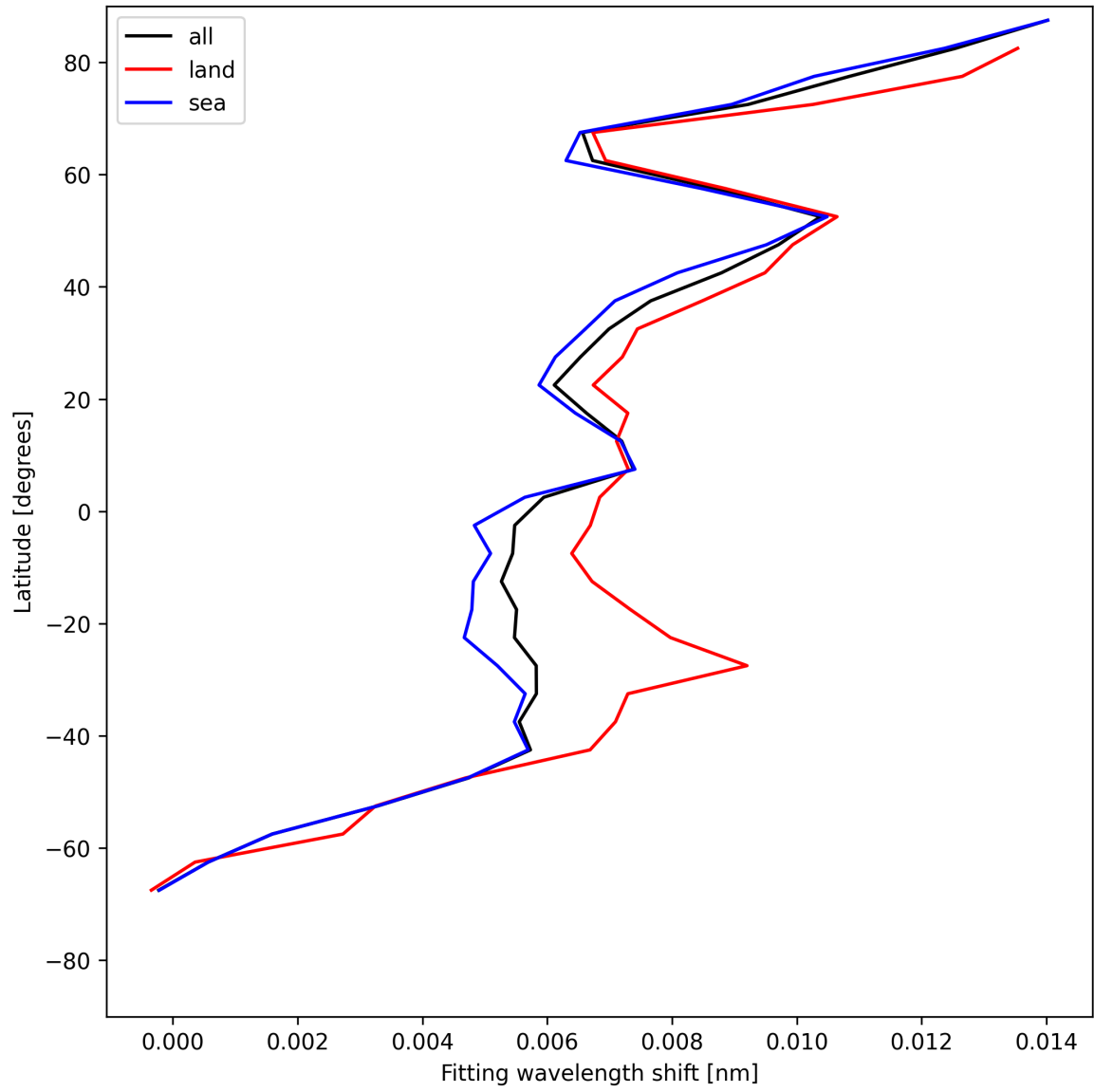
Figure 31: Zonal average of “Fitting wavelength shift” for 2025-05-28 to 2025-05-29.
