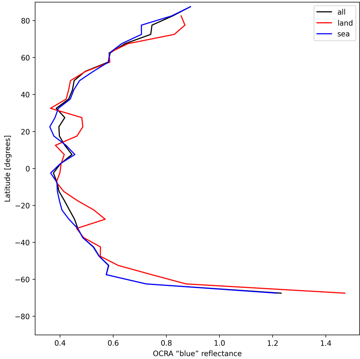
Figure 33: Zonal average of “OCRA “blue” reflectance” for 2025-05-28 to 2025-05-29.
