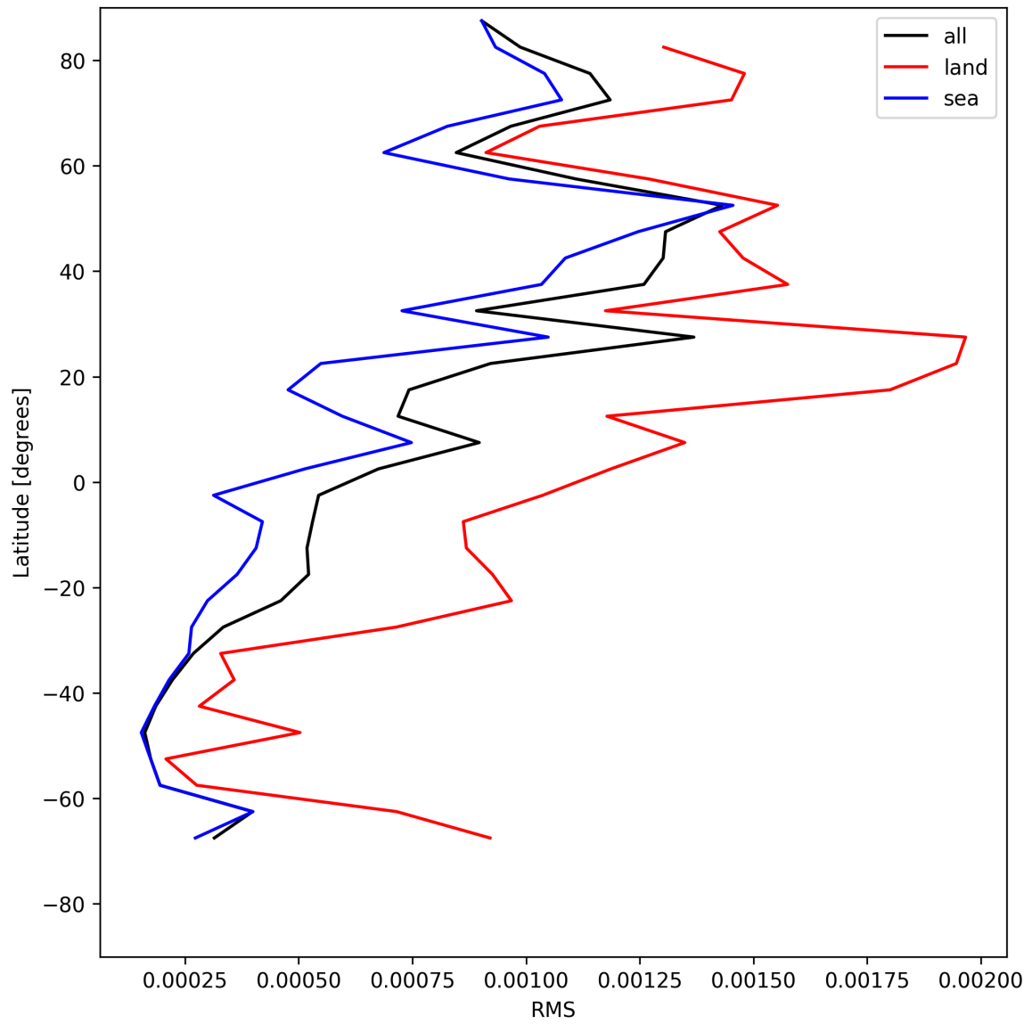
Figure 29: Zonal average of “RMS” for 2025-05-28 to 2025-05-29.
