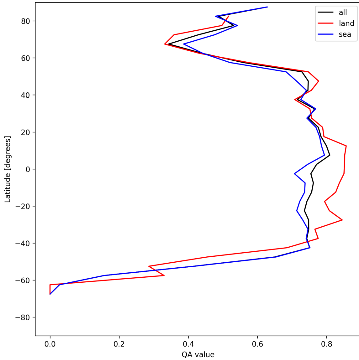
Figure 20: Zonal average of “QA value” for 2025-05-28 to 2025-05-29.
