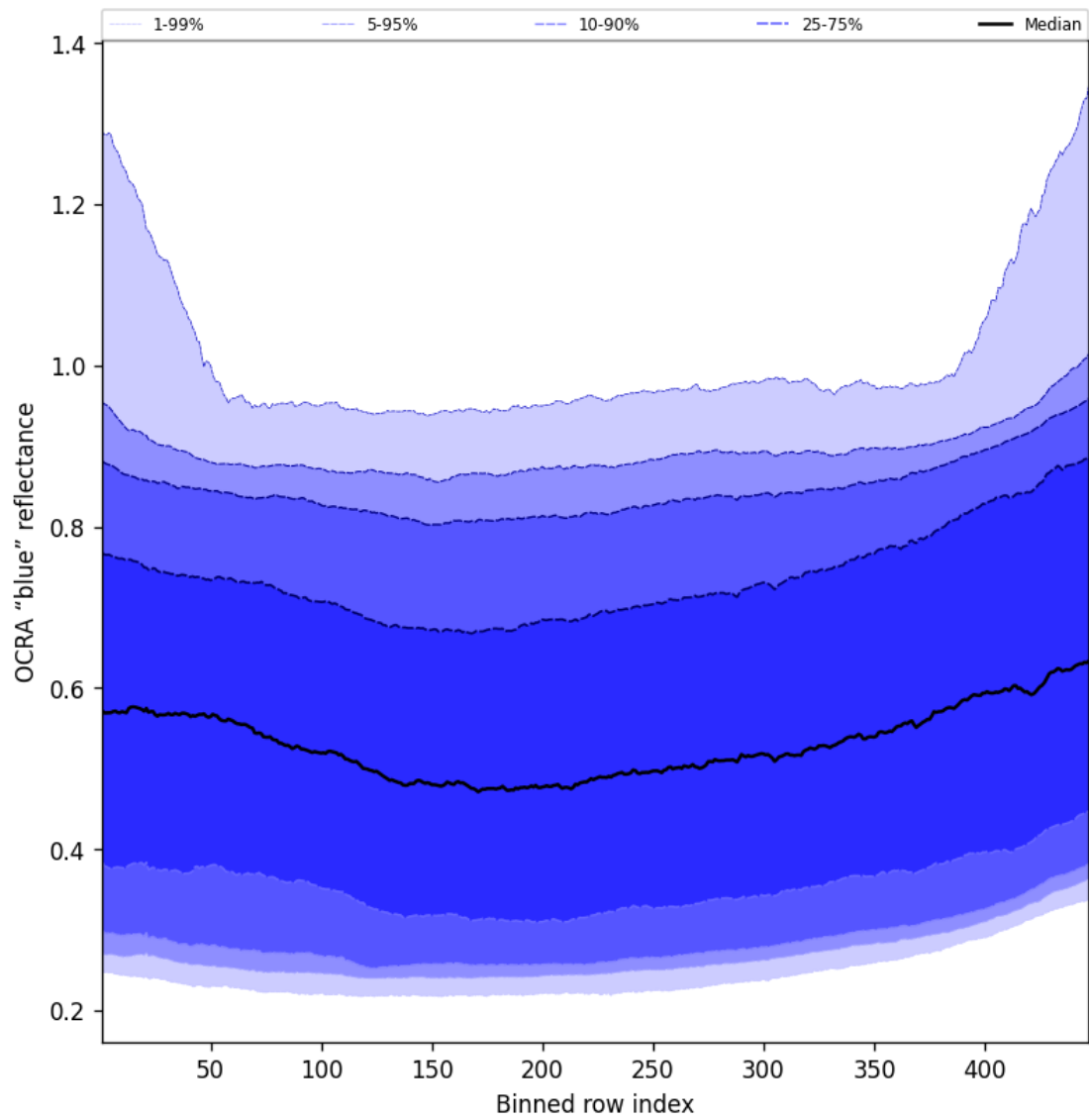
Figure 65: Along track statistics of “OCRA “blue” reflectance” for 2025-05-28 to 2025-05-29
