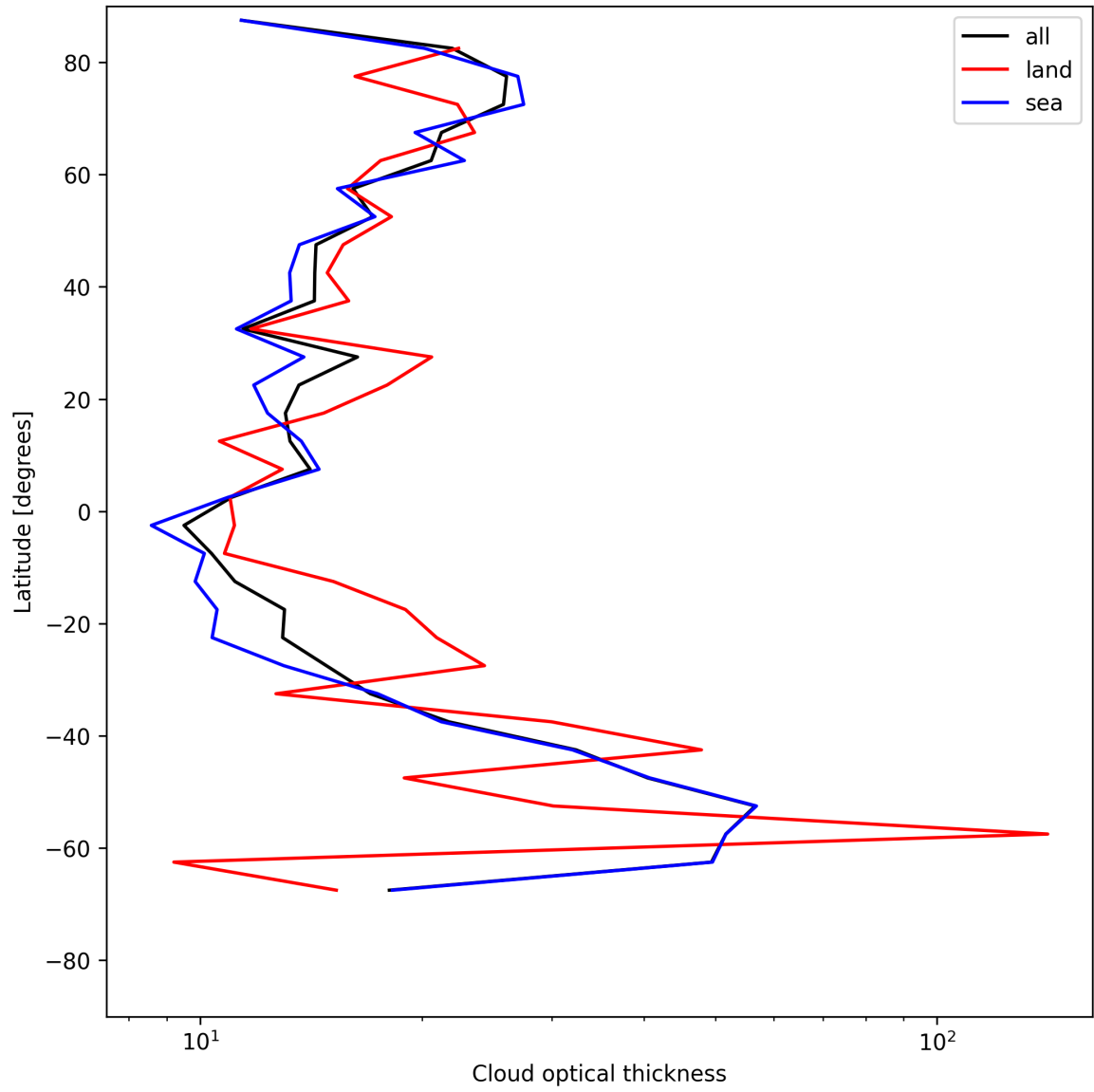
Figure 23: Zonal average of “Cloud optical thickness” for 2025-05-28 to 2025-05-29.
