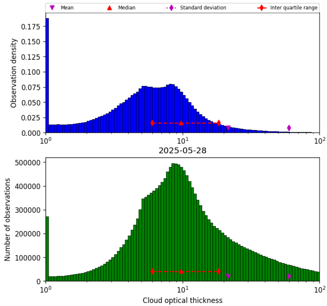
Figure 39: Histogram of “Cloud optical thickness” for 2025-05-28 to 2025-05-29
