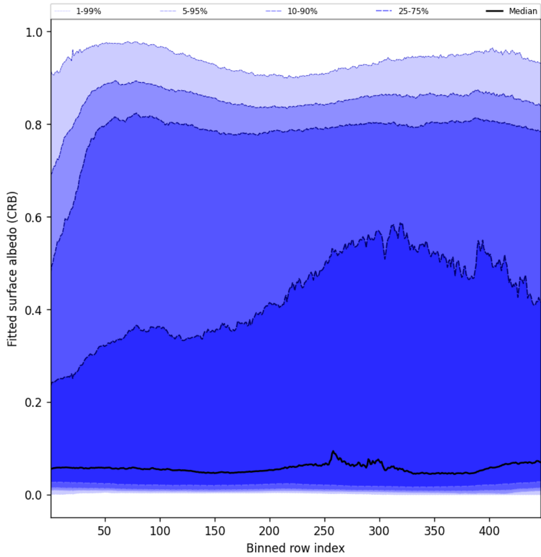
Figure 60: Along track statistics of “Fitted surface albedo (CRB)” for 2025-05-28 to 2025-05-29
