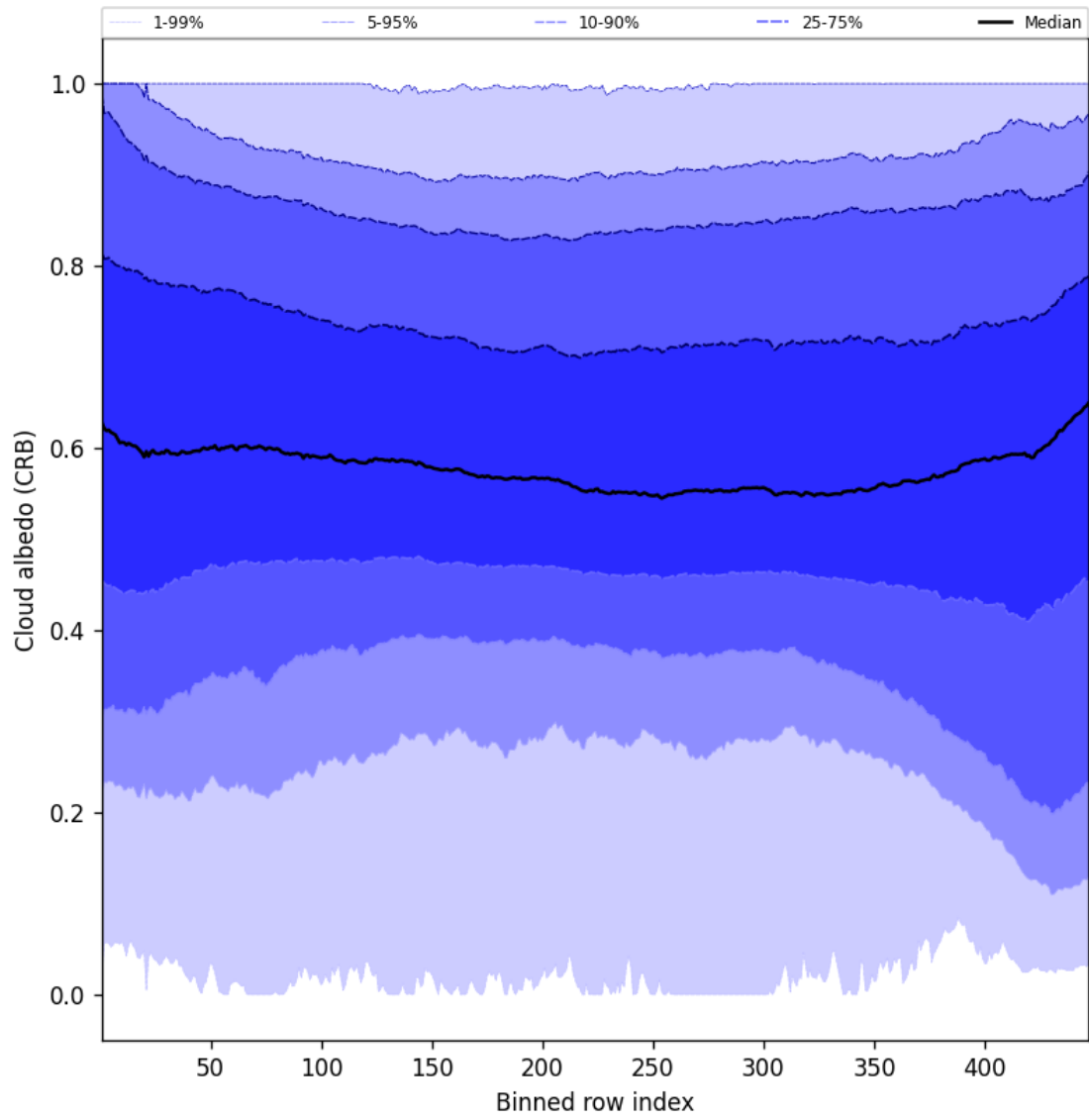
Figure 58: Along track statistics of “Cloud albedo (CRB)” for 2025-05-28 to 2025-05-29
