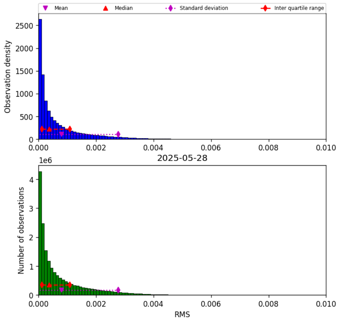
Figure 45: Histogram of “RMS” for 2025-05-28 to 2025-05-29
