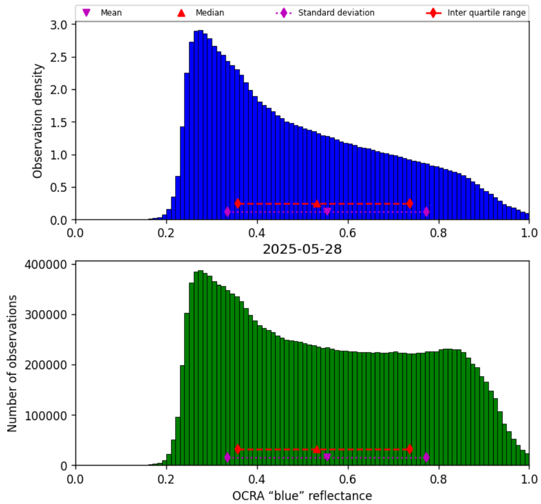
Figure 49: Histogram of “OCRA “blue” reflectance” for 2025-05-28 to 2025-05-29
