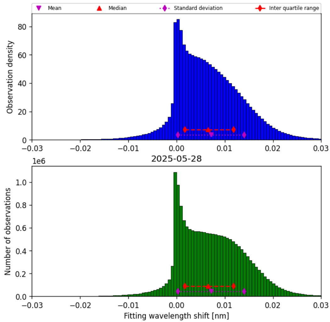
Figure 47: Histogram of “Fitting wavelength shift” for 2025-05-28 to 2025-05-29
