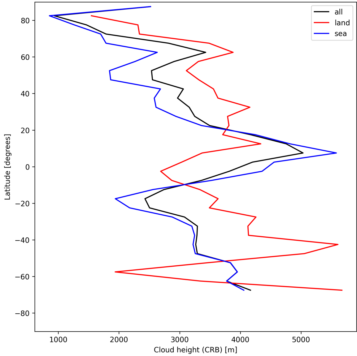
Figure 25: Zonal average of “Cloud height (CRB)” for 2025-05-28 to 2025-05-29.
