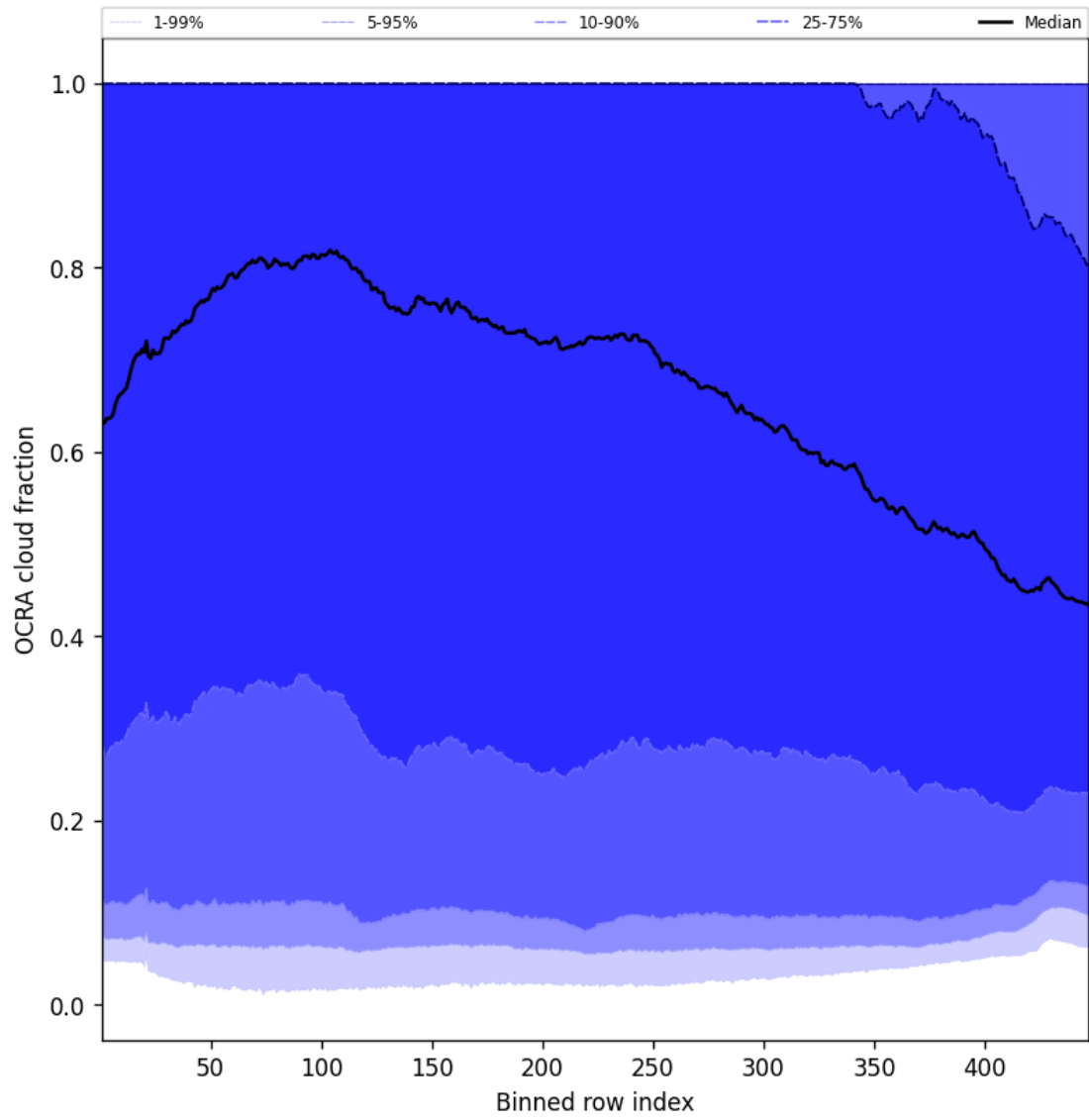
Figure 64: Along track statistics of “OCRA cloud fraction” for 2025-05-28 to 2025-05-29
