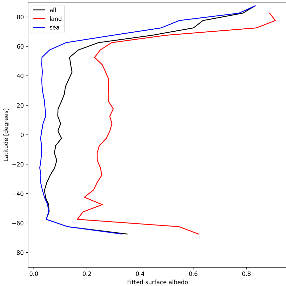
Figure 27: Zonal average of “Fitted surface albedo” for 2025-05-28 to 2025-05-29.
