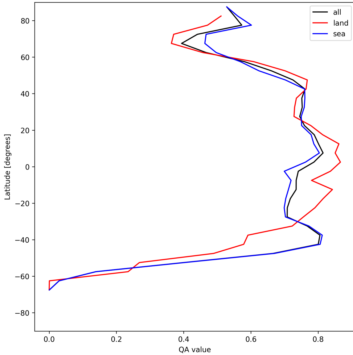
Figure 20: Zonal average of “QA value” for 2025-05-30 to 2025-05-31.
