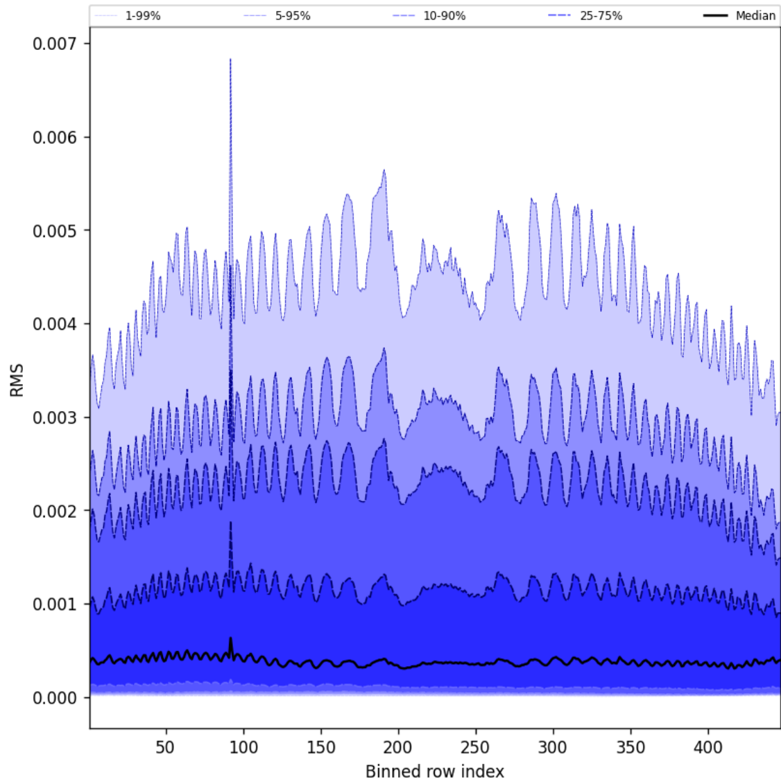
Figure 61: Along track statistics of “RMS” for 2025-05-30 to 2025-05-31
