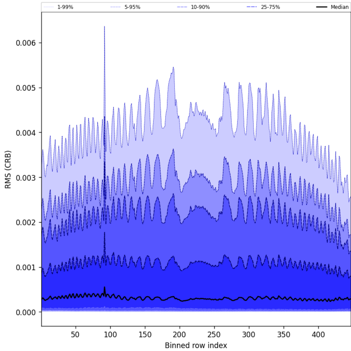
Figure 62: Along track statistics of “RMS (CRB)” for 2025-05-30 to 2025-05-31
