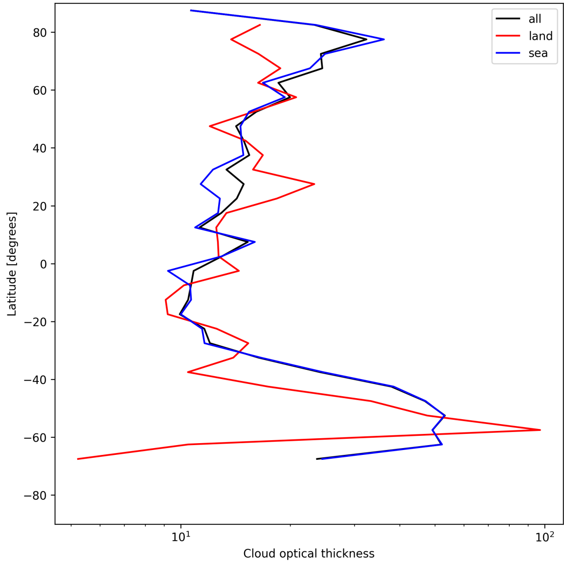
Figure 23: Zonal average of “Cloud optical thickness” for 2025-05-30 to 2025-05-31.
