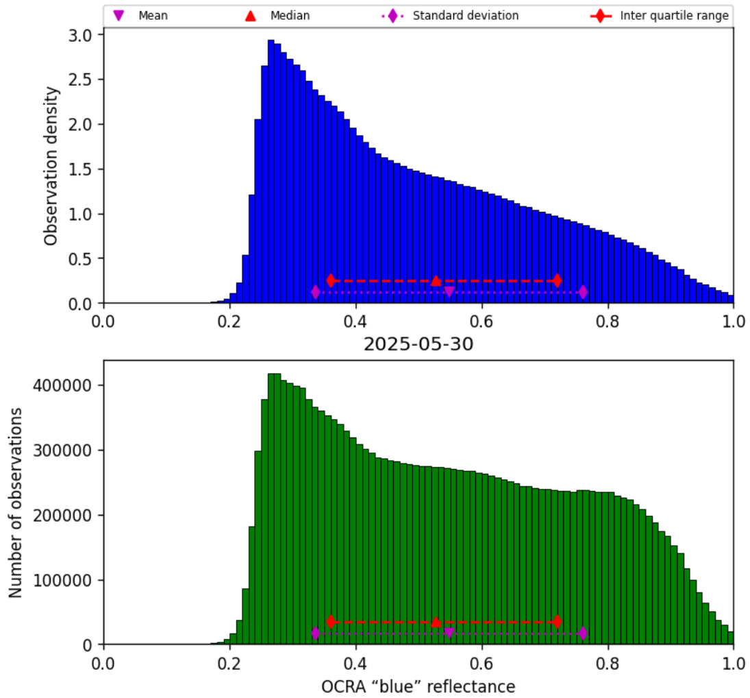
Figure 49: Histogram of “OCRA “blue” reflectance” for 2025-05-30 to 2025-05-31
