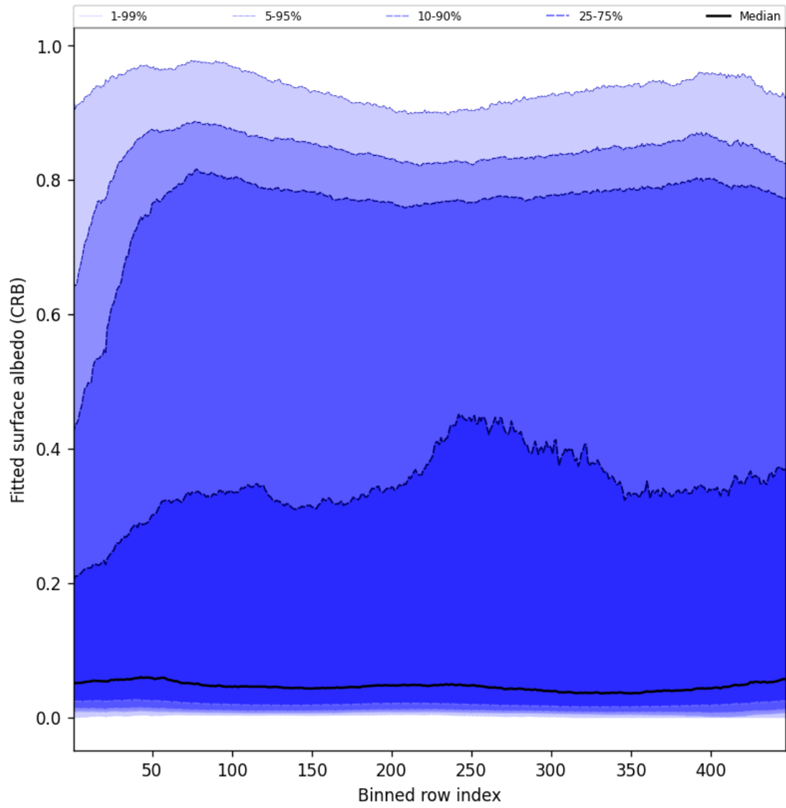
Figure 60: Along track statistics of “Fitted surface albedo (CRB)” for 2025-05-30 to 2025-05-31
