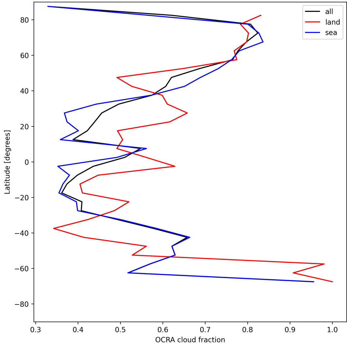
Figure 32: Zonal average of “OCRA cloud fraction” for 2025-05-30 to 2025-05-31.
