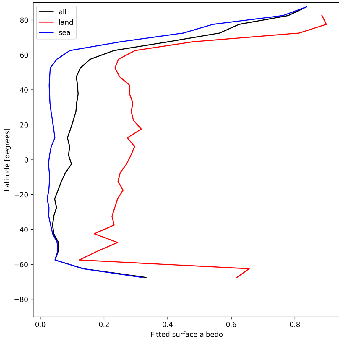
Figure 27: Zonal average of “Fitted surface albedo” for 2025-05-30 to 2025-05-31.
