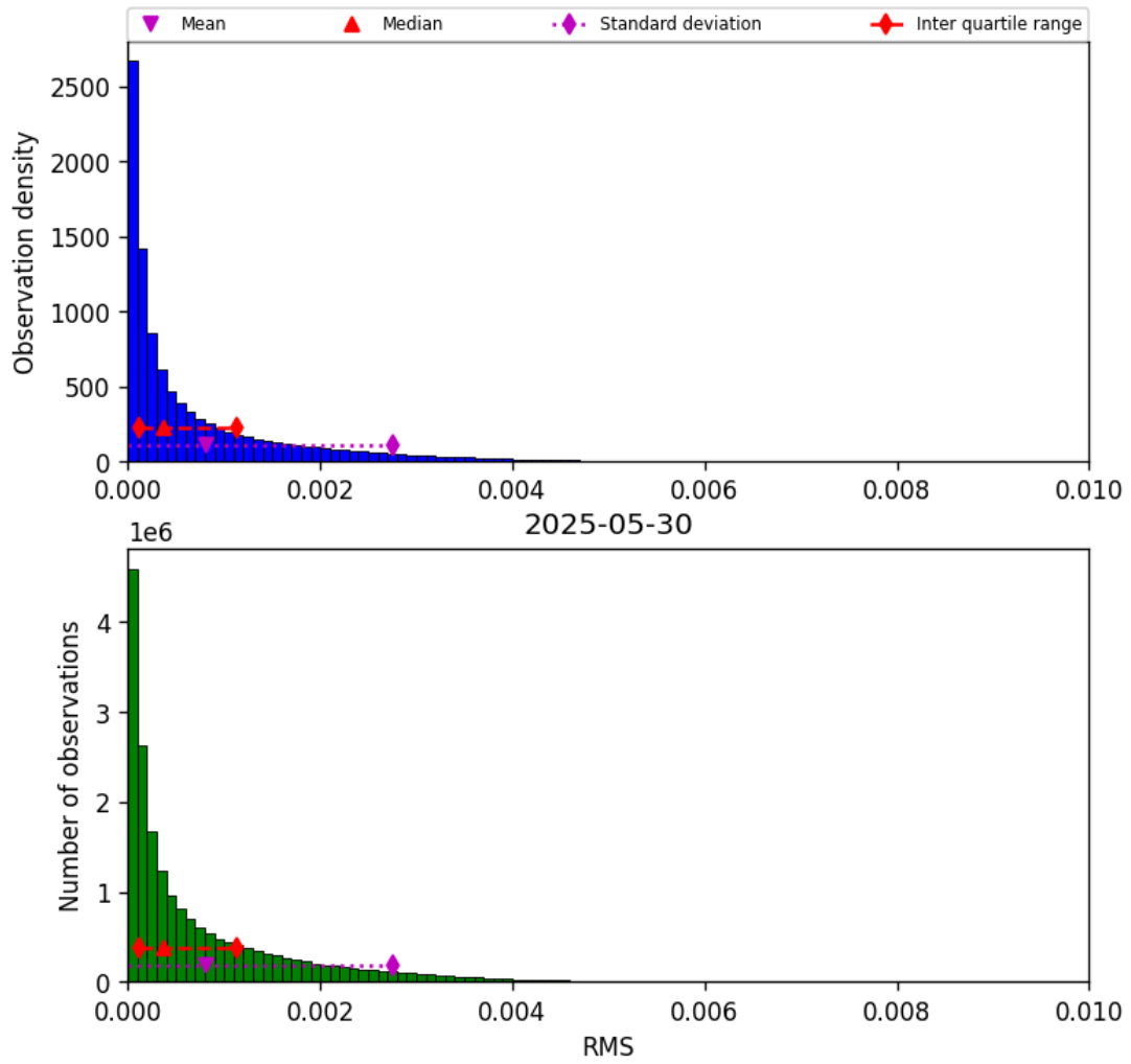
Figure 45: Histogram of “RMS” for 2025-05-30 to 2025-05-31
