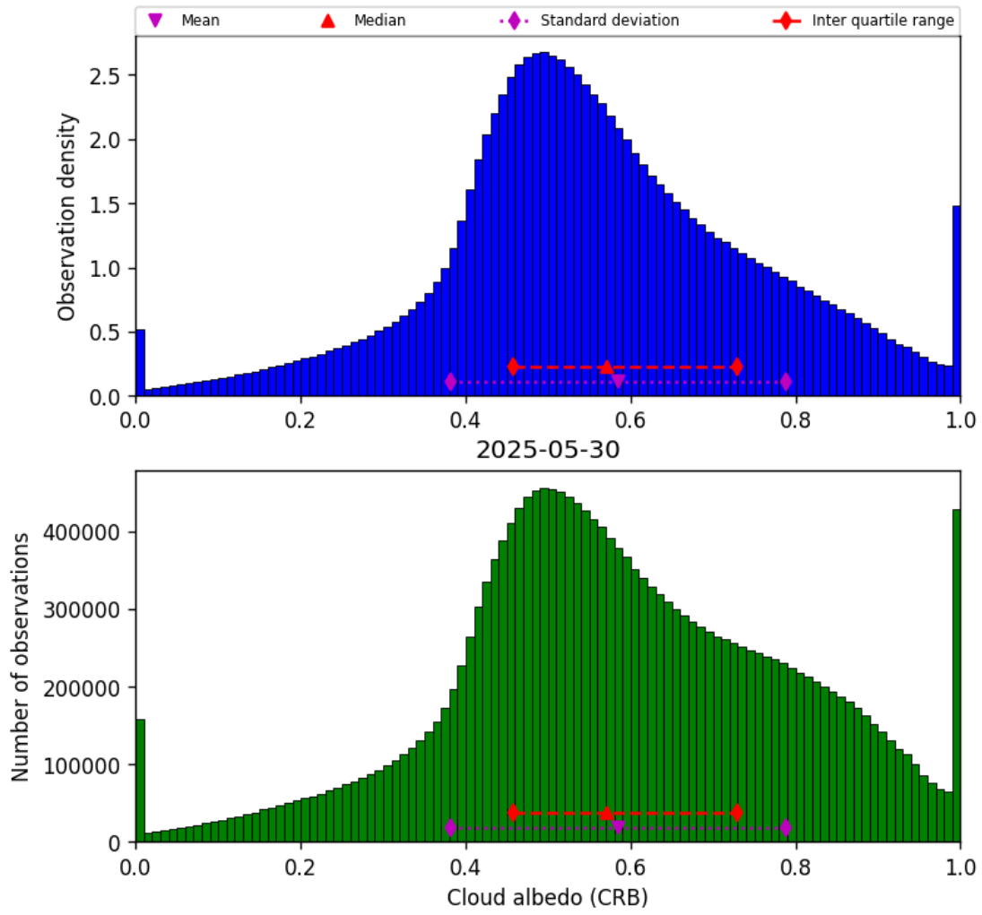
Figure 42: Histogram of “Cloud albedo (CRB)” for 2025-05-30 to 2025-05-31
