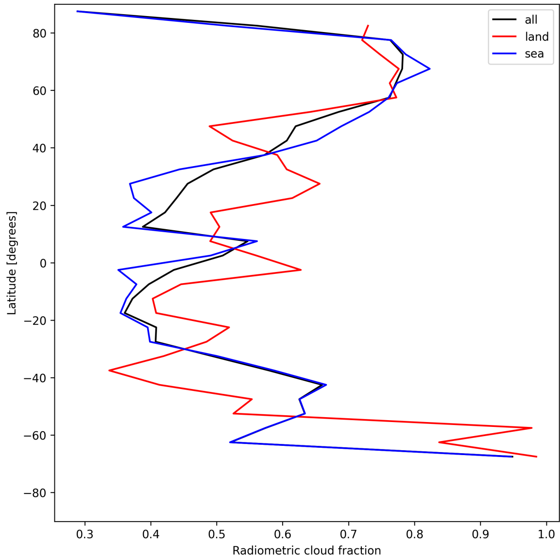
Figure 21: Zonal average of “Radiometric cloud fraction” for 2025-05-30 to 2025-05-31.
