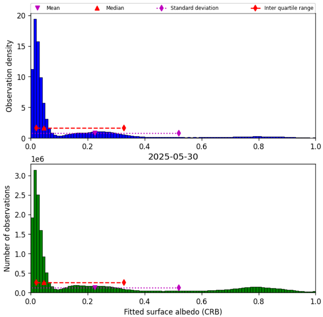
Figure 44: Histogram of “Fitted surface albedo (CRB)” for 2025-05-30 to 2025-05-31
