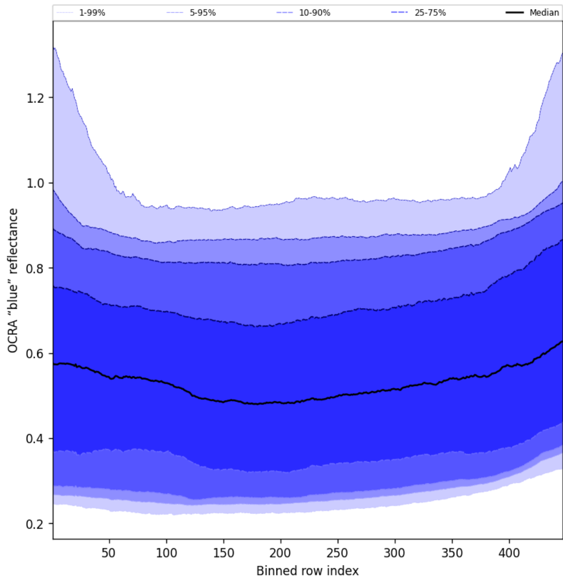
Figure 65: Along track statistics of “OCRA “blue” reflectance” for 2025-05-30 to 2025-05-31
