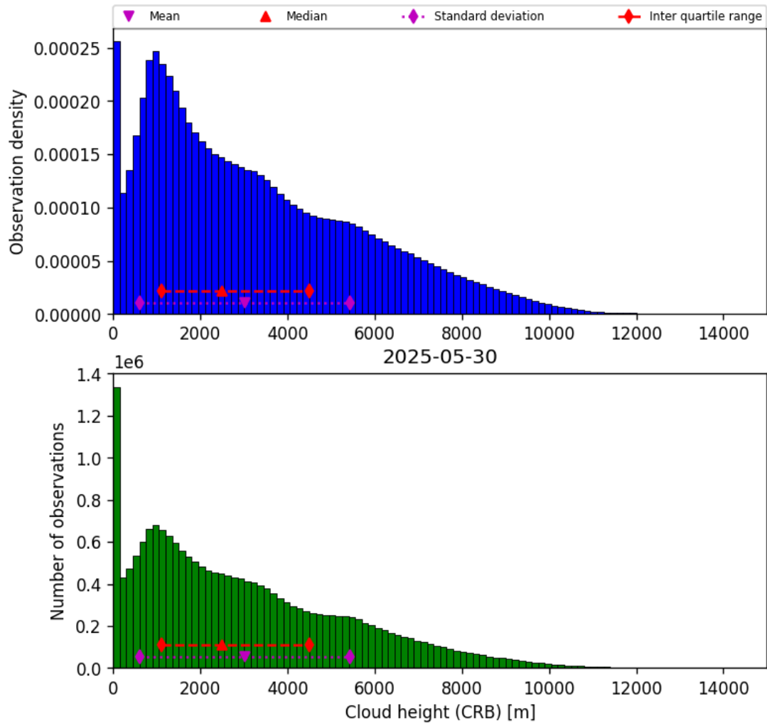
Figure 41: Histogram of “Cloud height (CRB)” for 2025-05-30 to 2025-05-31
