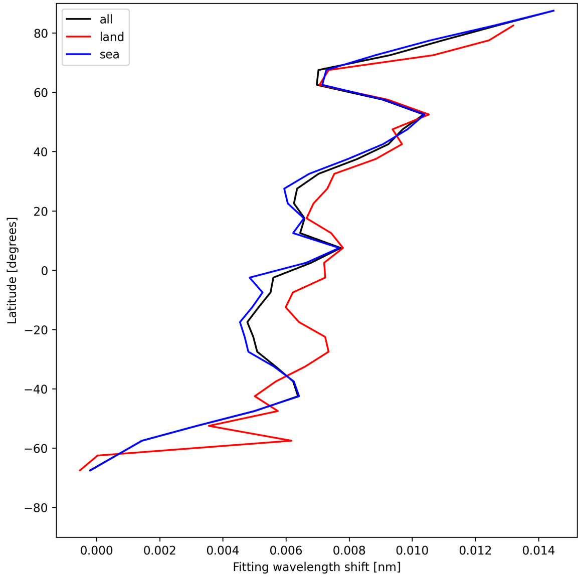
Figure 31: Zonal average of “Fitting wavelength shift” for 2025-05-30 to 2025-05-31.
