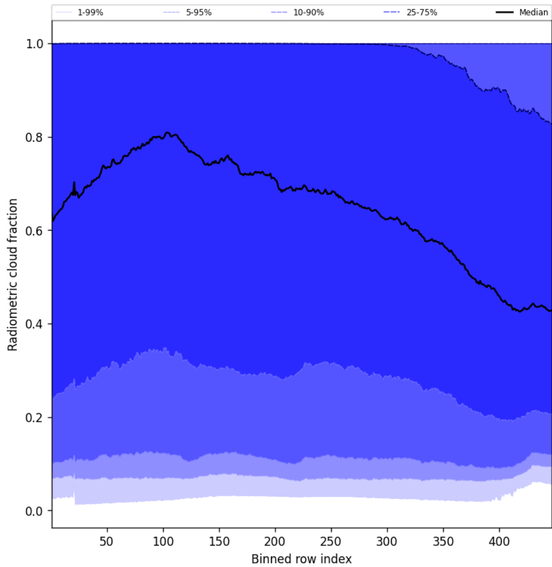
Figure 53: Along track statistics of “Radiometric cloud fraction” for 2025-05-30 to 2025-05-31
