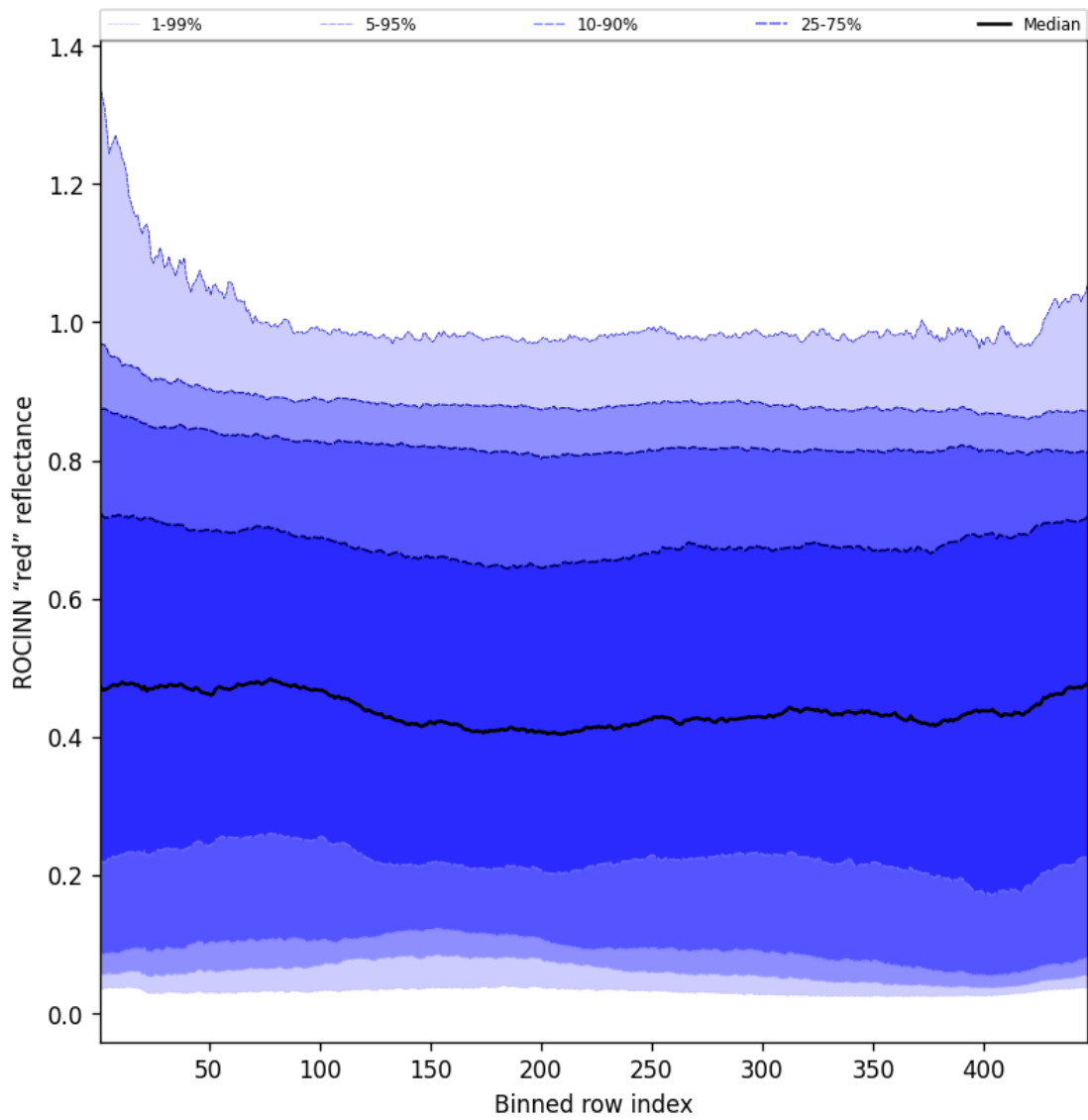
Figure 67: Along track statistics of "ROCINN "red" reflectance" for 2025-05-30 to 2025-05-31
