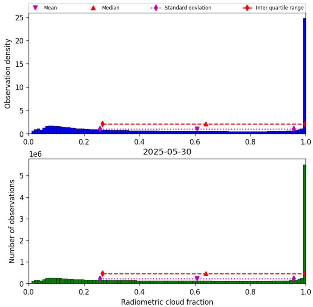
Figure 37: Histogram of “Radiometric cloud fraction” for 2025-05-30 to 2025-05-31
