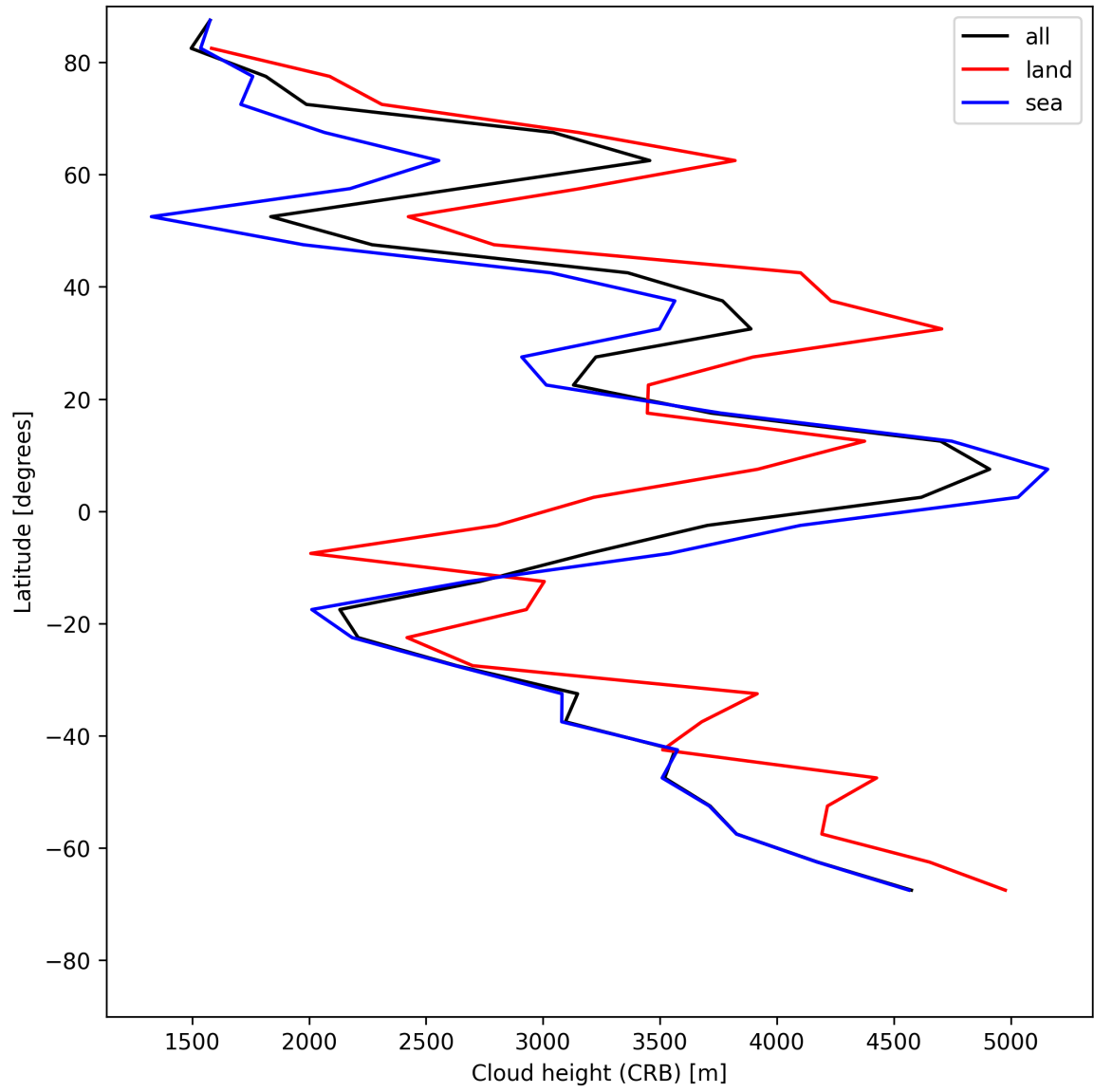
Figure 25: Zonal average of “Cloud height (CRB)” for 2025-05-30 to 2025-05-31.
