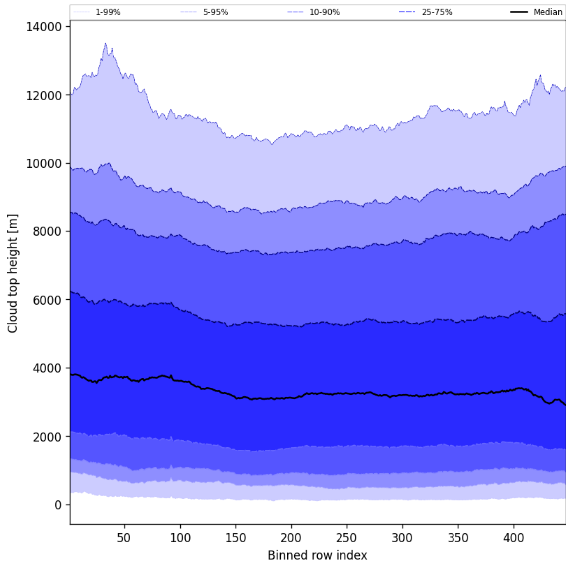
Figure 54: Along track statistics of “Cloud top height” for 2025-05-30 to 2025-05-31
