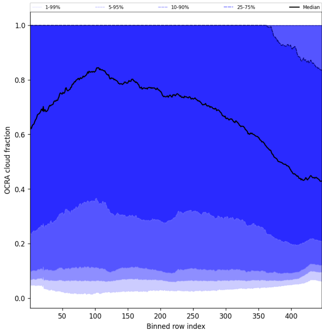
Figure 64: Along track statistics of “OCRA cloud fraction” for 2025-05-30 to 2025-05-31
