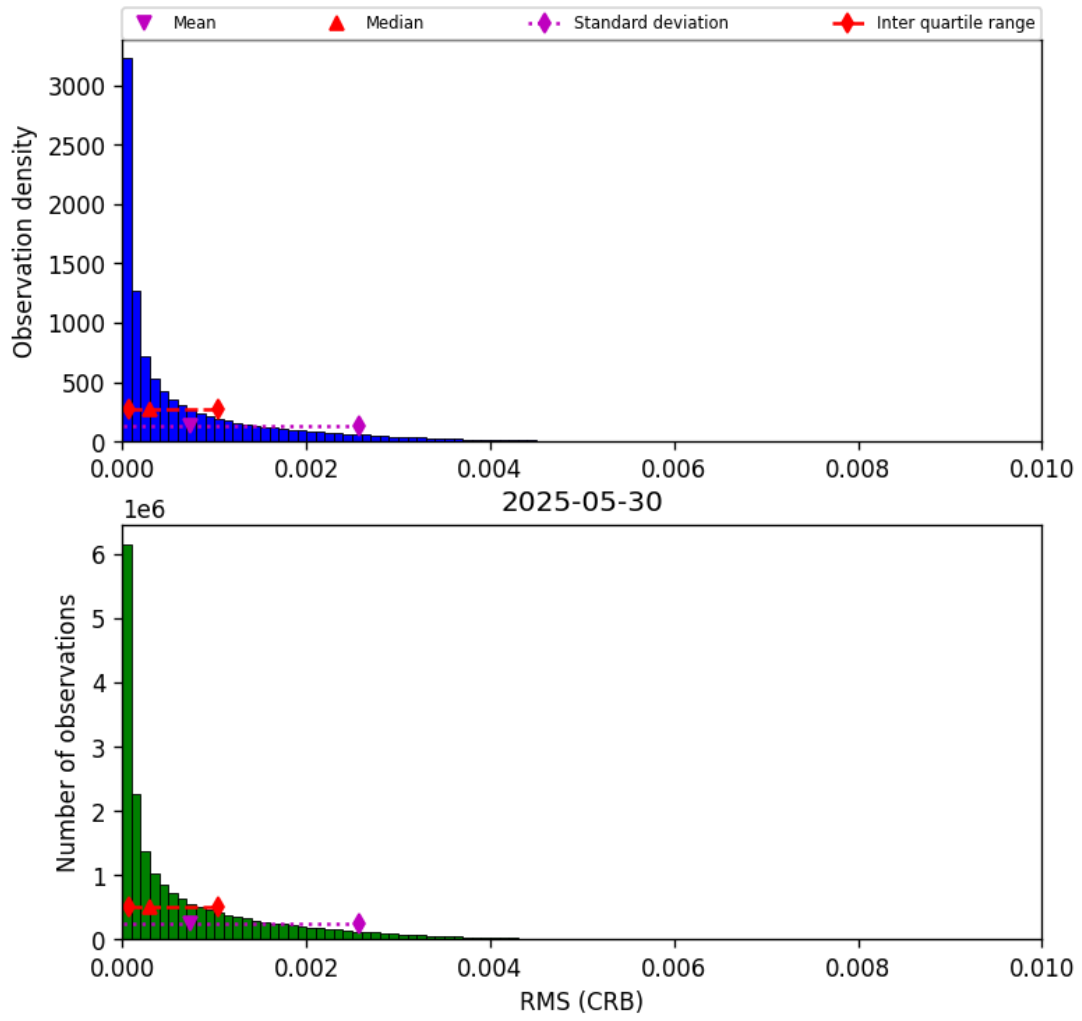
Figure 46: Histogram of “RMS (CRB)” for 2025-05-30 to 2025-05-31
