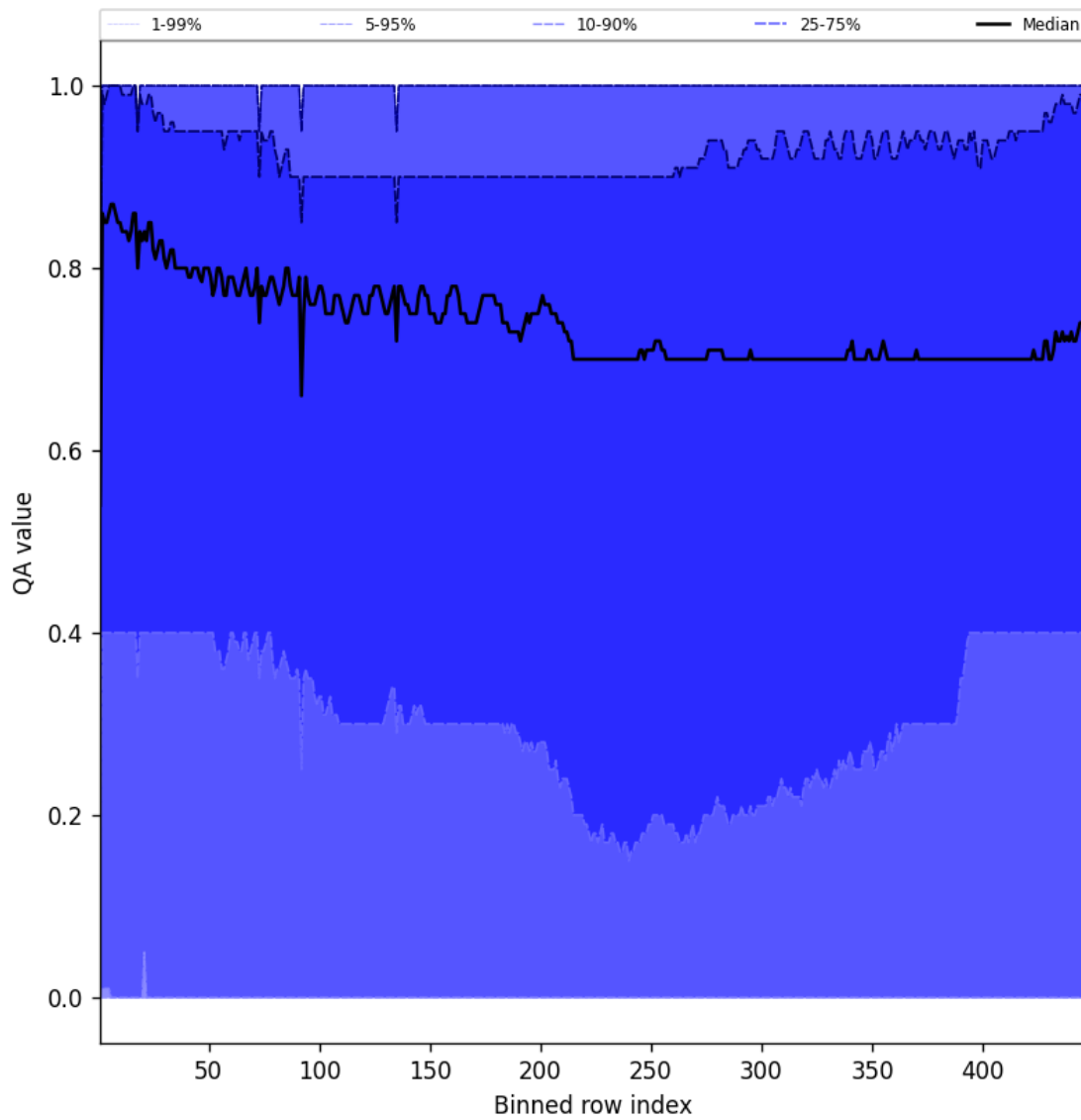
Figure 52: Along track statistics of “QA value” for 2025-05-30 to 2025-05-31
