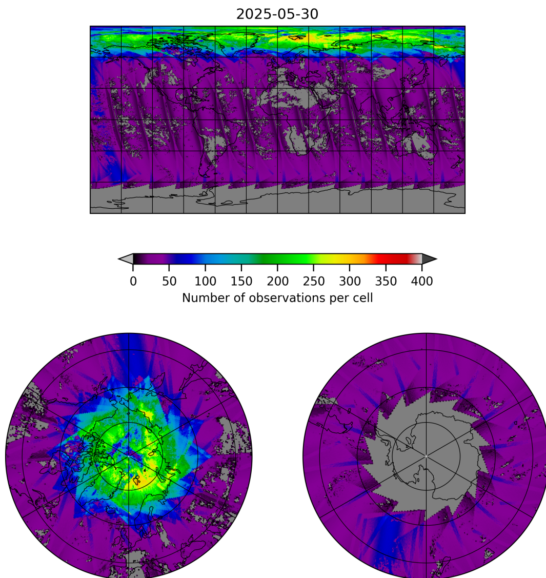
Figure 19: Map of the number of observations for 2025-05-30 to 2025-05-31
