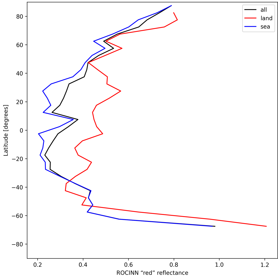
Figure 35: Zonal average of “ROCINN “red” reflectance” for 2025-05-30 to 2025-05-31.
