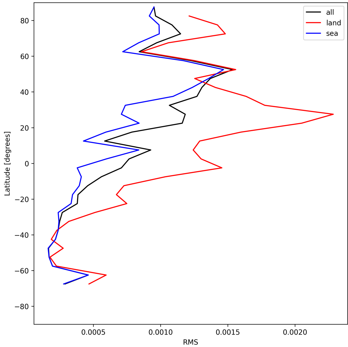
Figure 29: Zonal average of “RMS” for 2025-05-30 to 2025-05-31.
