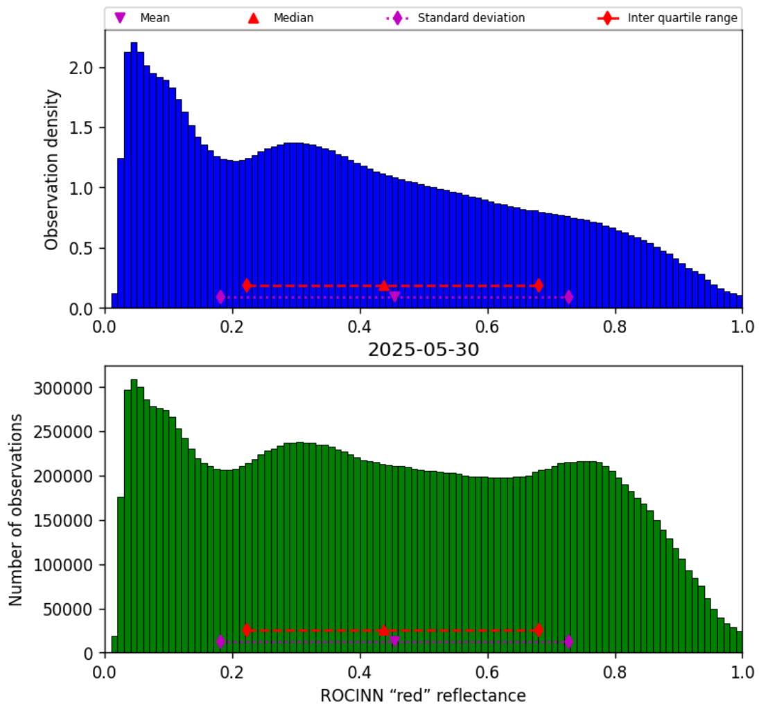
Figure 51: Histogram of “ROCINN “red” reflectance” for 2025-05-30 to 2025-05-31
