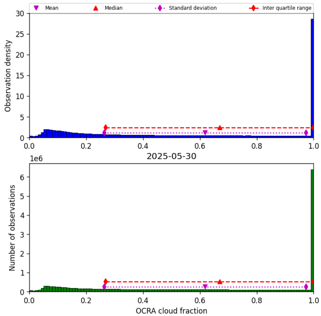
Figure 48: Histogram of “OCRA cloud fraction” for 2025-05-30 to 2025-05-31
