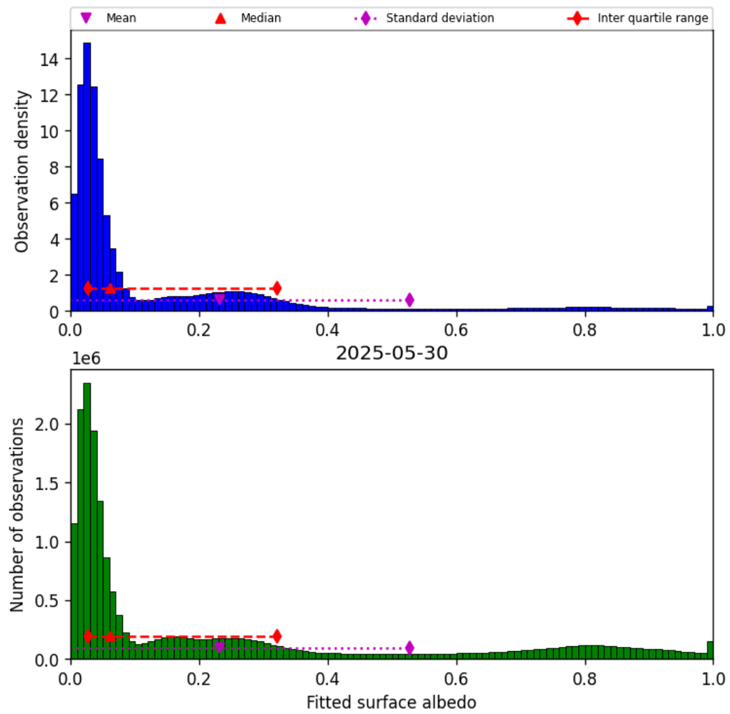
Figure 43: Histogram of “Fitted surface albedo” for 2025-05-30 to 2025-05-31
