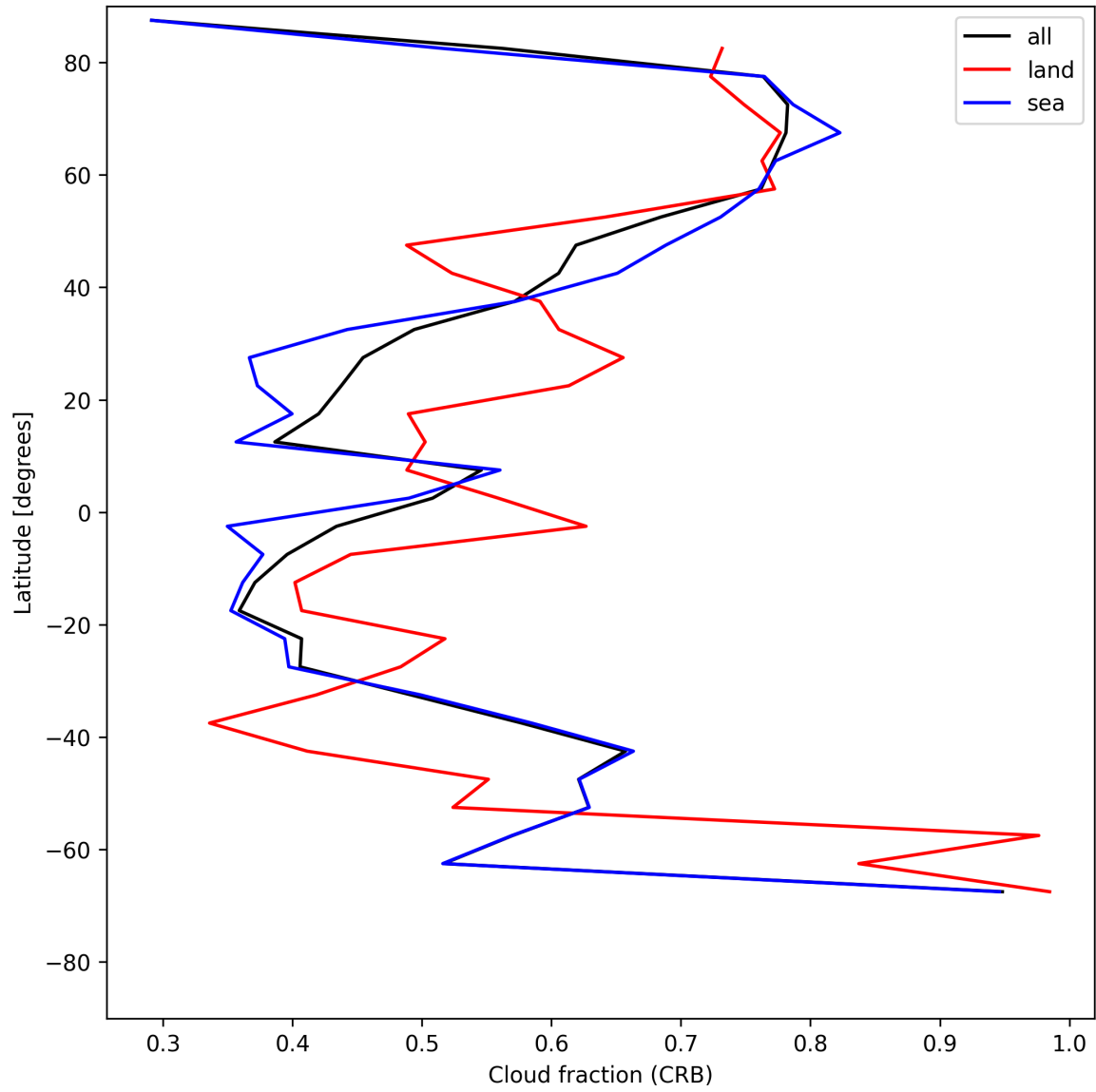
Figure 24: Zonal average of “Cloud fraction (CRB)” for 2025-05-30 to 2025-05-31.
