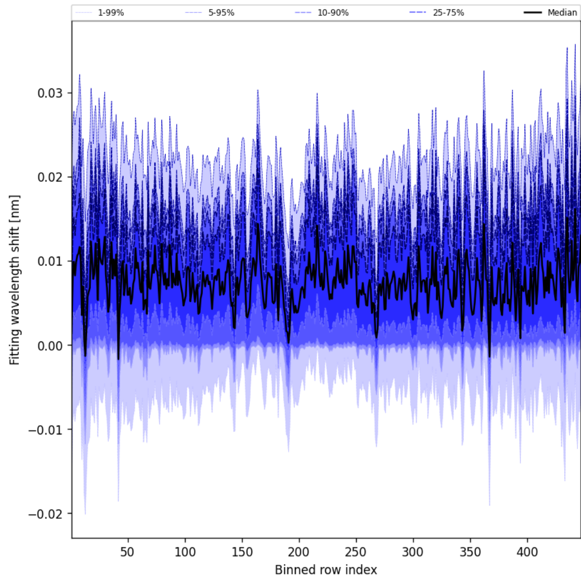
Figure 63: Along track statistics of “Fitting wavelength shift” for 2025-05-30 to 2025-05-31
