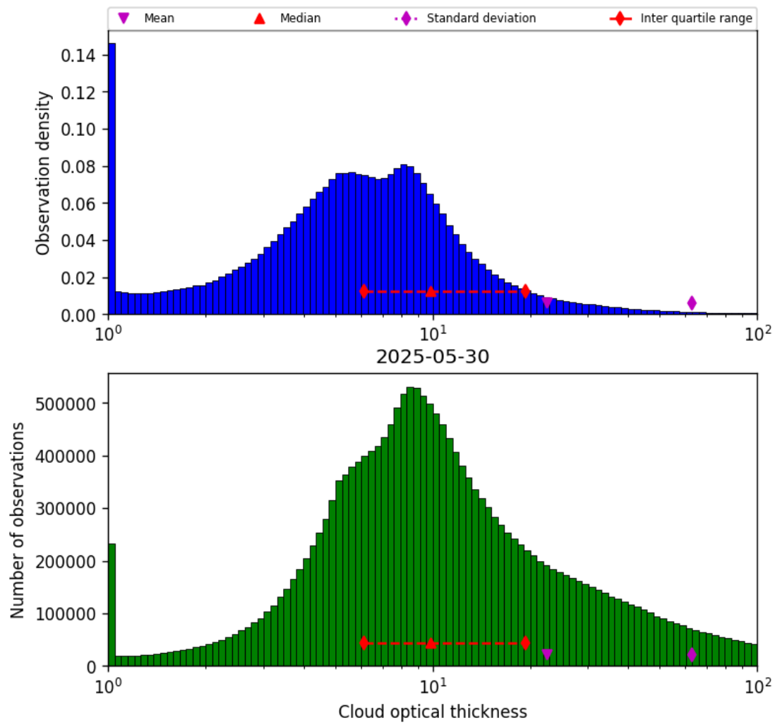
Figure 39: Histogram of “Cloud optical thickness” for 2025-05-30 to 2025-05-31
