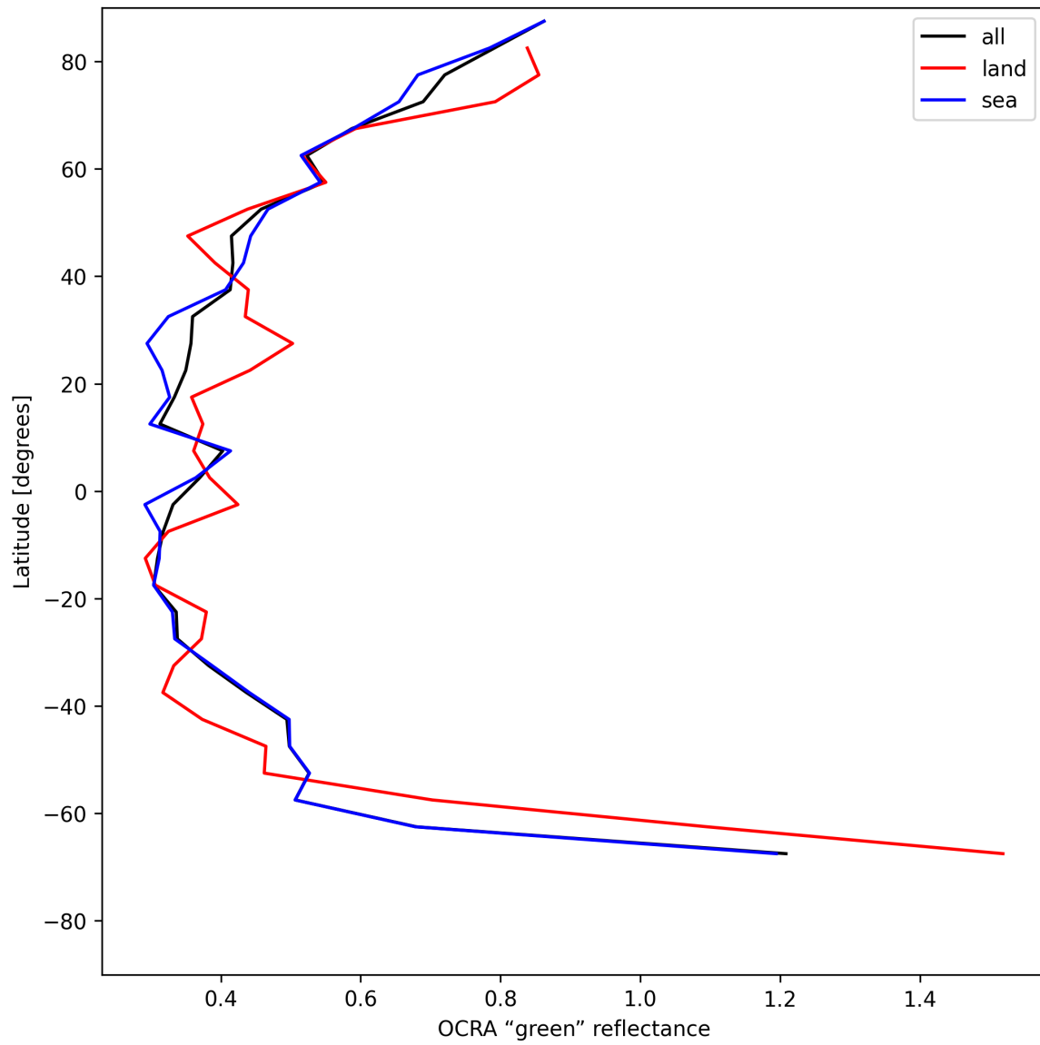
Figure 34: Zonal average of “OCRA “green” reflectance” for 2025-05-30 to 2025-05-31.
