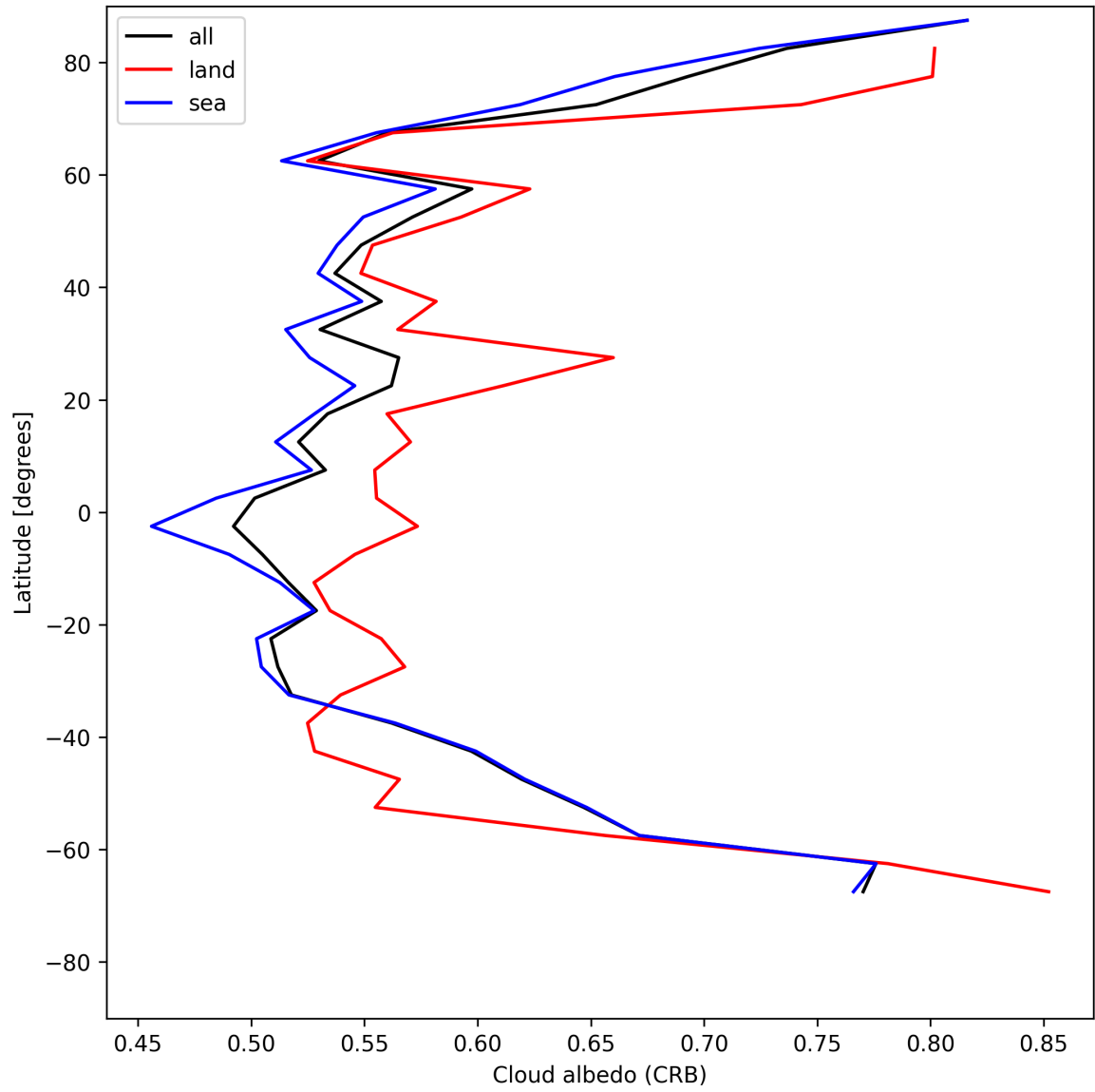
Figure 26: Zonal average of “Cloud albedo (CRB)” for 2025-05-30 to 2025-05-31.
