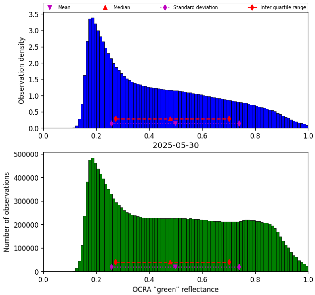
Figure 50: Histogram of “OCRA “green” reflectance” for 2025-05-30 to 2025-05-31
