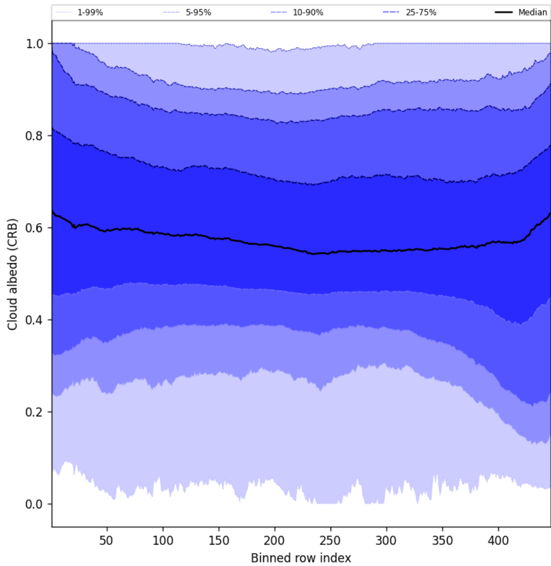
Figure 58: Along track statistics of “Cloud albedo (CRB)” for 2025-05-30 to 2025-05-31
