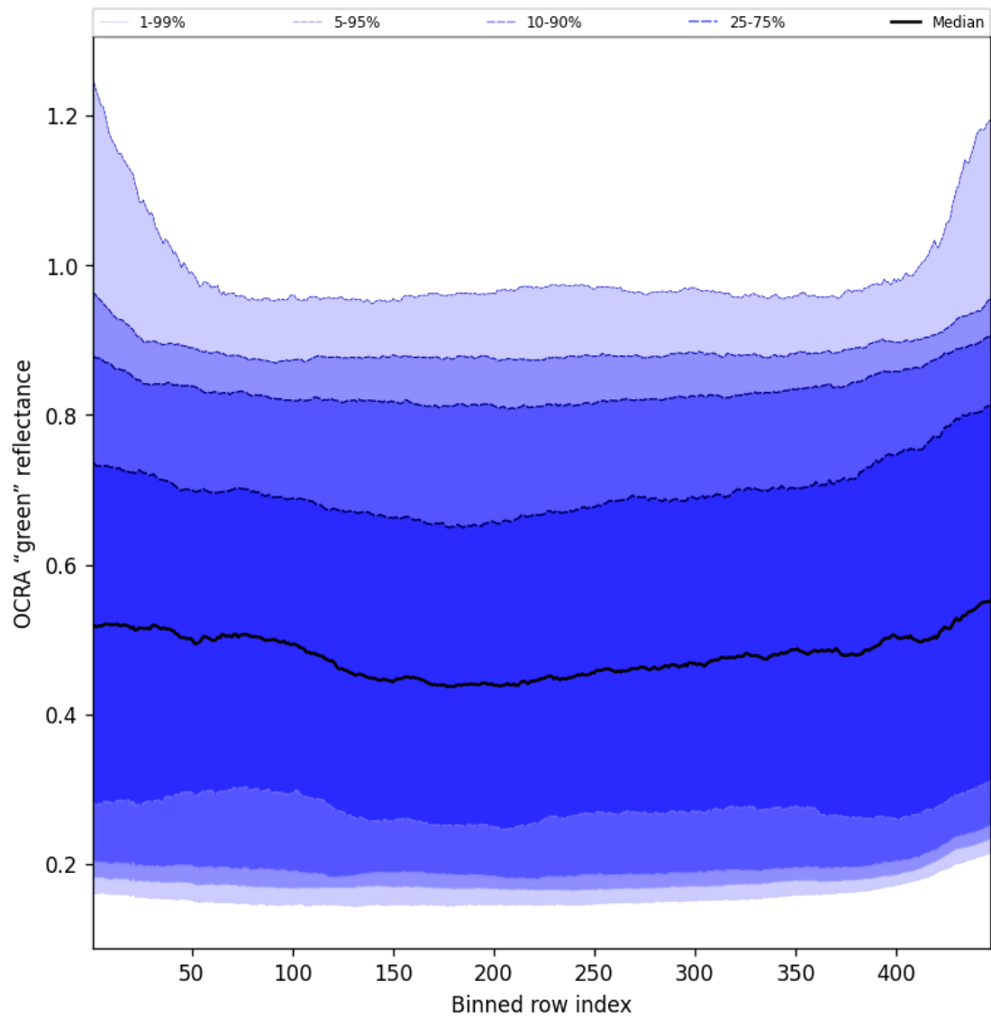
Figure 66: Along track statistics of “OCRA “green” reflectance” for 2025-05-30 to 2025-05-31
