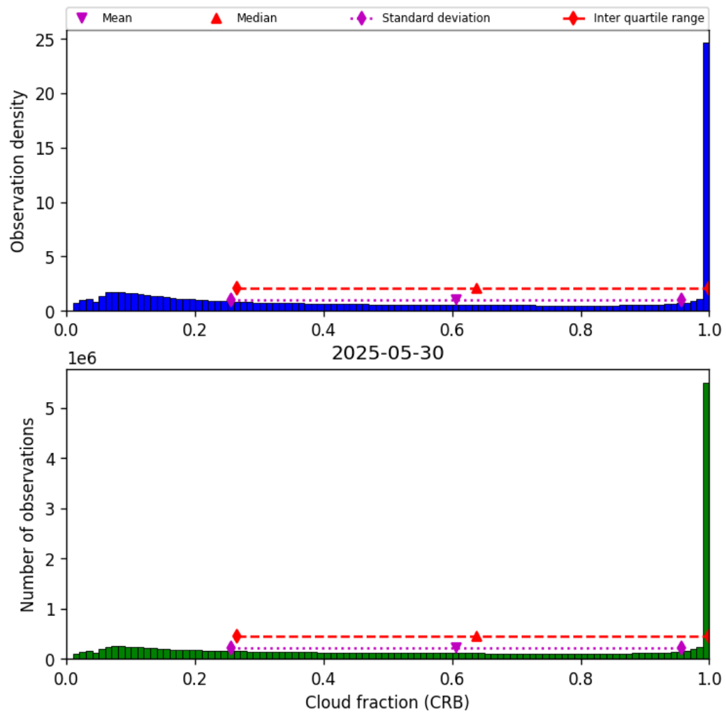
Figure 40: Histogram of “Cloud fraction (CRB)” for 2025-05-30 to 2025-05-31
