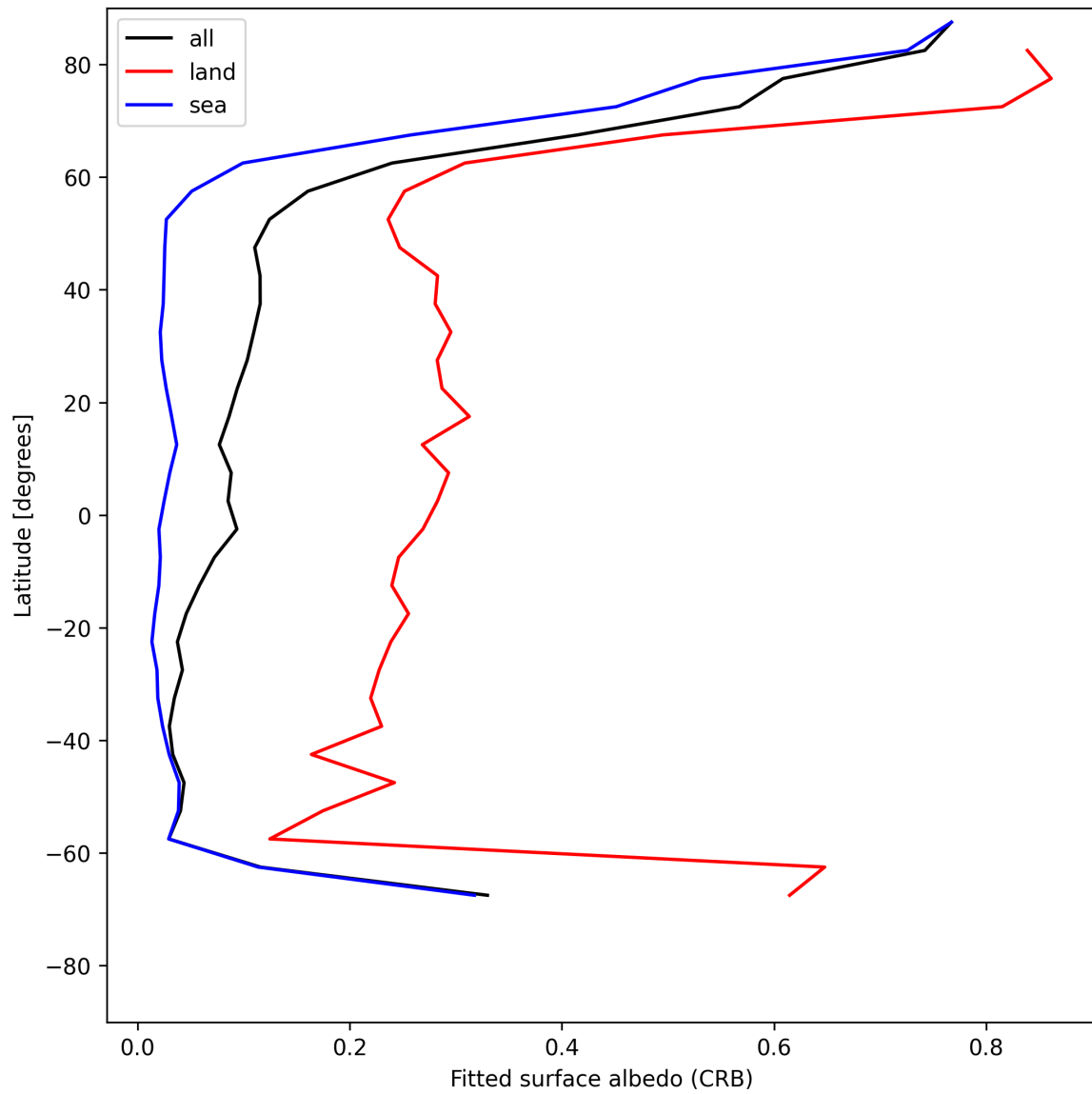
Figure 28: Zonal average of “Fitted surface albedo (CRB)” for 2025-05-30 to 2025-05-31.
