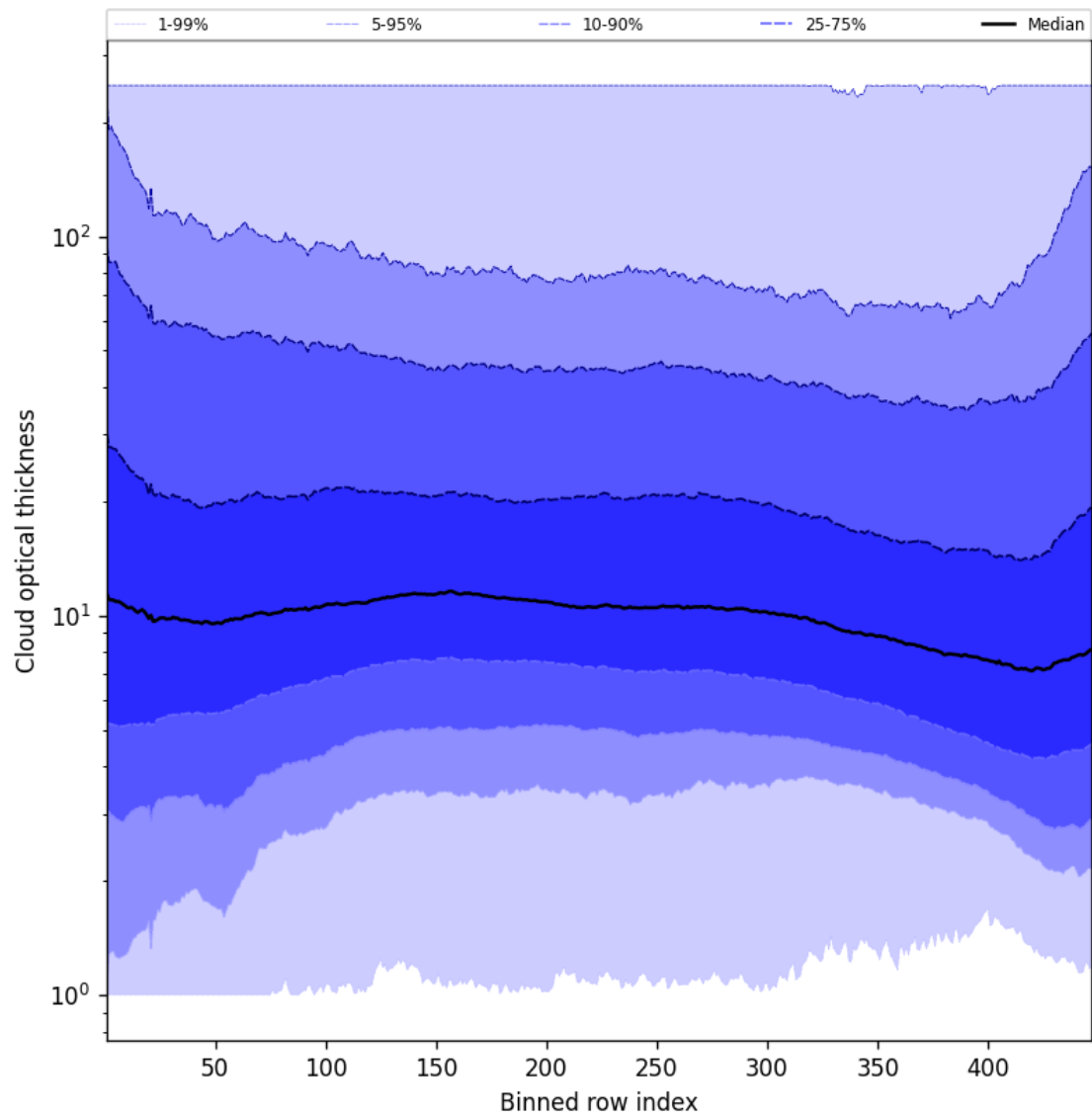
Figure 55: Along track statistics of “Cloud optical thickness” for 2025-05-30 to 2025-05-31
