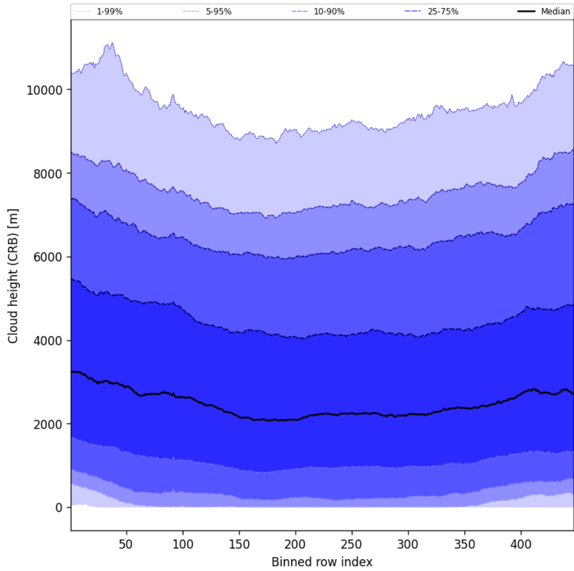
Figure 57: Along track statistics of “Cloud height (CRB)” for 2025-05-30 to 2025-05-31
