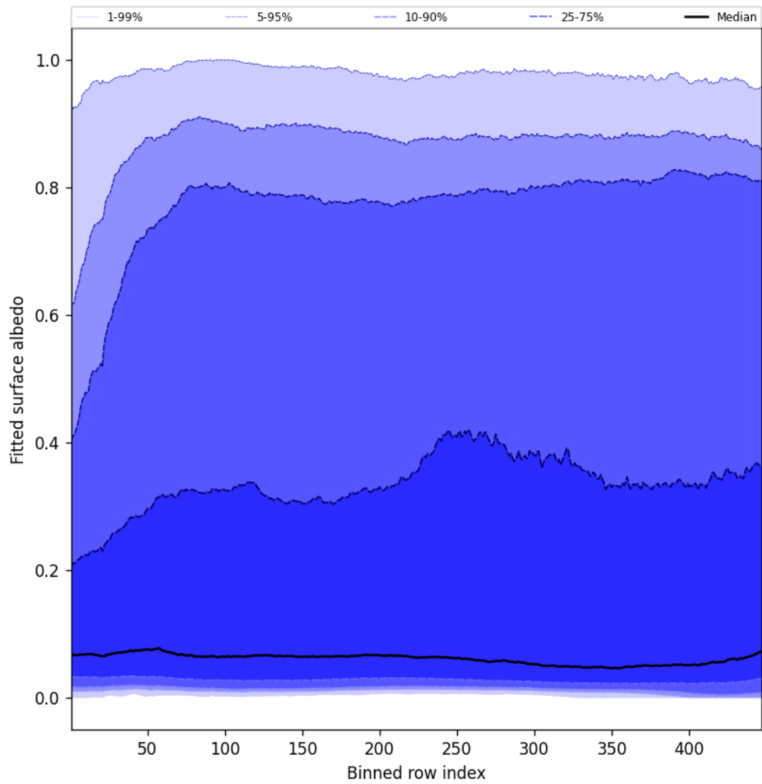
Figure 59: Along track statistics of “Fitted surface albedo” for 2025-05-30 to 2025-05-31
