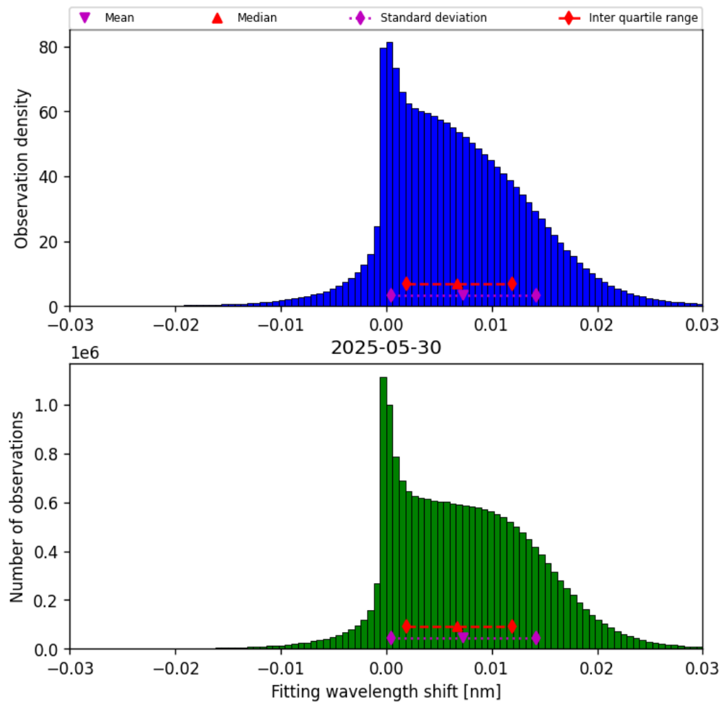
Figure 47: Histogram of “Fitting wavelength shift” for 2025-05-30 to 2025-05-31
