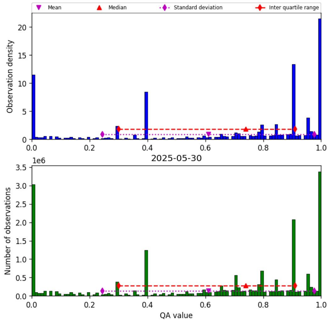
Figure 36: Histogram of “QA value” for 2025-05-30 to 2025-05-31
