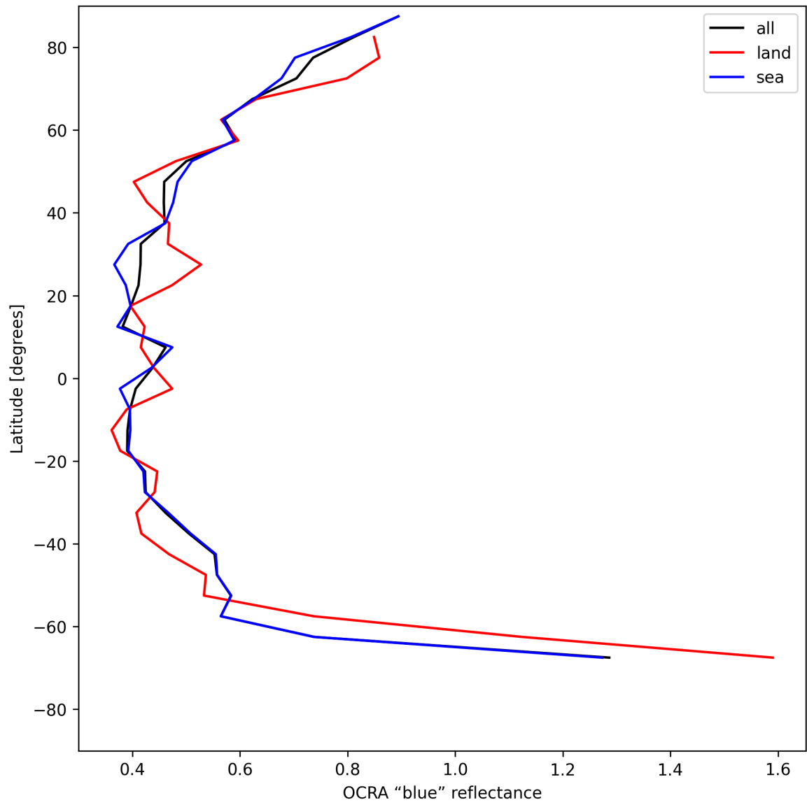
Figure 33: Zonal average of “OCRA “blue” reflectance” for 2025-05-30 to 2025-05-31.
