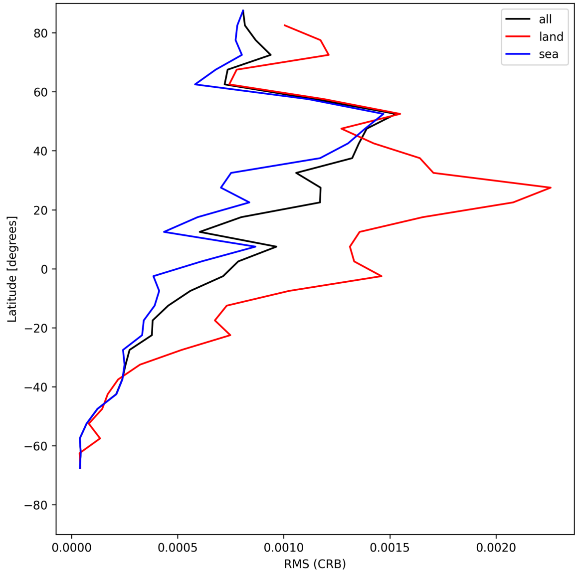
Figure 30: Zonal average of “RMS (CRB)” for 2025-05-30 to 2025-05-31.
