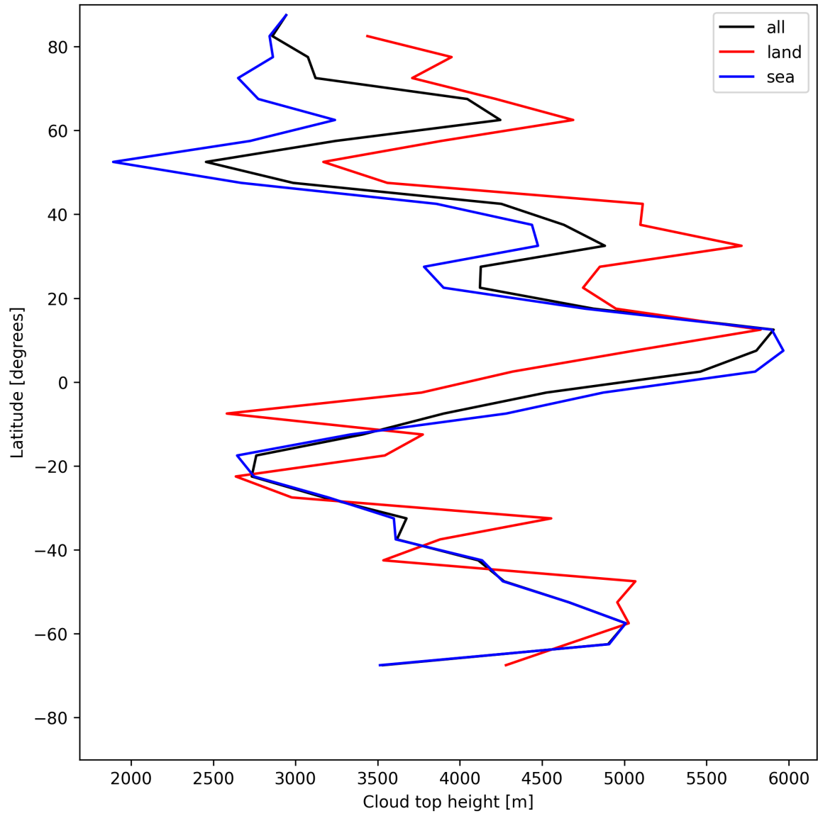
Figure 22: Zonal average of “Cloud top height” for 2025-05-30 to 2025-05-31.
