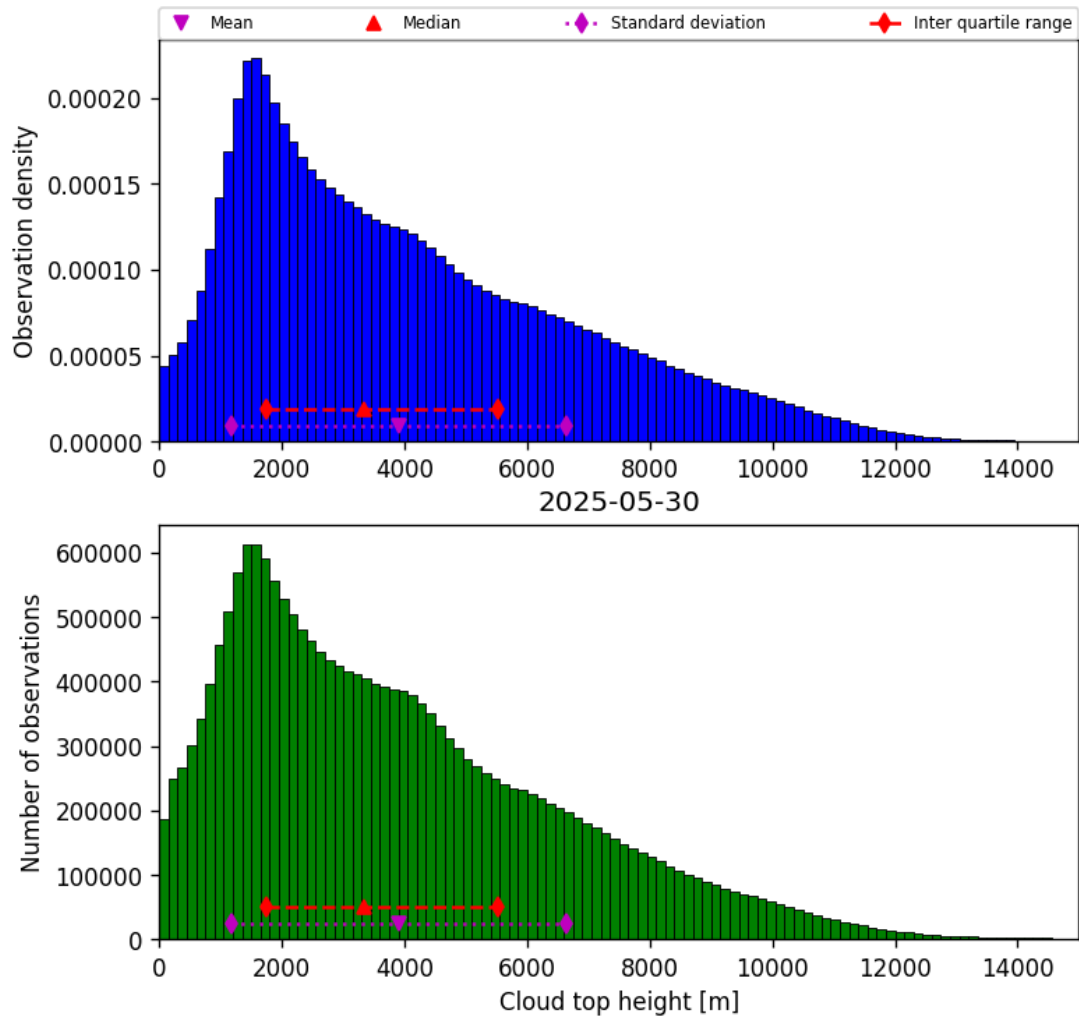
Figure 38: Histogram of “Cloud top height” for 2025-05-30 to 2025-05-31
