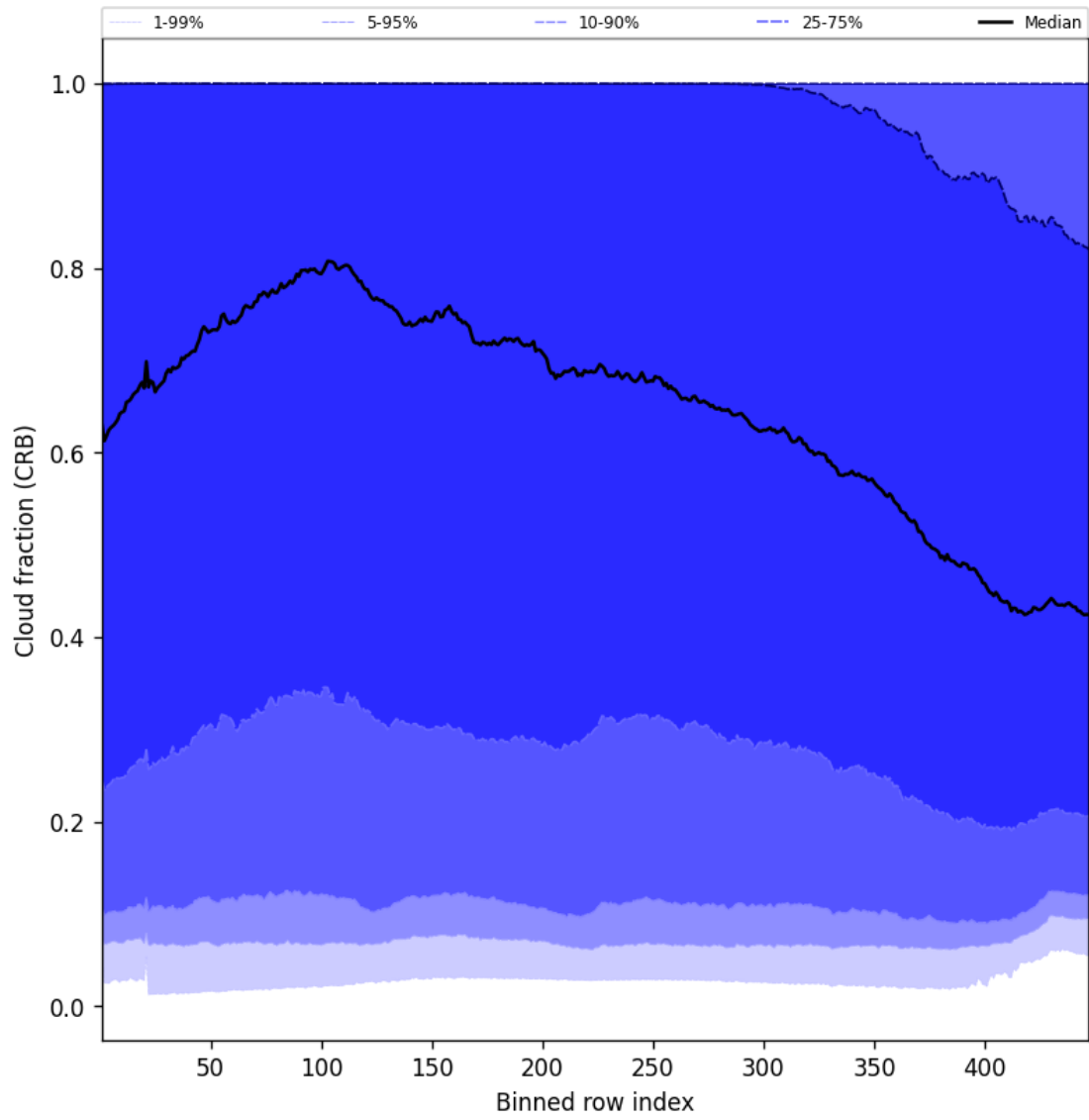
Figure 56: Along track statistics of “Cloud fraction (CRB)” for 2025-05-30 to 2025-05-31
