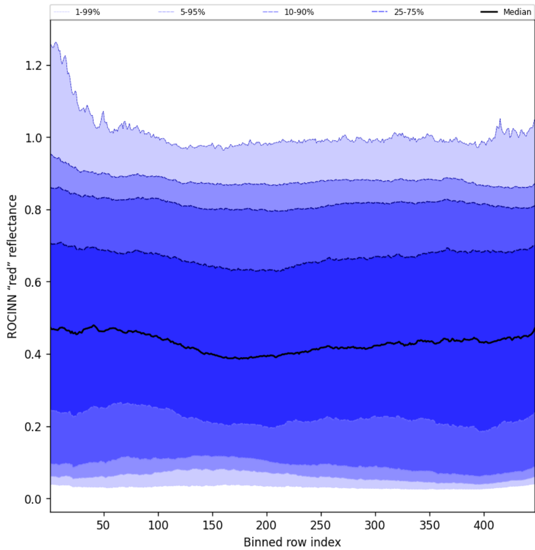
Figure 67: Along track statistics of "ROCINN "red" reflectance" for 2025-05-31 to 2025-06-01
