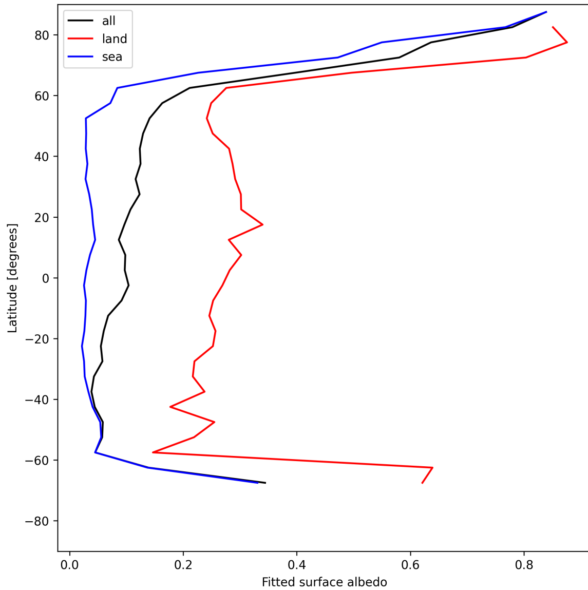
Figure 27: Zonal average of “Fitted surface albedo” for 2025-05-31 to 2025-06-01.
