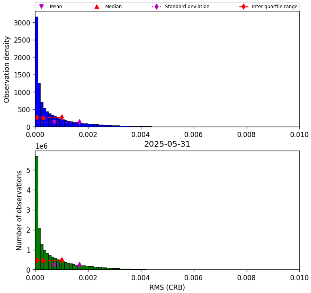
Figure 46: Histogram of “RMS (CRB)” for 2025-05-31 to 2025-06-01
