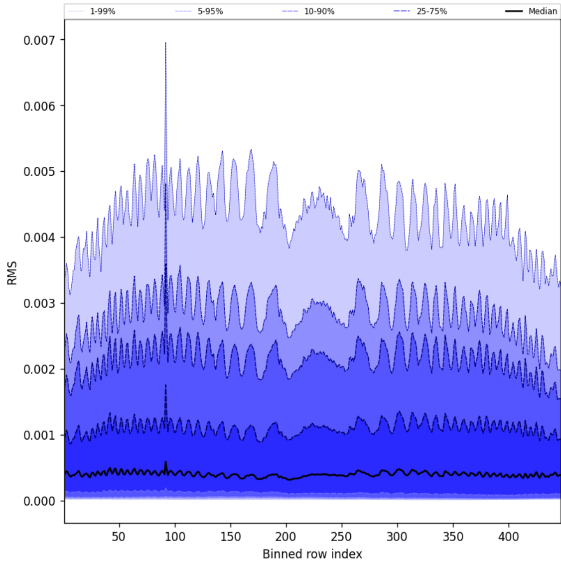
Figure 61: Along track statistics of “RMS” for 2025-05-31 to 2025-06-01
