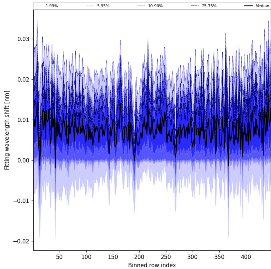
Figure 63: Along track statistics of “Fitting wavelength shift” for 2025-05-31 to 2025-06-01
