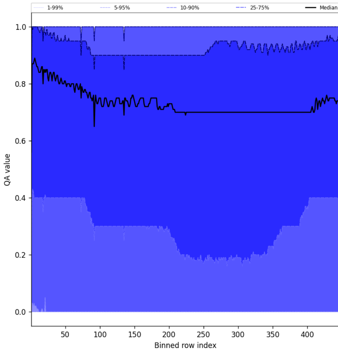
Figure 52: Along track statistics of “QA value” for 2025-05-31 to 2025-06-01
