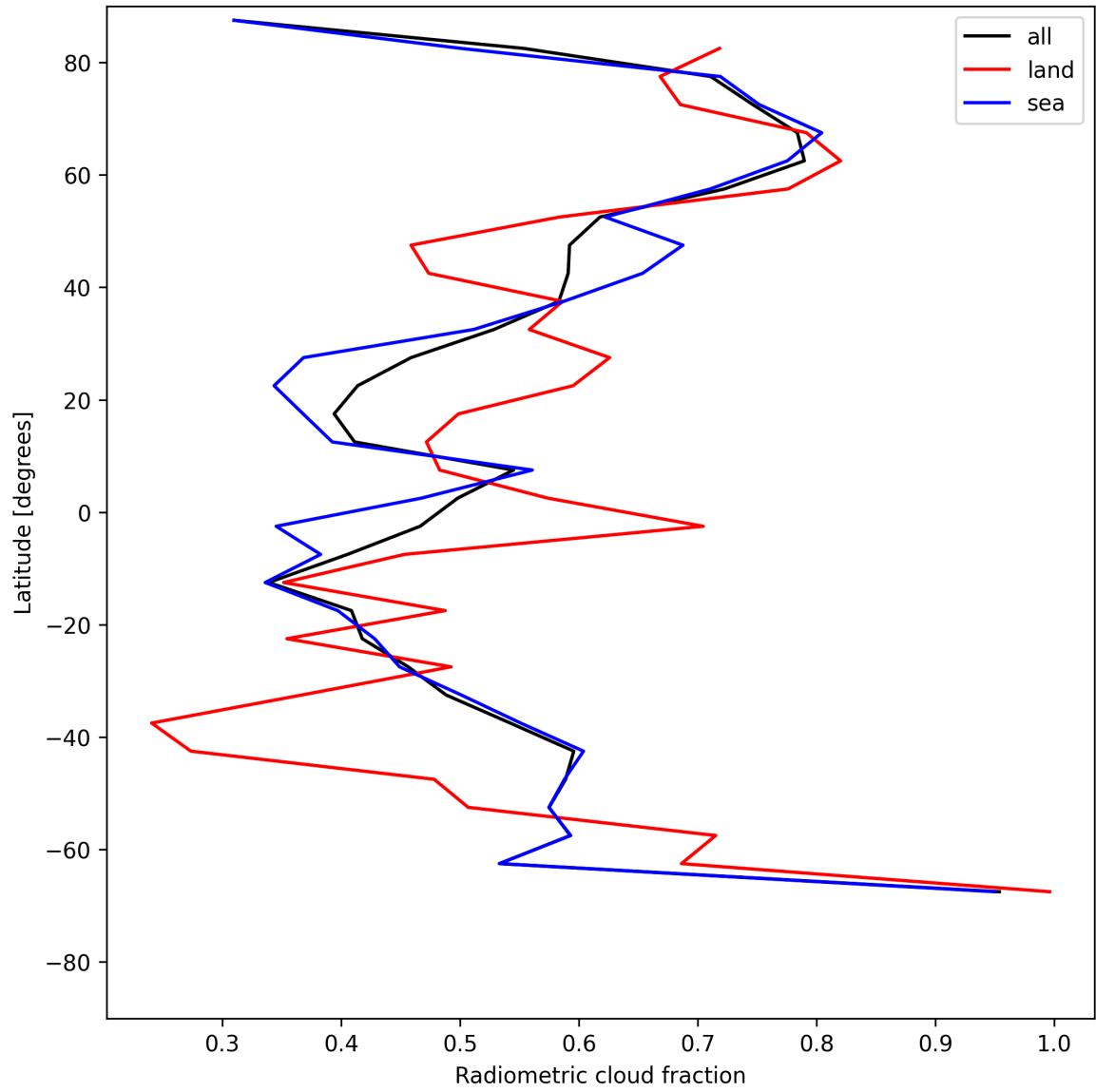
Figure 21: Zonal average of “Radiometric cloud fraction” for 2025-05-31 to 2025-06-01.
