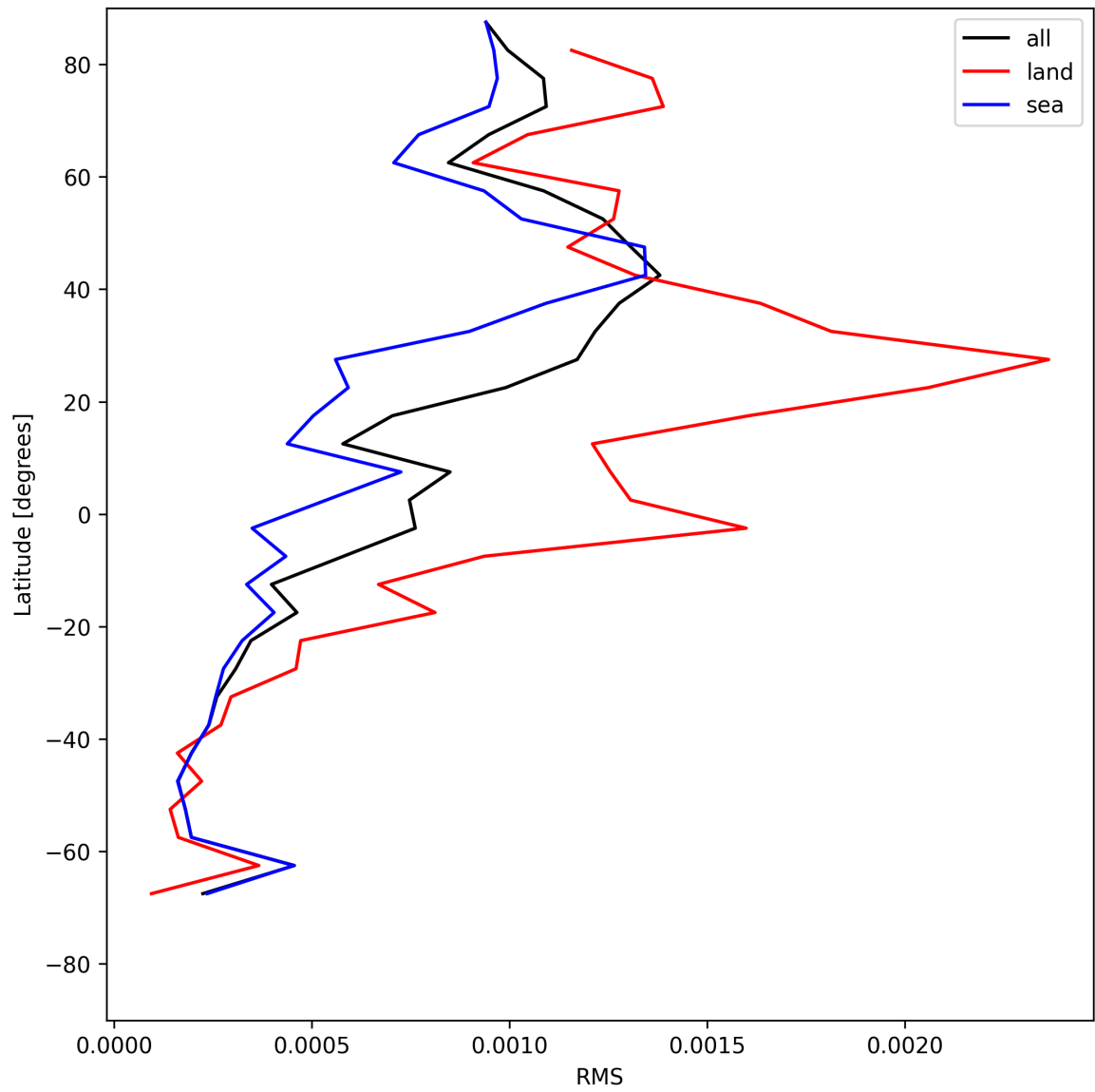
Figure 29: Zonal average of “RMS” for 2025-05-31 to 2025-06-01.
