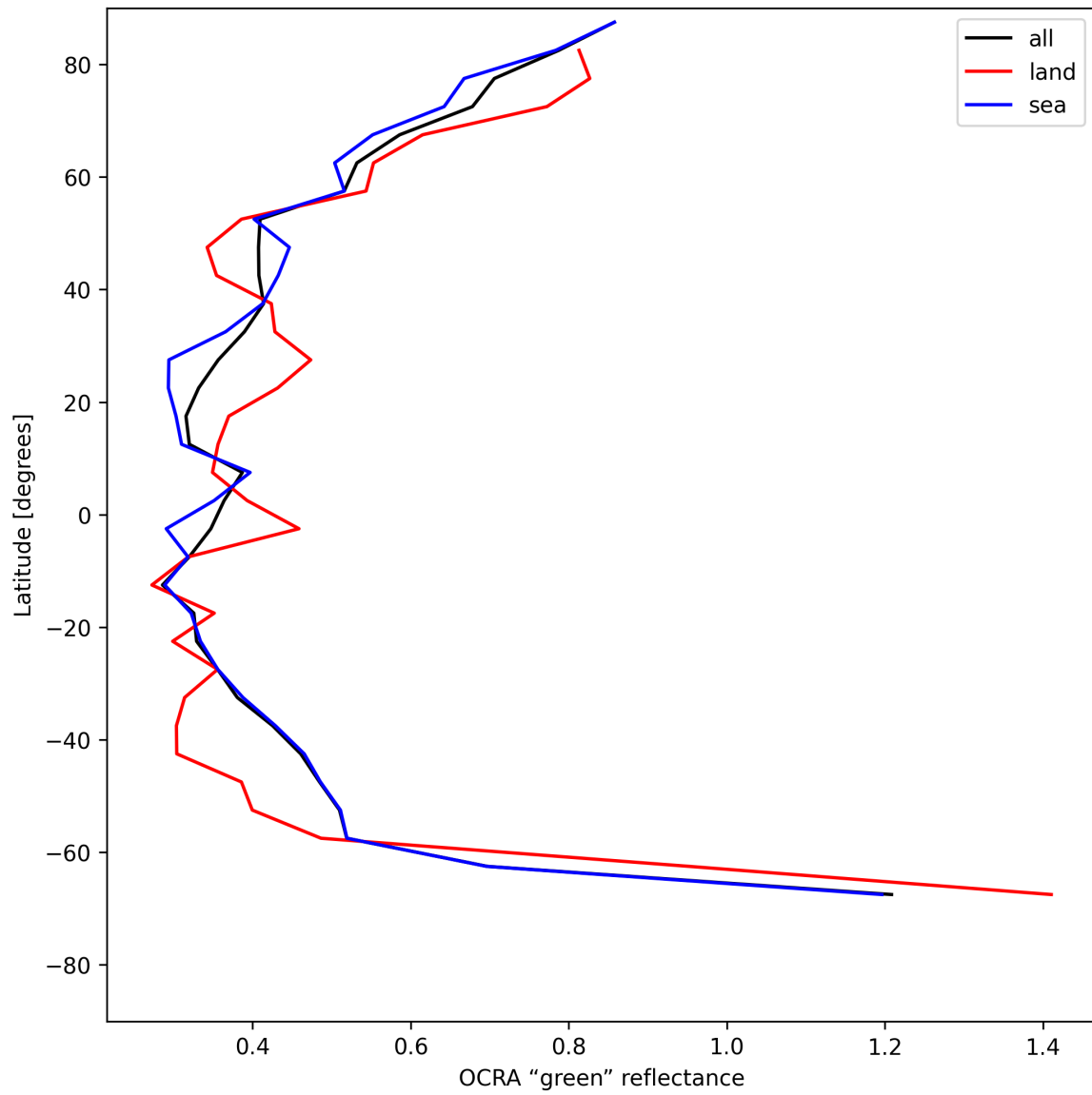
Figure 34: Zonal average of “OCRA “green” reflectance” for 2025-05-31 to 2025-06-01.
