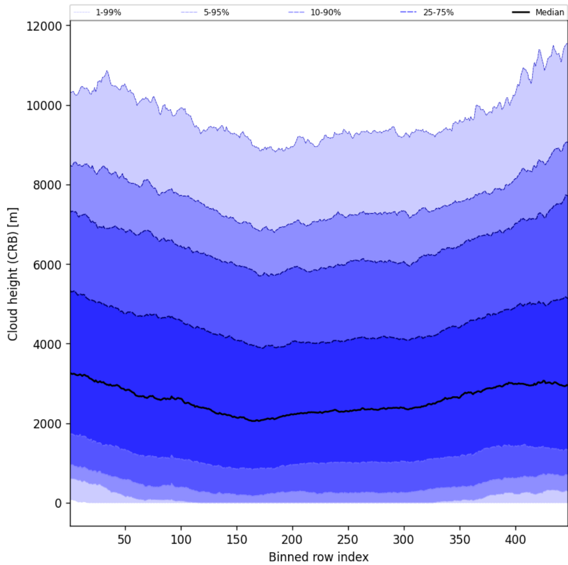
Figure 57: Along track statistics of “Cloud height (CRB)” for 2025-05-31 to 2025-06-01
