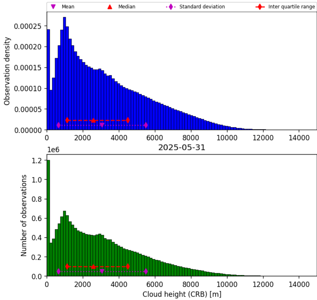
Figure 41: Histogram of “Cloud height (CRB)” for 2025-05-31 to 2025-06-01
