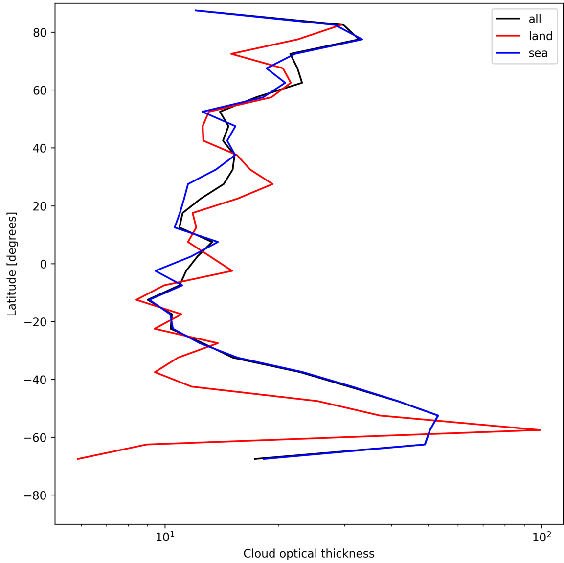
Figure 23: Zonal average of “Cloud optical thickness” for 2025-05-31 to 2025-06-01.
