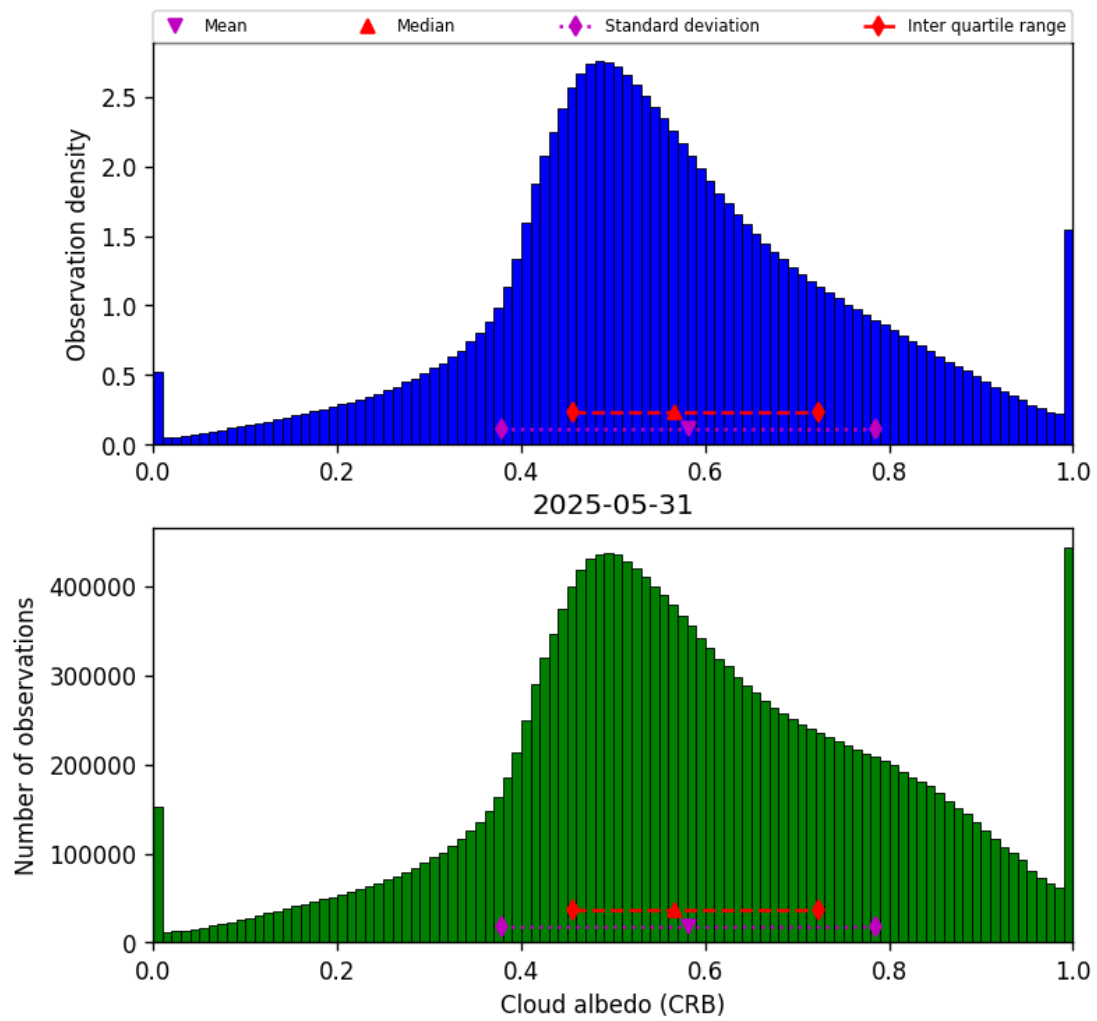
Figure 42: Histogram of “Cloud albedo (CRB)” for 2025-05-31 to 2025-06-01
