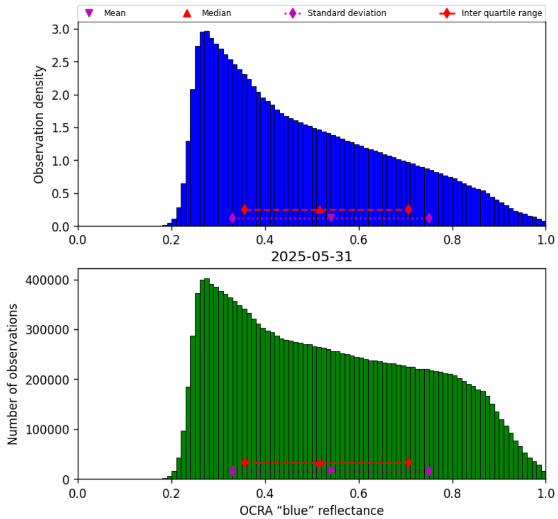
Figure 49: Histogram of “OCRA “blue” reflectance” for 2025-05-31 to 2025-06-01
