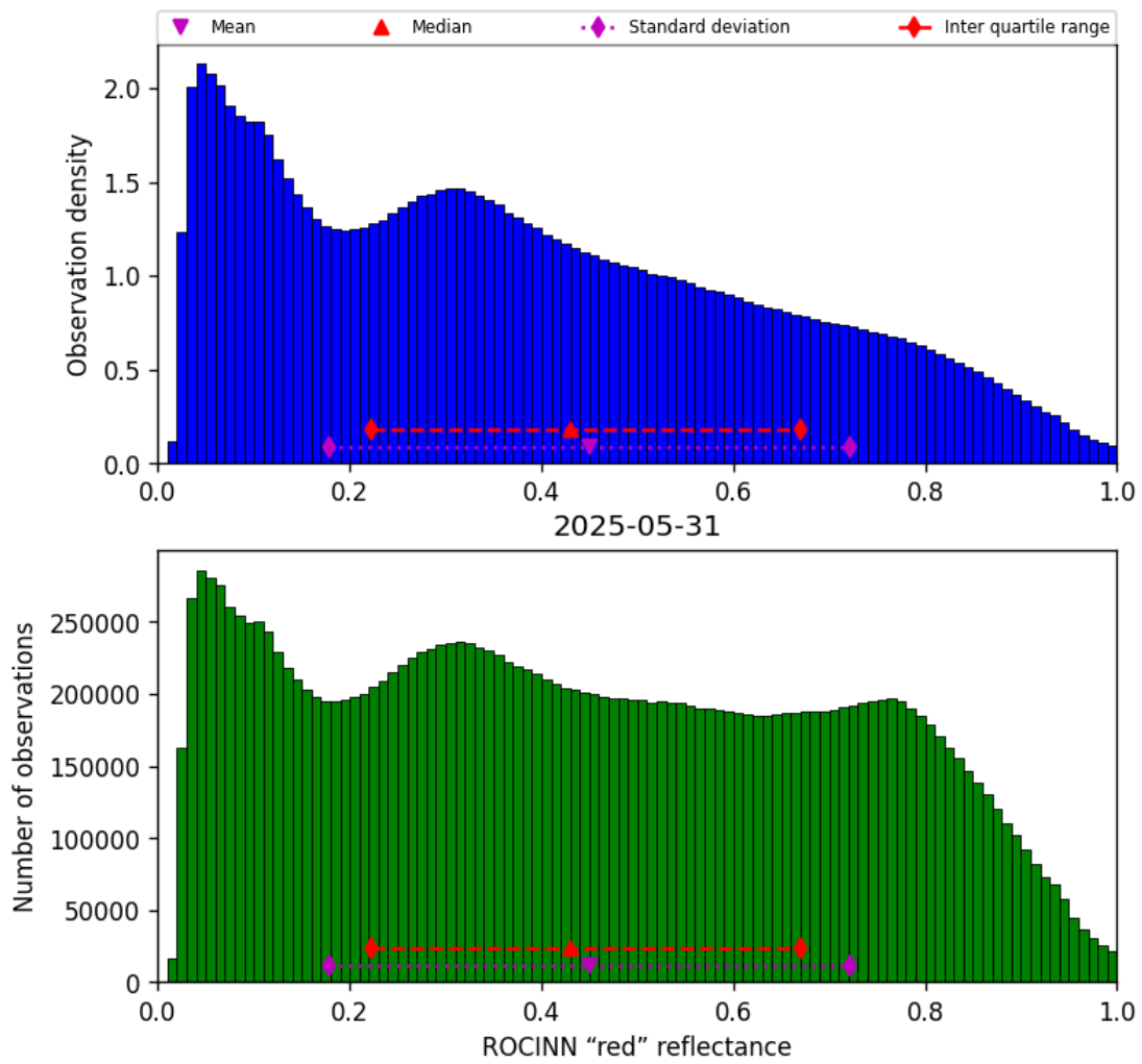
Figure 51: Histogram of “ROCINN “red” reflectance” for 2025-05-31 to 2025-06-01
