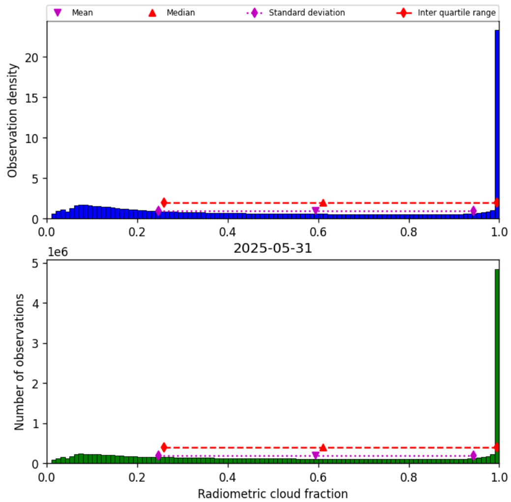
Figure 37: Histogram of “Radiometric cloud fraction” for 2025-05-31 to 2025-06-01
