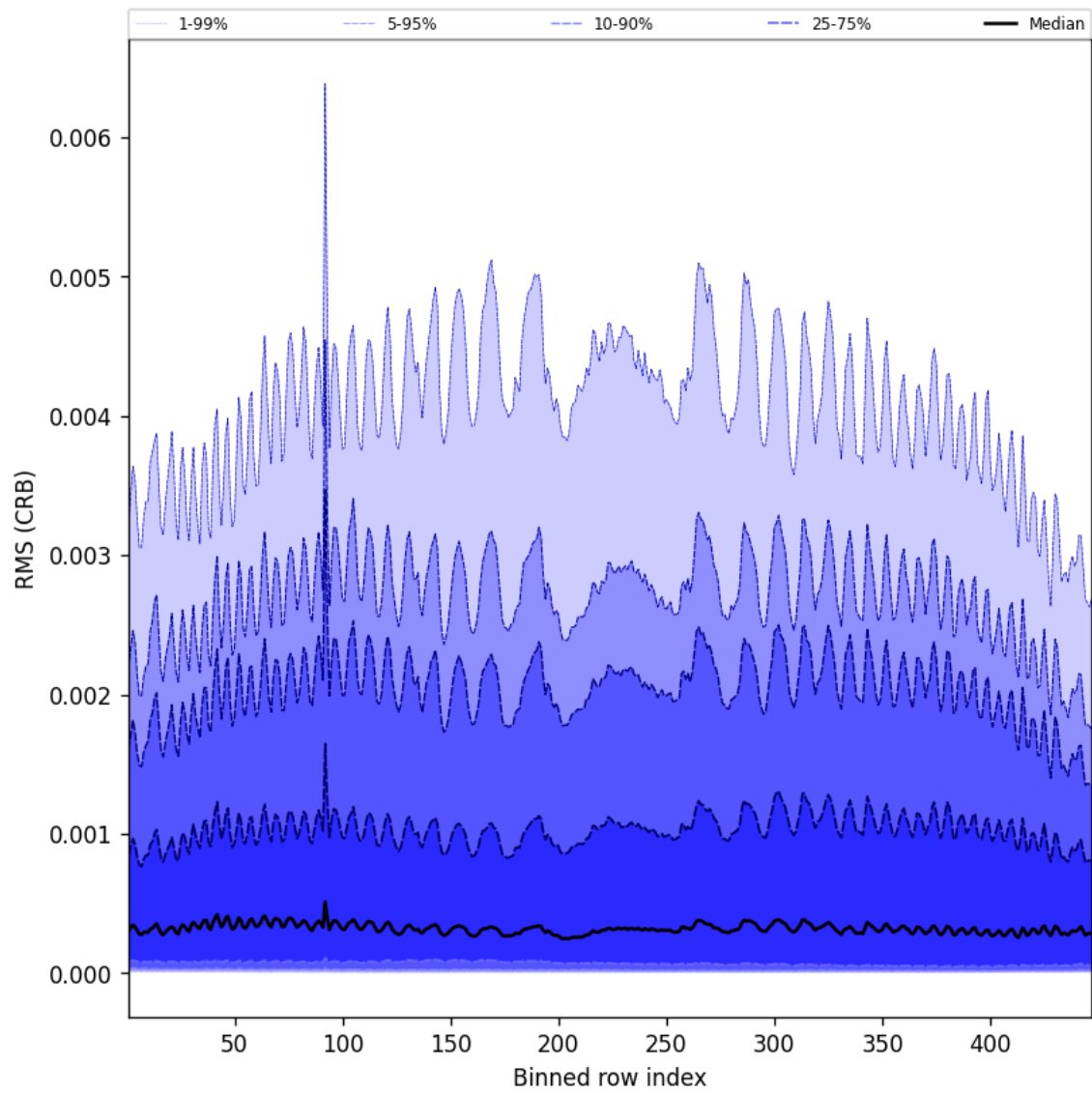
Figure 62: Along track statistics of “RMS (CRB)” for 2025-05-31 to 2025-06-01
