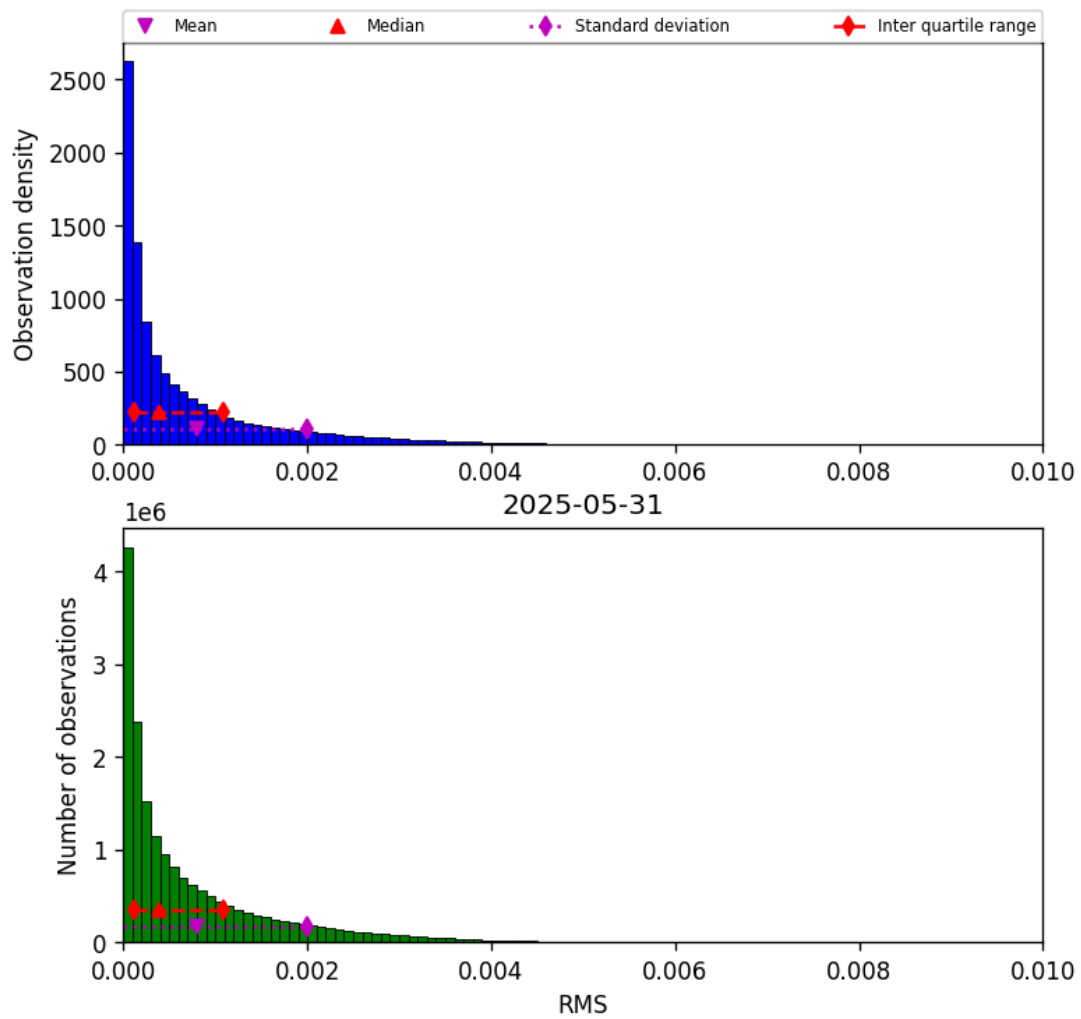
Figure 45: Histogram of “RMS” for 2025-05-31 to 2025-06-01
