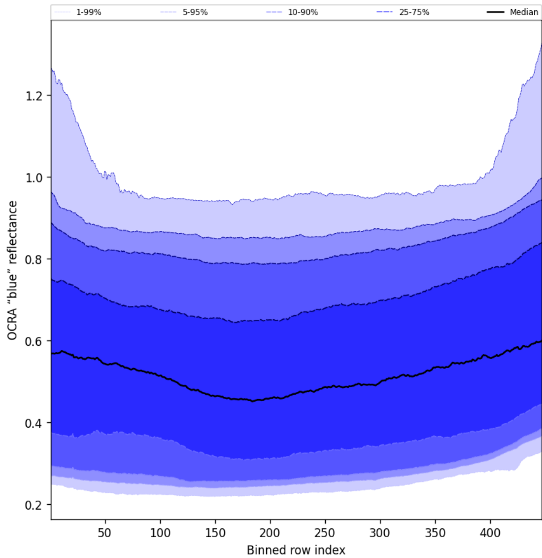
Figure 65: Along track statistics of “OCRA “blue” reflectance” for 2025-05-31 to 2025-06-01
