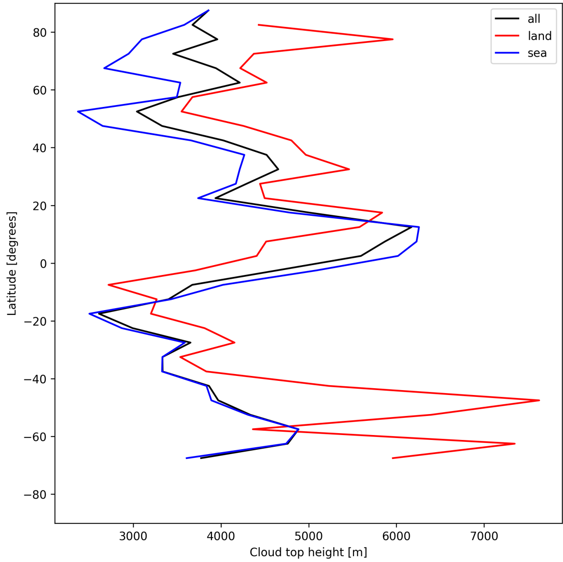
Figure 22: Zonal average of “Cloud top height” for 2025-05-31 to 2025-06-01.
