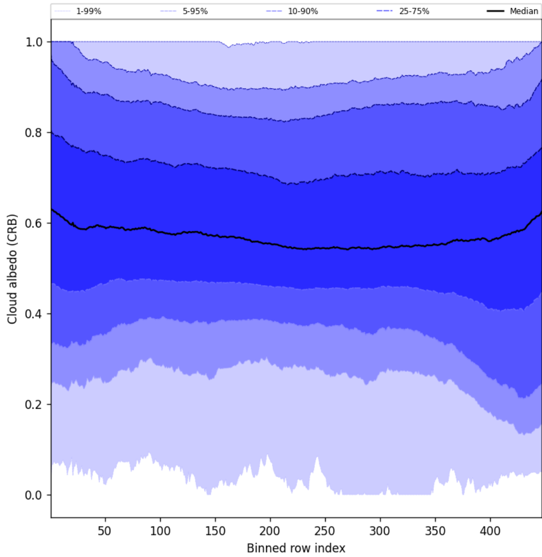
Figure 58: Along track statistics of “Cloud albedo (CRB)” for 2025-05-31 to 2025-06-01
