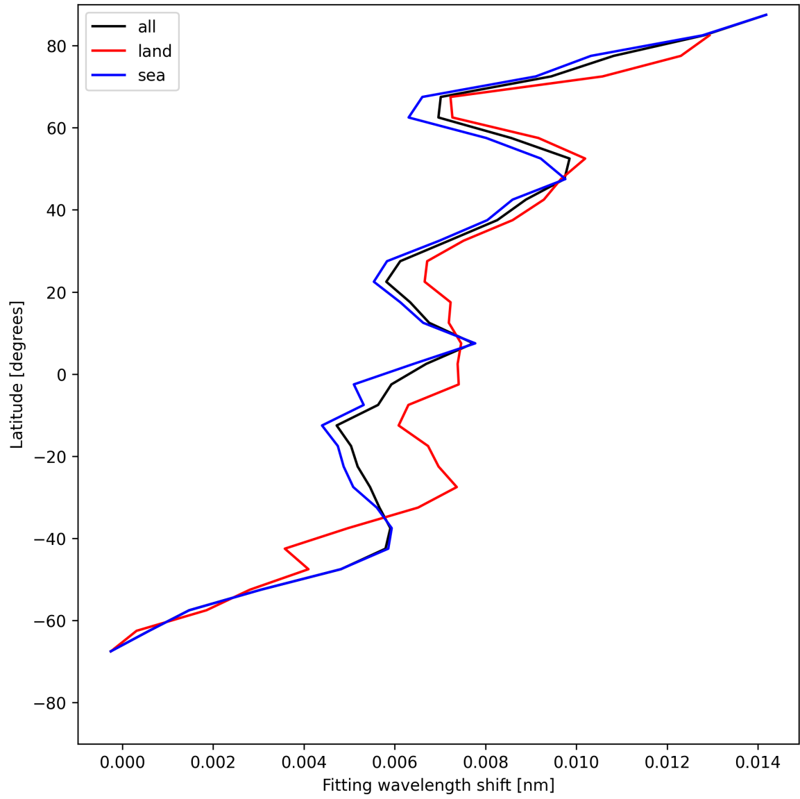
Figure 31: Zonal average of “Fitting wavelength shift” for 2025-05-31 to 2025-06-01.
