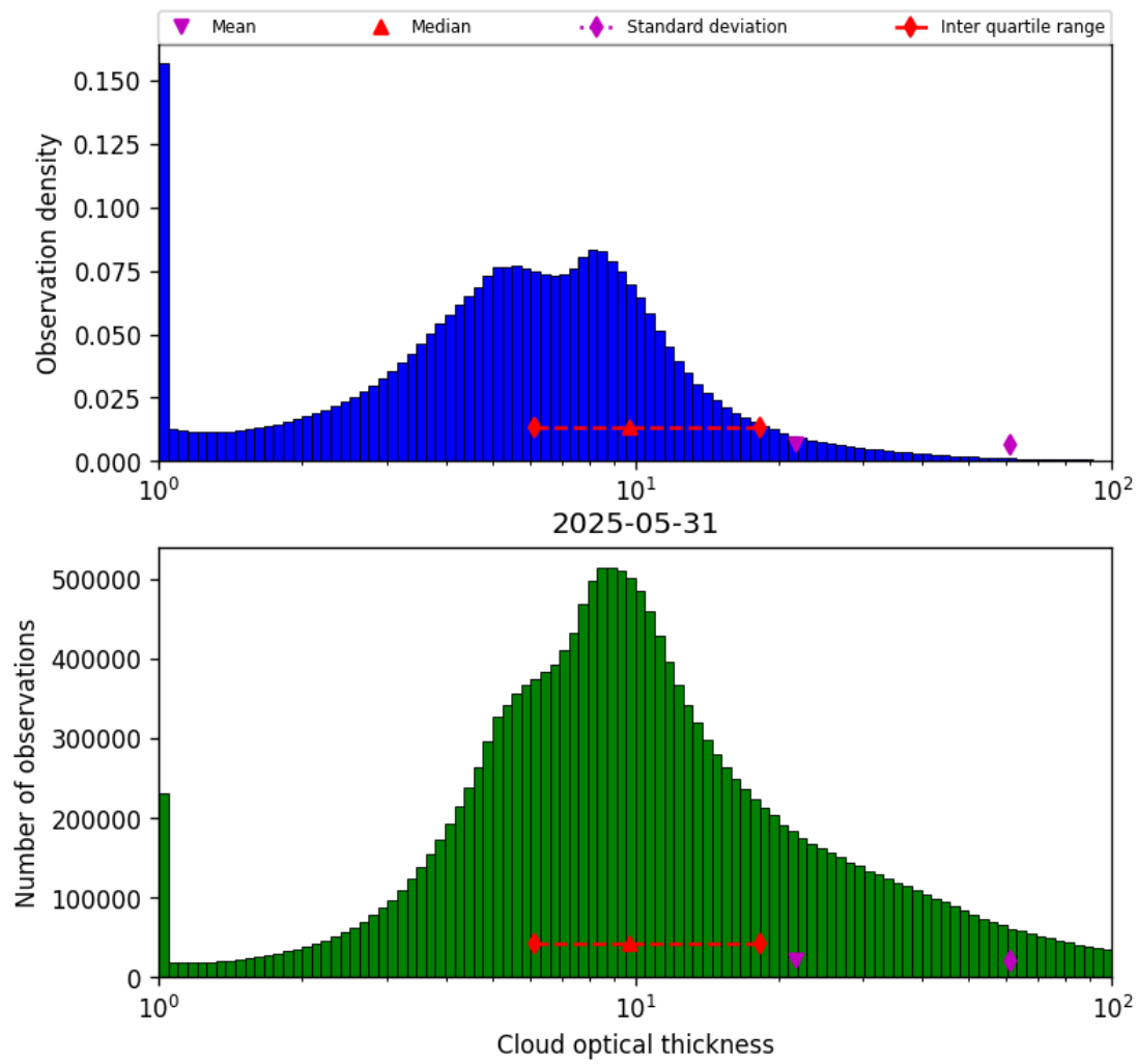
Figure 39: Histogram of “Cloud optical thickness” for 2025-05-31 to 2025-06-01
