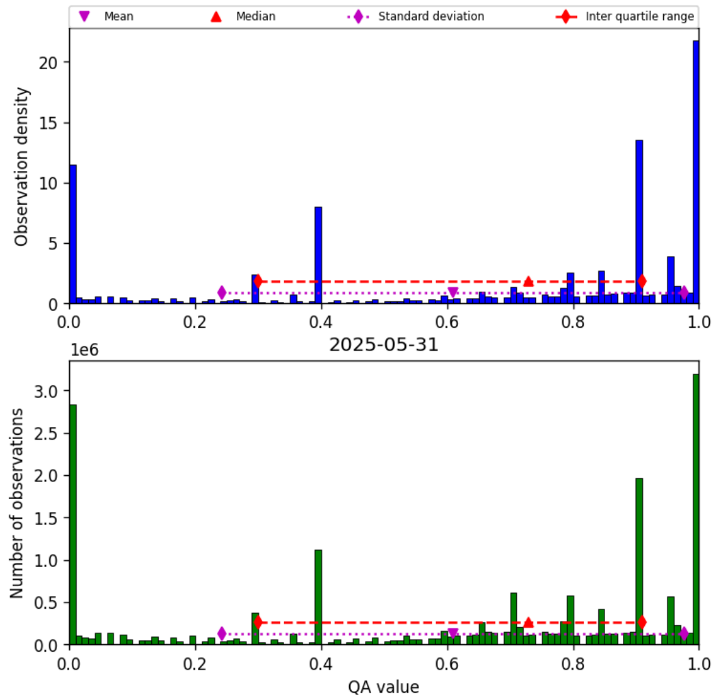
Figure 36: Histogram of “QA value” for 2025-05-31 to 2025-06-01
