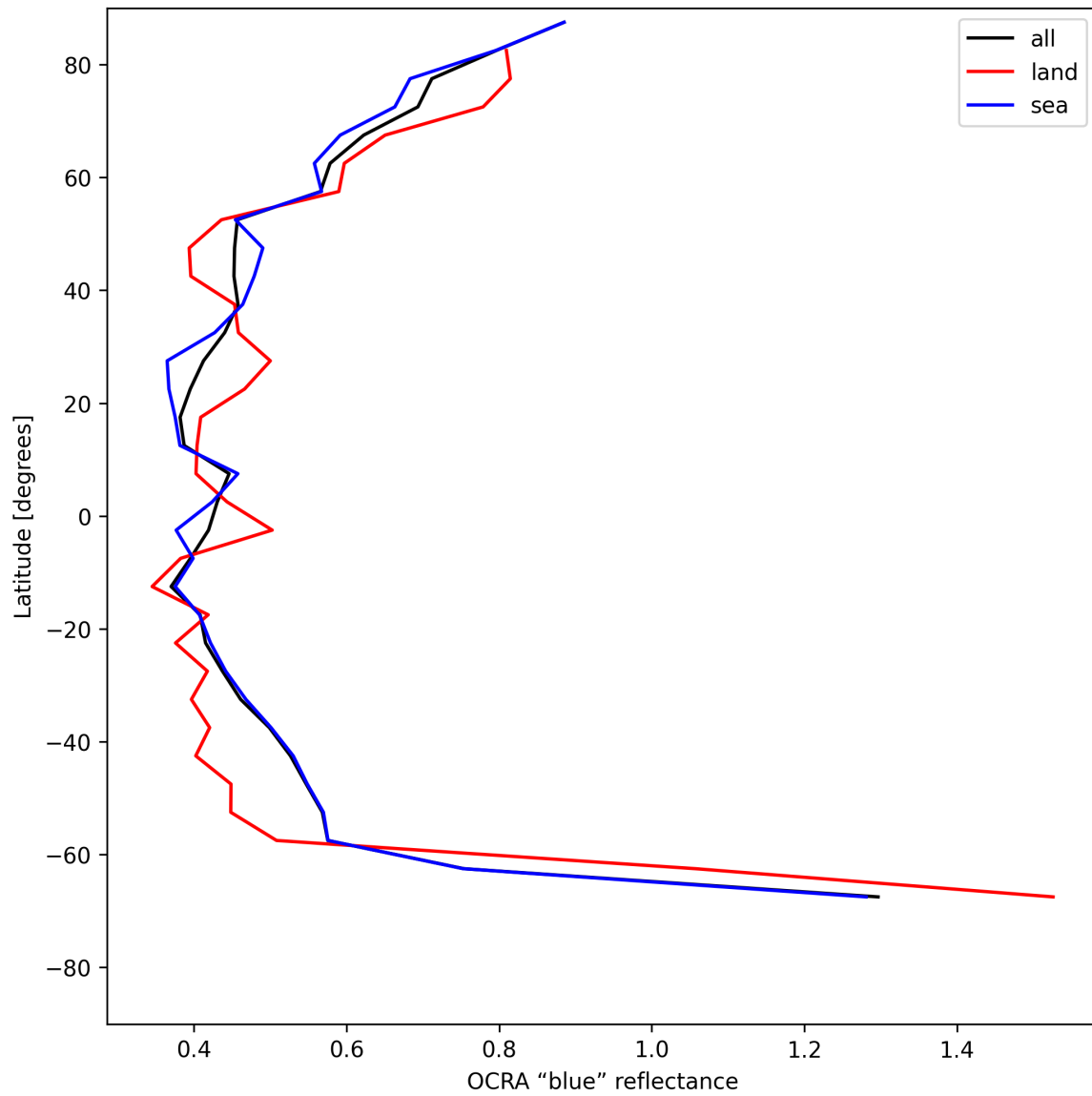
Figure 33: Zonal average of “OCRA “blue” reflectance” for 2025-05-31 to 2025-06-01.
