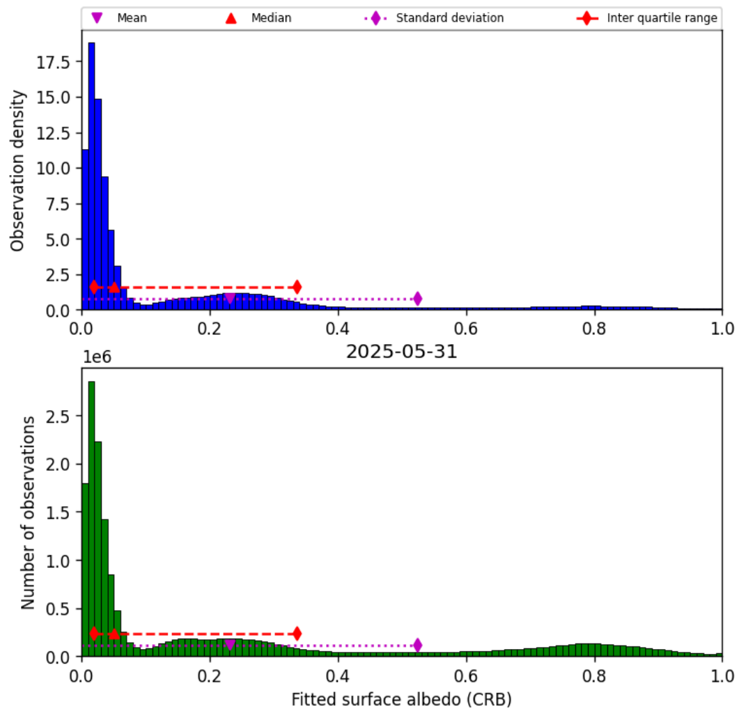
Figure 44: Histogram of “Fitted surface albedo (CRB)” for 2025-05-31 to 2025-06-01
