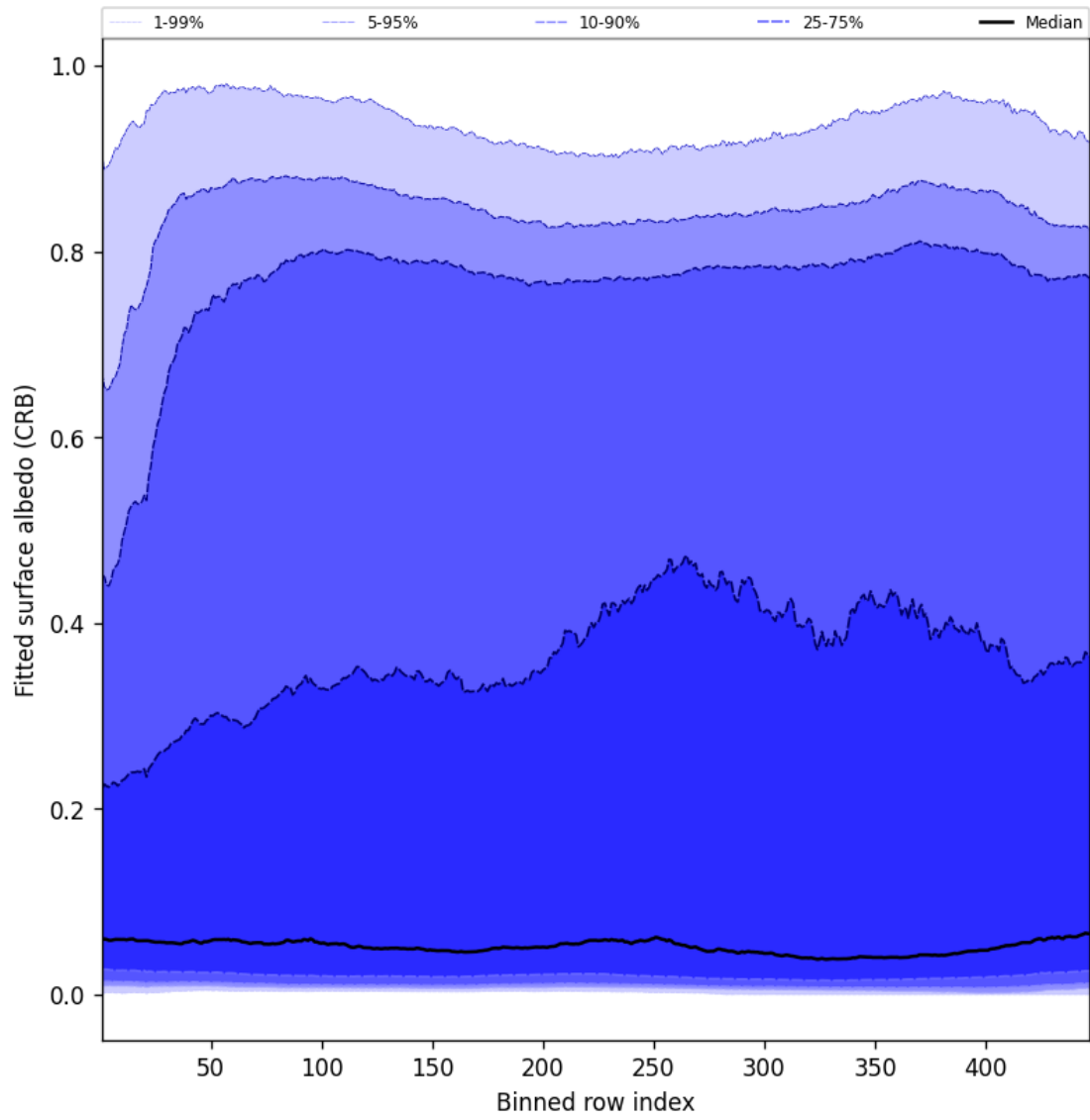
Figure 60: Along track statistics of “Fitted surface albedo (CRB)” for 2025-05-31 to 2025-06-01
