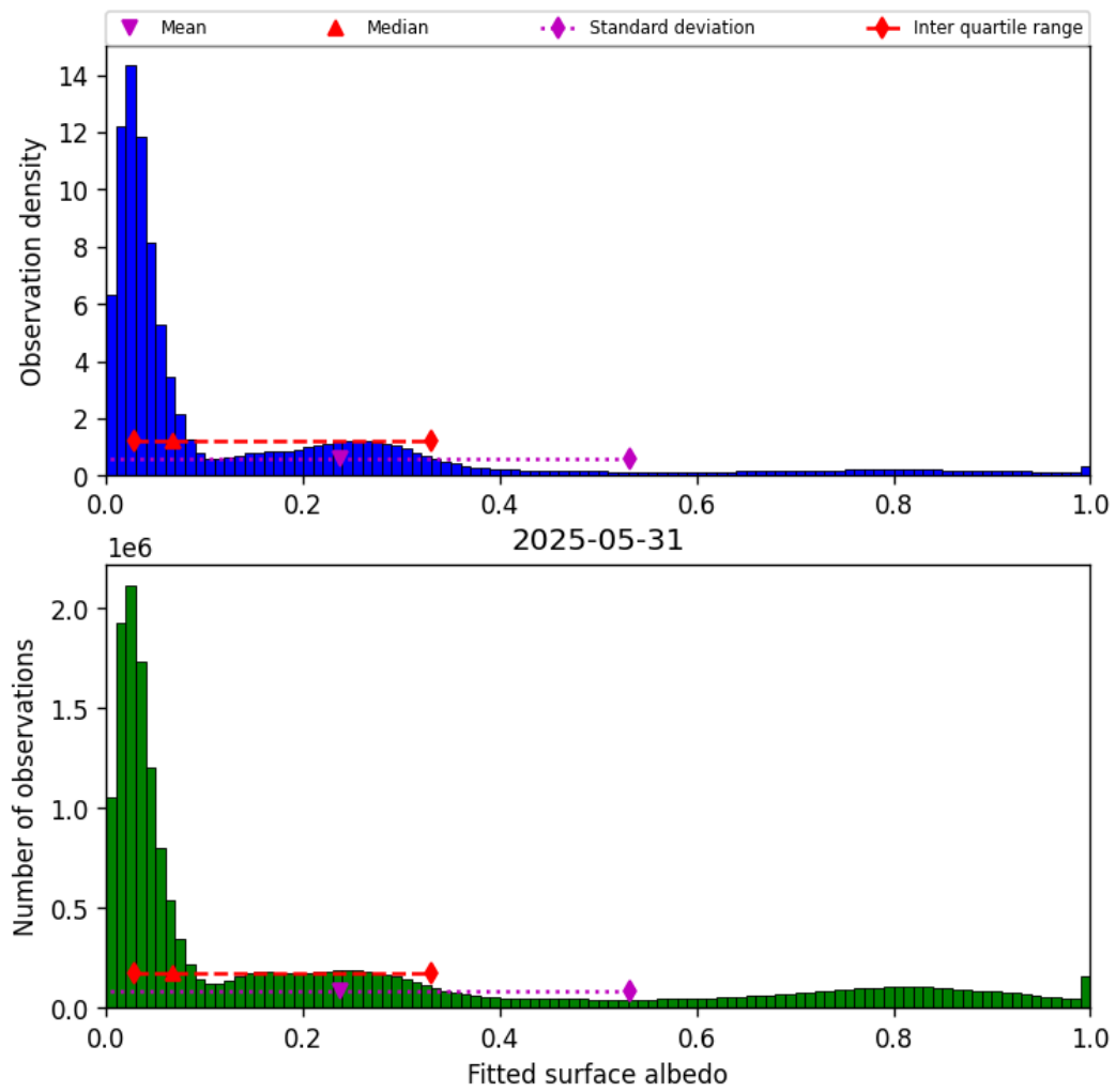
Figure 43: Histogram of “Fitted surface albedo” for 2025-05-31 to 2025-06-01
