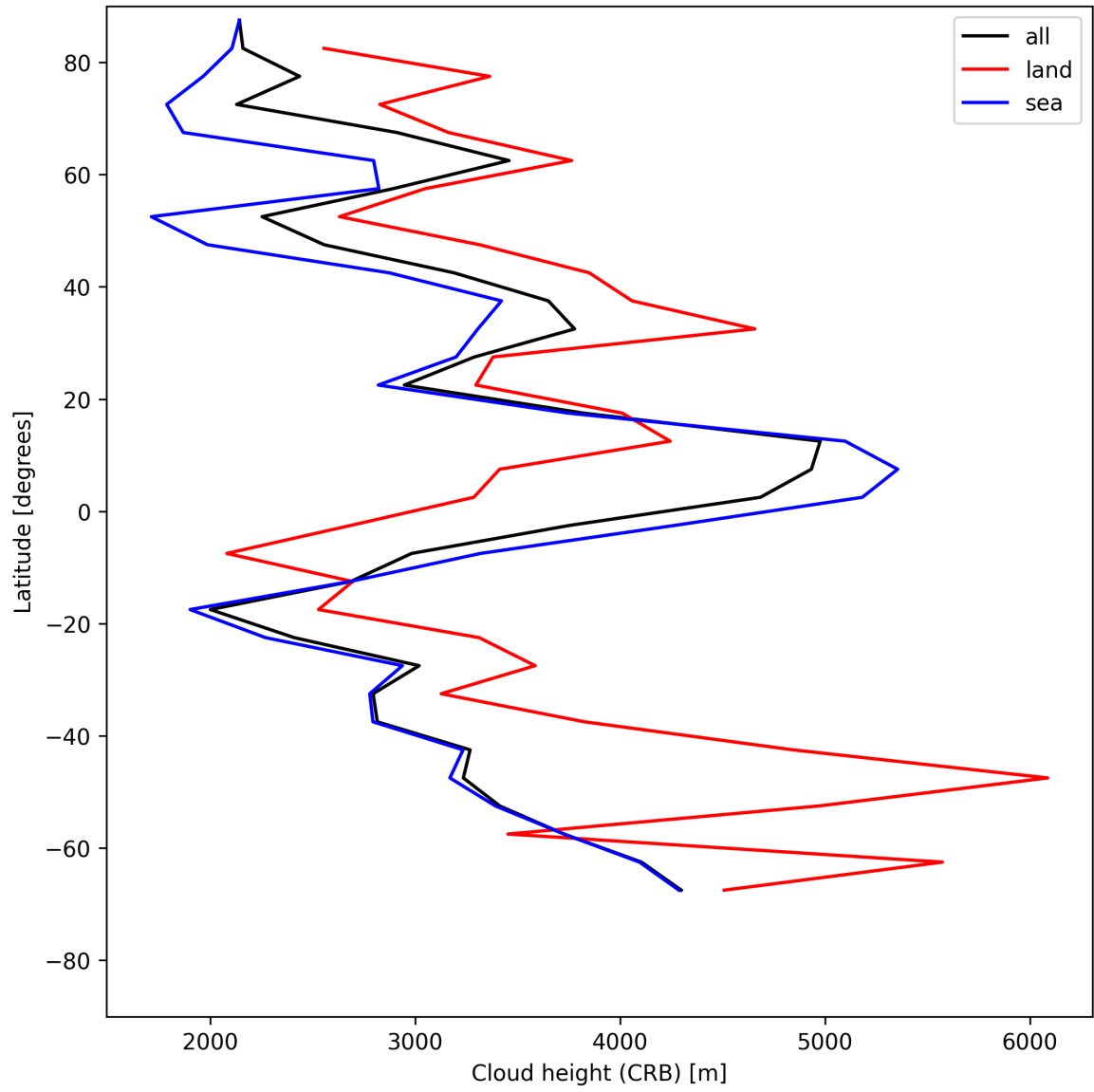
Figure 25: Zonal average of “Cloud height (CRB)” for 2025-05-31 to 2025-06-01.
