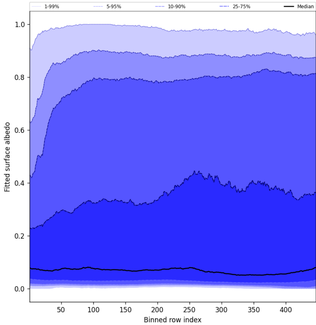
Figure 59: Along track statistics of “Fitted surface albedo” for 2025-05-31 to 2025-06-01
