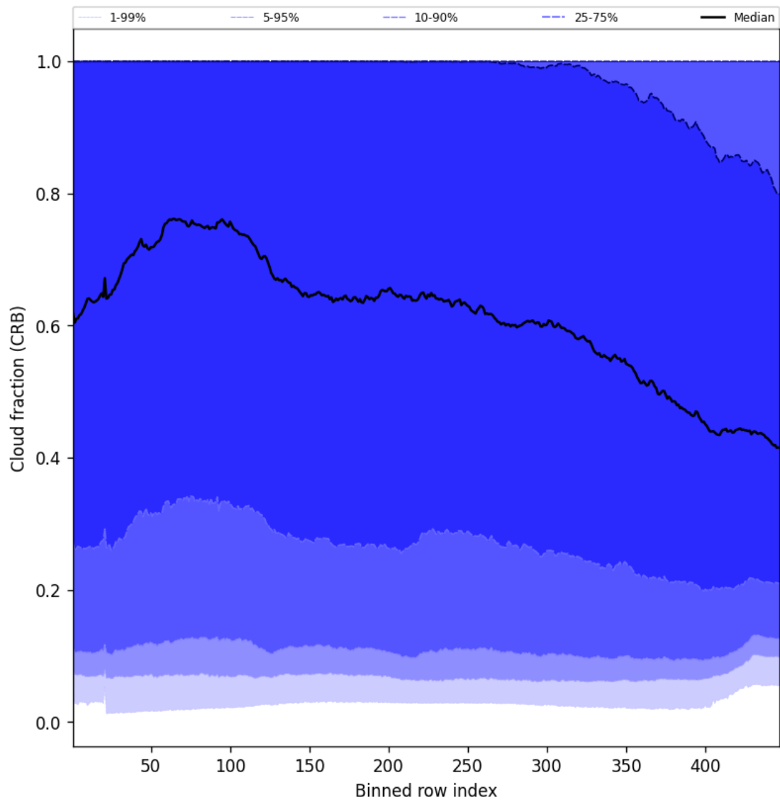
Figure 56: Along track statistics of “Cloud fraction (CRB)” for 2025-05-31 to 2025-06-01
