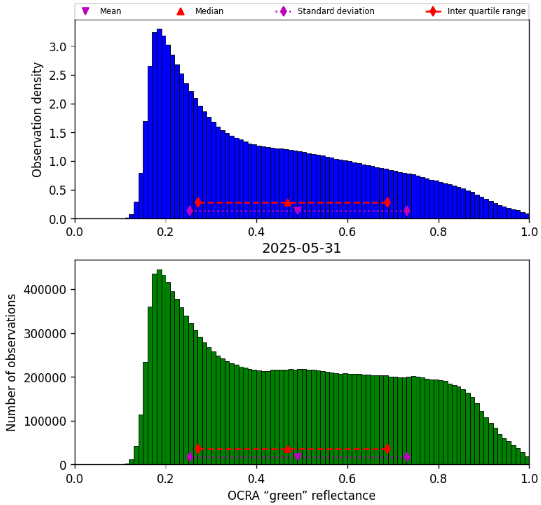
Figure 50: Histogram of “OCRA “green” reflectance” for 2025-05-31 to 2025-06-01
