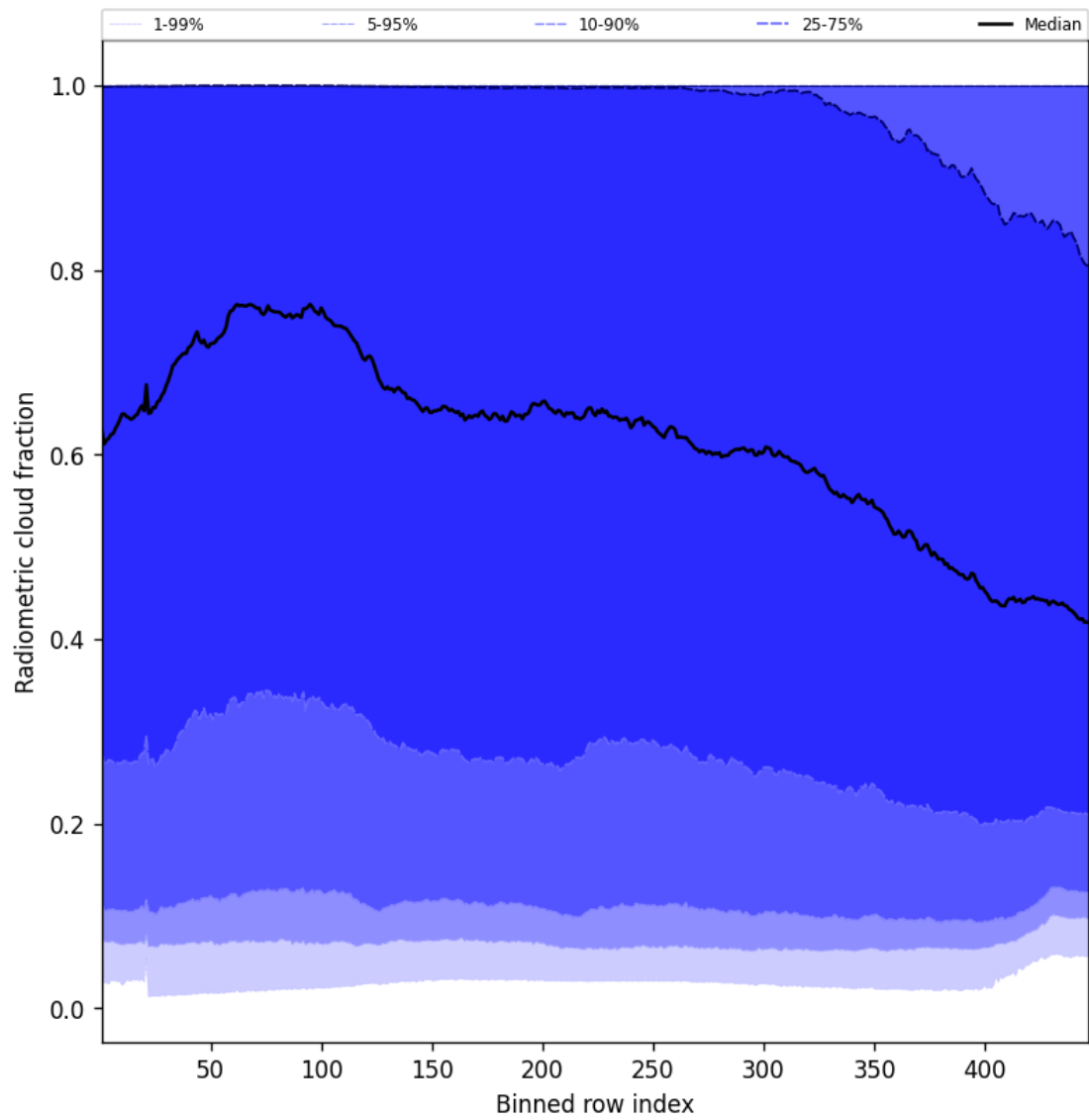
Figure 53: Along track statistics of “Radiometric cloud fraction” for 2025-05-31 to 2025-06-01
