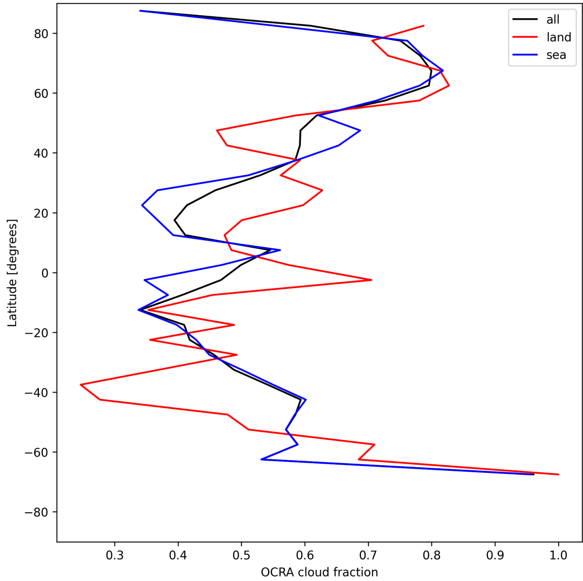
Figure 32: Zonal average of “OCRA cloud fraction” for 2025-05-31 to 2025-06-01.
