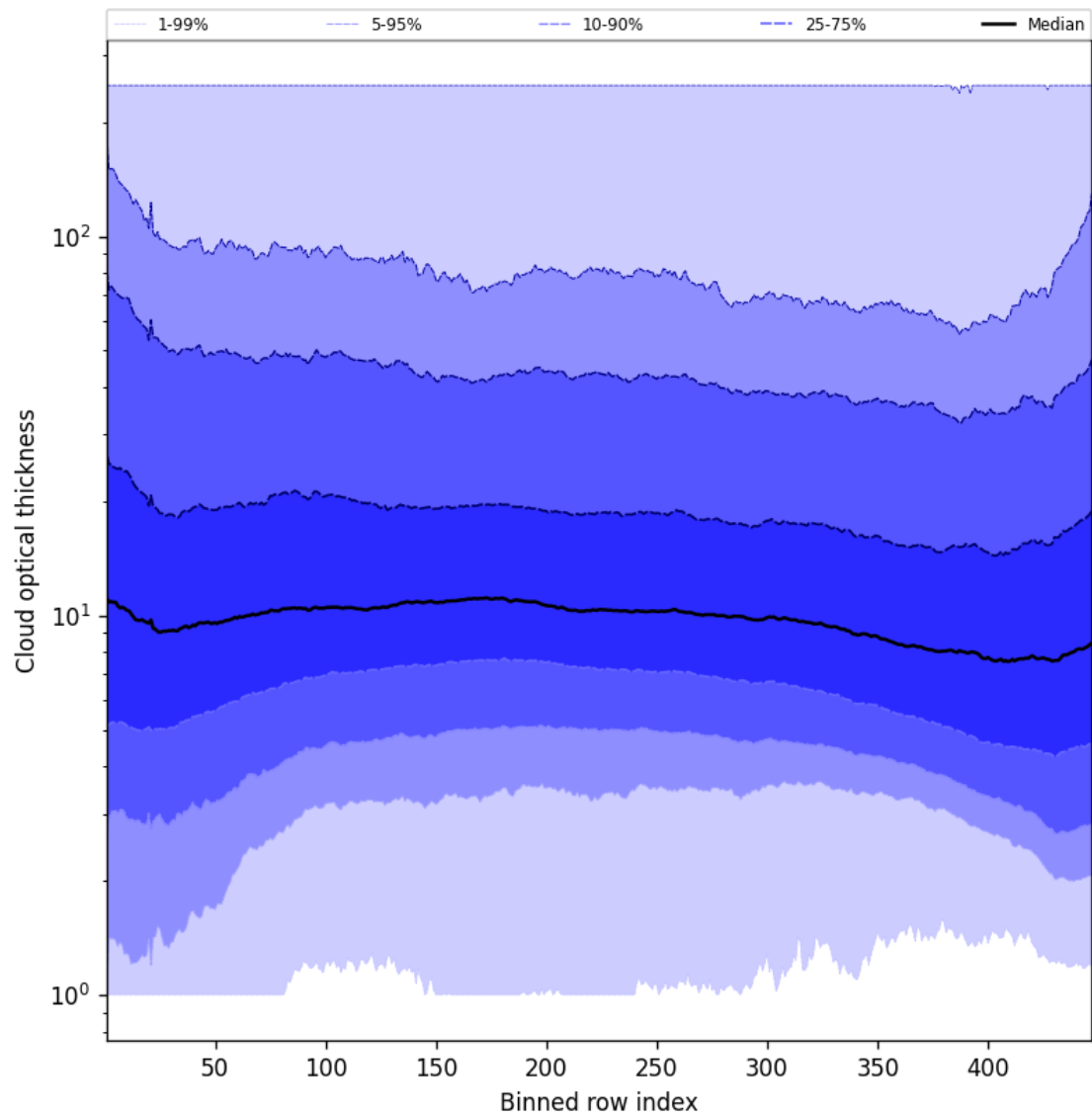
Figure 55: Along track statistics of “Cloud optical thickness” for 2025-05-31 to 2025-06-01
