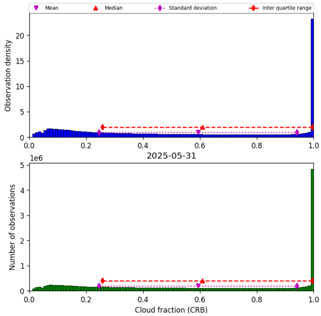
Figure 40: Histogram of “Cloud fraction (CRB)” for 2025-05-31 to 2025-06-01
