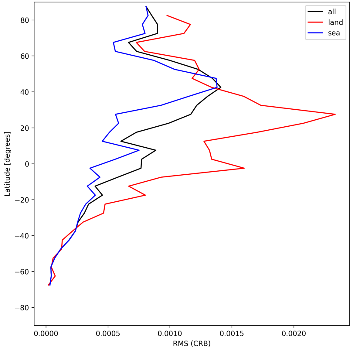
Figure 30: Zonal average of “RMS (CRB)” for 2025-05-31 to 2025-06-01.
