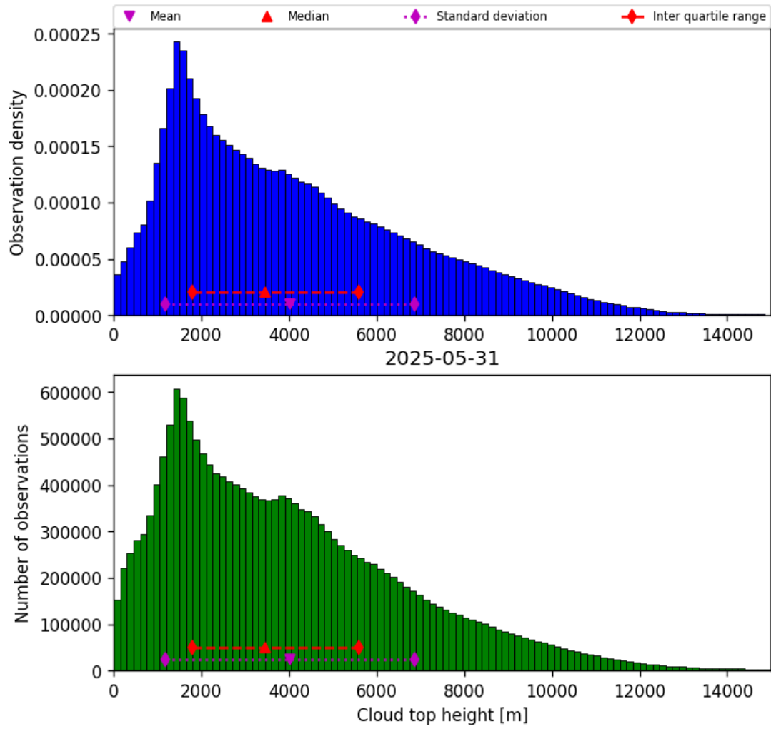
Figure 38: Histogram of “Cloud top height” for 2025-05-31 to 2025-06-01
