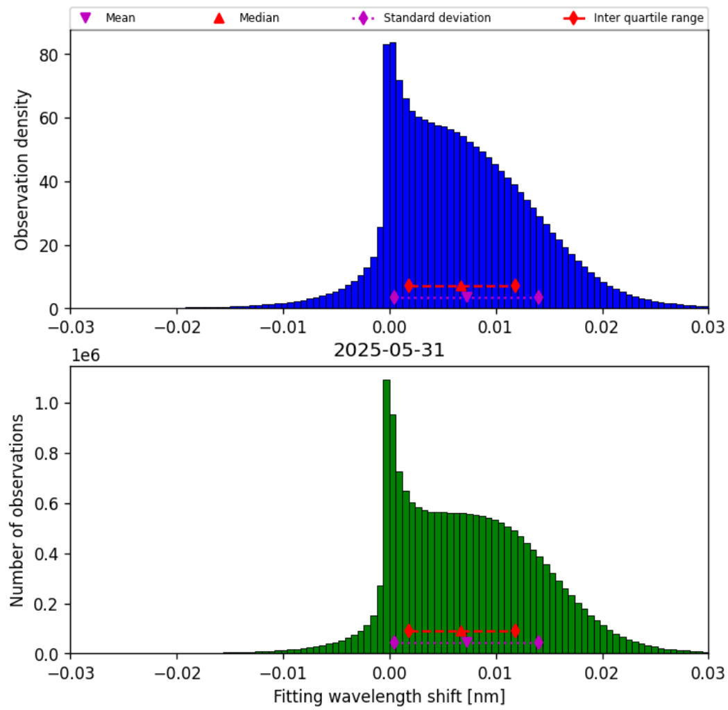
Figure 47: Histogram of “Fitting wavelength shift” for 2025-05-31 to 2025-06-01
