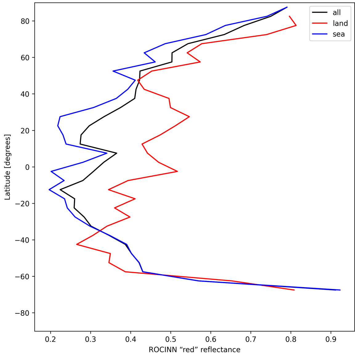
Figure 35: Zonal average of “ROCINN “red” reflectance” for 2025-05-31 to 2025-06-01.
