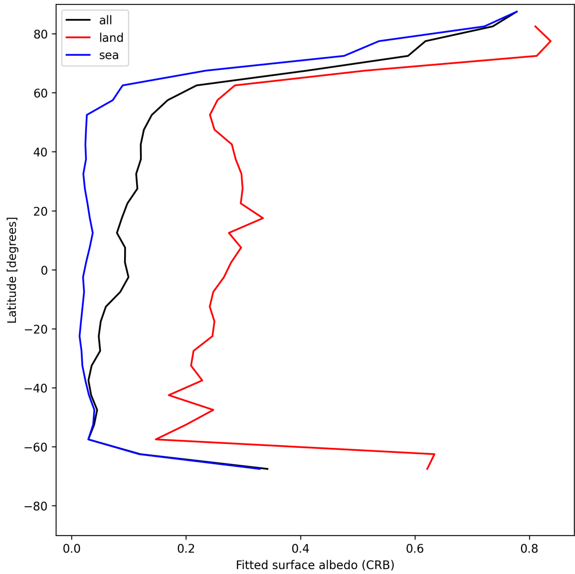
Figure 28: Zonal average of “Fitted surface albedo (CRB)” for 2025-05-31 to 2025-06-01.
