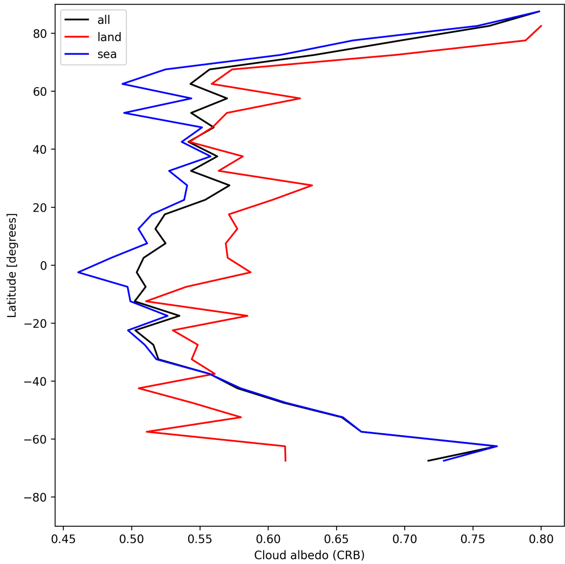
Figure 26: Zonal average of “Cloud albedo (CRB)” for 2025-05-31 to 2025-06-01.
