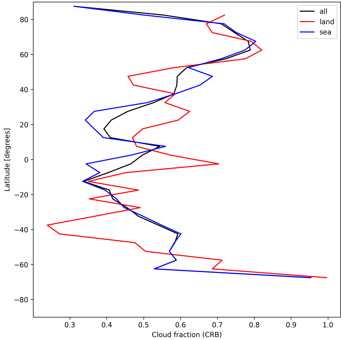
Figure 24: Zonal average of “Cloud fraction (CRB)” for 2025-05-31 to 2025-06-01.
