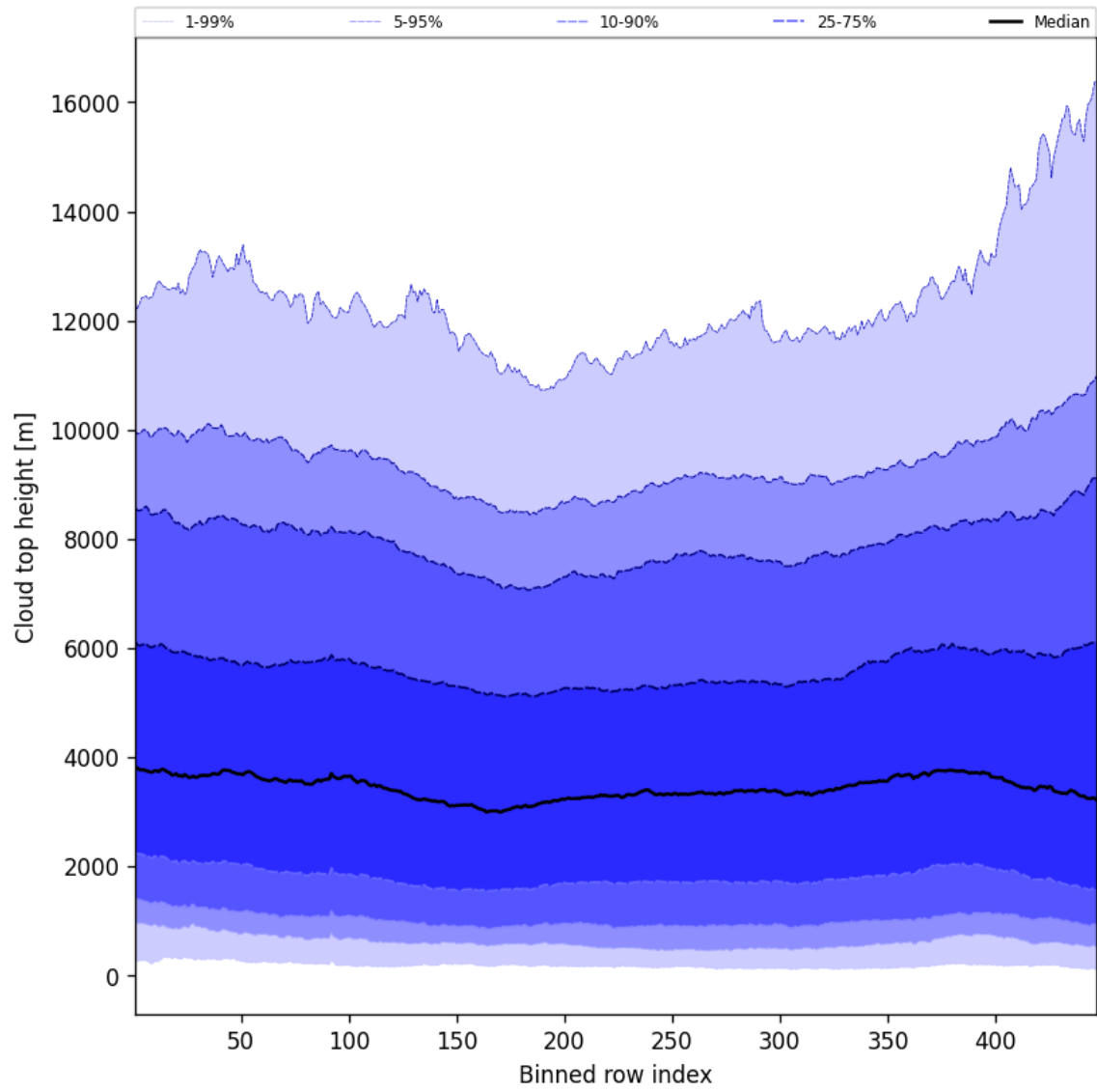
Figure 54: Along track statistics of “Cloud top height” for 2025-05-31 to 2025-06-01
