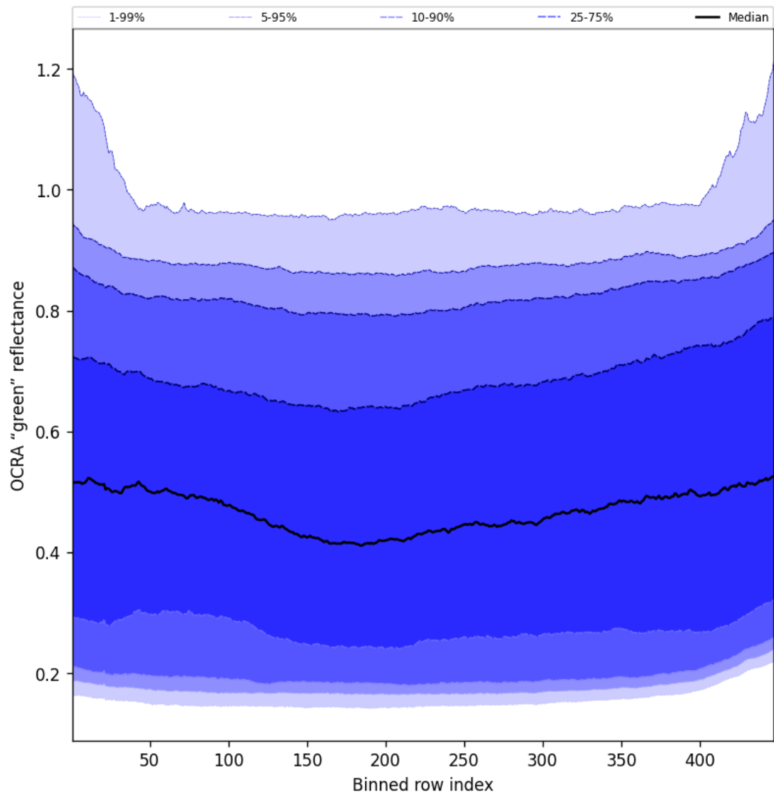
Figure 66: Along track statistics of "OCRA "green" reflectance" for 2025-05-31 to 2025-06-01
