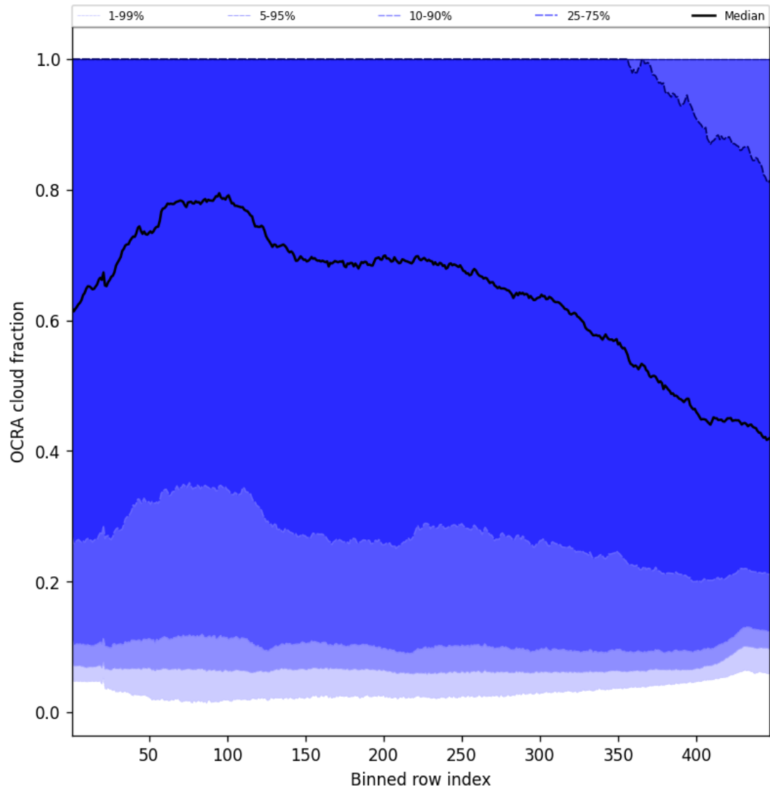
Figure 64: Along track statistics of “OCRA cloud fraction” for 2025-05-31 to 2025-06-01
