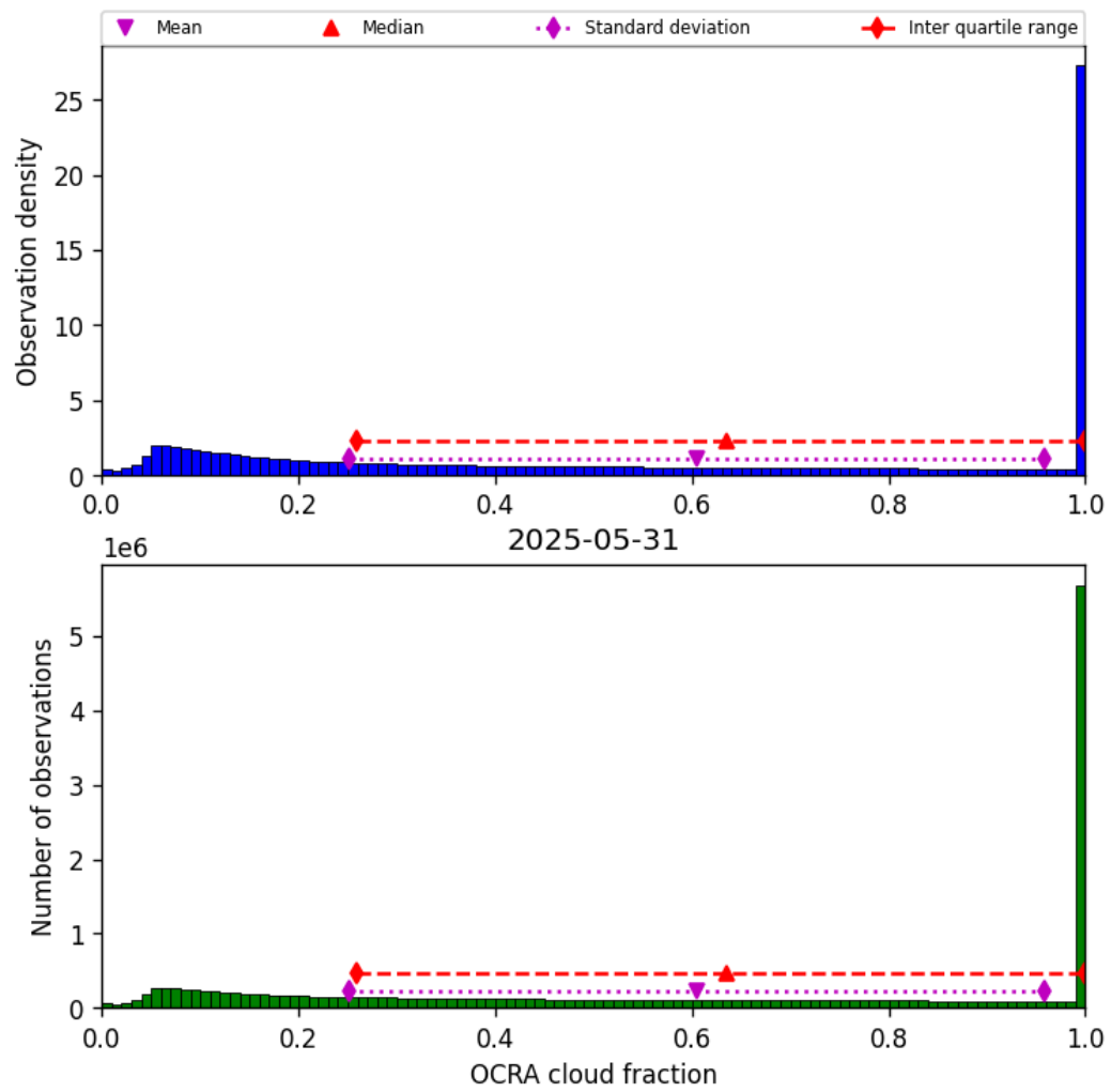
Figure 48: Histogram of “OCRA cloud fraction” for 2025-05-31 to 2025-06-01
