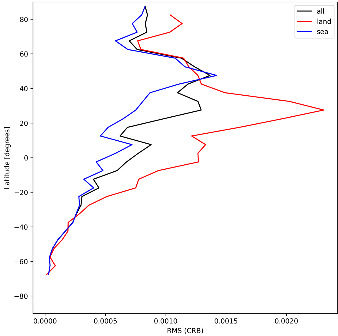
Figure 30: Zonal average of “RMS (CRB)” for 2025-06-01 to 2025-06-02.
