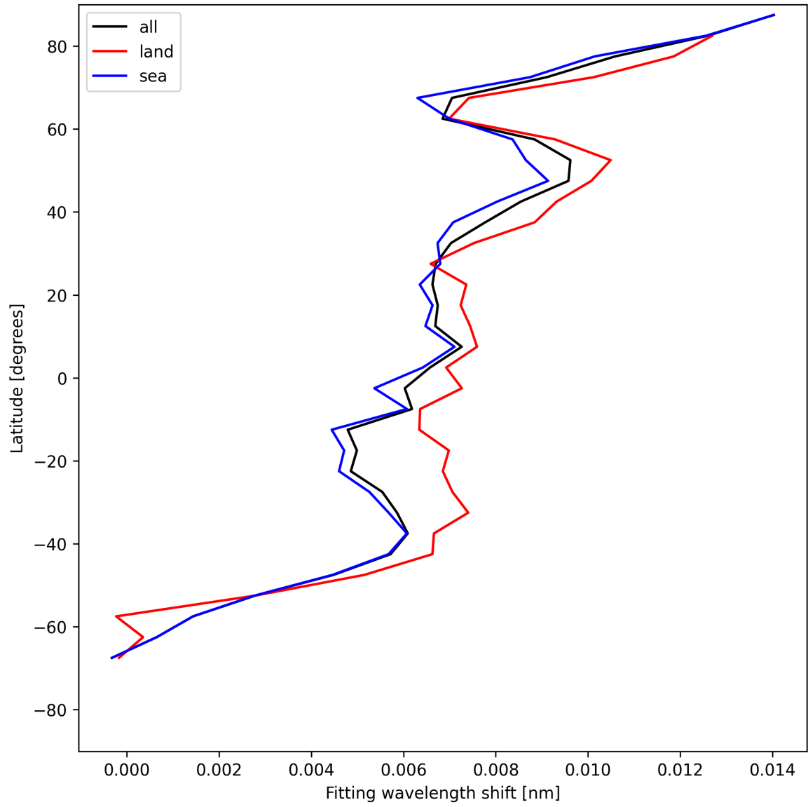
Figure 31: Zonal average of “Fitting wavelength shift” for 2025-06-01 to 2025-06-02.
