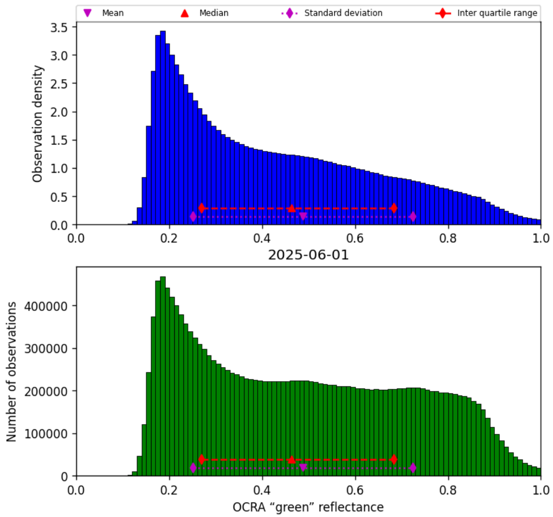
Figure 50: Histogram of “OCRA “green” reflectance” for 2025-06-01 to 2025-06-02
