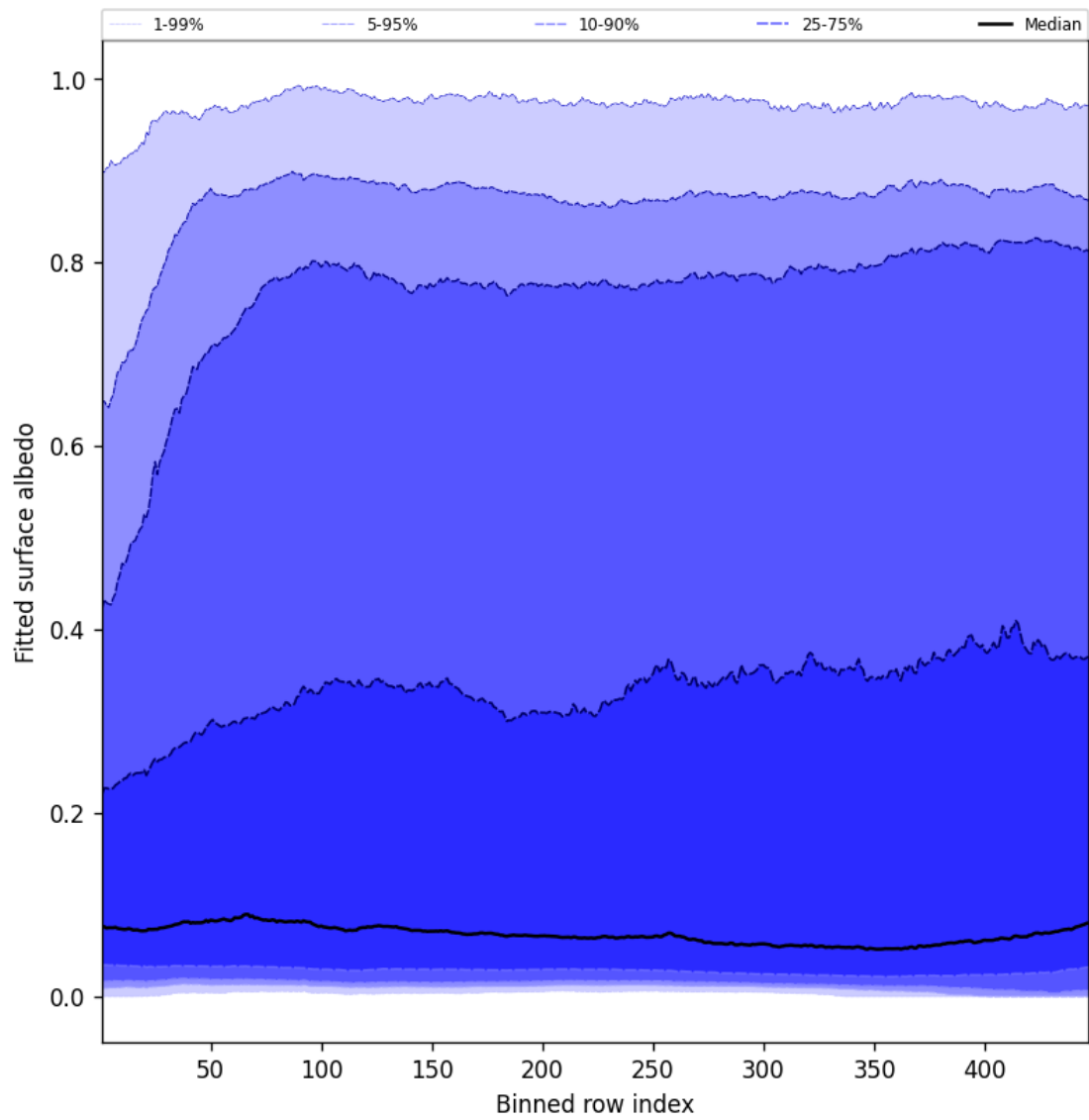
Figure 59: Along track statistics of “Fitted surface albedo” for 2025-06-01 to 2025-06-02
