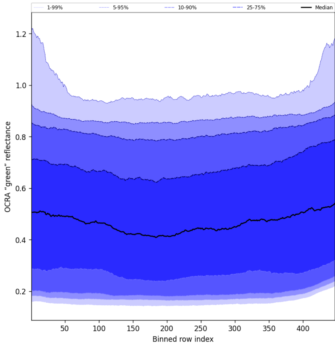
Figure 66: Along track statistics of “OCRA “green” reflectance” for 2025-06-01 to 2025-06-02
