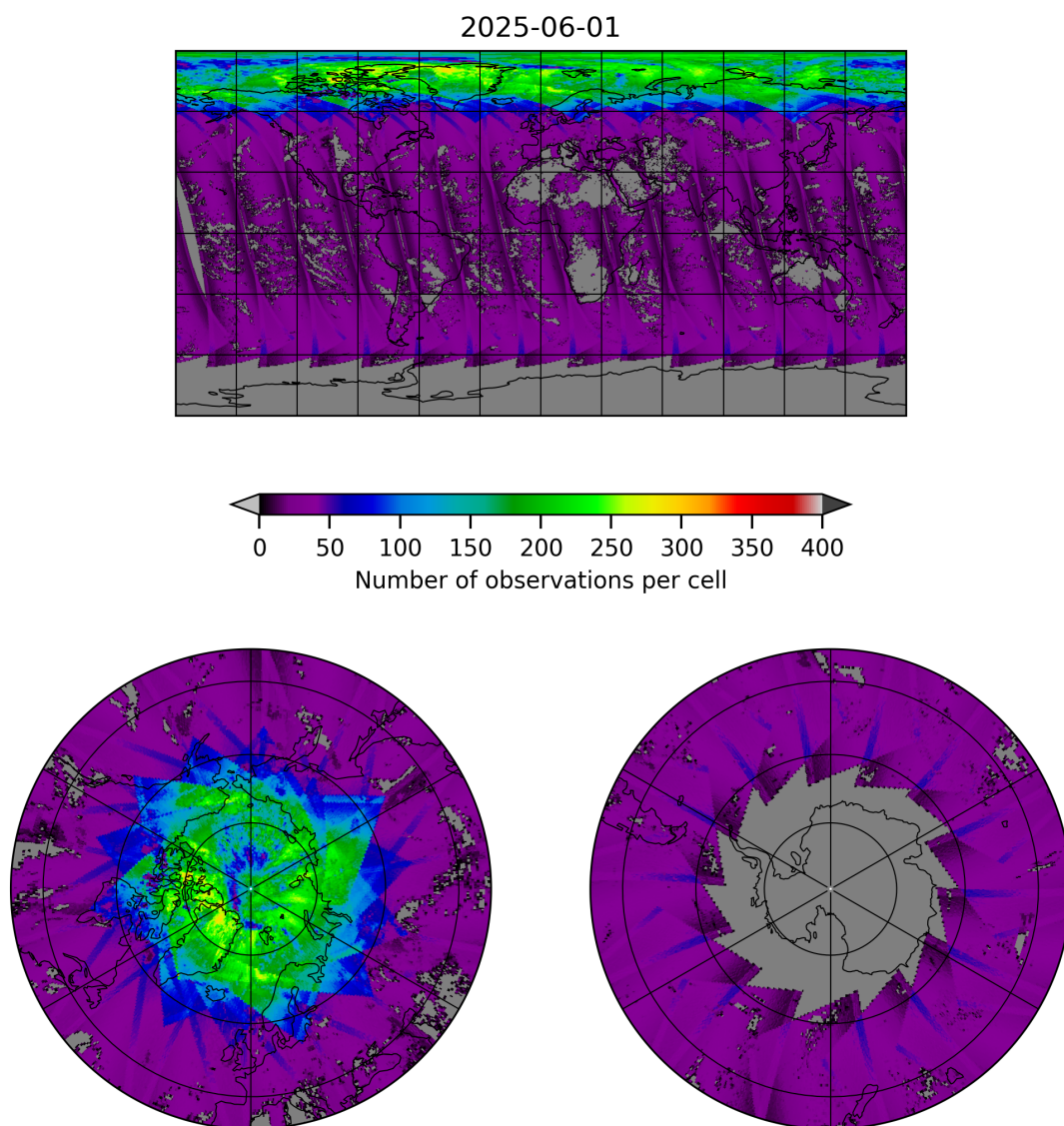
Figure 19: Map of the number of observations for 2025-06-01 to 2025-06-02
