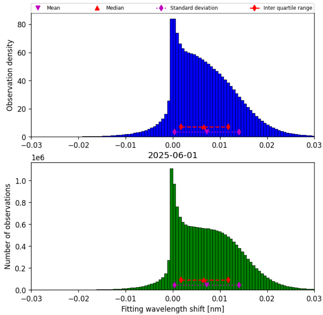
Figure 47: Histogram of “Fitting wavelength shift” for 2025-06-01 to 2025-06-02
