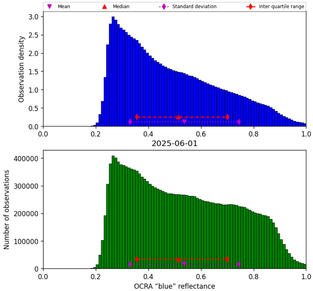
Figure 49: Histogram of “OCRA “blue” reflectance” for 2025-06-01 to 2025-06-02
