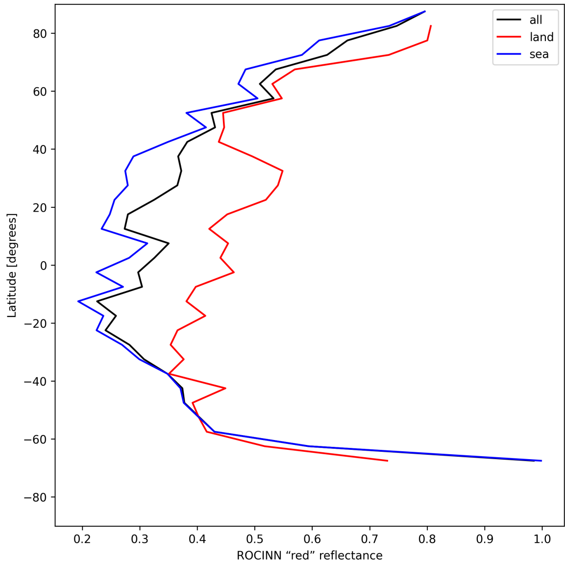
Figure 35: Zonal average of “ROCINN “red” reflectance” for 2025-06-01 to 2025-06-02.
