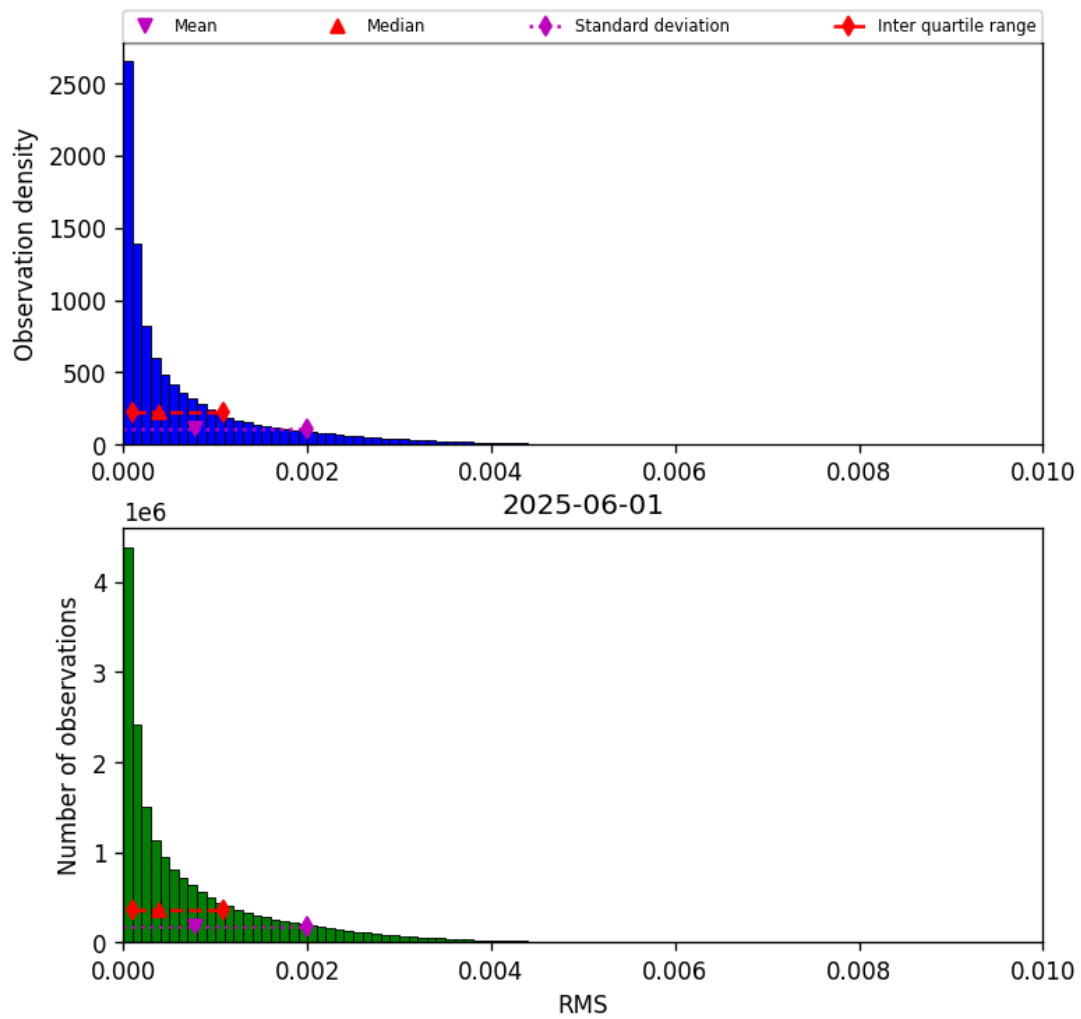
Figure 45: Histogram of “RMS” for 2025-06-01 to 2025-06-02
