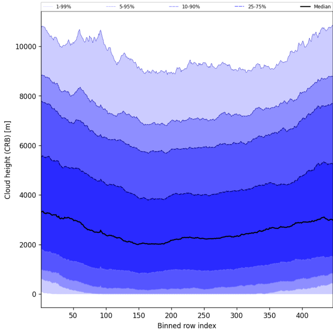
Figure 57: Along track statistics of “Cloud height (CRB)” for 2025-06-01 to 2025-06-02
