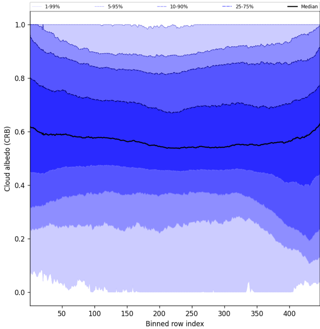
Figure 58: Along track statistics of “Cloud albedo (CRB)” for 2025-06-01 to 2025-06-02
