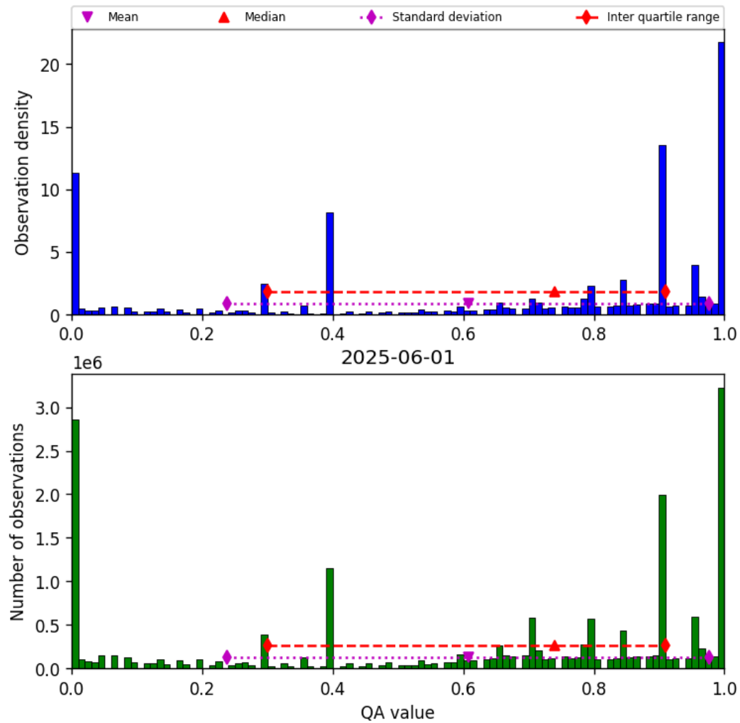
Figure 36: Histogram of “QA value” for 2025-06-01 to 2025-06-02
