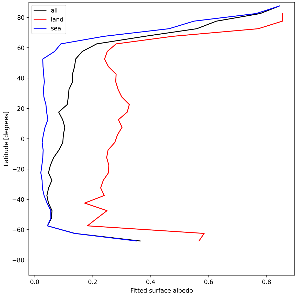
Figure 27: Zonal average of “Fitted surface albedo” for 2025-06-01 to 2025-06-02.
