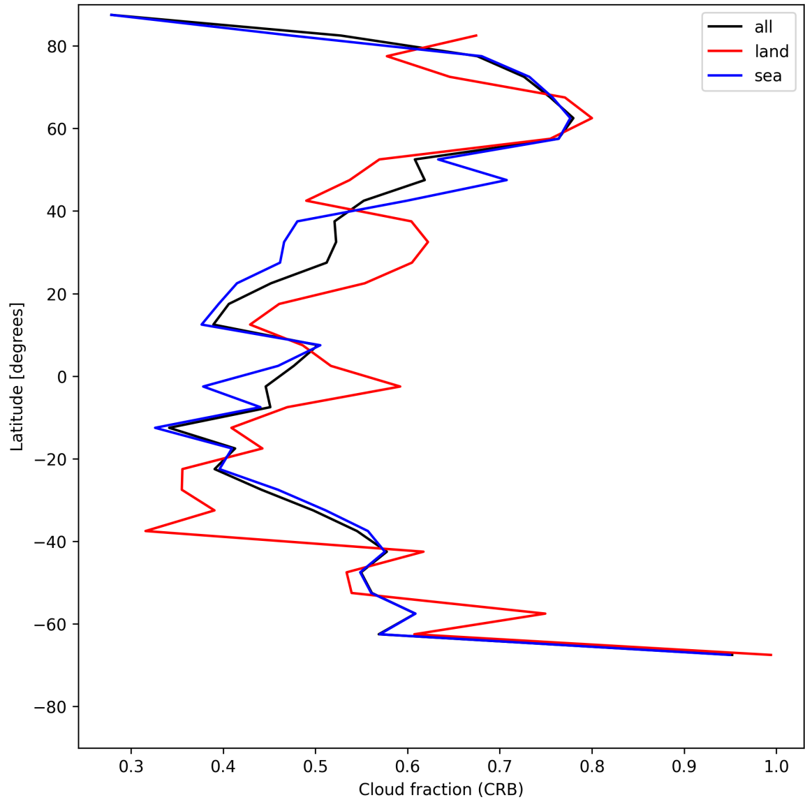
Figure 24: Zonal average of “Cloud fraction (CRB)” for 2025-06-01 to 2025-06-02.
