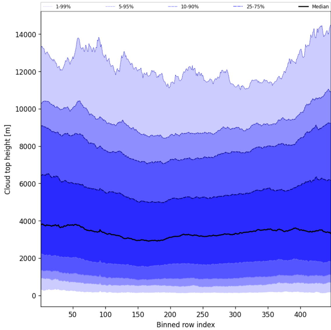
Figure 54: Along track statistics of “Cloud top height” for 2025-06-01 to 2025-06-02
