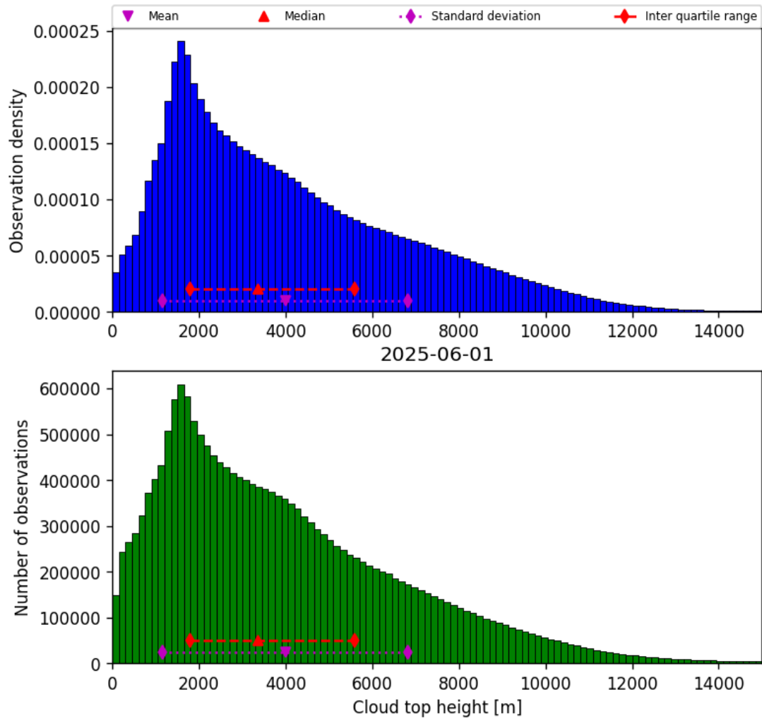
Figure 38: Histogram of “Cloud top height” for 2025-06-01 to 2025-06-02
