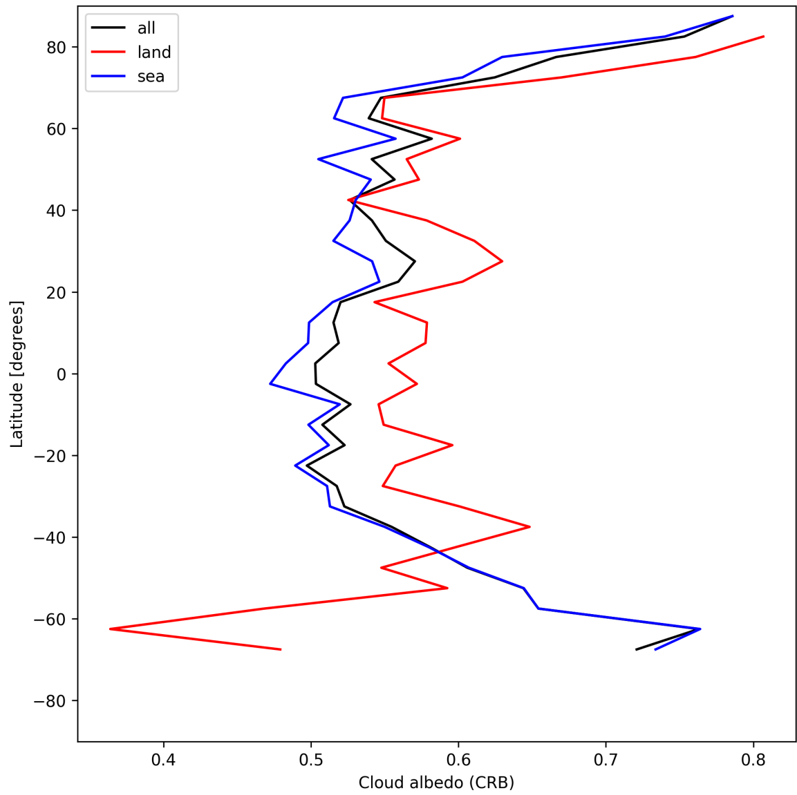
Figure 26: Zonal average of “Cloud albedo (CRB)” for 2025-06-01 to 2025-06-02.
