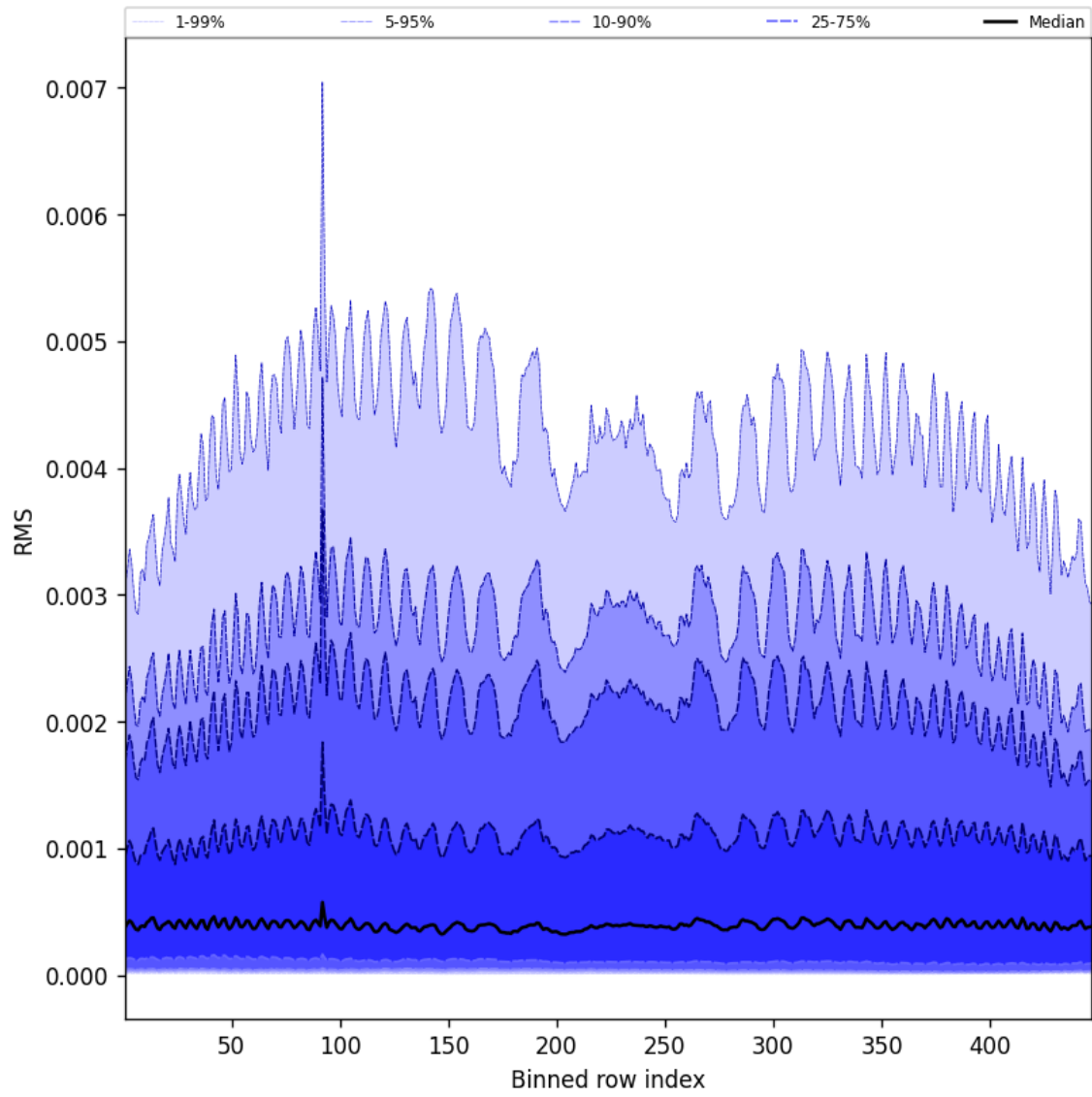
Figure 61: Along track statistics of “RMS” for 2025-06-01 to 2025-06-02
