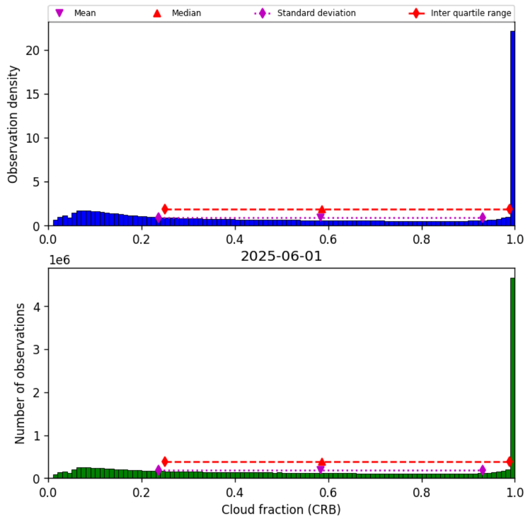
Figure 40: Histogram of “Cloud fraction (CRB)” for 2025-06-01 to 2025-06-02
