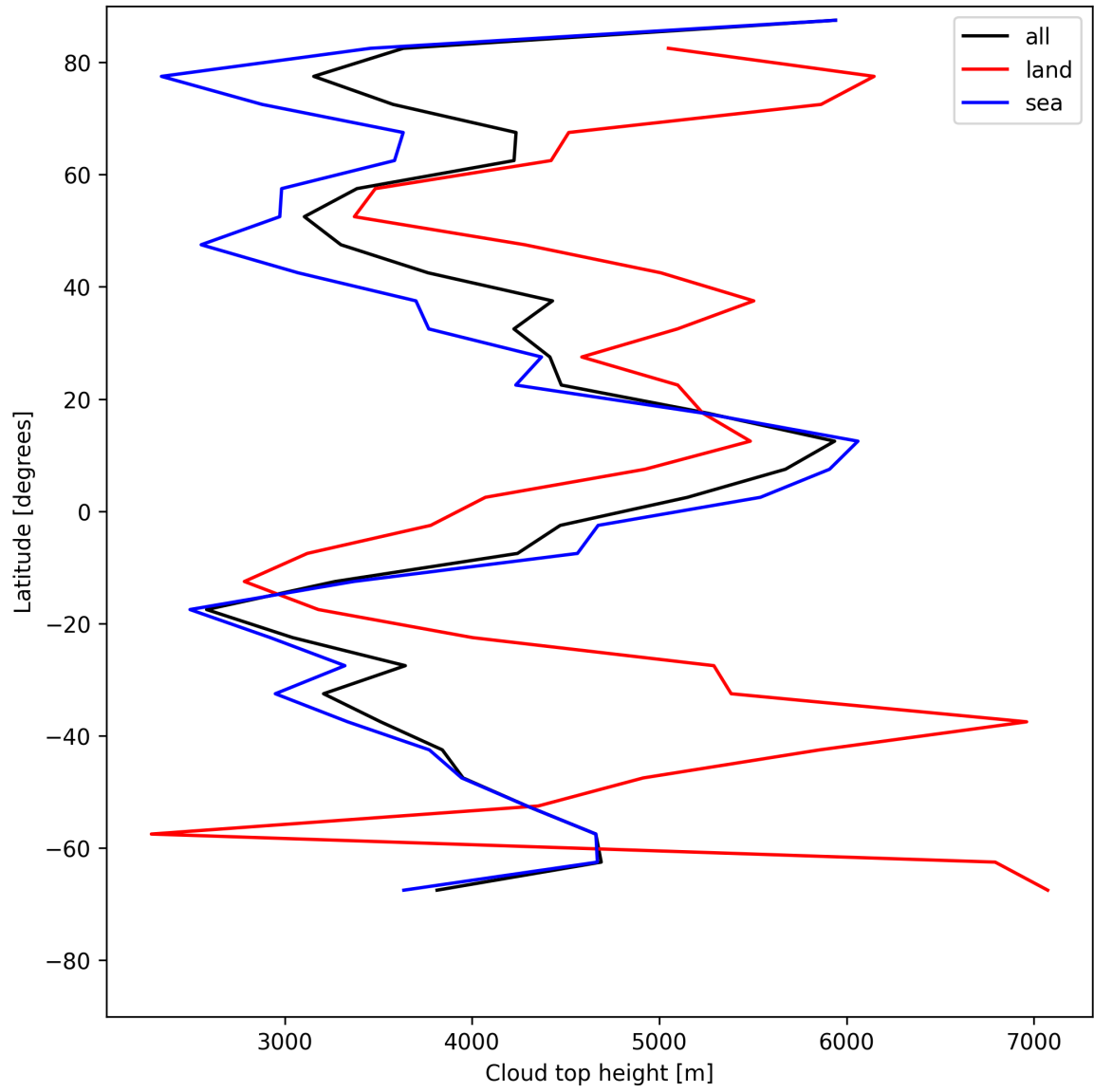
Figure 22: Zonal average of “Cloud top height” for 2025-06-01 to 2025-06-02.
