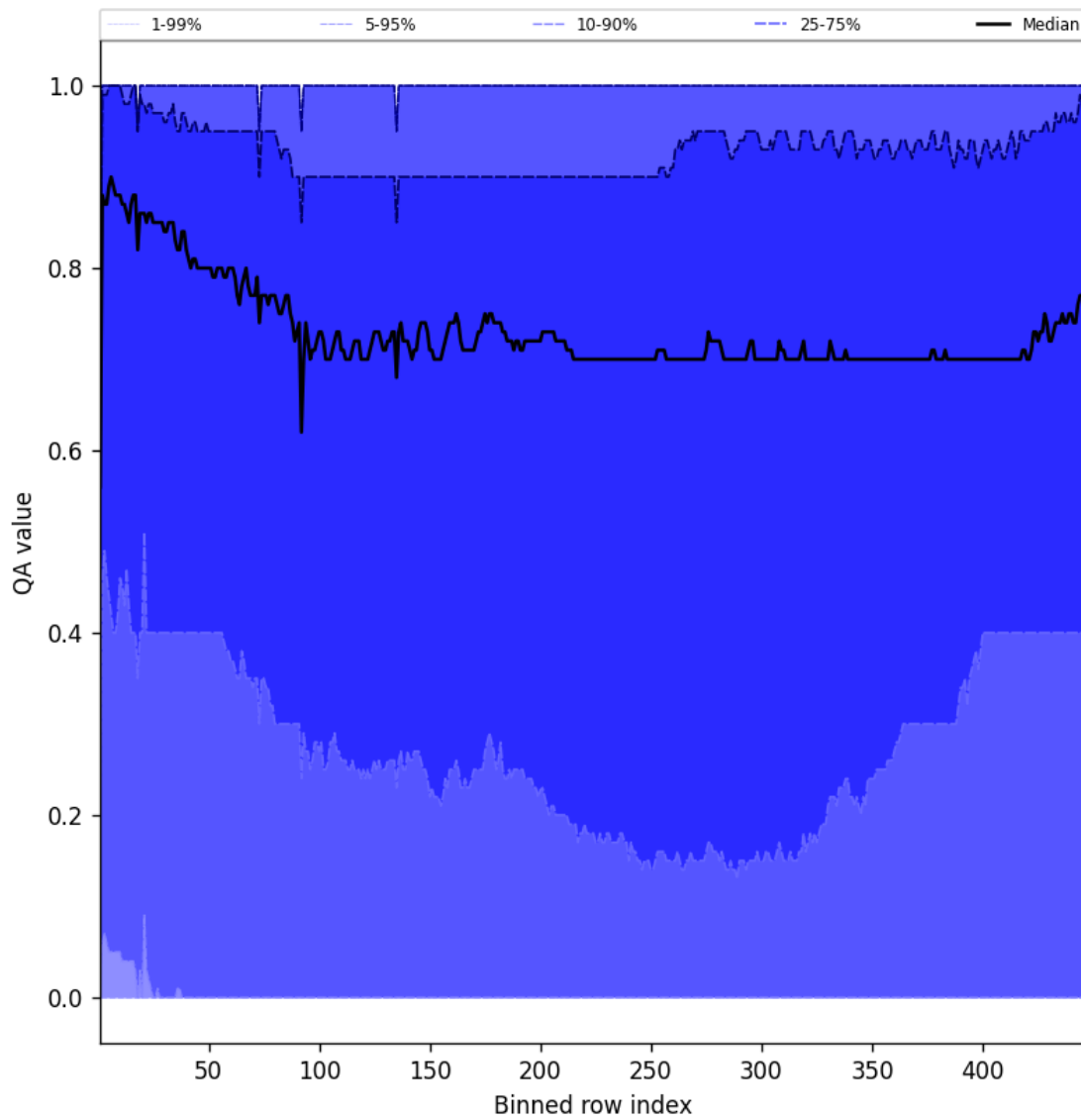
Figure 52: Along track statistics of “QA value” for 2025-06-01 to 2025-06-02
