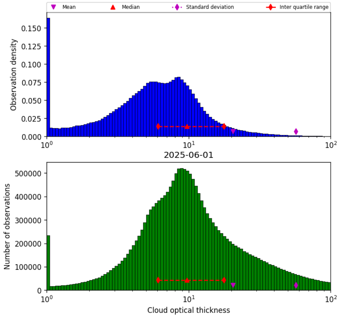
Figure 39: Histogram of “Cloud optical thickness” for 2025-06-01 to 2025-06-02
