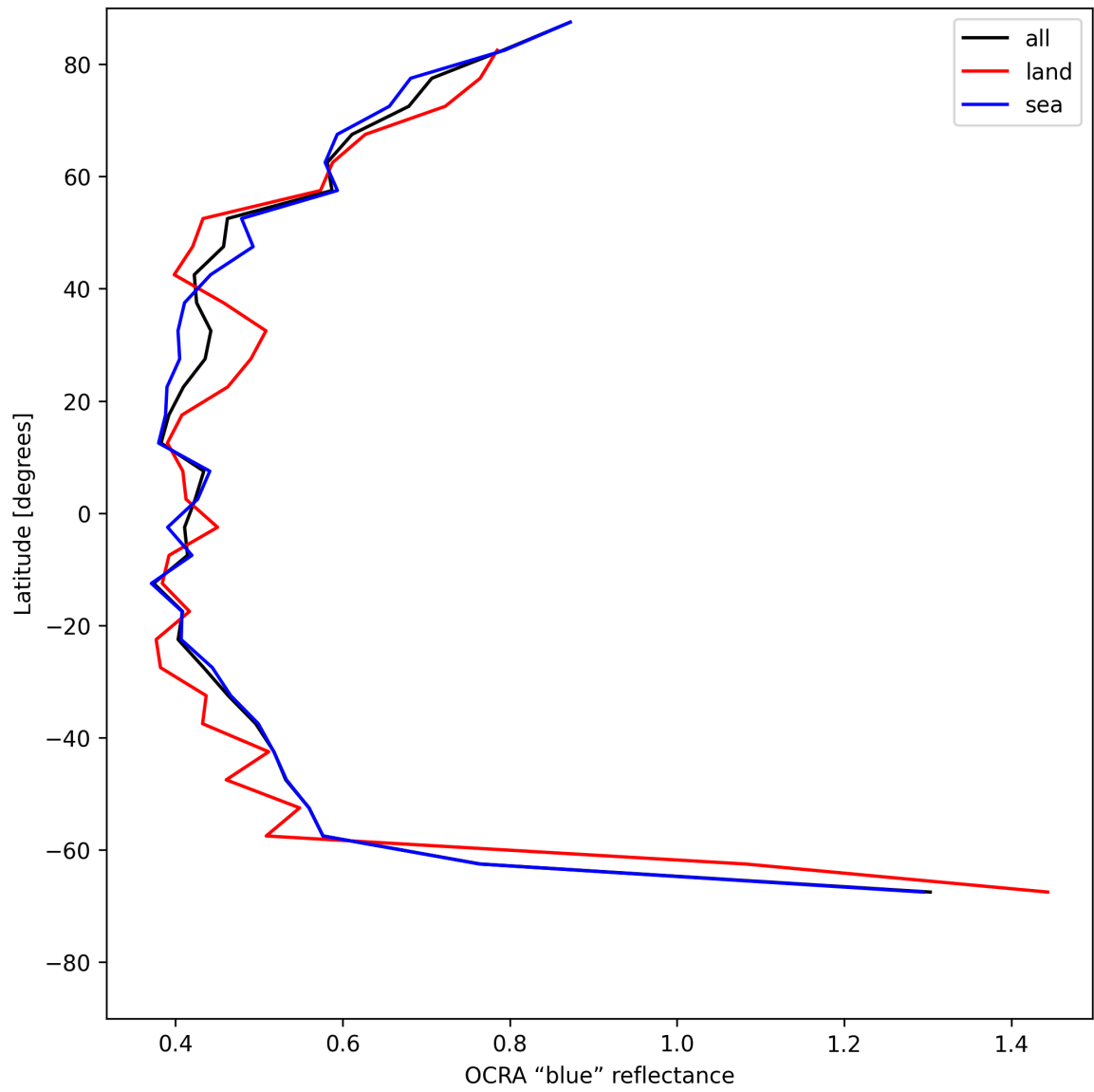
Figure 33: Zonal average of “OCRA “blue” reflectance” for 2025-06-01 to 2025-06-02.
