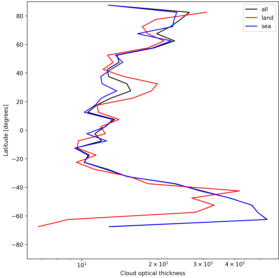
Figure 23: Zonal average of “Cloud optical thickness” for 2025-06-01 to 2025-06-02.
