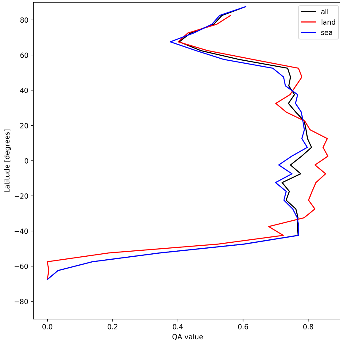
Figure 20: Zonal average of “QA value” for 2025-06-01 to 2025-06-02.
