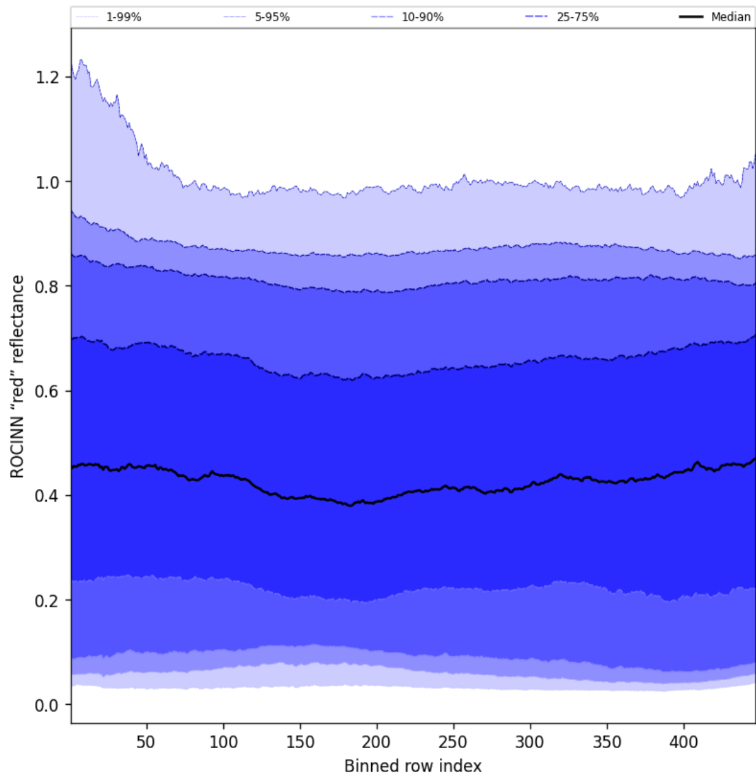
Figure 67: Along track statistics of "ROCINN "red" reflectance" for 2025-06-01 to 2025-06-02
