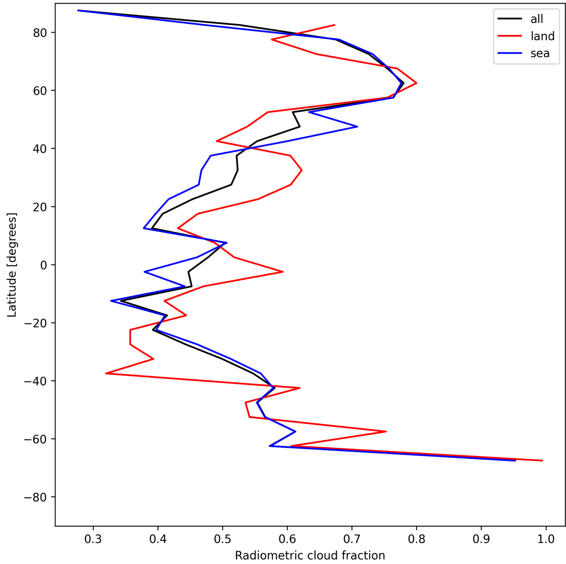
Figure 21: Zonal average of “Radiometric cloud fraction” for 2025-06-01 to 2025-06-02.
