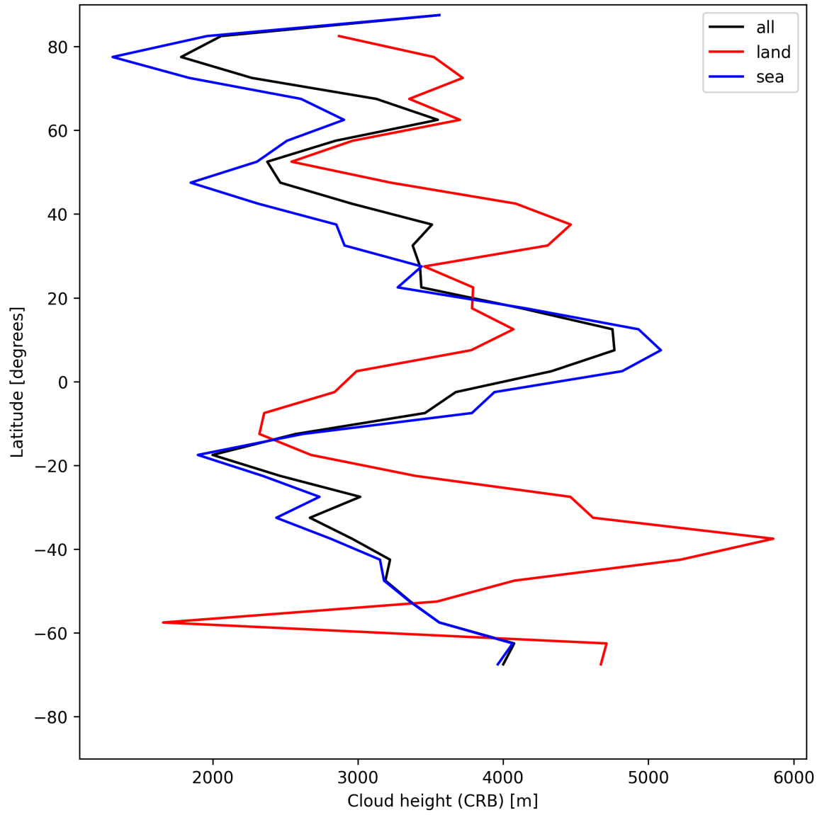
Figure 25: Zonal average of “Cloud height (CRB)” for 2025-06-01 to 2025-06-02.
