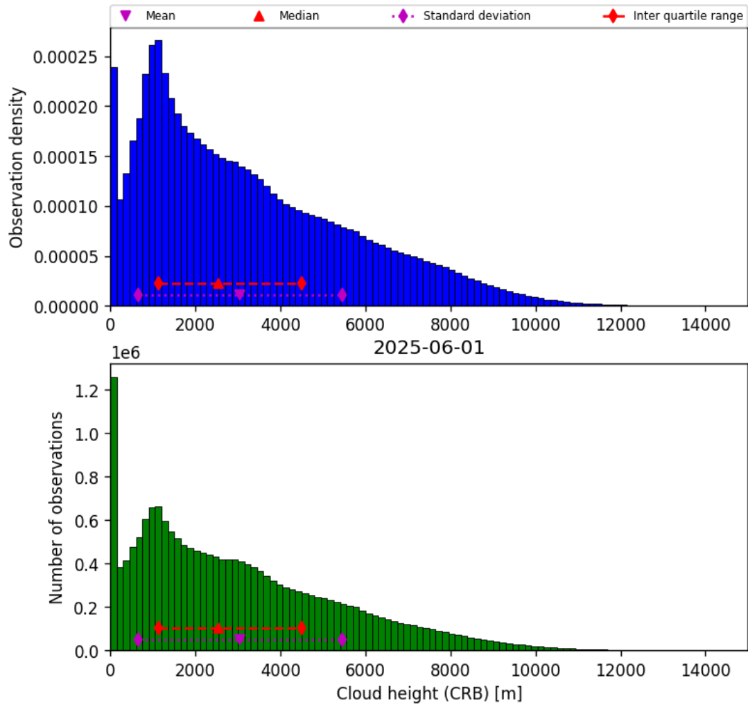
Figure 41: Histogram of “Cloud height (CRB)” for 2025-06-01 to 2025-06-02
