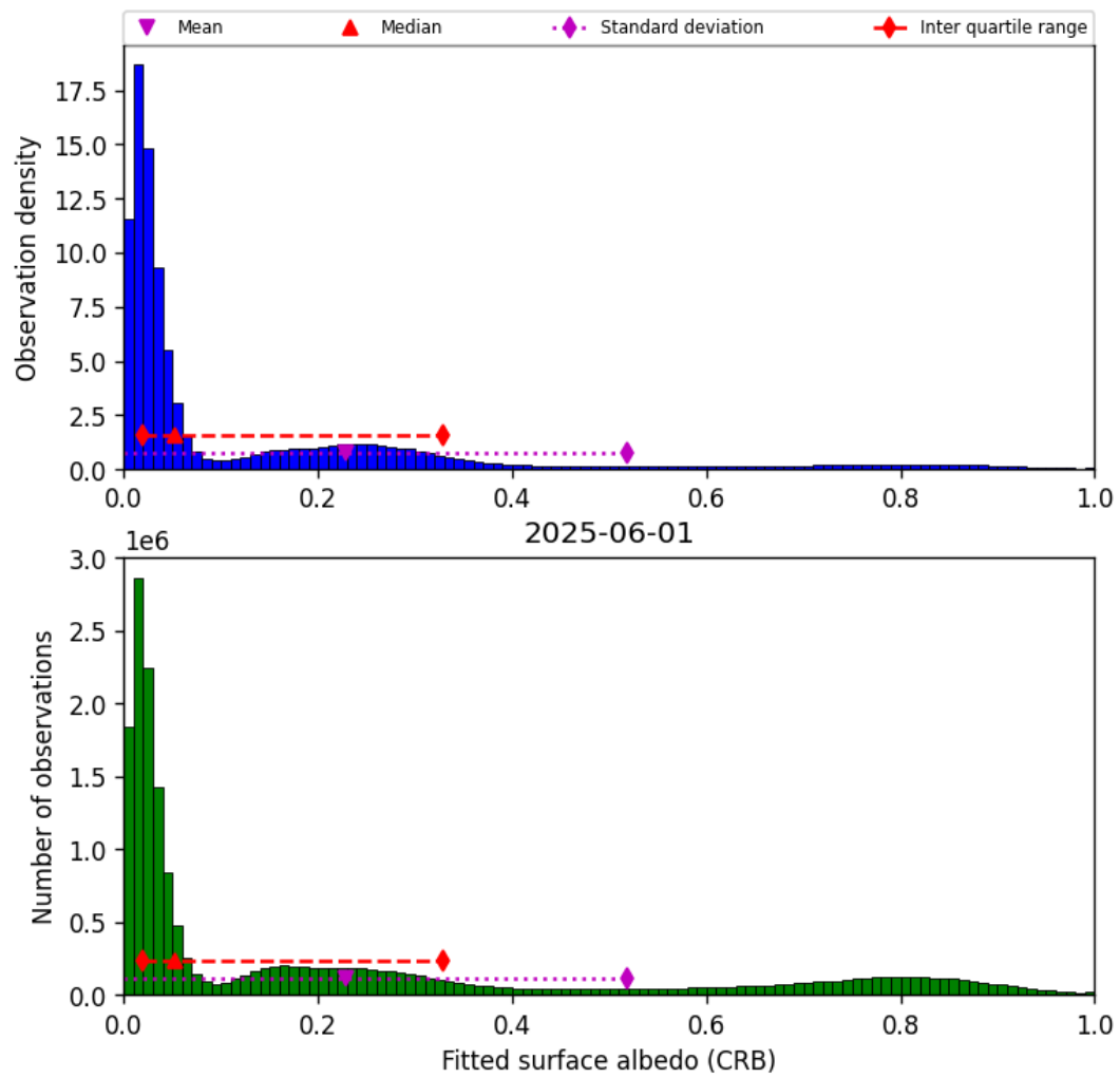
Figure 44: Histogram of “Fitted surface albedo (CRB)” for 2025-06-01 to 2025-06-02
