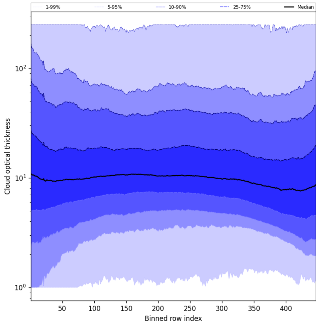
Figure 55: Along track statistics of “Cloud optical thickness” for 2025-06-01 to 2025-06-02
