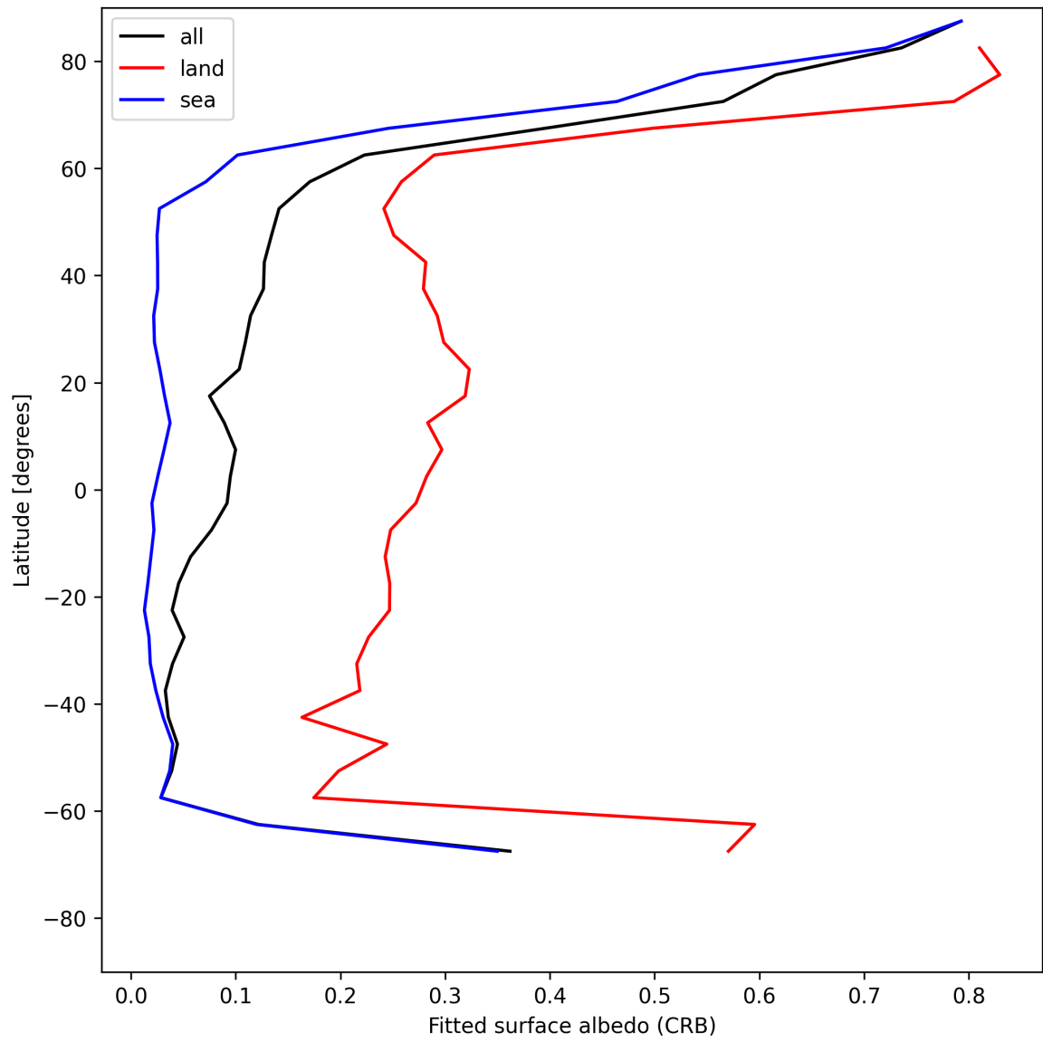
Figure 28: Zonal average of “Fitted surface albedo (CRB)” for 2025-06-01 to 2025-06-02.
