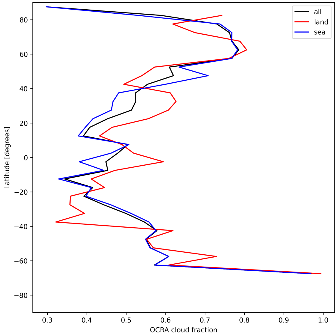
Figure 32: Zonal average of “OCRA cloud fraction” for 2025-06-01 to 2025-06-02.
