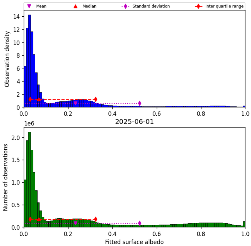
Figure 43: Histogram of “Fitted surface albedo” for 2025-06-01 to 2025-06-02
