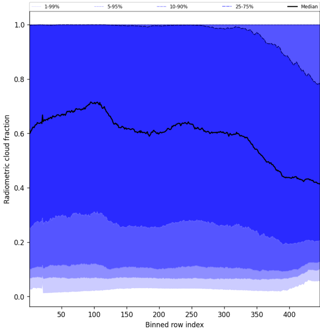
Figure 53: Along track statistics of “Radiometric cloud fraction” for 2025-06-01 to 2025-06-02
