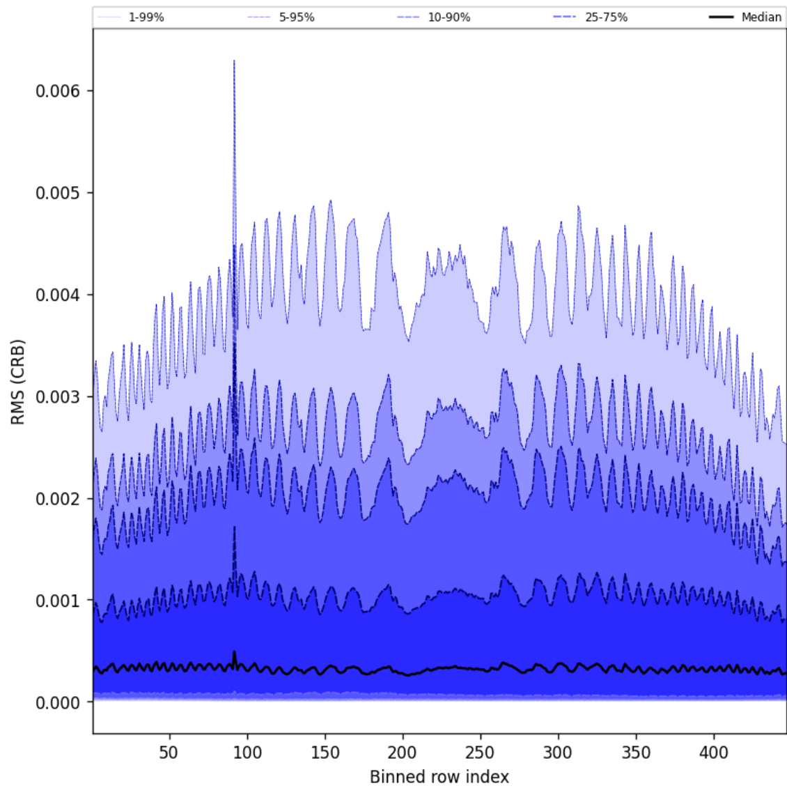
Figure 62: Along track statistics of “RMS (CRB)” for 2025-06-01 to 2025-06-02
