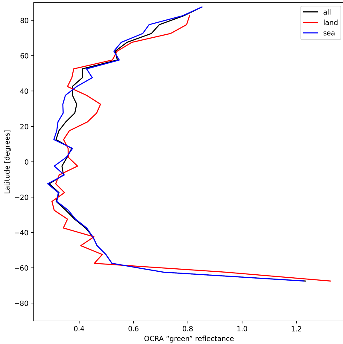
Figure 34: Zonal average of “OCRA “green” reflectance” for 2025-06-01 to 2025-06-02.
