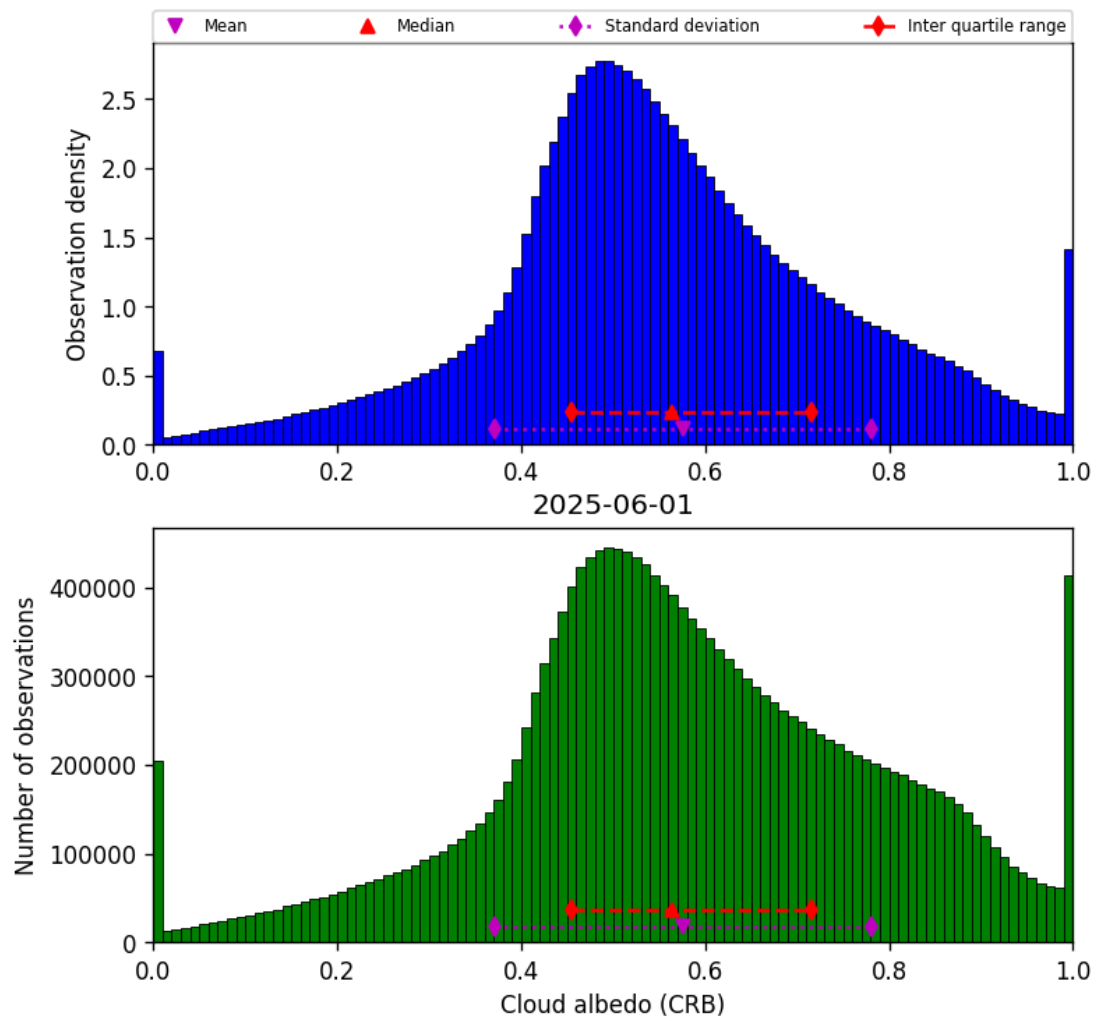
Figure 42: Histogram of “Cloud albedo (CRB)” for 2025-06-01 to 2025-06-02
