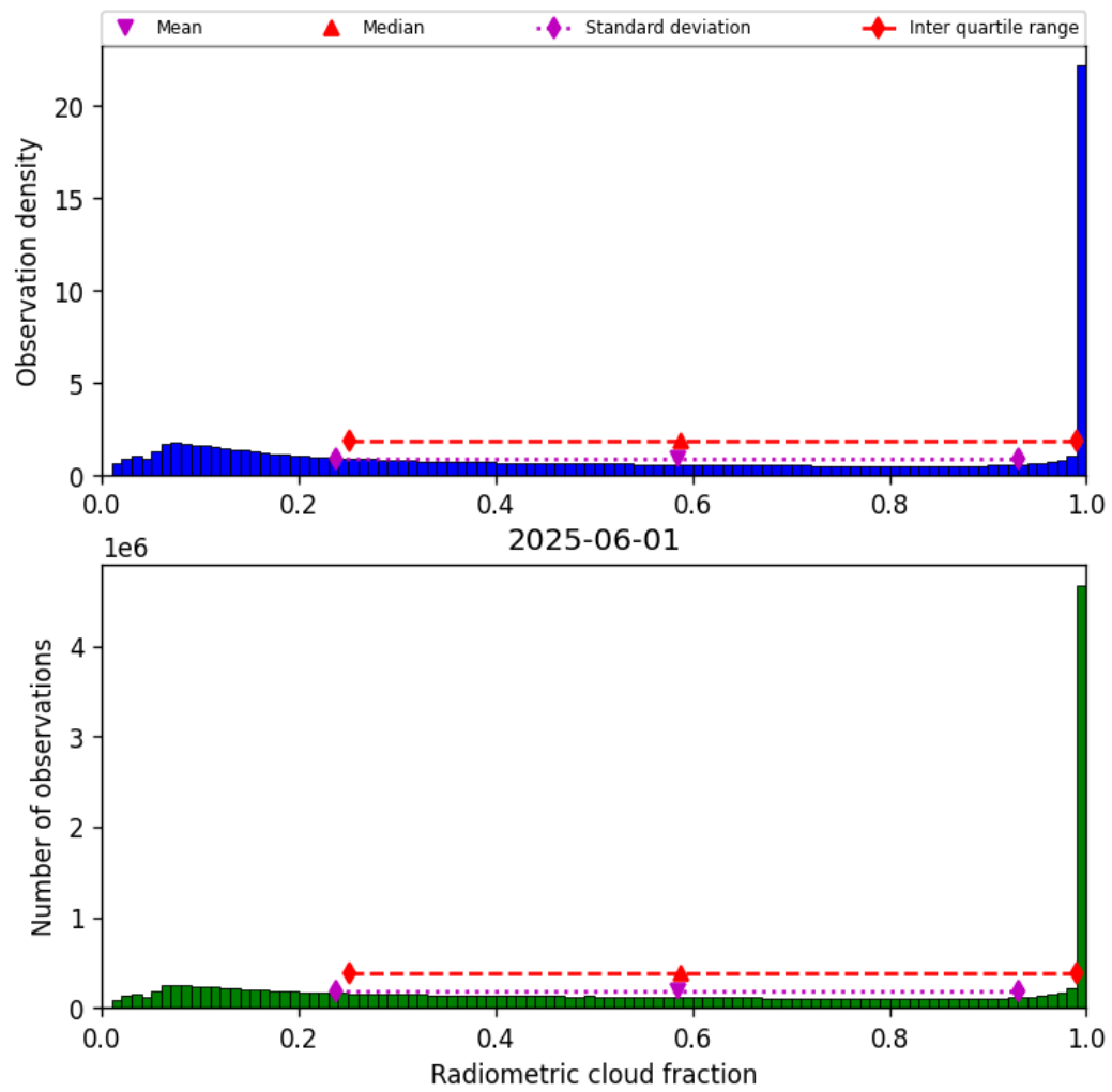
Figure 37: Histogram of “Radiometric cloud fraction” for 2025-06-01 to 2025-06-02
