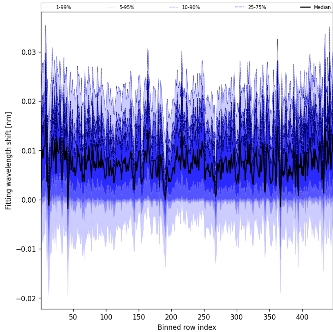
Figure 63: Along track statistics of “Fitting wavelength shift” for 2025-06-01 to 2025-06-02
