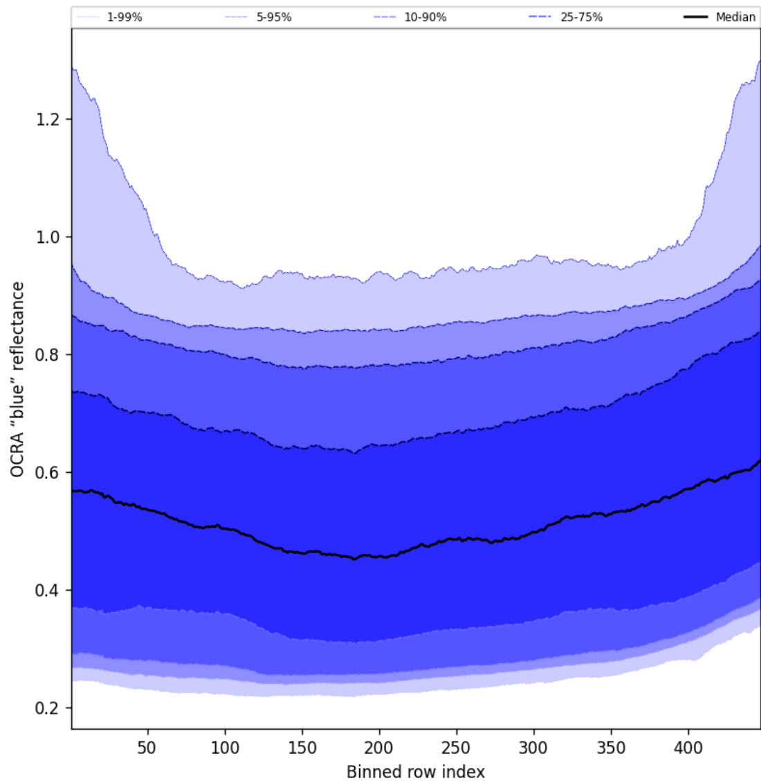
Figure 65: Along track statistics of “OCRA “blue” reflectance” for 2025-06-01 to 2025-06-02
