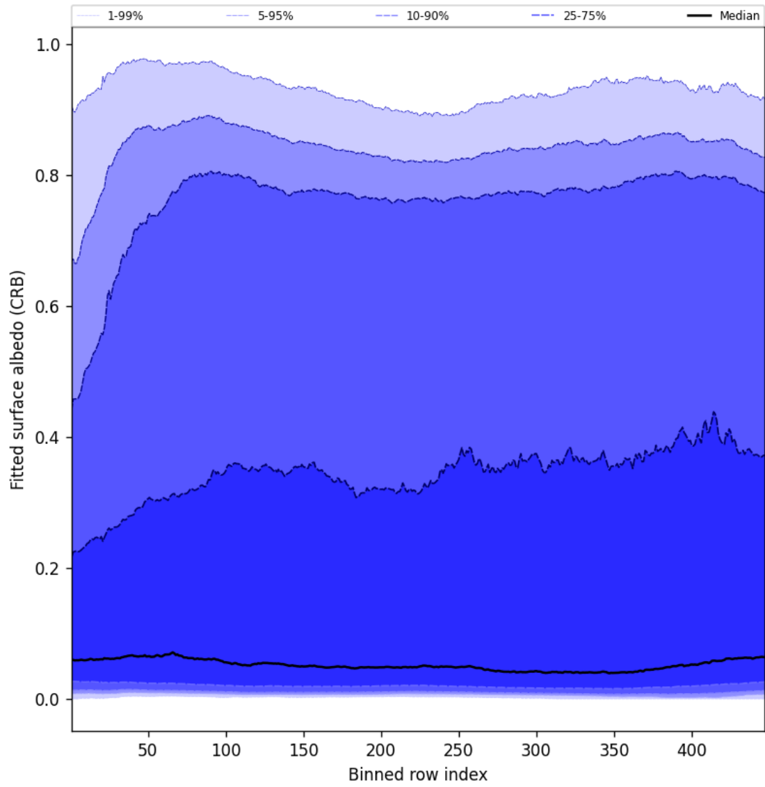
Figure 60: Along track statistics of “Fitted surface albedo (CRB)” for 2025-06-01 to 2025-06-02
