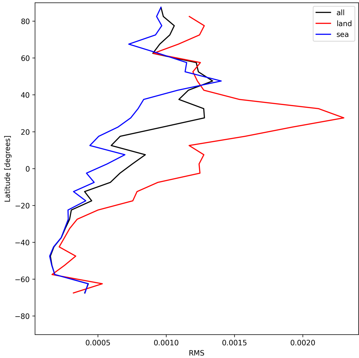
Figure 29: Zonal average of “RMS” for 2025-06-01 to 2025-06-02.
