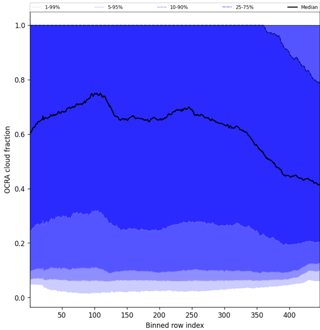
Figure 64: Along track statistics of “OCRA cloud fraction” for 2025-06-01 to 2025-06-02
