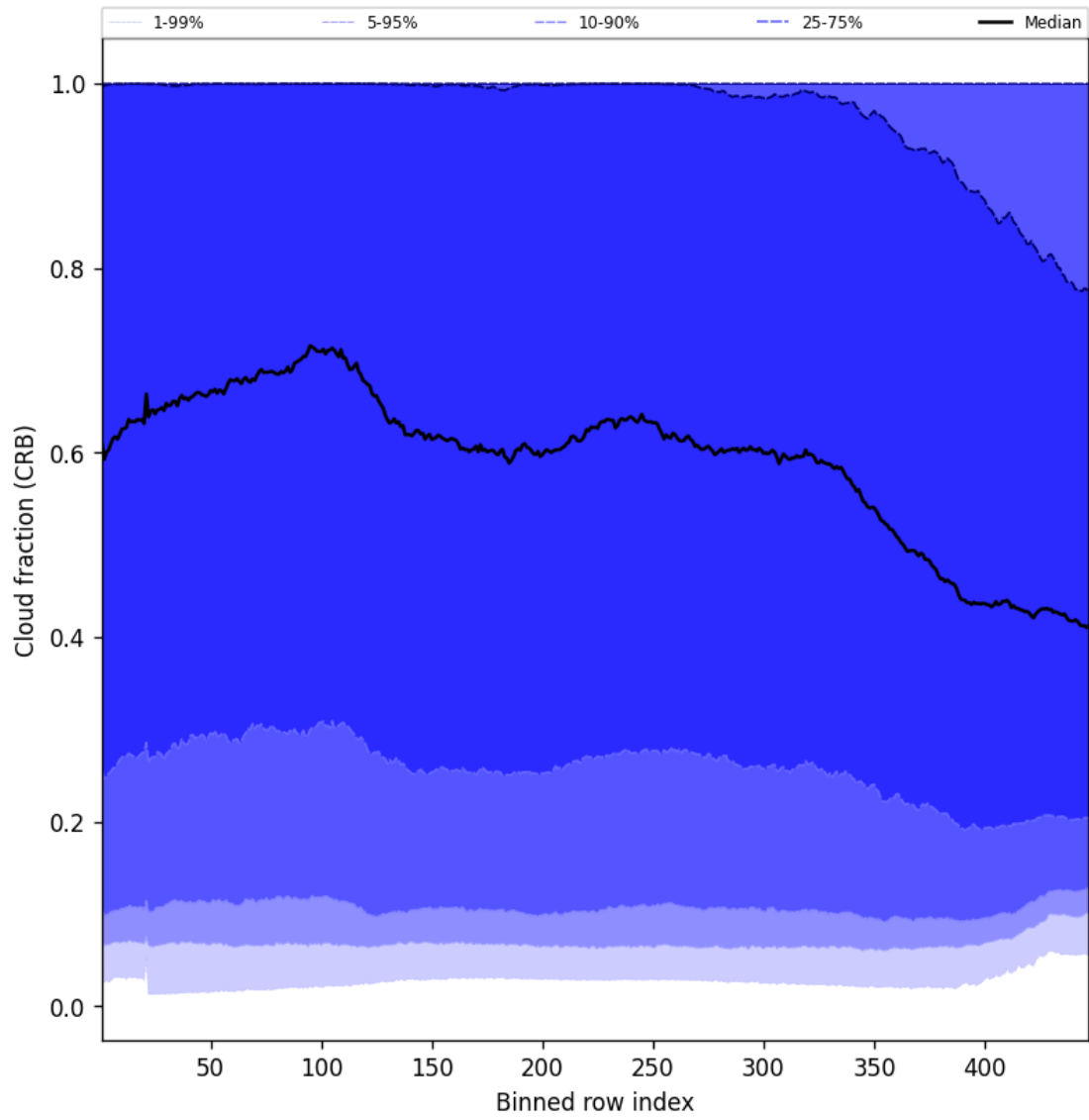
Figure 56: Along track statistics of “Cloud fraction (CRB)” for 2025-06-01 to 2025-06-02
