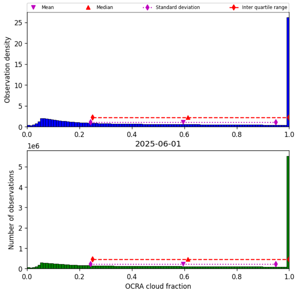
Figure 48: Histogram of “OCRA cloud fraction” for 2025-06-01 to 2025-06-02
