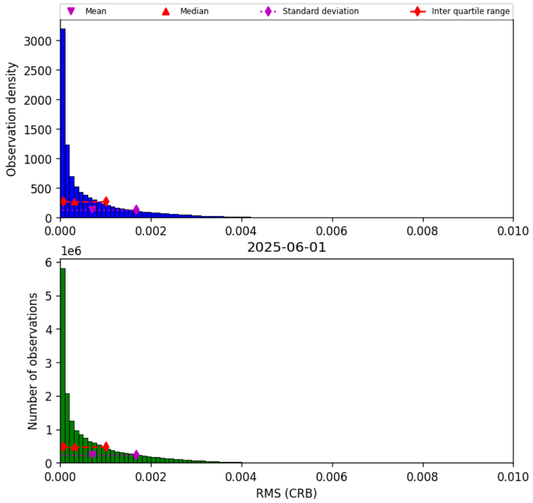
Figure 46: Histogram of “RMS (CRB)” for 2025-06-01 to 2025-06-02
