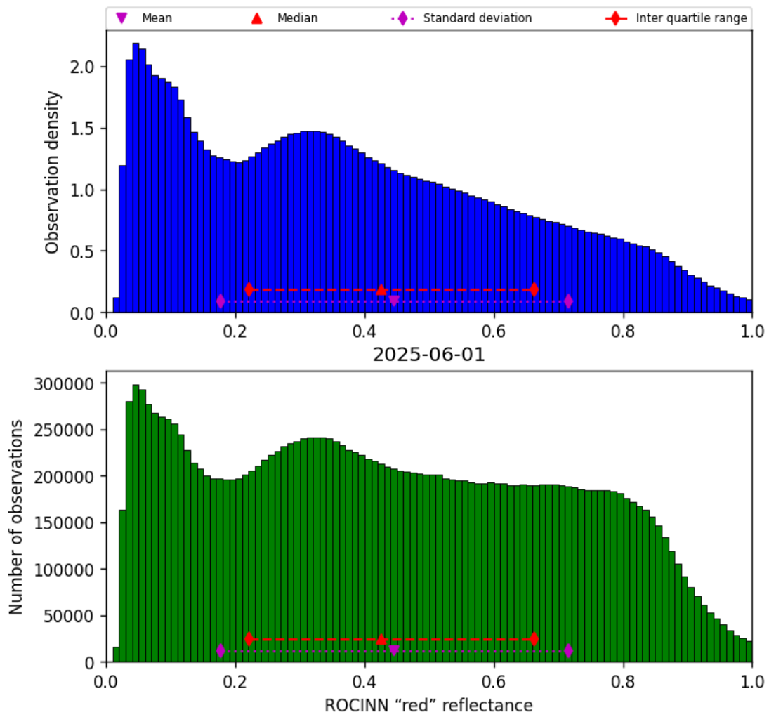
Figure 51: Histogram of “ROCINN “red” reflectance” for 2025-06-01 to 2025-06-02
