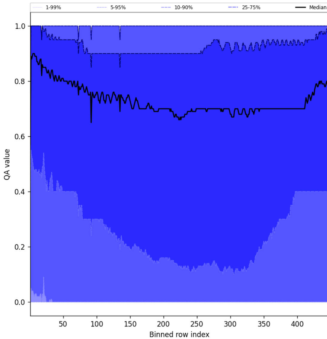
Figure 52: Along track statistics of “QA value” for 2025-06-02 to 2025-06-03
