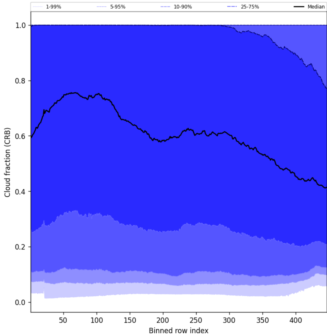
Figure 56: Along track statistics of “Cloud fraction (CRB)” for 2025-06-02 to 2025-06-03
