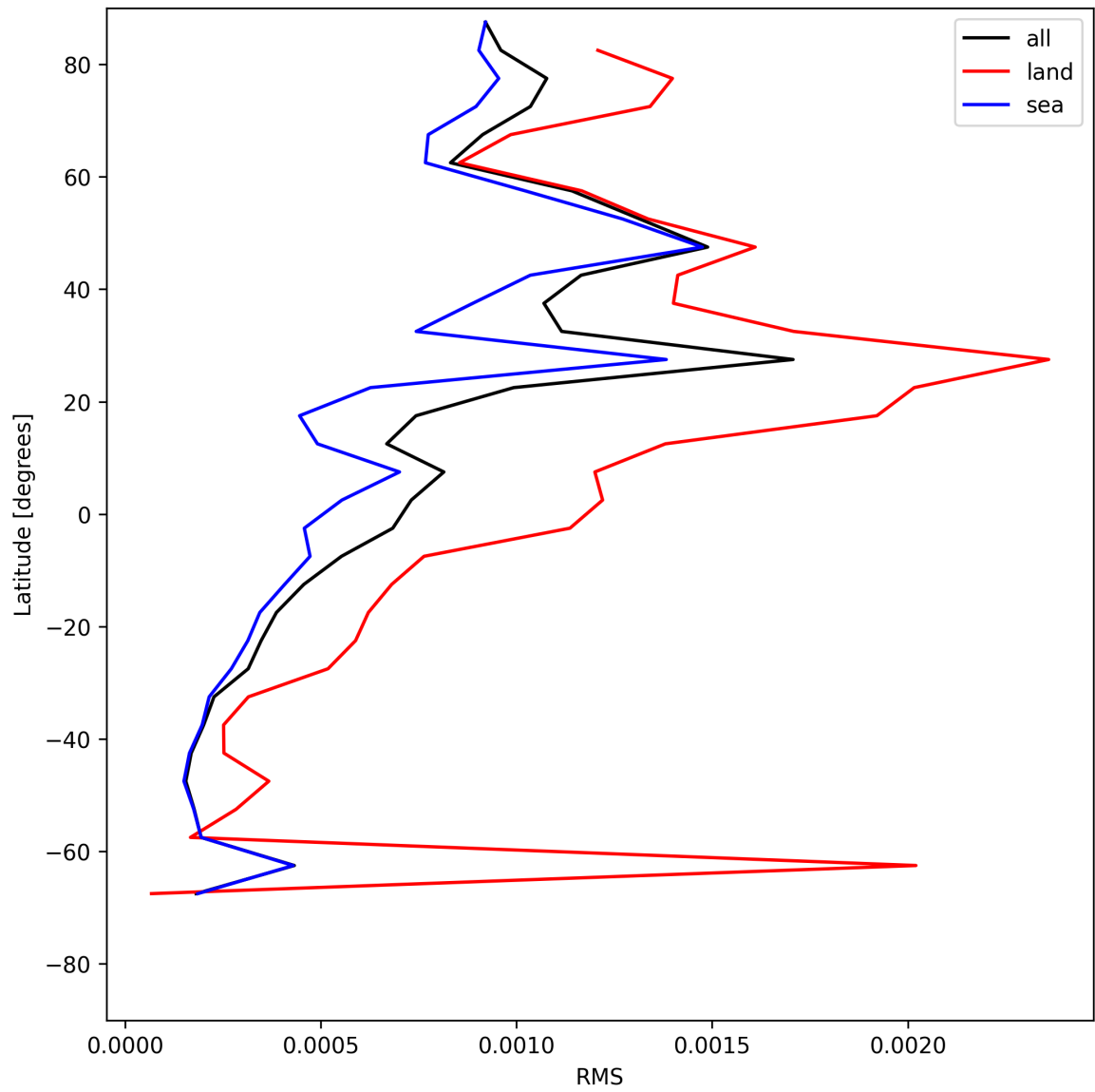
Figure 29: Zonal average of “RMS” for 2025-06-02 to 2025-06-03.
