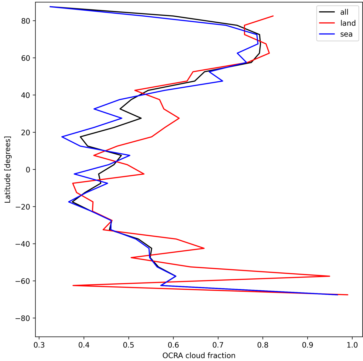
Figure 32: Zonal average of “OCRA cloud fraction” for 2025-06-02 to 2025-06-03.
