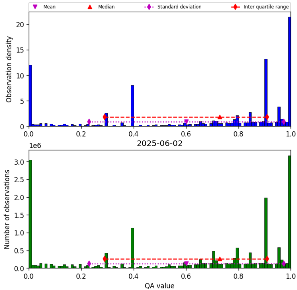
Figure 36: Histogram of “QA value” for 2025-06-02 to 2025-06-03
