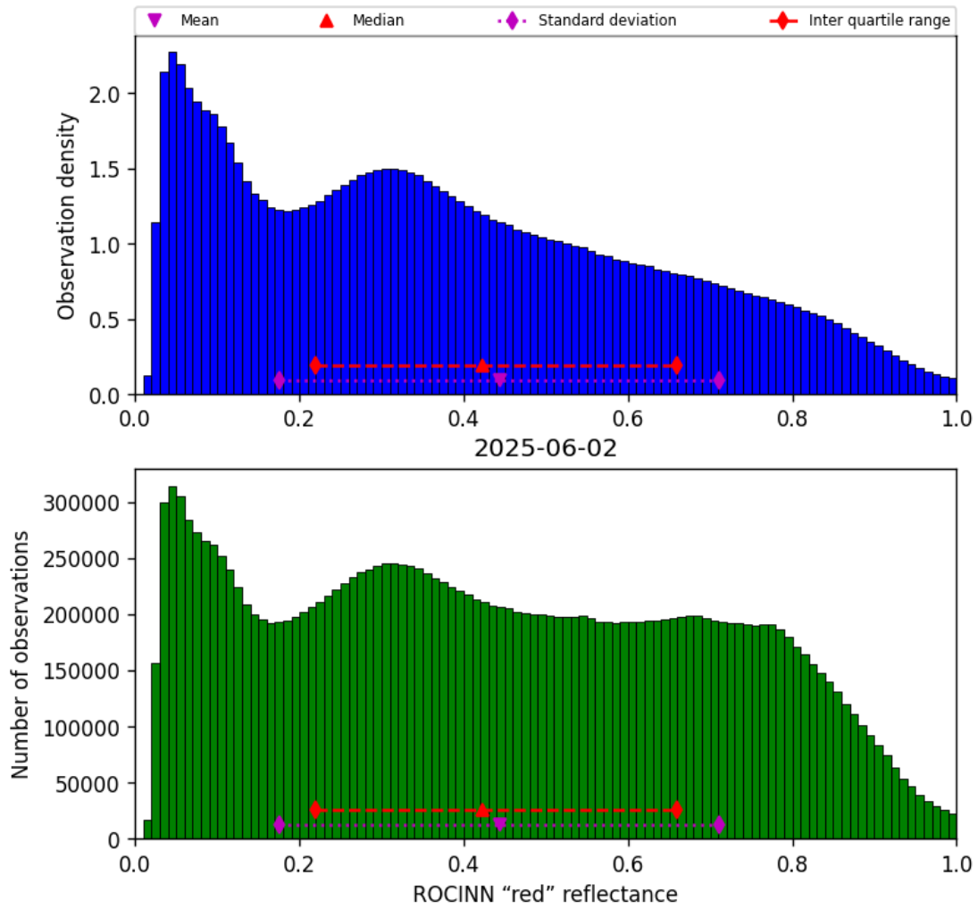
Figure 51: Histogram of “ROCINN “red” reflectance” for 2025-06-02 to 2025-06-03
