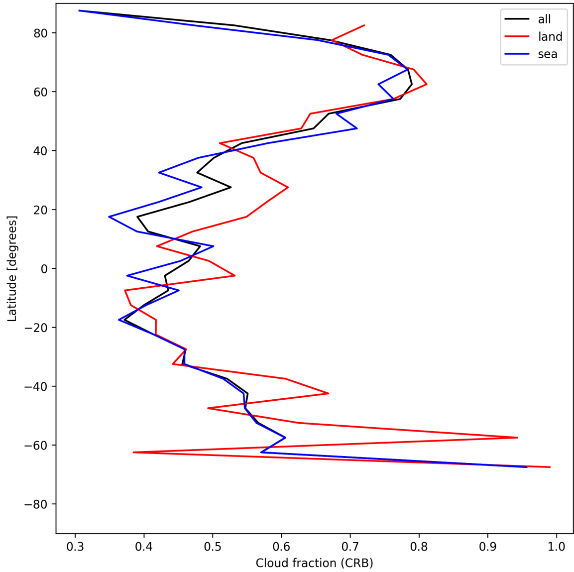
Figure 24: Zonal average of “Cloud fraction (CRB)” for 2025-06-02 to 2025-06-03.
