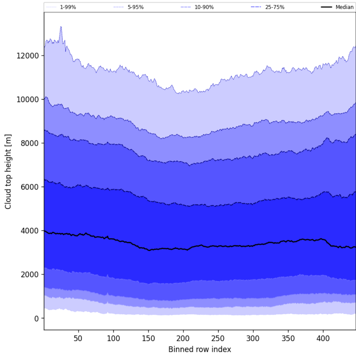
Figure 54: Along track statistics of “Cloud top height” for 2025-06-02 to 2025-06-03
