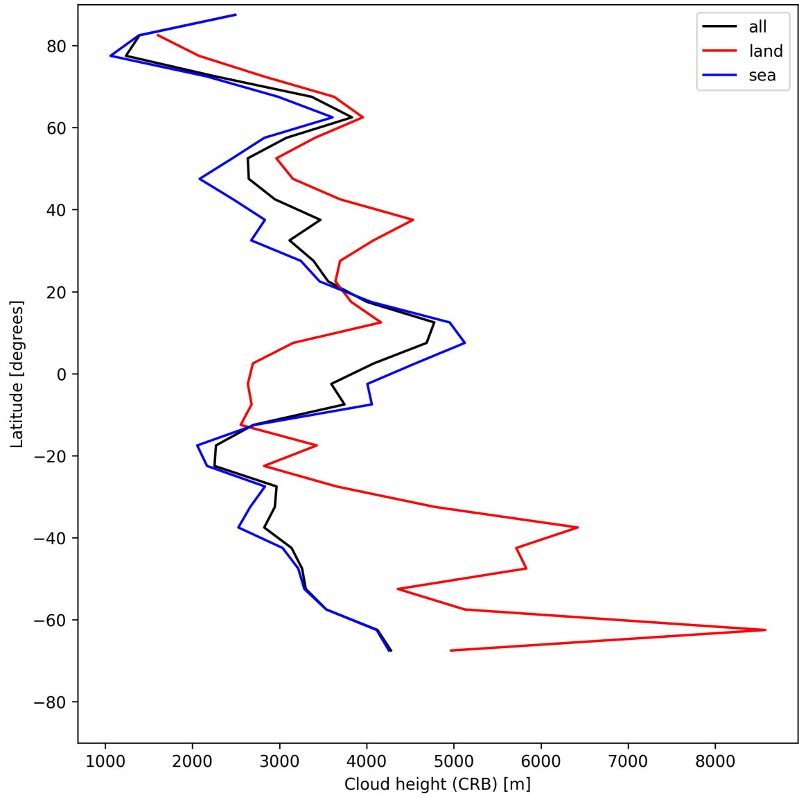
Figure 25: Zonal average of “Cloud height (CRB)” for 2025-06-02 to 2025-06-03.
