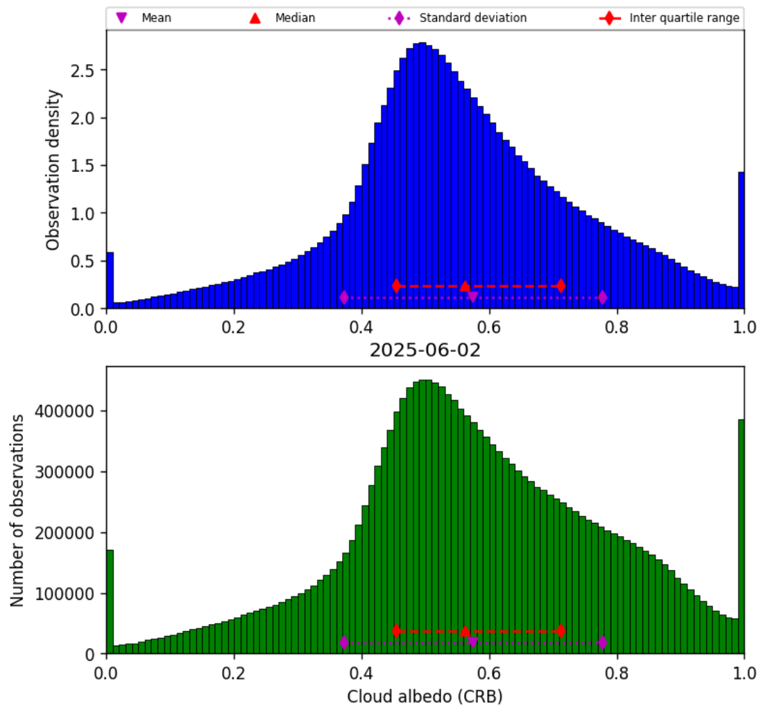
Figure 42: Histogram of “Cloud albedo (CRB)” for 2025-06-02 to 2025-06-03
