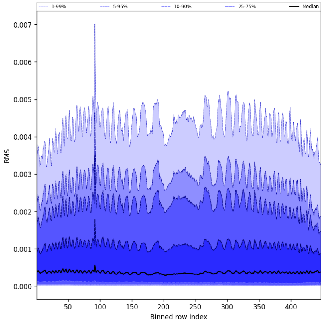
Figure 61: Along track statistics of “RMS” for 2025-06-02 to 2025-06-03
