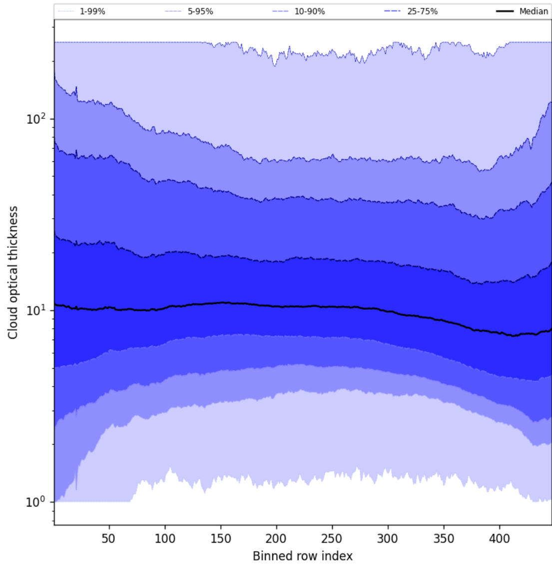
Figure 55: Along track statistics of “Cloud optical thickness” for 2025-06-02 to 2025-06-03
