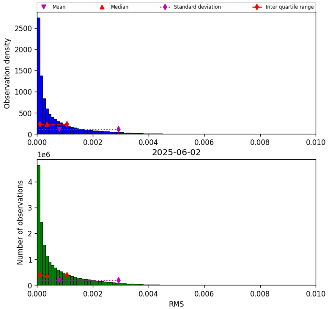
Figure 45: Histogram of “RMS” for 2025-06-02 to 2025-06-03
