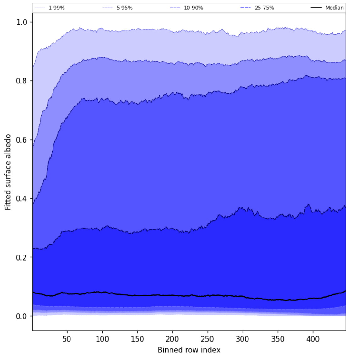
Figure 59: Along track statistics of “Fitted surface albedo” for 2025-06-02 to 2025-06-03
