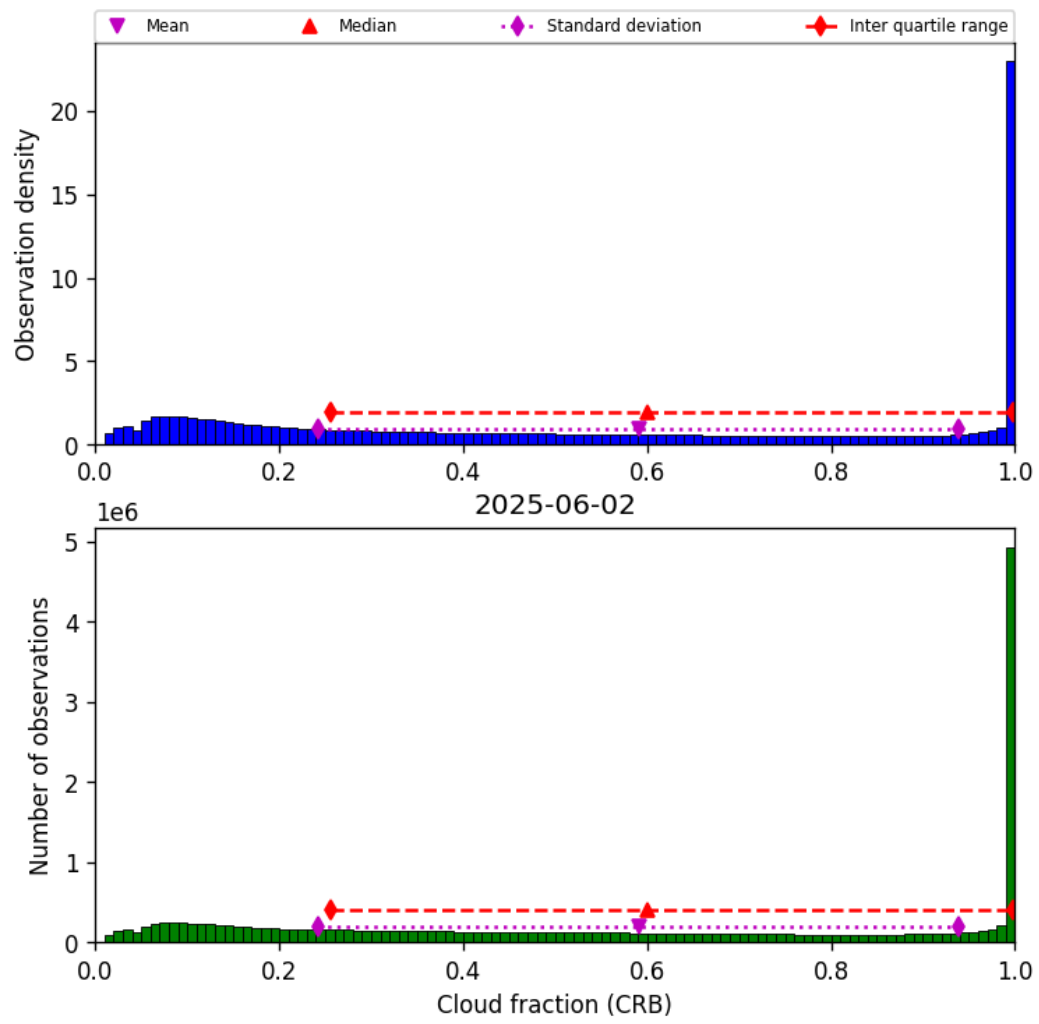
Figure 40: Histogram of “Cloud fraction (CRB)” for 2025-06-02 to 2025-06-03
