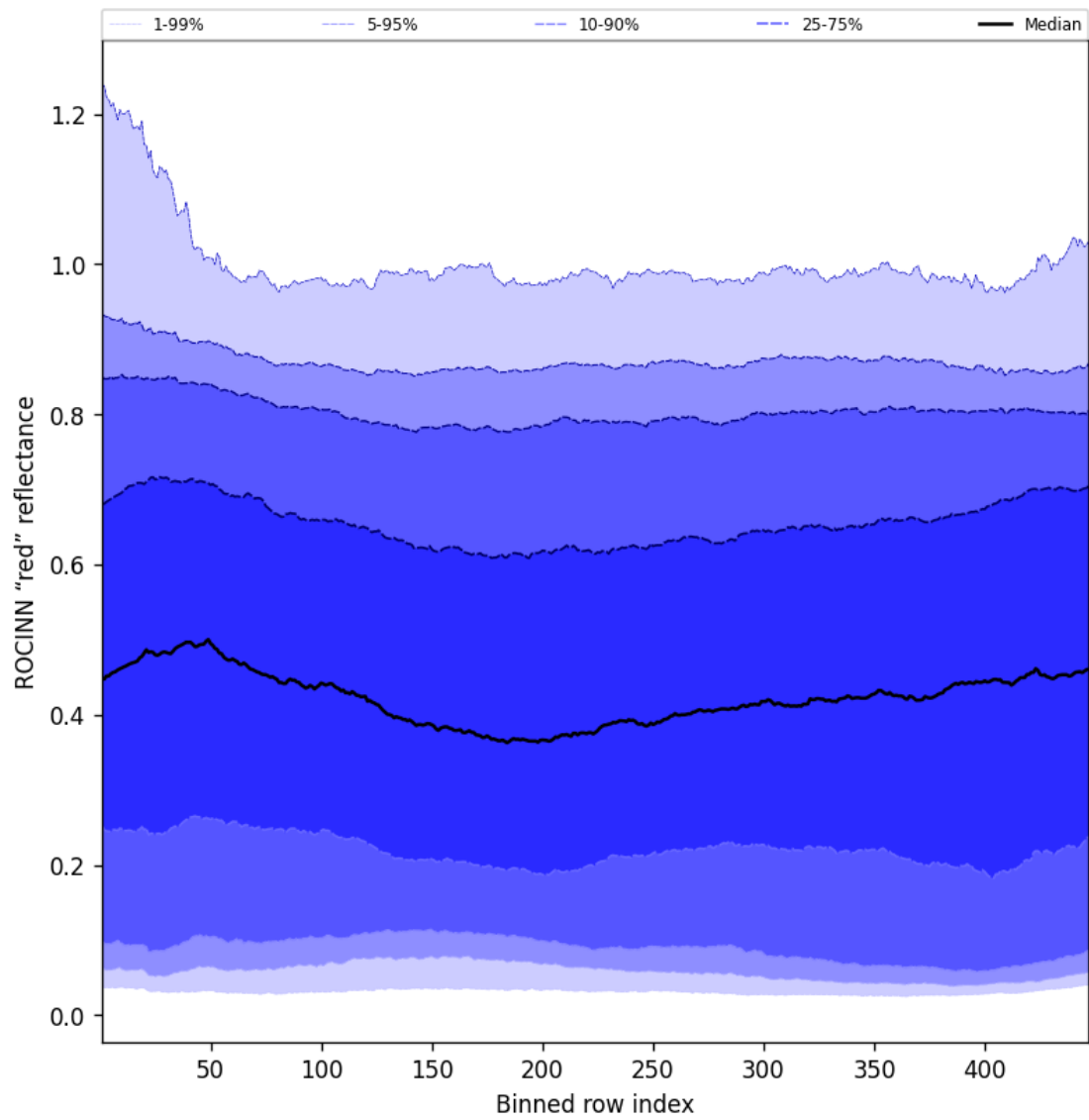
Figure 67: Along track statistics of “ROCINN “red” reflectance” for 2025-06-02 to 2025-06-03
