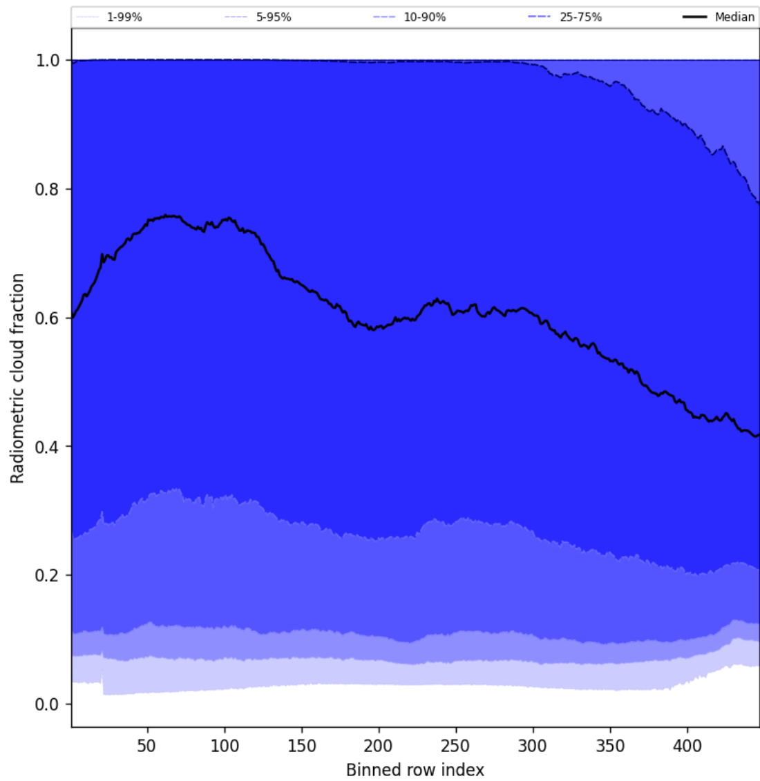
Figure 53: Along track statistics of “Radiometric cloud fraction” for 2025-06-02 to 2025-06-03
