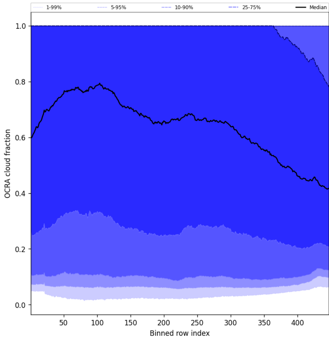
Figure 64: Along track statistics of “OCRA cloud fraction” for 2025-06-02 to 2025-06-03
