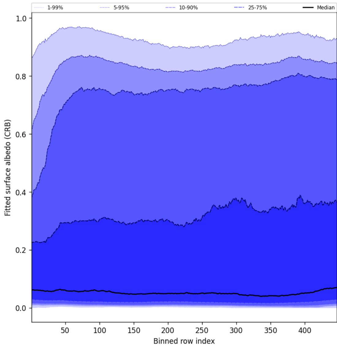
Figure 60: Along track statistics of “Fitted surface albedo (CRB)” for 2025-06-02 to 2025-06-03
