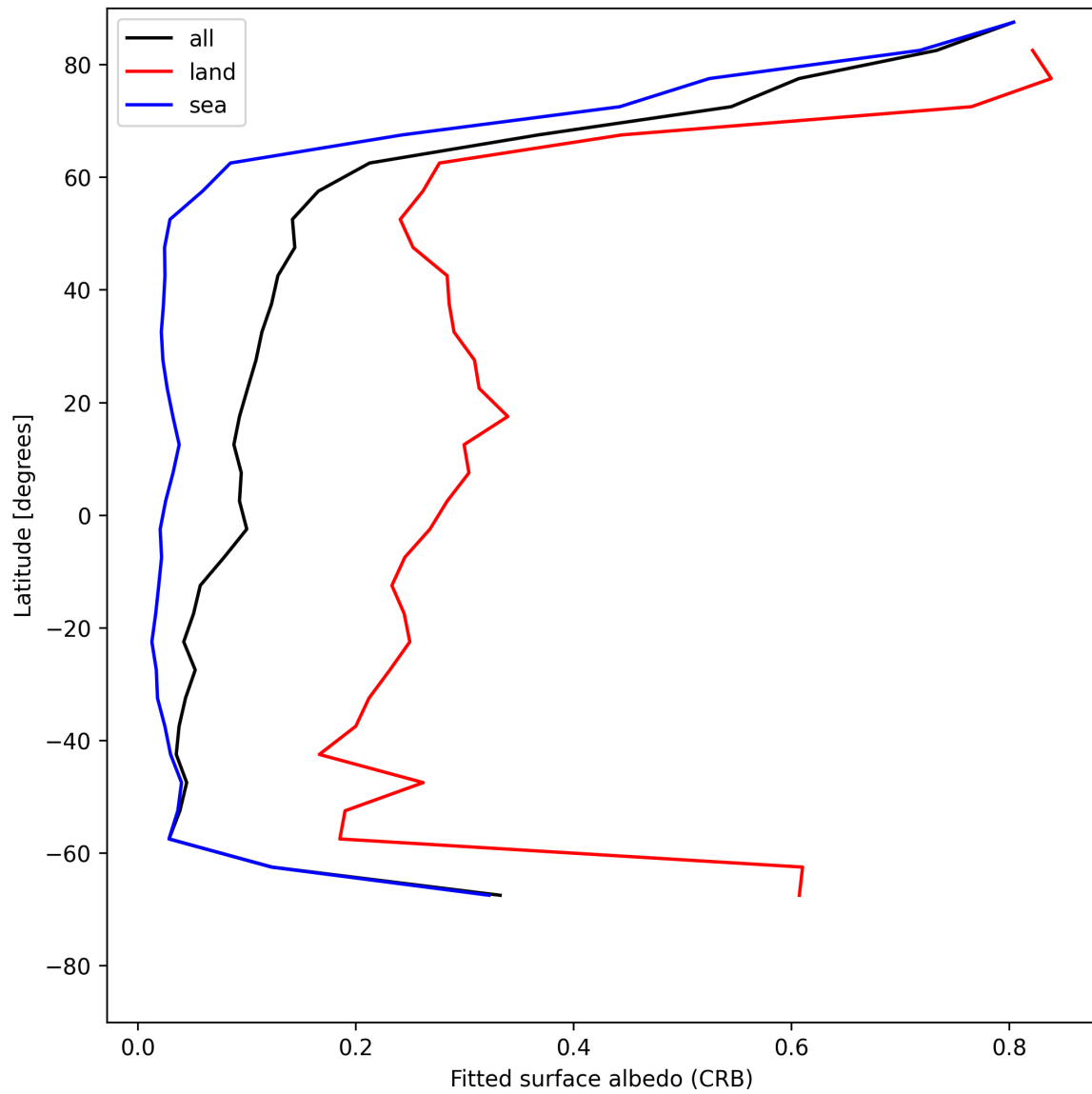
Figure 28: Zonal average of “Fitted surface albedo (CRB)” for 2025-06-02 to 2025-06-03.
