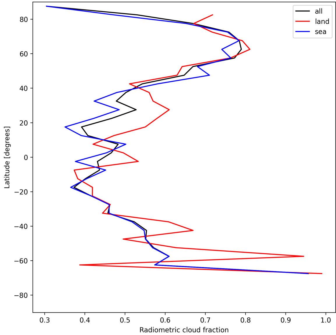
Figure 21: Zonal average of “Radiometric cloud fraction” for 2025-06-02 to 2025-06-03.
