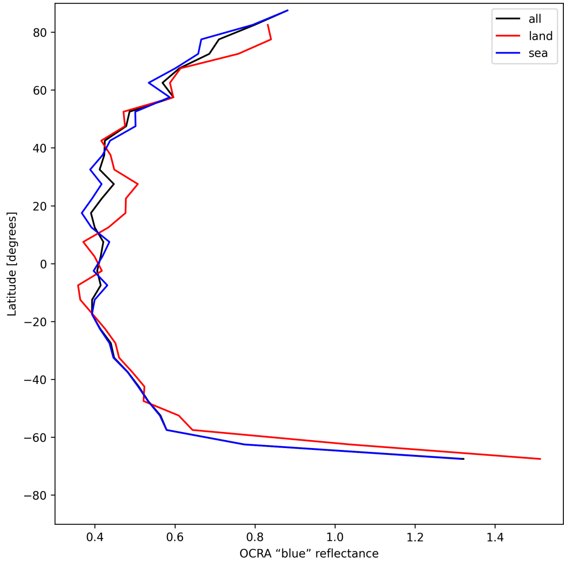
Figure 33: Zonal average of “OCRA “blue” reflectance” for 2025-06-02 to 2025-06-03.
