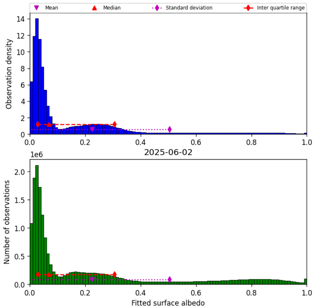
Figure 43: Histogram of “Fitted surface albedo” for 2025-06-02 to 2025-06-03
