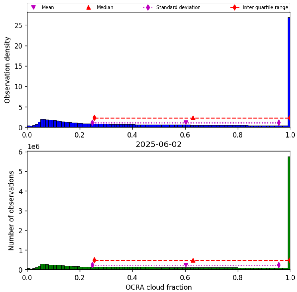
Figure 48: Histogram of “OCRA cloud fraction” for 2025-06-02 to 2025-06-03
