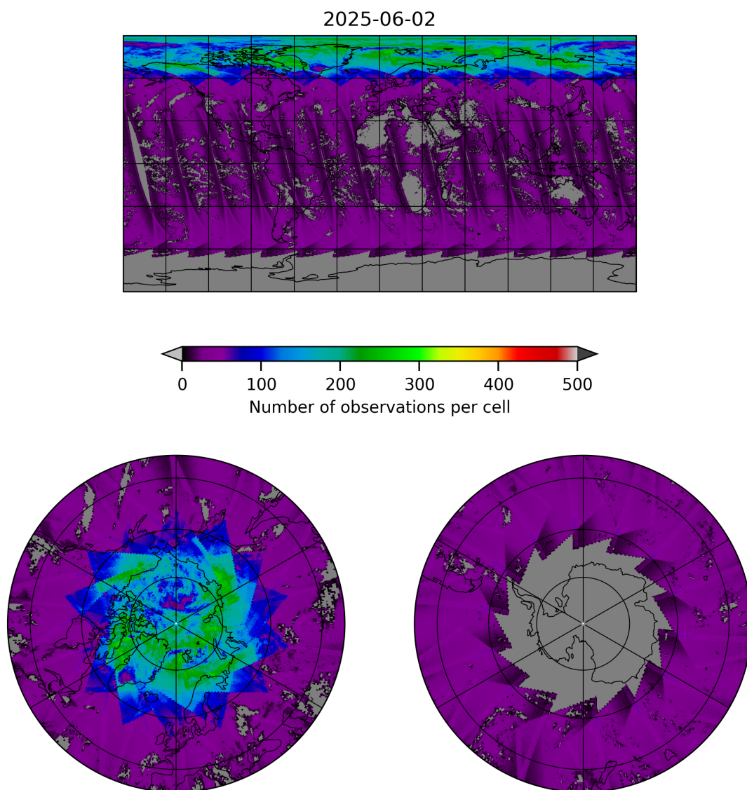
Figure 19: Map of the number of observations for 2025-06-02 to 2025-06-03
