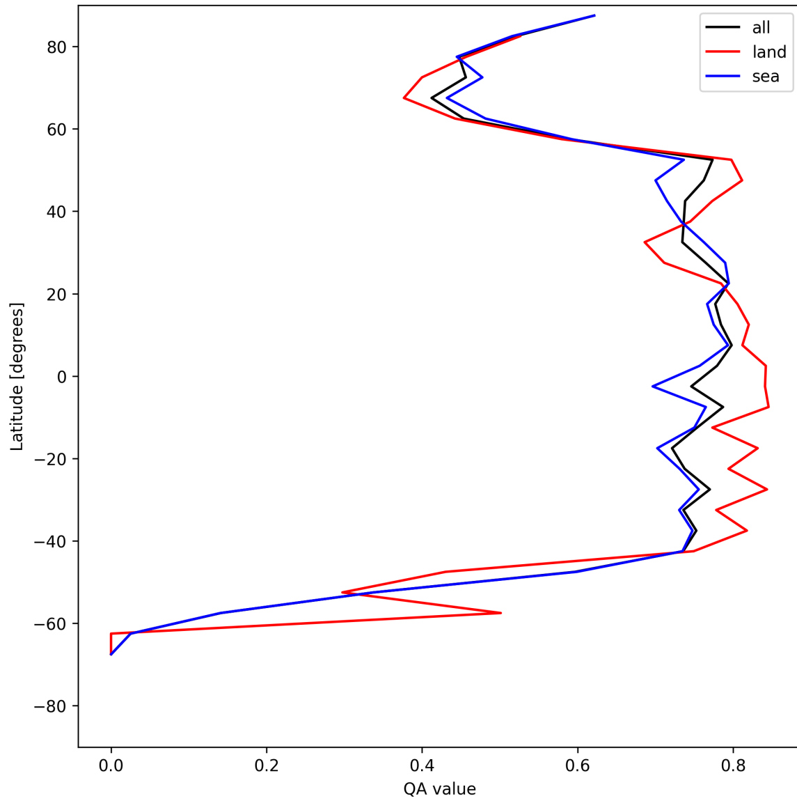
Figure 20: Zonal average of “QA value” for 2025-06-02 to 2025-06-03.
