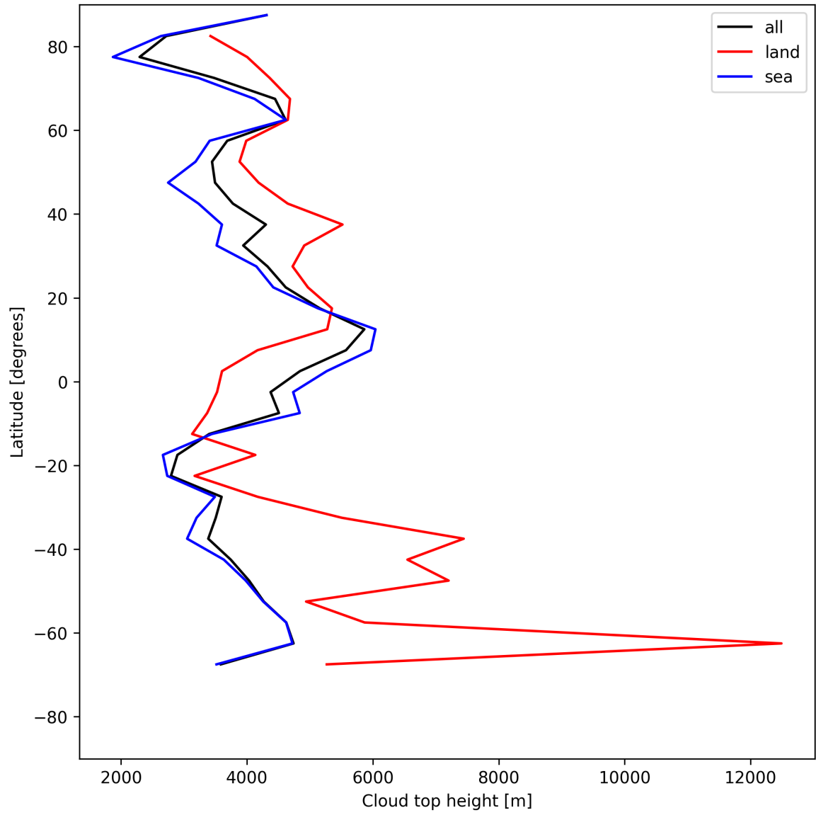
Figure 22: Zonal average of “Cloud top height” for 2025-06-02 to 2025-06-03.
