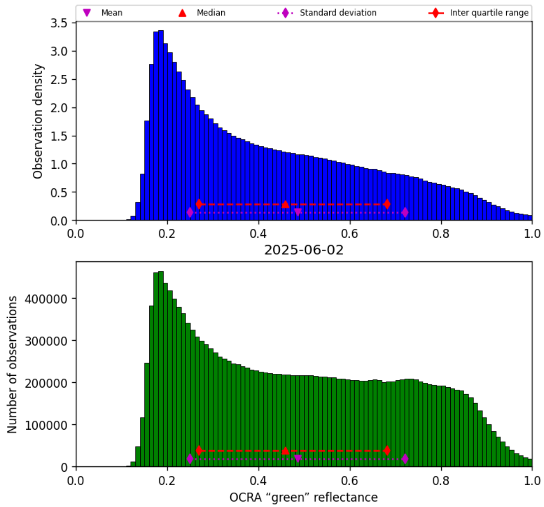
Figure 50: Histogram of “OCRA “green” reflectance” for 2025-06-02 to 2025-06-03
