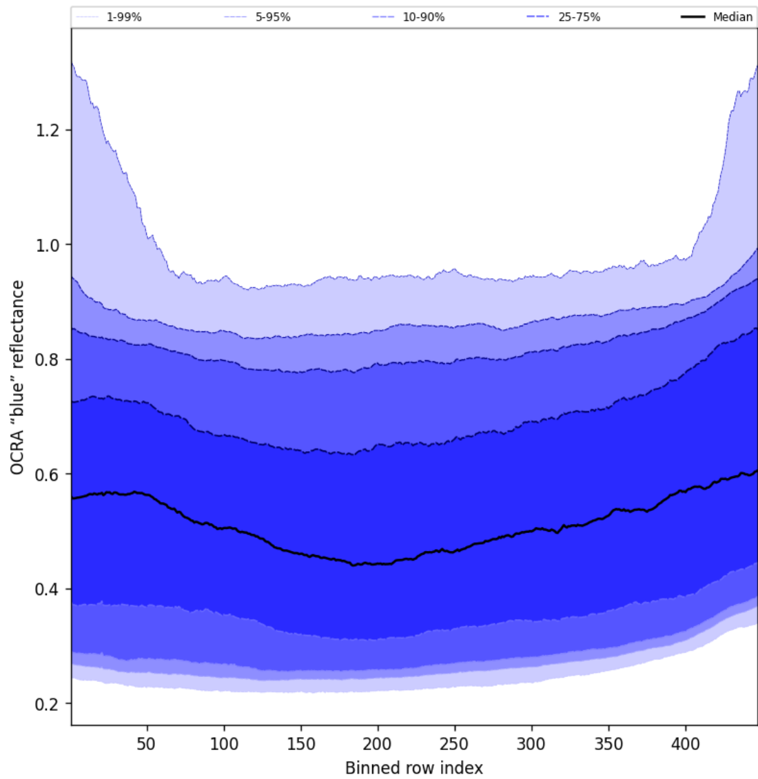
Figure 65: Along track statistics of “OCRA “blue” reflectance” for 2025-06-02 to 2025-06-03
