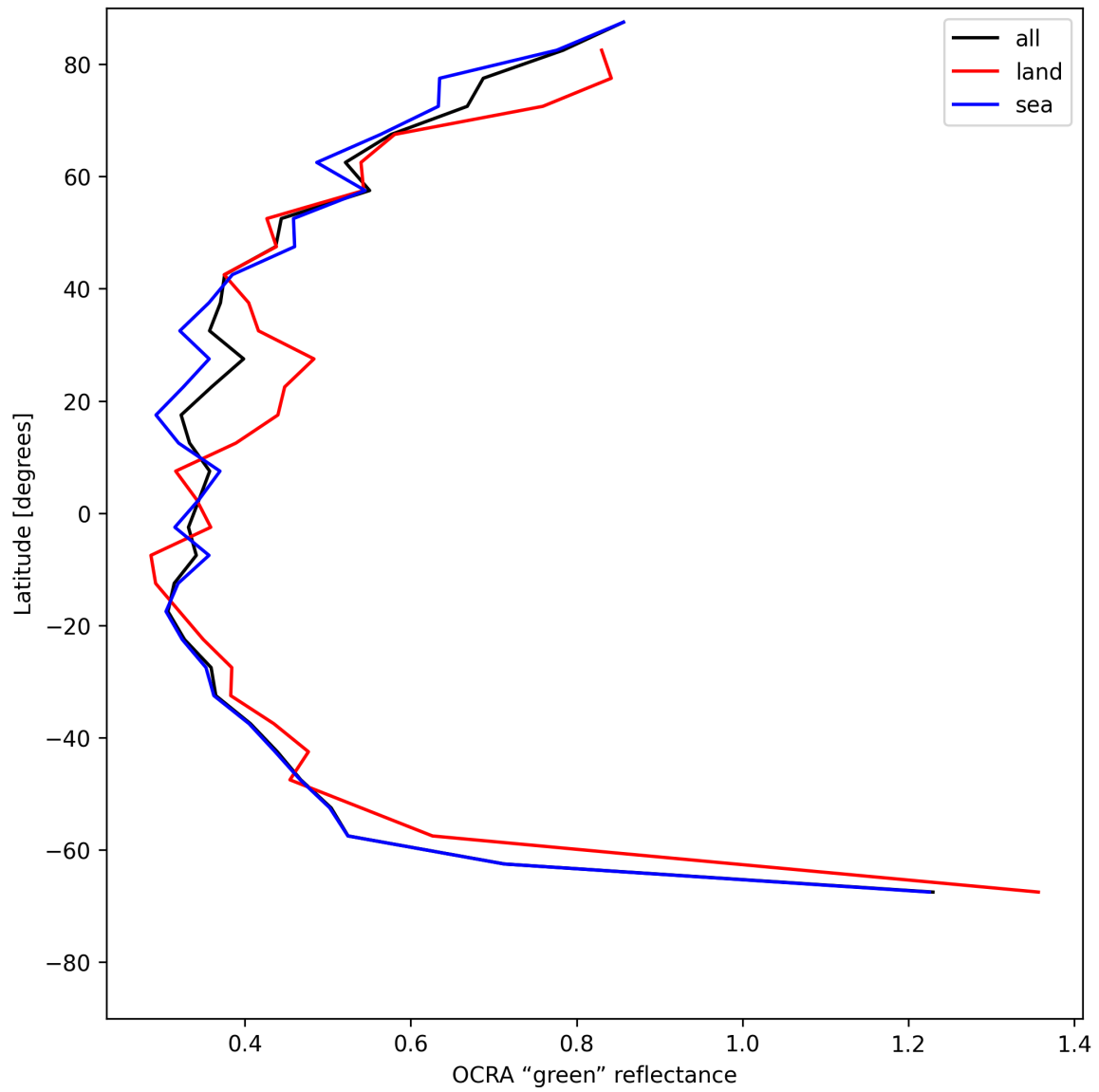
Figure 34: Zonal average of “OCRA “green” reflectance” for 2025-06-02 to 2025-06-03.
