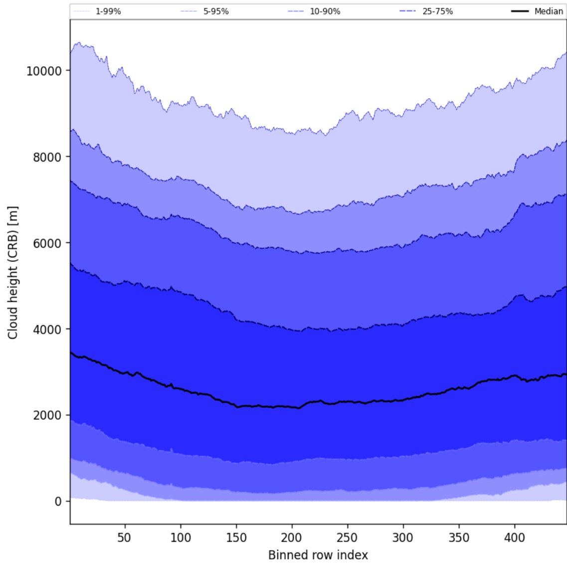
Figure 57: Along track statistics of “Cloud height (CRB)” for 2025-06-02 to 2025-06-03
