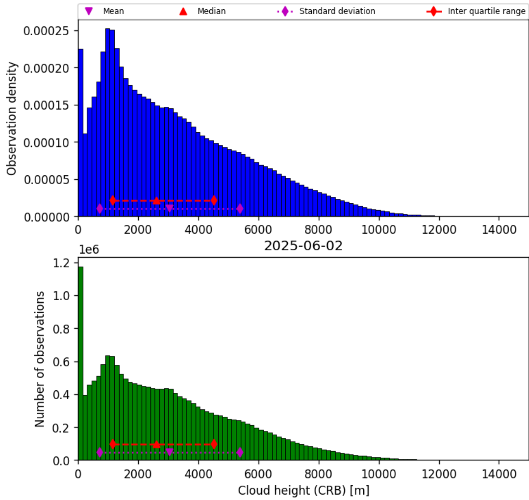
Figure 41: Histogram of “Cloud height (CRB)” for 2025-06-02 to 2025-06-03
