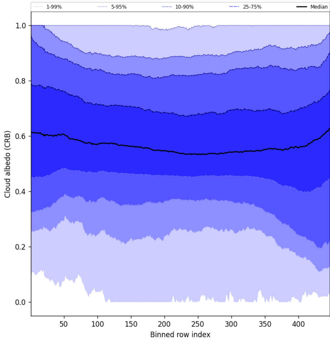
Figure 58: Along track statistics of “Cloud albedo (CRB)” for 2025-06-02 to 2025-06-03
