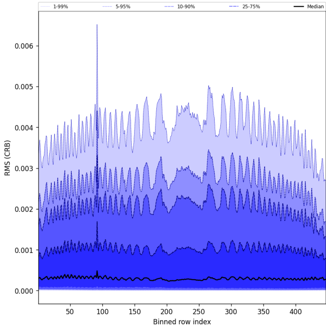
Figure 62: Along track statistics of “RMS (CRB)” for 2025-06-02 to 2025-06-03
