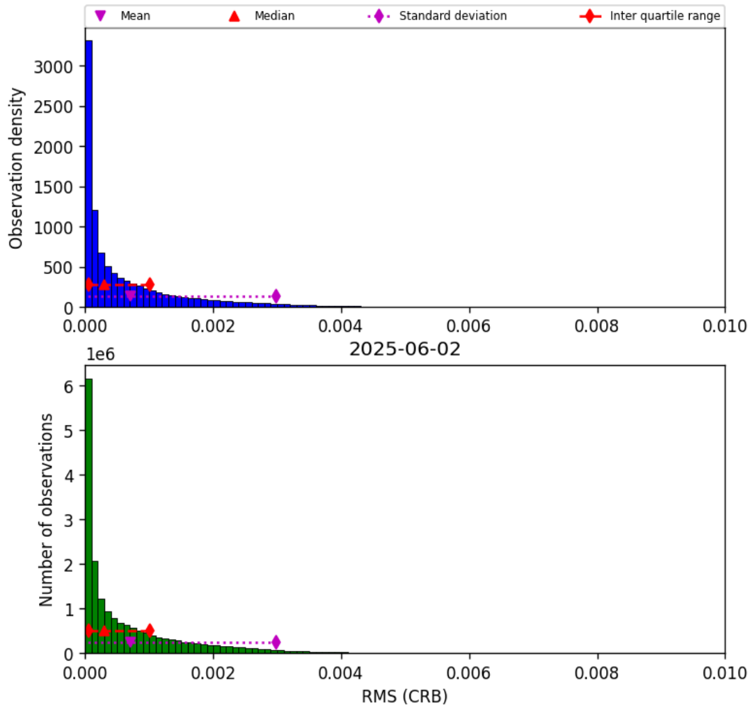
Figure 46: Histogram of “RMS (CRB)” for 2025-06-02 to 2025-06-03
