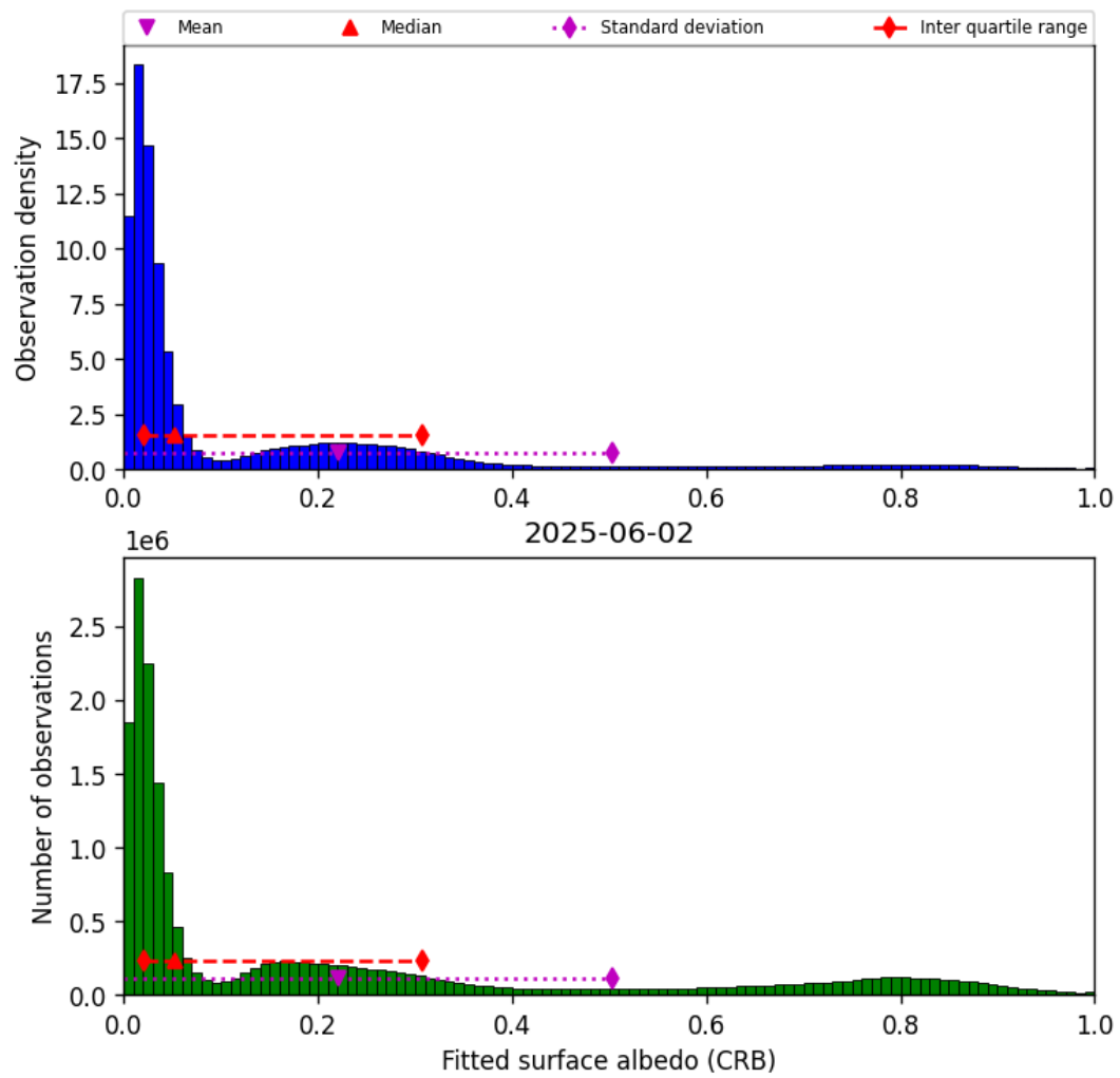
Figure 44: Histogram of “Fitted surface albedo (CRB)” for 2025-06-02 to 2025-06-03
