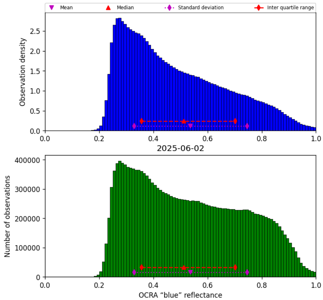
Figure 49: Histogram of “OCRA “blue” reflectance” for 2025-06-02 to 2025-06-03
