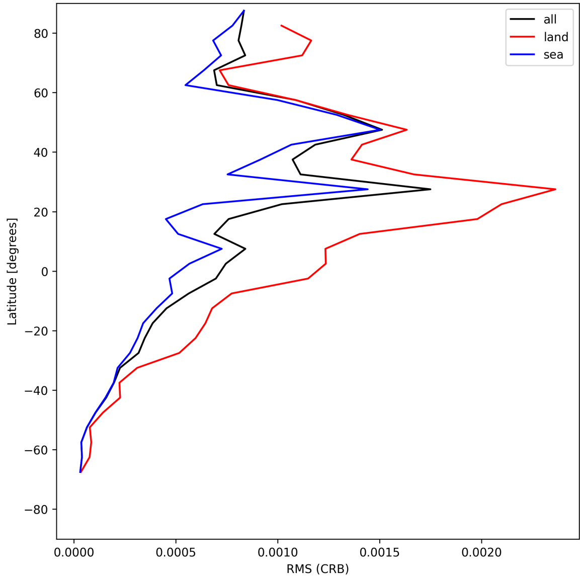
Figure 30: Zonal average of “RMS (CRB)” for 2025-06-02 to 2025-06-03.
