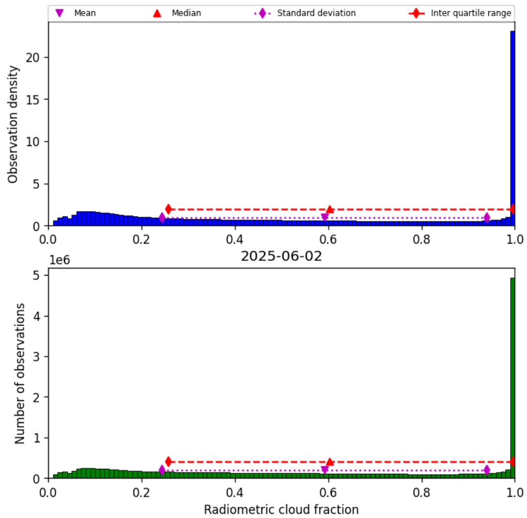
Figure 37: Histogram of “Radiometric cloud fraction” for 2025-06-02 to 2025-06-03
