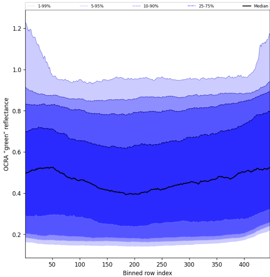
Figure 66: Along track statistics of “OCRA “green” reflectance” for 2025-06-02 to 2025-06-03
