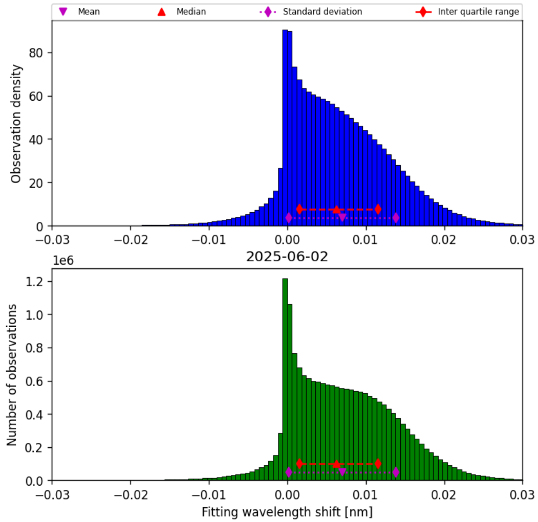
Figure 47: Histogram of “Fitting wavelength shift” for 2025-06-02 to 2025-06-03
