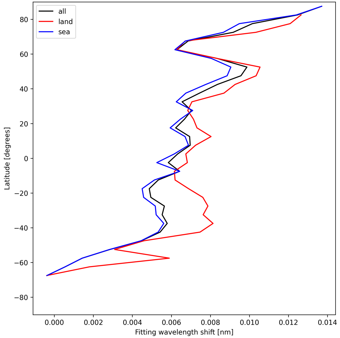
Figure 31: Zonal average of “Fitting wavelength shift” for 2025-06-02 to 2025-06-03.
