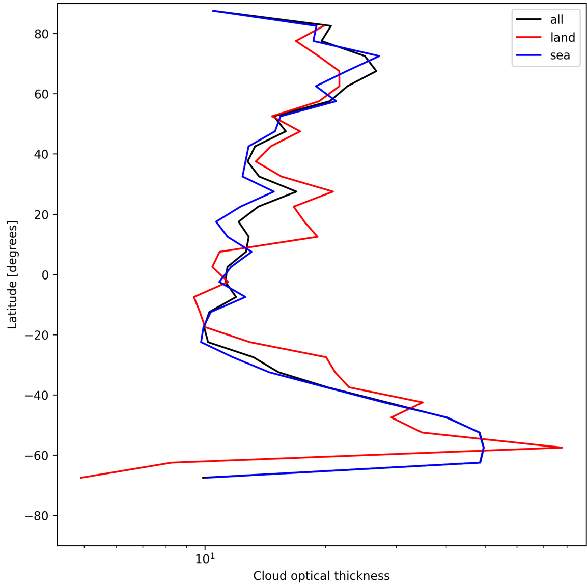
Figure 23: Zonal average of “Cloud optical thickness” for 2025-06-02 to 2025-06-03.
