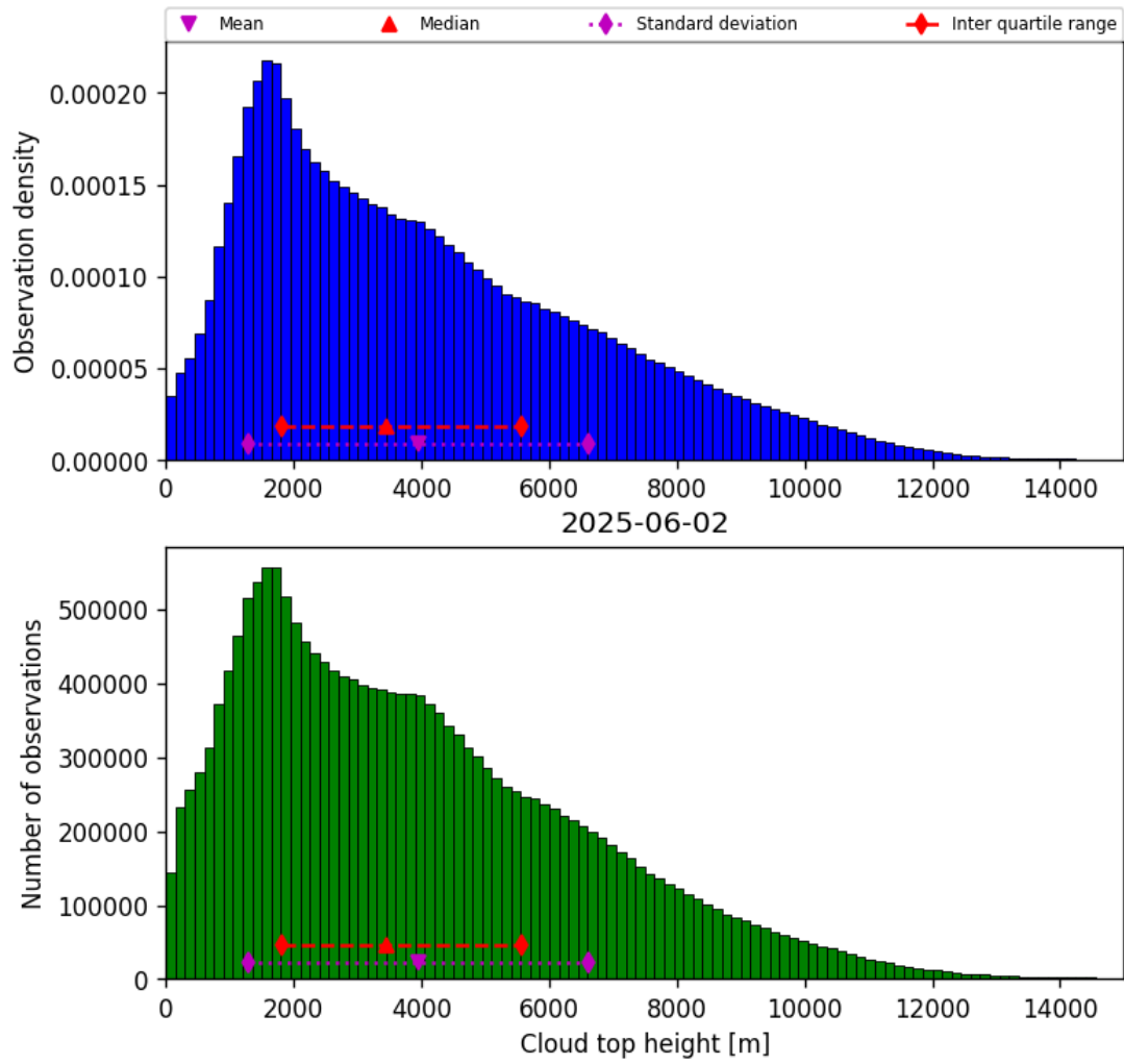
Figure 38: Histogram of “Cloud top height” for 2025-06-02 to 2025-06-03
