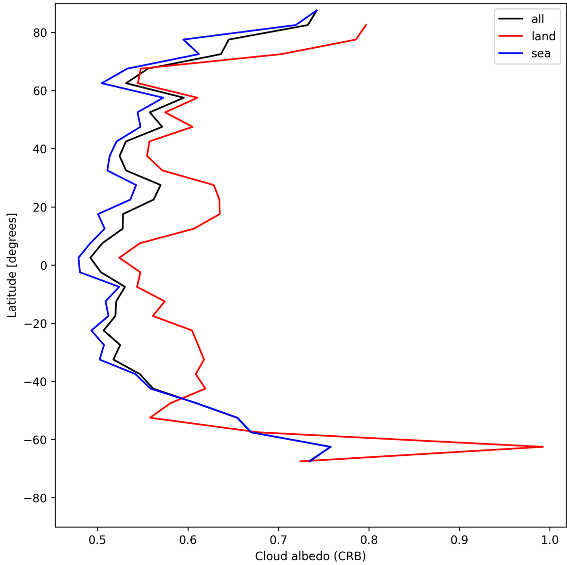
Figure 26: Zonal average of “Cloud albedo (CRB)” for 2025-06-02 to 2025-06-03.
