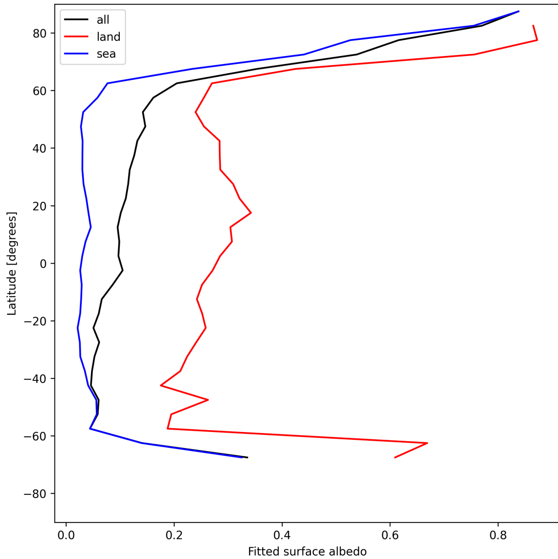
Figure 27: Zonal average of “Fitted surface albedo” for 2025-06-02 to 2025-06-03.
