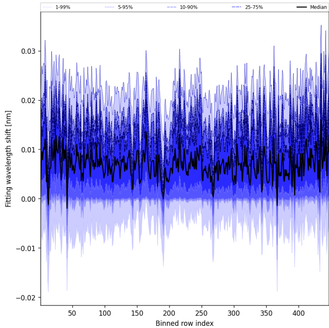
Figure 63: Along track statistics of “Fitting wavelength shift” for 2025-06-02 to 2025-06-03
