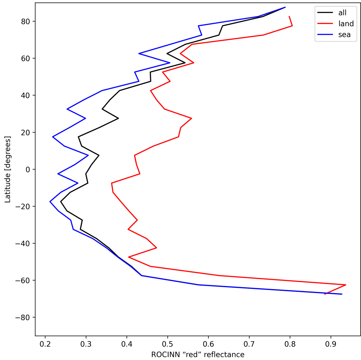
Figure 35: Zonal average of “ROCINN “red” reflectance” for 2025-06-02 to 2025-06-03.
