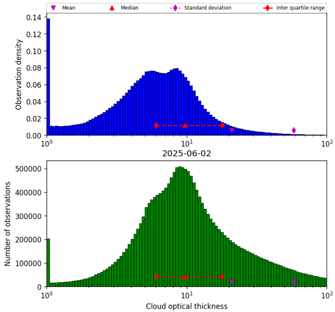
Figure 39: Histogram of “Cloud optical thickness” for 2025-06-02 to 2025-06-03
