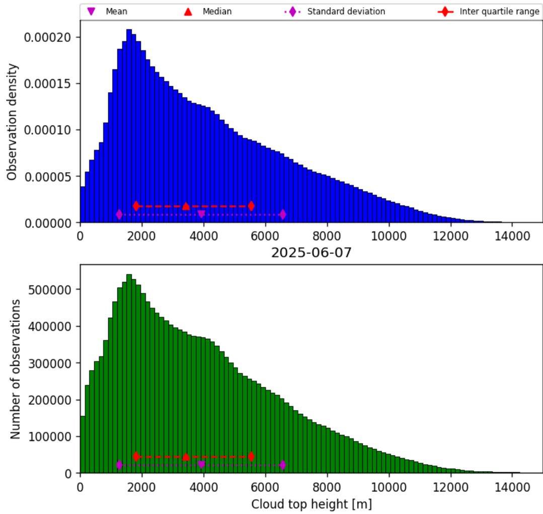
Figure 38: Histogram of “Cloud top height” for 2025-06-07 to 2025-06-08
