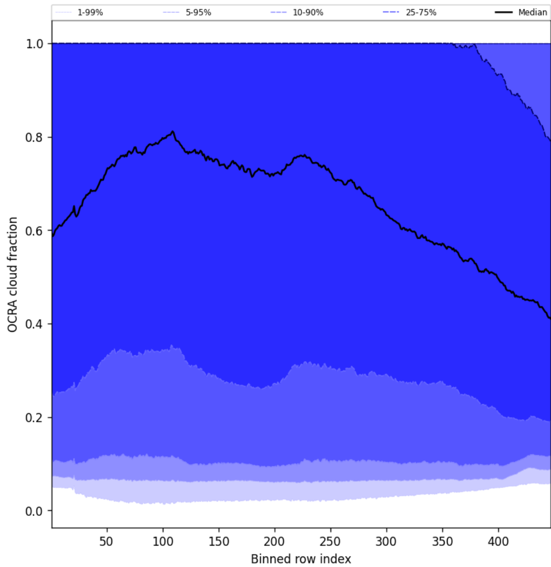
Figure 64: Along track statistics of “OCRA cloud fraction” for 2025-06-07 to 2025-06-08
