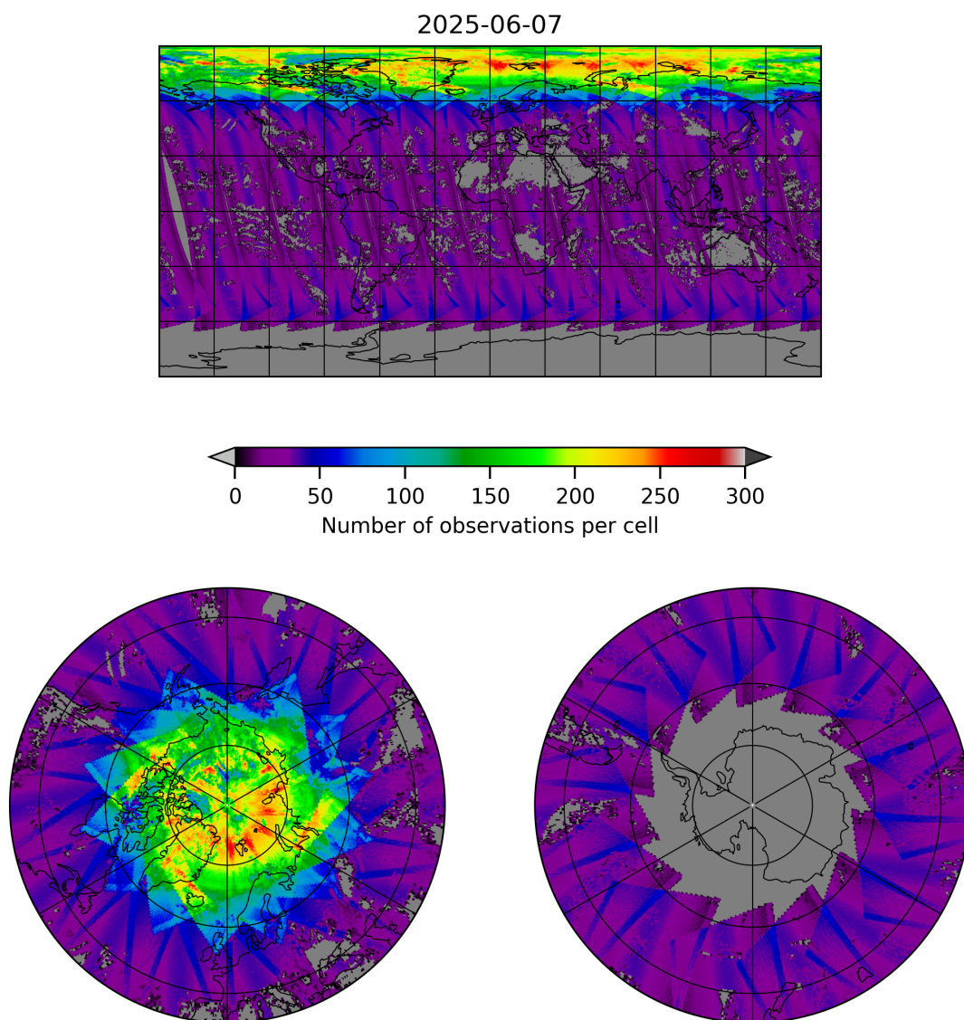
Figure 19: Map of the number of observations for 2025-06-07 to 2025-06-08
