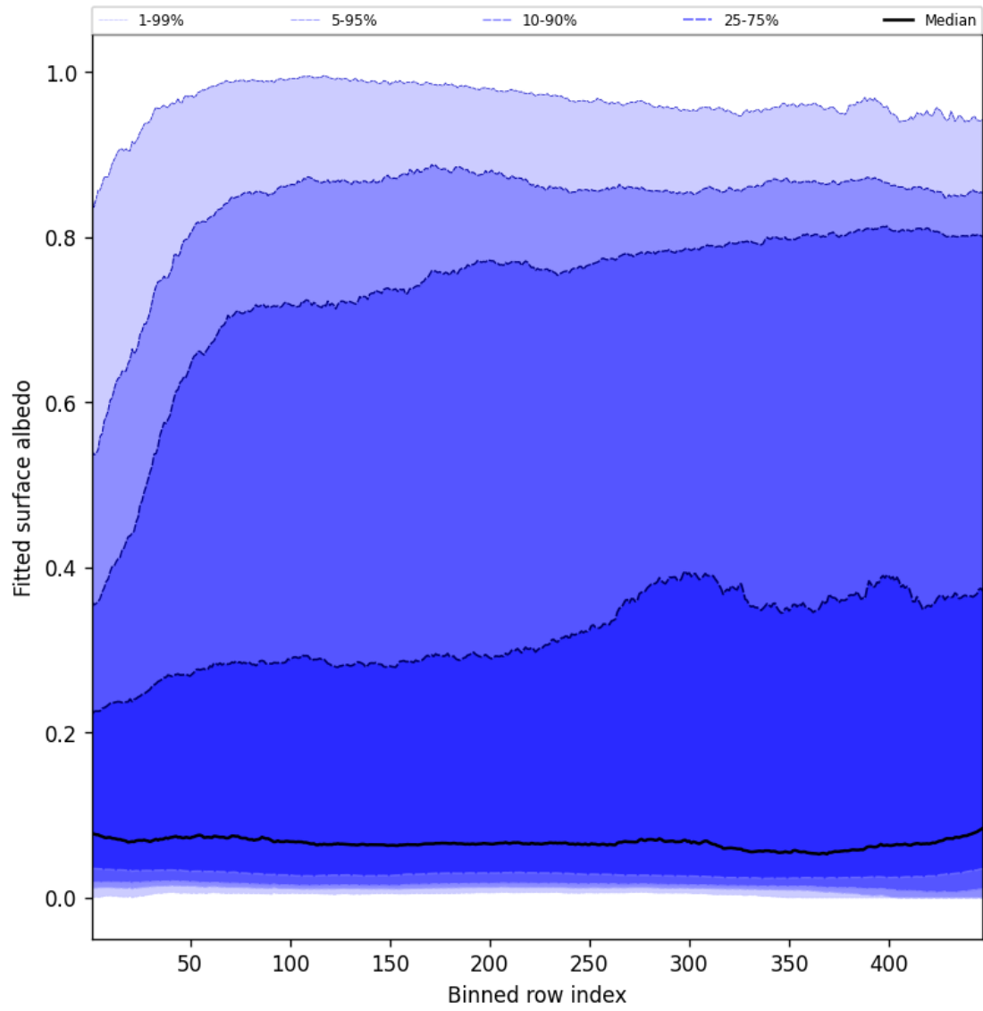
Figure 59: Along track statistics of “Fitted surface albedo” for 2025-06-07 to 2025-06-08
