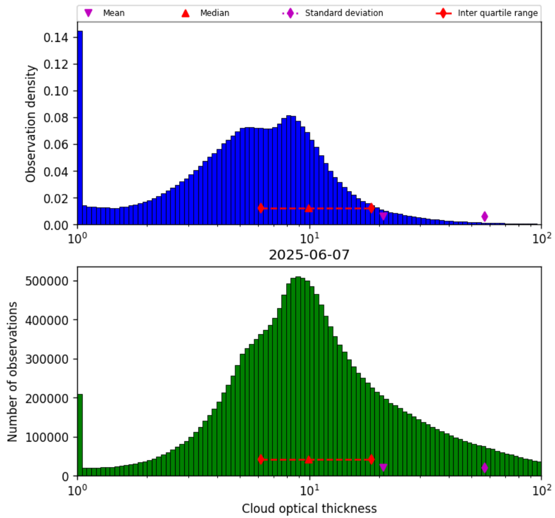
Figure 39: Histogram of “Cloud optical thickness” for 2025-06-07 to 2025-06-08
