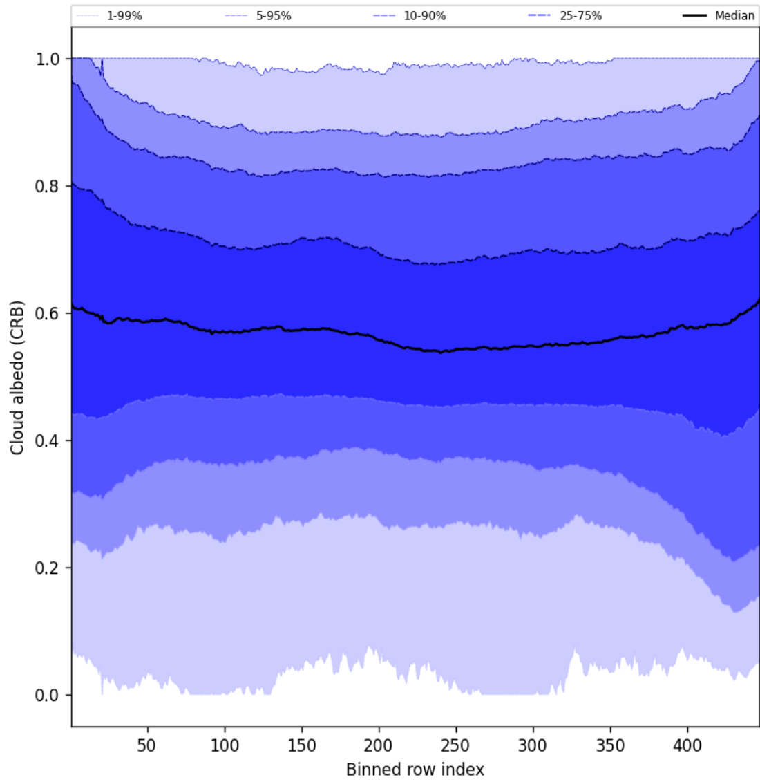
Figure 58: Along track statistics of “Cloud albedo (CRB)” for 2025-06-07 to 2025-06-08
