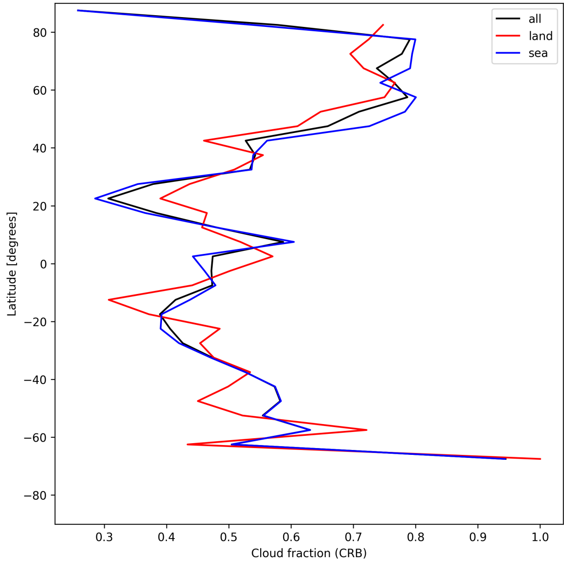
Figure 24: Zonal average of “Cloud fraction (CRB)” for 2025-06-07 to 2025-06-08.
