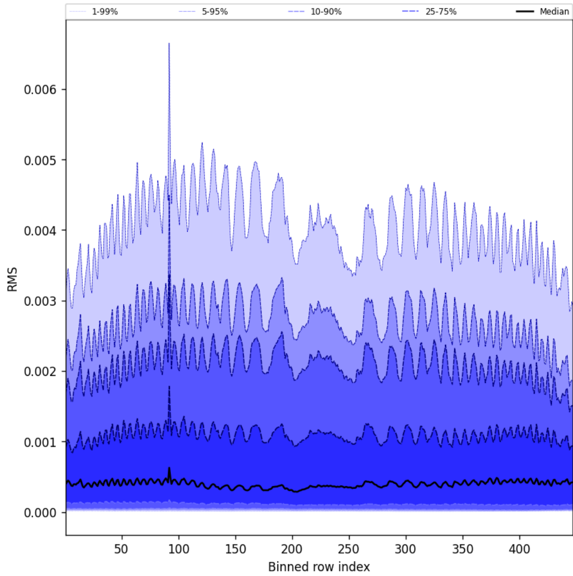
Figure 61: Along track statistics of “RMS” for 2025-06-07 to 2025-06-08
