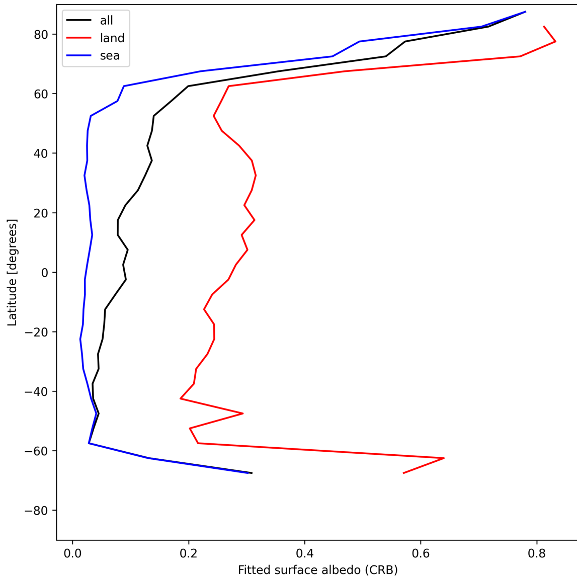
Figure 28: Zonal average of “Fitted surface albedo (CRB)” for 2025-06-07 to 2025-06-08.
