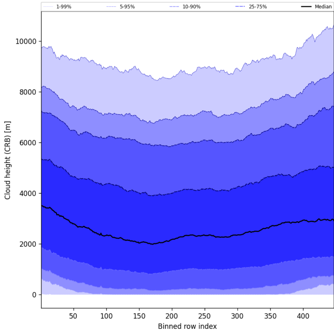
Figure 57: Along track statistics of “Cloud height (CRB)” for 2025-06-07 to 2025-06-08
