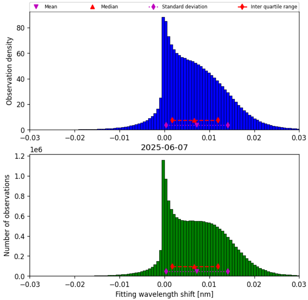
Figure 47: Histogram of “Fitting wavelength shift” for 2025-06-07 to 2025-06-08
