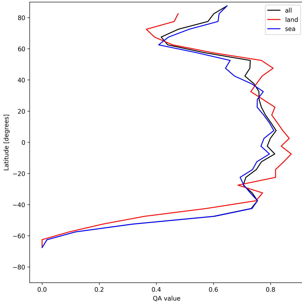
Figure 20: Zonal average of “QA value” for 2025-06-07 to 2025-06-08.
