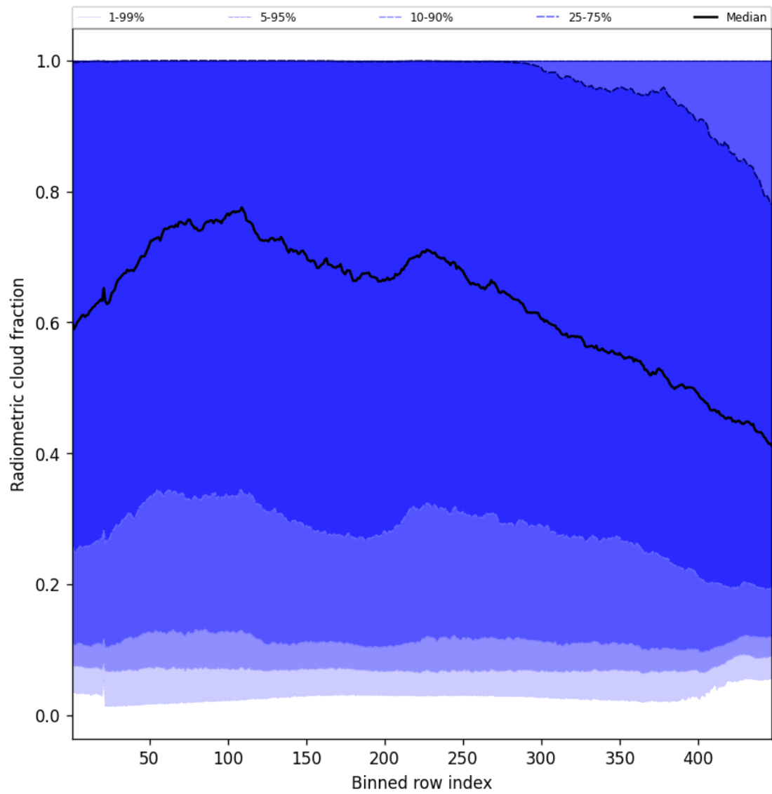
Figure 53: Along track statistics of “Radiometric cloud fraction” for 2025-06-07 to 2025-06-08
