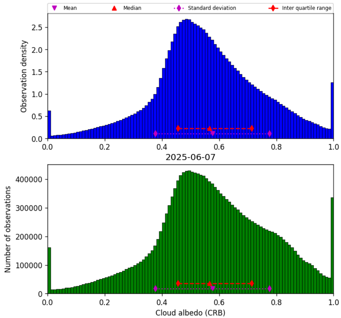
Figure 42: Histogram of “Cloud albedo (CRB)” for 2025-06-07 to 2025-06-08
