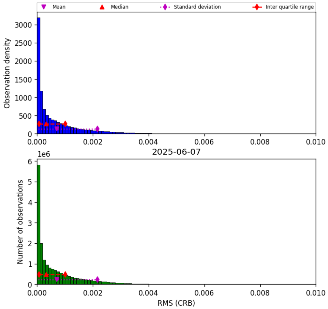
Figure 46: Histogram of “RMS (CRB)” for 2025-06-07 to 2025-06-08
