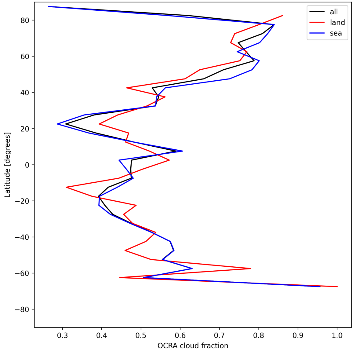
Figure 32: Zonal average of “OCRA cloud fraction” for 2025-06-07 to 2025-06-08.
