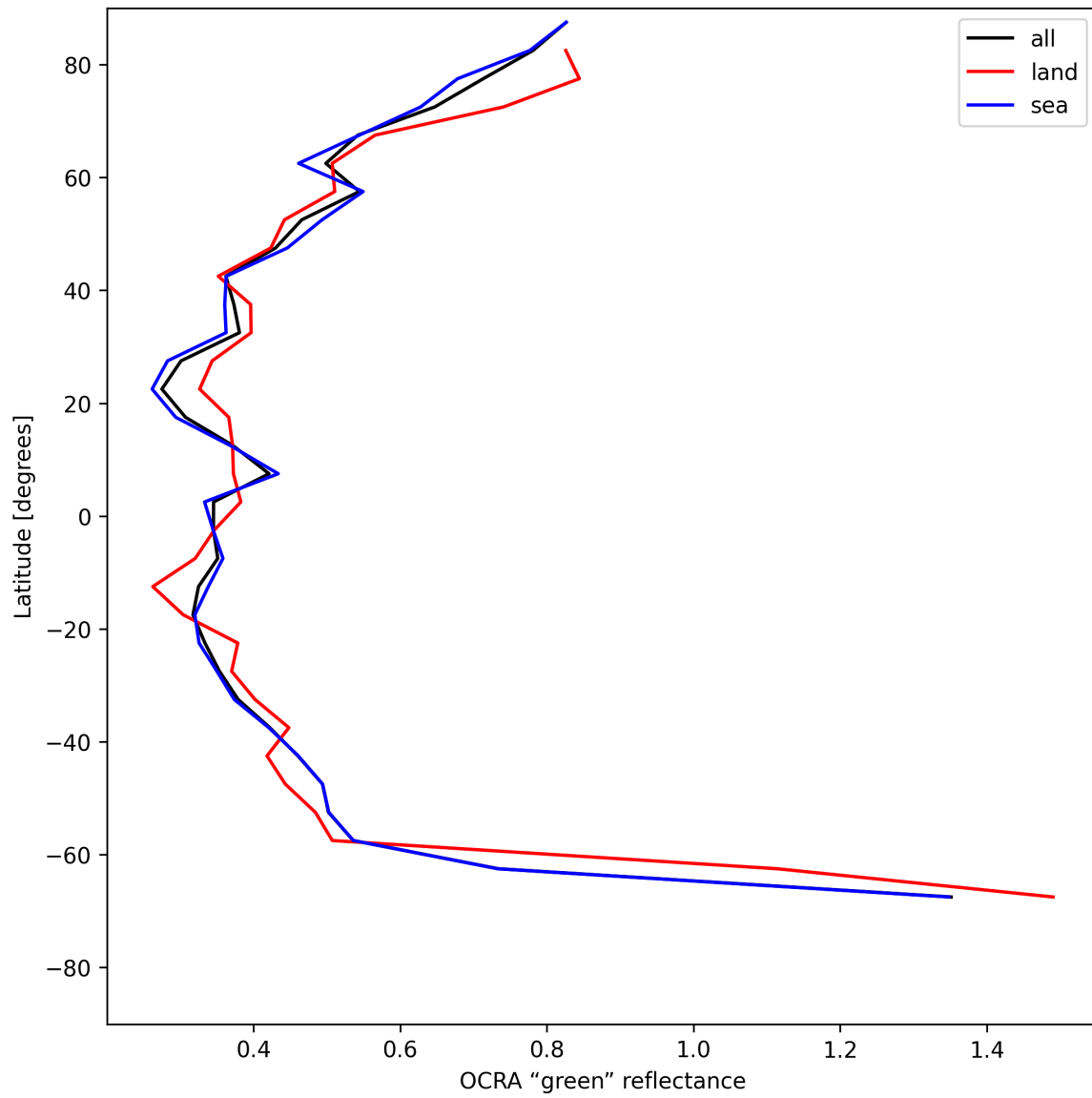
Figure 34: Zonal average of “OCRA “green” reflectance” for 2025-06-07 to 2025-06-08.
