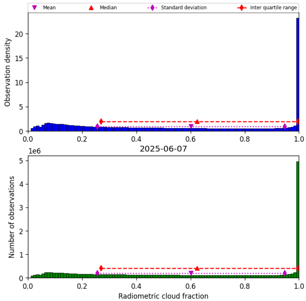
Figure 37: Histogram of “Radiometric cloud fraction” for 2025-06-07 to 2025-06-08
