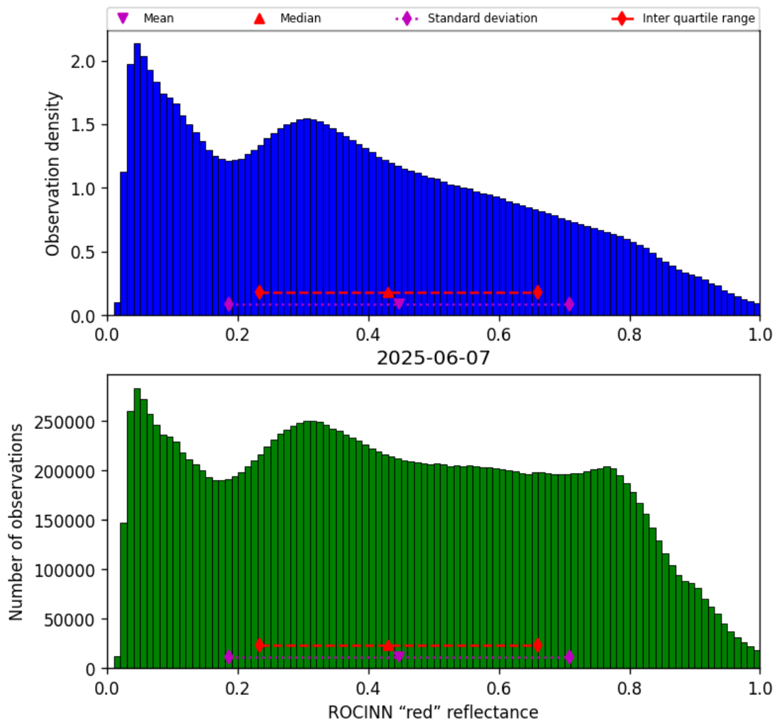
Figure 51: Histogram of “ROCINN “red” reflectance” for 2025-06-07 to 2025-06-08
