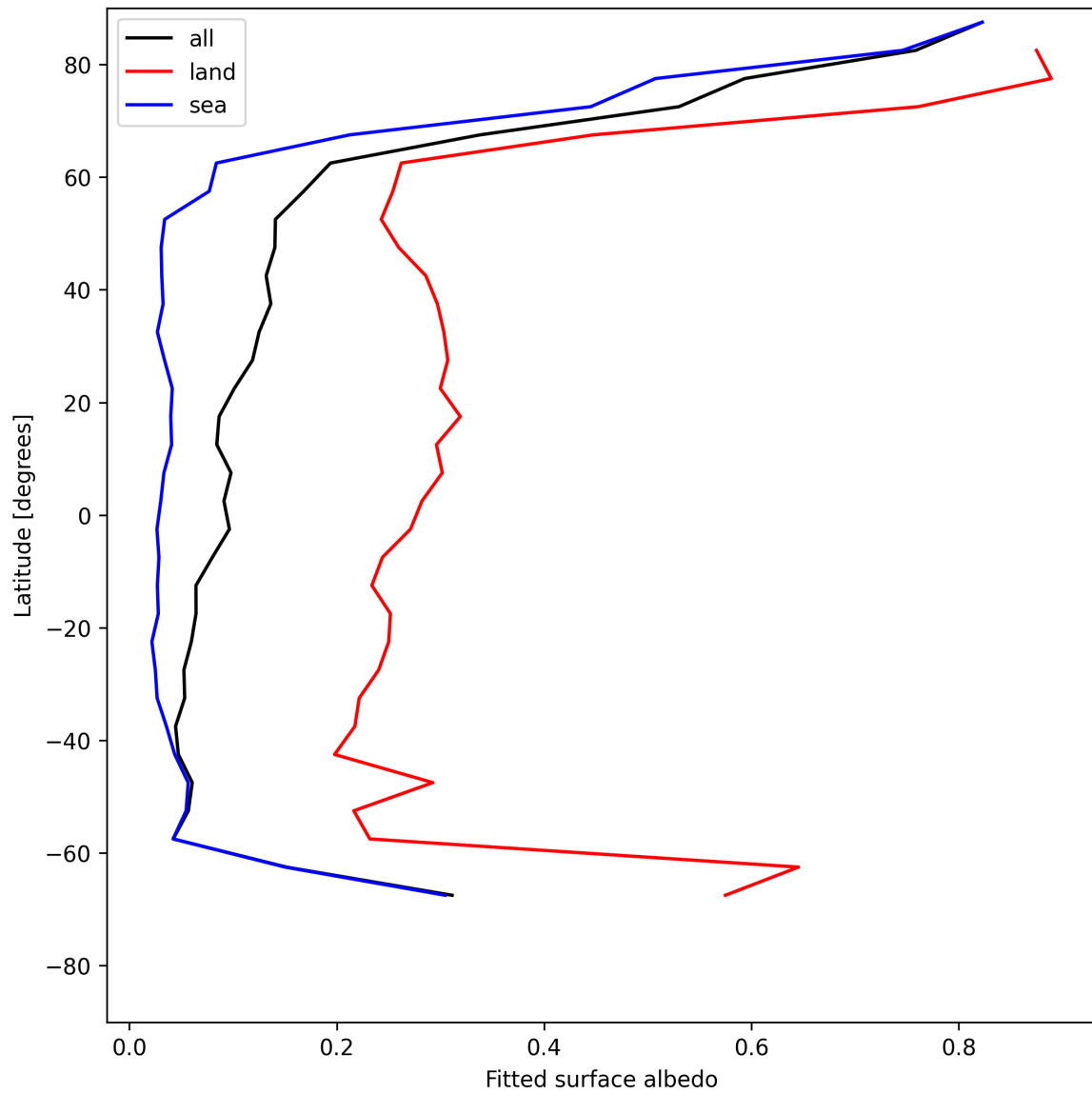
Figure 27: Zonal average of “Fitted surface albedo” for 2025-06-07 to 2025-06-08.
