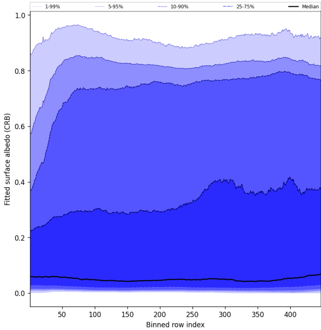
Figure 60: Along track statistics of “Fitted surface albedo (CRB)” for 2025-06-07 to 2025-06-08
