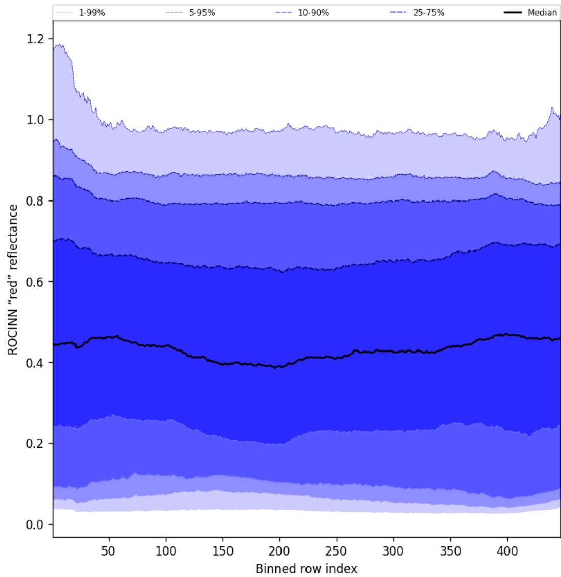
Figure 67: Along track statistics of “ROCINN “red” reflectance” for 2025-06-07 to 2025-06-08
