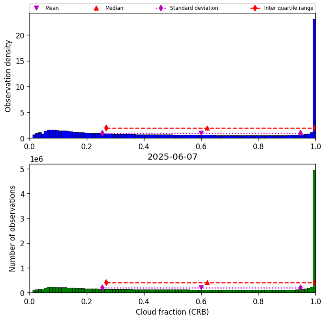
Figure 40: Histogram of “Cloud fraction (CRB)” for 2025-06-07 to 2025-06-08
