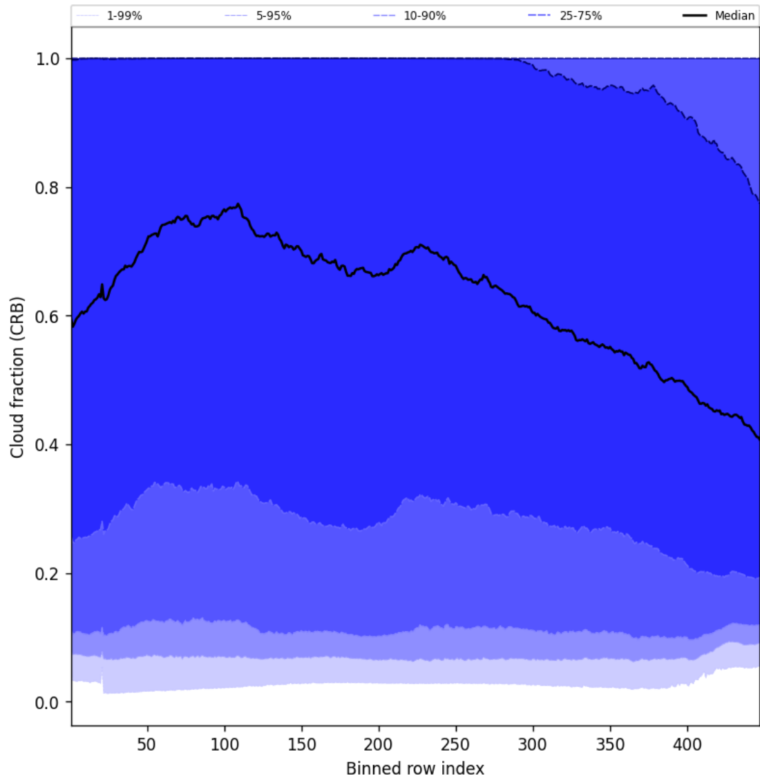
Figure 56: Along track statistics of “Cloud fraction (CRB)” for 2025-06-07 to 2025-06-08
