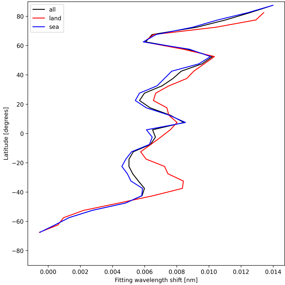
Figure 31: Zonal average of “Fitting wavelength shift” for 2025-06-07 to 2025-06-08.
