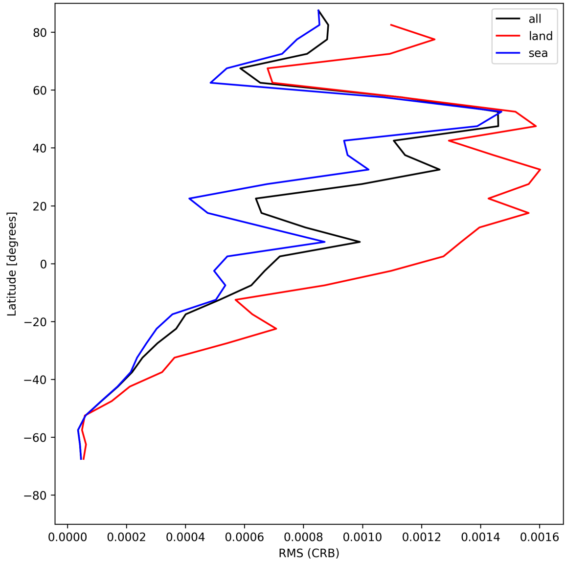
Figure 30: Zonal average of “RMS (CRB)” for 2025-06-07 to 2025-06-08.
