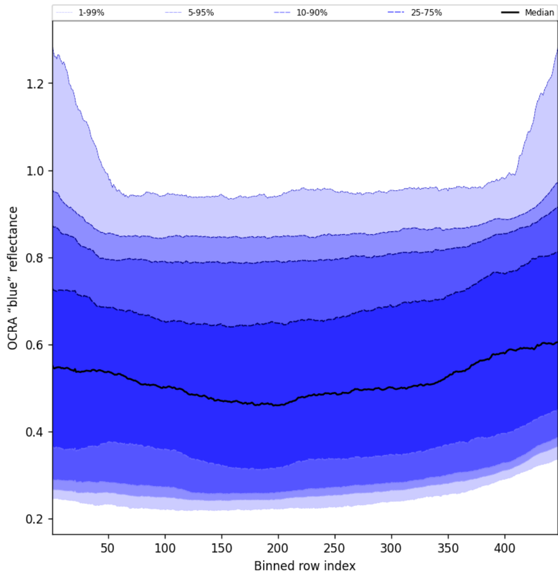
Figure 65: Along track statistics of “OCRA “blue” reflectance” for 2025-06-07 to 2025-06-08
