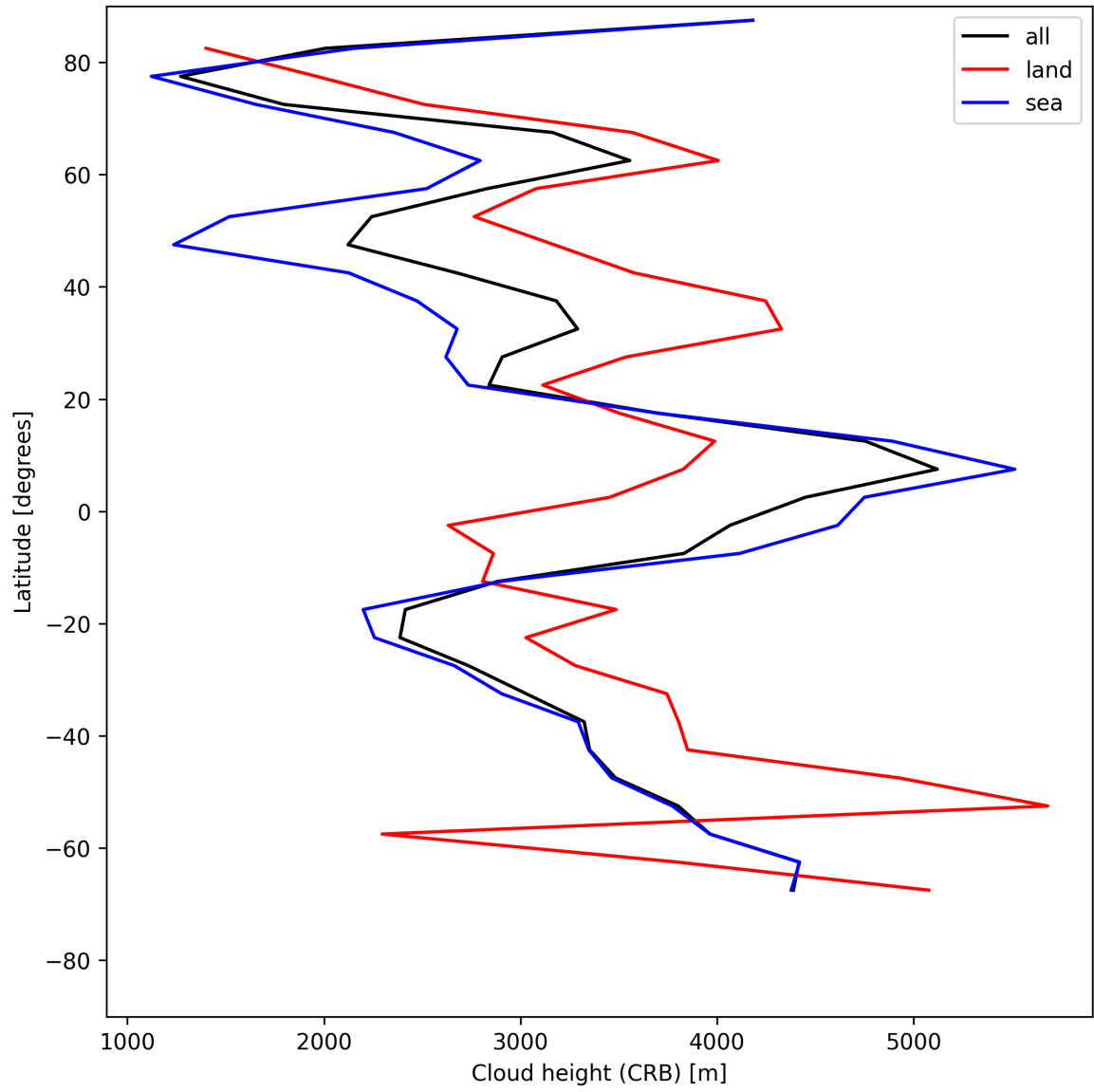
Figure 25: Zonal average of “Cloud height (CRB)” for 2025-06-07 to 2025-06-08.
