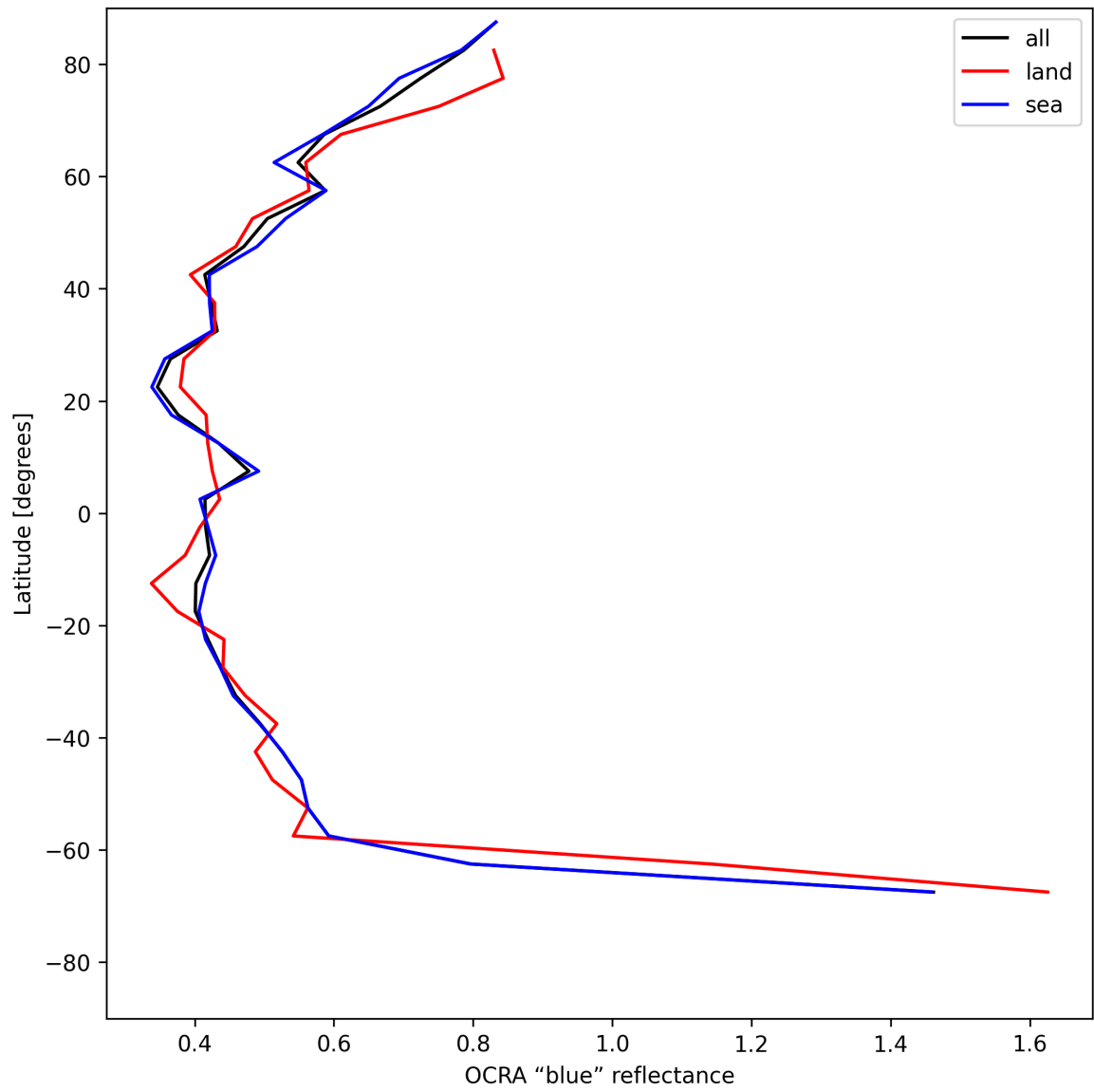
Figure 33: Zonal average of “OCRA “blue” reflectance” for 2025-06-07 to 2025-06-08.
