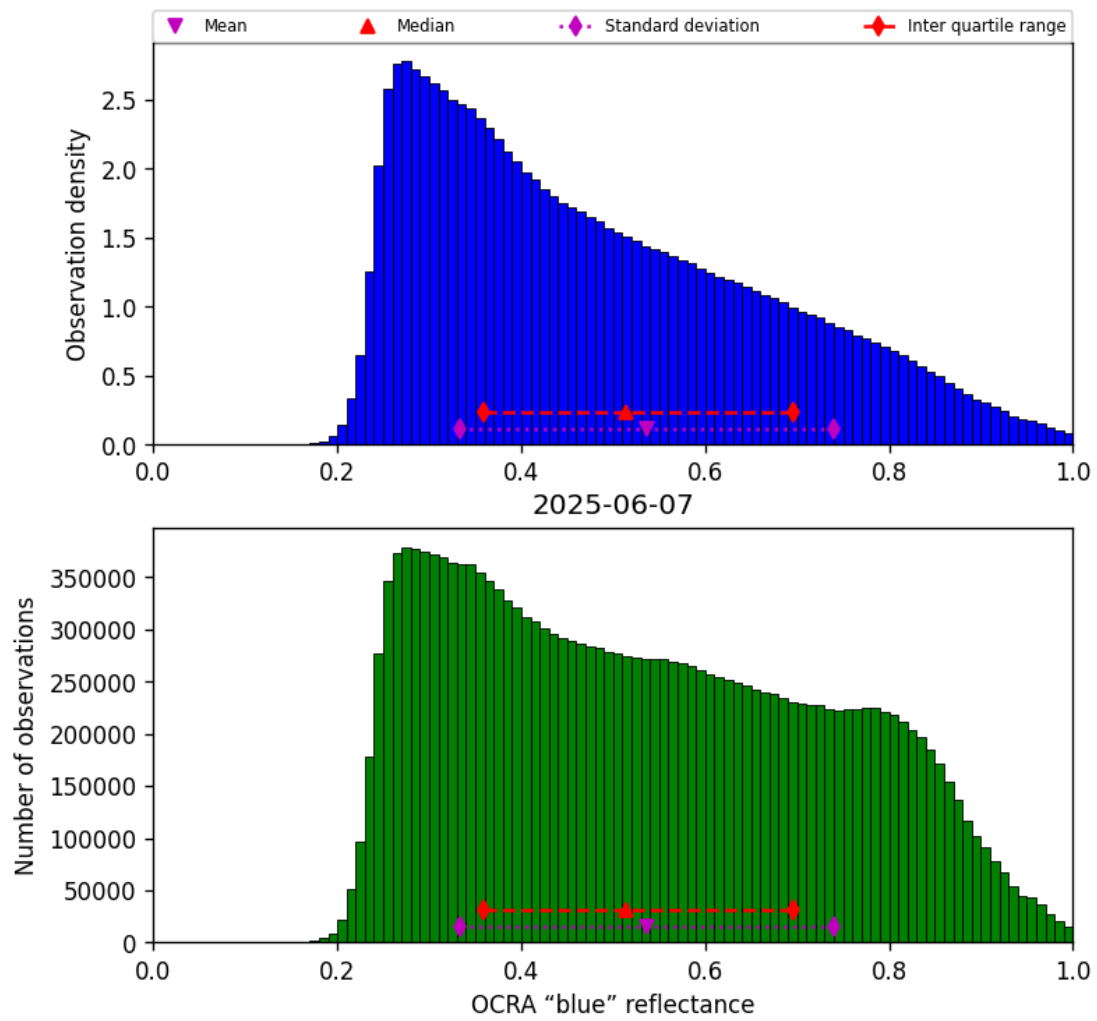
Figure 49: Histogram of “OCRA “blue” reflectance” for 2025-06-07 to 2025-06-08
