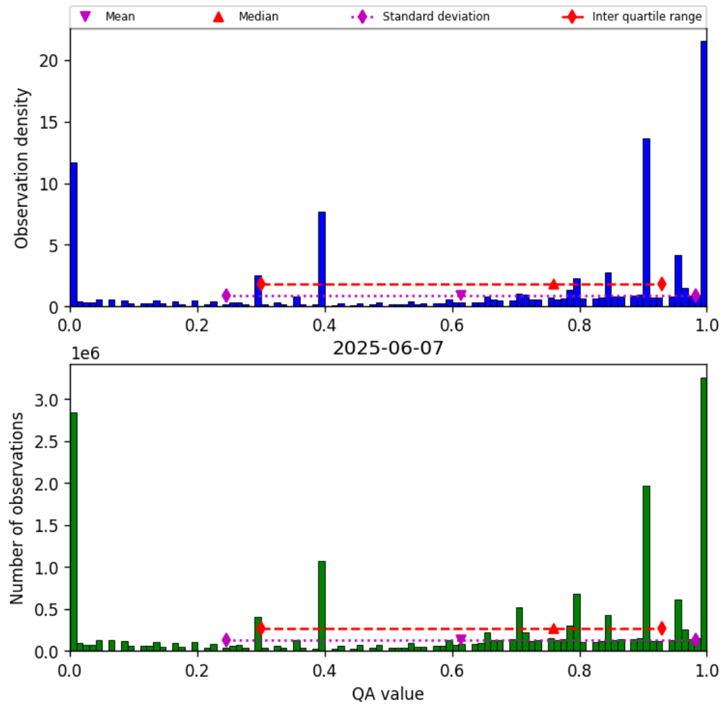
Figure 36: Histogram of “QA value” for 2025-06-07 to 2025-06-08
