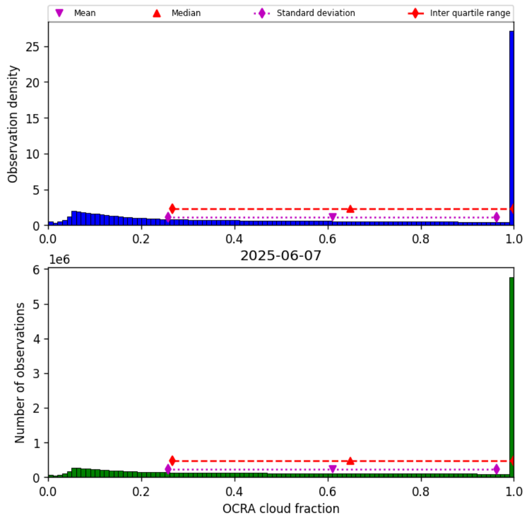
Figure 48: Histogram of “OCRA cloud fraction” for 2025-06-07 to 2025-06-08
