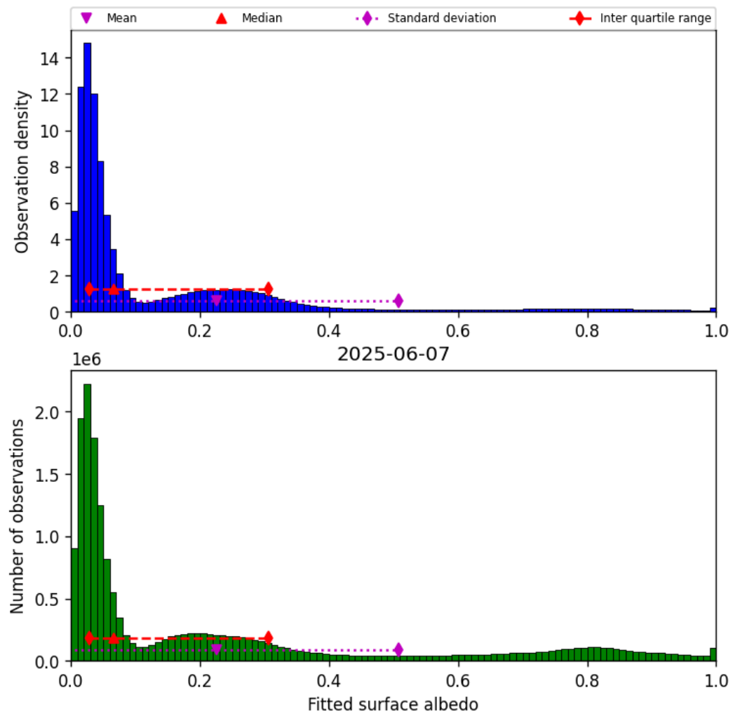
Figure 43: Histogram of “Fitted surface albedo” for 2025-06-07 to 2025-06-08
