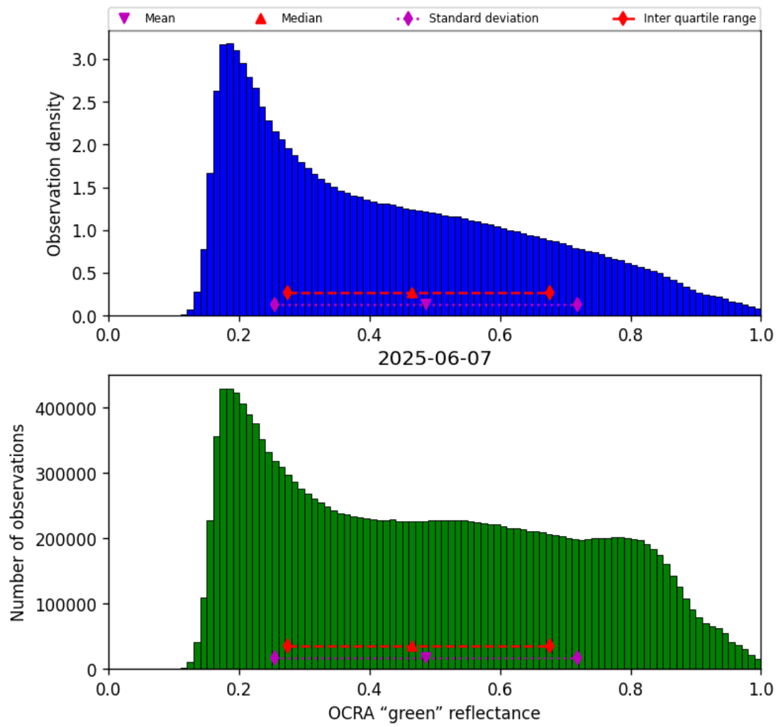
Figure 50: Histogram of “OCRA “green” reflectance” for 2025-06-07 to 2025-06-08
