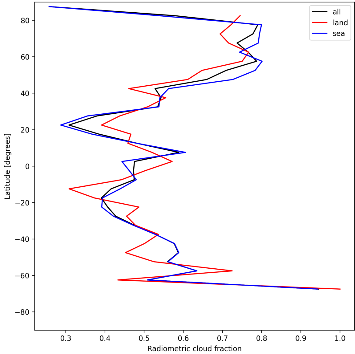
Figure 21: Zonal average of “Radiometric cloud fraction” for 2025-06-07 to 2025-06-08.
