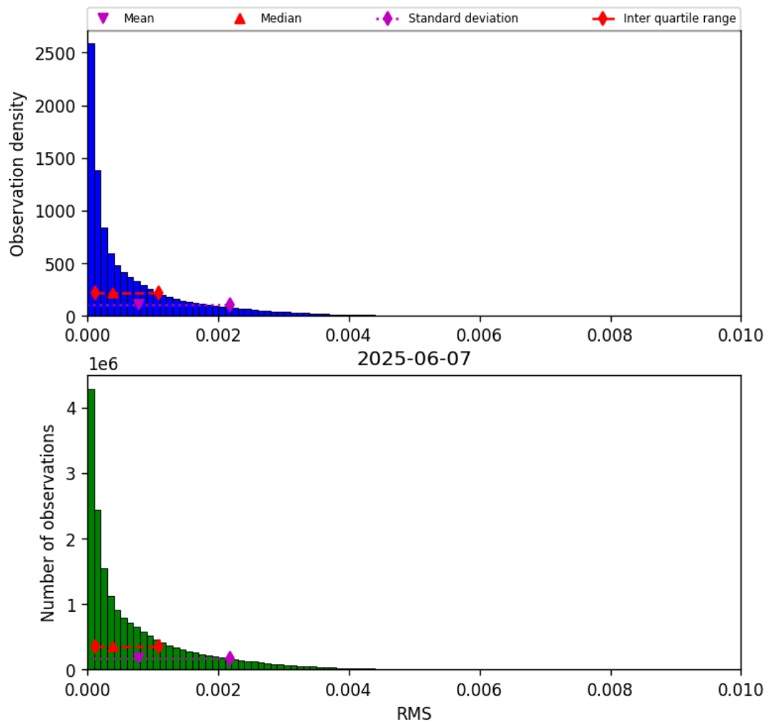
Figure 45: Histogram of “RMS” for 2025-06-07 to 2025-06-08
