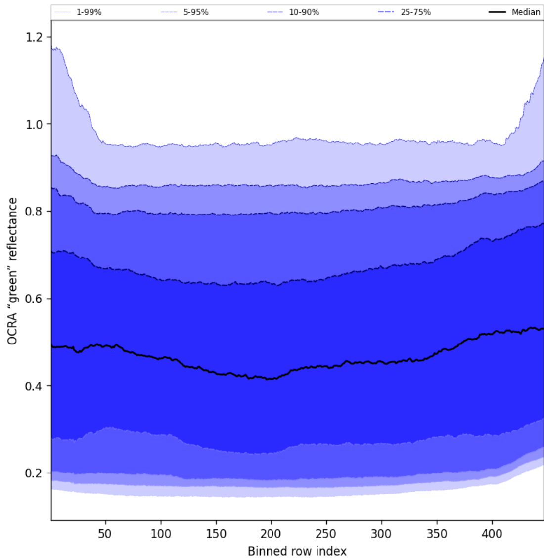
Figure 66: Along track statistics of "OCRA "green" reflectance" for 2025-06-07 to 2025-06-08
