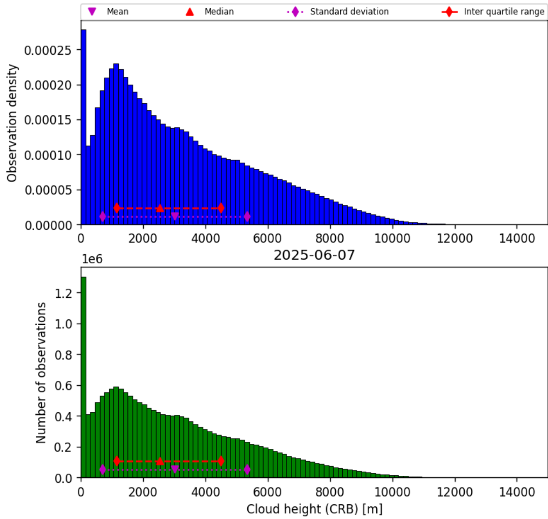
Figure 41: Histogram of “Cloud height (CRB)” for 2025-06-07 to 2025-06-08
