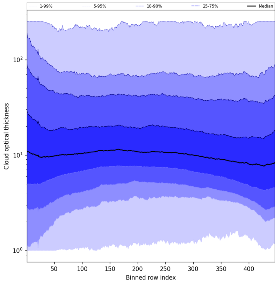
Figure 55: Along track statistics of “Cloud optical thickness” for 2025-06-07 to 2025-06-08
