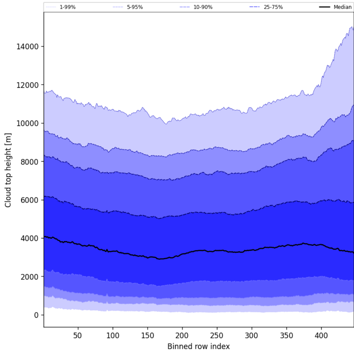
Figure 54: Along track statistics of “Cloud top height” for 2025-06-07 to 2025-06-08
