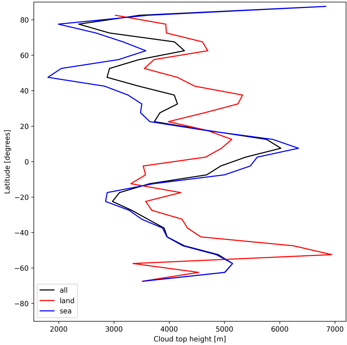
Figure 22: Zonal average of “Cloud top height” for 2025-06-07 to 2025-06-08.
