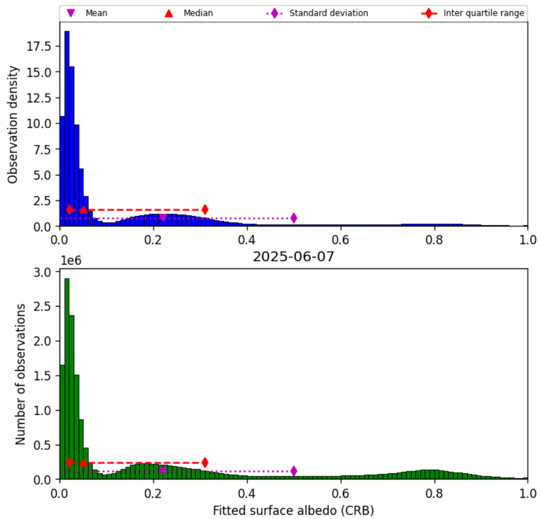
Figure 44: Histogram of “Fitted surface albedo (CRB)” for 2025-06-07 to 2025-06-08
