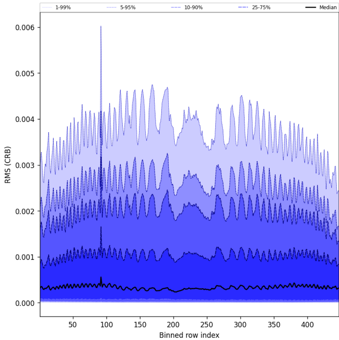
Figure 62: Along track statistics of “RMS (CRB)” for 2025-06-07 to 2025-06-08
