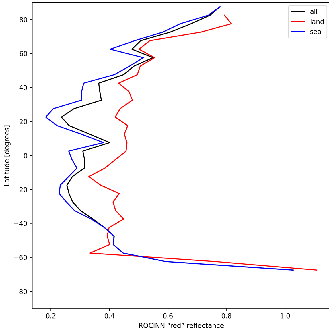
Figure 35: Zonal average of “ROCINN “red” reflectance” for 2025-06-07 to 2025-06-08.
