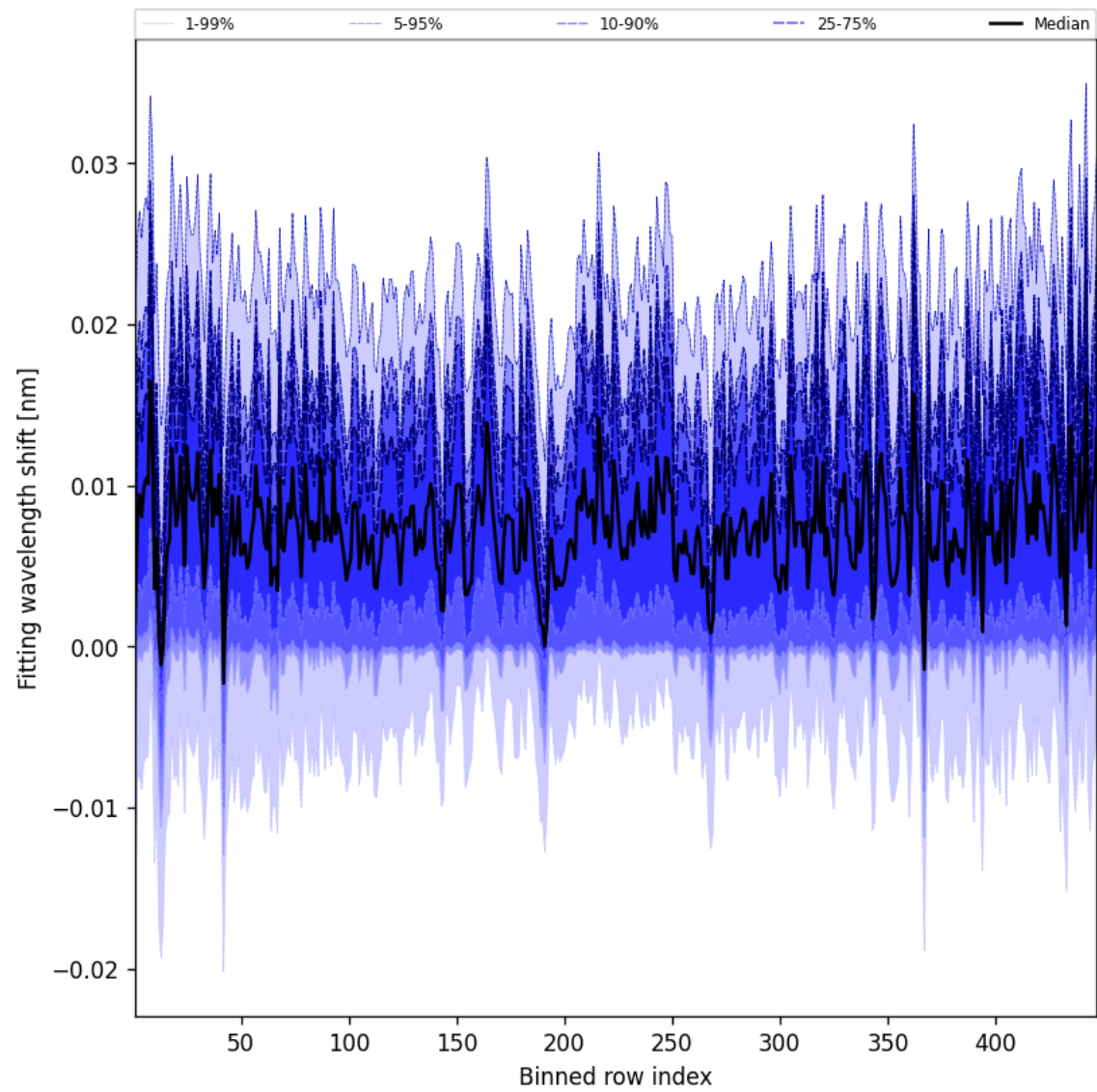
Figure 63: Along track statistics of “Fitting wavelength shift” for 2025-06-07 to 2025-06-08
