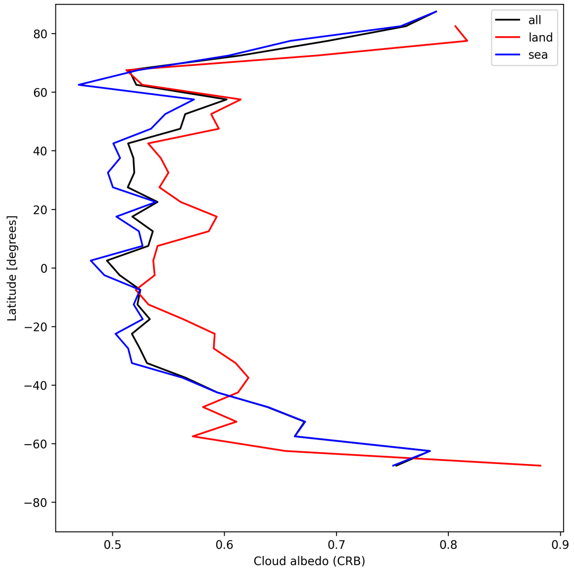
Figure 26: Zonal average of “Cloud albedo (CRB)” for 2025-06-07 to 2025-06-08.
