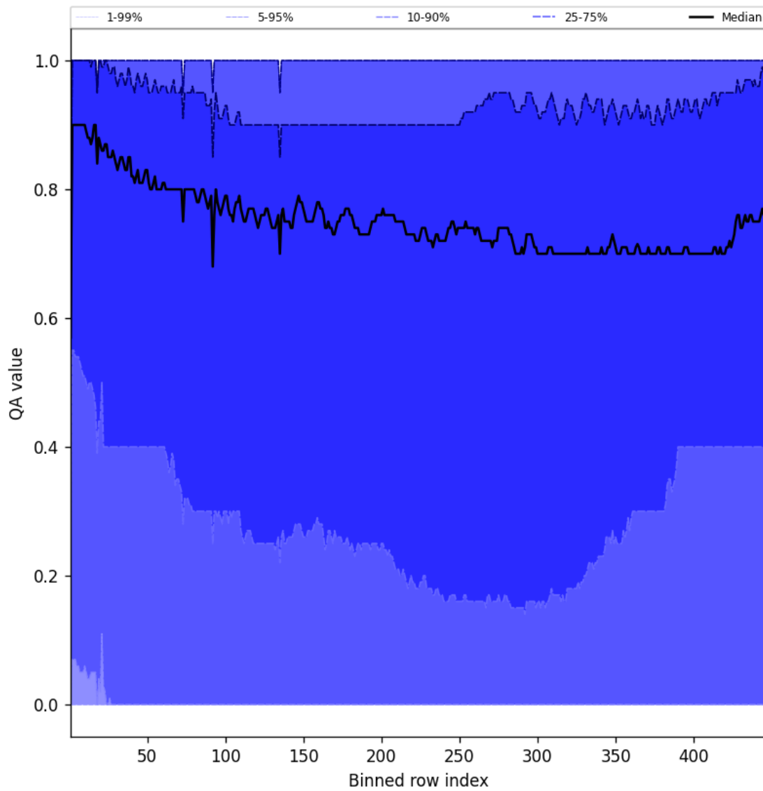
Figure 52: Along track statistics of “QA value” for 2025-06-07 to 2025-06-08
