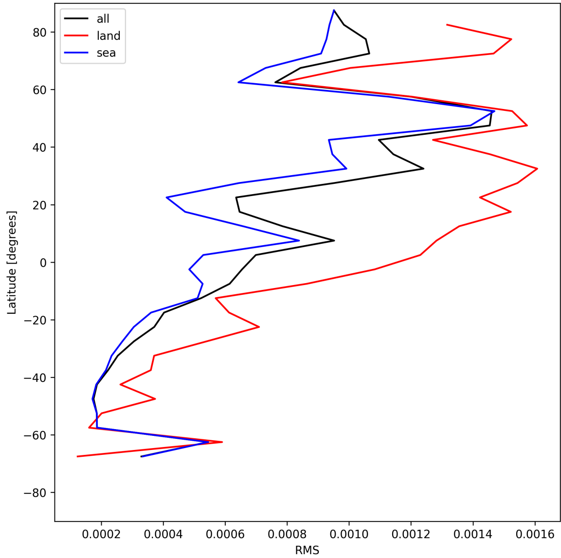
Figure 29: Zonal average of “RMS” for 2025-06-07 to 2025-06-08.
