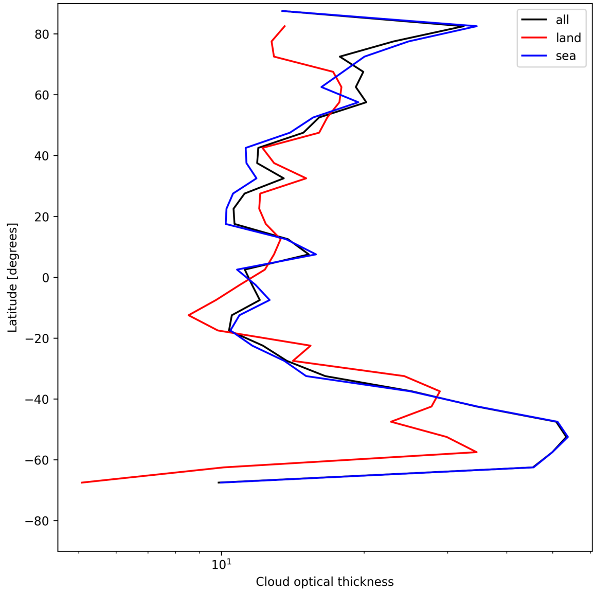
Figure 23: Zonal average of “Cloud optical thickness” for 2025-06-07 to 2025-06-08.
