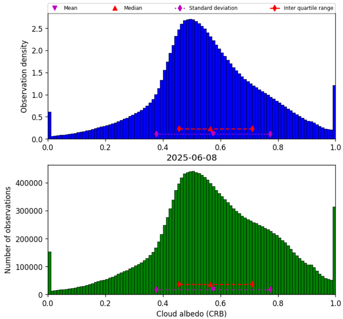
Figure 42: Histogram of “Cloud albedo (CRB)” for 2025-06-08 to 2025-06-09
