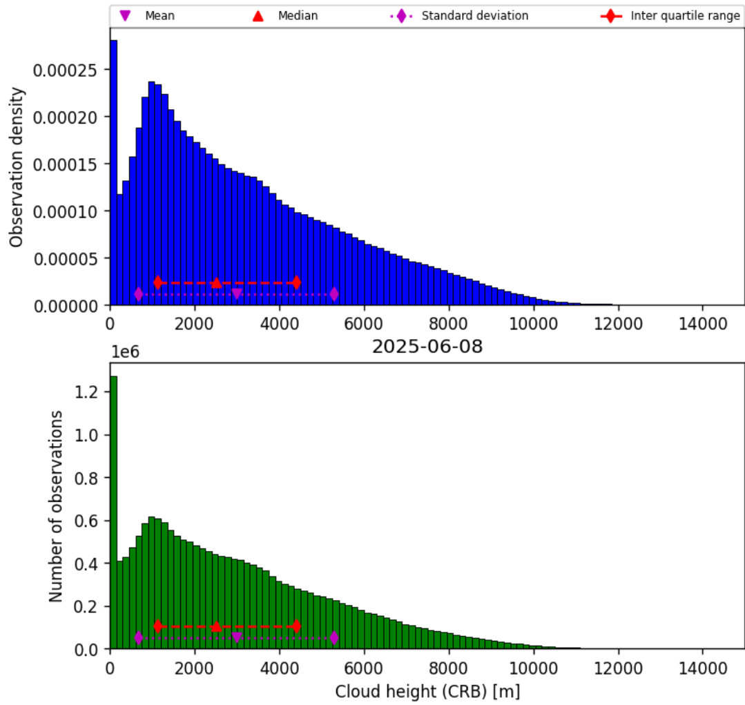
Figure 41: Histogram of “Cloud height (CRB)” for 2025-06-08 to 2025-06-09
