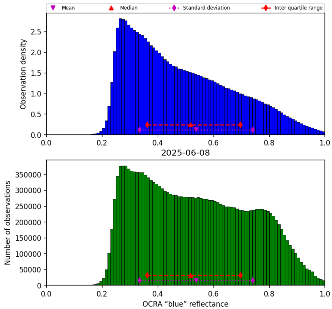
Figure 49: Histogram of “OCRA “blue” reflectance” for 2025-06-08 to 2025-06-09
