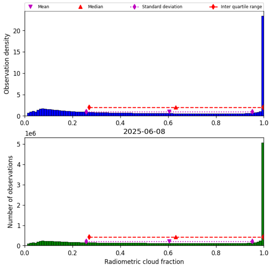
Figure 37: Histogram of “Radiometric cloud fraction” for 2025-06-08 to 2025-06-09
