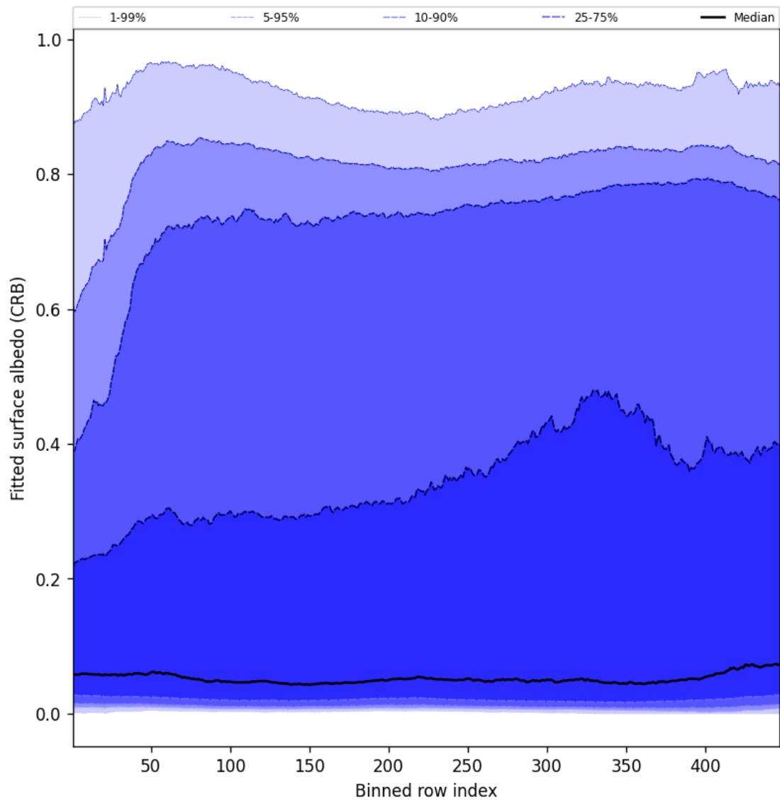
Figure 60: Along track statistics of “Fitted surface albedo (CRB)” for 2025-06-08 to 2025-06-09
