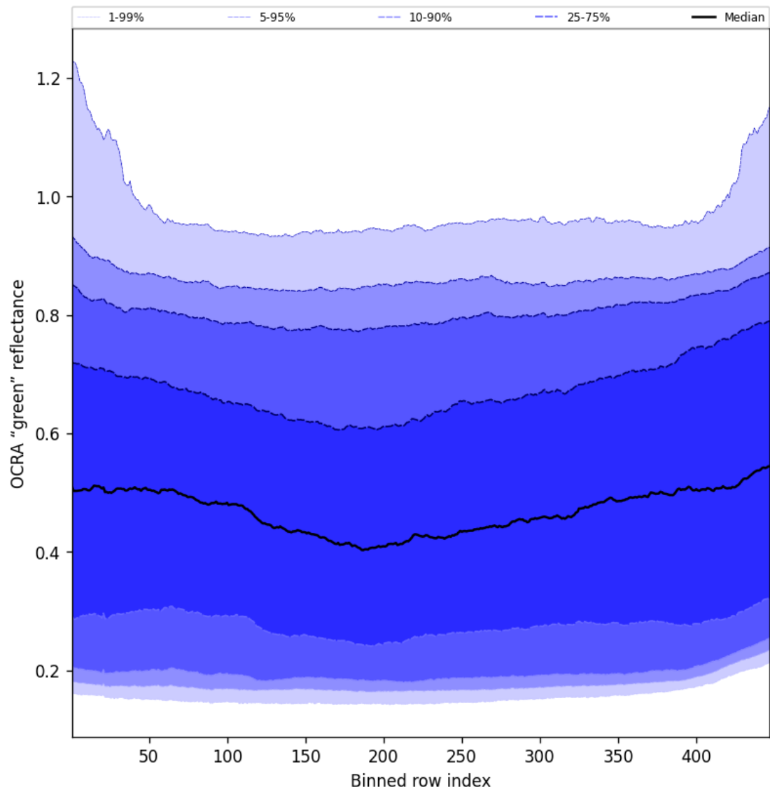
Figure 66: Along track statistics of "OCRA "green" reflectance" for 2025-06-08 to 2025-06-09
