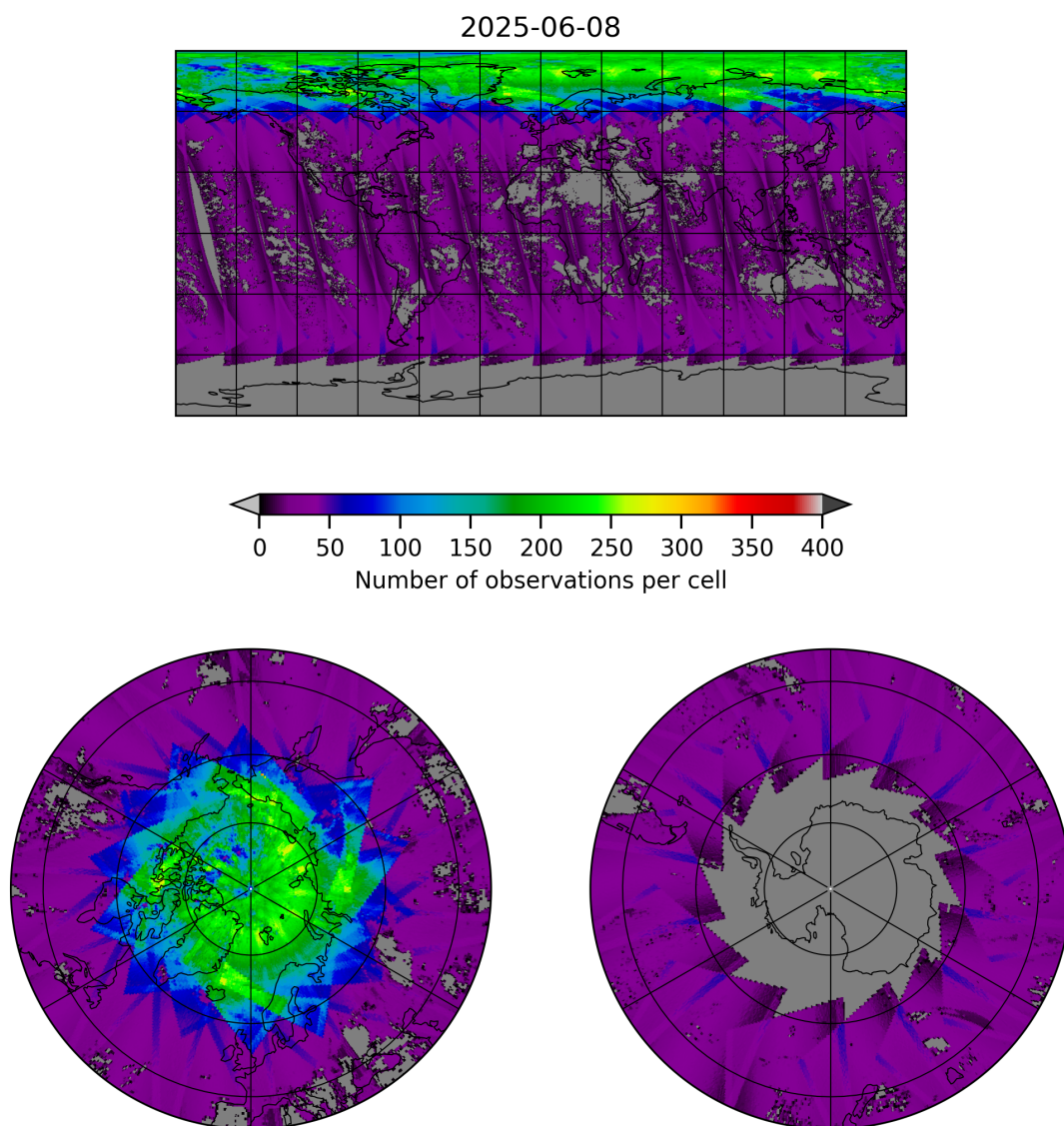
Figure 19: Map of the number of observations for 2025-06-08 to 2025-06-09
