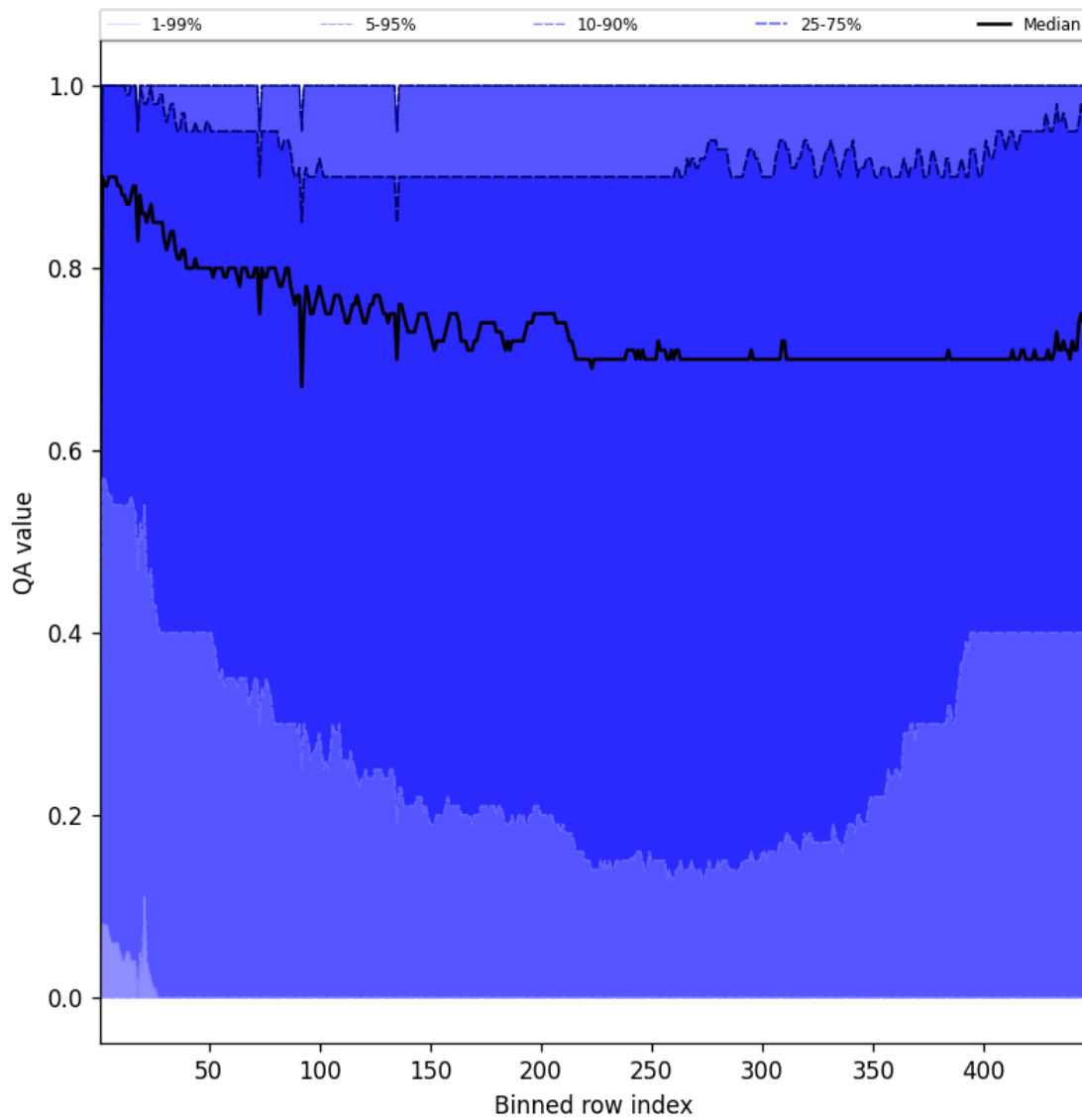
Figure 52: Along track statistics of “QA value” for 2025-06-08 to 2025-06-09
