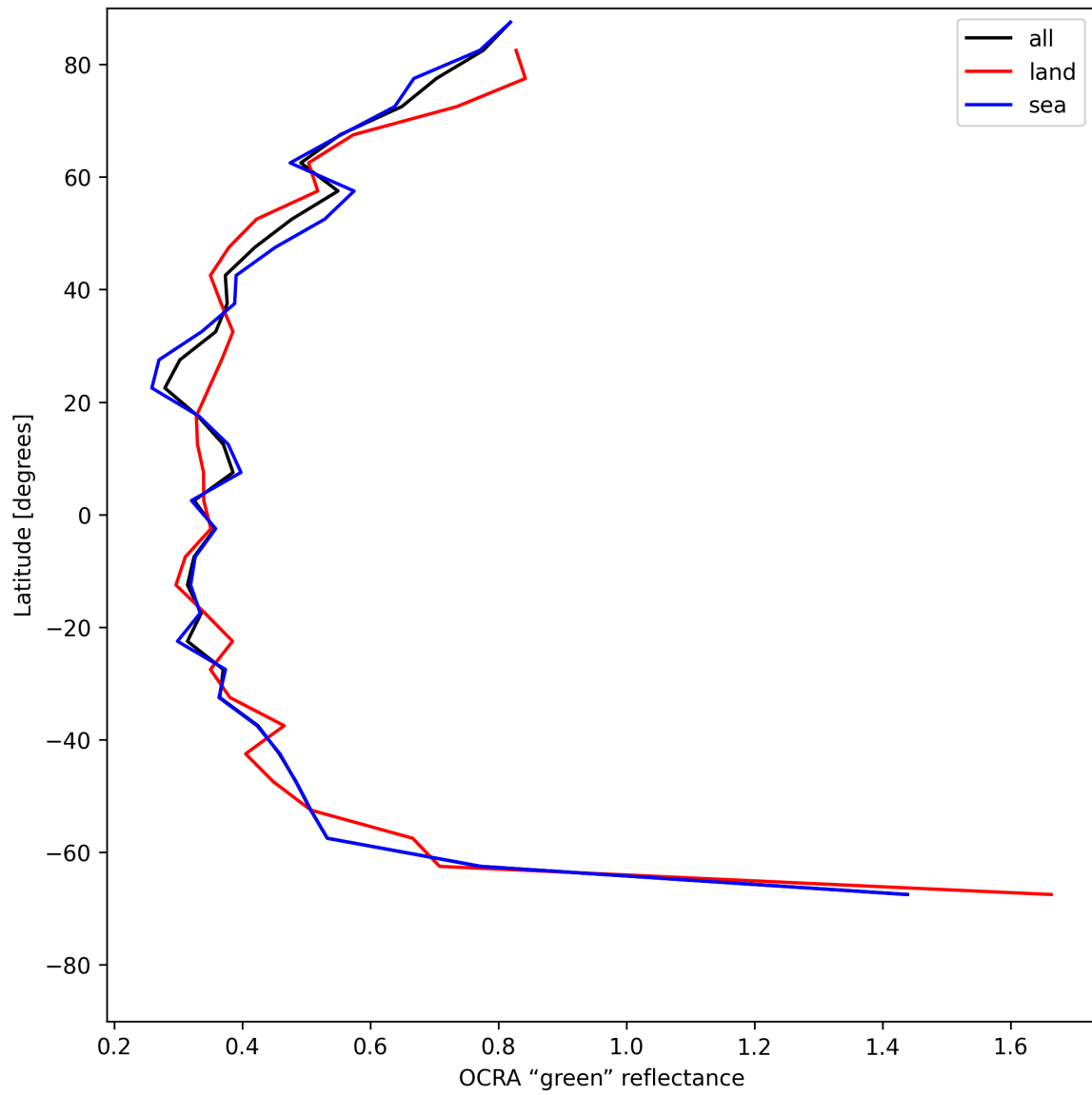
Figure 34: Zonal average of “OCRA “green” reflectance” for 2025-06-08 to 2025-06-09.
