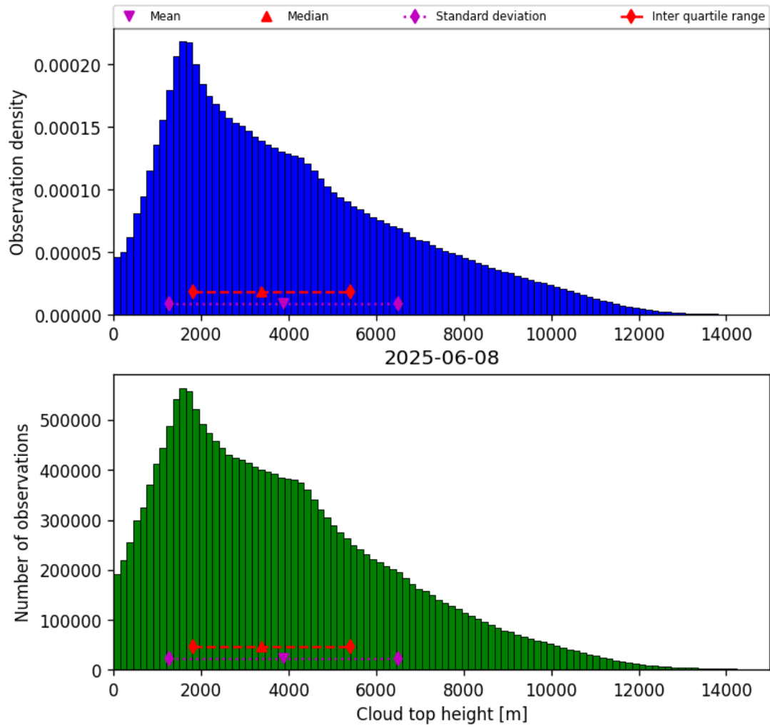
Figure 38: Histogram of “Cloud top height” for 2025-06-08 to 2025-06-09
