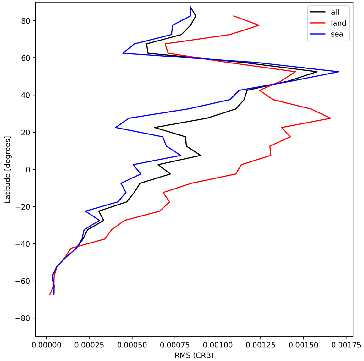
Figure 30: Zonal average of “RMS (CRB)” for 2025-06-08 to 2025-06-09.
