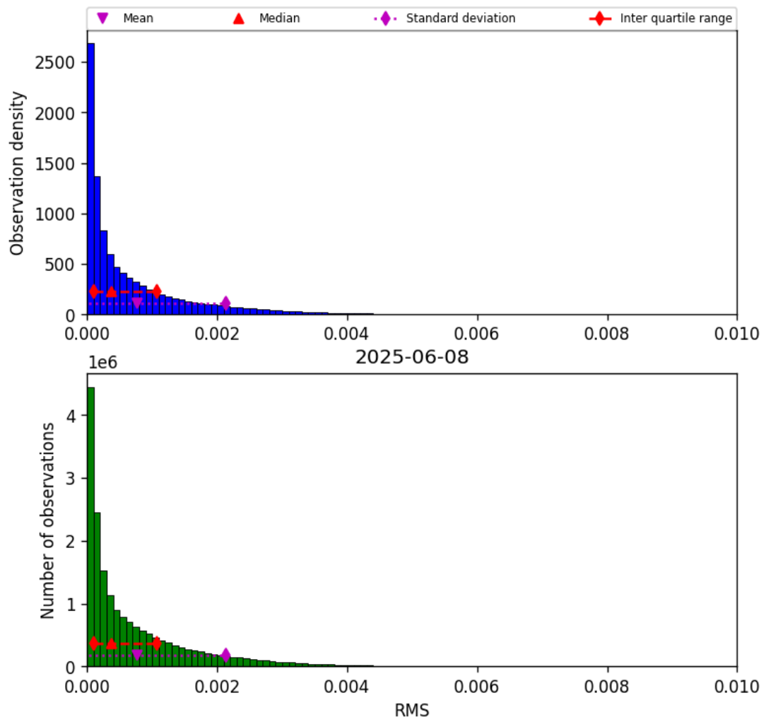
Figure 45: Histogram of “RMS” for 2025-06-08 to 2025-06-09
