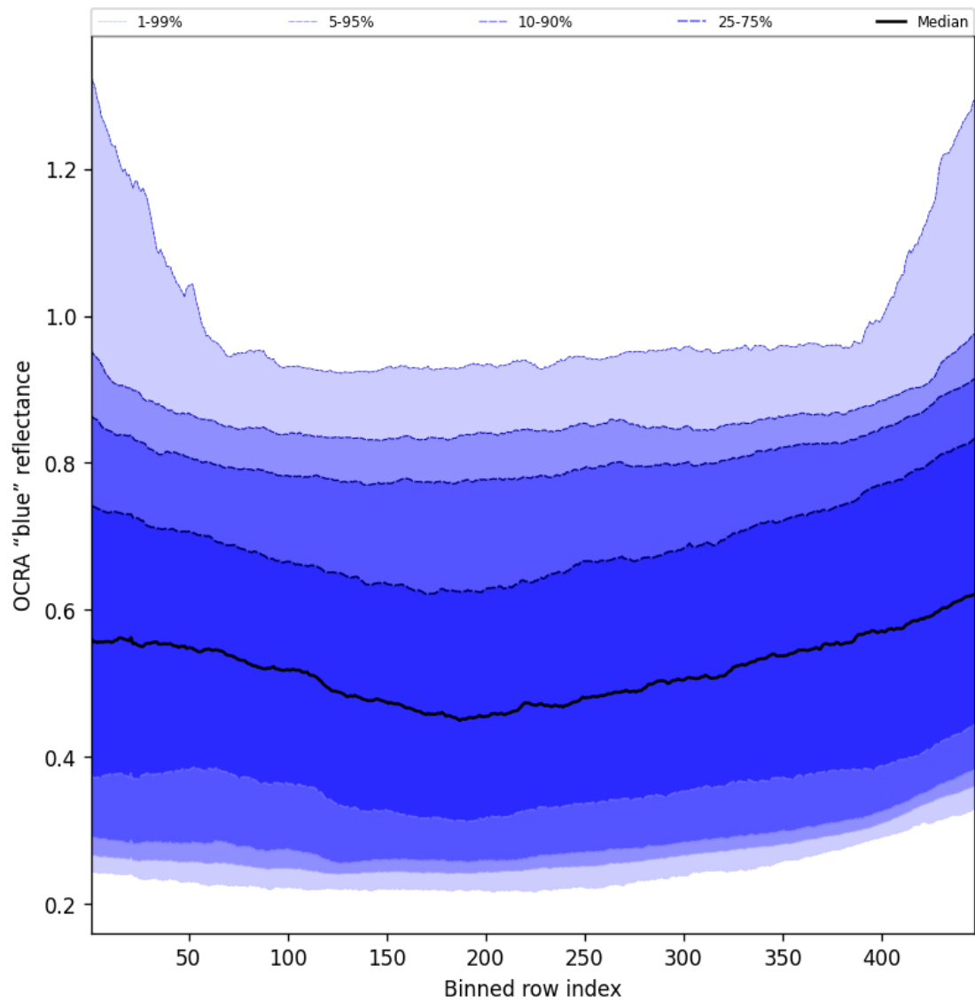
Figure 65: Along track statistics of “OCRA “blue” reflectance” for 2025-06-08 to 2025-06-09
