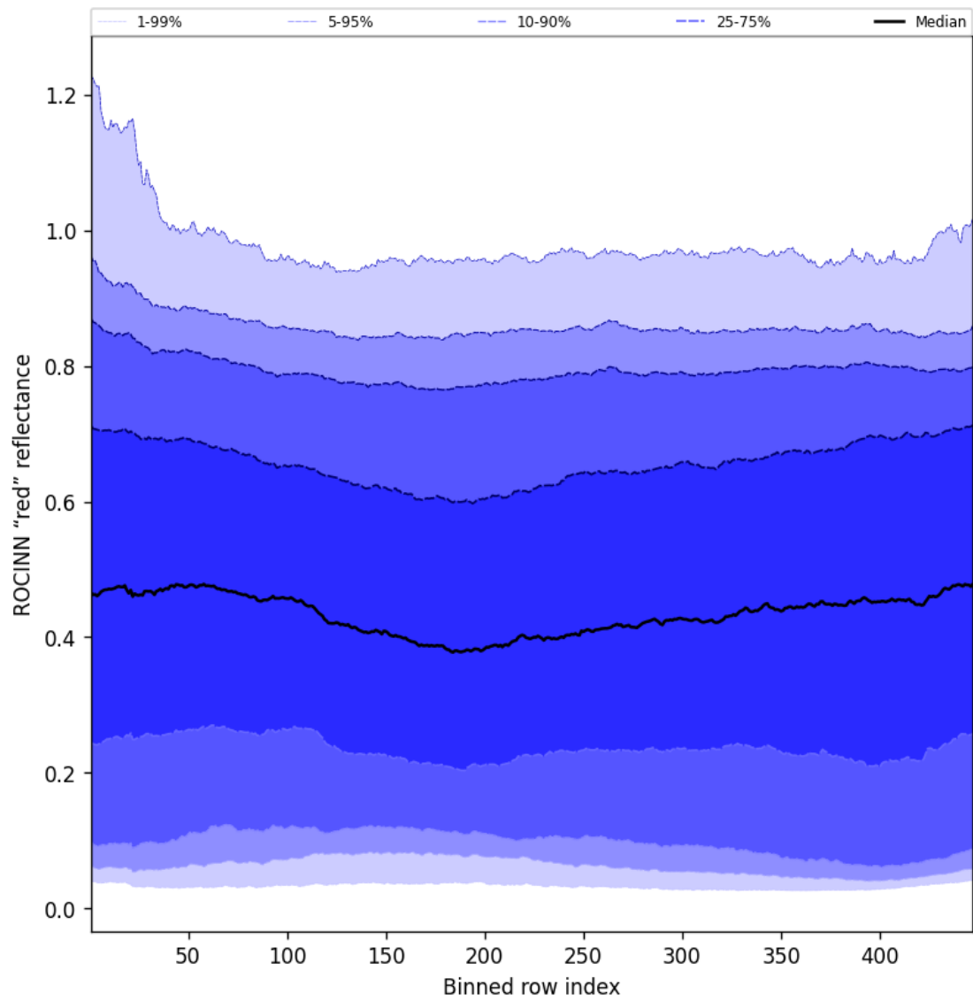
Figure 67: Along track statistics of “ROCINN “red” reflectance” for 2025-06-08 to 2025-06-09
