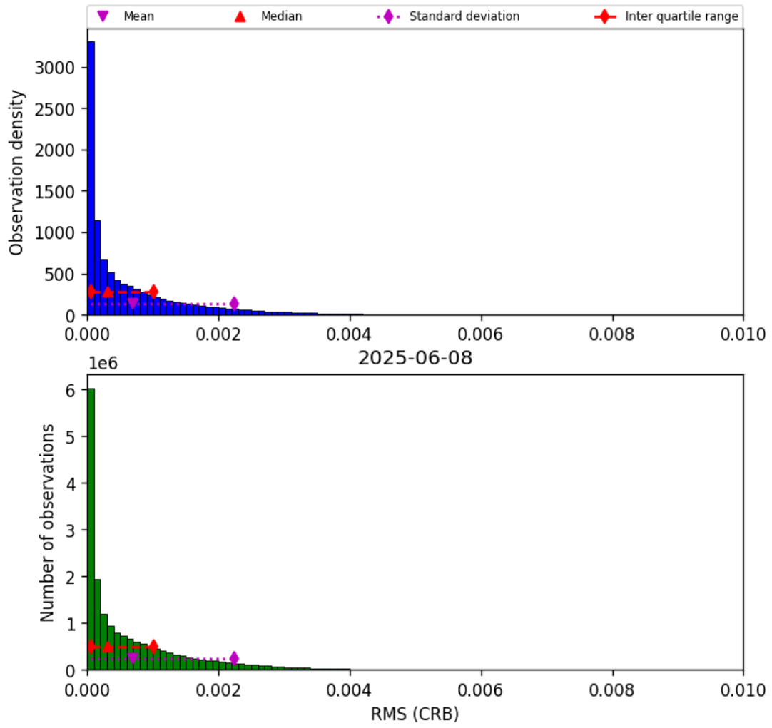
Figure 46: Histogram of "RMS (CRB)" for 2025-06-08 to 2025-06-09
