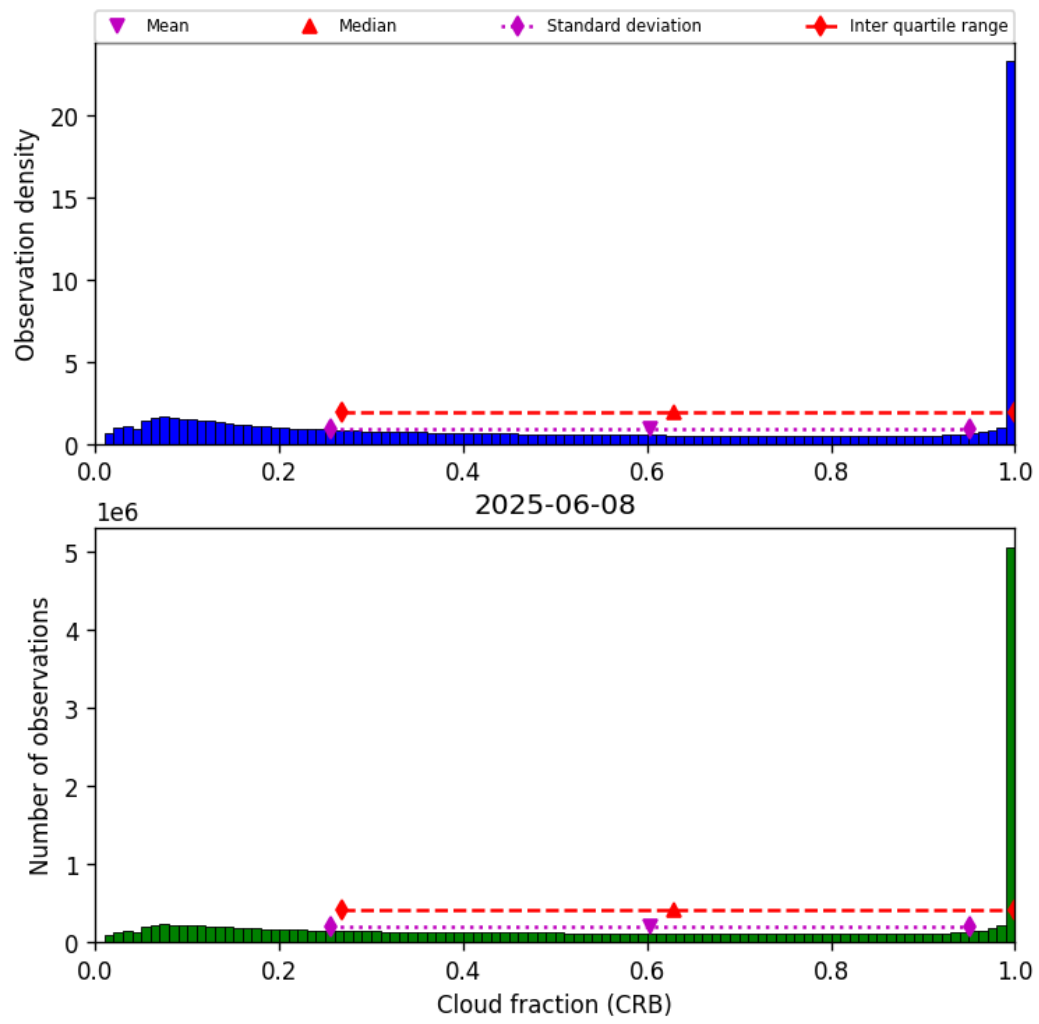
Figure 40: Histogram of “Cloud fraction (CRB)” for 2025-06-08 to 2025-06-09
