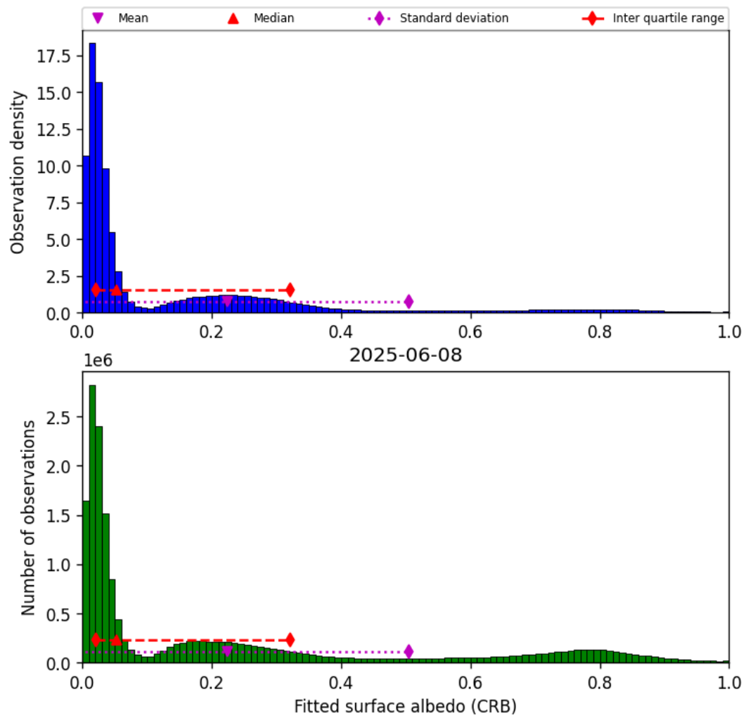
Figure 44: Histogram of “Fitted surface albedo (CRB)” for 2025-06-08 to 2025-06-09
