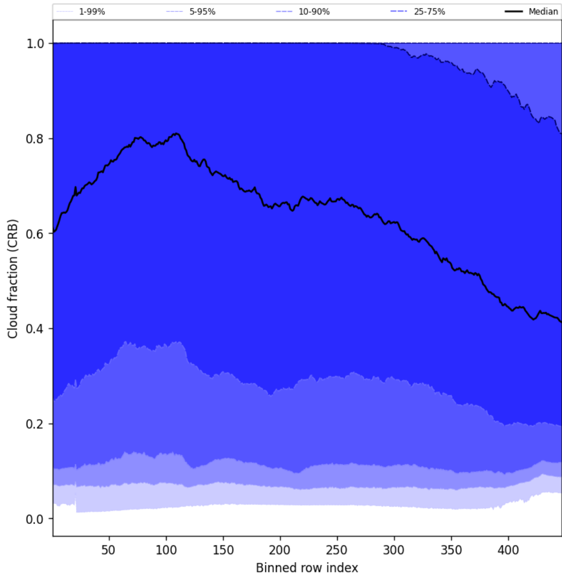
Figure 56: Along track statistics of “Cloud fraction (CRB)” for 2025-06-08 to 2025-06-09
