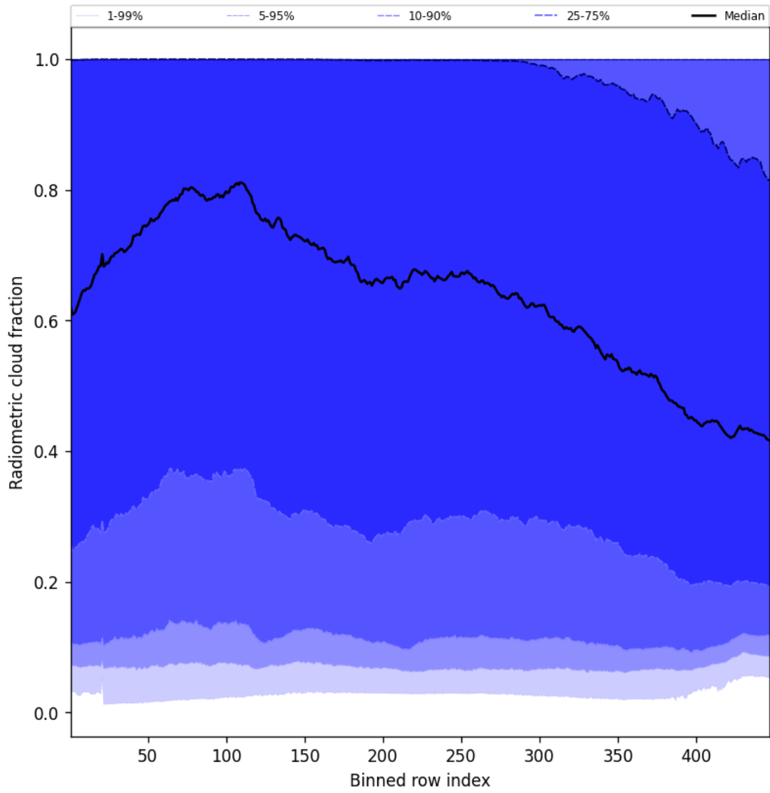
Figure 53: Along track statistics of “Radiometric cloud fraction” for 2025-06-08 to 2025-06-09
