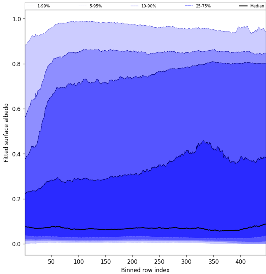
Figure 59: Along track statistics of “Fitted surface albedo” for 2025-06-08 to 2025-06-09
