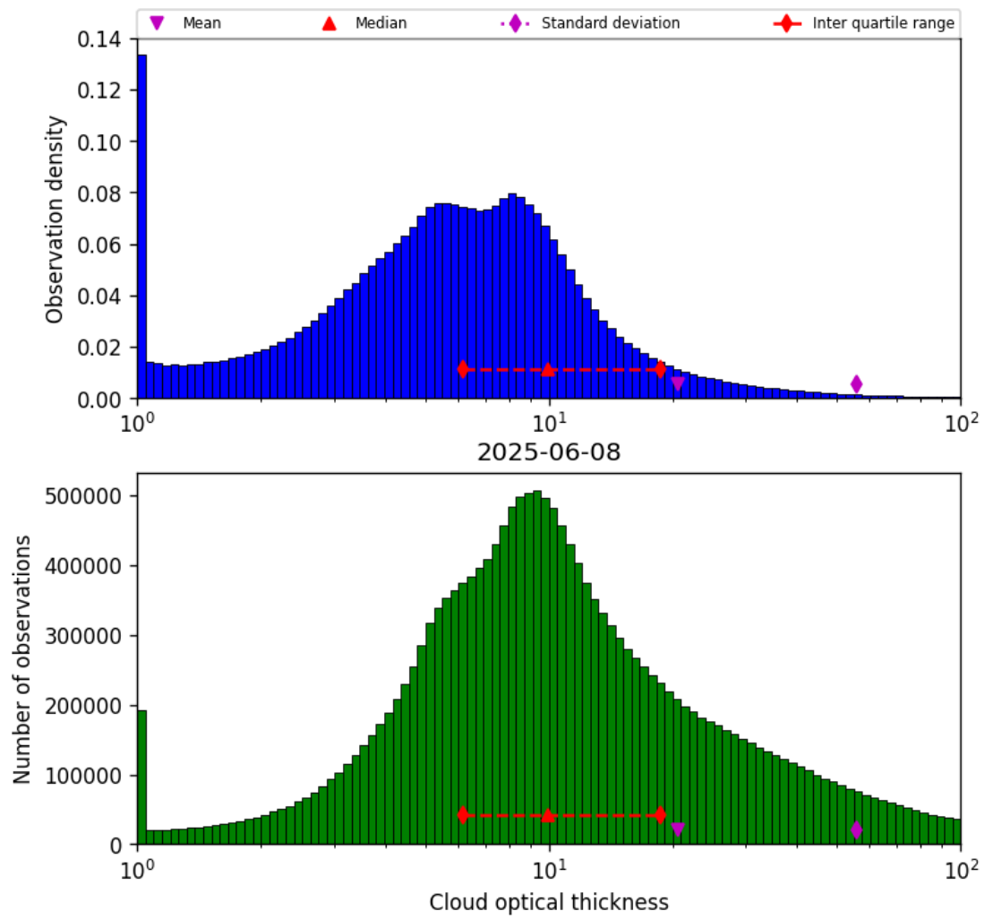
Figure 39: Histogram of “Cloud optical thickness” for 2025-06-08 to 2025-06-09
