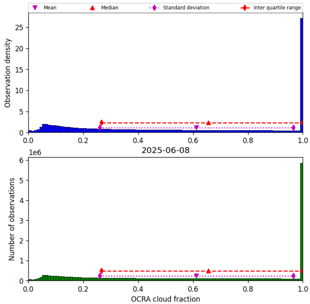
Figure 48: Histogram of “OCRA cloud fraction” for 2025-06-08 to 2025-06-09
