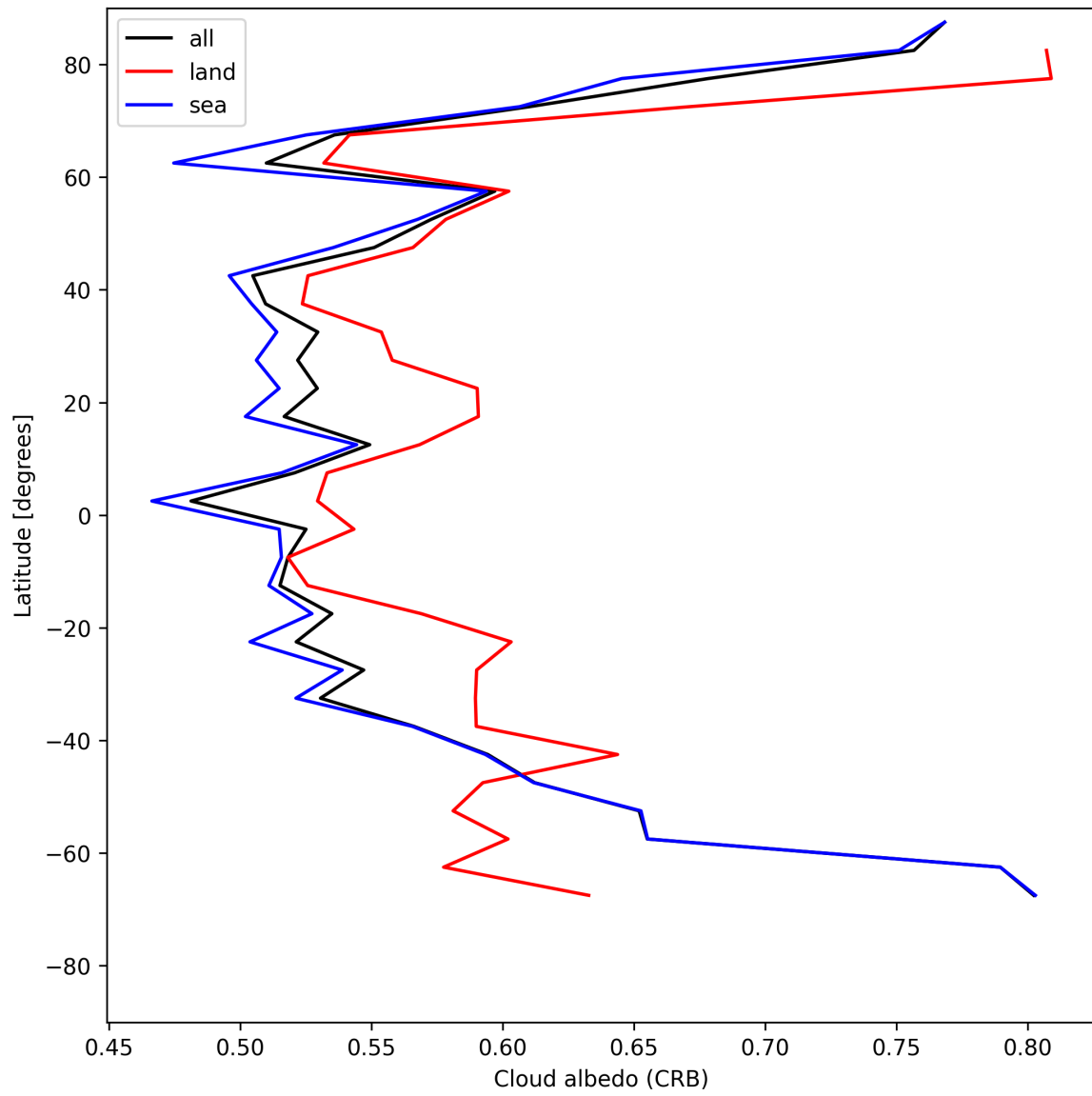
Figure 26: Zonal average of “Cloud albedo (CRB)” for 2025-06-08 to 2025-06-09.
