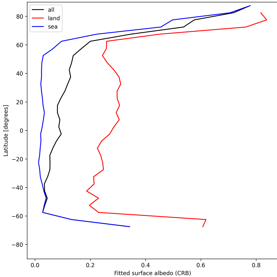
Figure 28: Zonal average of “Fitted surface albedo (CRB)” for 2025-06-08 to 2025-06-09.
