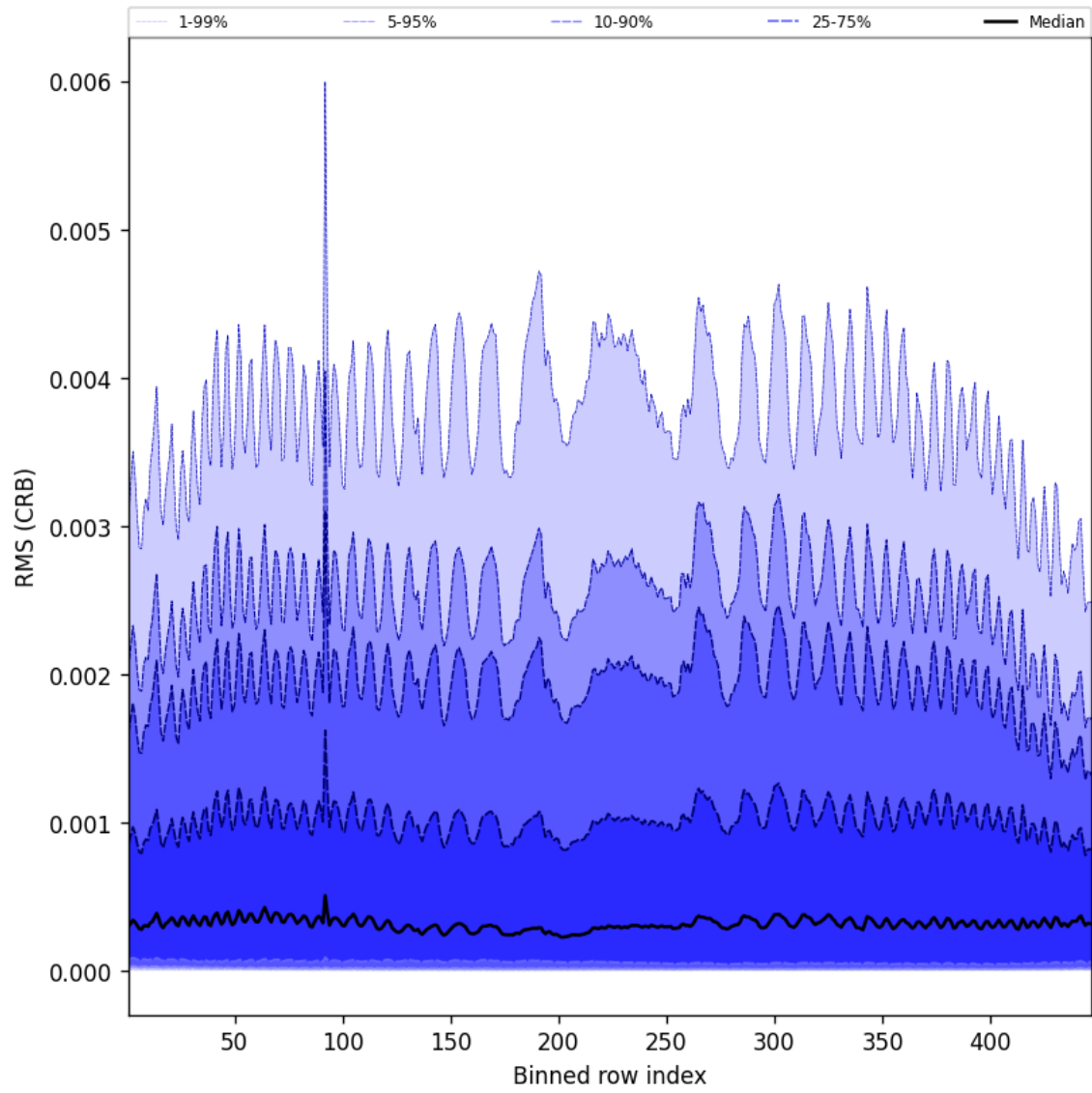
Figure 62: Along track statistics of “RMS (CRB)” for 2025-06-08 to 2025-06-09
