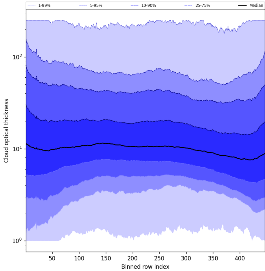
Figure 55: Along track statistics of “Cloud optical thickness” for 2025-06-08 to 2025-06-09
