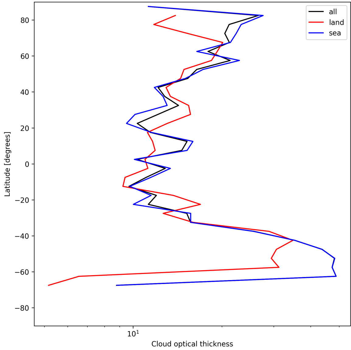
Figure 23: Zonal average of “Cloud optical thickness” for 2025-06-08 to 2025-06-09.
