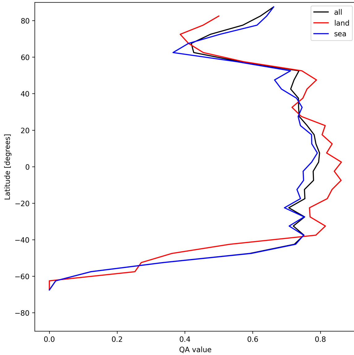
Figure 20: Zonal average of “QA value” for 2025-06-08 to 2025-06-09.
