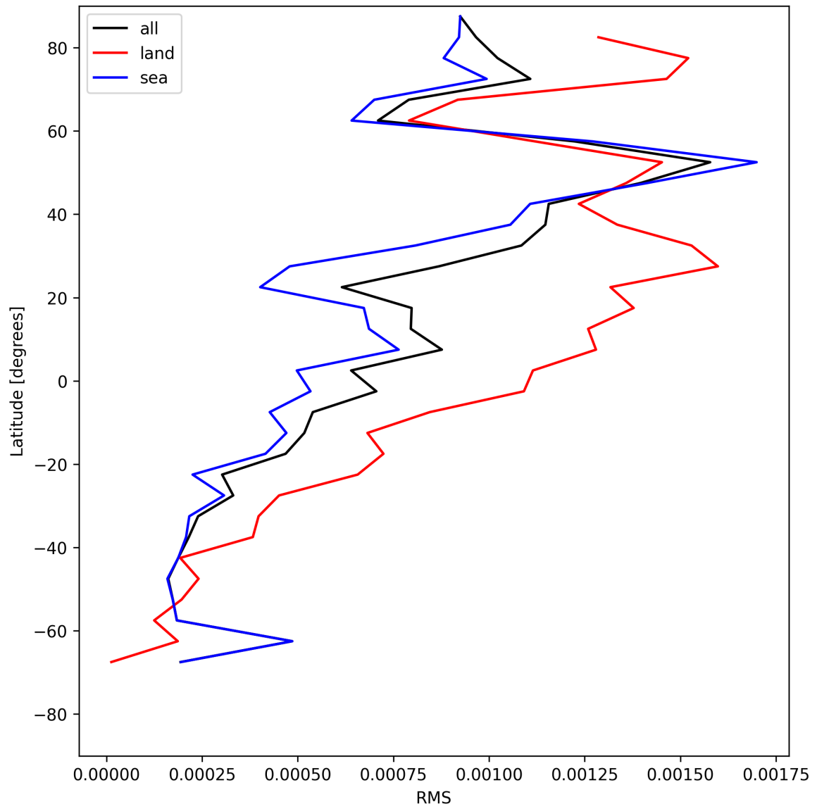
Figure 29: Zonal average of “RMS” for 2025-06-08 to 2025-06-09.
