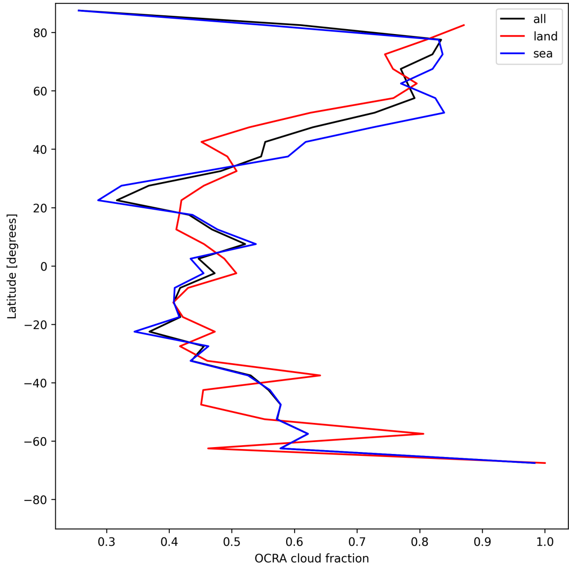
Figure 32: Zonal average of “OCRA cloud fraction” for 2025-06-08 to 2025-06-09.
