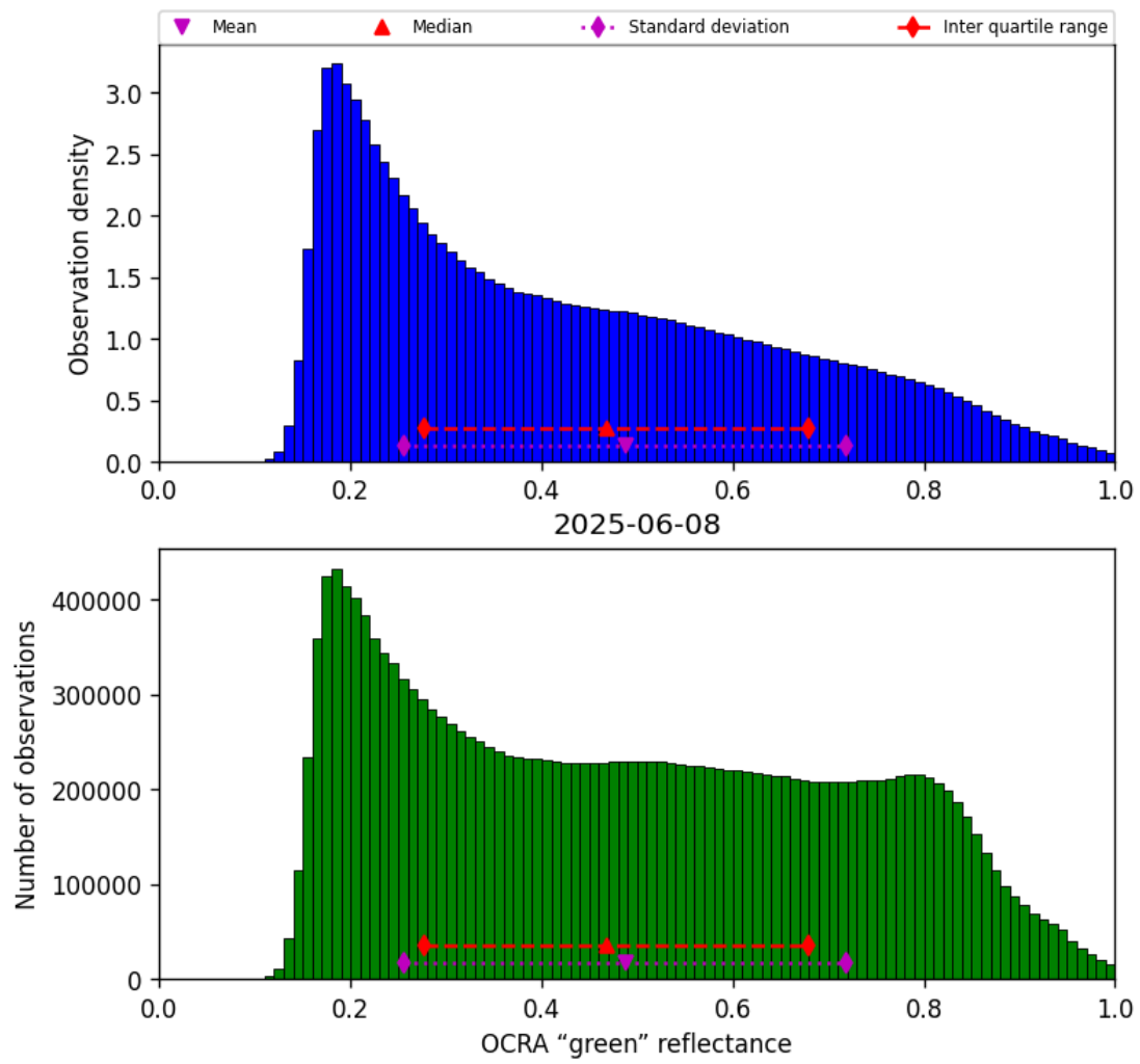
Figure 50: Histogram of “OCRA “green” reflectance” for 2025-06-08 to 2025-06-09
