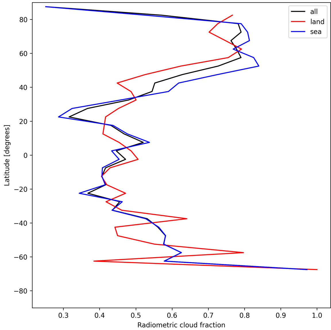
Figure 21: Zonal average of “Radiometric cloud fraction” for 2025-06-08 to 2025-06-09.
