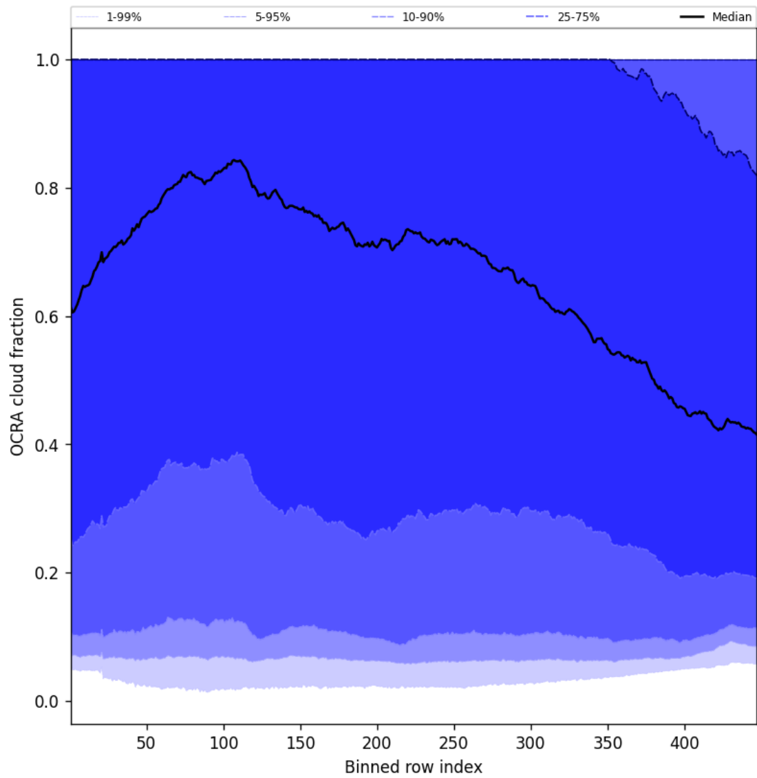
Figure 64: Along track statistics of “OCRA cloud fraction” for 2025-06-08 to 2025-06-09
