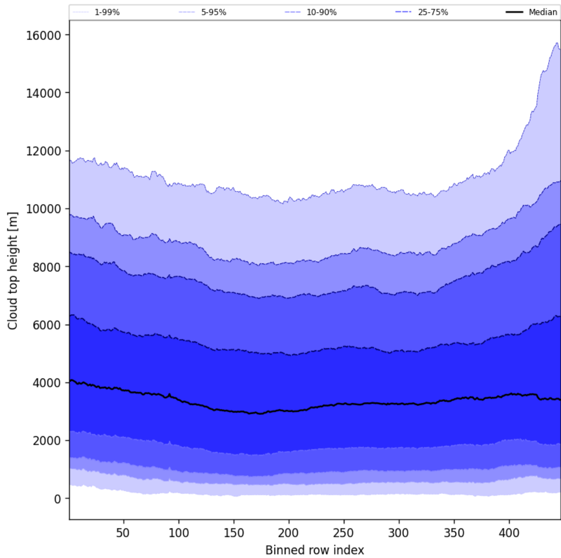
Figure 54: Along track statistics of “Cloud top height” for 2025-06-08 to 2025-06-09
