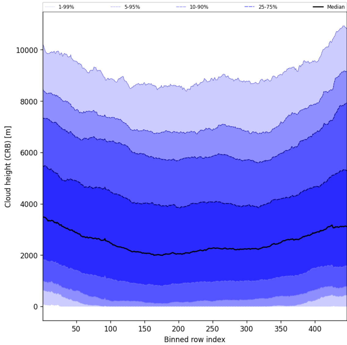
Figure 57: Along track statistics of “Cloud height (CRB)” for 2025-06-08 to 2025-06-09
