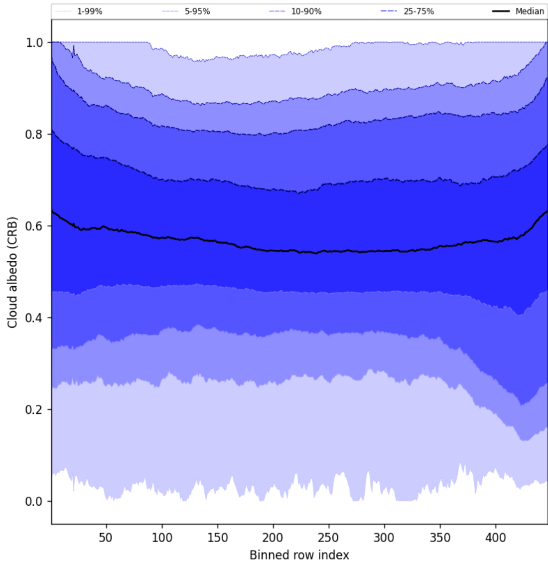
Figure 58: Along track statistics of “Cloud albedo (CRB)” for 2025-06-08 to 2025-06-09
