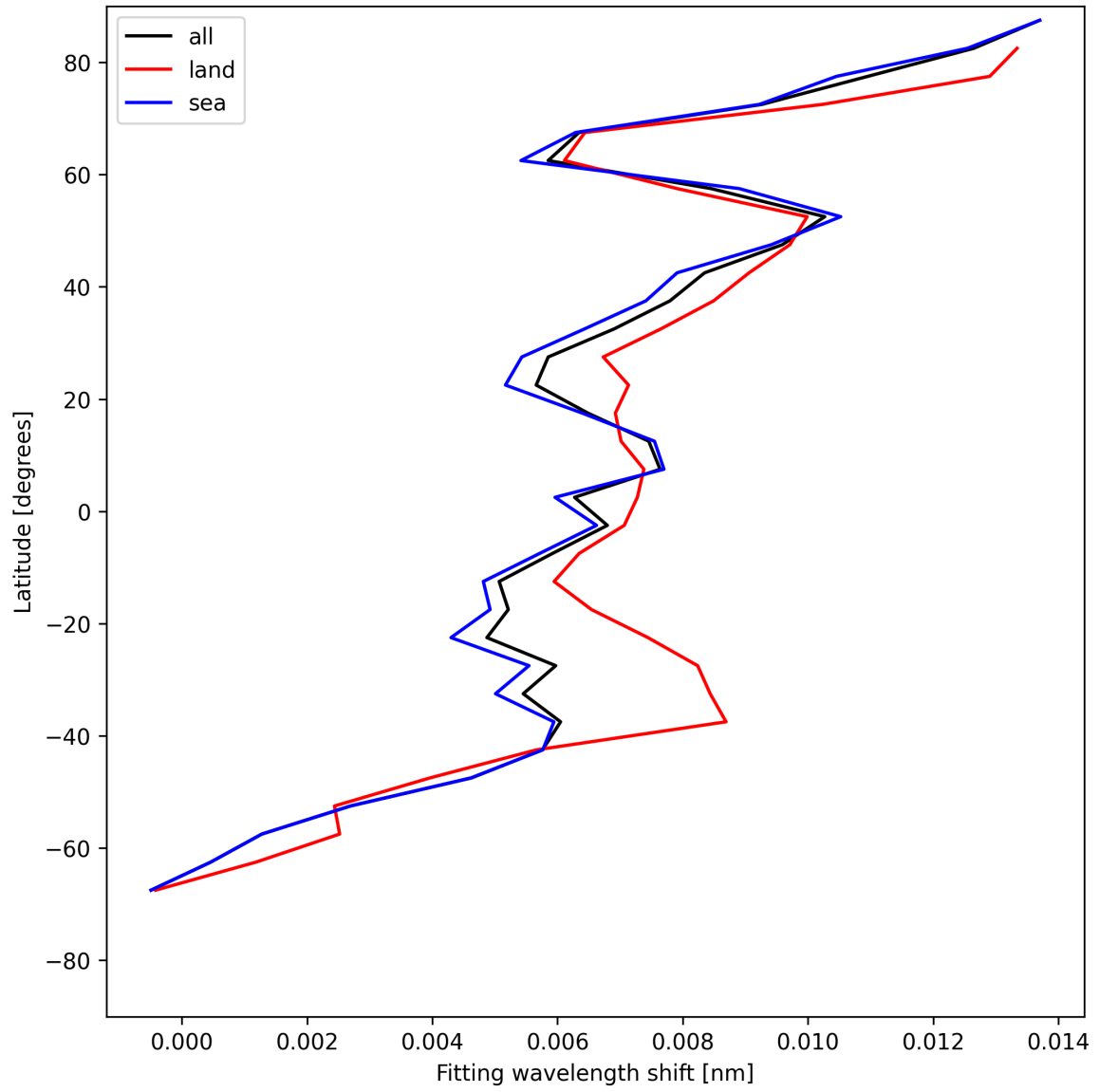
Figure 31: Zonal average of “Fitting wavelength shift” for 2025-06-08 to 2025-06-09.
