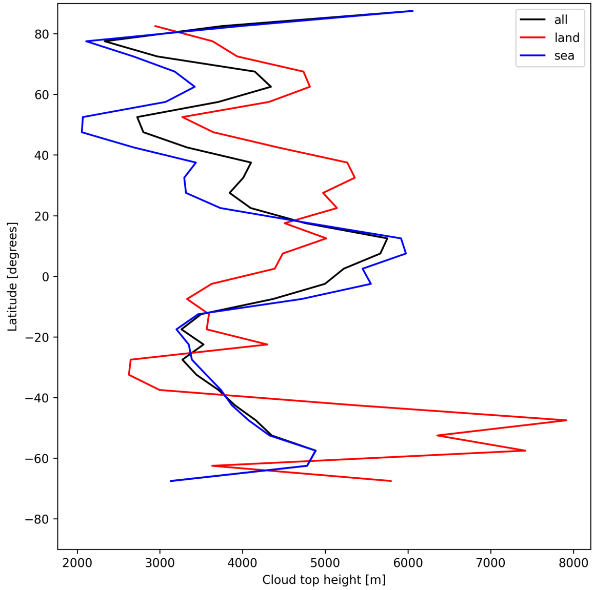
Figure 22: Zonal average of “Cloud top height” for 2025-06-08 to 2025-06-09.
