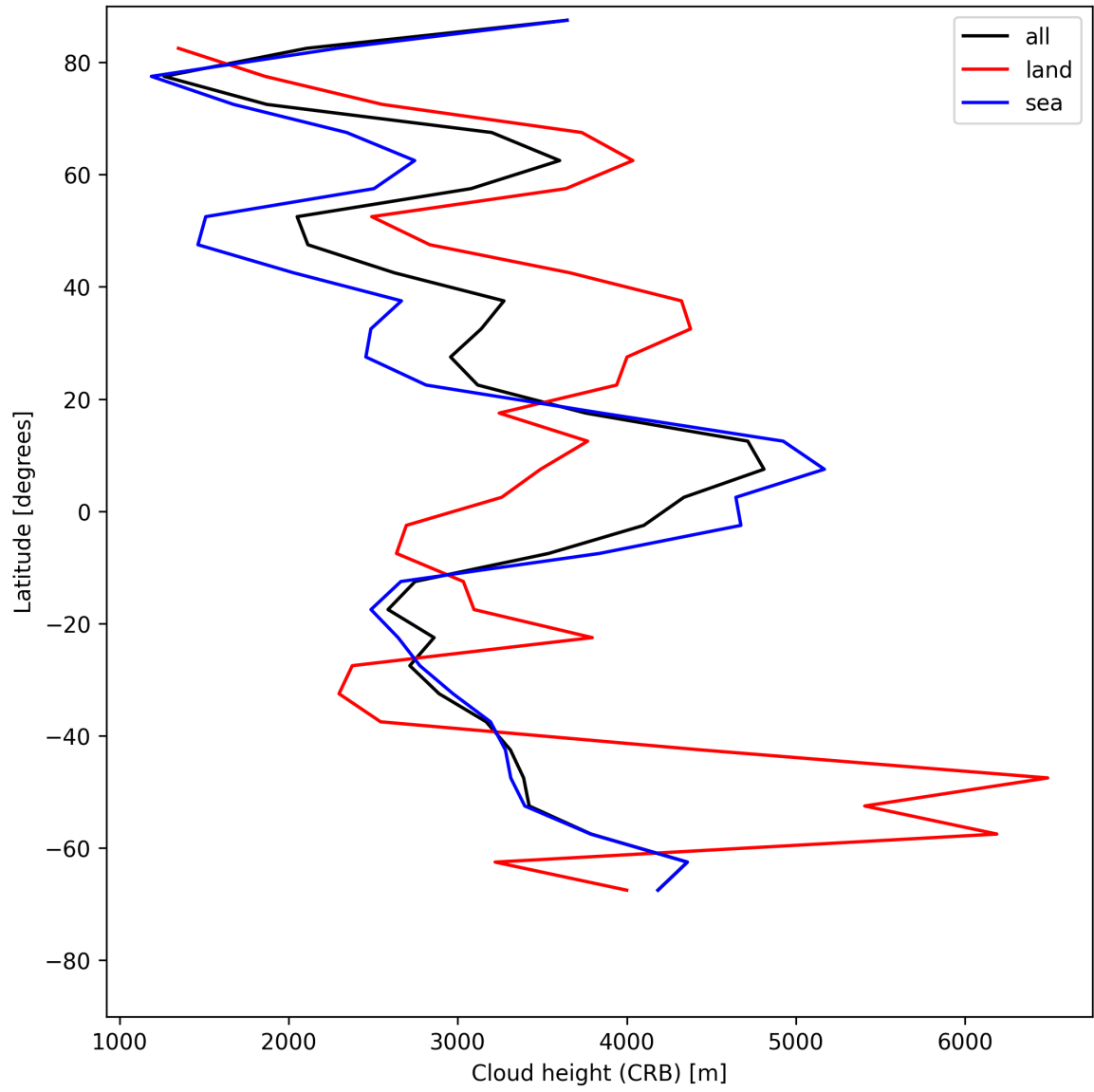
Figure 25: Zonal average of “Cloud height (CRB)” for 2025-06-08 to 2025-06-09.
