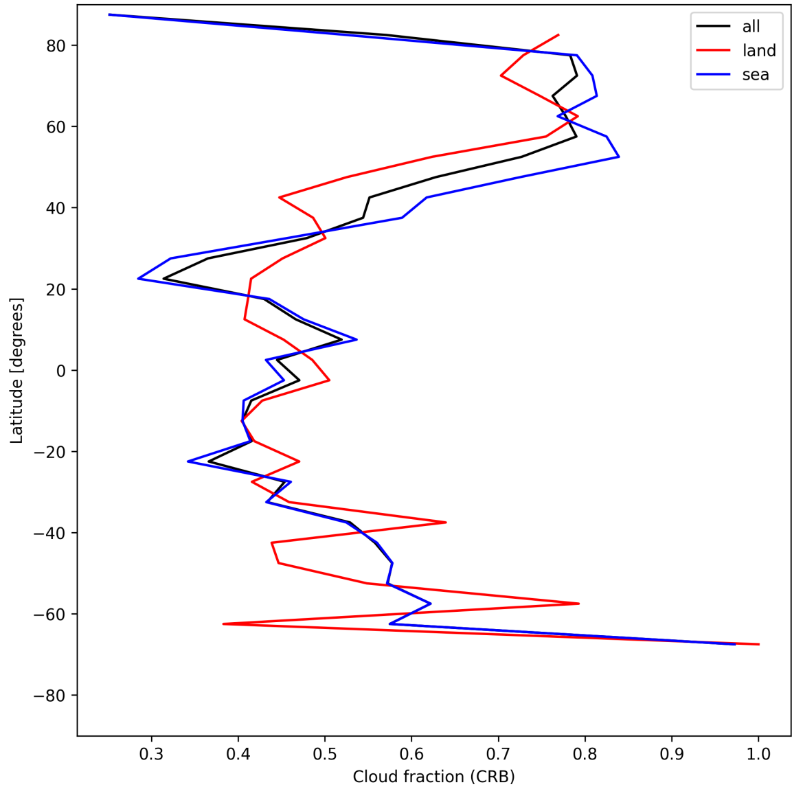
Figure 24: Zonal average of “Cloud fraction (CRB)” for 2025-06-08 to 2025-06-09.
