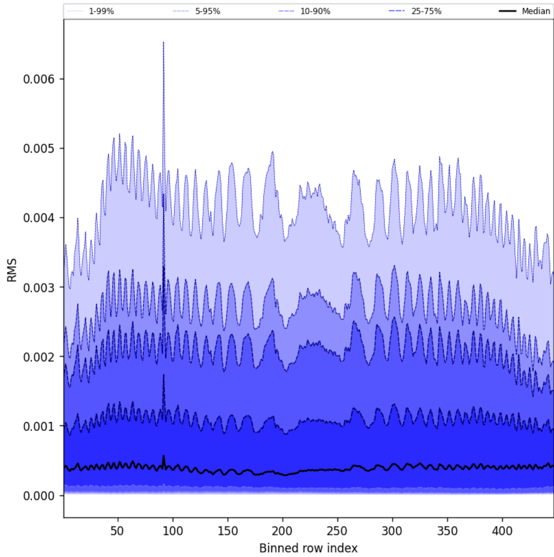
Figure 61: Along track statistics of “RMS” for 2025-06-08 to 2025-06-09
