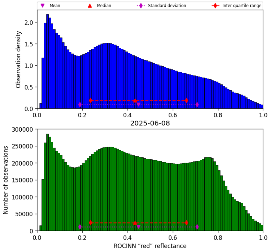
Figure 51: Histogram of “ROCINN “red” reflectance” for 2025-06-08 to 2025-06-09
