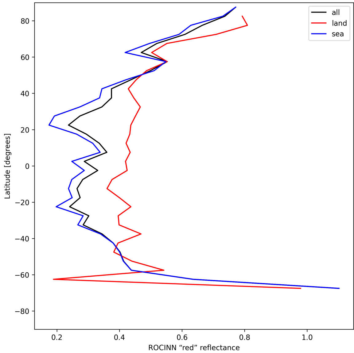
Figure 35: Zonal average of “ROCINN “red” reflectance” for 2025-06-08 to 2025-06-09.
