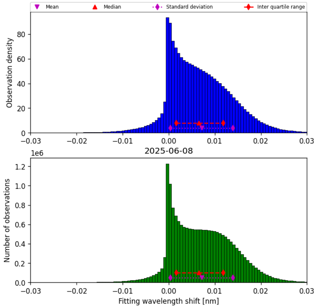
Figure 47: Histogram of “Fitting wavelength shift” for 2025-06-08 to 2025-06-09
