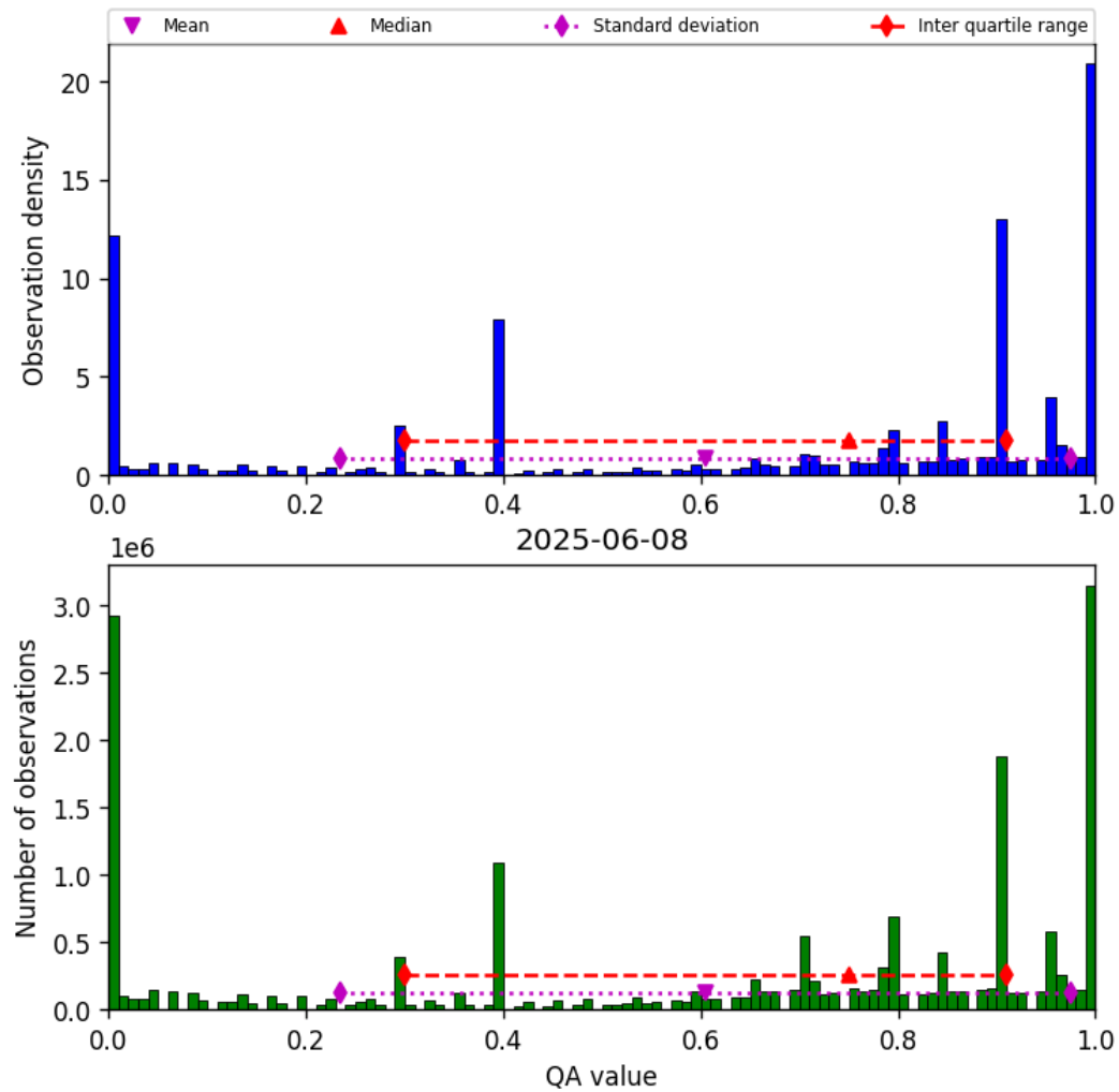
Figure 36: Histogram of “QA value” for 2025-06-08 to 2025-06-09
