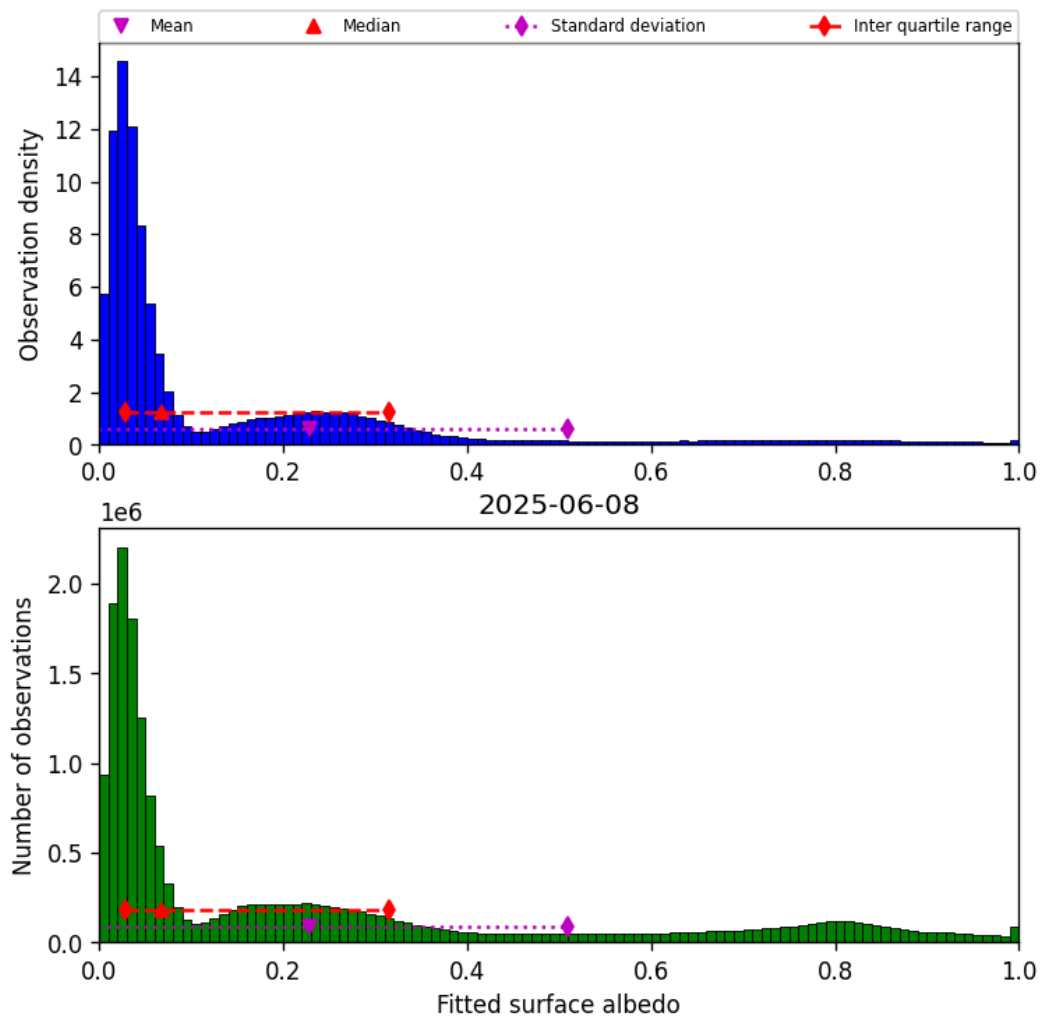
Figure 43: Histogram of “Fitted surface albedo” for 2025-06-08 to 2025-06-09
