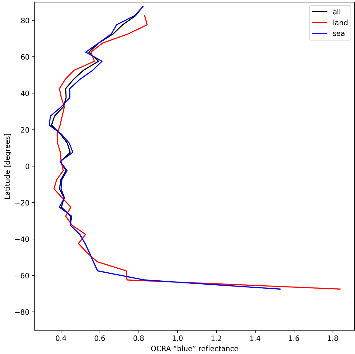
Figure 33: Zonal average of “OCRA “blue” reflectance” for 2025-06-08 to 2025-06-09.
