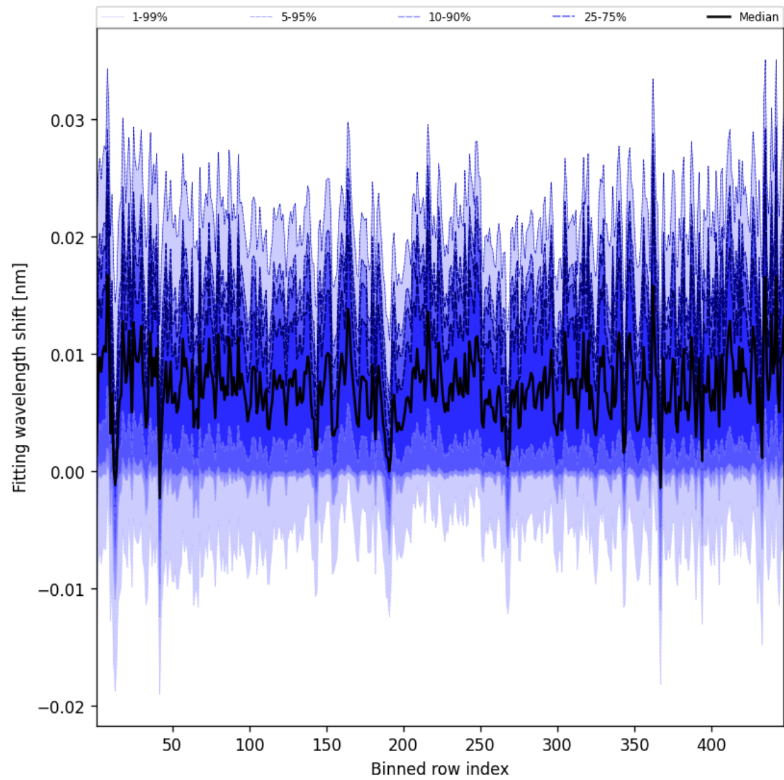
Figure 63: Along track statistics of “Fitting wavelength shift” for 2025-06-08 to 2025-06-09
