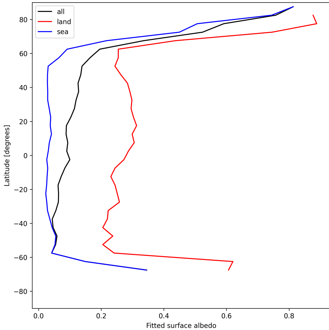
Figure 27: Zonal average of “Fitted surface albedo” for 2025-06-08 to 2025-06-09.
