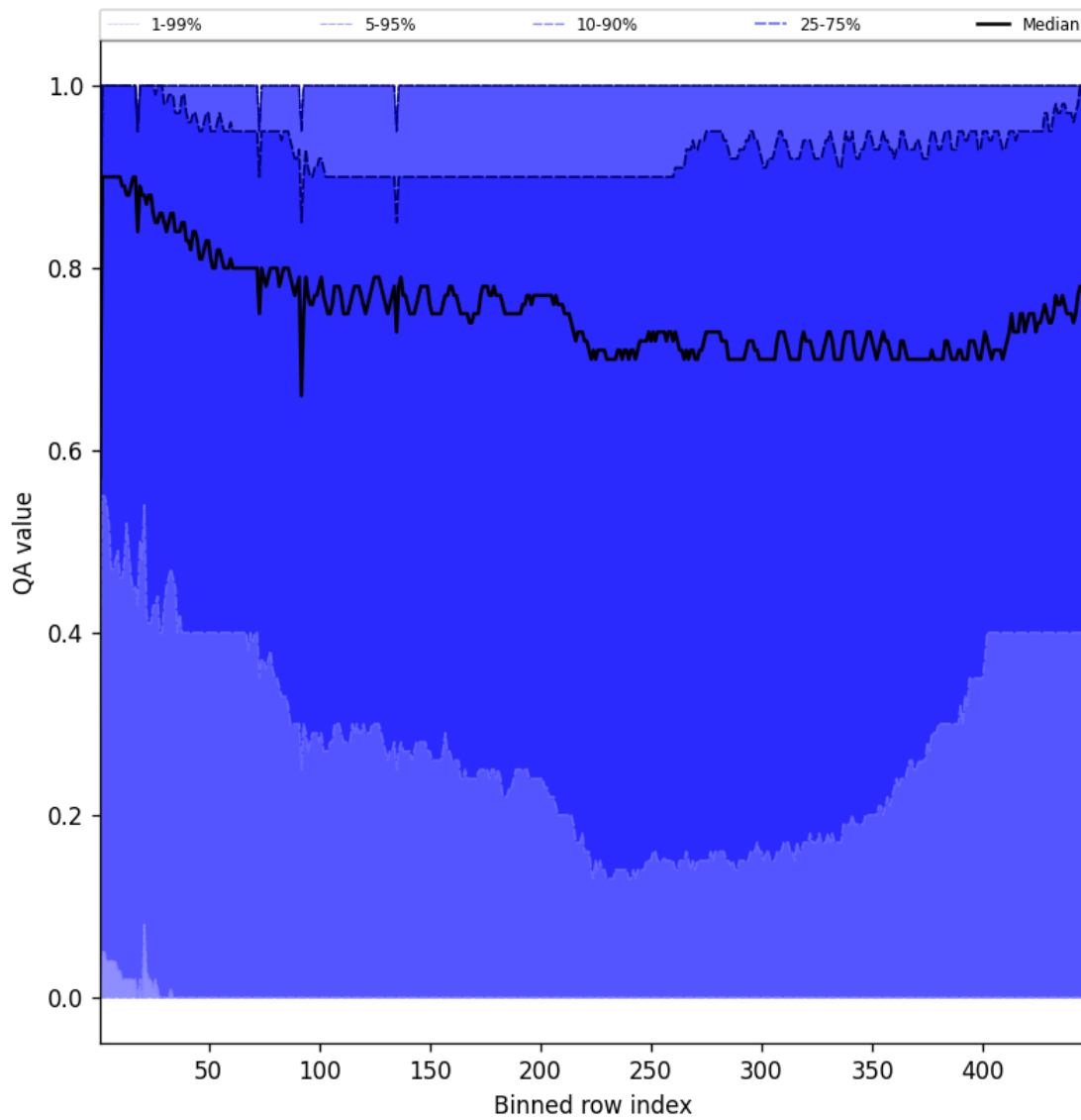
Figure 52: Along track statistics of “QA value” for 2025-06-10 to 2025-06-11
