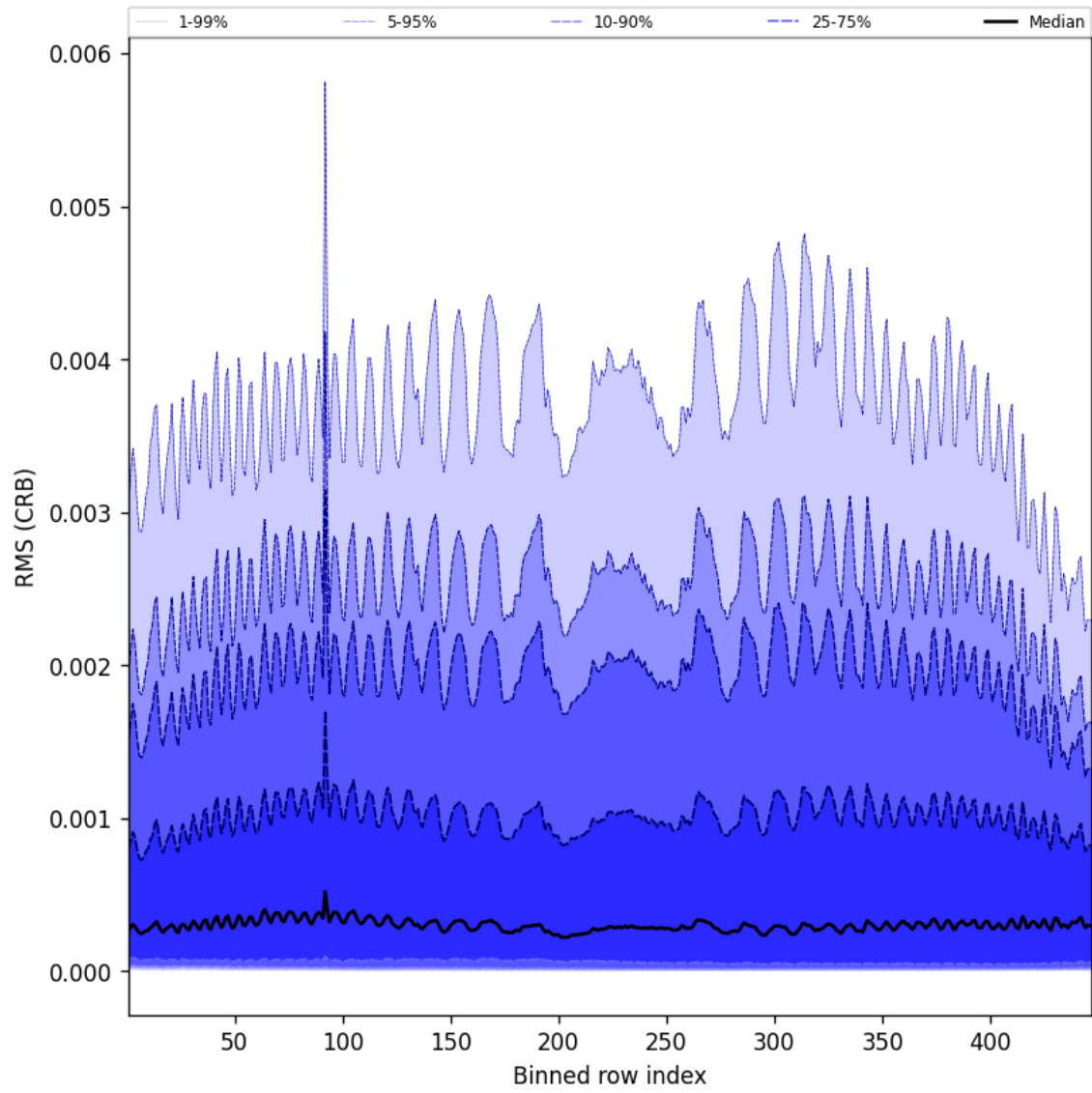
Figure 62: Along track statistics of “RMS (CRB)” for 2025-06-10 to 2025-06-11
