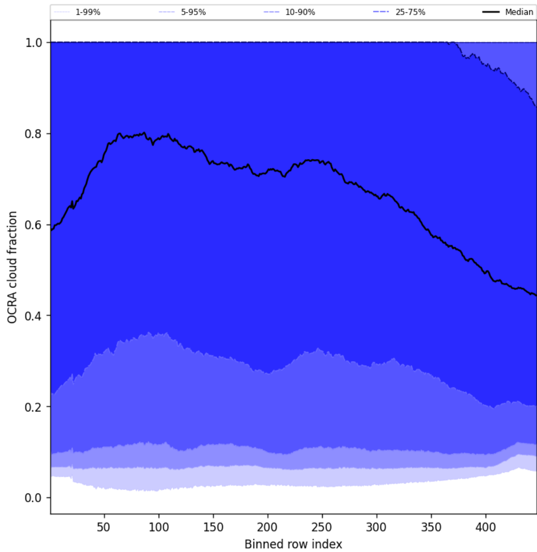
Figure 64: Along track statistics of “OCRA cloud fraction” for 2025-06-10 to 2025-06-11
