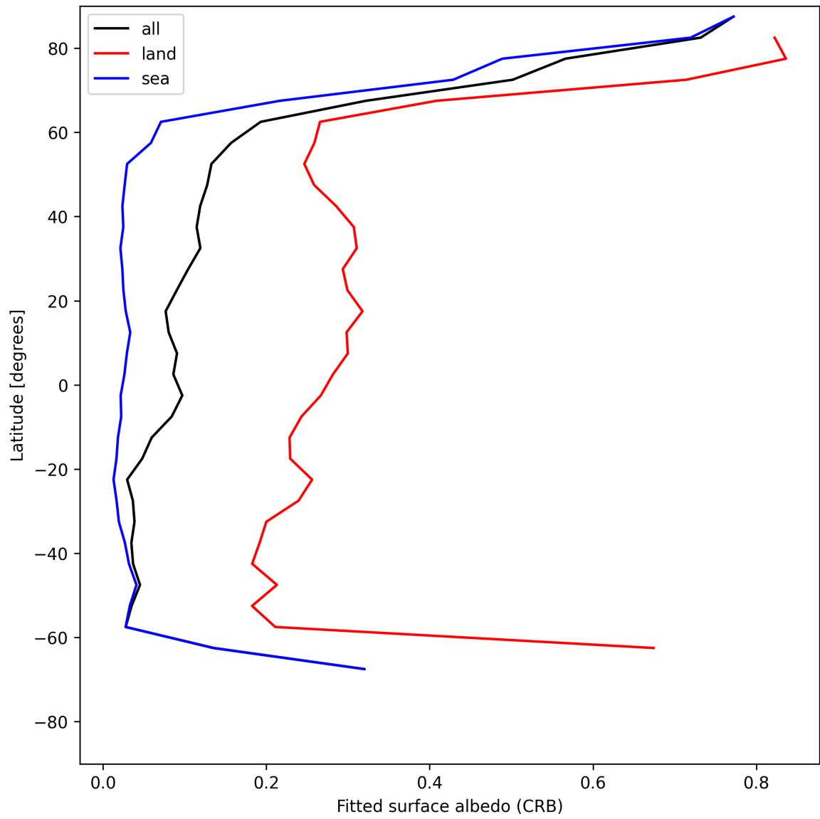
Figure 28: Zonal average of “Fitted surface albedo (CRB)” for 2025-06-10 to 2025-06-11.
