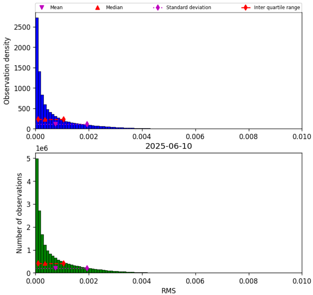
Figure 45: Histogram of “RMS” for 2025-06-10 to 2025-06-11
