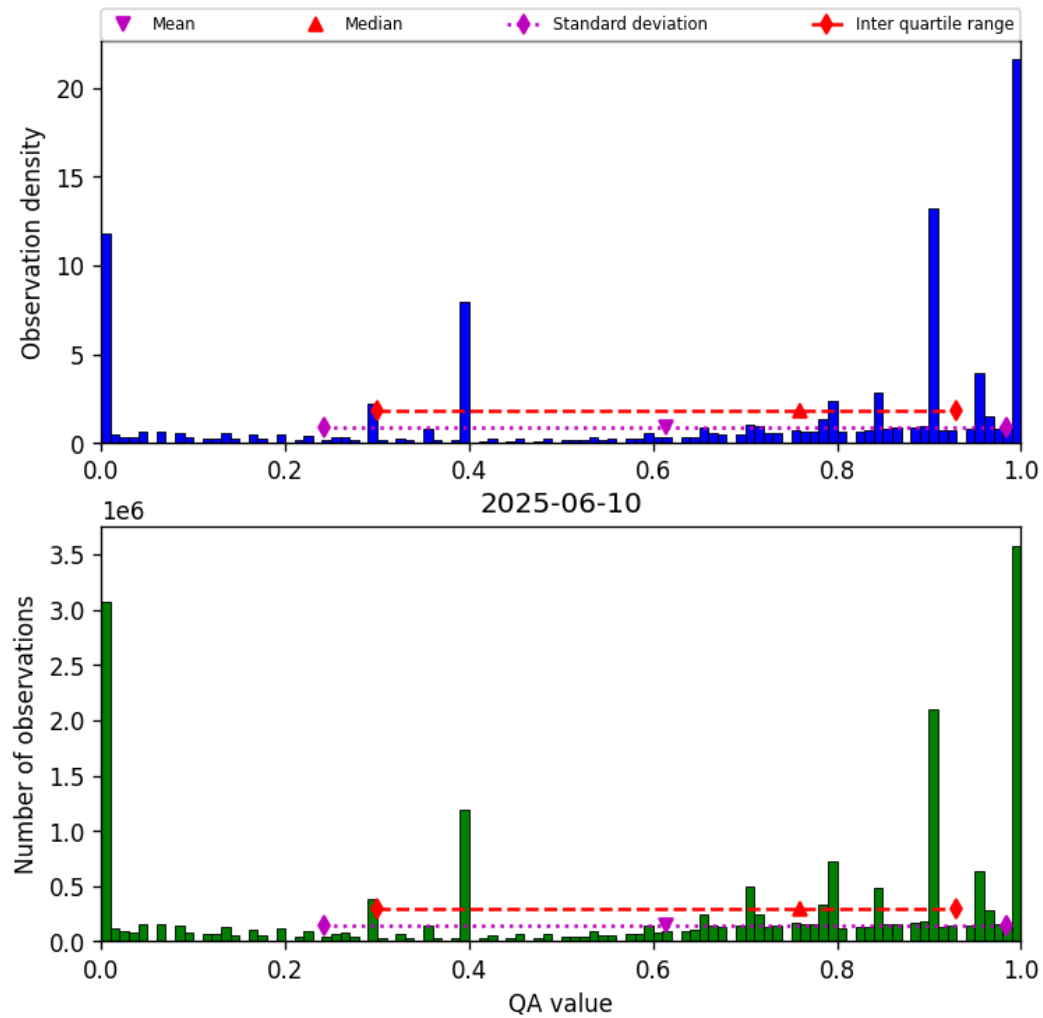
Figure 36: Histogram of “QA value” for 2025-06-10 to 2025-06-11
