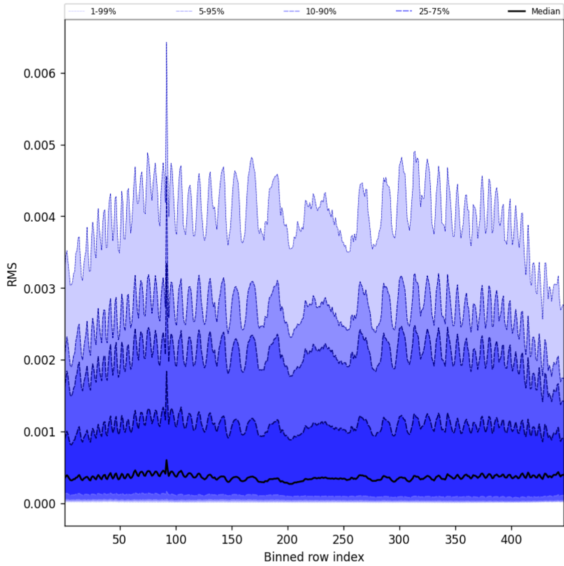
Figure 61: Along track statistics of “RMS” for 2025-06-10 to 2025-06-11
