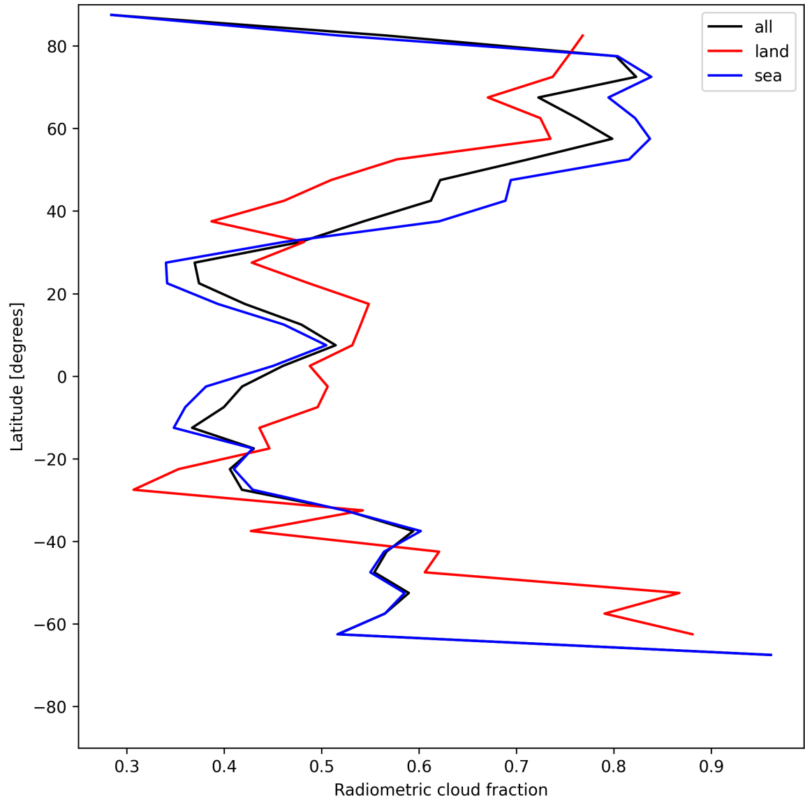
Figure 21: Zonal average of “Radiometric cloud fraction” for 2025-06-10 to 2025-06-11.
