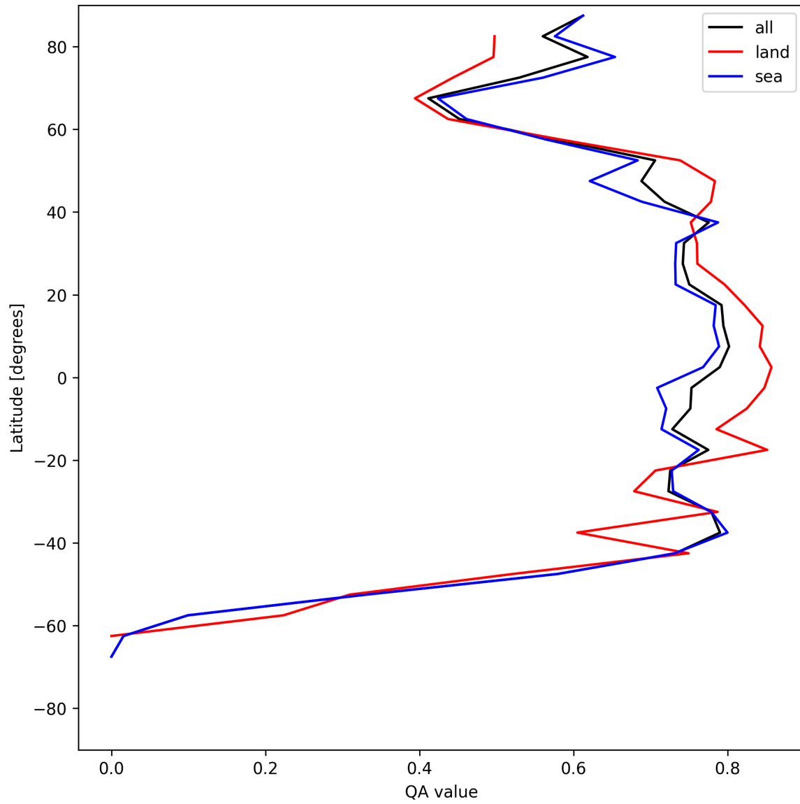
Figure 20: Zonal average of “QA value” for 2025-06-10 to 2025-06-11.
