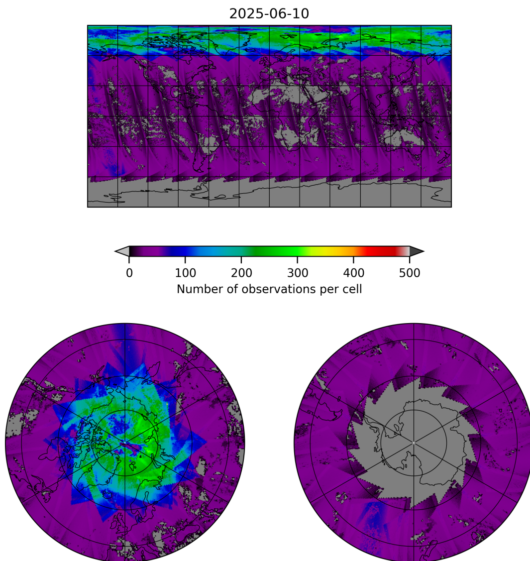
Figure 19: Map of the number of observations for 2025-06-10 to 2025-06-11
