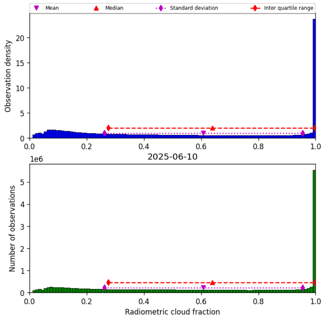
Figure 37: Histogram of “Radiometric cloud fraction” for 2025-06-10 to 2025-06-11
