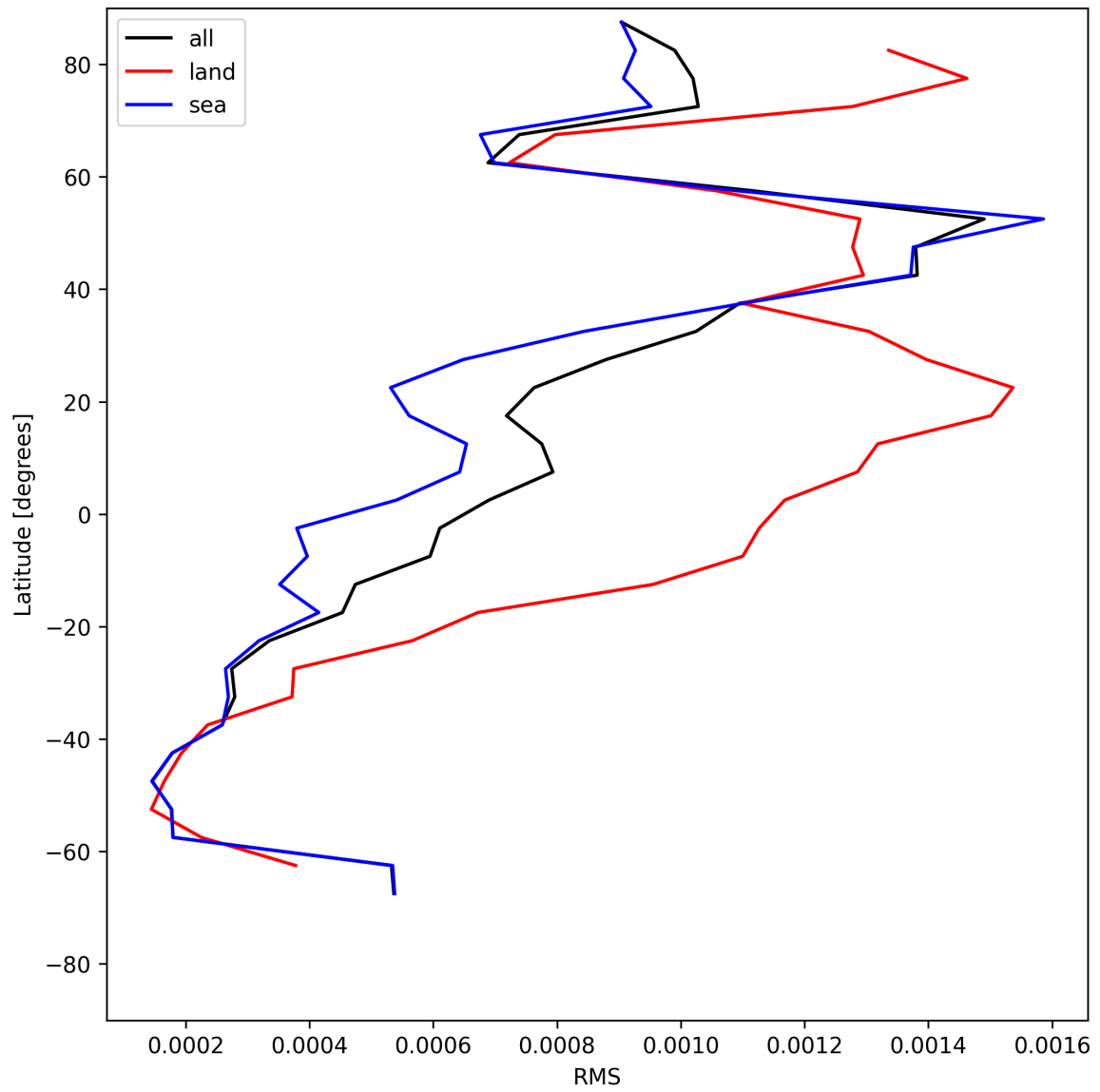
Figure 29: Zonal average of “RMS” for 2025-06-10 to 2025-06-11.
