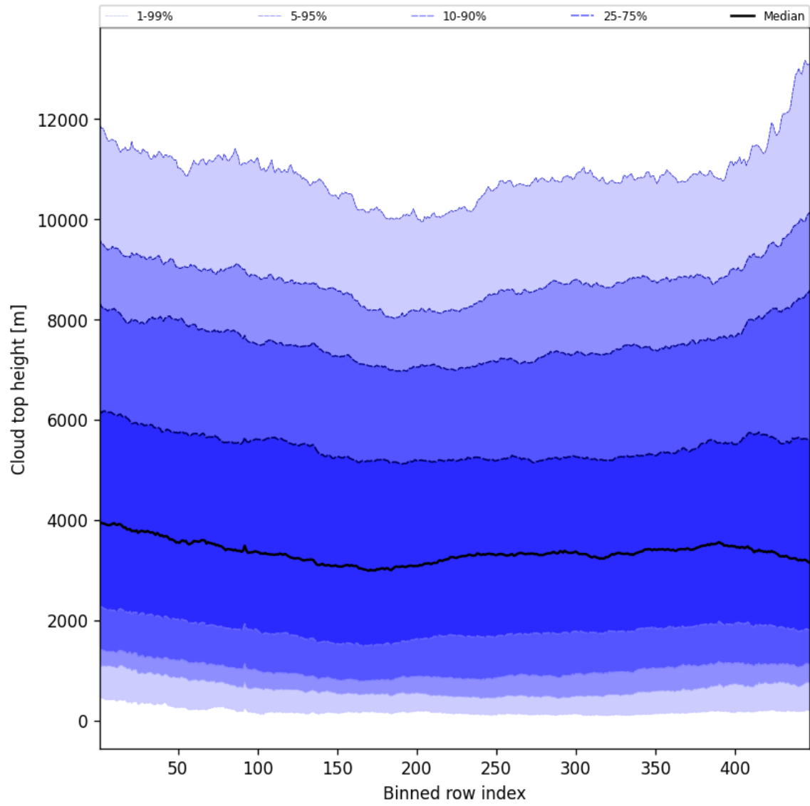
Figure 54: Along track statistics of “Cloud top height” for 2025-06-10 to 2025-06-11
