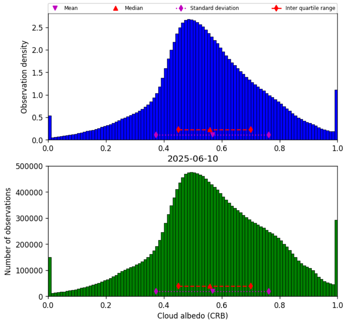
Figure 42: Histogram of “Cloud albedo (CRB)” for 2025-06-10 to 2025-06-11
