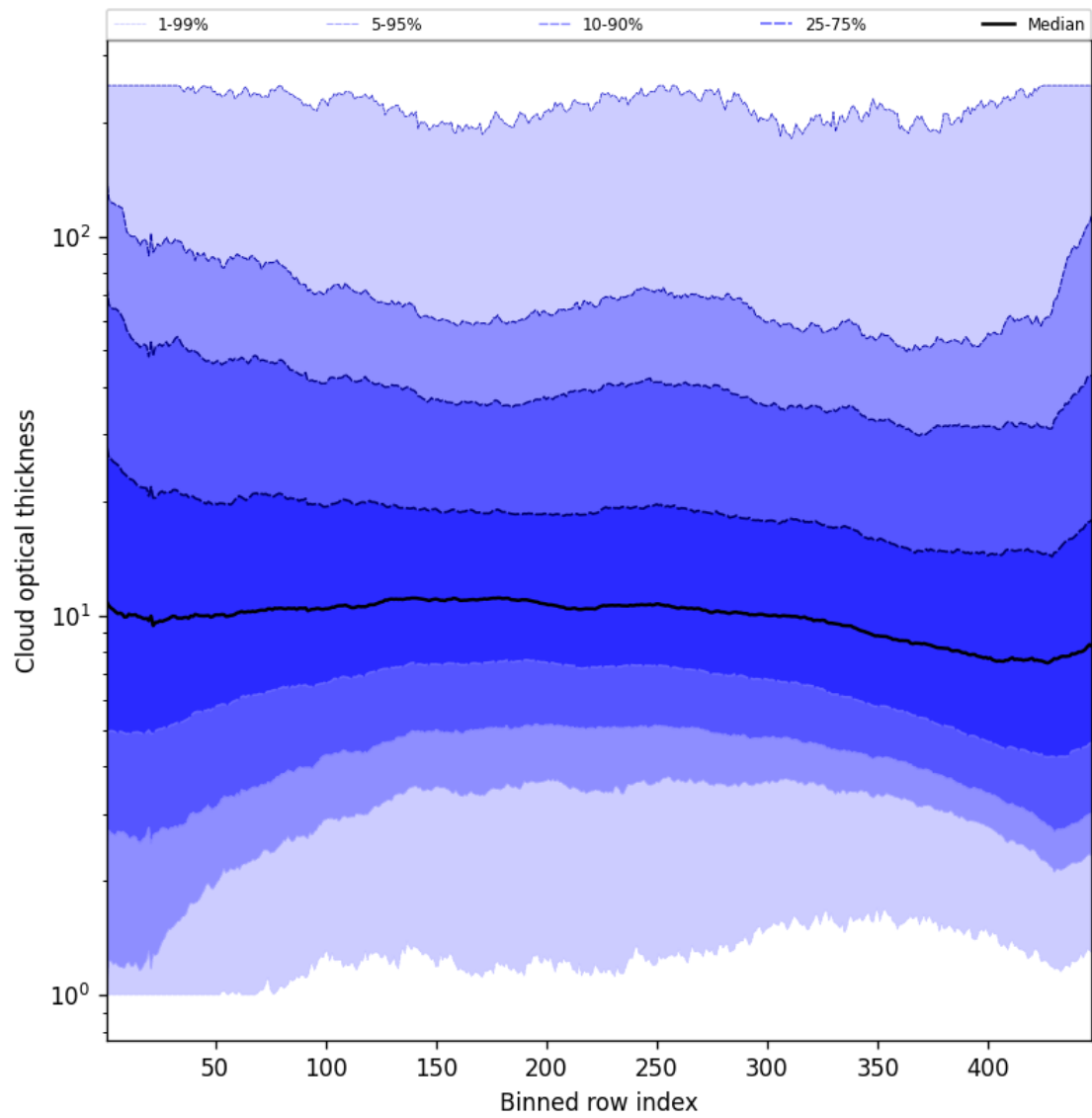
Figure 55: Along track statistics of “Cloud optical thickness” for 2025-06-10 to 2025-06-11
