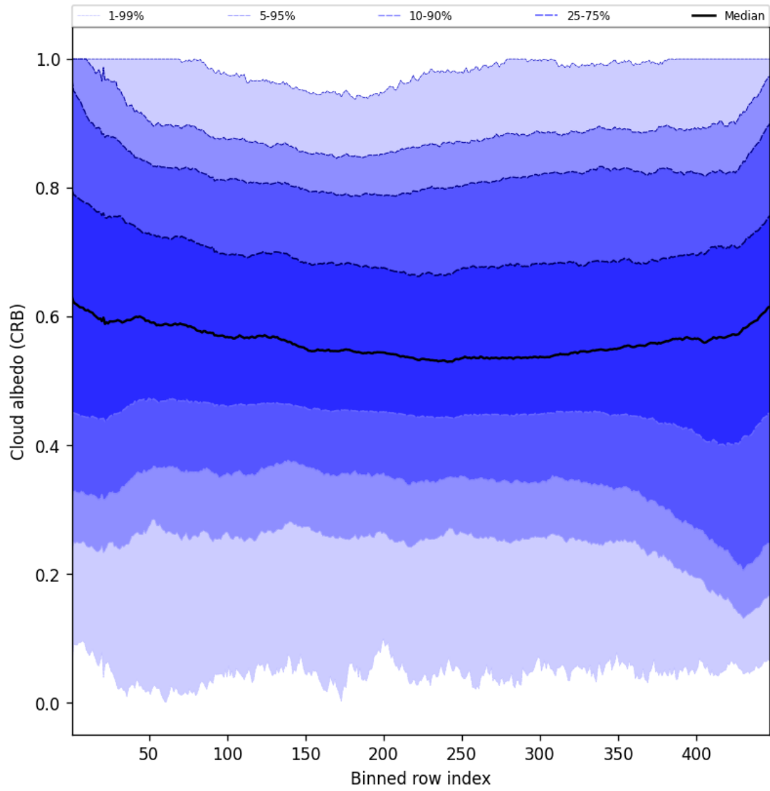
Figure 58: Along track statistics of “Cloud albedo (CRB)” for 2025-06-10 to 2025-06-11
