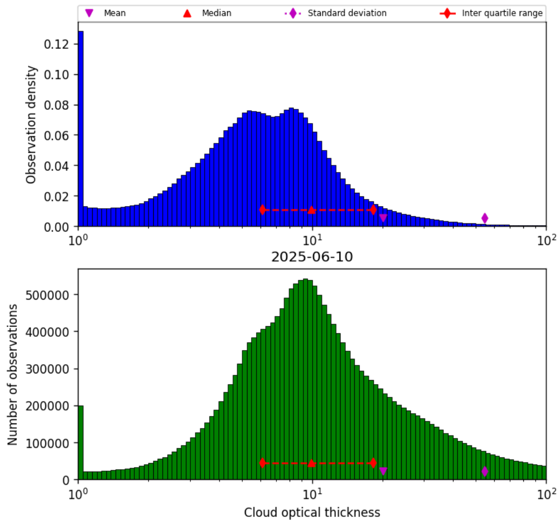
Figure 39: Histogram of “Cloud optical thickness” for 2025-06-10 to 2025-06-11
