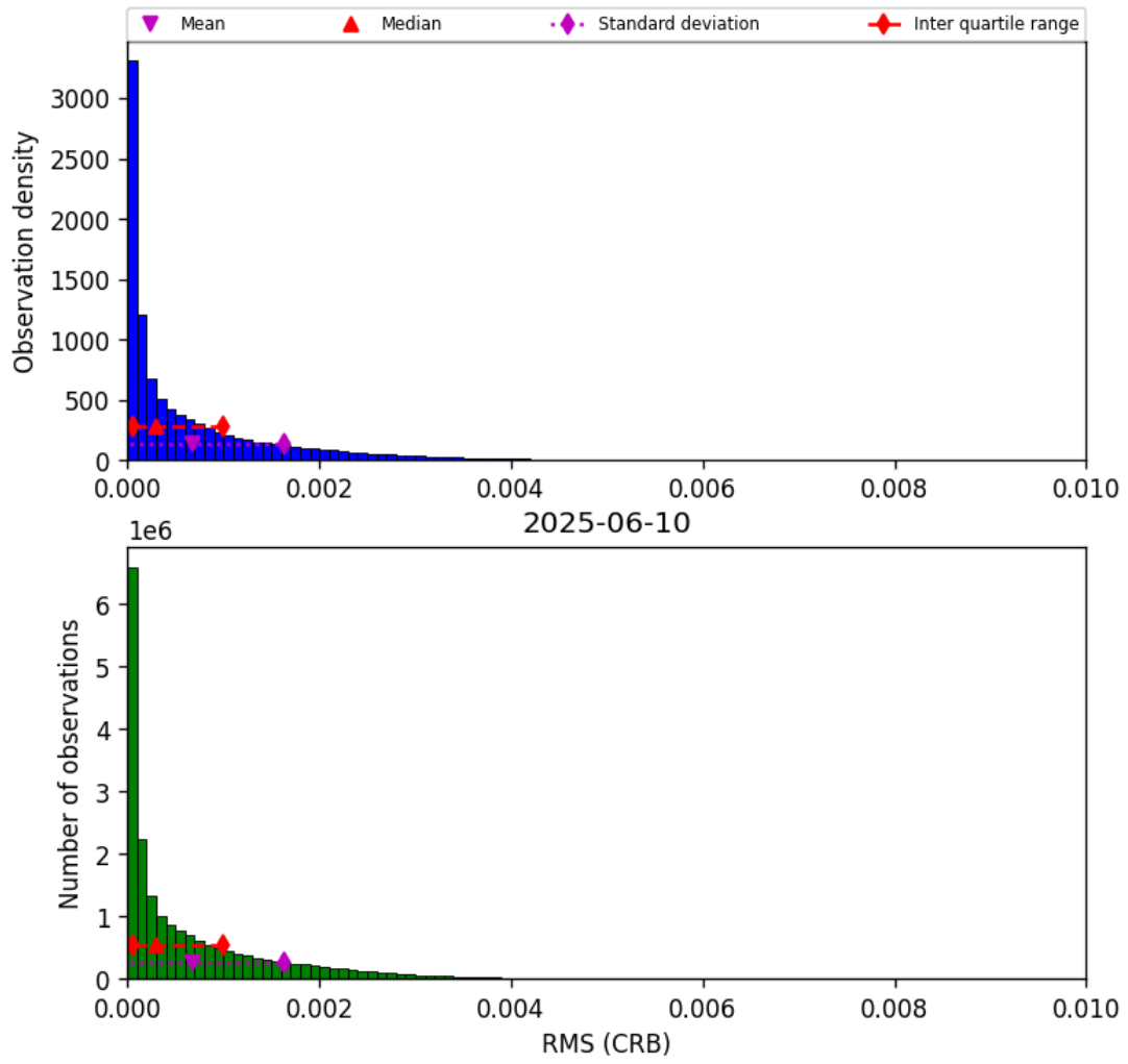
Figure 46: Histogram of “RMS (CRB)” for 2025-06-10 to 2025-06-11
