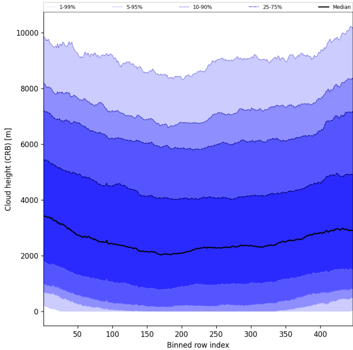
Figure 57: Along track statistics of “Cloud height (CRB)” for 2025-06-10 to 2025-06-11
