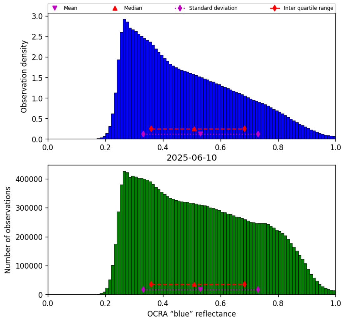
Figure 49: Histogram of “OCRA “blue” reflectance” for 2025-06-10 to 2025-06-11
