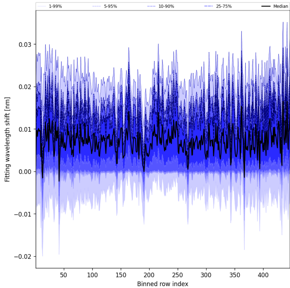
Figure 63: Along track statistics of “Fitting wavelength shift” for 2025-06-10 to 2025-06-11
