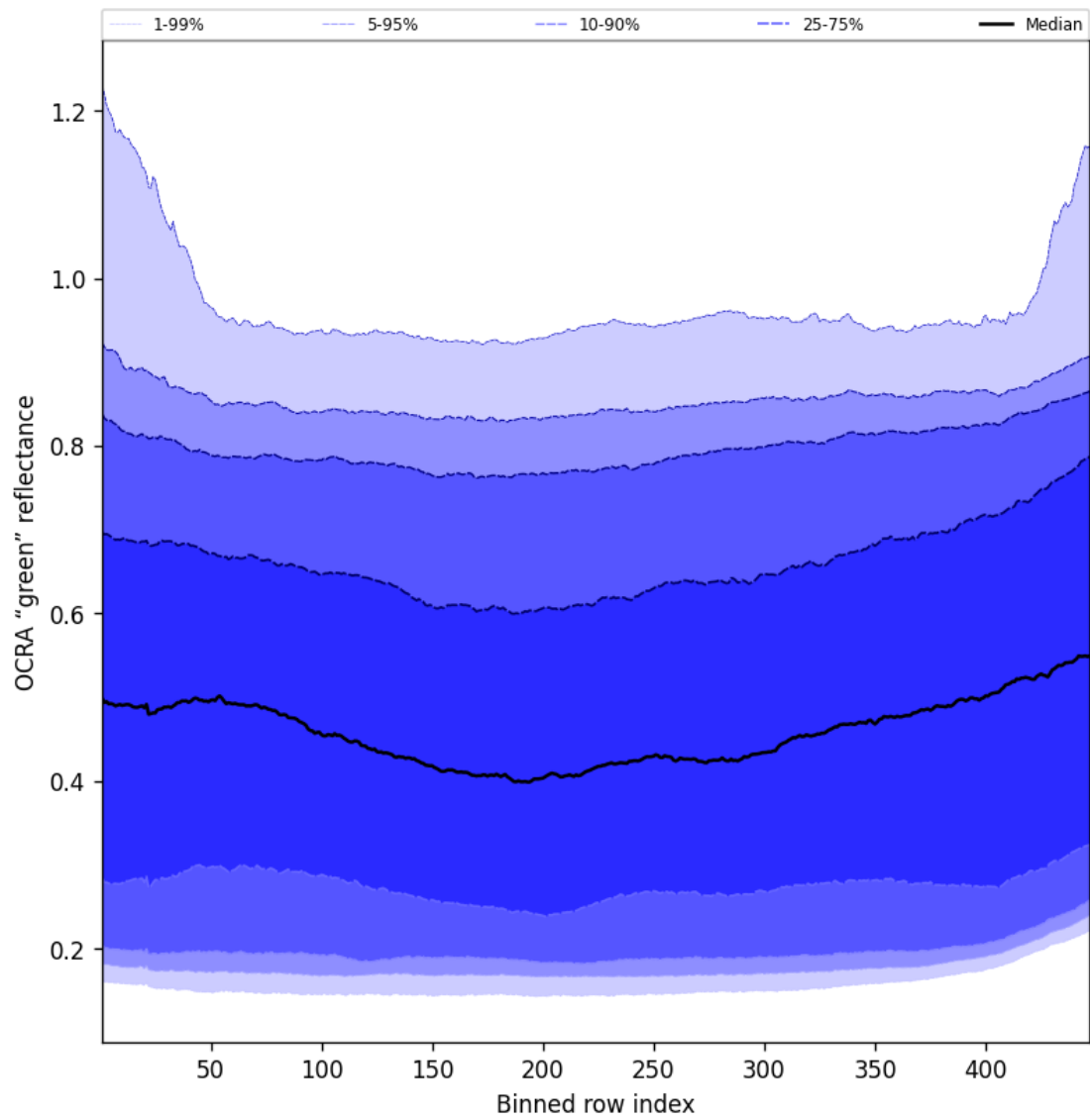
Figure 66: Along track statistics of “OCRA “green” reflectance” for 2025-06-10 to 2025-06-11
