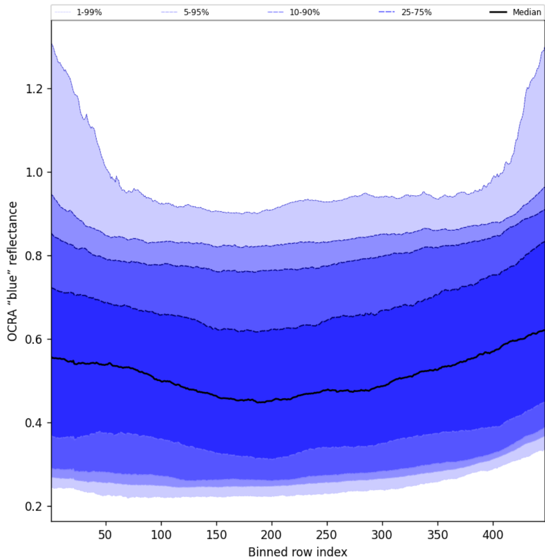
Figure 65: Along track statistics of “OCRA “blue” reflectance” for 2025-06-10 to 2025-06-11
