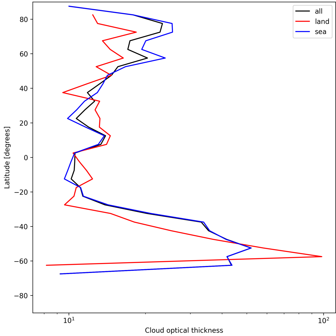
Figure 23: Zonal average of “Cloud optical thickness” for 2025-06-10 to 2025-06-11.
