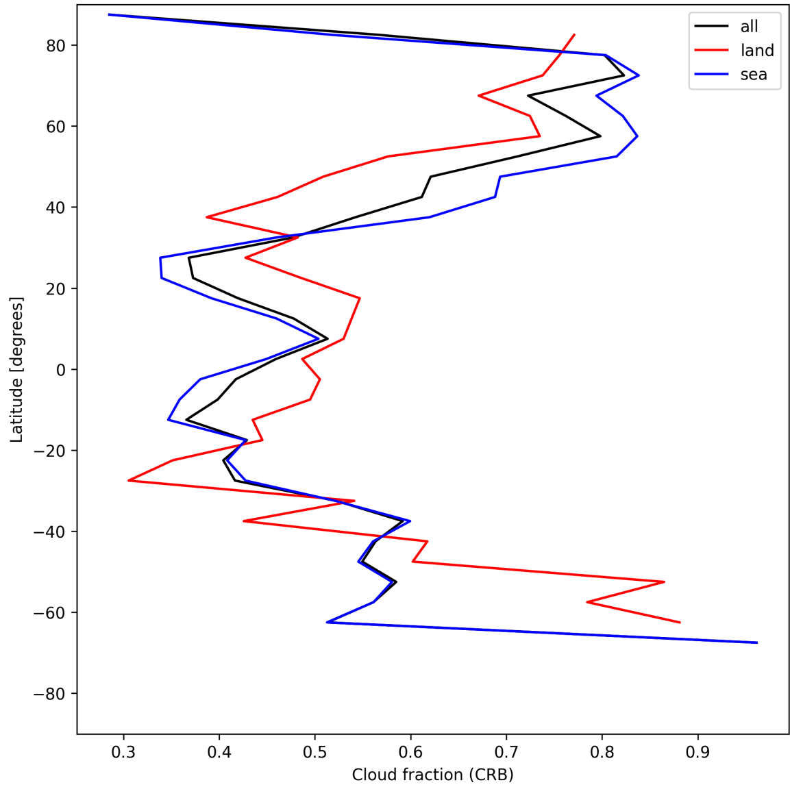
Figure 24: Zonal average of “Cloud fraction (CRB)” for 2025-06-10 to 2025-06-11.
