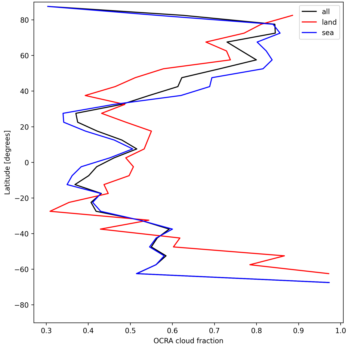
Figure 32: Zonal average of “OCRA cloud fraction” for 2025-06-10 to 2025-06-11.
