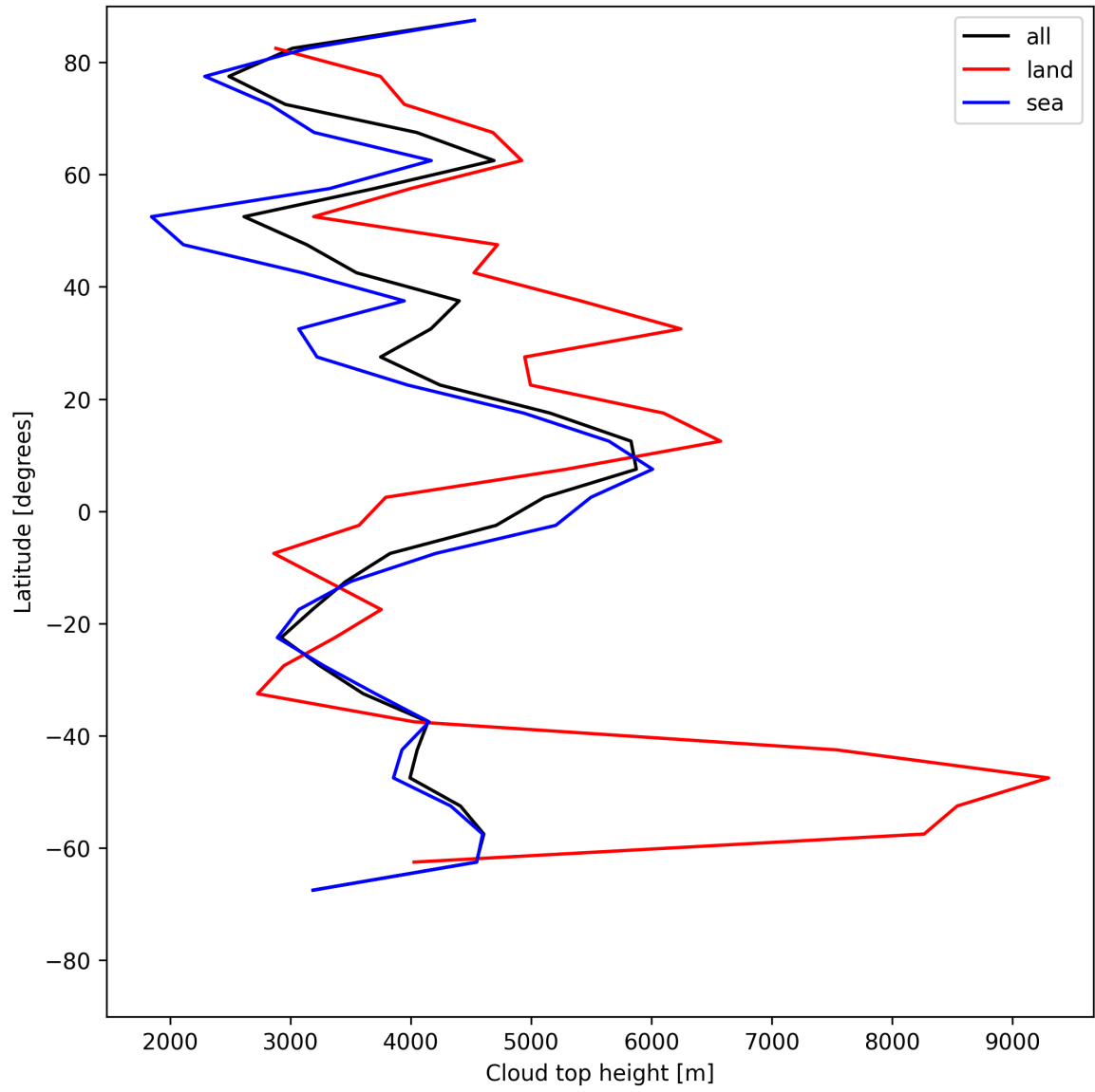
Figure 22: Zonal average of “Cloud top height” for 2025-06-10 to 2025-06-11.
