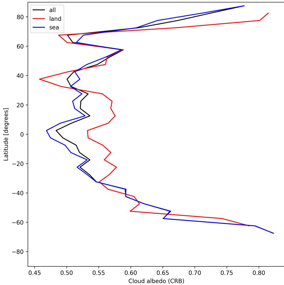
Figure 26: Zonal average of “Cloud albedo (CRB)” for 2025-06-10 to 2025-06-11.
