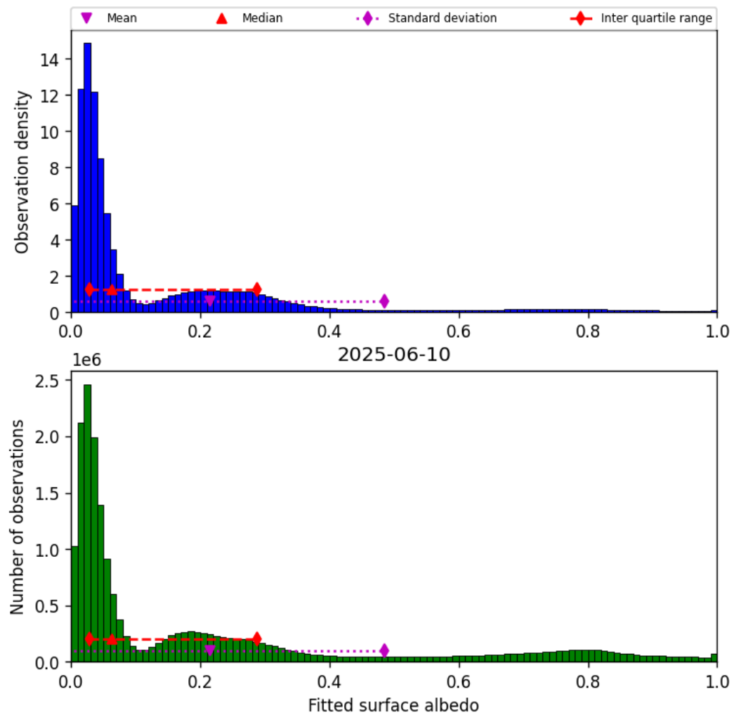
Figure 43: Histogram of “Fitted surface albedo” for 2025-06-10 to 2025-06-11
