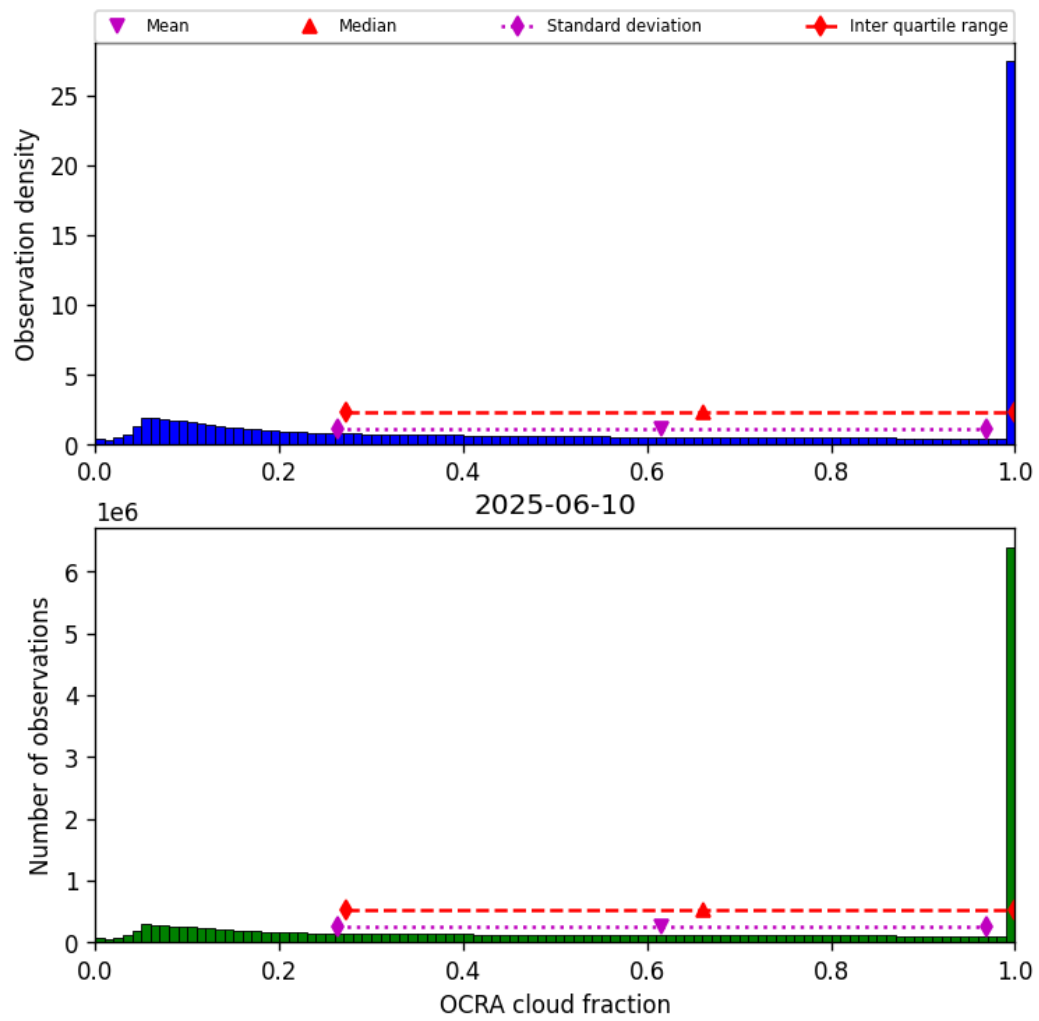
Figure 48: Histogram of “OCRA cloud fraction” for 2025-06-10 to 2025-06-11
