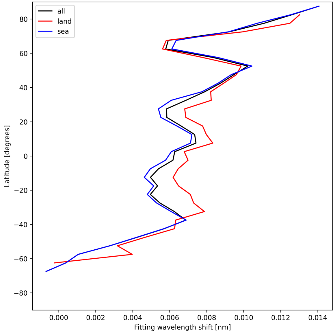
Figure 31: Zonal average of “Fitting wavelength shift” for 2025-06-10 to 2025-06-11.
