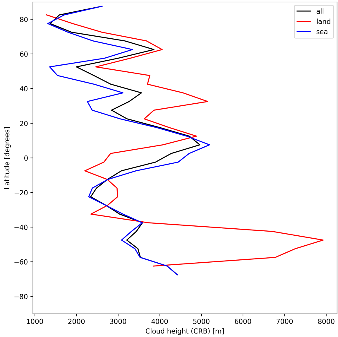
Figure 25: Zonal average of “Cloud height (CRB)” for 2025-06-10 to 2025-06-11.
