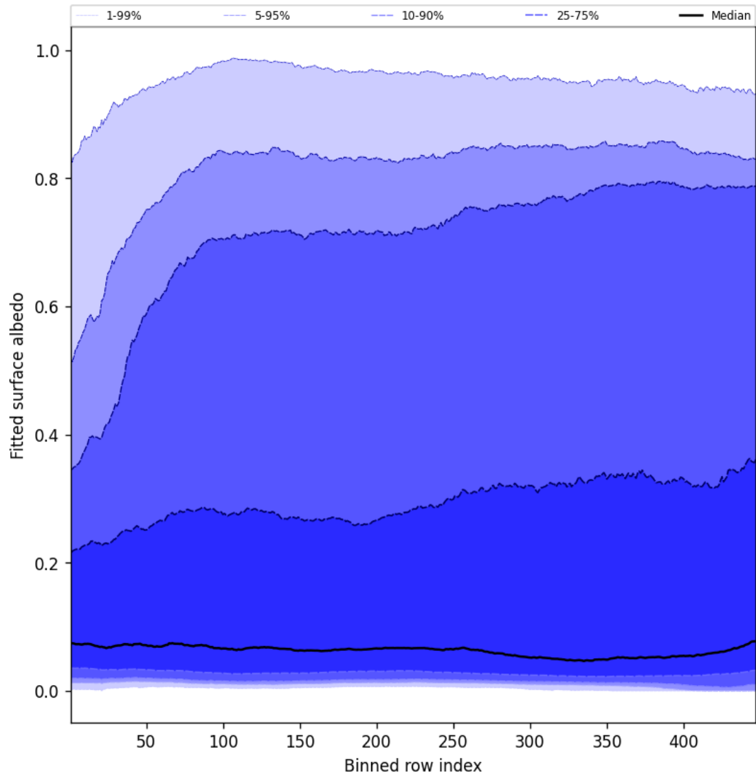
Figure 59: Along track statistics of “Fitted surface albedo” for 2025-06-10 to 2025-06-11
