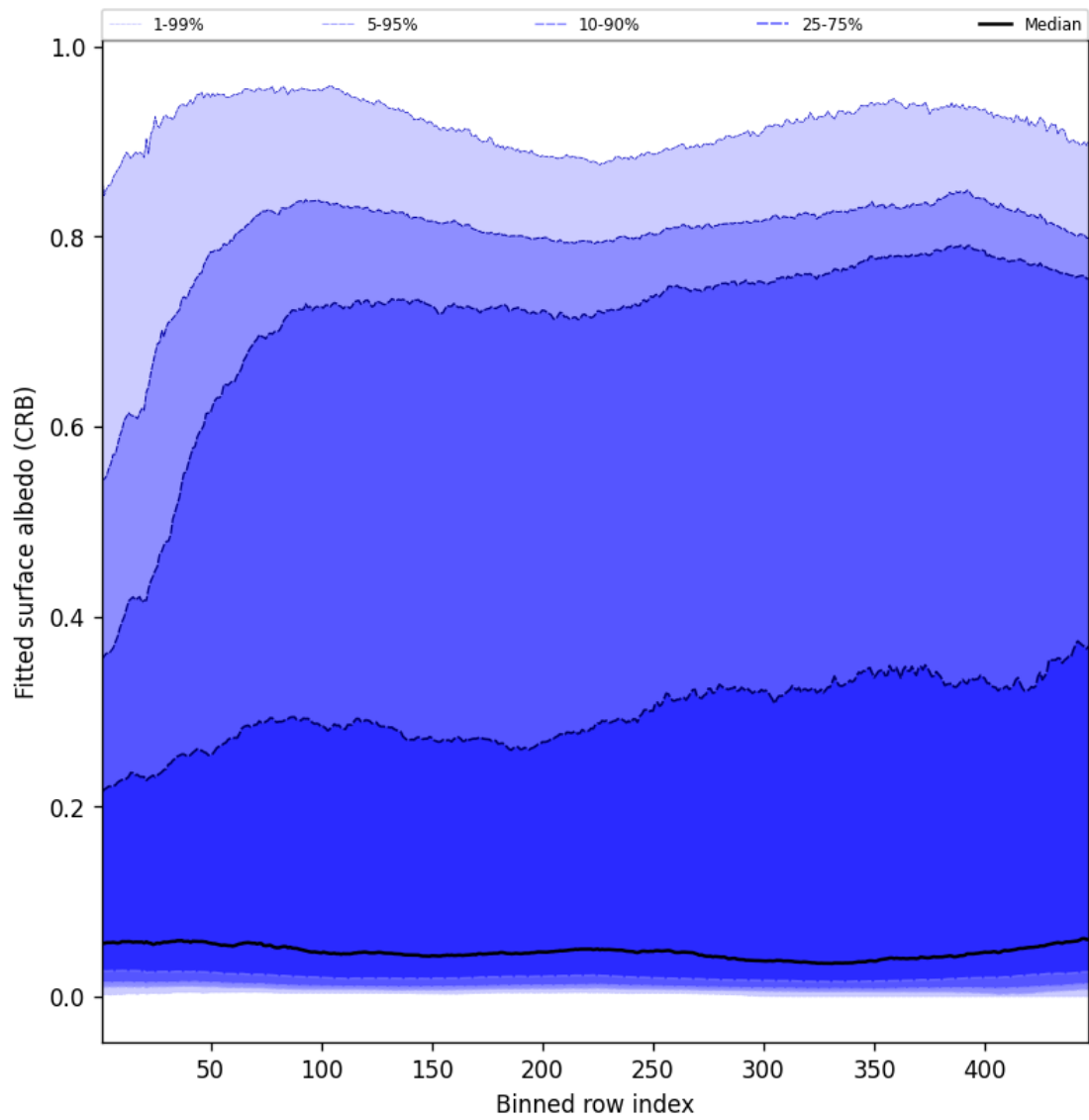
Figure 60: Along track statistics of “Fitted surface albedo (CRB)” for 2025-06-10 to 2025-06-11
