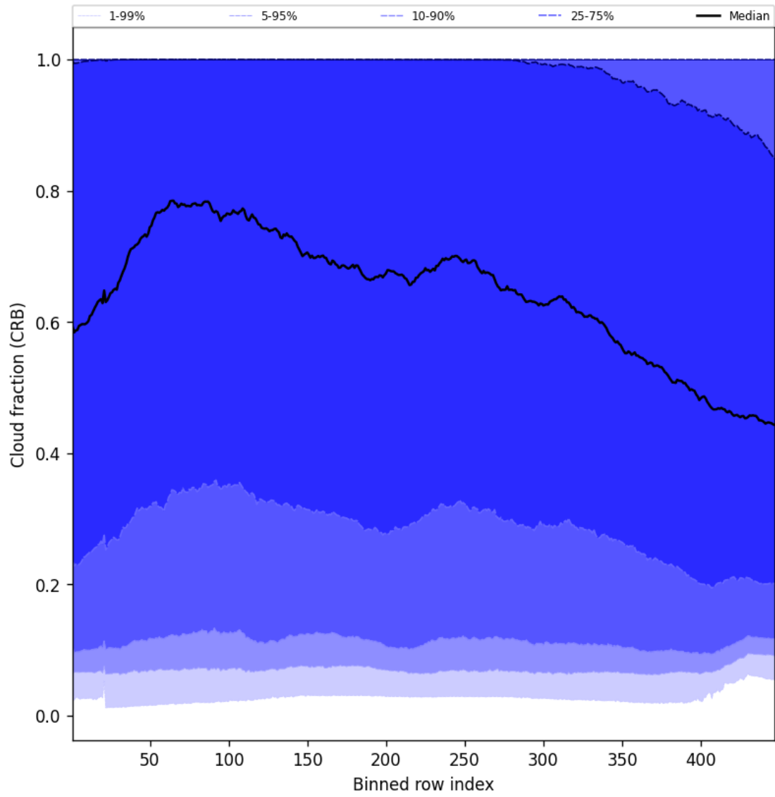
Figure 56: Along track statistics of “Cloud fraction (CRB)” for 2025-06-10 to 2025-06-11
