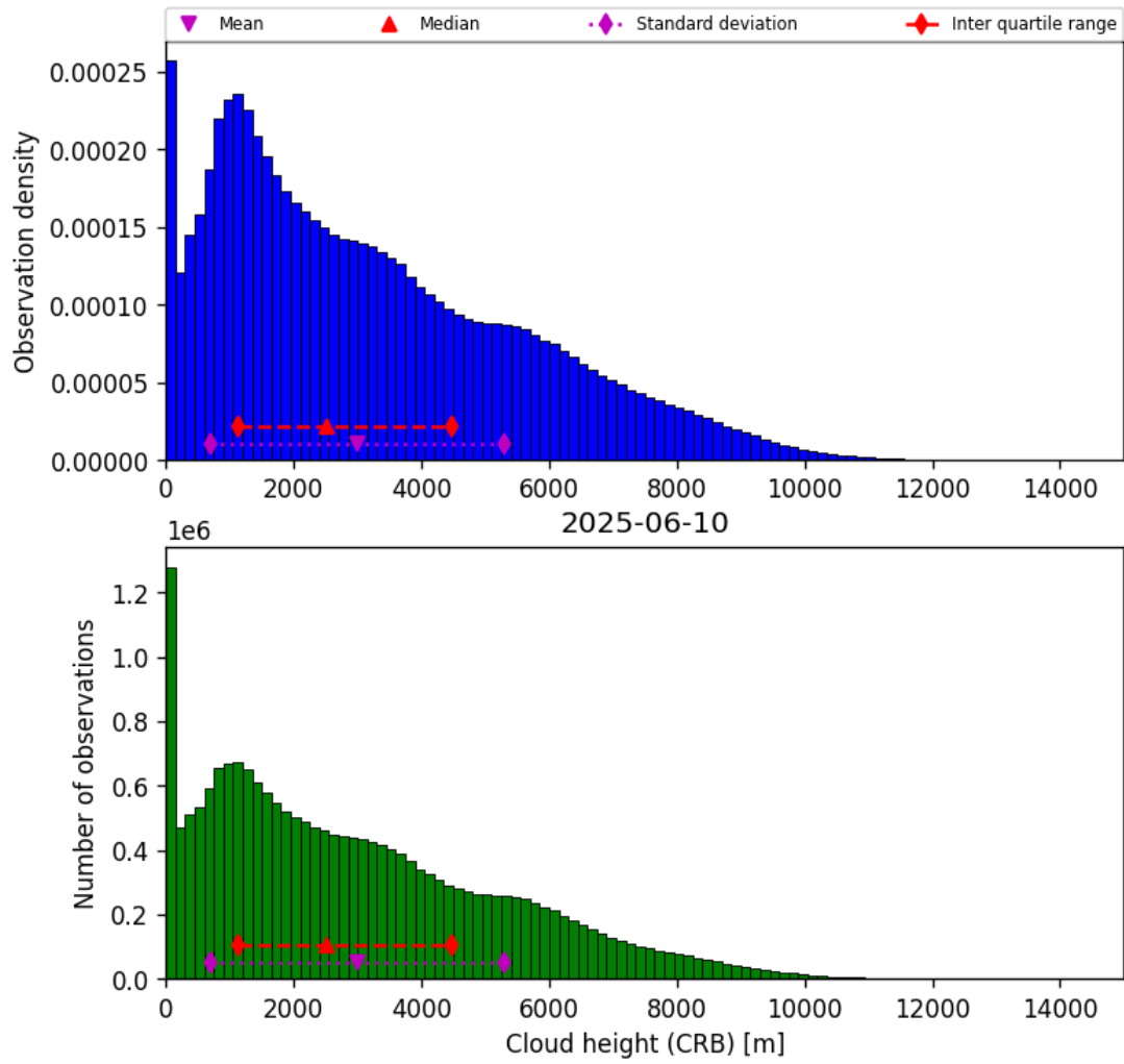
Figure 41: Histogram of “Cloud height (CRB)” for 2025-06-10 to 2025-06-11
