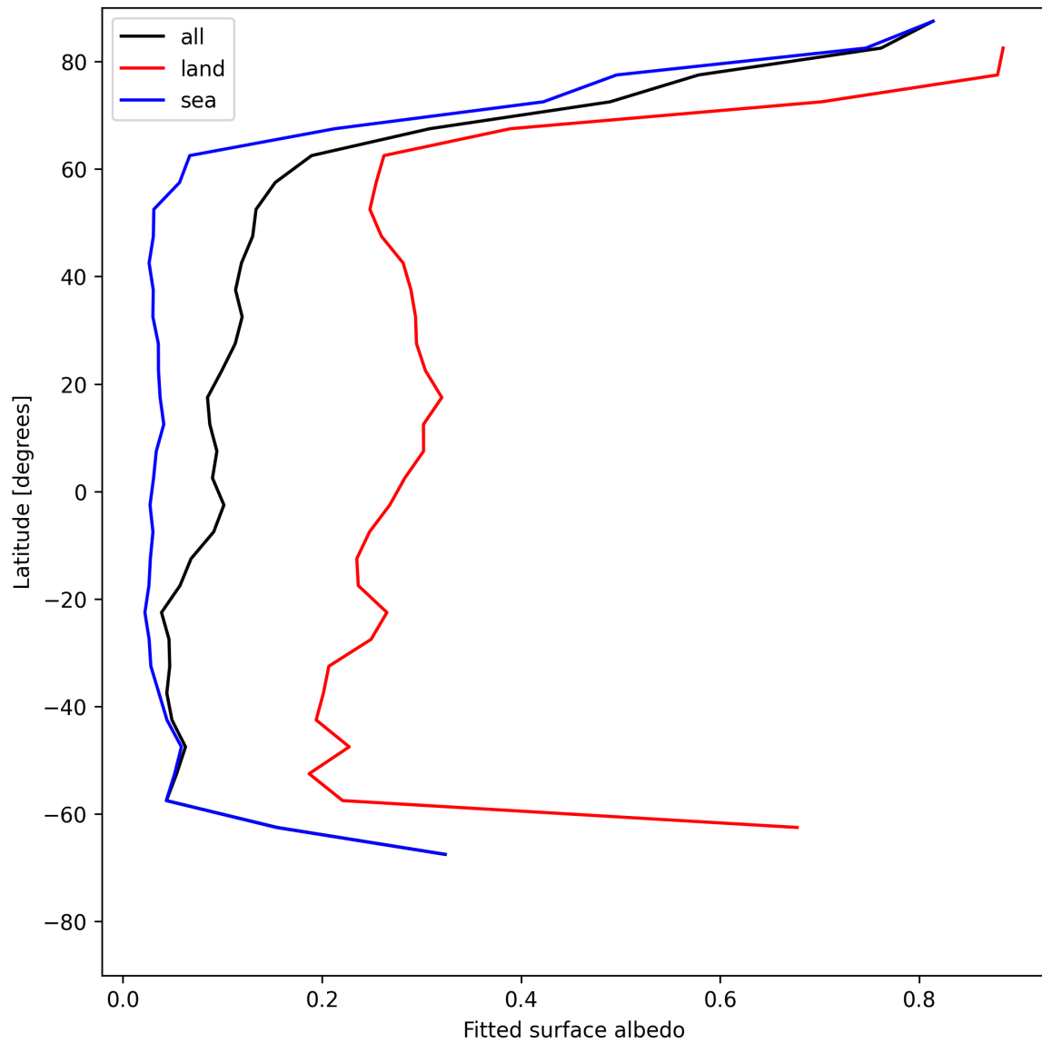
Figure 27: Zonal average of “Fitted surface albedo” for 2025-06-10 to 2025-06-11.
