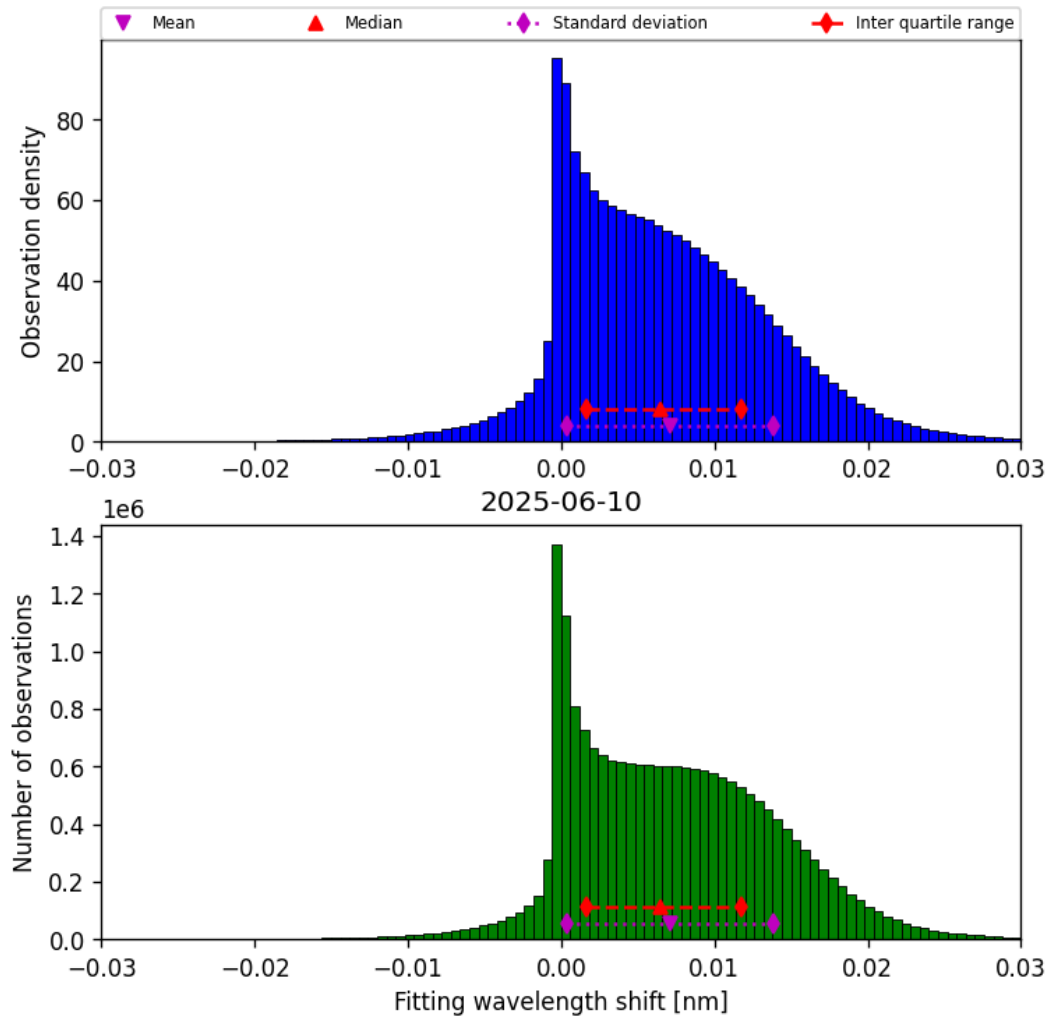
Figure 47: Histogram of “Fitting wavelength shift” for 2025-06-10 to 2025-06-11
