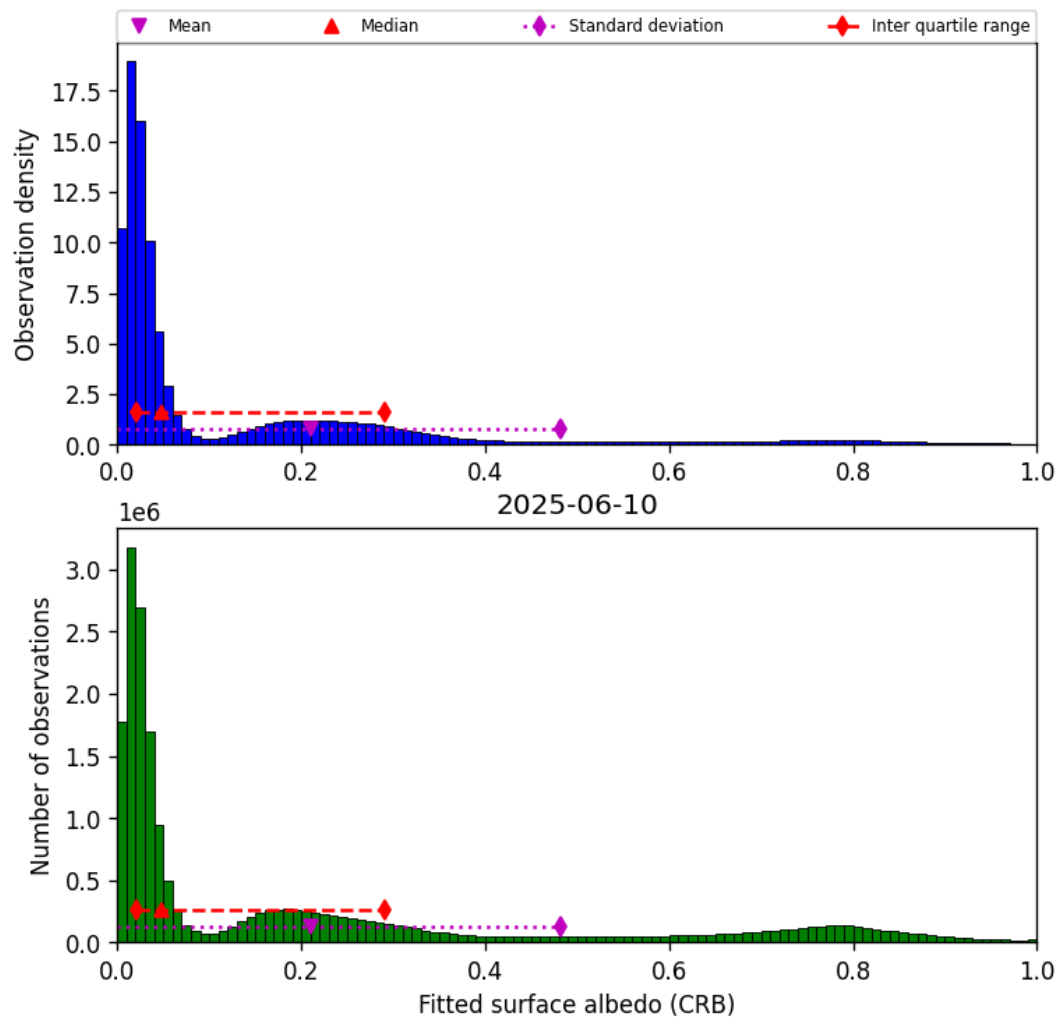
Figure 44: Histogram of “Fitted surface albedo (CRB)” for 2025-06-10 to 2025-06-11
