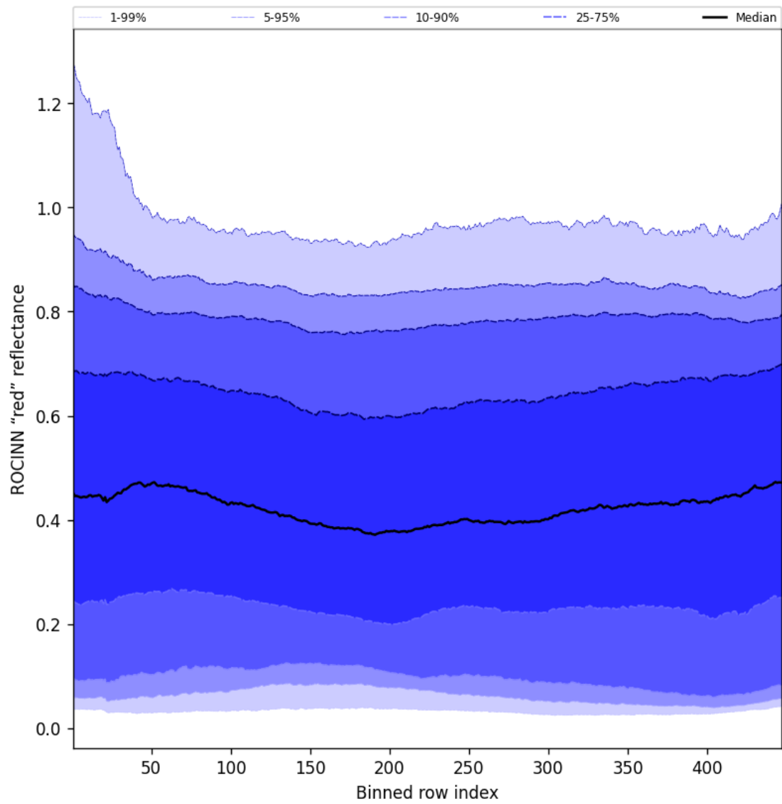
Figure 67: Along track statistics of “ROCINN “red” reflectance” for 2025-06-10 to 2025-06-11
