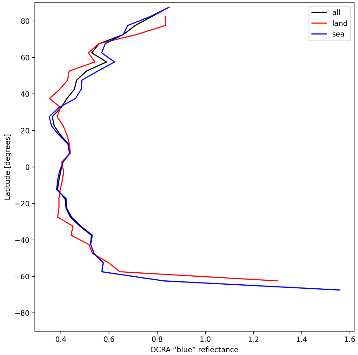
Figure 33: Zonal average of “OCRA “blue” reflectance” for 2025-06-10 to 2025-06-11.
