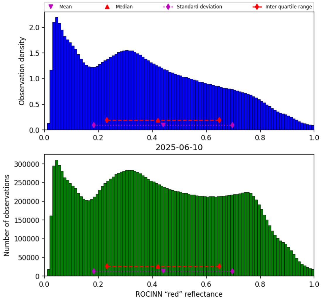
Figure 51: Histogram of “ROCINN “red” reflectance” for 2025-06-10 to 2025-06-11
