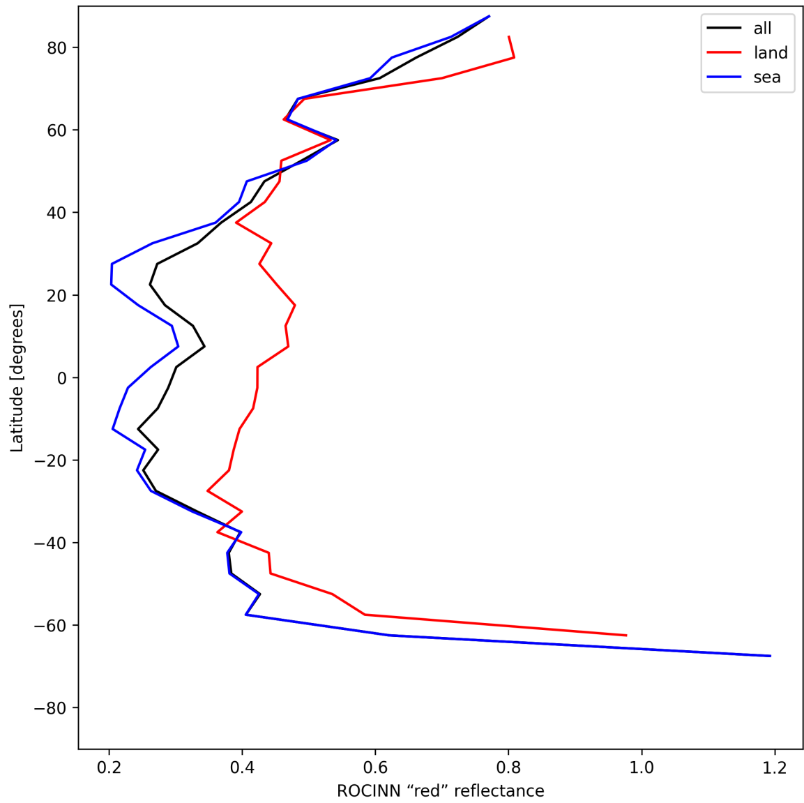
Figure 35: Zonal average of “ROCINN “red” reflectance” for 2025-06-10 to 2025-06-11.
