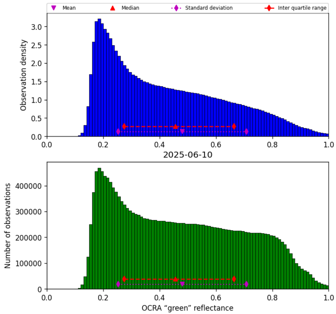
Figure 50: Histogram of “OCRA “green” reflectance” for 2025-06-10 to 2025-06-11
