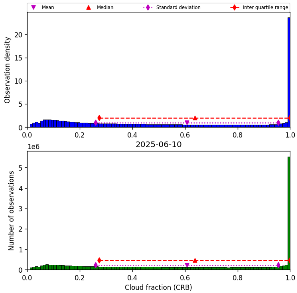
Figure 40: Histogram of “Cloud fraction (CRB)” for 2025-06-10 to 2025-06-11
