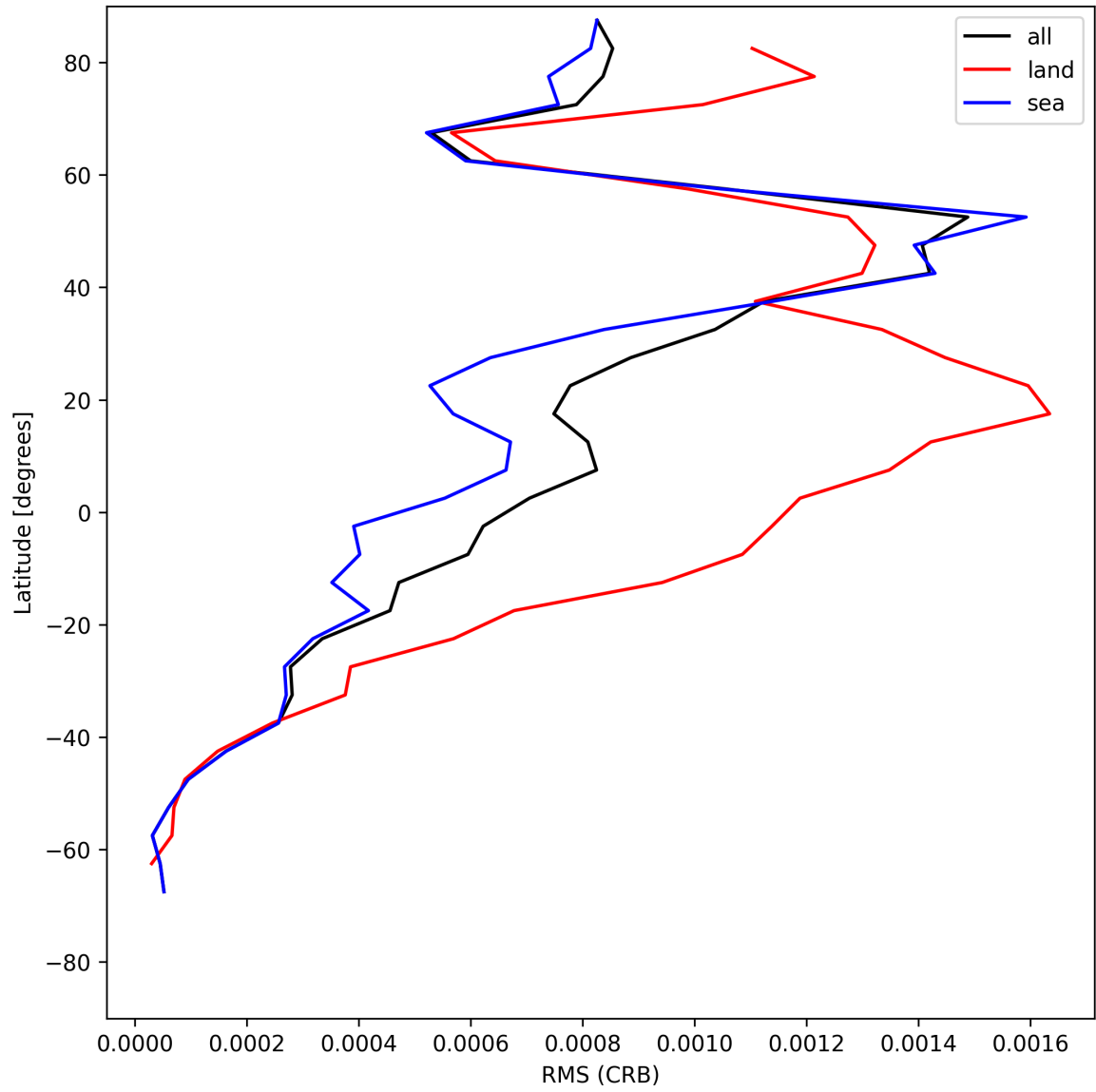
Figure 30: Zonal average of “RMS (CRB)” for 2025-06-10 to 2025-06-11.
