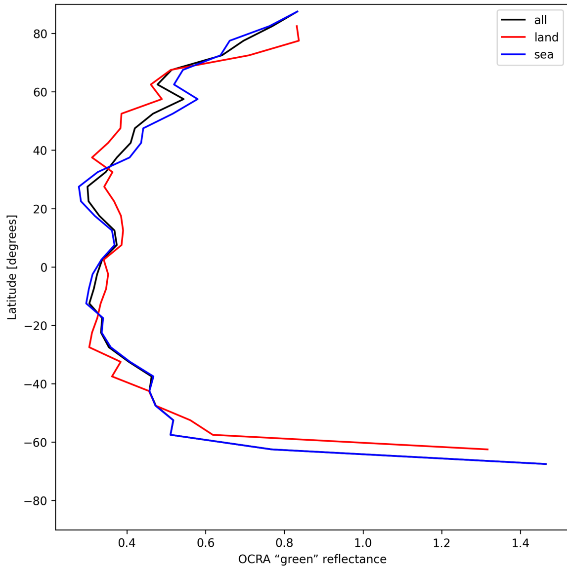
Figure 34: Zonal average of “OCRA “green” reflectance” for 2025-06-10 to 2025-06-11.
