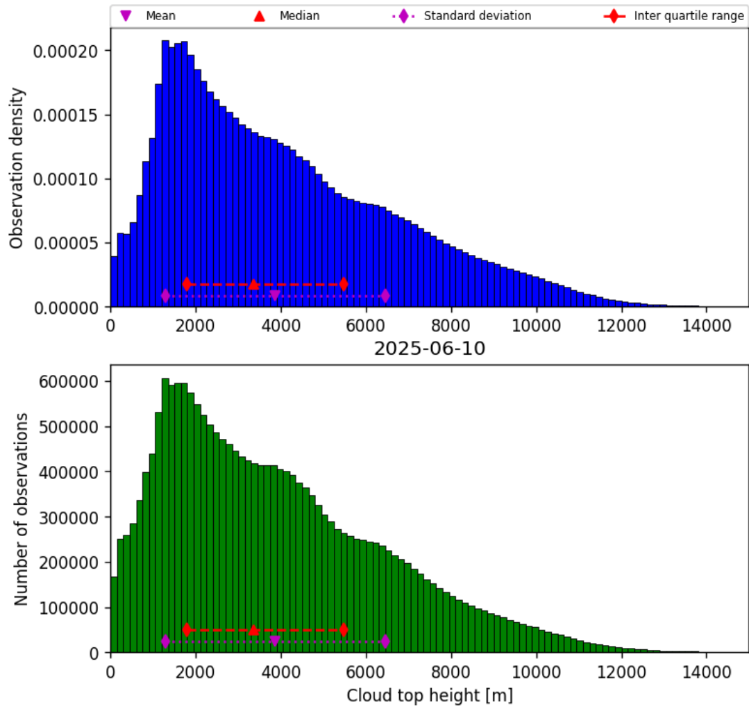
Figure 38: Histogram of “Cloud top height” for 2025-06-10 to 2025-06-11
