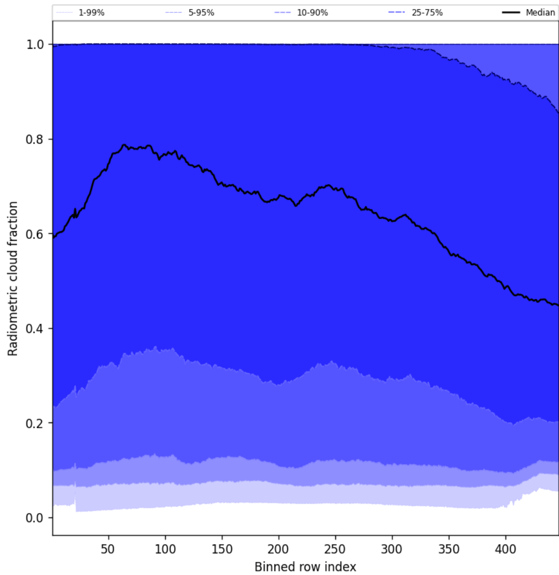
Figure 53: Along track statistics of “Radiometric cloud fraction” for 2025-06-10 to 2025-06-11
