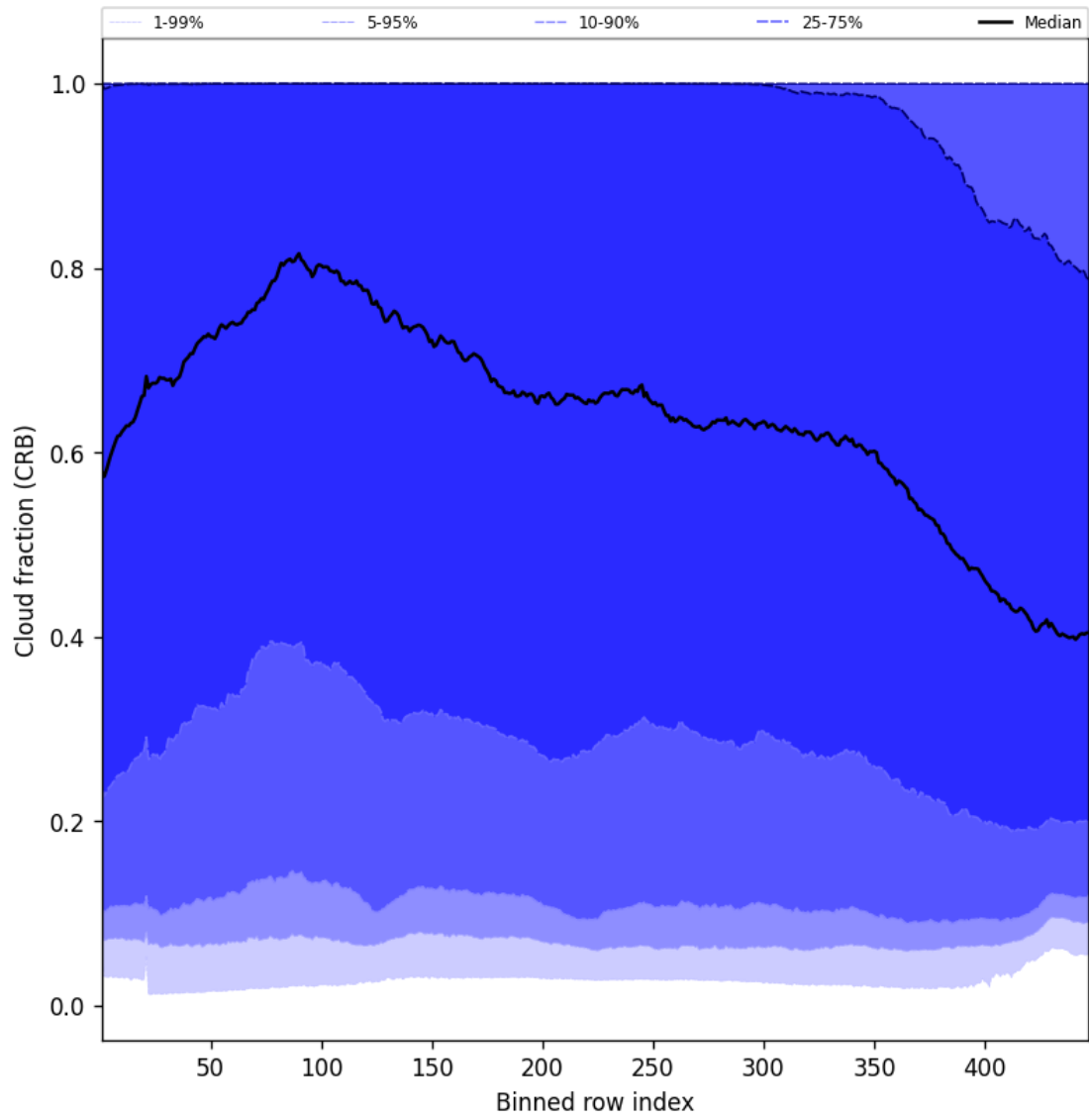
Figure 56: Along track statistics of “Cloud fraction (CRB)” for 2025-06-12 to 2025-06-13
