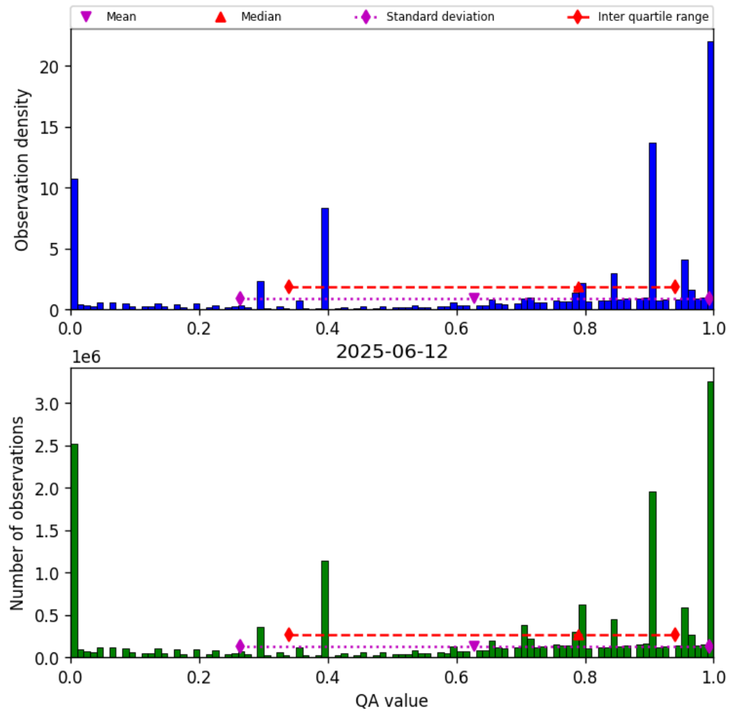
Figure 36: Histogram of “QA value” for 2025-06-12 to 2025-06-13
