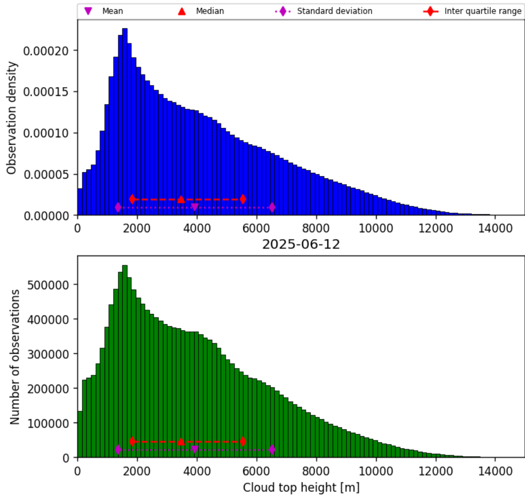
Figure 38: Histogram of “Cloud top height” for 2025-06-12 to 2025-06-13
