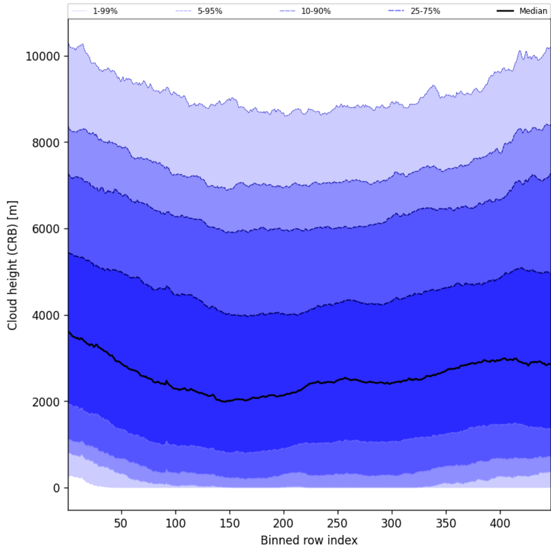
Figure 57: Along track statistics of “Cloud height (CRB)” for 2025-06-12 to 2025-06-13
