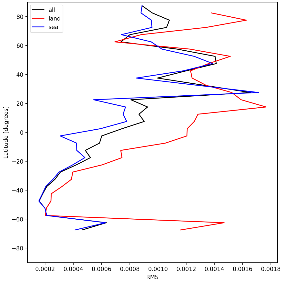
Figure 29: Zonal average of “RMS” for 2025-06-12 to 2025-06-13.
