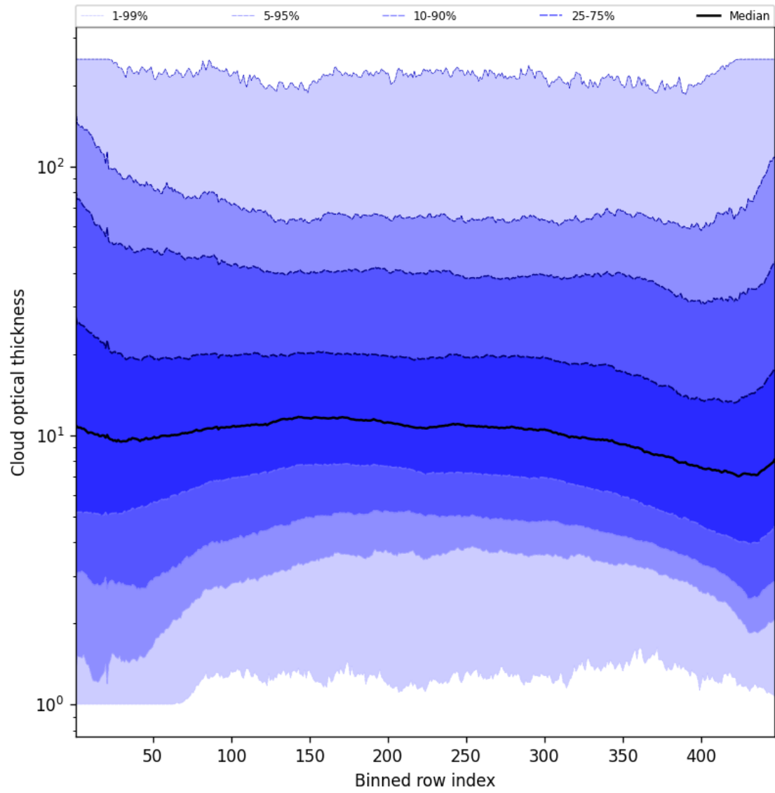
Figure 55: Along track statistics of “Cloud optical thickness” for 2025-06-12 to 2025-06-13
