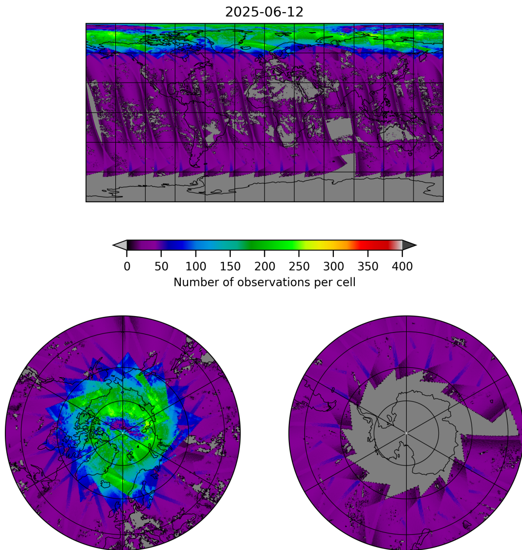
Figure 19: Map of the number of observations for 2025-06-12 to 2025-06-13
