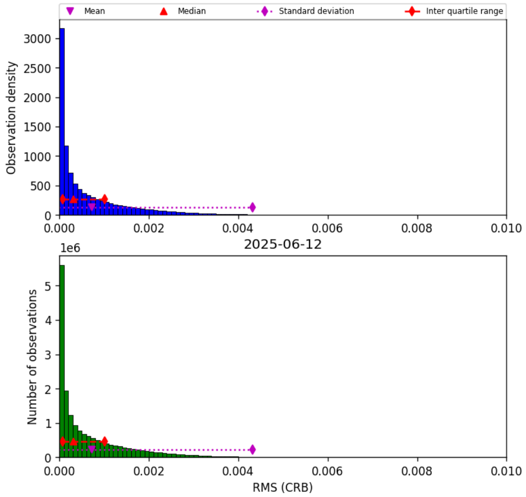
Figure 46: Histogram of "RMS (CRB)" for 2025-06-12 to 2025-06-13
