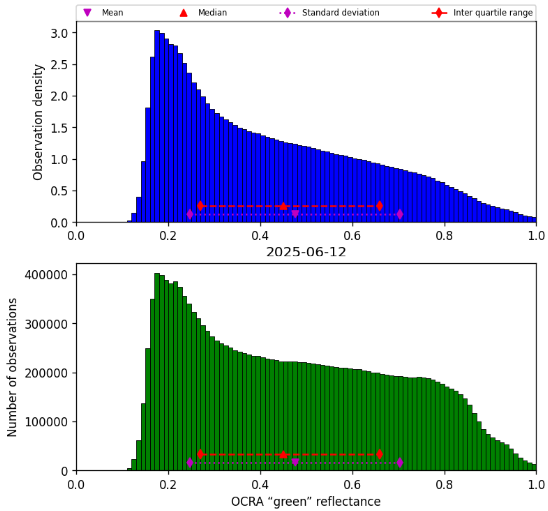
Figure 50: Histogram of “OCRA “green” reflectance” for 2025-06-12 to 2025-06-13
