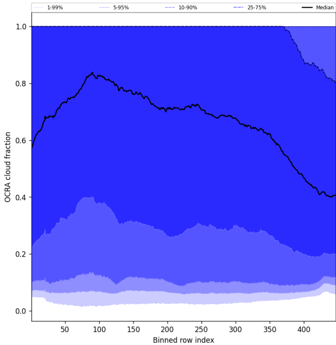
Figure 64: Along track statistics of “OCRA cloud fraction” for 2025-06-12 to 2025-06-13
