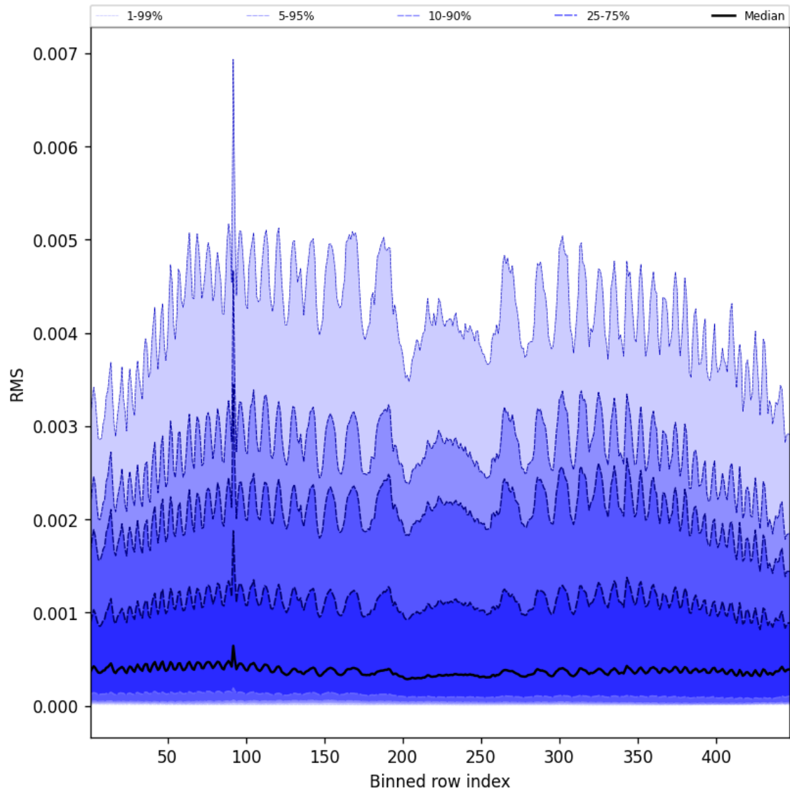
Figure 61: Along track statistics of “RMS” for 2025-06-12 to 2025-06-13
