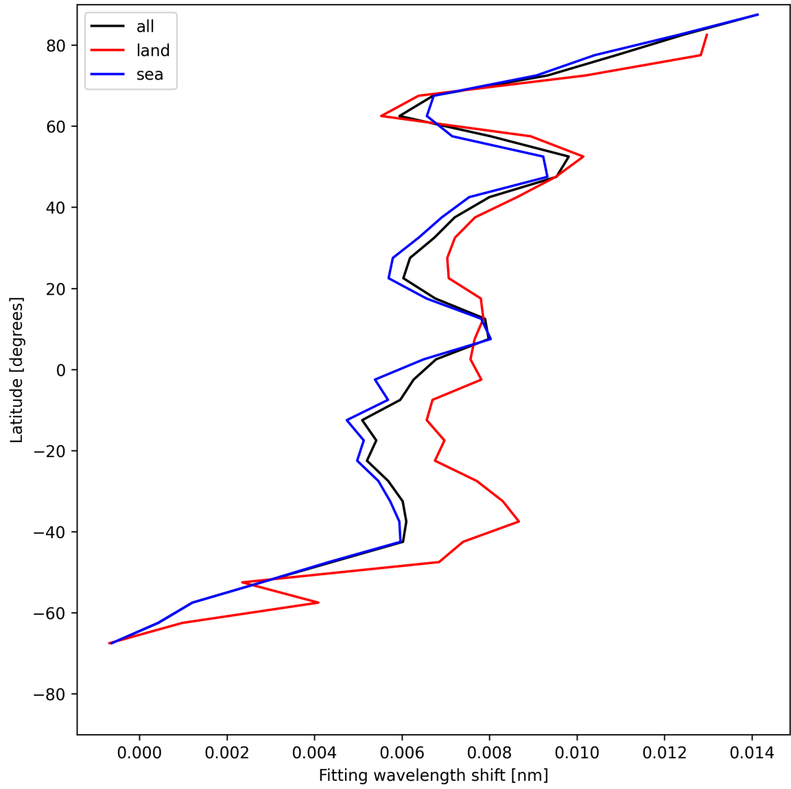
Figure 31: Zonal average of “Fitting wavelength shift” for 2025-06-12 to 2025-06-13.
