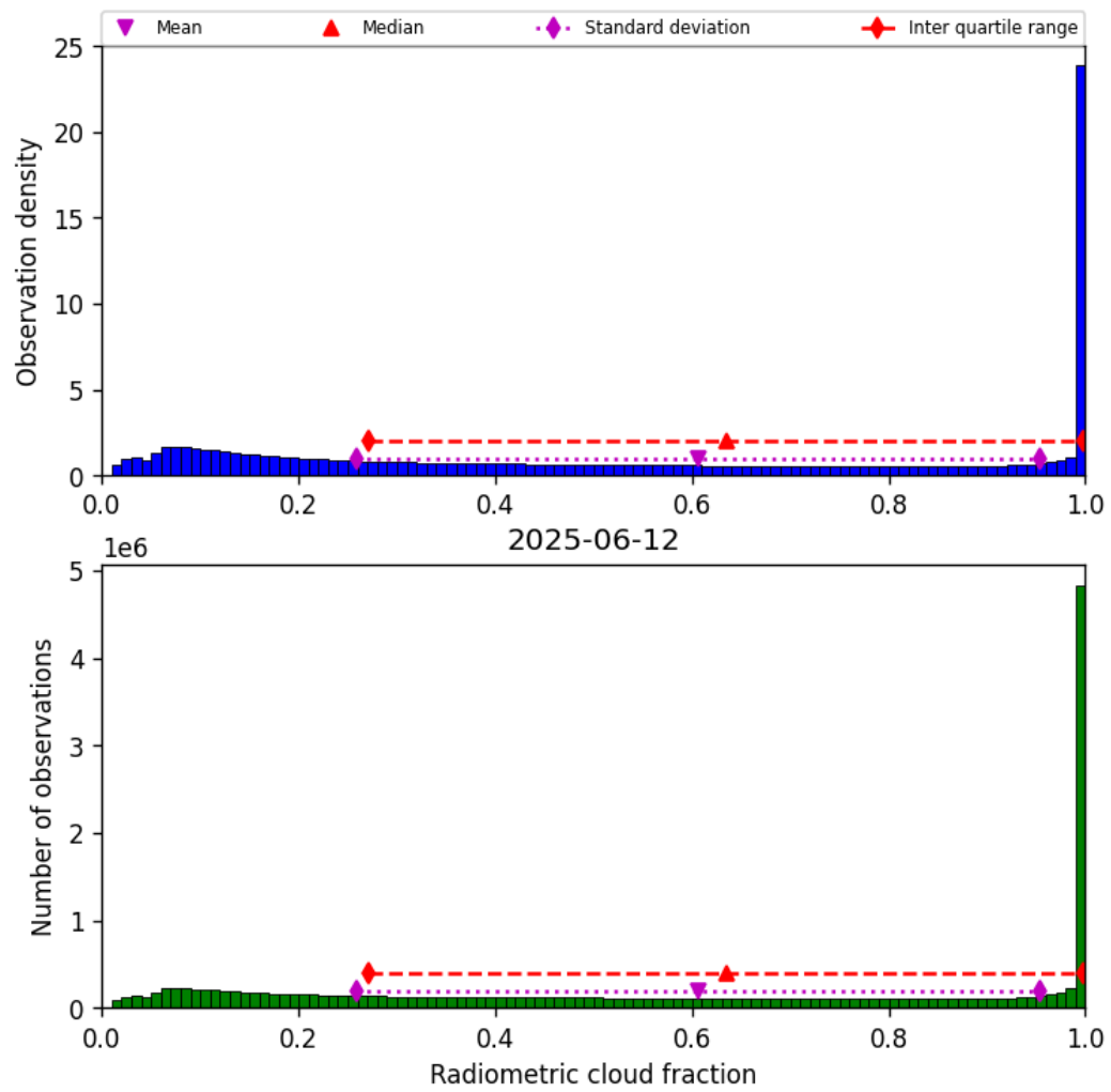
Figure 37: Histogram of “Radiometric cloud fraction” for 2025-06-12 to 2025-06-13
