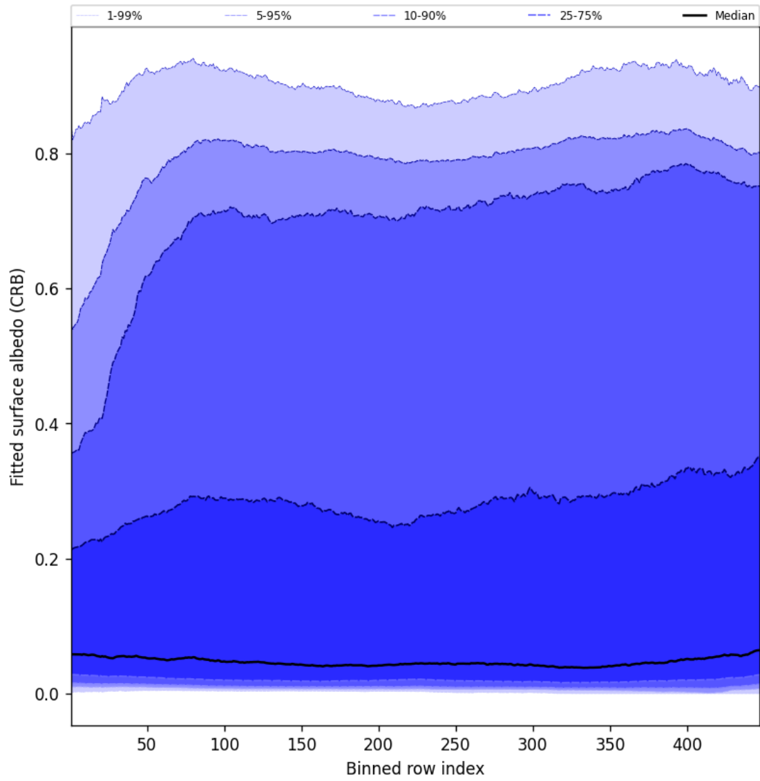
Figure 60: Along track statistics of “Fitted surface albedo (CRB)” for 2025-06-12 to 2025-06-13
