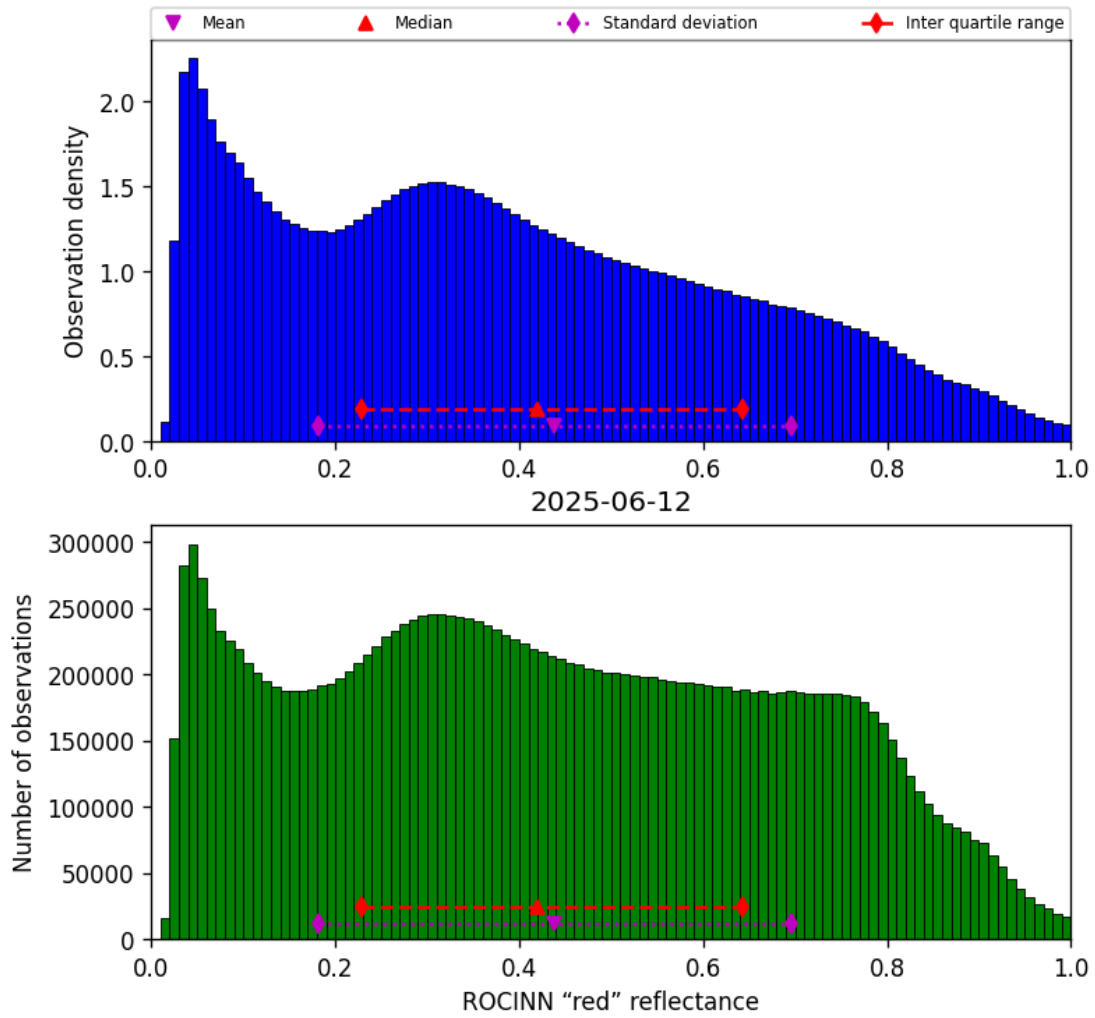
Figure 51: Histogram of “ROCINN “red” reflectance” for 2025-06-12 to 2025-06-13
