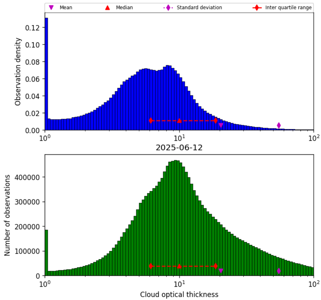
Figure 39: Histogram of “Cloud optical thickness” for 2025-06-12 to 2025-06-13
