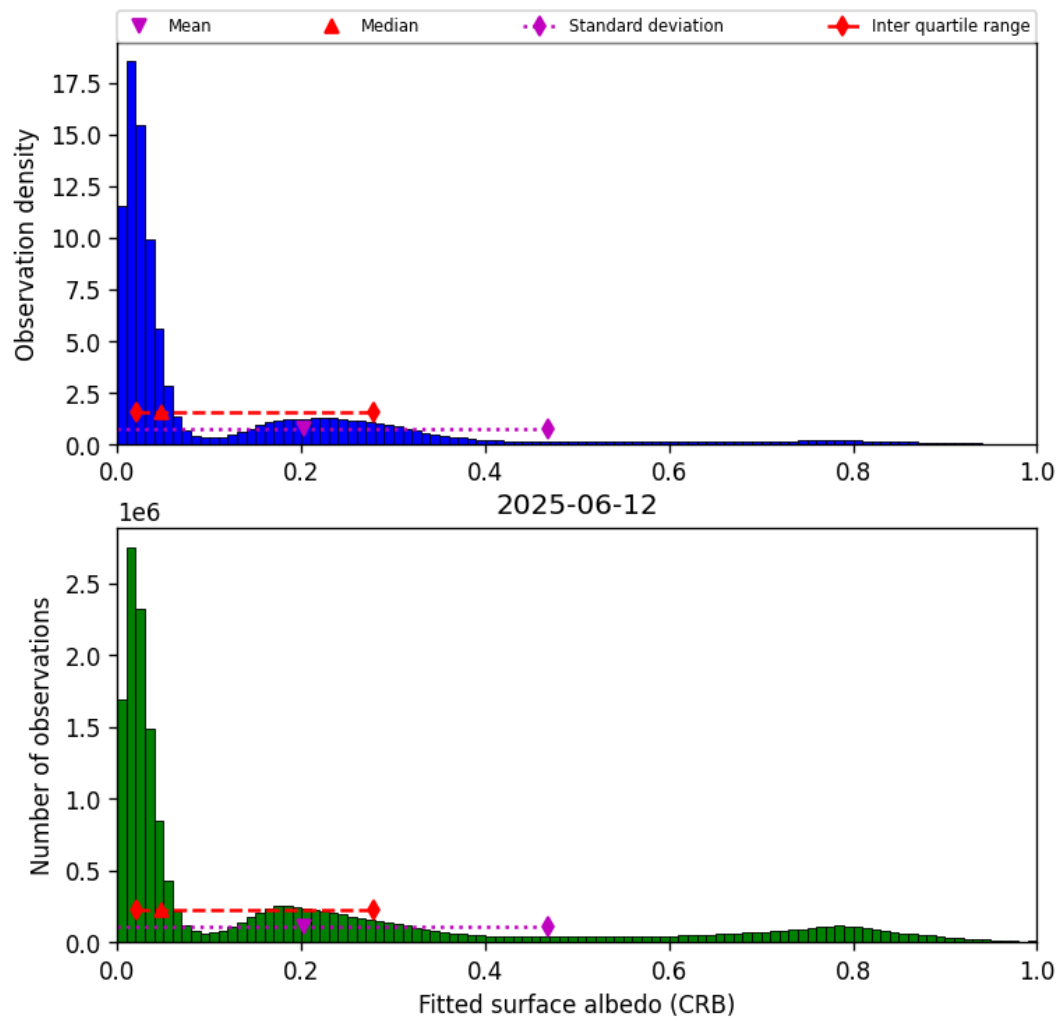
Figure 44: Histogram of “Fitted surface albedo (CRB)” for 2025-06-12 to 2025-06-13
