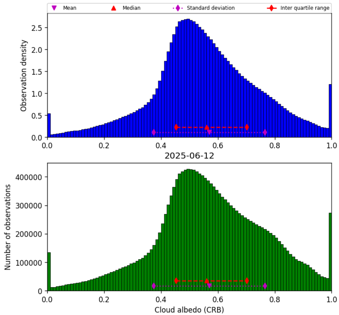
Figure 42: Histogram of “Cloud albedo (CRB)” for 2025-06-12 to 2025-06-13
