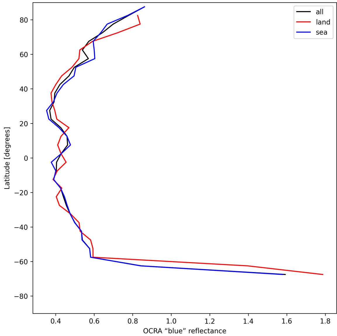
Figure 33: Zonal average of “OCRA “blue” reflectance” for 2025-06-12 to 2025-06-13.
