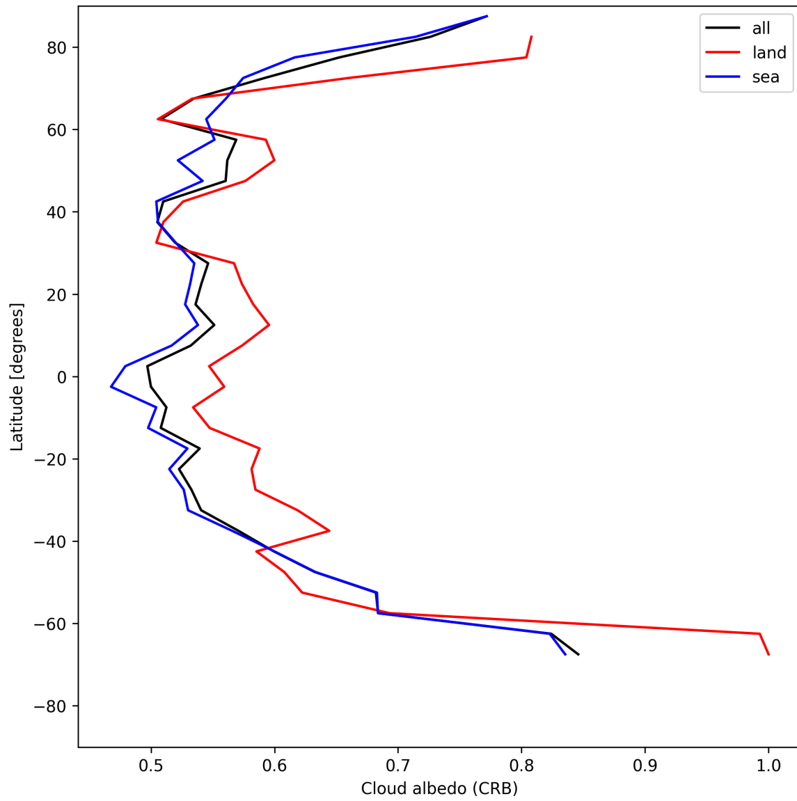
Figure 26: Zonal average of “Cloud albedo (CRB)” for 2025-06-12 to 2025-06-13.
