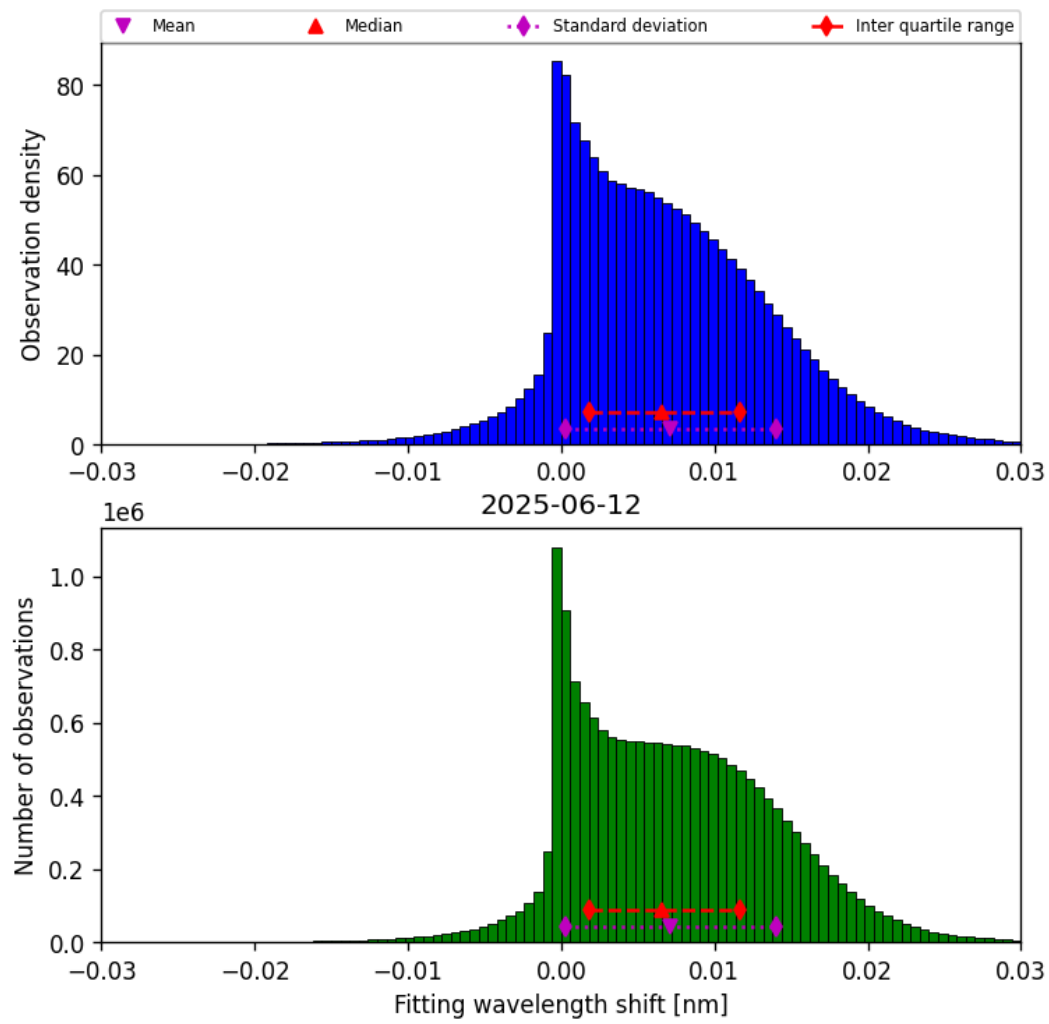
Figure 47: Histogram of “Fitting wavelength shift” for 2025-06-12 to 2025-06-13
