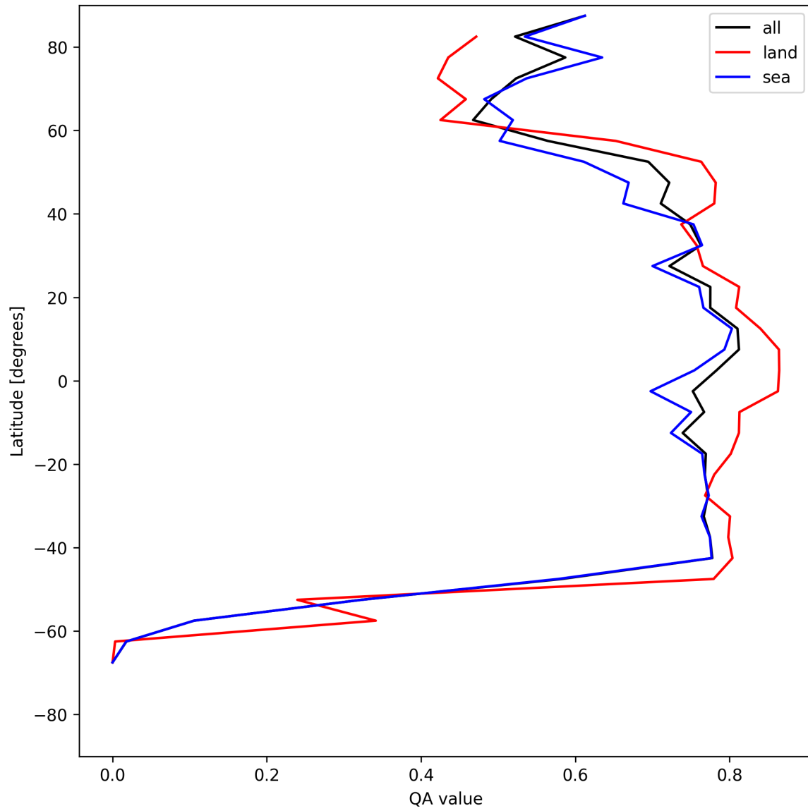
Figure 20: Zonal average of “QA value” for 2025-06-12 to 2025-06-13.
