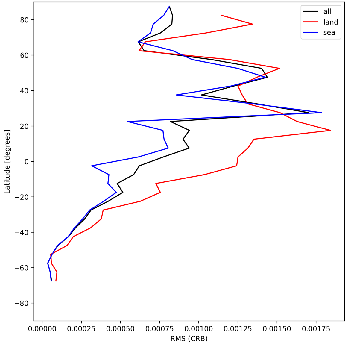
Figure 30: Zonal average of “RMS (CRB)” for 2025-06-12 to 2025-06-13.
