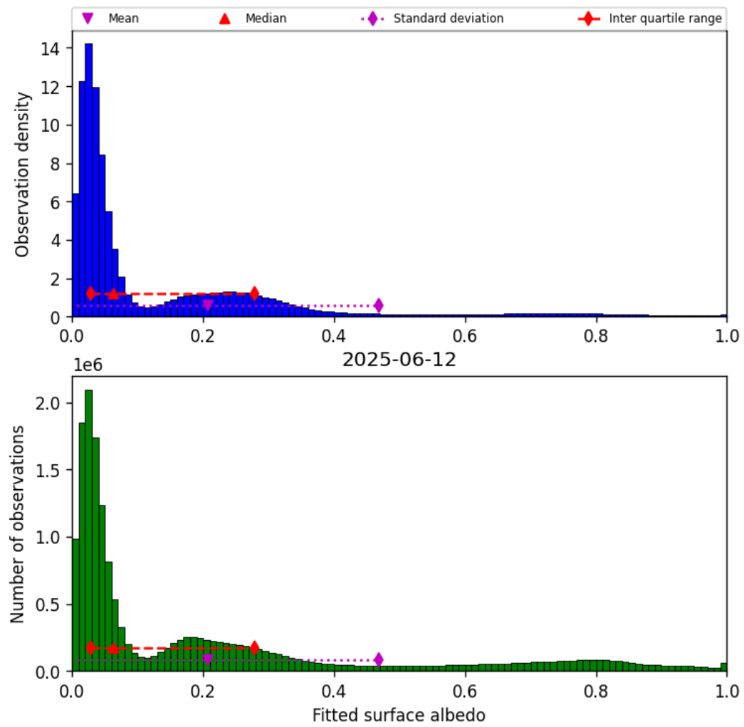
Figure 43: Histogram of “Fitted surface albedo” for 2025-06-12 to 2025-06-13
