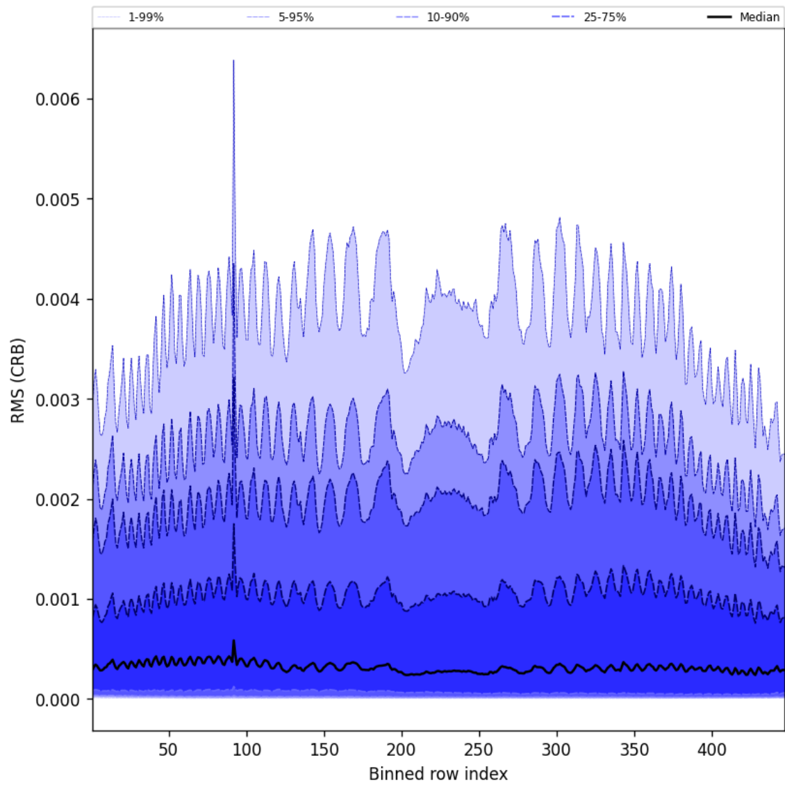
Figure 62: Along track statistics of “RMS (CRB)” for 2025-06-12 to 2025-06-13
