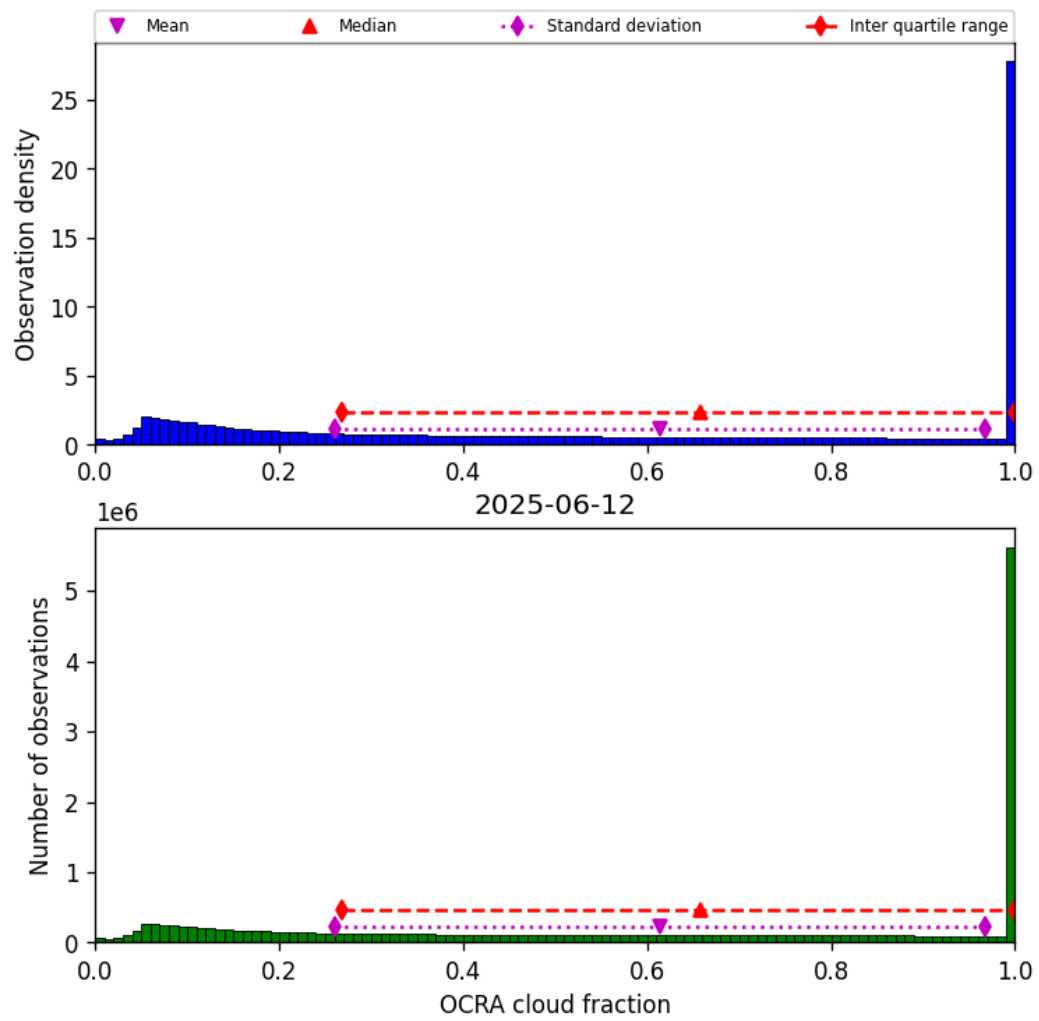
Figure 48: Histogram of “OCRA cloud fraction” for 2025-06-12 to 2025-06-13
