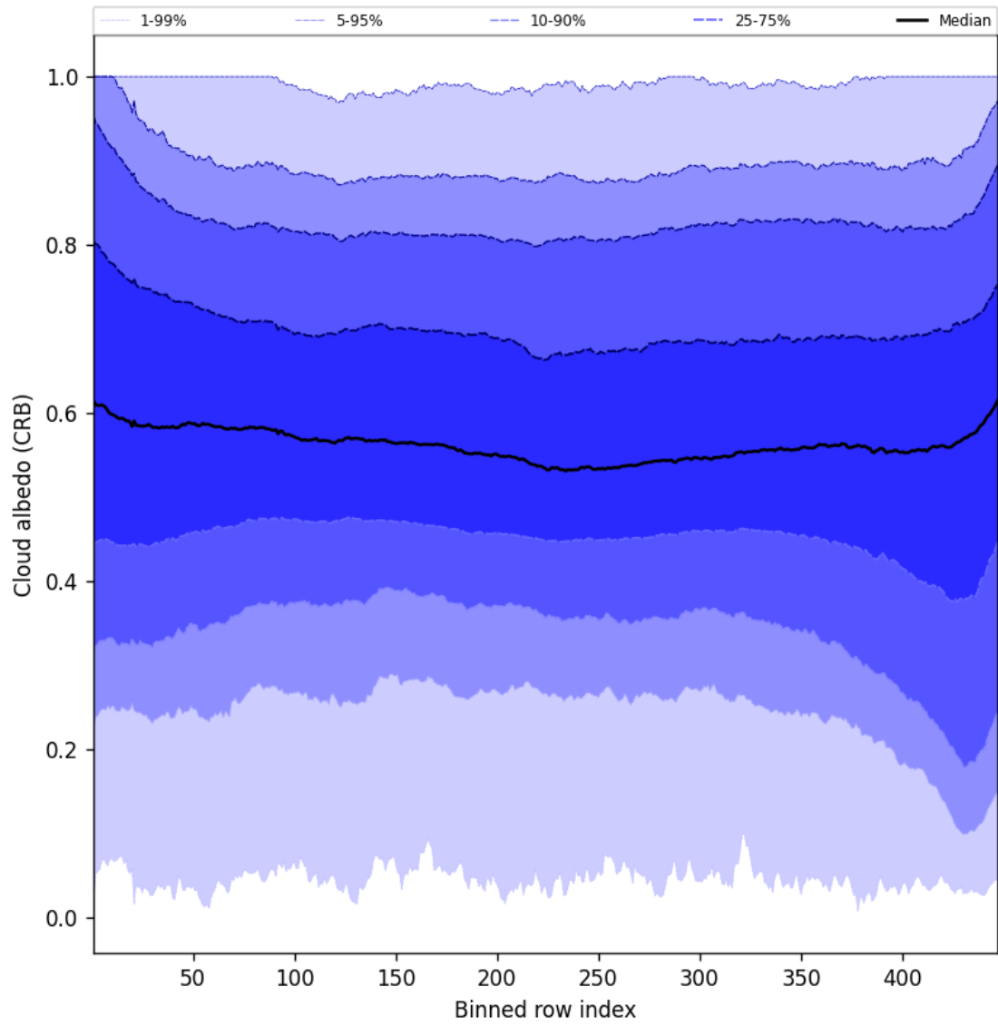
Figure 58: Along track statistics of “Cloud albedo (CRB)” for 2025-06-12 to 2025-06-13
