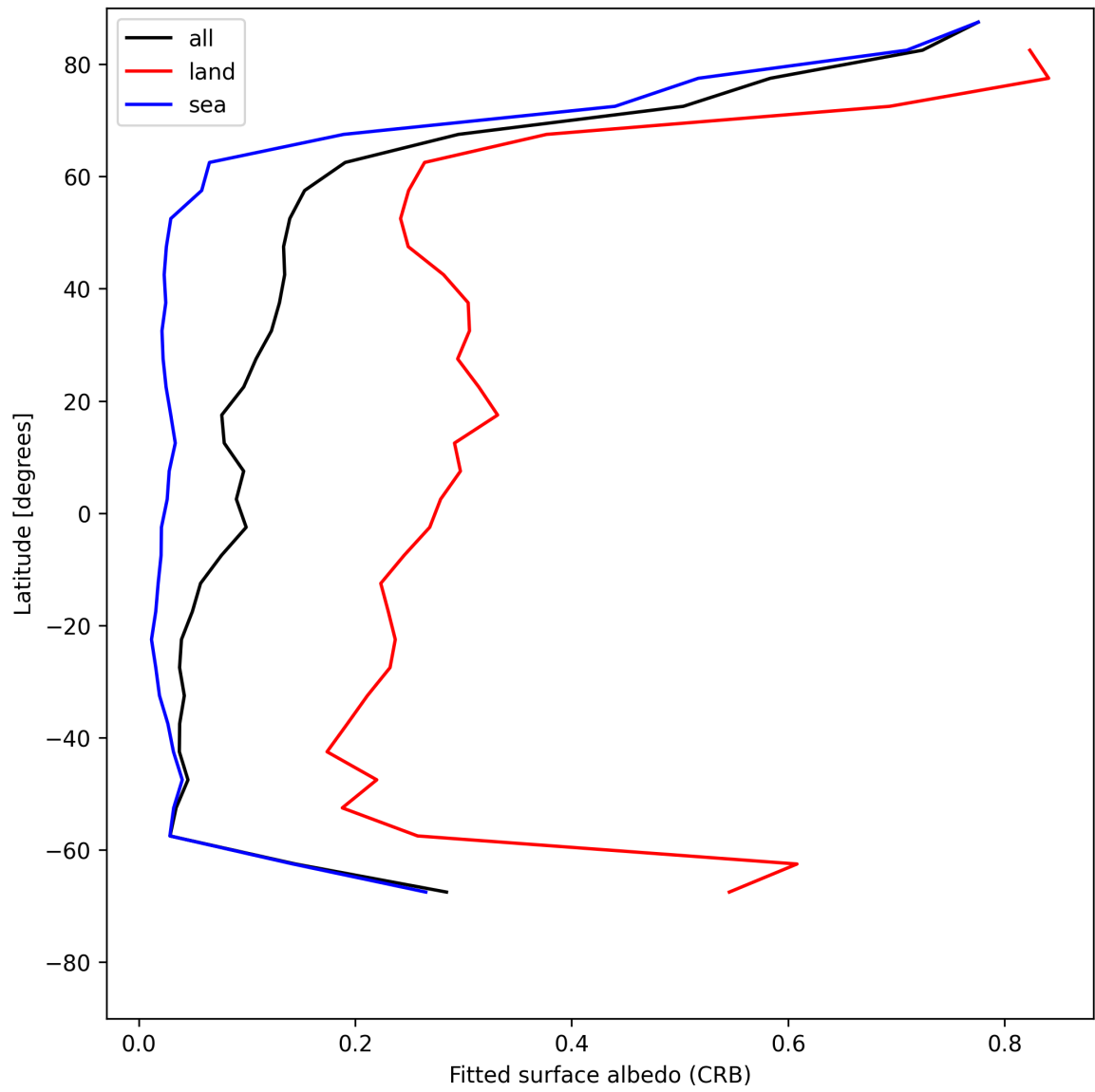
Figure 28: Zonal average of “Fitted surface albedo (CRB)” for 2025-06-12 to 2025-06-13.
