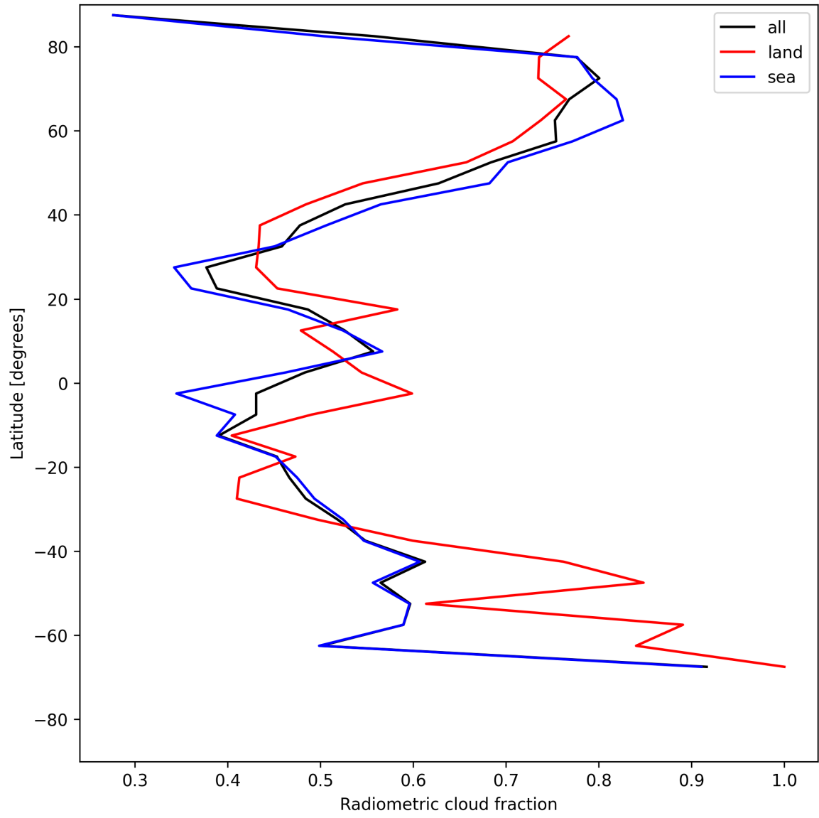
Figure 21: Zonal average of “Radiometric cloud fraction” for 2025-06-12 to 2025-06-13.
