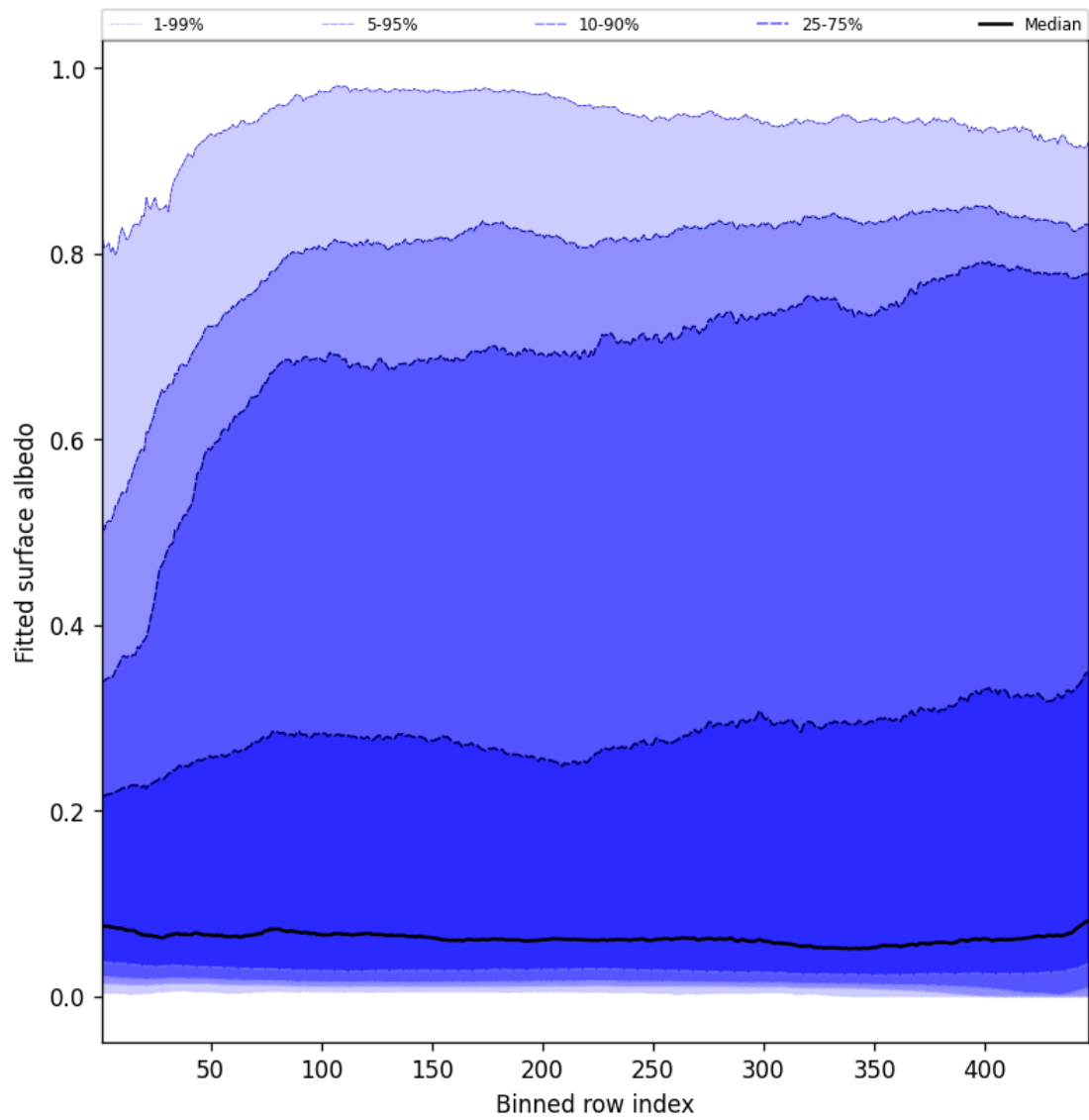
Figure 59: Along track statistics of “Fitted surface albedo” for 2025-06-12 to 2025-06-13
