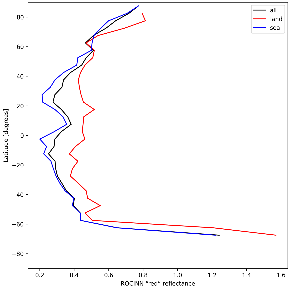
Figure 35: Zonal average of “ROCINN “red” reflectance” for 2025-06-12 to 2025-06-13.
