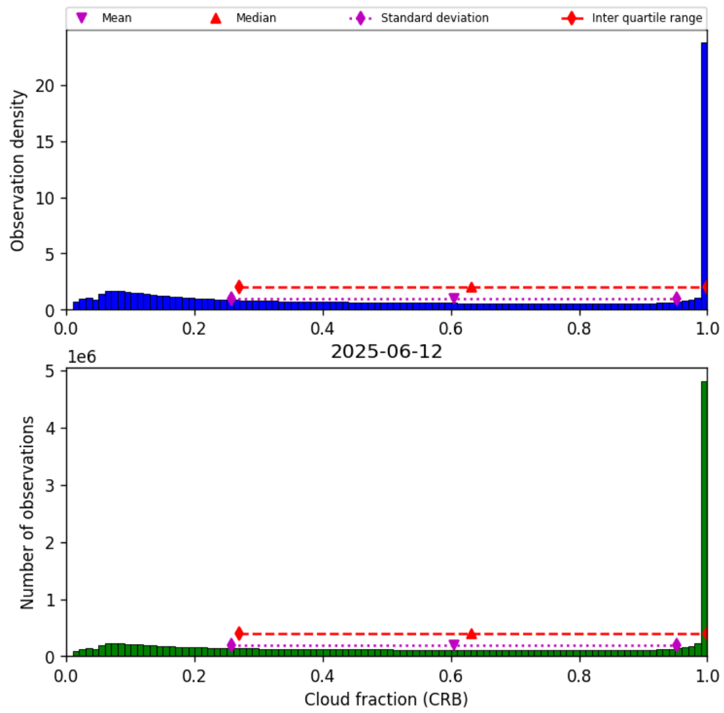
Figure 40: Histogram of “Cloud fraction (CRB)” for 2025-06-12 to 2025-06-13
