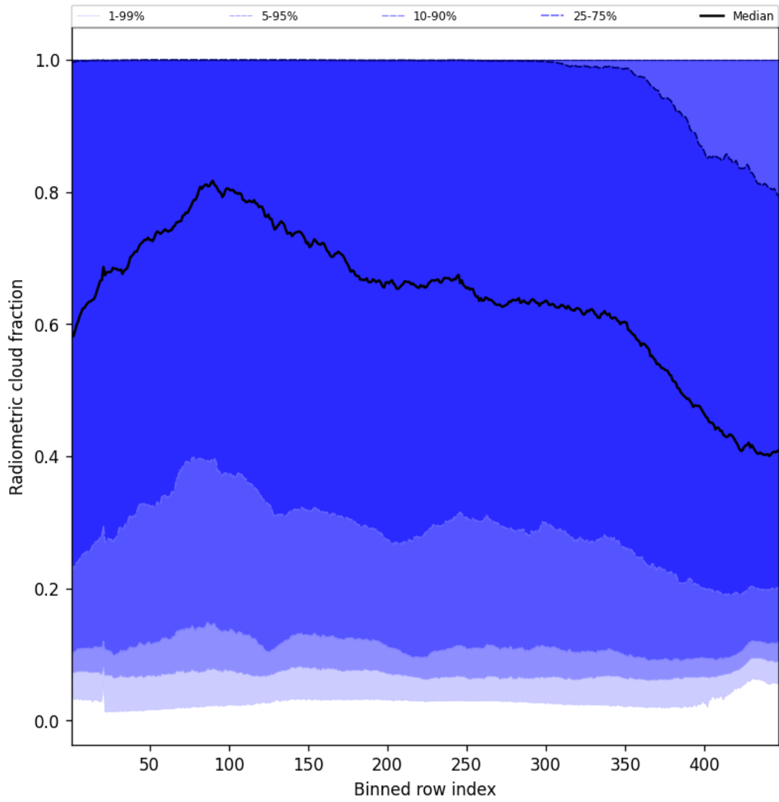
Figure 53: Along track statistics of "Radiometric cloud fraction" for 2025-06-12 to 2025-06-13
