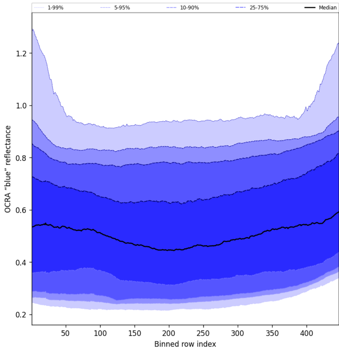
Figure 65: Along track statistics of "OCRA "blue" reflectance" for 2025-06-12 to 2025-06-13
