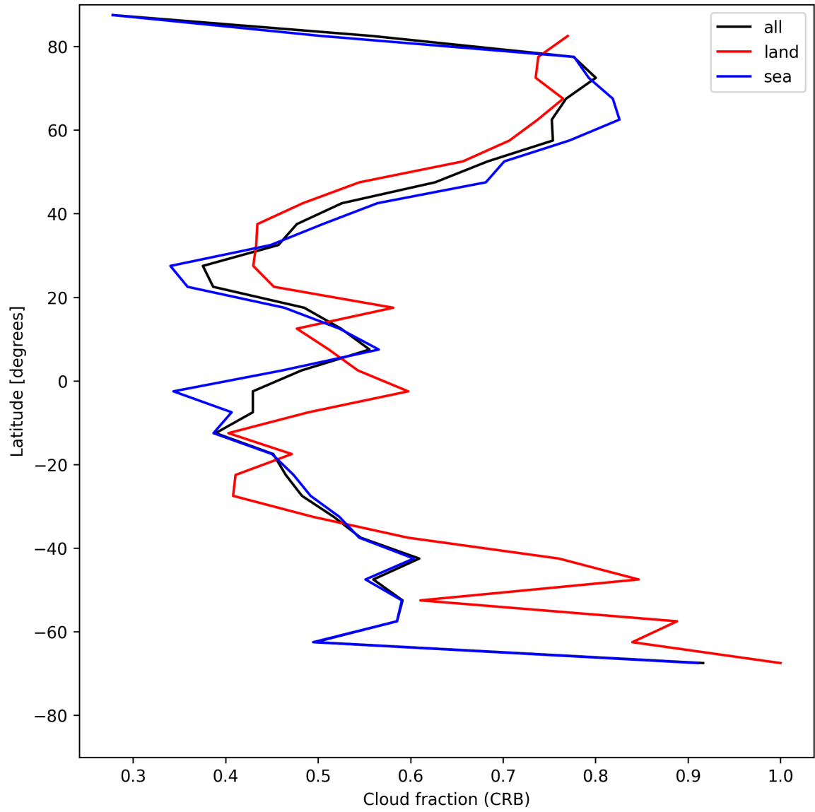
Figure 24: Zonal average of “Cloud fraction (CRB)” for 2025-06-12 to 2025-06-13.
