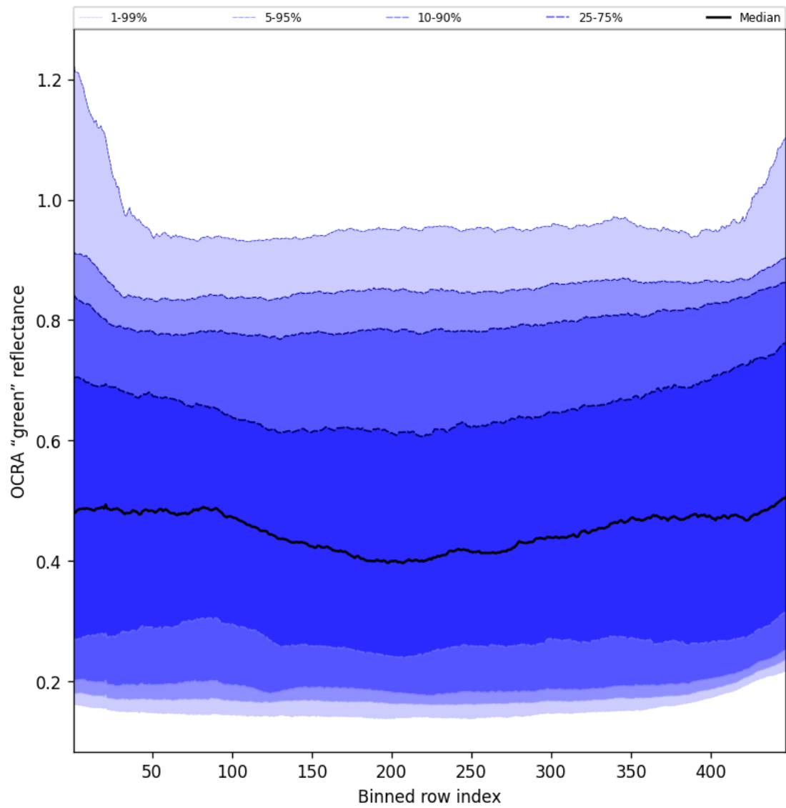
Figure 66: Along track statistics of “OCRA “green” reflectance” for 2025-06-12 to 2025-06-13
