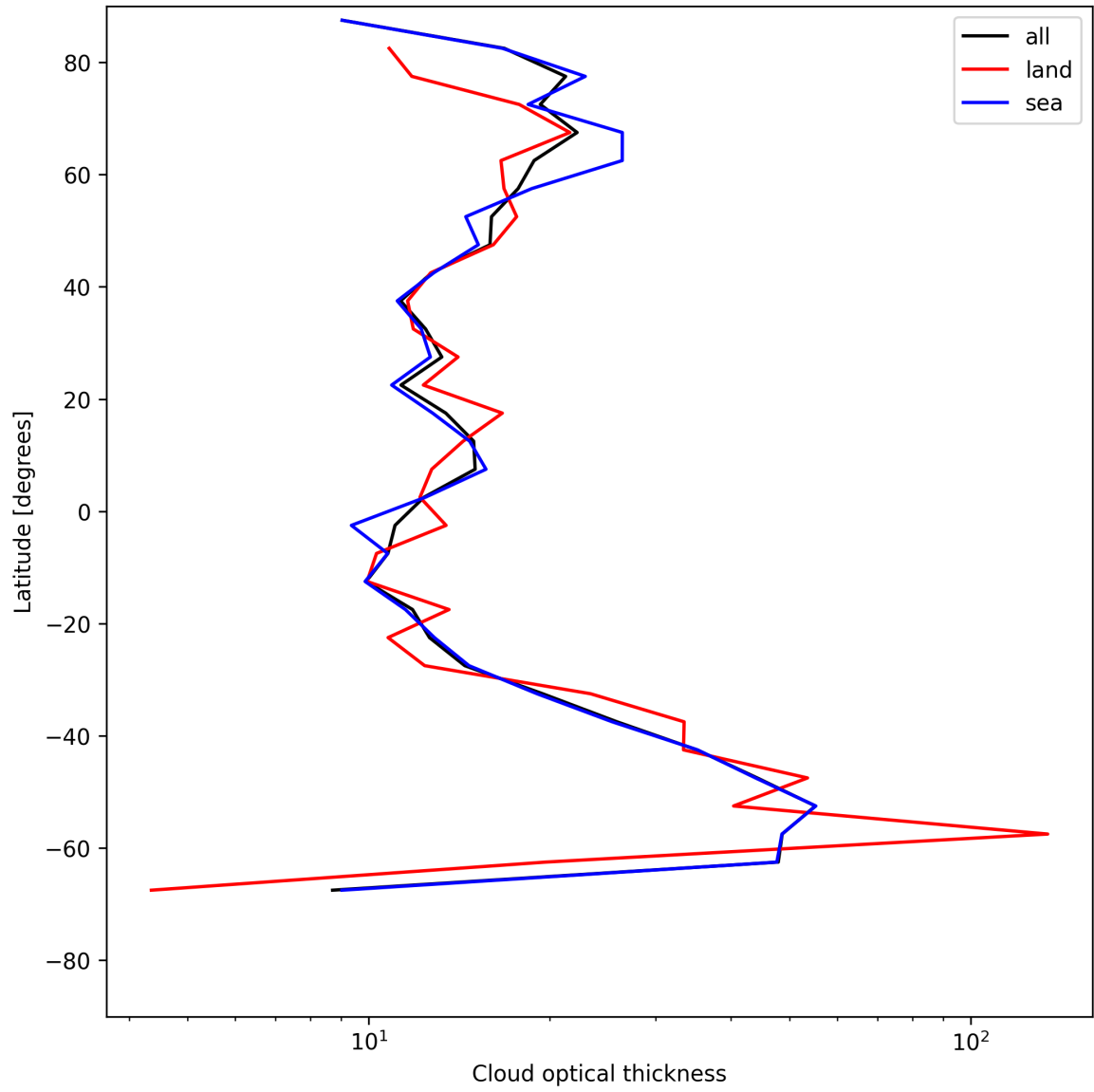
Figure 23: Zonal average of “Cloud optical thickness” for 2025-06-12 to 2025-06-13.
