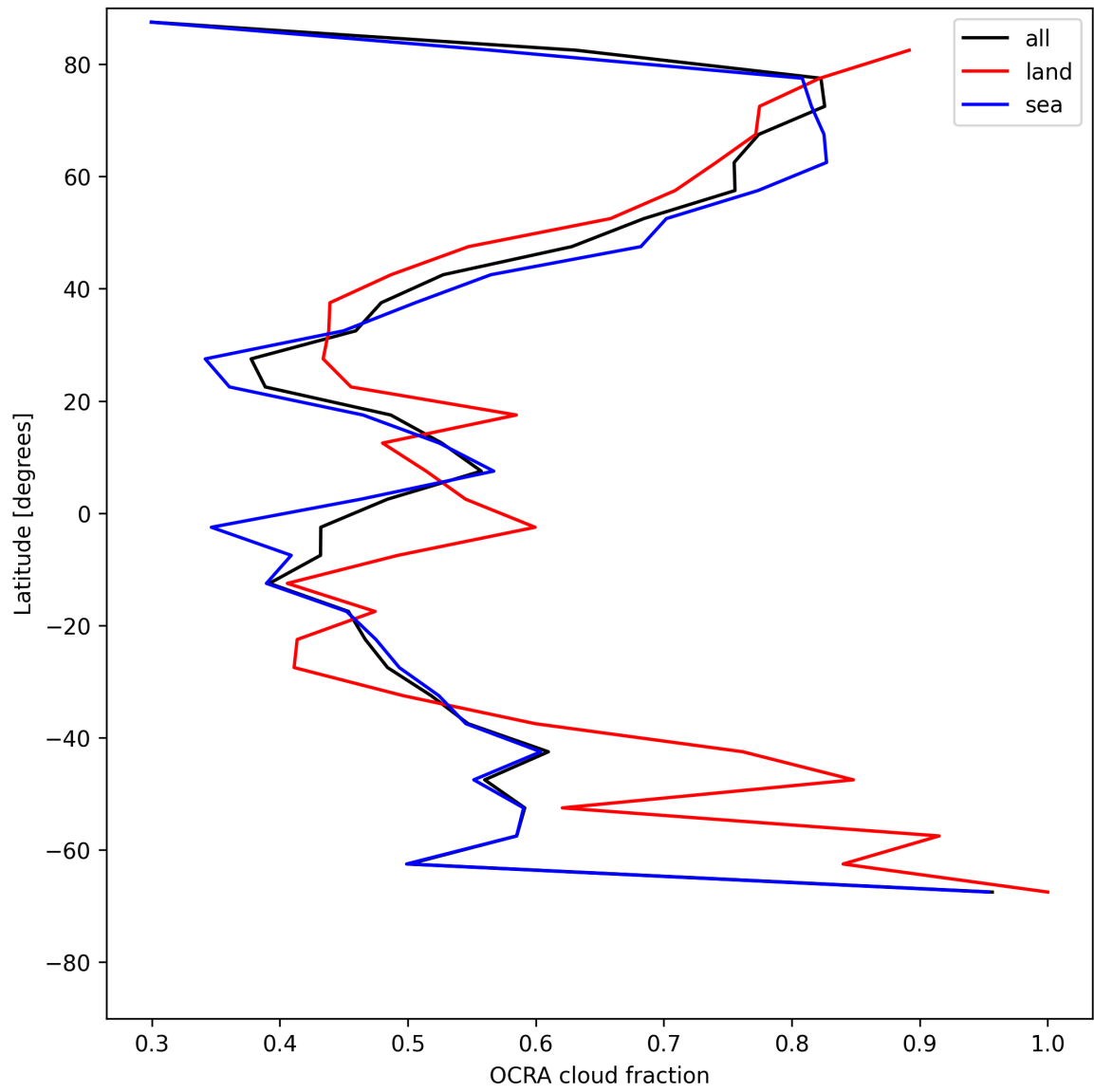
Figure 32: Zonal average of “OCRA cloud fraction” for 2025-06-12 to 2025-06-13.
