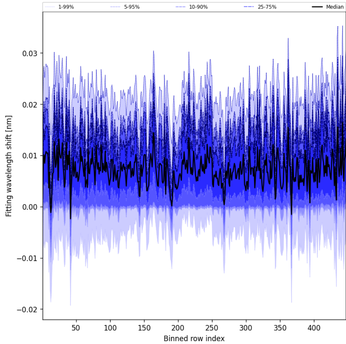
Figure 63: Along track statistics of “Fitting wavelength shift” for 2025-06-12 to 2025-06-13
