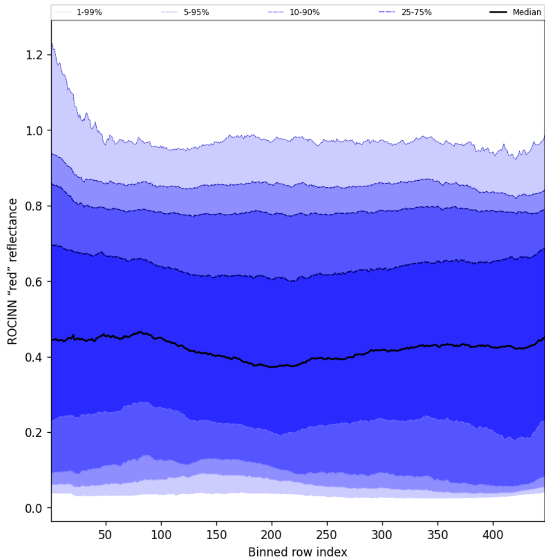
Figure 67: Along track statistics of “ROCINN “red” reflectance” for 2025-06-12 to 2025-06-13
