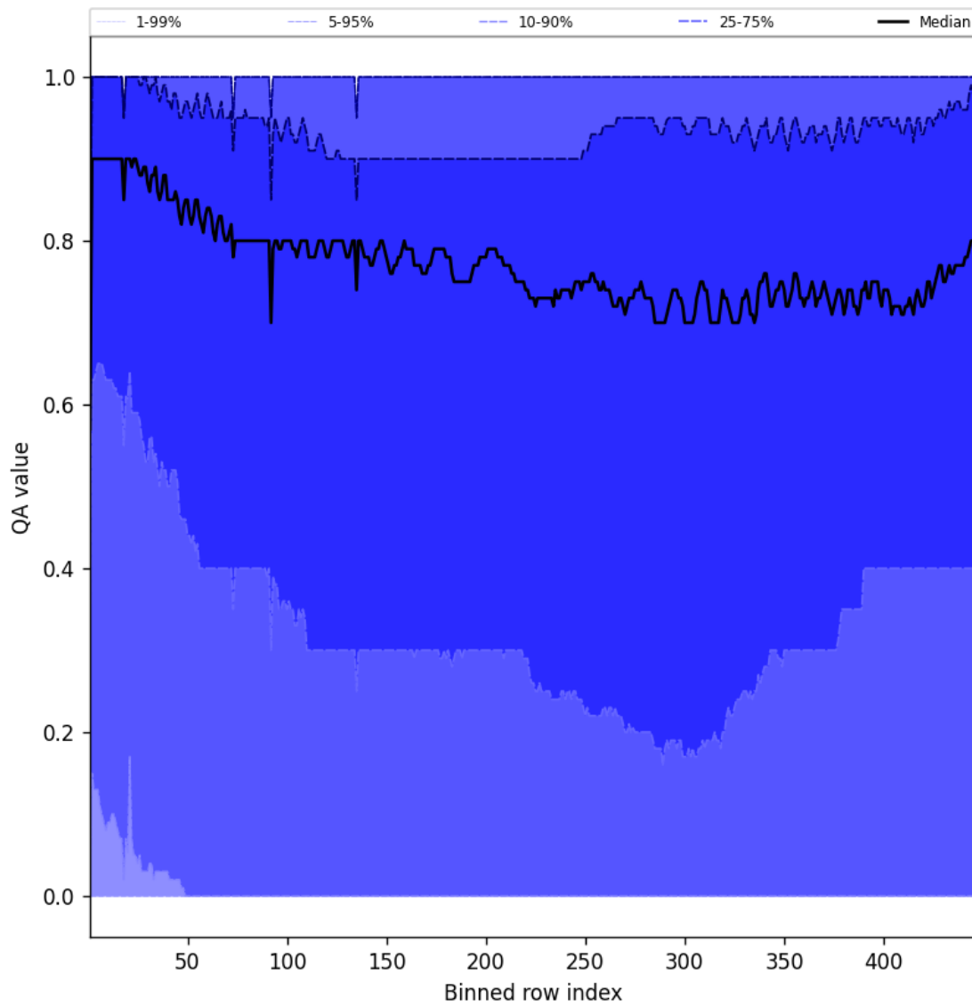
Figure 52: Along track statistics of “QA value” for 2025-06-12 to 2025-06-13
