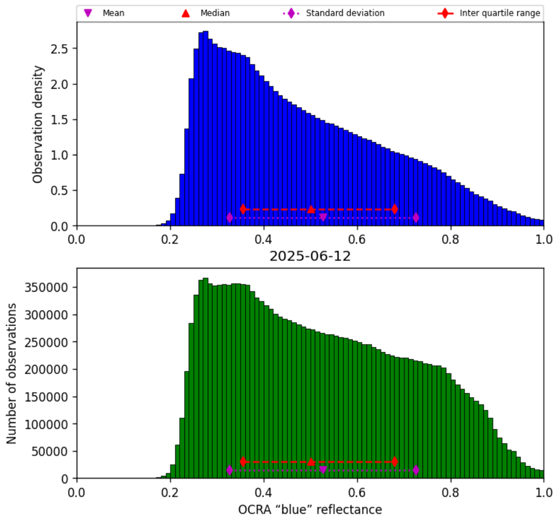
Figure 49: Histogram of “OCRA “blue” reflectance” for 2025-06-12 to 2025-06-13
