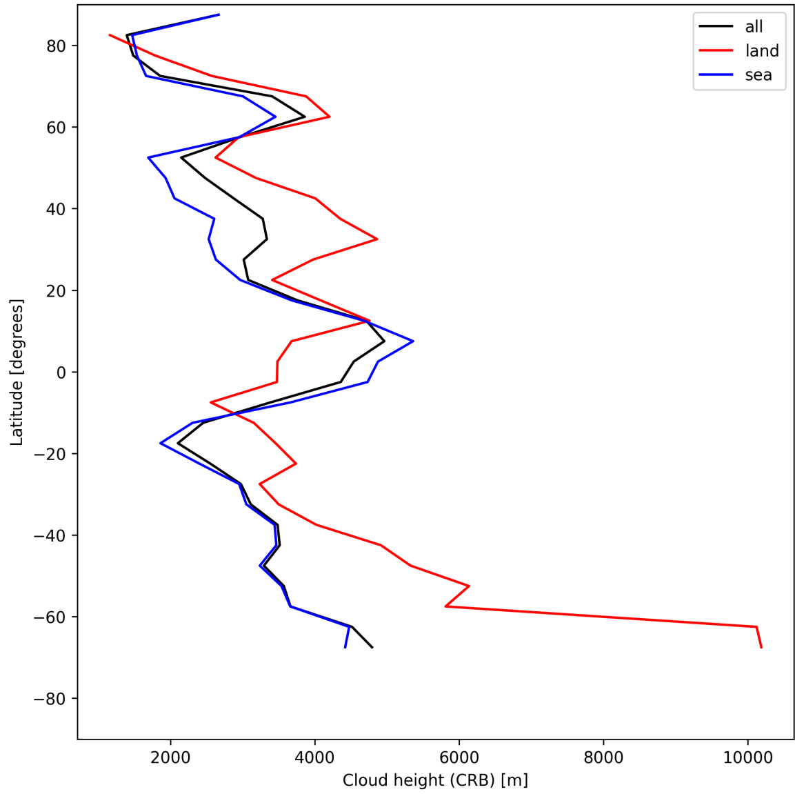
Figure 25: Zonal average of “Cloud height (CRB)” for 2025-06-12 to 2025-06-13.
