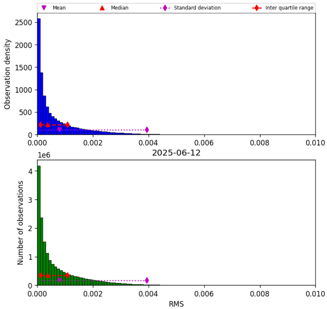
Figure 45: Histogram of “RMS” for 2025-06-12 to 2025-06-13
