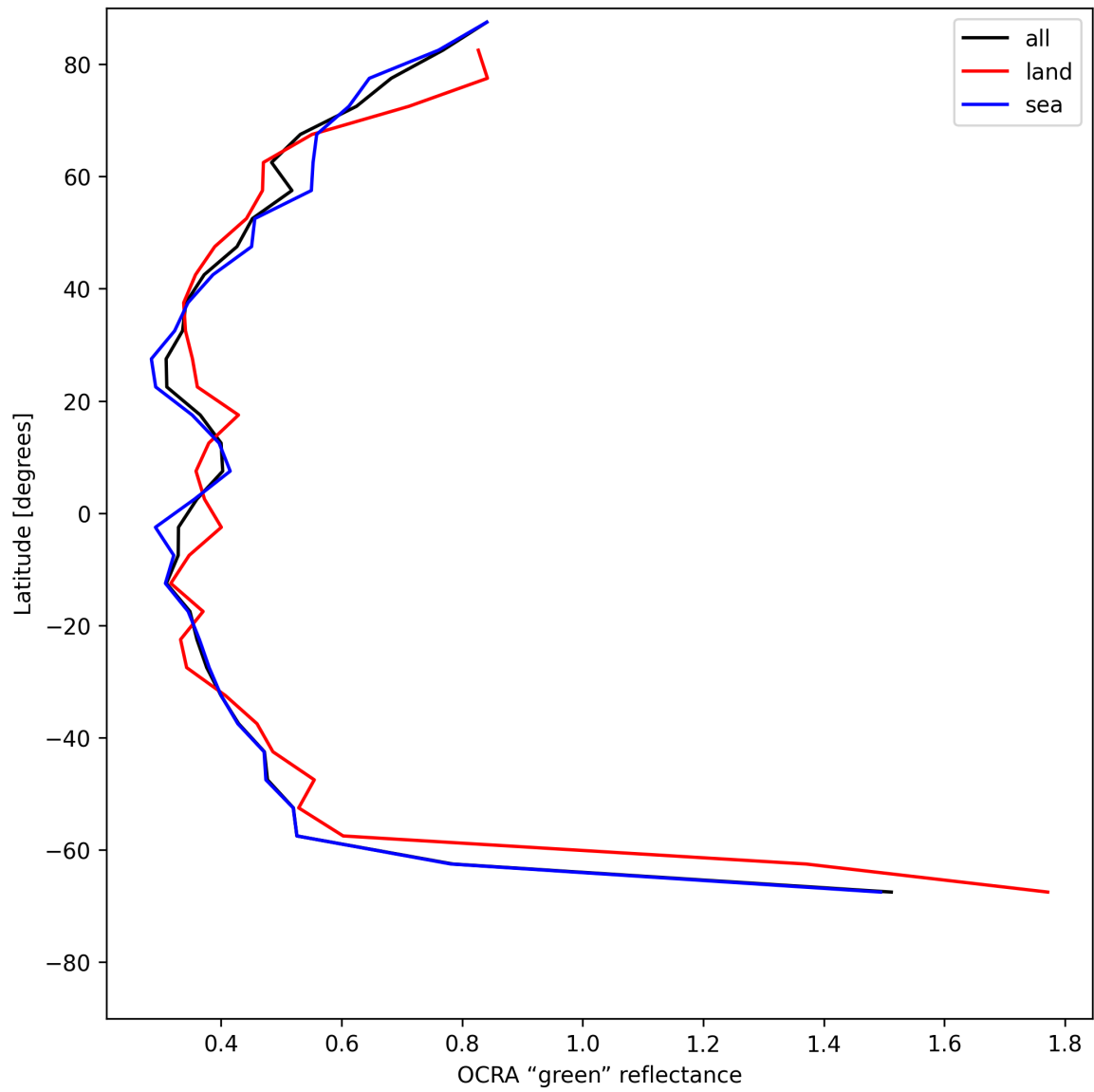
Figure 34: Zonal average of “OCRA “green” reflectance” for 2025-06-12 to 2025-06-13.
