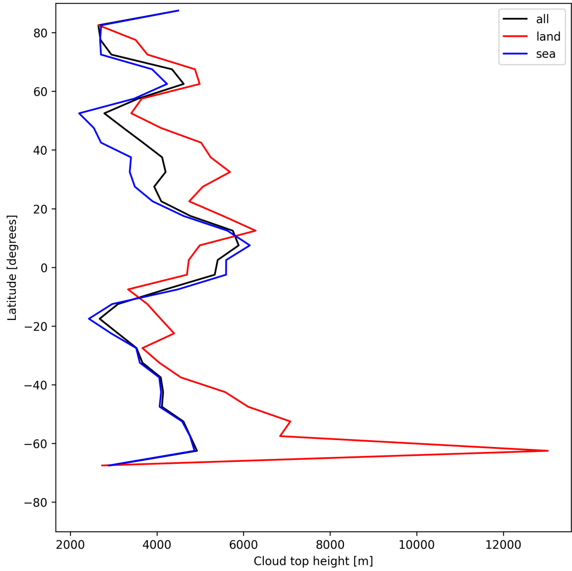
Figure 22: Zonal average of “Cloud top height” for 2025-06-12 to 2025-06-13.
