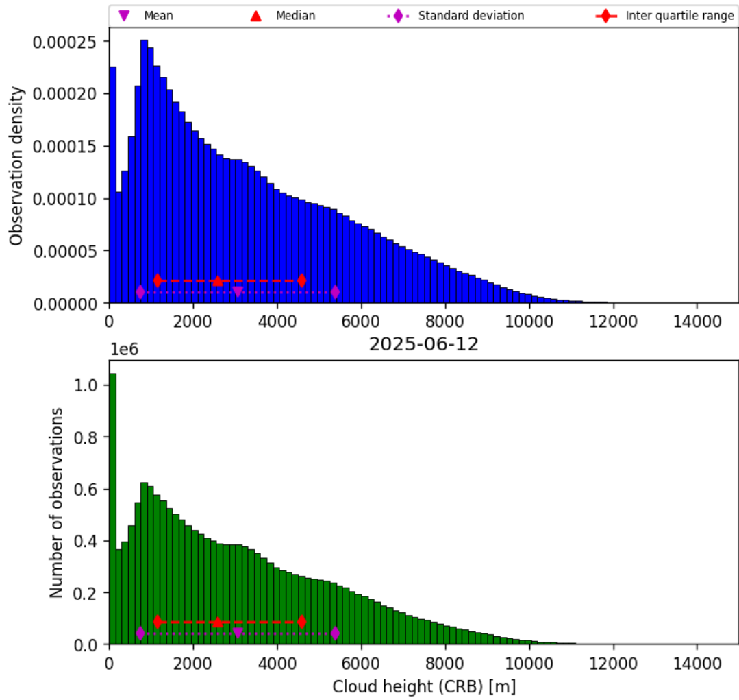
Figure 41: Histogram of “Cloud height (CRB)” for 2025-06-12 to 2025-06-13
