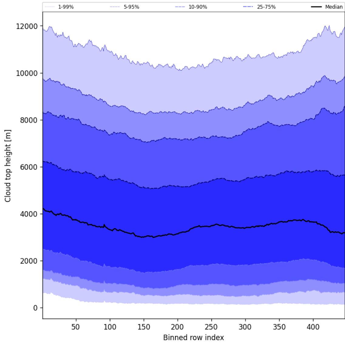
Figure 54: Along track statistics of “Cloud top height” for 2025-06-12 to 2025-06-13
