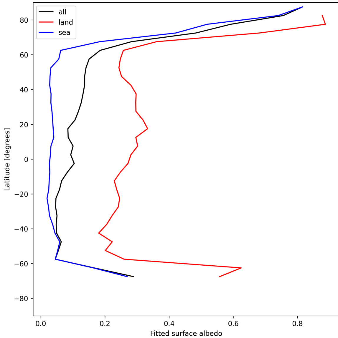
Figure 27: Zonal average of “Fitted surface albedo” for 2025-06-12 to 2025-06-13.
