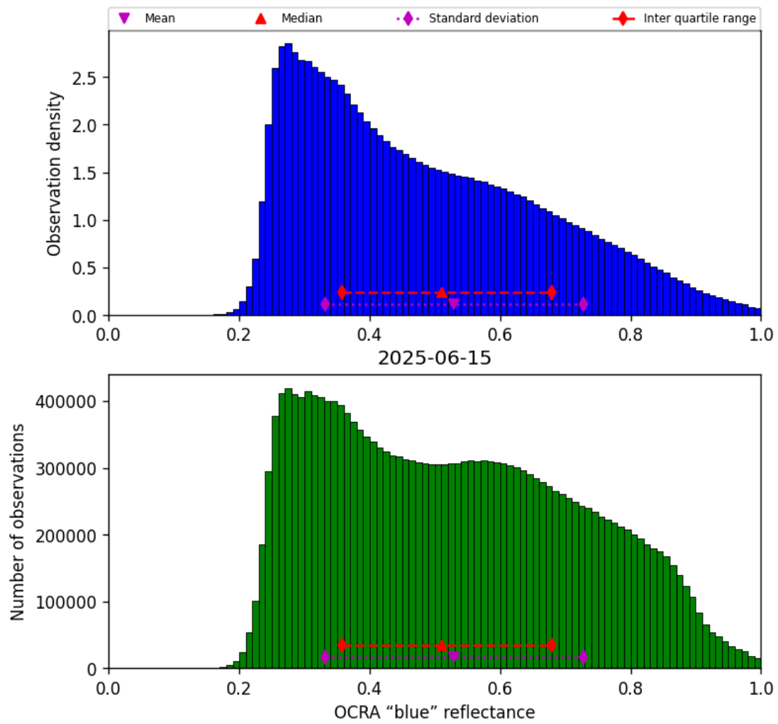
Figure 49: Histogram of “OCRA “blue” reflectance” for 2025-06-15 to 2025-06-16
