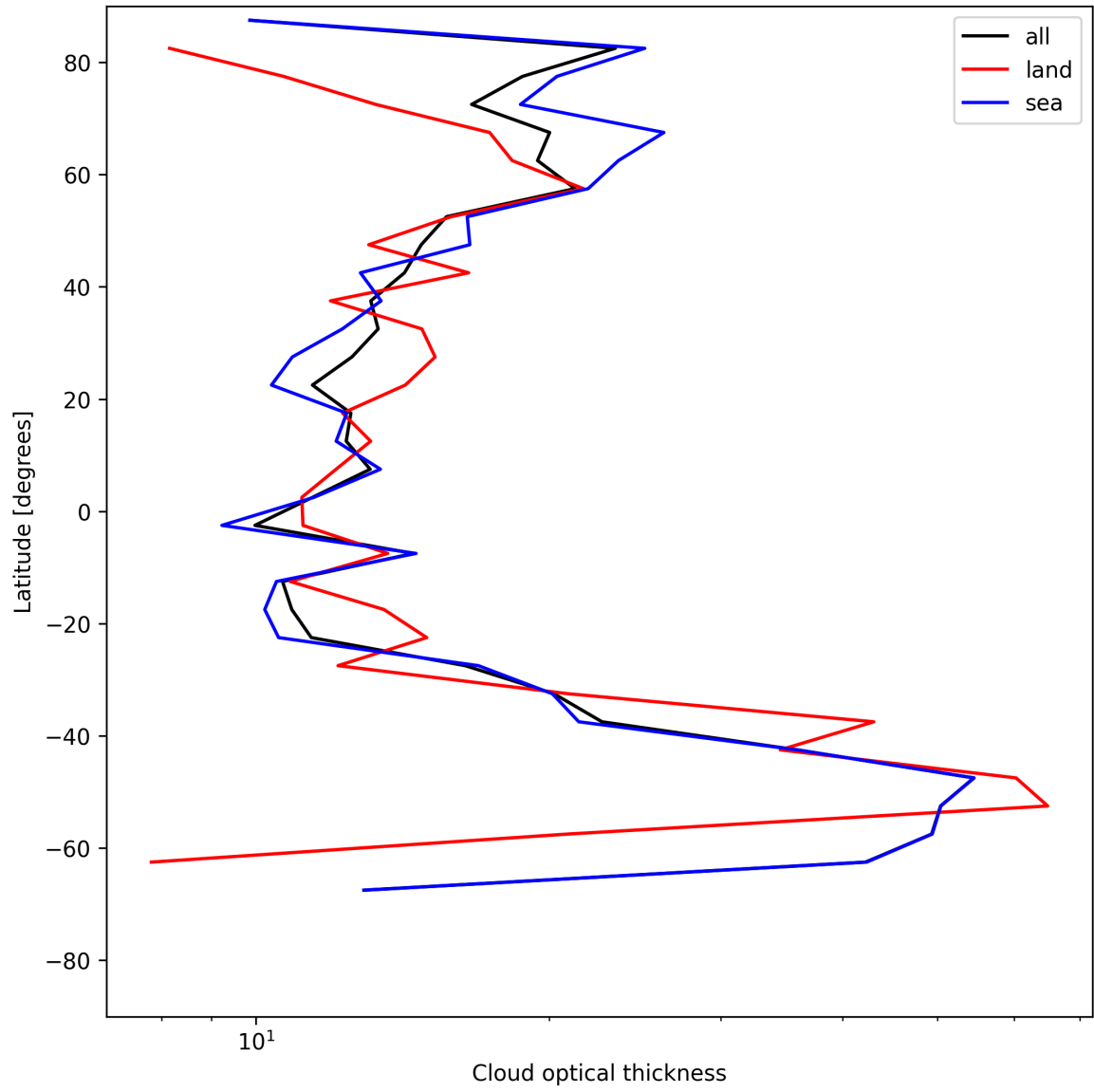
Figure 23: Zonal average of “Cloud optical thickness” for 2025-06-15 to 2025-06-16.
