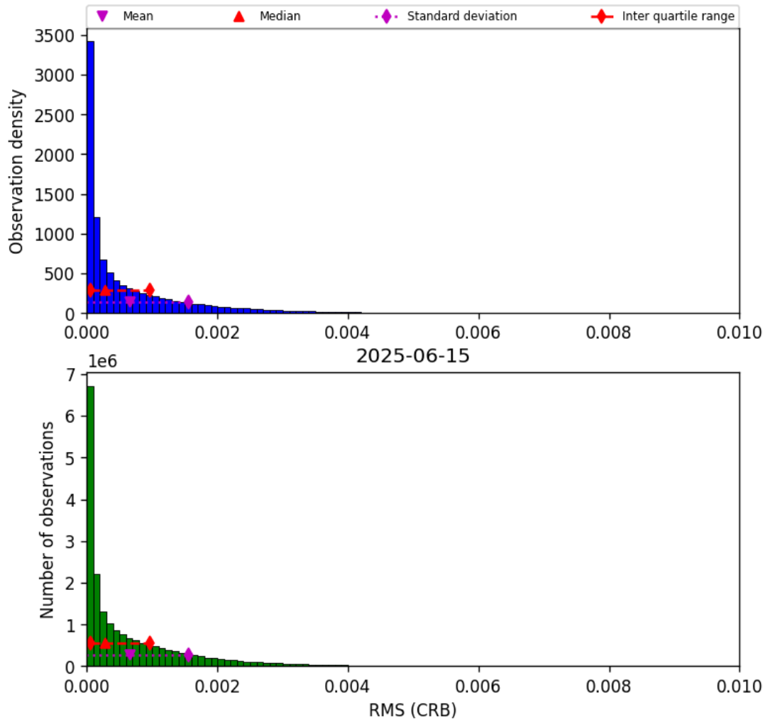
Figure 46: Histogram of “RMS (CRB)” for 2025-06-15 to 2025-06-16
