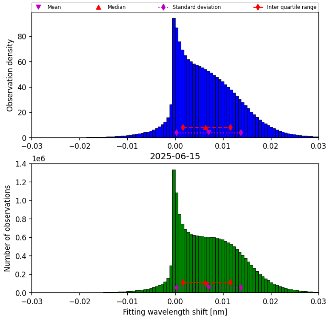
Figure 47: Histogram of “Fitting wavelength shift” for 2025-06-15 to 2025-06-16
