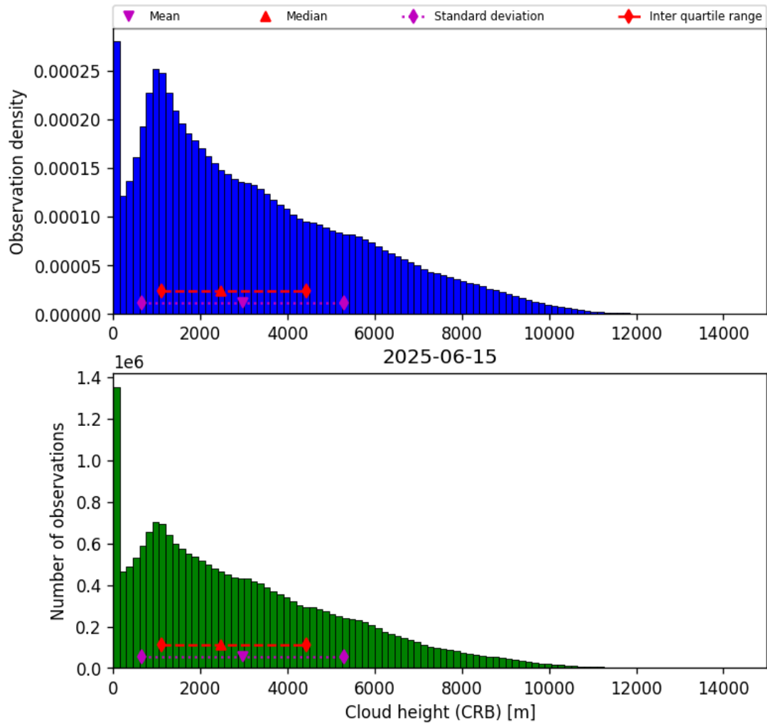
Figure 41: Histogram of “Cloud height (CRB)” for 2025-06-15 to 2025-06-16
