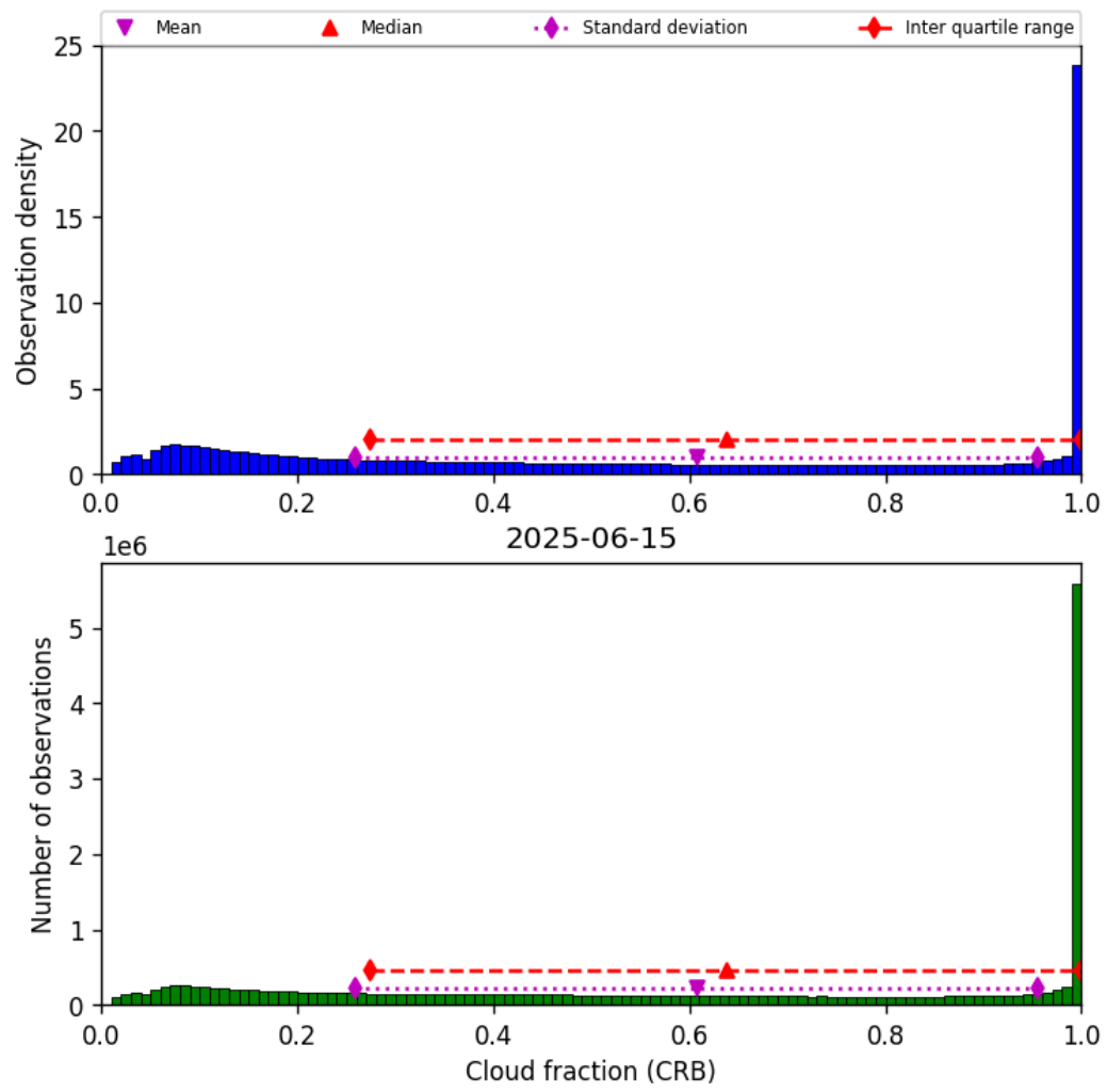
Figure 40: Histogram of “Cloud fraction (CRB)” for 2025-06-15 to 2025-06-16
