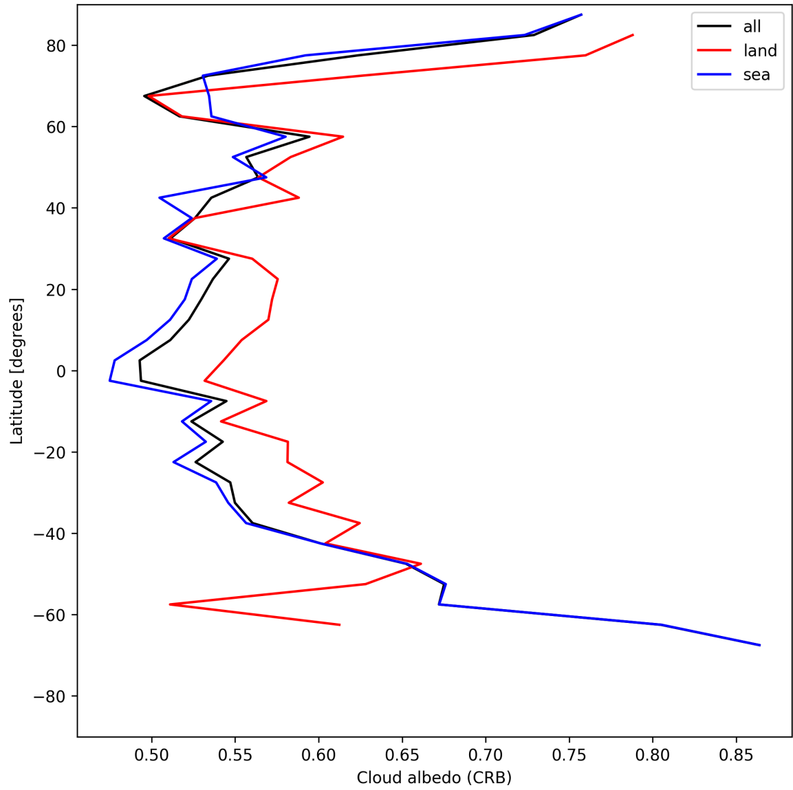
Figure 26: Zonal average of “Cloud albedo (CRB)” for 2025-06-15 to 2025-06-16.
