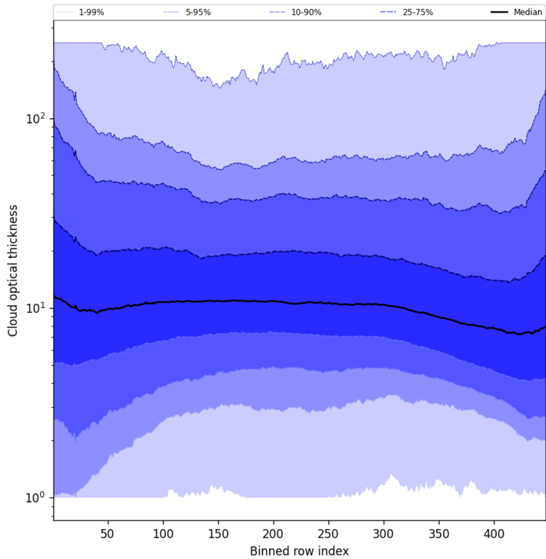
Figure 55: Along track statistics of “Cloud optical thickness” for 2025-06-15 to 2025-06-16
