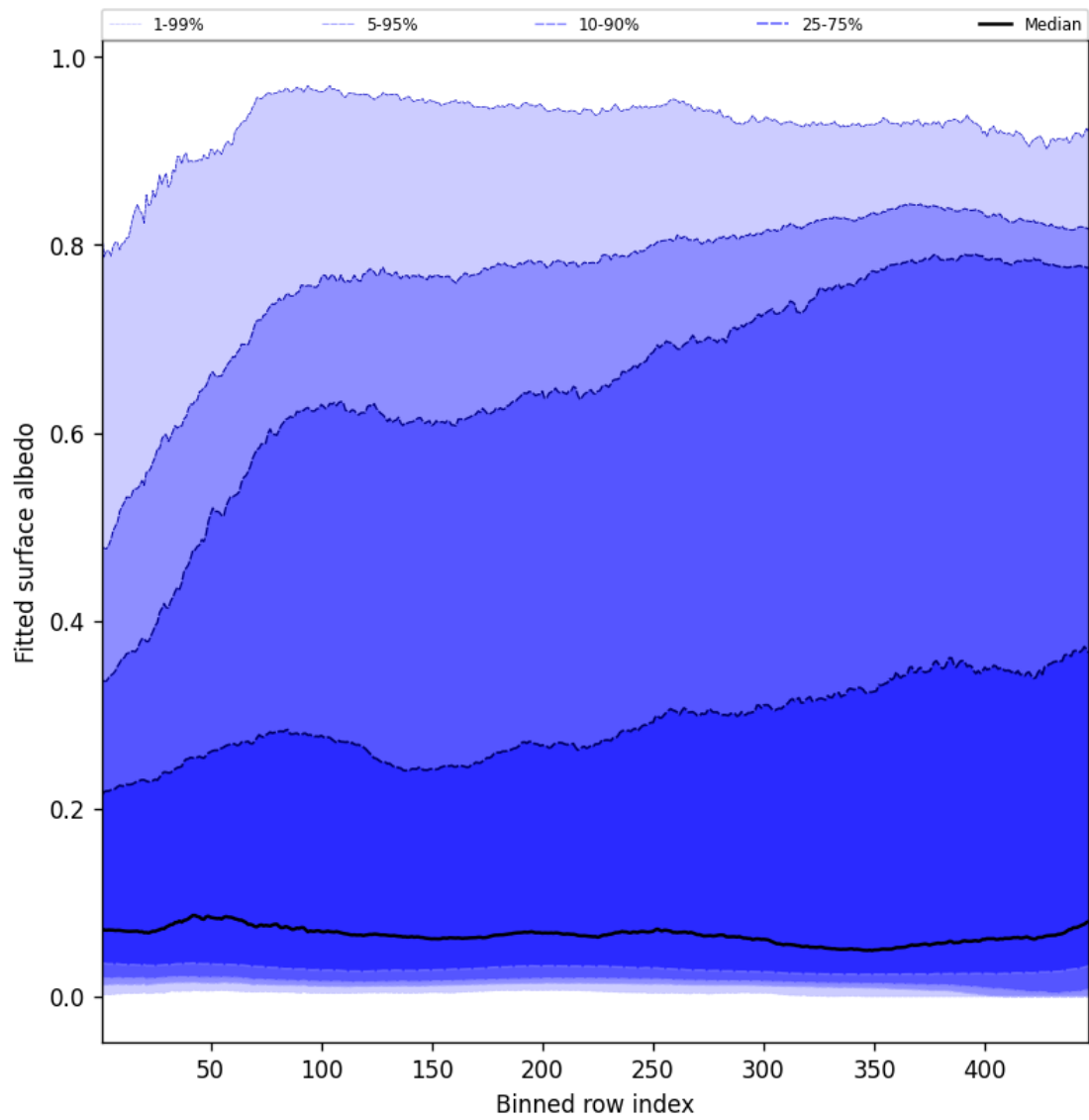
Figure 59: Along track statistics of “Fitted surface albedo” for 2025-06-15 to 2025-06-16
