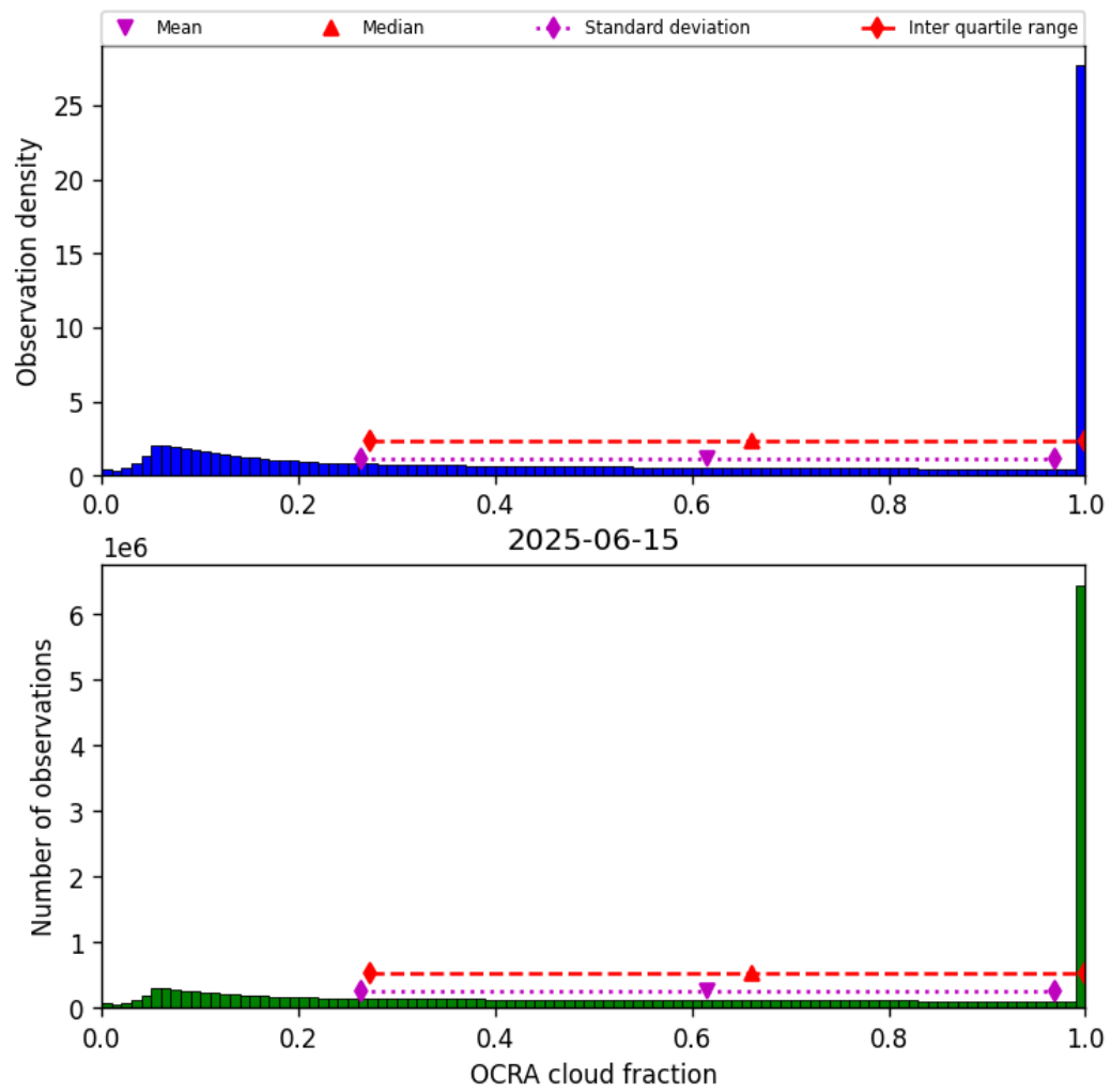
Figure 48: Histogram of “OCRA cloud fraction” for 2025-06-15 to 2025-06-16
