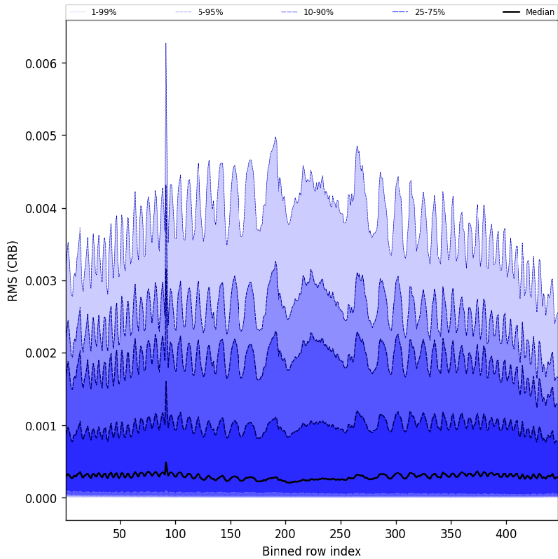
Figure 62: Along track statistics of “RMS (CRB)” for 2025-06-15 to 2025-06-16
