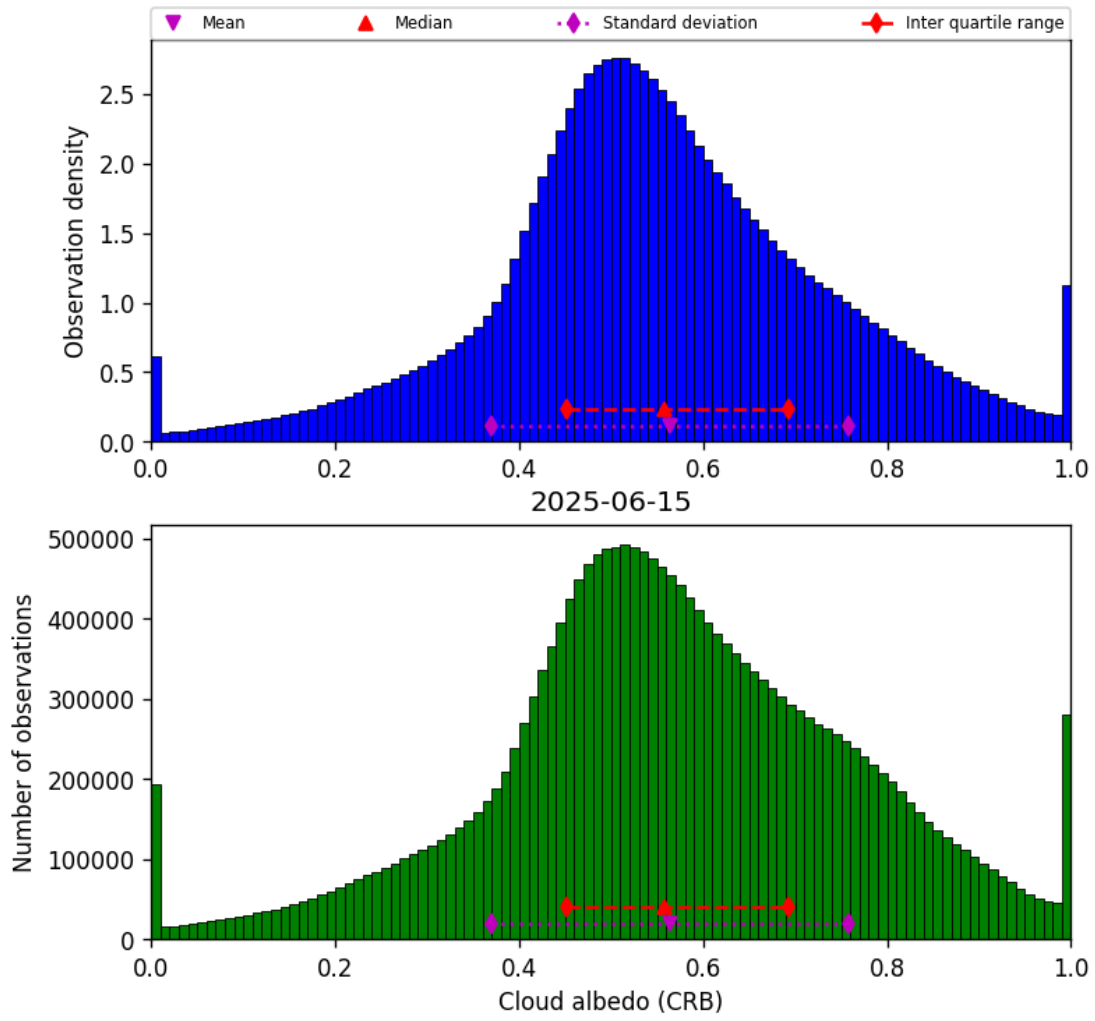
Figure 42: Histogram of “Cloud albedo (CRB)” for 2025-06-15 to 2025-06-16
