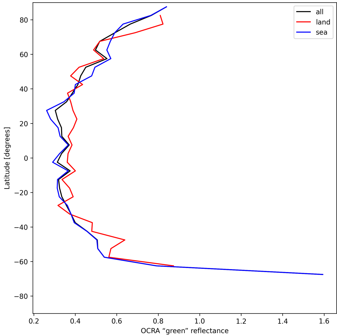
Figure 34: Zonal average of “OCRA “green” reflectance” for 2025-06-15 to 2025-06-16.
