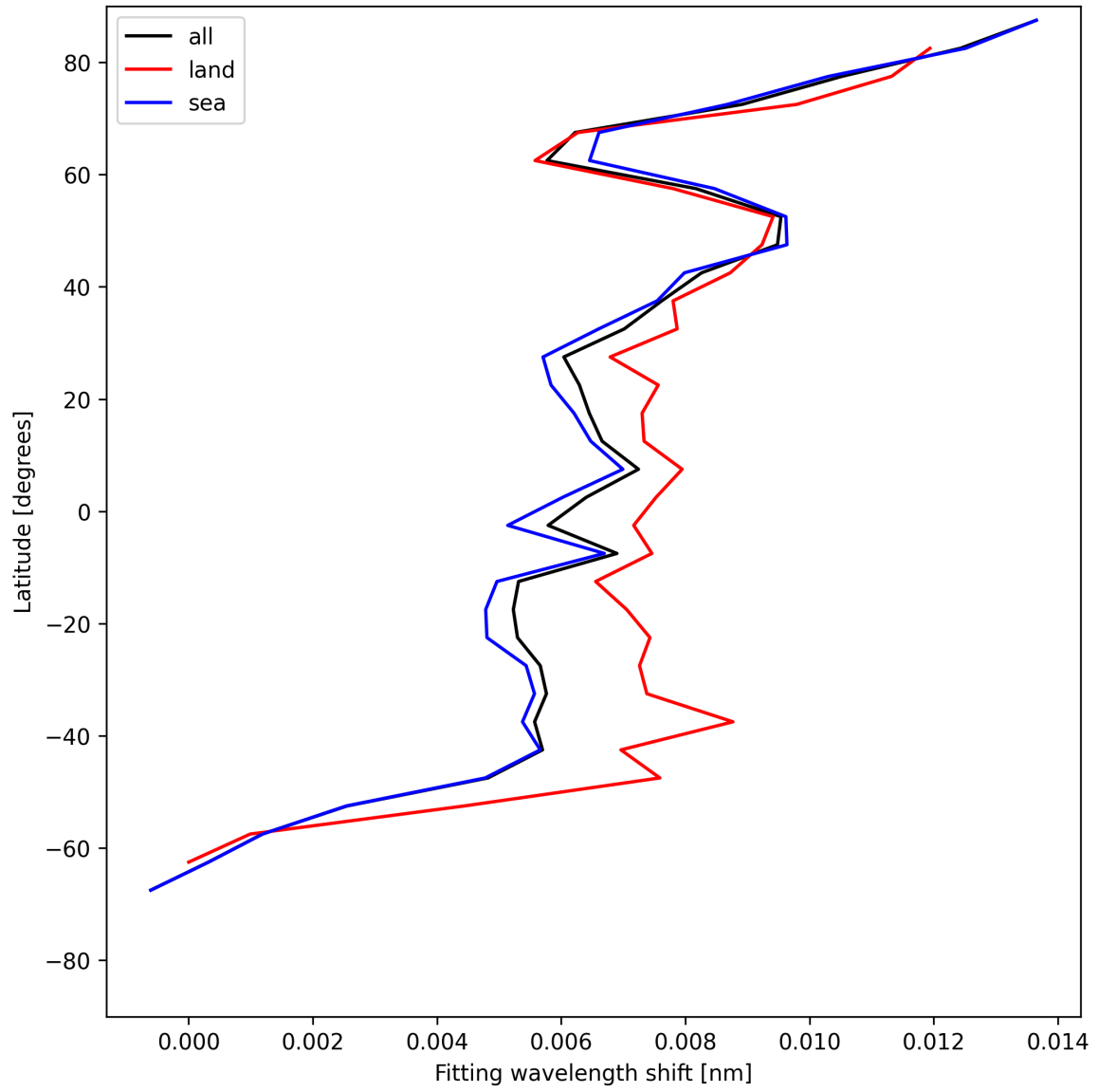
Figure 31: Zonal average of “Fitting wavelength shift” for 2025-06-15 to 2025-06-16.
