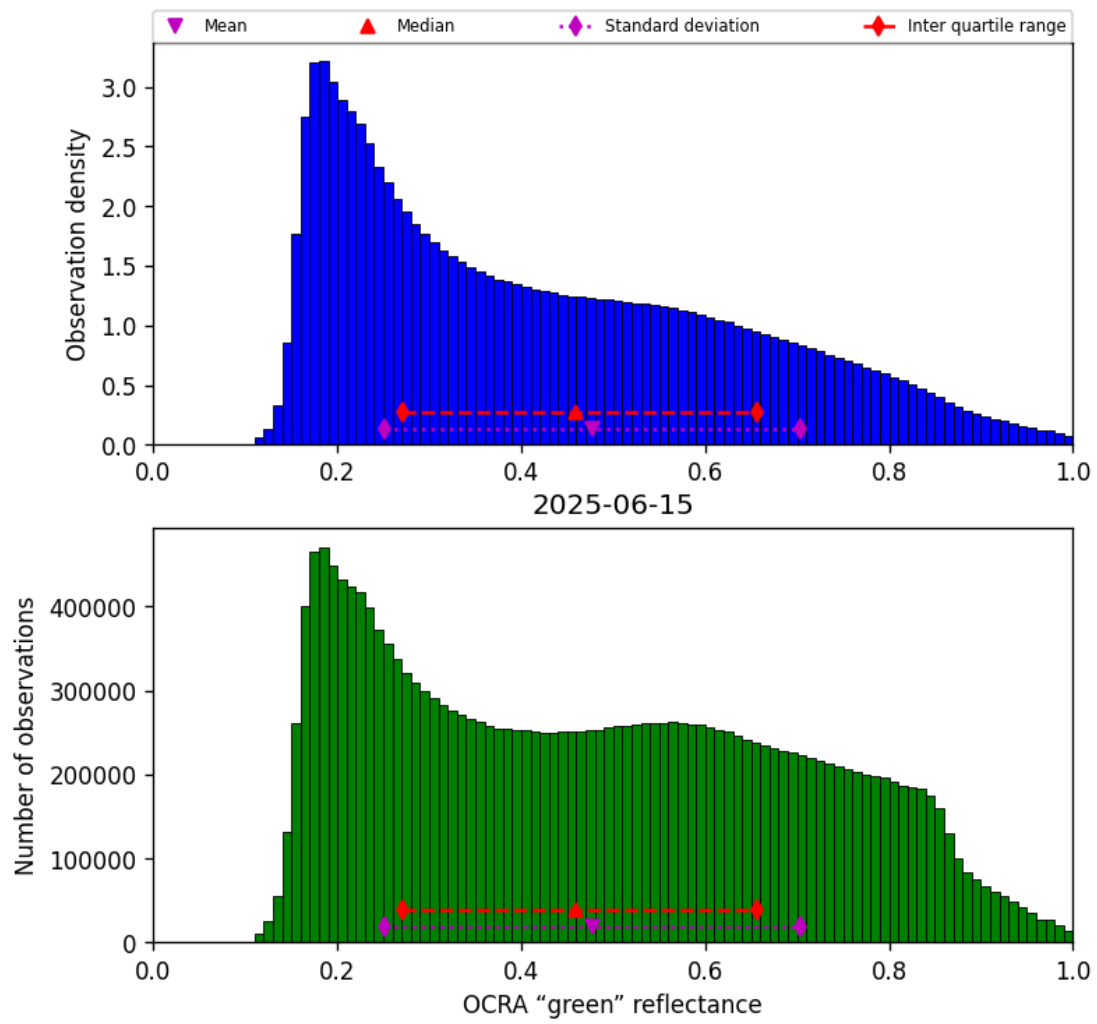
Figure 50: Histogram of “OCRA “green” reflectance” for 2025-06-15 to 2025-06-16
