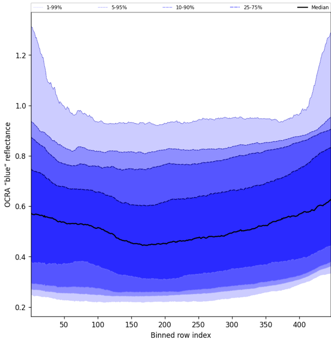
Figure 65: Along track statistics of “OCRA “blue” reflectance” for 2025-06-15 to 2025-06-16
