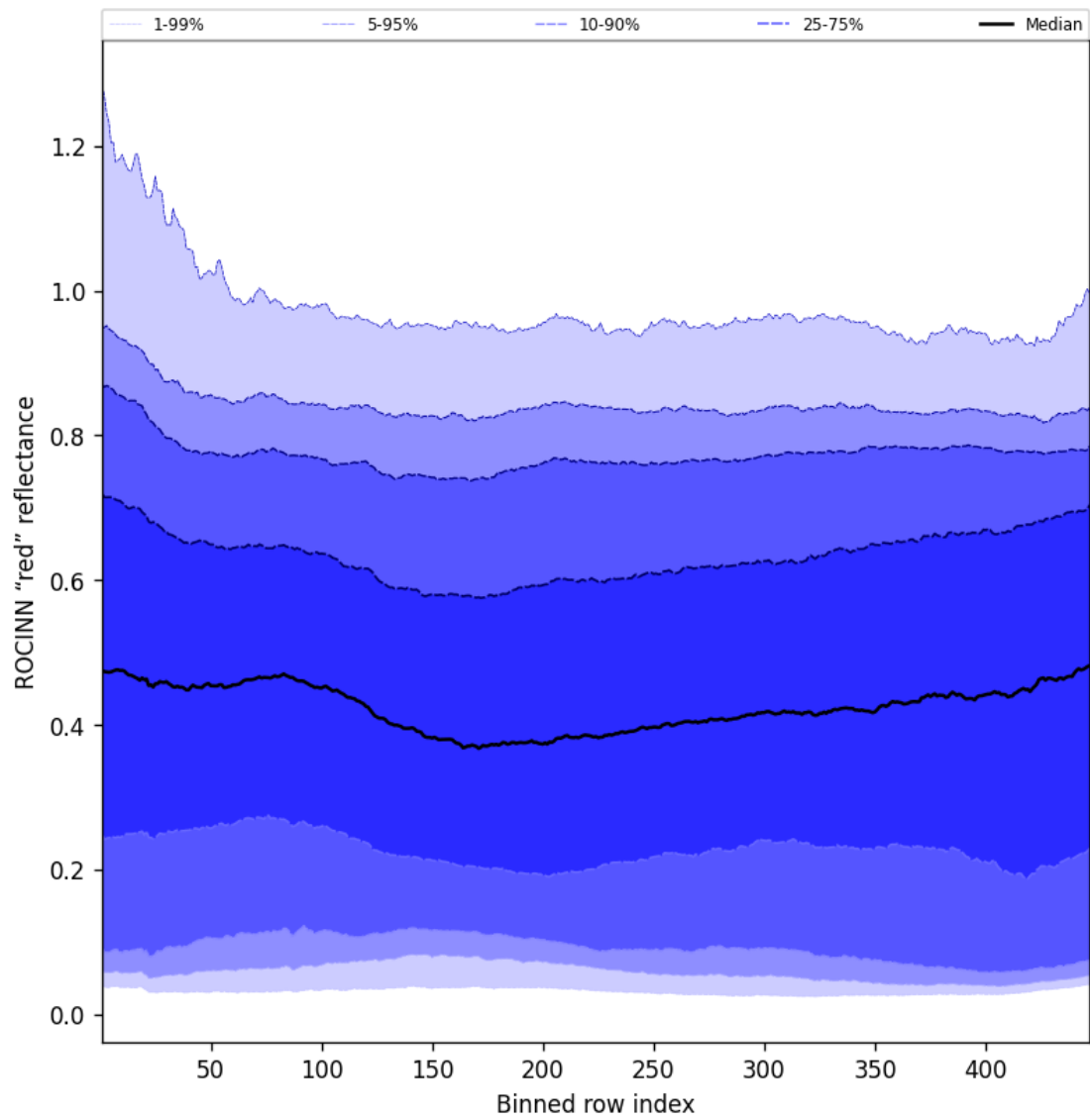
Figure 67: Along track statistics of “ROCINN “red” reflectance” for 2025-06-15 to 2025-06-16
