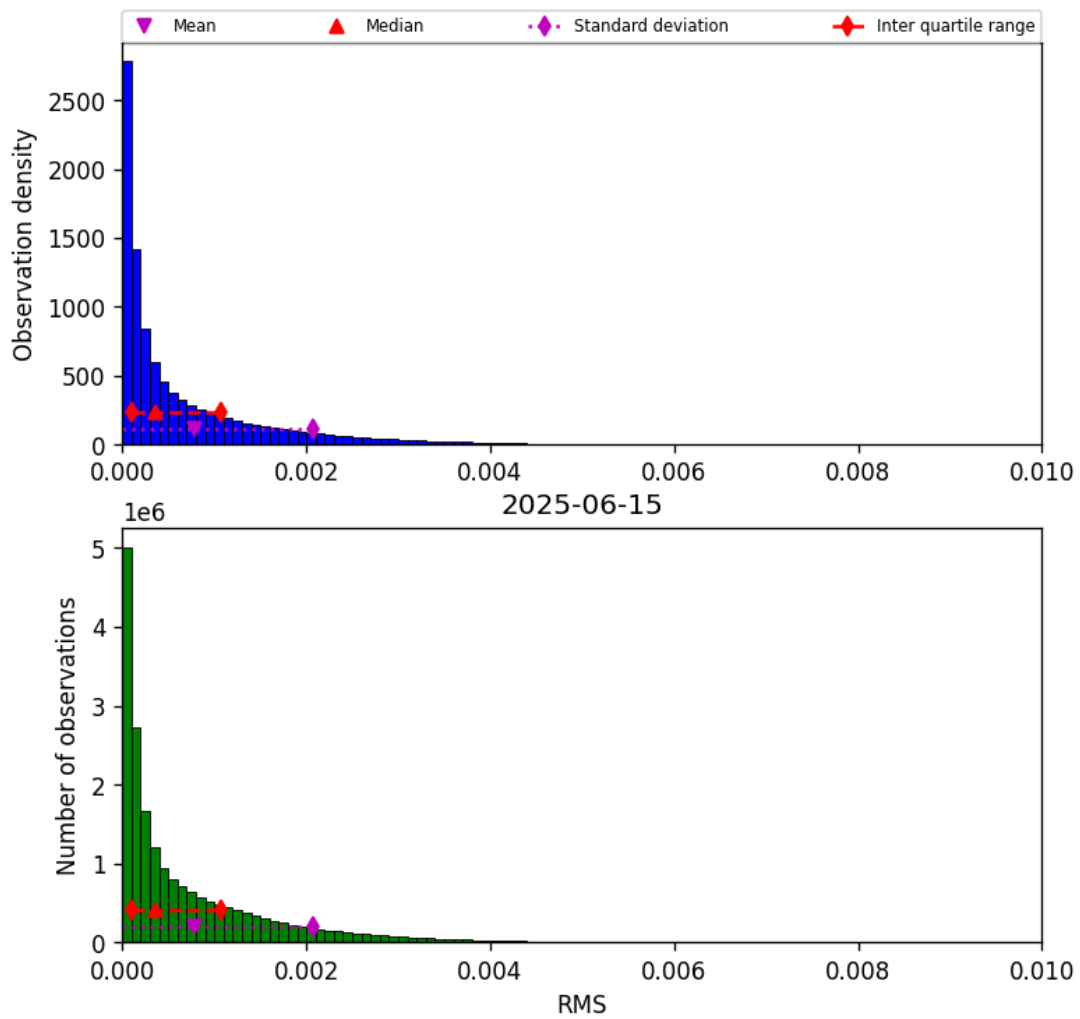
Figure 45: Histogram of “RMS” for 2025-06-15 to 2025-06-16
