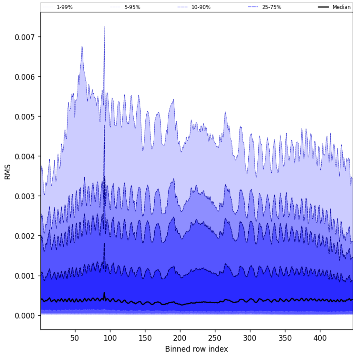
Figure 61: Along track statistics of “RMS” for 2025-06-15 to 2025-06-16
