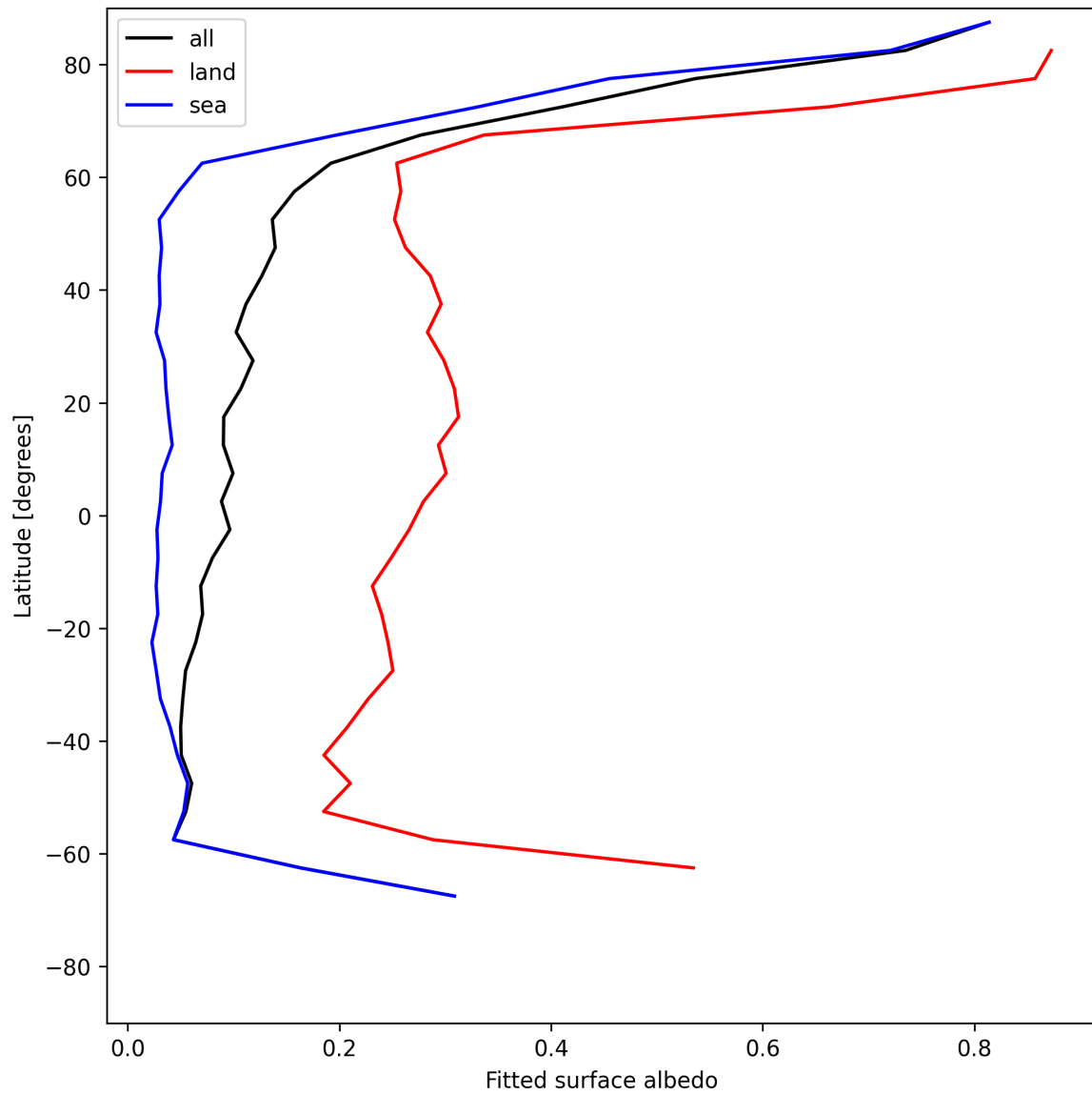
Figure 27: Zonal average of “Fitted surface albedo” for 2025-06-15 to 2025-06-16.
