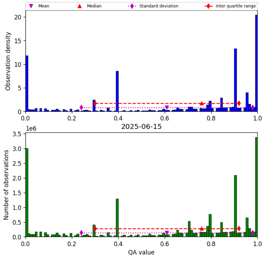
Figure 36: Histogram of “QA value” for 2025-06-15 to 2025-06-16
