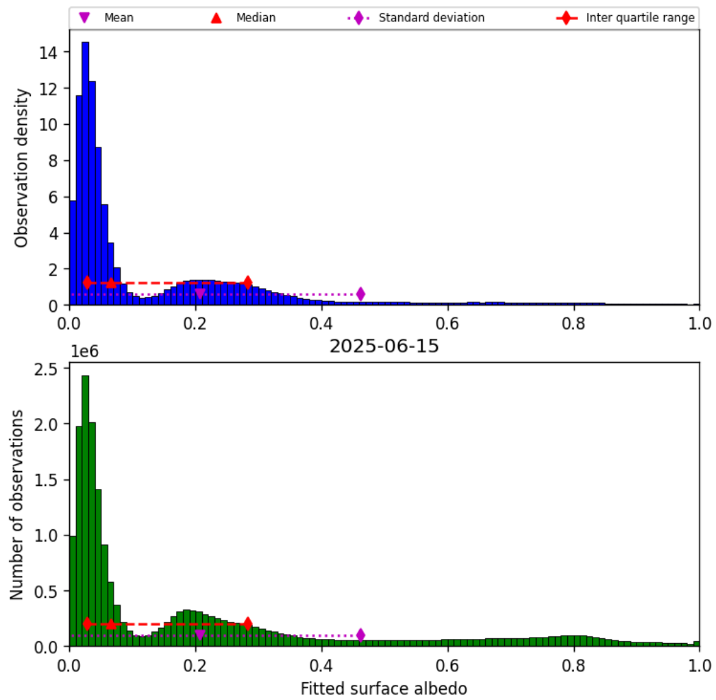
Figure 43: Histogram of “Fitted surface albedo” for 2025-06-15 to 2025-06-16
