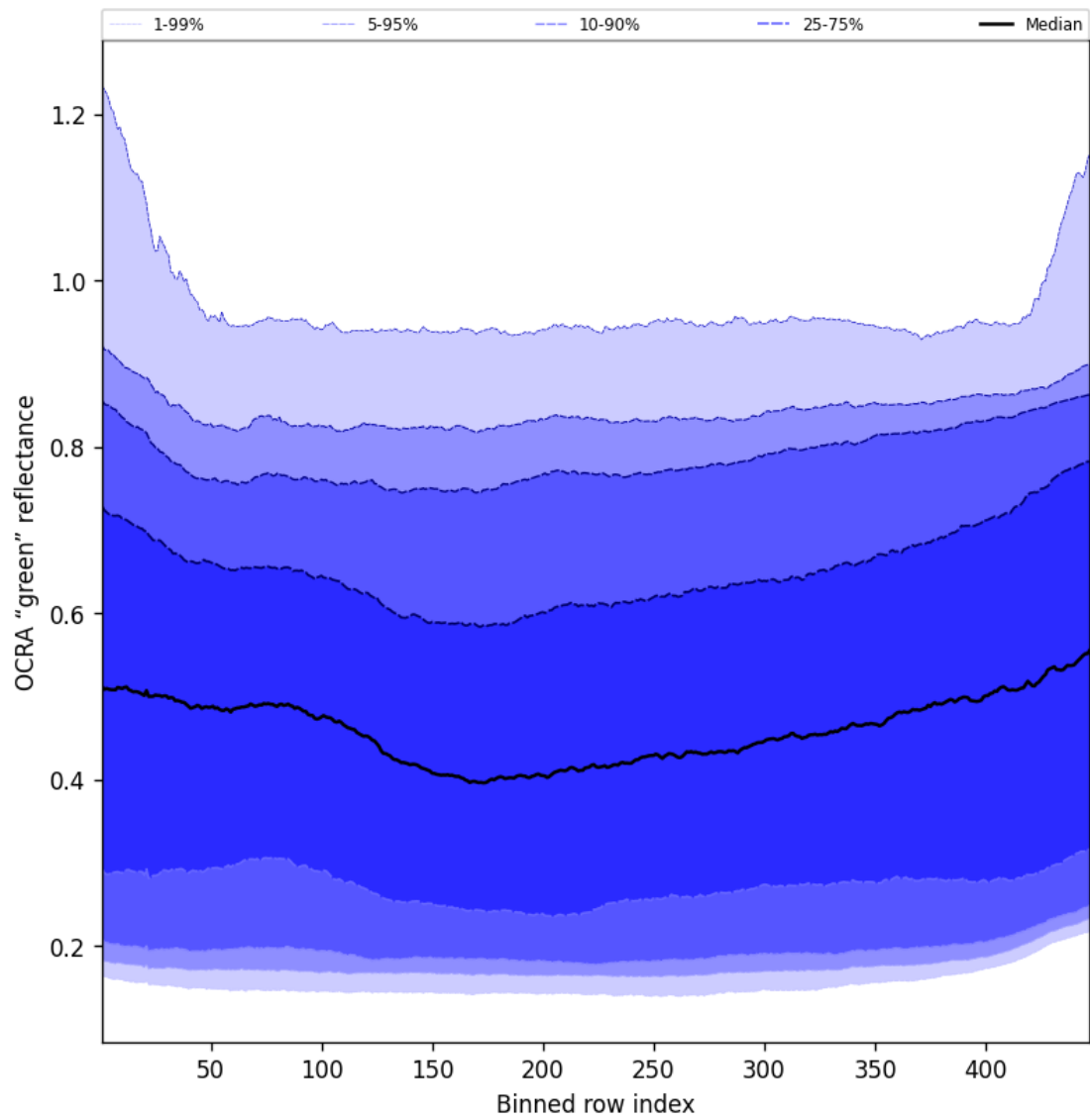
Figure 66: Along track statistics of "OCRA "green" reflectance" for 2025-06-15 to 2025-06-16
