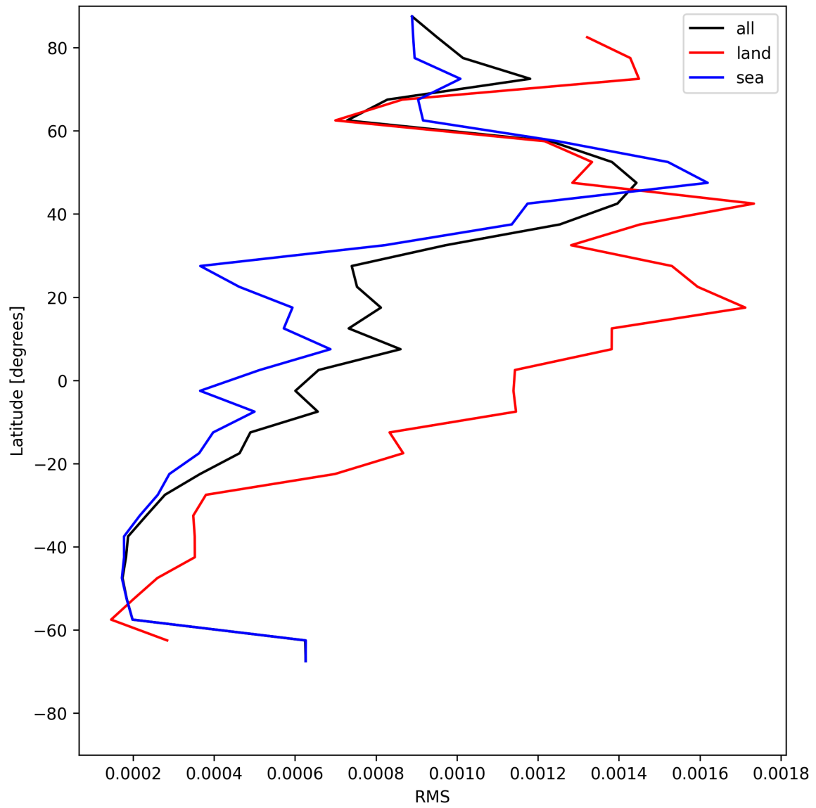
Figure 29: Zonal average of “RMS” for 2025-06-15 to 2025-06-16.
