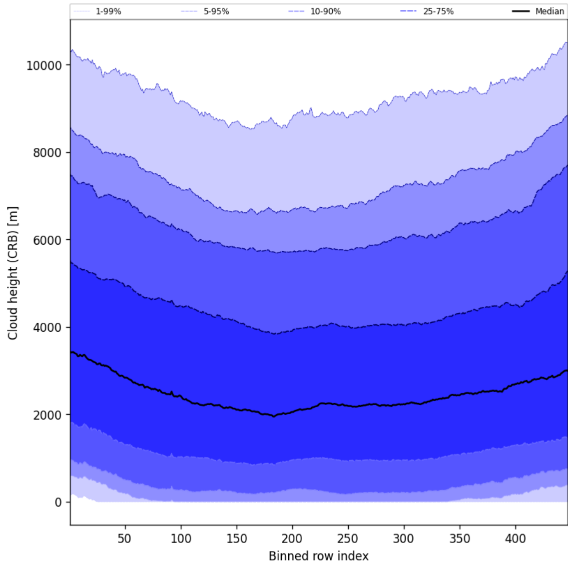
Figure 57: Along track statistics of “Cloud height (CRB)” for 2025-06-15 to 2025-06-16
