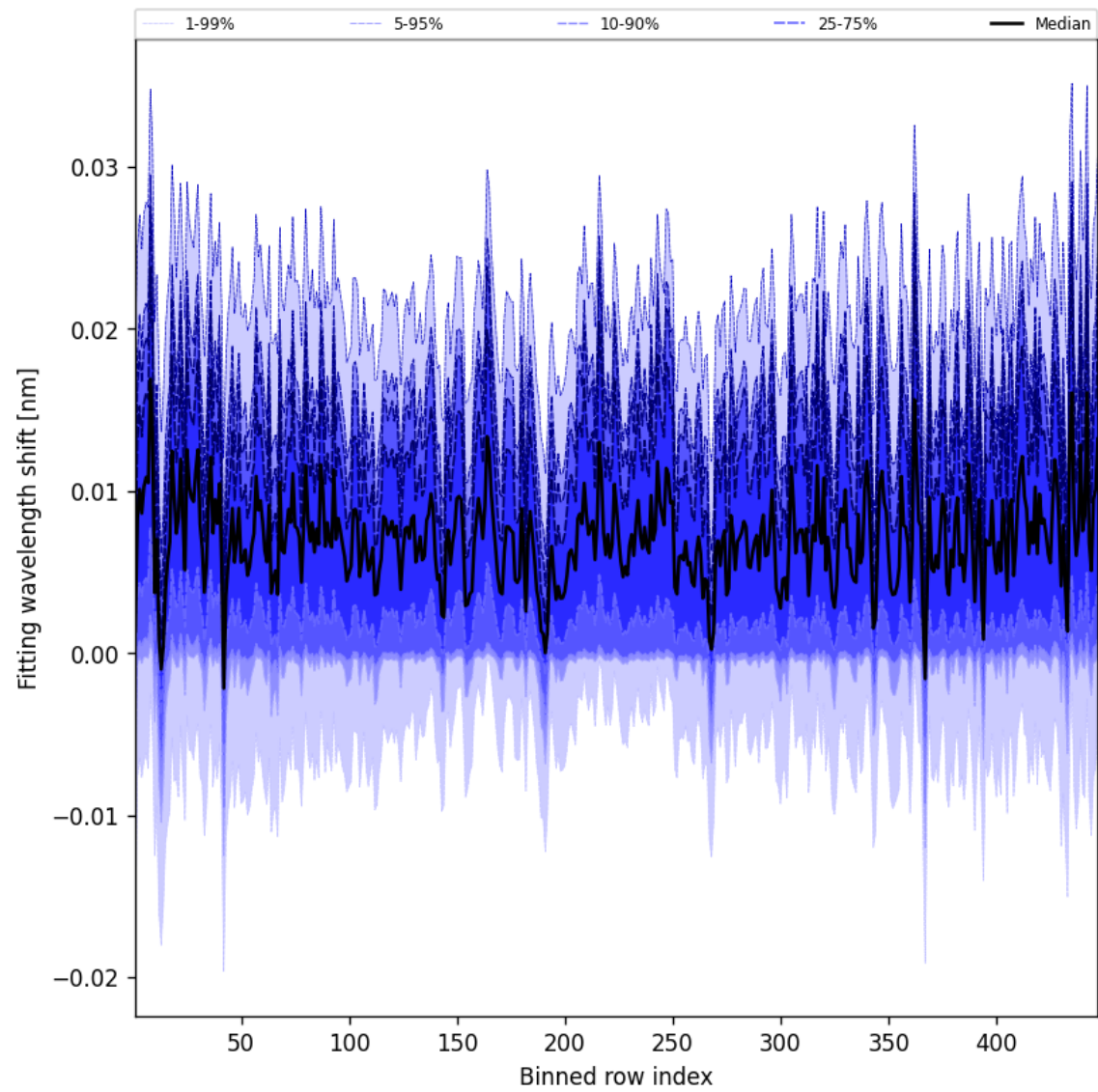
Figure 63: Along track statistics of “Fitting wavelength shift” for 2025-06-15 to 2025-06-16
