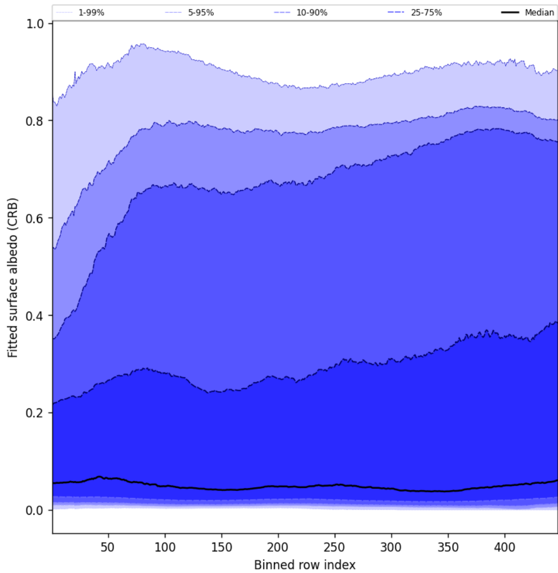
Figure 60: Along track statistics of “Fitted surface albedo (CRB)” for 2025-06-15 to 2025-06-16
