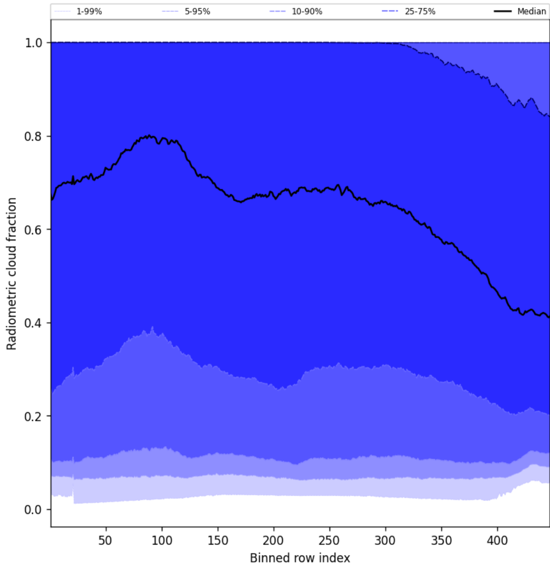
Figure 53: Along track statistics of “Radiometric cloud fraction” for 2025-06-15 to 2025-06-16
