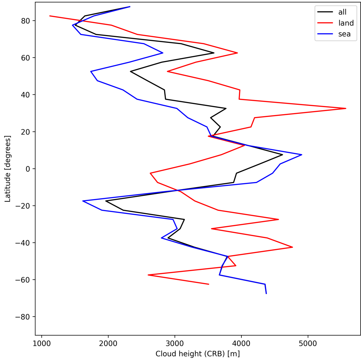
Figure 25: Zonal average of “Cloud height (CRB)” for 2025-06-15 to 2025-06-16.
