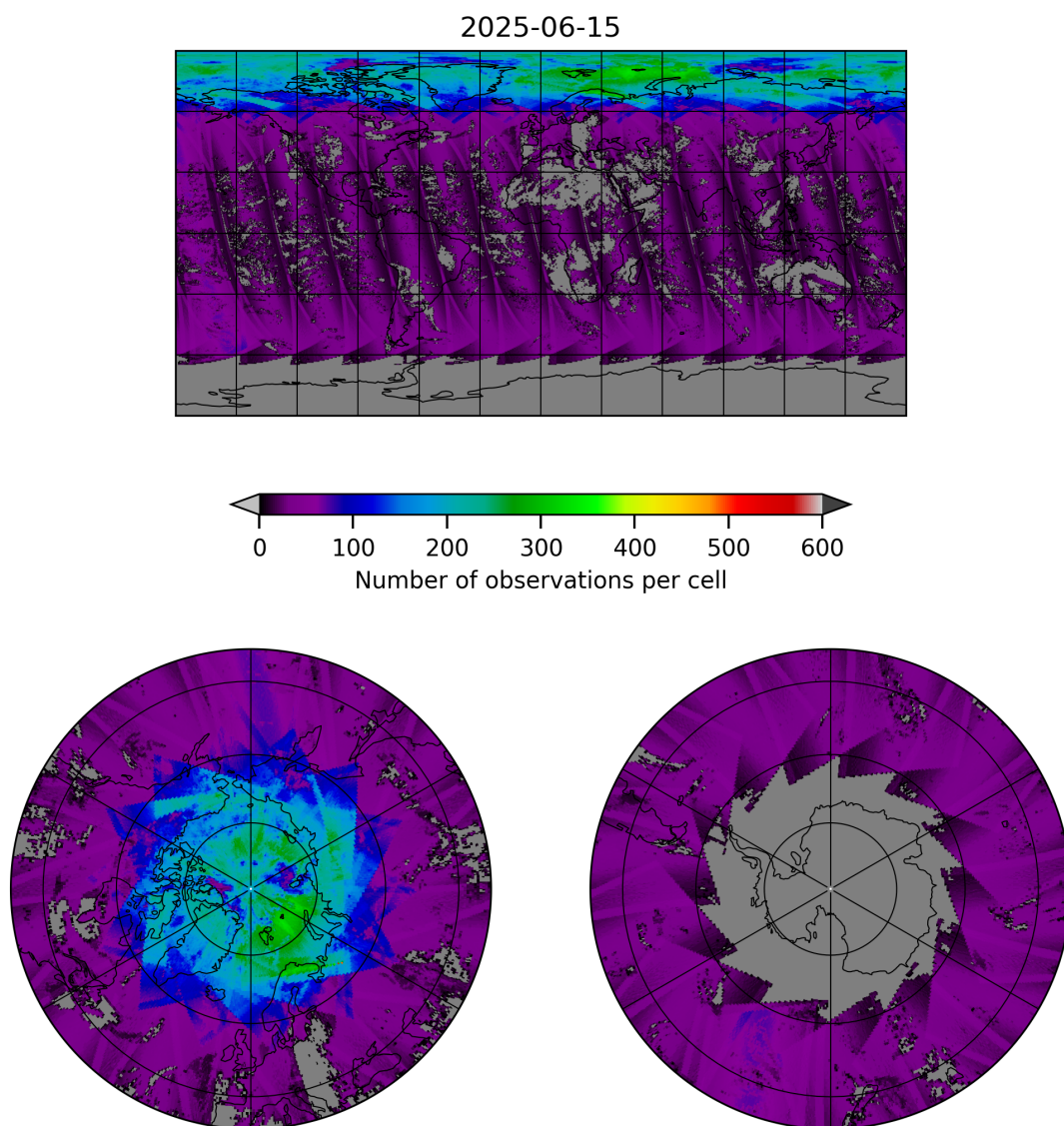
Figure 19: Map of the number of observations for 2025-06-15 to 2025-06-16
