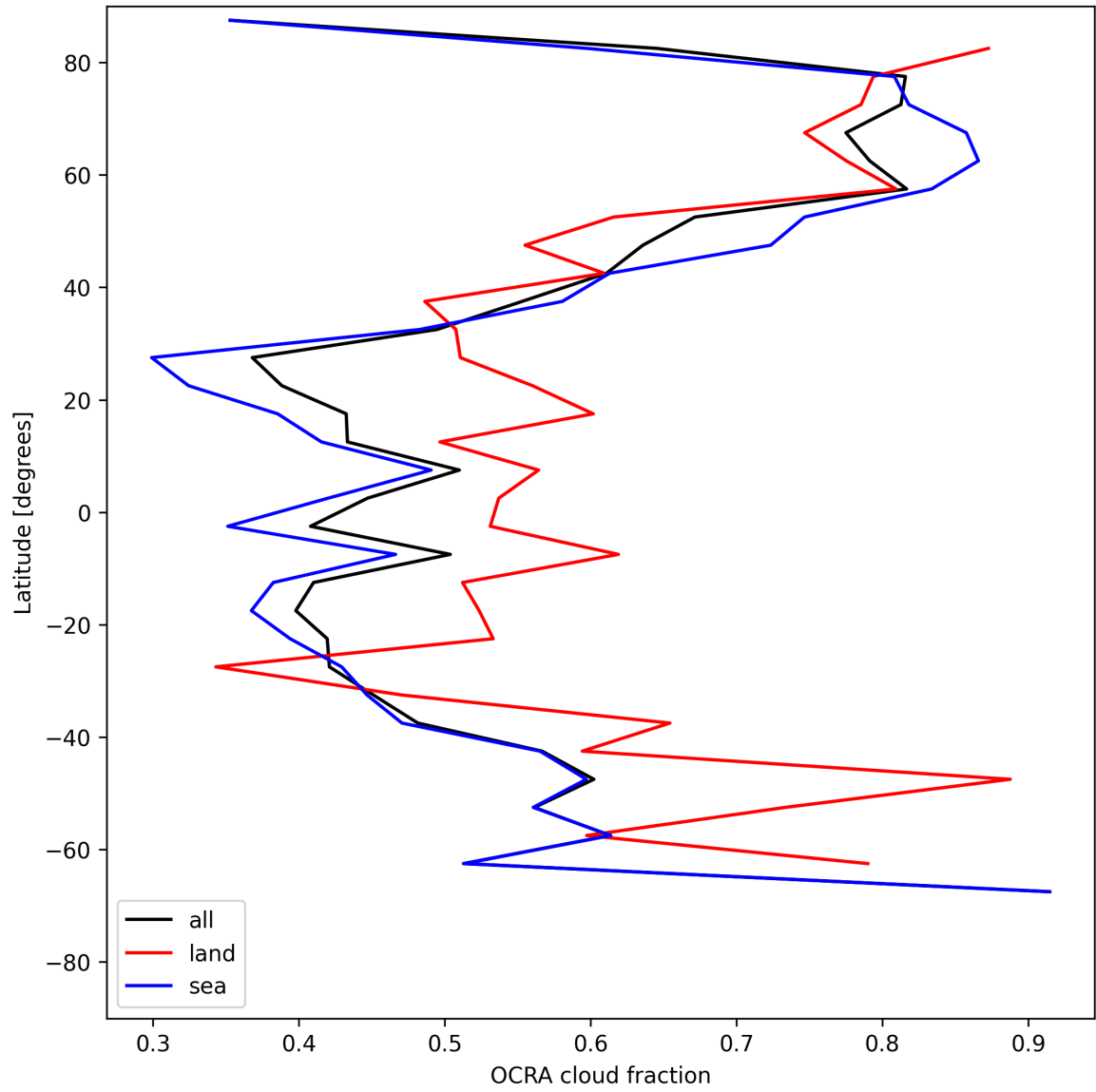
Figure 32: Zonal average of “OCRA cloud fraction” for 2025-06-15 to 2025-06-16.
