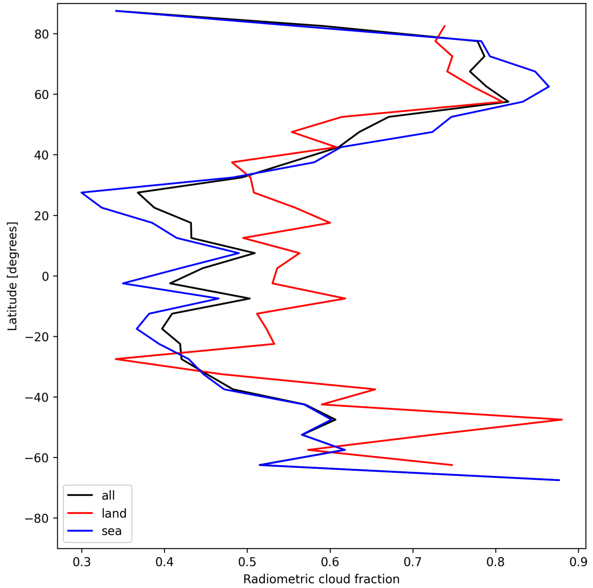
Figure 21: Zonal average of “Radiometric cloud fraction” for 2025-06-15 to 2025-06-16.
