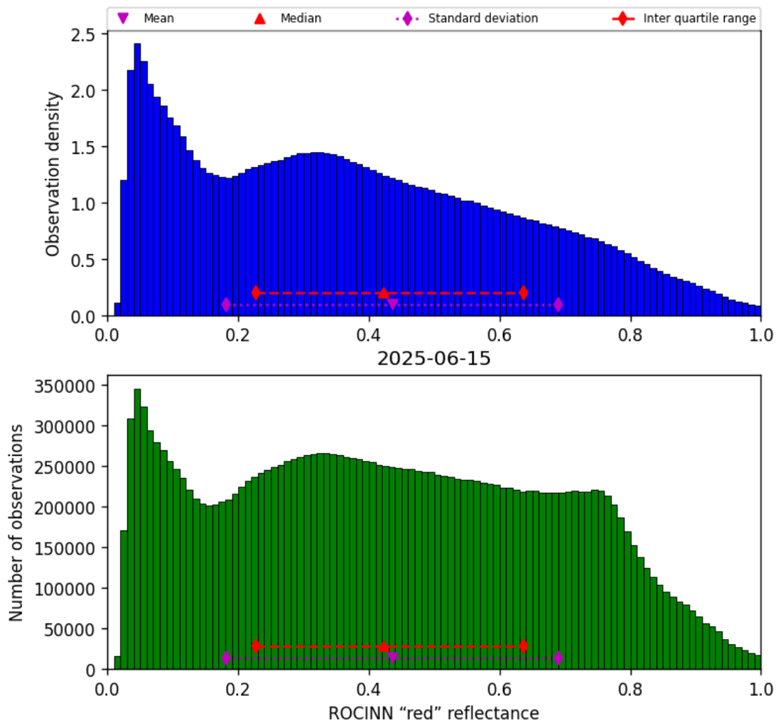
Figure 51: Histogram of “ROCINN “red” reflectance” for 2025-06-15 to 2025-06-16
