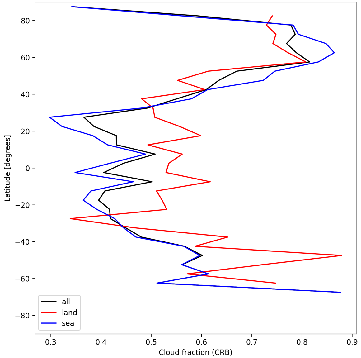
Figure 24: Zonal average of “Cloud fraction (CRB)” for 2025-06-15 to 2025-06-16.
