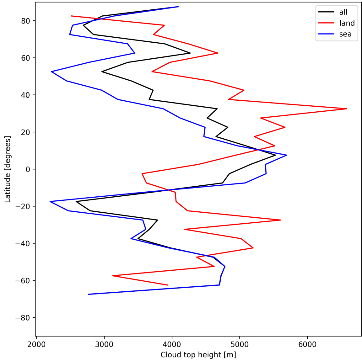
Figure 22: Zonal average of “Cloud top height” for 2025-06-15 to 2025-06-16.
