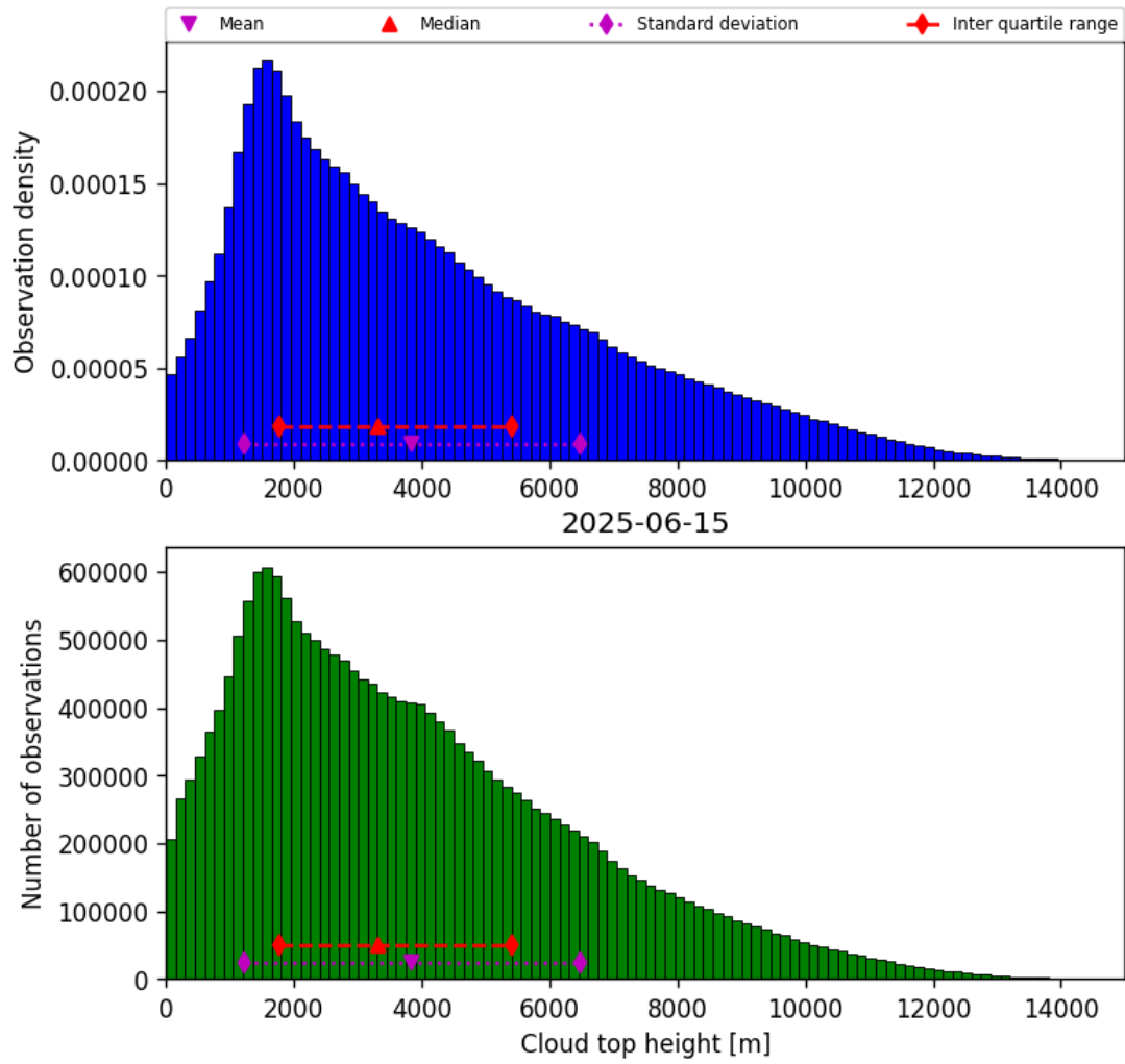
Figure 38: Histogram of “Cloud top height” for 2025-06-15 to 2025-06-16
