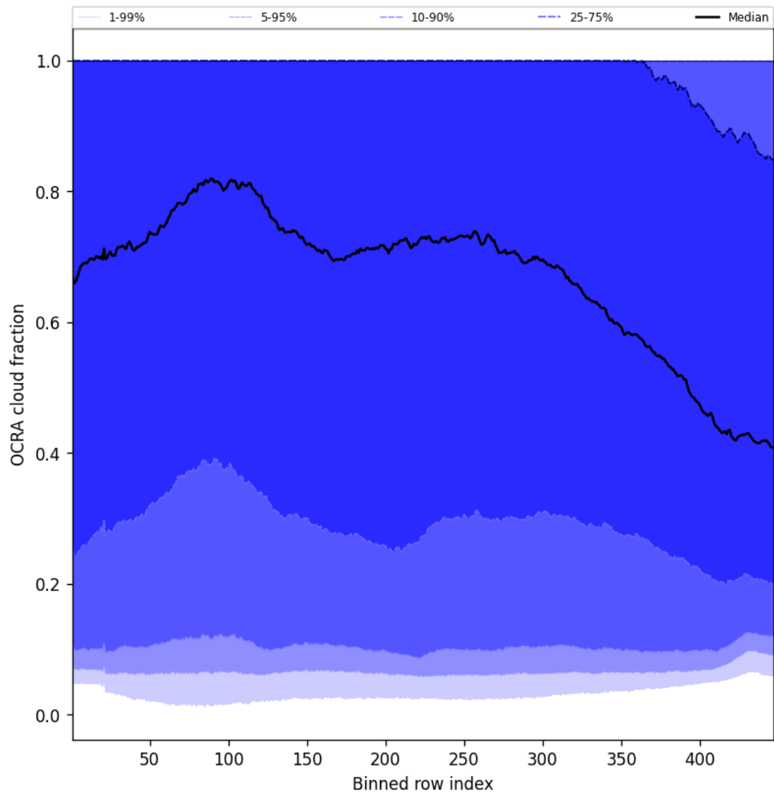
Figure 64: Along track statistics of “OCRA cloud fraction” for 2025-06-15 to 2025-06-16
