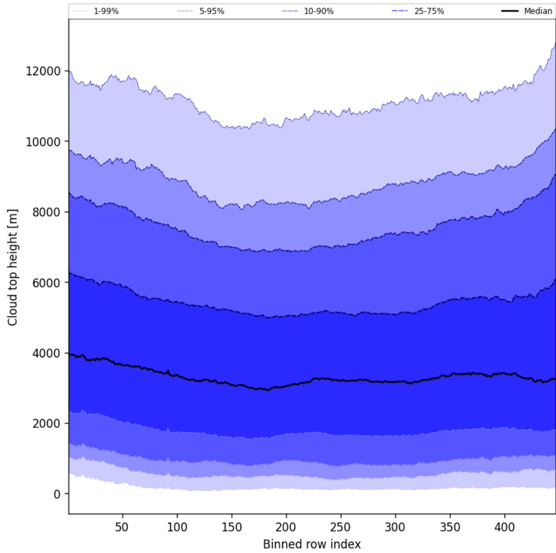
Figure 54: Along track statistics of “Cloud top height” for 2025-06-15 to 2025-06-16
