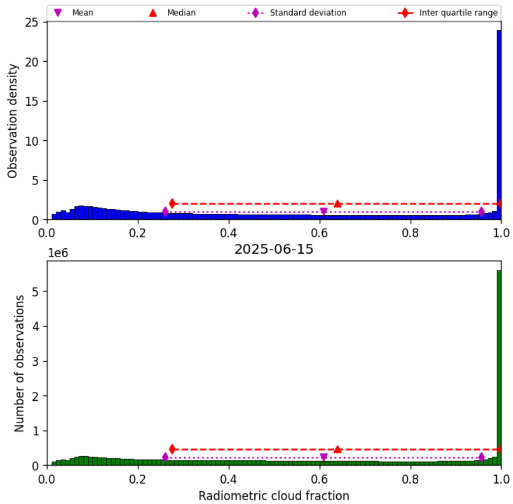
Figure 37: Histogram of “Radiometric cloud fraction” for 2025-06-15 to 2025-06-16
