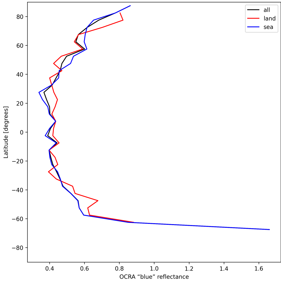
Figure 33: Zonal average of “OCRA “blue” reflectance” for 2025-06-15 to 2025-06-16.
