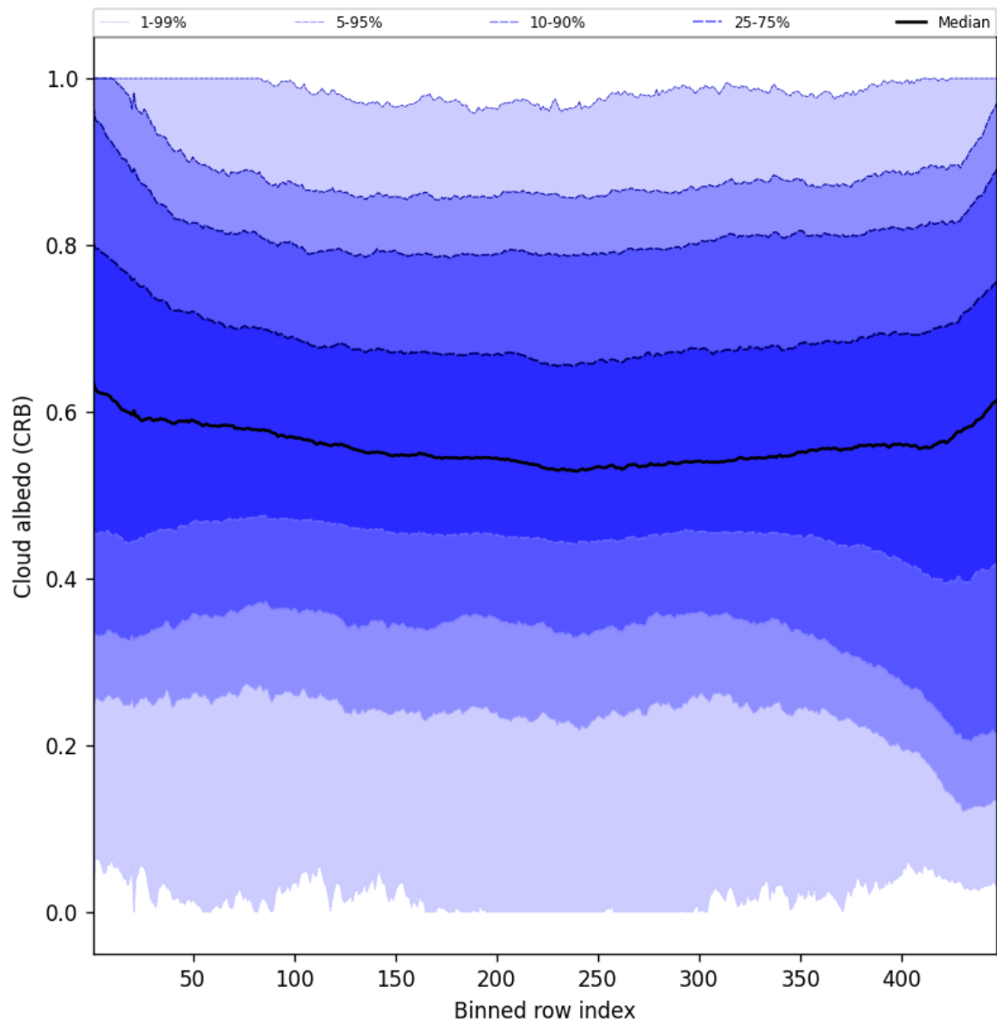
Figure 58: Along track statistics of “Cloud albedo (CRB)” for 2025-06-15 to 2025-06-16
