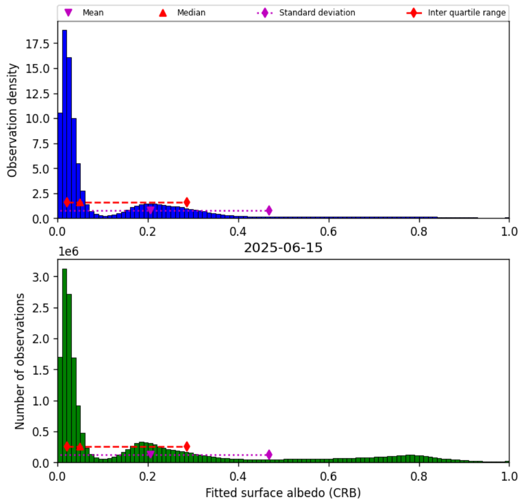
Figure 44: Histogram of “Fitted surface albedo (CRB)” for 2025-06-15 to 2025-06-16
