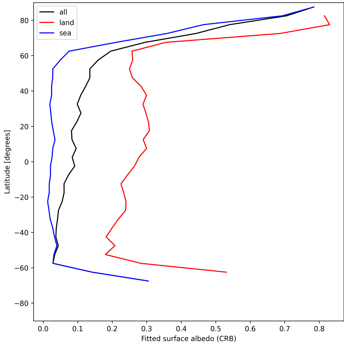
Figure 28: Zonal average of “Fitted surface albedo (CRB)” for 2025-06-15 to 2025-06-16.
