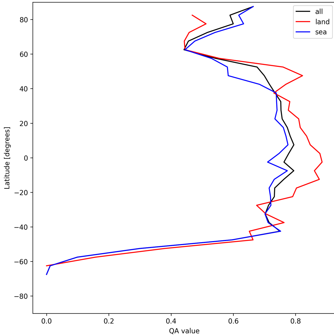
Figure 20: Zonal average of “QA value” for 2025-06-15 to 2025-06-16.
