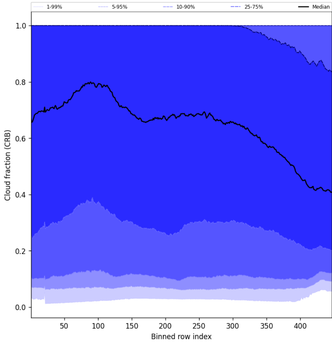
Figure 56: Along track statistics of “Cloud fraction (CRB)” for 2025-06-15 to 2025-06-16
