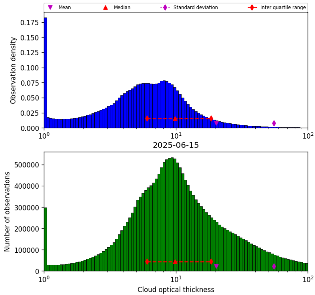
Figure 39: Histogram of “Cloud optical thickness” for 2025-06-15 to 2025-06-16
