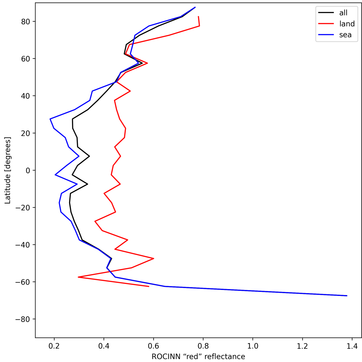
Figure 35: Zonal average of “ROCINN “red” reflectance” for 2025-06-15 to 2025-06-16.
