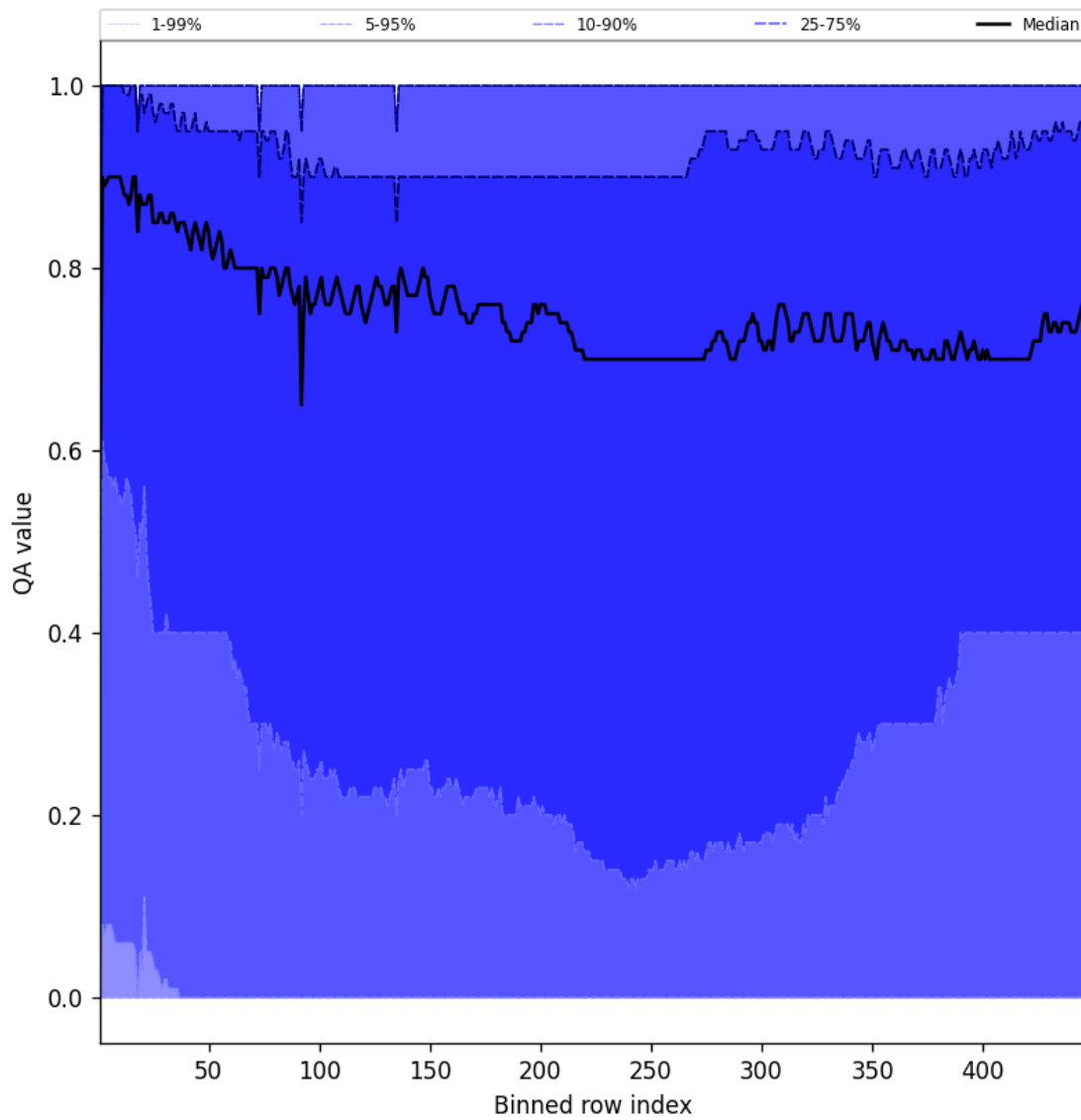
Figure 52: Along track statistics of “QA value” for 2025-06-15 to 2025-06-16
