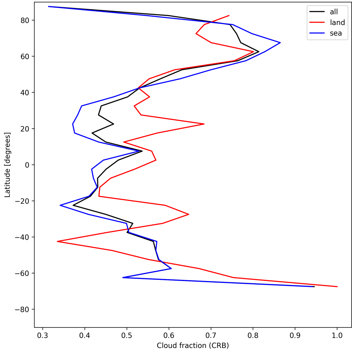
Figure 24: Zonal average of "Cloud fraction (CRB)" for 2025-06-17 to 2025-06-17.
