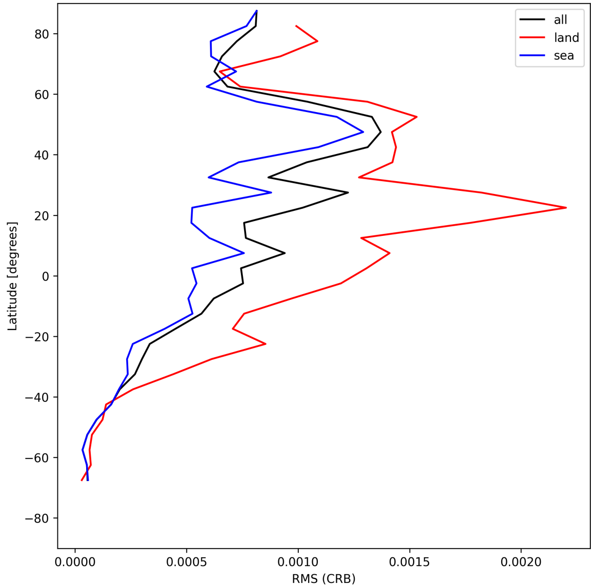
Figure 30: Zonal average of “RMS (CRB)” for 2025-06-17 to 2025-06-17.
