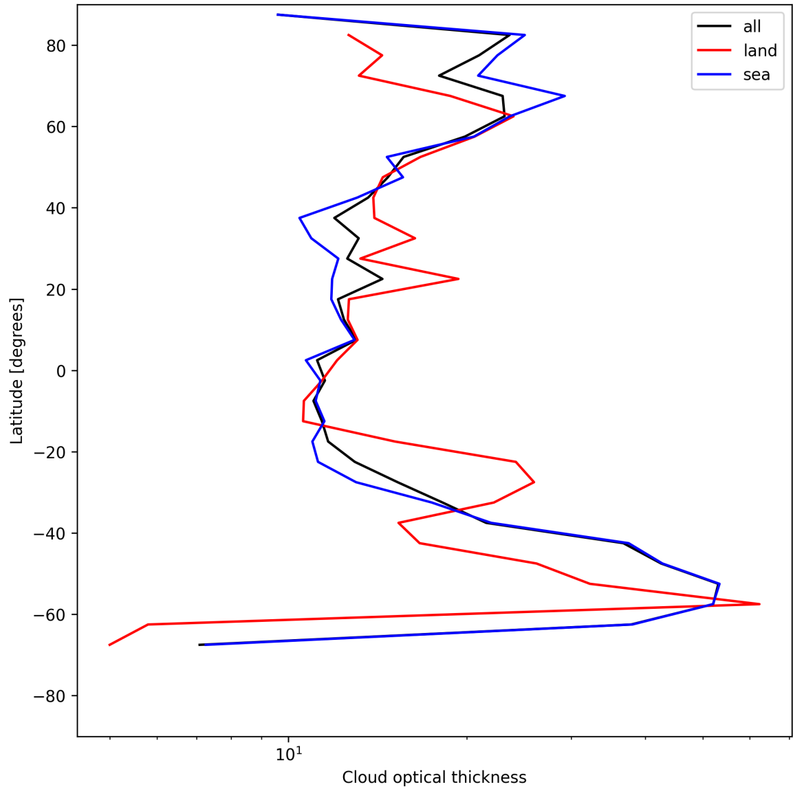
Figure 23: Zonal average of “Cloud optical thickness” for 2025-06-17 to 2025-06-17.
