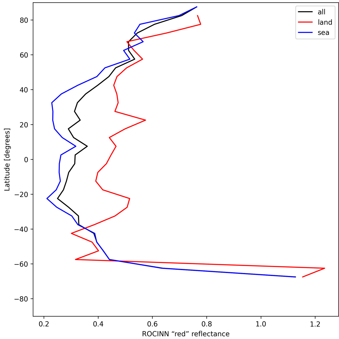
Figure 35: Zonal average of “ROCINN “red” reflectance” for 2025-06-17 to 2025-06-17.
