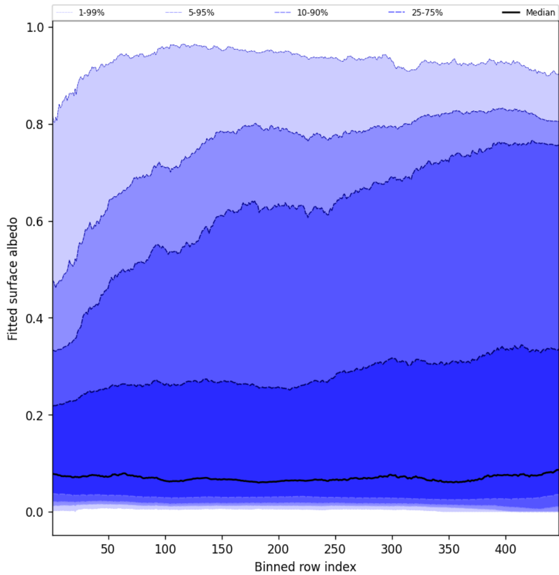
Figure 59: Along track statistics of “Fitted surface albedo” for 2025-06-17 to 2025-06-17
