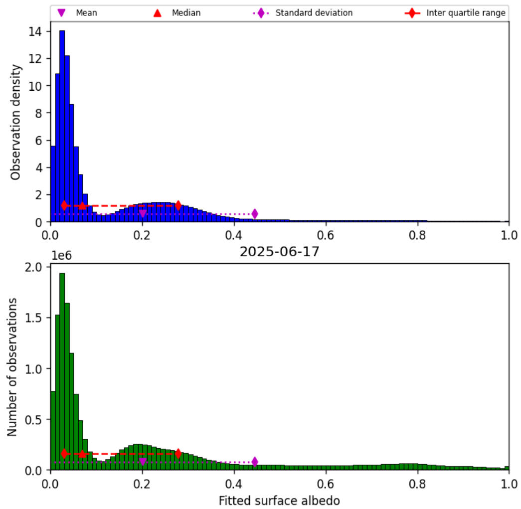
Figure 43: Histogram of “Fitted surface albedo” for 2025-06-17 to 2025-06-17
