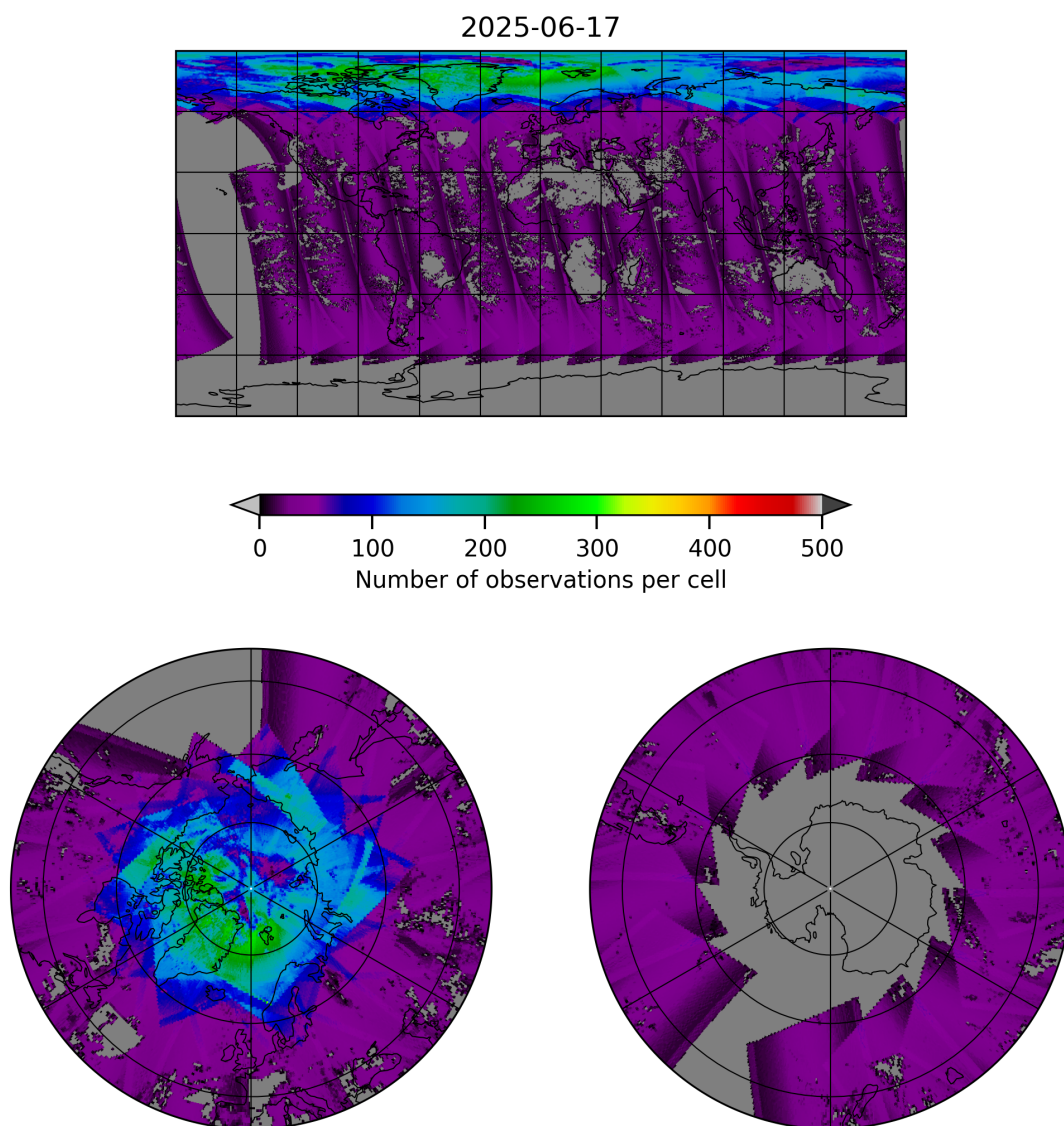
Figure 19: Map of the number of observations for 2025-06-17 to 2025-06-17
