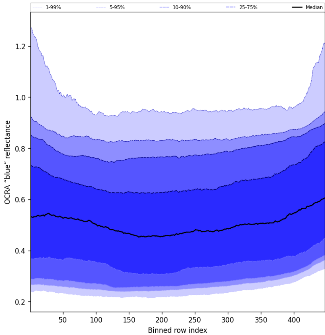
Figure 65: Along track statistics of “OCRA “blue” reflectance” for 2025-06-17 to 2025-06-17
