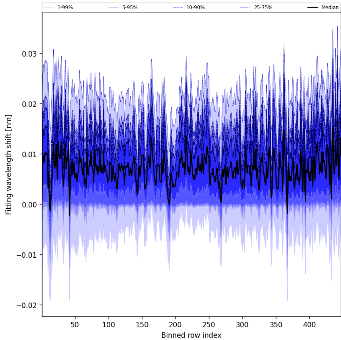
Figure 63: Along track statistics of “Fitting wavelength shift” for 2025-06-17 to 2025-06-17
