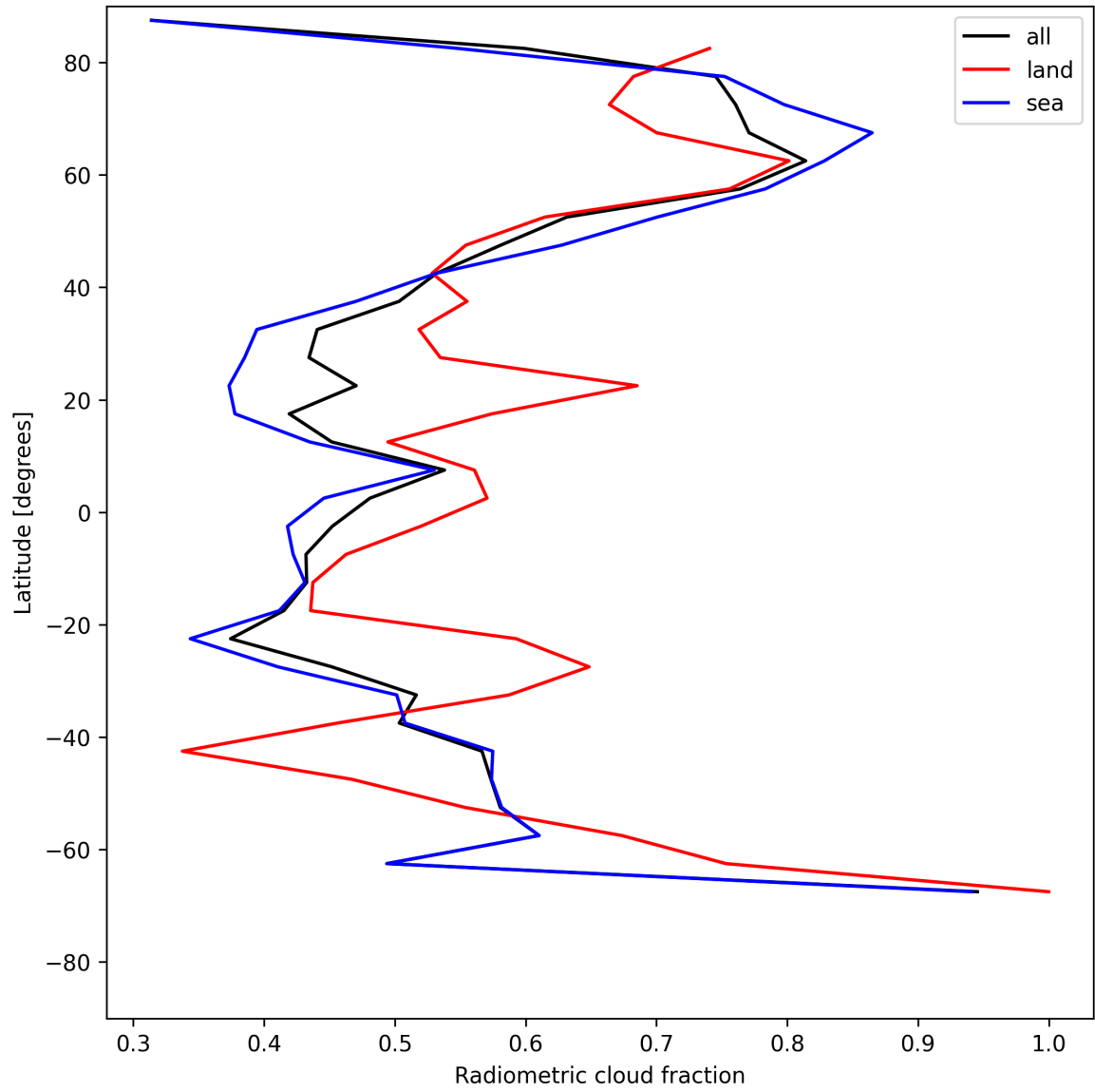
Figure 21: Zonal average of “Radiometric cloud fraction” for 2025-06-17 to 2025-06-17.
