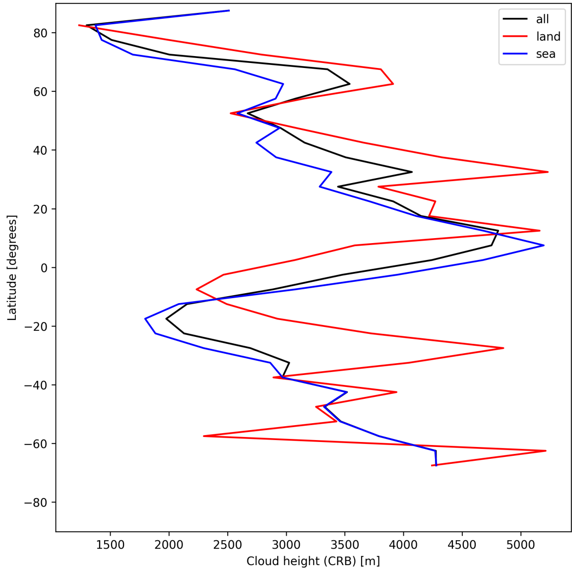
Figure 25: Zonal average of “Cloud height (CRB)” for 2025-06-17 to 2025-06-17.
