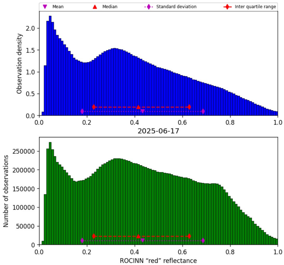
Figure 51: Histogram of “ROCINN “red” reflectance” for 2025-06-17 to 2025-06-17
