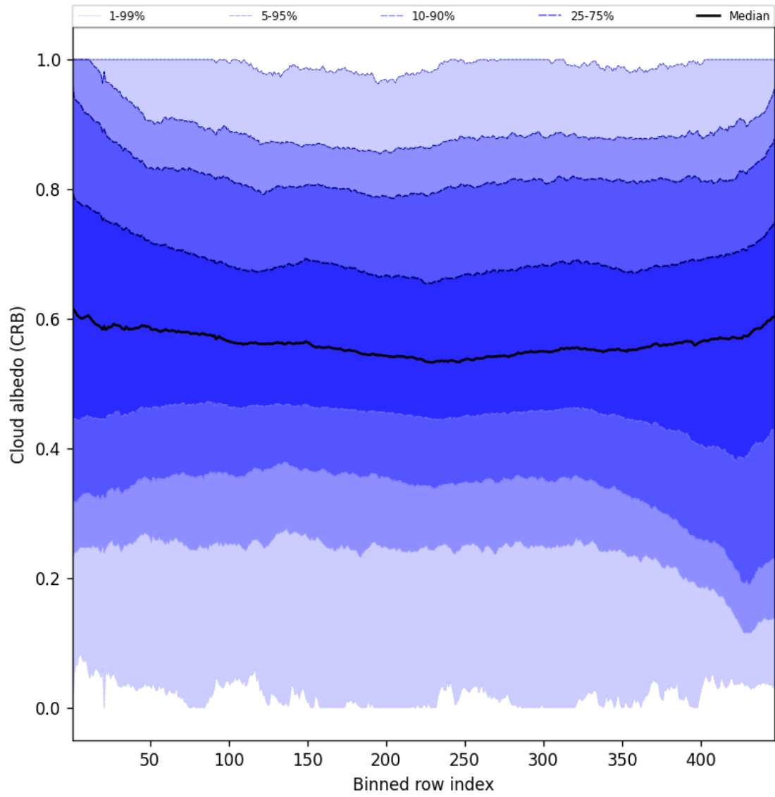
Figure 58: Along track statistics of “Cloud albedo (CRB)” for 2025-06-17 to 2025-06-17
