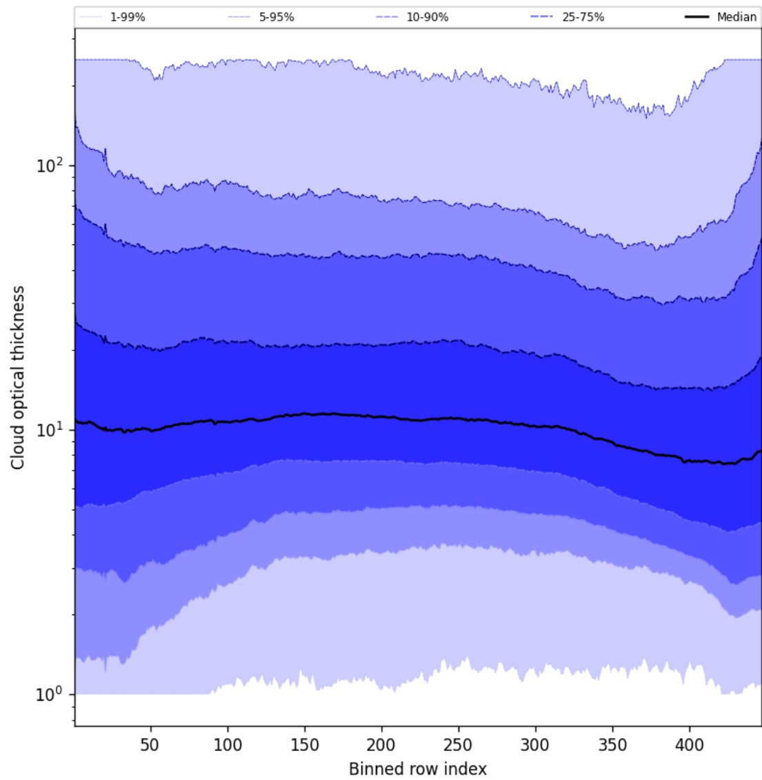
Figure 55: Along track statistics of “Cloud optical thickness” for 2025-06-17 to 2025-06-17
