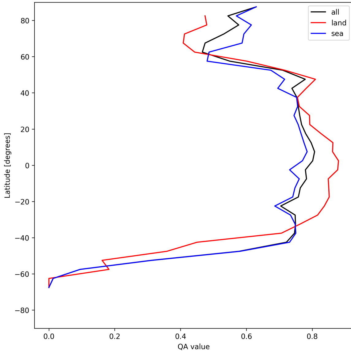
Figure 20: Zonal average of “QA value” for 2025-06-17 to 2025-06-17.
