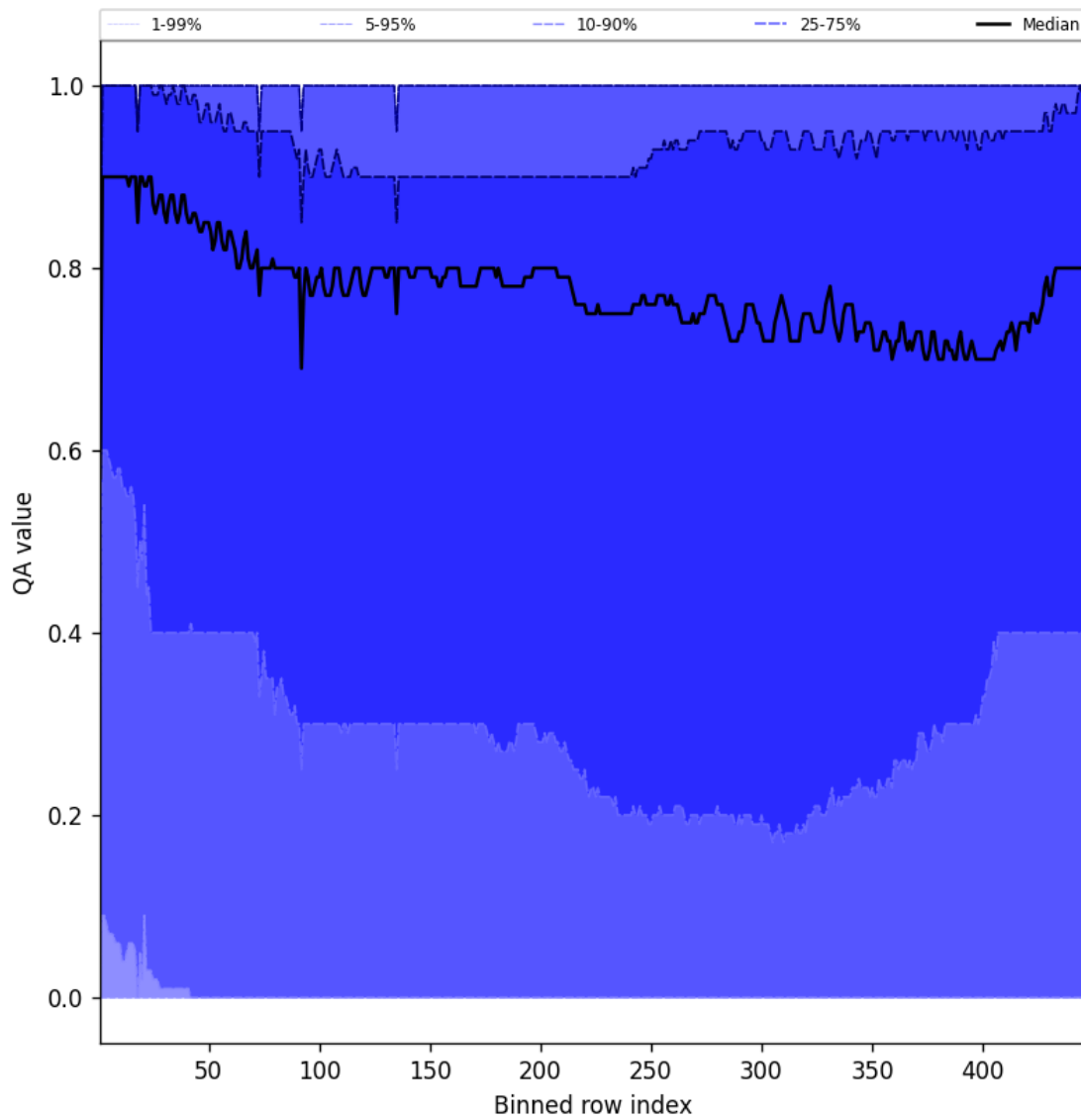
Figure 52: Along track statistics of “QA value” for 2025-06-17 to 2025-06-17
