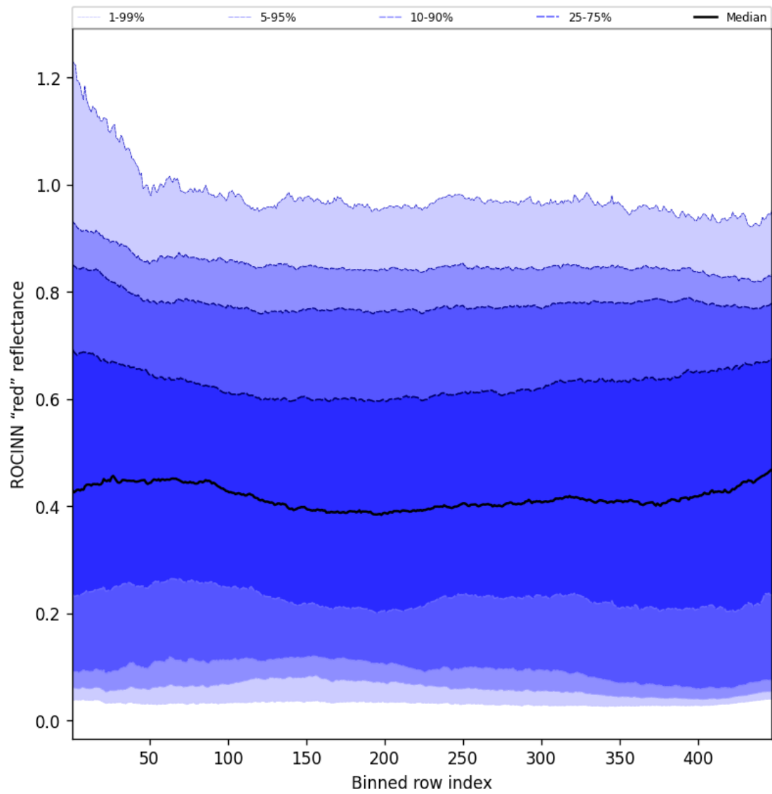
Figure 67: Along track statistics of “ROCINN “red” reflectance” for 2025-06-17 to 2025-06-17
