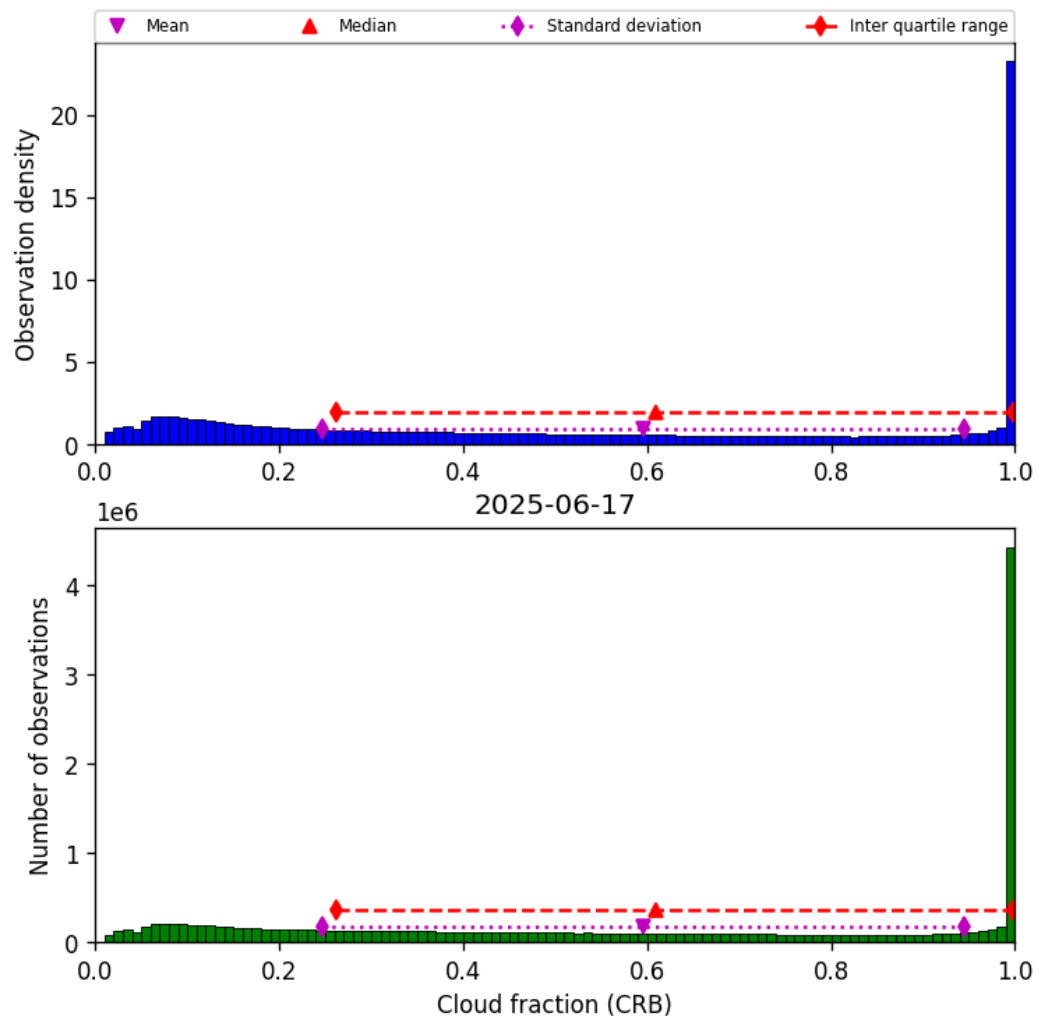
Figure 40: Histogram of “Cloud fraction (CRB)” for 2025-06-17 to 2025-06-17
