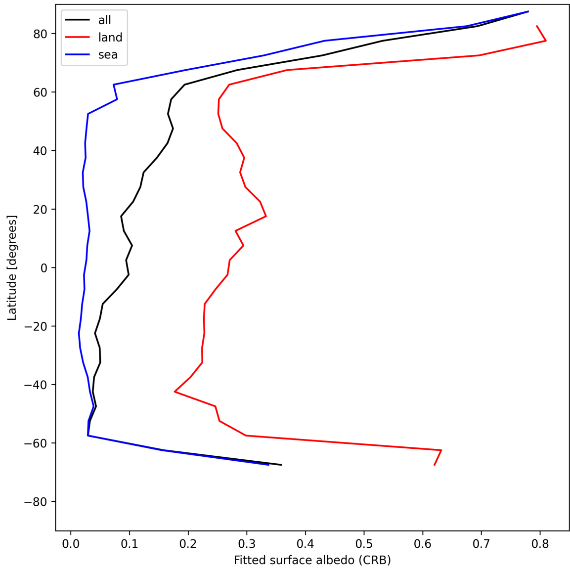
Figure 28: Zonal average of “Fitted surface albedo (CRB)” for 2025-06-17 to 2025-06-17.
