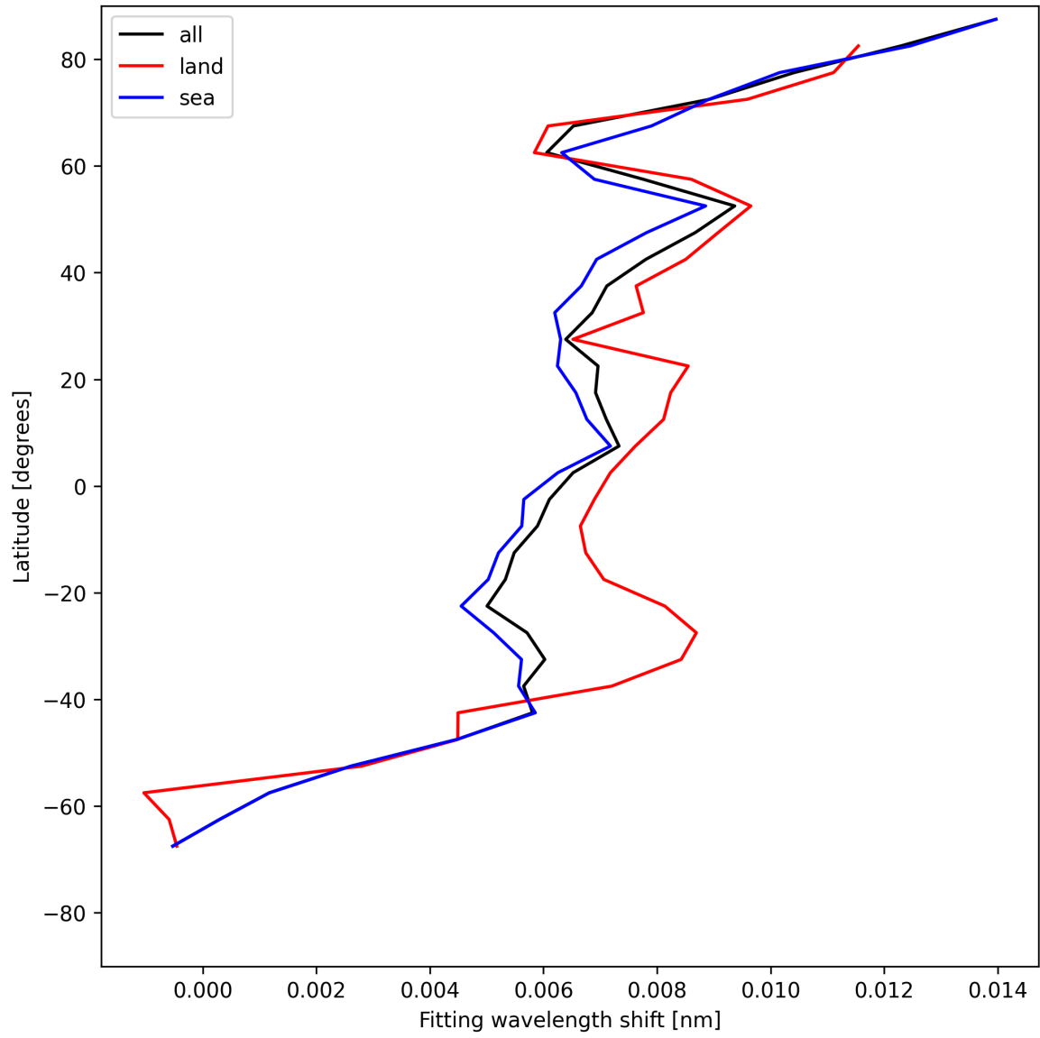
Figure 31: Zonal average of “Fitting wavelength shift” for 2025-06-17 to 2025-06-17.
