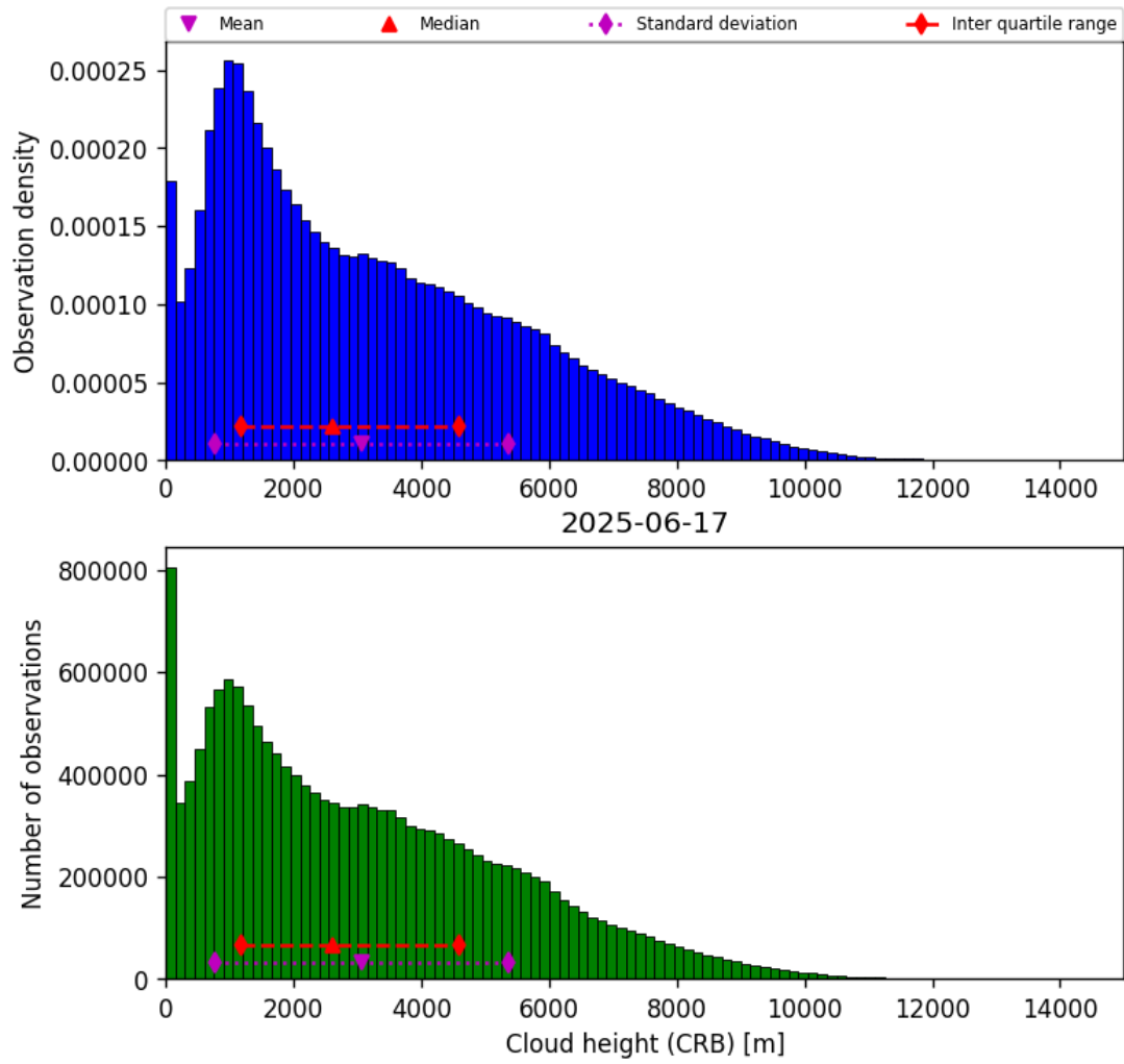
Figure 41: Histogram of “Cloud height (CRB)” for 2025-06-17 to 2025-06-17
