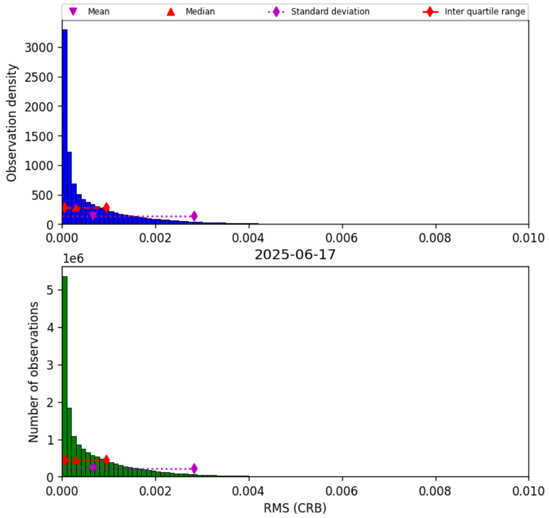
Figure 46: Histogram of “RMS (CRB)” for 2025-06-17 to 2025-06-17
