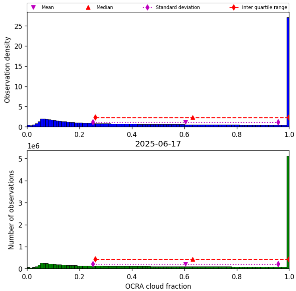
Figure 48: Histogram of “OCRA cloud fraction” for 2025-06-17 to 2025-06-17
