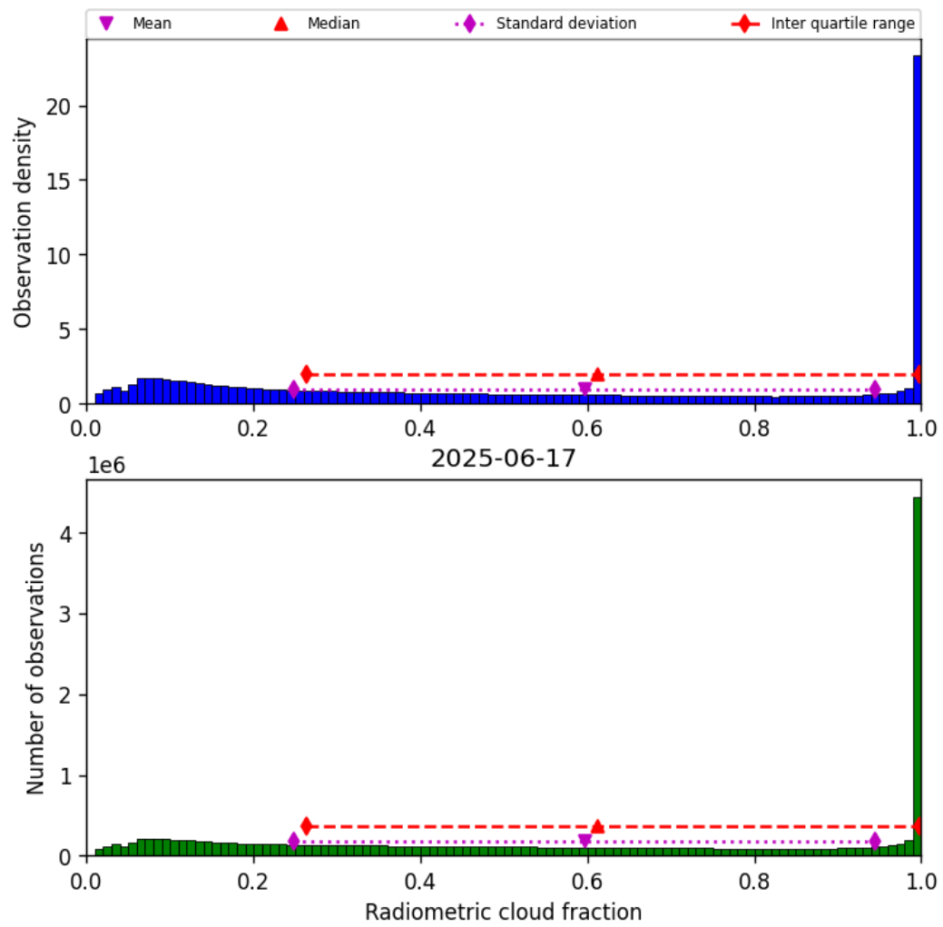
Figure 37: Histogram of “Radiometric cloud fraction” for 2025-06-17 to 2025-06-17
