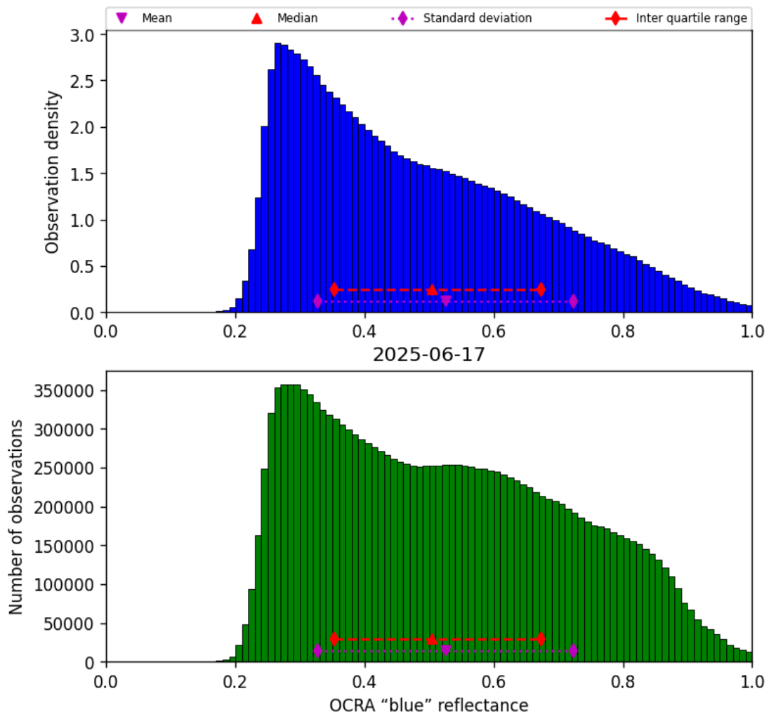
Figure 49: Histogram of “OCRA “blue” reflectance” for 2025-06-17 to 2025-06-17
