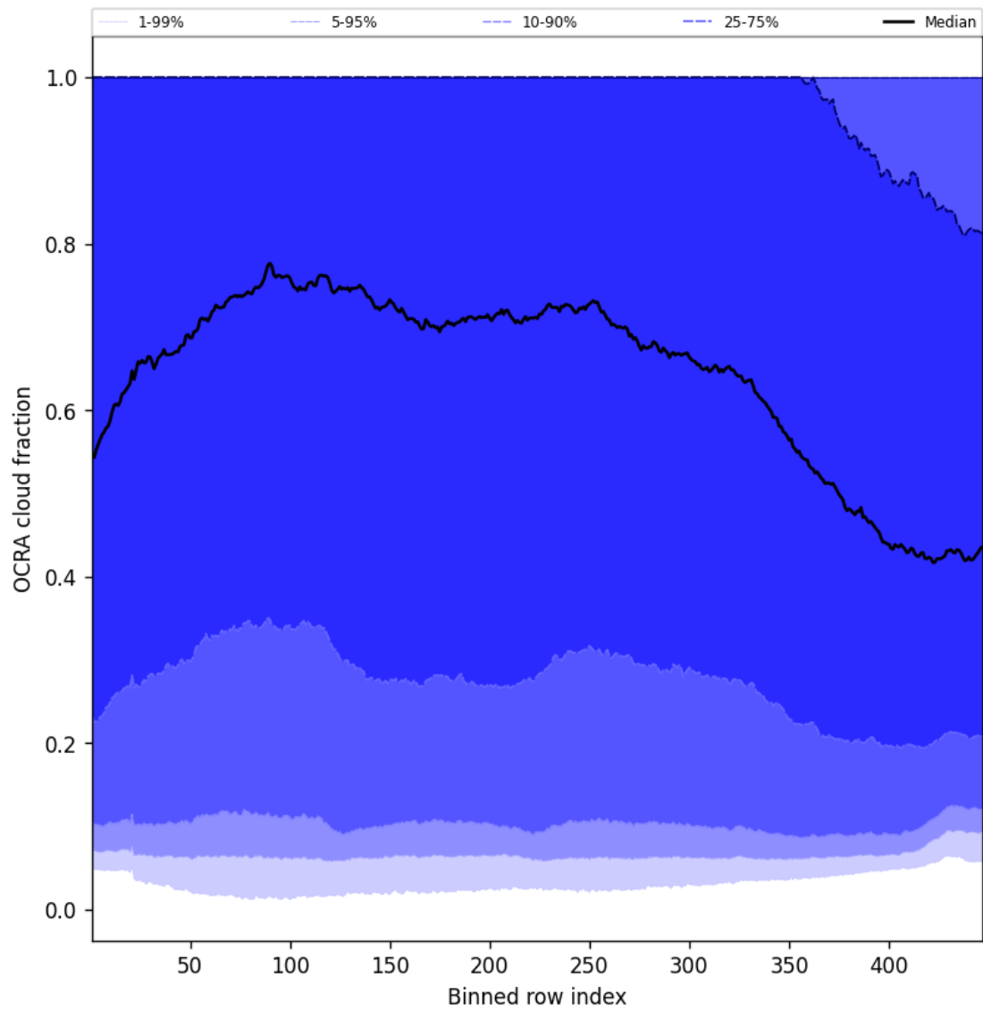
Figure 64: Along track statistics of “OCRA cloud fraction” for 2025-06-17 to 2025-06-17
