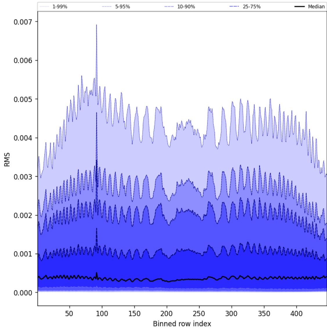
Figure 61: Along track statistics of “RMS” for 2025-06-17 to 2025-06-17
