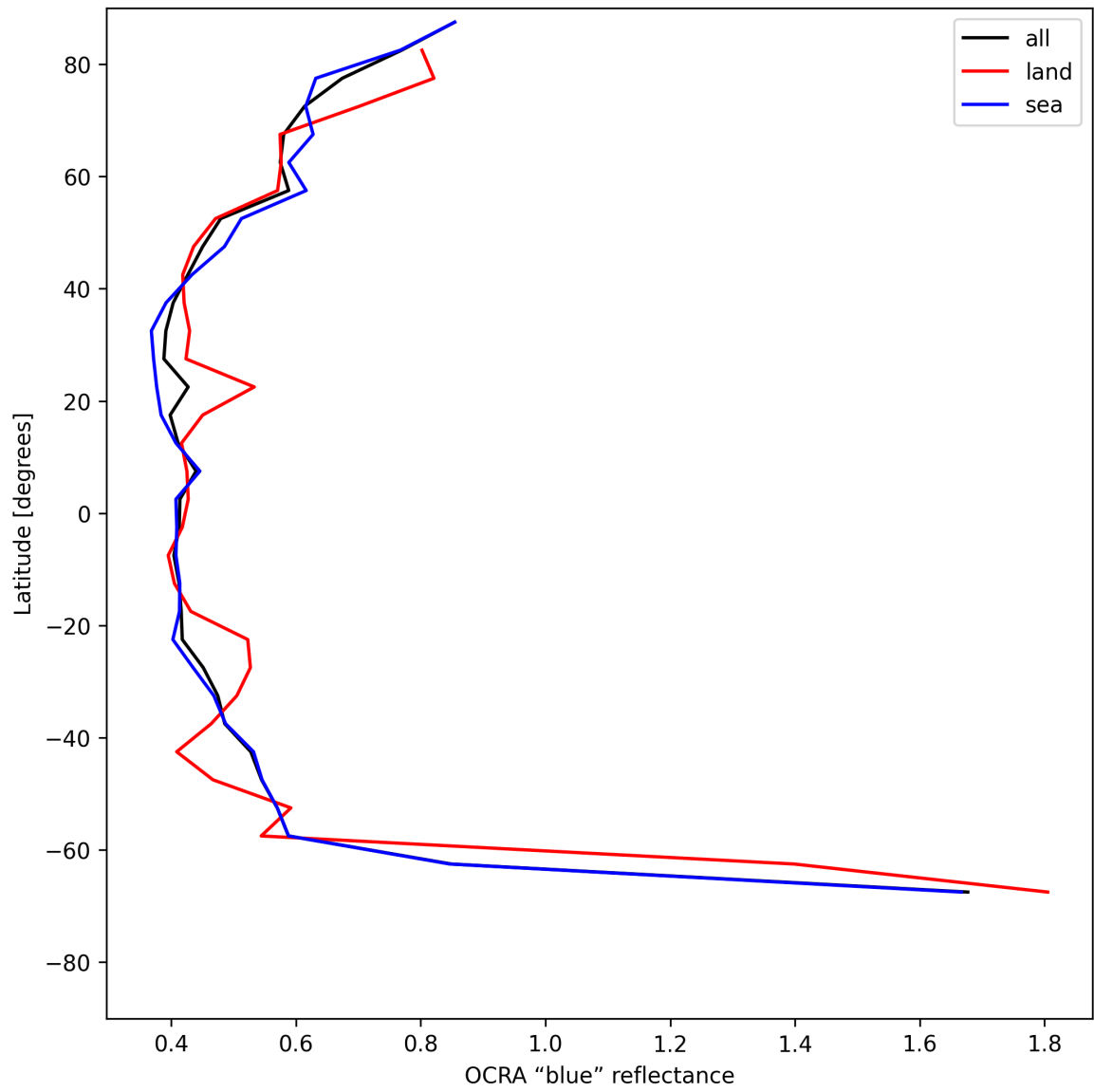
Figure 33: Zonal average of “OCRA “blue” reflectance” for 2025-06-17 to 2025-06-17.
