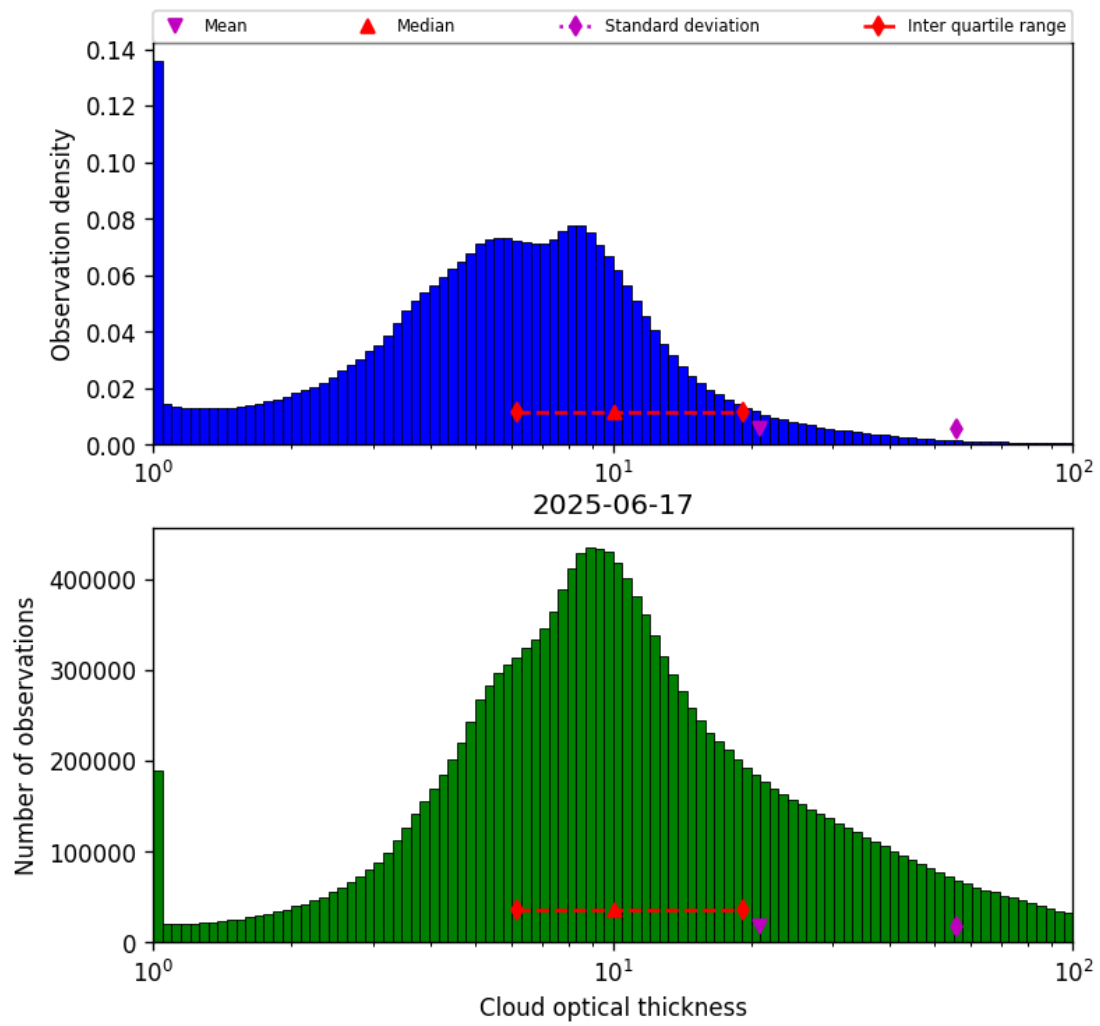
Figure 39: Histogram of “Cloud optical thickness” for 2025-06-17 to 2025-06-17
