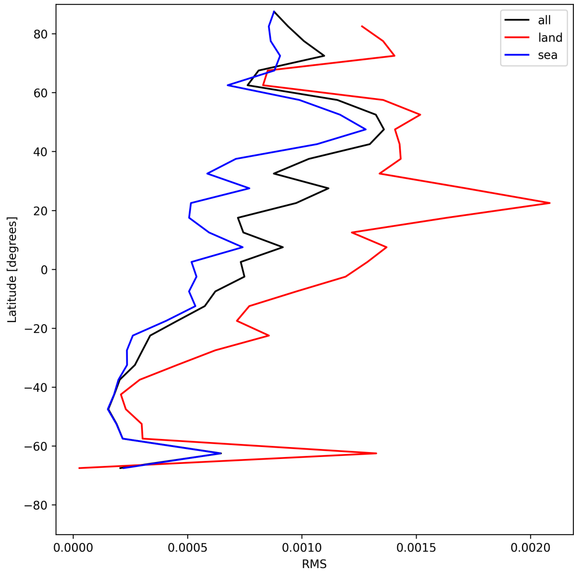
Figure 29: Zonal average of “RMS” for 2025-06-17 to 2025-06-17.
