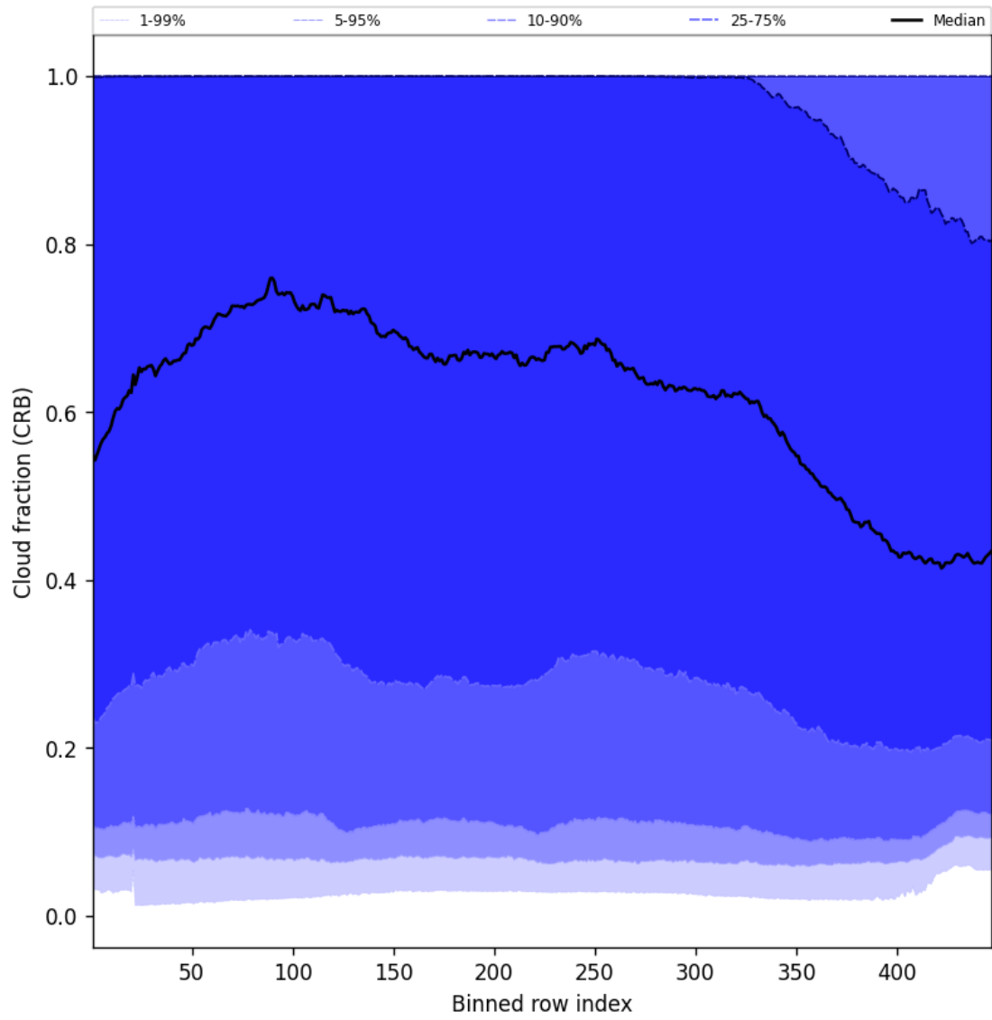
Figure 56: Along track statistics of “Cloud fraction (CRB)” for 2025-06-17 to 2025-06-17
