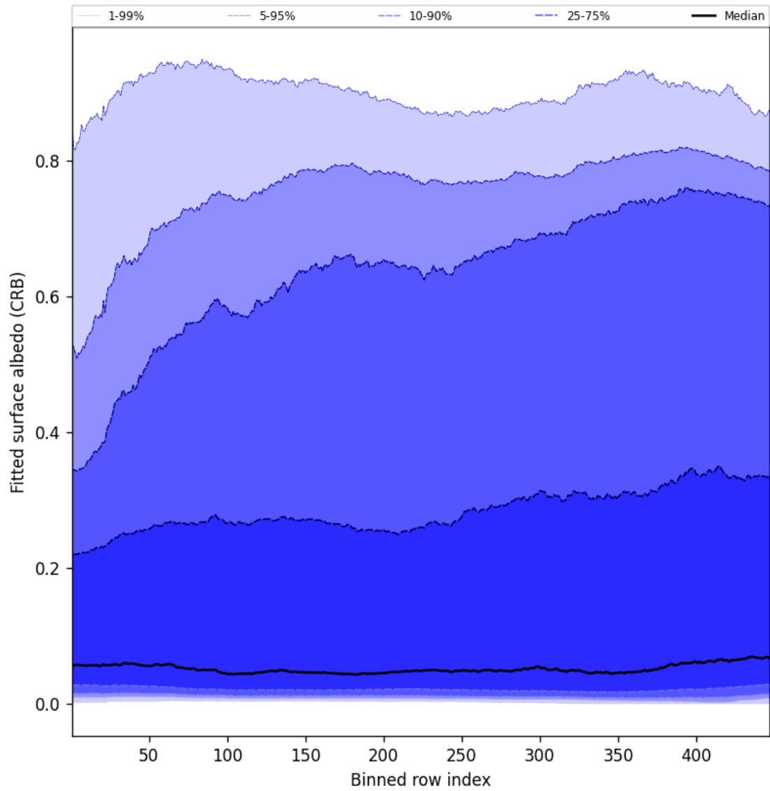
Figure 60: Along track statistics of “Fitted surface albedo (CRB)” for 2025-06-17 to 2025-06-17
