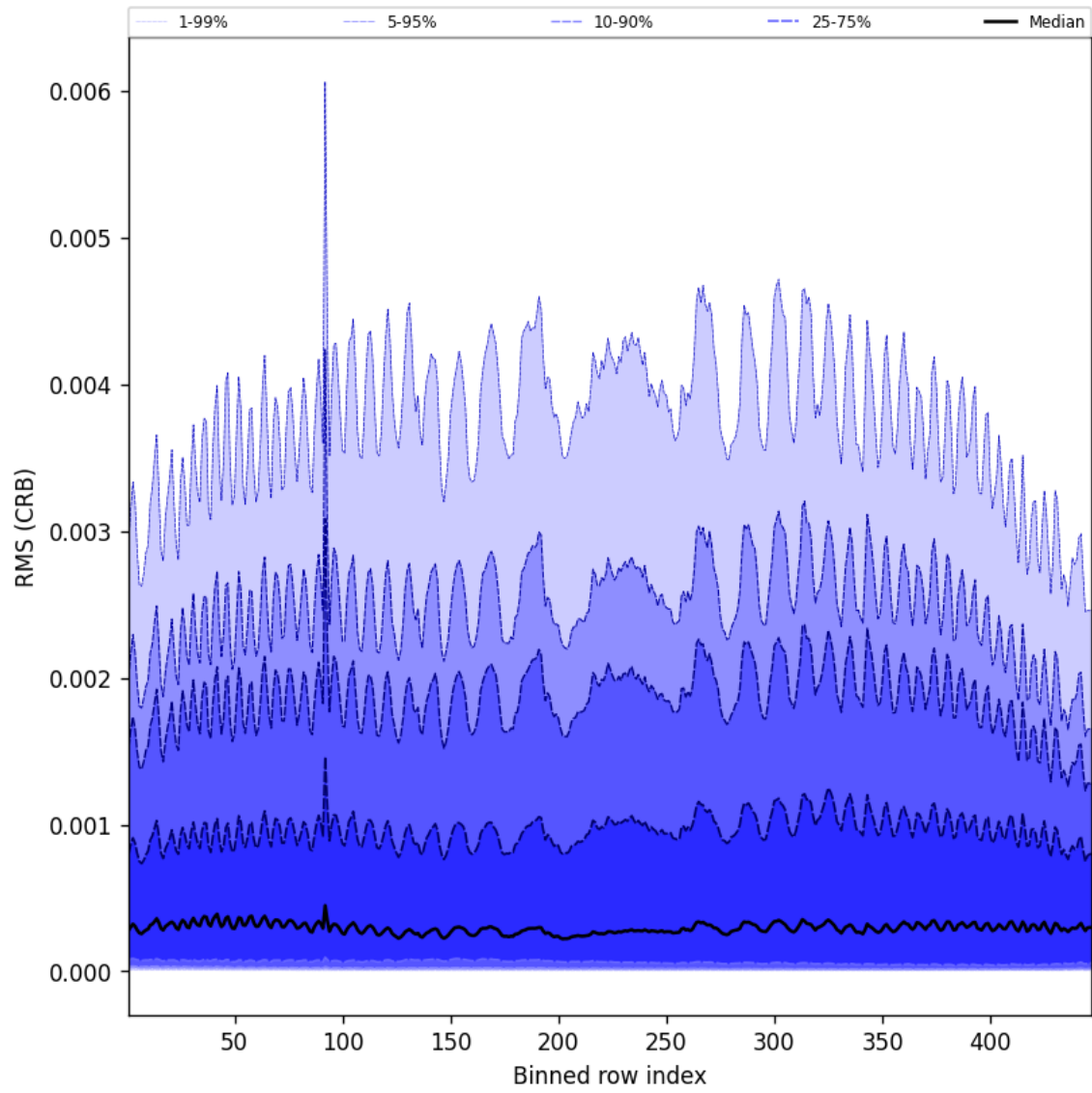
Figure 62: Along track statistics of “RMS (CRB)” for 2025-06-17 to 2025-06-17
