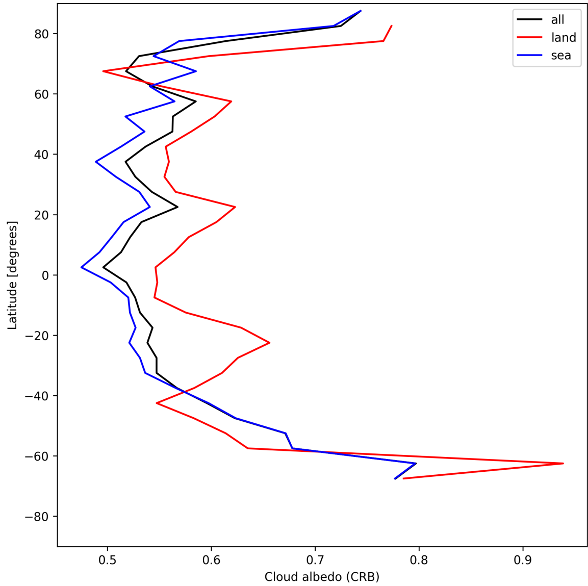
Figure 26: Zonal average of “Cloud albedo (CRB)” for 2025-06-17 to 2025-06-17.
