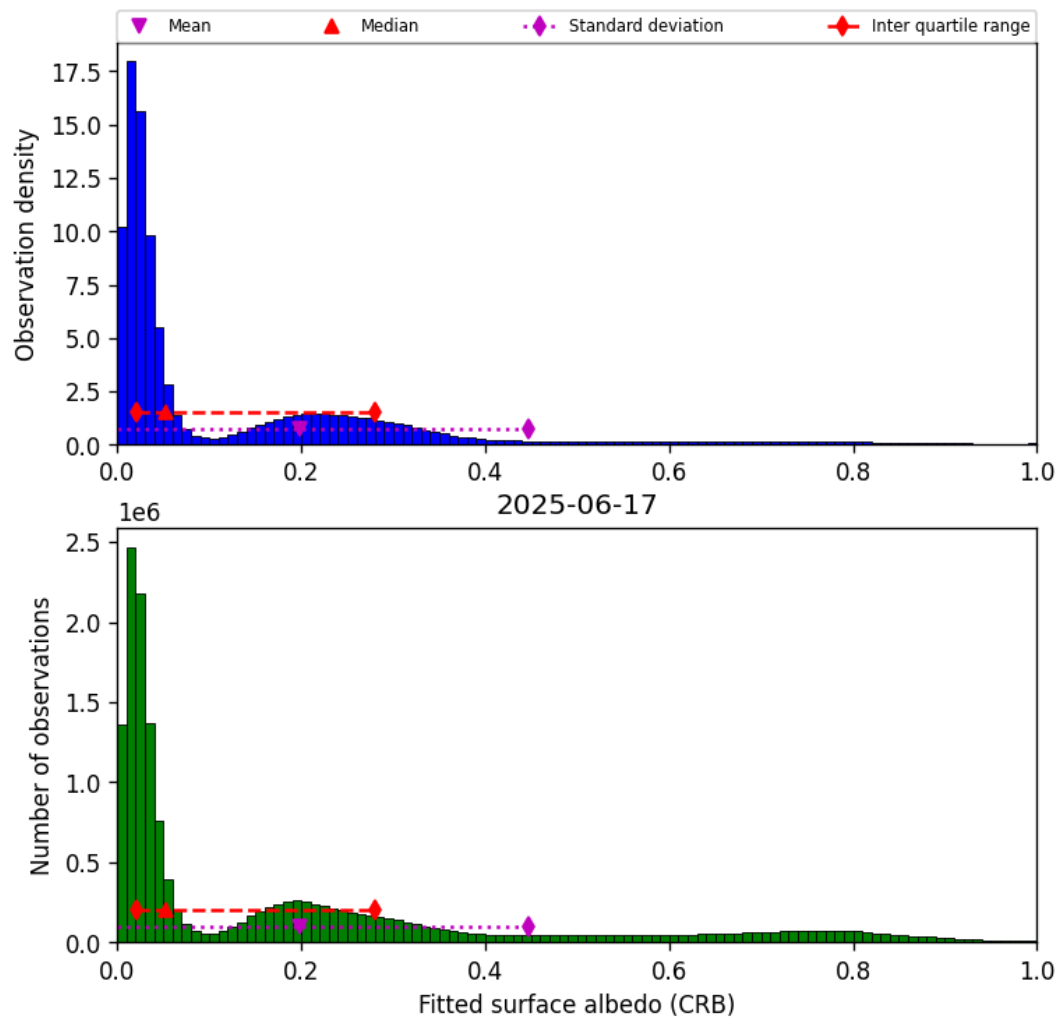
Figure 44: Histogram of “Fitted surface albedo (CRB)” for 2025-06-17 to 2025-06-17
