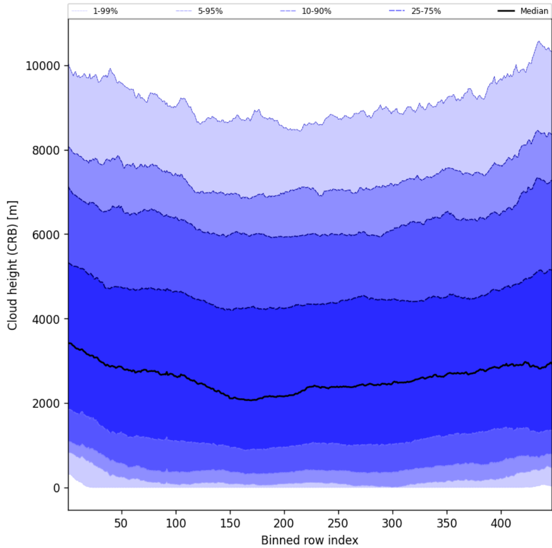
Figure 57: Along track statistics of “Cloud height (CRB)” for 2025-06-17 to 2025-06-17
