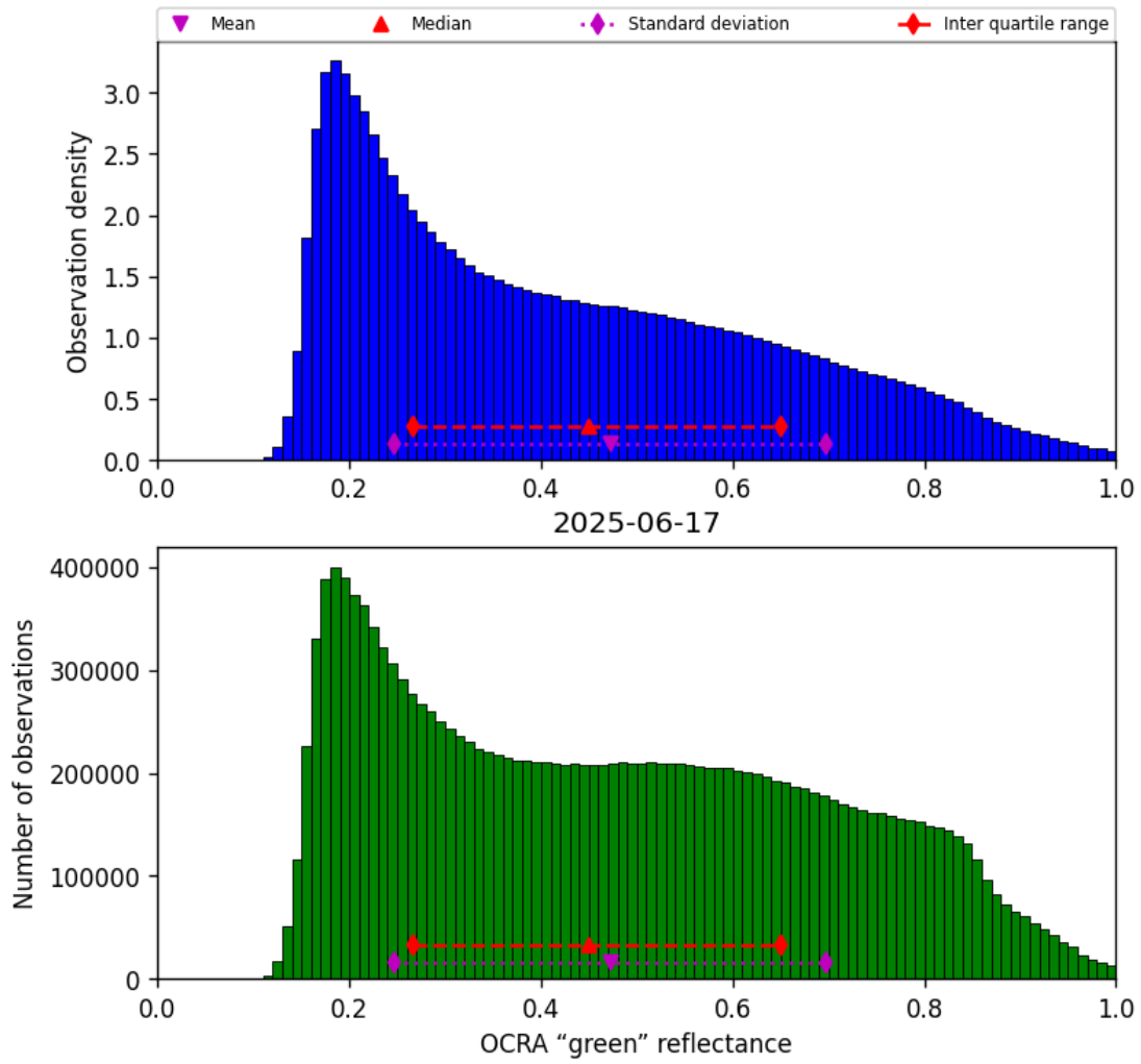
Figure 50: Histogram of “OCRA “green” reflectance” for 2025-06-17 to 2025-06-17
