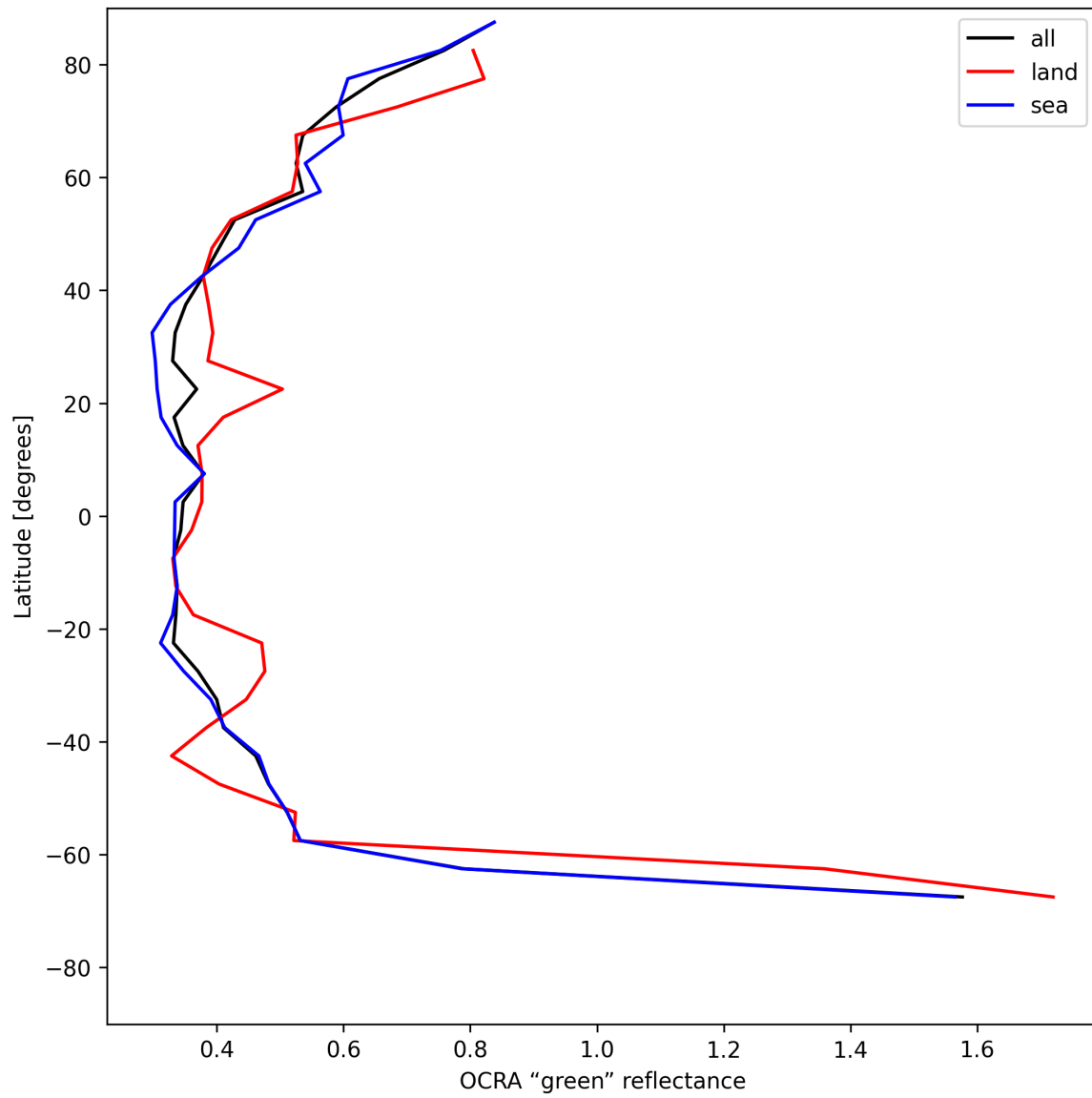
Figure 34: Zonal average of “OCRA “green” reflectance” for 2025-06-17 to 2025-06-17.
