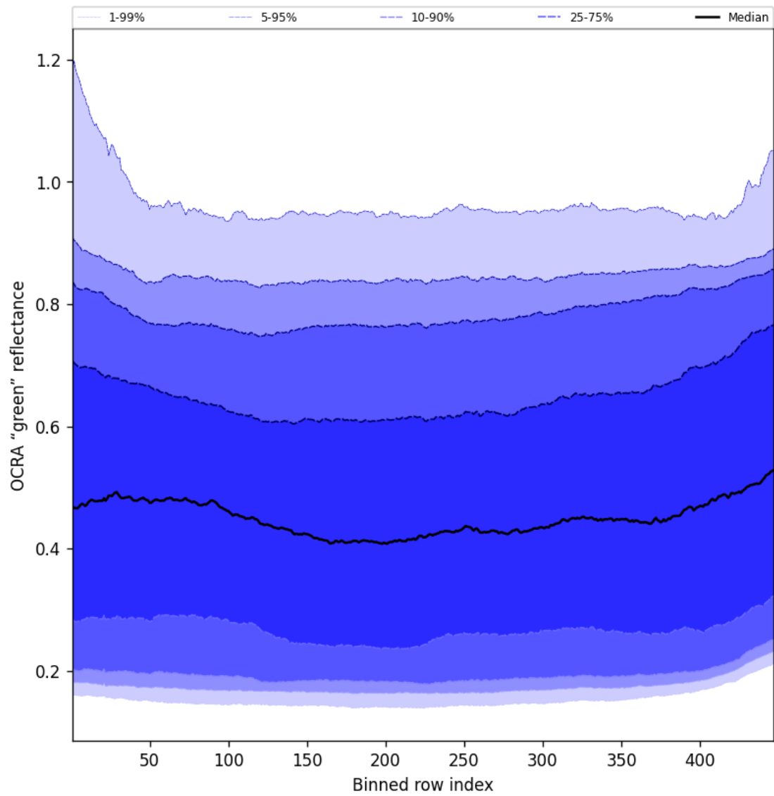
Figure 66: Along track statistics of "OCRA "green" reflectance" for 2025-06-17 to 2025-06-17
