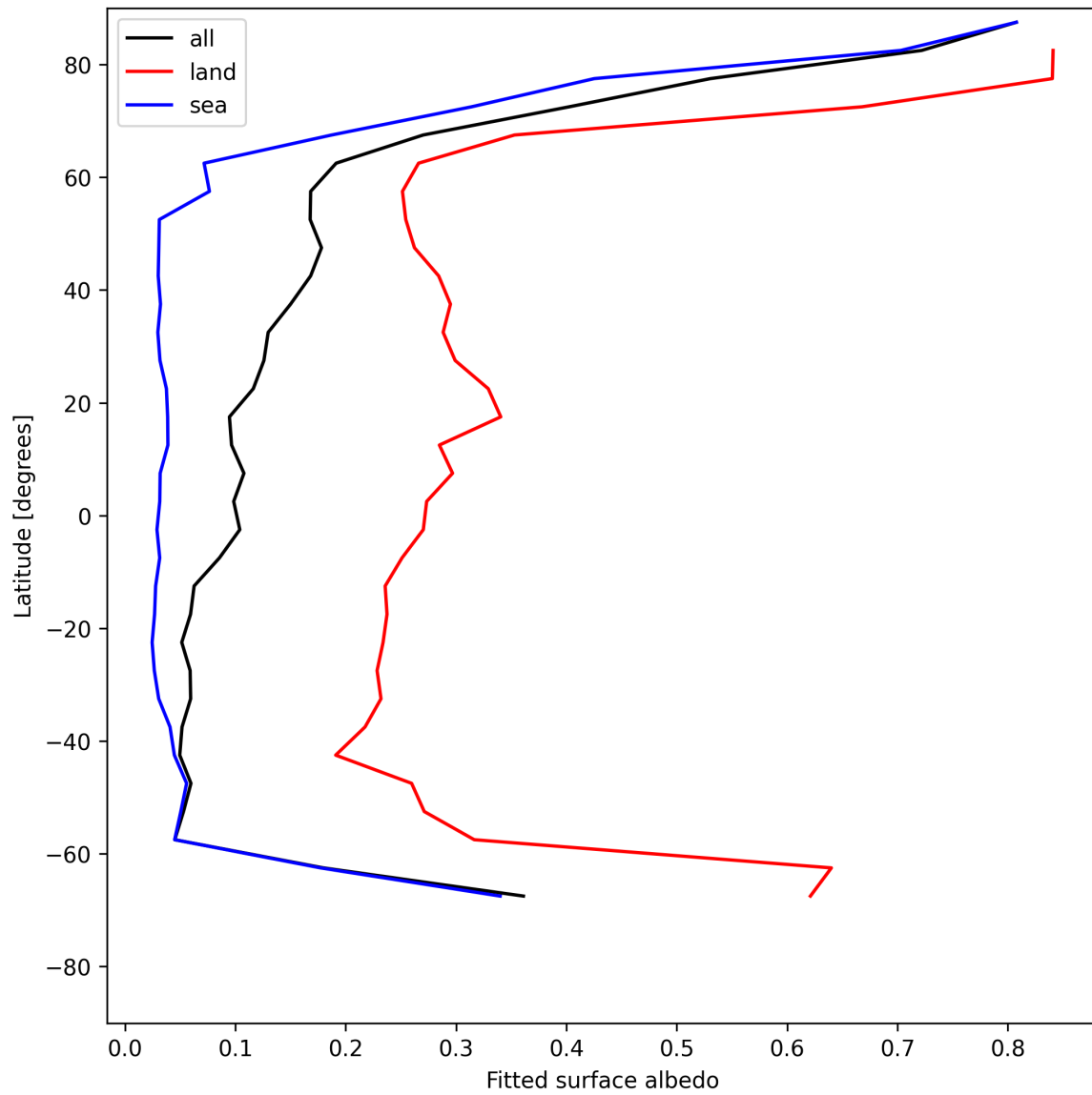
Figure 27: Zonal average of “Fitted surface albedo” for 2025-06-17 to 2025-06-17.
