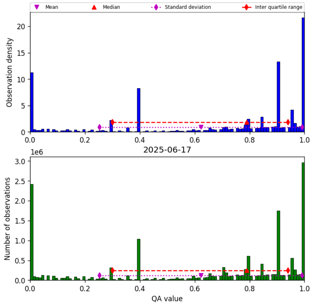
Figure 36: Histogram of “QA value” for 2025-06-17 to 2025-06-17
