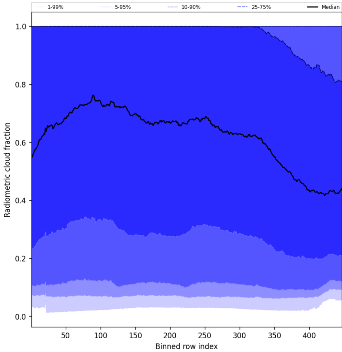
Figure 53: Along track statistics of “Radiometric cloud fraction” for 2025-06-17 to 2025-06-17
