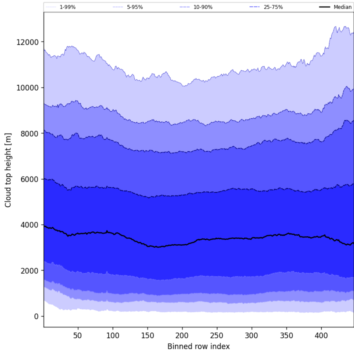
Figure 54: Along track statistics of “Cloud top height” for 2025-06-17 to 2025-06-17
