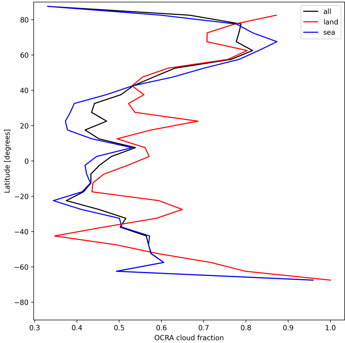
Figure 32: Zonal average of “OCRA cloud fraction” for 2025-06-17 to 2025-06-17.
