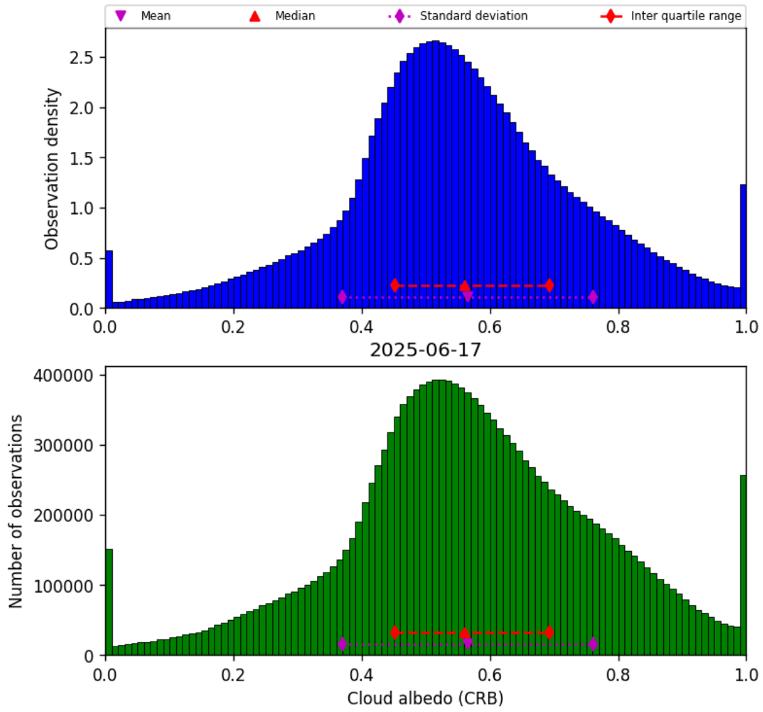
Figure 42: Histogram of “Cloud albedo (CRB)” for 2025-06-17 to 2025-06-17
