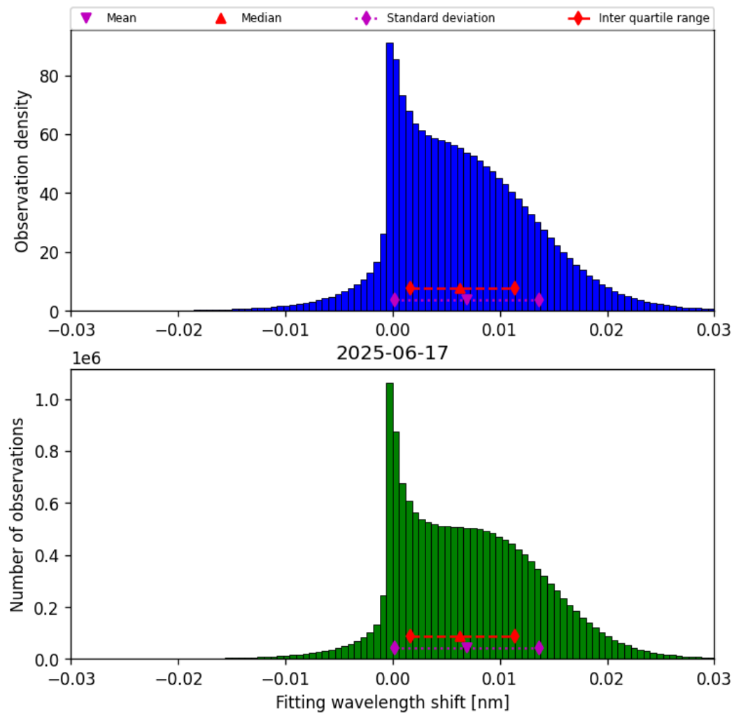
Figure 47: Histogram of “Fitting wavelength shift” for 2025-06-17 to 2025-06-17
