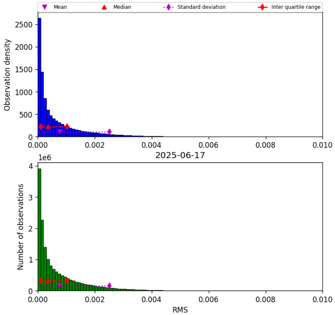
Figure 45: Histogram of “RMS” for 2025-06-17 to 2025-06-17
