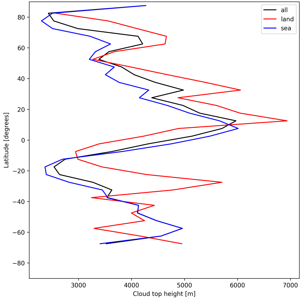
Figure 22: Zonal average of “Cloud top height” for 2025-06-17 to 2025-06-17.
