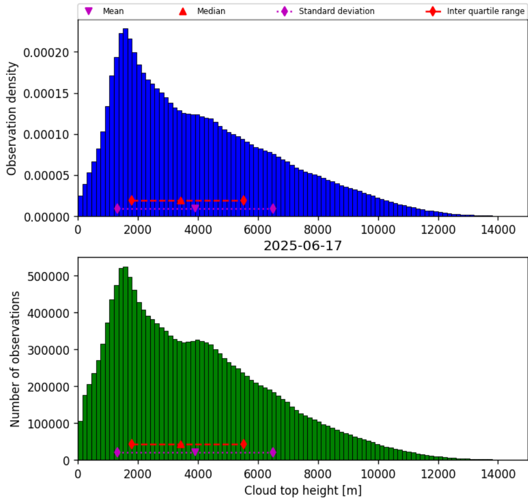
Figure 38: Histogram of “Cloud top height” for 2025-06-17 to 2025-06-17
