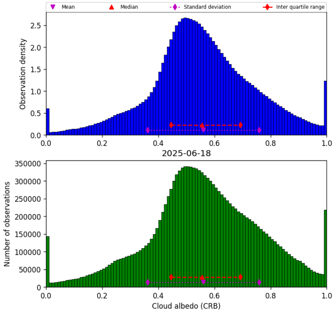
Figure 42: Histogram of “Cloud albedo (CRB)” for 2025-06-18 to 2025-06-19
