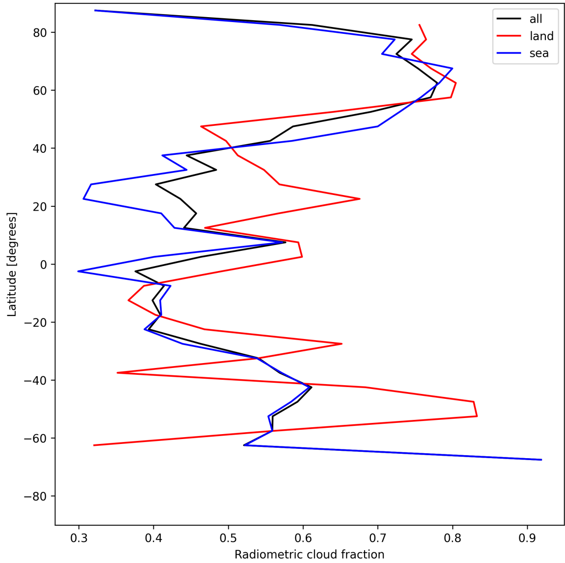
Figure 21: Zonal average of “Radiometric cloud fraction” for 2025-06-18 to 2025-06-19.
