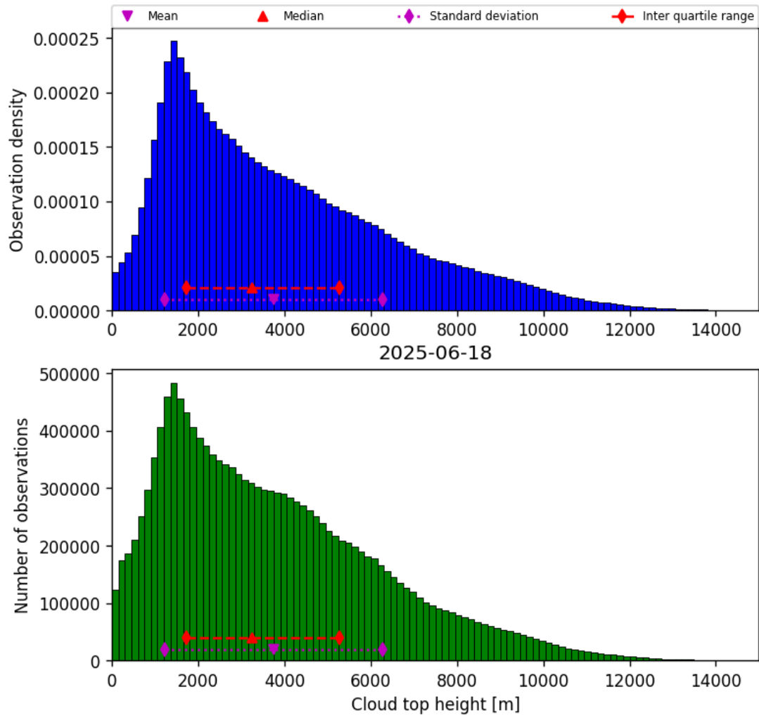
Figure 38: Histogram of “Cloud top height” for 2025-06-18 to 2025-06-19
