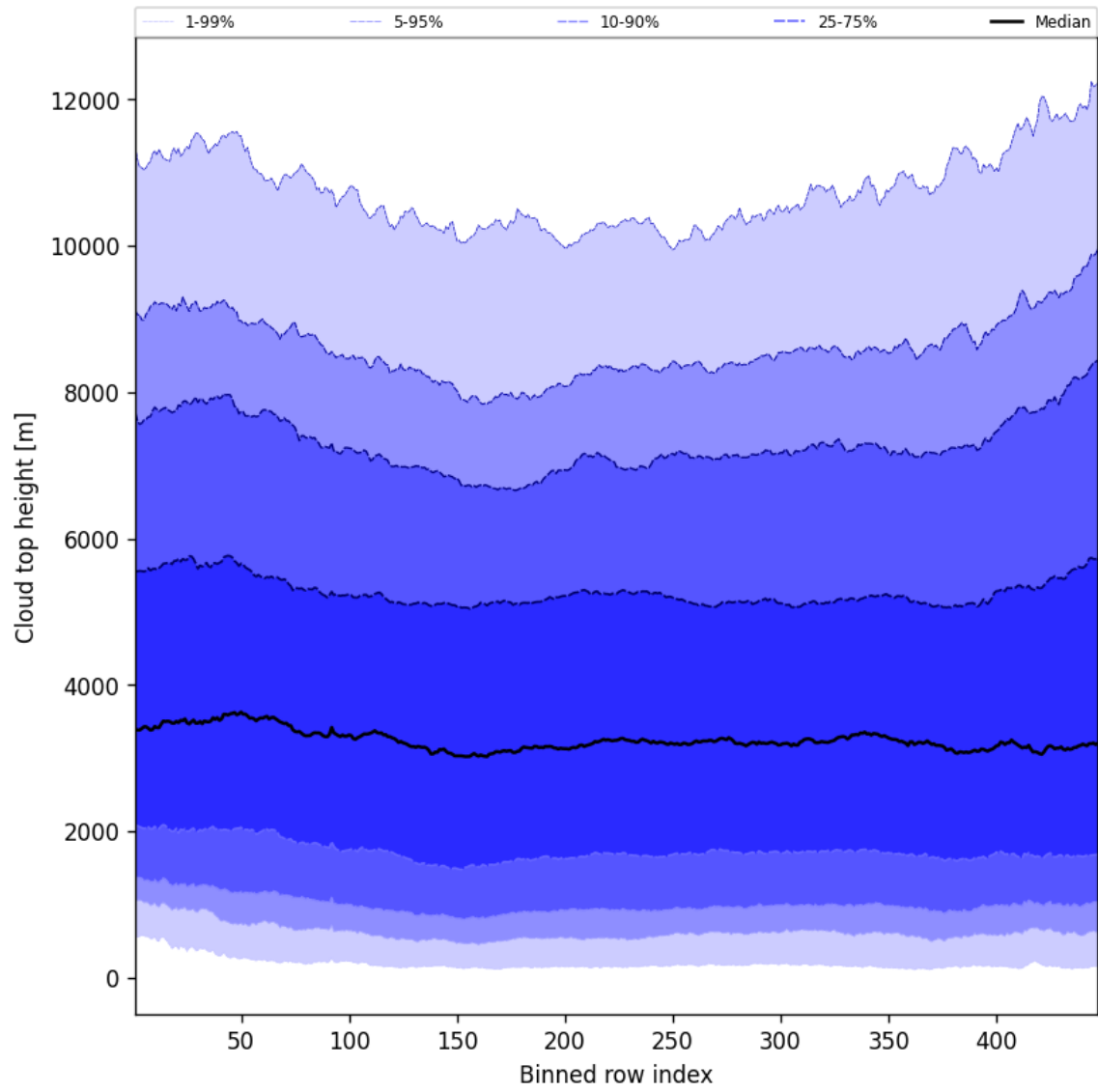
Figure 54: Along track statistics of “Cloud top height” for 2025-06-18 to 2025-06-19
