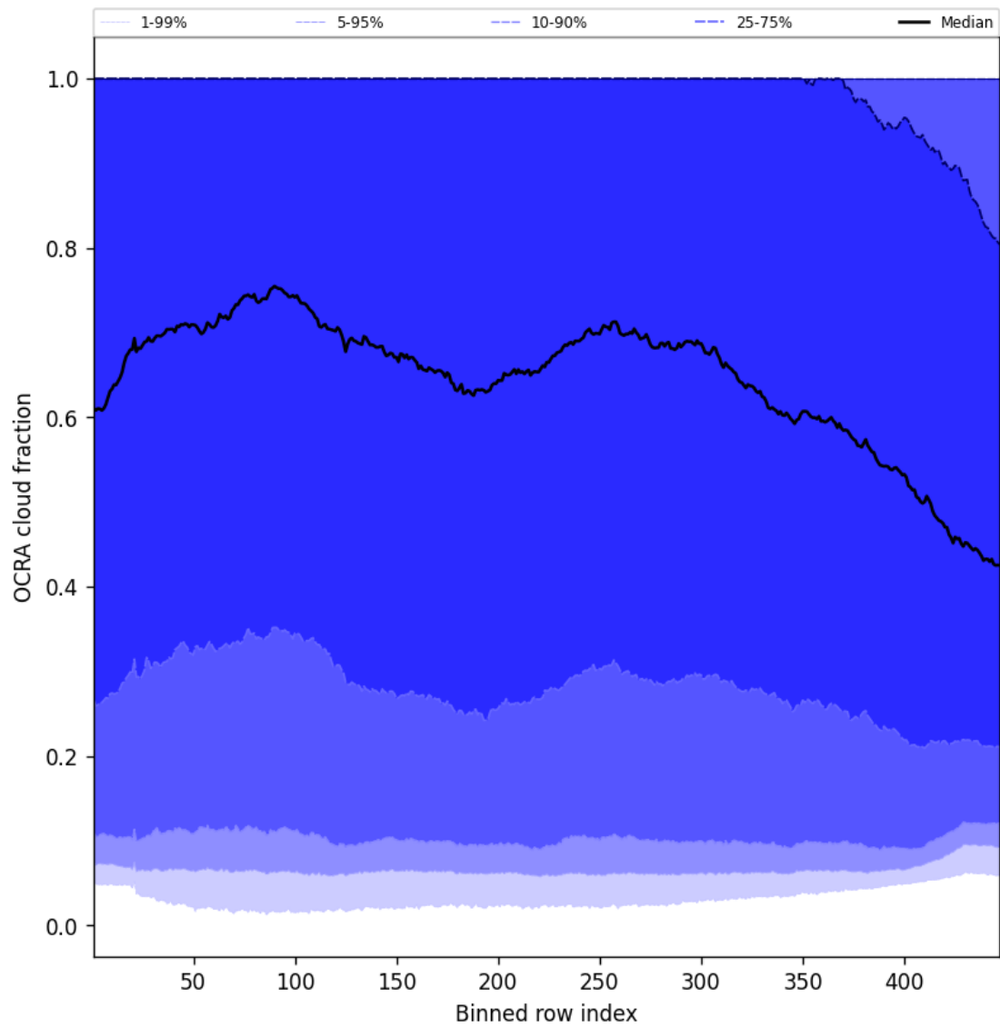
Figure 64: Along track statistics of “OCRA cloud fraction” for 2025-06-18 to 2025-06-19
