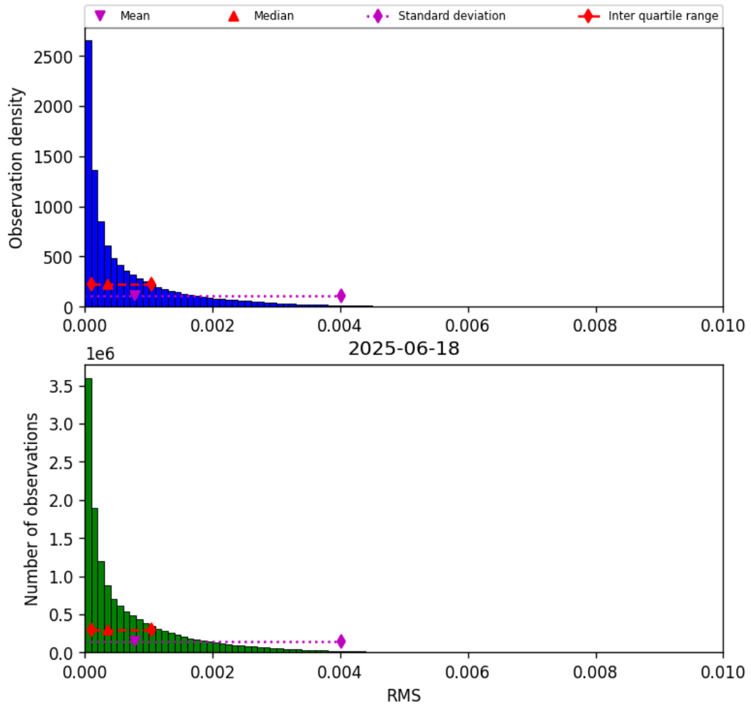
Figure 45: Histogram of “RMS” for 2025-06-18 to 2025-06-19
