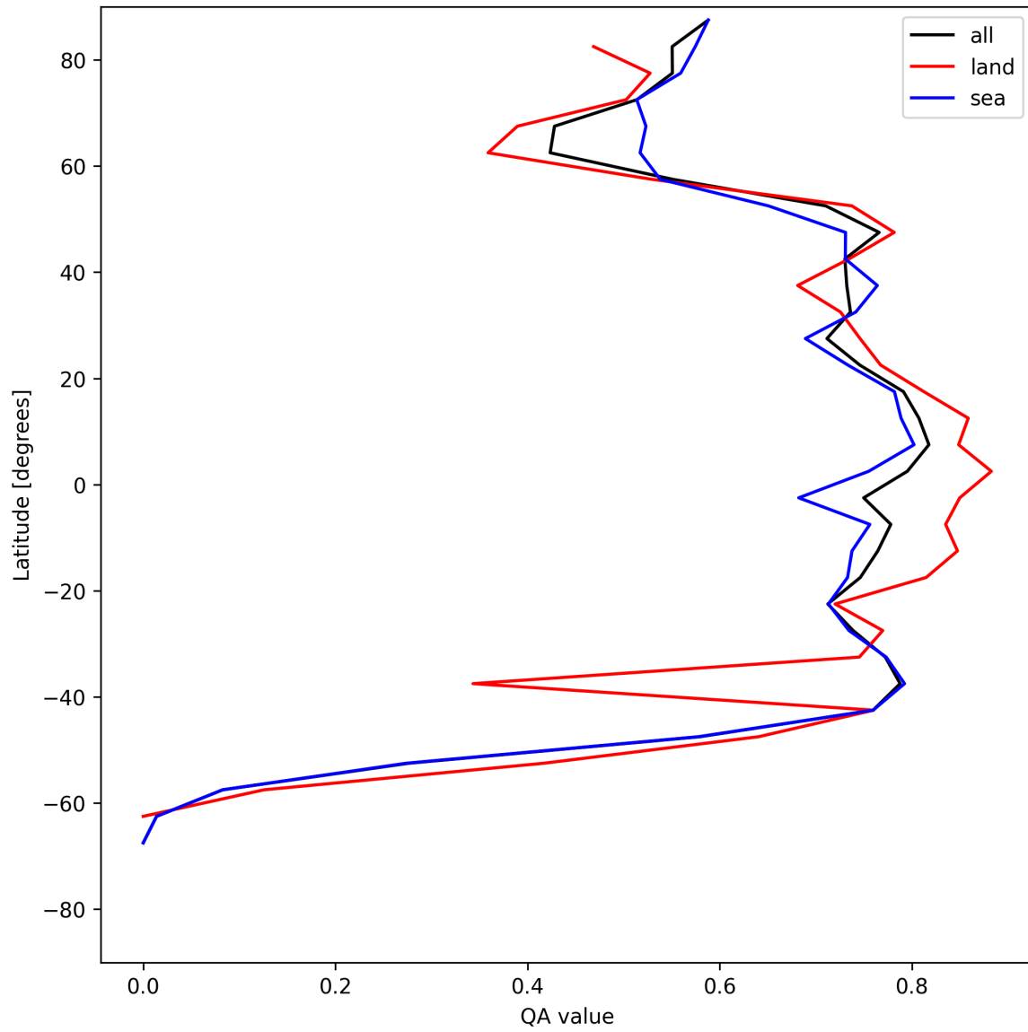
Figure 20: Zonal average of “QA value” for 2025-06-18 to 2025-06-19.
