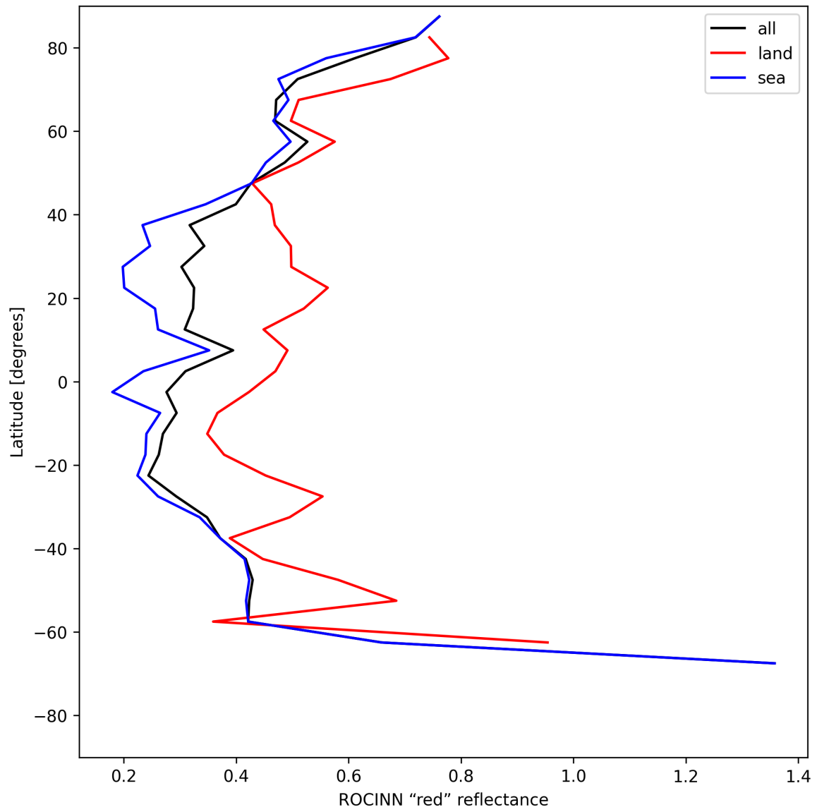
Figure 35: Zonal average of “ROCINN “red” reflectance” for 2025-06-18 to 2025-06-19.
