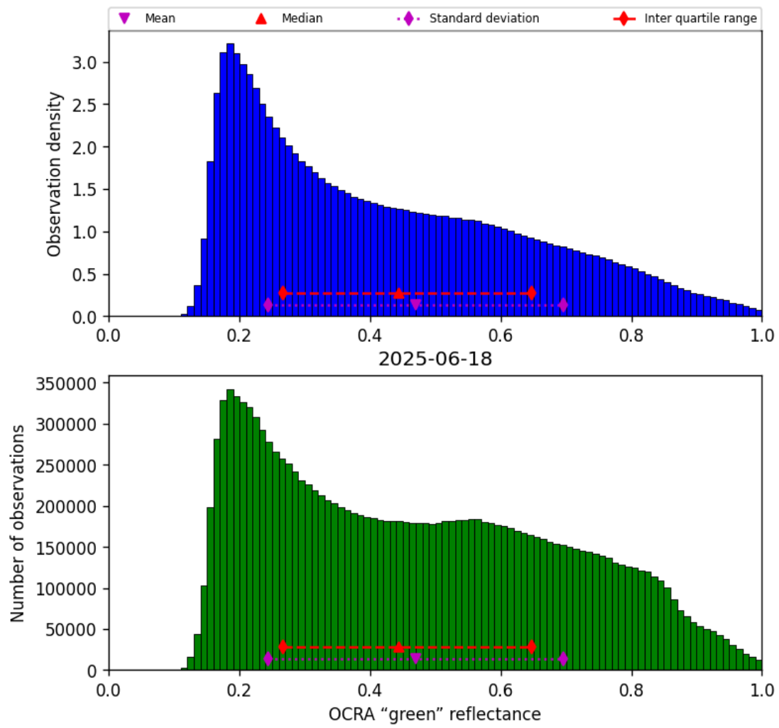
Figure 50: Histogram of “OCRA “green” reflectance” for 2025-06-18 to 2025-06-19
