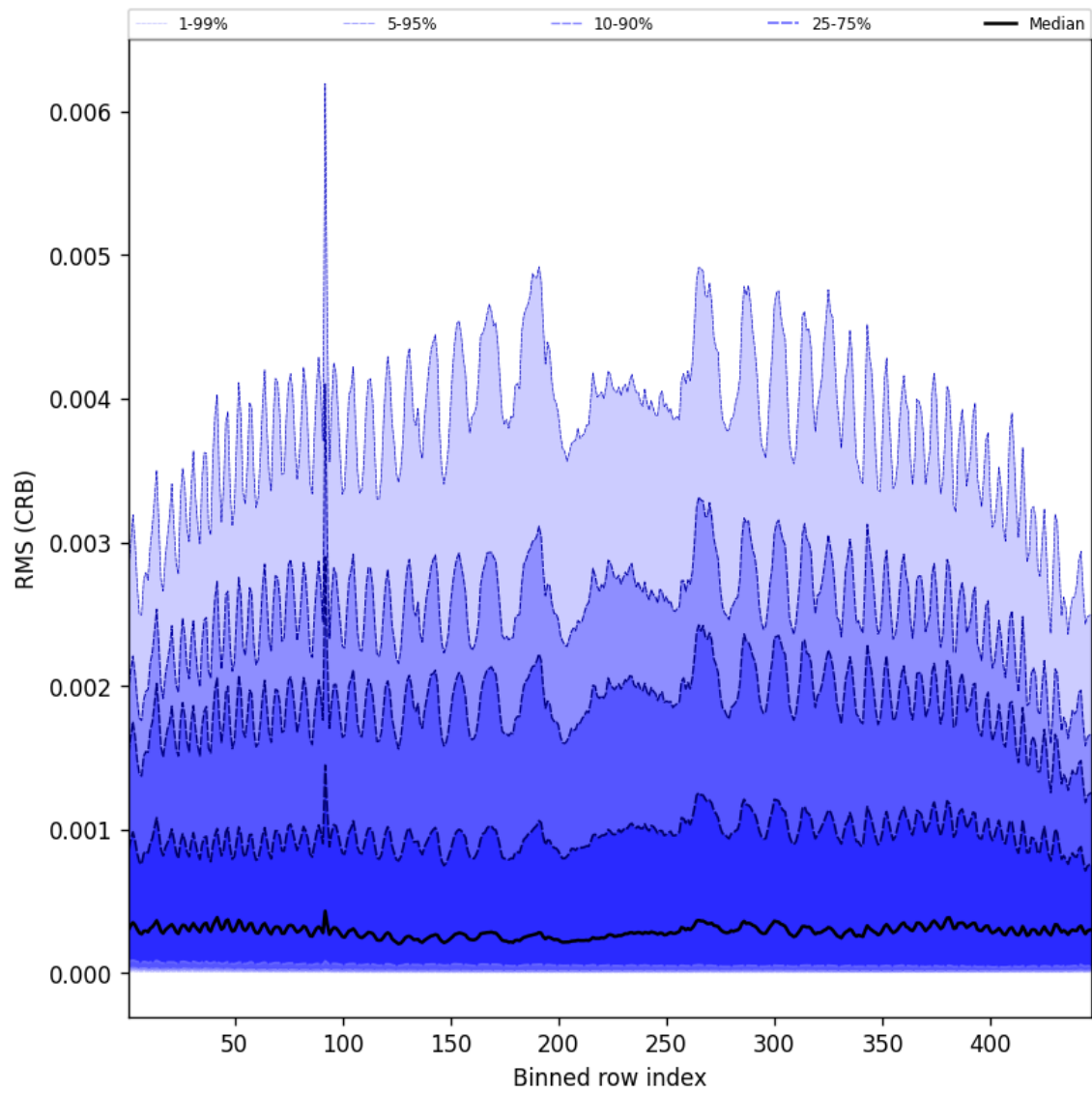
Figure 62: Along track statistics of “RMS (CRB)” for 2025-06-18 to 2025-06-19
