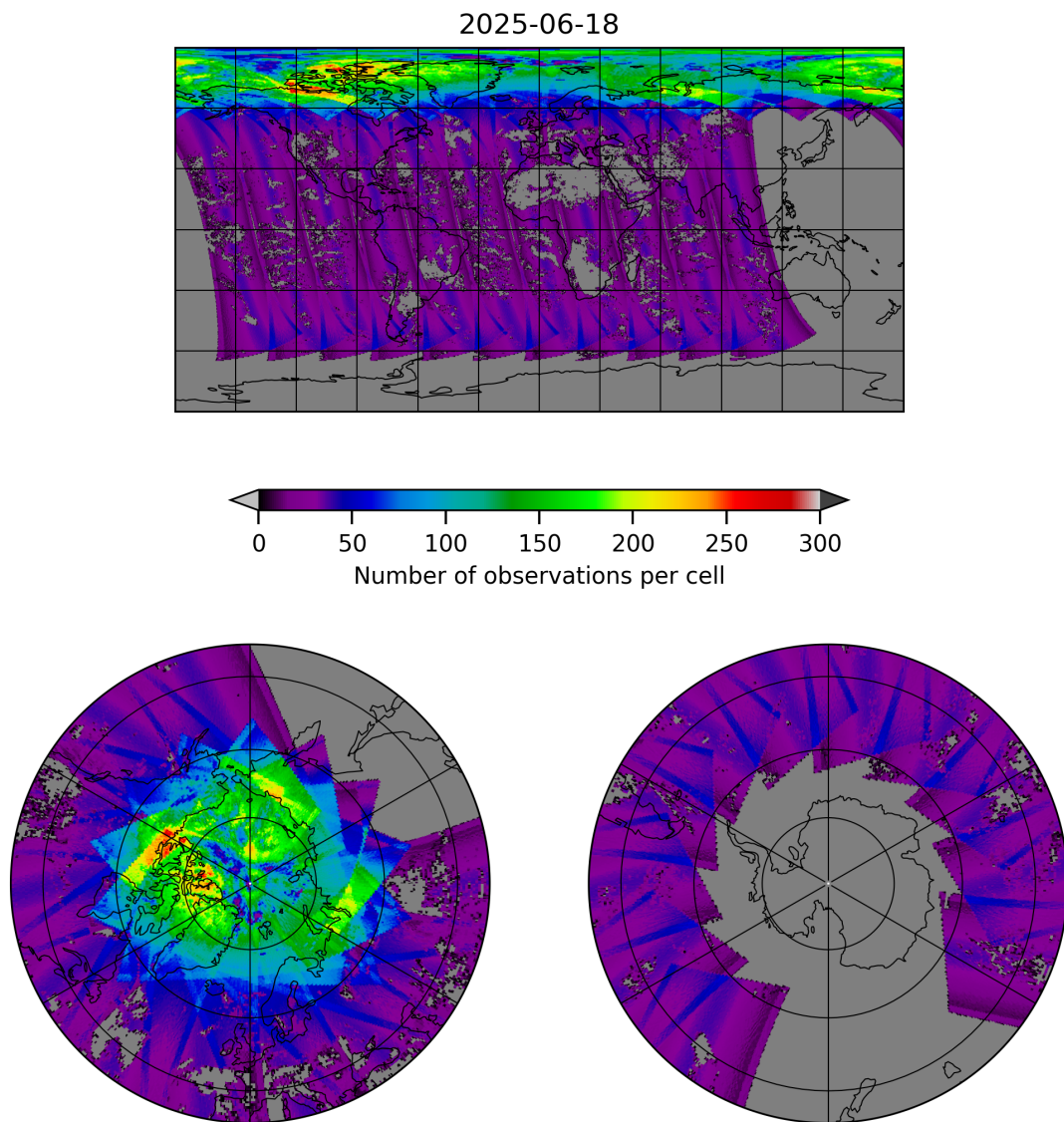
Figure 19: Map of the number of observations for 2025-06-18 to 2025-06-19
