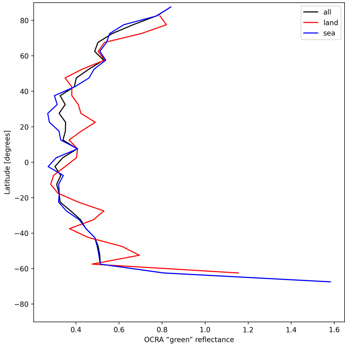
Figure 34: Zonal average of “OCRA “green” reflectance” for 2025-06-18 to 2025-06-19.
