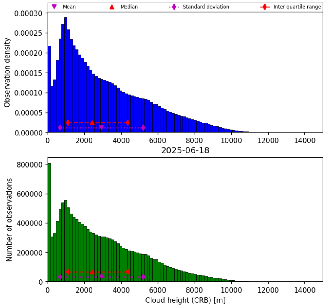
Figure 41: Histogram of “Cloud height (CRB)” for 2025-06-18 to 2025-06-19
