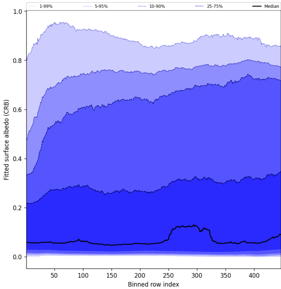
Figure 60: Along track statistics of “Fitted surface albedo (CRB)” for 2025-06-18 to 2025-06-19
