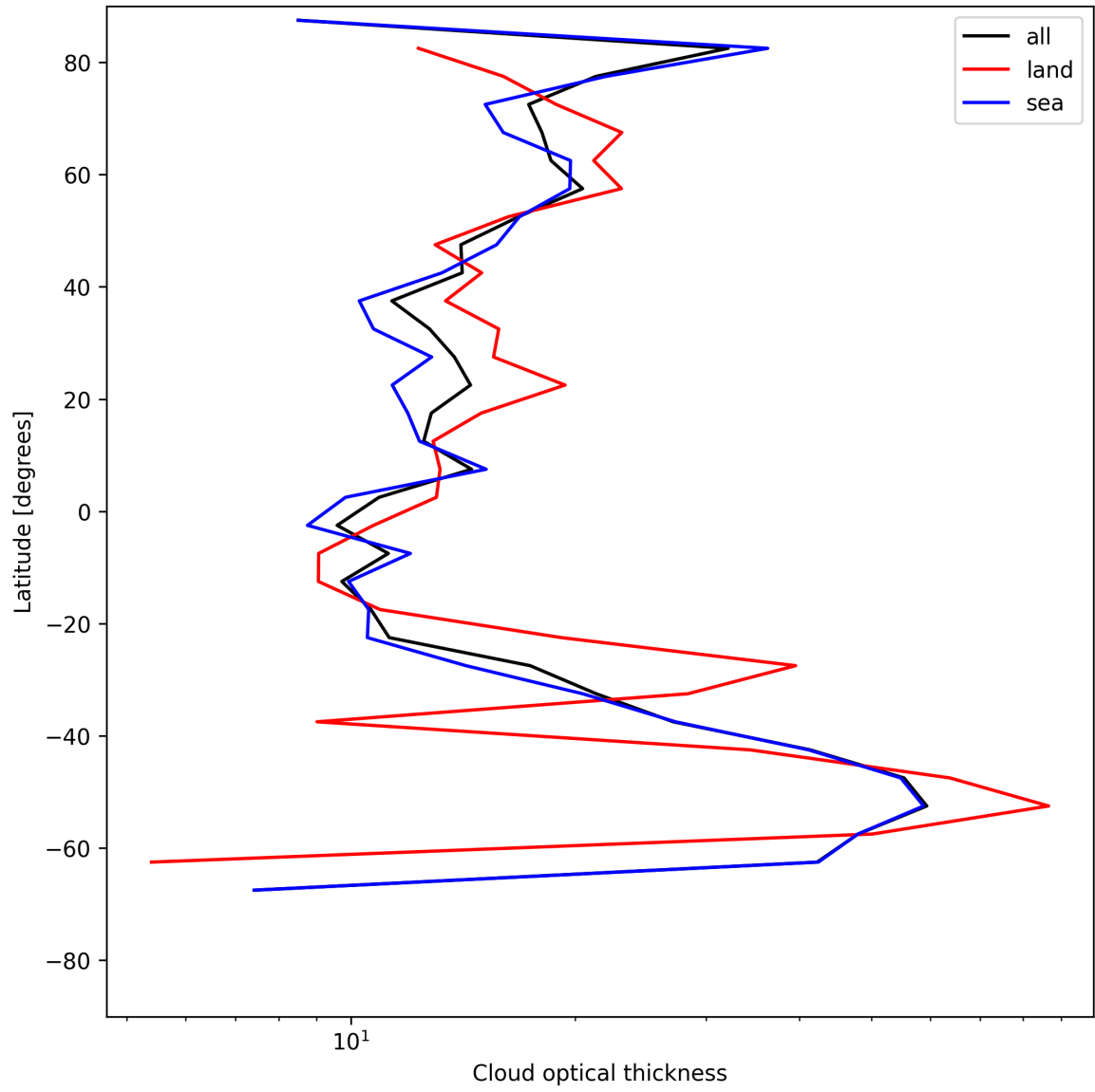
Figure 23: Zonal average of “Cloud optical thickness” for 2025-06-18 to 2025-06-19.
