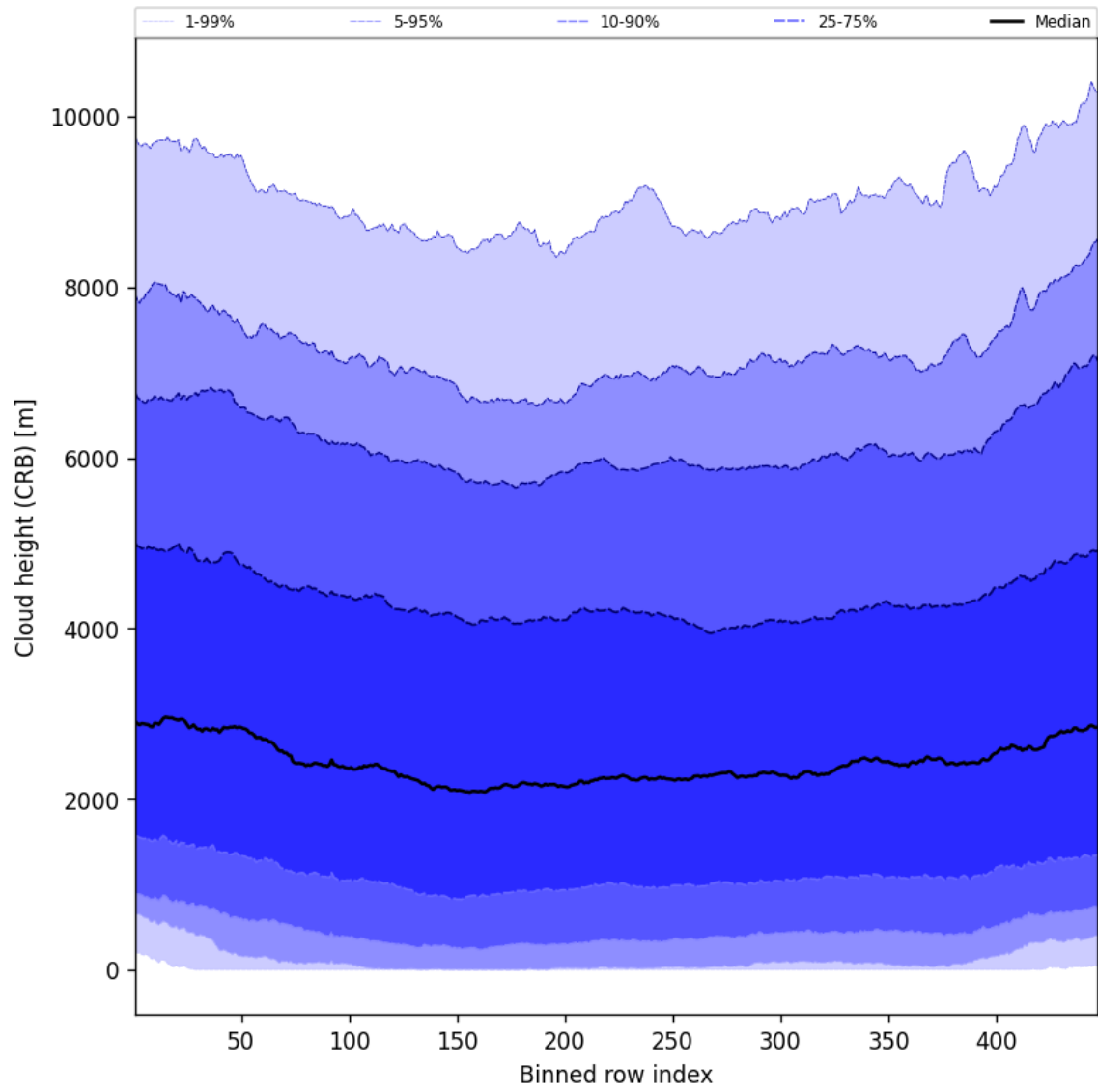
Figure 57: Along track statistics of “Cloud height (CRB)” for 2025-06-18 to 2025-06-19
