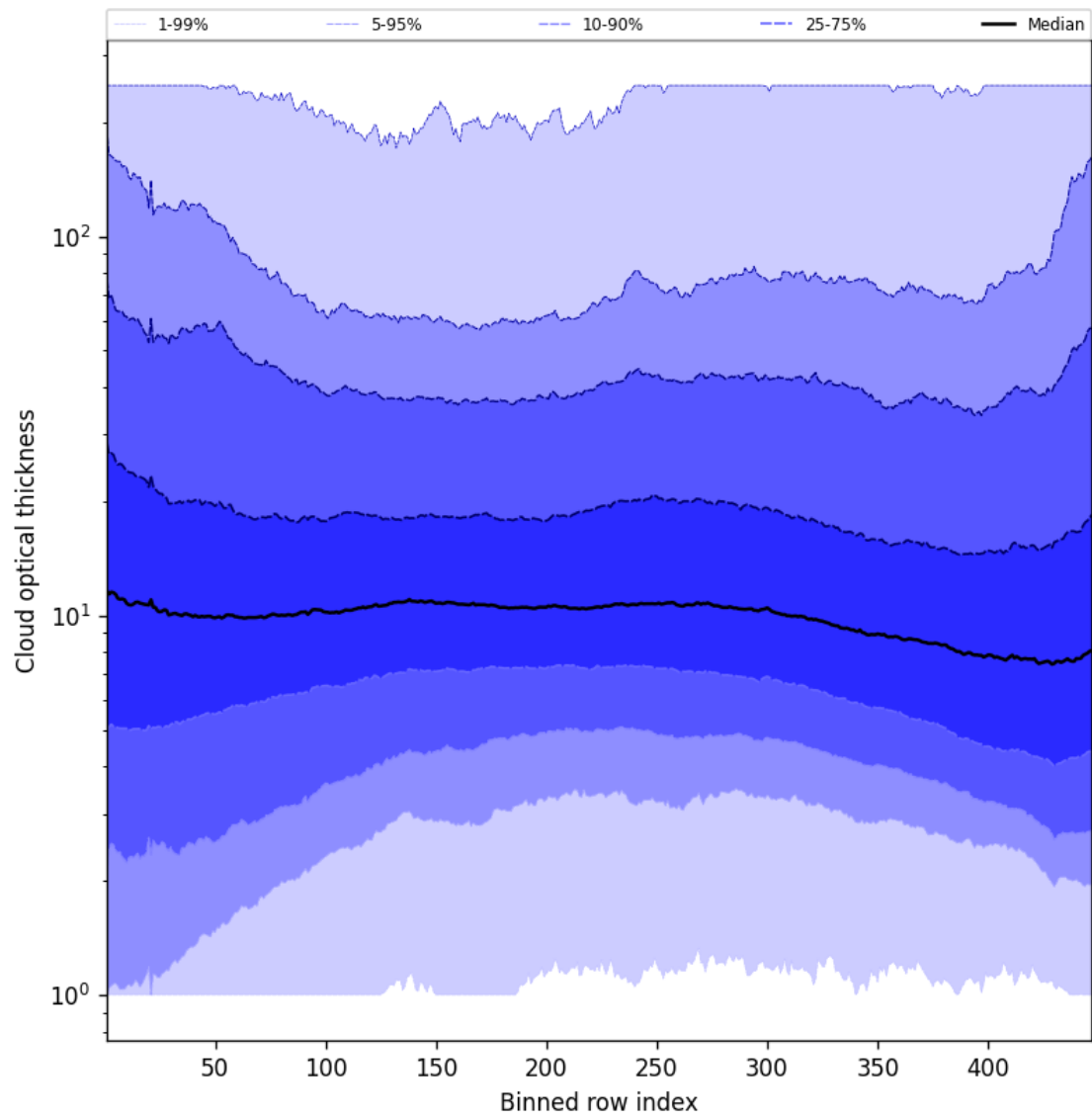
Figure 55: Along track statistics of “Cloud optical thickness” for 2025-06-18 to 2025-06-19
