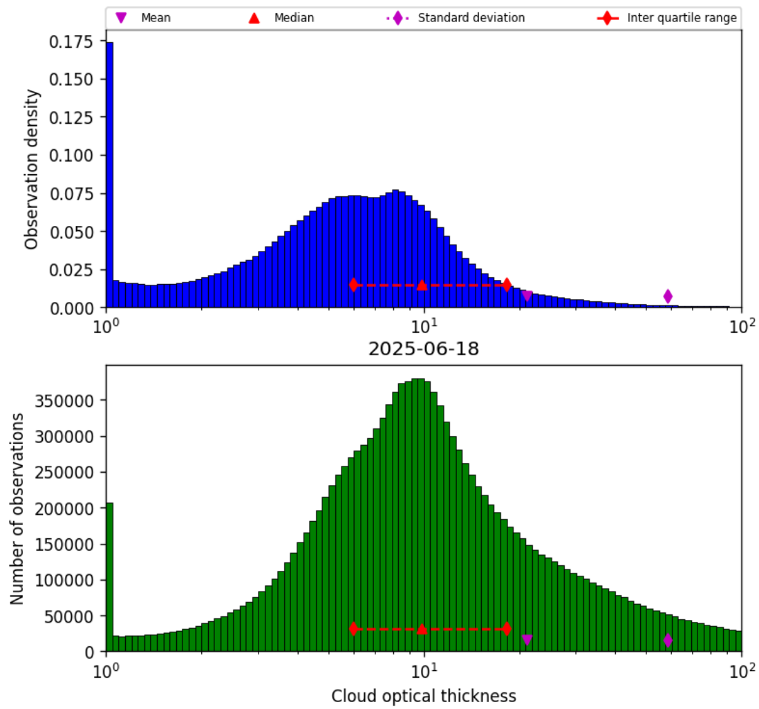
Figure 39: Histogram of “Cloud optical thickness” for 2025-06-18 to 2025-06-19
