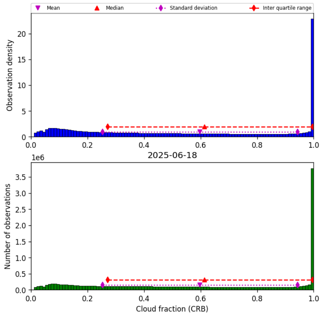
Figure 40: Histogram of “Cloud fraction (CRB)” for 2025-06-18 to 2025-06-19
