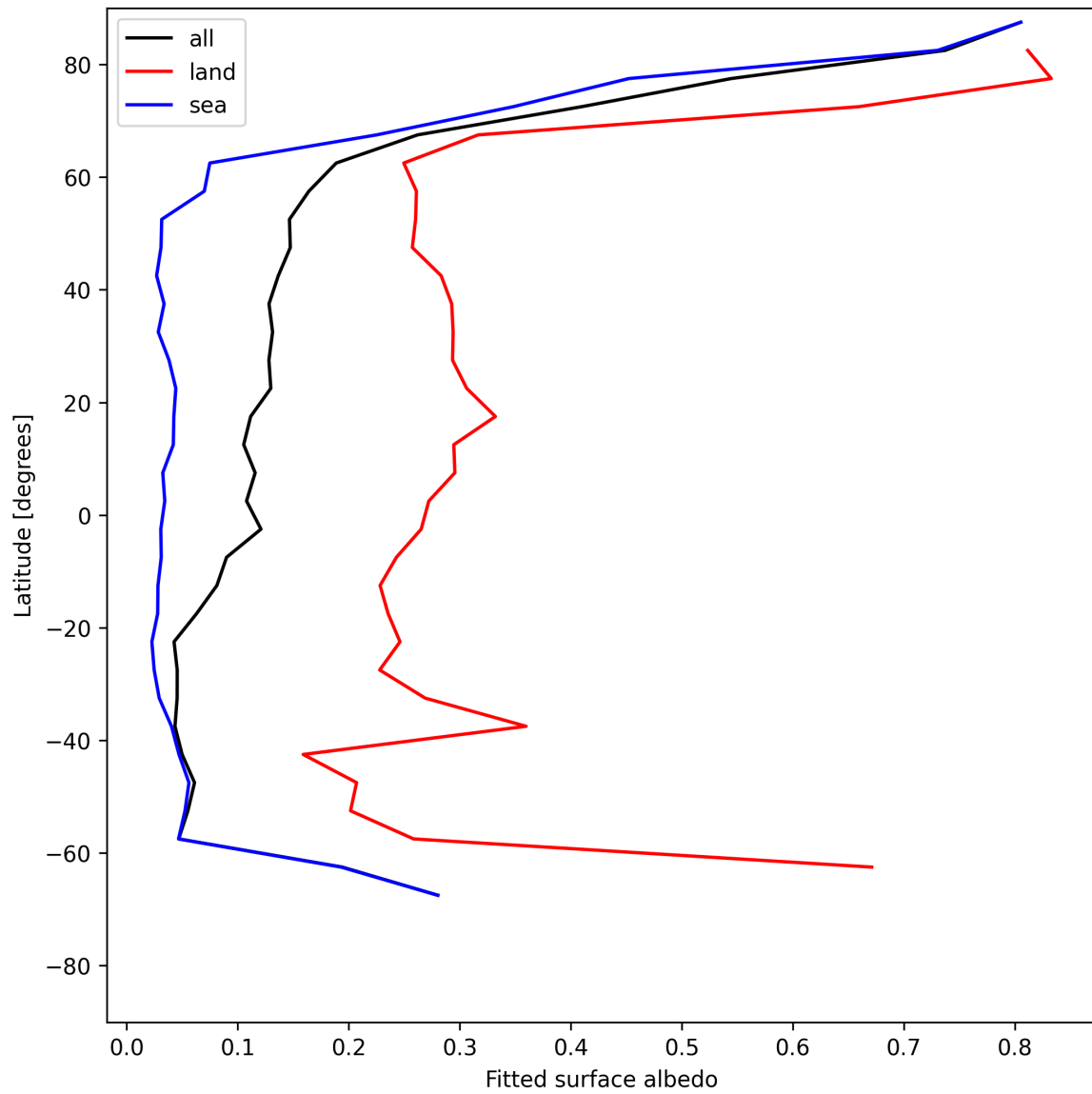
Figure 27: Zonal average of “Fitted surface albedo” for 2025-06-18 to 2025-06-19.
