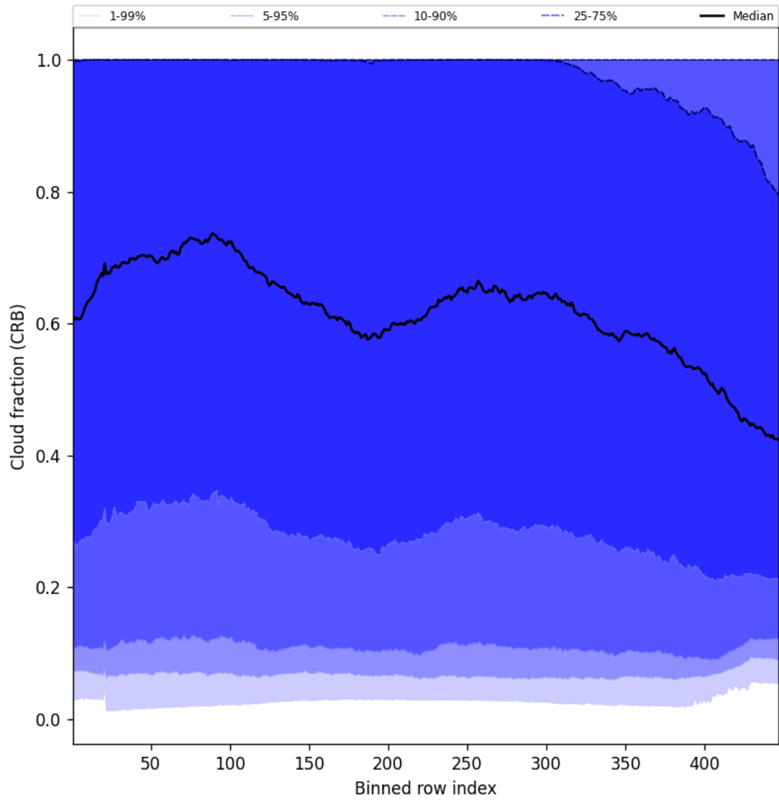
Figure 56: Along track statistics of “Cloud fraction (CRB)” for 2025-06-18 to 2025-06-19
