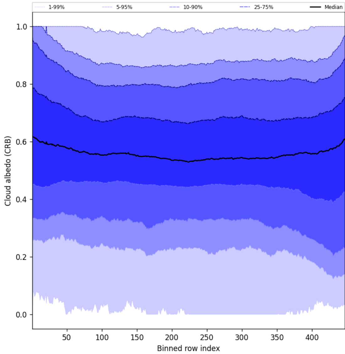
Figure 58: Along track statistics of “Cloud albedo (CRB)” for 2025-06-18 to 2025-06-19
