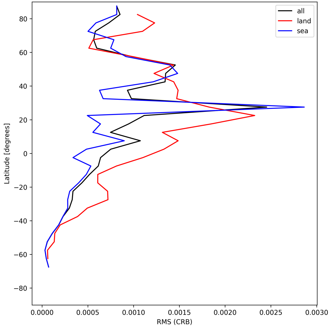
Figure 30: Zonal average of “RMS (CRB)” for 2025-06-18 to 2025-06-19.
