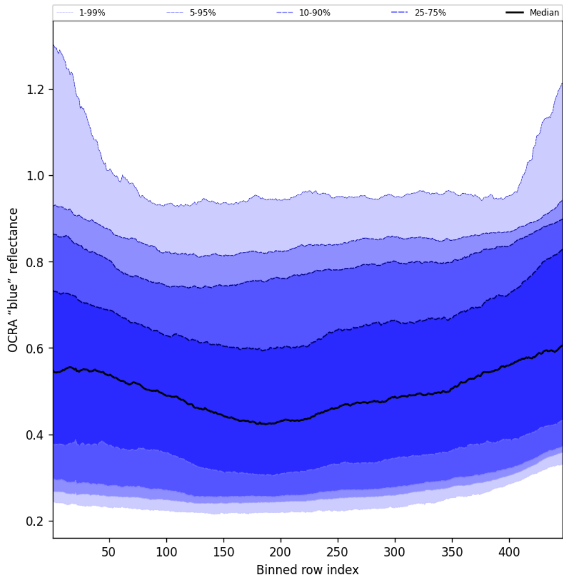
Figure 65: Along track statistics of “OCRA “blue” reflectance” for 2025-06-18 to 2025-06-19
