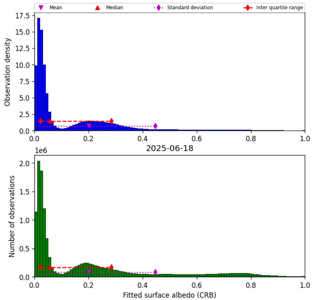
Figure 44: Histogram of “Fitted surface albedo (CRB)” for 2025-06-18 to 2025-06-19
