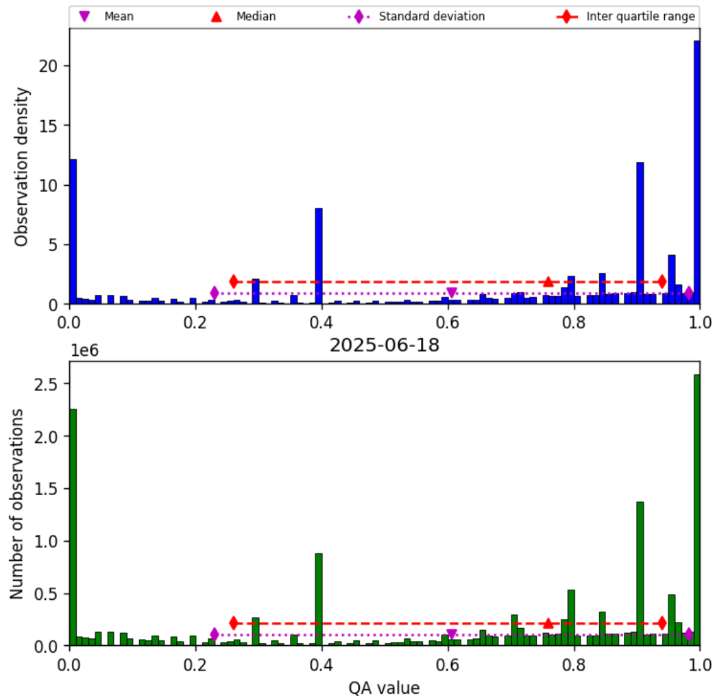
Figure 36: Histogram of “QA value” for 2025-06-18 to 2025-06-19
