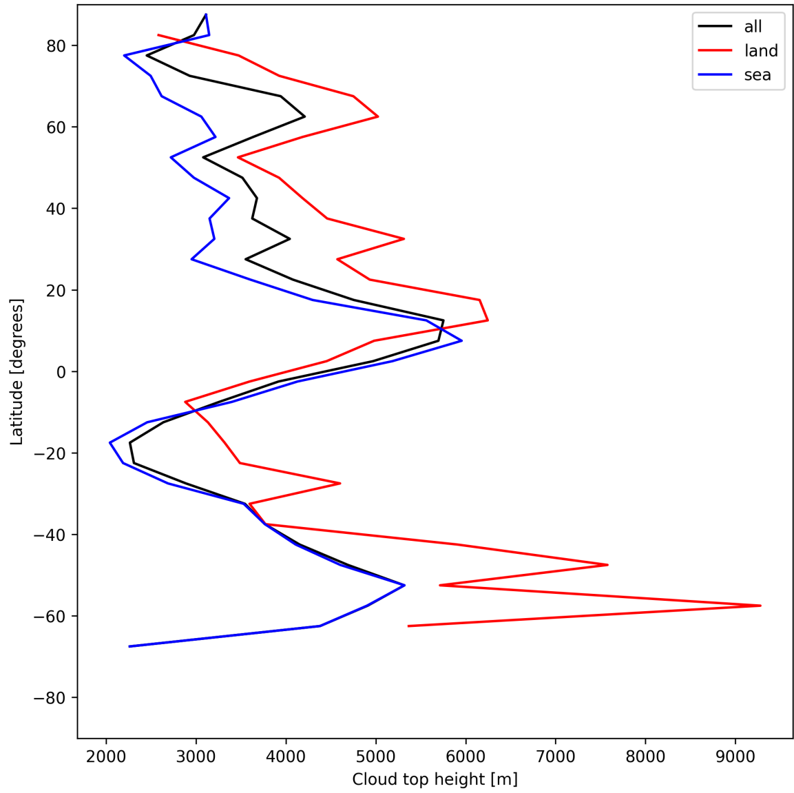
Figure 22: Zonal average of “Cloud top height” for 2025-06-18 to 2025-06-19.
