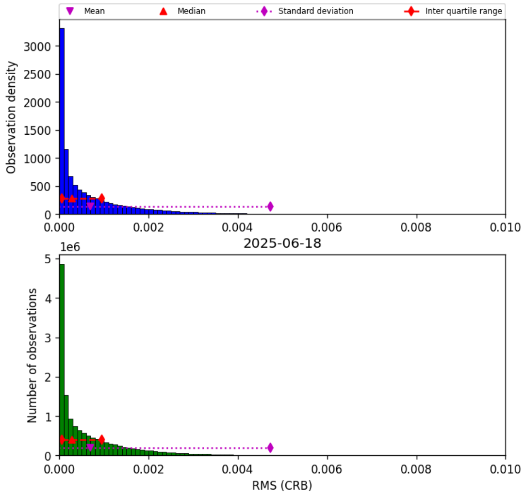
Figure 46: Histogram of “RMS (CRB)” for 2025-06-18 to 2025-06-19
