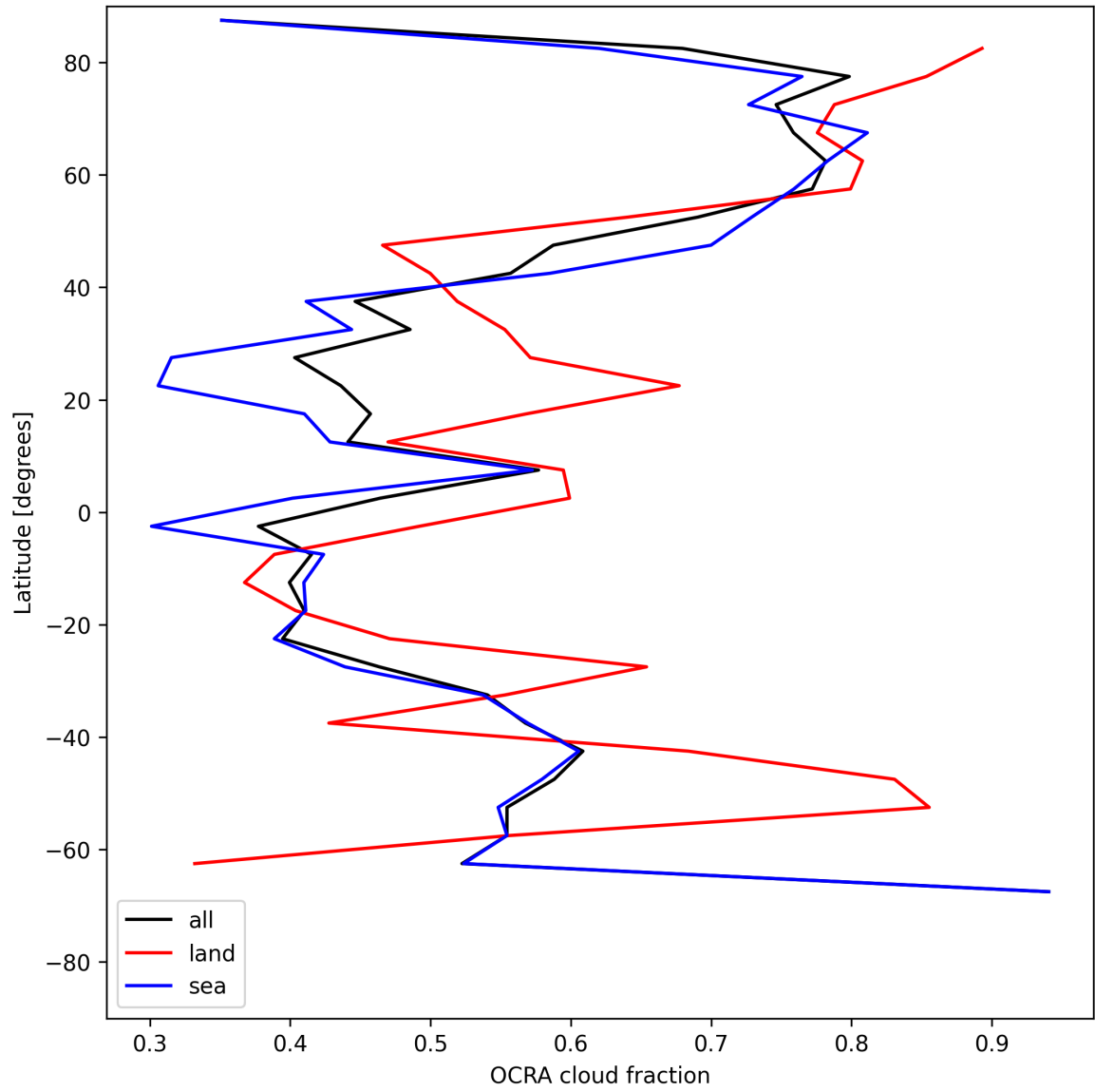
Figure 32: Zonal average of “OCRA cloud fraction” for 2025-06-18 to 2025-06-19.
