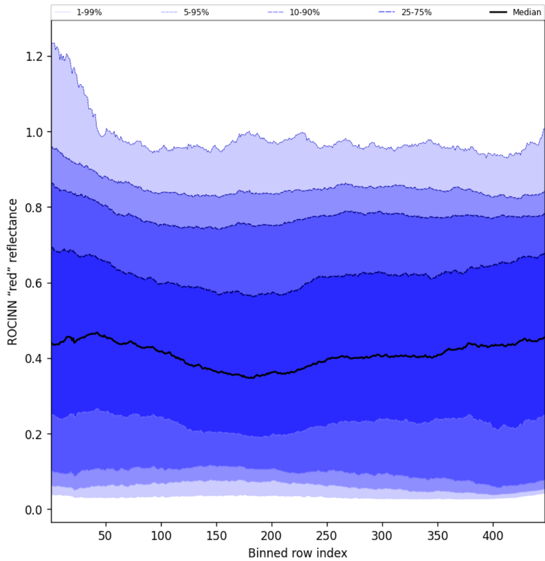
Figure 67: Along track statistics of "ROCINN "red" reflectance" for 2025-06-18 to 2025-06-19
