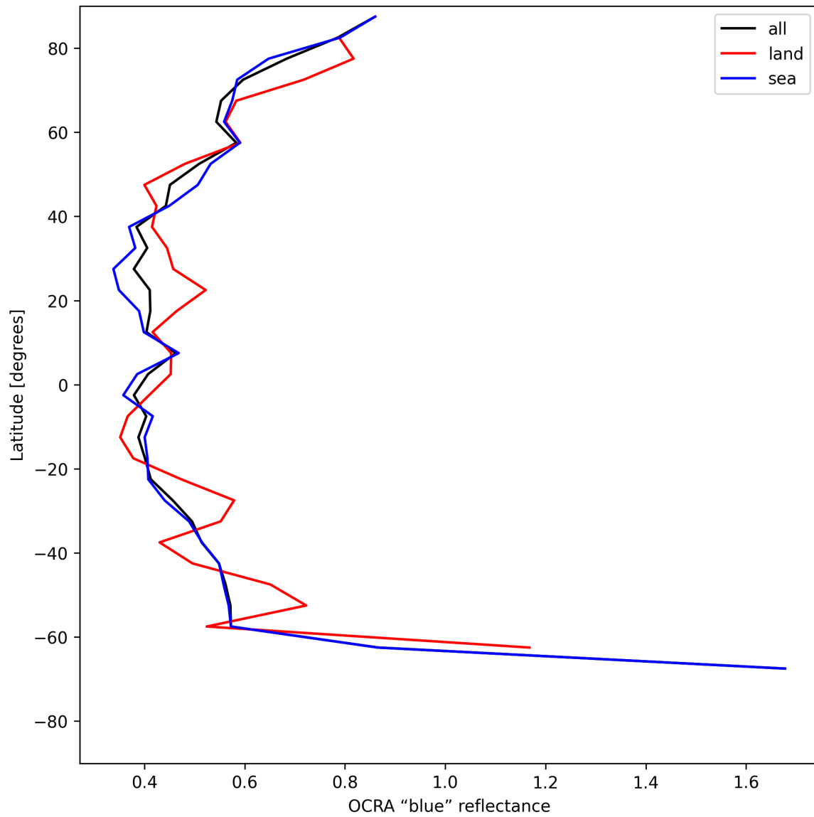
Figure 33: Zonal average of “OCRA “blue” reflectance” for 2025-06-18 to 2025-06-19.
