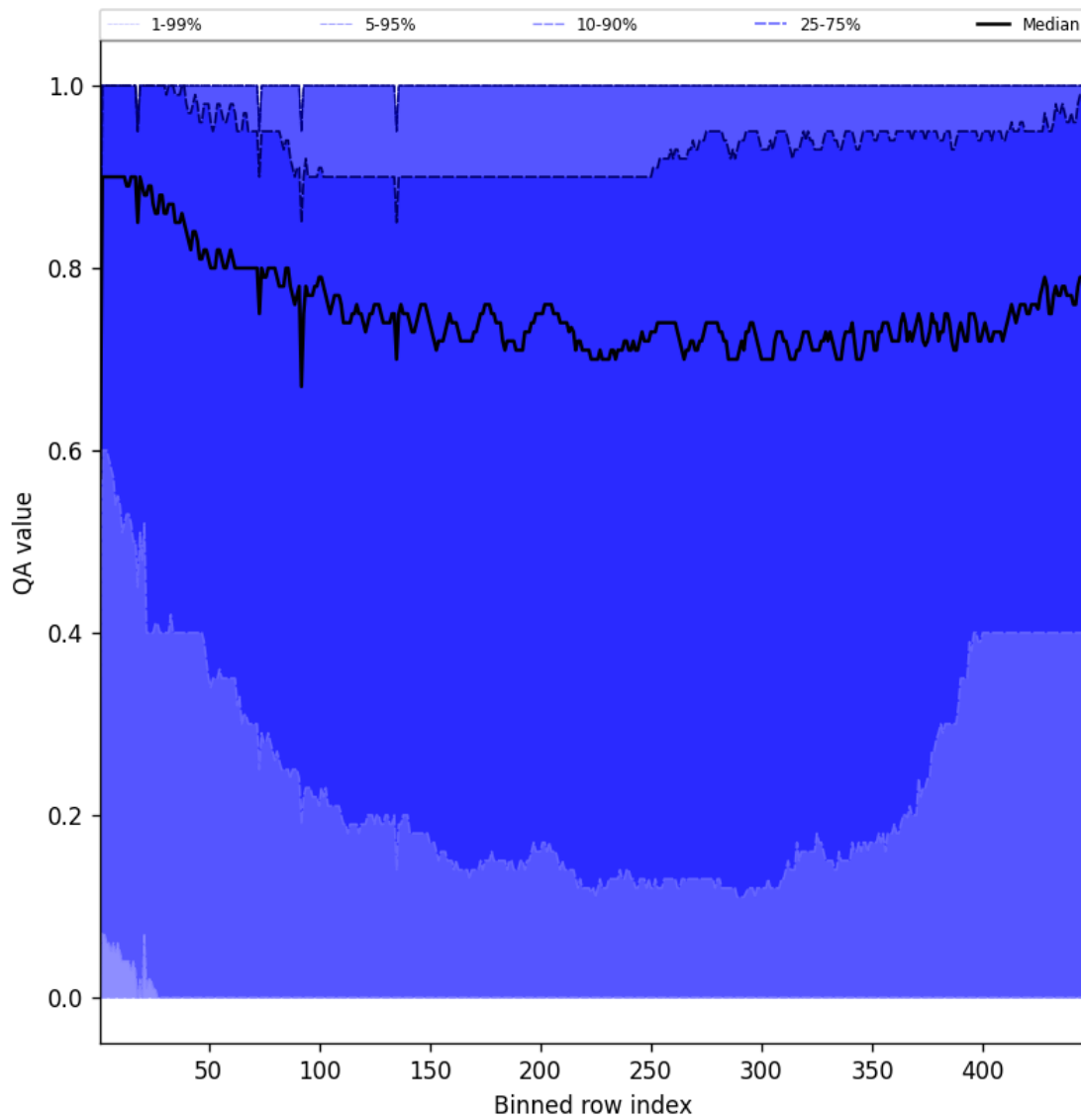
Figure 52: Along track statistics of “QA value” for 2025-06-18 to 2025-06-19
