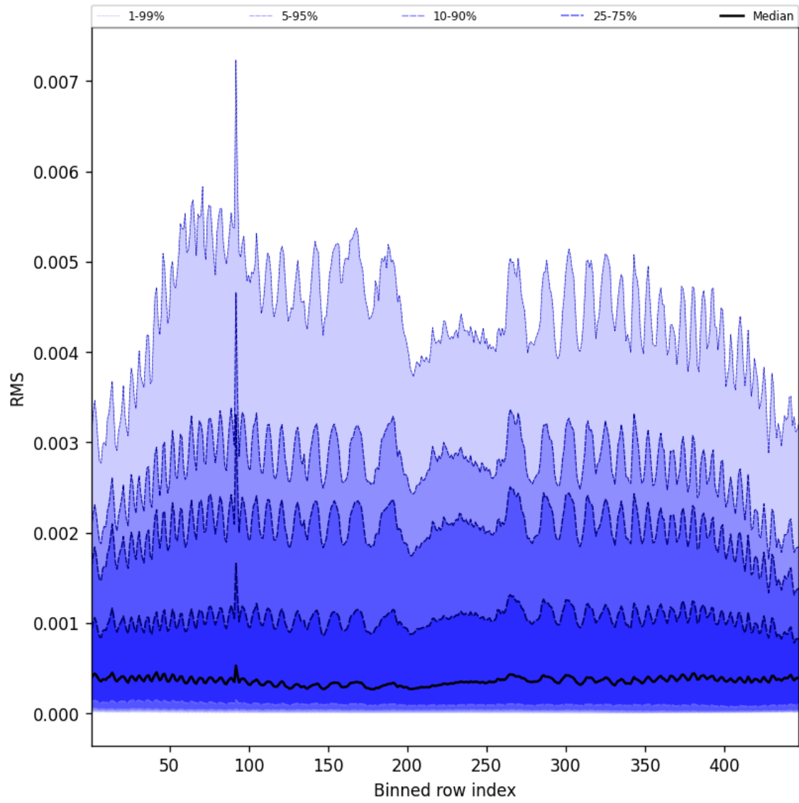
Figure 61: Along track statistics of “RMS” for 2025-06-18 to 2025-06-19
