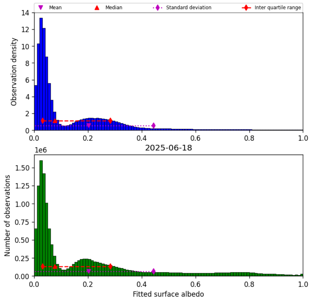
Figure 43: Histogram of “Fitted surface albedo” for 2025-06-18 to 2025-06-19
