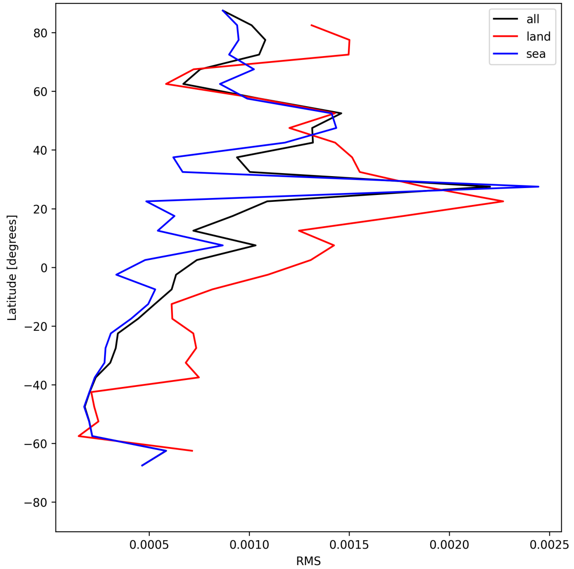
Figure 29: Zonal average of “RMS” for 2025-06-18 to 2025-06-19.
