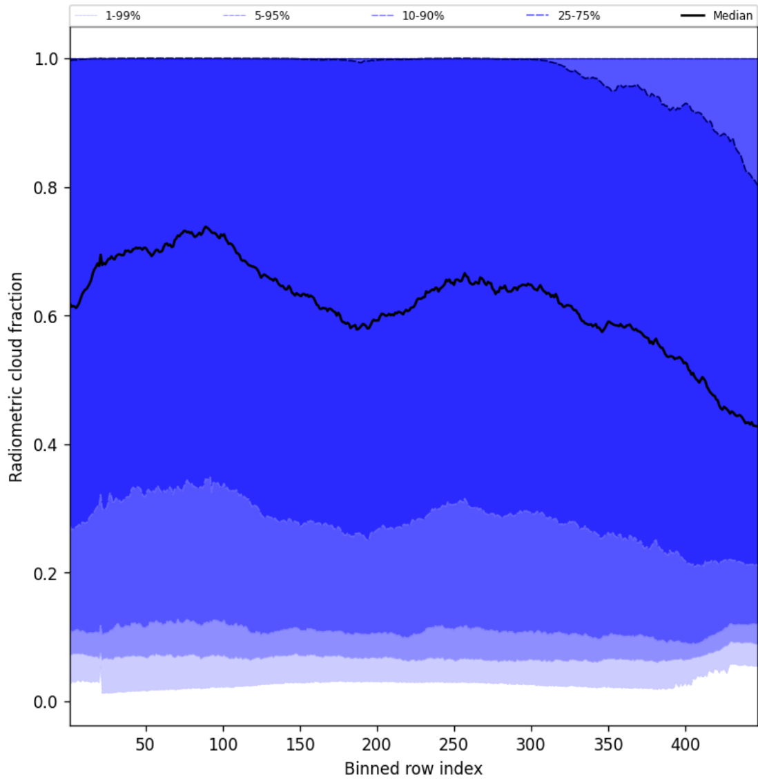
Figure 53: Along track statistics of “Radiometric cloud fraction” for 2025-06-18 to 2025-06-19
