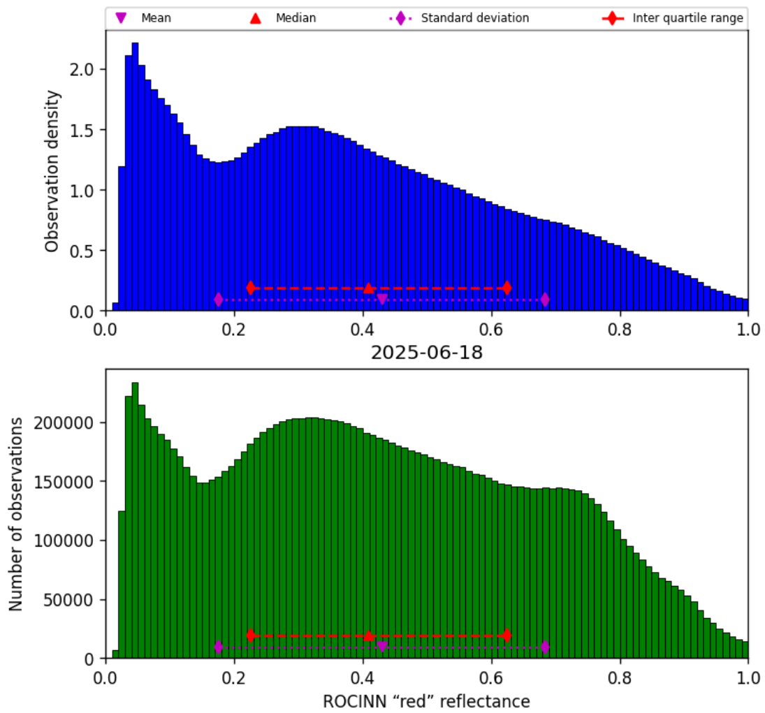
Figure 51: Histogram of “ROCINN “red” reflectance” for 2025-06-18 to 2025-06-19
