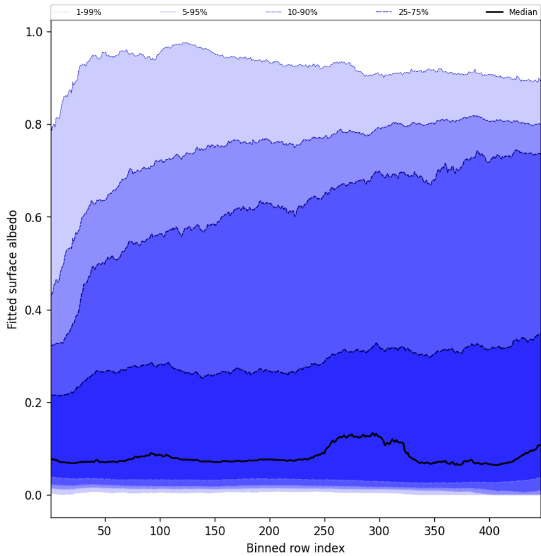
Figure 59: Along track statistics of “Fitted surface albedo” for 2025-06-18 to 2025-06-19
