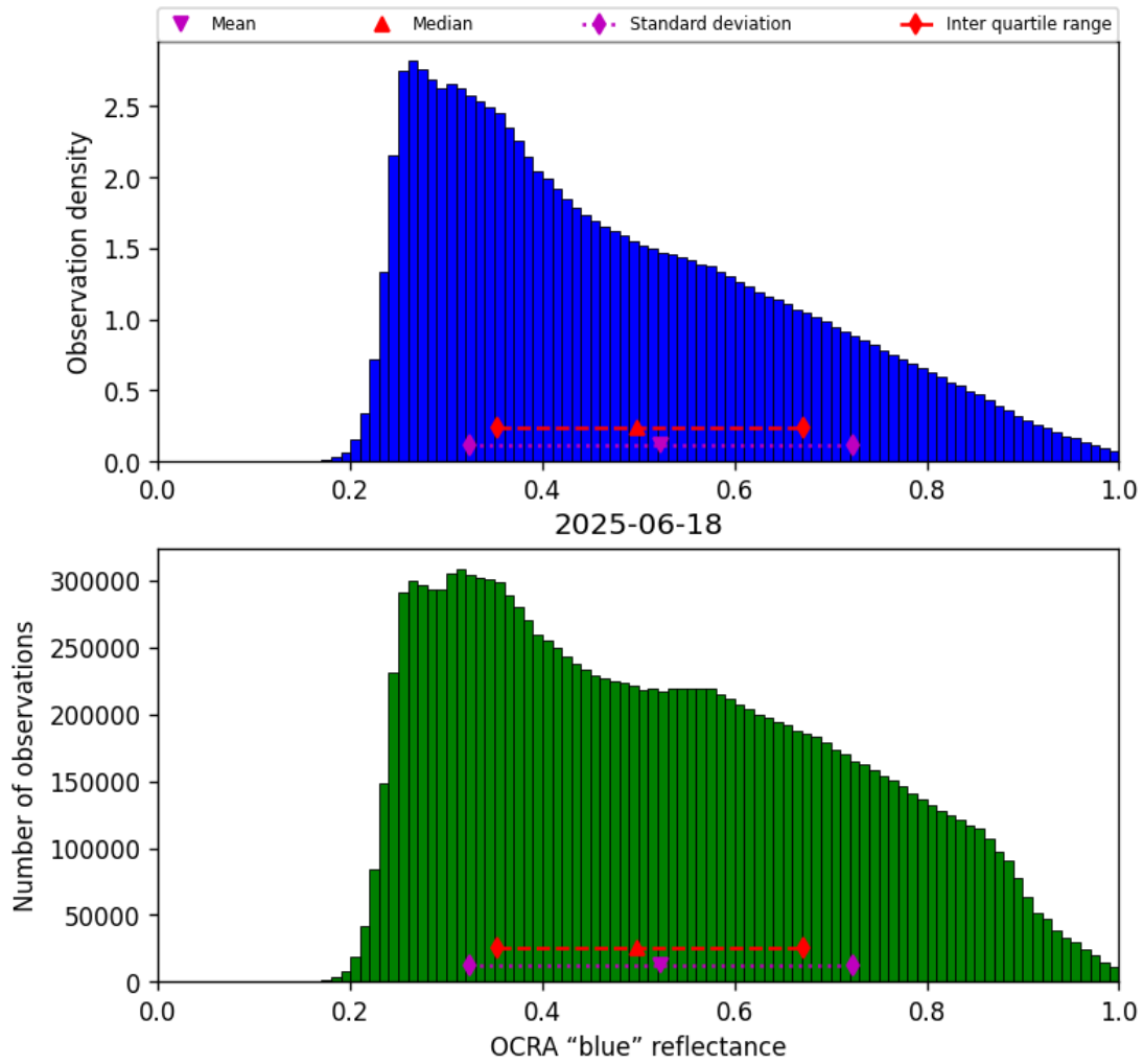
Figure 49: Histogram of “OCRA “blue” reflectance” for 2025-06-18 to 2025-06-19
