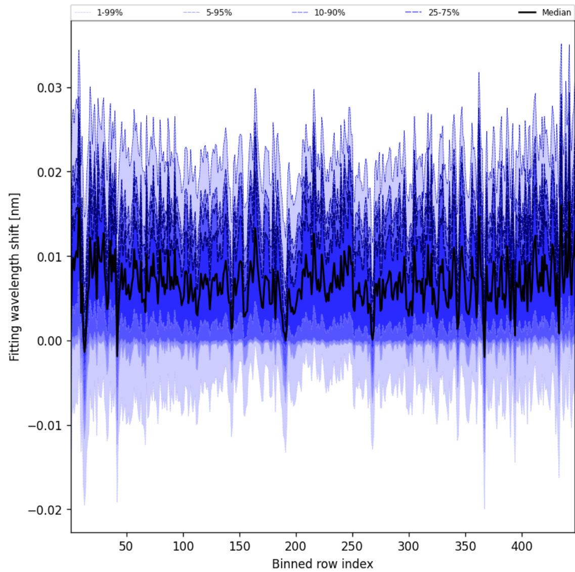
Figure 63: Along track statistics of “Fitting wavelength shift” for 2025-06-18 to 2025-06-19
