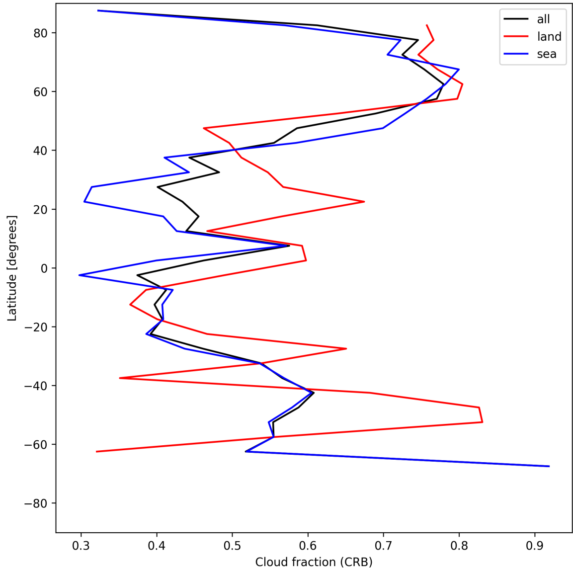
Figure 24: Zonal average of “Cloud fraction (CRB)” for 2025-06-18 to 2025-06-19.
