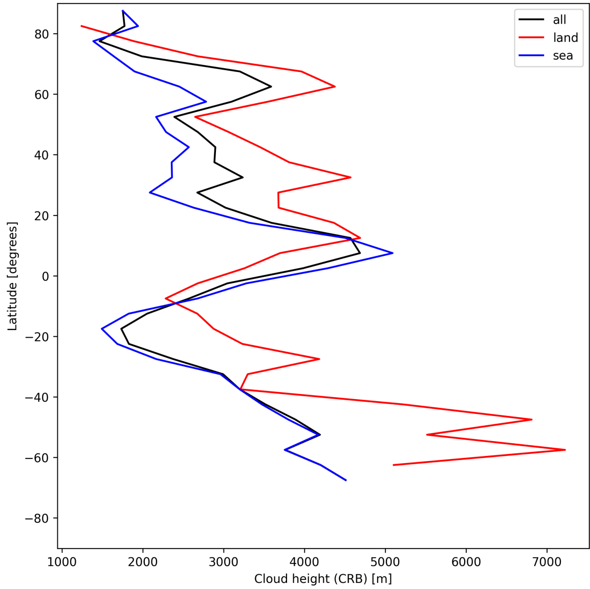
Figure 25: Zonal average of “Cloud height (CRB)” for 2025-06-18 to 2025-06-19.
