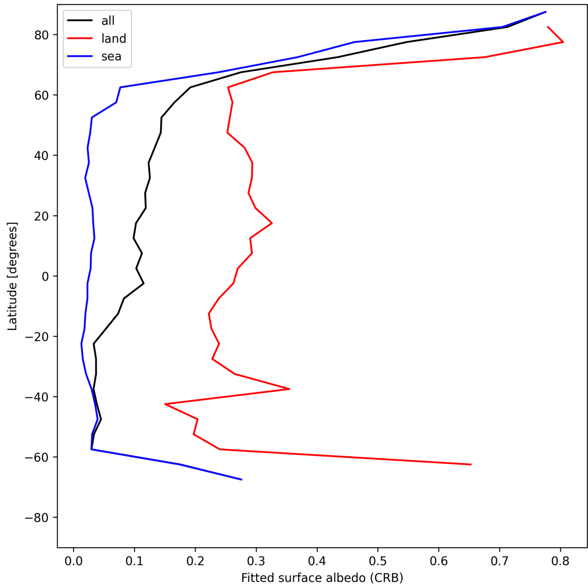
Figure 28: Zonal average of “Fitted surface albedo (CRB)” for 2025-06-18 to 2025-06-19.
