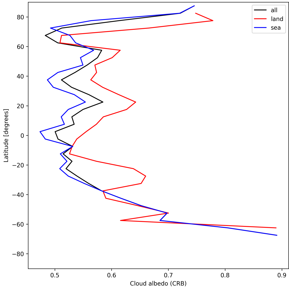
Figure 26: Zonal average of “Cloud albedo (CRB)” for 2025-06-18 to 2025-06-19.
