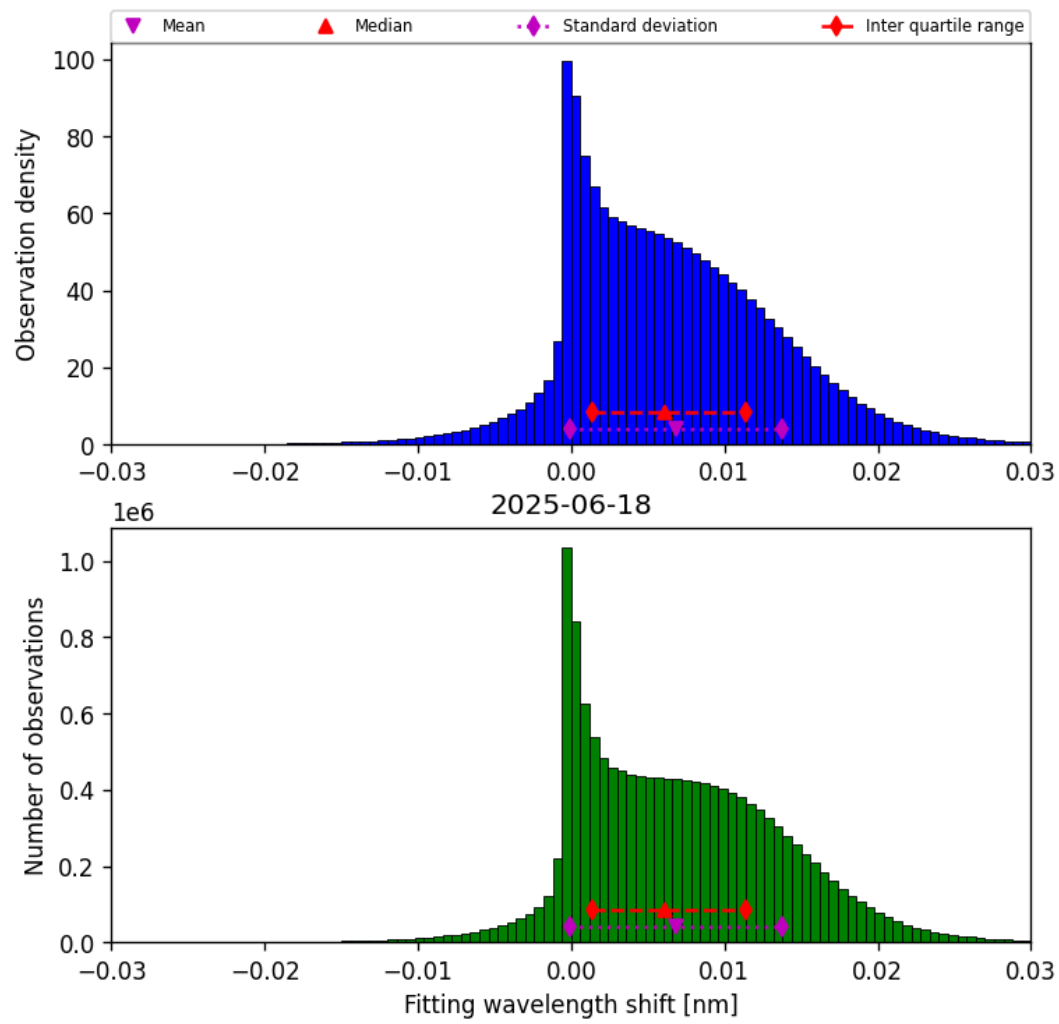
Figure 47: Histogram of “Fitting wavelength shift” for 2025-06-18 to 2025-06-19
