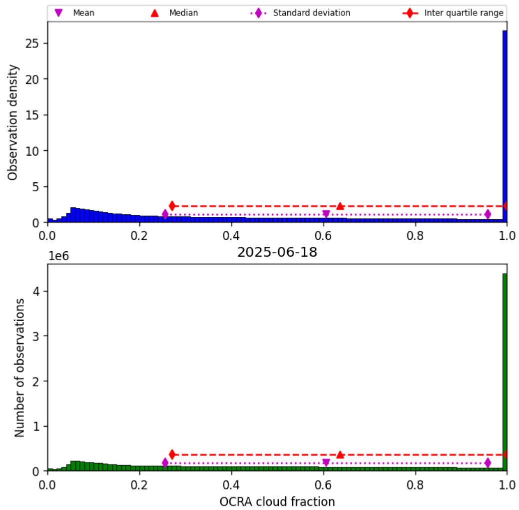
Figure 48: Histogram of “OCRA cloud fraction” for 2025-06-18 to 2025-06-19
