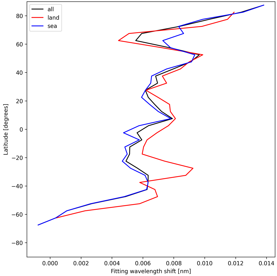
Figure 31: Zonal average of “Fitting wavelength shift” for 2025-06-18 to 2025-06-19.
