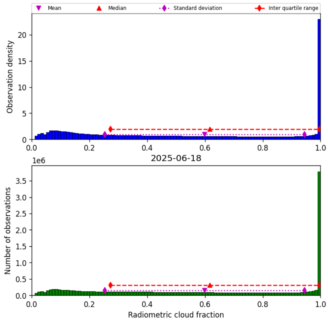
Figure 37: Histogram of “Radiometric cloud fraction” for 2025-06-18 to 2025-06-19
