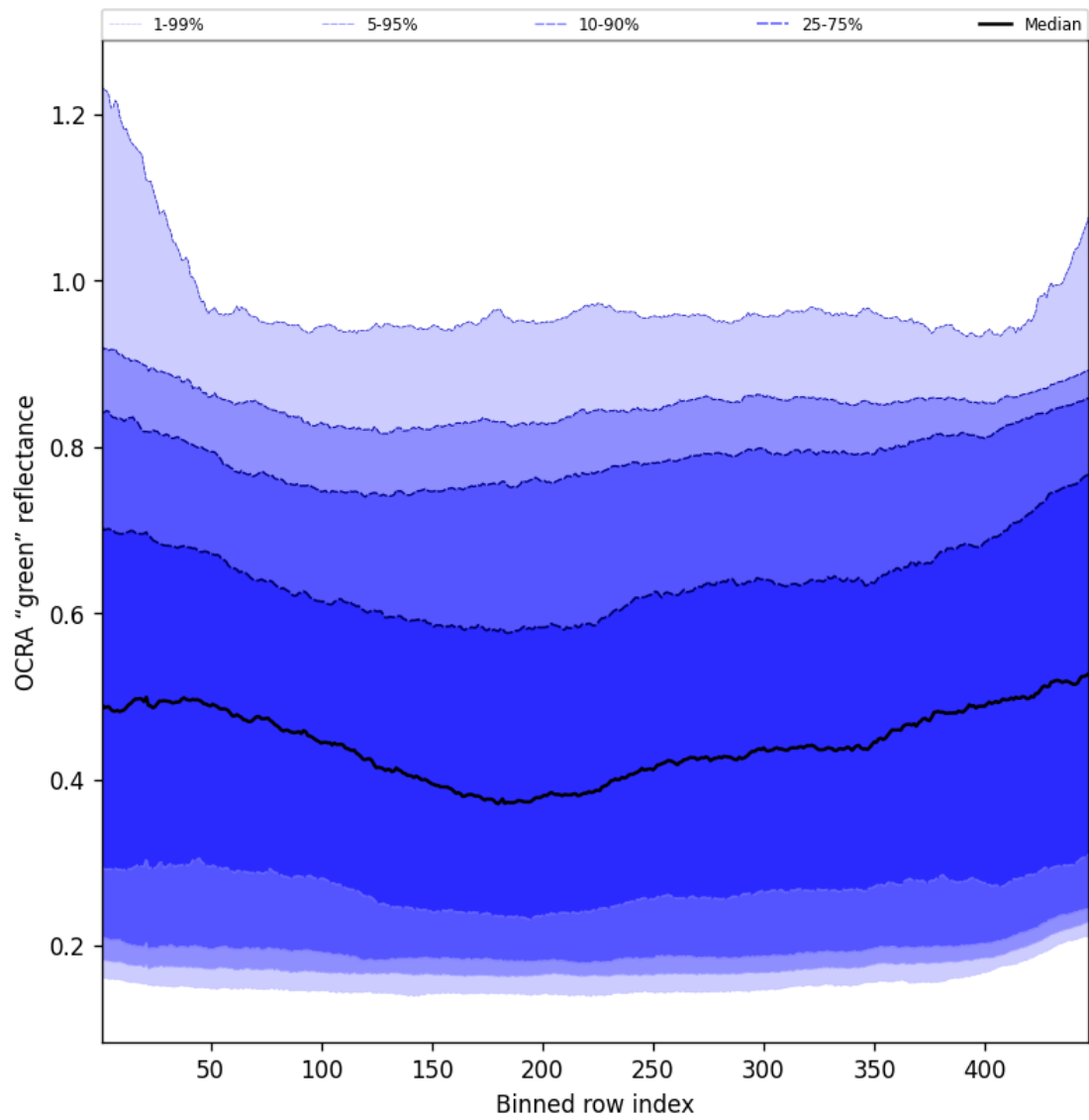
Figure 66: Along track statistics of “OCRA “green” reflectance” for 2025-06-18 to 2025-06-19
