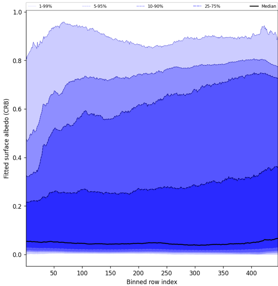
Figure 60: Along track statistics of “Fitted surface albedo (CRB)” for 2025-06-19 to 2025-06-20
