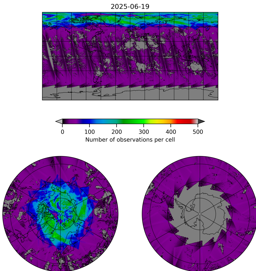
Figure 19: Map of the number of observations for 2025-06-19 to 2025-06-20
