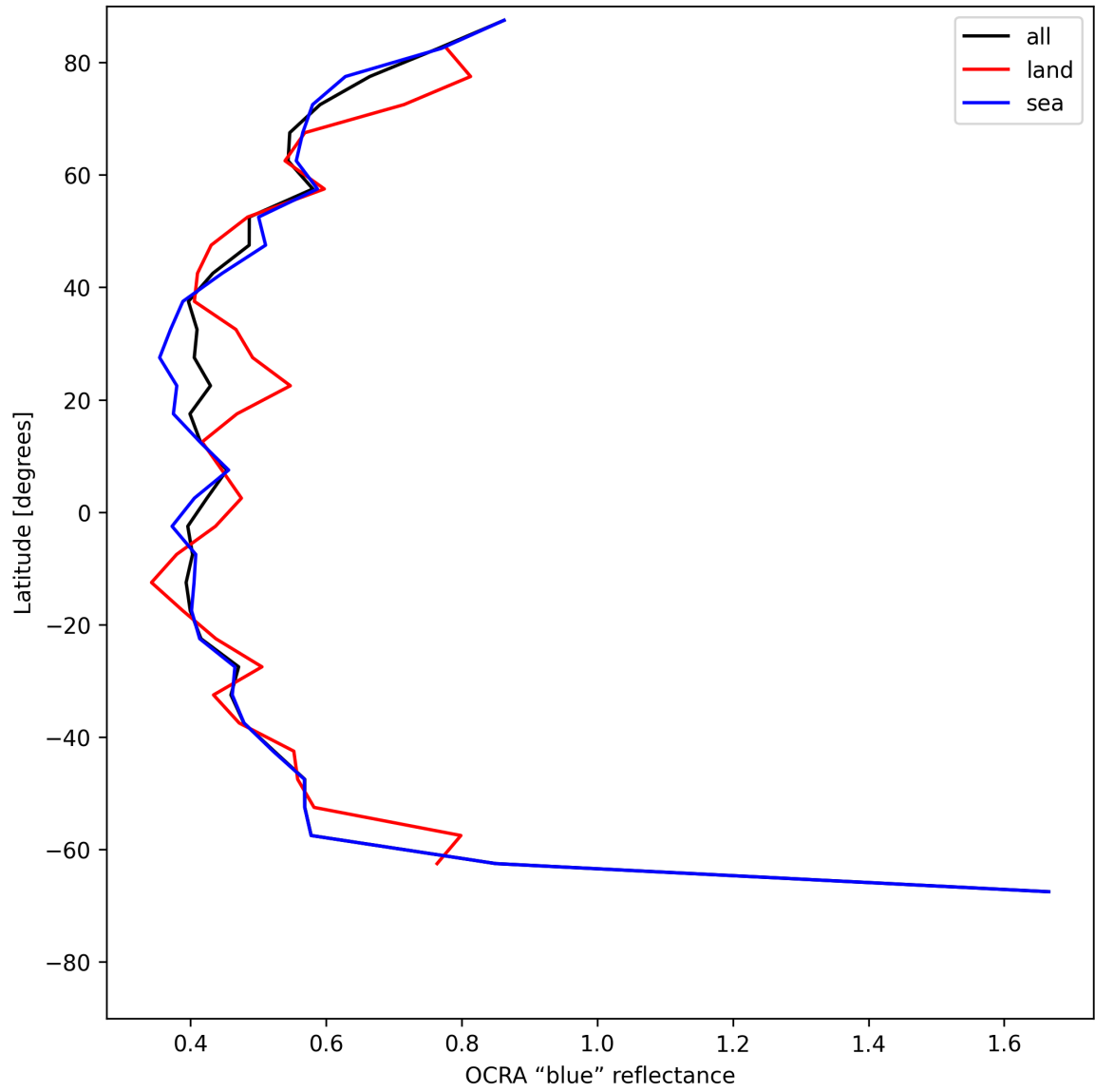
Figure 33: Zonal average of “OCRA “blue” reflectance” for 2025-06-19 to 2025-06-20.
