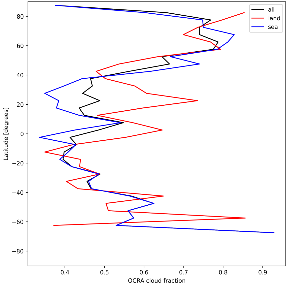
Figure 32: Zonal average of “OCRA cloud fraction” for 2025-06-19 to 2025-06-20.
