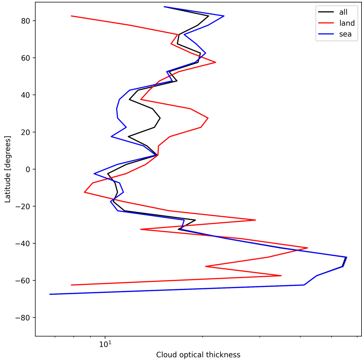
Figure 23: Zonal average of “Cloud optical thickness” for 2025-06-19 to 2025-06-20.
