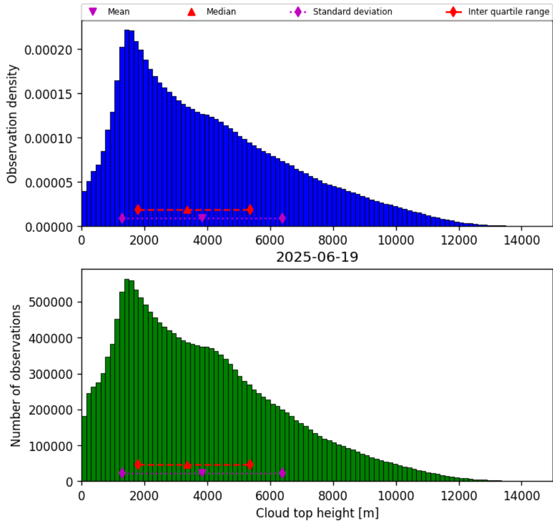
Figure 38: Histogram of “Cloud top height” for 2025-06-19 to 2025-06-20
