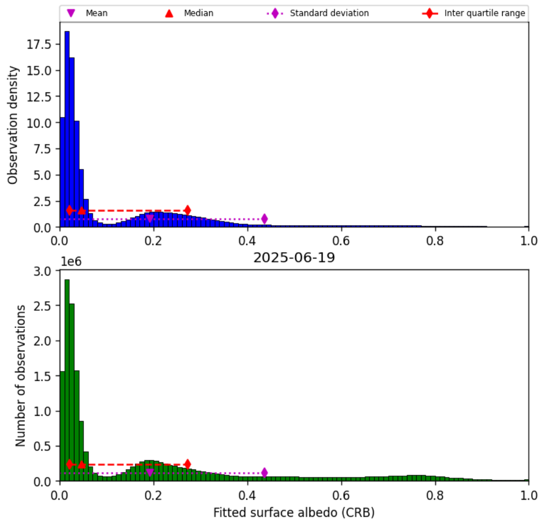
Figure 44: Histogram of “Fitted surface albedo (CRB)” for 2025-06-19 to 2025-06-20
