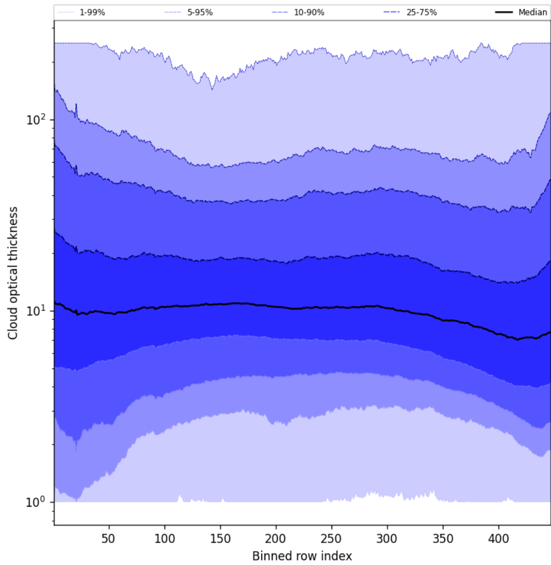
Figure 55: Along track statistics of “Cloud optical thickness” for 2025-06-19 to 2025-06-20
