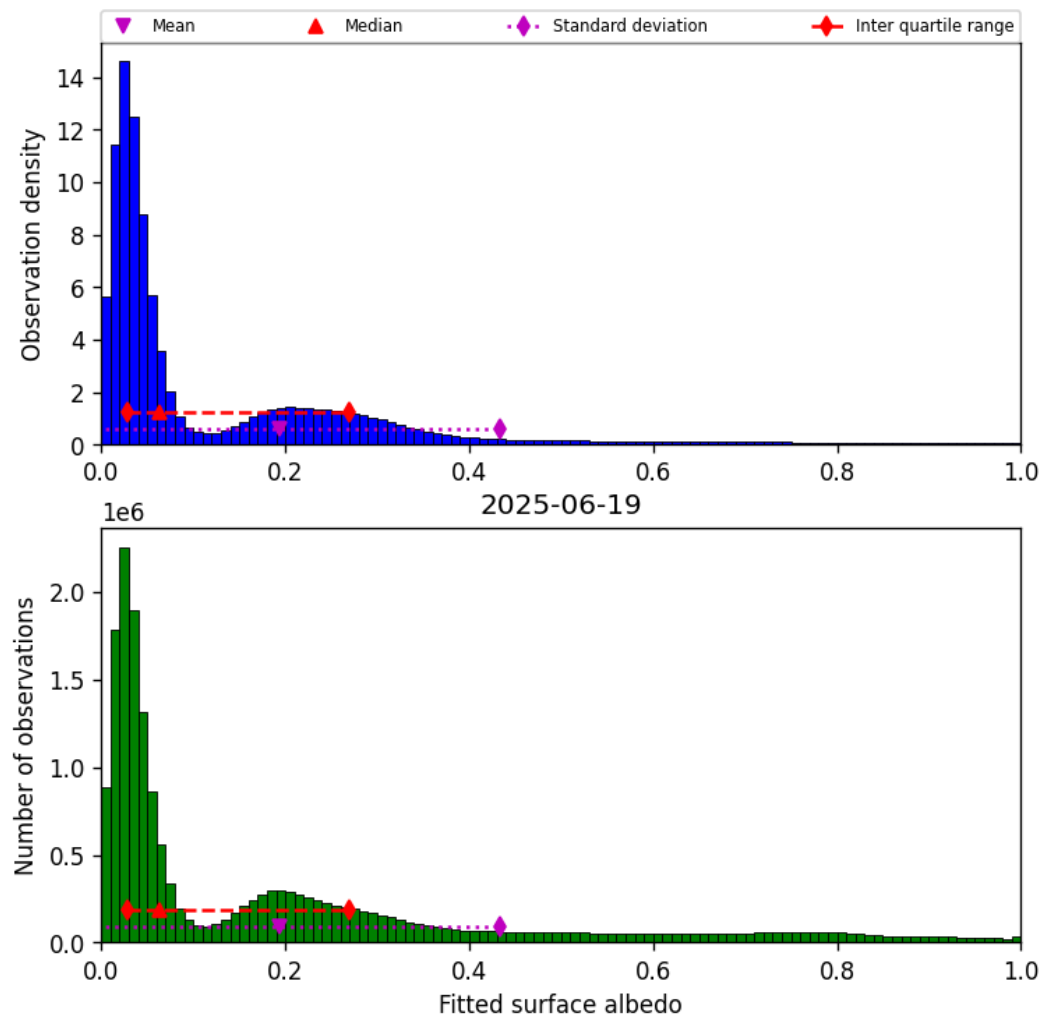
Figure 43: Histogram of “Fitted surface albedo” for 2025-06-19 to 2025-06-20
