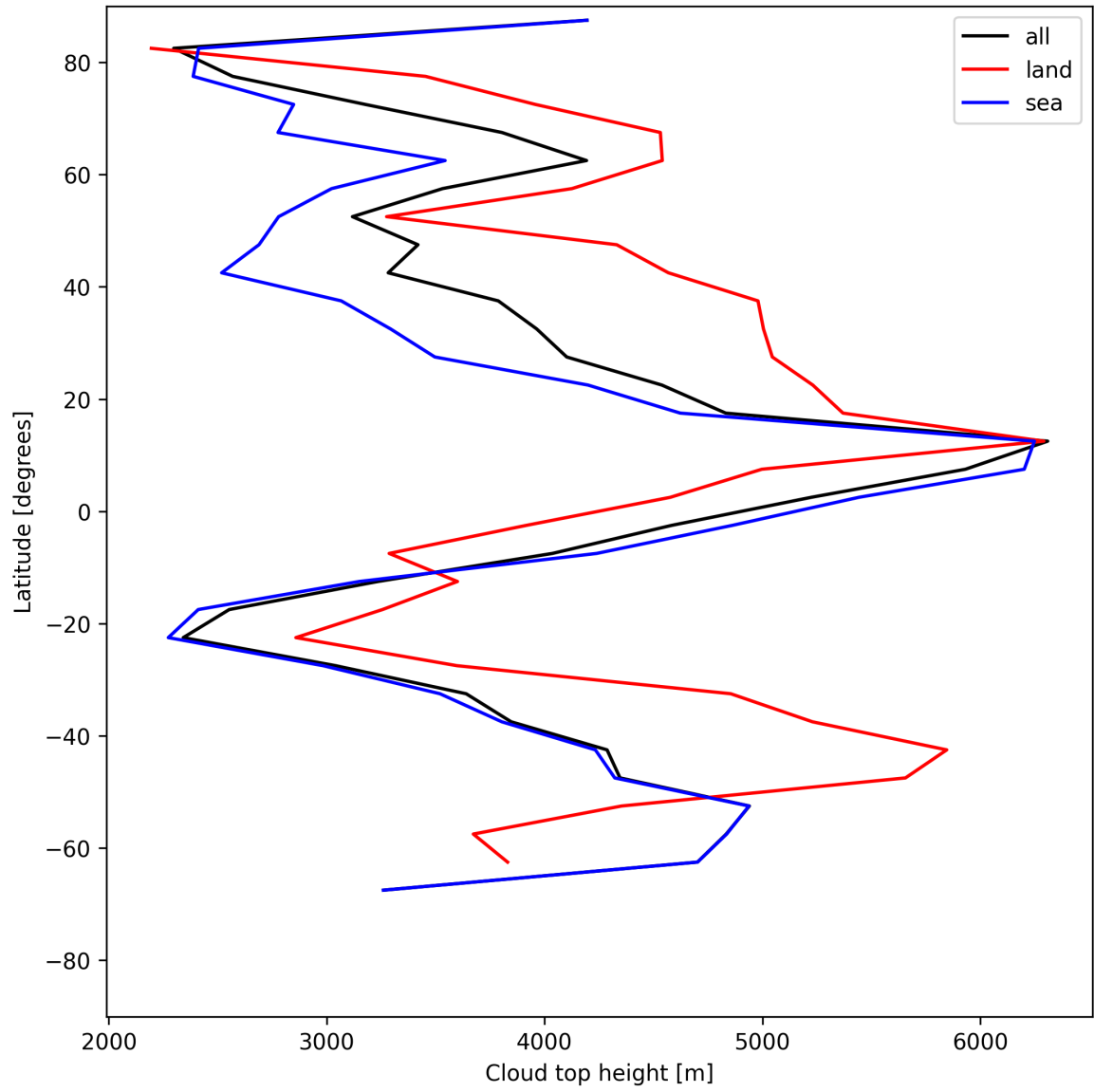
Figure 22: Zonal average of “Cloud top height” for 2025-06-19 to 2025-06-20.
