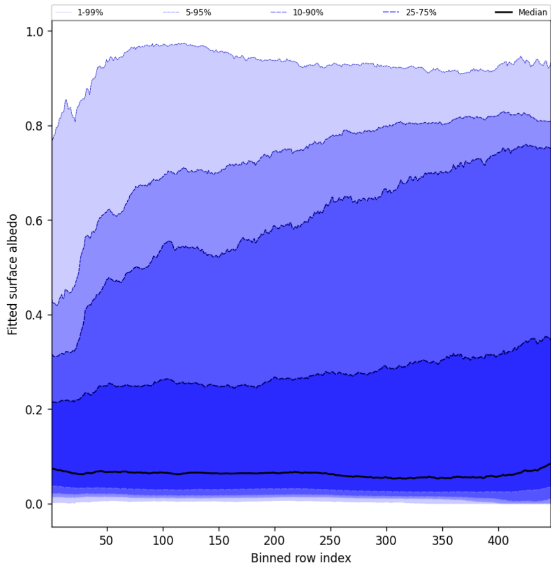
Figure 59: Along track statistics of “Fitted surface albedo” for 2025-06-19 to 2025-06-20
