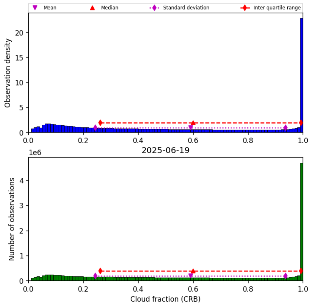
Figure 40: Histogram of “Cloud fraction (CRB)” for 2025-06-19 to 2025-06-20
