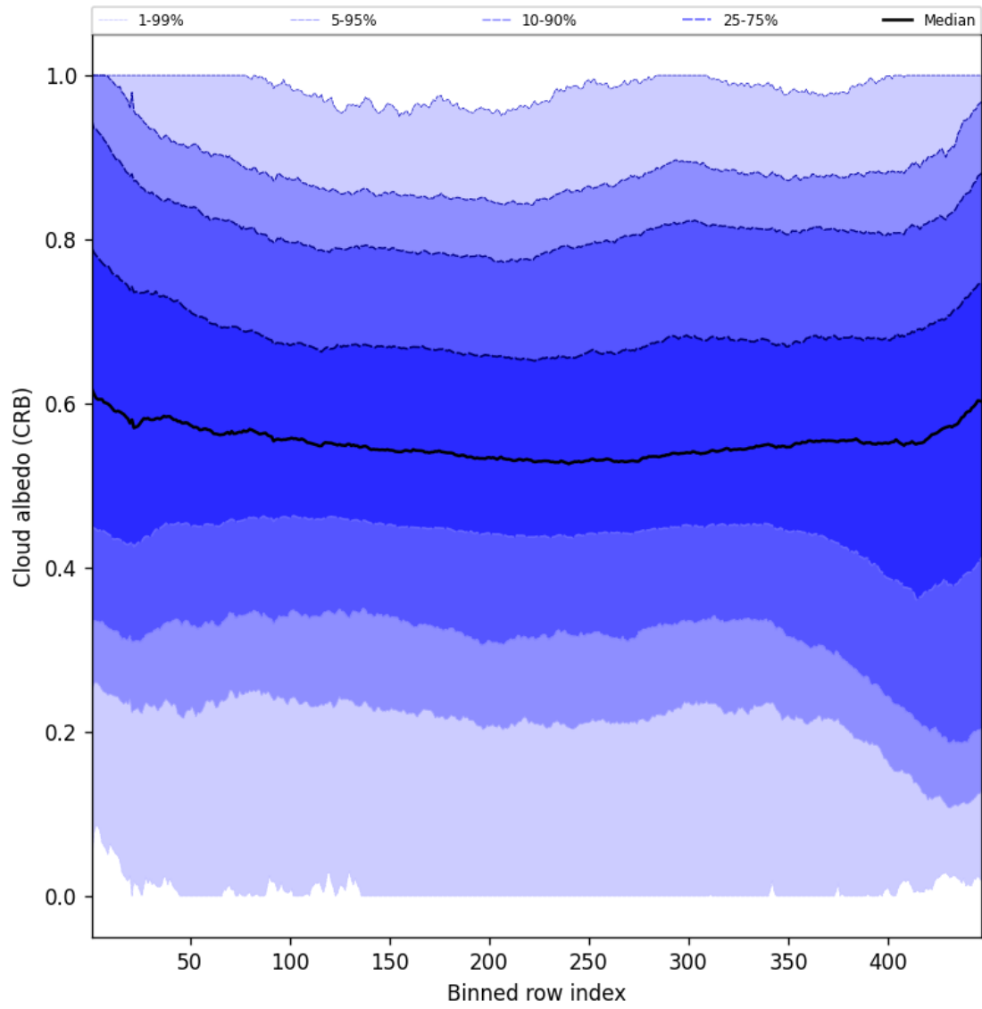
Figure 58: Along track statistics of “Cloud albedo (CRB)” for 2025-06-19 to 2025-06-20
