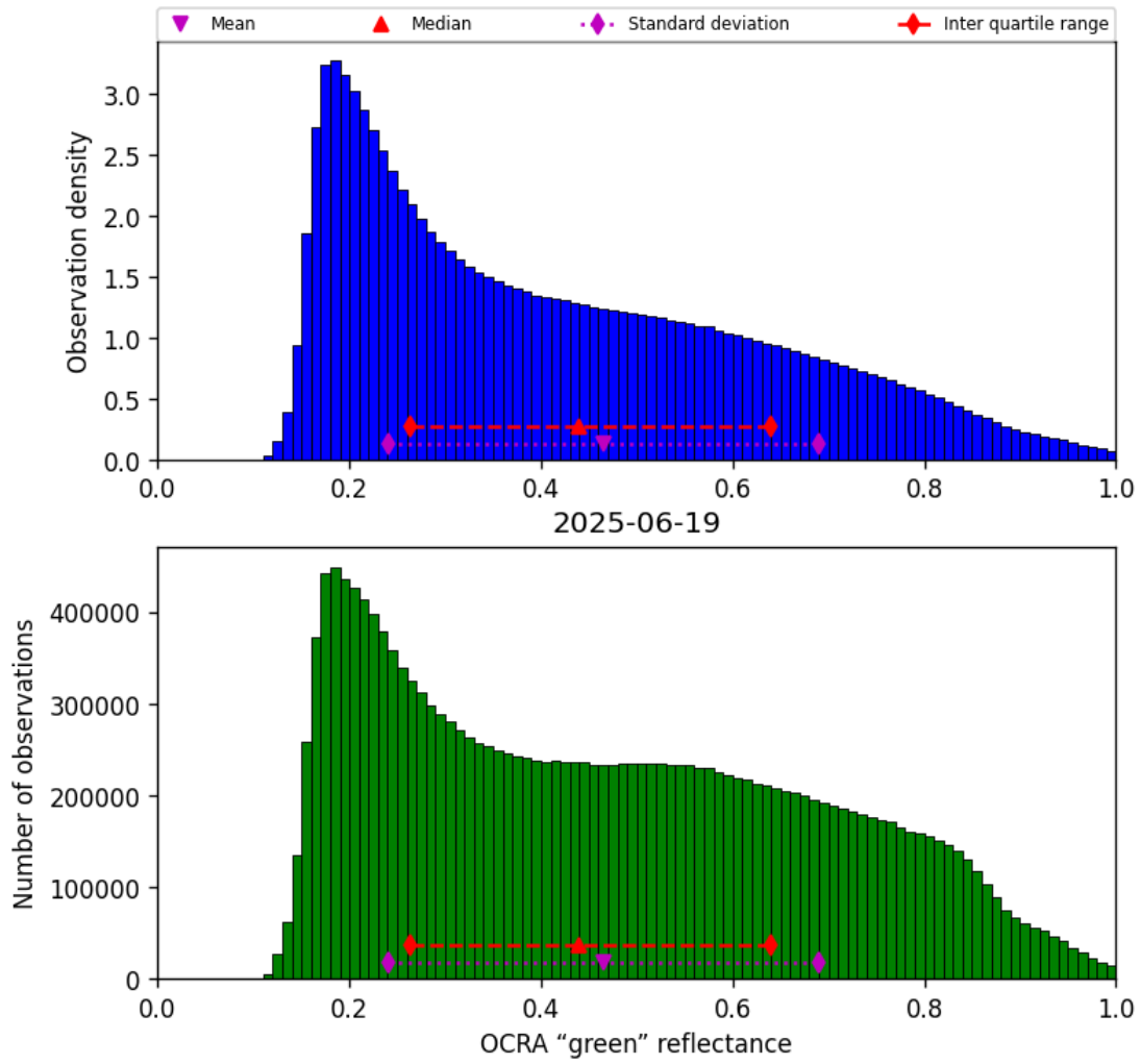
Figure 50: Histogram of “OCRA “green” reflectance” for 2025-06-19 to 2025-06-20
