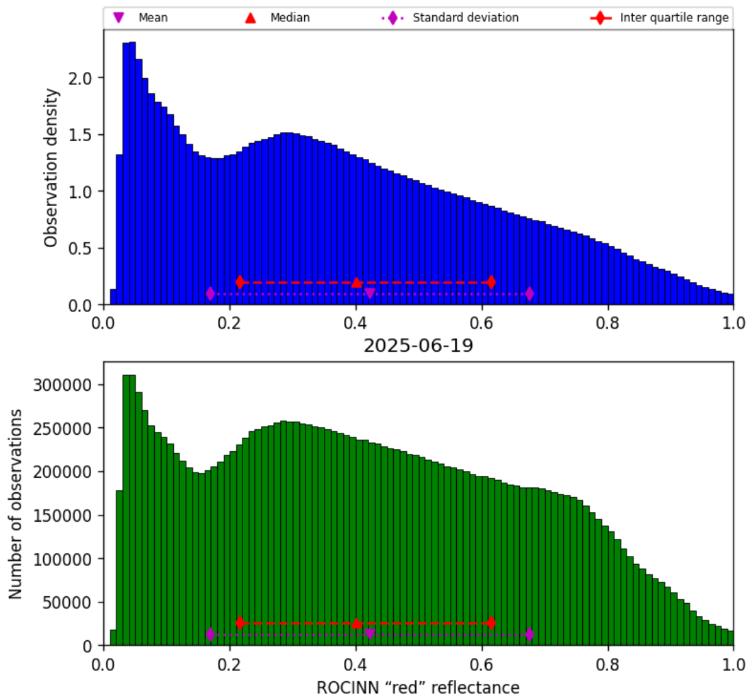
Figure 51: Histogram of “ROCINN “red” reflectance” for 2025-06-19 to 2025-06-20
