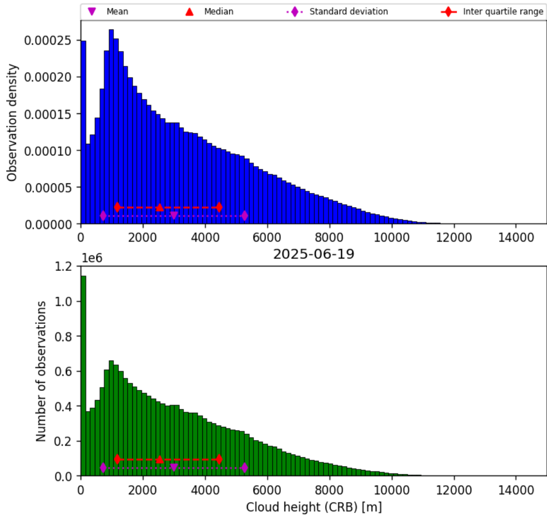
Figure 41: Histogram of “Cloud height (CRB)” for 2025-06-19 to 2025-06-20
