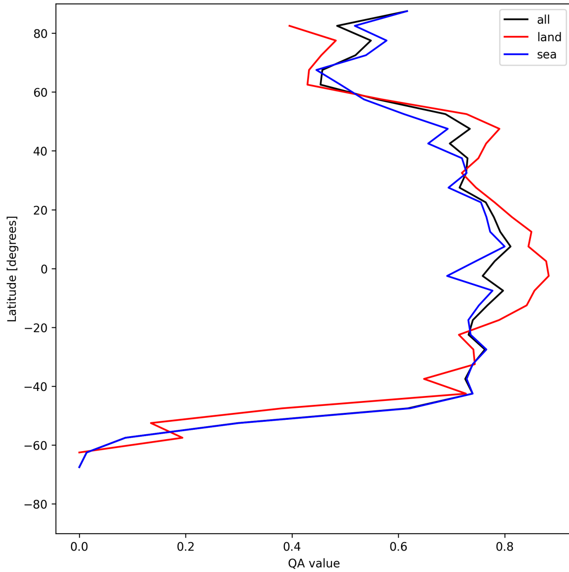
Figure 20: Zonal average of “QA value” for 2025-06-19 to 2025-06-20.
