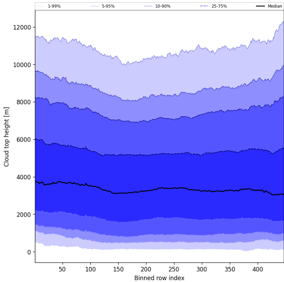
Figure 54: Along track statistics of “Cloud top height” for 2025-06-19 to 2025-06-20
