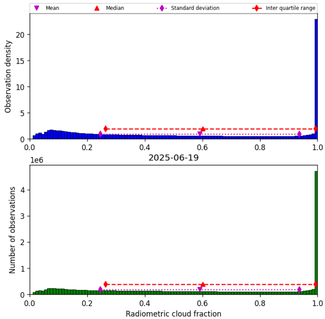
Figure 37: Histogram of “Radiometric cloud fraction” for 2025-06-19 to 2025-06-20
