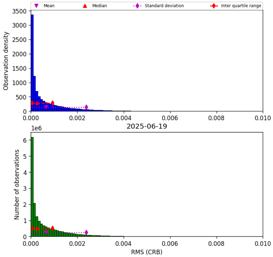
Figure 46: Histogram of “RMS (CRB)” for 2025-06-19 to 2025-06-20
