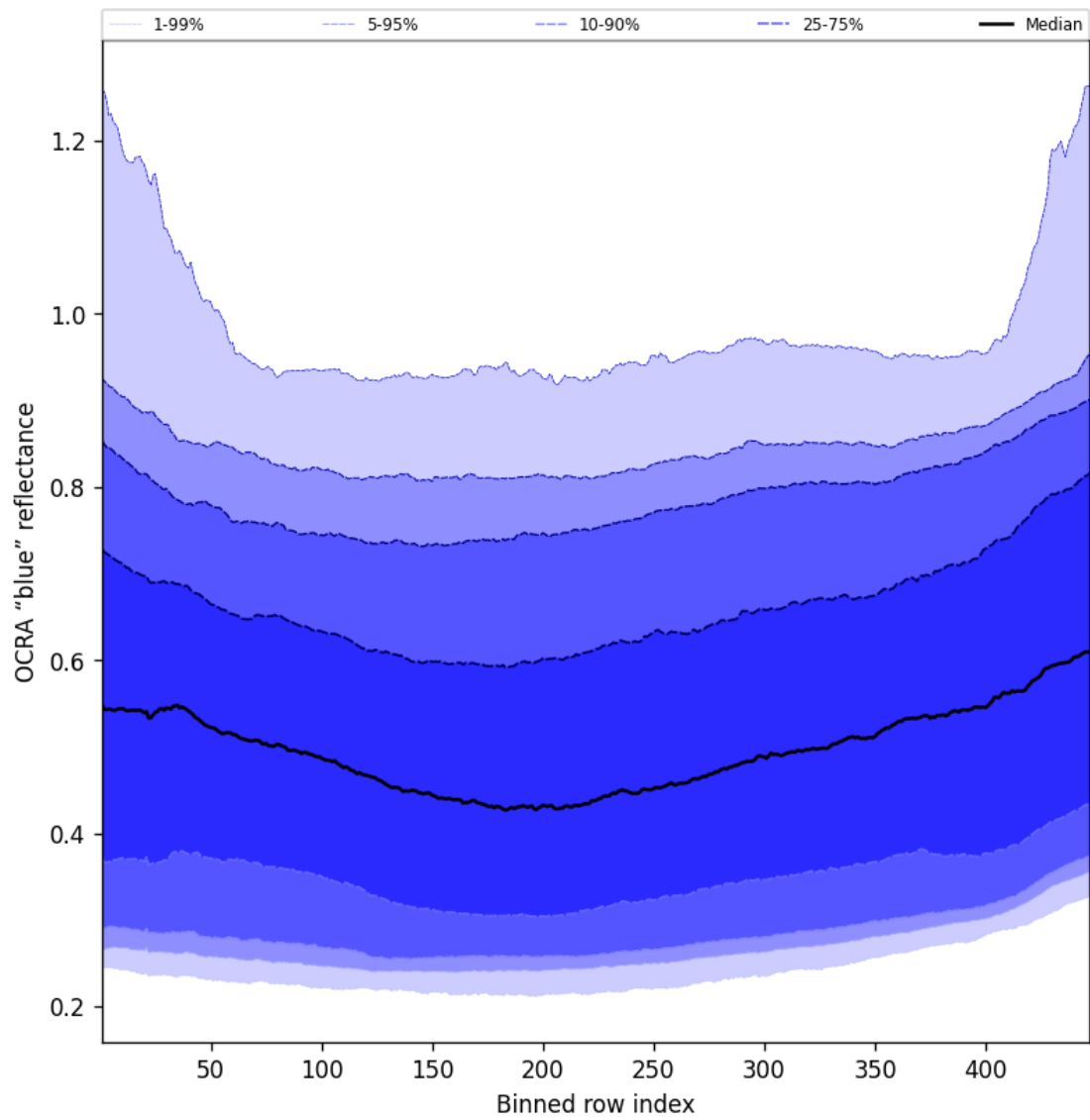
Figure 65: Along track statistics of “OCRA “blue” reflectance” for 2025-06-19 to 2025-06-20
