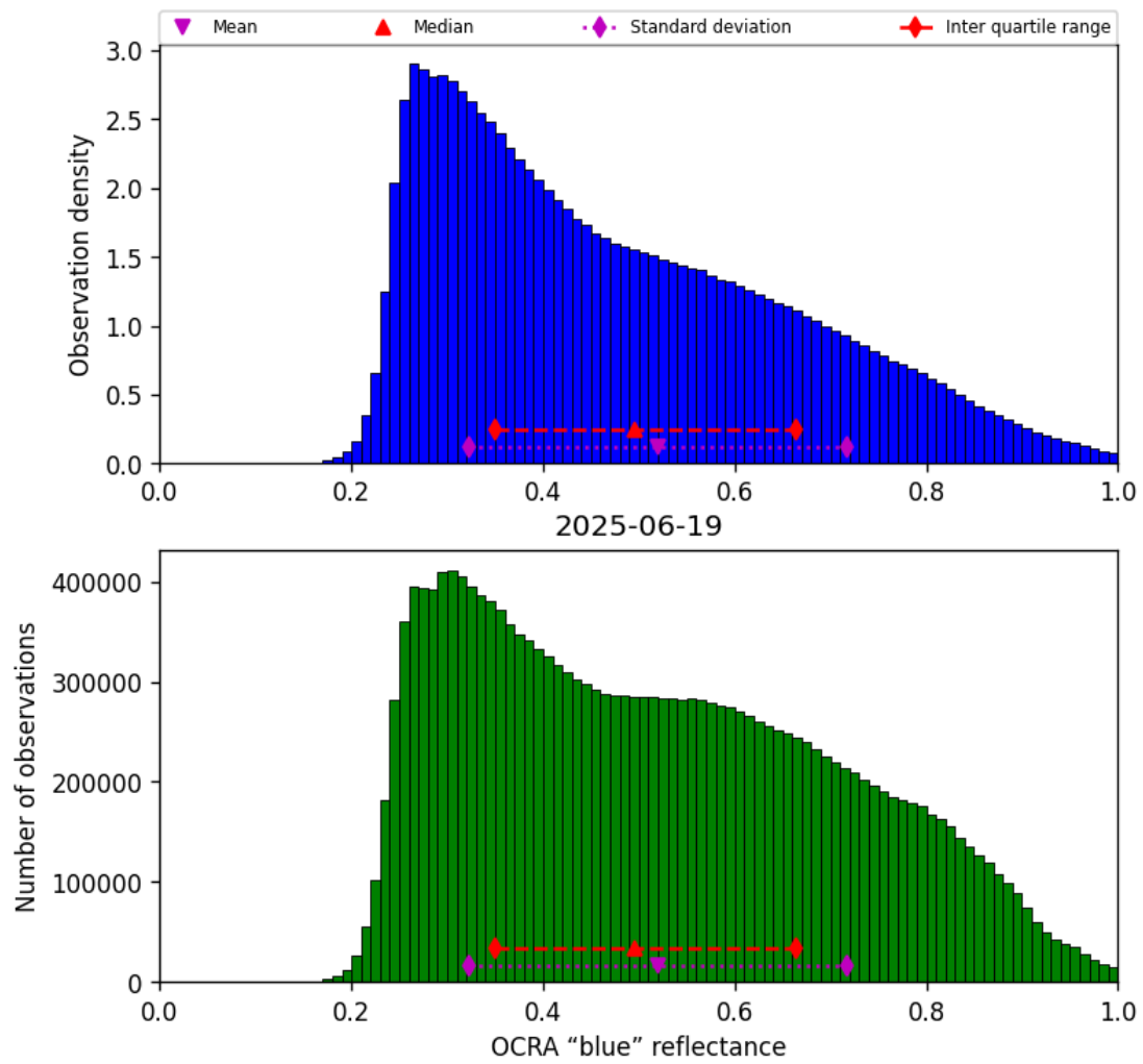
Figure 49: Histogram of “OCRA “blue” reflectance” for 2025-06-19 to 2025-06-20
