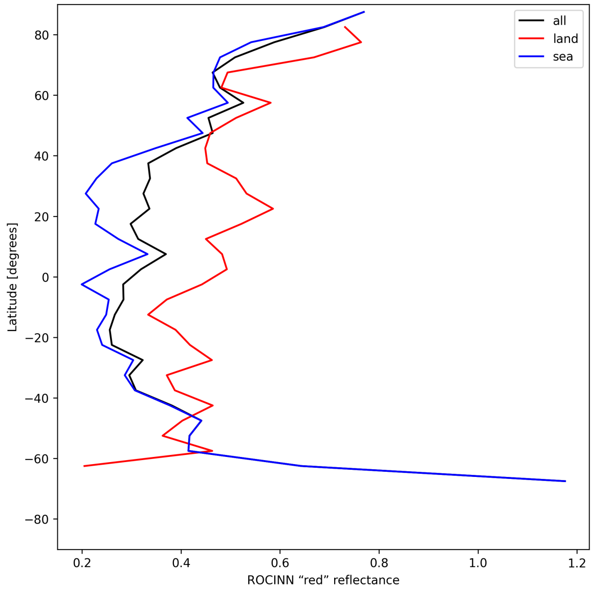
Figure 35: Zonal average of “ROCINN “red” reflectance” for 2025-06-19 to 2025-06-20.
