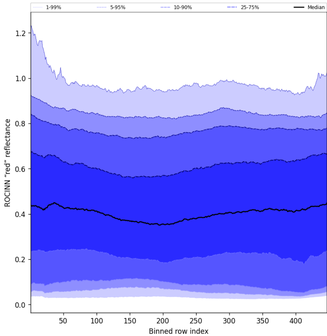
Figure 67: Along track statistics of "ROCINN "red" reflectance" for 2025-06-19 to 2025-06-20
