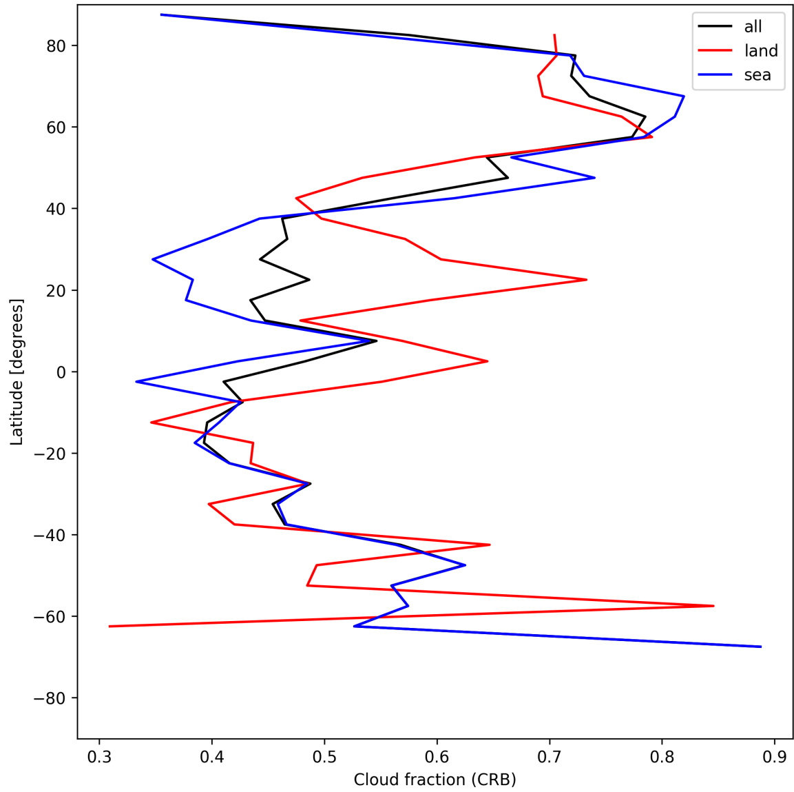
Figure 24: Zonal average of “Cloud fraction (CRB)” for 2025-06-19 to 2025-06-20.
