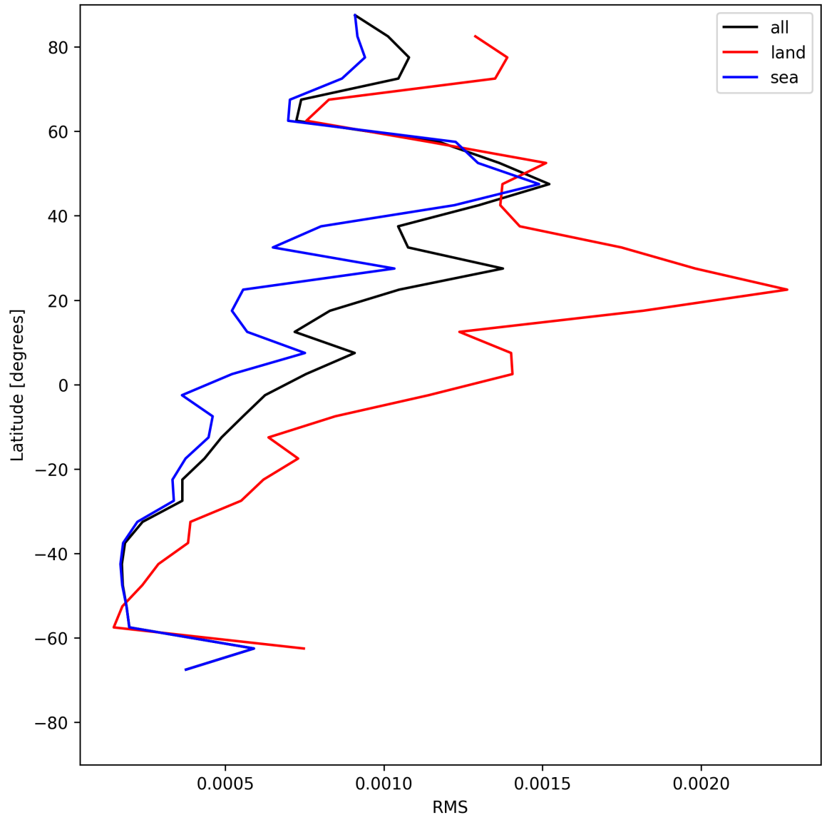
Figure 29: Zonal average of “RMS” for 2025-06-19 to 2025-06-20.
