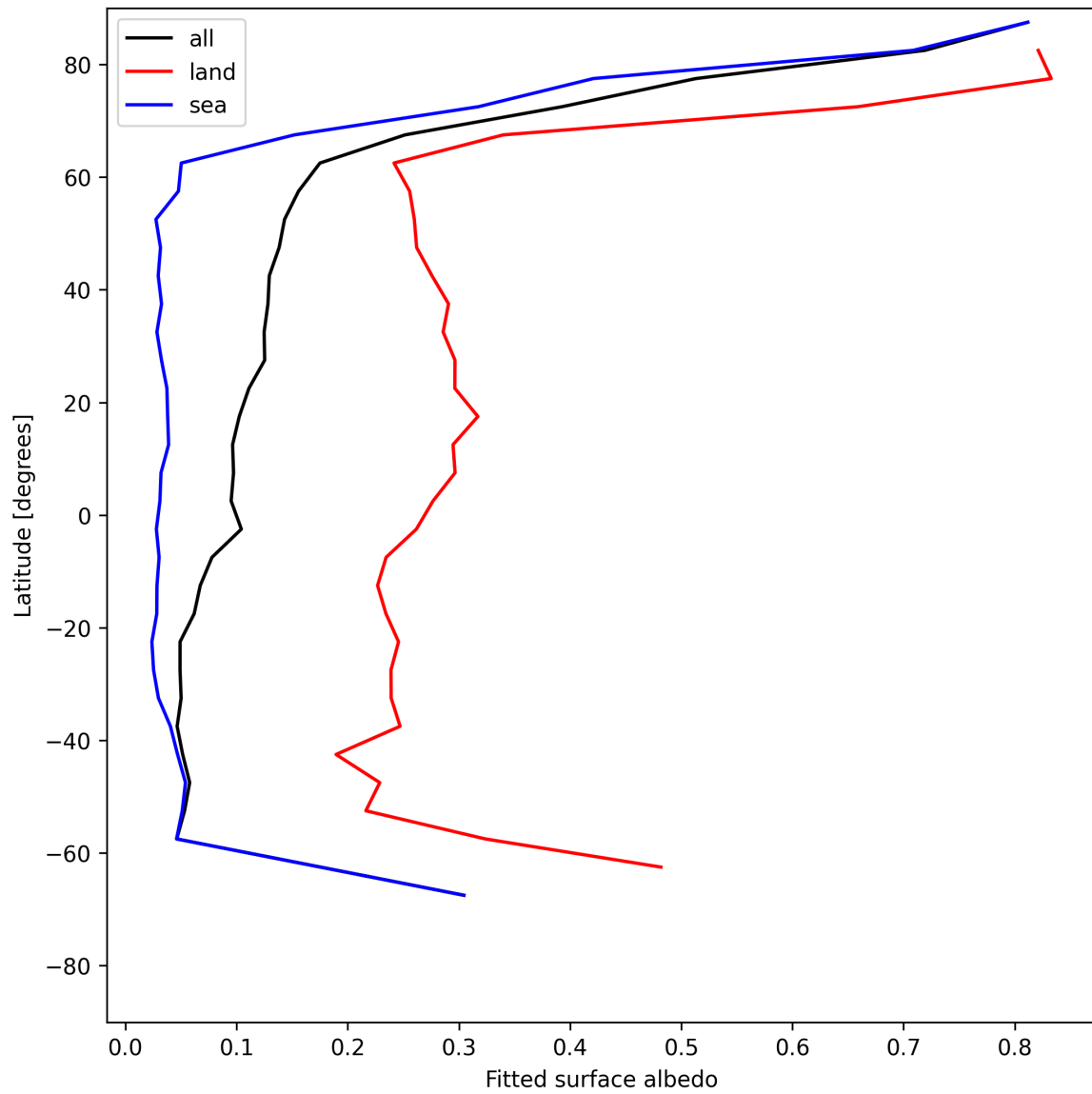
Figure 27: Zonal average of “Fitted surface albedo” for 2025-06-19 to 2025-06-20.
