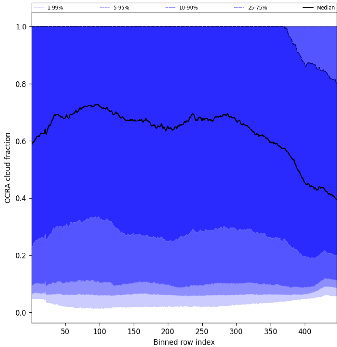
Figure 64: Along track statistics of “OCRA cloud fraction” for 2025-06-19 to 2025-06-20
