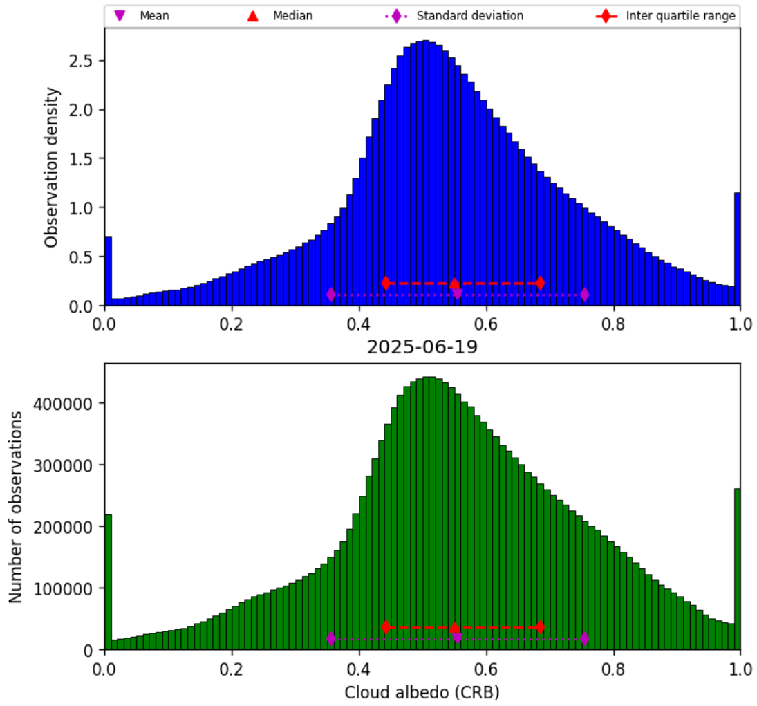
Figure 42: Histogram of “Cloud albedo (CRB)” for 2025-06-19 to 2025-06-20
