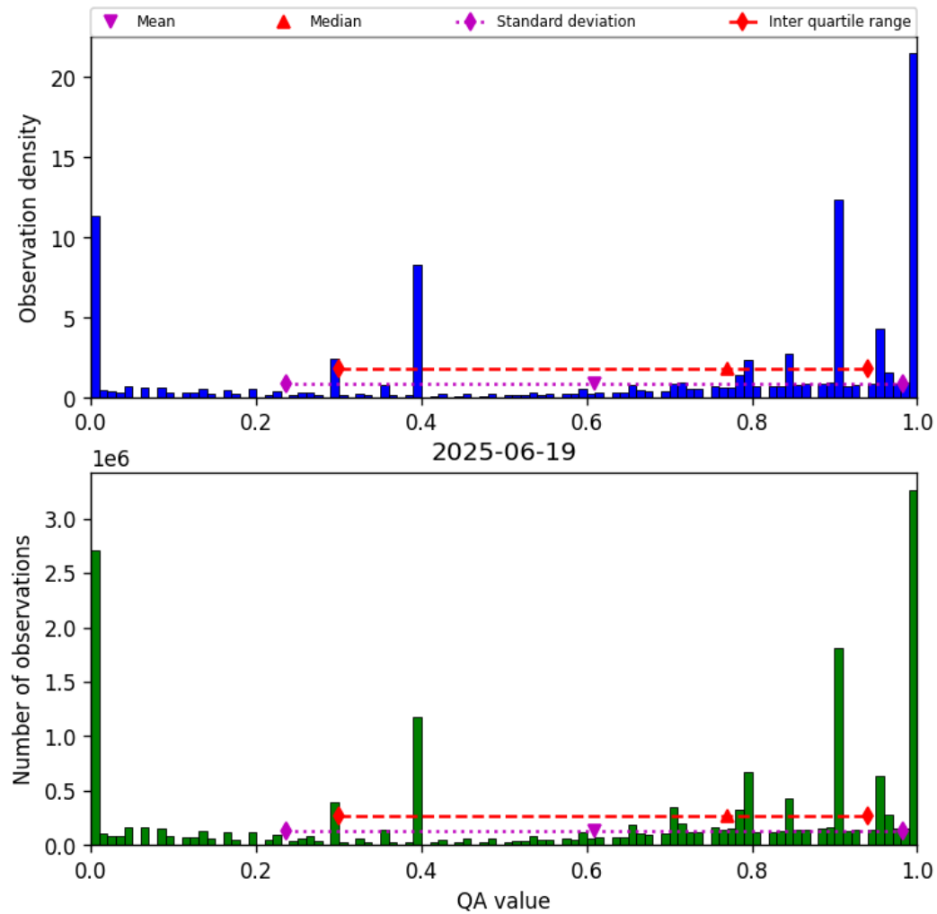
Figure 36: Histogram of “QA value” for 2025-06-19 to 2025-06-20
