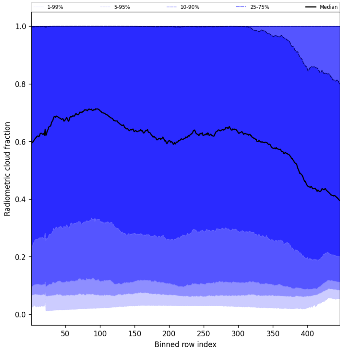
Figure 53: Along track statistics of “Radiometric cloud fraction” for 2025-06-19 to 2025-06-20
