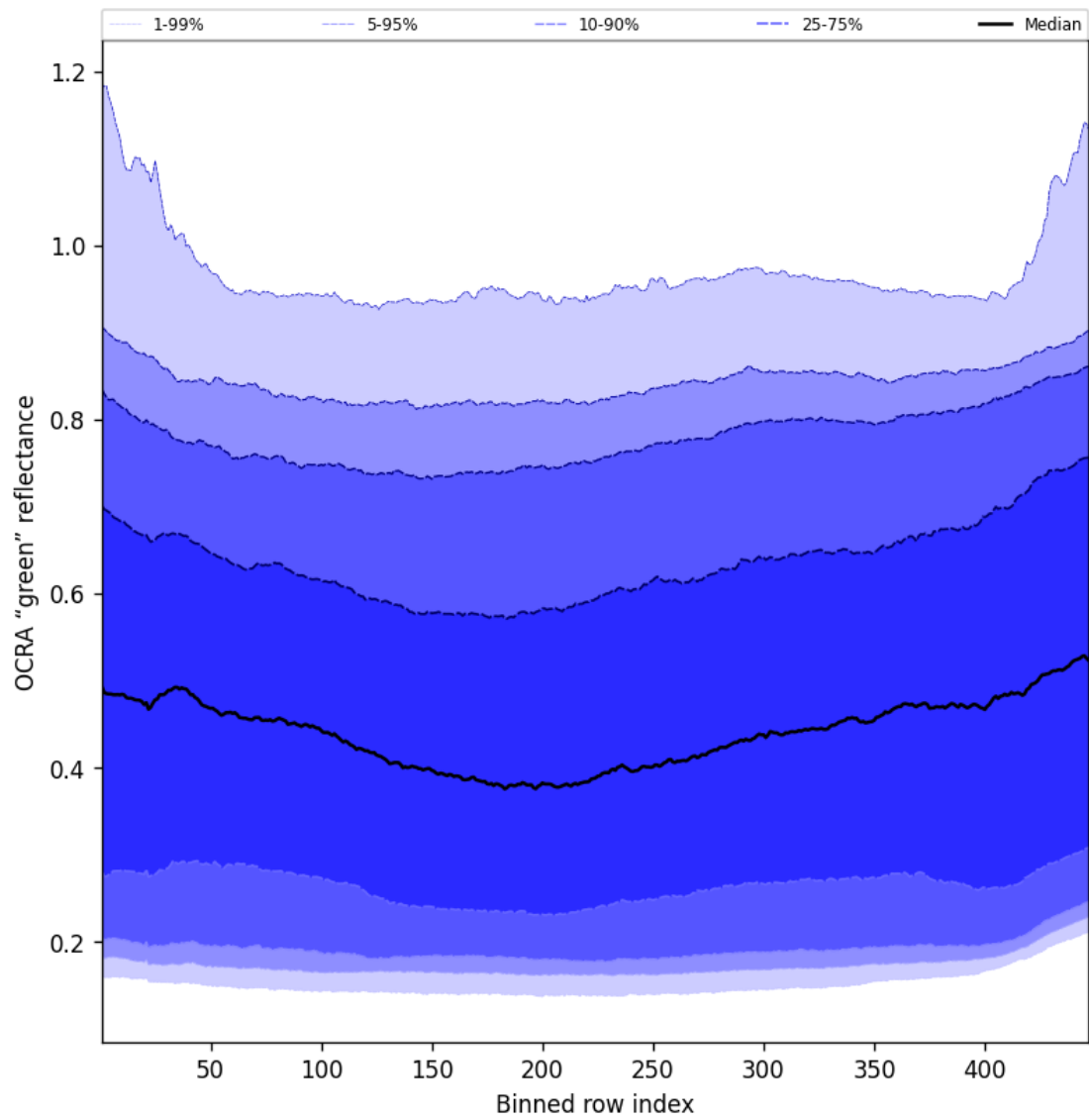
Figure 66: Along track statistics of “OCRA “green” reflectance” for 2025-06-19 to 2025-06-20
