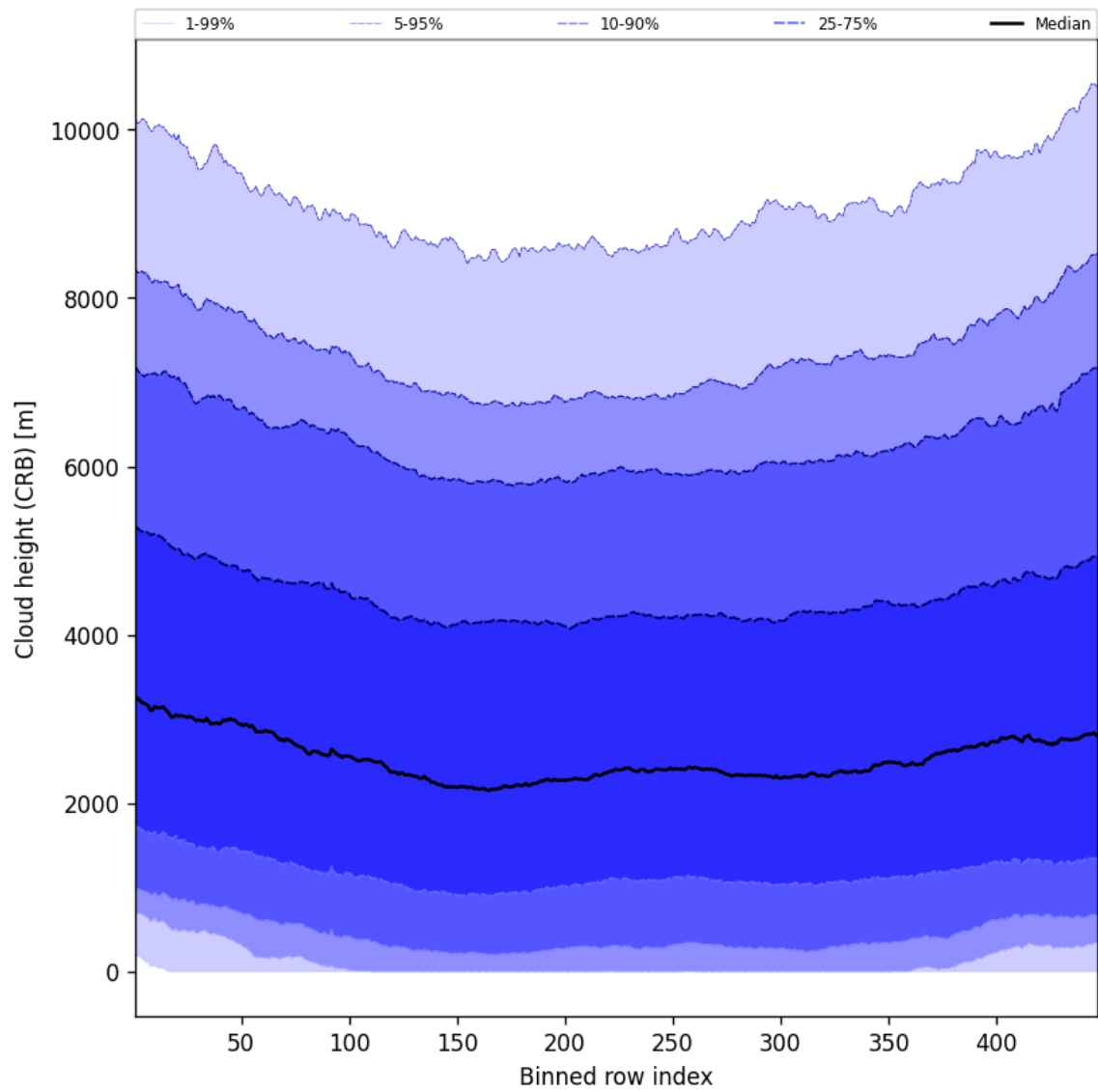
Figure 57: Along track statistics of “Cloud height (CRB)” for 2025-06-19 to 2025-06-20
