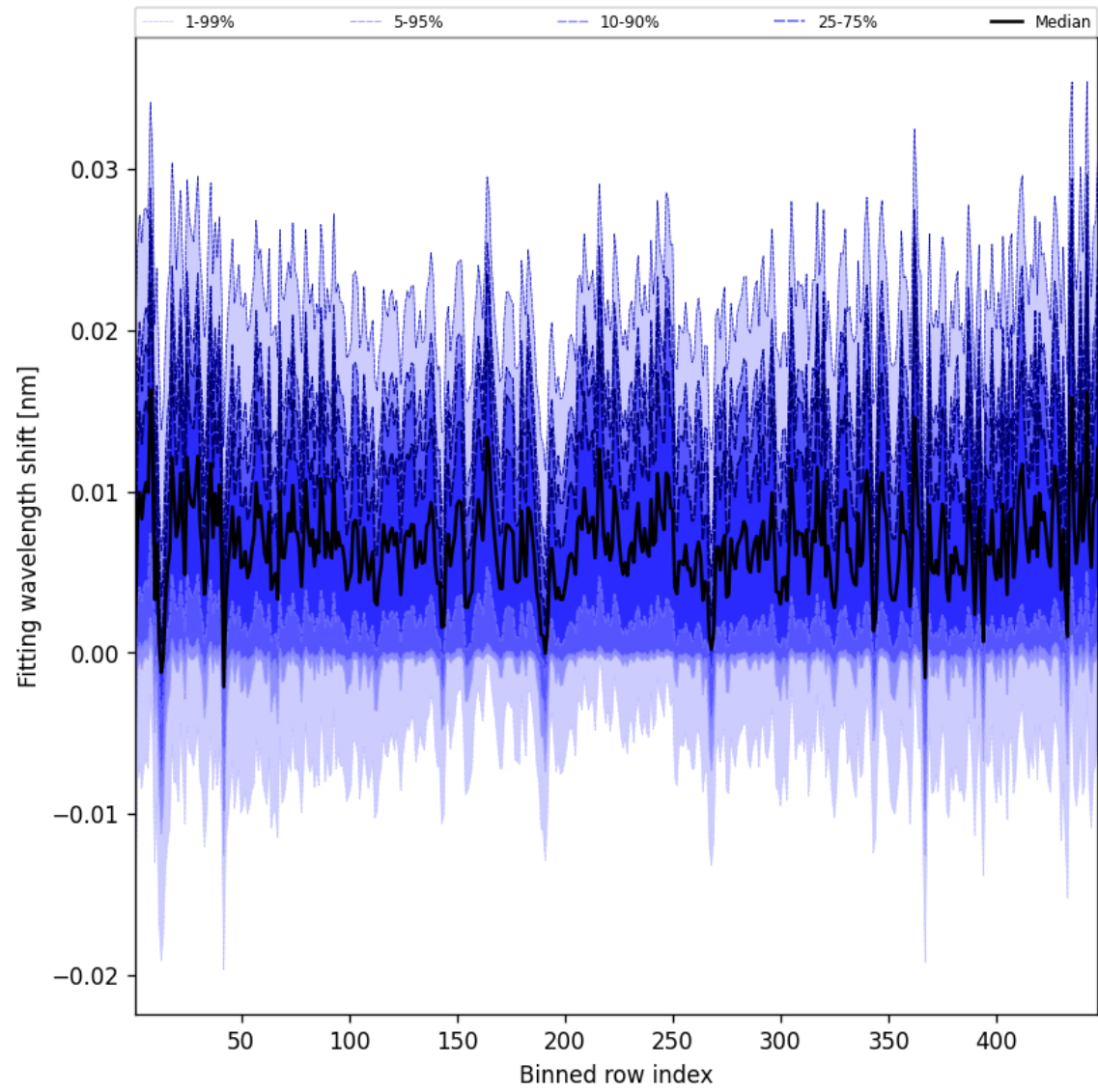
Figure 63: Along track statistics of “Fitting wavelength shift” for 2025-06-19 to 2025-06-20
