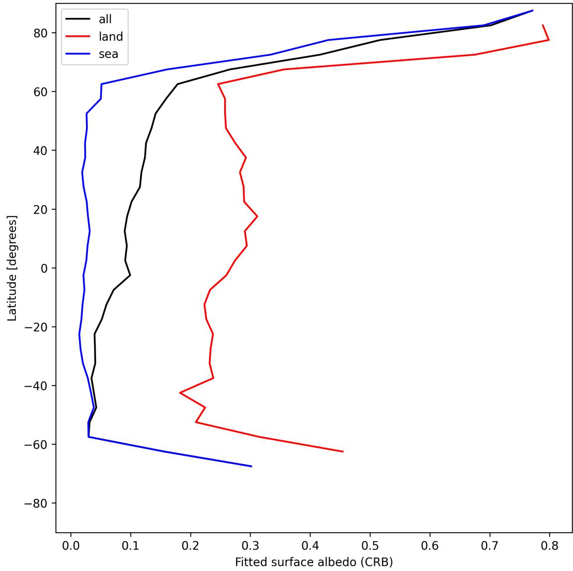
Figure 28: Zonal average of “Fitted surface albedo (CRB)” for 2025-06-19 to 2025-06-20.
