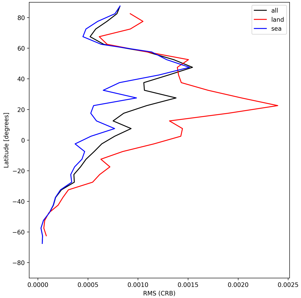
Figure 30: Zonal average of “RMS (CRB)” for 2025-06-19 to 2025-06-20.
