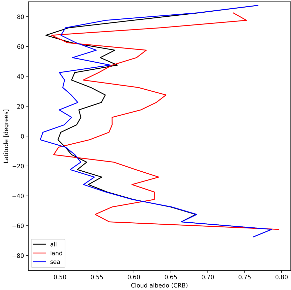
Figure 26: Zonal average of “Cloud albedo (CRB)” for 2025-06-19 to 2025-06-20.
