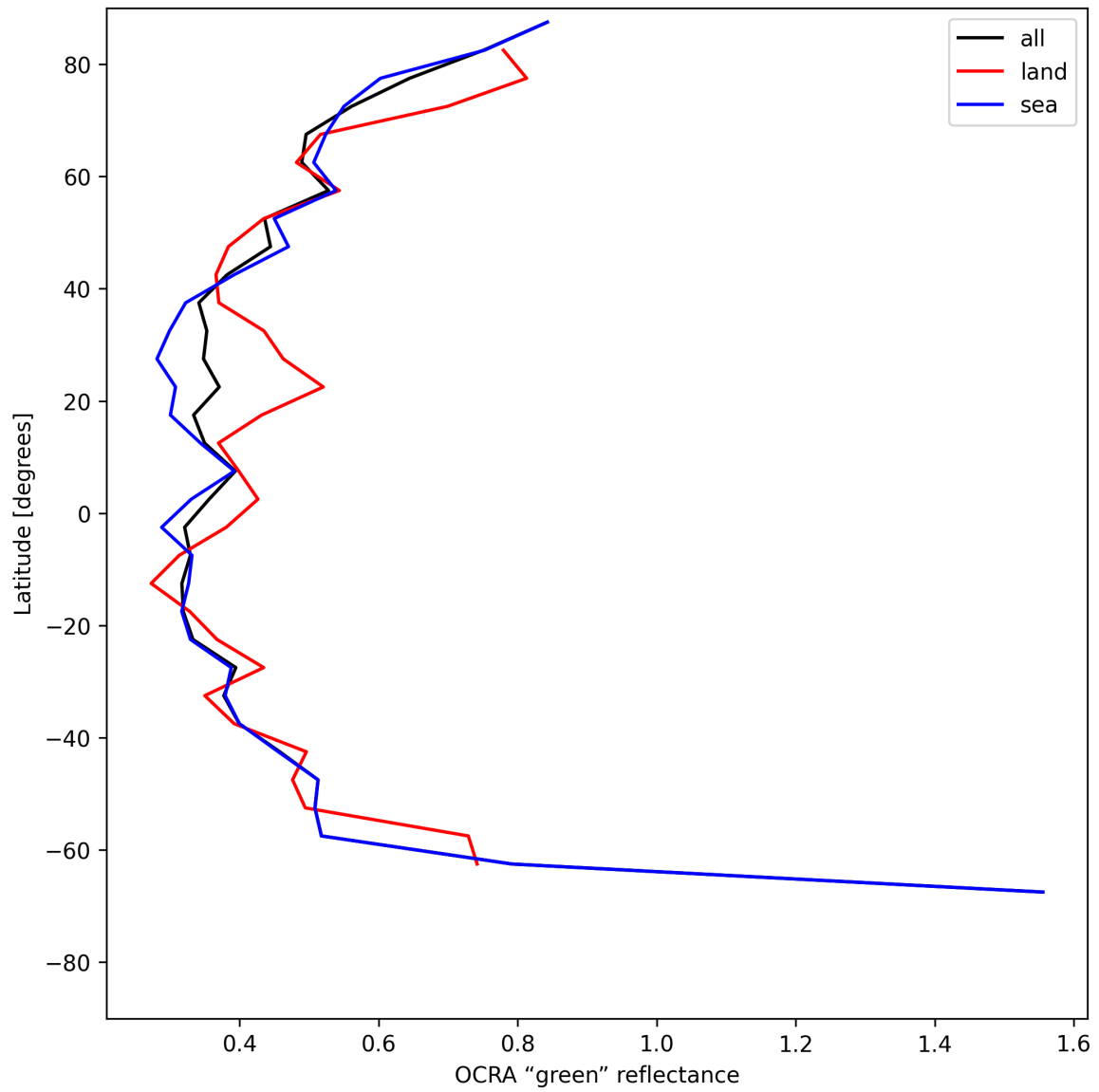
Figure 34: Zonal average of “OCRA “green” reflectance” for 2025-06-19 to 2025-06-20.
