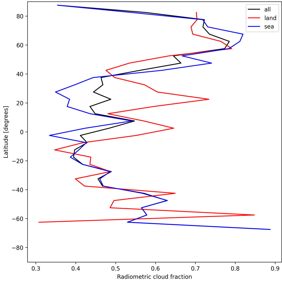
Figure 21: Zonal average of “Radiometric cloud fraction” for 2025-06-19 to 2025-06-20.
