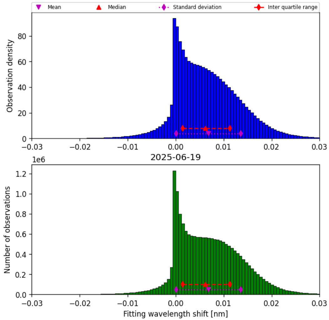
Figure 47: Histogram of “Fitting wavelength shift” for 2025-06-19 to 2025-06-20
