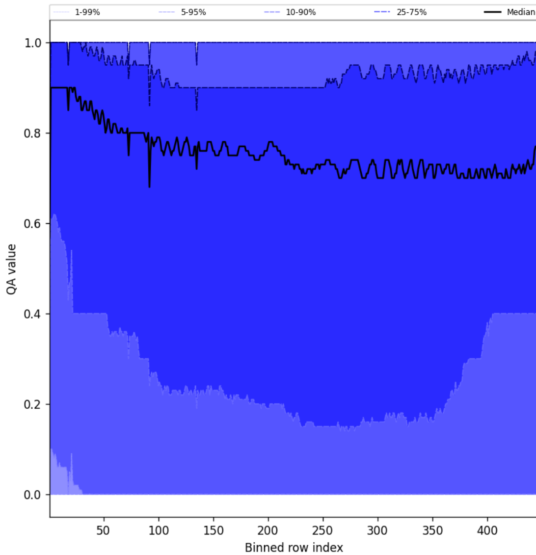
Figure 52: Along track statistics of “QA value” for 2025-06-19 to 2025-06-20
