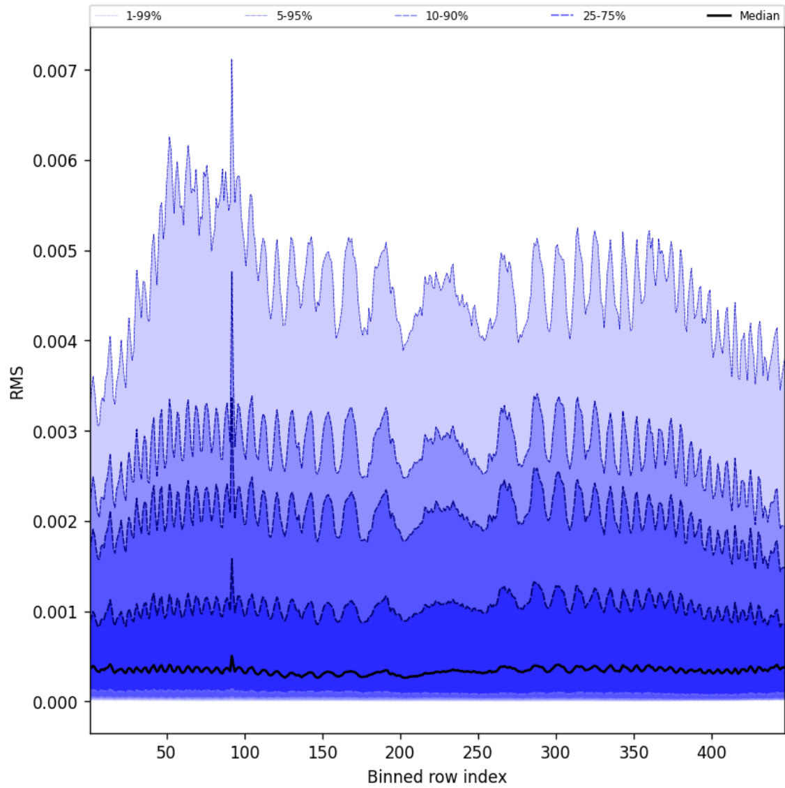
Figure 61: Along track statistics of “RMS” for 2025-06-19 to 2025-06-20
