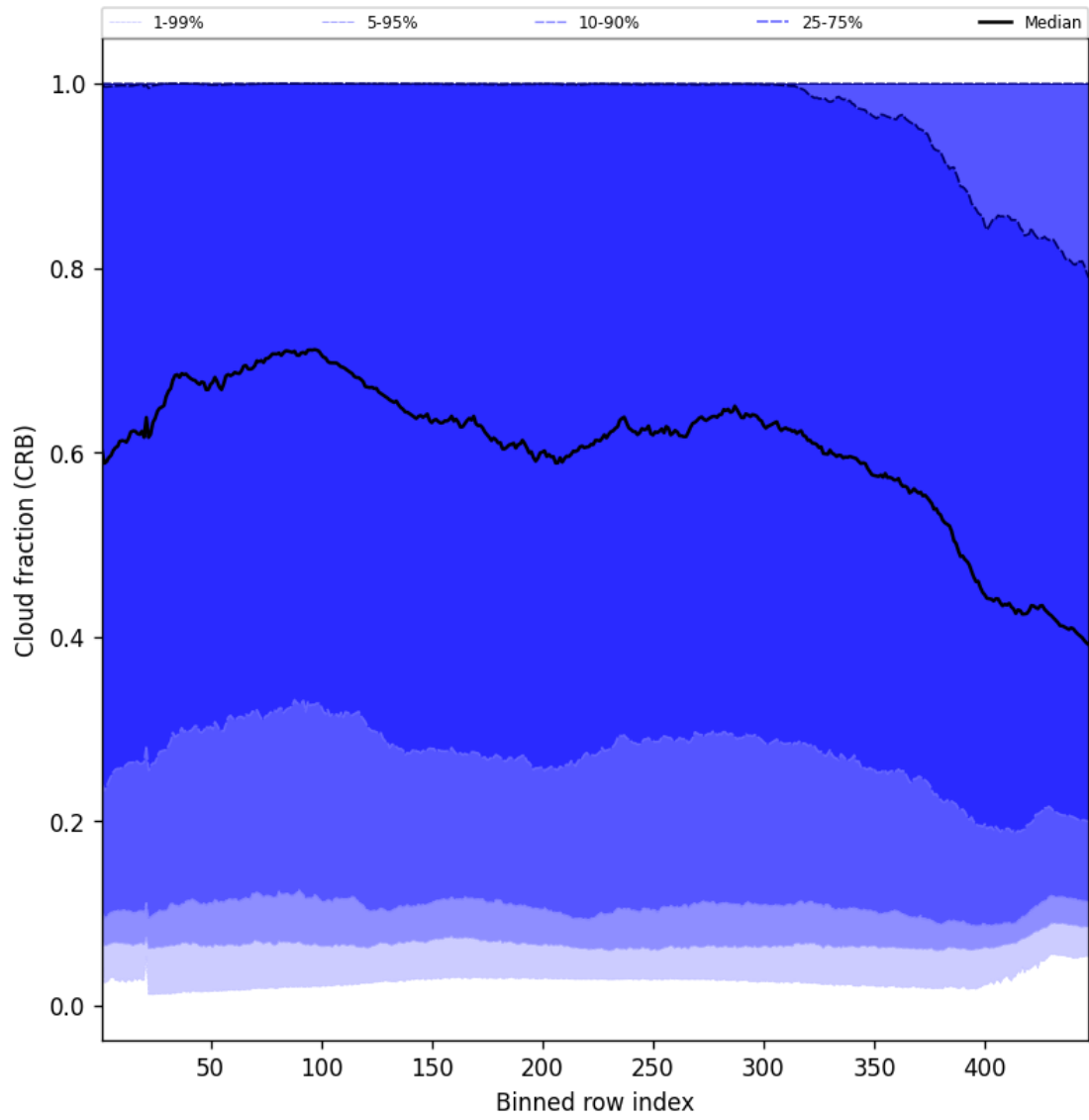
Figure 56: Along track statistics of “Cloud fraction (CRB)” for 2025-06-19 to 2025-06-20
