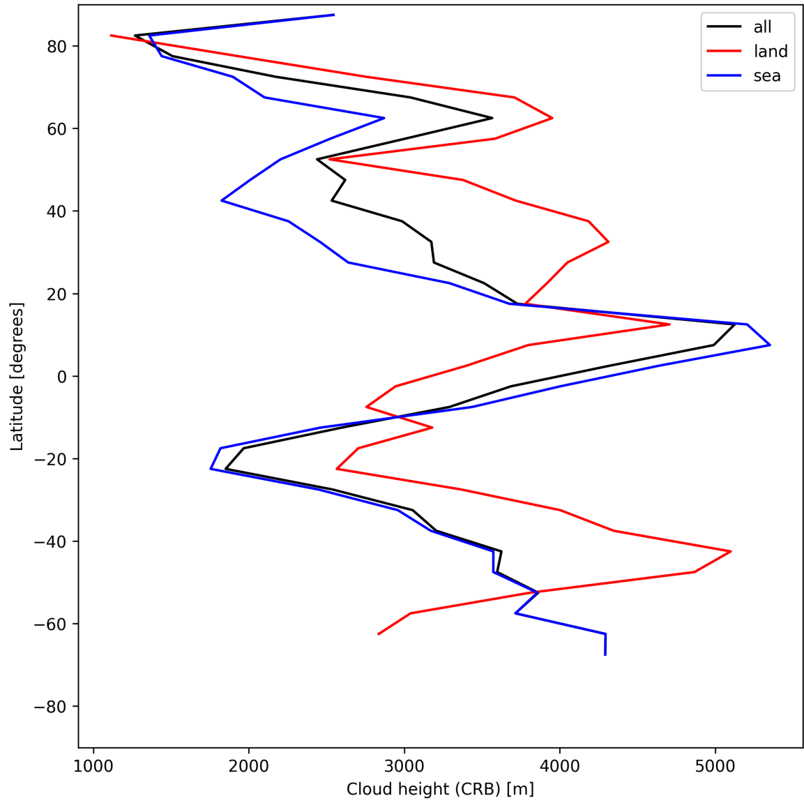
Figure 25: Zonal average of “Cloud height (CRB)” for 2025-06-19 to 2025-06-20.
