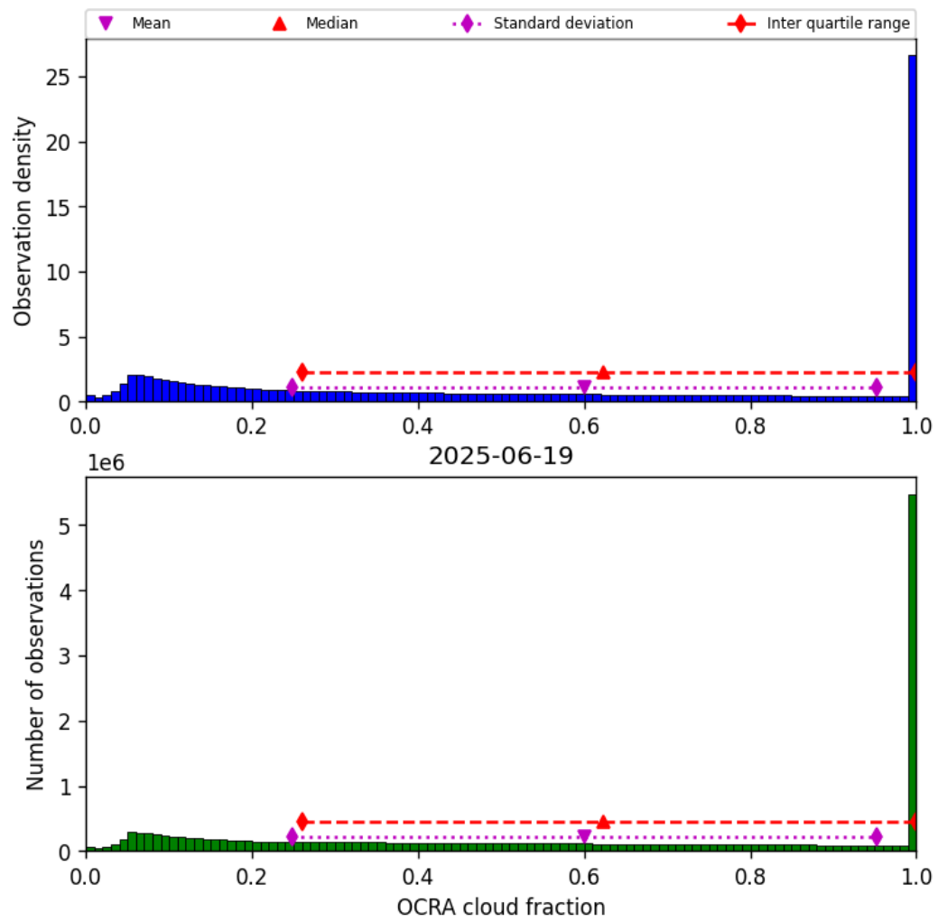
Figure 48: Histogram of “OCRA cloud fraction” for 2025-06-19 to 2025-06-20
