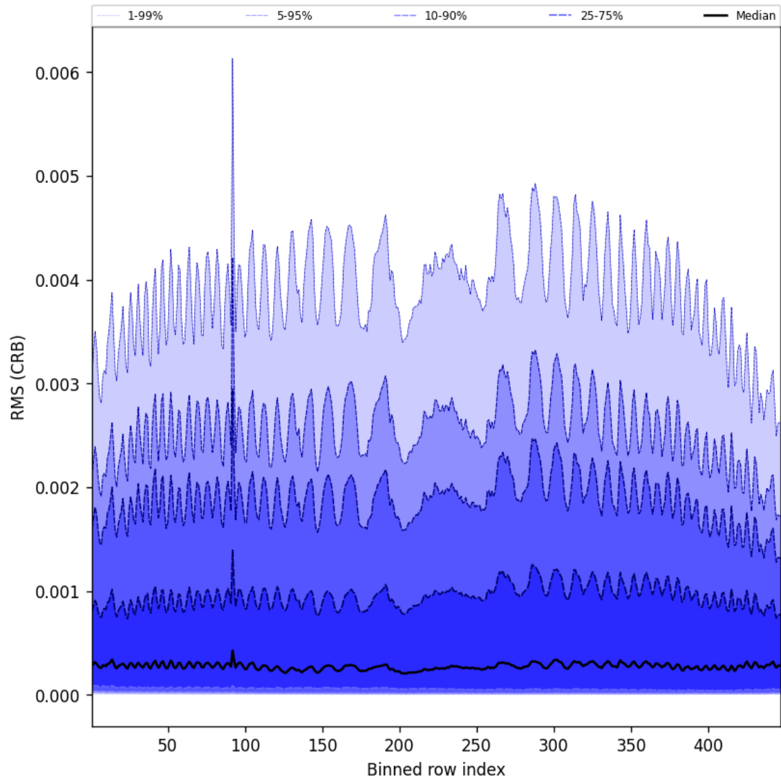
Figure 62: Along track statistics of “RMS (CRB)” for 2025-06-19 to 2025-06-20
