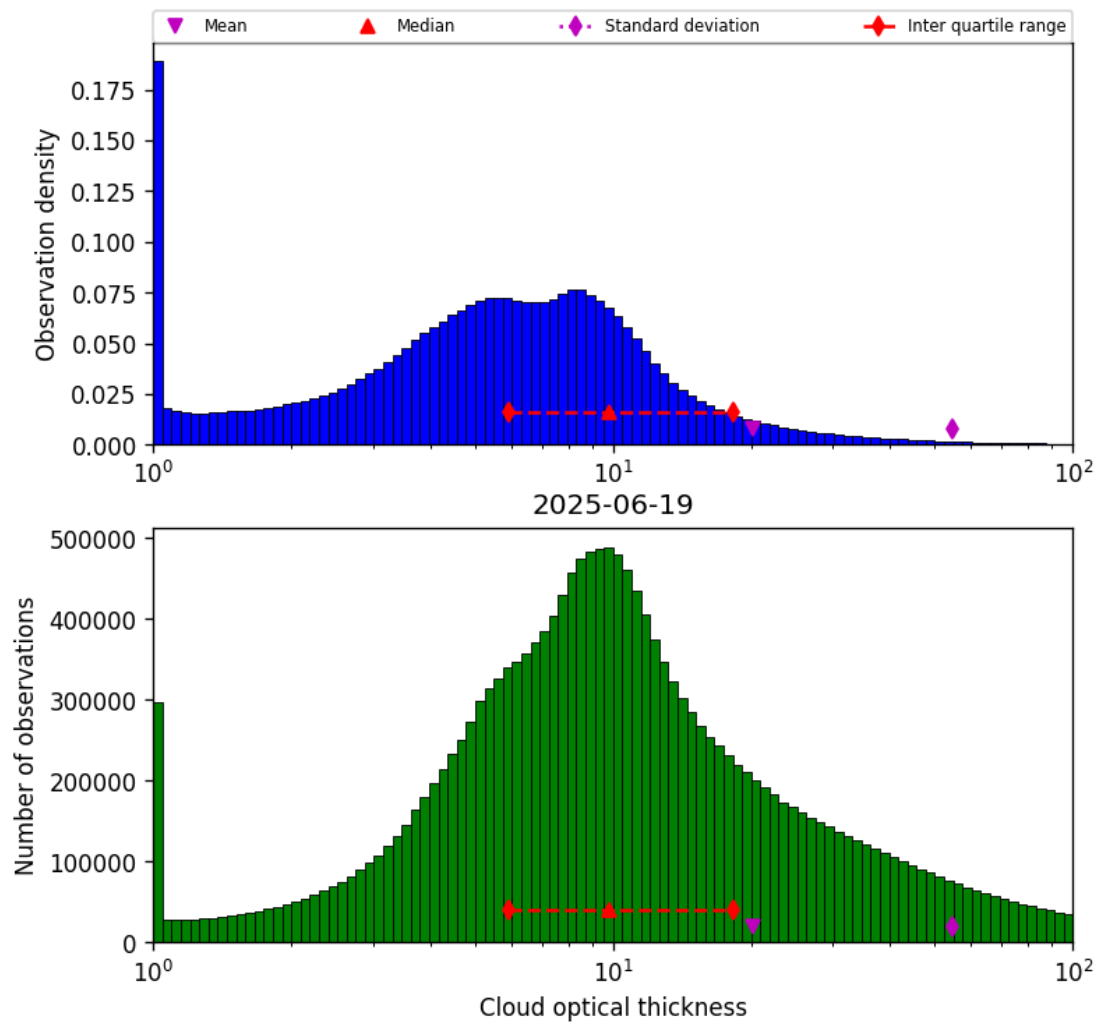
Figure 39: Histogram of “Cloud optical thickness” for 2025-06-19 to 2025-06-20
