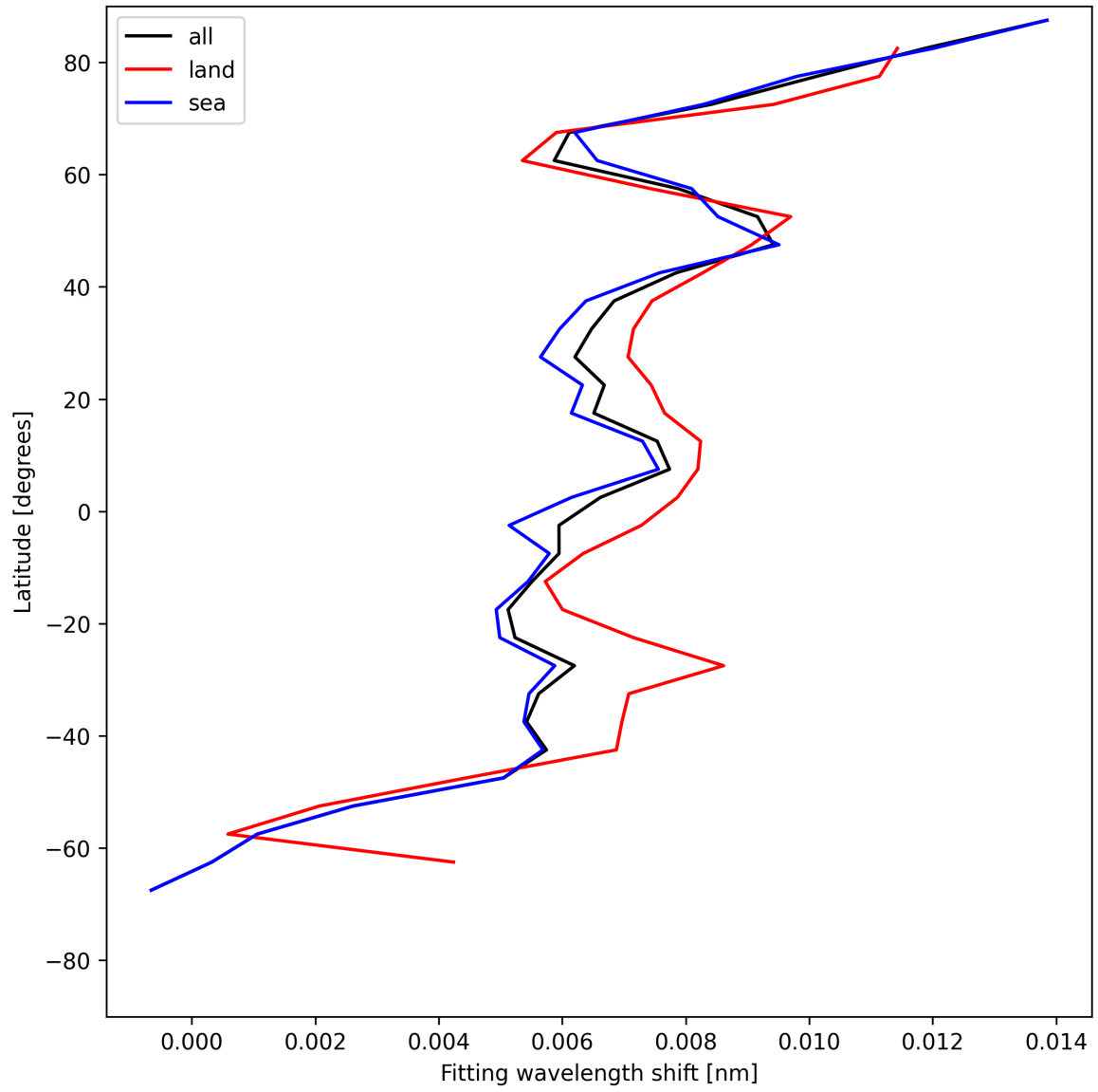
Figure 31: Zonal average of “Fitting wavelength shift” for 2025-06-19 to 2025-06-20.
