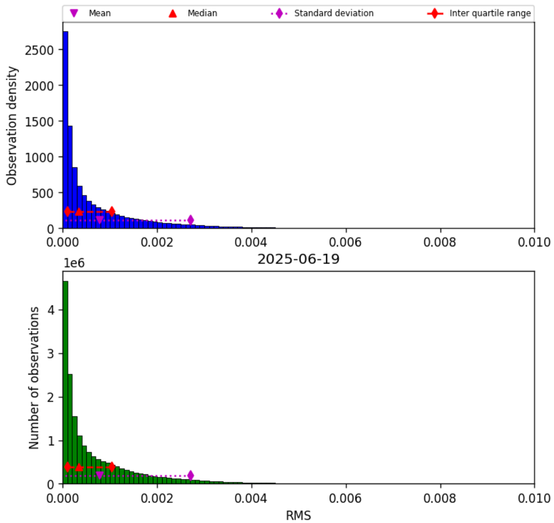
Figure 45: Histogram of “RMS” for 2025-06-19 to 2025-06-20
