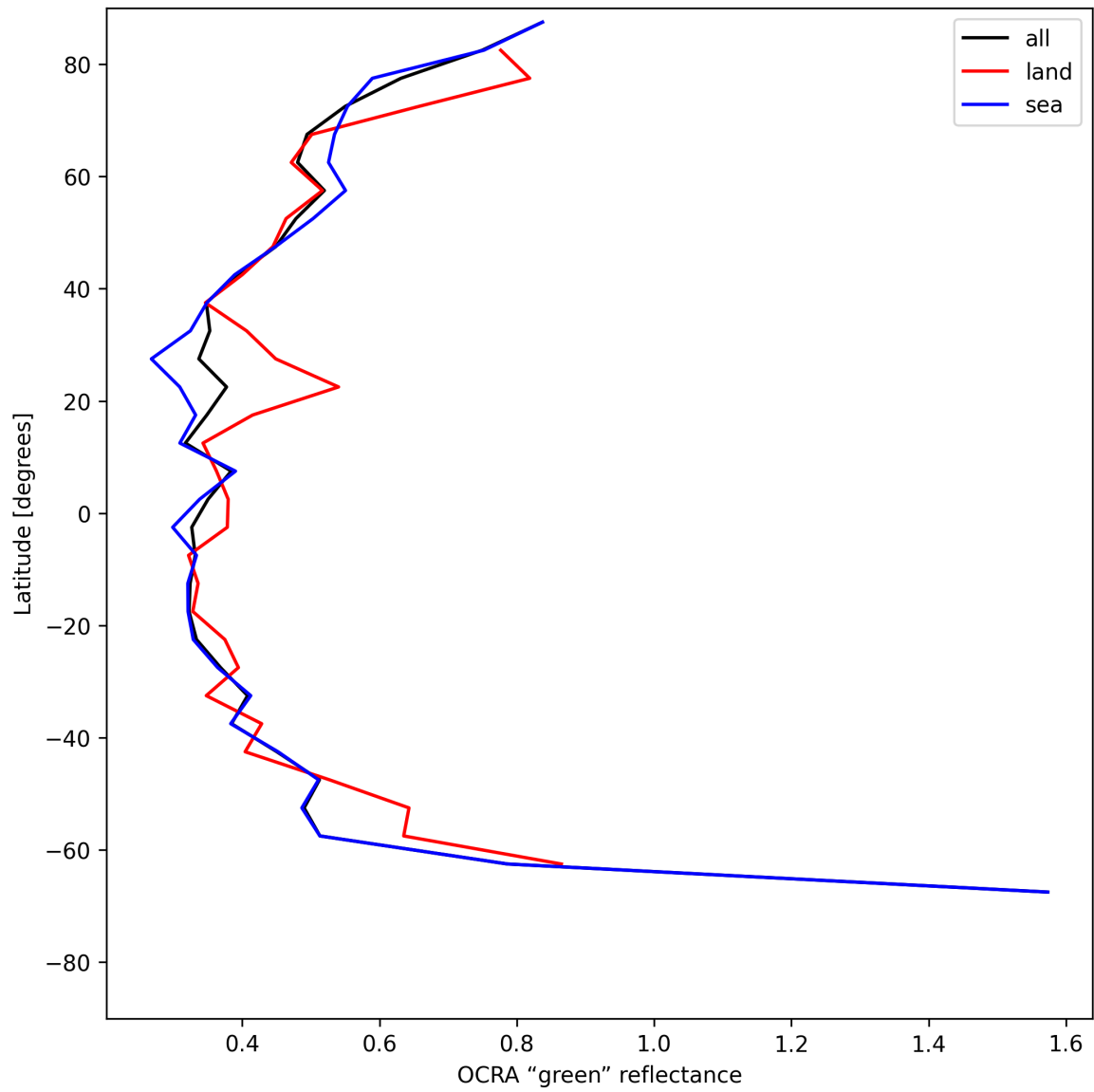
Figure 34: Zonal average of “OCRA “green” reflectance” for 2025-06-20 to 2025-06-20.
