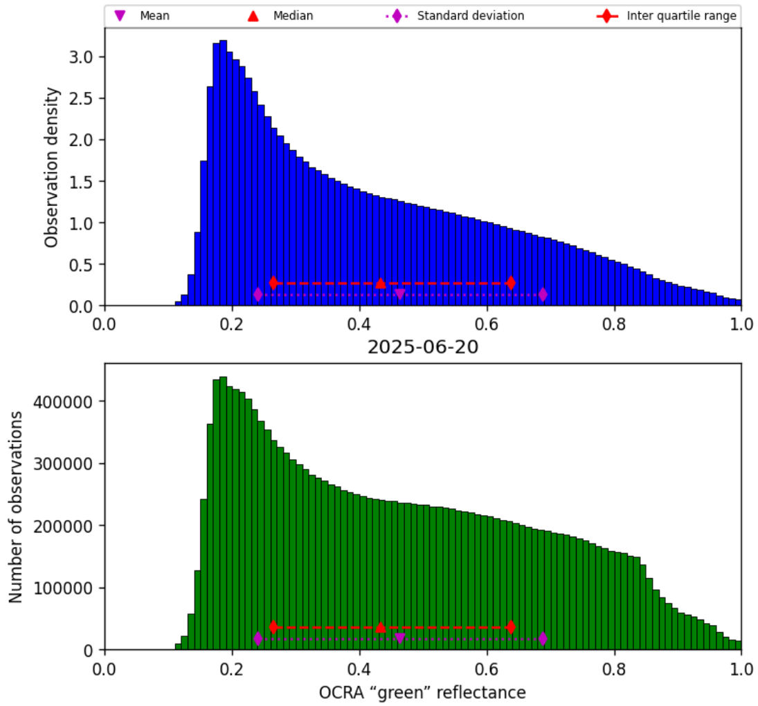
Figure 50: Histogram of “OCRA “green” reflectance” for 2025-06-20 to 2025-06-20
