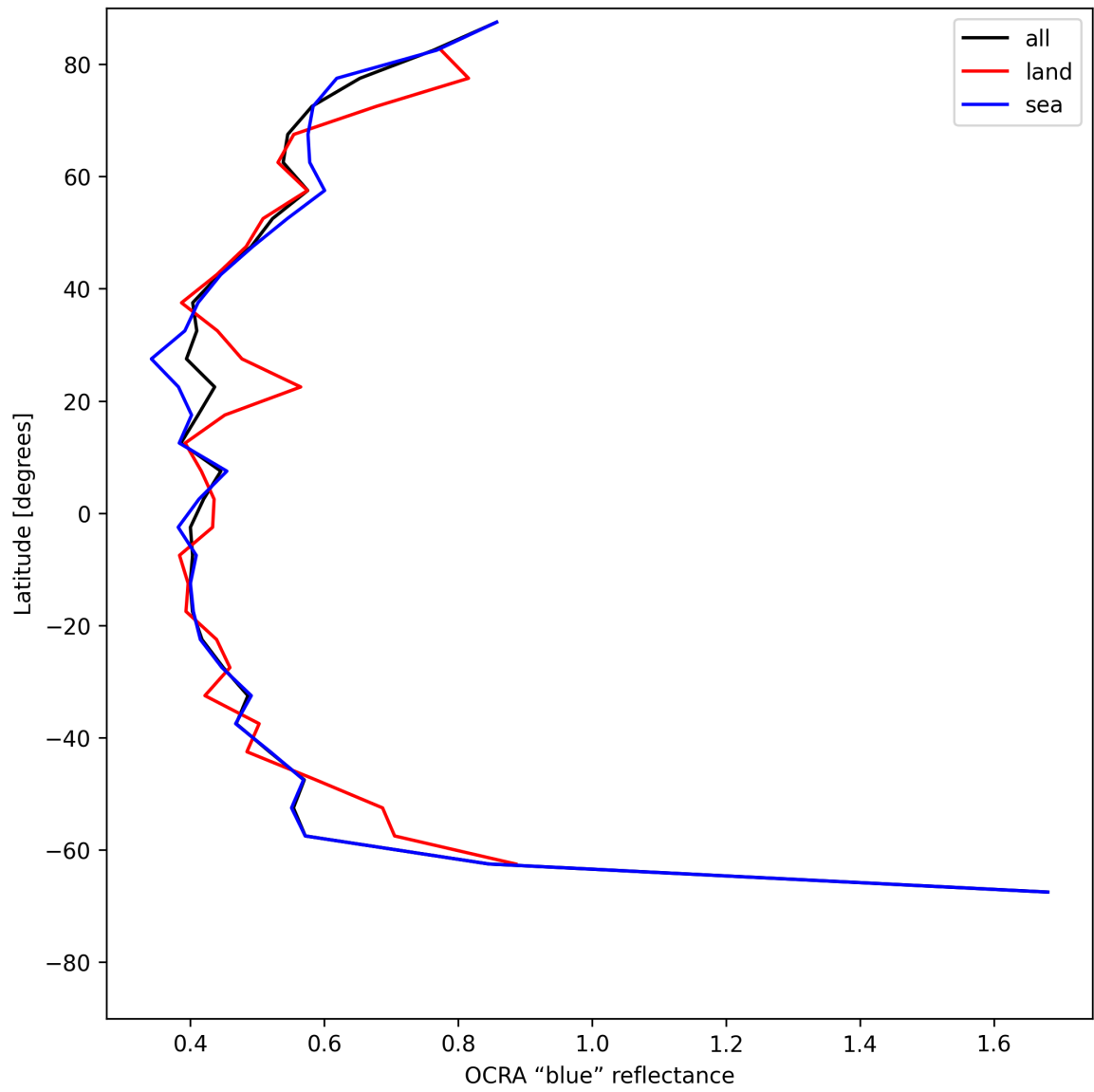
Figure 33: Zonal average of “OCRA “blue” reflectance” for 2025-06-20 to 2025-06-20.
