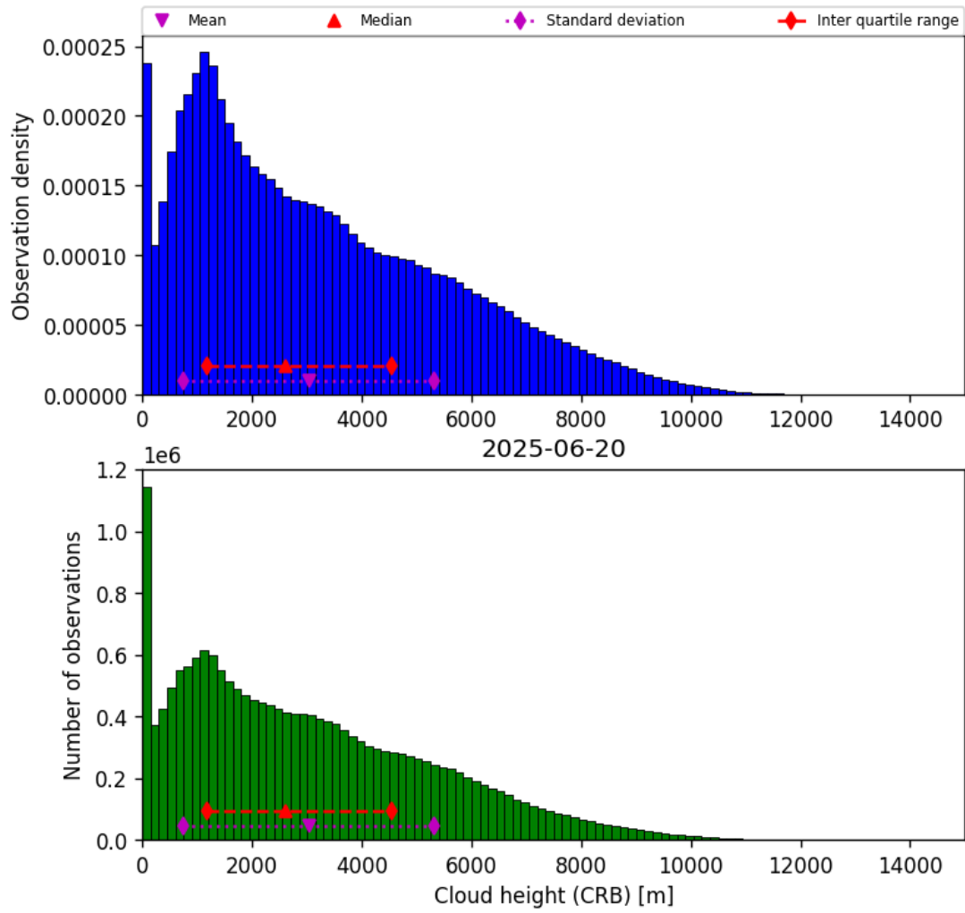
Figure 41: Histogram of “Cloud height (CRB)” for 2025-06-20 to 2025-06-20
