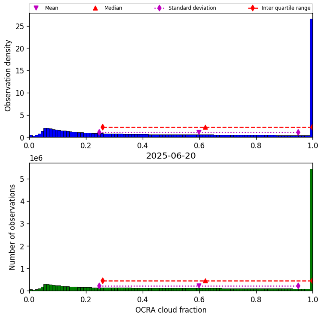
Figure 48: Histogram of “OCRA cloud fraction” for 2025-06-20 to 2025-06-20
