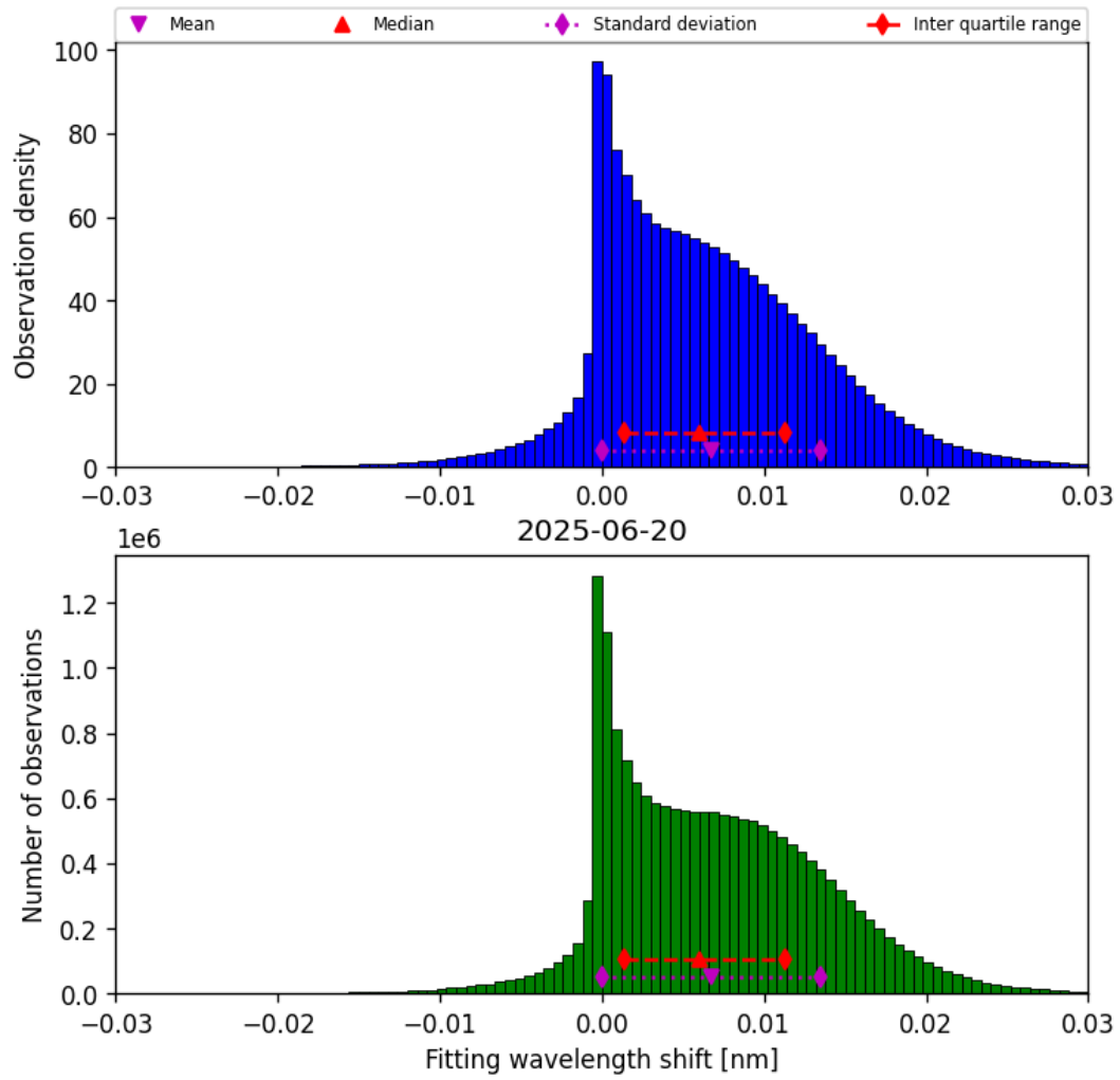
Figure 47: Histogram of “Fitting wavelength shift” for 2025-06-20 to 2025-06-20
