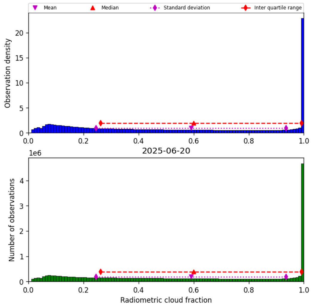
Figure 37: Histogram of “Radiometric cloud fraction” for 2025-06-20 to 2025-06-20
