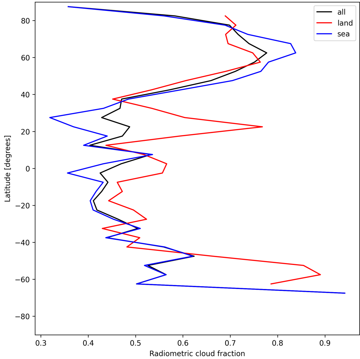
Figure 21: Zonal average of “Radiometric cloud fraction” for 2025-06-20 to 2025-06-20.
