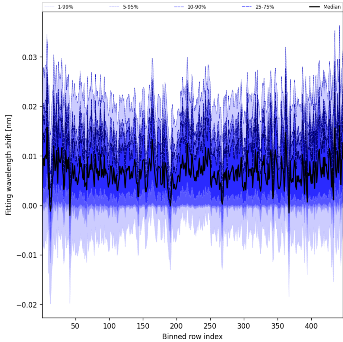
Figure 63: Along track statistics of “Fitting wavelength shift” for 2025-06-20 to 2025-06-20
