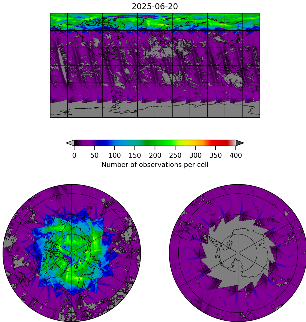
Figure 19: Map of the number of observations for 2025-06-20 to 2025-06-20
