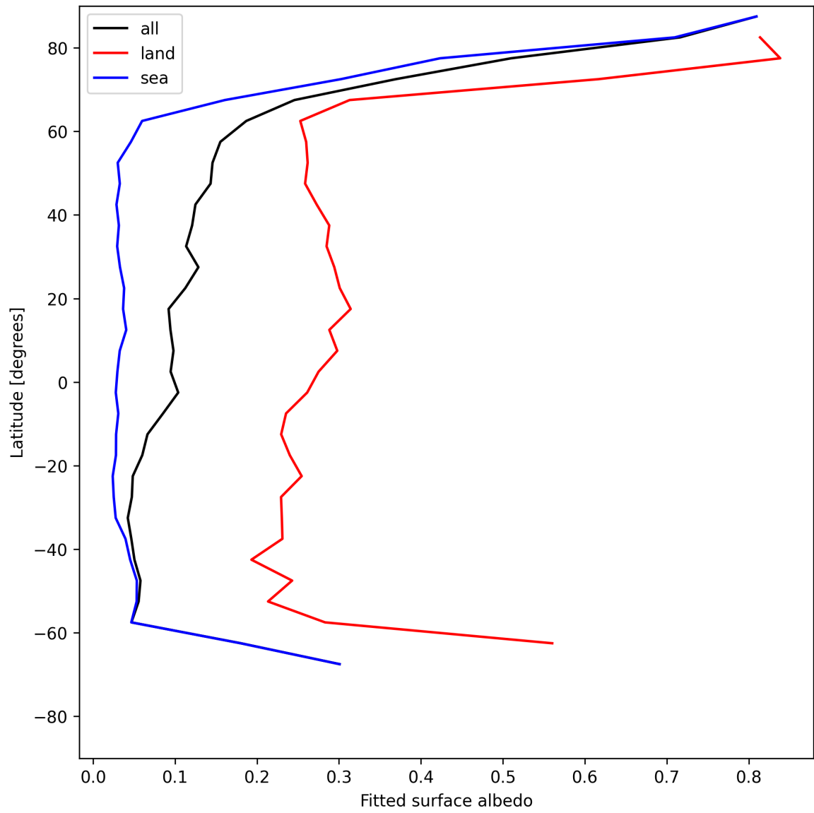
Figure 27: Zonal average of “Fitted surface albedo” for 2025-06-20 to 2025-06-20.
