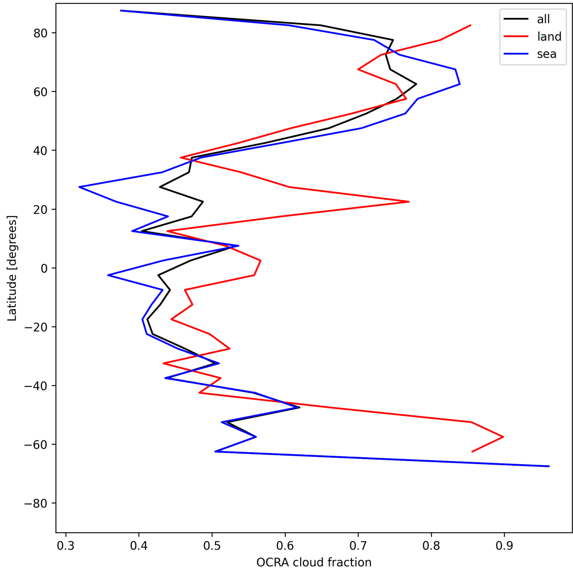
Figure 32: Zonal average of “OCRA cloud fraction” for 2025-06-20 to 2025-06-20.
