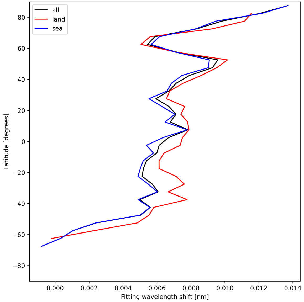
Figure 31: Zonal average of “Fitting wavelength shift” for 2025-06-20 to 2025-06-20.
