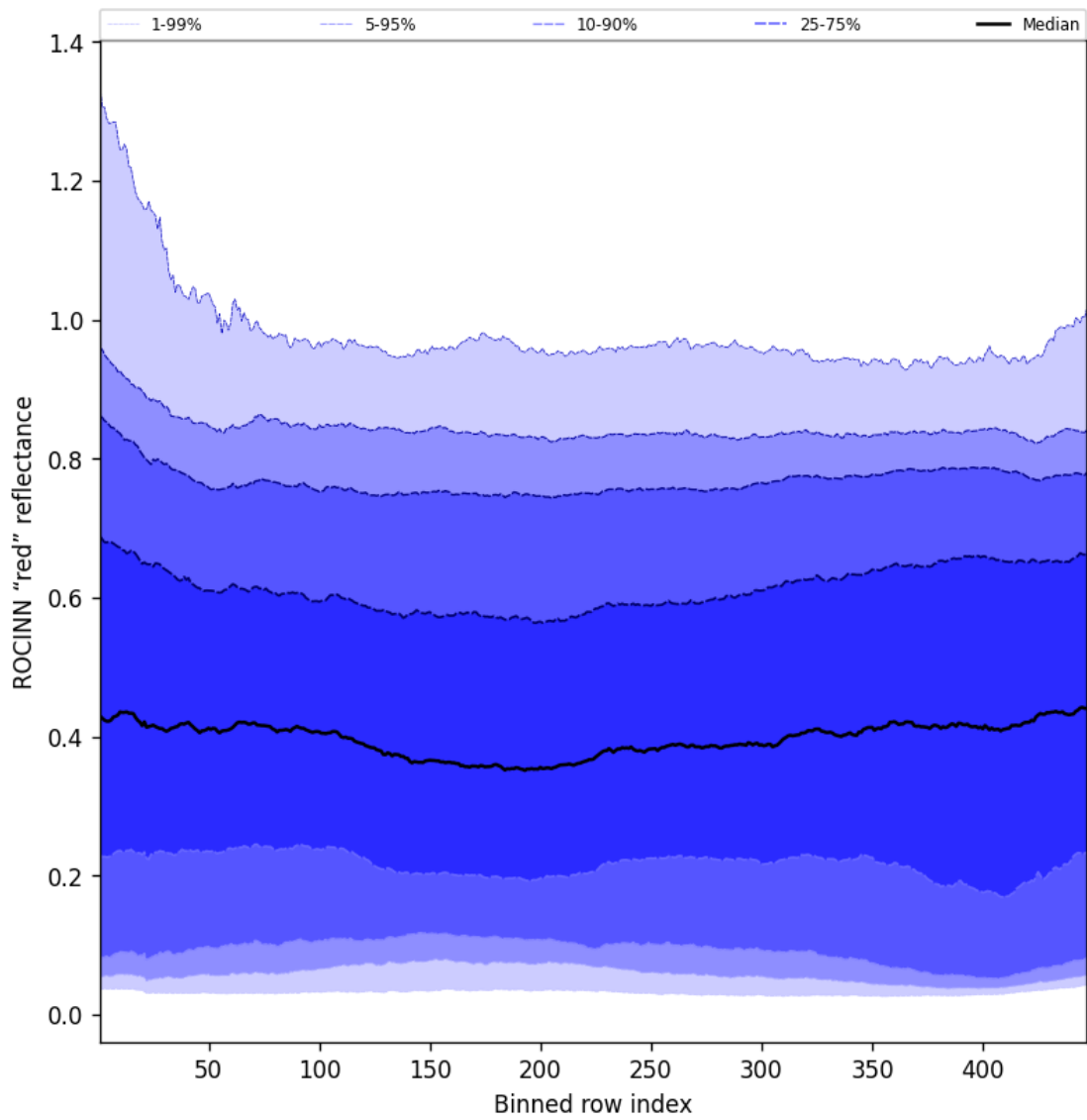
Figure 67: Along track statistics of “ROCINN “red” reflectance” for 2025-06-20 to 2025-06-20
