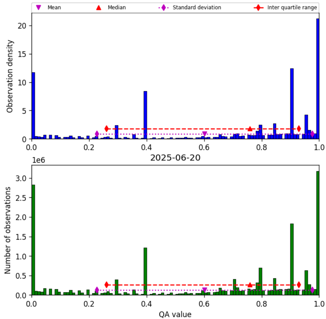
Figure 36: Histogram of “QA value” for 2025-06-20 to 2025-06-20
