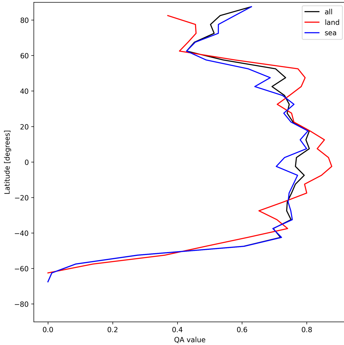
Figure 20: Zonal average of “QA value” for 2025-06-20 to 2025-06-20.
