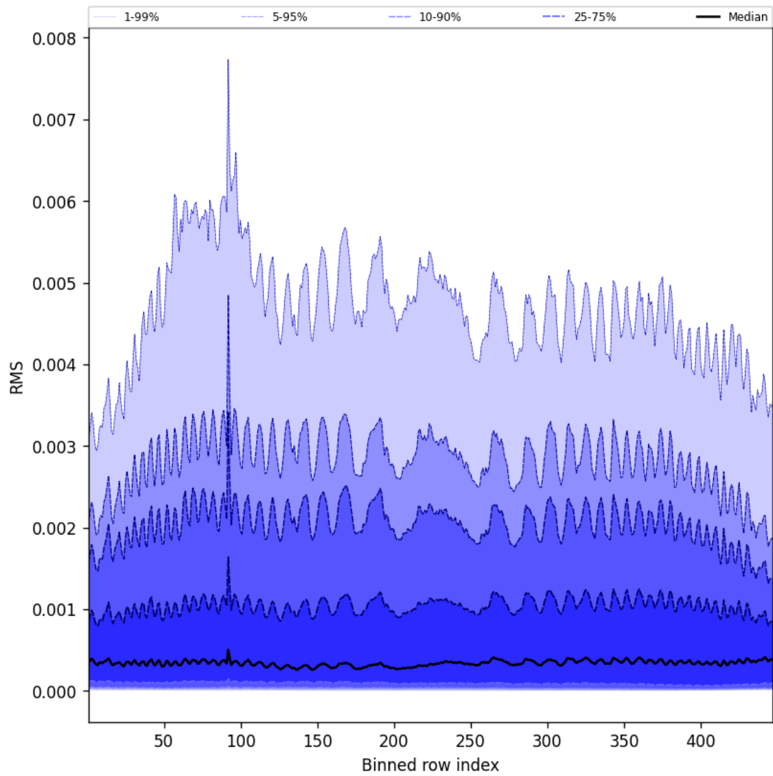
Figure 61: Along track statistics of “RMS” for 2025-06-20 to 2025-06-20
