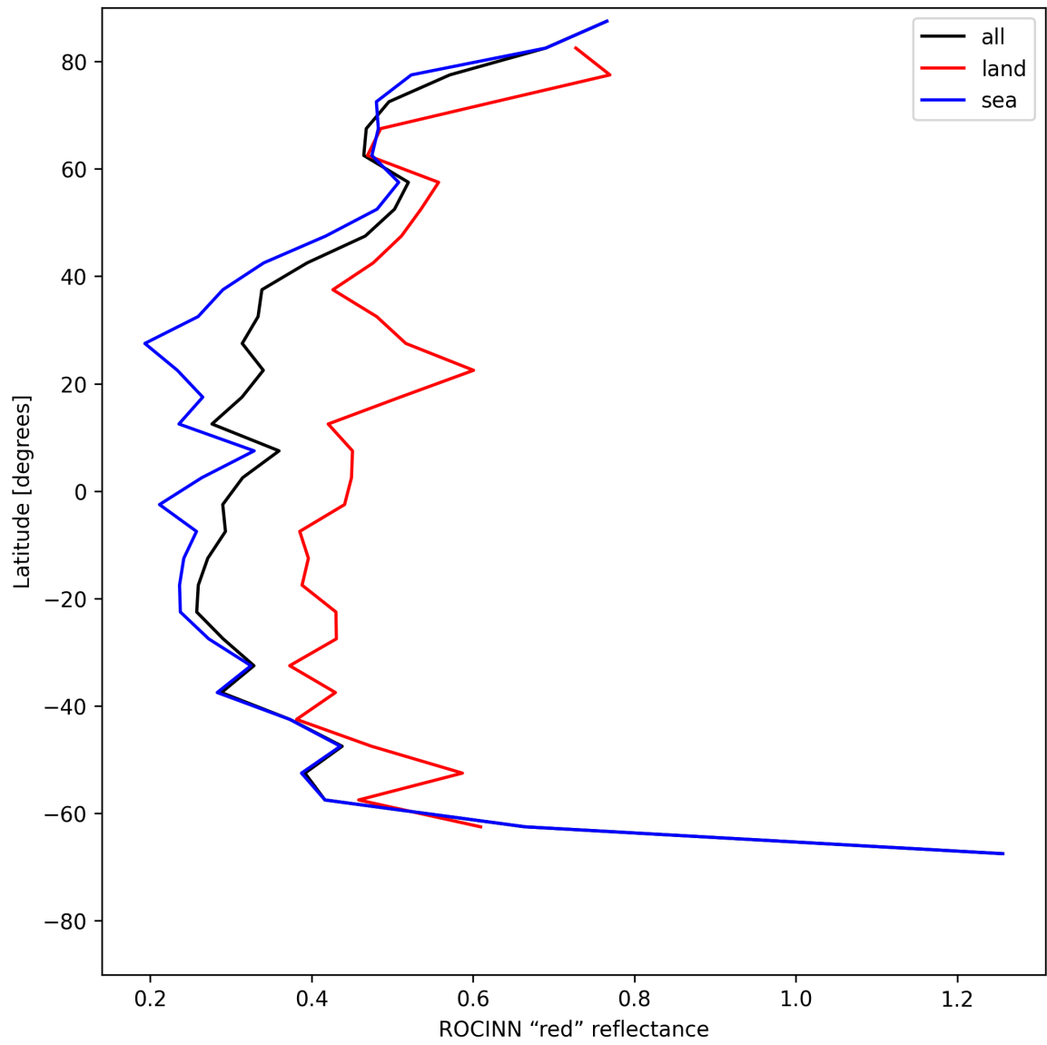
Figure 35: Zonal average of "ROCINN "red" reflectance" for 2025-06-20 to 2025-06-20.
