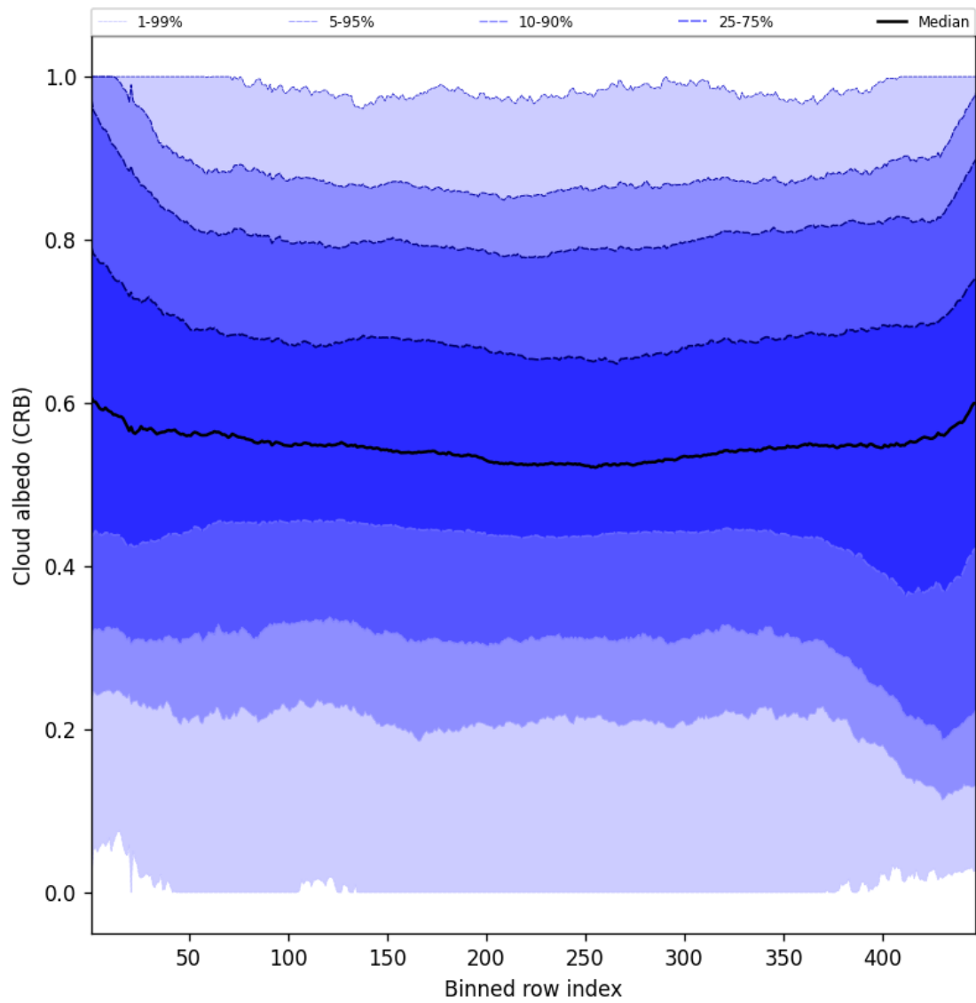
Figure 58: Along track statistics of “Cloud albedo (CRB)” for 2025-06-20 to 2025-06-20
