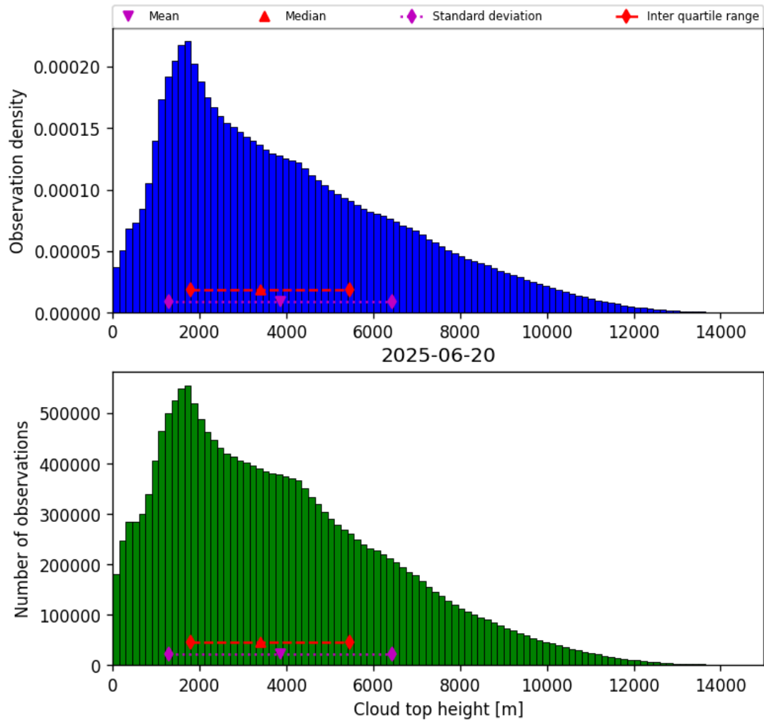
Figure 38: Histogram of “Cloud top height” for 2025-06-20 to 2025-06-20
