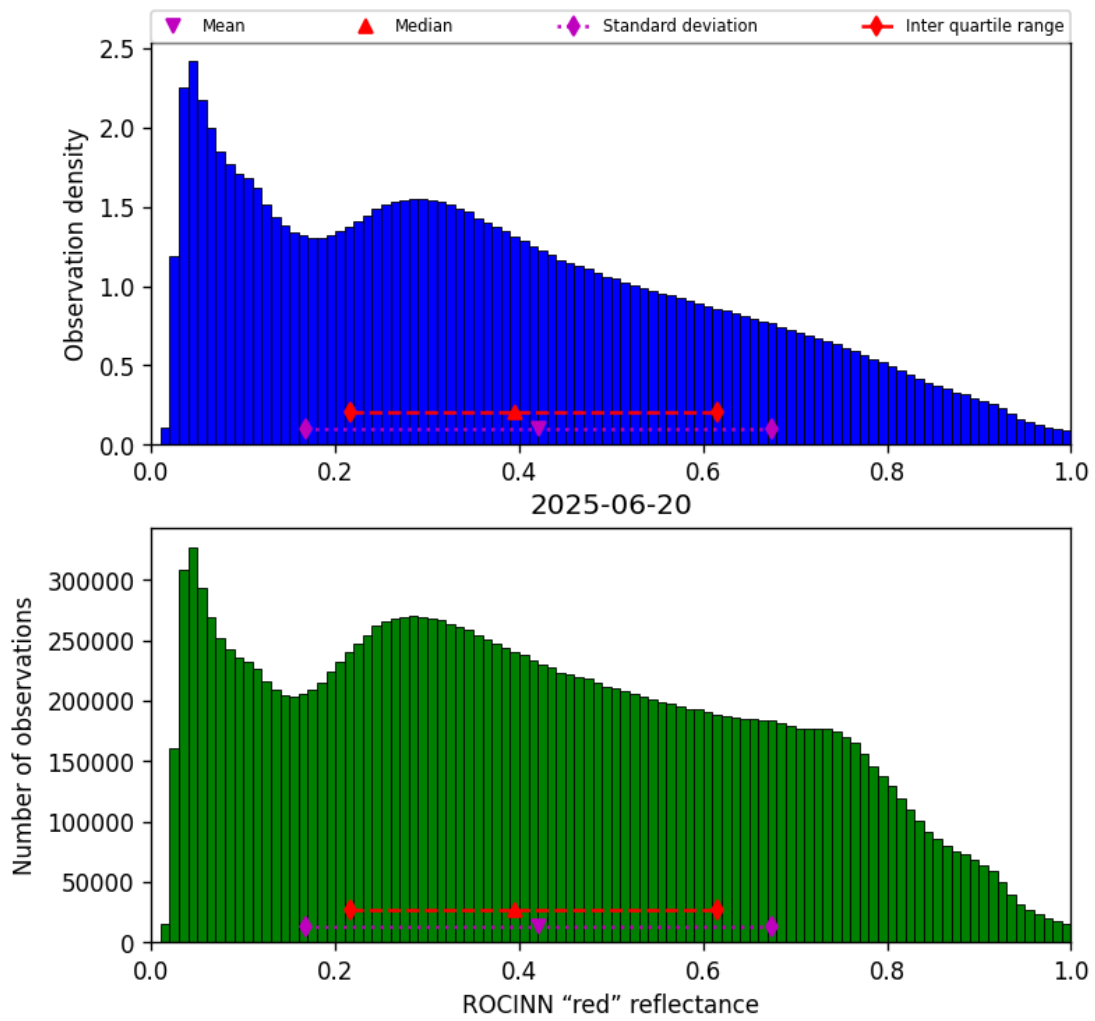
Figure 51: Histogram of “ROCINN “red” reflectance” for 2025-06-20 to 2025-06-20
