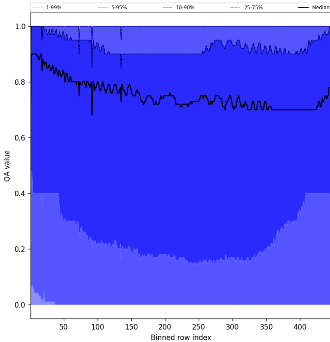
Figure 52: Along track statistics of “QA value” for 2025-06-20 to 2025-06-20
