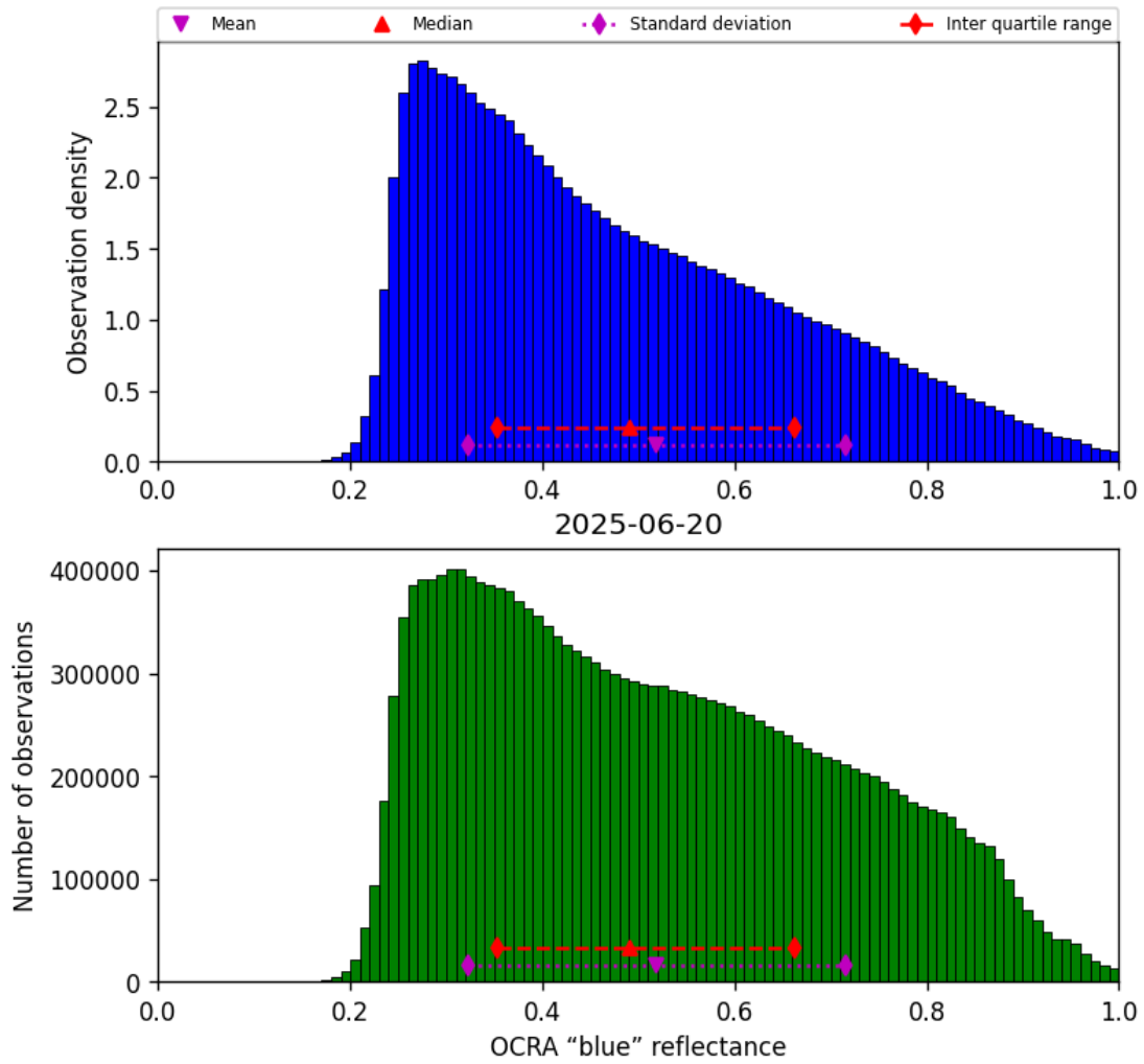
Figure 49: Histogram of “OCRA “blue” reflectance” for 2025-06-20 to 2025-06-20
