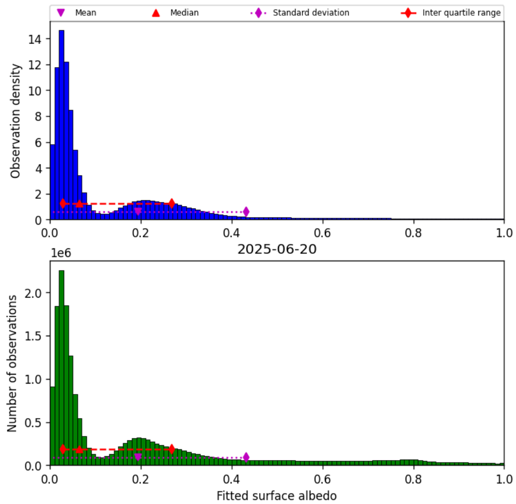
Figure 43: Histogram of “Fitted surface albedo” for 2025-06-20 to 2025-06-20
