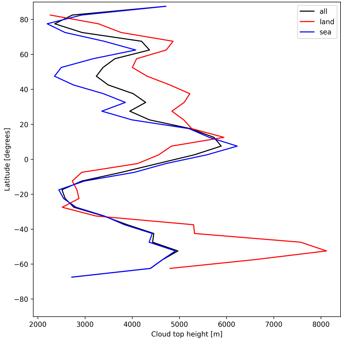
Figure 22: Zonal average of “Cloud top height” for 2025-06-20 to 2025-06-20.
