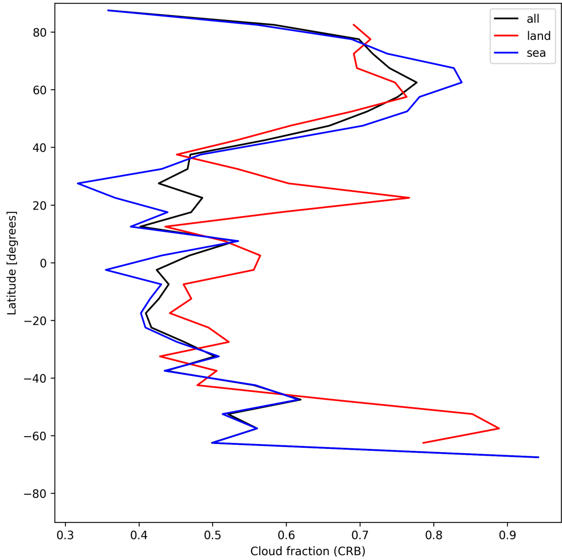
Figure 24: Zonal average of “Cloud fraction (CRB)” for 2025-06-20 to 2025-06-20.
