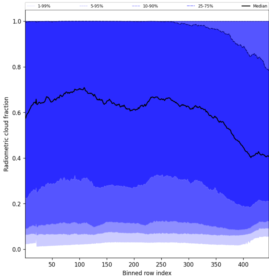
Figure 53: Along track statistics of “Radiometric cloud fraction” for 2025-06-20 to 2025-06-20
