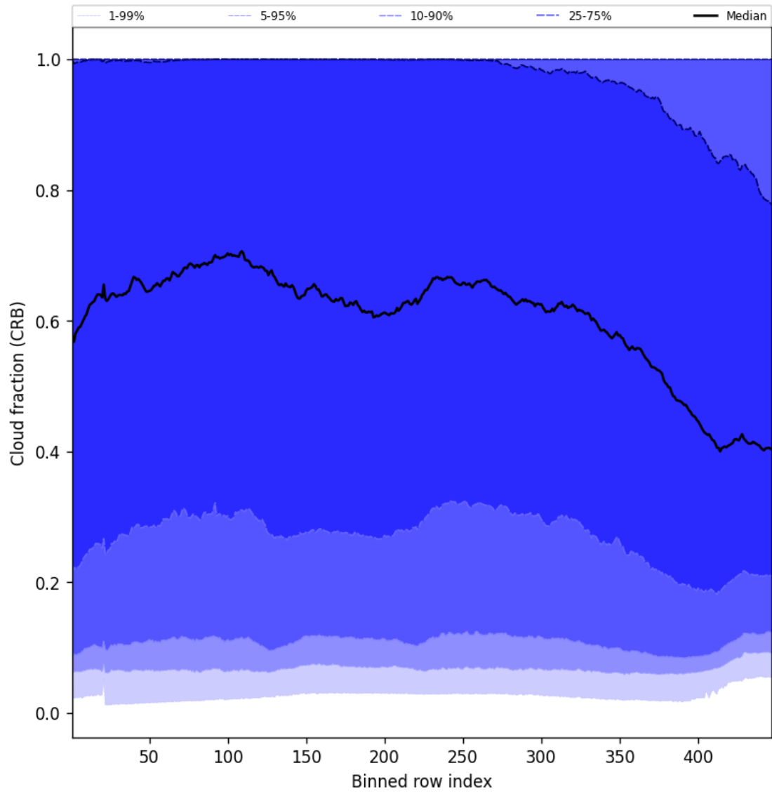
Figure 56: Along track statistics of “Cloud fraction (CRB)” for 2025-06-20 to 2025-06-20
