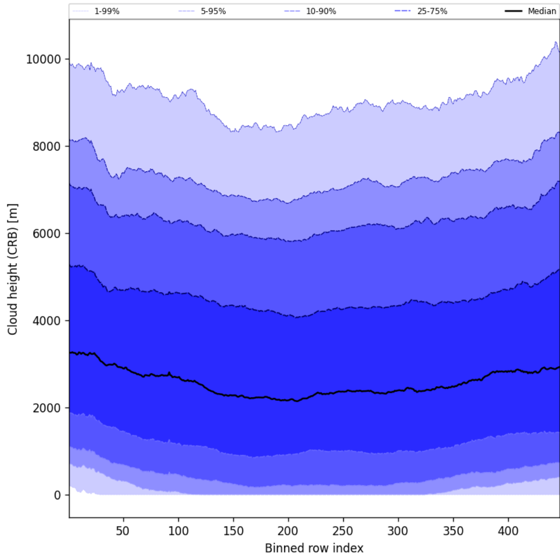
Figure 57: Along track statistics of “Cloud height (CRB)” for 2025-06-20 to 2025-06-20
