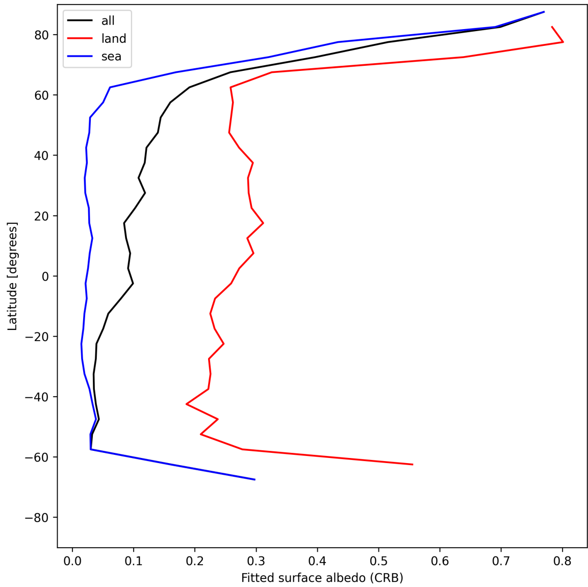
Figure 28: Zonal average of “Fitted surface albedo (CRB)” for 2025-06-20 to 2025-06-20.
