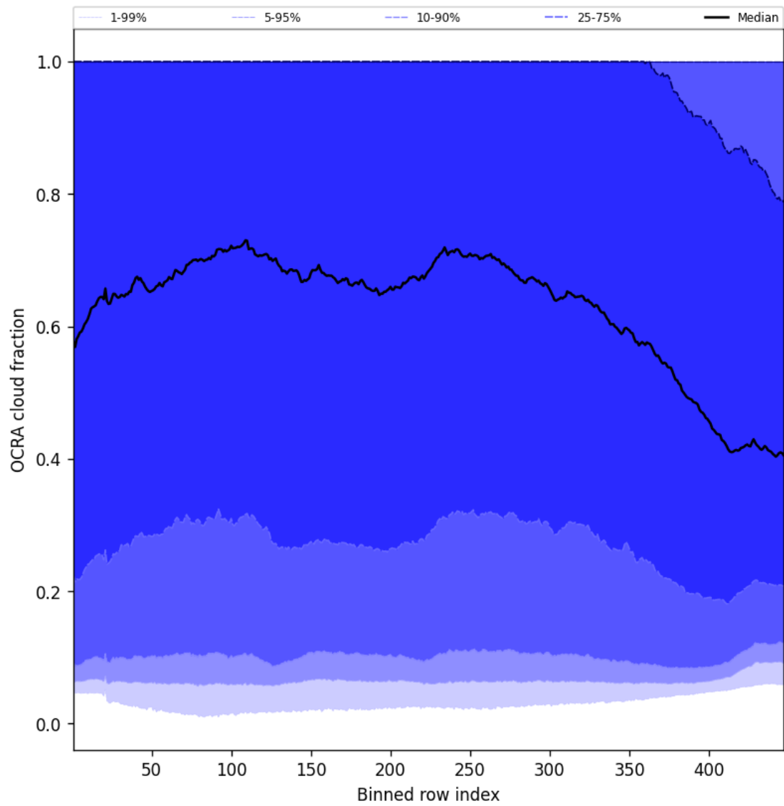
Figure 64: Along track statistics of “OCRA cloud fraction” for 2025-06-20 to 2025-06-20
