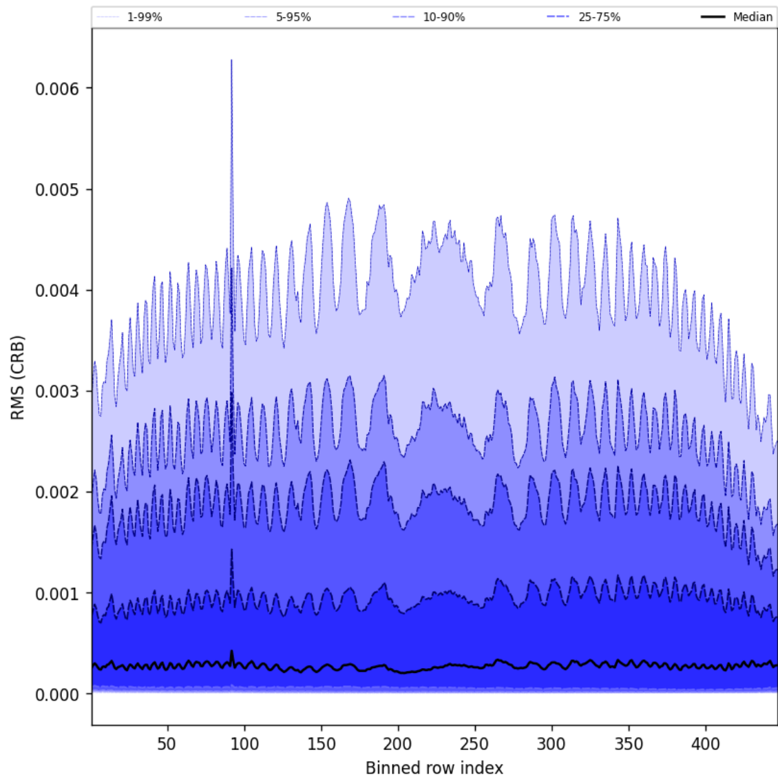
Figure 62: Along track statistics of “RMS (CRB)” for 2025-06-20 to 2025-06-20
