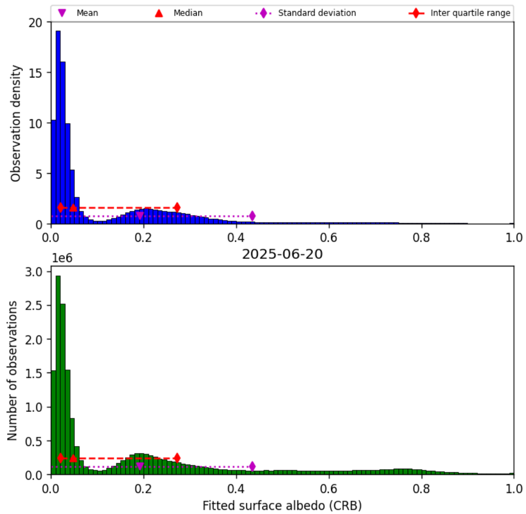
Figure 44: Histogram of “Fitted surface albedo (CRB)” for 2025-06-20 to 2025-06-20
