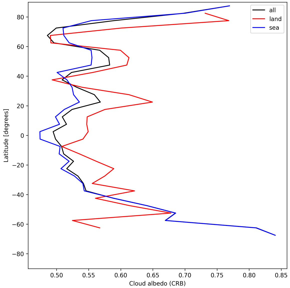
Figure 26: Zonal average of “Cloud albedo (CRB)” for 2025-06-20 to 2025-06-20.
