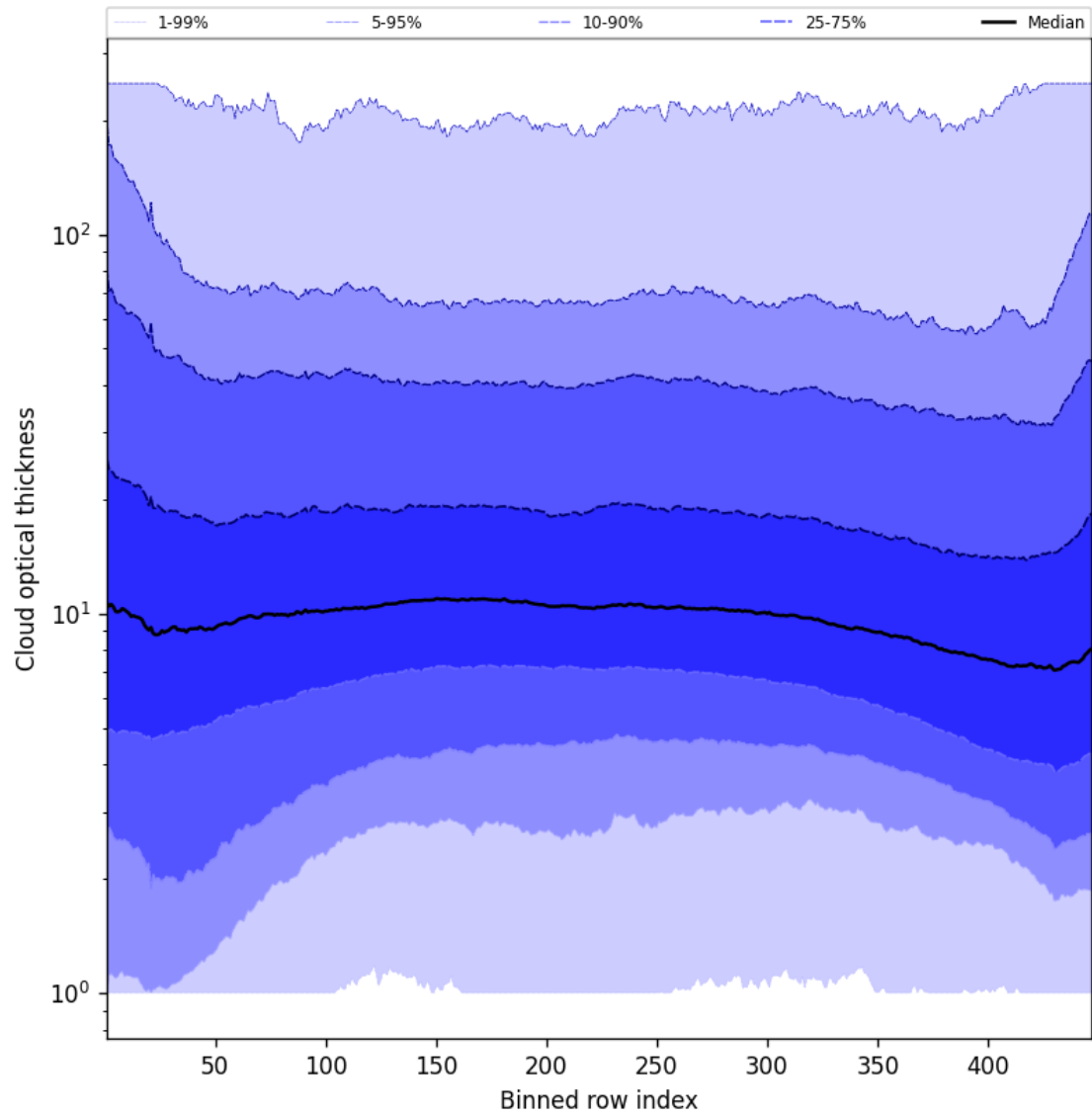
Figure 55: Along track statistics of “Cloud optical thickness” for 2025-06-20 to 2025-06-20
