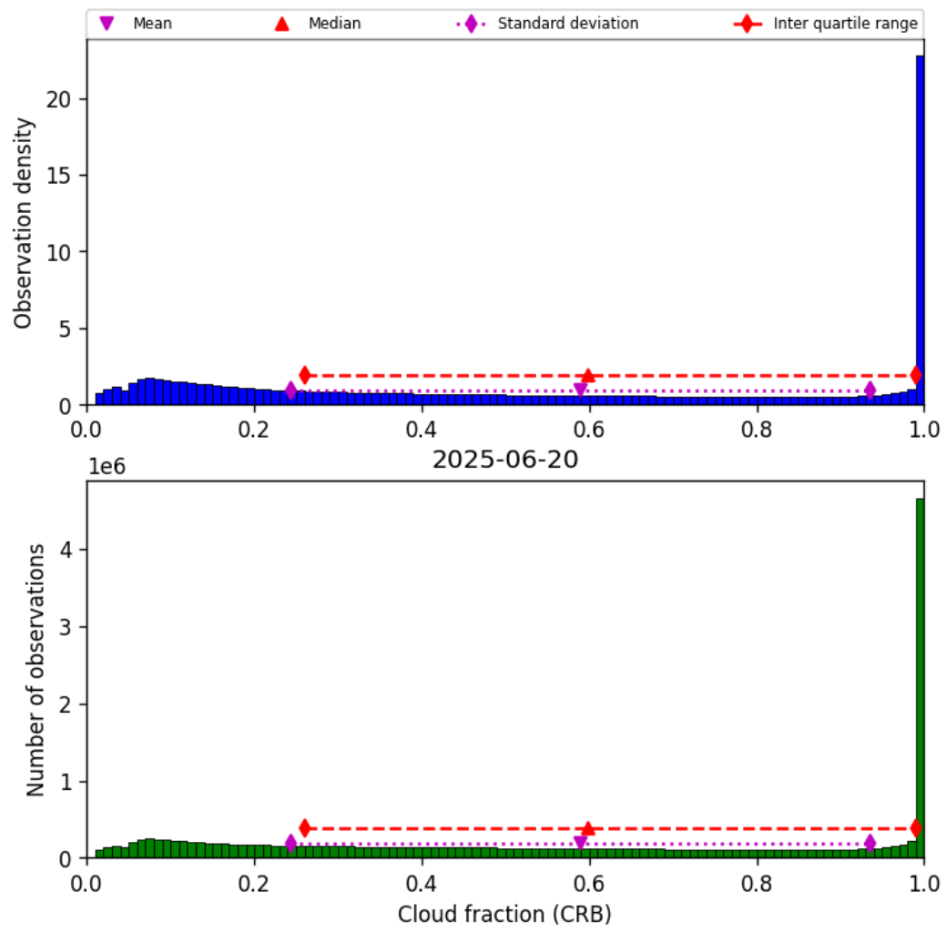
Figure 40: Histogram of “Cloud fraction (CRB)” for 2025-06-20 to 2025-06-20
