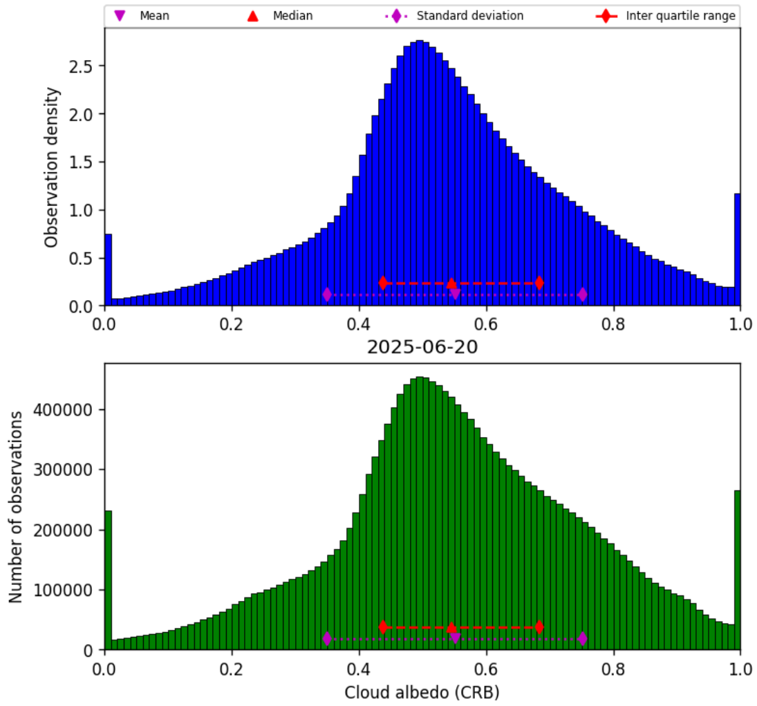
Figure 42: Histogram of “Cloud albedo (CRB)” for 2025-06-20 to 2025-06-20
