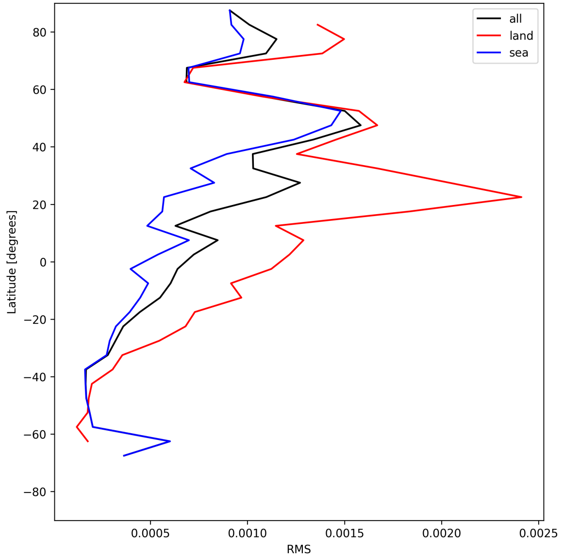
Figure 29: Zonal average of “RMS” for 2025-06-20 to 2025-06-20.
