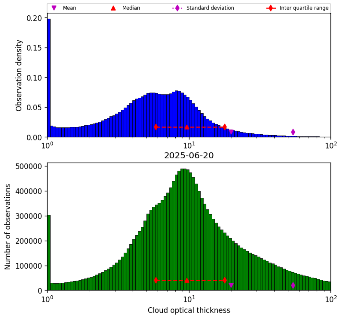
Figure 39: Histogram of “Cloud optical thickness” for 2025-06-20 to 2025-06-20
