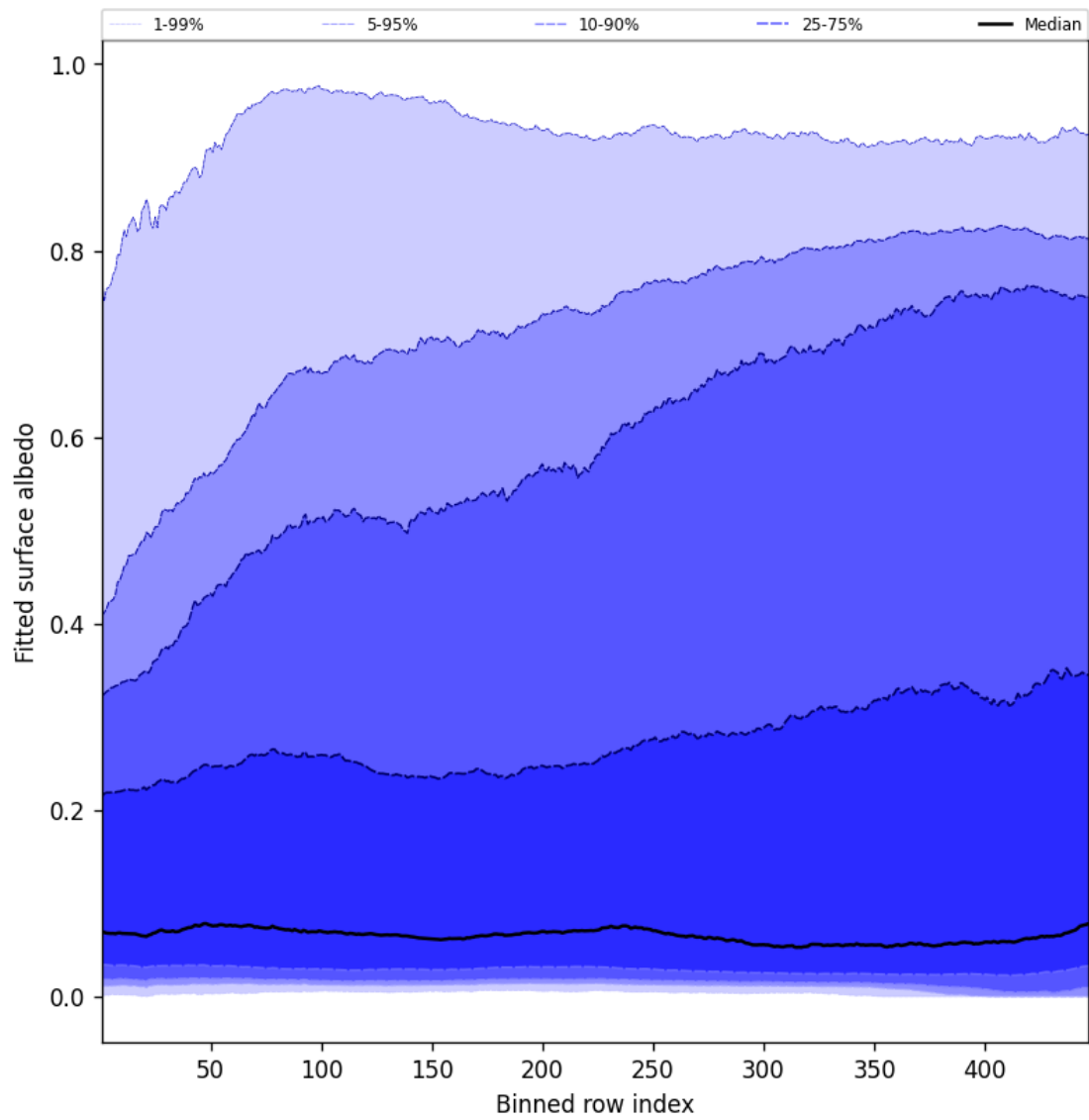
Figure 59: Along track statistics of “Fitted surface albedo” for 2025-06-20 to 2025-06-20
