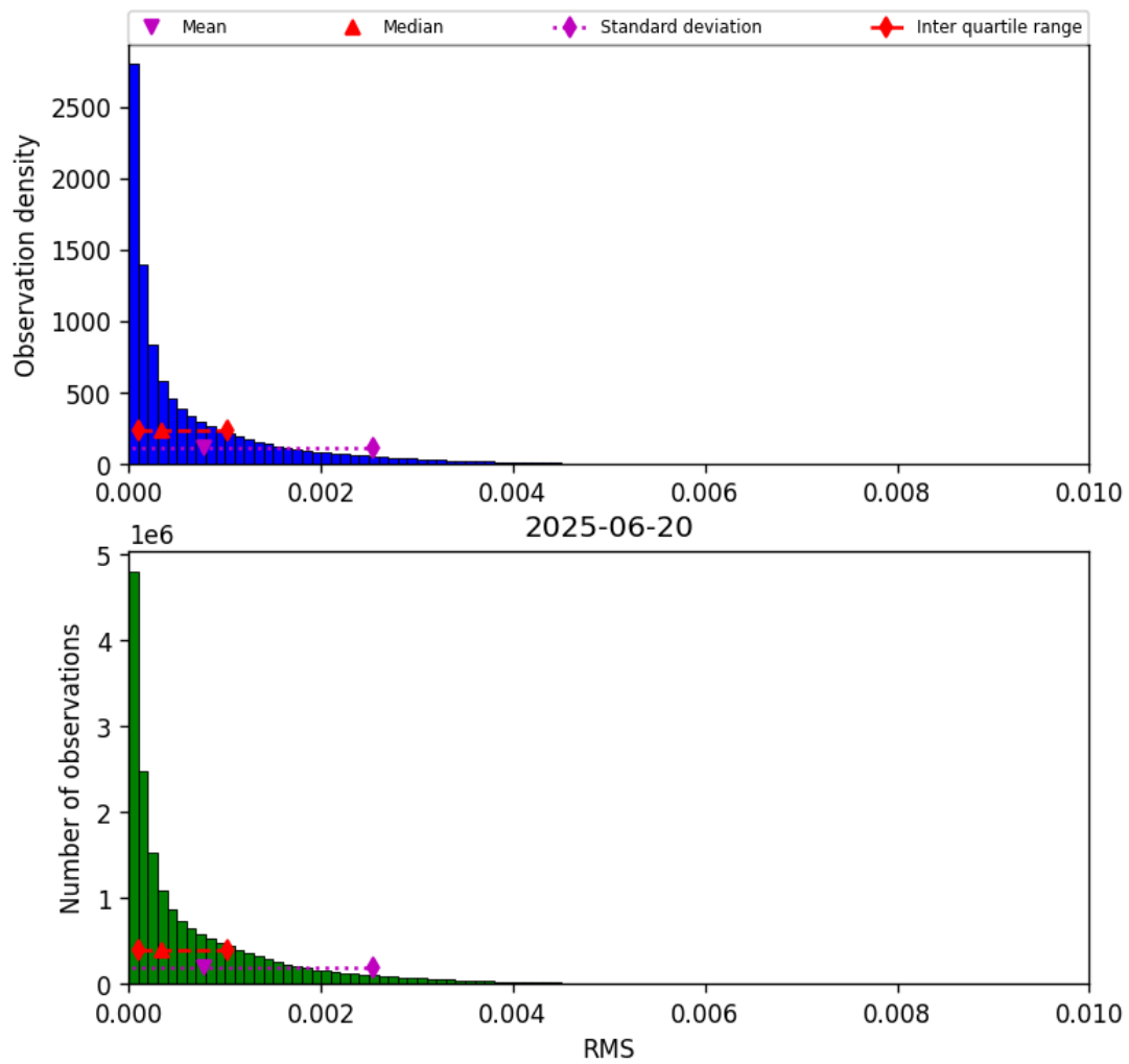
Figure 45: Histogram of “RMS” for 2025-06-20 to 2025-06-20
