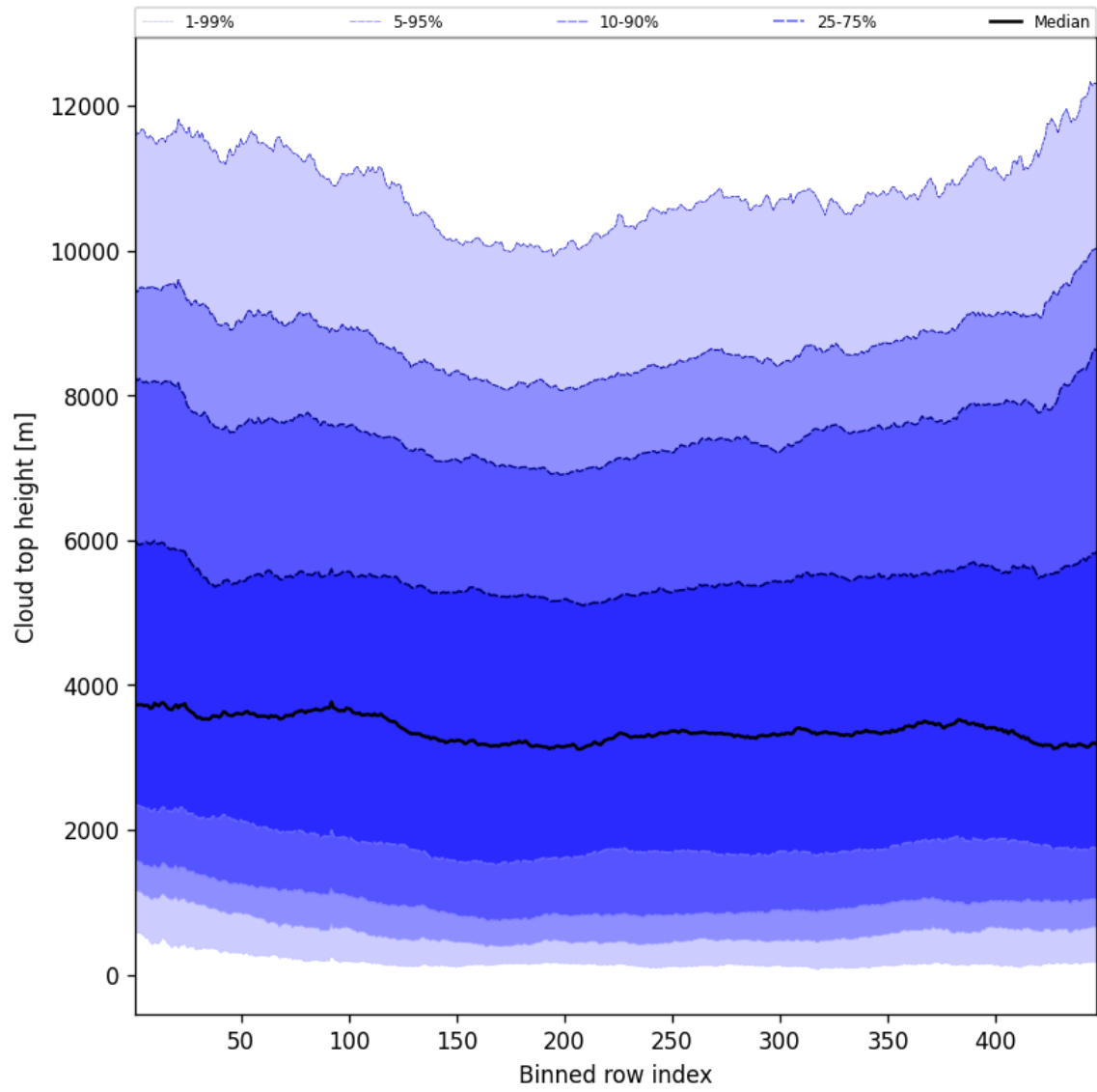
Figure 54: Along track statistics of “Cloud top height” for 2025-06-20 to 2025-06-20
