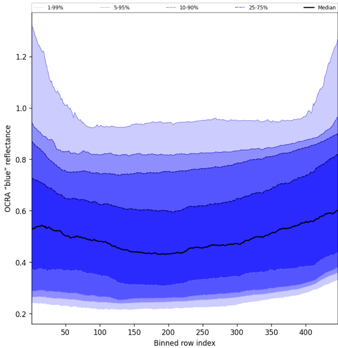
Figure 65: Along track statistics of “OCRA “blue” reflectance” for 2025-06-20 to 2025-06-20
