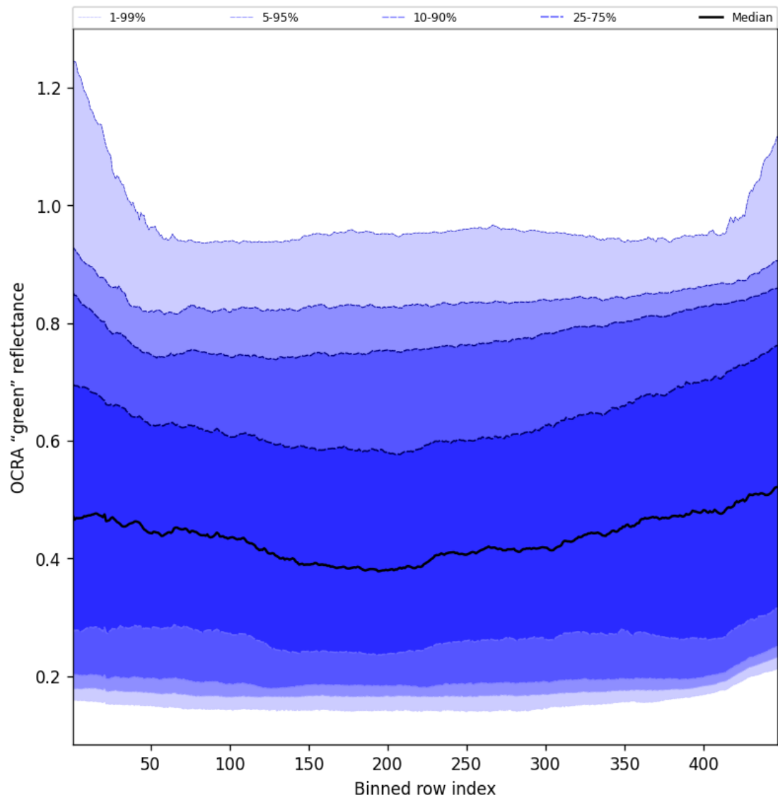
Figure 66: Along track statistics of "OCRA "green" reflectance" for 2025-06-20 to 2025-06-20
