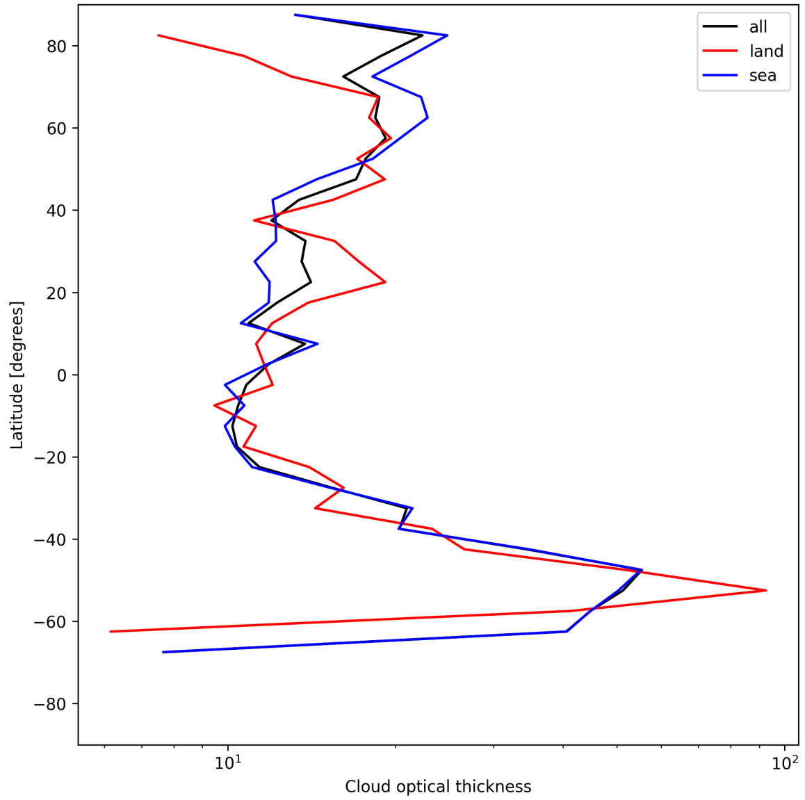
Figure 23: Zonal average of “Cloud optical thickness” for 2025-06-20 to 2025-06-20.
