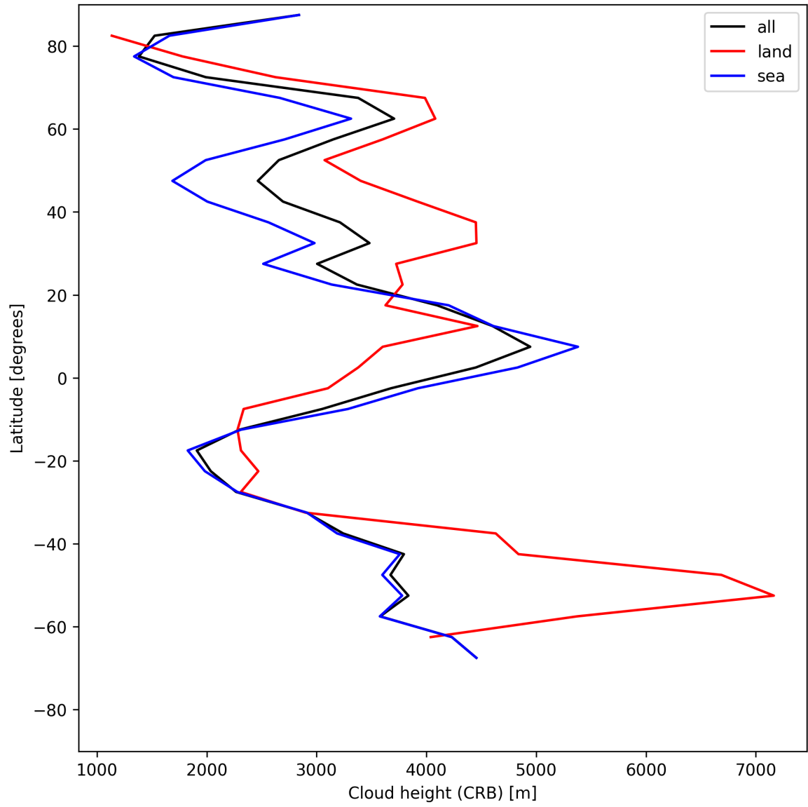
Figure 25: Zonal average of “Cloud height (CRB)” for 2025-06-20 to 2025-06-20.
