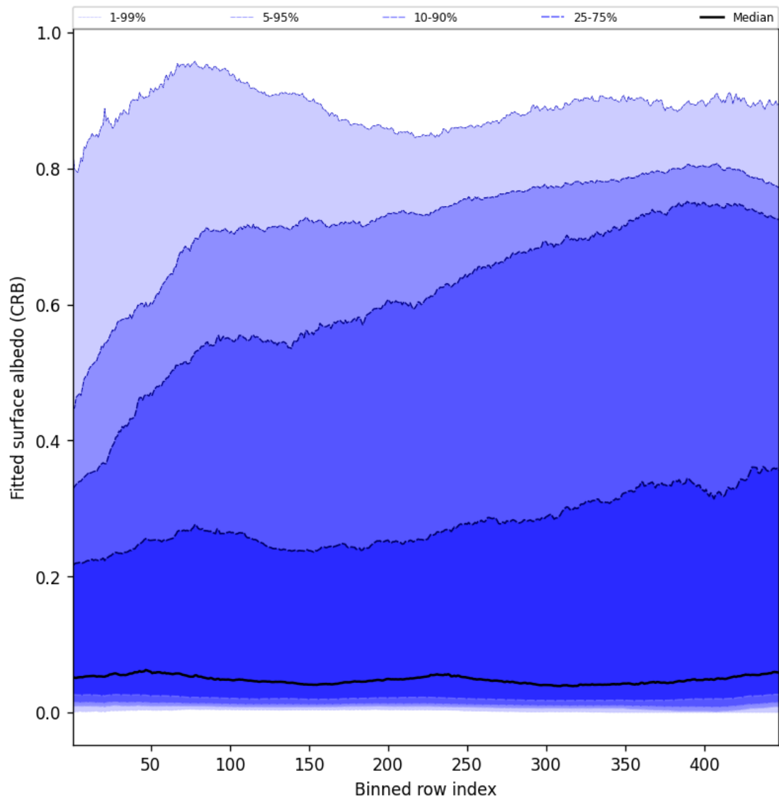
Figure 60: Along track statistics of “Fitted surface albedo (CRB)” for 2025-06-20 to 2025-06-20
