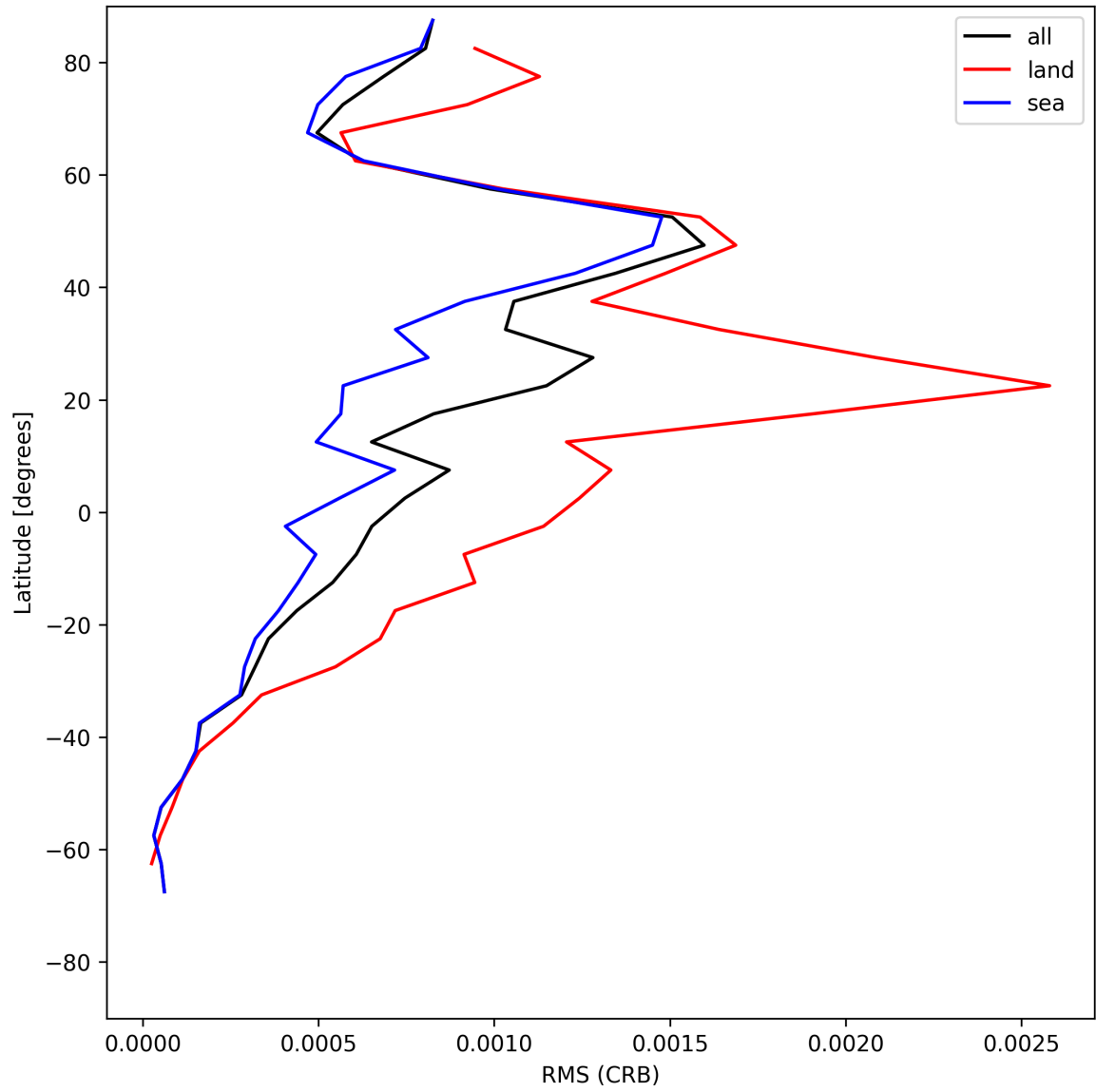
Figure 30: Zonal average of “RMS (CRB)” for 2025-06-20 to 2025-06-20.
