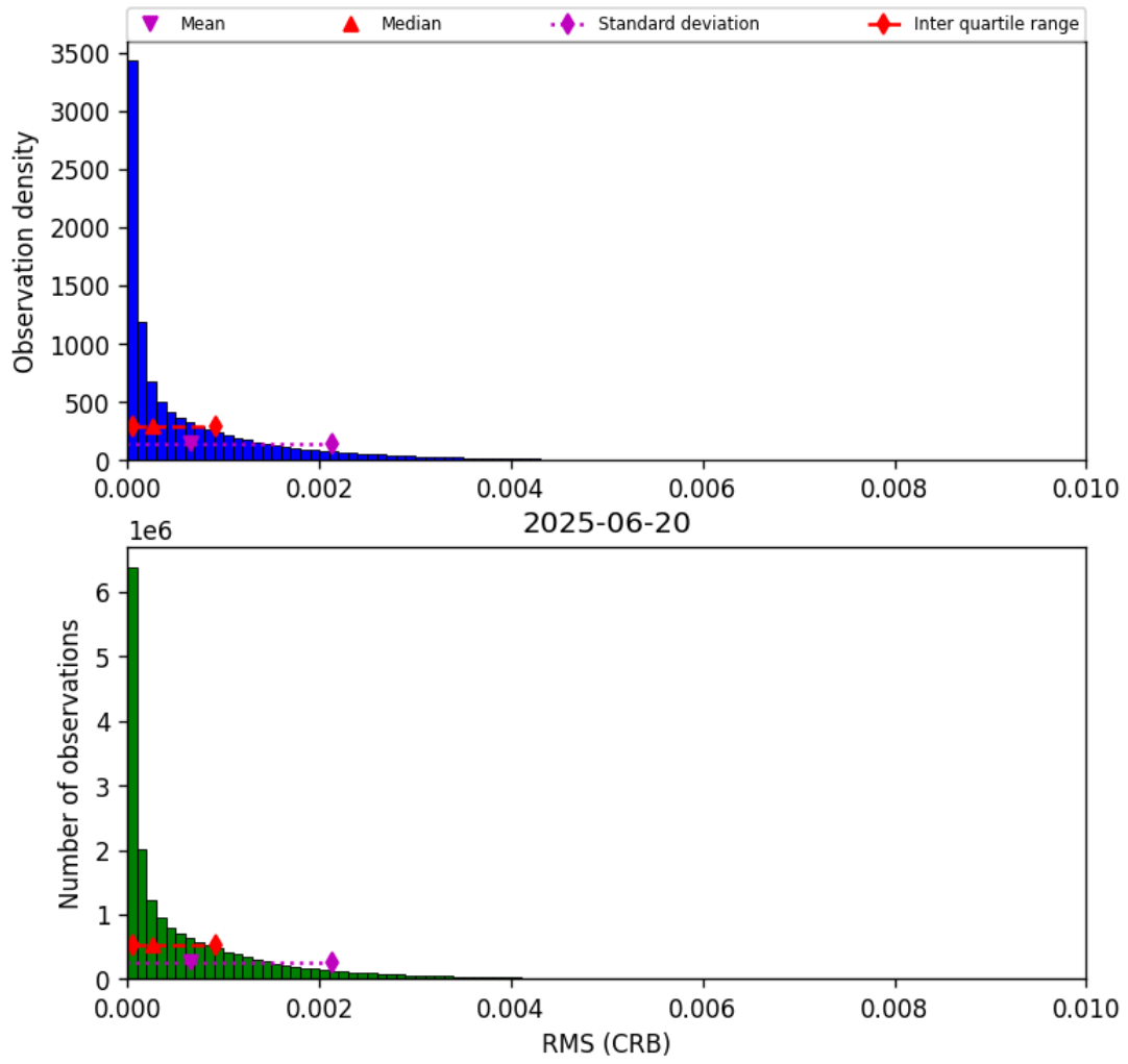
Figure 46: Histogram of “RMS (CRB)” for 2025-06-20 to 2025-06-20
