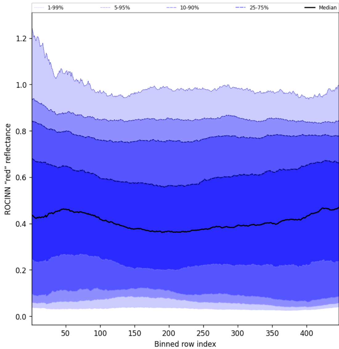
Figure 67: Along track statistics of “ROCINN “red” reflectance” for 2025-06-22 to 2025-06-23
