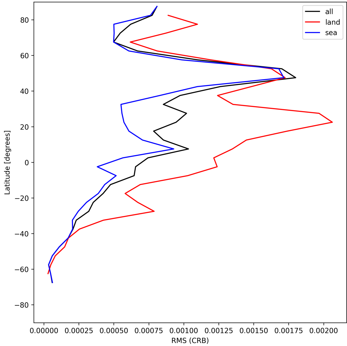
Figure 30: Zonal average of “RMS (CRB)” for 2025-06-22 to 2025-06-23.
