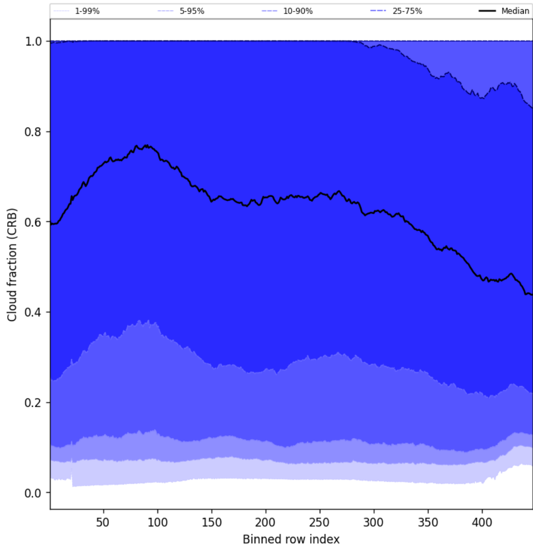
Figure 56: Along track statistics of “Cloud fraction (CRB)” for 2025-06-22 to 2025-06-23
