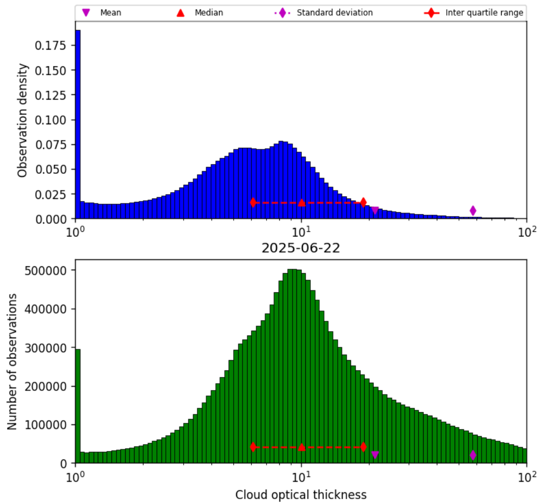
Figure 39: Histogram of “Cloud optical thickness” for 2025-06-22 to 2025-06-23
