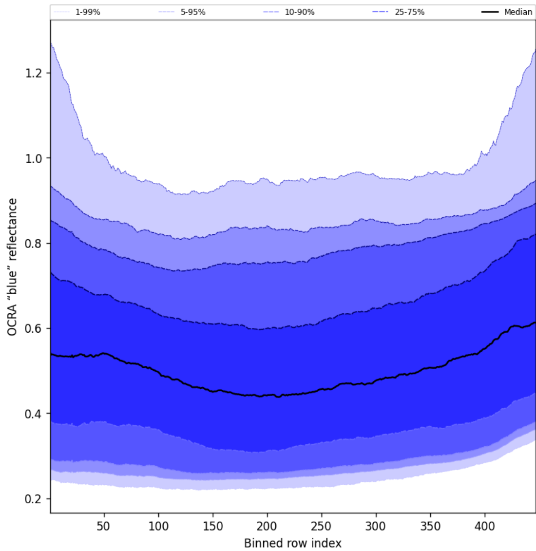
Figure 65: Along track statistics of “OCRA “blue” reflectance” for 2025-06-22 to 2025-06-23
