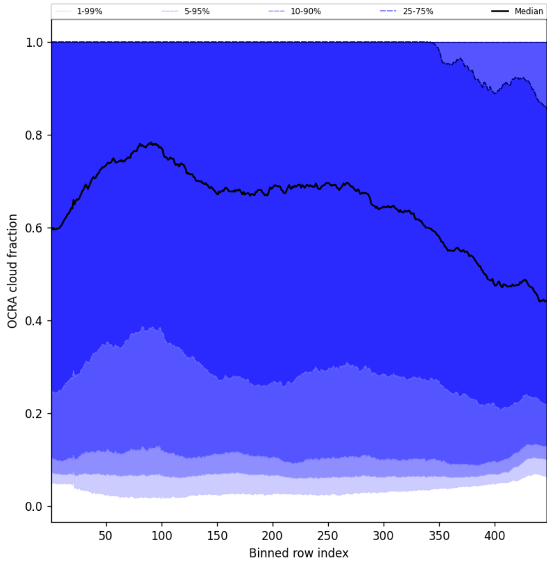
Figure 64: Along track statistics of “OCRA cloud fraction” for 2025-06-22 to 2025-06-23
