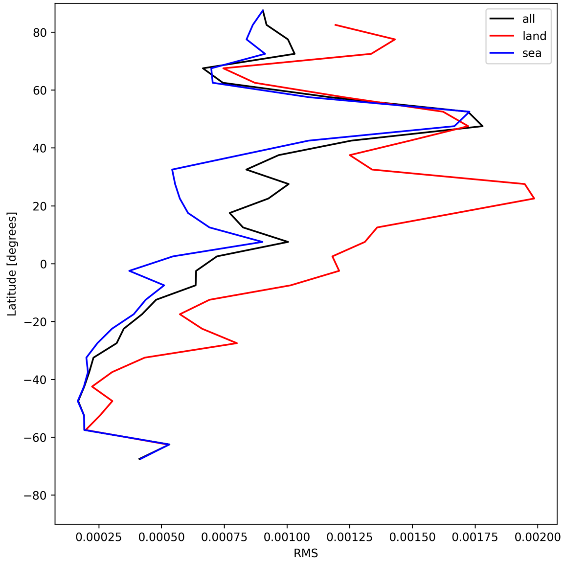
Figure 29: Zonal average of “RMS” for 2025-06-22 to 2025-06-23.
