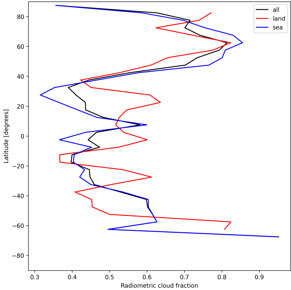
Figure 21: Zonal average of “Radiometric cloud fraction” for 2025-06-22 to 2025-06-23.
