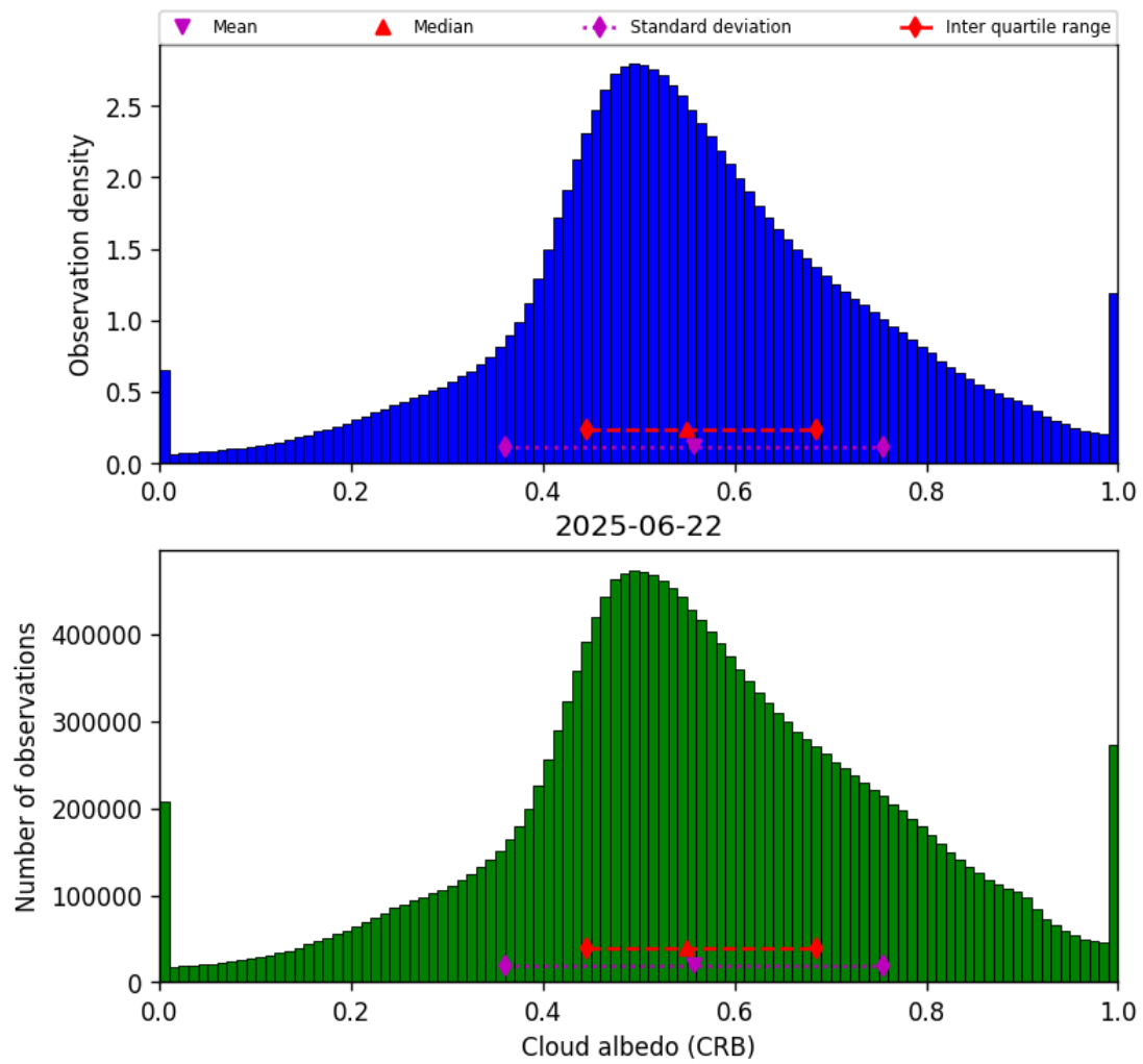
Figure 42: Histogram of “Cloud albedo (CRB)” for 2025-06-22 to 2025-06-23
