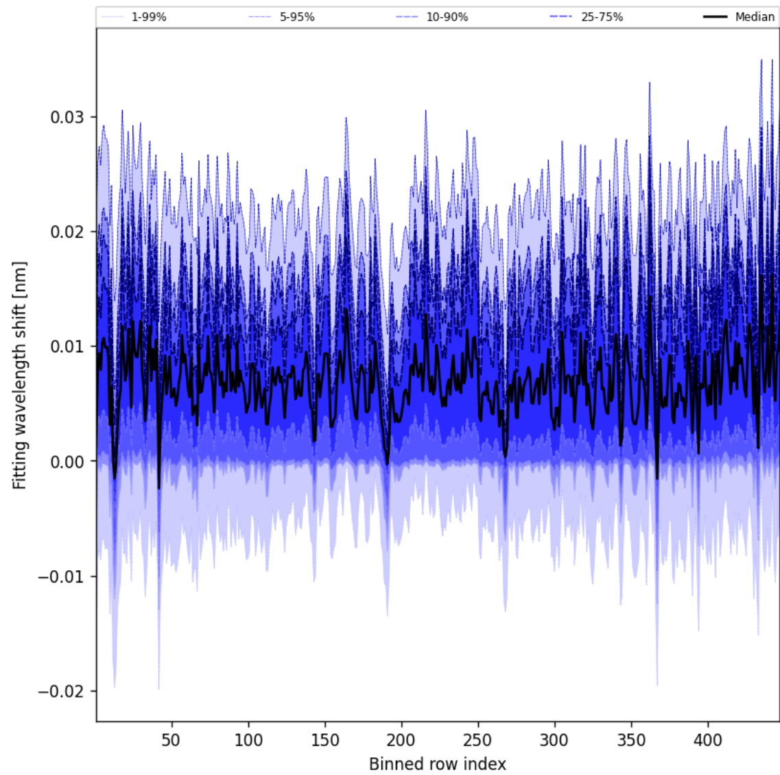
Figure 63: Along track statistics of “Fitting wavelength shift” for 2025-06-22 to 2025-06-23
