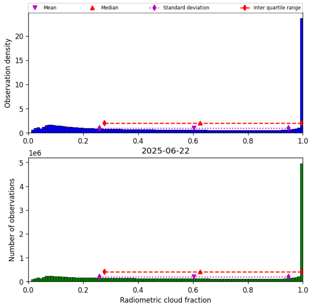
Figure 37: Histogram of “Radiometric cloud fraction” for 2025-06-22 to 2025-06-23
