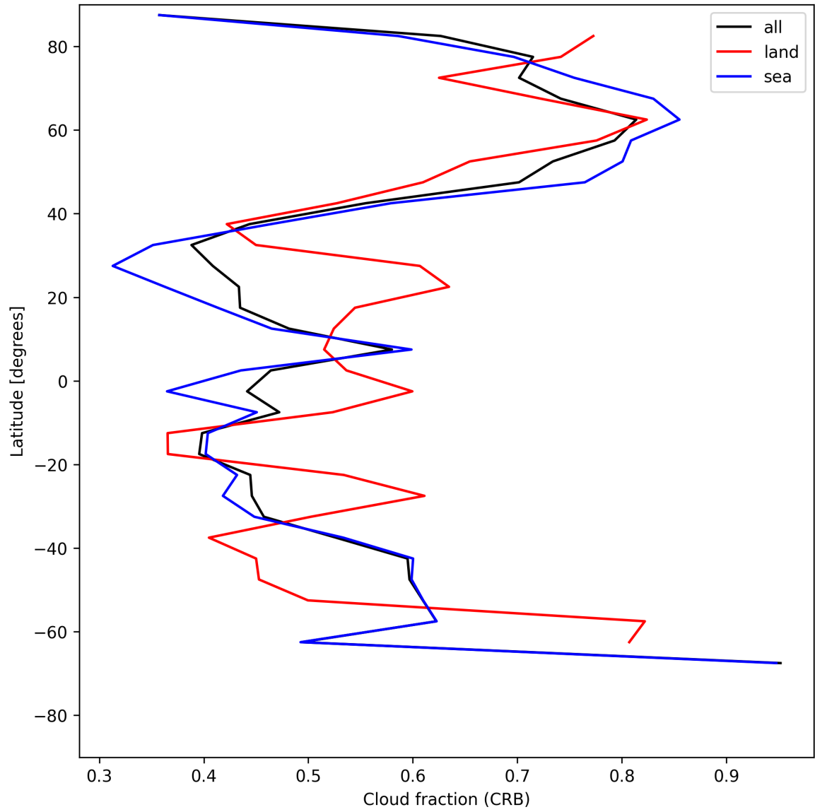
Figure 24: Zonal average of “Cloud fraction (CRB)” for 2025-06-22 to 2025-06-23.
