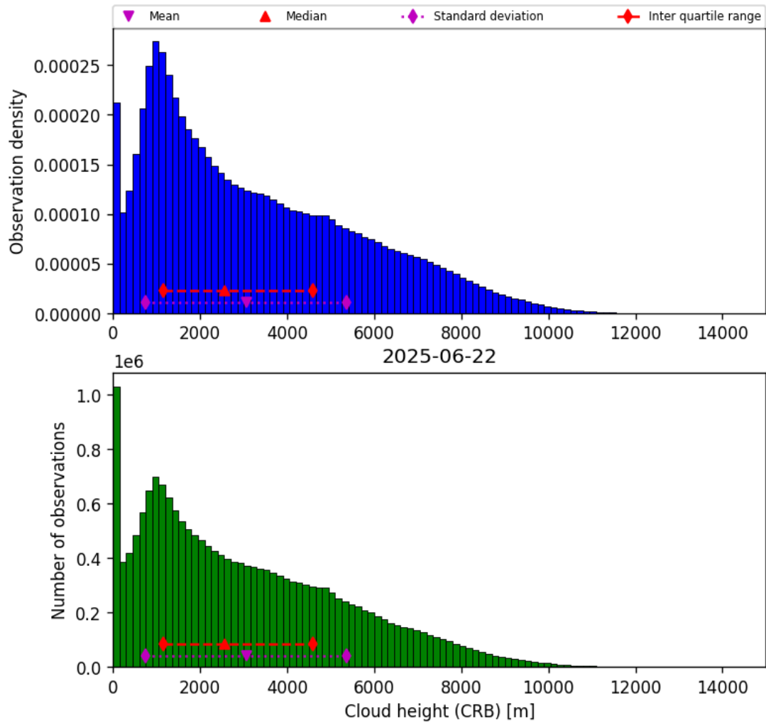
Figure 41: Histogram of “Cloud height (CRB)” for 2025-06-22 to 2025-06-23
