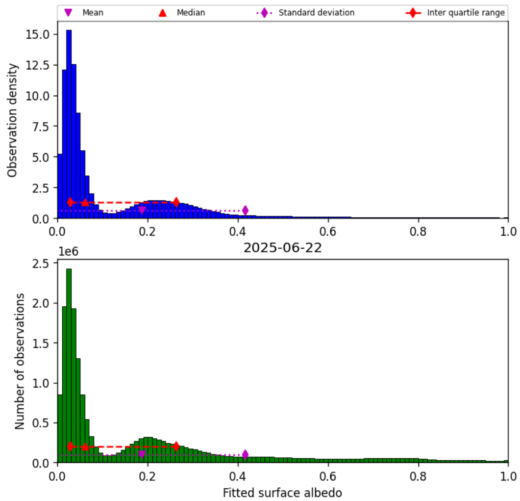
Figure 43: Histogram of “Fitted surface albedo” for 2025-06-22 to 2025-06-23
