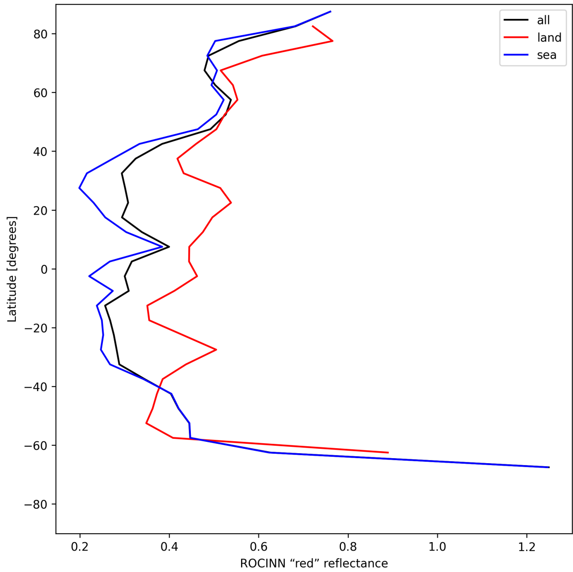
Figure 35: Zonal average of “ROCINN “red” reflectance” for 2025-06-22 to 2025-06-23.
