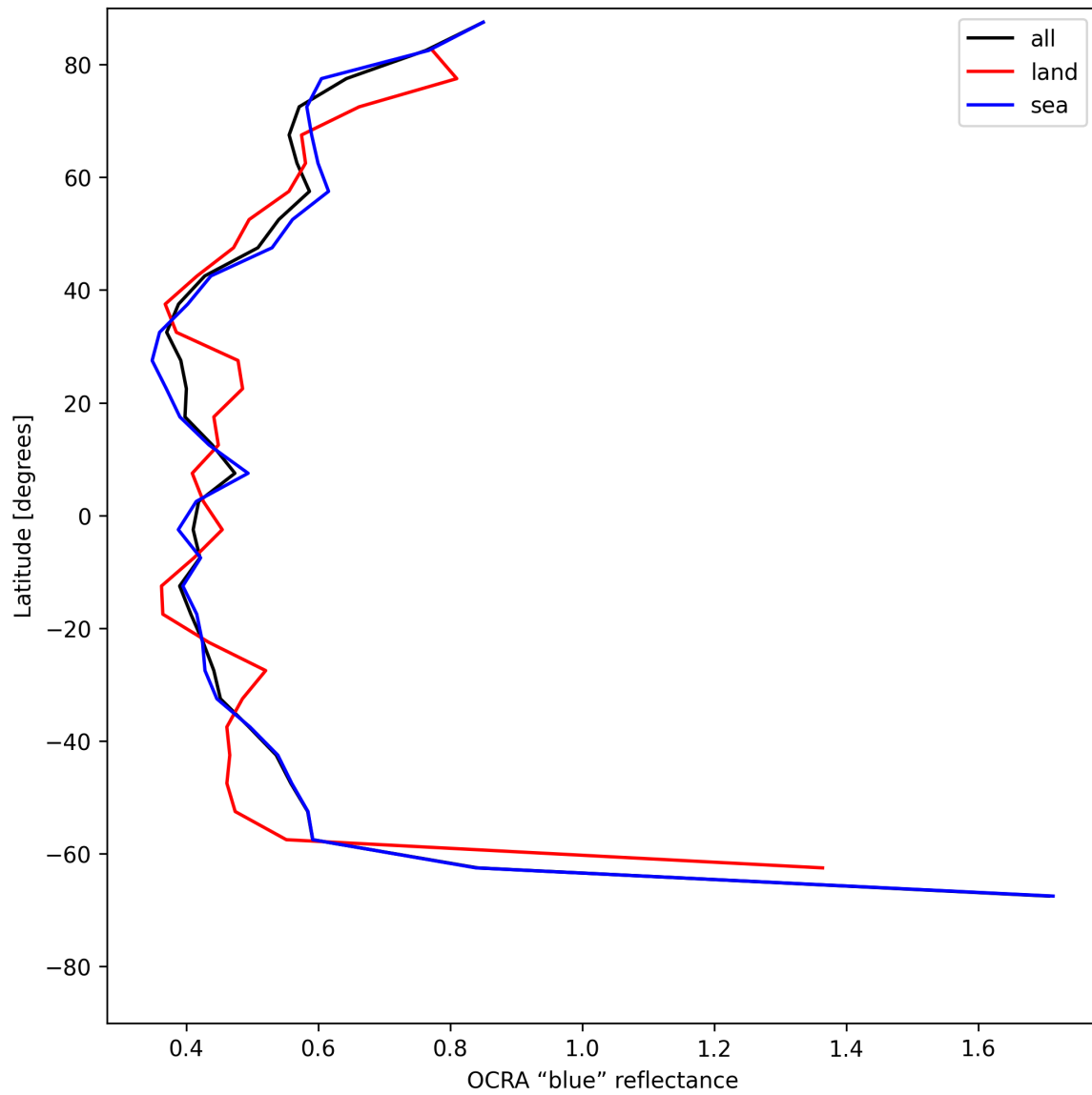
Figure 33: Zonal average of “OCRA “blue” reflectance” for 2025-06-22 to 2025-06-23.
