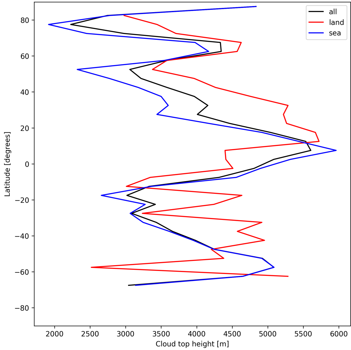
Figure 22: Zonal average of “Cloud top height” for 2025-06-22 to 2025-06-23.
