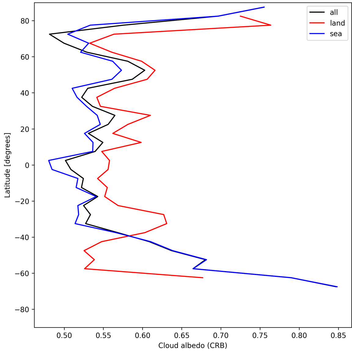
Figure 26: Zonal average of “Cloud albedo (CRB)” for 2025-06-22 to 2025-06-23.
