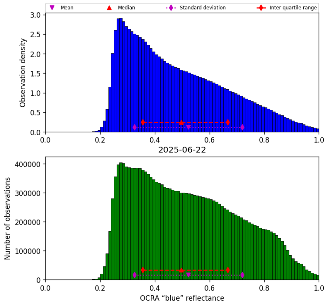
Figure 49: Histogram of “OCRA “blue” reflectance” for 2025-06-22 to 2025-06-23
