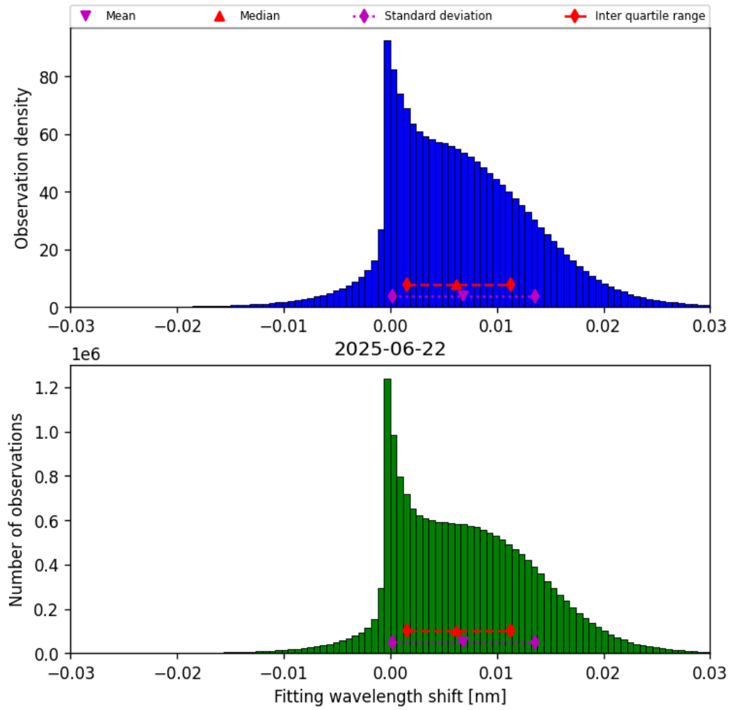
Figure 47: Histogram of “Fitting wavelength shift” for 2025-06-22 to 2025-06-23
