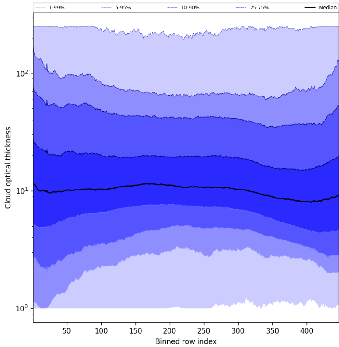
Figure 55: Along track statistics of “Cloud optical thickness” for 2025-06-22 to 2025-06-23
