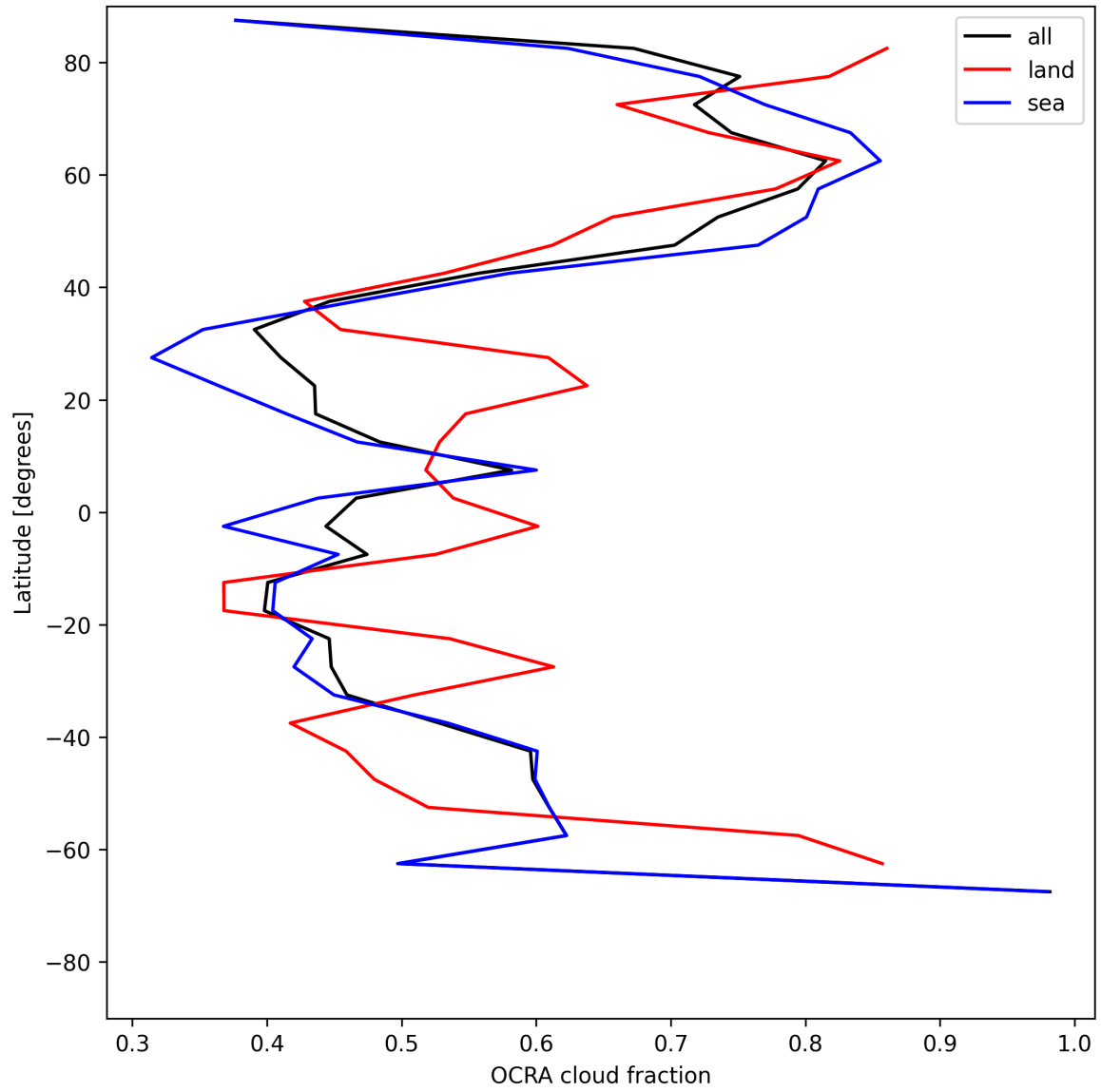
Figure 32: Zonal average of “OCRA cloud fraction” for 2025-06-22 to 2025-06-23.
