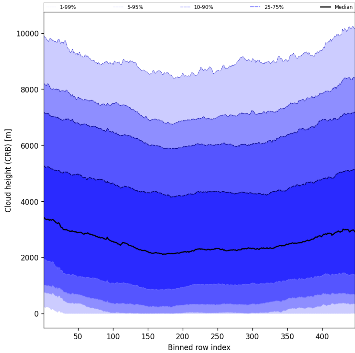
Figure 57: Along track statistics of “Cloud height (CRB)” for 2025-06-22 to 2025-06-23
