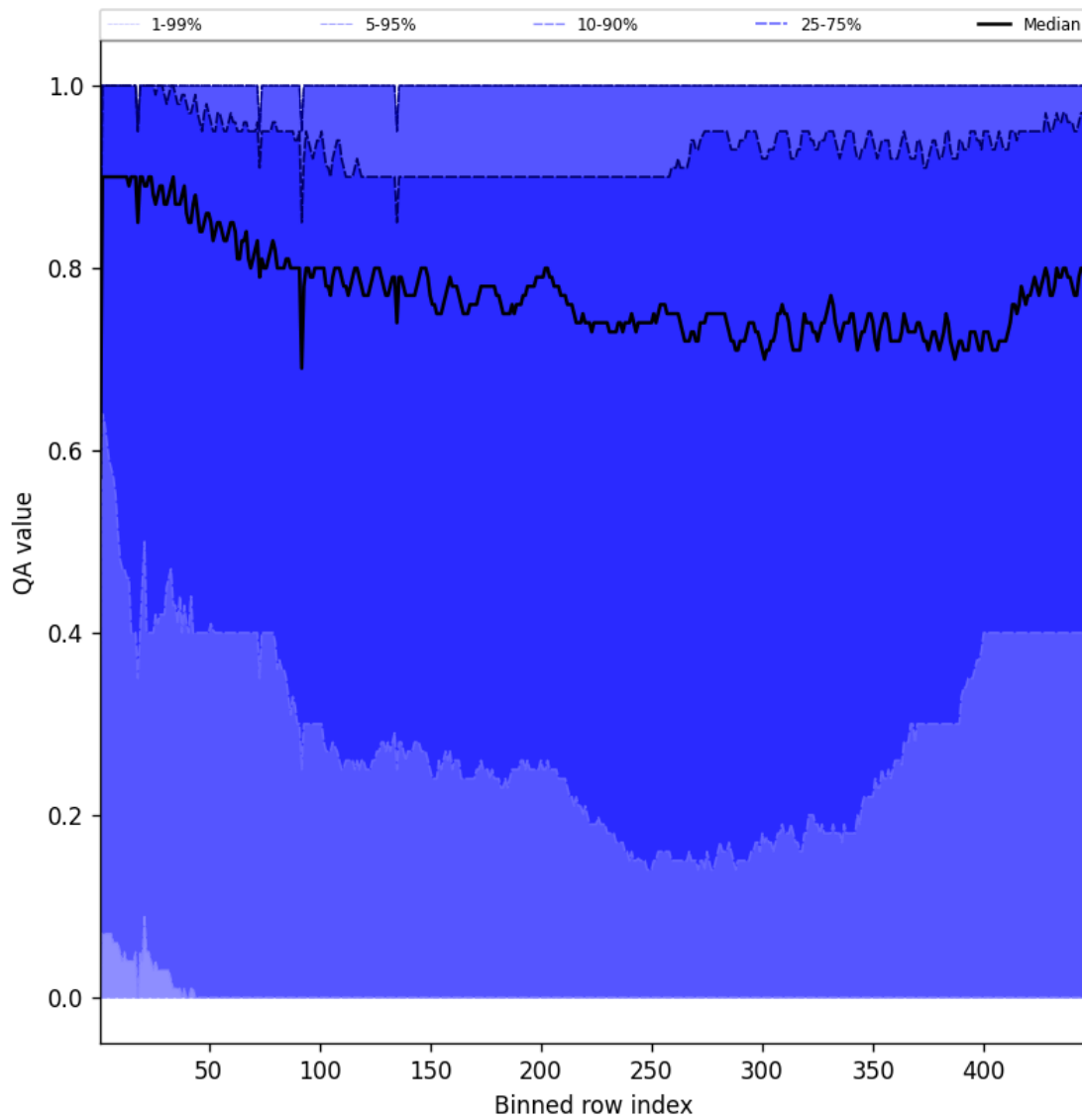
Figure 52: Along track statistics of “QA value” for 2025-06-22 to 2025-06-23
