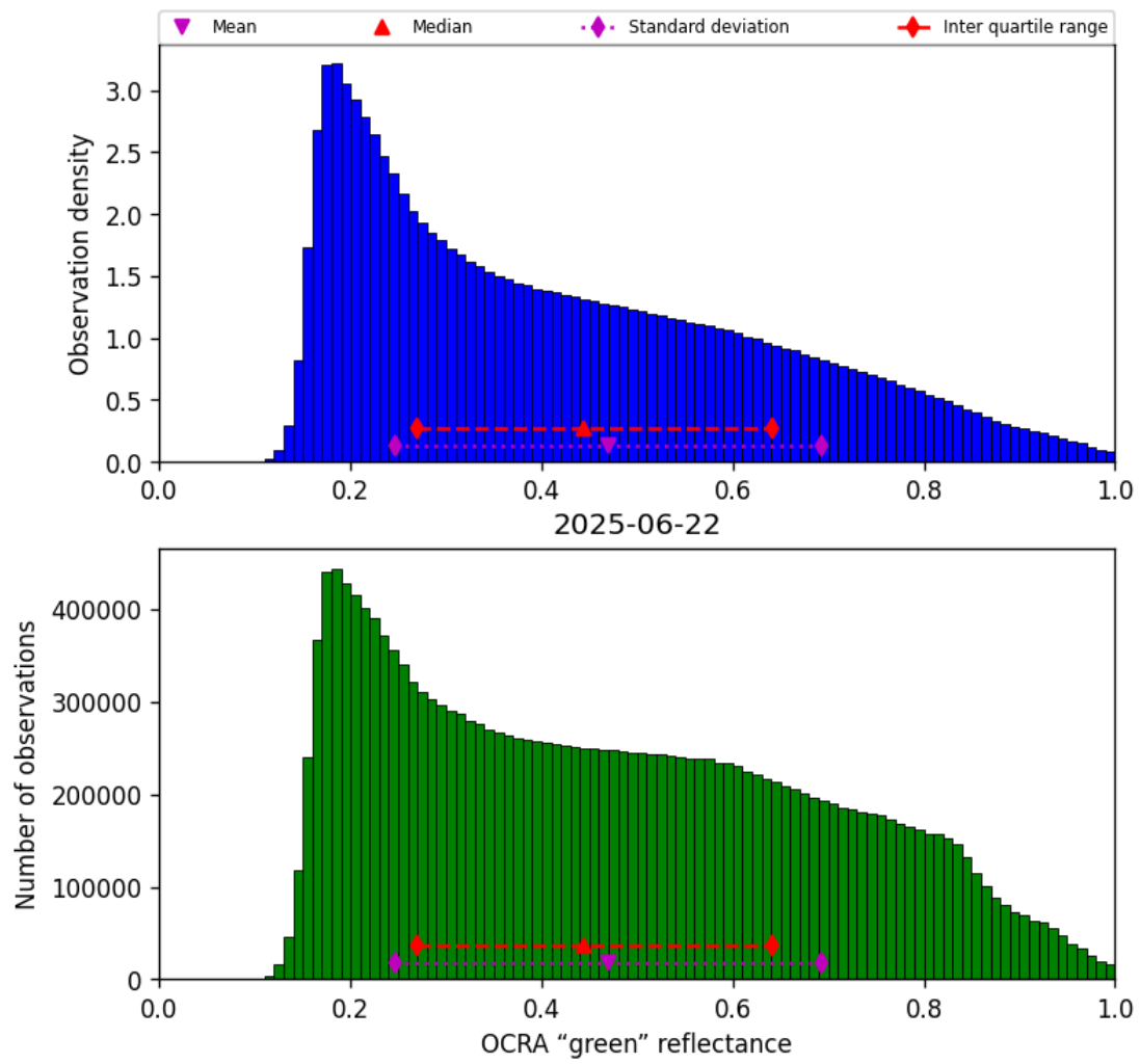
Figure 50: Histogram of “OCRA “green” reflectance” for 2025-06-22 to 2025-06-23
