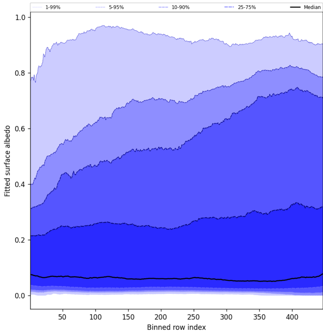
Figure 59: Along track statistics of “Fitted surface albedo” for 2025-06-22 to 2025-06-23
