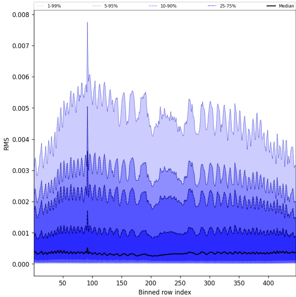
Figure 61: Along track statistics of “RMS” for 2025-06-22 to 2025-06-23
