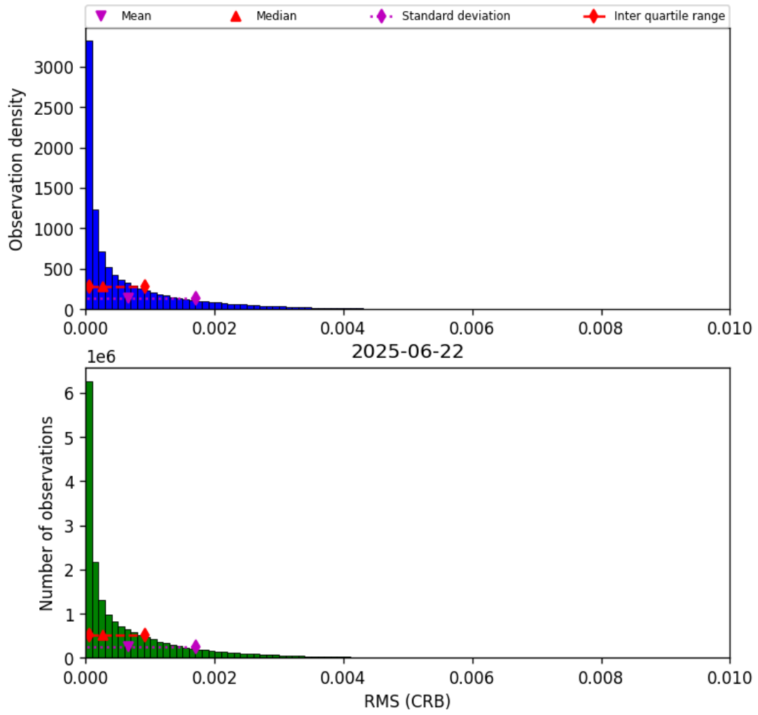
Figure 46: Histogram of “RMS (CRB)” for 2025-06-22 to 2025-06-23
