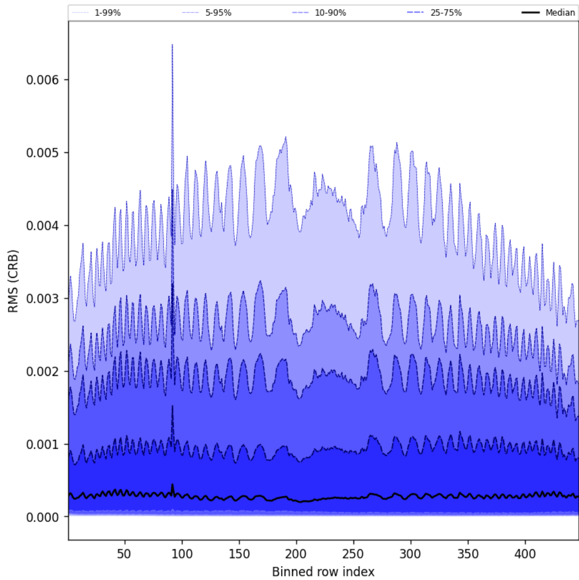
Figure 62: Along track statistics of “RMS (CRB)” for 2025-06-22 to 2025-06-23
