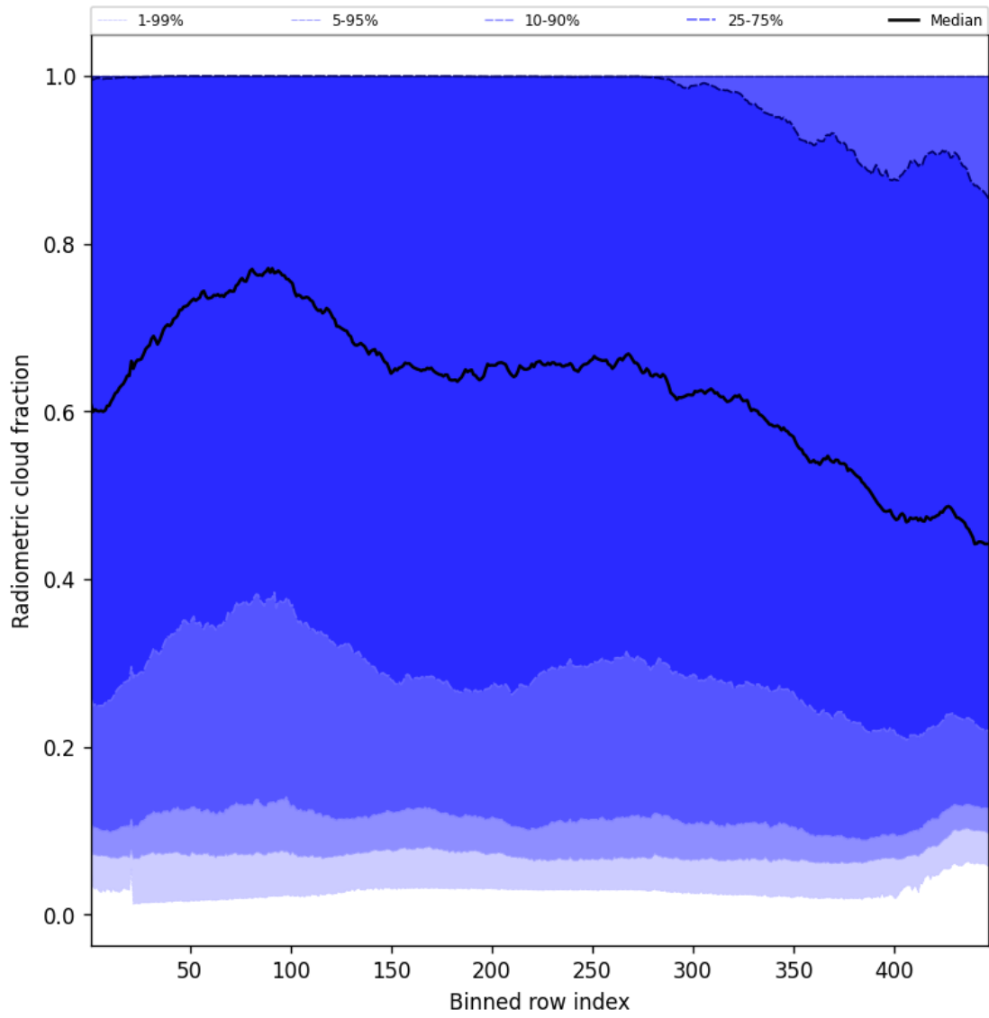
Figure 53: Along track statistics of “Radiometric cloud fraction” for 2025-06-22 to 2025-06-23
