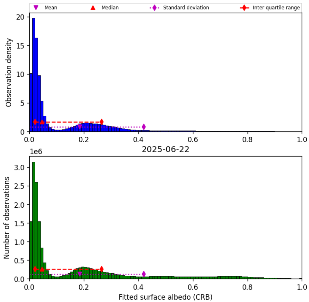
Figure 44: Histogram of “Fitted surface albedo (CRB)” for 2025-06-22 to 2025-06-23
