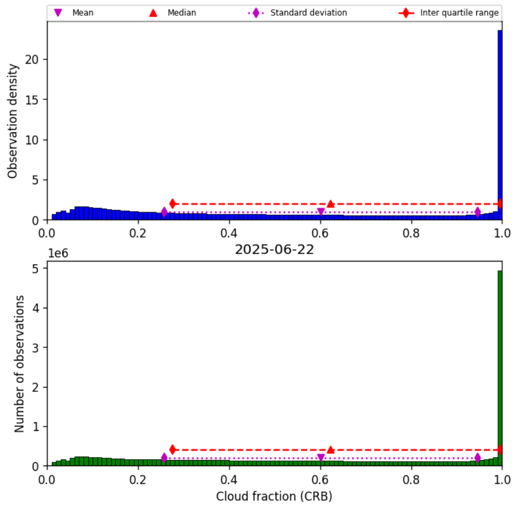
Figure 40: Histogram of “Cloud fraction (CRB)” for 2025-06-22 to 2025-06-23
