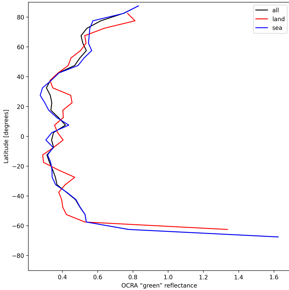
Figure 34: Zonal average of “OCRA “green” reflectance” for 2025-06-22 to 2025-06-23.
