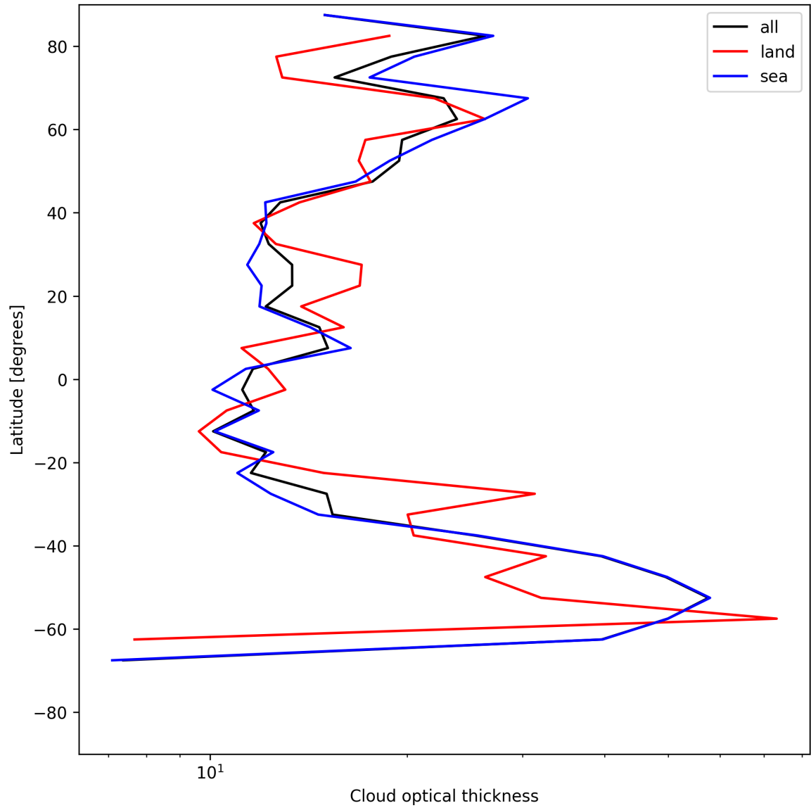
Figure 23: Zonal average of “Cloud optical thickness” for 2025-06-22 to 2025-06-23.
