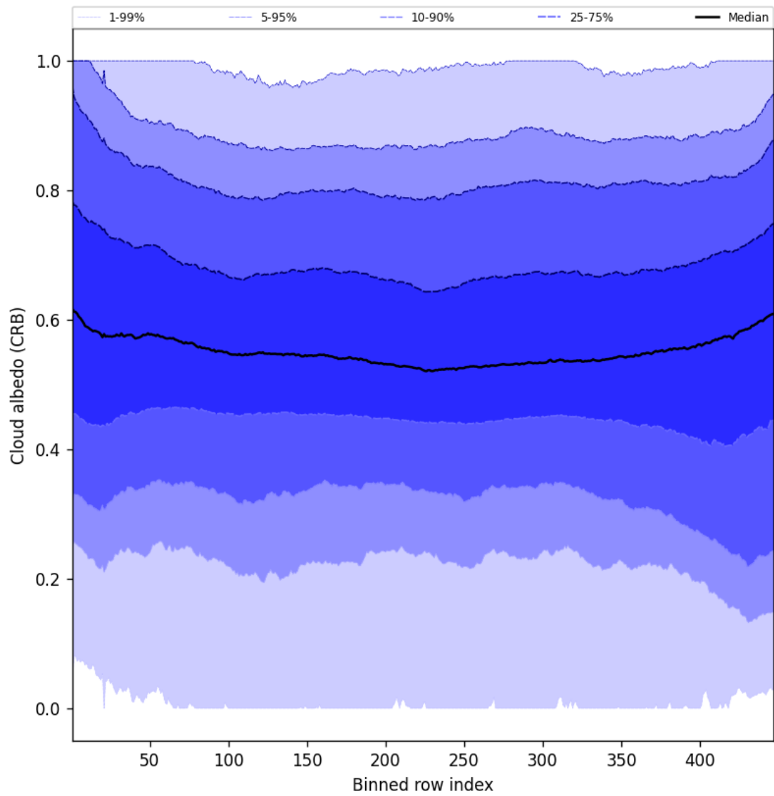
Figure 58: Along track statistics of “Cloud albedo (CRB)” for 2025-06-22 to 2025-06-23
