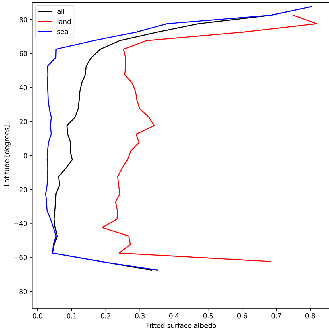
Figure 27: Zonal average of “Fitted surface albedo” for 2025-06-22 to 2025-06-23.
