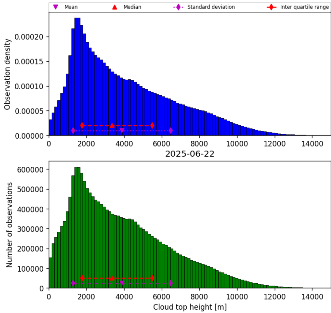
Figure 38: Histogram of “Cloud top height” for 2025-06-22 to 2025-06-23
