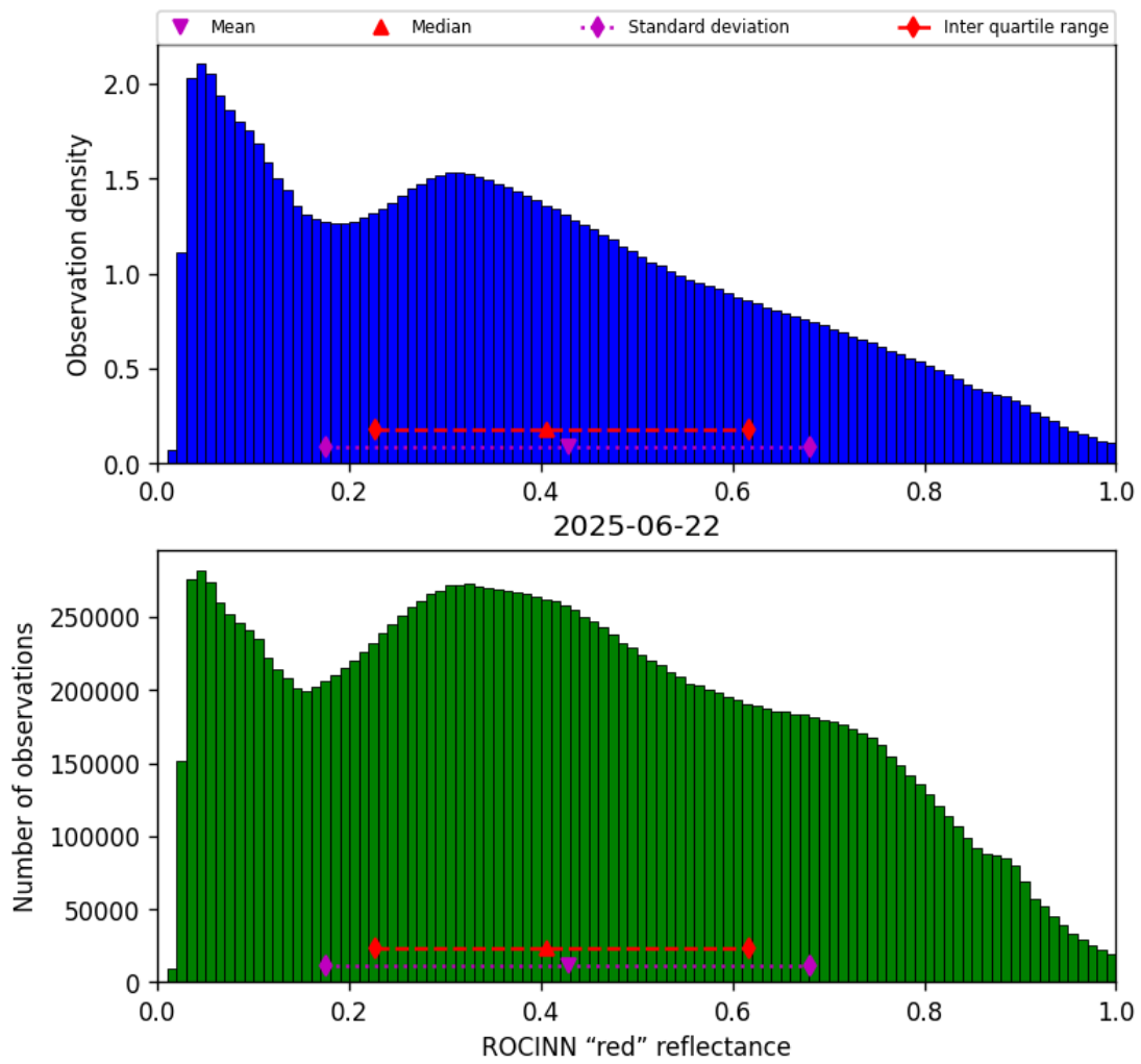
Figure 51: Histogram of "ROCINN "red" reflectance" for 2025-06-22 to 2025-06-23
