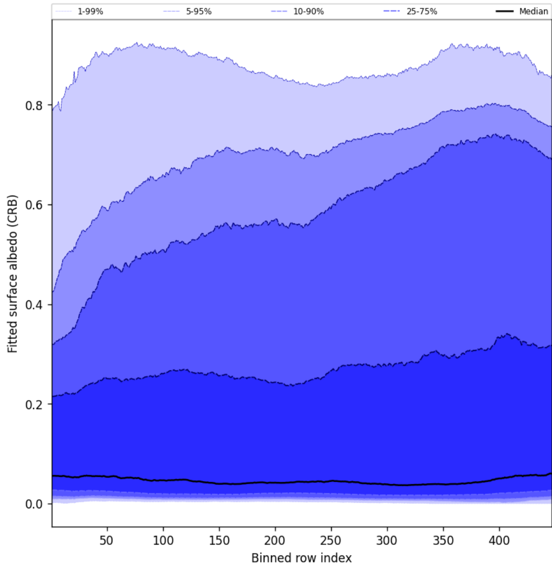
Figure 60: Along track statistics of “Fitted surface albedo (CRB)” for 2025-06-22 to 2025-06-23
