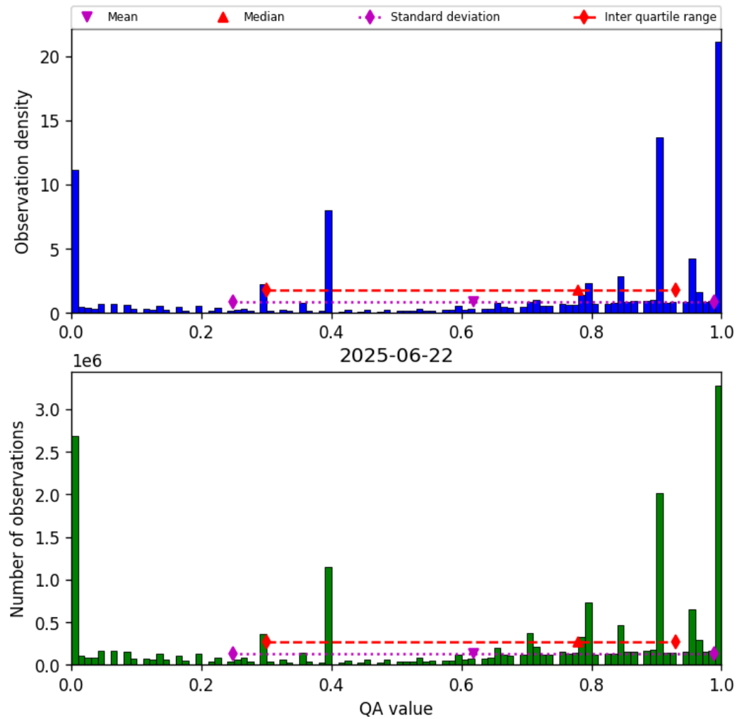
Figure 36: Histogram of “QA value” for 2025-06-22 to 2025-06-23
