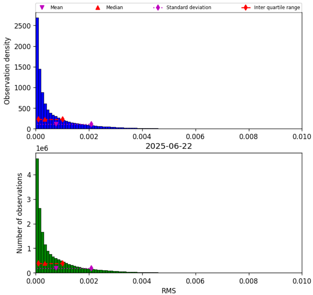
Figure 45: Histogram of “RMS” for 2025-06-22 to 2025-06-23
