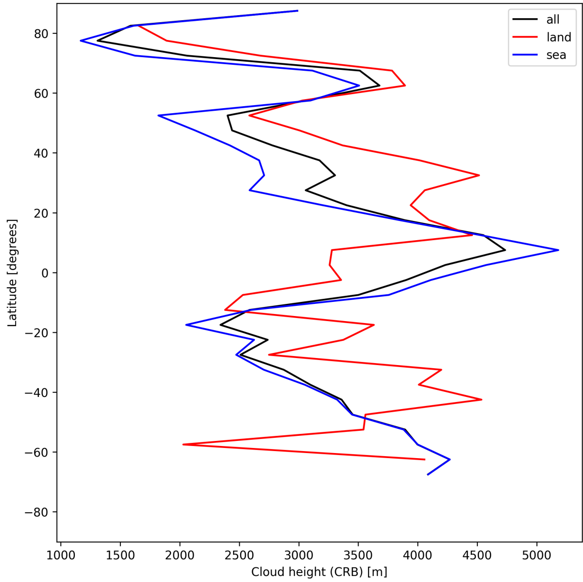
Figure 25: Zonal average of “Cloud height (CRB)” for 2025-06-22 to 2025-06-23.
