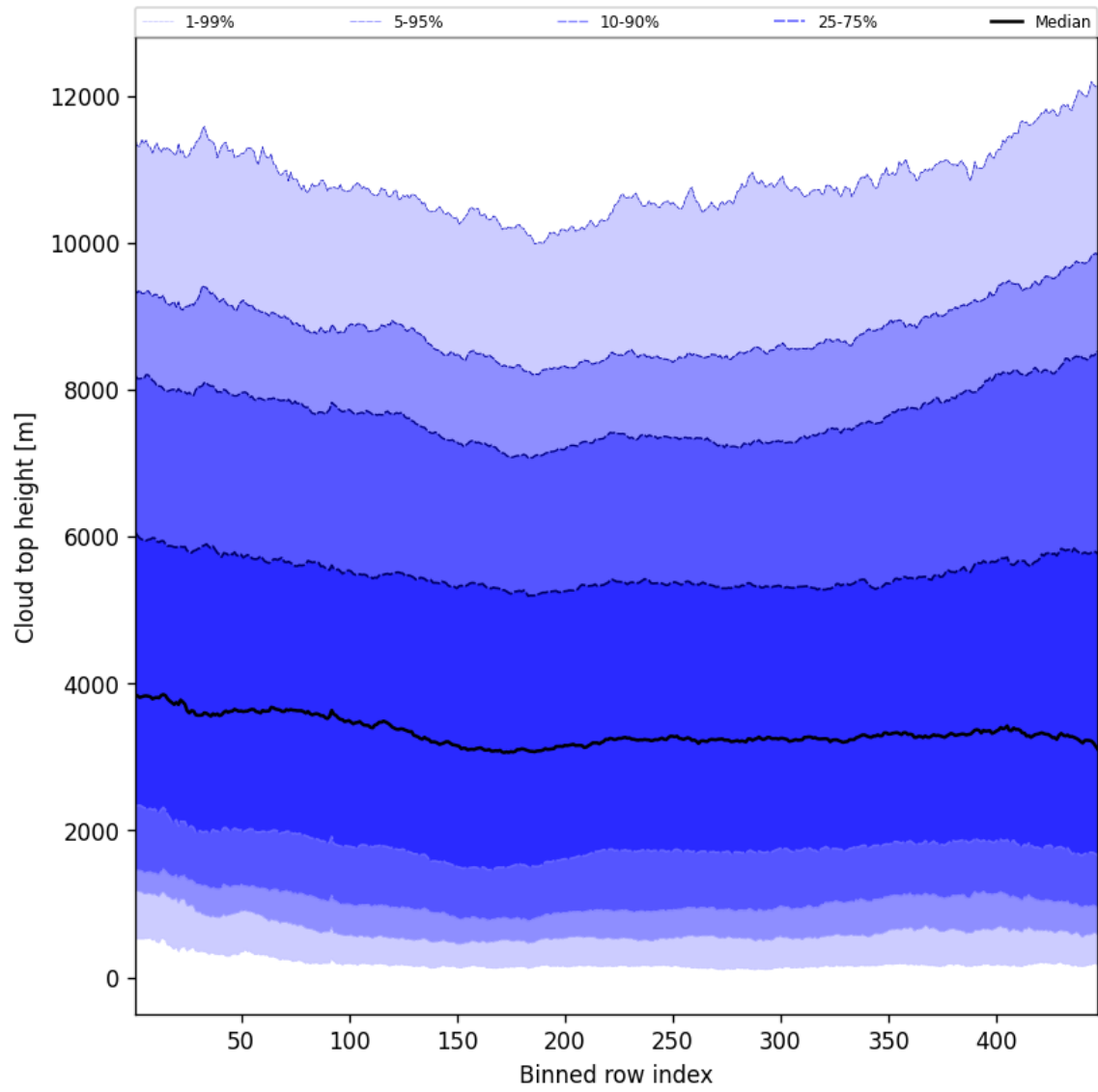
Figure 54: Along track statistics of “Cloud top height” for 2025-06-22 to 2025-06-23
