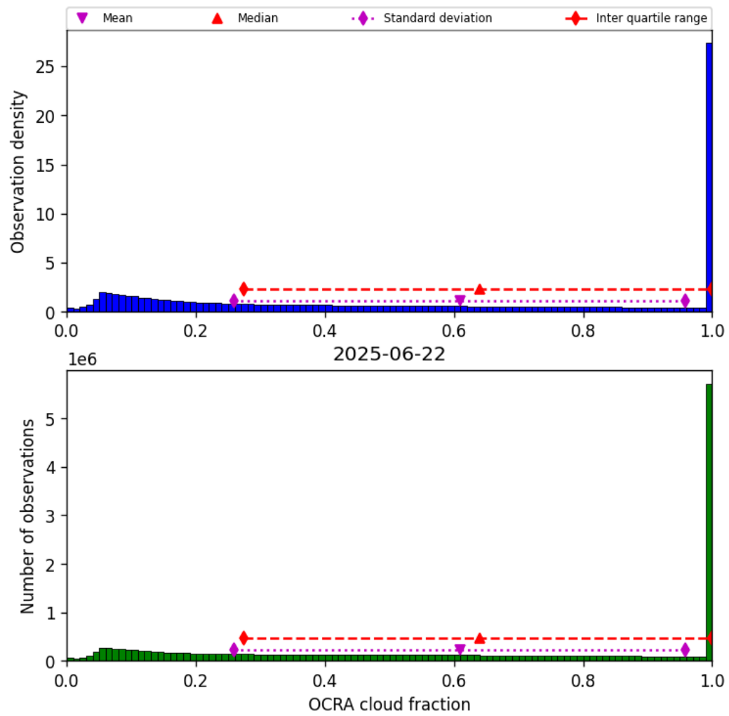
Figure 48: Histogram of “OCRA cloud fraction” for 2025-06-22 to 2025-06-23
