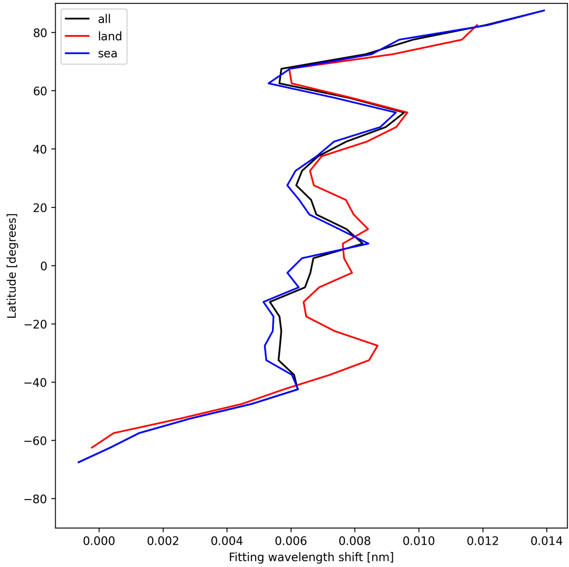
Figure 31: Zonal average of “Fitting wavelength shift” for 2025-06-22 to 2025-06-23.
