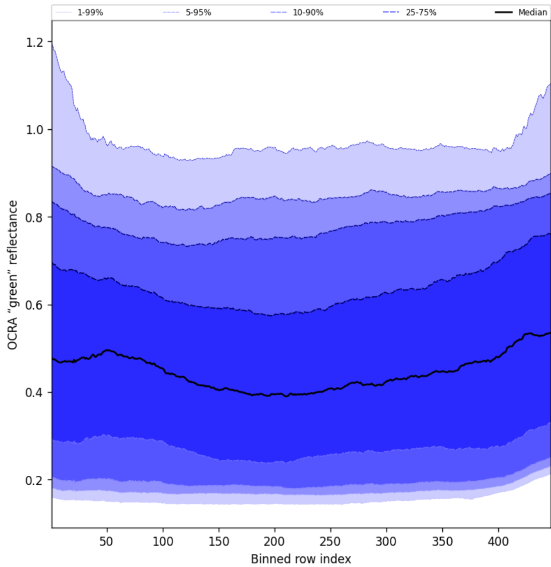
Figure 66: Along track statistics of “OCRA “green” reflectance” for 2025-06-22 to 2025-06-23
