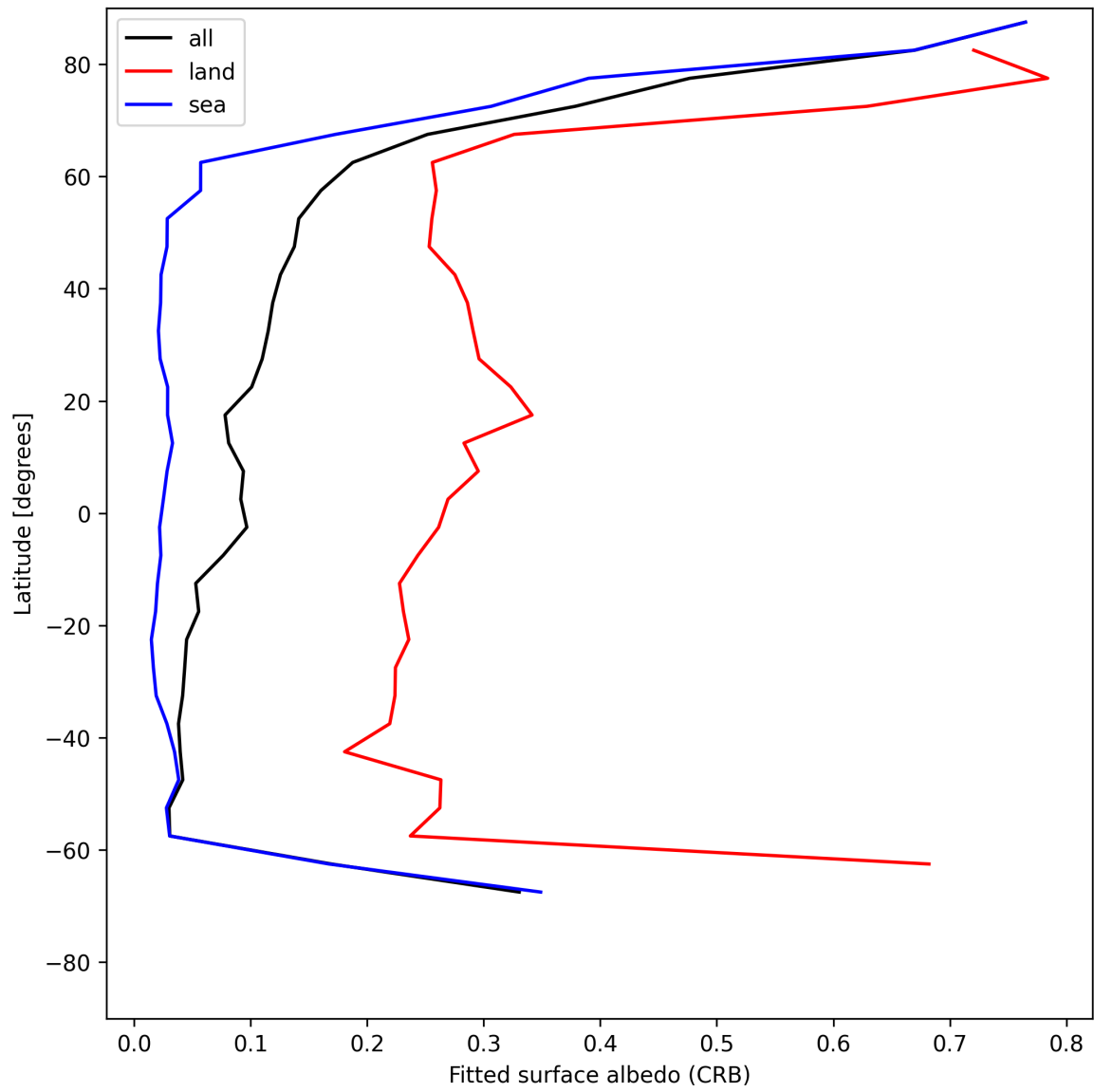
Figure 28: Zonal average of “Fitted surface albedo (CRB)” for 2025-06-22 to 2025-06-23.
