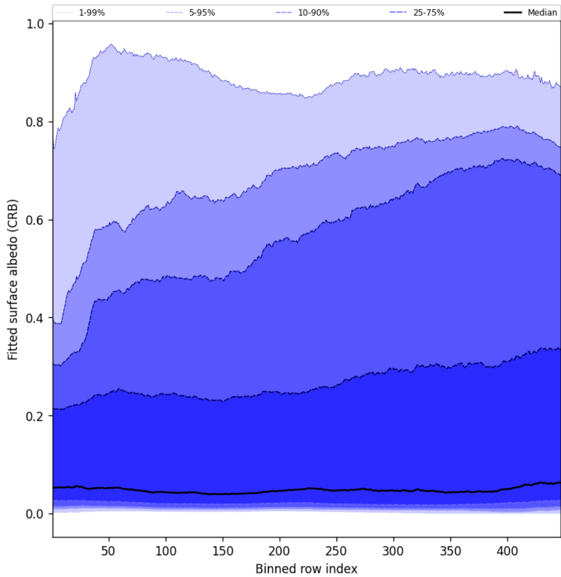
Figure 60: Along track statistics of “Fitted surface albedo (CRB)” for 2025-06-24 to 2025-06-25
