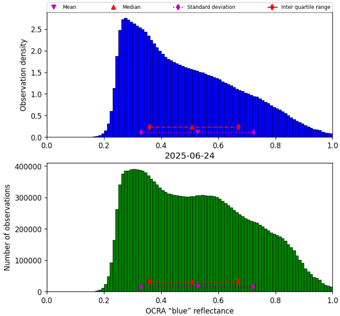
Figure 49: Histogram of “OCRA “blue” reflectance” for 2025-06-24 to 2025-06-25
