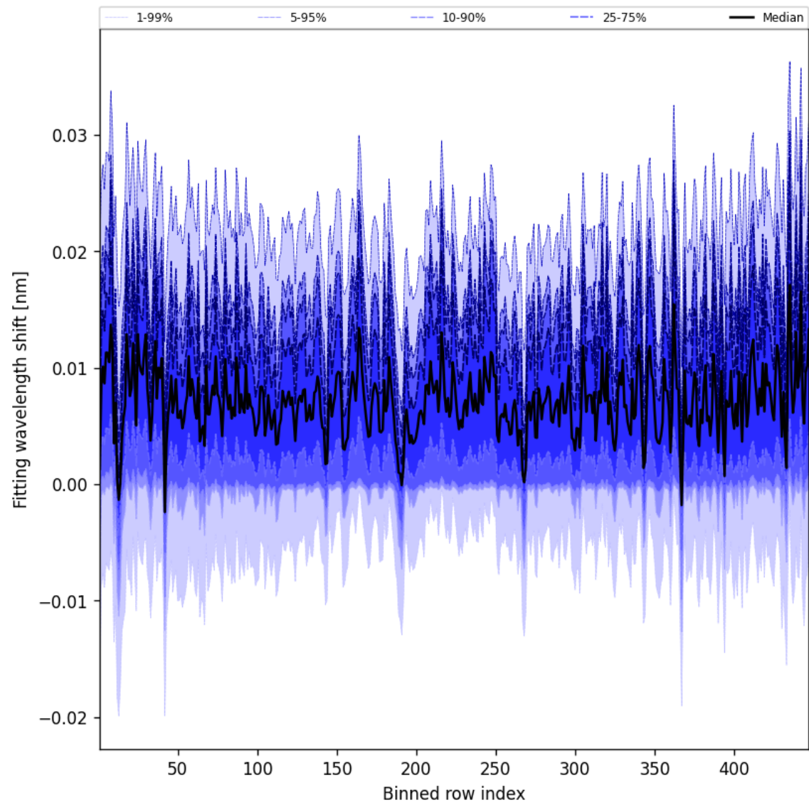
Figure 63: Along track statistics of “Fitting wavelength shift” for 2025-06-24 to 2025-06-25
