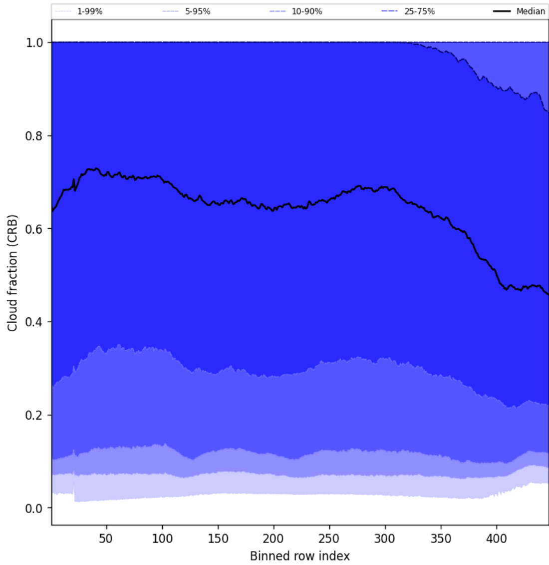
Figure 56: Along track statistics of “Cloud fraction (CRB)” for 2025-06-24 to 2025-06-25
