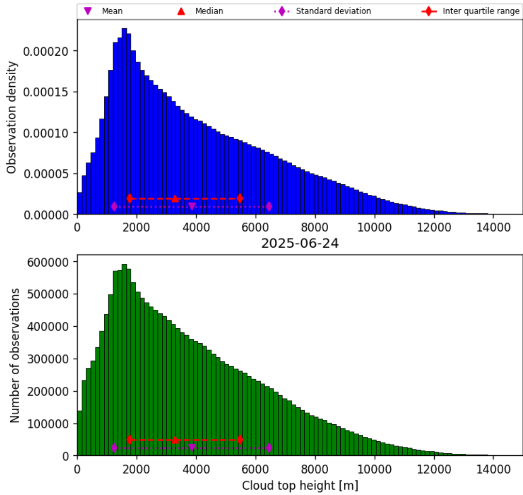
Figure 38: Histogram of “Cloud top height” for 2025-06-24 to 2025-06-25
