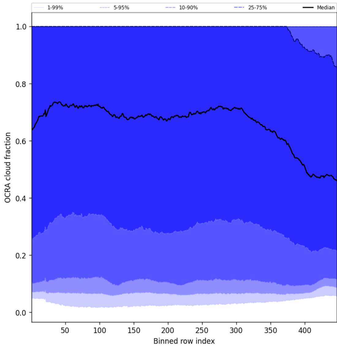
Figure 64: Along track statistics of “OCRA cloud fraction” for 2025-06-24 to 2025-06-25
