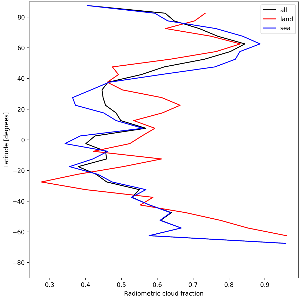
Figure 21: Zonal average of “Radiometric cloud fraction” for 2025-06-24 to 2025-06-25.
