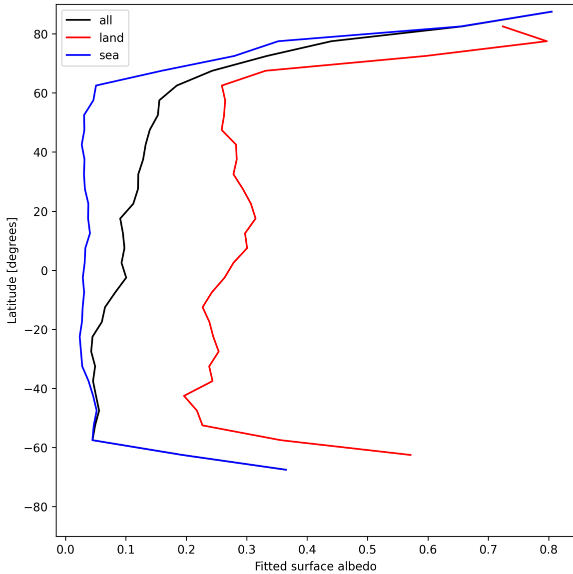
Figure 27: Zonal average of “Fitted surface albedo” for 2025-06-24 to 2025-06-25.
