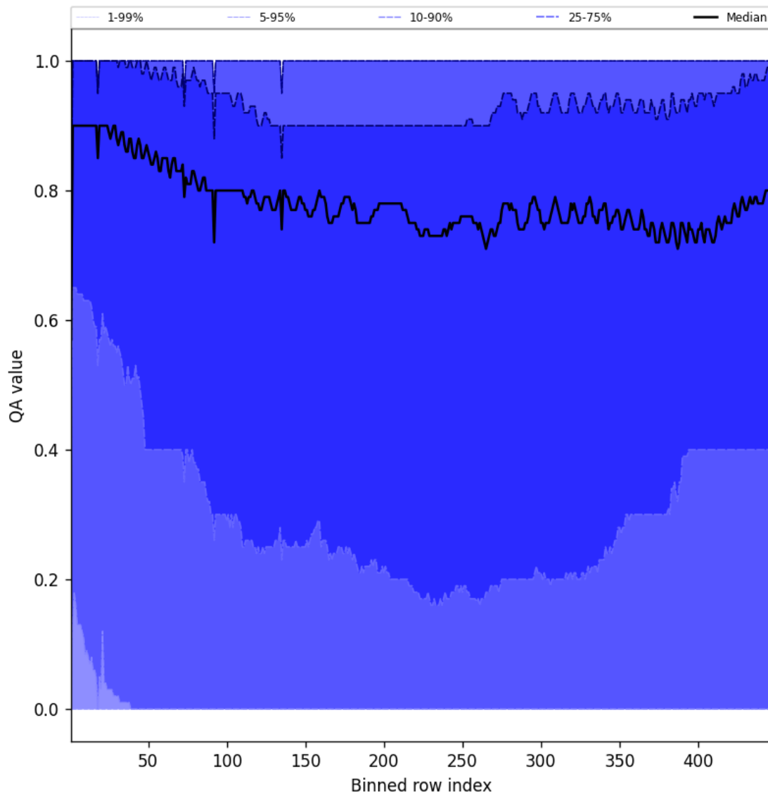
Figure 52: Along track statistics of “QA value” for 2025-06-24 to 2025-06-25
