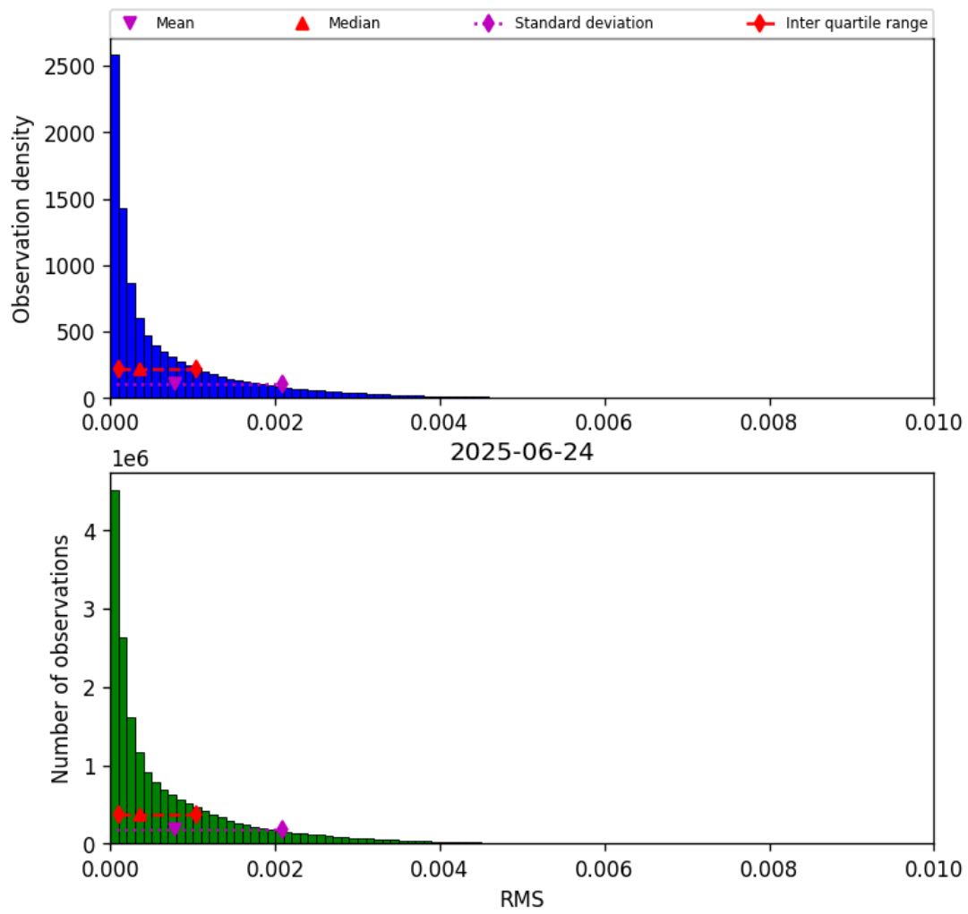
Figure 45: Histogram of “RMS” for 2025-06-24 to 2025-06-25
