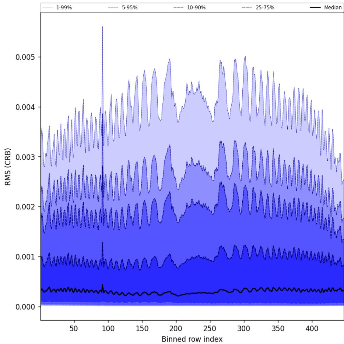
Figure 62: Along track statistics of “RMS (CRB)” for 2025-06-24 to 2025-06-25
