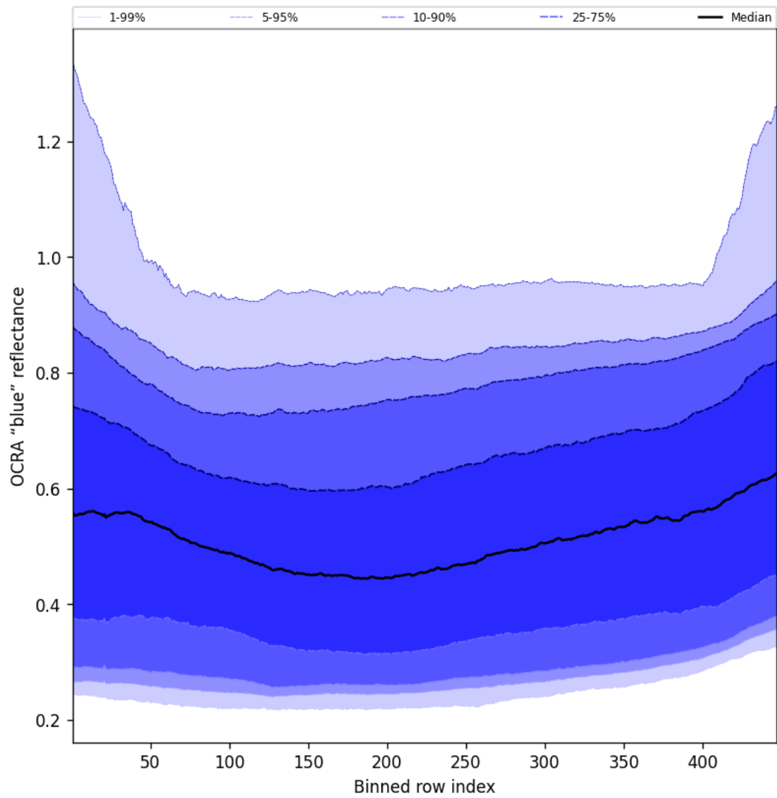
Figure 65: Along track statistics of “OCRA “blue” reflectance” for 2025-06-24 to 2025-06-25
