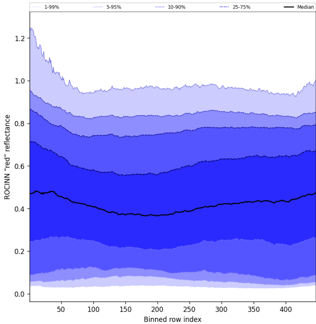
Figure 67: Along track statistics of "ROCINN "red" reflectance" for 2025-06-24 to 2025-06-25
