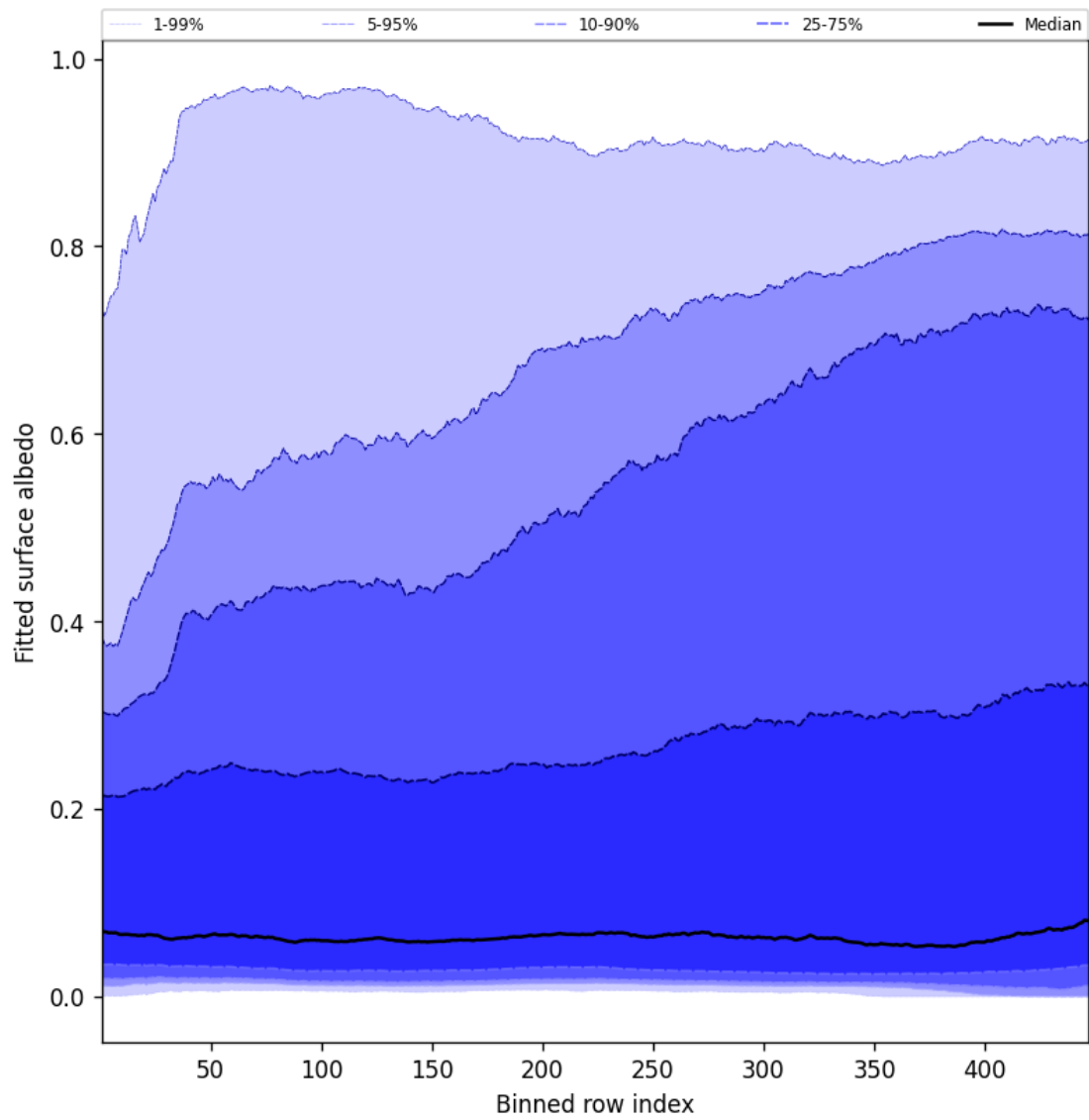
Figure 59: Along track statistics of “Fitted surface albedo” for 2025-06-24 to 2025-06-25
