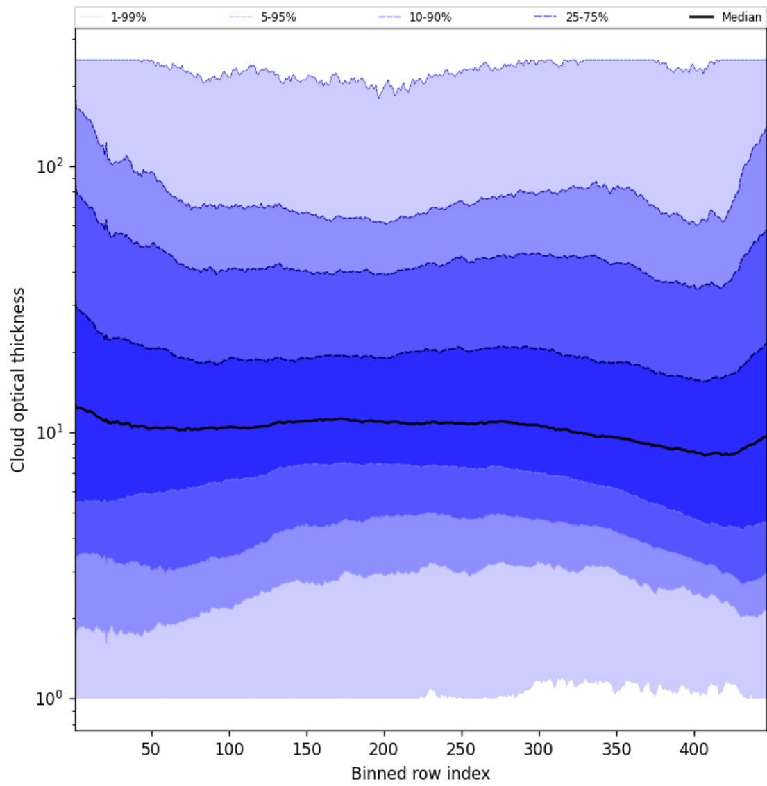
Figure 55: Along track statistics of “Cloud optical thickness” for 2025-06-24 to 2025-06-25
