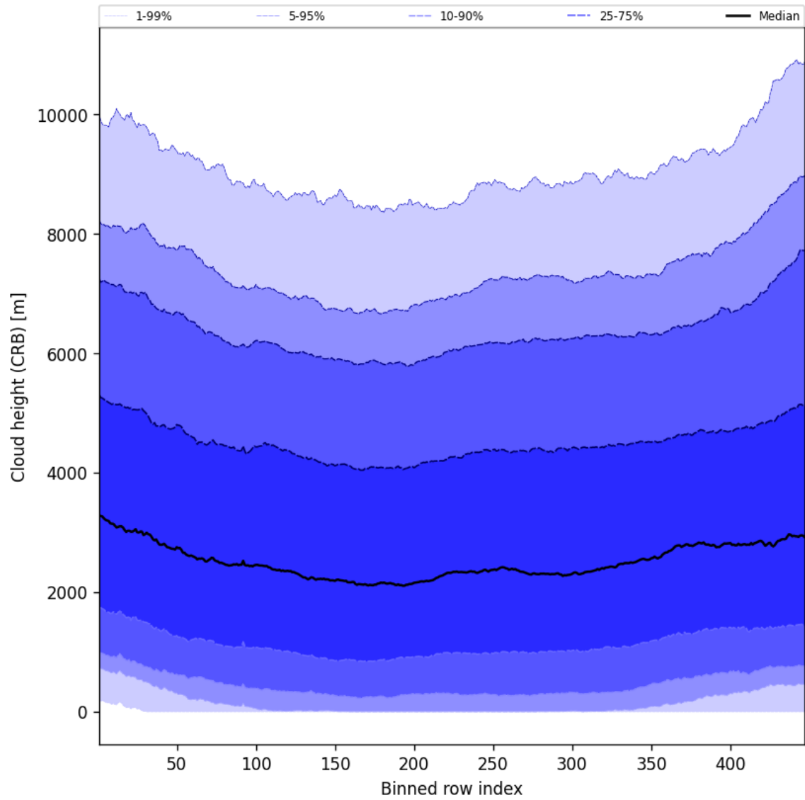
Figure 57: Along track statistics of “Cloud height (CRB)” for 2025-06-24 to 2025-06-25
