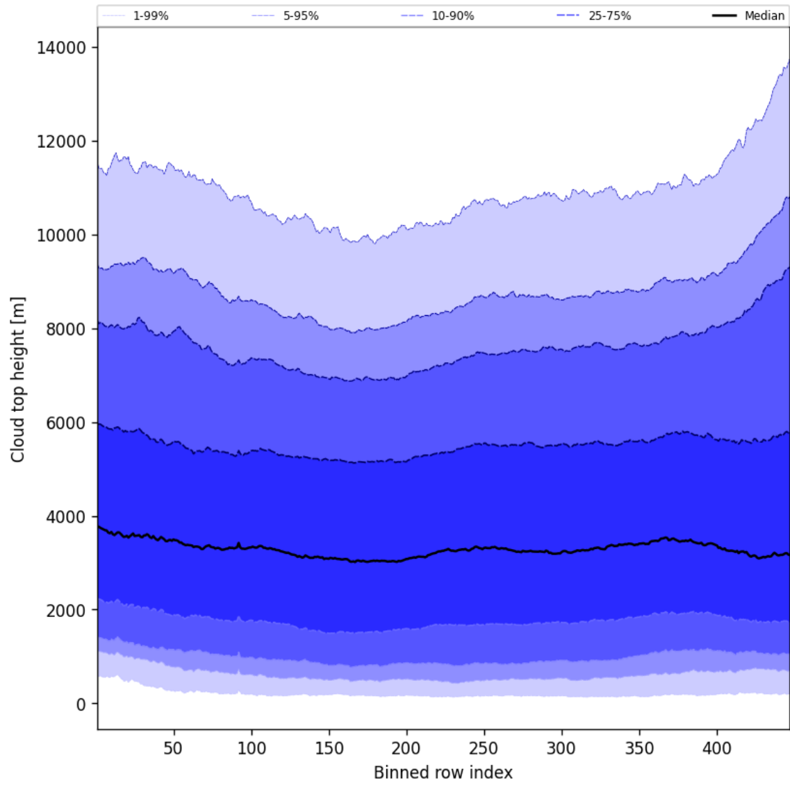
Figure 54: Along track statistics of “Cloud top height” for 2025-06-24 to 2025-06-25
