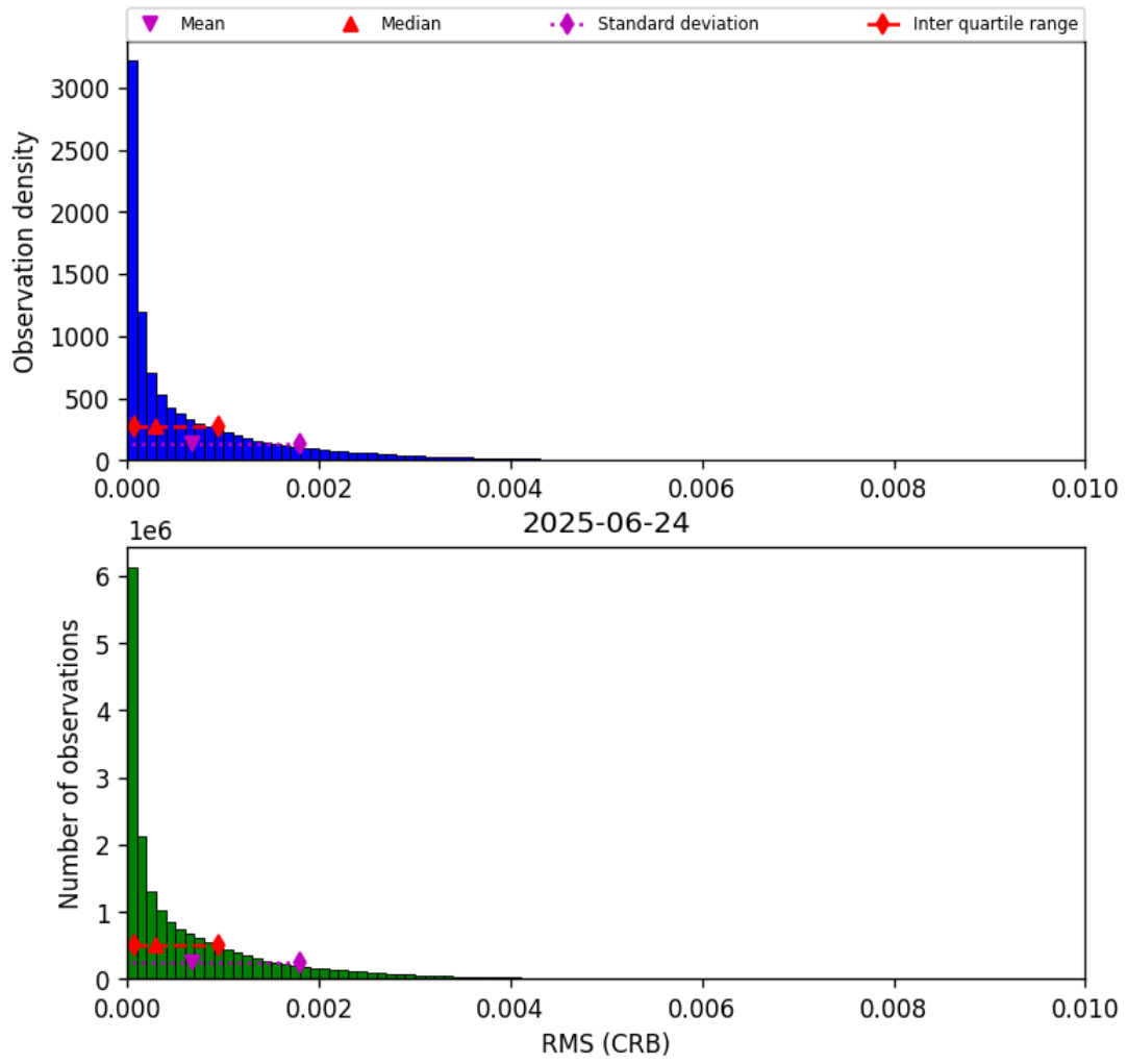
Figure 46: Histogram of “RMS (CRB)” for 2025-06-24 to 2025-06-25
