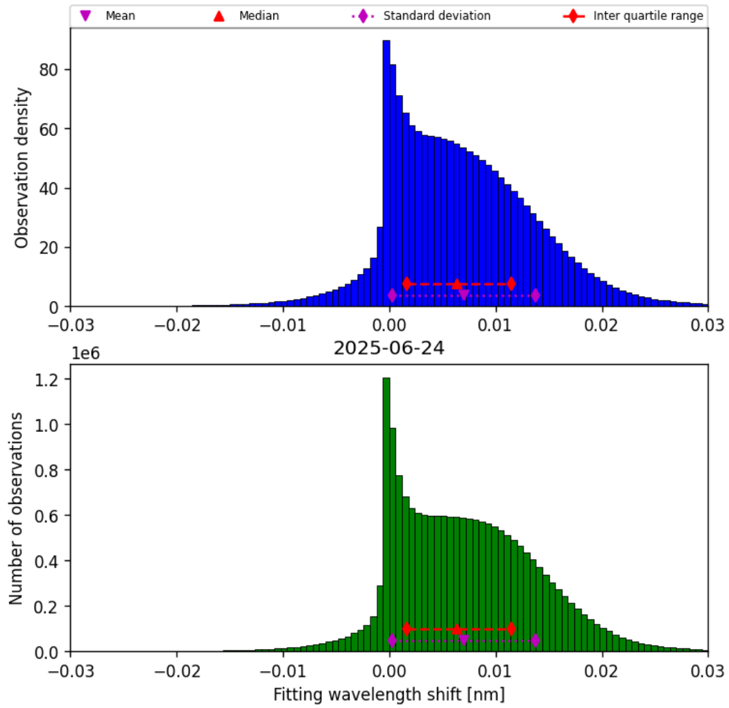
Figure 47: Histogram of “Fitting wavelength shift” for 2025-06-24 to 2025-06-25
