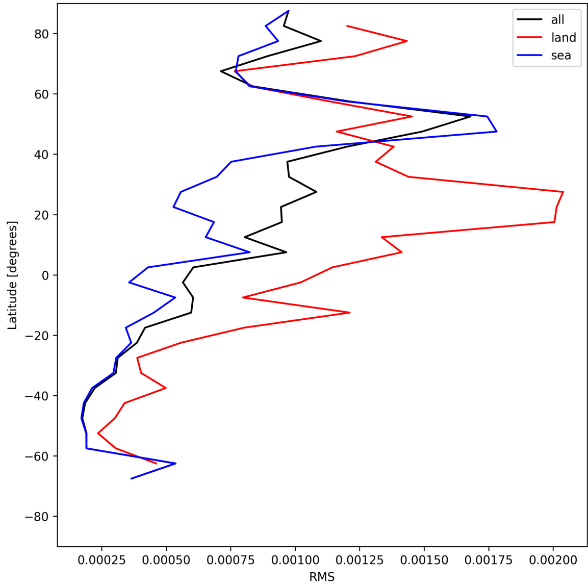
Figure 29: Zonal average of “RMS” for 2025-06-24 to 2025-06-25.
