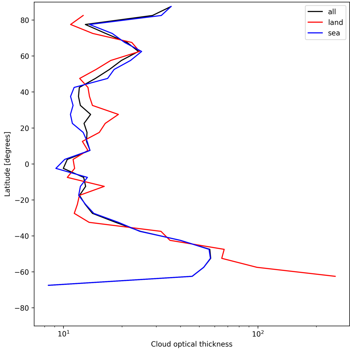
Figure 23: Zonal average of “Cloud optical thickness” for 2025-06-24 to 2025-06-25.
