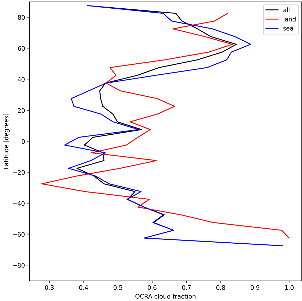
Figure 32: Zonal average of “OCRA cloud fraction” for 2025-06-24 to 2025-06-25.
