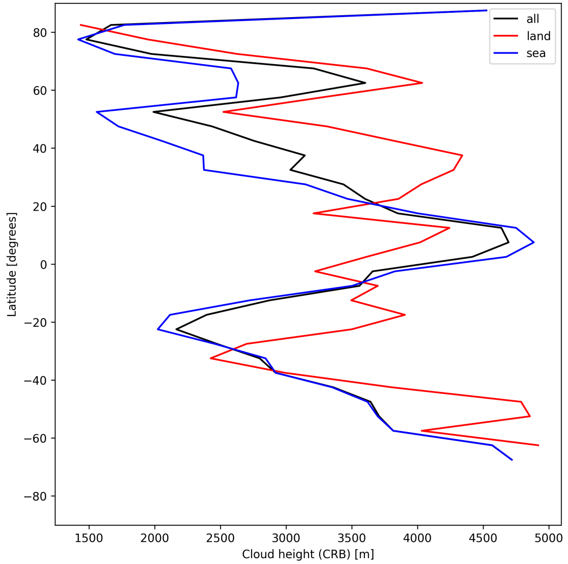
Figure 25: Zonal average of “Cloud height (CRB)” for 2025-06-24 to 2025-06-25.
