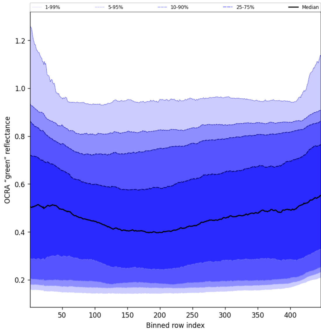
Figure 66: Along track statistics of “OCRA “green” reflectance” for 2025-06-24 to 2025-06-25
