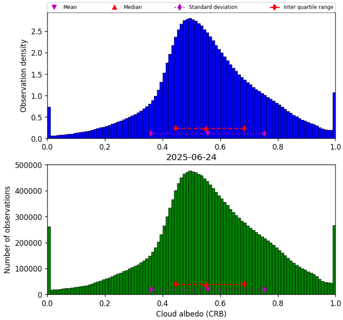
Figure 42: Histogram of “Cloud albedo (CRB)” for 2025-06-24 to 2025-06-25
