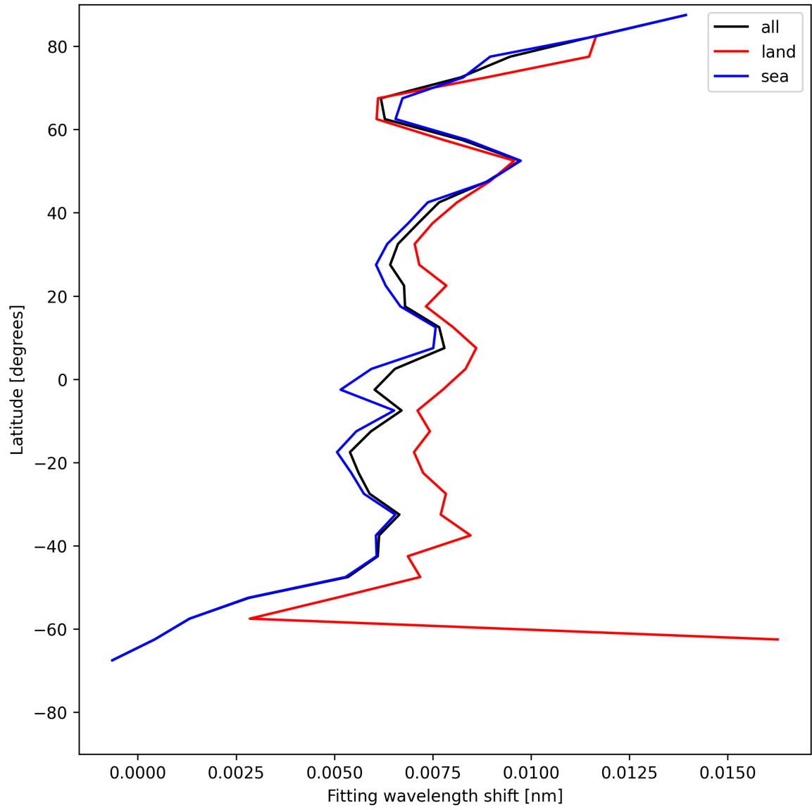
Figure 31: Zonal average of “Fitting wavelength shift” for 2025-06-24 to 2025-06-25.
