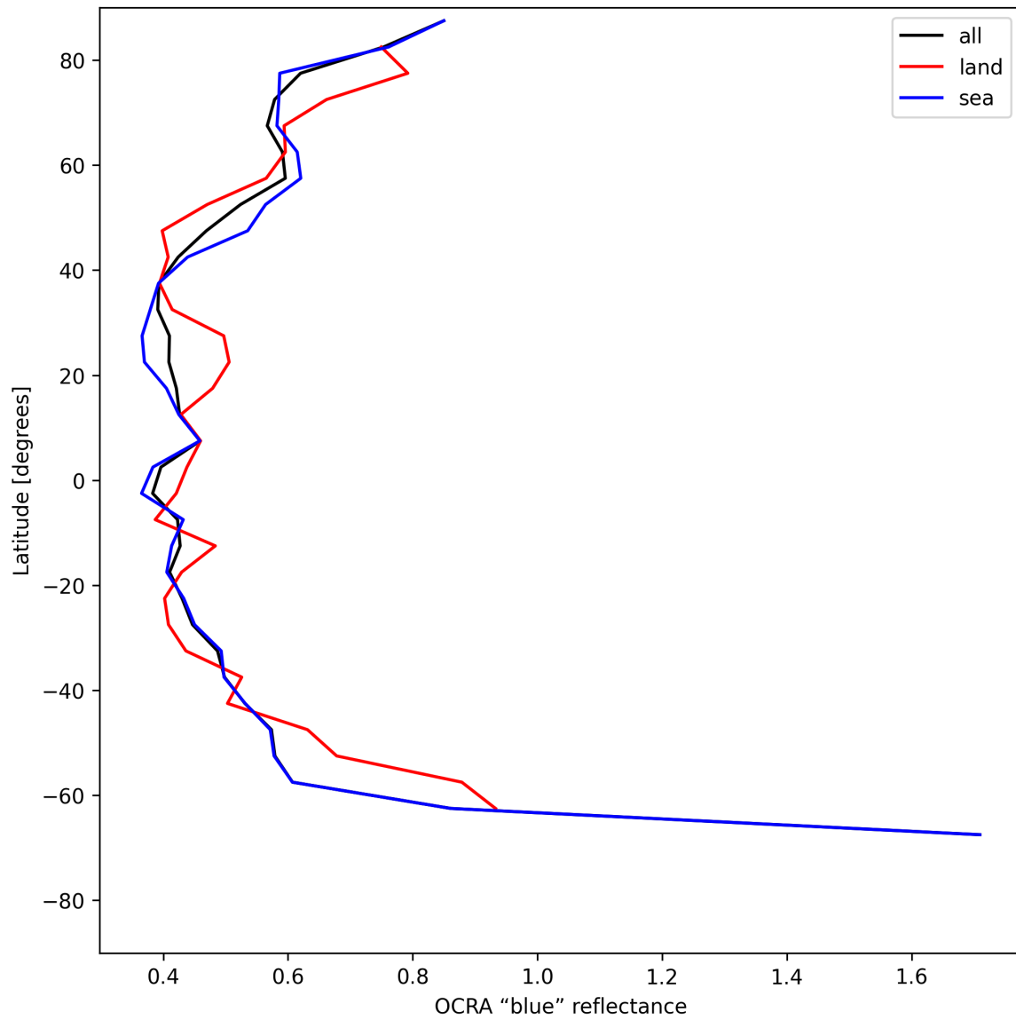
Figure 33: Zonal average of “OCRA “blue” reflectance” for 2025-06-24 to 2025-06-25.
