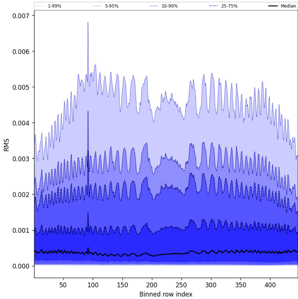
Figure 61: Along track statistics of “RMS” for 2025-06-24 to 2025-06-25
