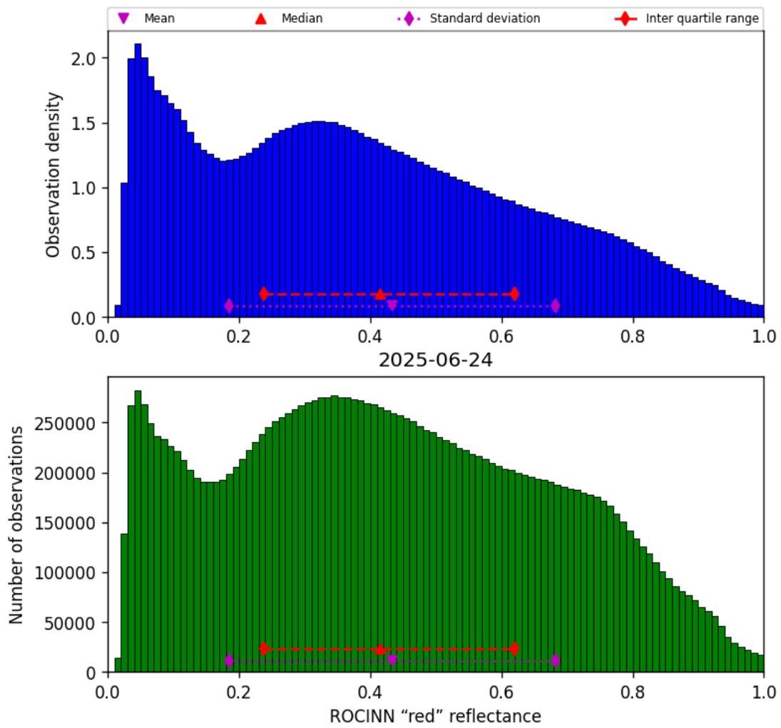
Figure 51: Histogram of “ROCINN “red” reflectance” for 2025-06-24 to 2025-06-25
