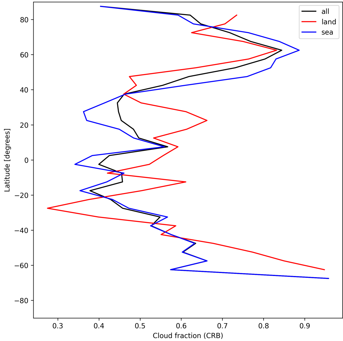
Figure 24: Zonal average of “Cloud fraction (CRB)” for 2025-06-24 to 2025-06-25.
