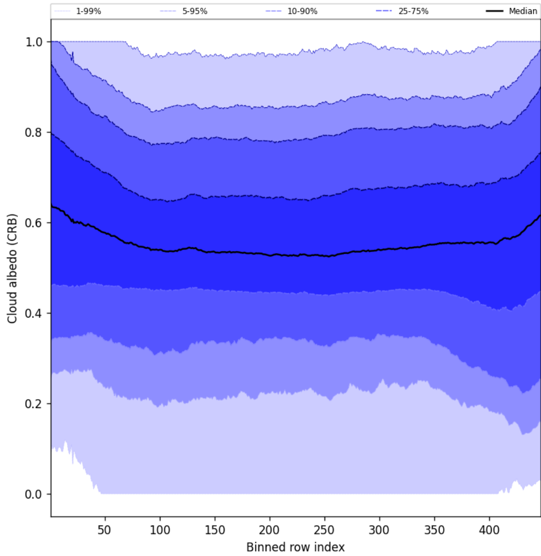
Figure 58: Along track statistics of “Cloud albedo (CRB)” for 2025-06-24 to 2025-06-25
