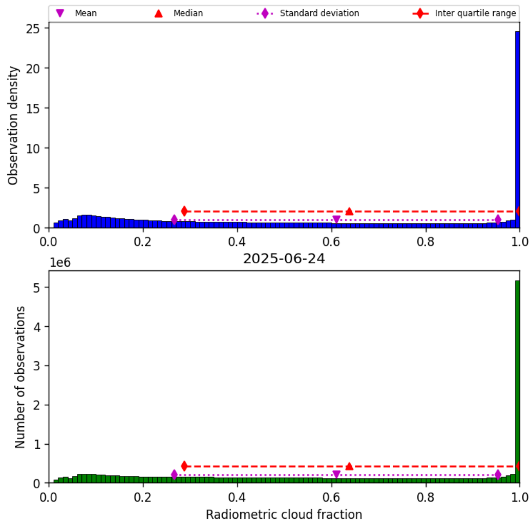
Figure 37: Histogram of “Radiometric cloud fraction” for 2025-06-24 to 2025-06-25
