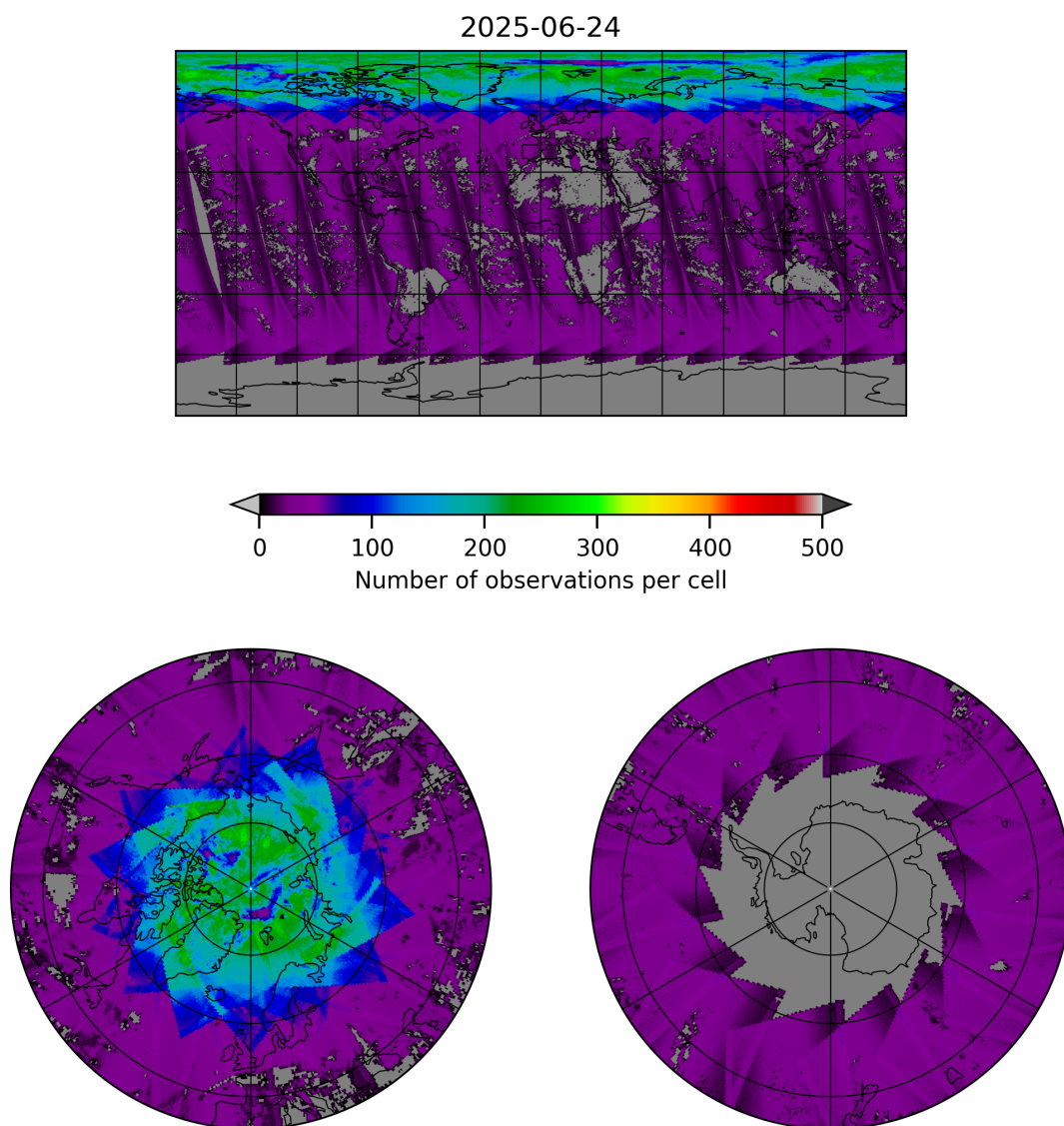
Figure 19: Map of the number of observations for 2025-06-24 to 2025-06-25
