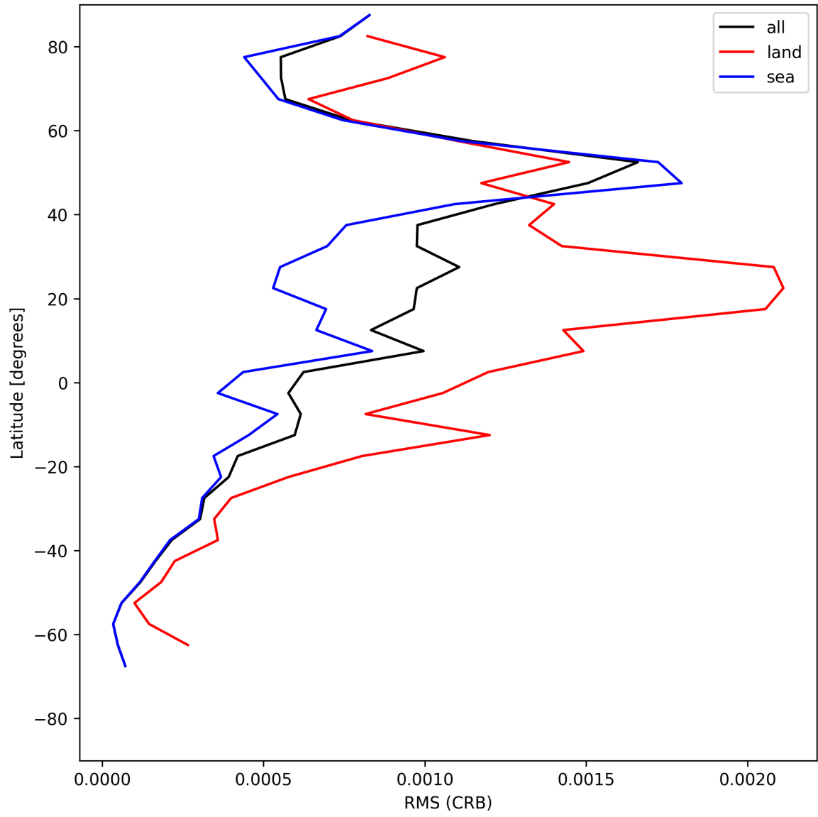
Figure 30: Zonal average of “RMS (CRB)” for 2025-06-24 to 2025-06-25.
