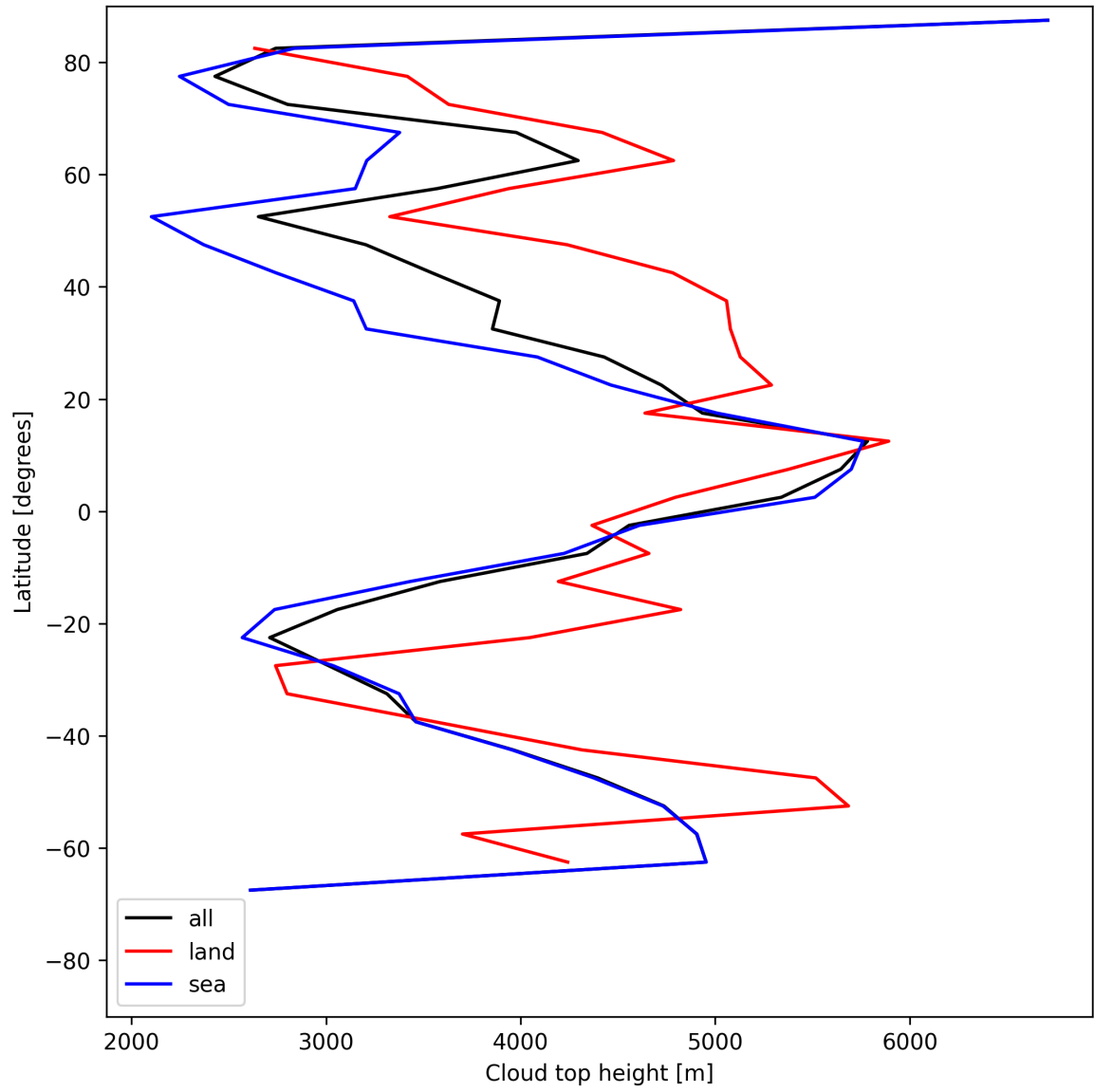
Figure 22: Zonal average of “Cloud top height” for 2025-06-24 to 2025-06-25.
