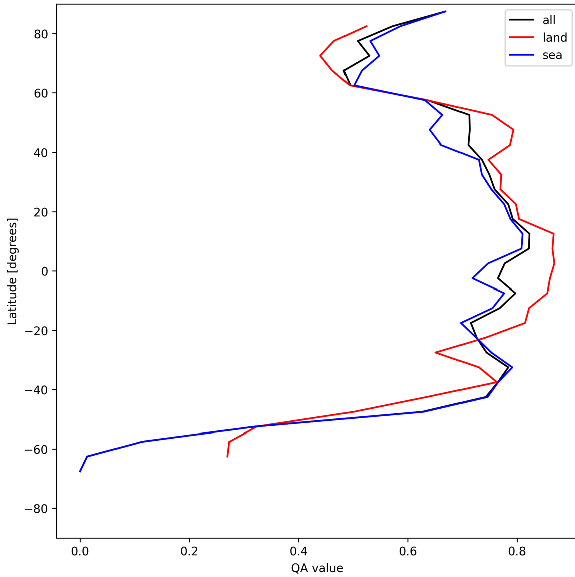
Figure 20: Zonal average of “QA value” for 2025-06-24 to 2025-06-25.
