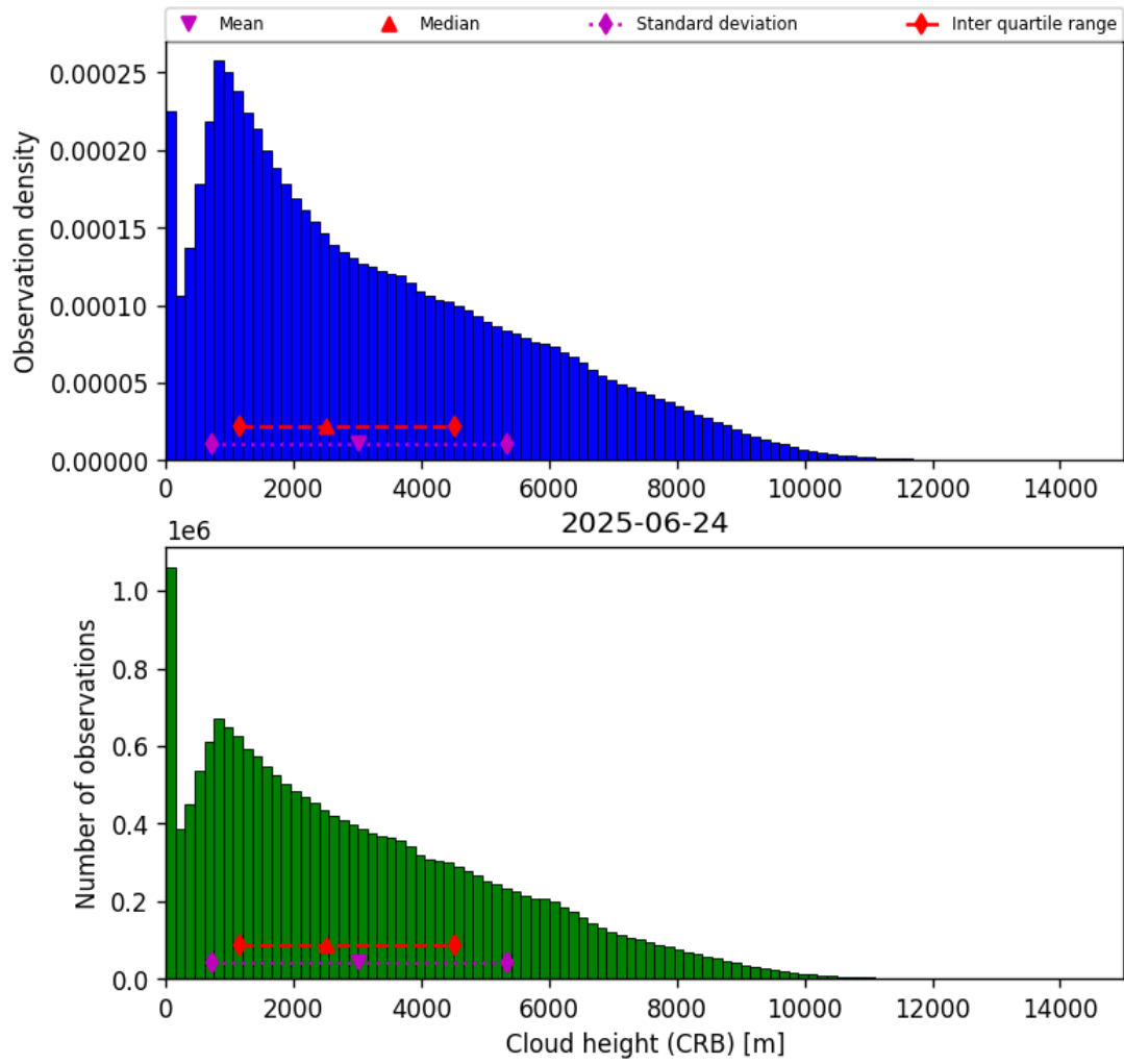
Figure 41: Histogram of “Cloud height (CRB)” for 2025-06-24 to 2025-06-25
