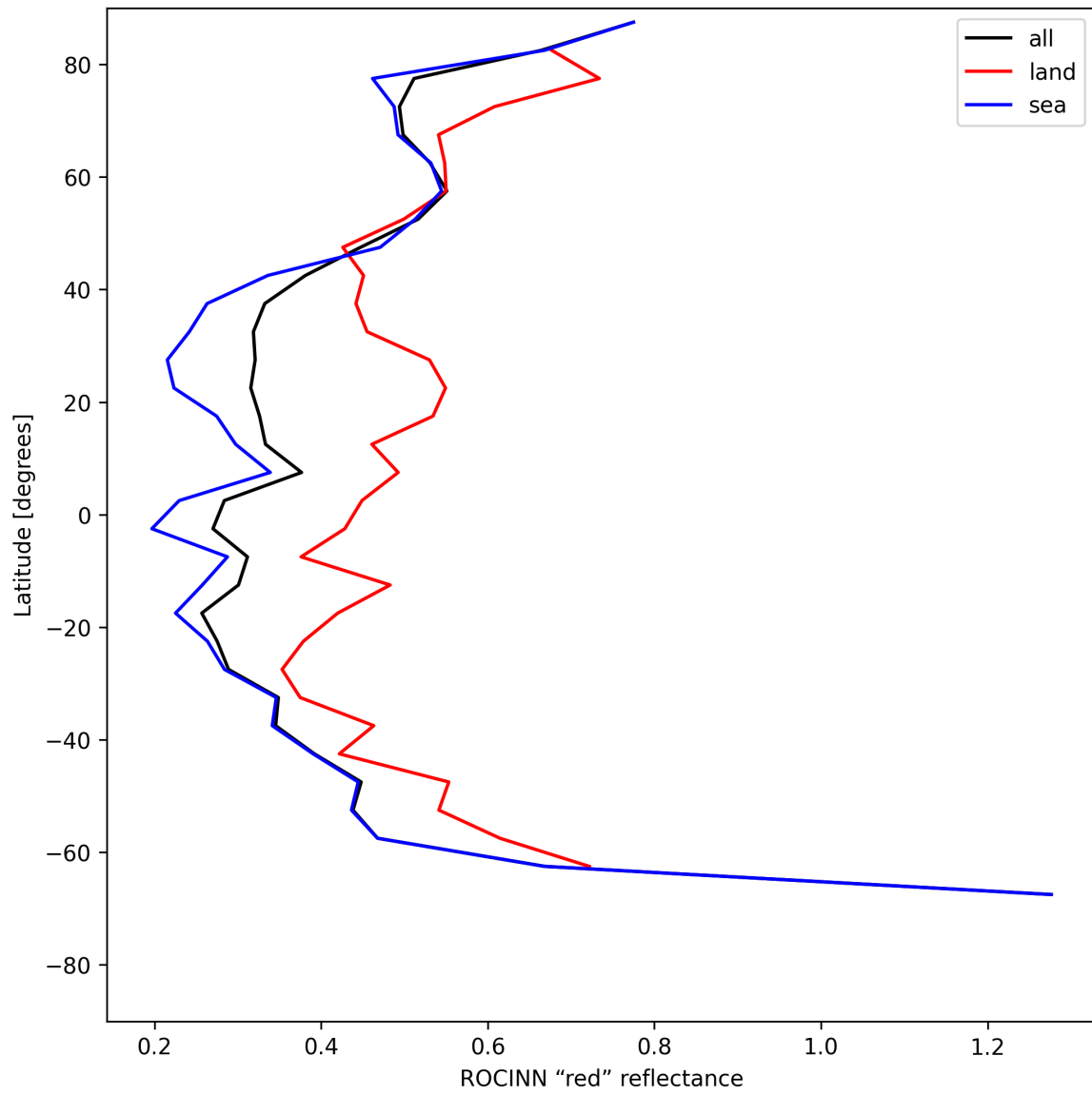
Figure 35: Zonal average of “ROCINN “red” reflectance” for 2025-06-24 to 2025-06-25.
