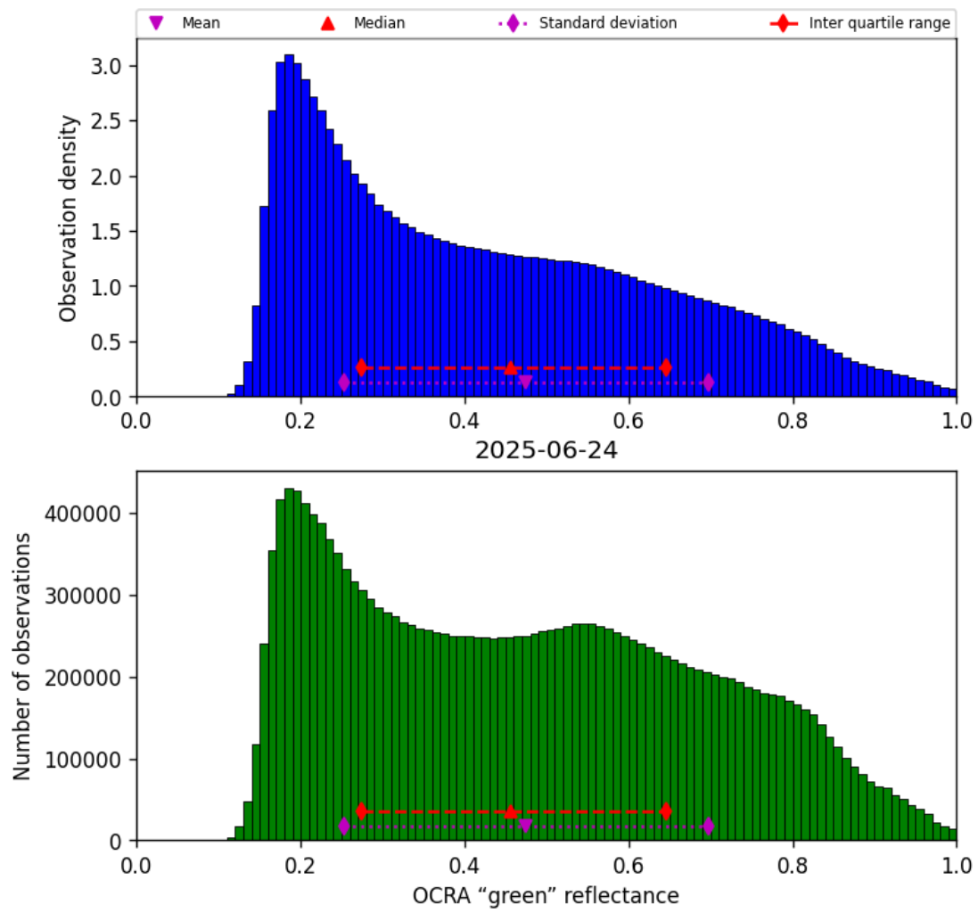
Figure 50: Histogram of “OCRA “green” reflectance” for 2025-06-24 to 2025-06-25
