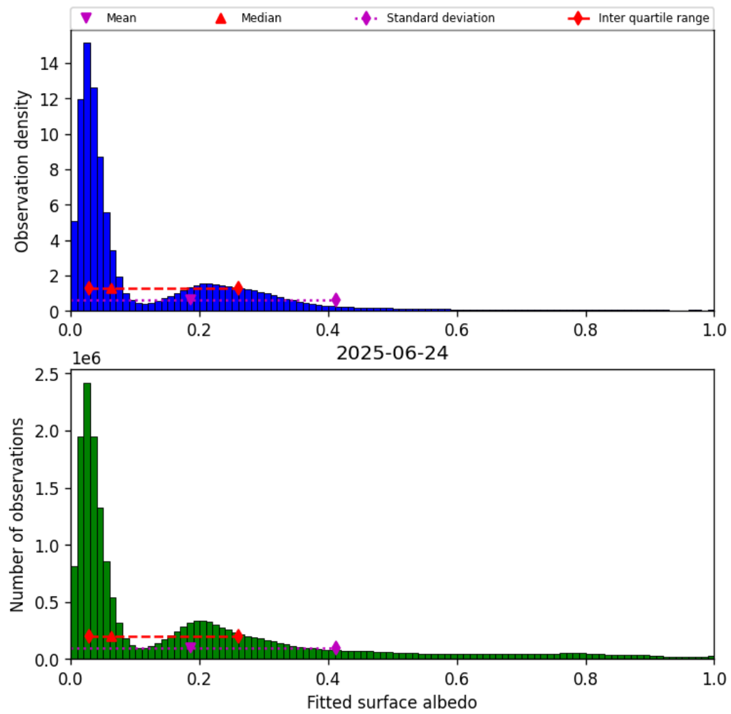
Figure 43: Histogram of “Fitted surface albedo” for 2025-06-24 to 2025-06-25
