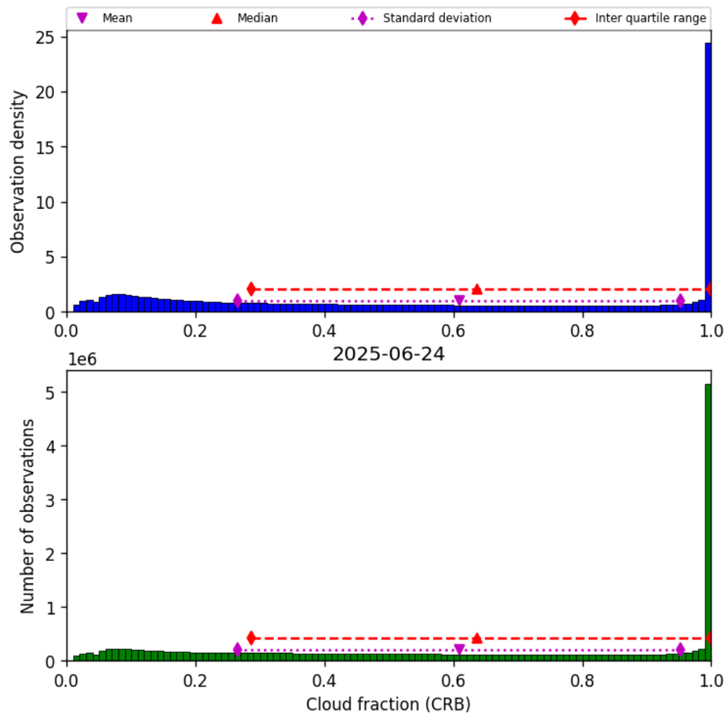
Figure 40: Histogram of “Cloud fraction (CRB)” for 2025-06-24 to 2025-06-25
