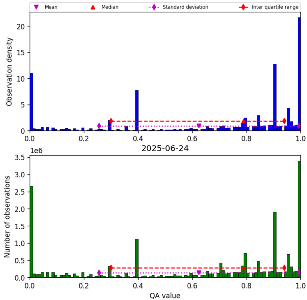
Figure 36: Histogram of “QA value” for 2025-06-24 to 2025-06-25
