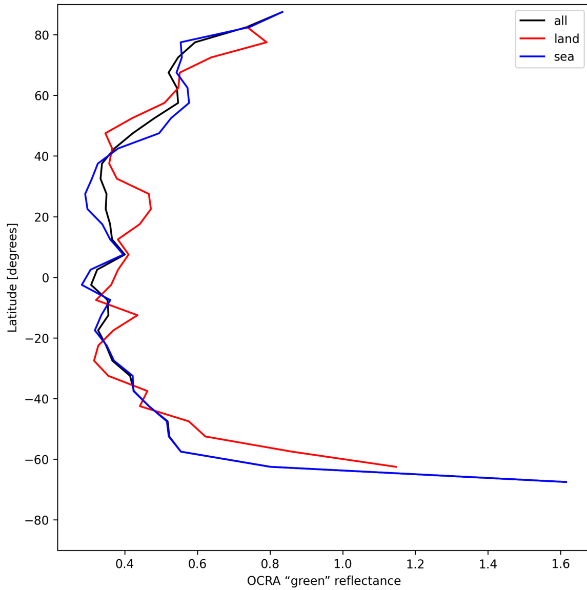
Figure 34: Zonal average of “OCRA “green” reflectance” for 2025-06-24 to 2025-06-25.
