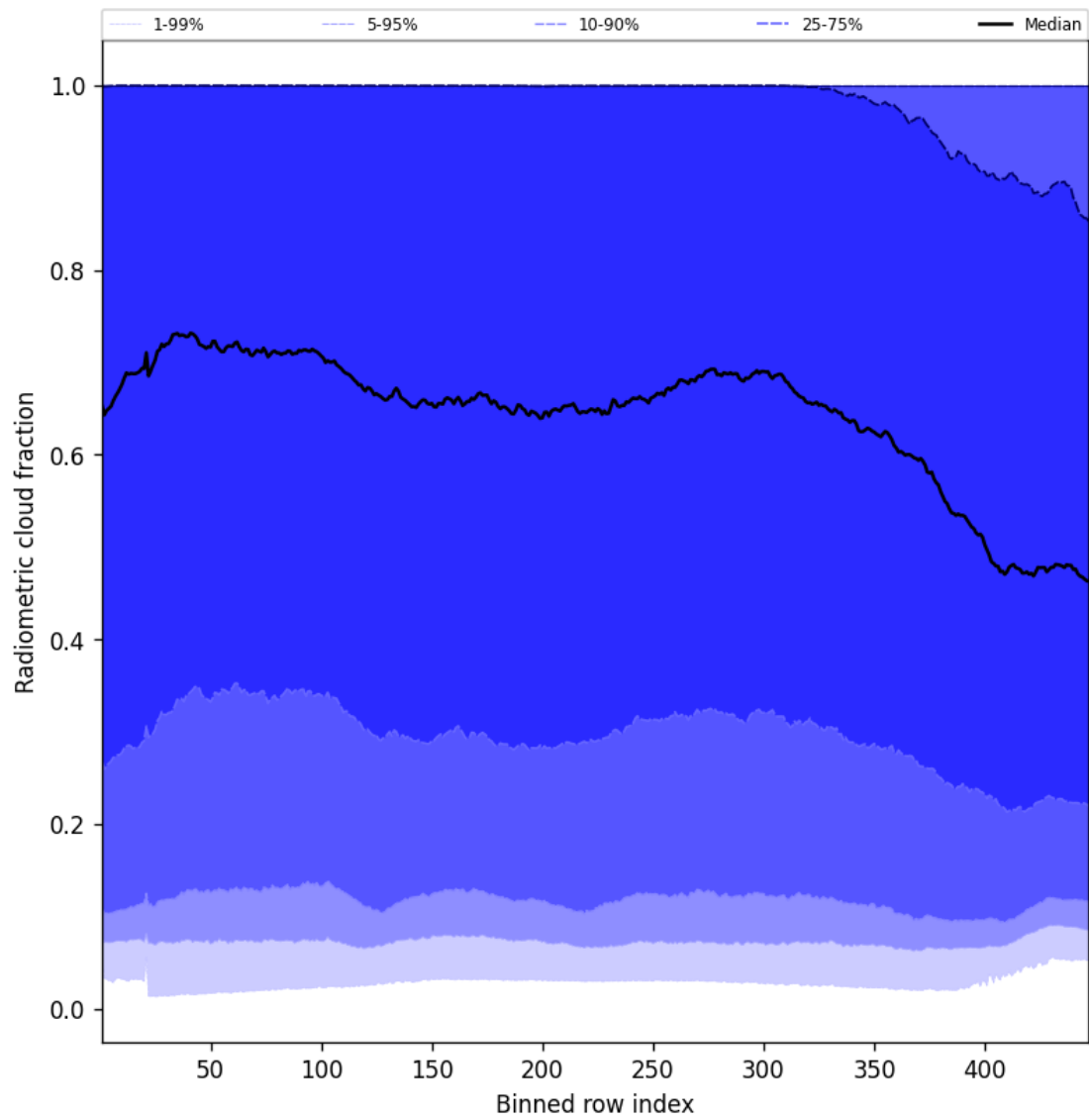
Figure 53: Along track statistics of “Radiometric cloud fraction” for 2025-06-24 to 2025-06-25
