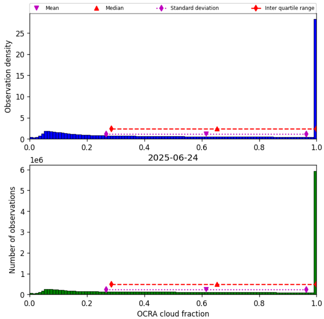
Figure 48: Histogram of “OCRA cloud fraction” for 2025-06-24 to 2025-06-25
