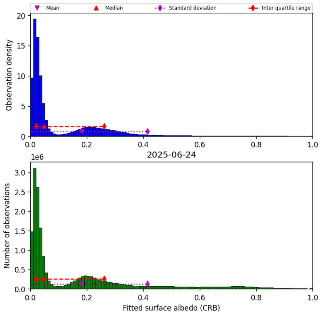
Figure 44: Histogram of “Fitted surface albedo (CRB)” for 2025-06-24 to 2025-06-25
