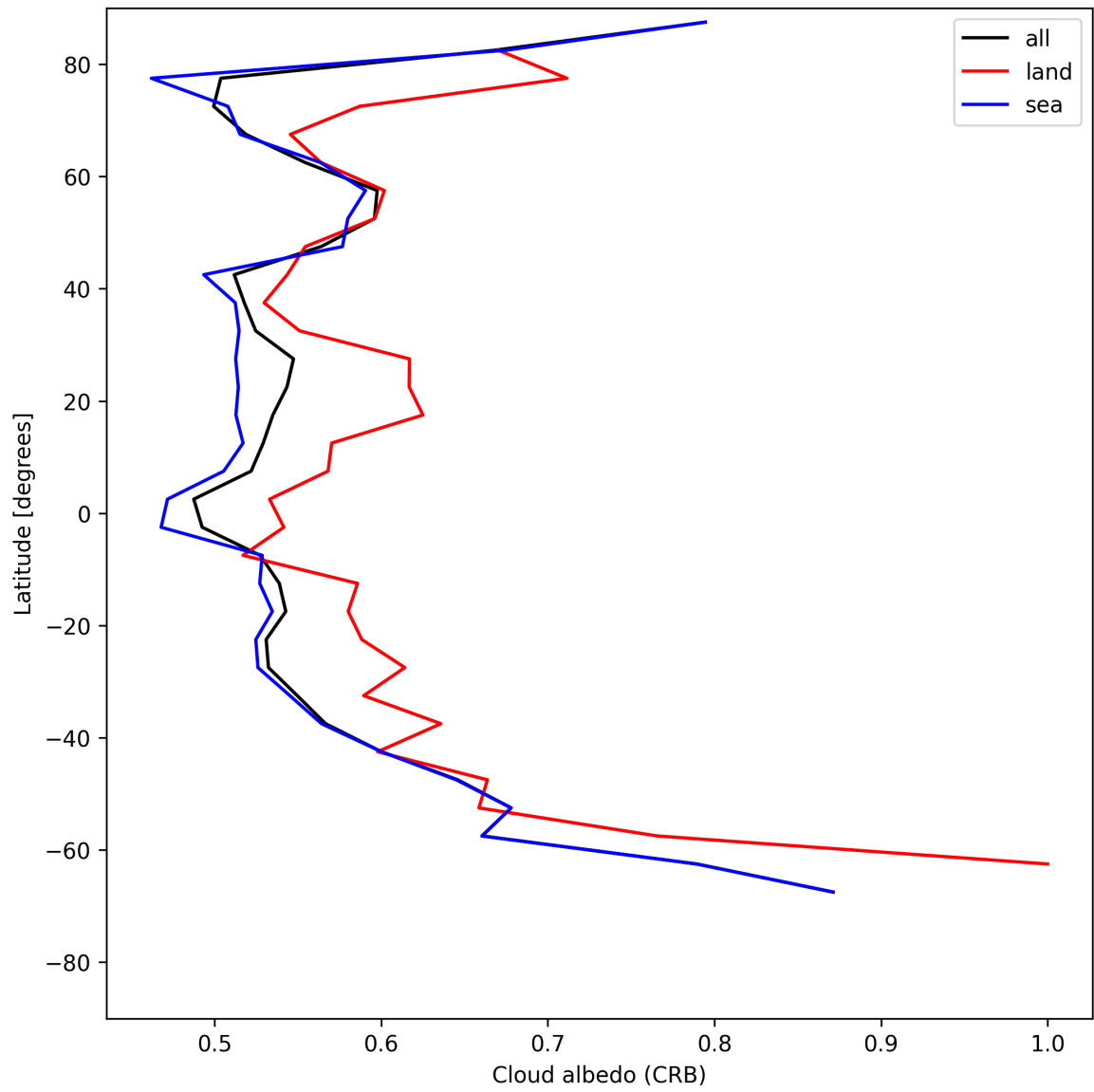
Figure 26: Zonal average of “Cloud albedo (CRB)” for 2025-06-24 to 2025-06-25.
