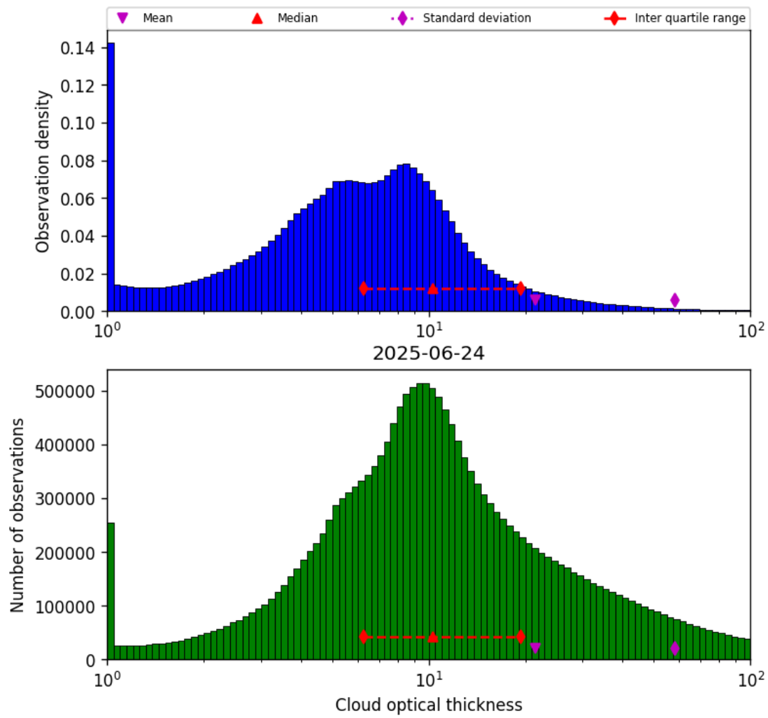
Figure 39: Histogram of “Cloud optical thickness” for 2025-06-24 to 2025-06-25
