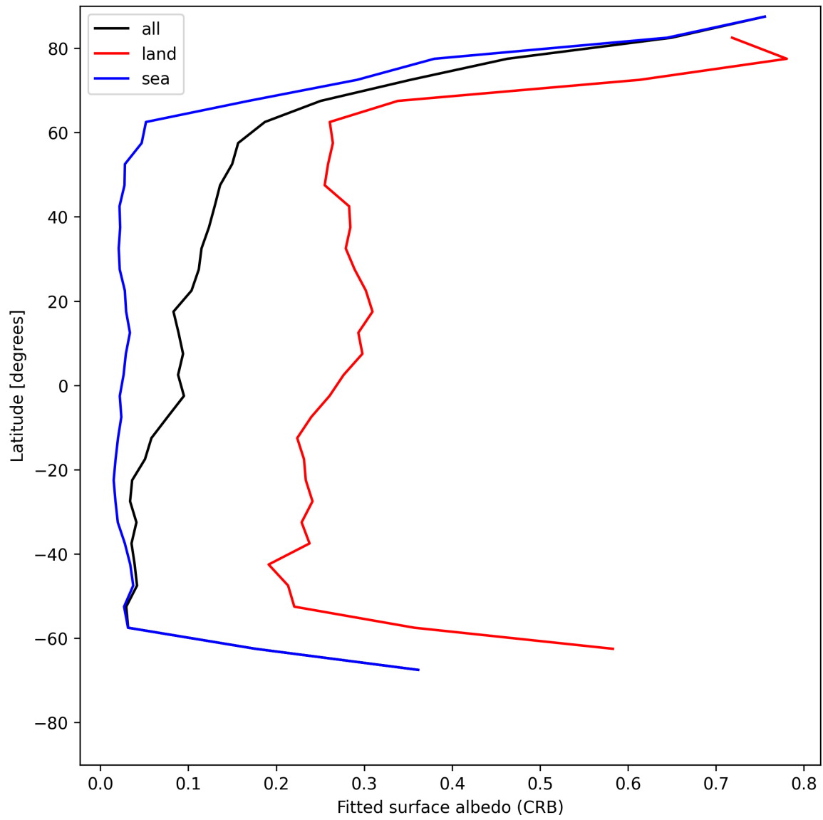
Figure 28: Zonal average of “Fitted surface albedo (CRB)” for 2025-06-24 to 2025-06-25.
