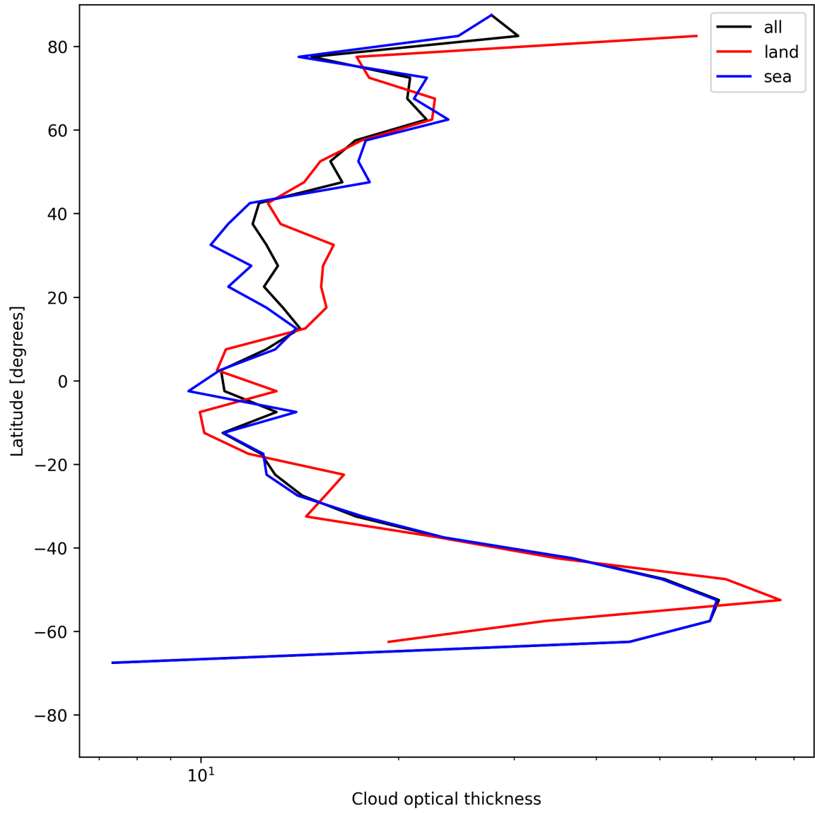
Figure 23: Zonal average of “Cloud optical thickness” for 2025-06-25 to 2025-06-25.
