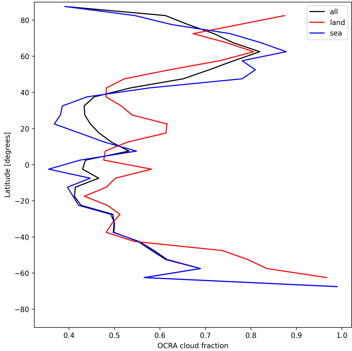
Figure 32: Zonal average of “OCRA cloud fraction” for 2025-06-25 to 2025-06-25.
