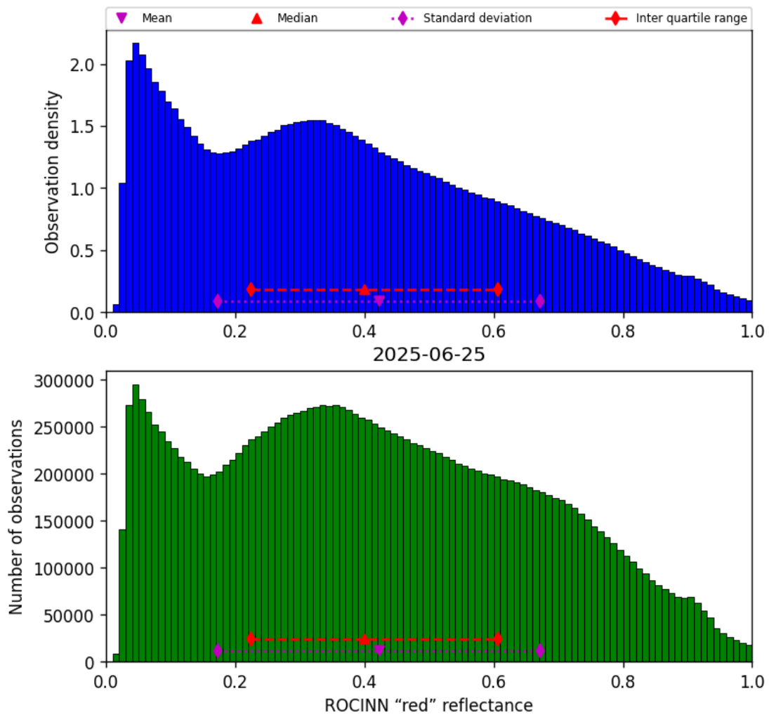
Figure 51: Histogram of “ROCINN “red” reflectance” for 2025-06-25 to 2025-06-25
