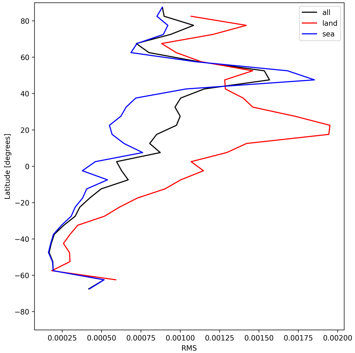
Figure 29: Zonal average of “RMS” for 2025-06-25 to 2025-06-25.
