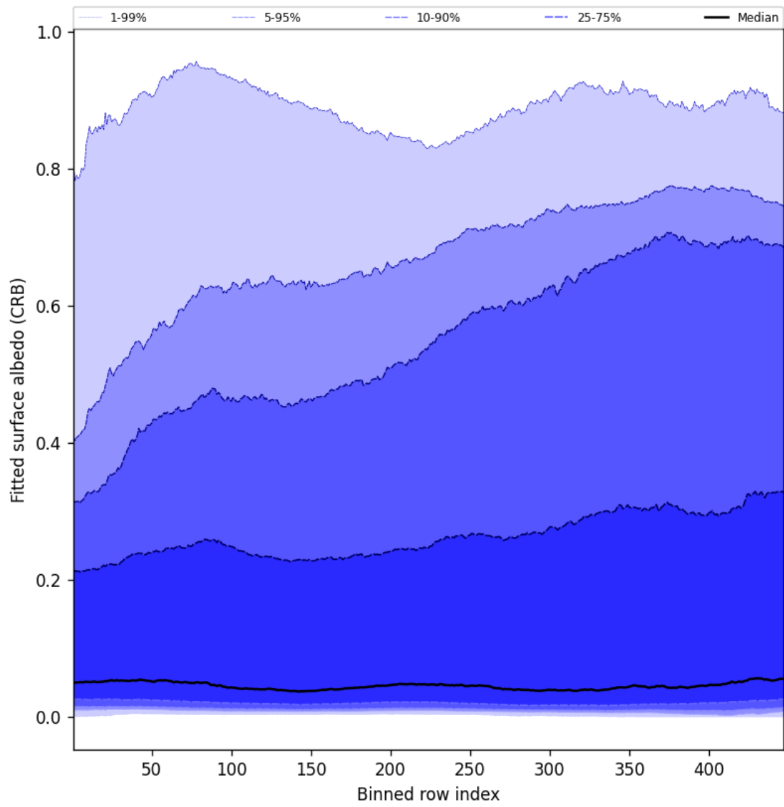
Figure 60: Along track statistics of “Fitted surface albedo (CRB)” for 2025-06-25 to 2025-06-25
