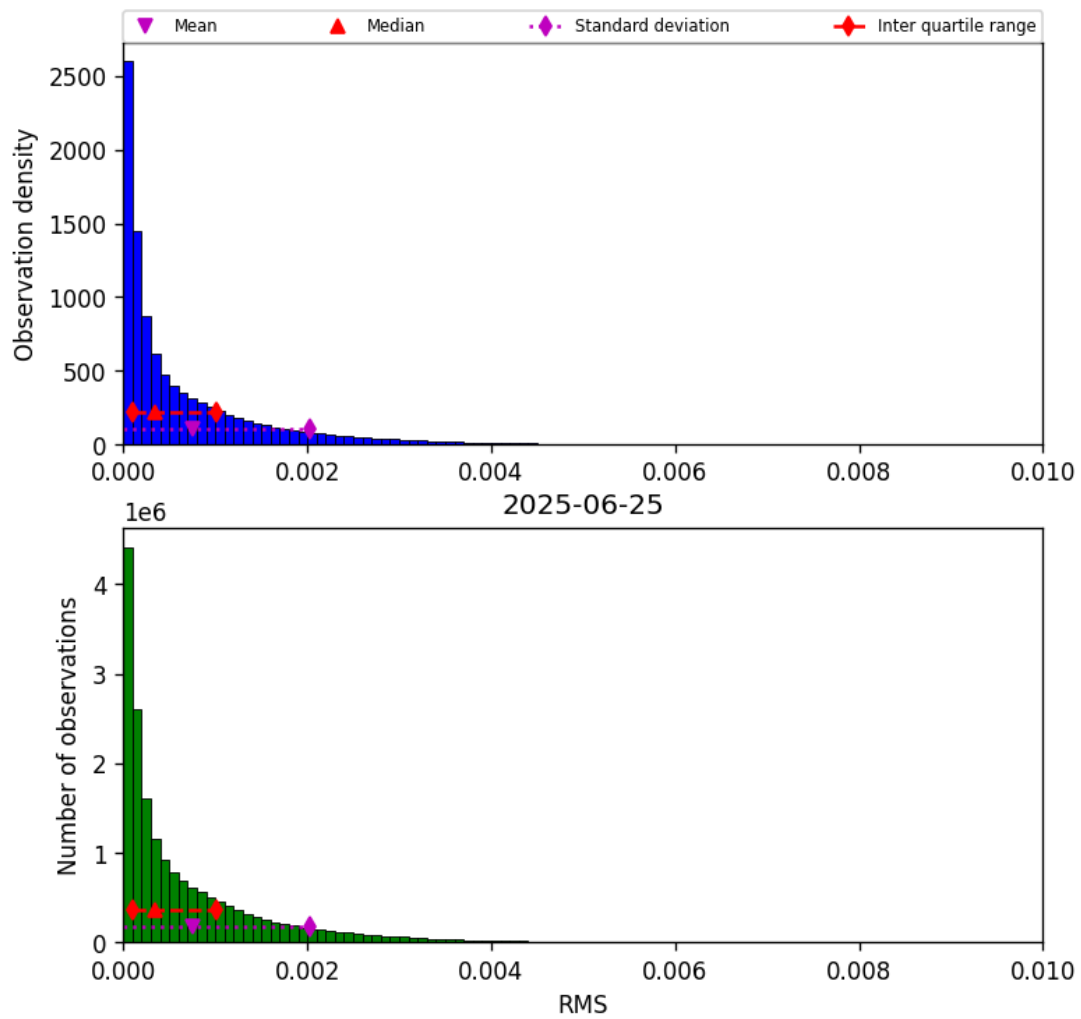
Figure 45: Histogram of “RMS” for 2025-06-25 to 2025-06-25
