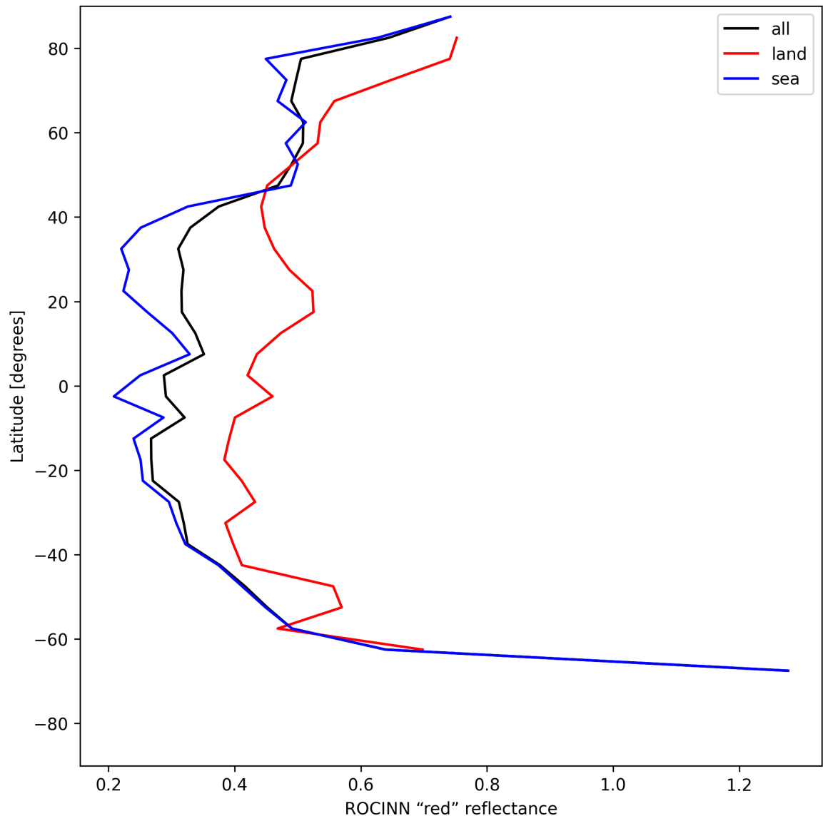
Figure 35: Zonal average of “ROCINN “red” reflectance” for 2025-06-25 to 2025-06-25.
