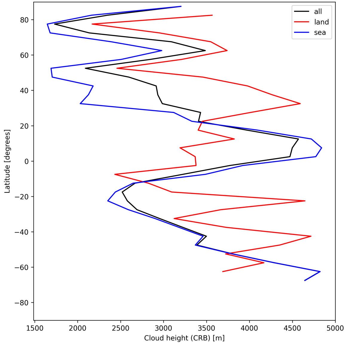
Figure 25: Zonal average of “Cloud height (CRB)” for 2025-06-25 to 2025-06-25.
