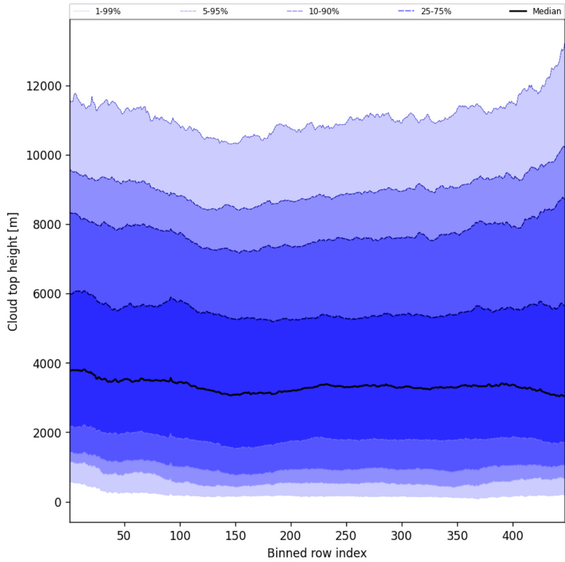
Figure 54: Along track statistics of “Cloud top height” for 2025-06-25 to 2025-06-25
