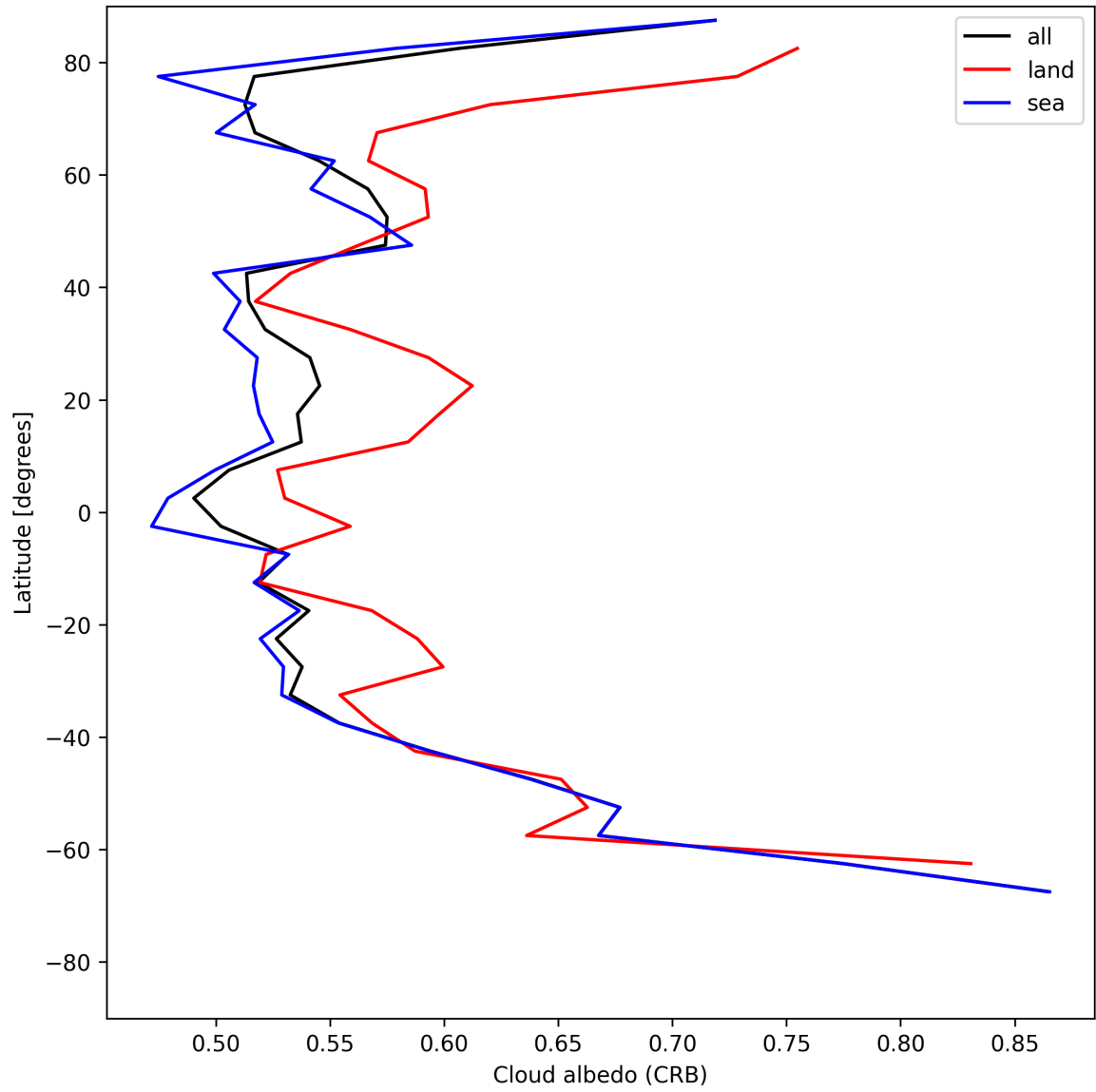
Figure 26: Zonal average of “Cloud albedo (CRB)” for 2025-06-25 to 2025-06-25.
