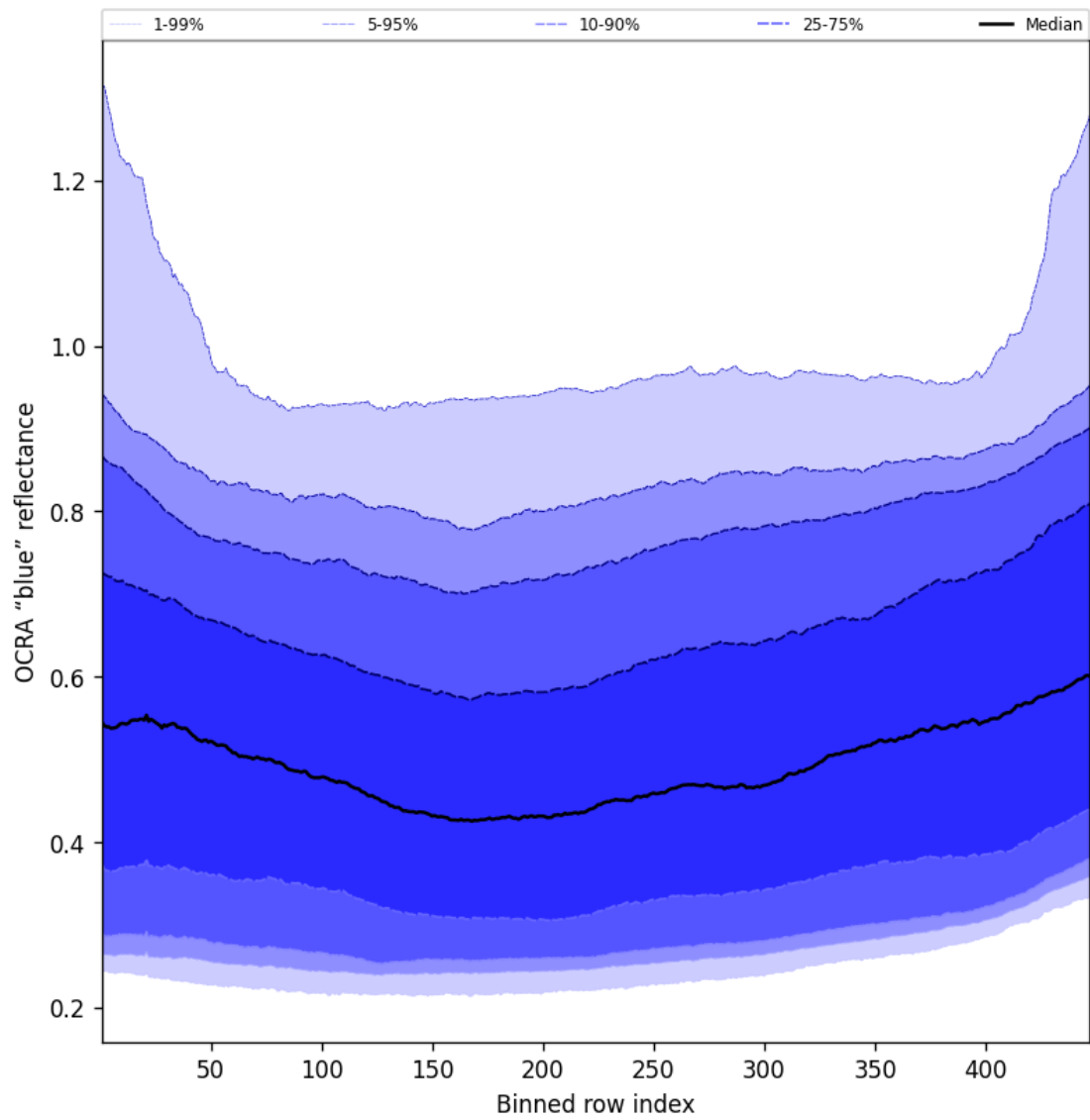
Figure 65: Along track statistics of “OCRA “blue” reflectance” for 2025-06-25 to 2025-06-25
