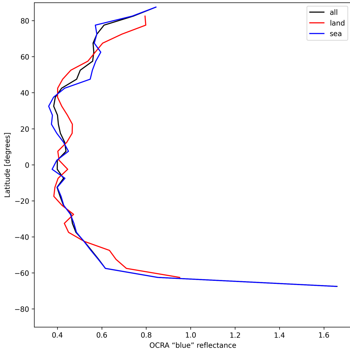
Figure 33: Zonal average of “OCRA “blue” reflectance” for 2025-06-25 to 2025-06-25.
