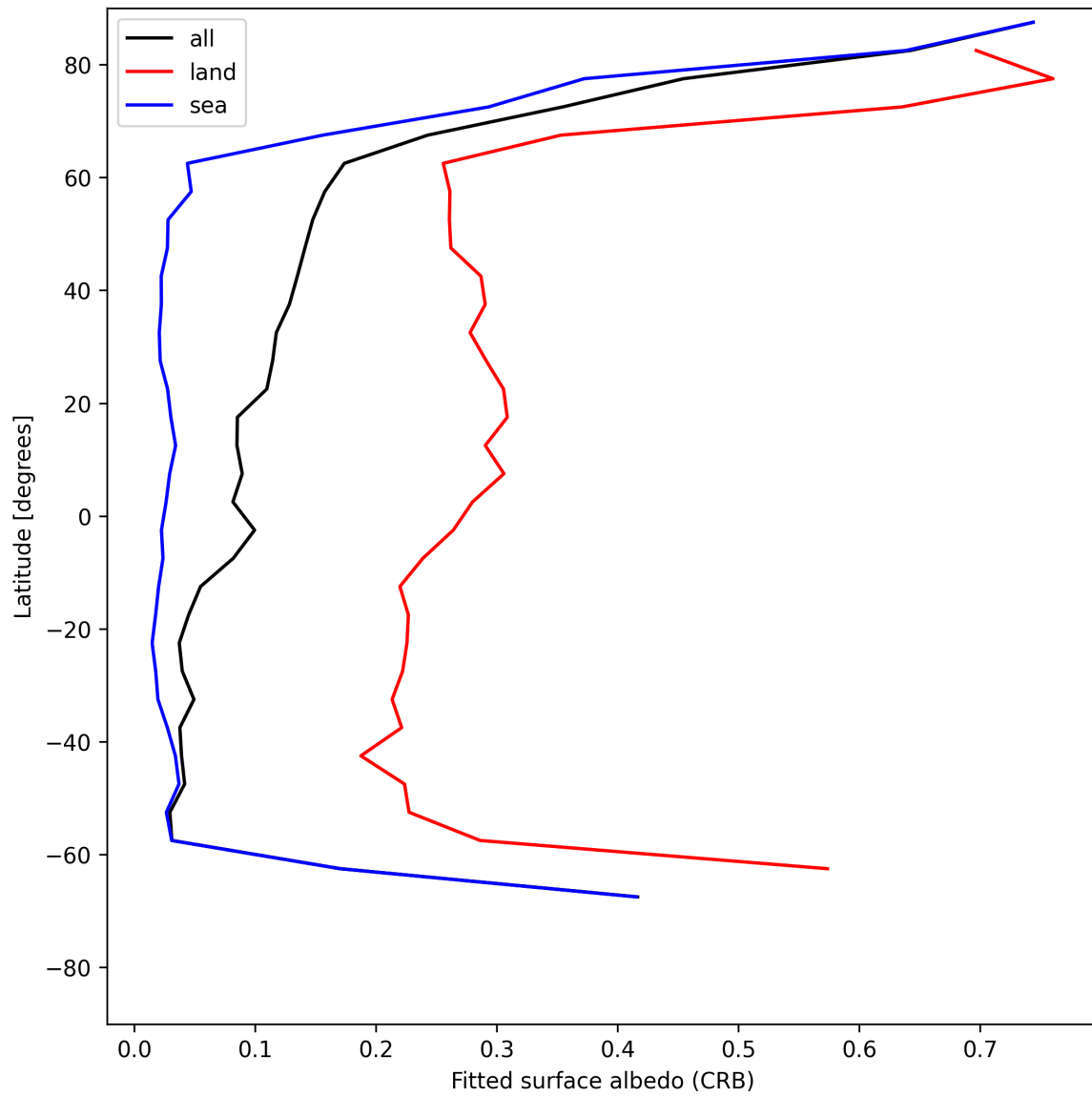
Figure 28: Zonal average of “Fitted surface albedo (CRB)” for 2025-06-25 to 2025-06-25.
