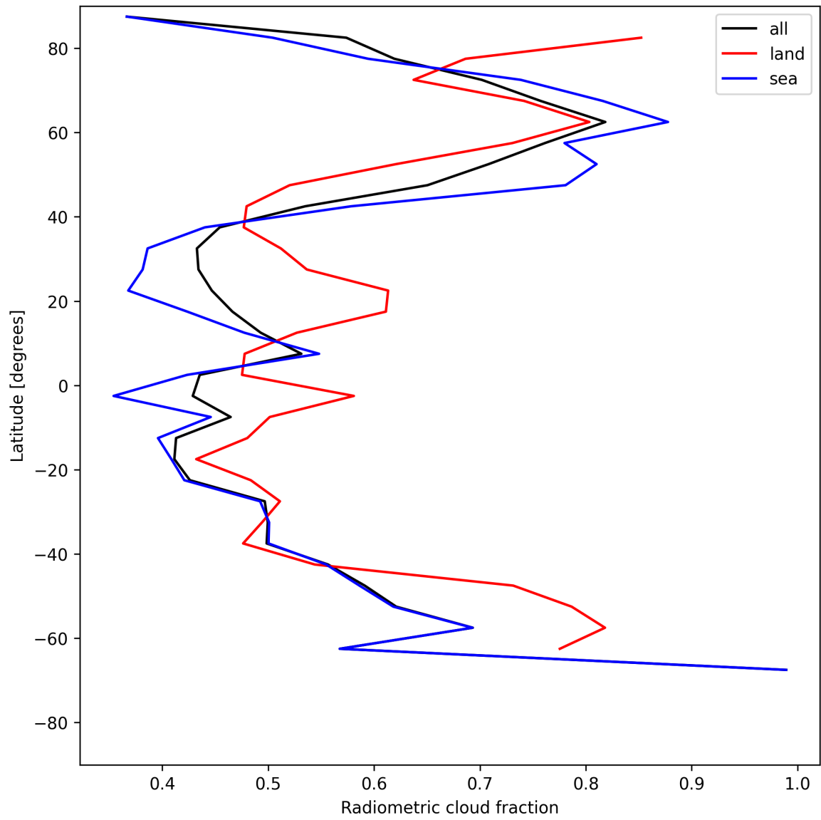
Figure 21: Zonal average of “Radiometric cloud fraction” for 2025-06-25 to 2025-06-25.
