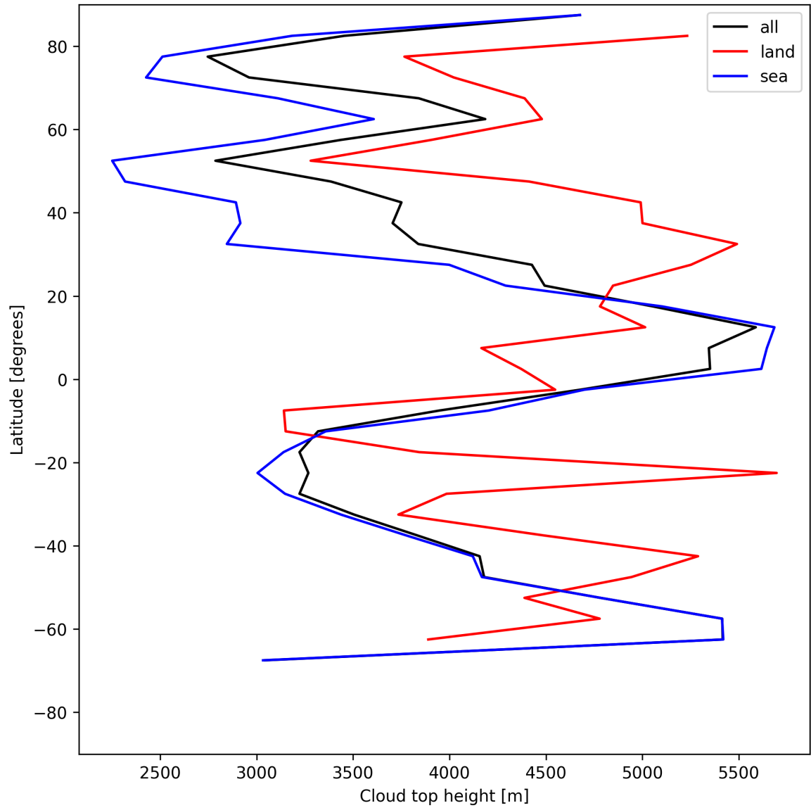
Figure 22: Zonal average of “Cloud top height” for 2025-06-25 to 2025-06-25.
