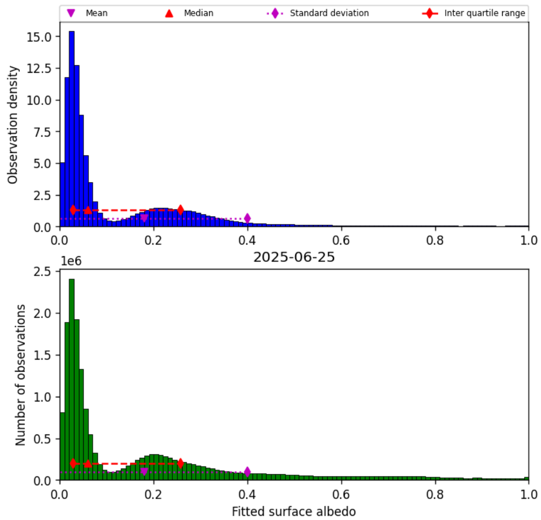
Figure 43: Histogram of “Fitted surface albedo” for 2025-06-25 to 2025-06-25
