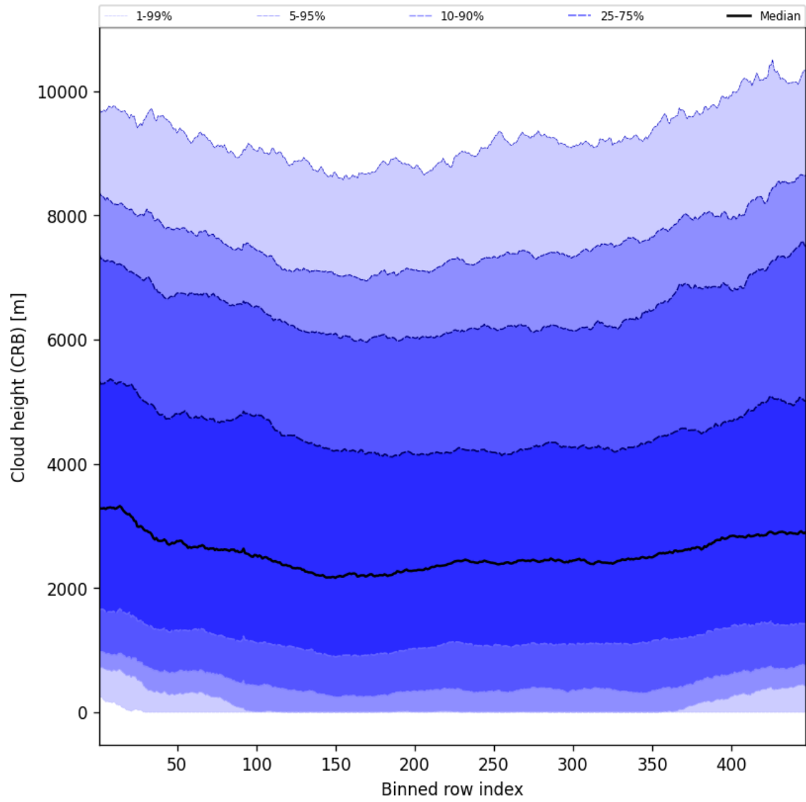
Figure 57: Along track statistics of “Cloud height (CRB)” for 2025-06-25 to 2025-06-25
