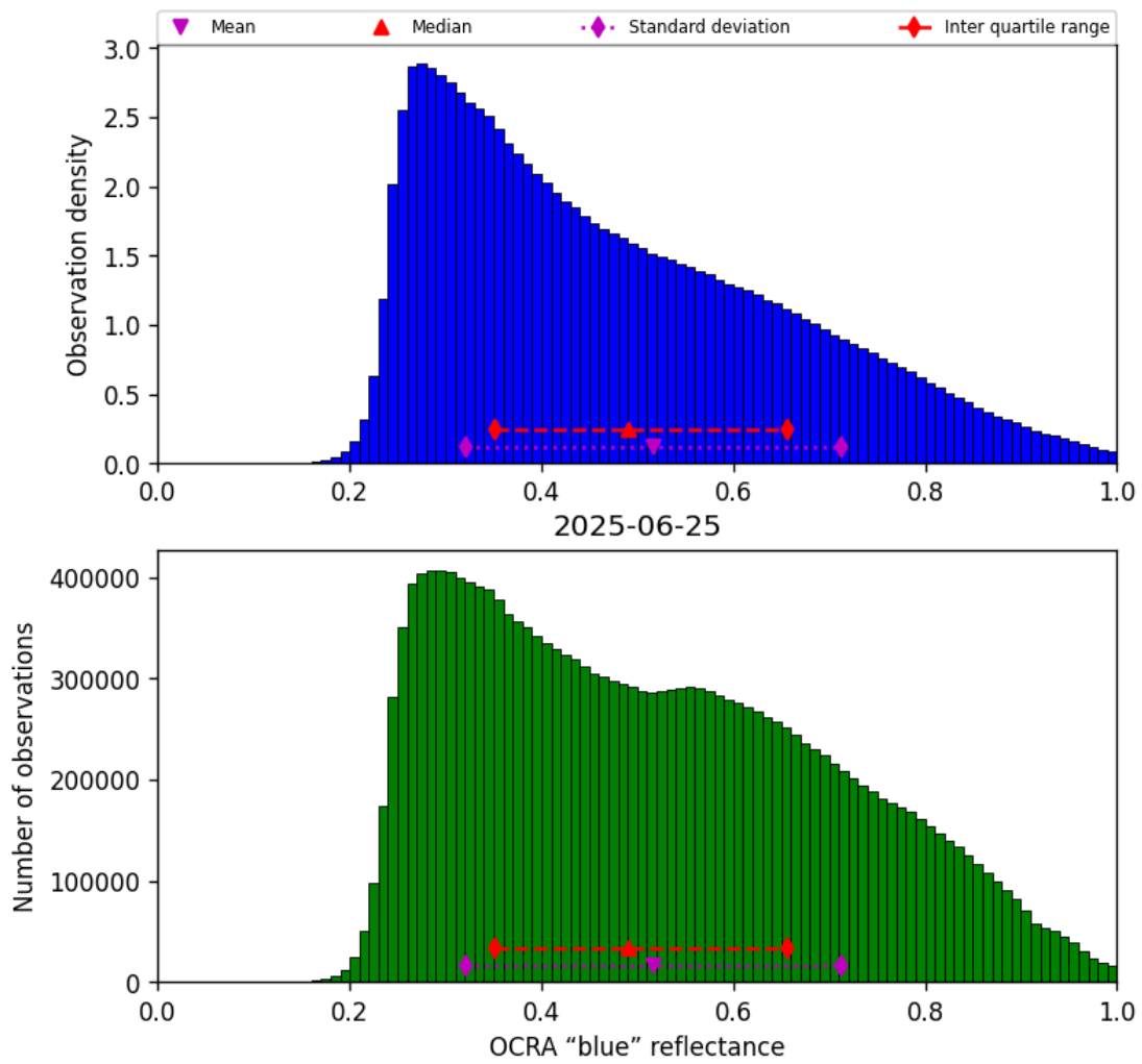
Figure 49: Histogram of “OCRA “blue” reflectance” for 2025-06-25 to 2025-06-25
