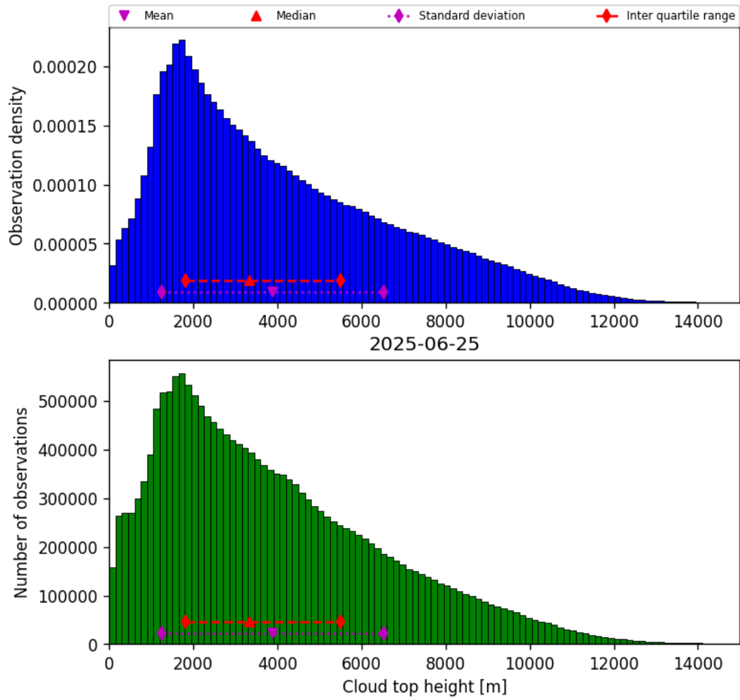
Figure 38: Histogram of “Cloud top height” for 2025-06-25 to 2025-06-25
