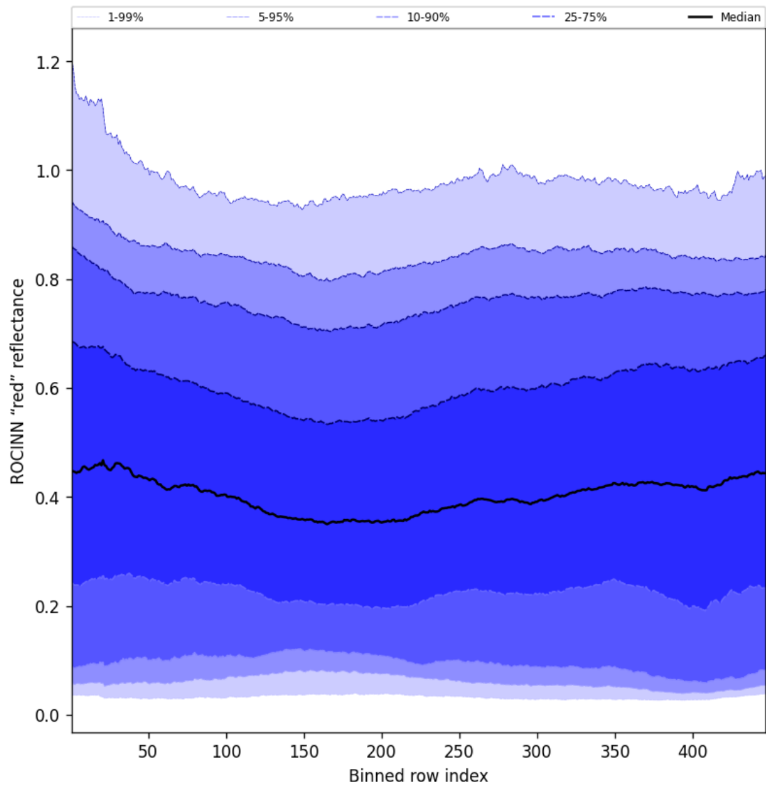
Figure 67: Along track statistics of "ROCINN "red" reflectance" for 2025-06-25 to 2025-06-25
