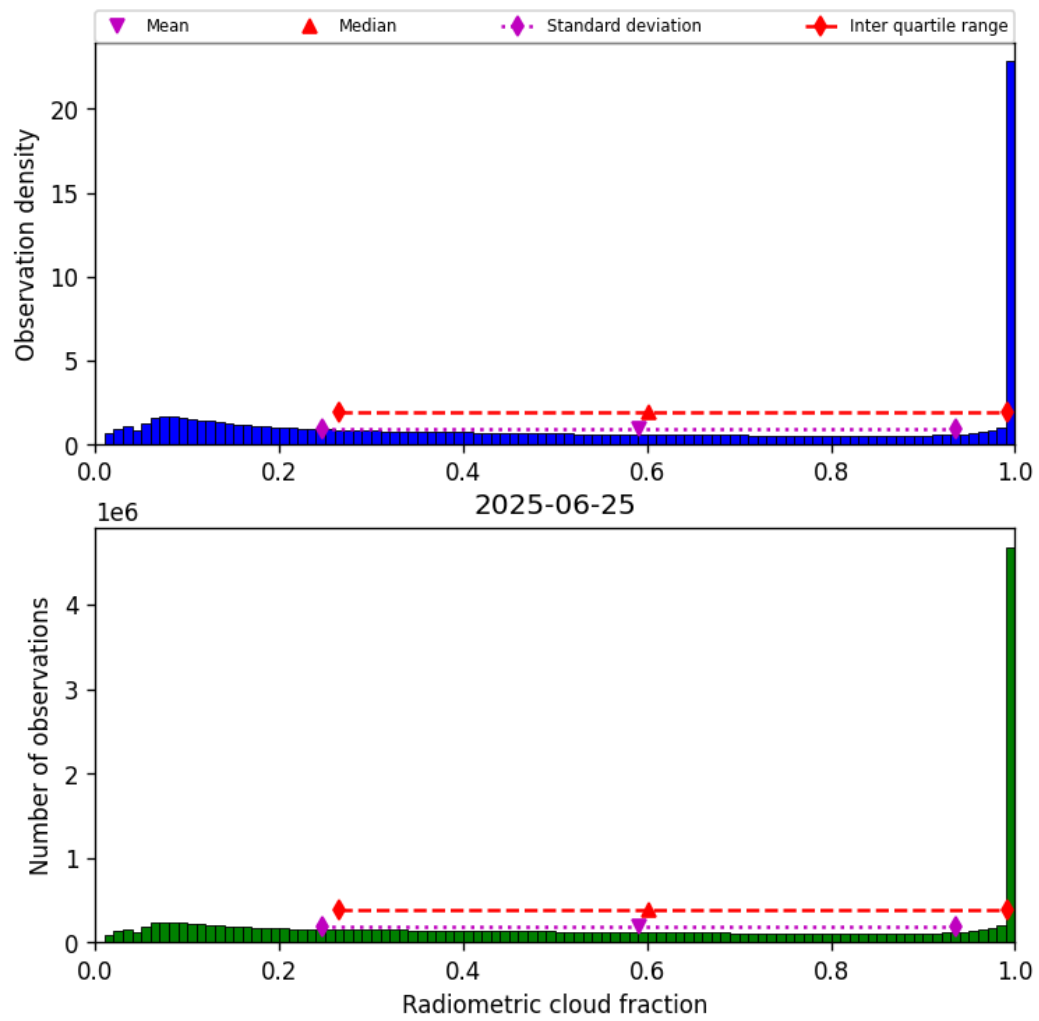
Figure 37: Histogram of “Radiometric cloud fraction” for 2025-06-25 to 2025-06-25
