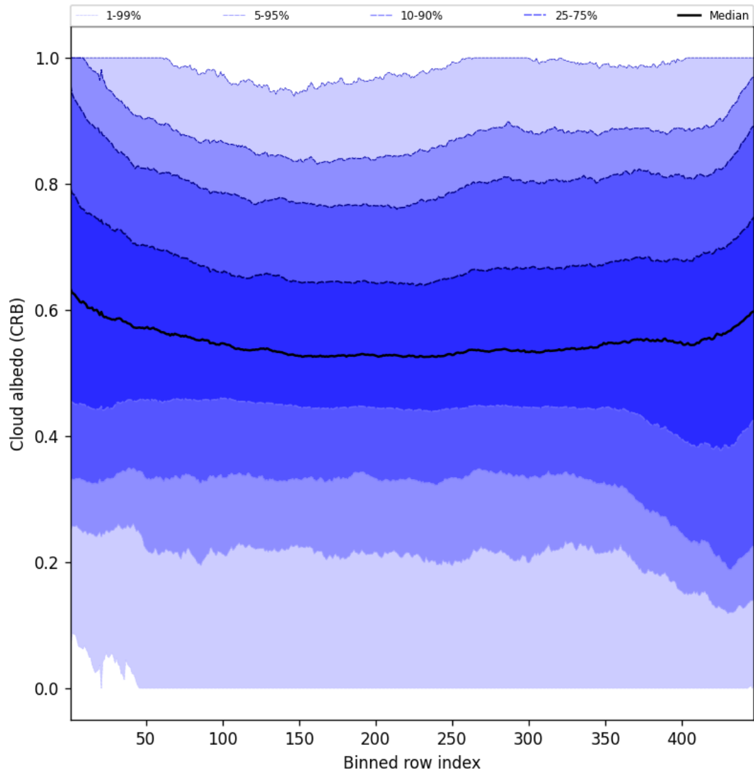
Figure 58: Along track statistics of “Cloud albedo (CRB)” for 2025-06-25 to 2025-06-25
