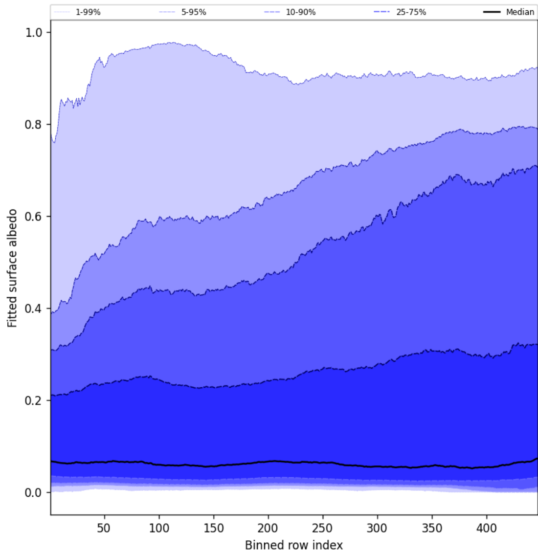
Figure 59: Along track statistics of “Fitted surface albedo” for 2025-06-25 to 2025-06-25
