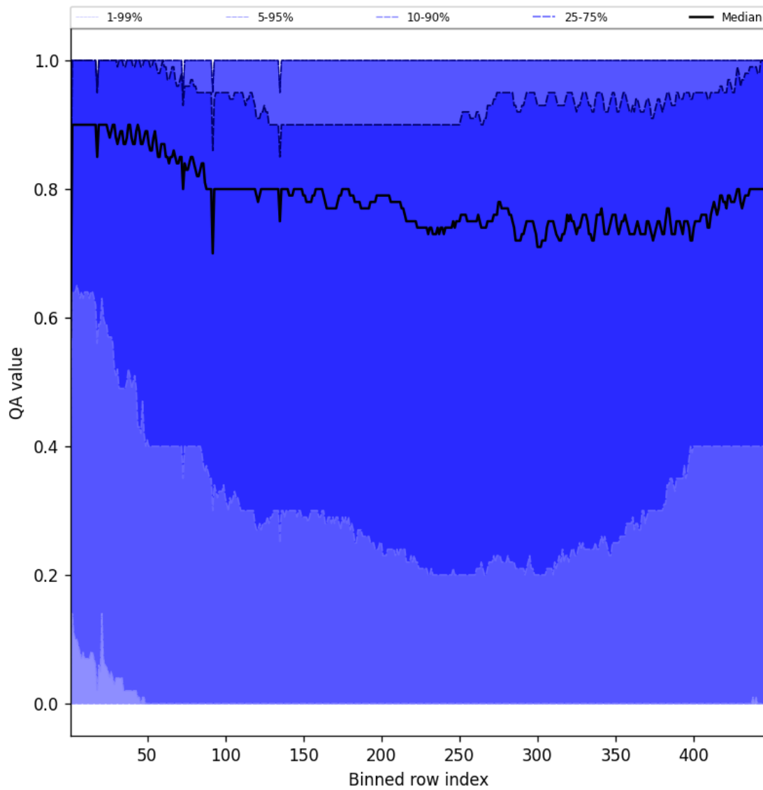
Figure 52: Along track statistics of “QA value” for 2025-06-25 to 2025-06-25
