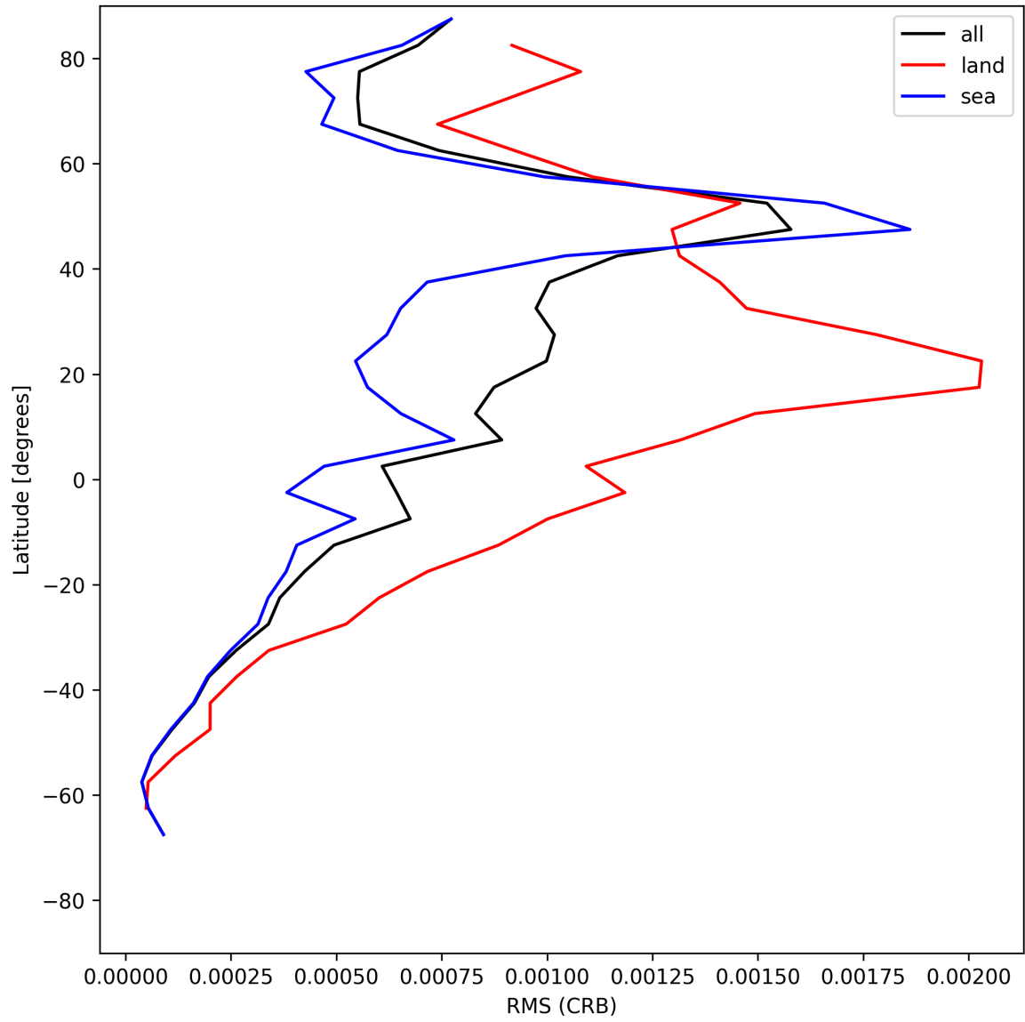
Figure 30: Zonal average of “RMS (CRB)” for 2025-06-25 to 2025-06-25.
