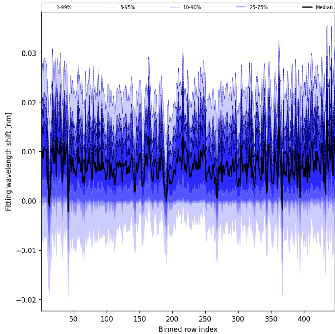
Figure 63: Along track statistics of “Fitting wavelength shift” for 2025-06-25 to 2025-06-25
