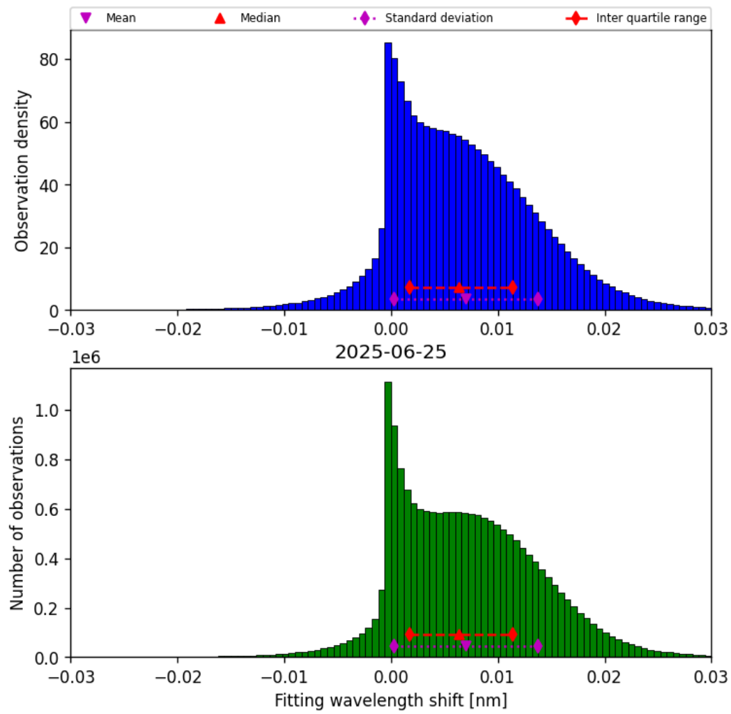
Figure 47: Histogram of “Fitting wavelength shift” for 2025-06-25 to 2025-06-25
