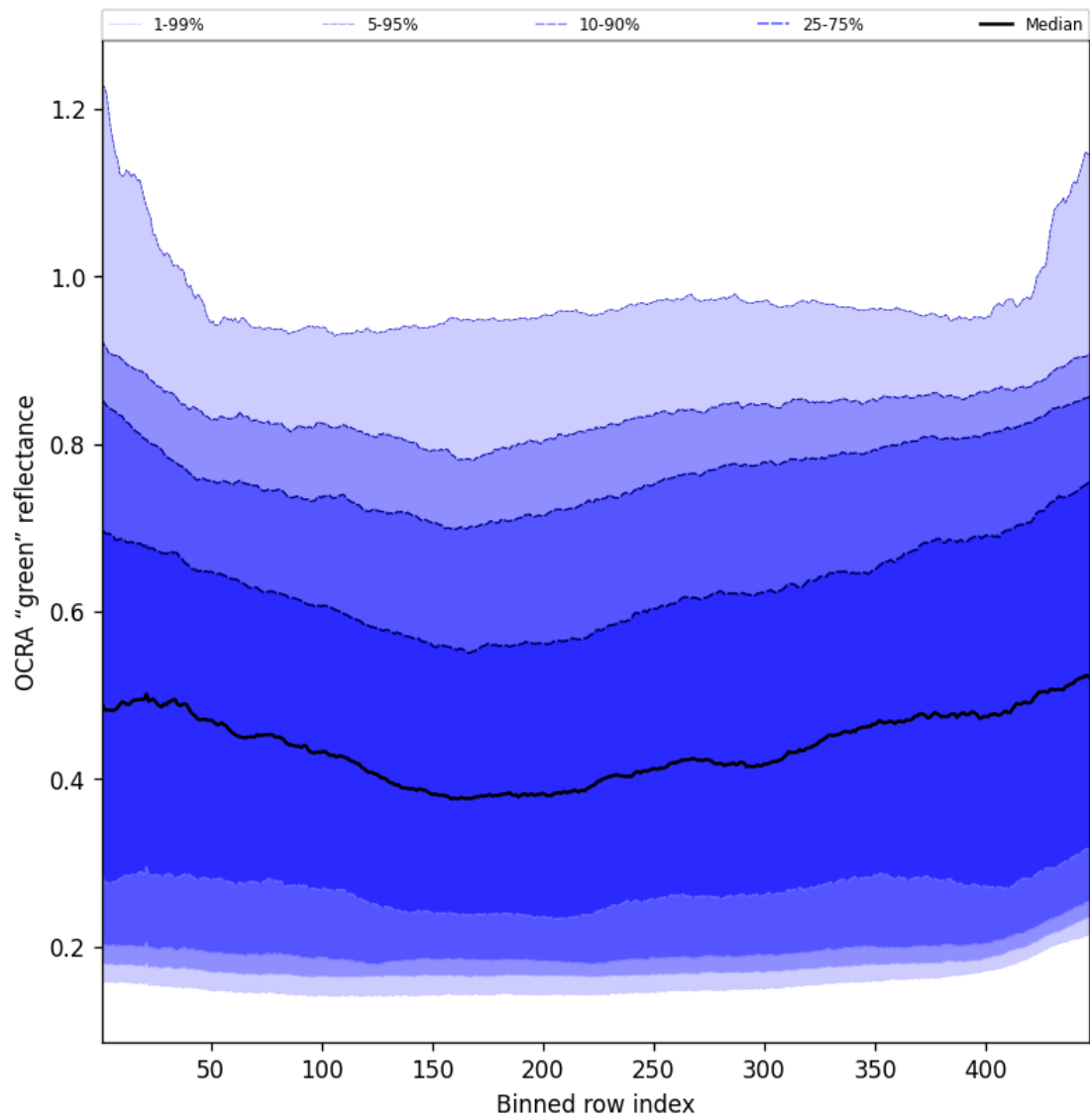
Figure 66: Along track statistics of “OCRA “green” reflectance” for 2025-06-25 to 2025-06-25
