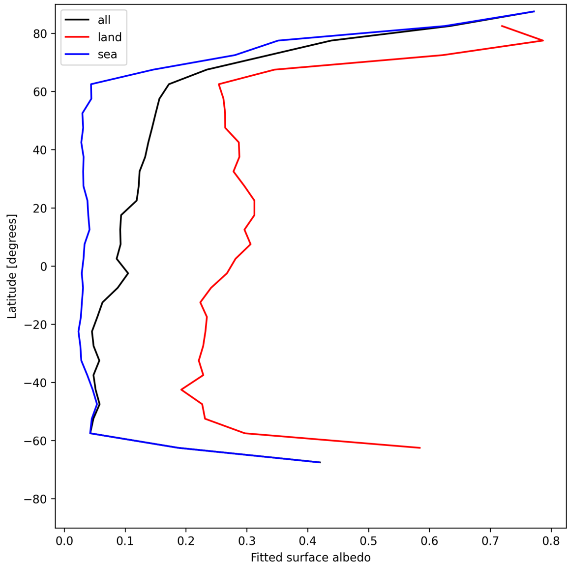
Figure 27: Zonal average of “Fitted surface albedo” for 2025-06-25 to 2025-06-25.
