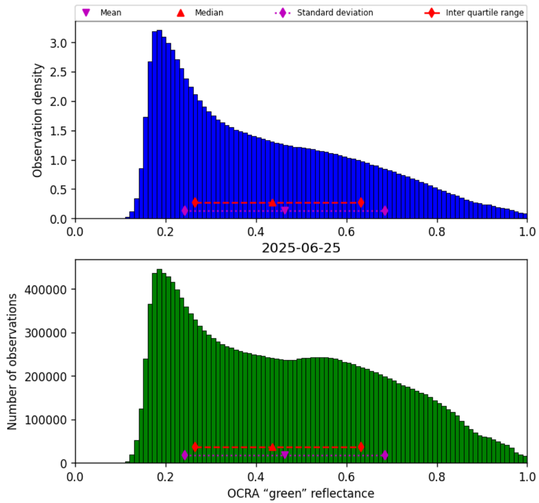
Figure 50: Histogram of “OCRA “green” reflectance” for 2025-06-25 to 2025-06-25
