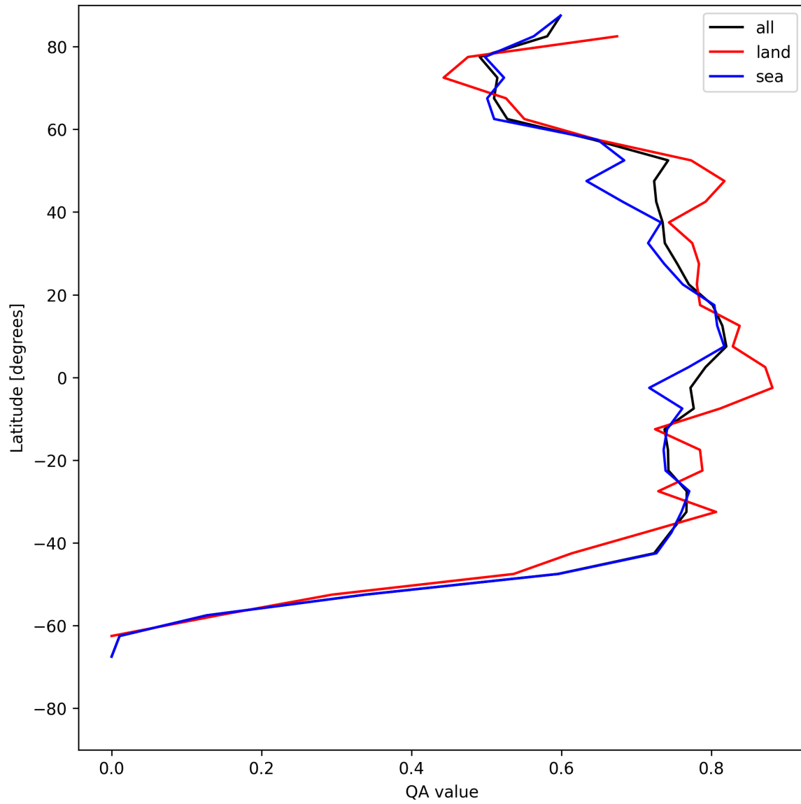
Figure 20: Zonal average of “QA value” for 2025-06-25 to 2025-06-25.
