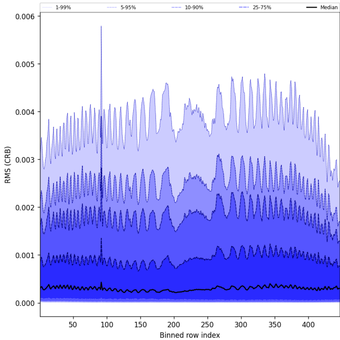
Figure 62: Along track statistics of “RMS (CRB)” for 2025-06-25 to 2025-06-25
