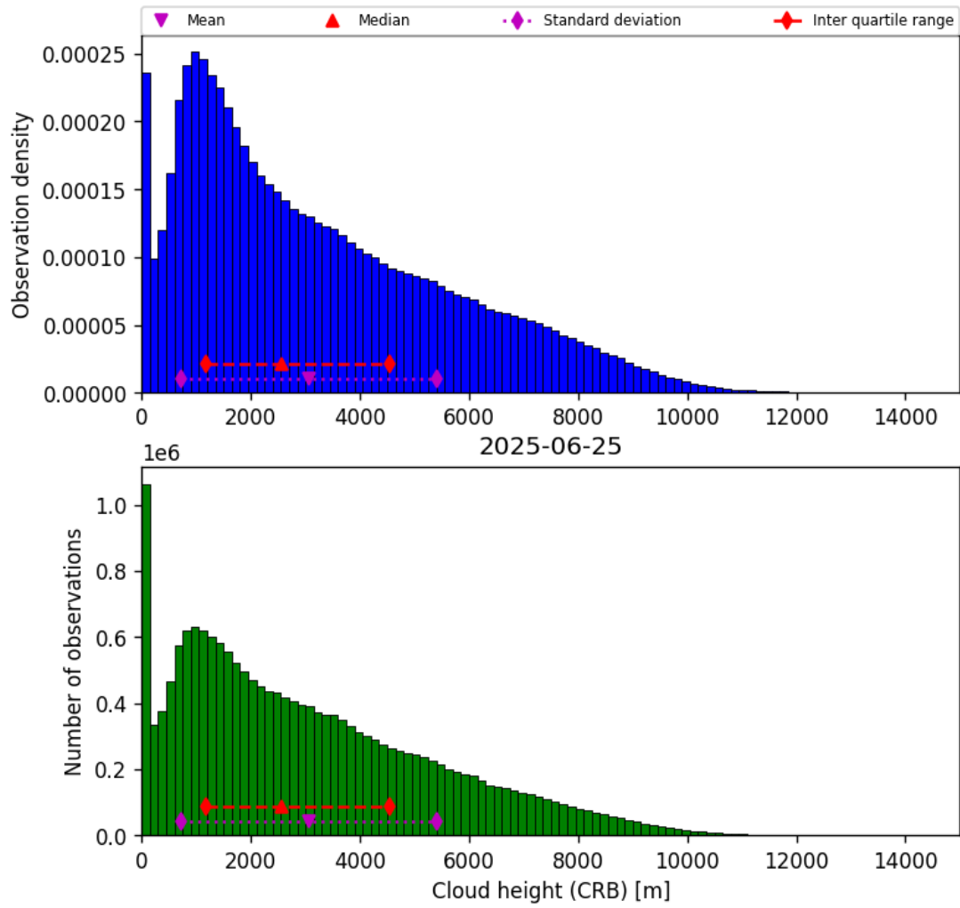
Figure 41: Histogram of “Cloud height (CRB)” for 2025-06-25 to 2025-06-25
