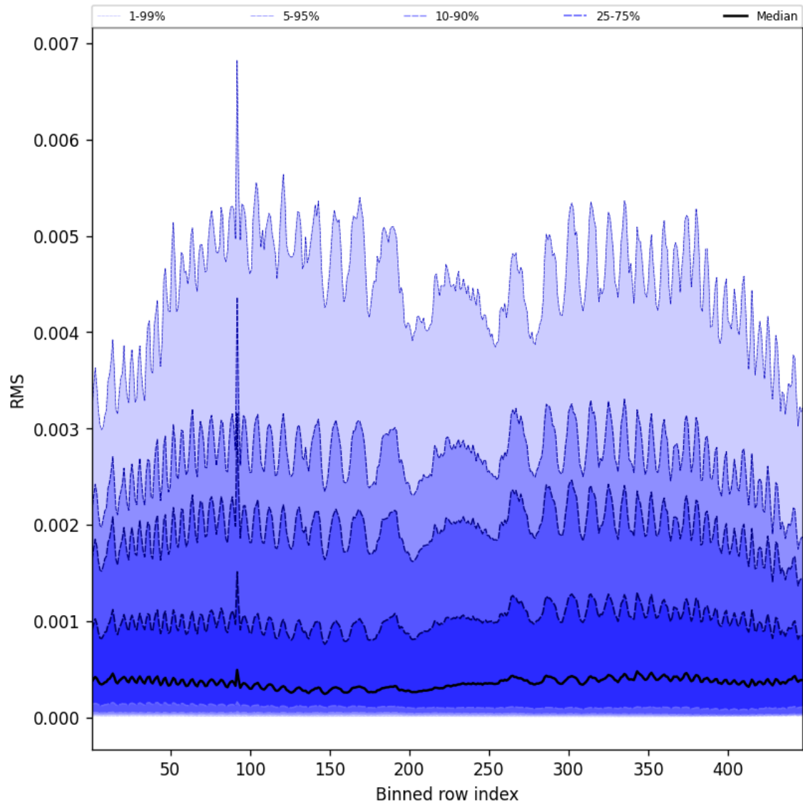
Figure 61: Along track statistics of “RMS” for 2025-06-25 to 2025-06-25
