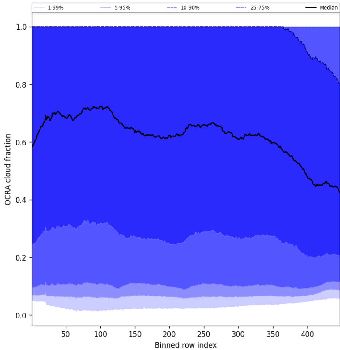
Figure 64: Along track statistics of “OCRA cloud fraction” for 2025-06-25 to 2025-06-25
