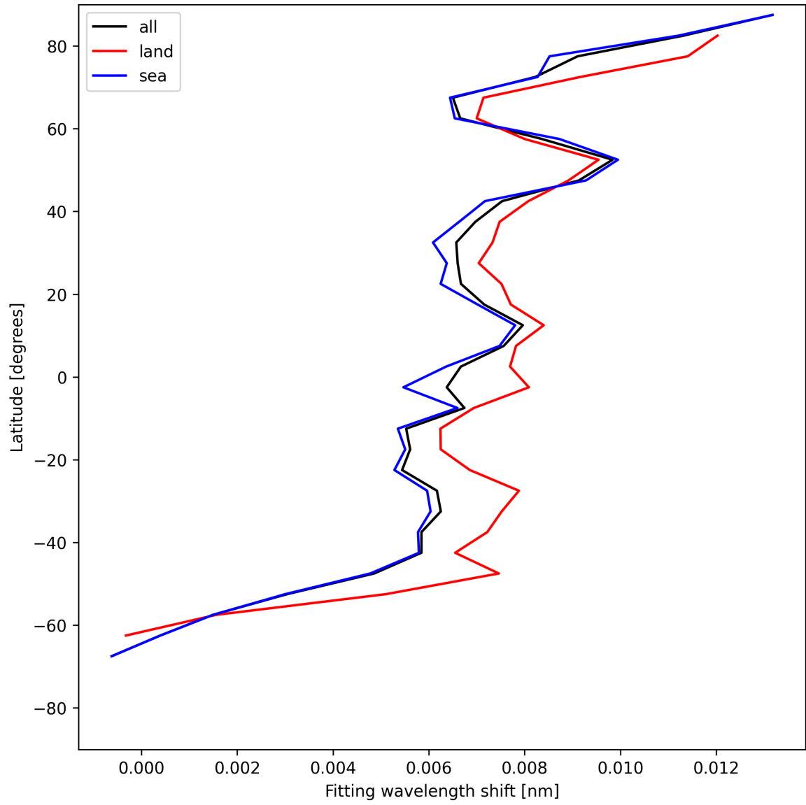
Figure 31: Zonal average of “Fitting wavelength shift” for 2025-06-25 to 2025-06-25.
