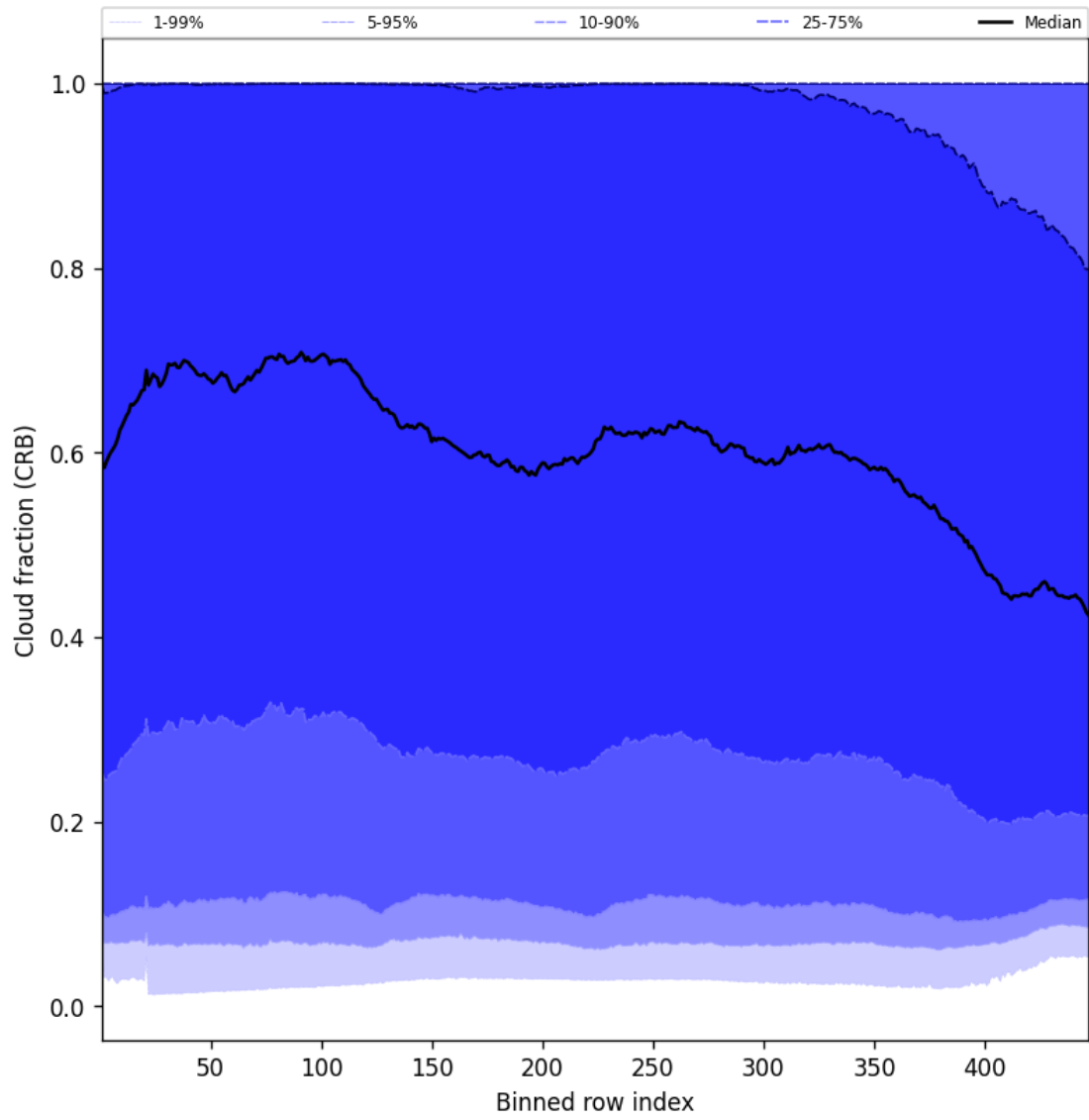
Figure 56: Along track statistics of “Cloud fraction (CRB)” for 2025-06-25 to 2025-06-25
