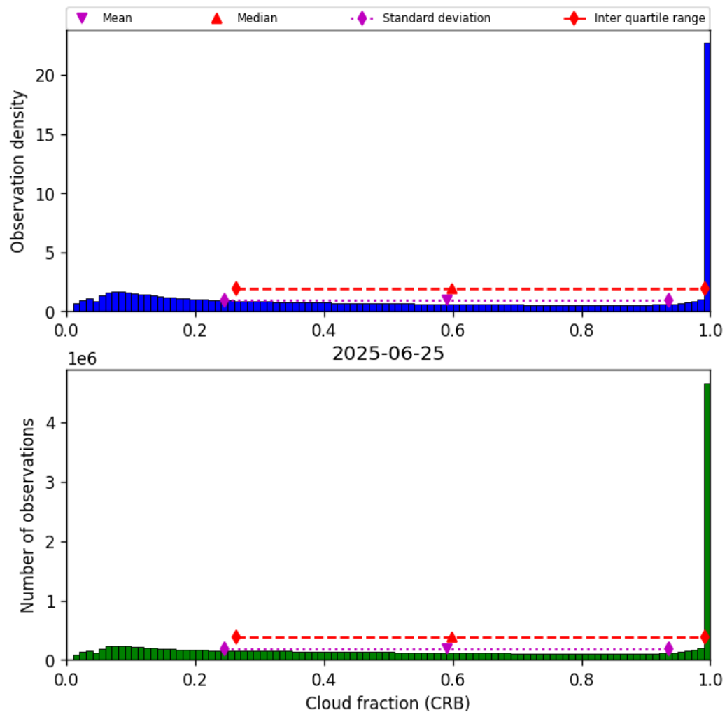
Figure 40: Histogram of “Cloud fraction (CRB)” for 2025-06-25 to 2025-06-25
