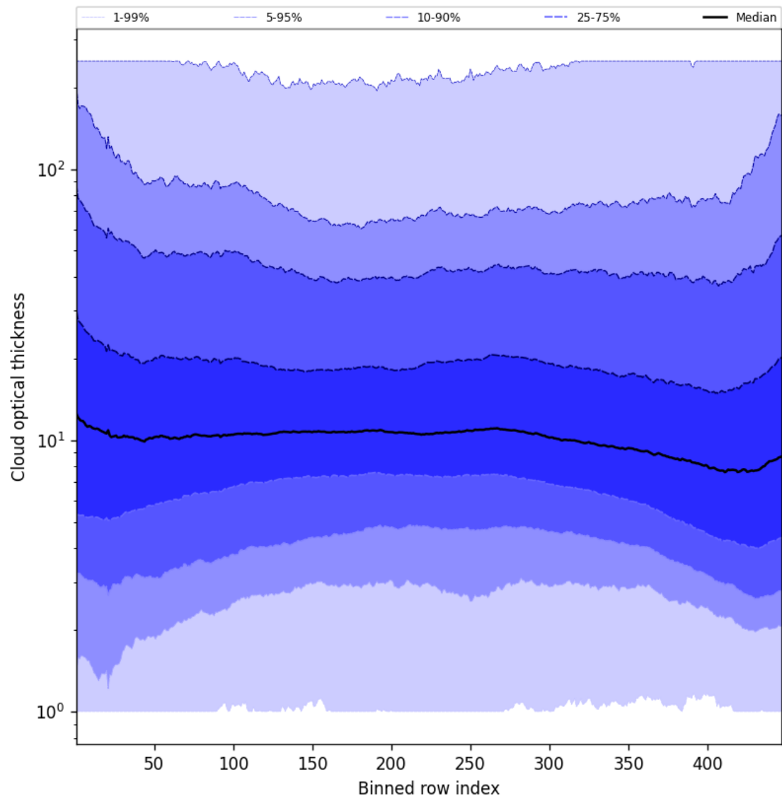
Figure 55: Along track statistics of “Cloud optical thickness” for 2025-06-25 to 2025-06-25
