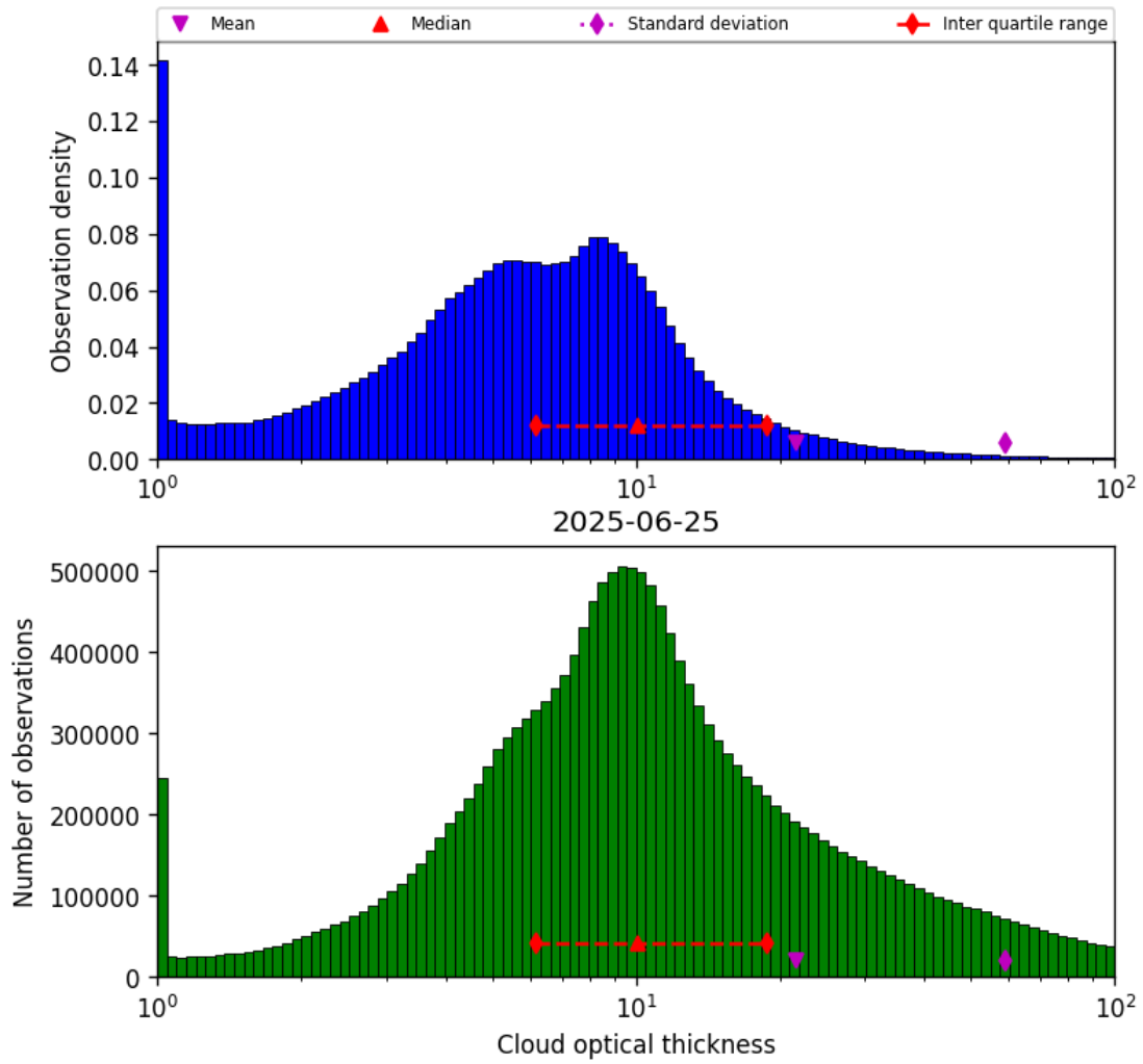
Figure 39: Histogram of “Cloud optical thickness” for 2025-06-25 to 2025-06-25
