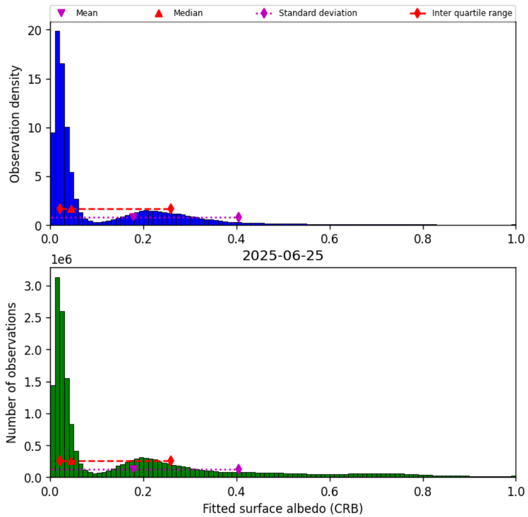
Figure 44: Histogram of “Fitted surface albedo (CRB)” for 2025-06-25 to 2025-06-25
