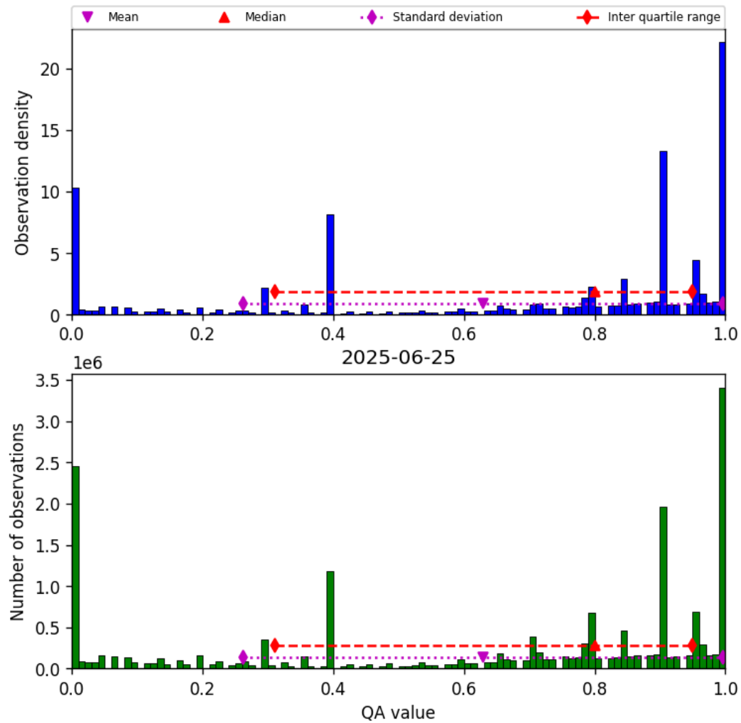
Figure 36: Histogram of “QA value” for 2025-06-25 to 2025-06-25
