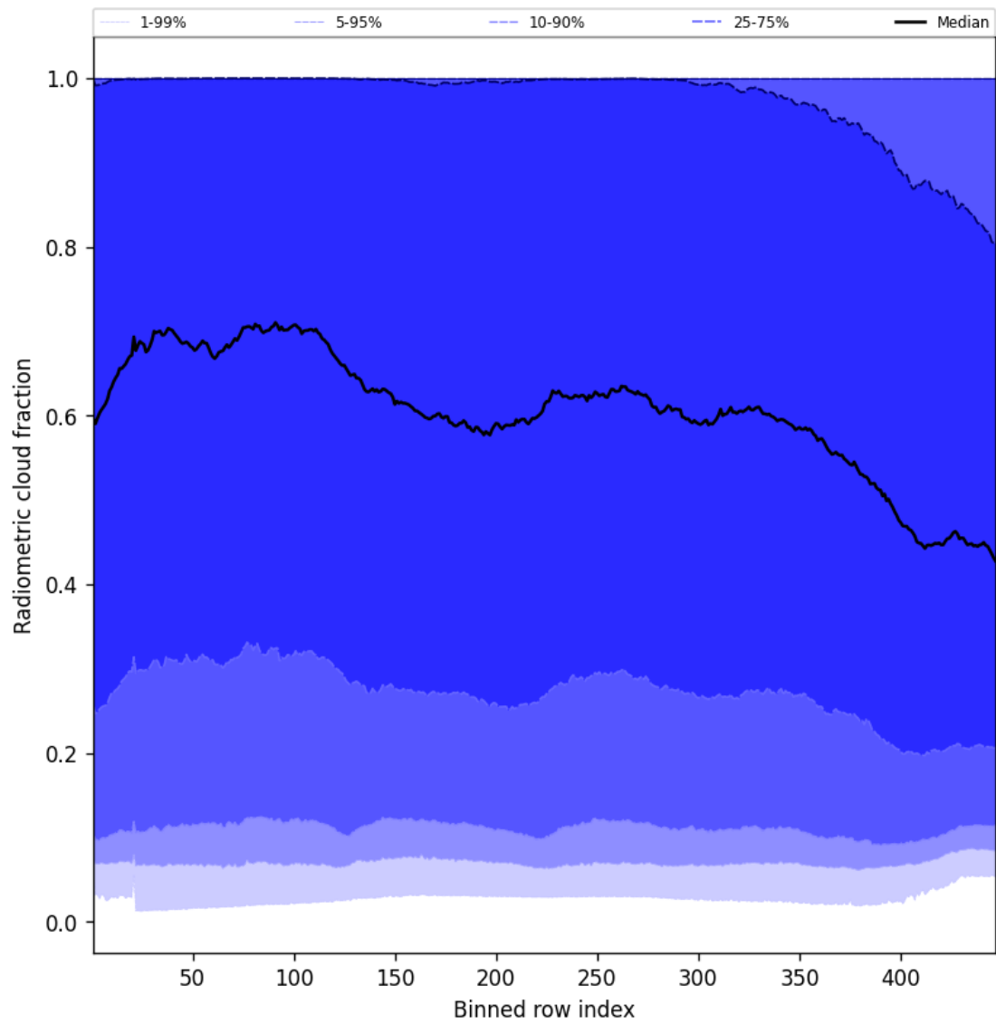
Figure 53: Along track statistics of “Radiometric cloud fraction” for 2025-06-25 to 2025-06-25
