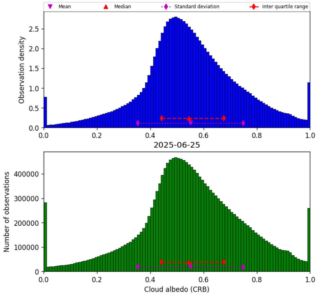
Figure 42: Histogram of “Cloud albedo (CRB)” for 2025-06-25 to 2025-06-25
