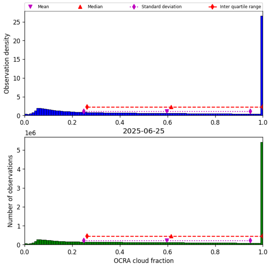
Figure 48: Histogram of “OCRA cloud fraction” for 2025-06-25 to 2025-06-25
