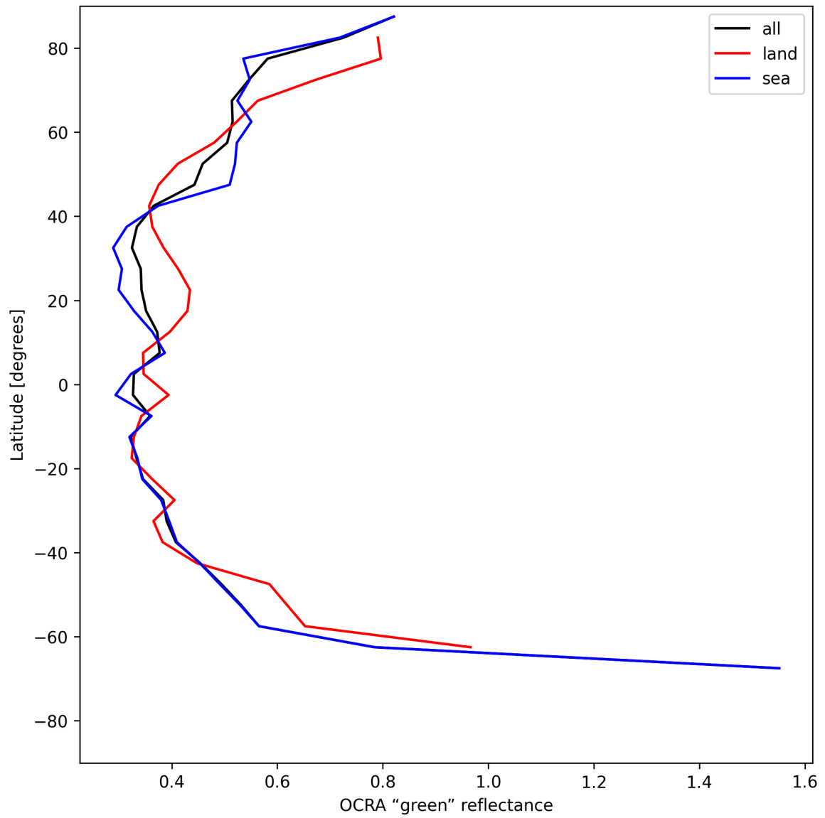
Figure 34: Zonal average of “OCRA “green” reflectance” for 2025-06-25 to 2025-06-25.
