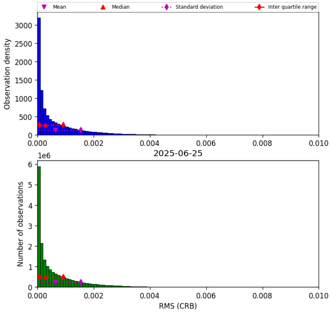
Figure 46: Histogram of “RMS (CRB)” for 2025-06-25 to 2025-06-25
