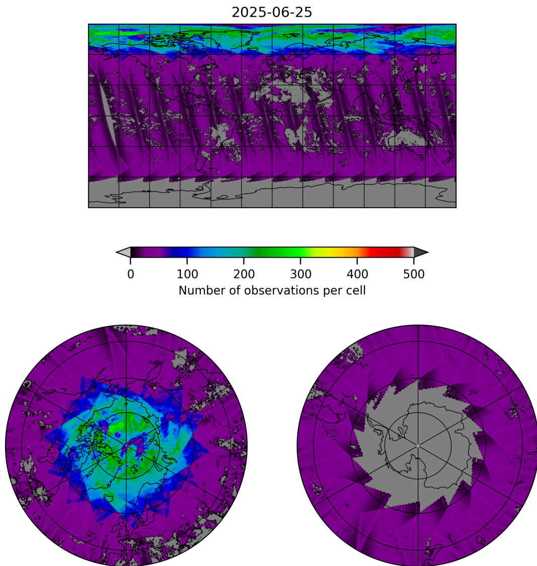
Figure 19: Map of the number of observations for 2025-06-25 to 2025-06-25
