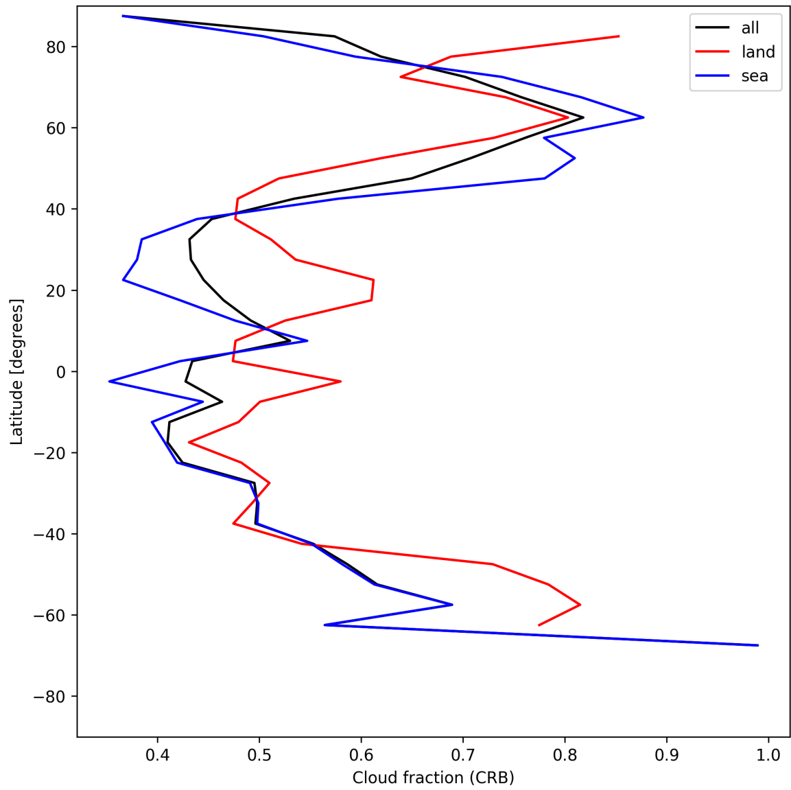
Figure 24: Zonal average of “Cloud fraction (CRB)” for 2025-06-25 to 2025-06-25.
