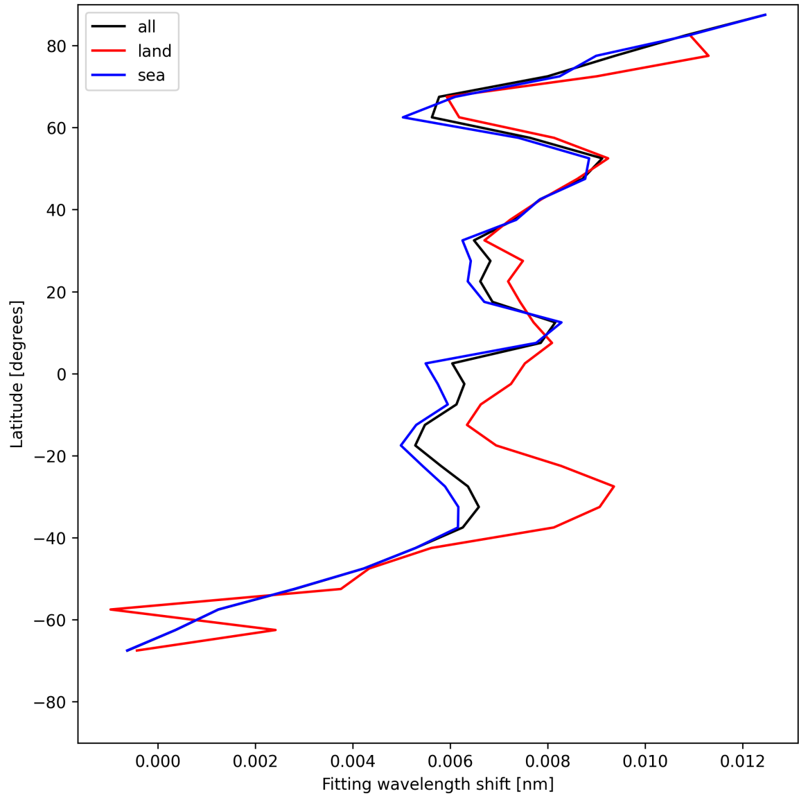
Figure 31: Zonal average of “Fitting wavelength shift” for 2025-06-29 to 2025-06-30.
