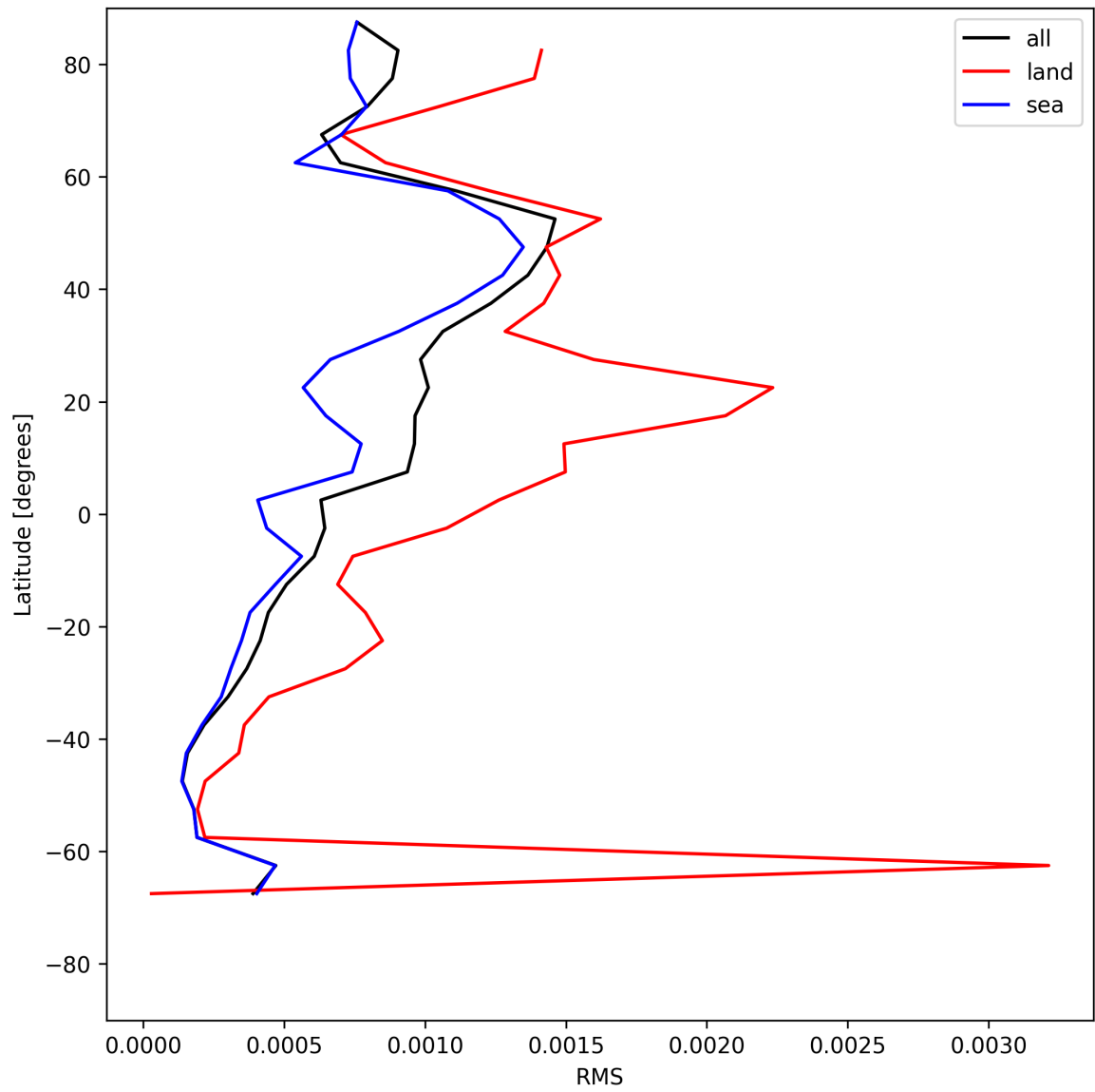
Figure 29: Zonal average of “RMS” for 2025-06-29 to 2025-06-30.
