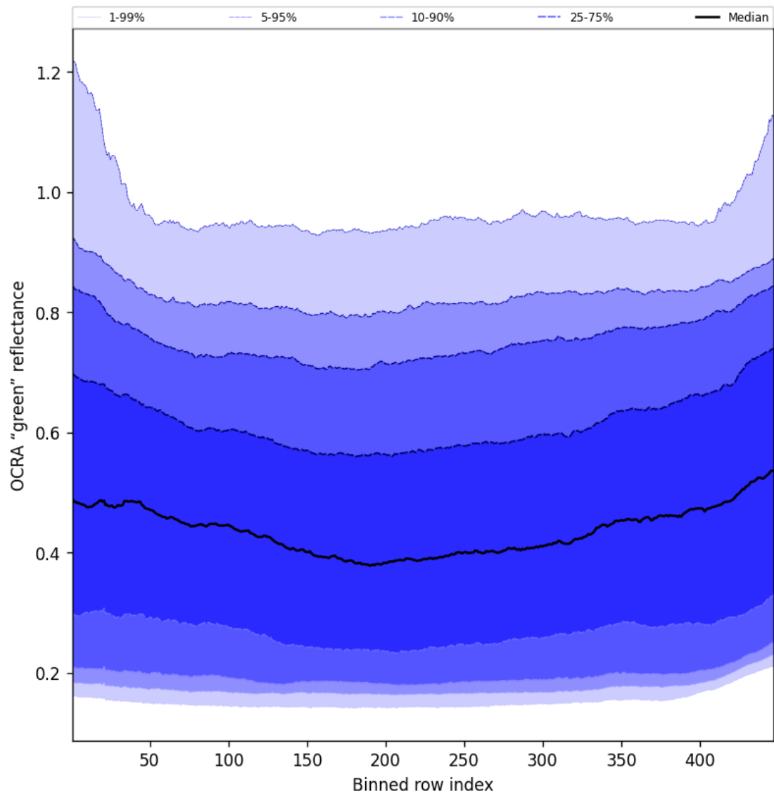
Figure 66: Along track statistics of “OCRA “green” reflectance” for 2025-06-29 to 2025-06-30
