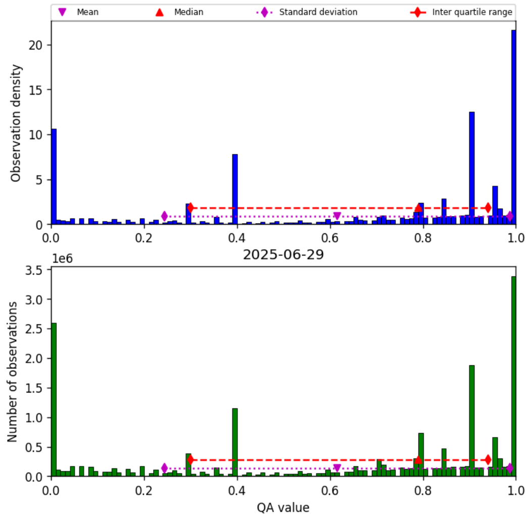
Figure 36: Histogram of “QA value” for 2025-06-29 to 2025-06-30
