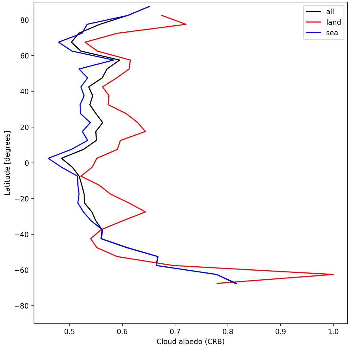
Figure 26: Zonal average of “Cloud albedo (CRB)” for 2025-06-29 to 2025-06-30.
