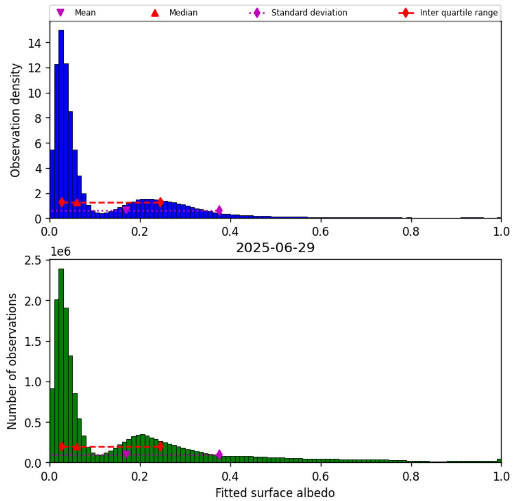
Figure 43: Histogram of “Fitted surface albedo” for 2025-06-29 to 2025-06-30
