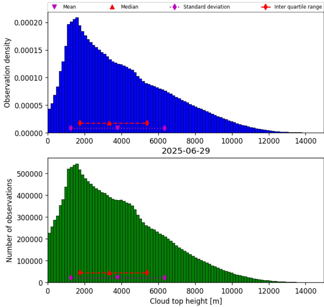
Figure 38: Histogram of “Cloud top height” for 2025-06-29 to 2025-06-30
