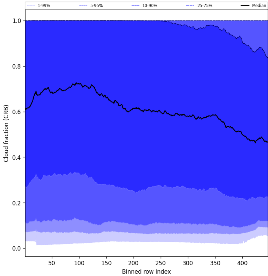
Figure 56: Along track statistics of “Cloud fraction (CRB)” for 2025-06-29 to 2025-06-30
