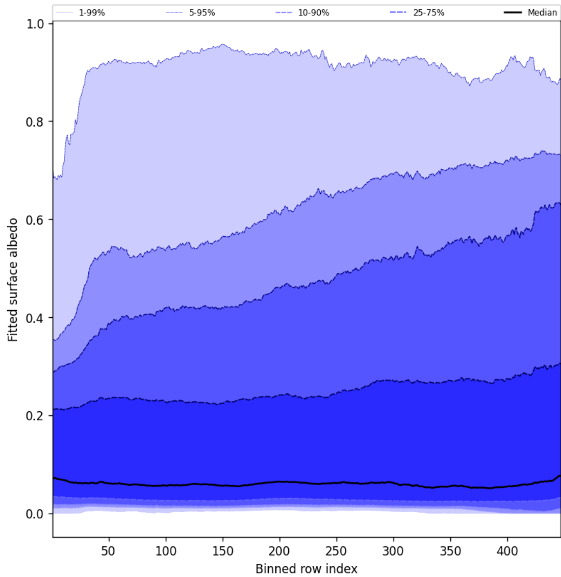
Figure 59: Along track statistics of “Fitted surface albedo” for 2025-06-29 to 2025-06-30
