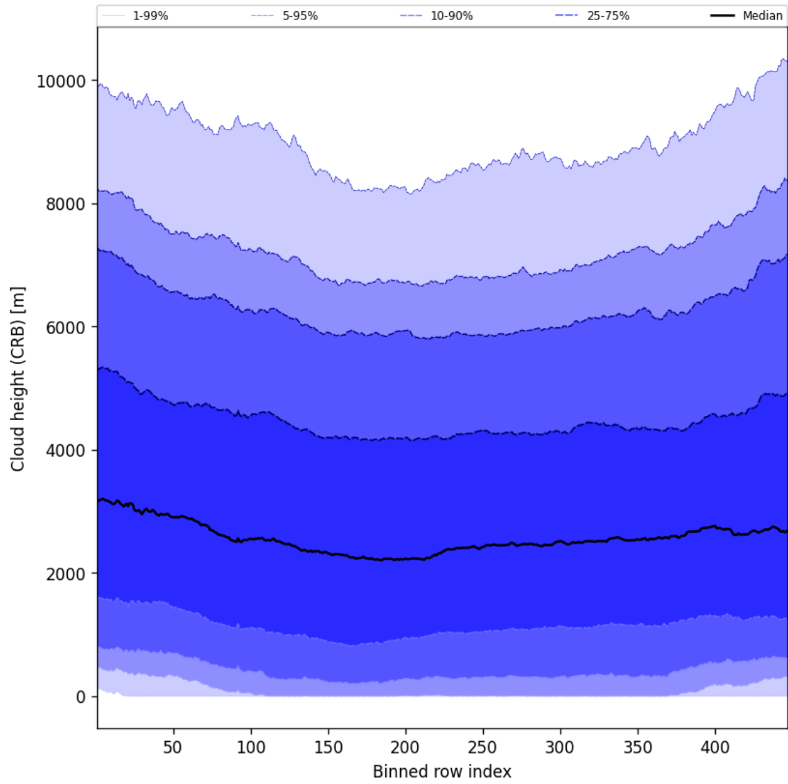
Figure 57: Along track statistics of “Cloud height (CRB)” for 2025-06-29 to 2025-06-30
