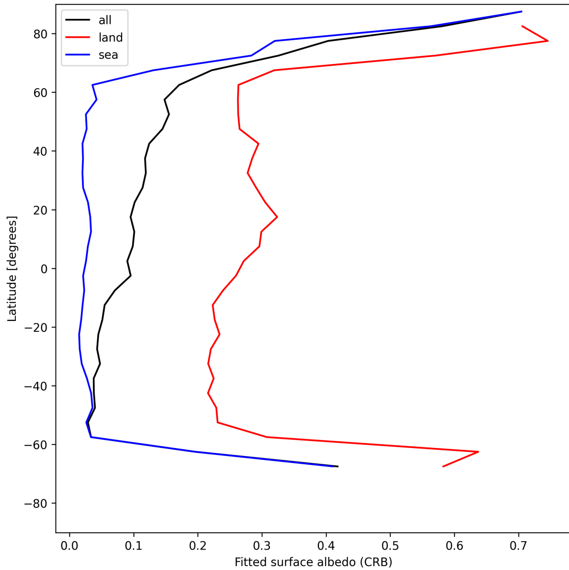
Figure 28: Zonal average of “Fitted surface albedo (CRB)” for 2025-06-29 to 2025-06-30.
