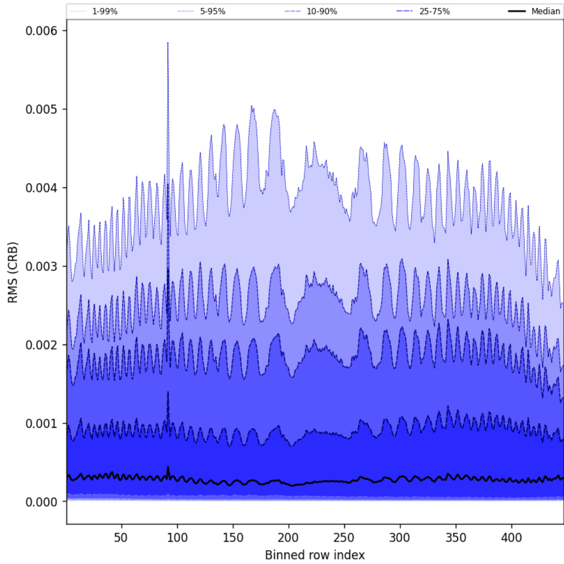
Figure 62: Along track statistics of “RMS (CRB)” for 2025-06-29 to 2025-06-30
