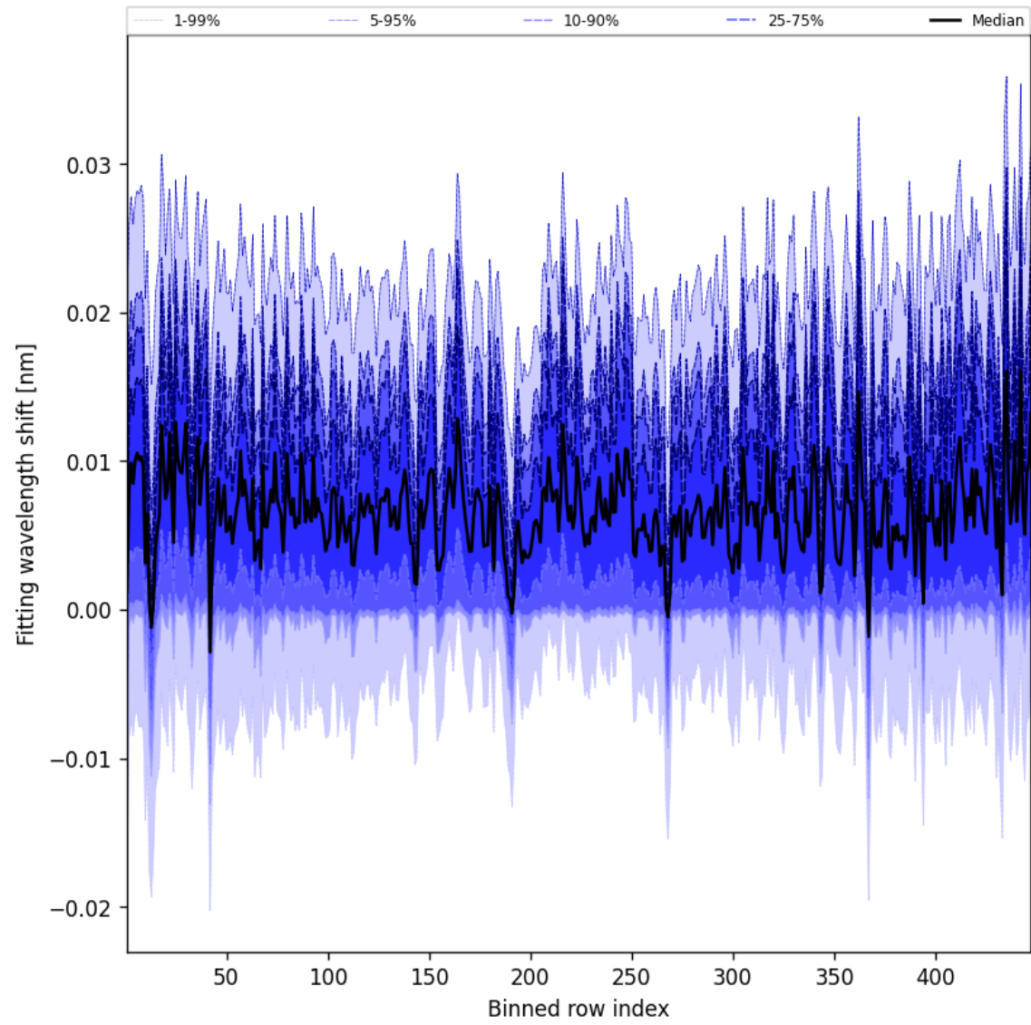
Figure 63: Along track statistics of “Fitting wavelength shift” for 2025-06-29 to 2025-06-30
