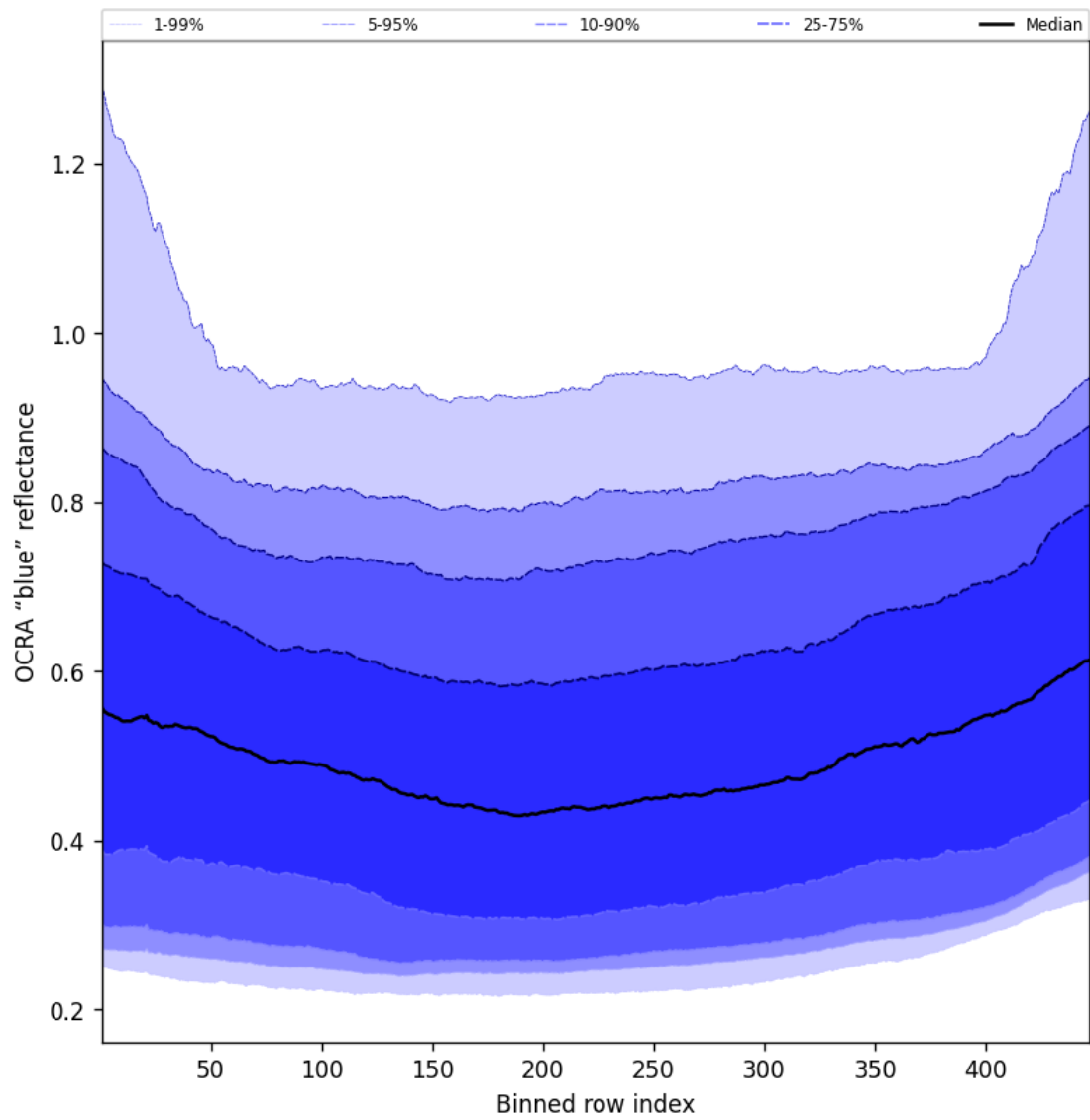
Figure 65: Along track statistics of “OCRA “blue” reflectance” for 2025-06-29 to 2025-06-30
