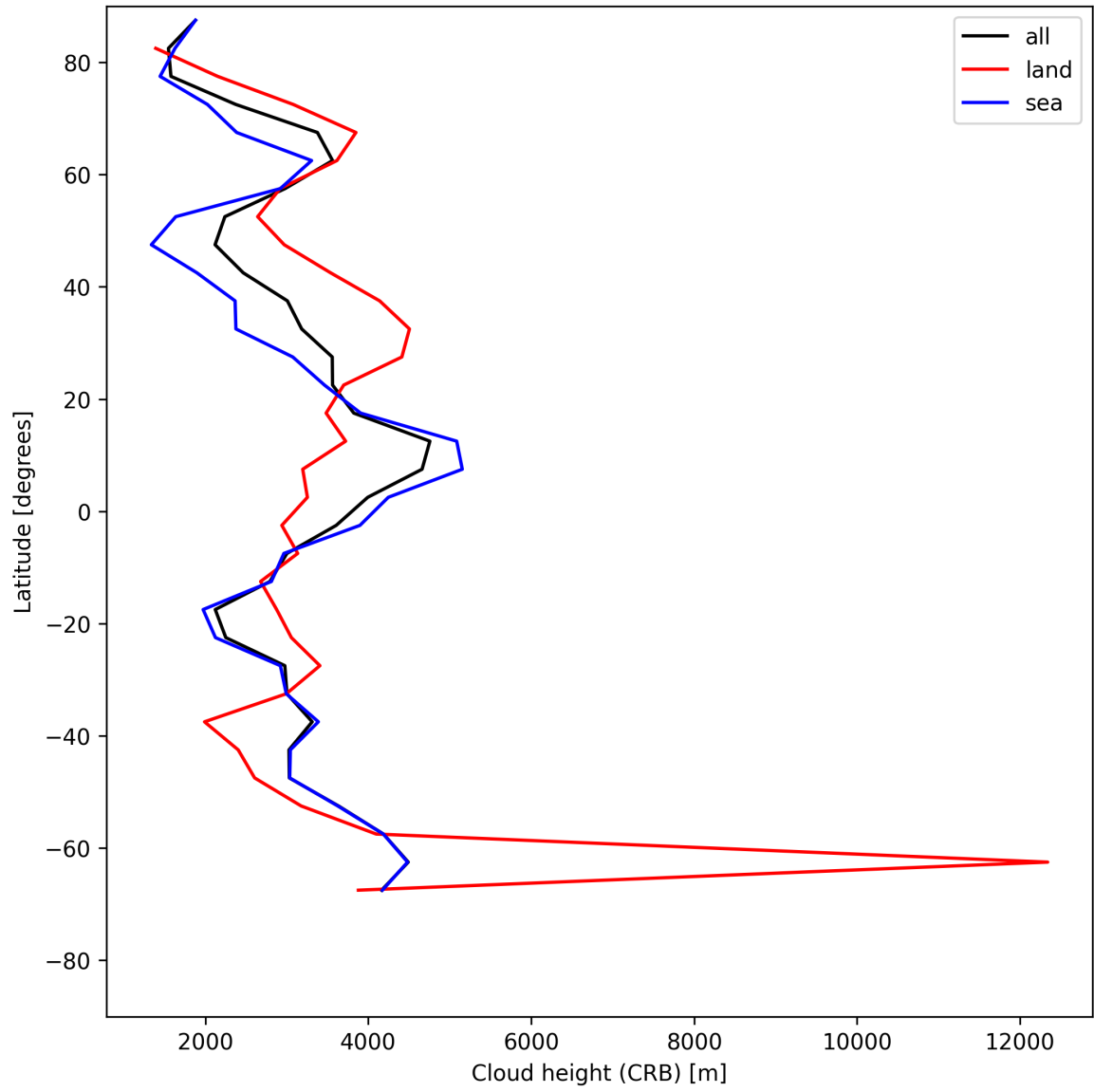
Figure 25: Zonal average of “Cloud height (CRB)” for 2025-06-29 to 2025-06-30.
