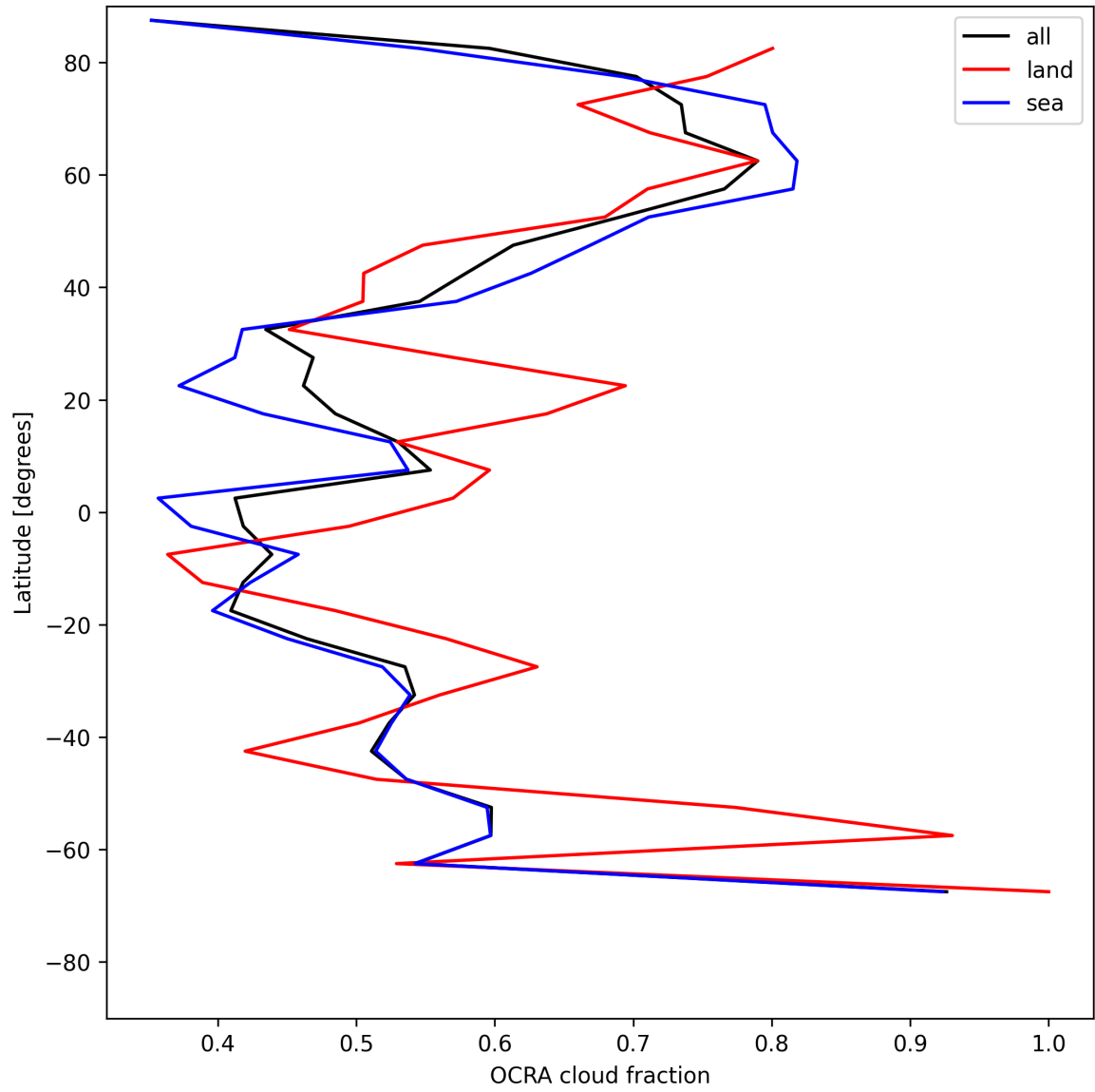
Figure 32: Zonal average of “OCRA cloud fraction” for 2025-06-29 to 2025-06-30.
