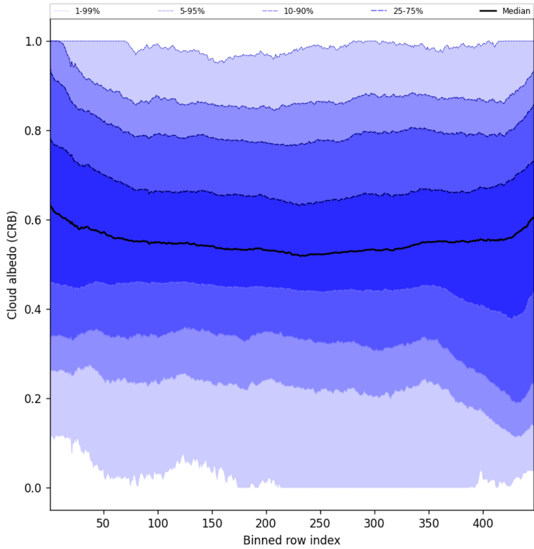
Figure 58: Along track statistics of “Cloud albedo (CRB)” for 2025-06-29 to 2025-06-30
