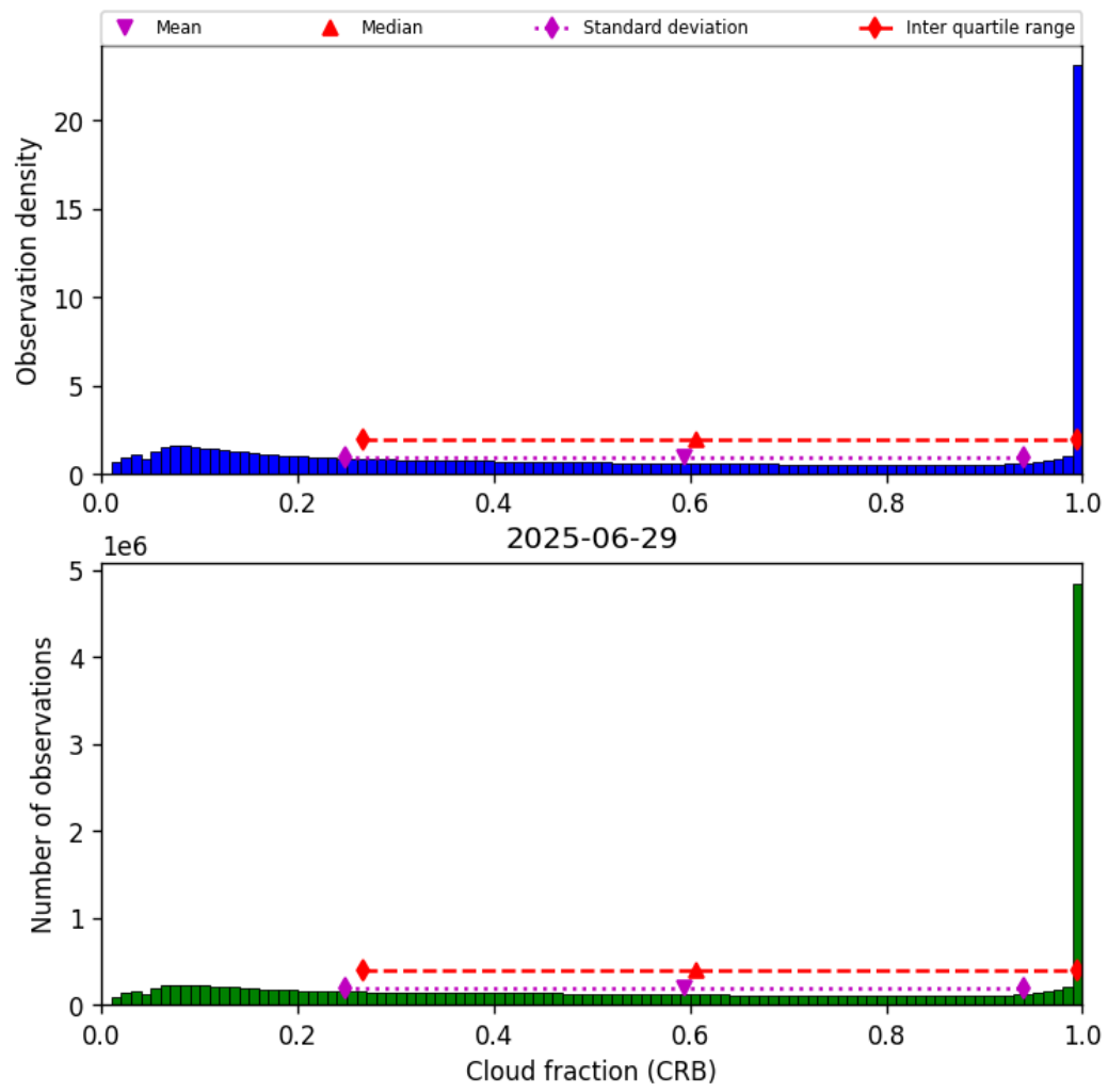
Figure 40: Histogram of “Cloud fraction (CRB)” for 2025-06-29 to 2025-06-30
