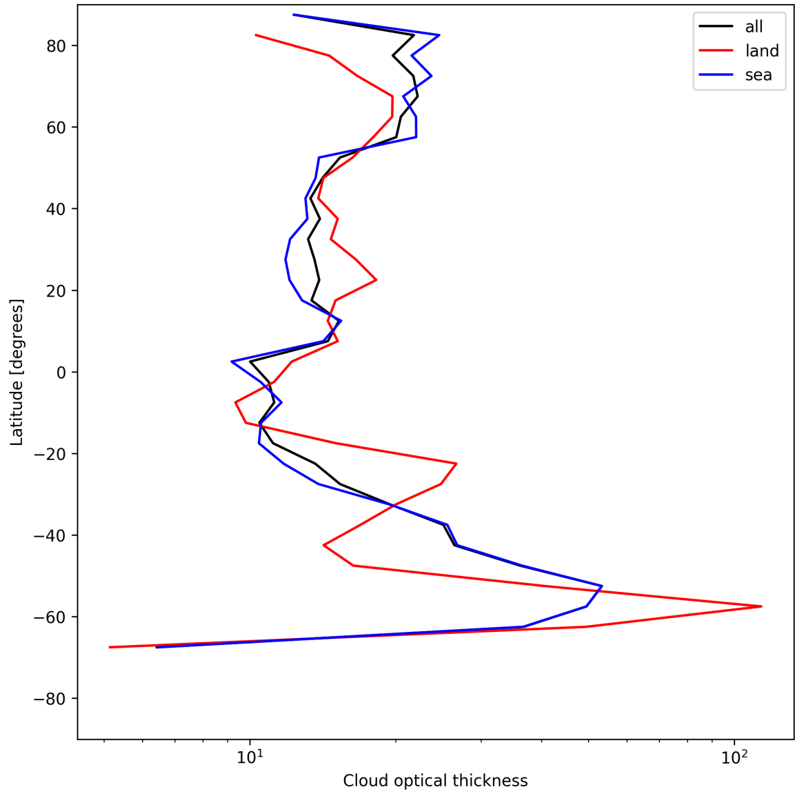
Figure 23: Zonal average of “Cloud optical thickness” for 2025-06-29 to 2025-06-30.
