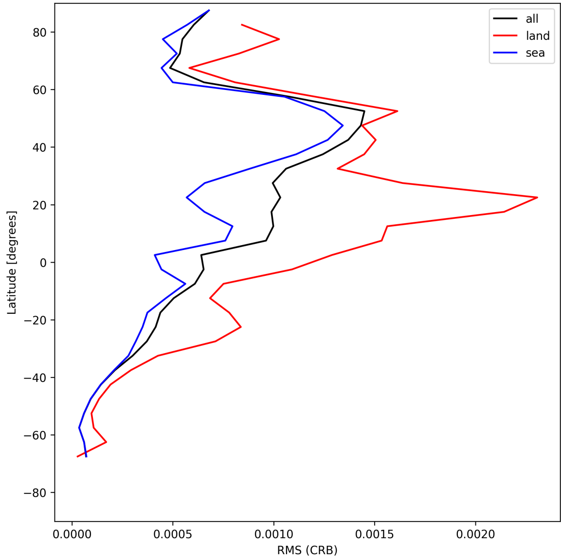
Figure 30: Zonal average of “RMS (CRB)” for 2025-06-29 to 2025-06-30.
