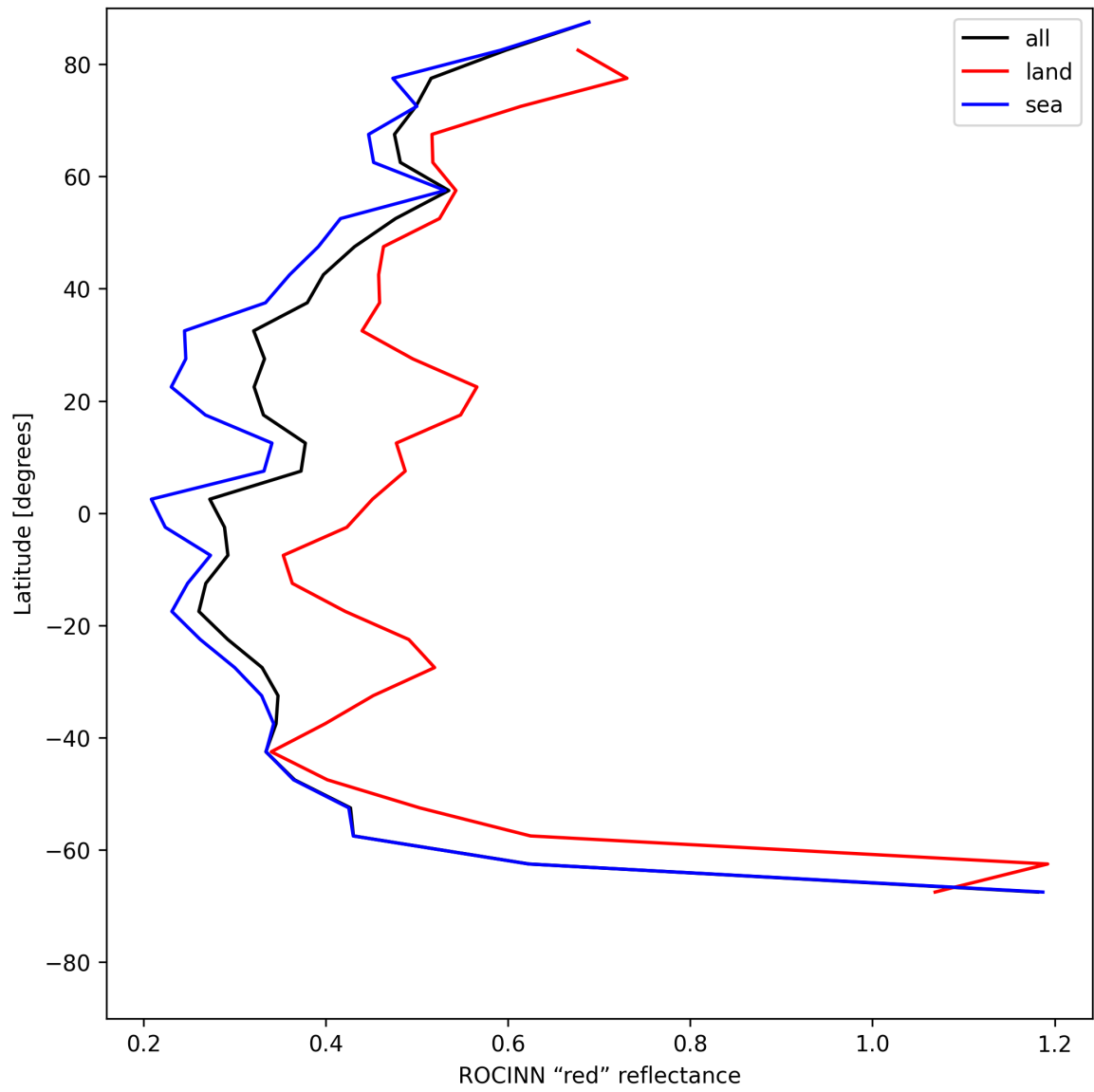
Figure 35: Zonal average of “ROCINN “red” reflectance” for 2025-06-29 to 2025-06-30.
