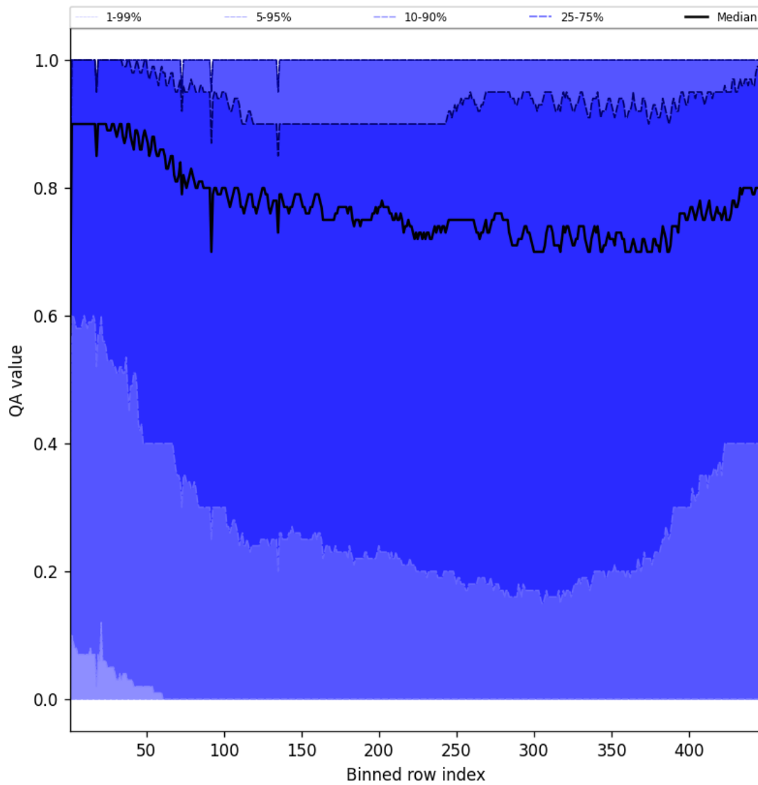
Figure 52: Along track statistics of “QA value” for 2025-06-29 to 2025-06-30
