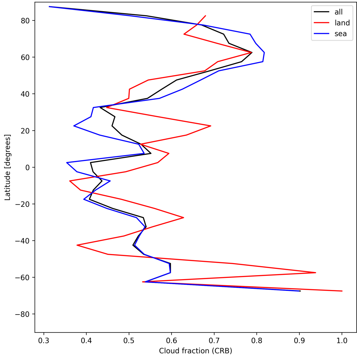
Figure 24: Zonal average of “Cloud fraction (CRB)” for 2025-06-29 to 2025-06-30.
