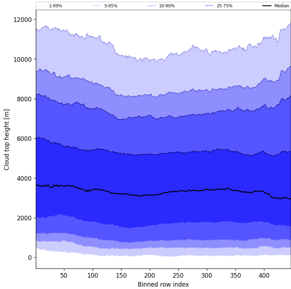
Figure 54: Along track statistics of “Cloud top height” for 2025-06-29 to 2025-06-30
