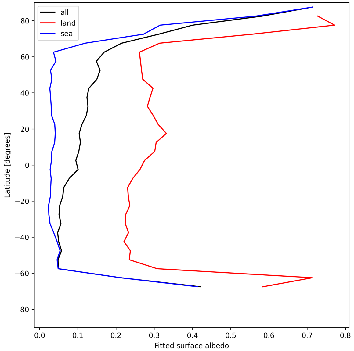
Figure 27: Zonal average of “Fitted surface albedo” for 2025-06-29 to 2025-06-30.
