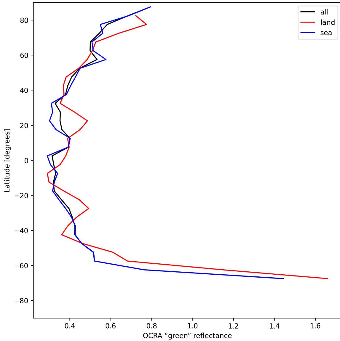
Figure 34: Zonal average of “OCRA “green” reflectance” for 2025-06-29 to 2025-06-30.
