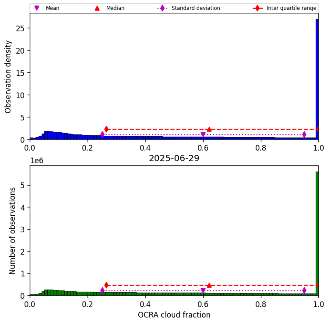
Figure 48: Histogram of “OCRA cloud fraction” for 2025-06-29 to 2025-06-30
