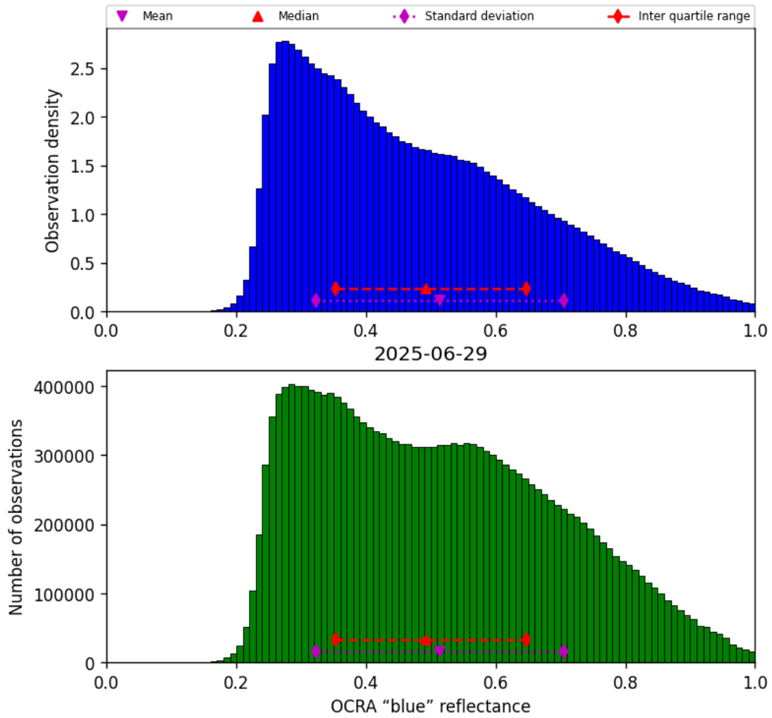
Figure 49: Histogram of “OCRA “blue” reflectance” for 2025-06-29 to 2025-06-30
