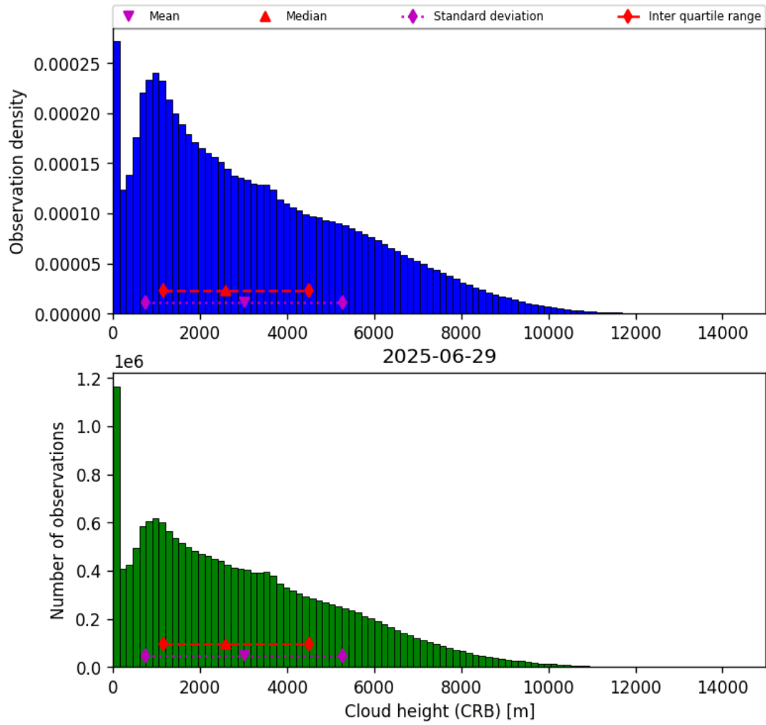
Figure 41: Histogram of “Cloud height (CRB)” for 2025-06-29 to 2025-06-30
