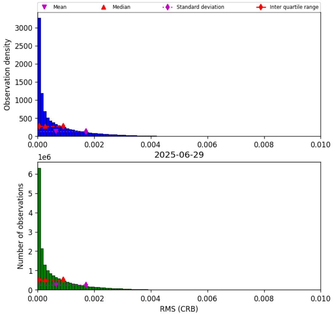
Figure 46: Histogram of “RMS (CRB)” for 2025-06-29 to 2025-06-30
