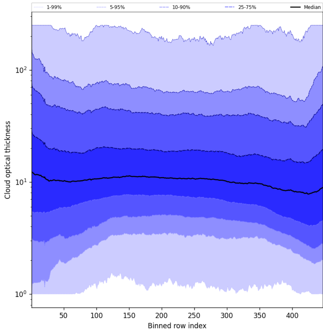
Figure 55: Along track statistics of “Cloud optical thickness” for 2025-06-29 to 2025-06-30
