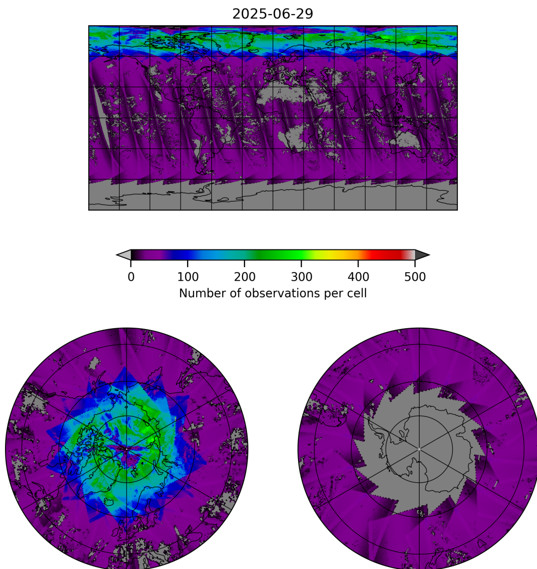
Figure 19: Map of the number of observations for 2025-06-29 to 2025-06-30
