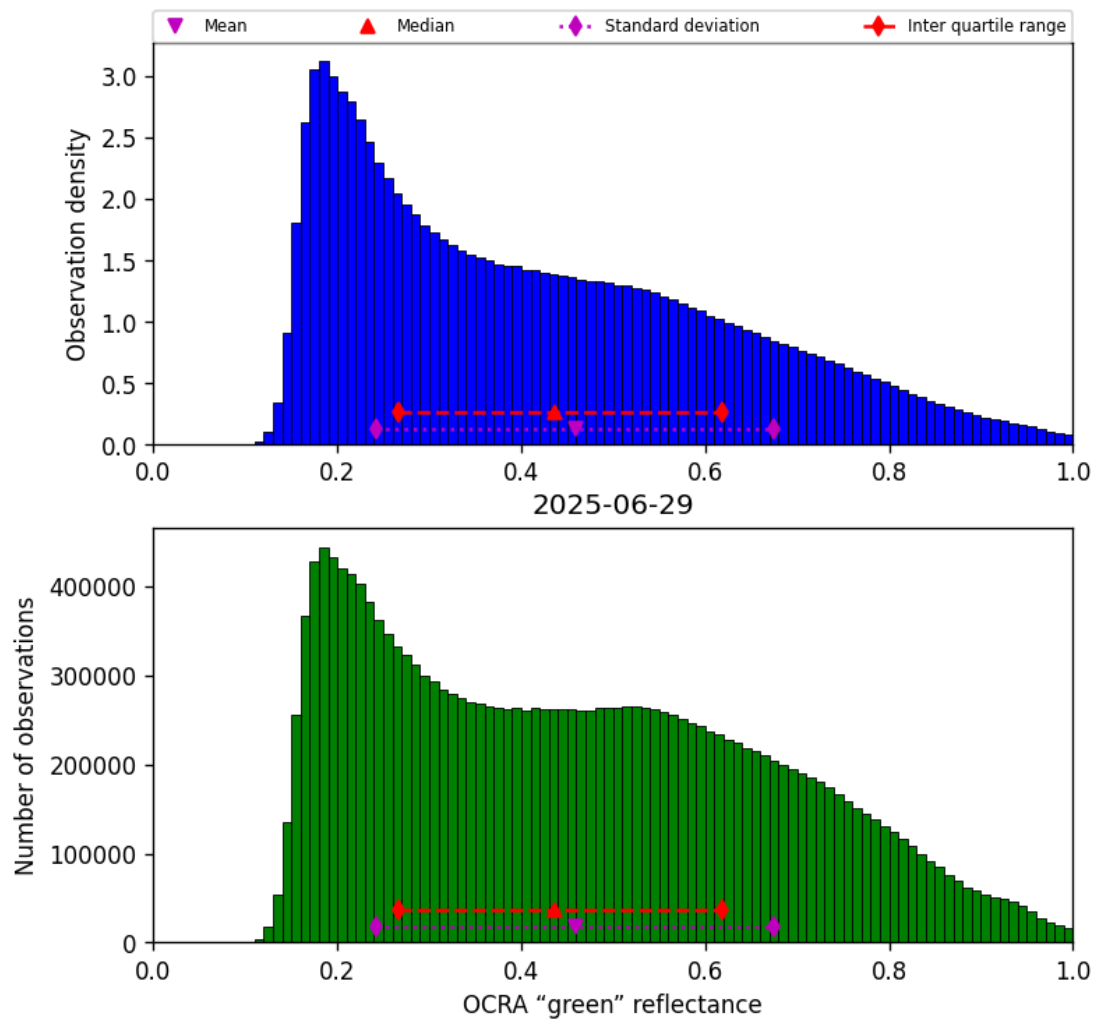
Figure 50: Histogram of “OCRA “green” reflectance” for 2025-06-29 to 2025-06-30
