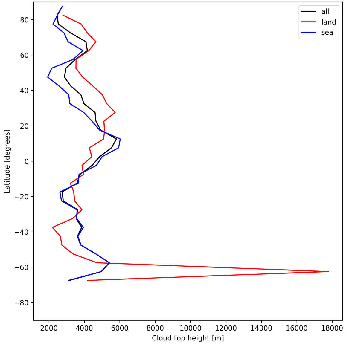
Figure 22: Zonal average of “Cloud top height” for 2025-06-29 to 2025-06-30.
