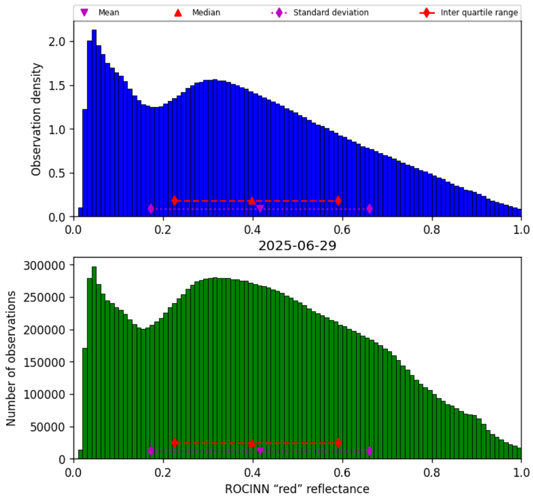
Figure 51: Histogram of “ROCINN “red” reflectance” for 2025-06-29 to 2025-06-30
