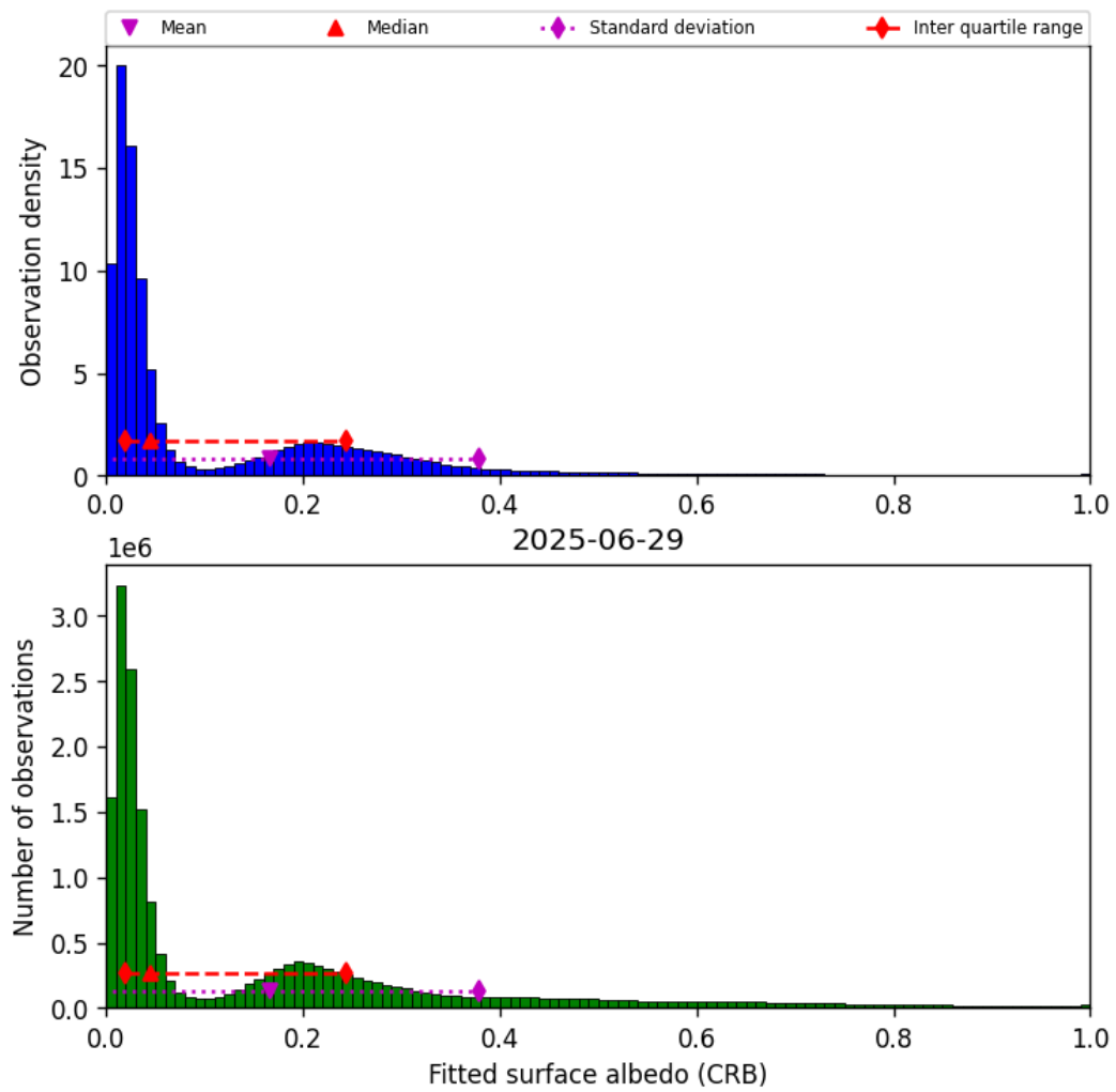
Figure 44: Histogram of “Fitted surface albedo (CRB)” for 2025-06-29 to 2025-06-30
