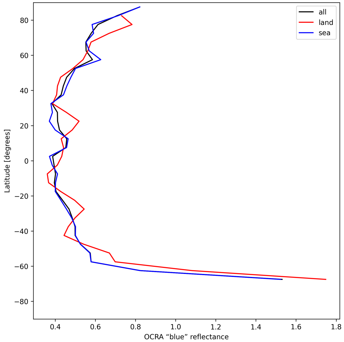
Figure 33: Zonal average of “OCRA “blue” reflectance” for 2025-06-29 to 2025-06-30.
