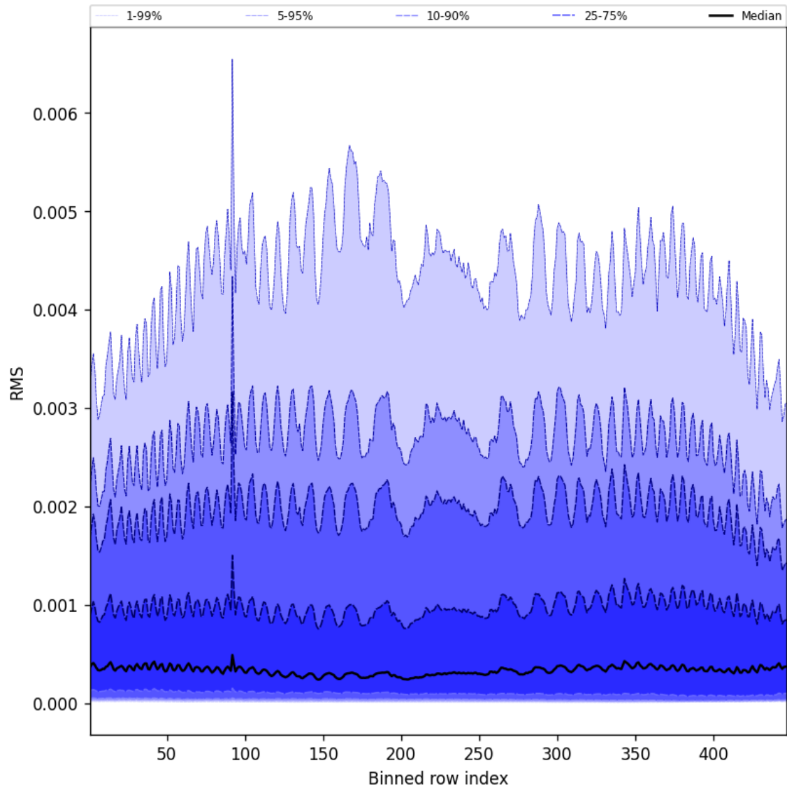
Figure 61: Along track statistics of “RMS” for 2025-06-29 to 2025-06-30
