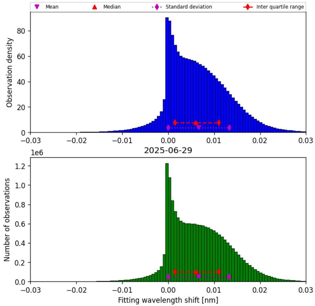
Figure 47: Histogram of “Fitting wavelength shift” for 2025-06-29 to 2025-06-30
