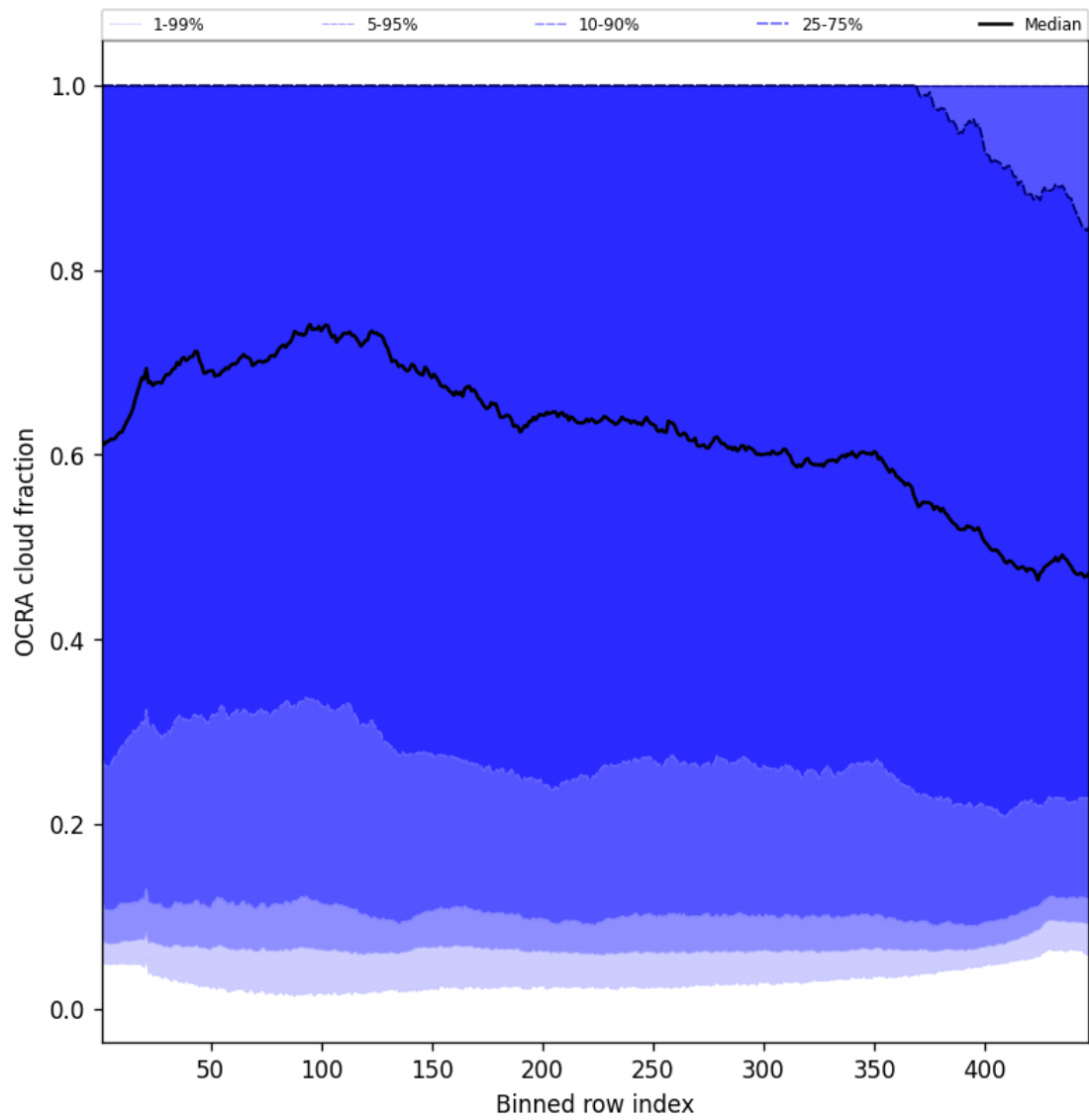
Figure 64: Along track statistics of “OCRA cloud fraction” for 2025-06-29 to 2025-06-30
