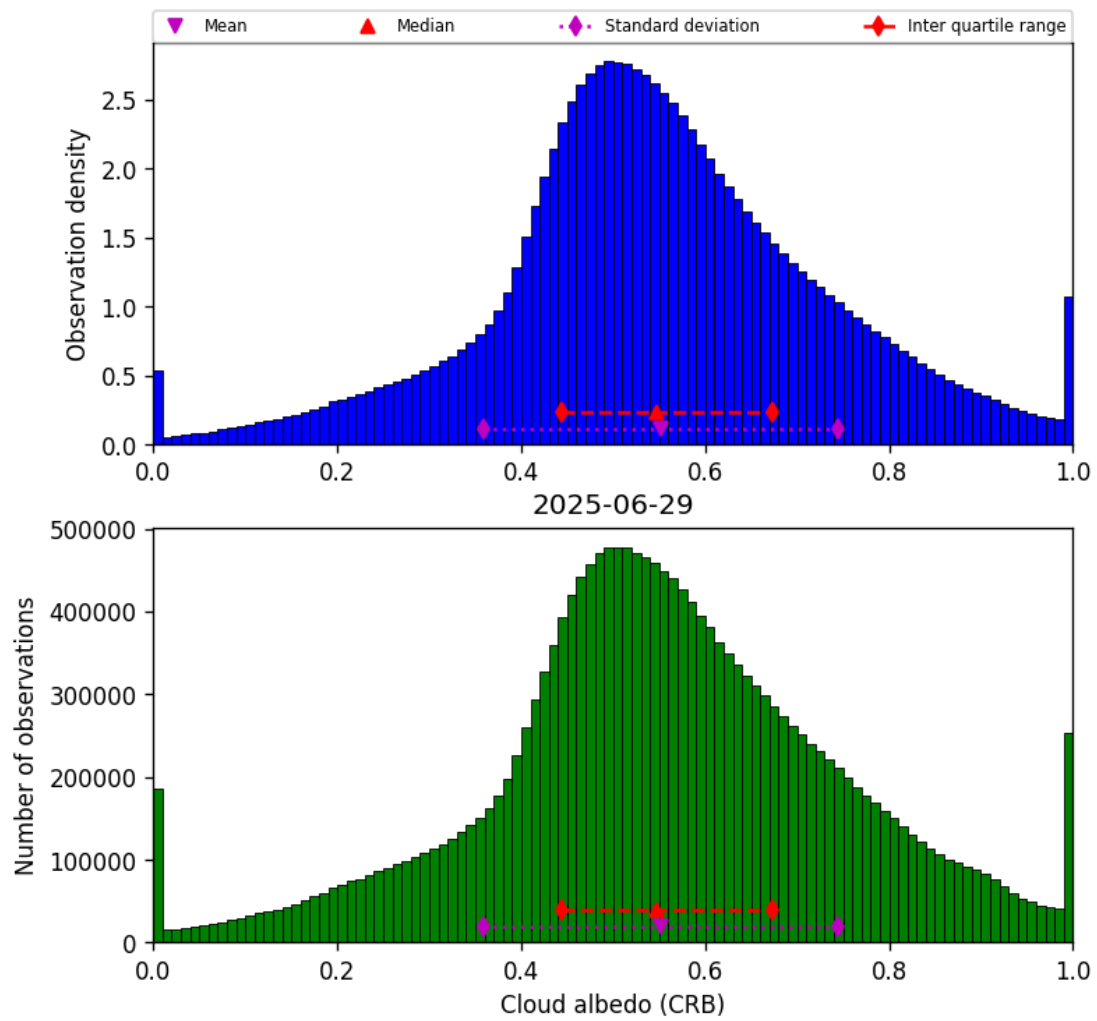
Figure 42: Histogram of “Cloud albedo (CRB)” for 2025-06-29 to 2025-06-30
