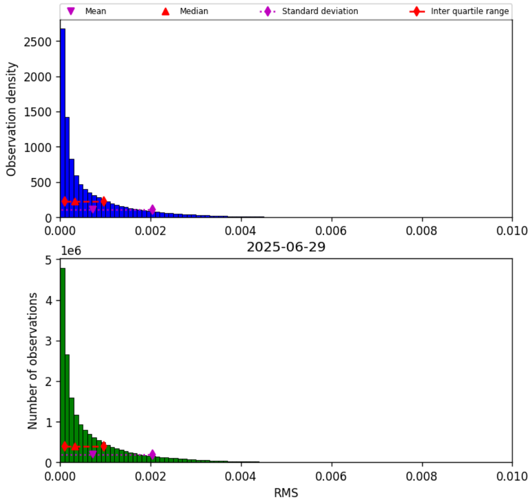
Figure 45: Histogram of “RMS” for 2025-06-29 to 2025-06-30
