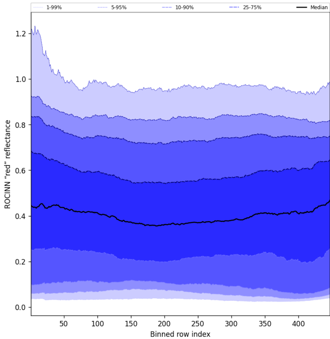
Figure 67: Along track statistics of "ROCINN "red" reflectance" for 2025-06-29 to 2025-06-30
