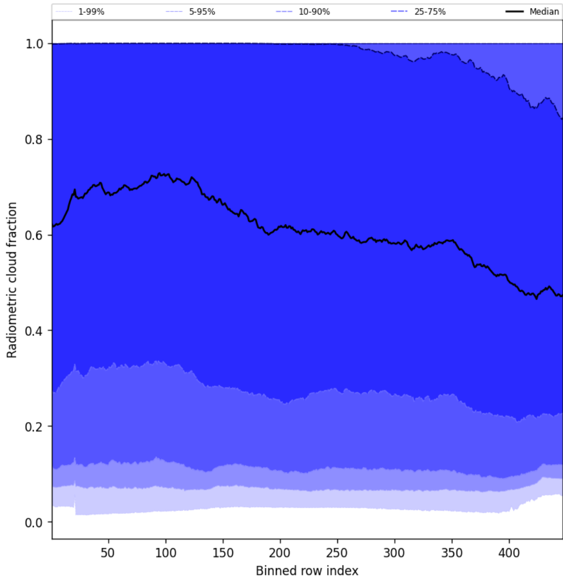
Figure 53: Along track statistics of “Radiometric cloud fraction” for 2025-06-29 to 2025-06-30
