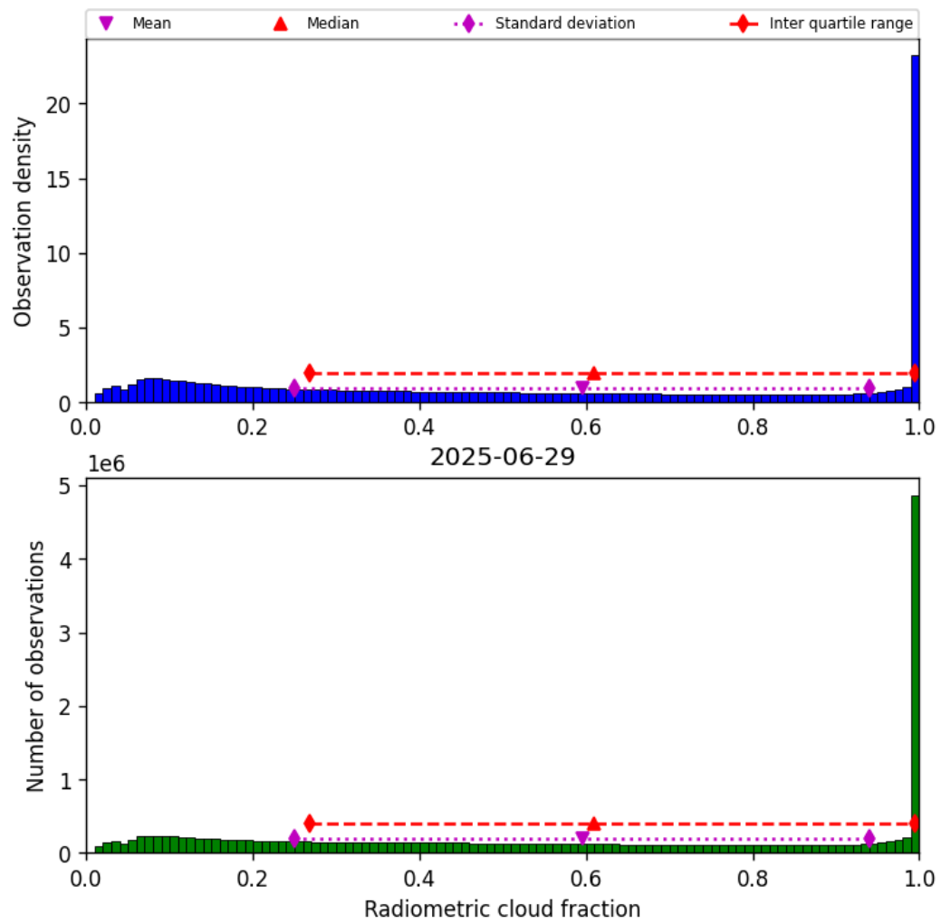
Figure 37: Histogram of “Radiometric cloud fraction” for 2025-06-29 to 2025-06-30
