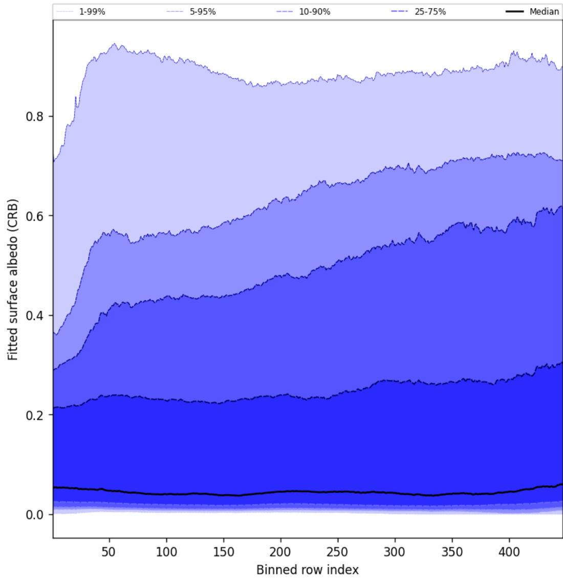
Figure 60: Along track statistics of “Fitted surface albedo (CRB)” for 2025-06-29 to 2025-06-30
