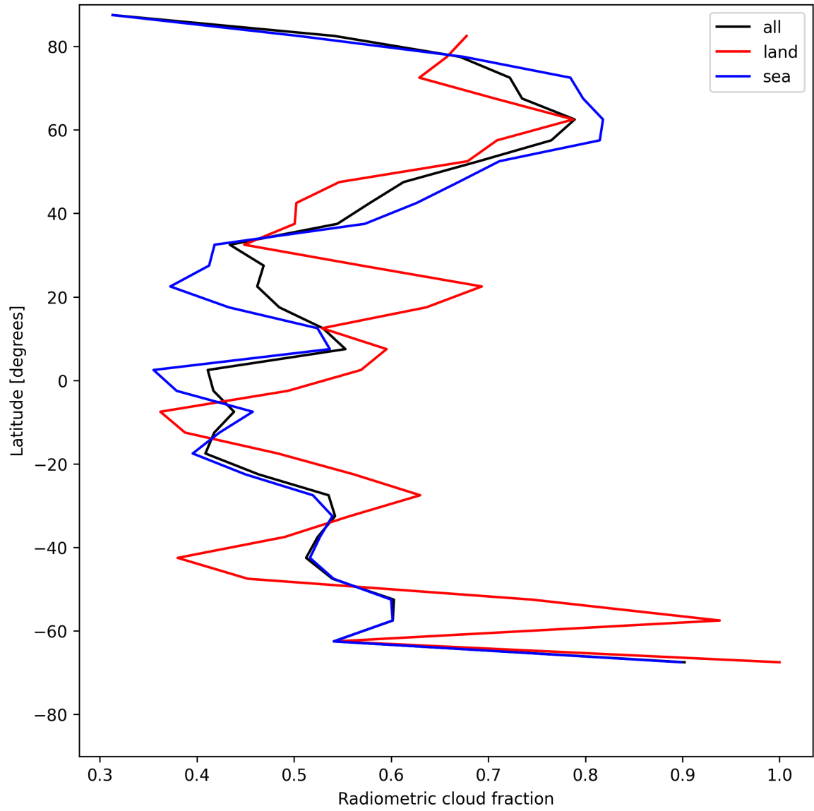
Figure 21: Zonal average of “Radiometric cloud fraction” for 2025-06-29 to 2025-06-30.
