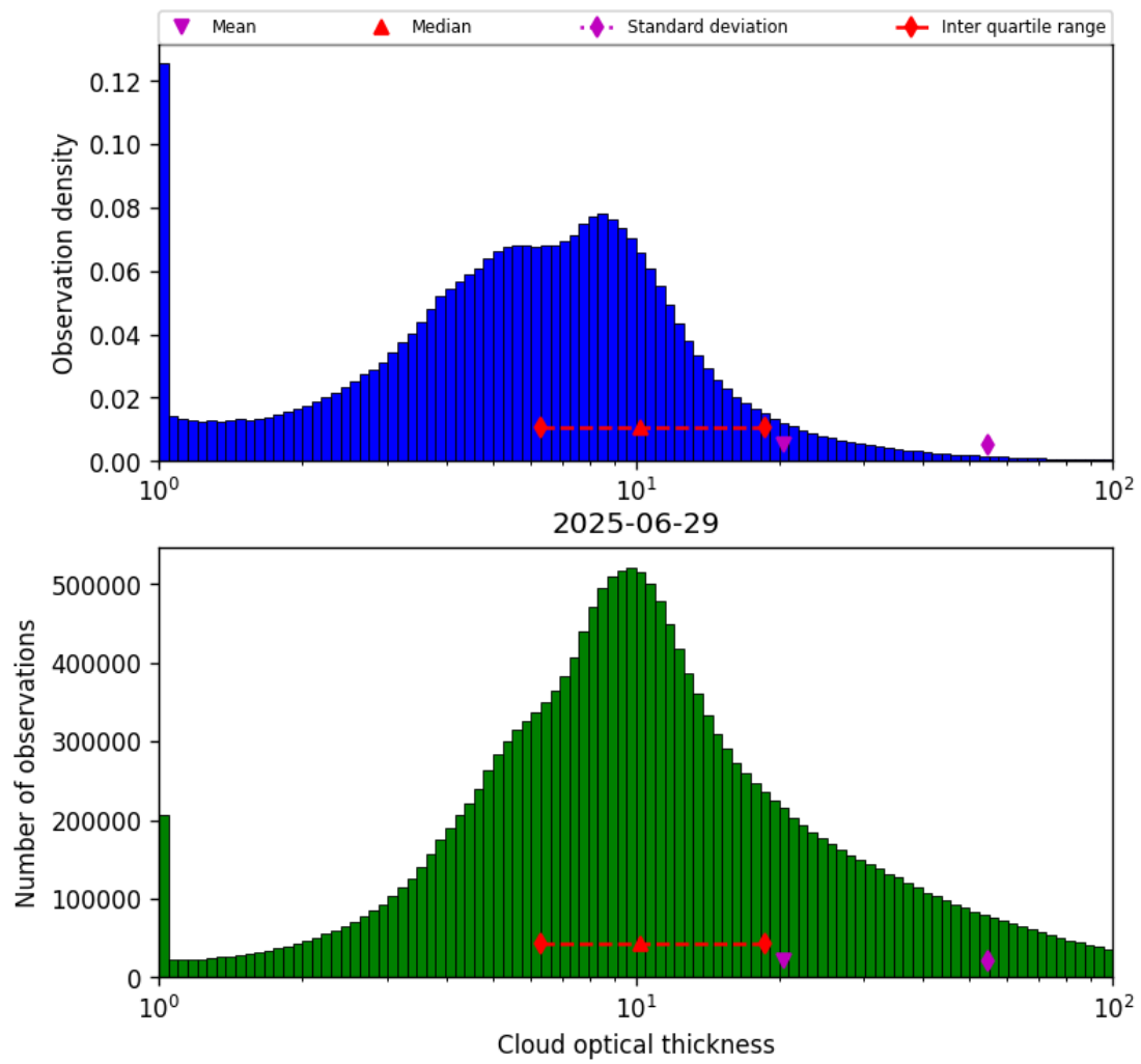
Figure 39: Histogram of “Cloud optical thickness” for 2025-06-29 to 2025-06-30
