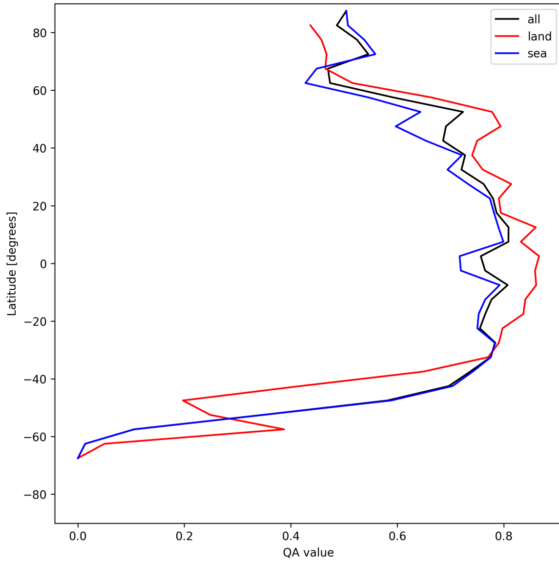
Figure 20: Zonal average of “QA value” for 2025-06-29 to 2025-06-30.
