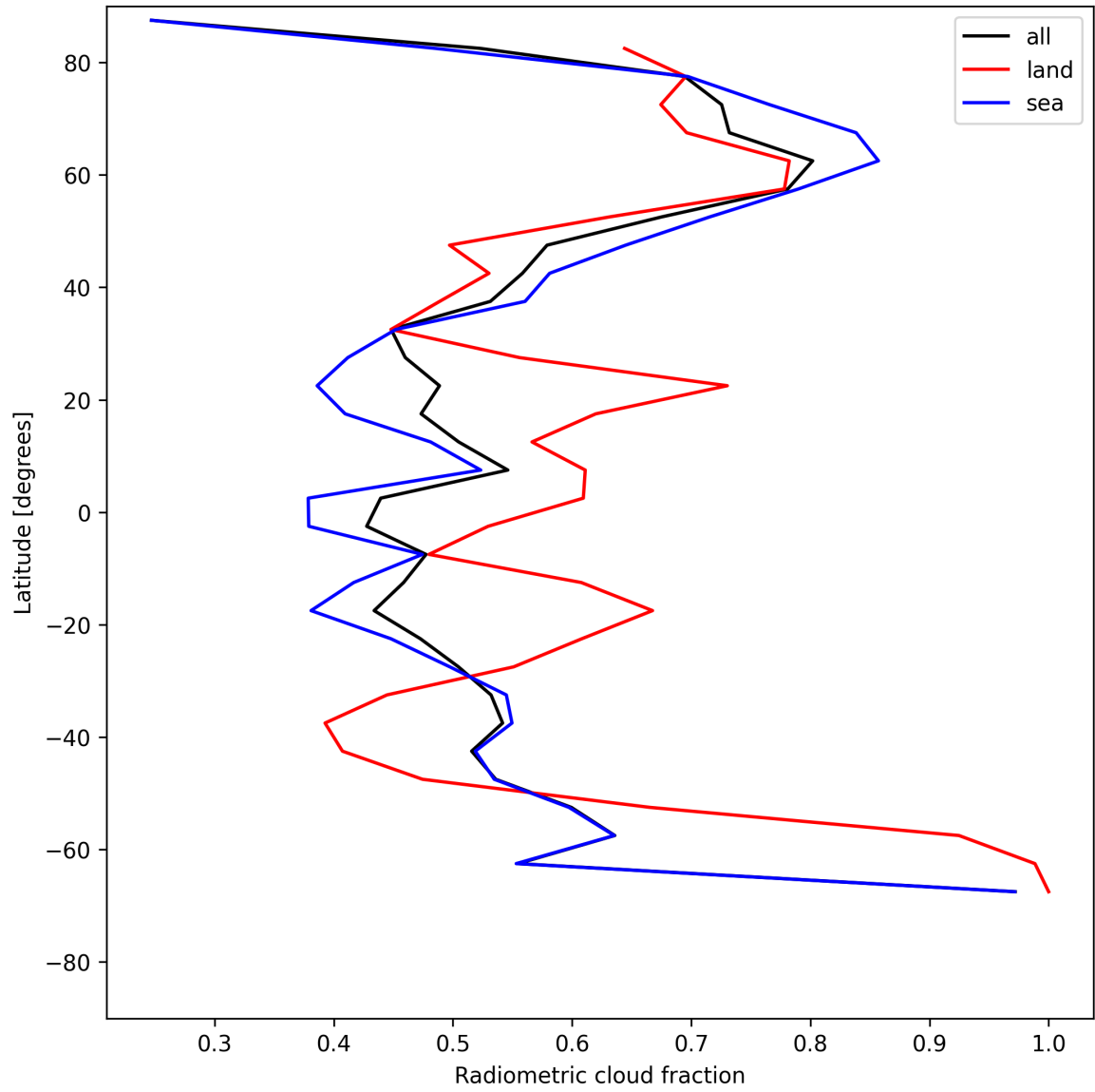
Figure 21: Zonal average of “Radiometric cloud fraction” for 2025-06-30 to 2025-06-30.
