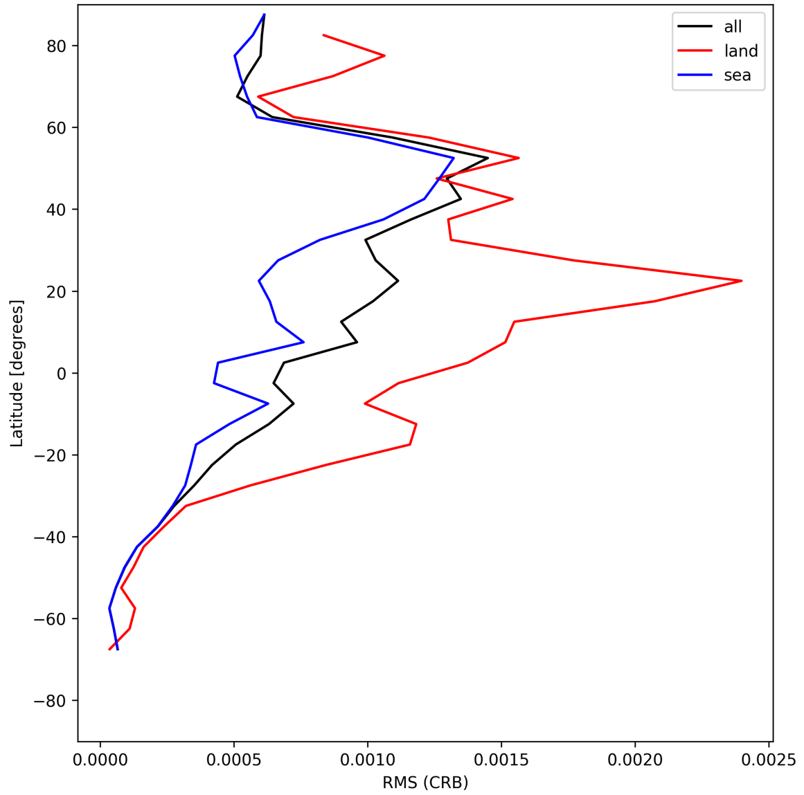
Figure 30: Zonal average of “RMS (CRB)” for 2025-06-30 to 2025-06-30.
