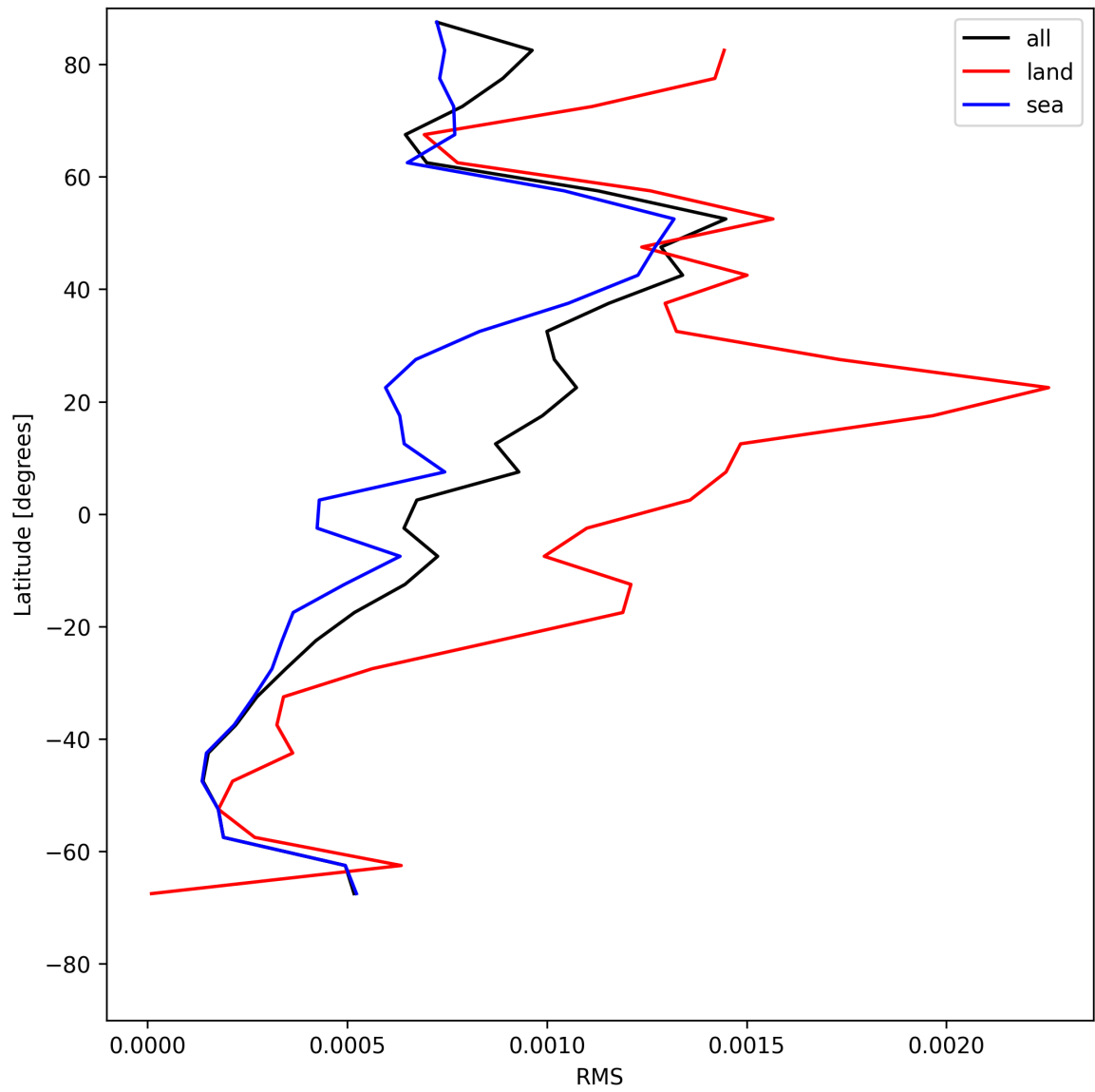
Figure 29: Zonal average of “RMS” for 2025-06-30 to 2025-06-30.
