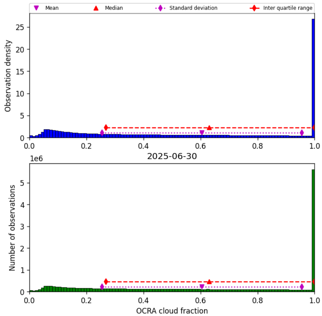
Figure 48: Histogram of “OCRA cloud fraction” for 2025-06-30 to 2025-06-30
