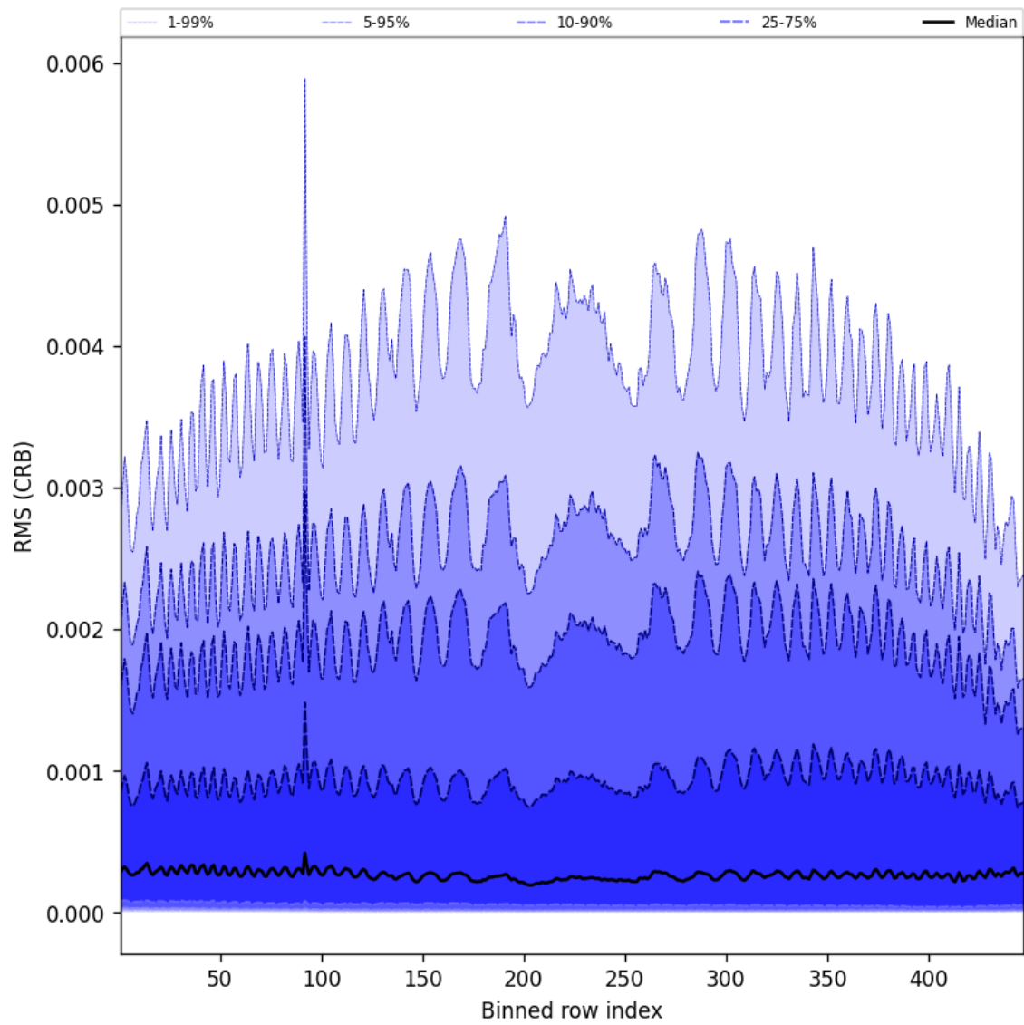
Figure 62: Along track statistics of “RMS (CRB)” for 2025-06-30 to 2025-06-30
