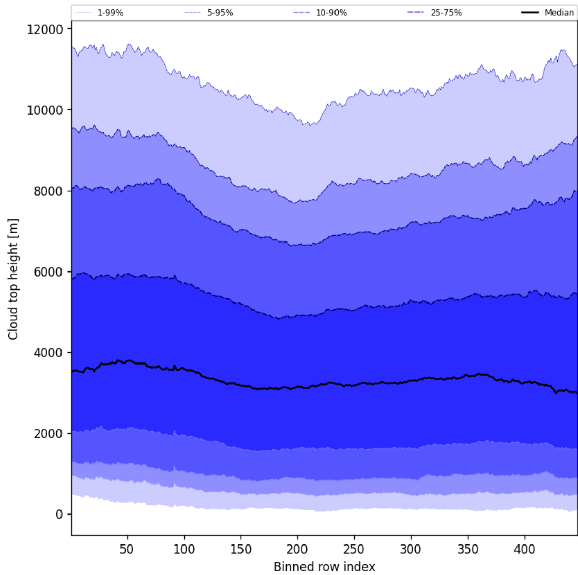
Figure 54: Along track statistics of “Cloud top height” for 2025-06-30 to 2025-06-30
