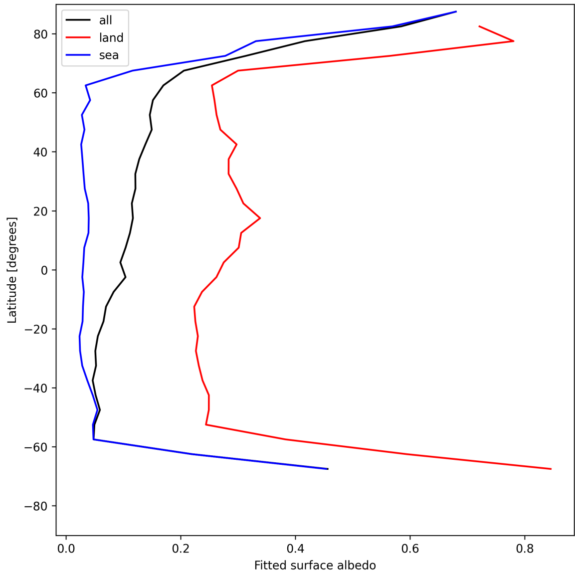
Figure 27: Zonal average of “Fitted surface albedo” for 2025-06-30 to 2025-06-30.
