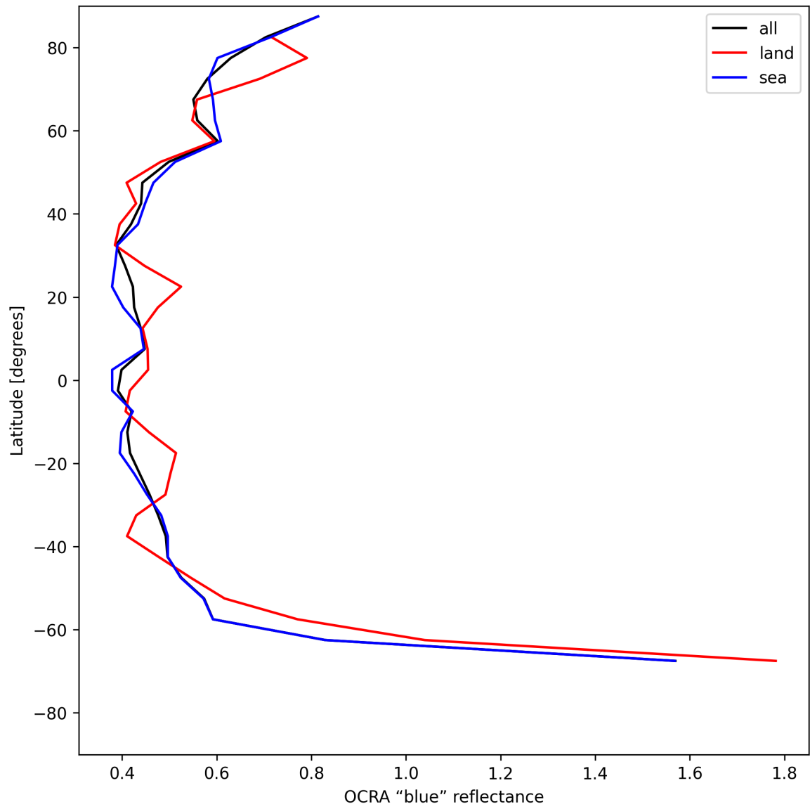
Figure 33: Zonal average of “OCRA “blue” reflectance” for 2025-06-30 to 2025-06-30.
