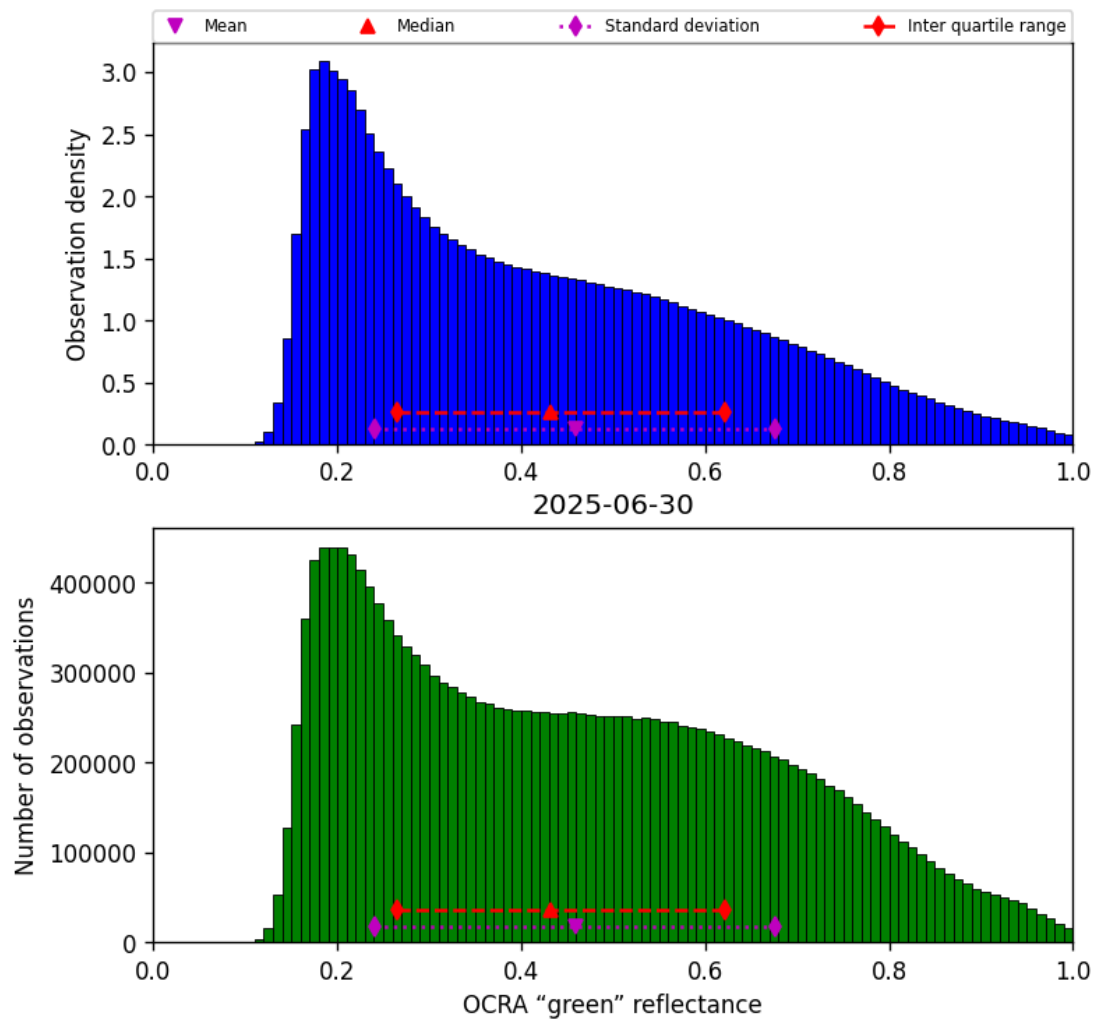
Figure 50: Histogram of “OCRA “green” reflectance” for 2025-06-30 to 2025-06-30
