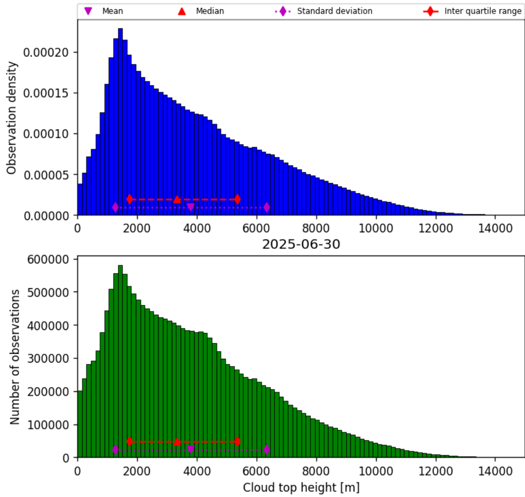
Figure 38: Histogram of “Cloud top height” for 2025-06-30 to 2025-06-30
