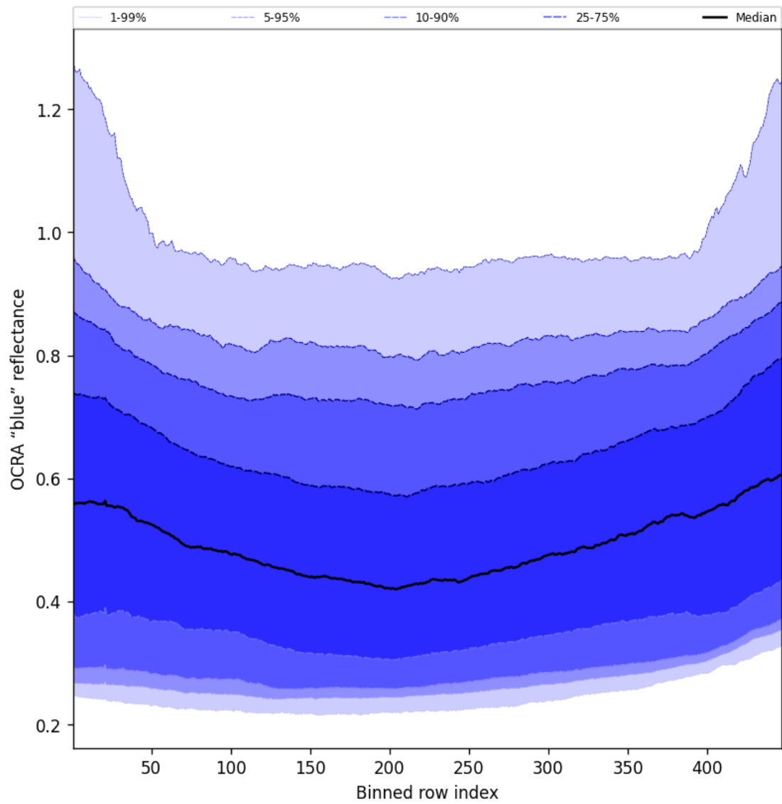
Figure 65: Along track statistics of “OCRA “blue” reflectance” for 2025-06-30 to 2025-06-30
