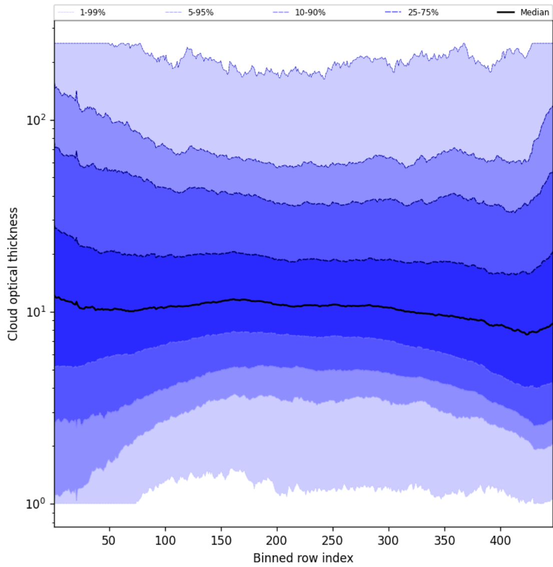
Figure 55: Along track statistics of “Cloud optical thickness” for 2025-06-30 to 2025-06-30
