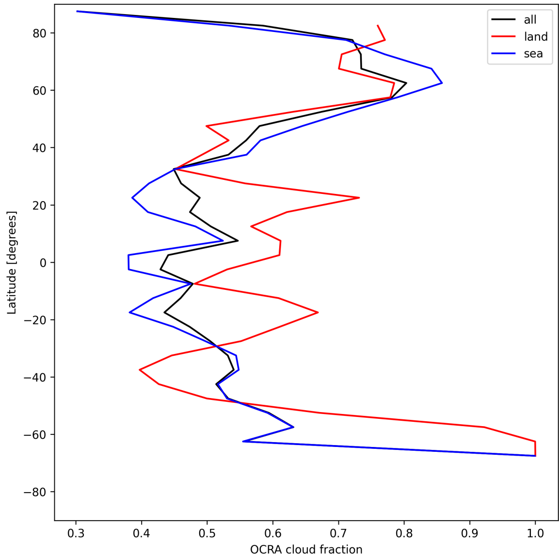
Figure 32: Zonal average of “OCRA cloud fraction” for 2025-06-30 to 2025-06-30.
