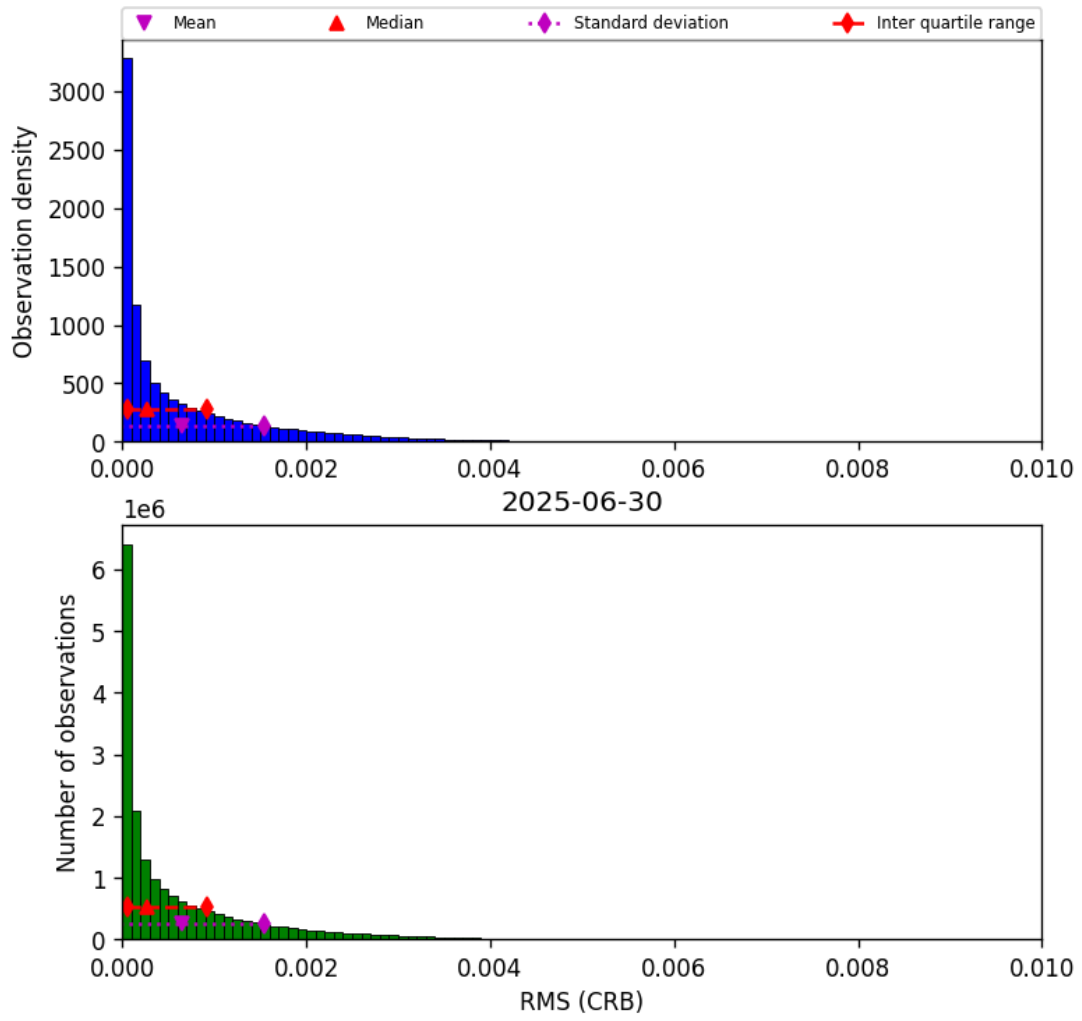
Figure 46: Histogram of “RMS (CRB)” for 2025-06-30 to 2025-06-30
