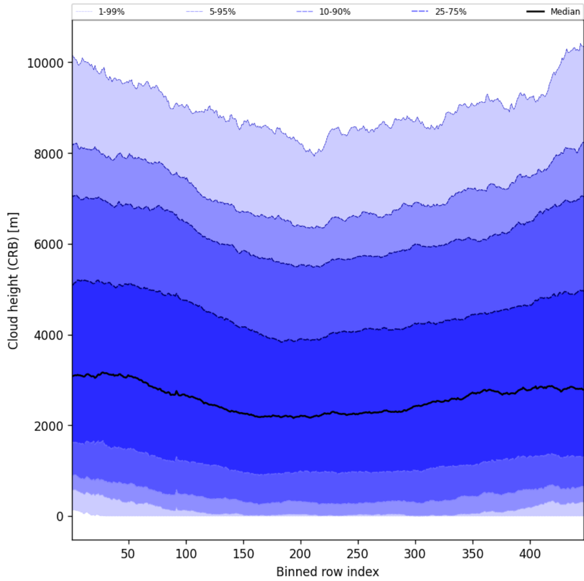
Figure 57: Along track statistics of “Cloud height (CRB)” for 2025-06-30 to 2025-06-30
