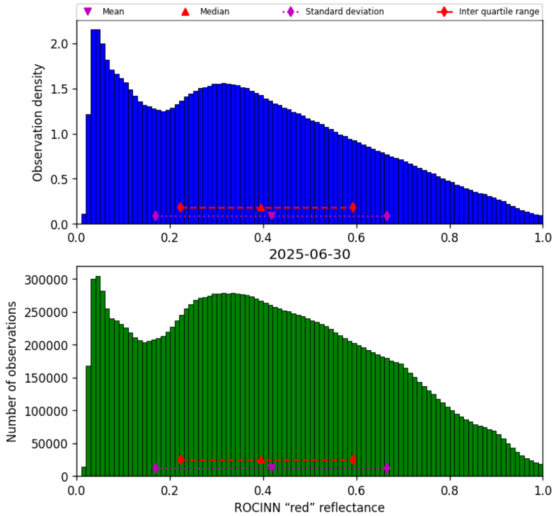
Figure 51: Histogram of "ROCINN "red" reflectance" for 2025-06-30 to 2025-06-30
