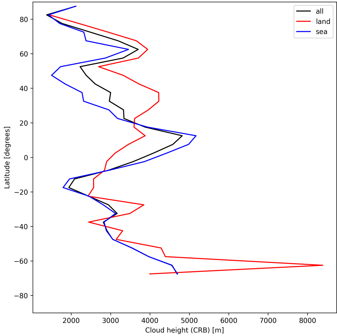
Figure 25: Zonal average of “Cloud height (CRB)” for 2025-06-30 to 2025-06-30.
