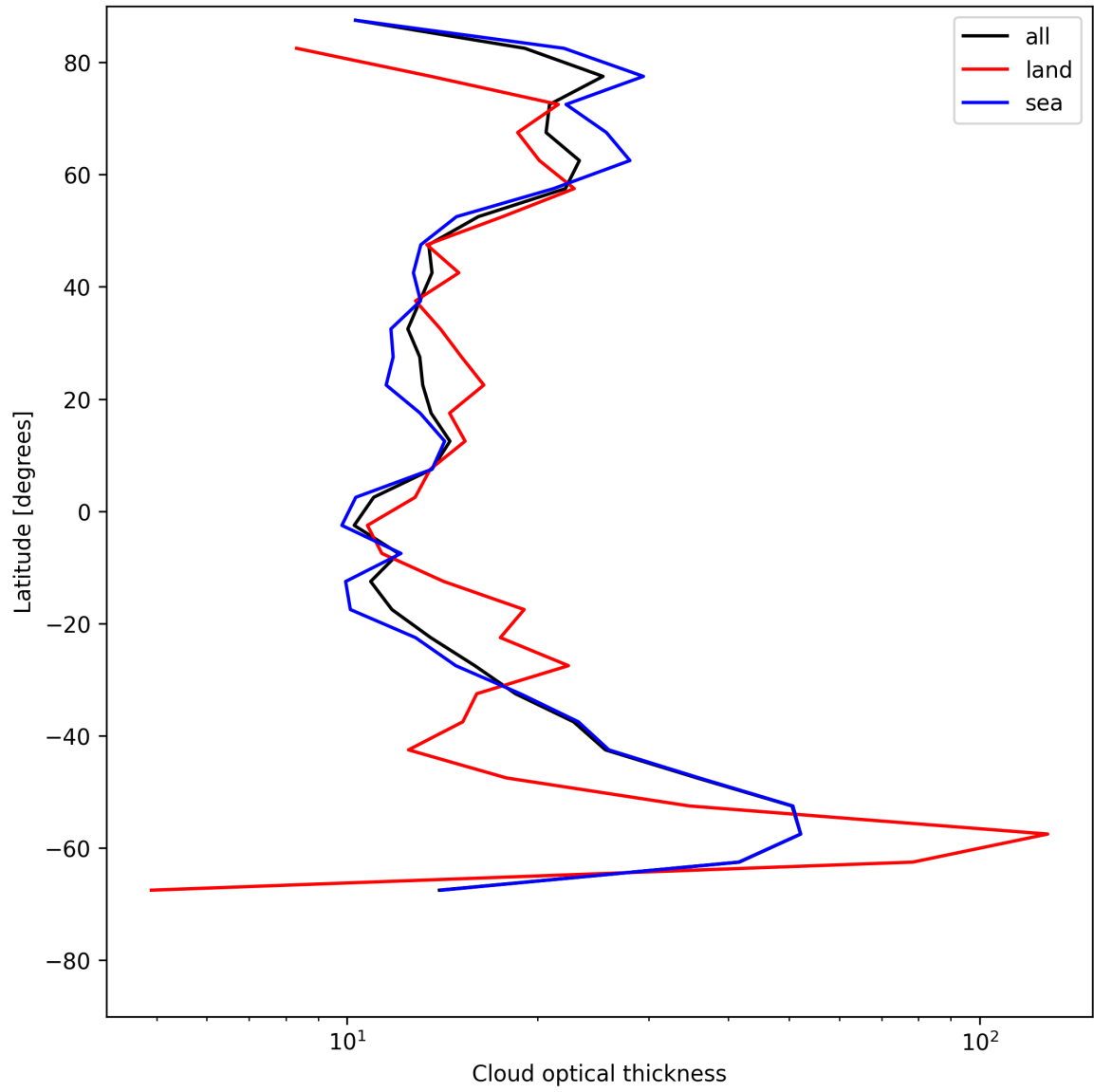
Figure 23: Zonal average of “Cloud optical thickness” for 2025-06-30 to 2025-06-30.
