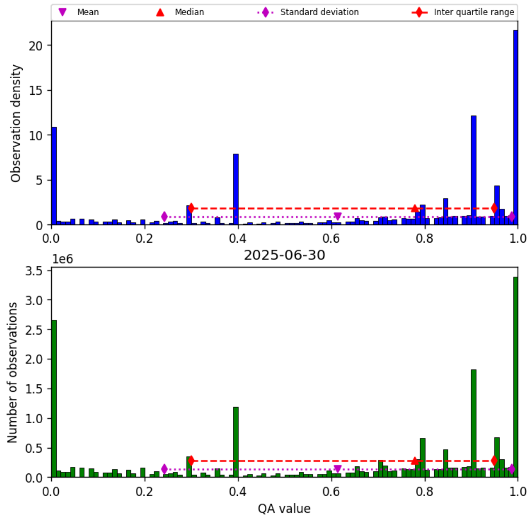
Figure 36: Histogram of “QA value” for 2025-06-30 to 2025-06-30
