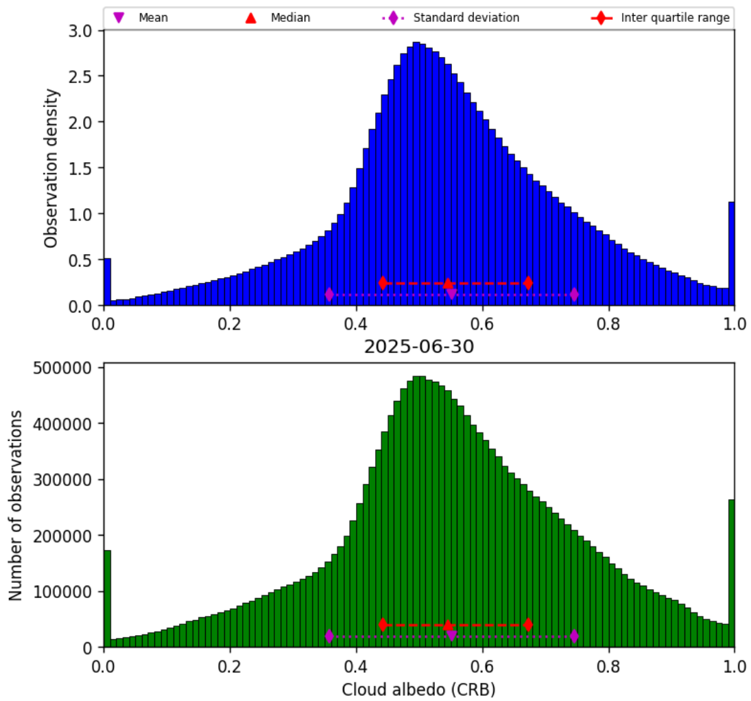
Figure 42: Histogram of “Cloud albedo (CRB)” for 2025-06-30 to 2025-06-30
