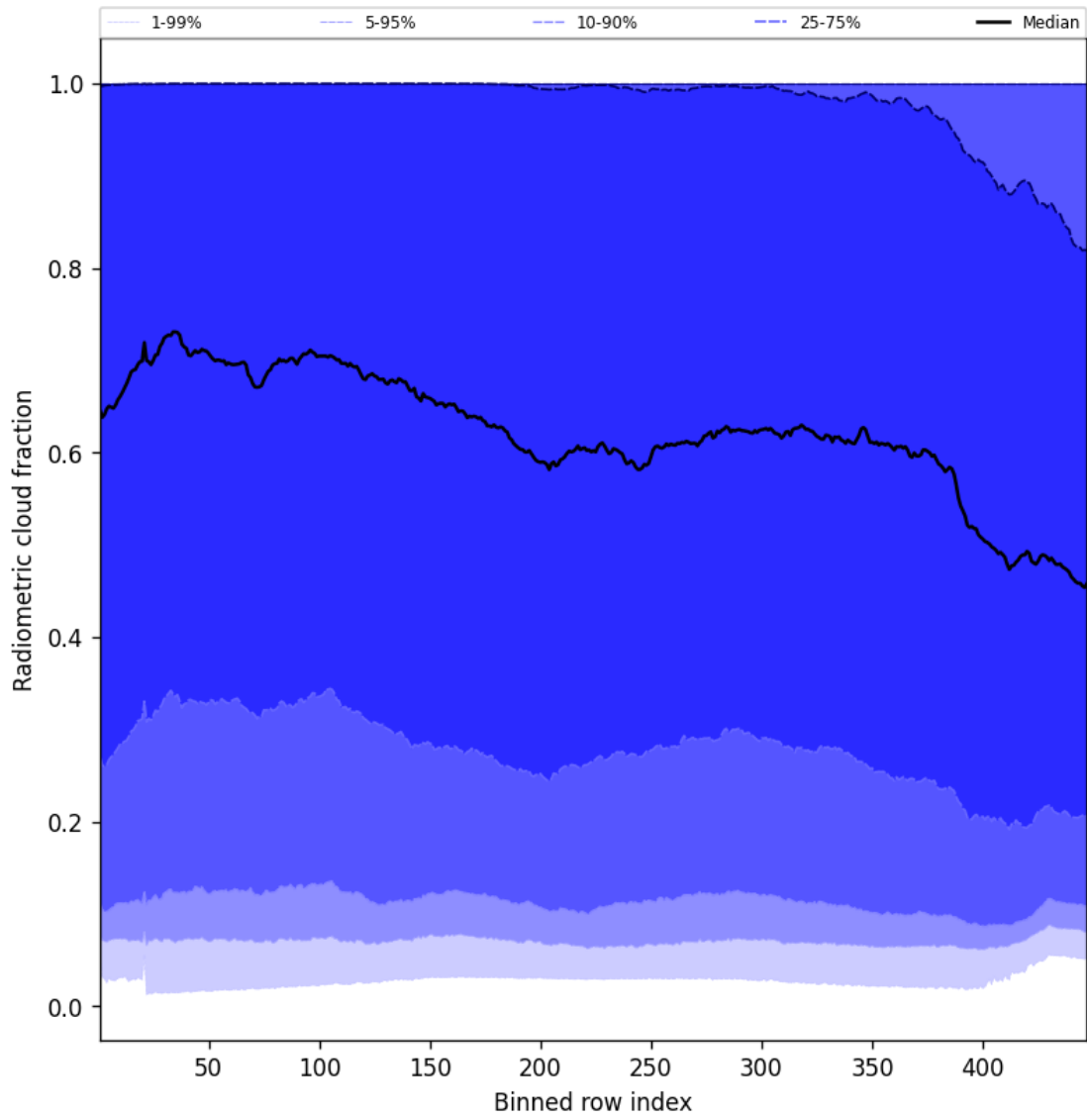
Figure 53: Along track statistics of “Radiometric cloud fraction” for 2025-06-30 to 2025-06-30
