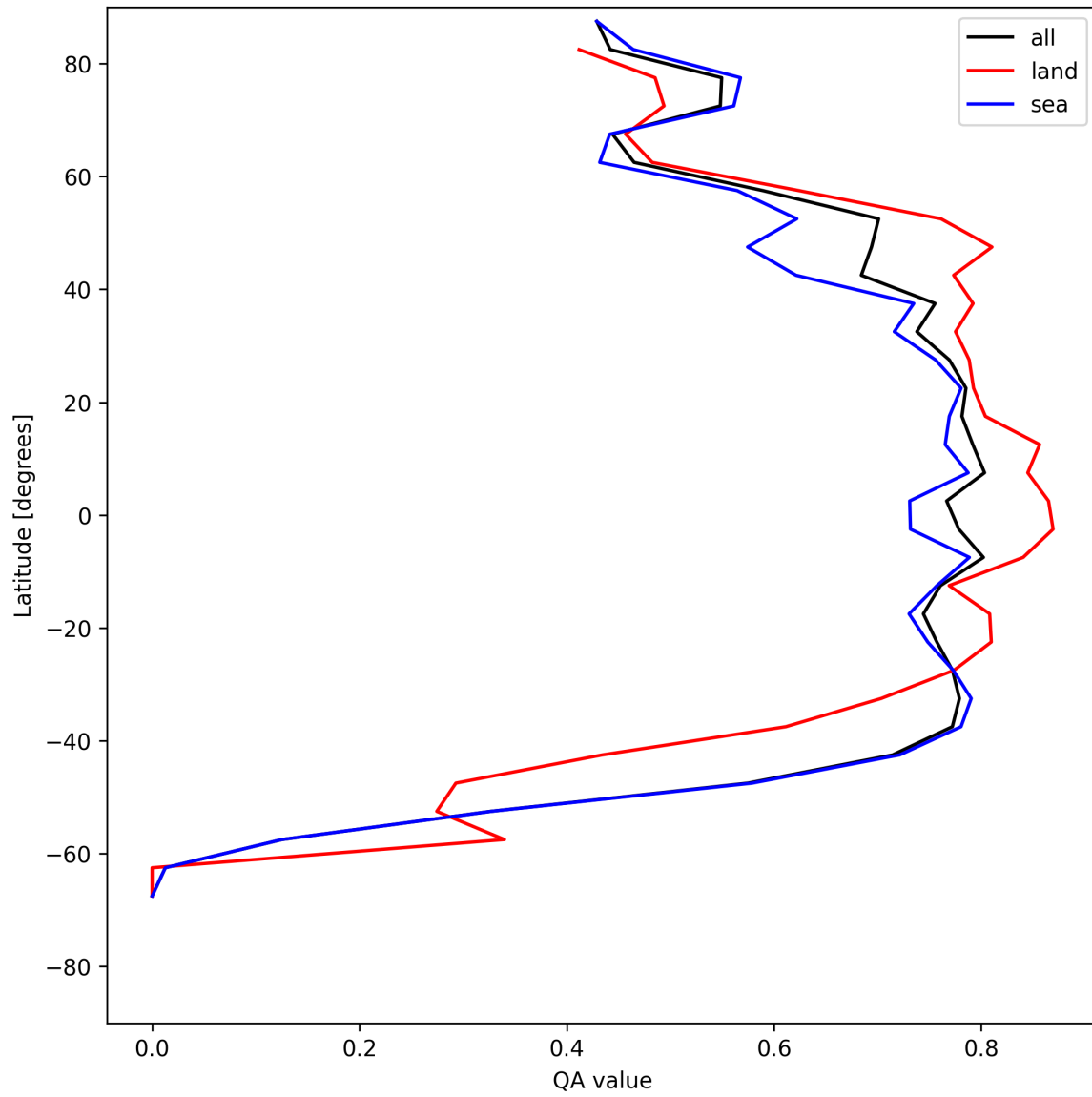
Figure 20: Zonal average of “QA value” for 2025-06-30 to 2025-06-30.
