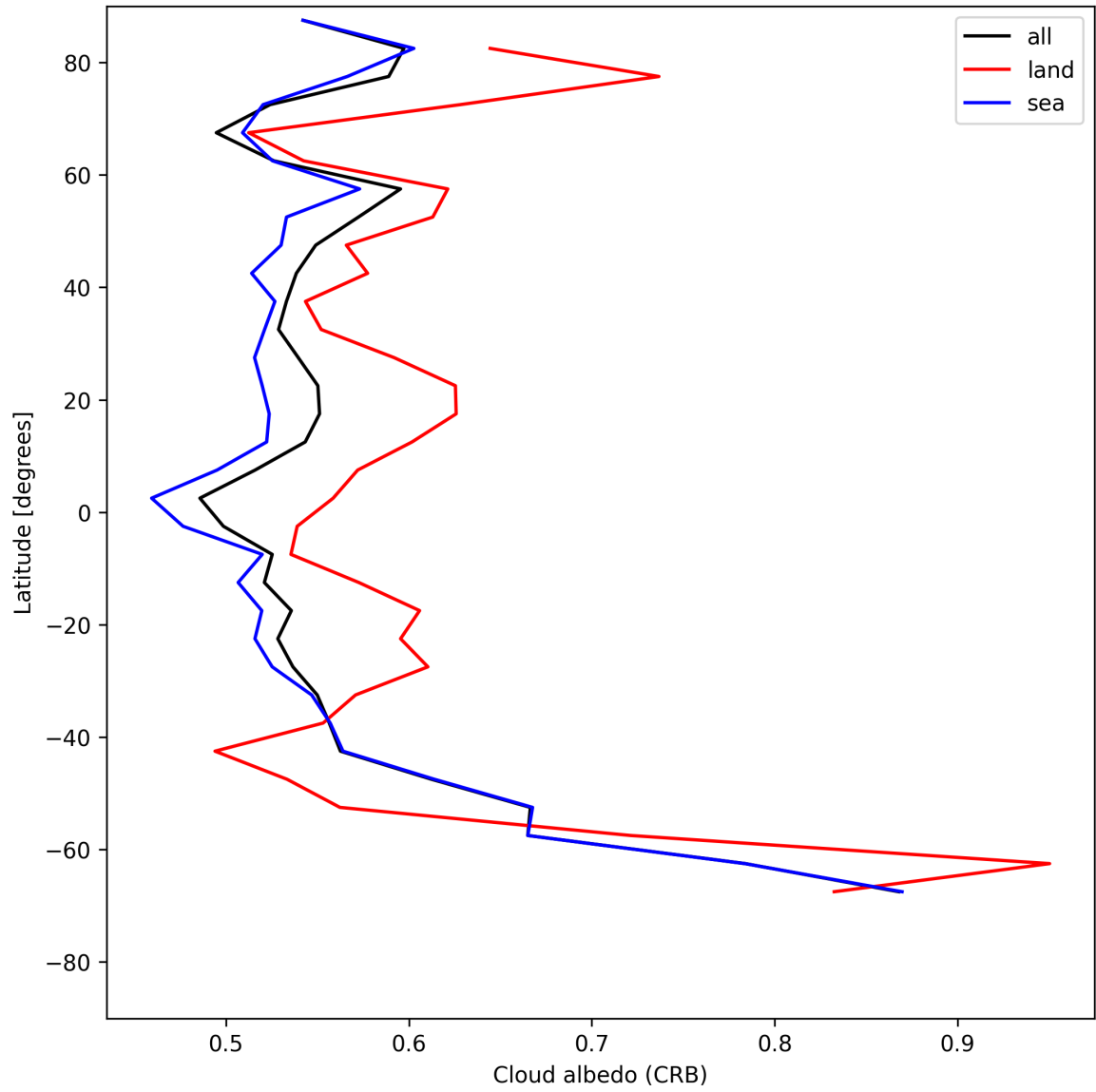
Figure 26: Zonal average of “Cloud albedo (CRB)” for 2025-06-30 to 2025-06-30.
