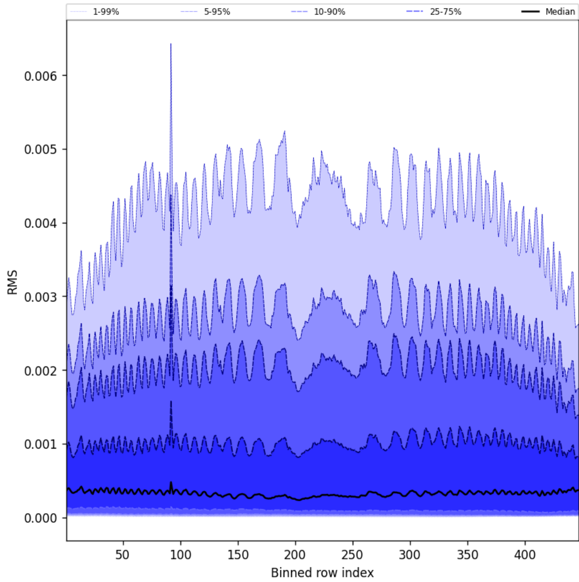
Figure 61: Along track statistics of “RMS” for 2025-06-30 to 2025-06-30
