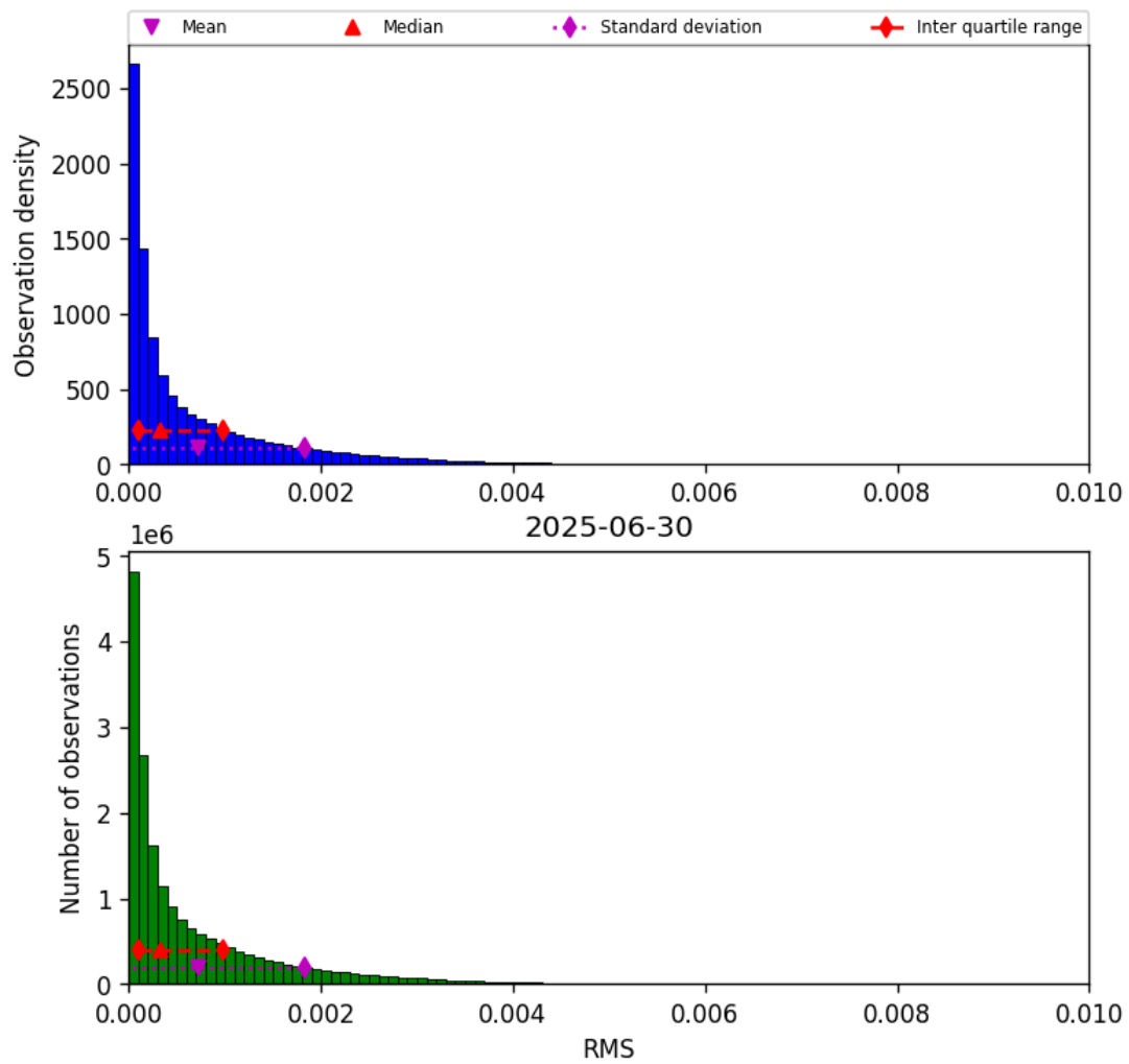
Figure 45: Histogram of “RMS” for 2025-06-30 to 2025-06-30
