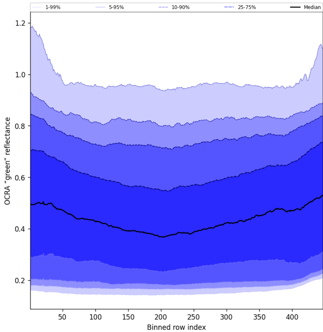
Figure 66: Along track statistics of “OCRA “green” reflectance” for 2025-06-30 to 2025-06-30
