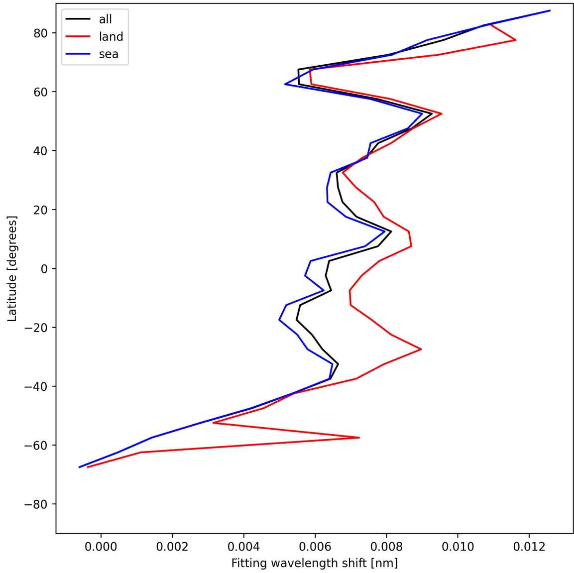
Figure 31: Zonal average of “Fitting wavelength shift” for 2025-06-30 to 2025-06-30.
