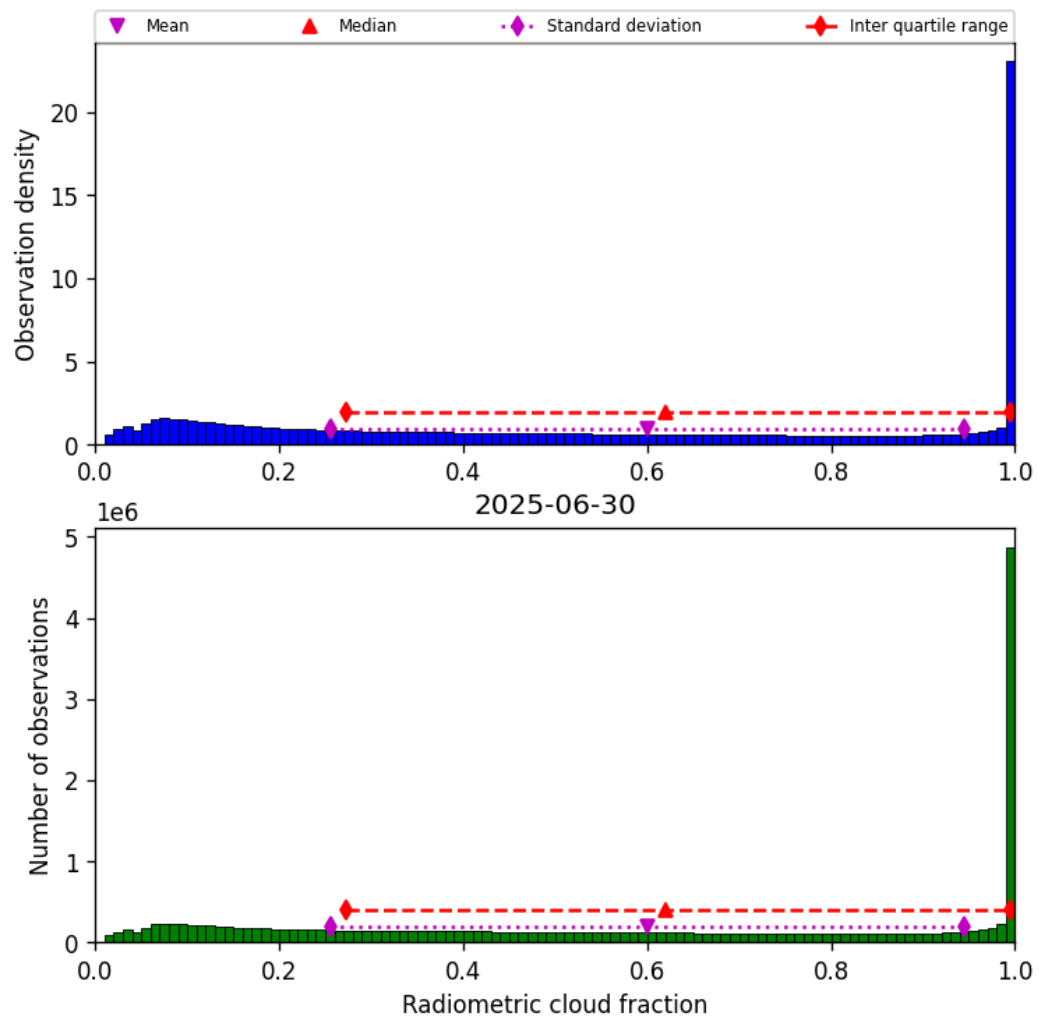
Figure 37: Histogram of “Radiometric cloud fraction” for 2025-06-30 to 2025-06-30
