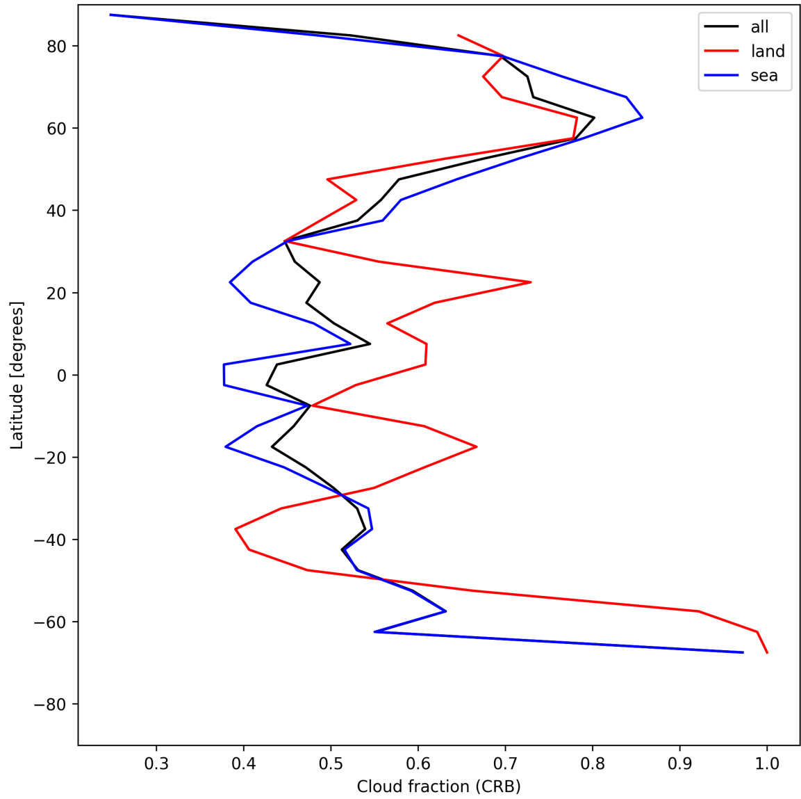
Figure 24: Zonal average of “Cloud fraction (CRB)” for 2025-06-30 to 2025-06-30.
