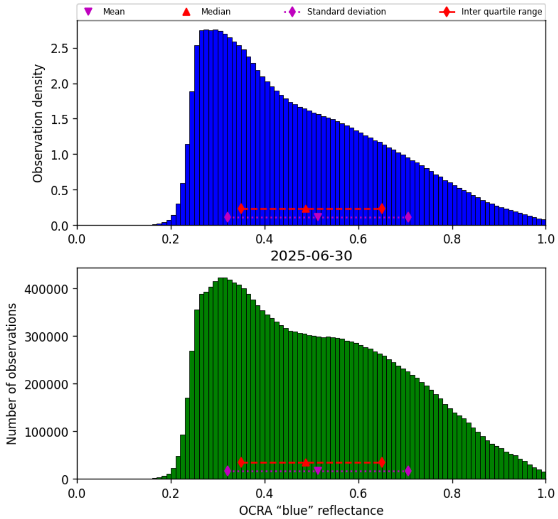
Figure 49: Histogram of “OCRA “blue” reflectance” for 2025-06-30 to 2025-06-30
