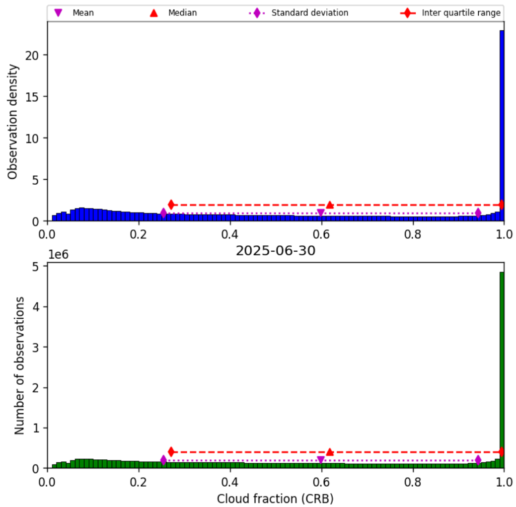
Figure 40: Histogram of “Cloud fraction (CRB)” for 2025-06-30 to 2025-06-30
