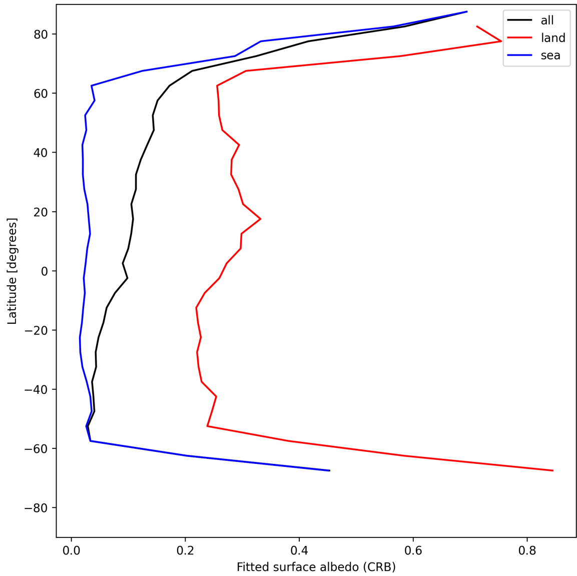
Figure 28: Zonal average of “Fitted surface albedo (CRB)” for 2025-06-30 to 2025-06-30.
