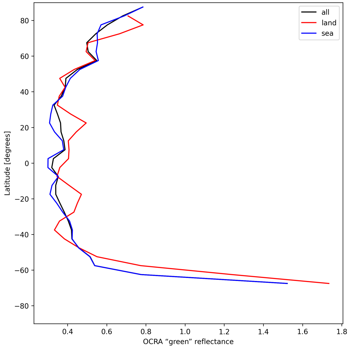
Figure 34: Zonal average of “OCRA “green” reflectance” for 2025-06-30 to 2025-06-30.
