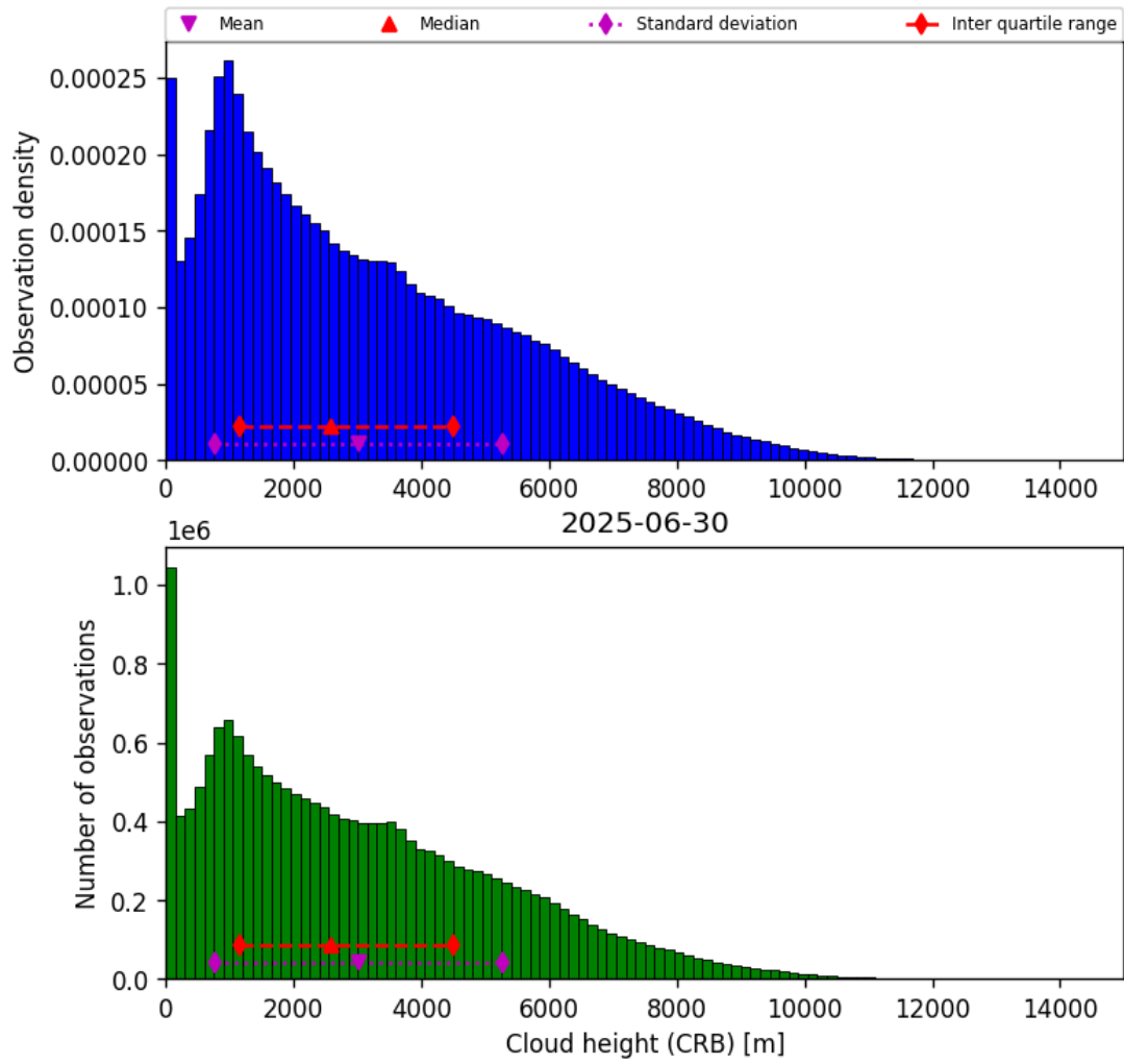
Figure 41: Histogram of “Cloud height (CRB)” for 2025-06-30 to 2025-06-30
