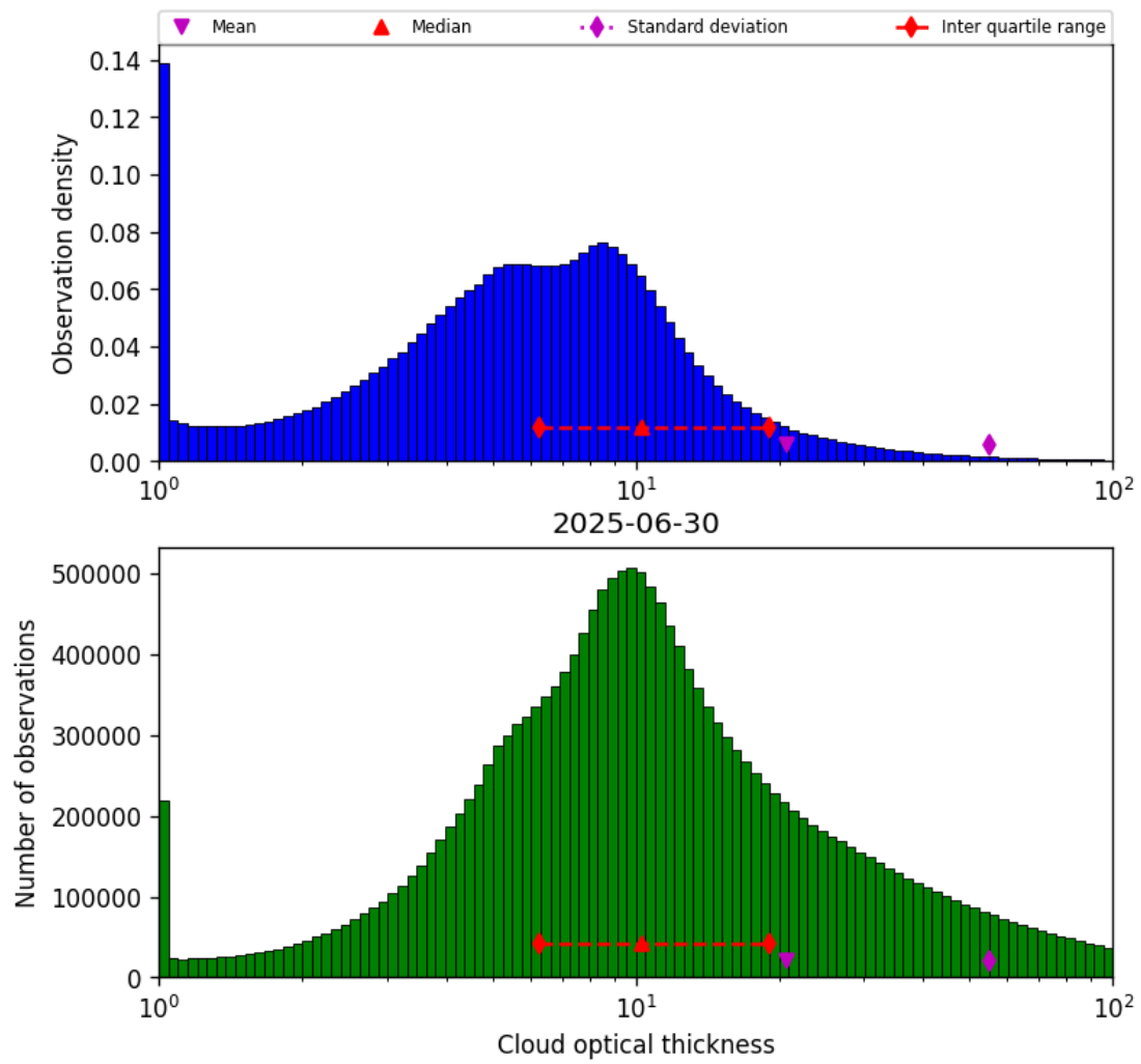
Figure 39: Histogram of “Cloud optical thickness” for 2025-06-30 to 2025-06-30
