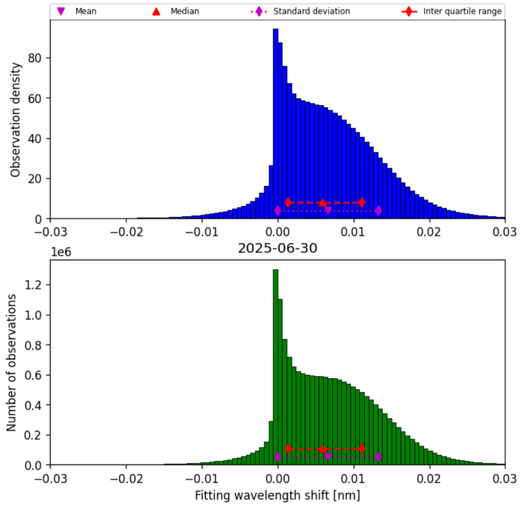
Figure 47: Histogram of “Fitting wavelength shift” for 2025-06-30 to 2025-06-30
