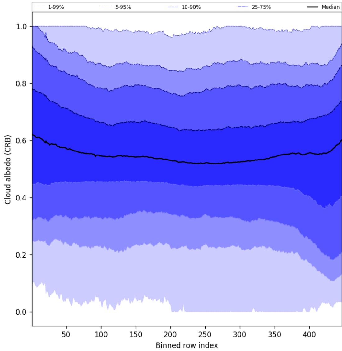
Figure 58: Along track statistics of “Cloud albedo (CRB)” for 2025-06-30 to 2025-06-30
