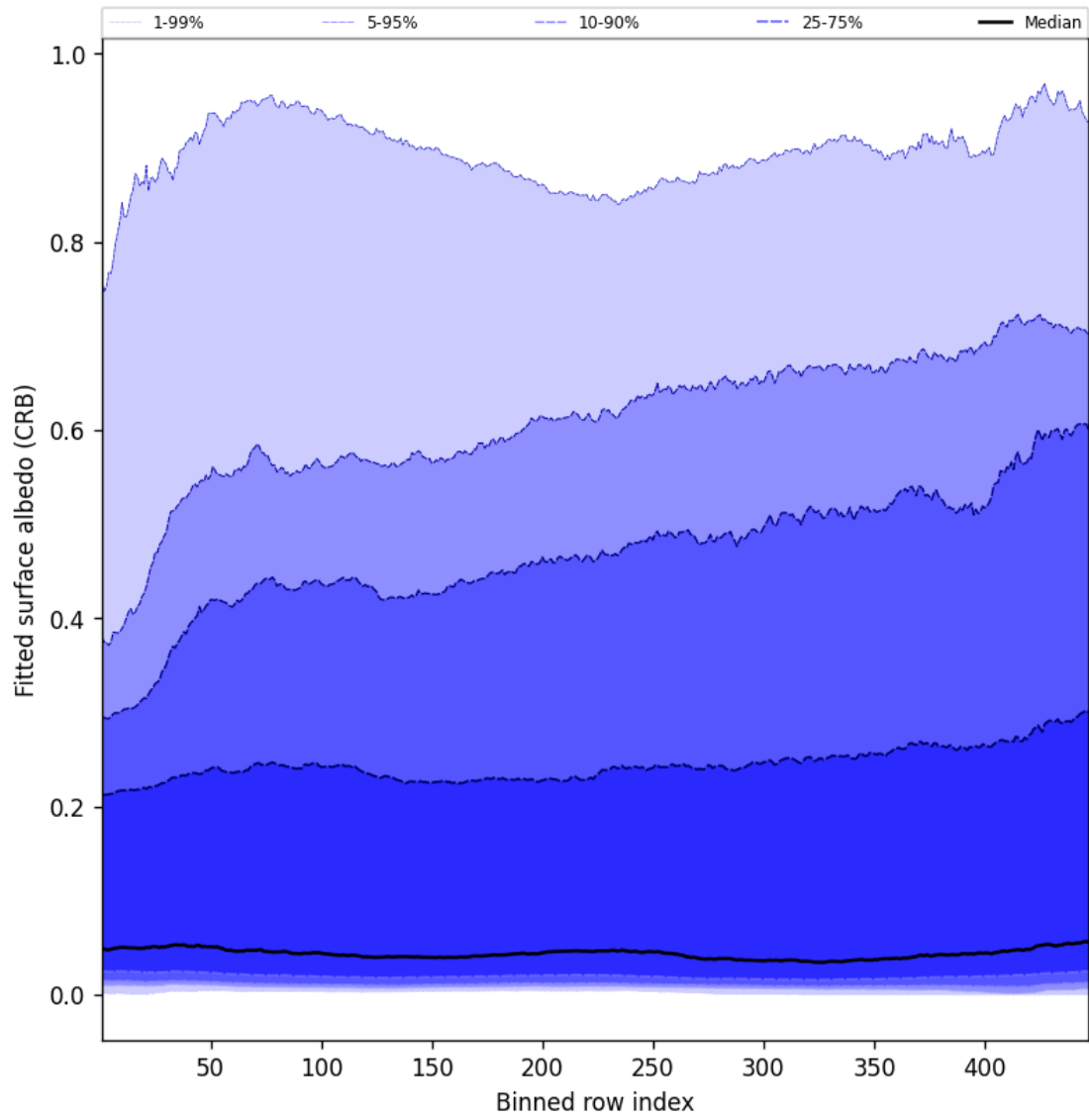
Figure 60: Along track statistics of “Fitted surface albedo (CRB)” for 2025-06-30 to 2025-06-30
