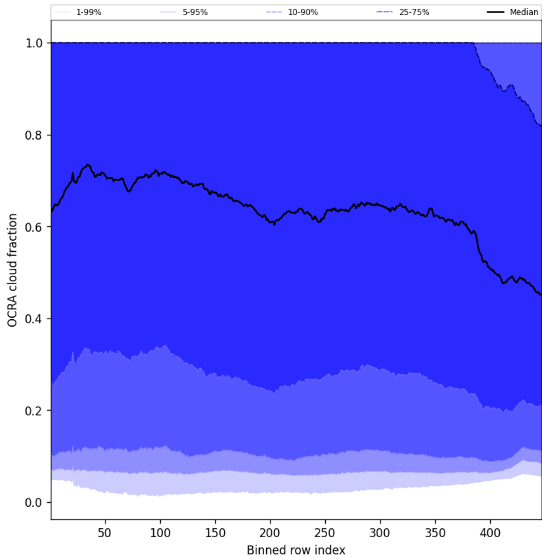
Figure 64: Along track statistics of “OCRA cloud fraction” for 2025-06-30 to 2025-06-30
