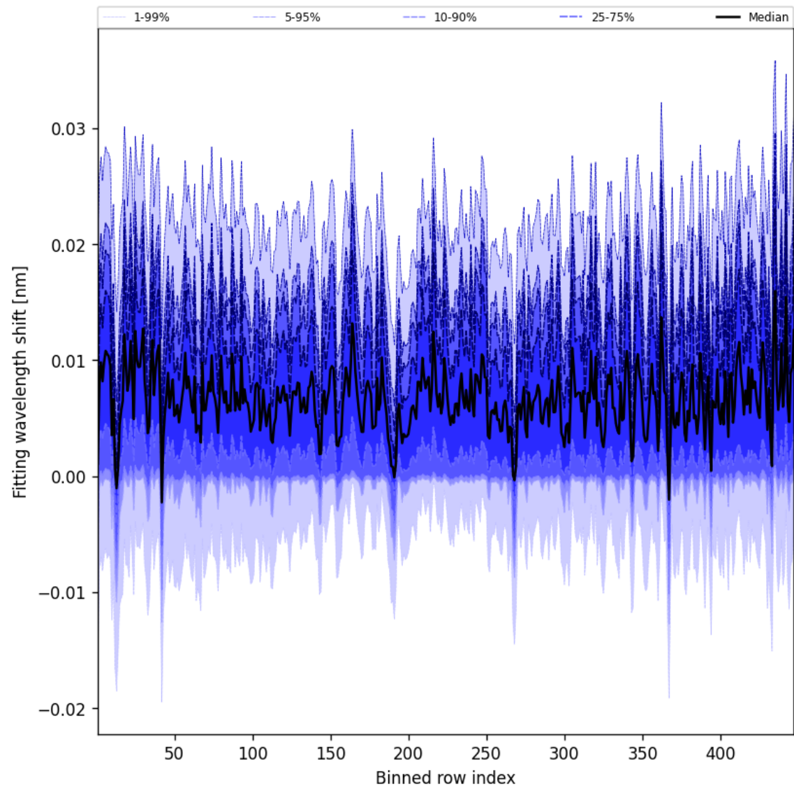
Figure 63: Along track statistics of “Fitting wavelength shift” for 2025-06-30 to 2025-06-30
