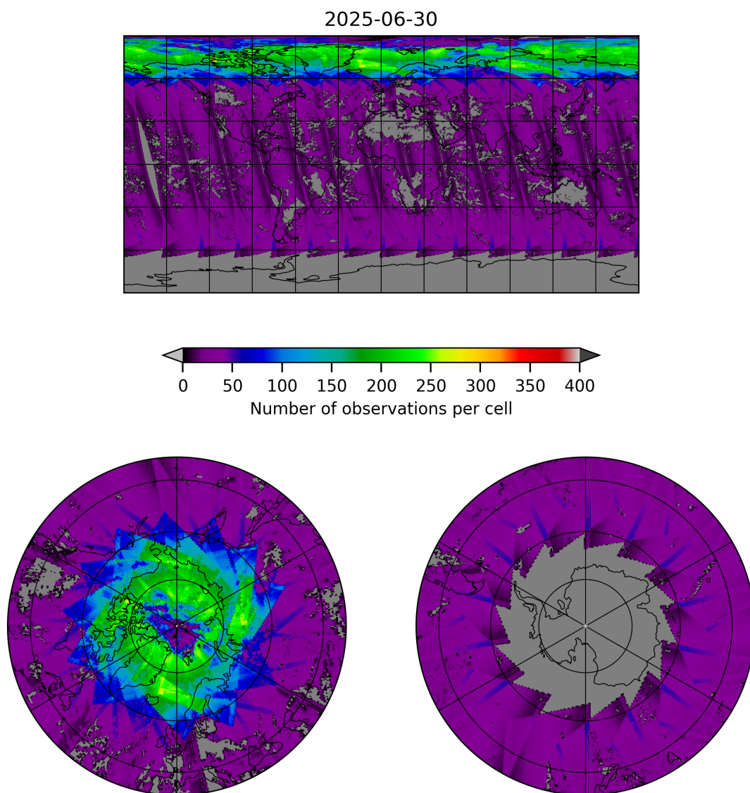
Figure 19: Map of the number of observations for 2025-06-30 to 2025-06-30
