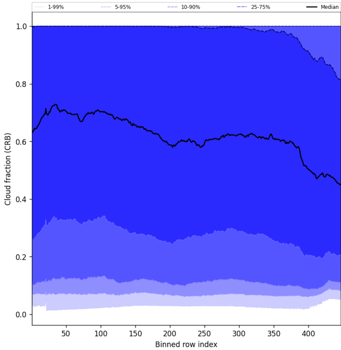
Figure 56: Along track statistics of “Cloud fraction (CRB)” for 2025-06-30 to 2025-06-30
