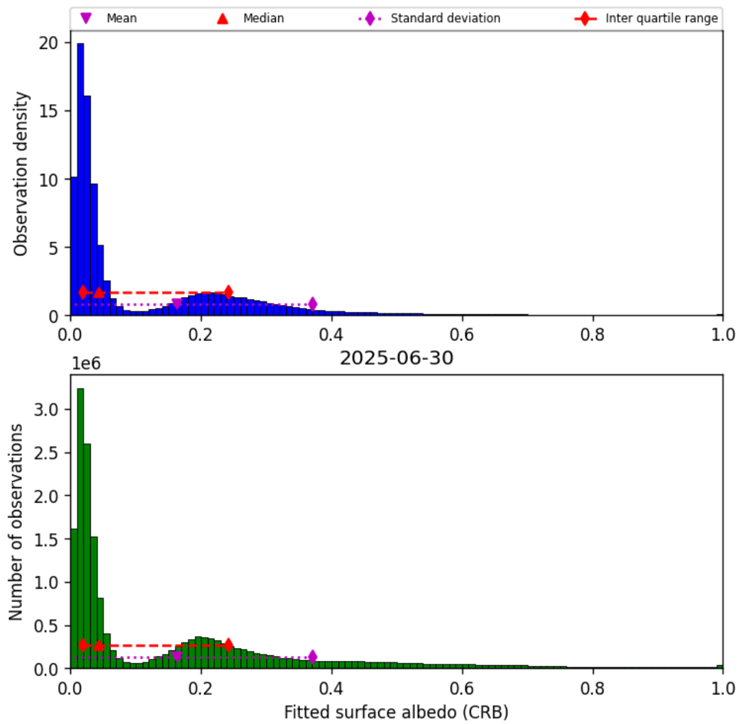
Figure 44: Histogram of “Fitted surface albedo (CRB)” for 2025-06-30 to 2025-06-30
