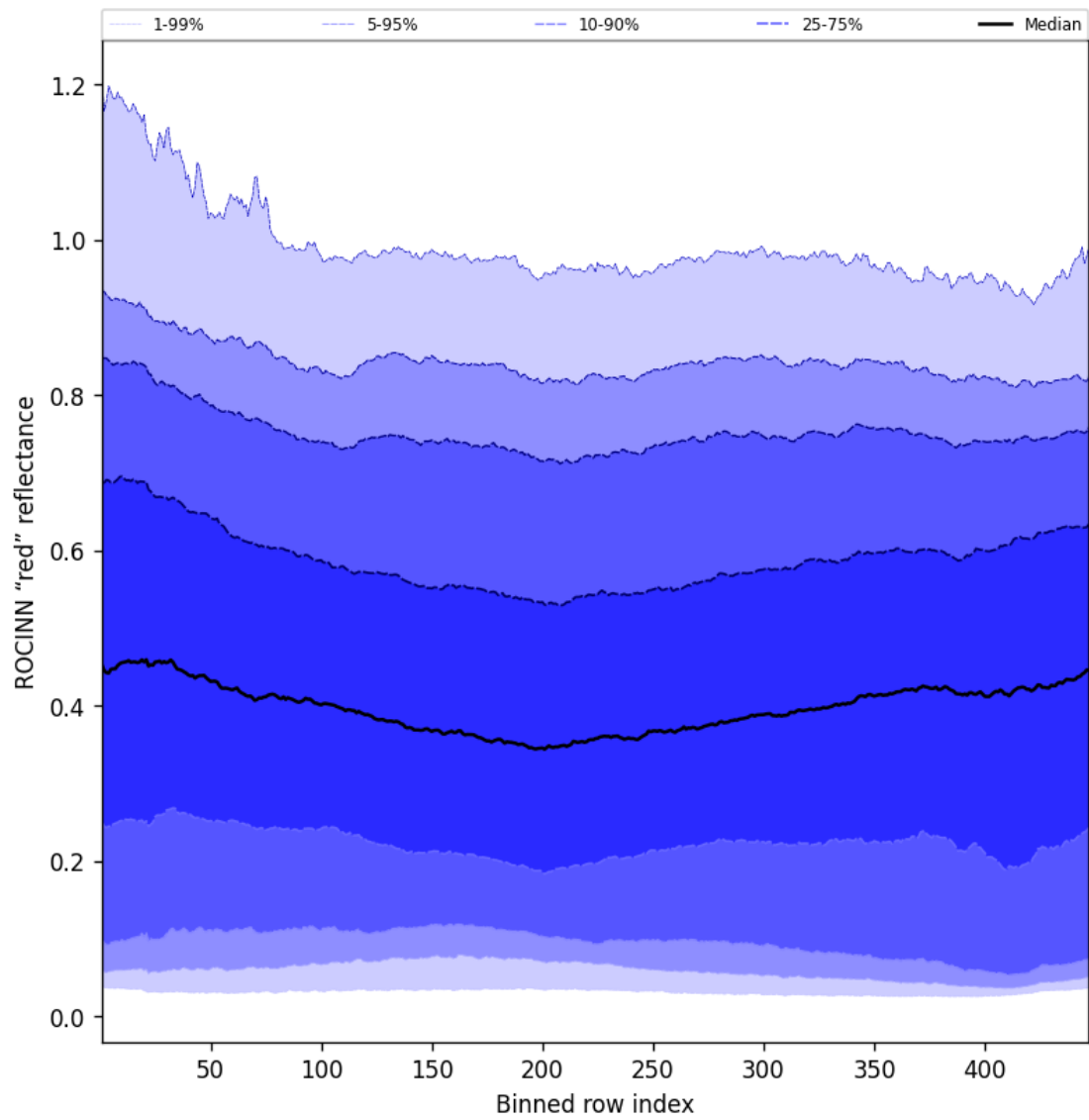
Figure 67: Along track statistics of "ROCINN red" reflectance" for 2025-06-30 to 2025-06-30
