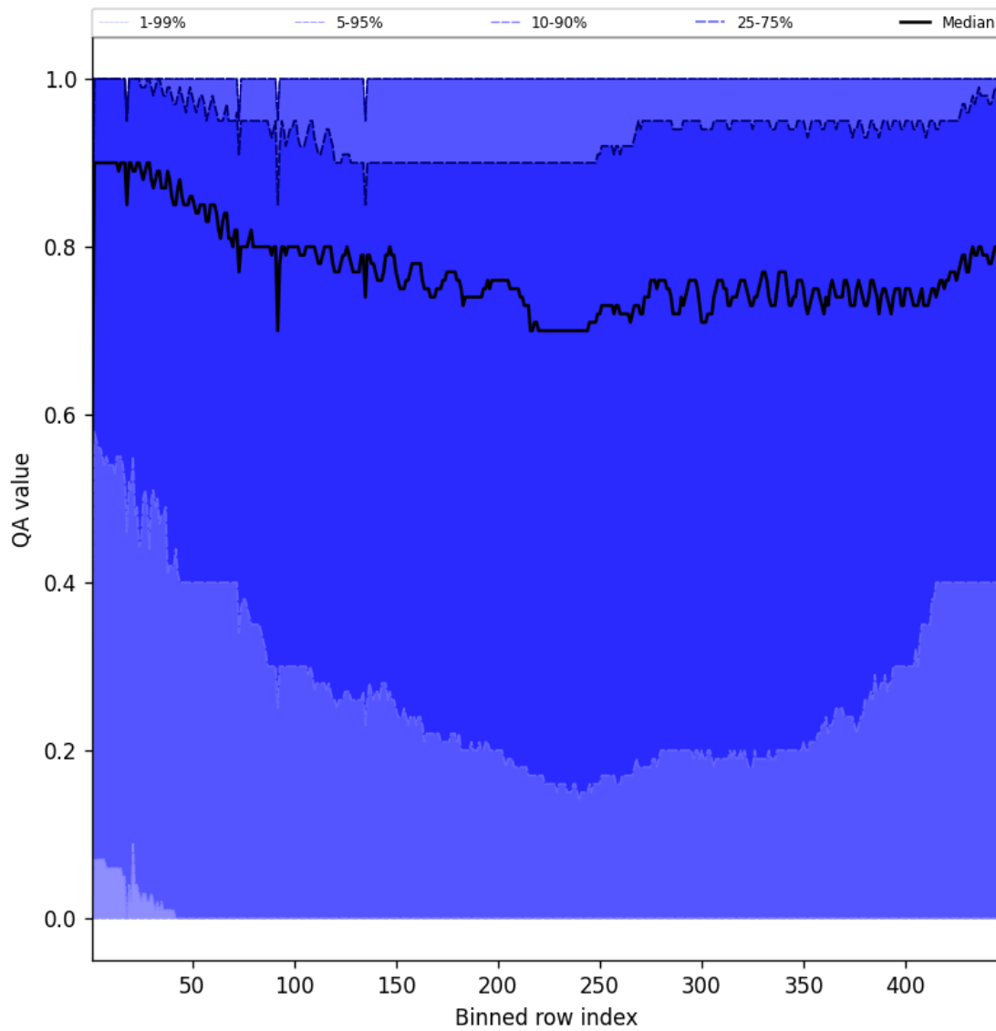
Figure 52: Along track statistics of “QA value” for 2025-06-30 to 2025-06-30
