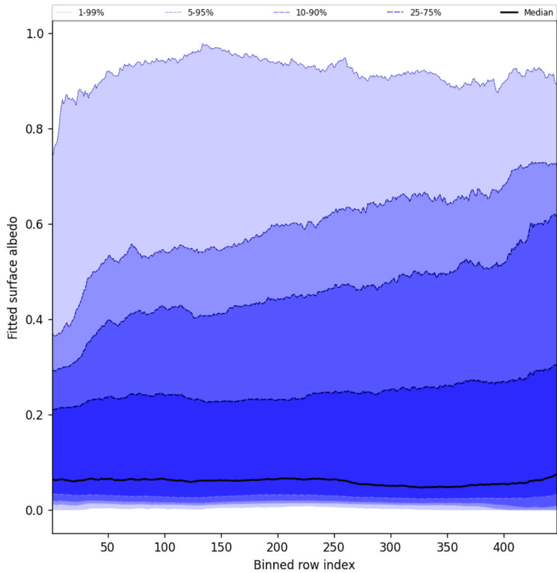
Figure 59: Along track statistics of “Fitted surface albedo” for 2025-06-30 to 2025-06-30
