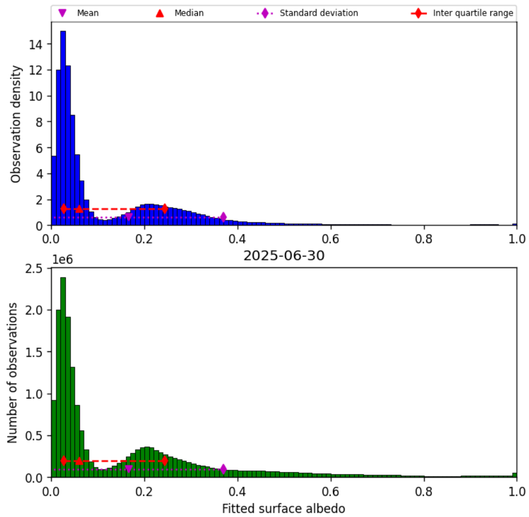
Figure 43: Histogram of “Fitted surface albedo” for 2025-06-30 to 2025-06-30
