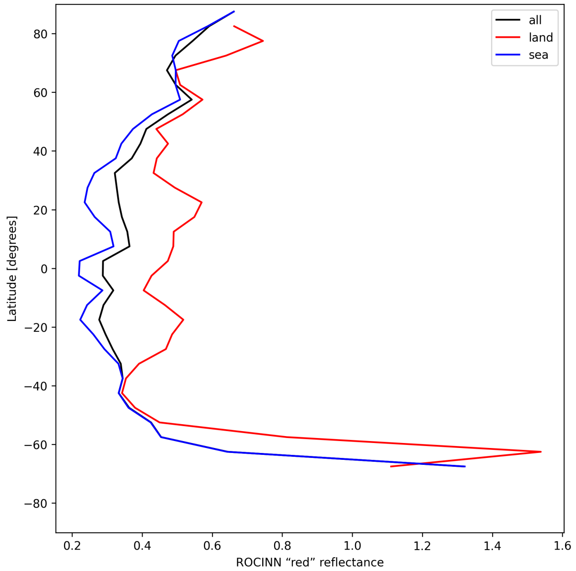
Figure 35: Zonal average of "ROCINN "red" reflectance" for 2025-06-30 to 2025-06-30.
