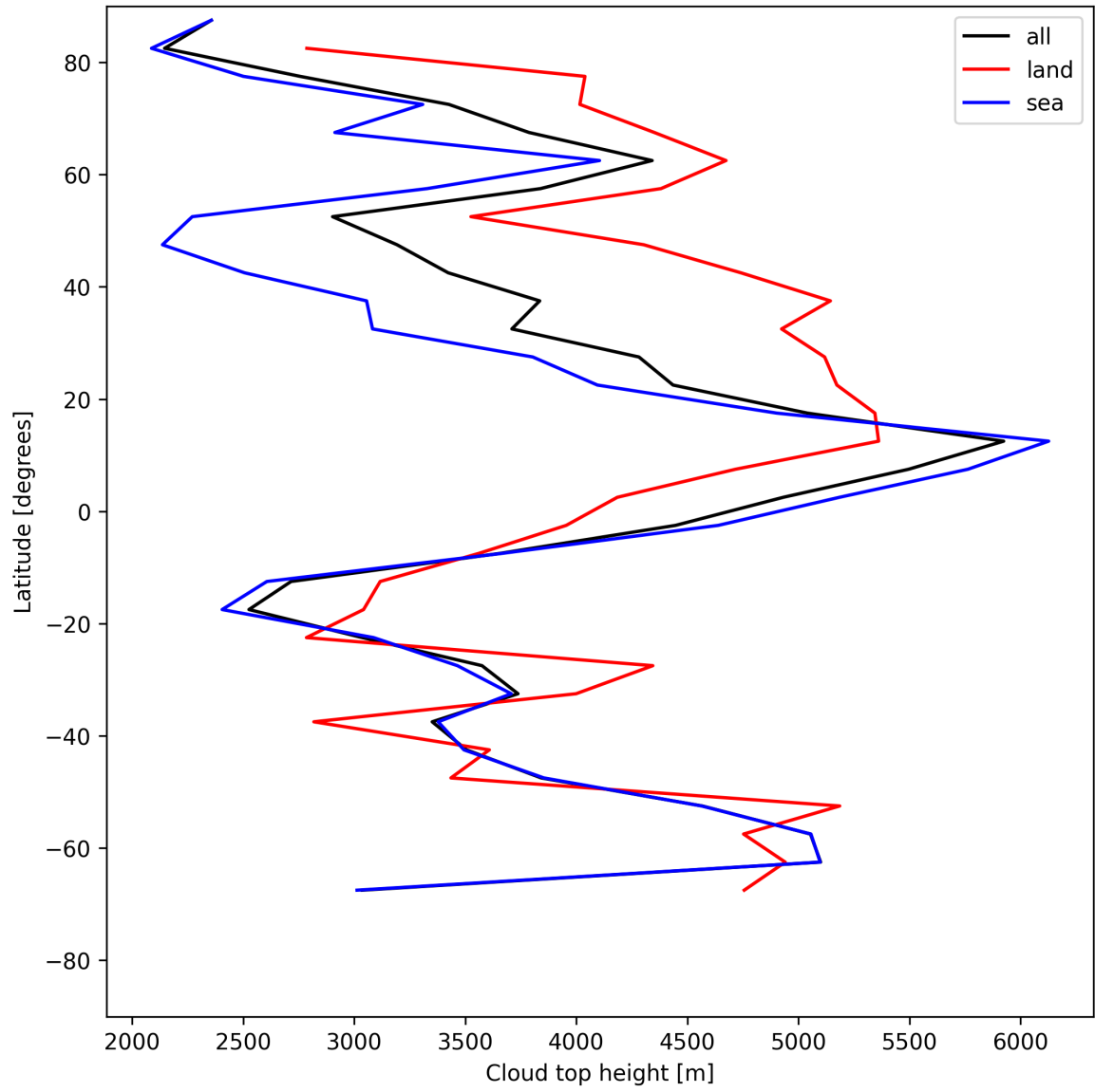
Figure 22: Zonal average of “Cloud top height” for 2025-06-30 to 2025-06-30.
