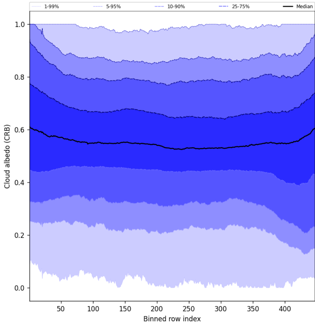
Figure 58: Along track statistics of “Cloud albedo (CRB)” for 2025-07-02 to 2025-07-03
