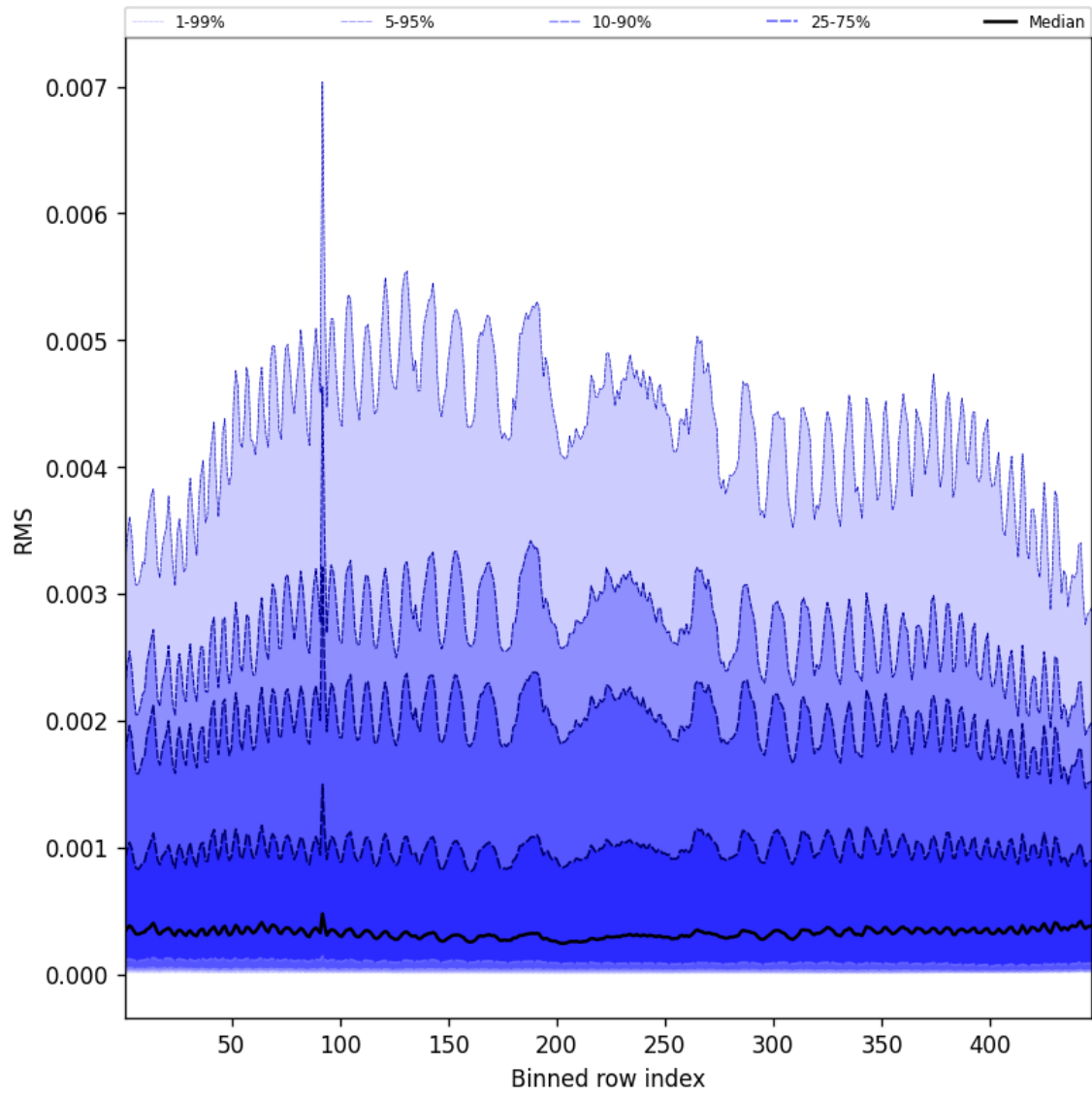
Figure 61: Along track statistics of “RMS” for 2025-07-02 to 2025-07-03
