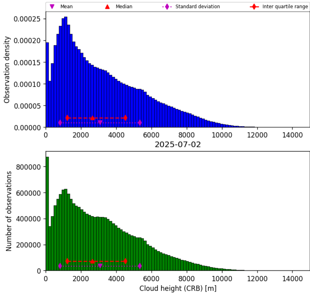
Figure 41: Histogram of “Cloud height (CRB)” for 2025-07-02 to 2025-07-03
