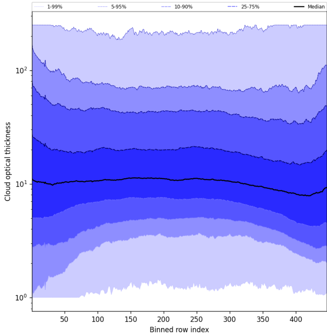
Figure 55: Along track statistics of “Cloud optical thickness” for 2025-07-02 to 2025-07-03
