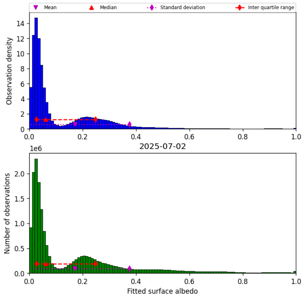
Figure 43: Histogram of “Fitted surface albedo” for 2025-07-02 to 2025-07-03
