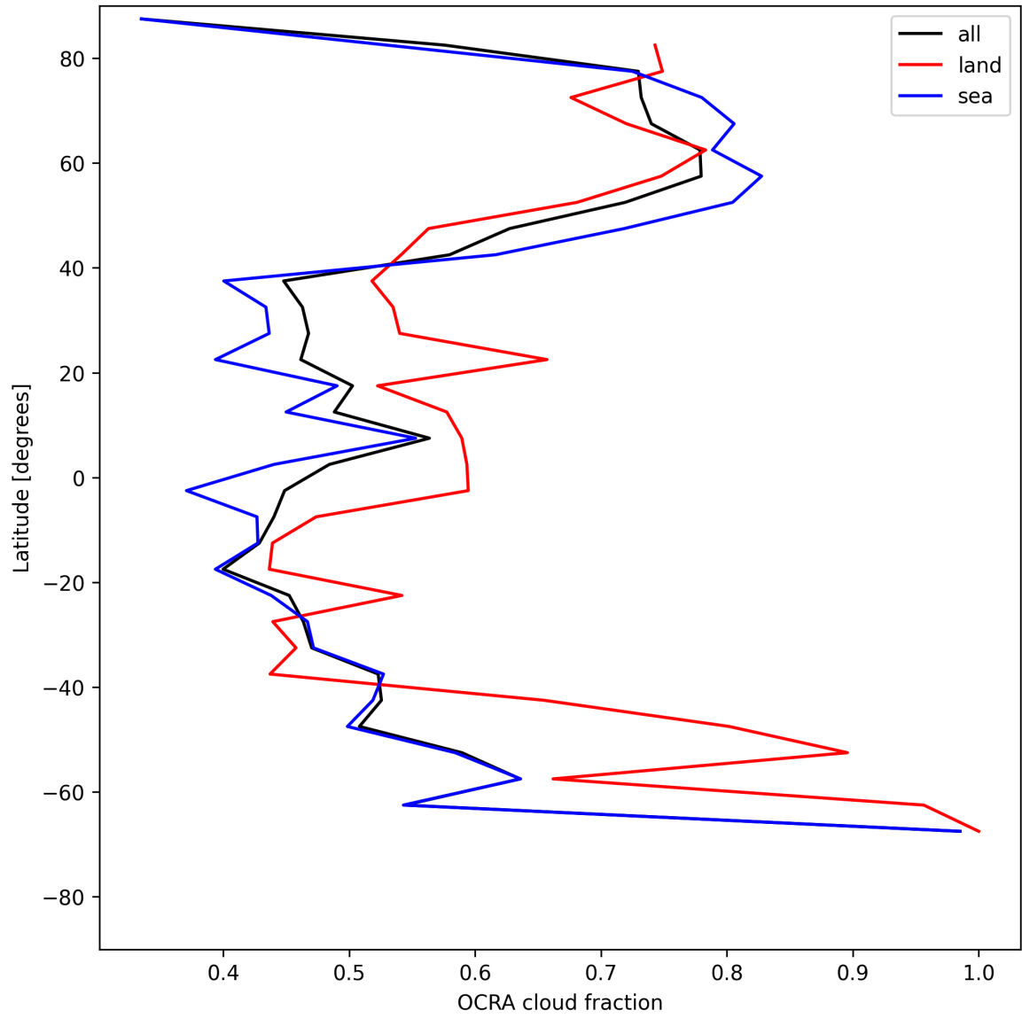
Figure 32: Zonal average of “OCRA cloud fraction” for 2025-07-02 to 2025-07-03.
