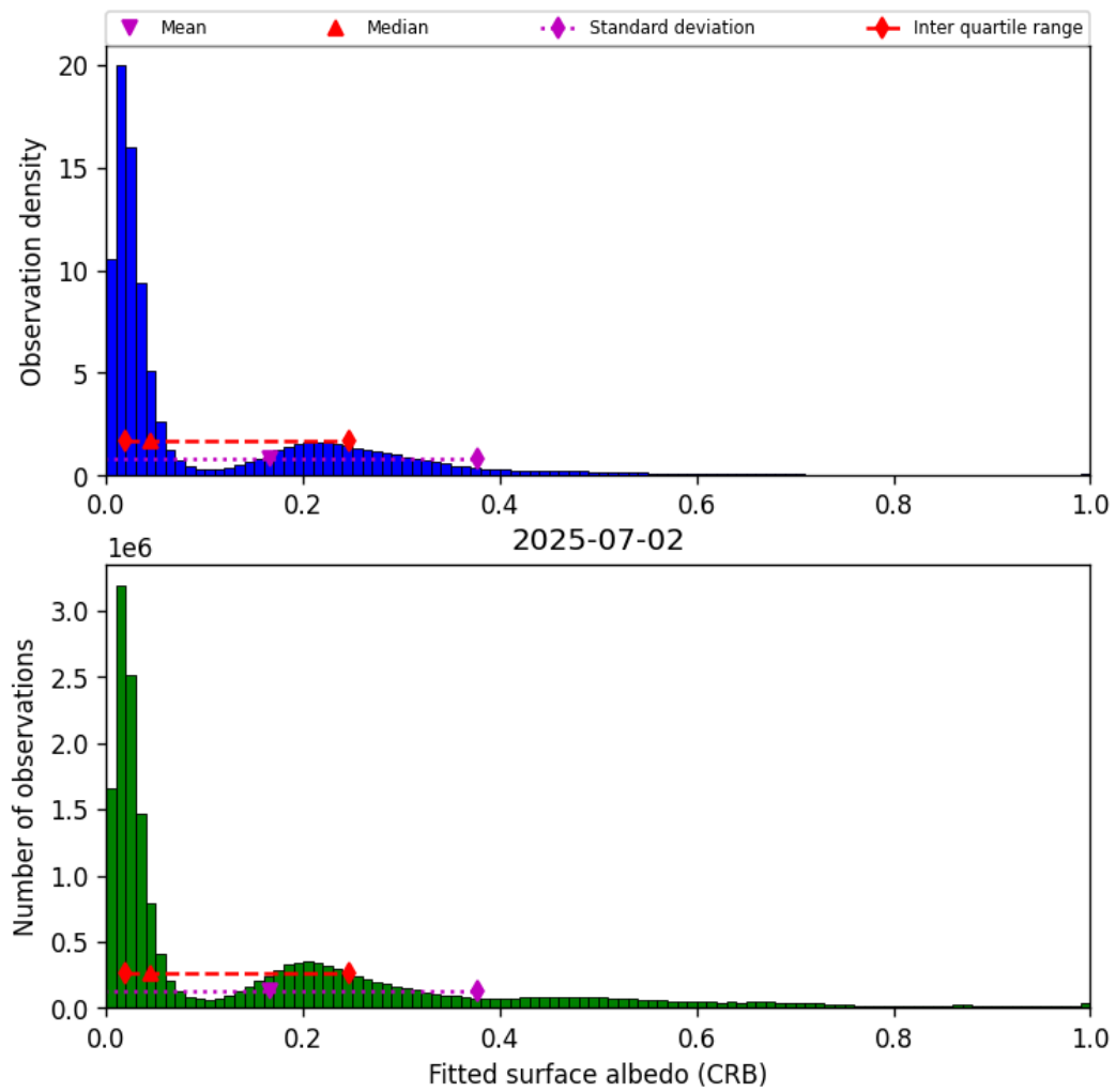
Figure 44: Histogram of “Fitted surface albedo (CRB)” for 2025-07-02 to 2025-07-03
