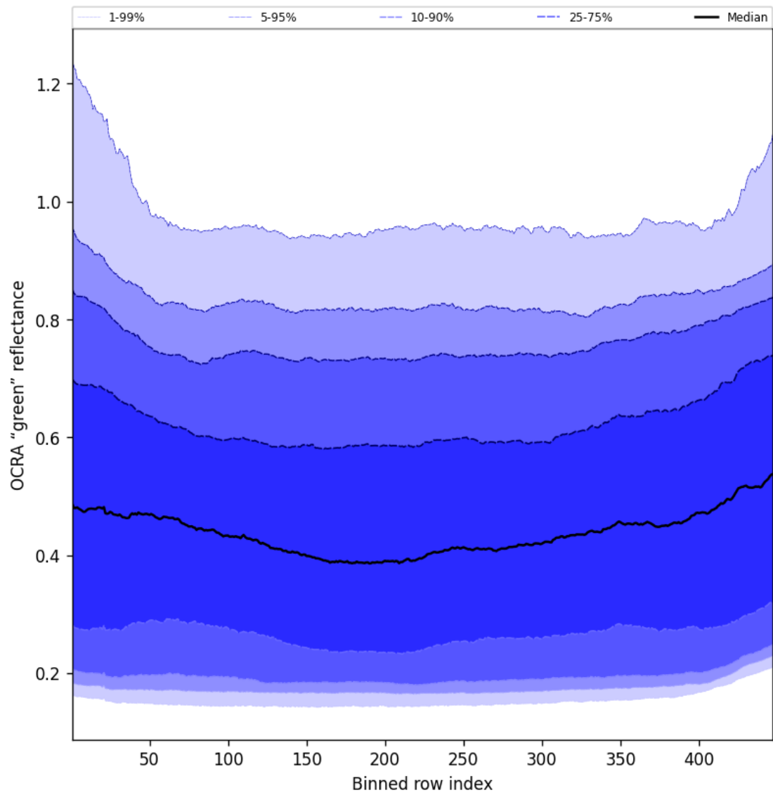
Figure 66: Along track statistics of “OCRA “green” reflectance” for 2025-07-02 to 2025-07-03
