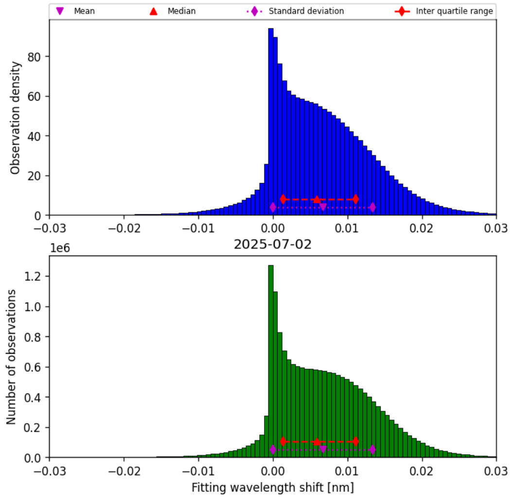
Figure 47: Histogram of “Fitting wavelength shift” for 2025-07-02 to 2025-07-03
