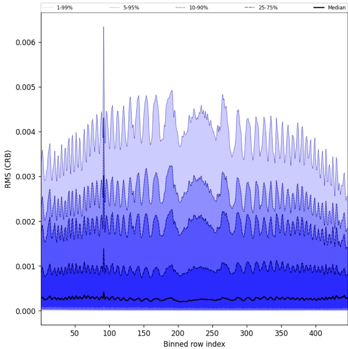
Figure 62: Along track statistics of “RMS (CRB)” for 2025-07-02 to 2025-07-03
