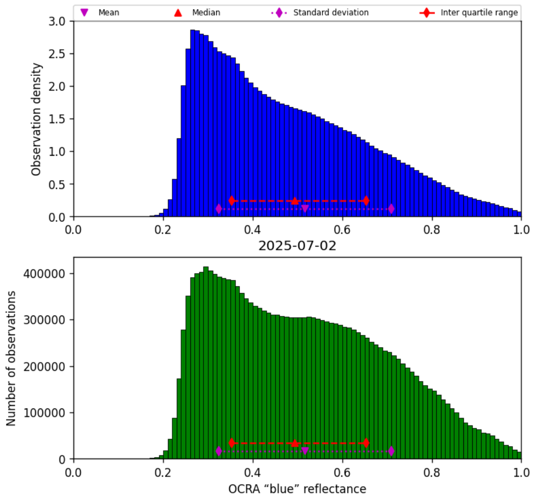
Figure 49: Histogram of “OCRA “blue” reflectance” for 2025-07-02 to 2025-07-03
