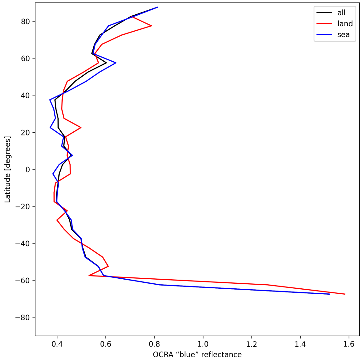
Figure 33: Zonal average of “OCRA “blue” reflectance” for 2025-07-02 to 2025-07-03.
