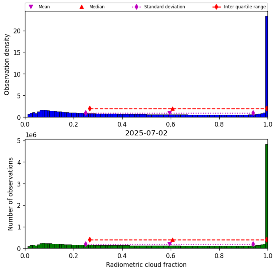
Figure 37: Histogram of “Radiometric cloud fraction” for 2025-07-02 to 2025-07-03
