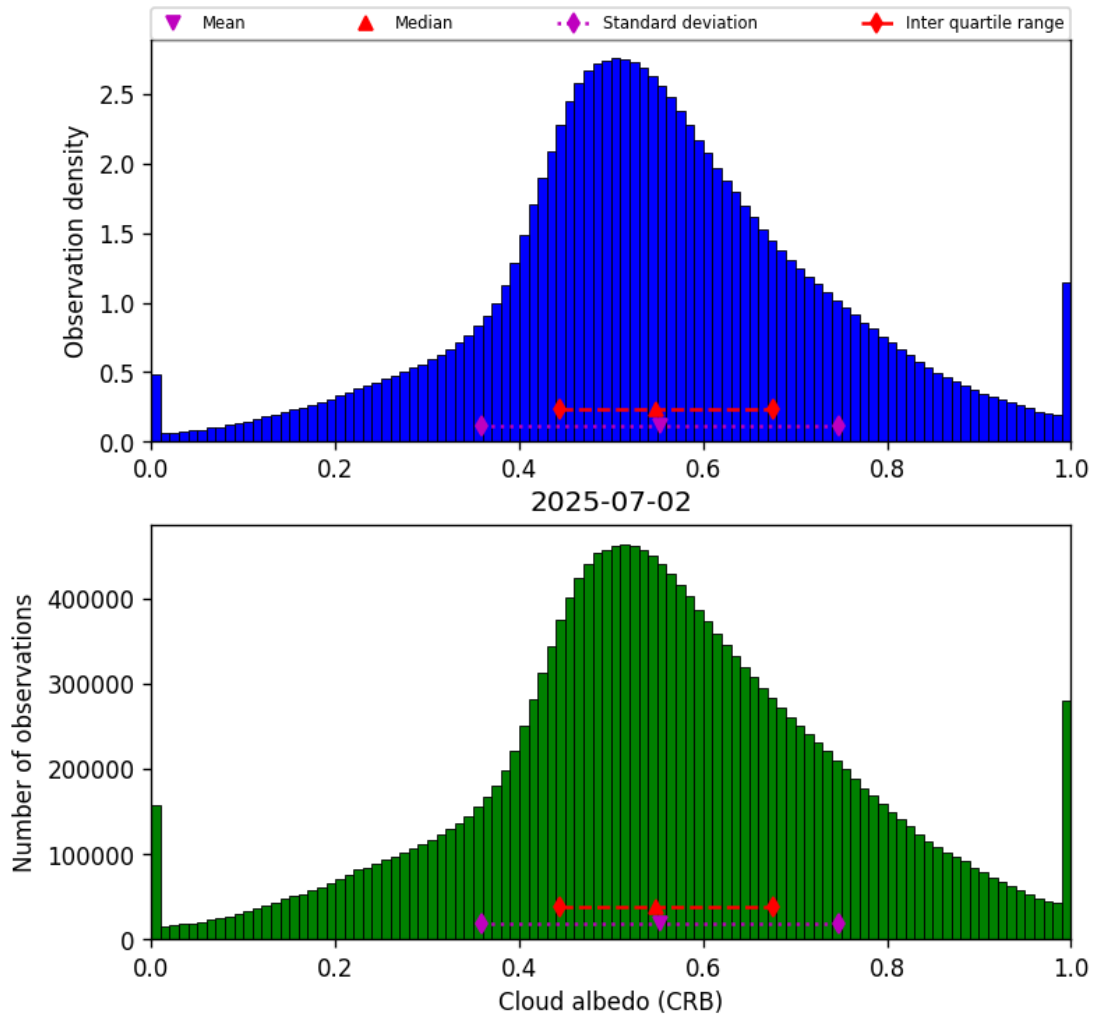
Figure 42: Histogram of “Cloud albedo (CRB)” for 2025-07-02 to 2025-07-03
