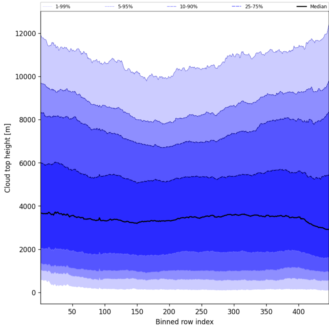
Figure 54: Along track statistics of “Cloud top height” for 2025-07-02 to 2025-07-03
