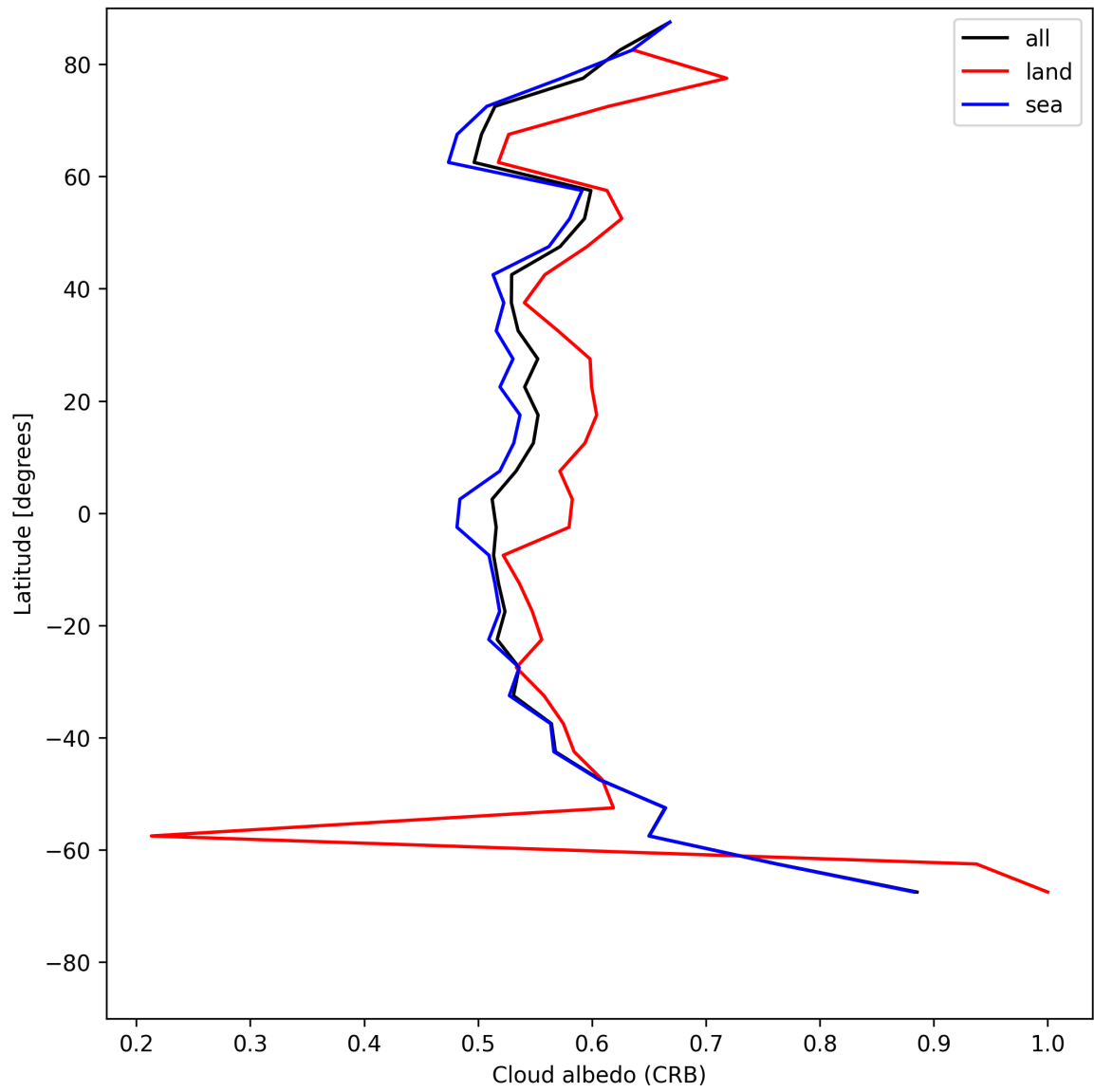
Figure 26: Zonal average of “Cloud albedo (CRB)” for 2025-07-02 to 2025-07-03.
