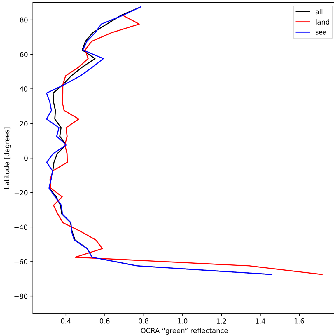
Figure 34: Zonal average of “OCRA “green” reflectance” for 2025-07-02 to 2025-07-03.
