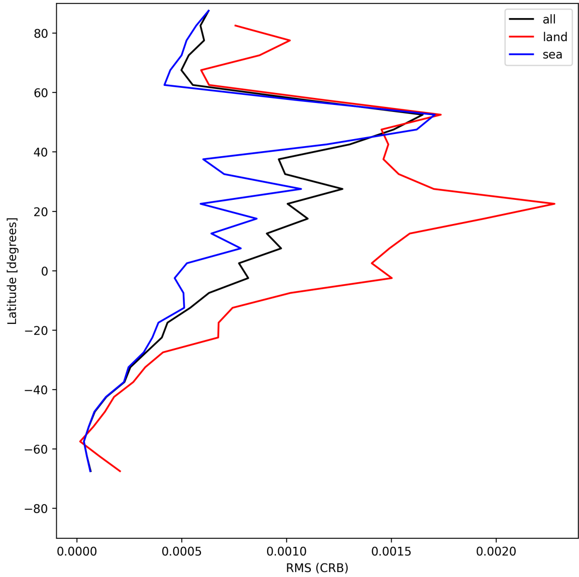
Figure 30: Zonal average of “RMS (CRB)” for 2025-07-02 to 2025-07-03.
