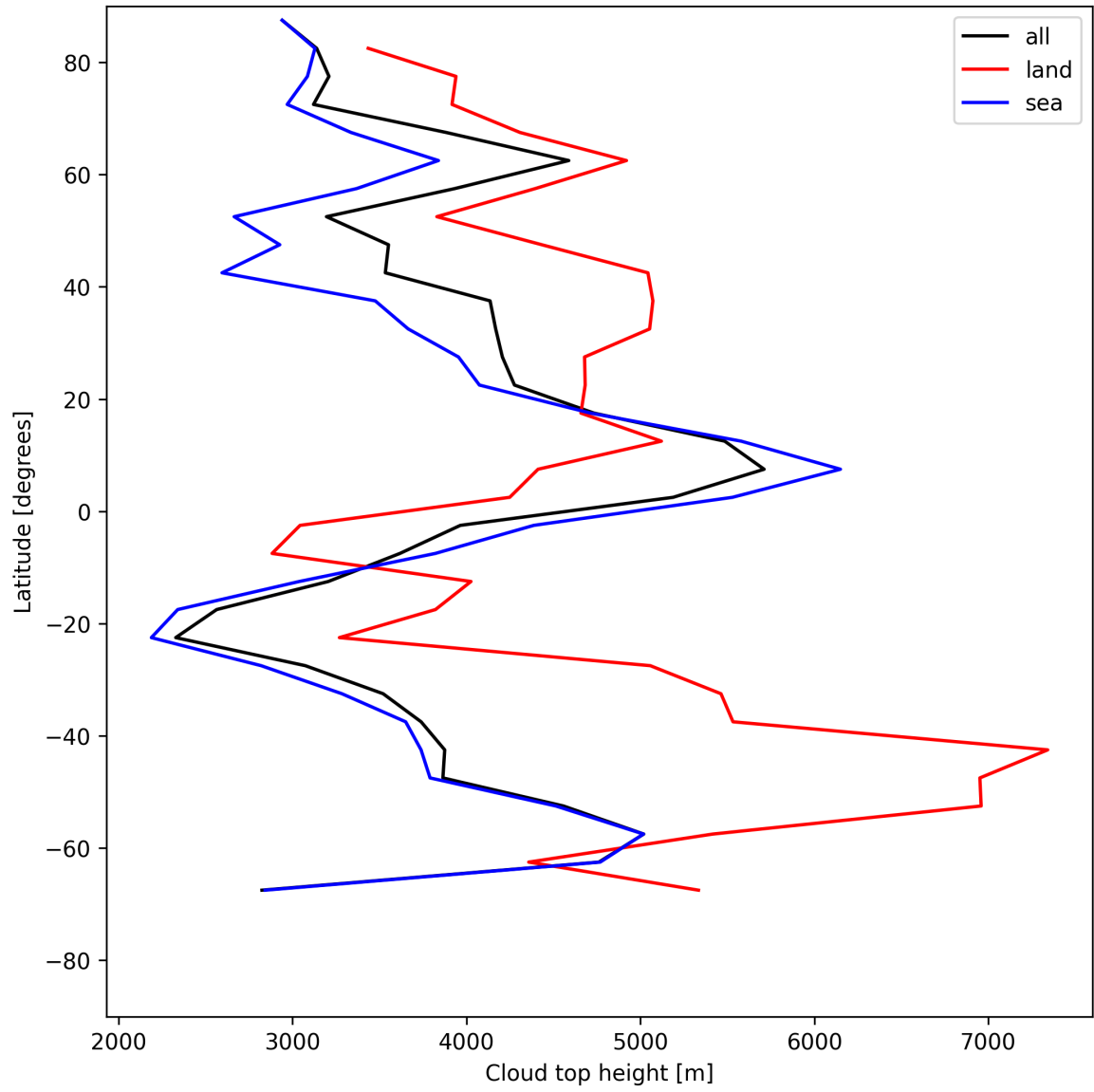
Figure 22: Zonal average of “Cloud top height” for 2025-07-02 to 2025-07-03.
