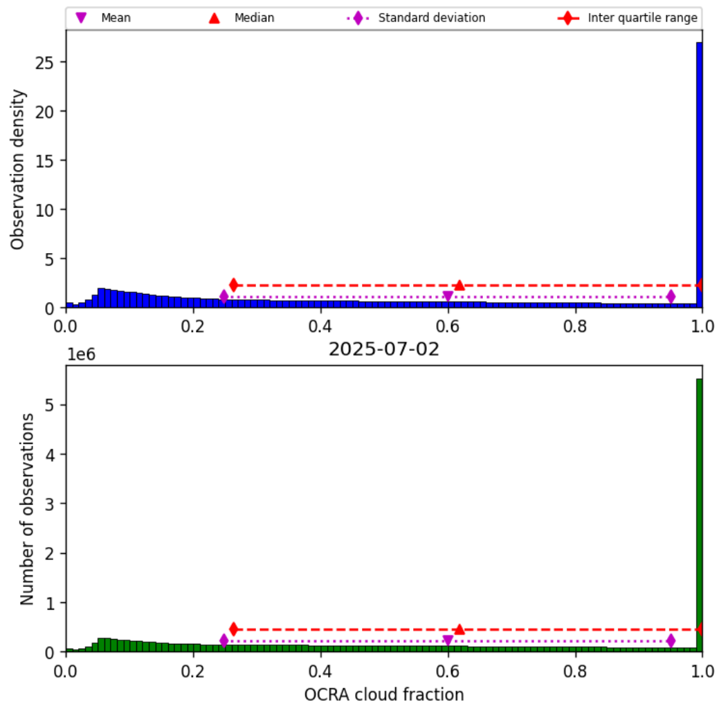
Figure 48: Histogram of “OCRA cloud fraction” for 2025-07-02 to 2025-07-03
