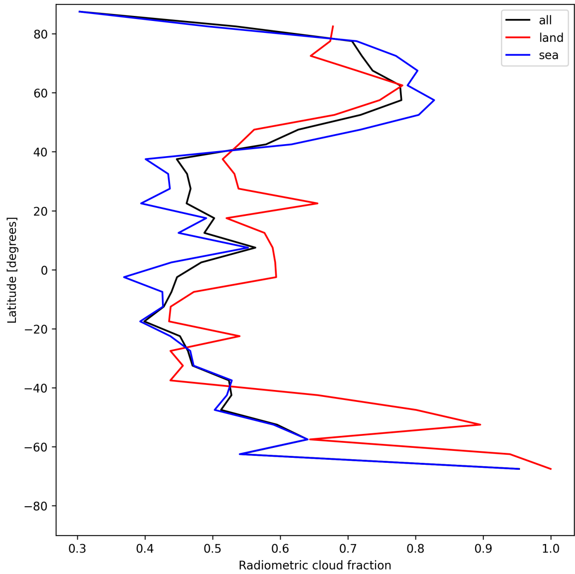
Figure 21: Zonal average of “Radiometric cloud fraction” for 2025-07-02 to 2025-07-03.
