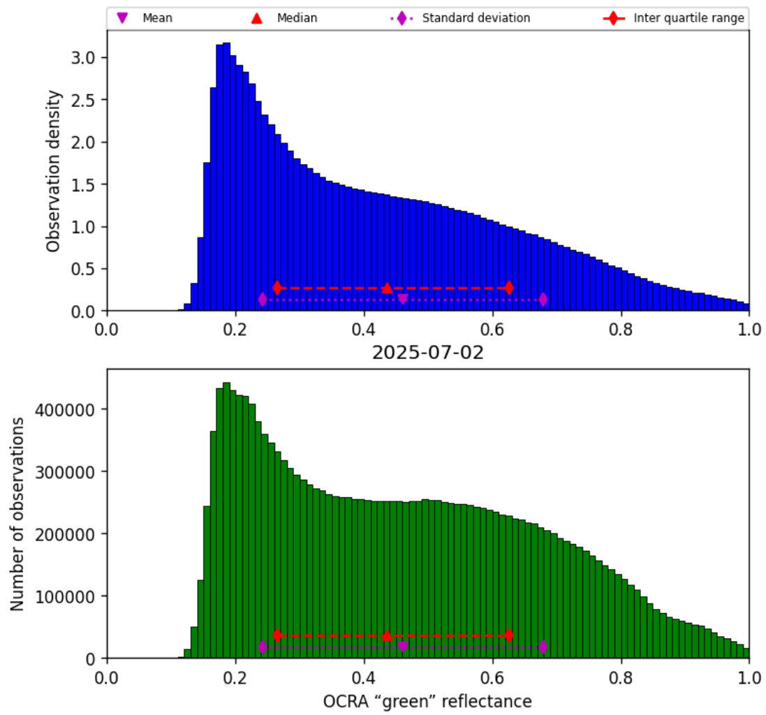
Figure 50: Histogram of “OCRA “green” reflectance” for 2025-07-02 to 2025-07-03
