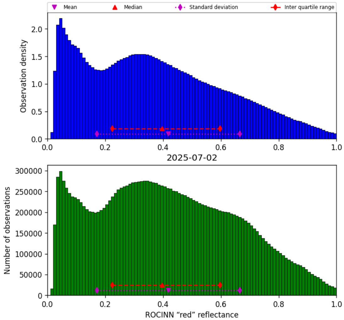
Figure 51: Histogram of “ROCINN “red” reflectance” for 2025-07-02 to 2025-07-03
