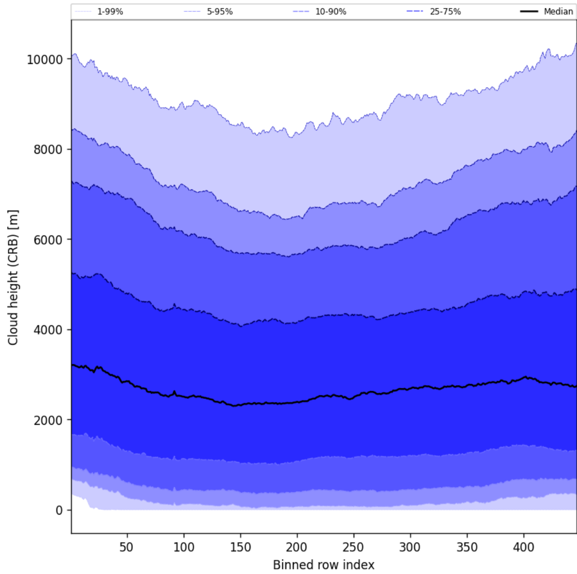
Figure 57: Along track statistics of “Cloud height (CRB)” for 2025-07-02 to 2025-07-03
