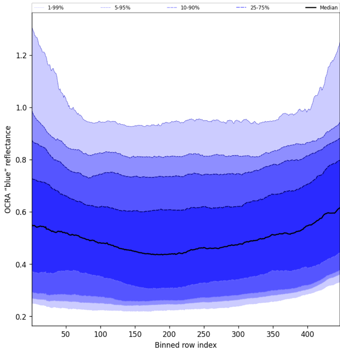
Figure 65: Along track statistics of “OCRA “blue” reflectance” for 2025-07-02 to 2025-07-03
