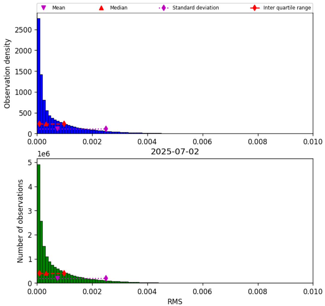
Figure 45: Histogram of “RMS” for 2025-07-02 to 2025-07-03
