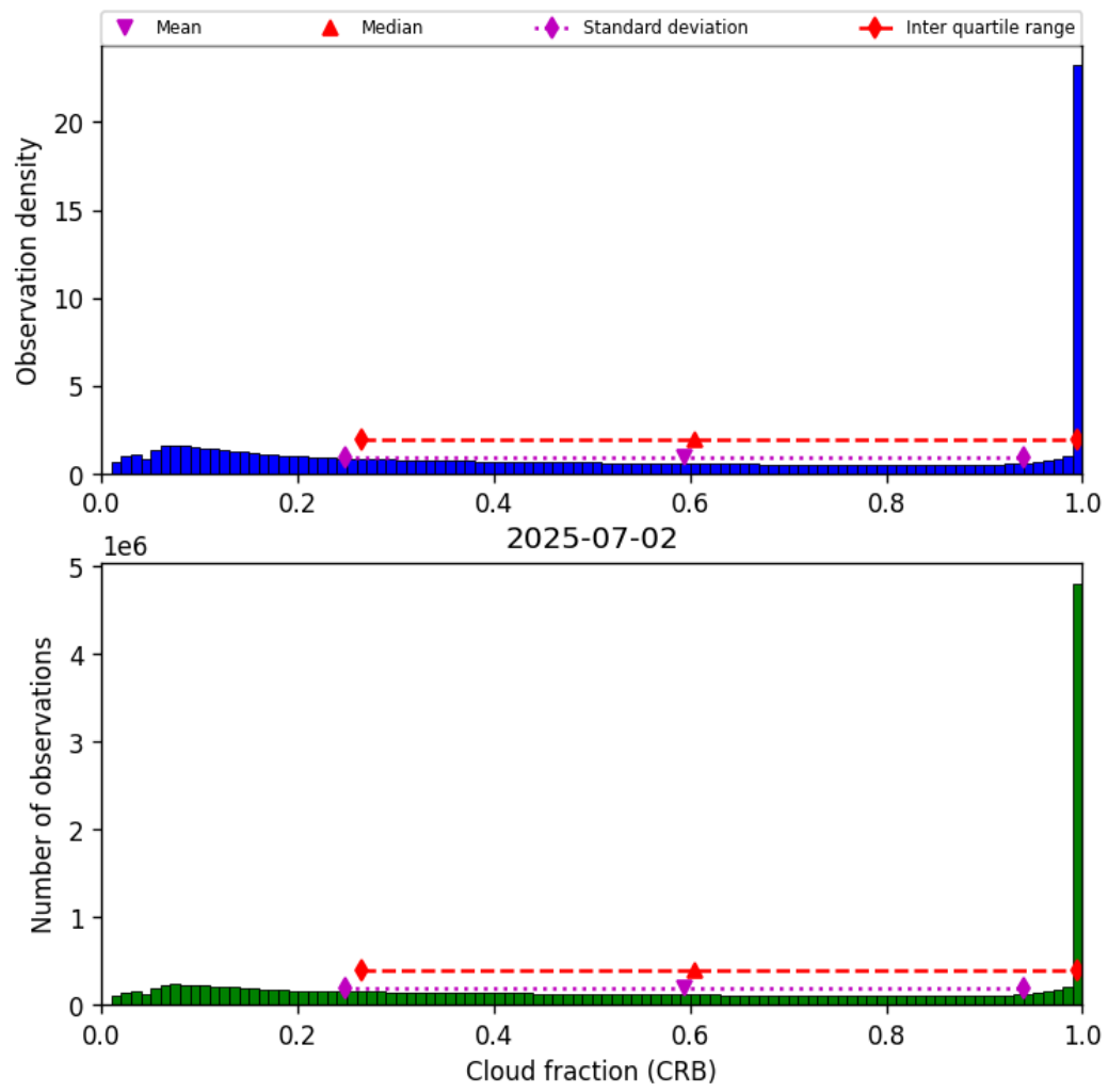
Figure 40: Histogram of “Cloud fraction (CRB)” for 2025-07-02 to 2025-07-03
