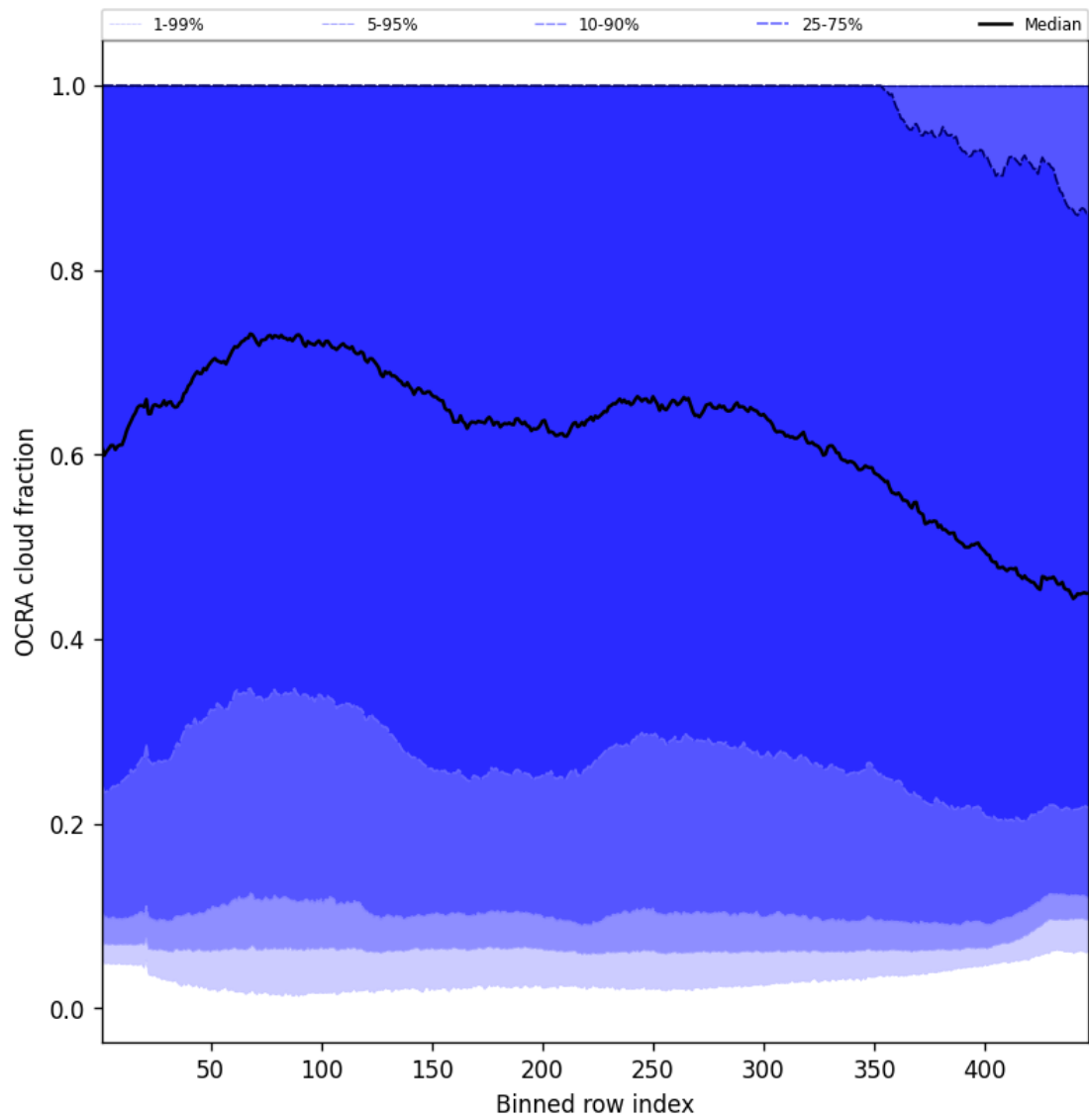
Figure 64: Along track statistics of “OCRA cloud fraction” for 2025-07-02 to 2025-07-03
