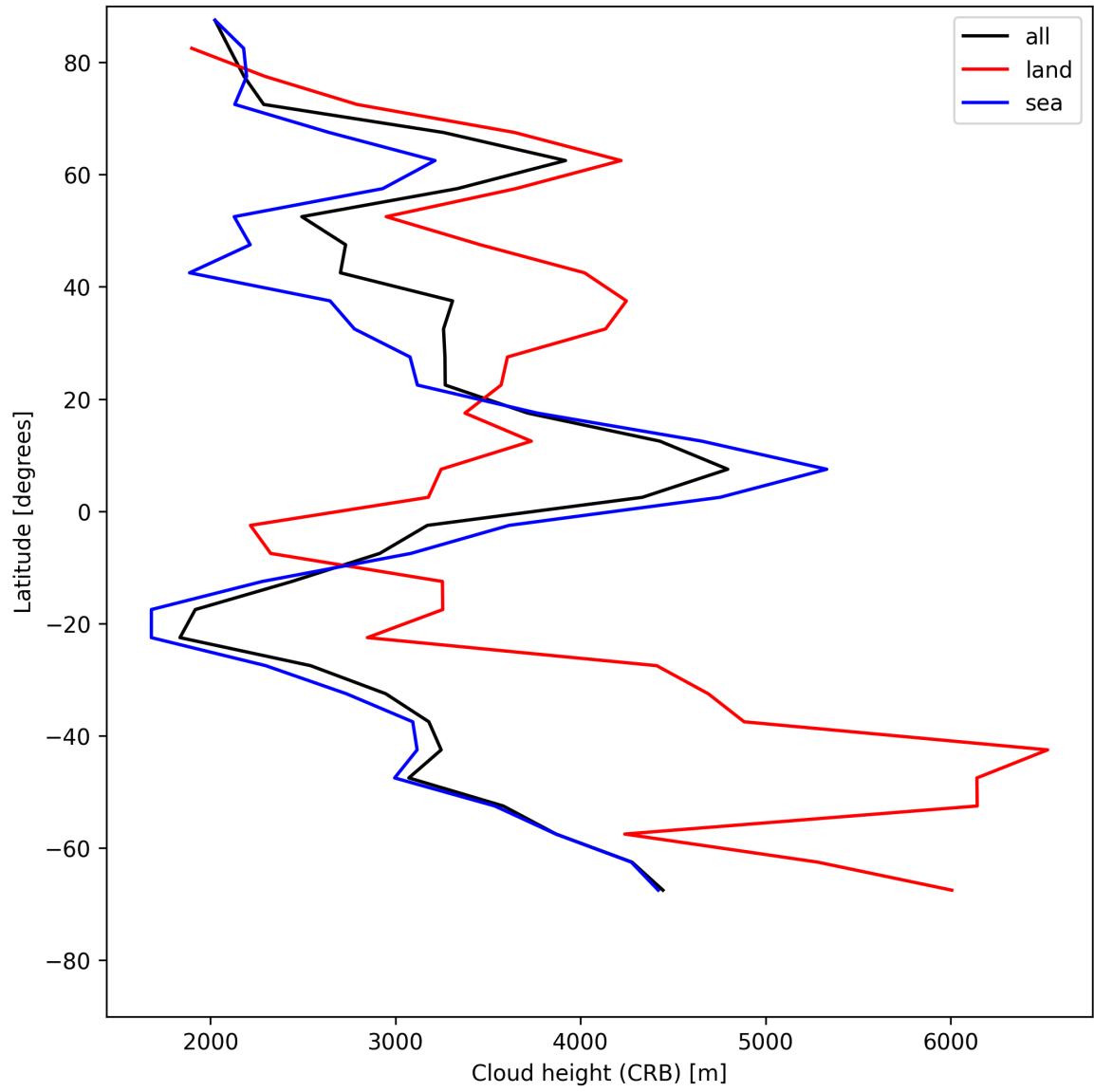
Figure 25: Zonal average of “Cloud height (CRB)” for 2025-07-02 to 2025-07-03.
