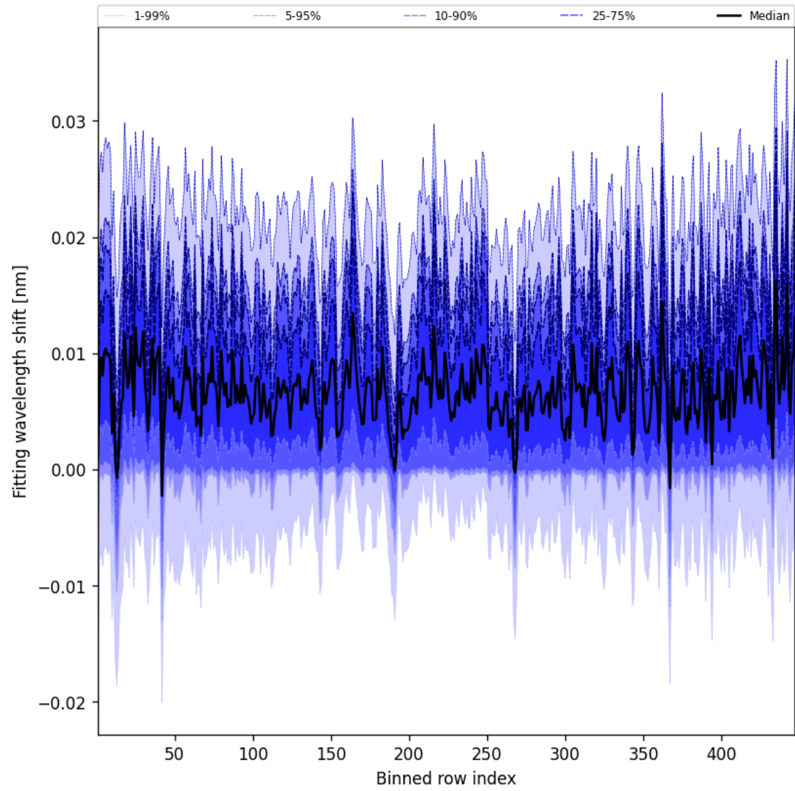
Figure 63: Along track statistics of “Fitting wavelength shift” for 2025-07-02 to 2025-07-03
