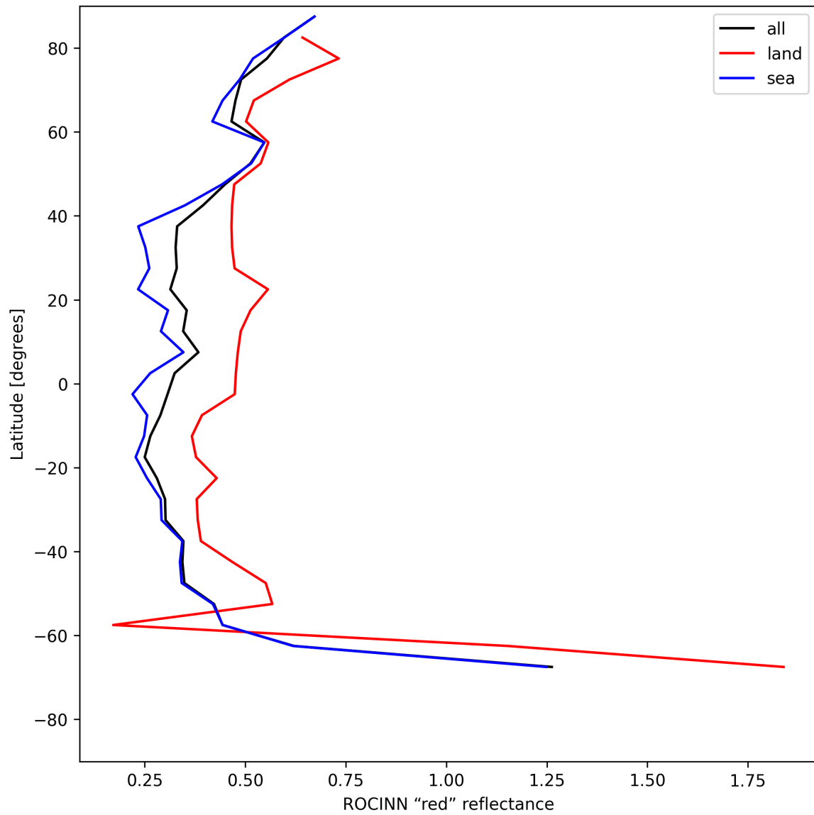
Figure 35: Zonal average of “ROCINN “red” reflectance” for 2025-07-02 to 2025-07-03.
