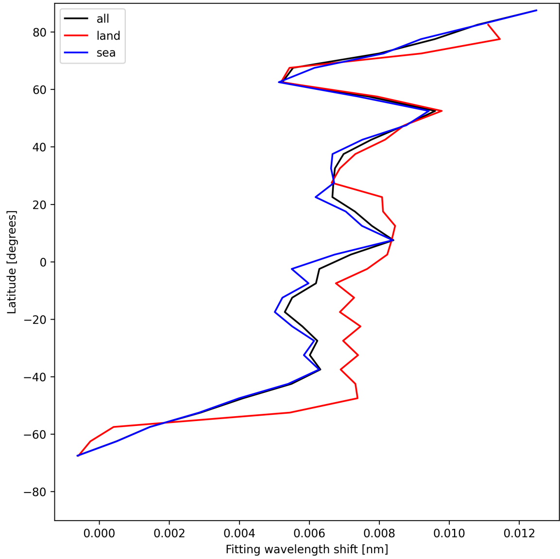
Figure 31: Zonal average of “Fitting wavelength shift” for 2025-07-02 to 2025-07-03.
