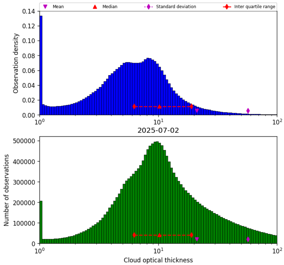
Figure 39: Histogram of “Cloud optical thickness” for 2025-07-02 to 2025-07-03
