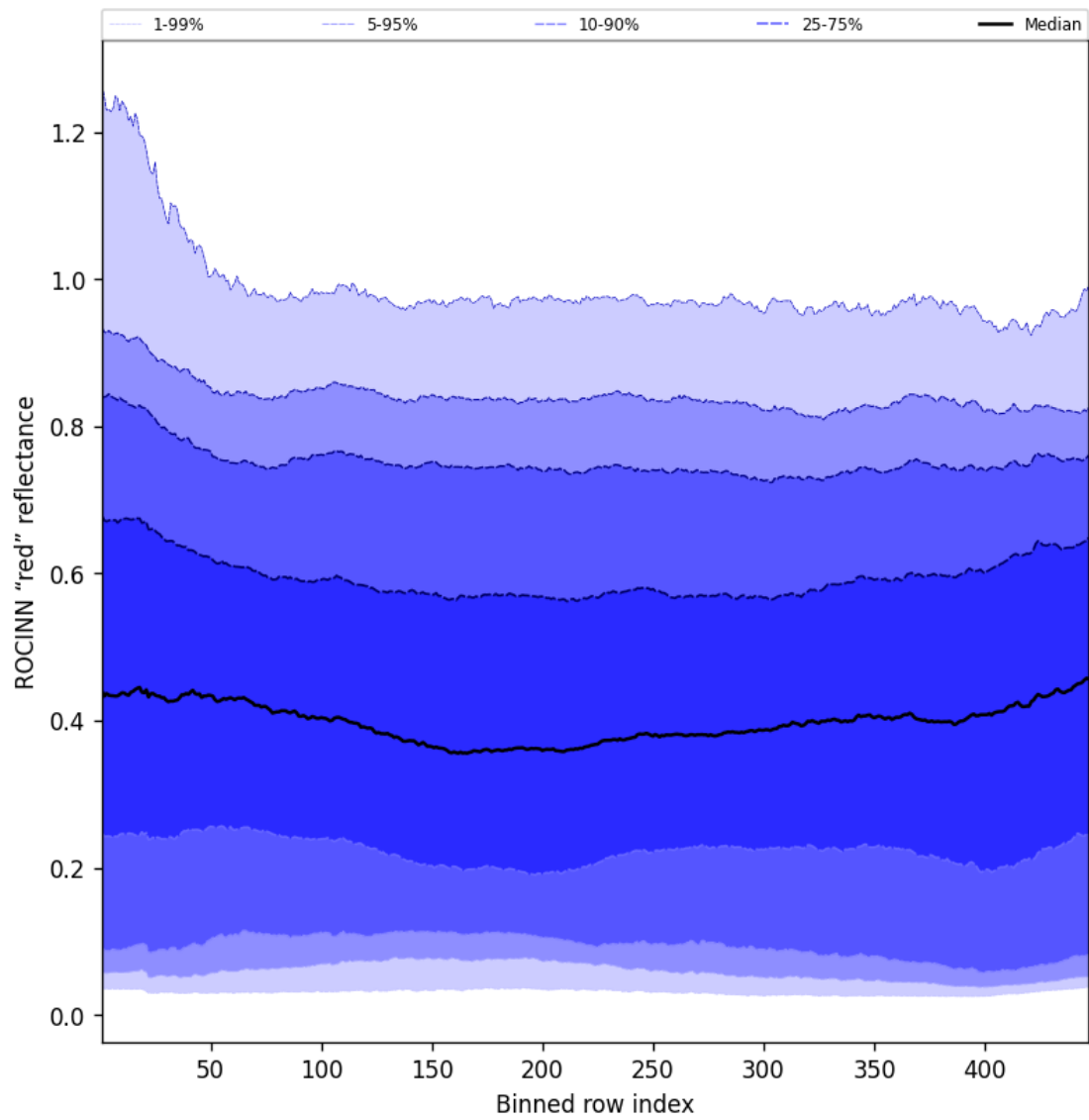
Figure 67: Along track statistics of "ROCINN "red" reflectance" for 2025-07-02 to 2025-07-03
