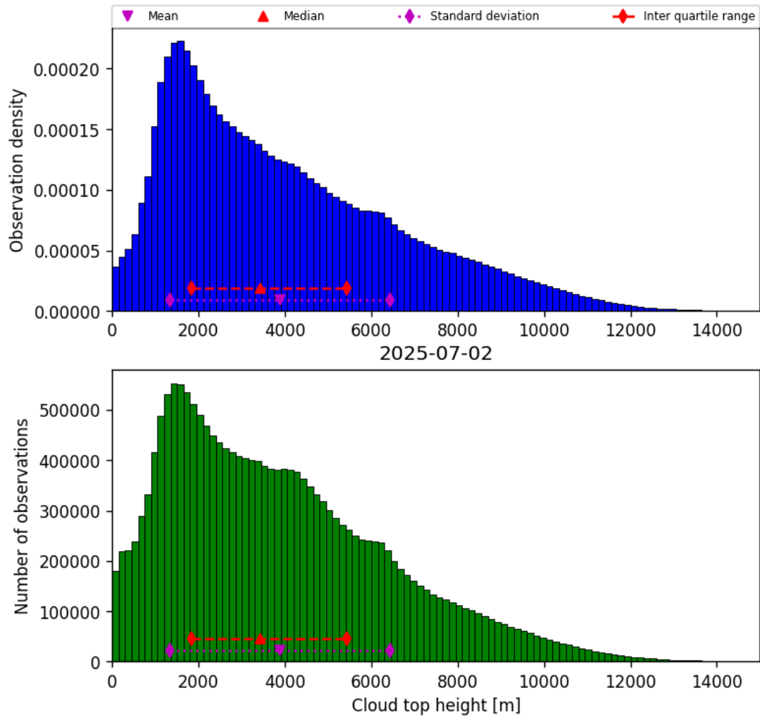
Figure 38: Histogram of “Cloud top height” for 2025-07-02 to 2025-07-03
