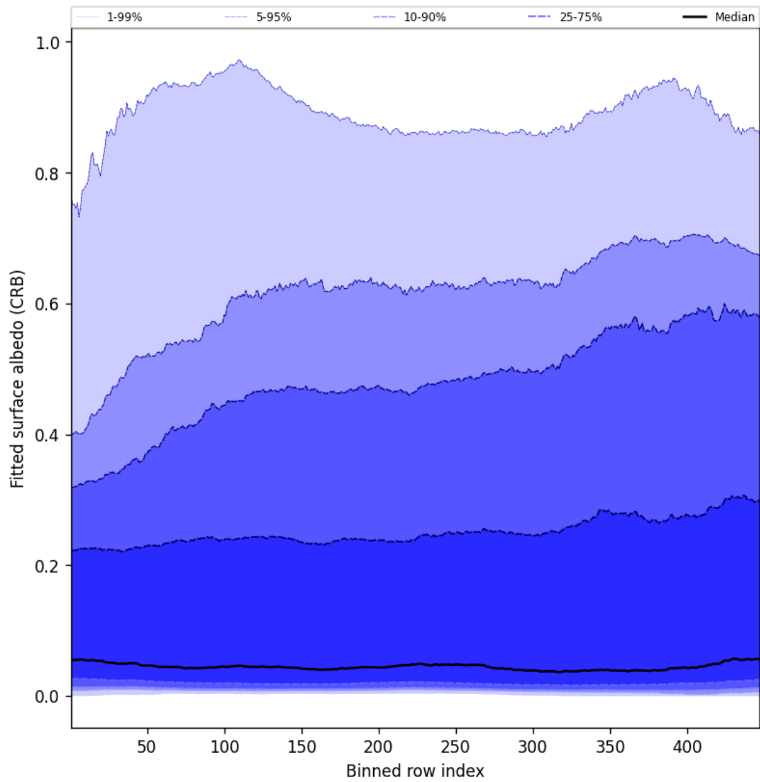
Figure 60: Along track statistics of “Fitted surface albedo (CRB)” for 2025-07-02 to 2025-07-03
