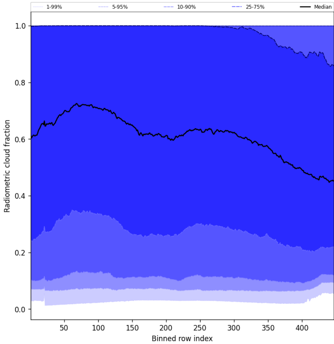
Figure 53: Along track statistics of “Radiometric cloud fraction” for 2025-07-02 to 2025-07-03
