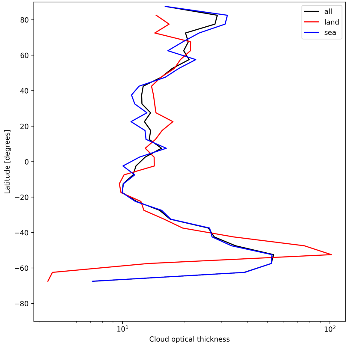
Figure 23: Zonal average of “Cloud optical thickness” for 2025-07-02 to 2025-07-03.
