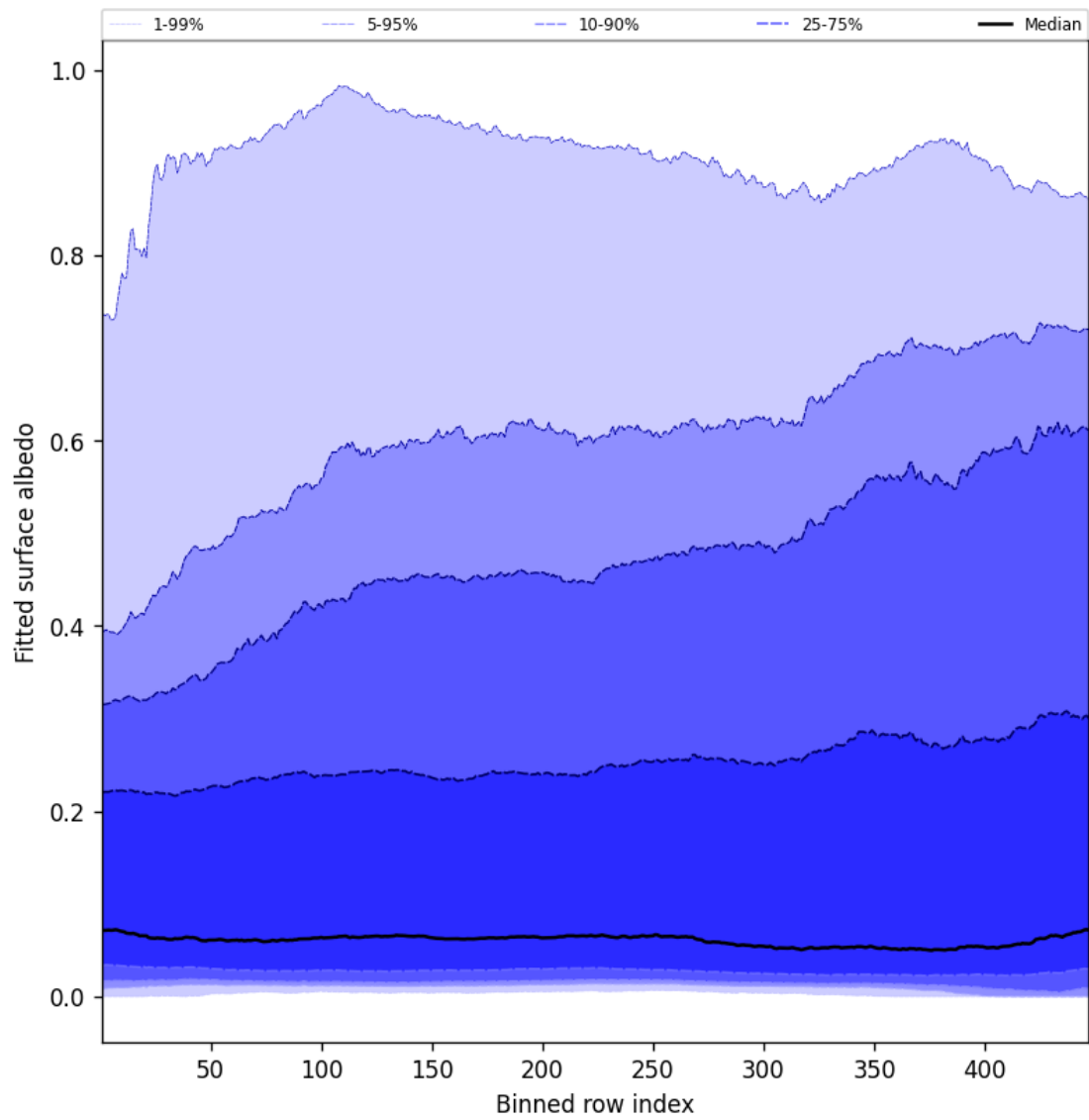
Figure 59: Along track statistics of “Fitted surface albedo” for 2025-07-02 to 2025-07-03
