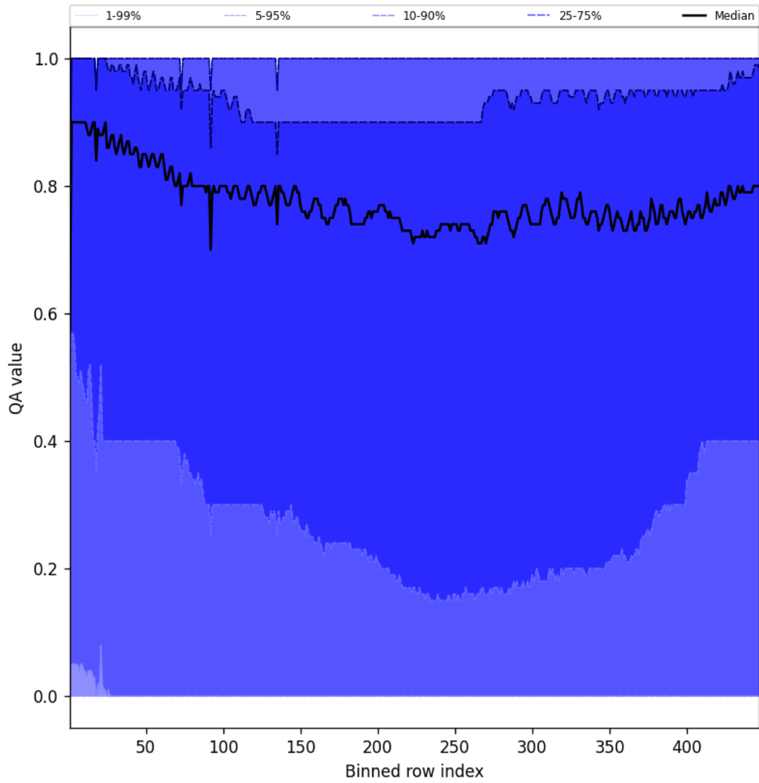
Figure 52: Along track statistics of “QA value” for 2025-07-02 to 2025-07-03
