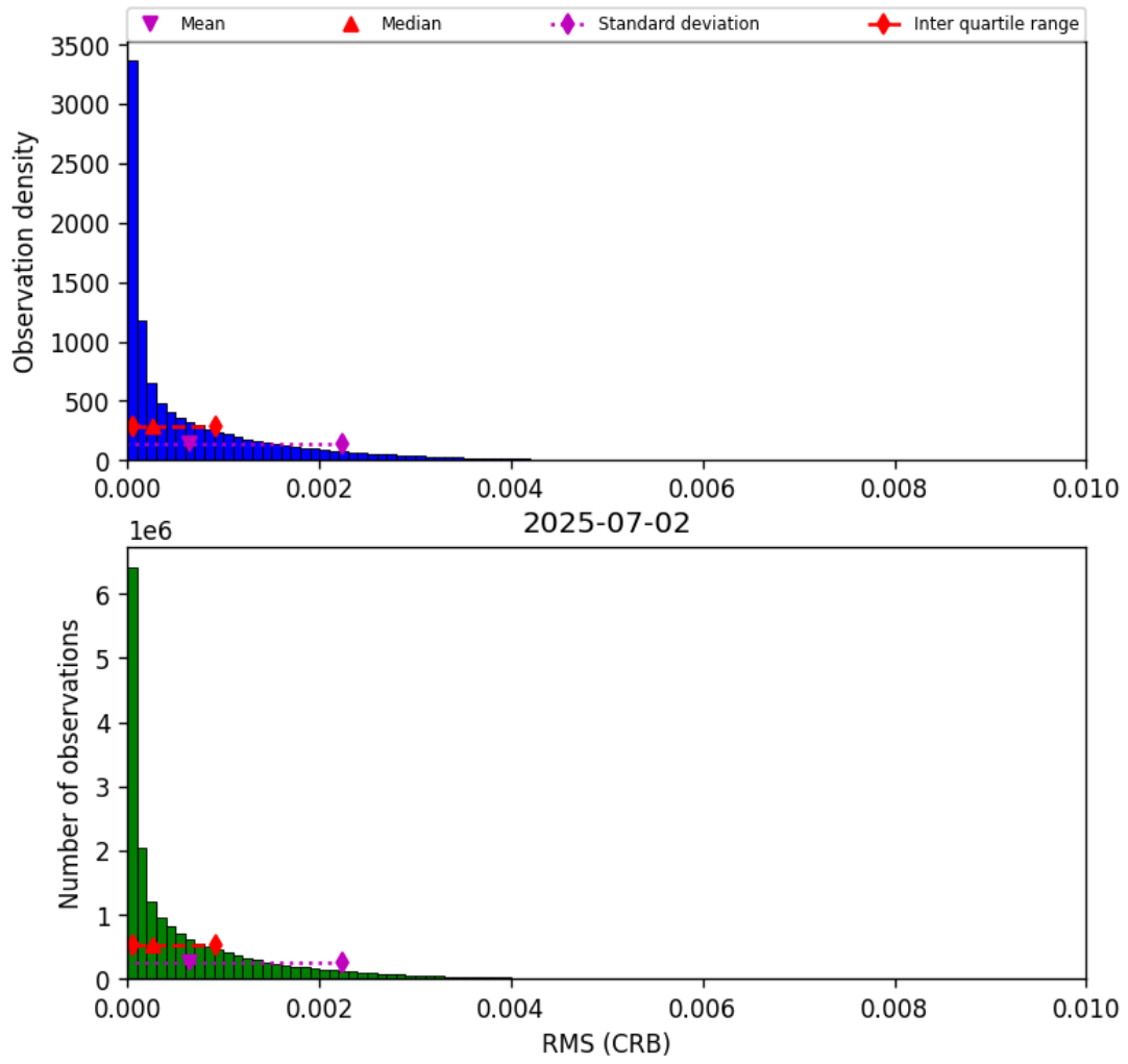
Figure 46: Histogram of “RMS (CRB)” for 2025-07-02 to 2025-07-03
