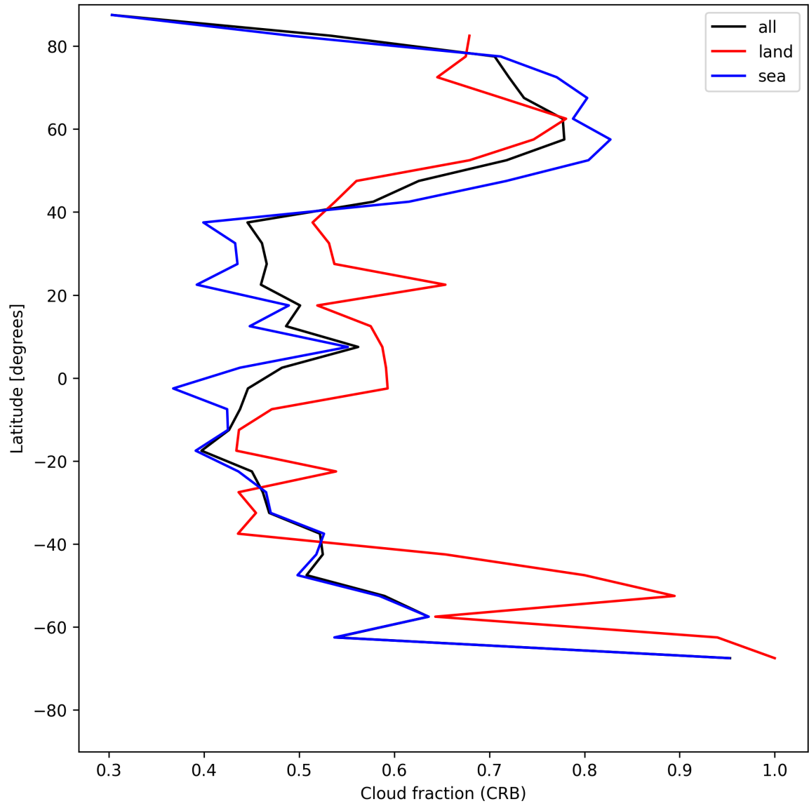
Figure 24: Zonal average of “Cloud fraction (CRB)” for 2025-07-02 to 2025-07-03.
