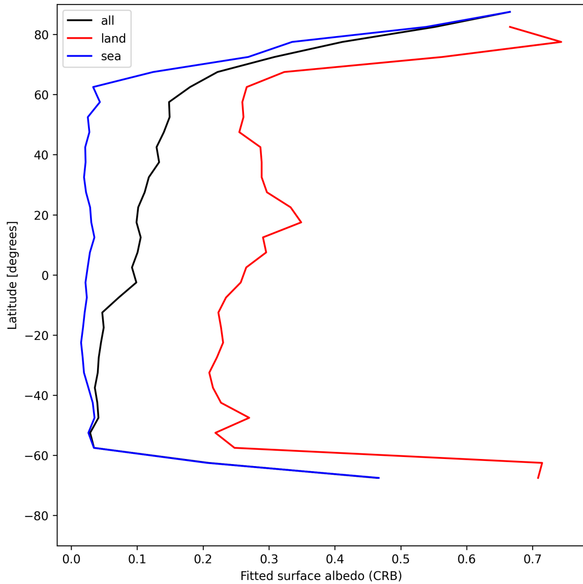
Figure 28: Zonal average of "Fitted surface albedo (CRB)" for 2025-07-02 to 2025-07-03.
