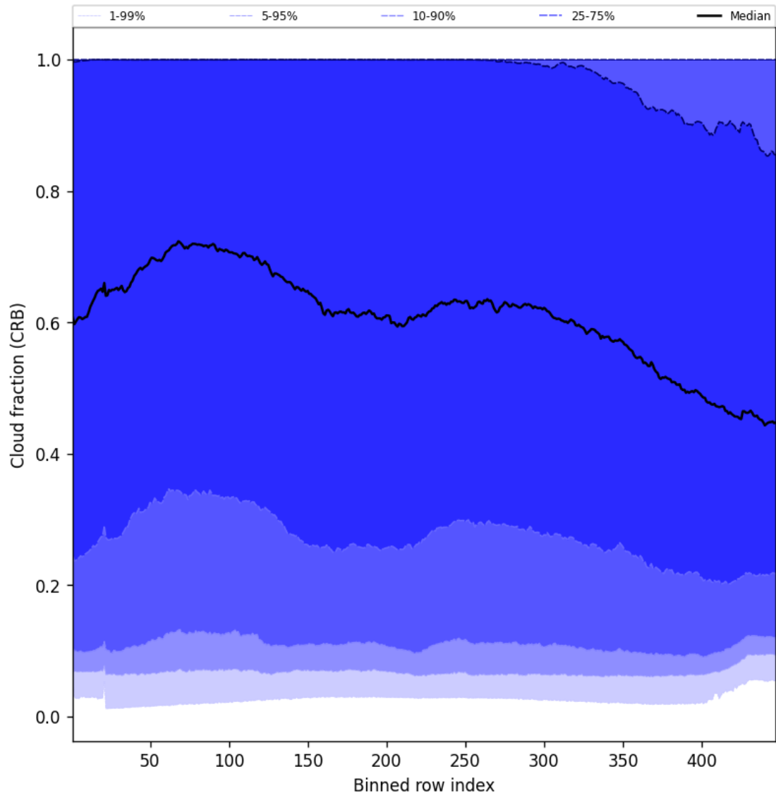
Figure 56: Along track statistics of “Cloud fraction (CRB)” for 2025-07-02 to 2025-07-03
