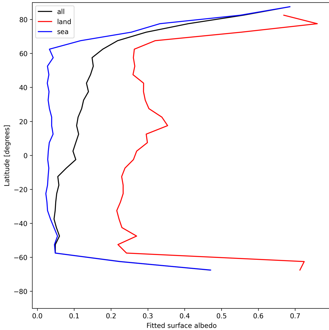
Figure 27: Zonal average of “Fitted surface albedo” for 2025-07-02 to 2025-07-03.
