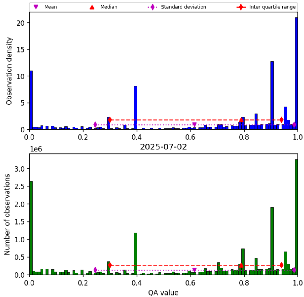
Figure 36: Histogram of “QA value” for 2025-07-02 to 2025-07-03
