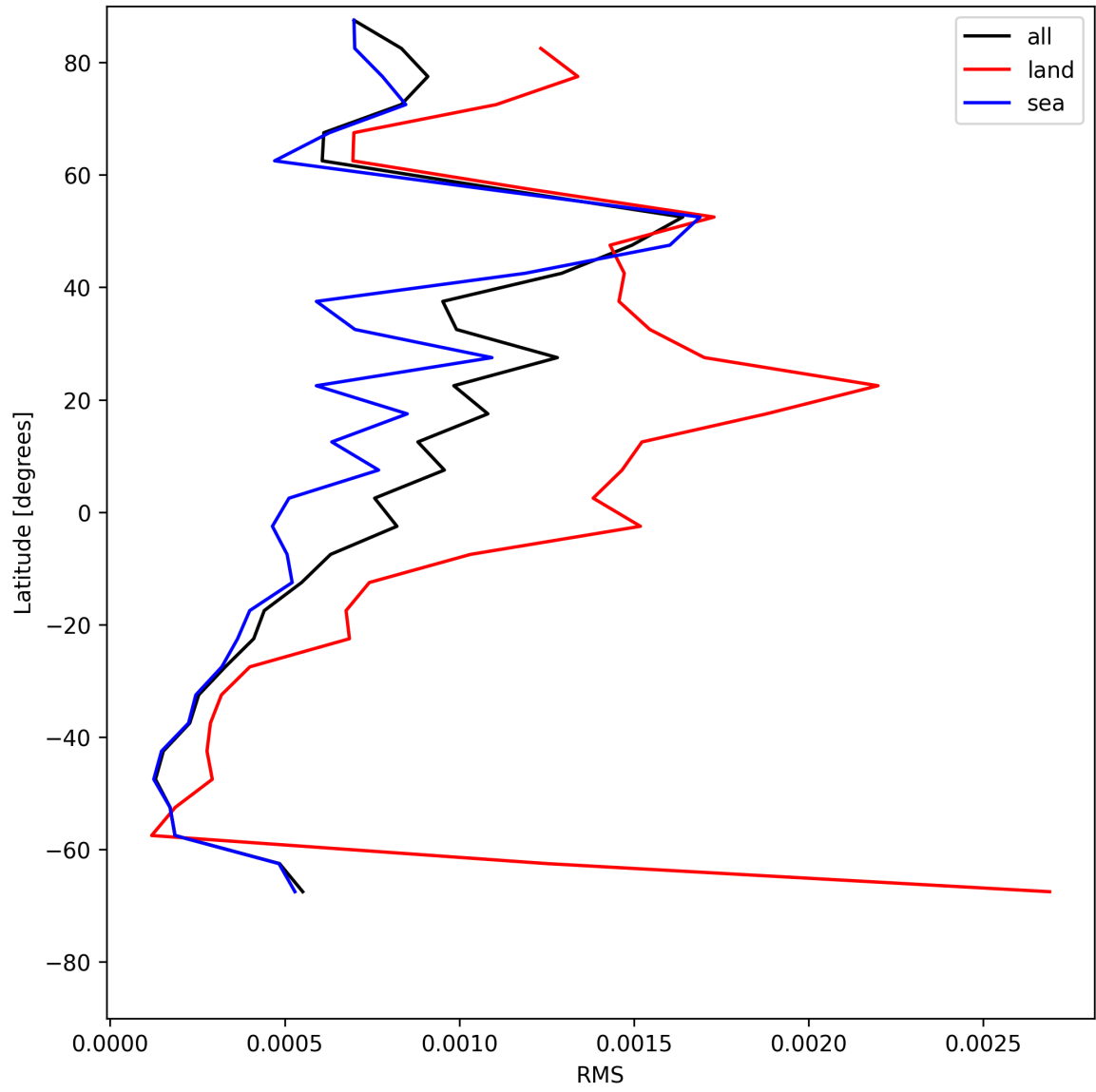
Figure 29: Zonal average of “RMS” for 2025-07-02 to 2025-07-03.
