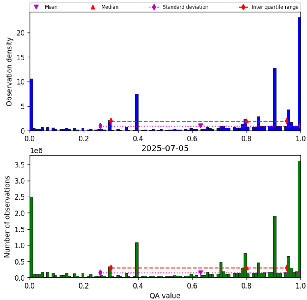
Figure 36: Histogram of “QA value” for 2025-07-05 to 2025-07-06
