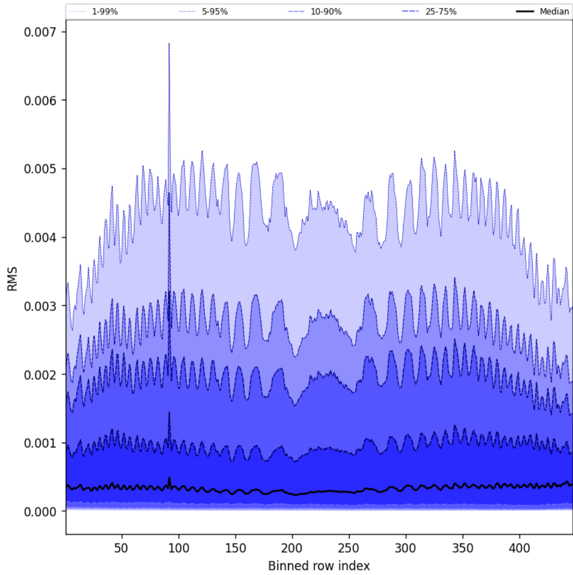
Figure 61: Along track statistics of “RMS” for 2025-07-05 to 2025-07-06
