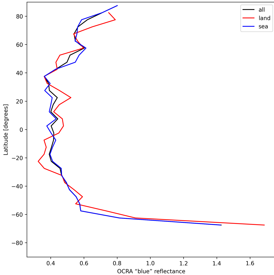
Figure 33: Zonal average of “OCRA “blue” reflectance” for 2025-07-05 to 2025-07-06.
