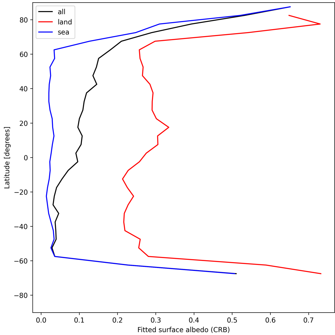
Figure 28: Zonal average of “Fitted surface albedo (CRB)” for 2025-07-05 to 2025-07-06.
