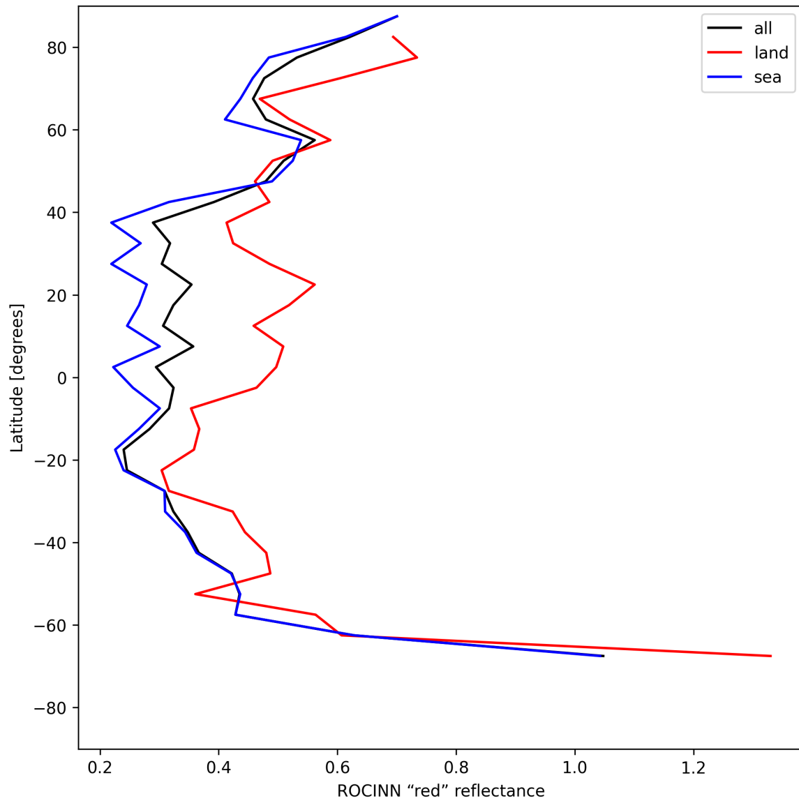
Figure 35: Zonal average of “ROCINN “red” reflectance” for 2025-07-05 to 2025-07-06.
