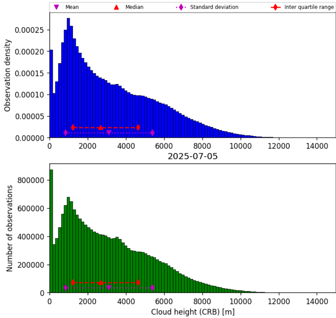
Figure 41: Histogram of “Cloud height (CRB)” for 2025-07-05 to 2025-07-06
