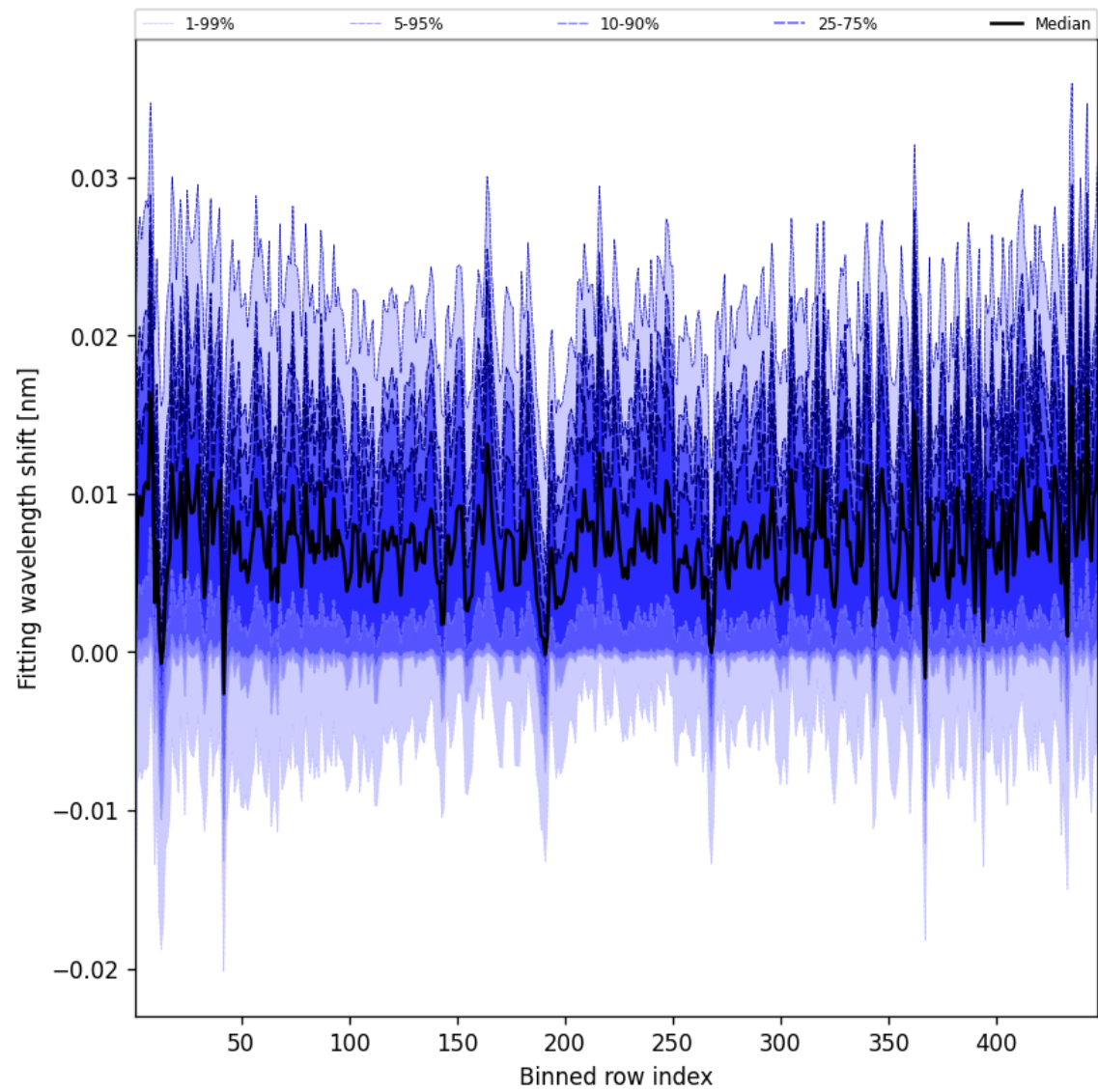
Figure 63: Along track statistics of “Fitting wavelength shift” for 2025-07-05 to 2025-07-06
