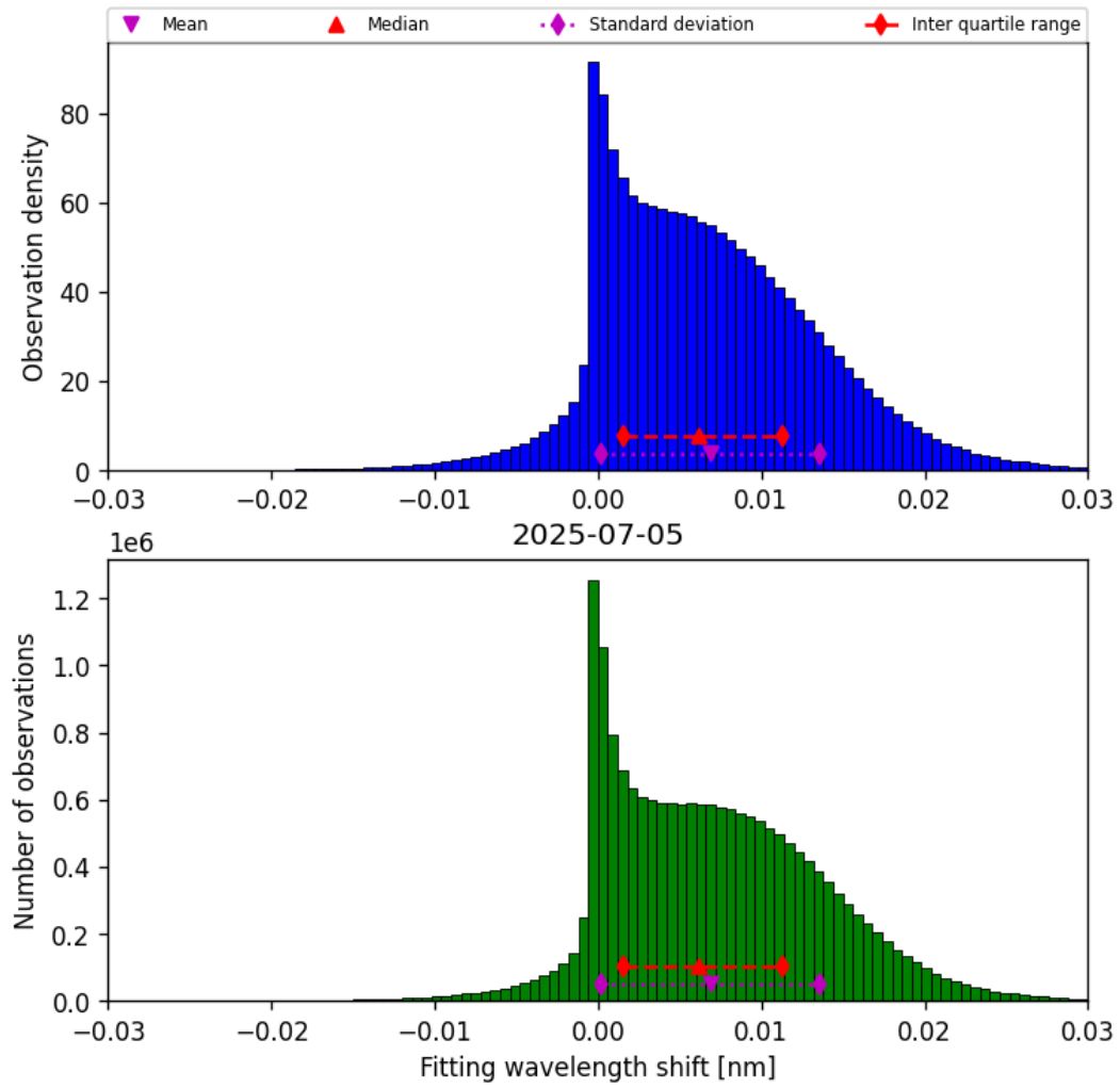
Figure 47: Histogram of “Fitting wavelength shift” for 2025-07-05 to 2025-07-06
