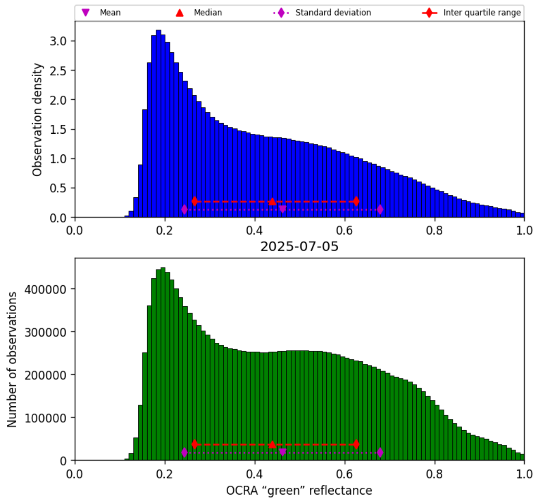
Figure 50: Histogram of “OCRA “green” reflectance” for 2025-07-05 to 2025-07-06
