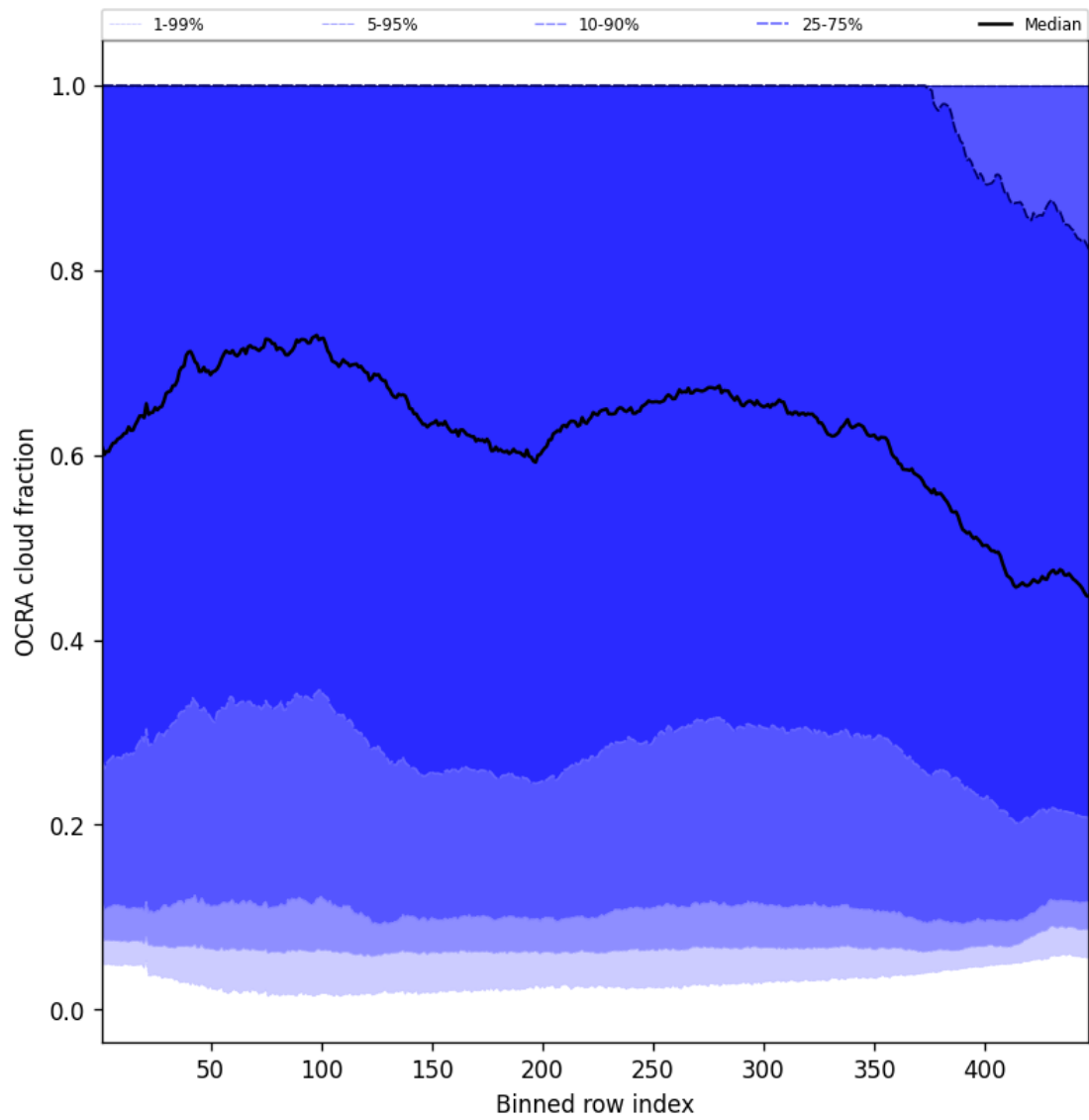
Figure 64: Along track statistics of “OCRA cloud fraction” for 2025-07-05 to 2025-07-06
