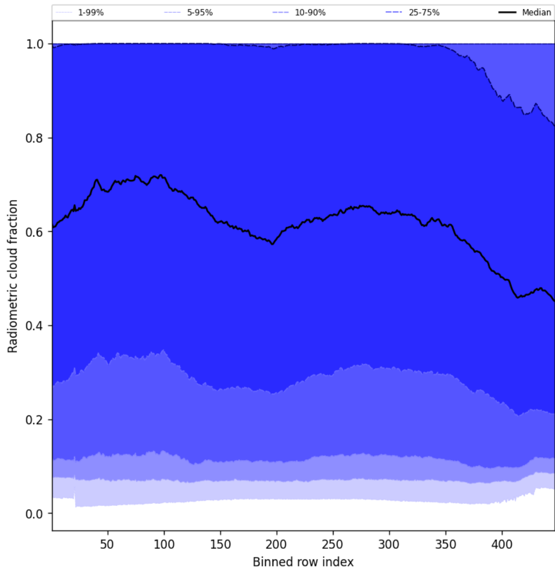
Figure 53: Along track statistics of “Radiometric cloud fraction” for 2025-07-05 to 2025-07-06
