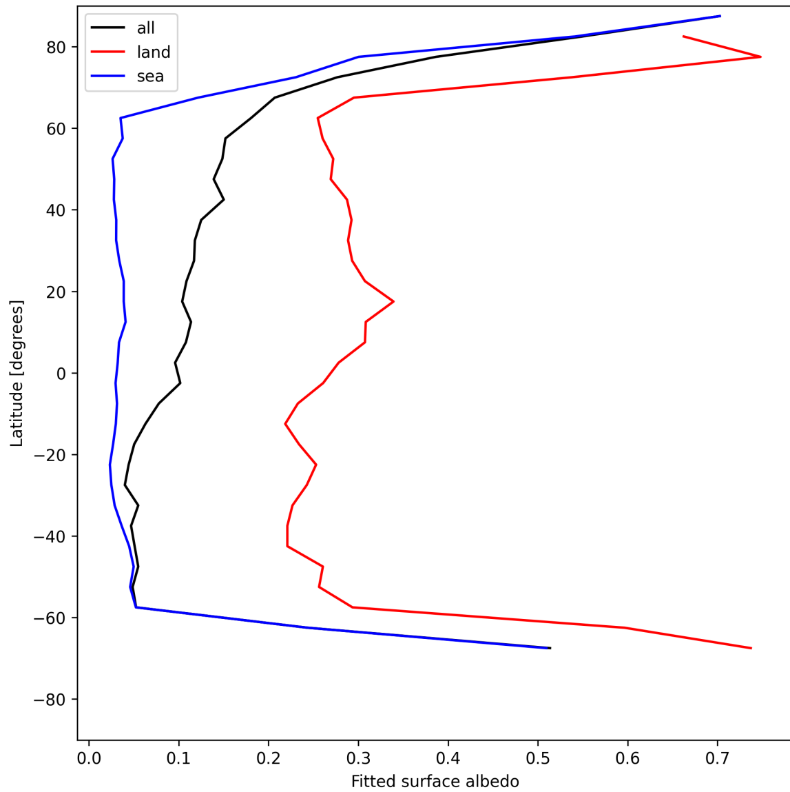
Figure 27: Zonal average of “Fitted surface albedo” for 2025-07-05 to 2025-07-06.
