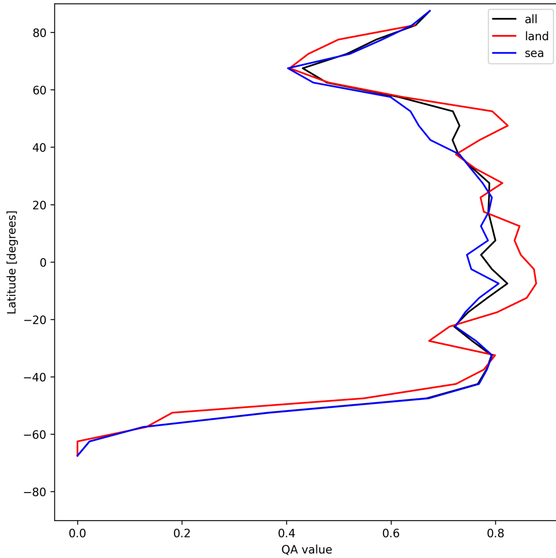
Figure 20: Zonal average of “QA value” for 2025-07-05 to 2025-07-06.
