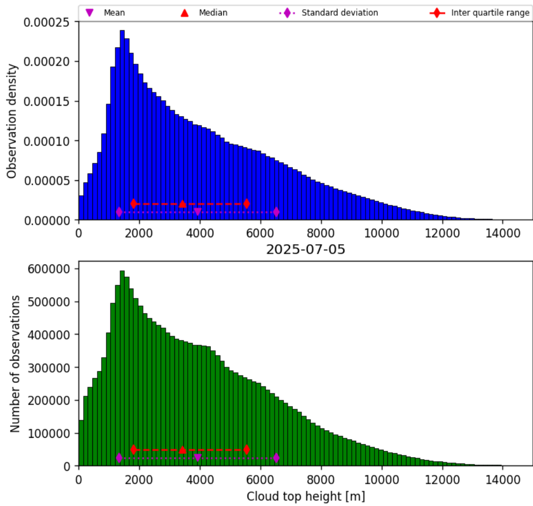
Figure 38: Histogram of “Cloud top height” for 2025-07-05 to 2025-07-06
