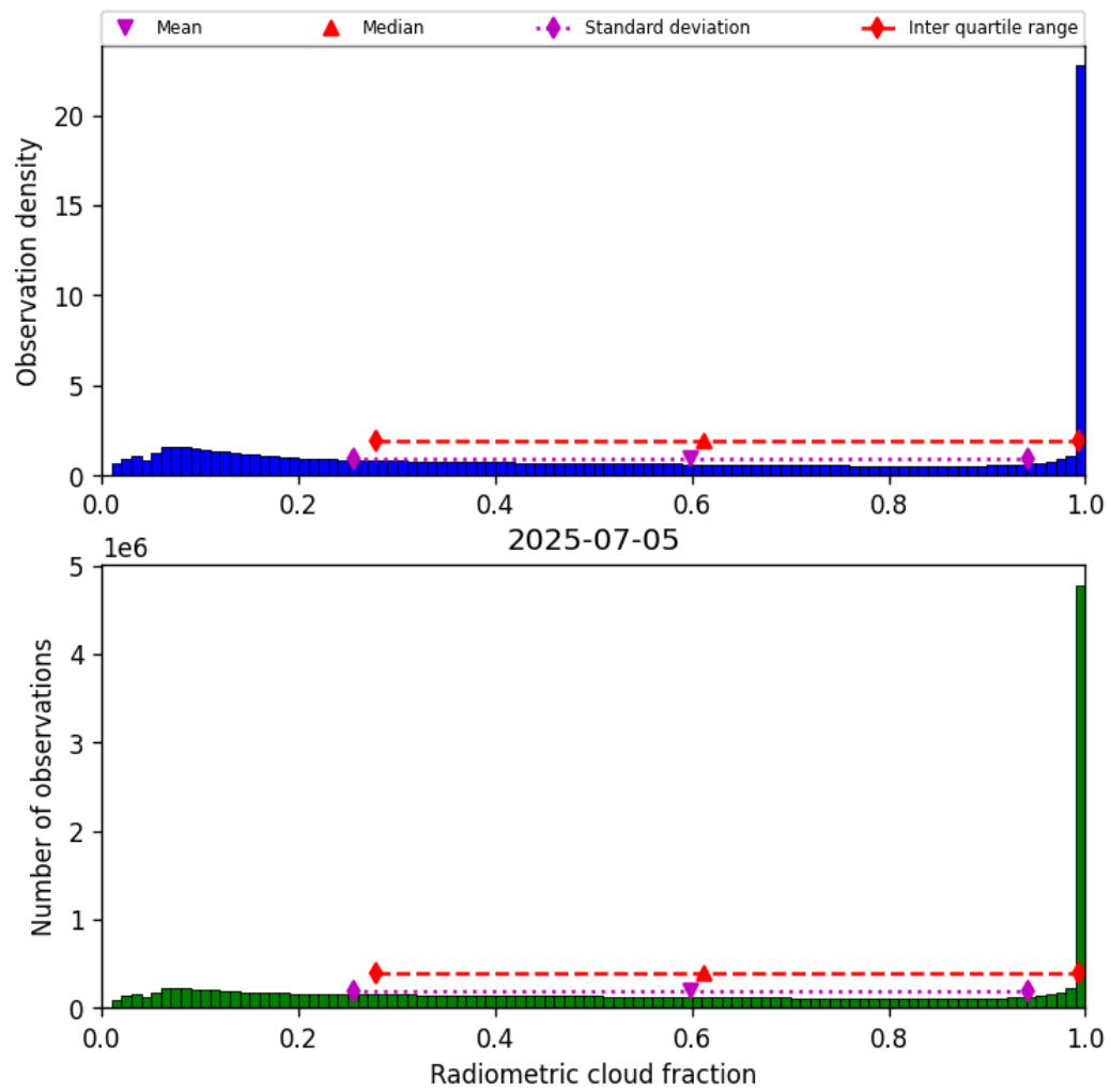
Figure 37: Histogram of “Radiometric cloud fraction” for 2025-07-05 to 2025-07-06
