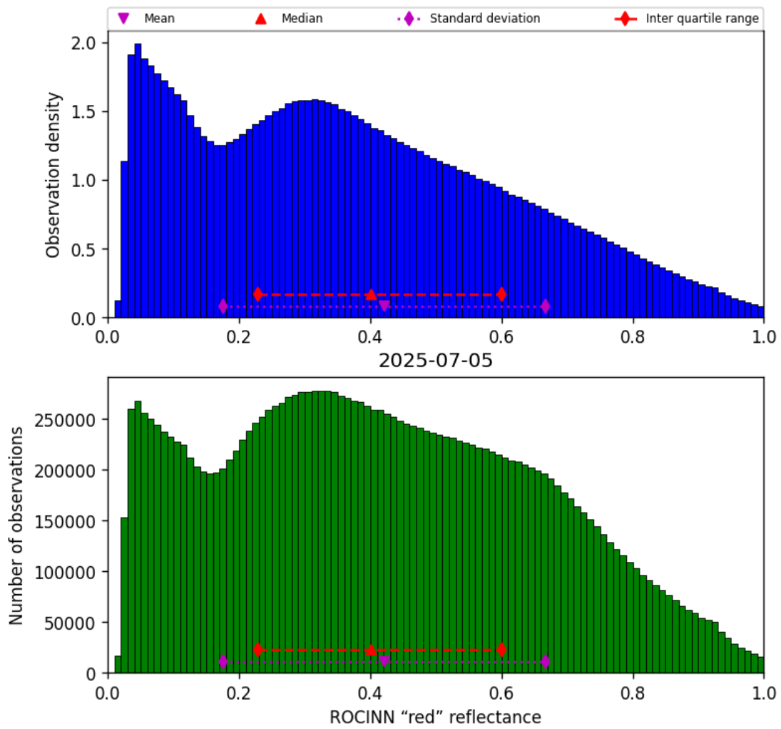
Figure 51: Histogram of “ROCINN “red” reflectance” for 2025-07-05 to 2025-07-06
