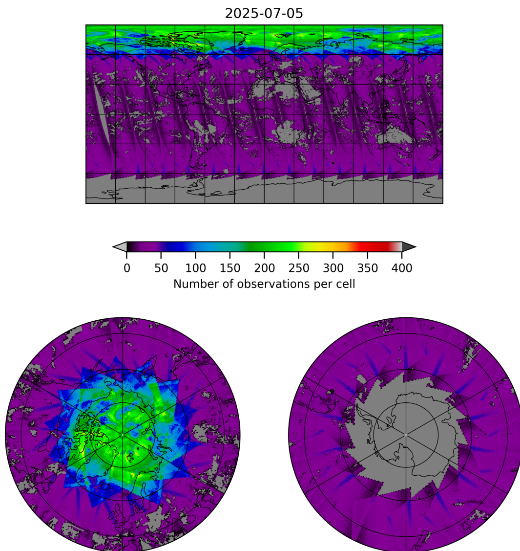
Figure 19: Map of the number of observations for 2025-07-05 to 2025-07-06
