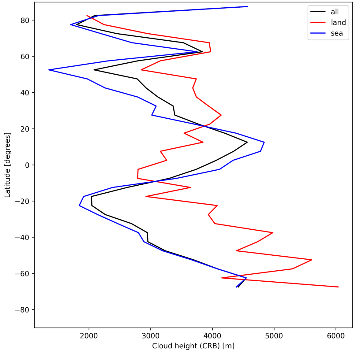
Figure 25: Zonal average of “Cloud height (CRB)” for 2025-07-05 to 2025-07-06.
