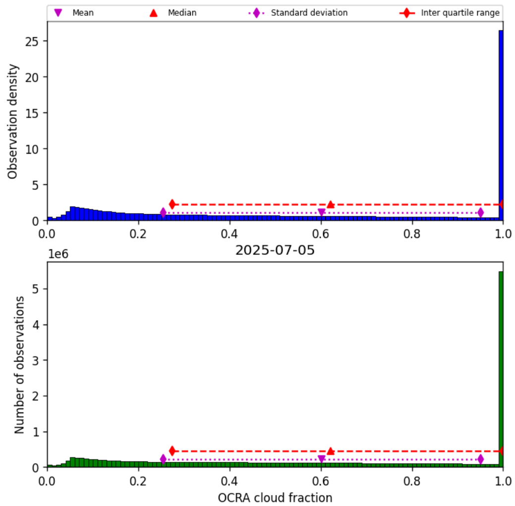
Figure 48: Histogram of “OCRA cloud fraction” for 2025-07-05 to 2025-07-06
