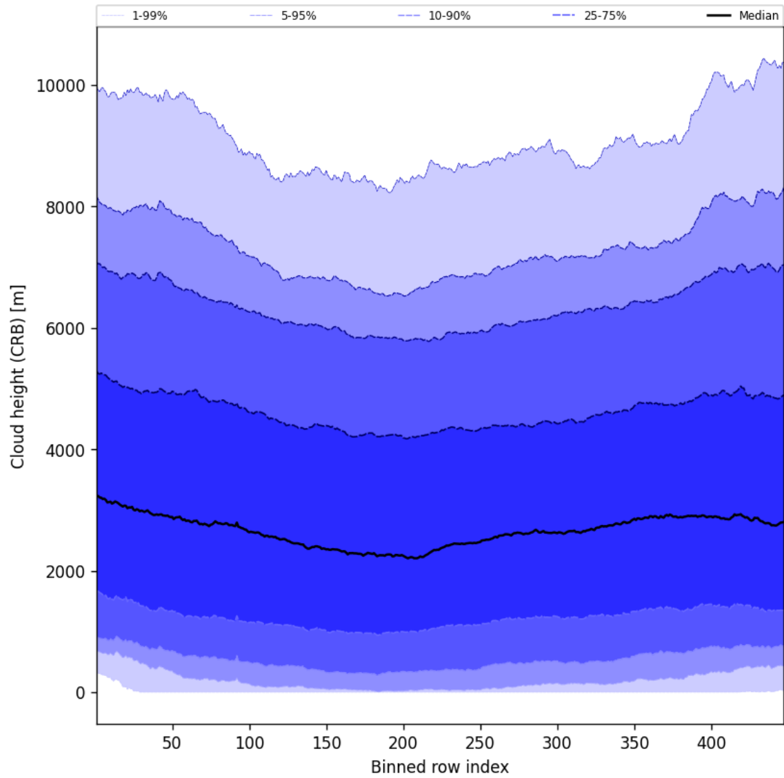
Figure 57: Along track statistics of “Cloud height (CRB)” for 2025-07-05 to 2025-07-06
