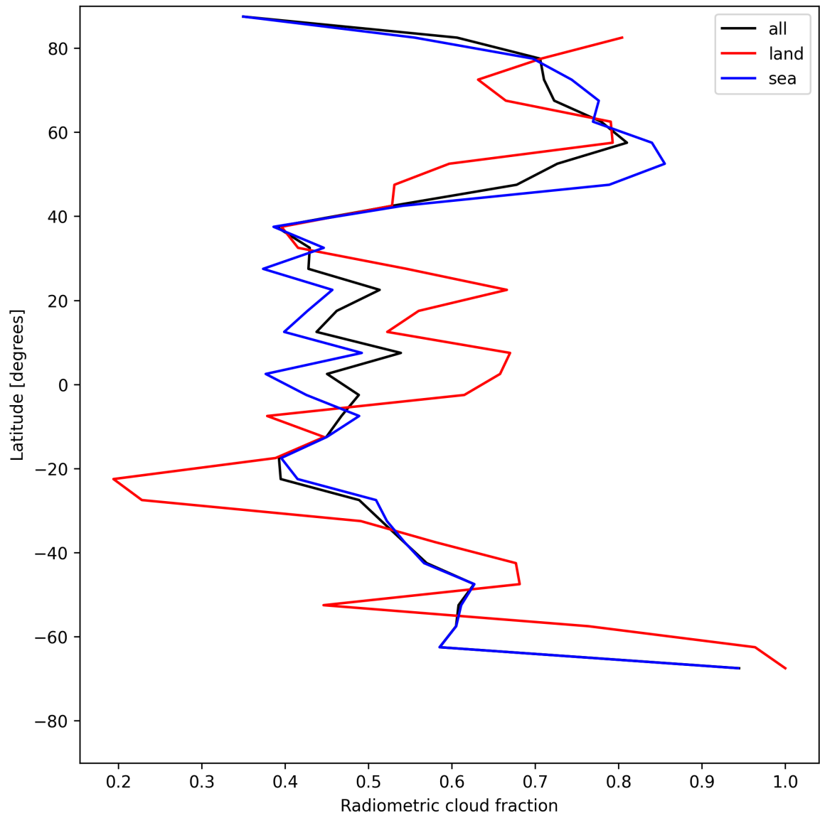
Figure 21: Zonal average of “Radiometric cloud fraction” for 2025-07-05 to 2025-07-06.
