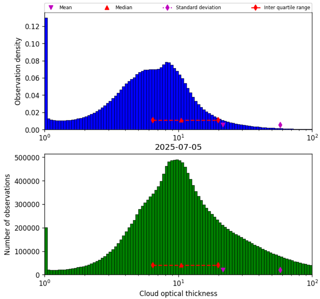
Figure 39: Histogram of “Cloud optical thickness” for 2025-07-05 to 2025-07-06
