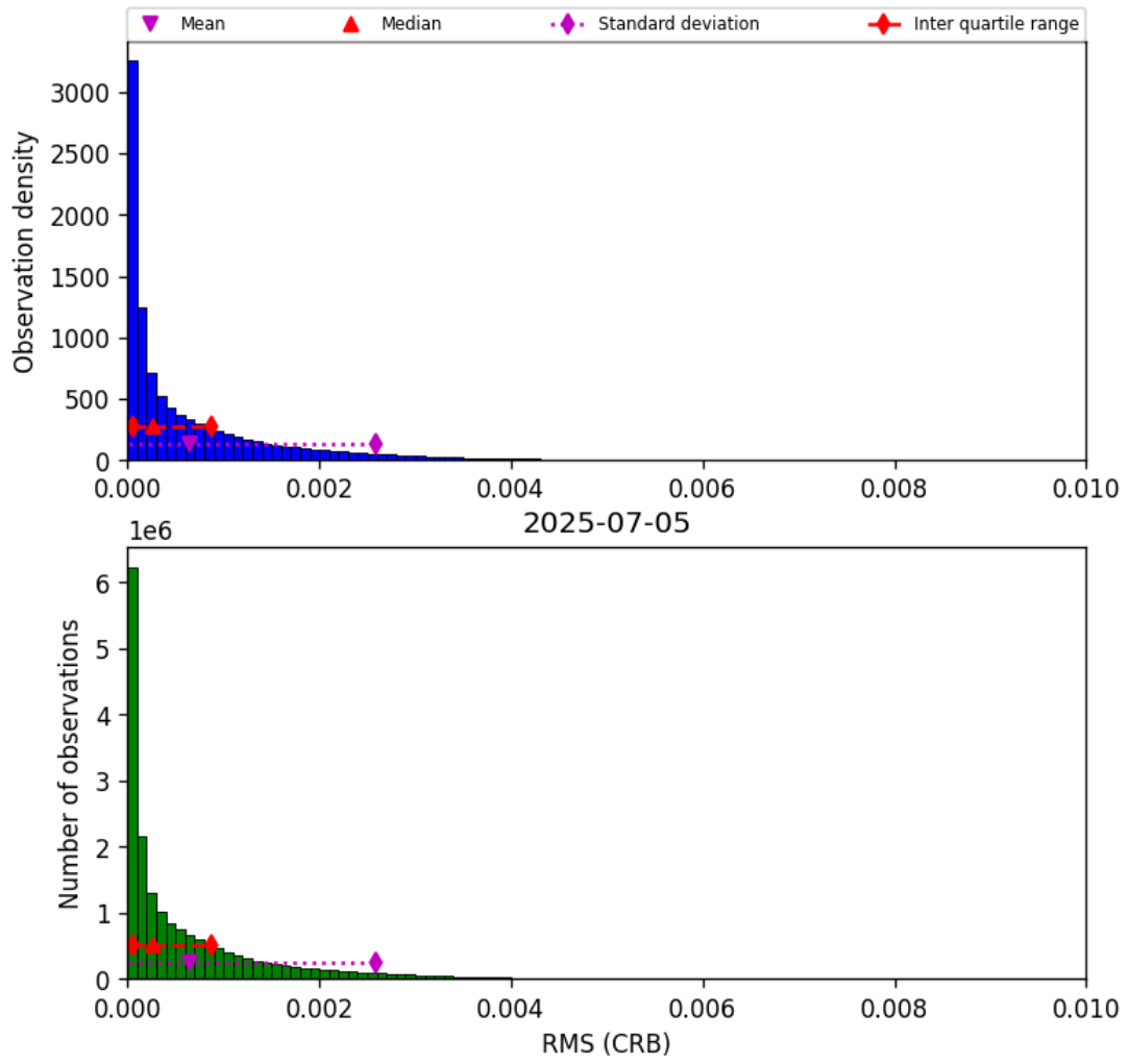
Figure 46: Histogram of “RMS (CRB)” for 2025-07-05 to 2025-07-06
