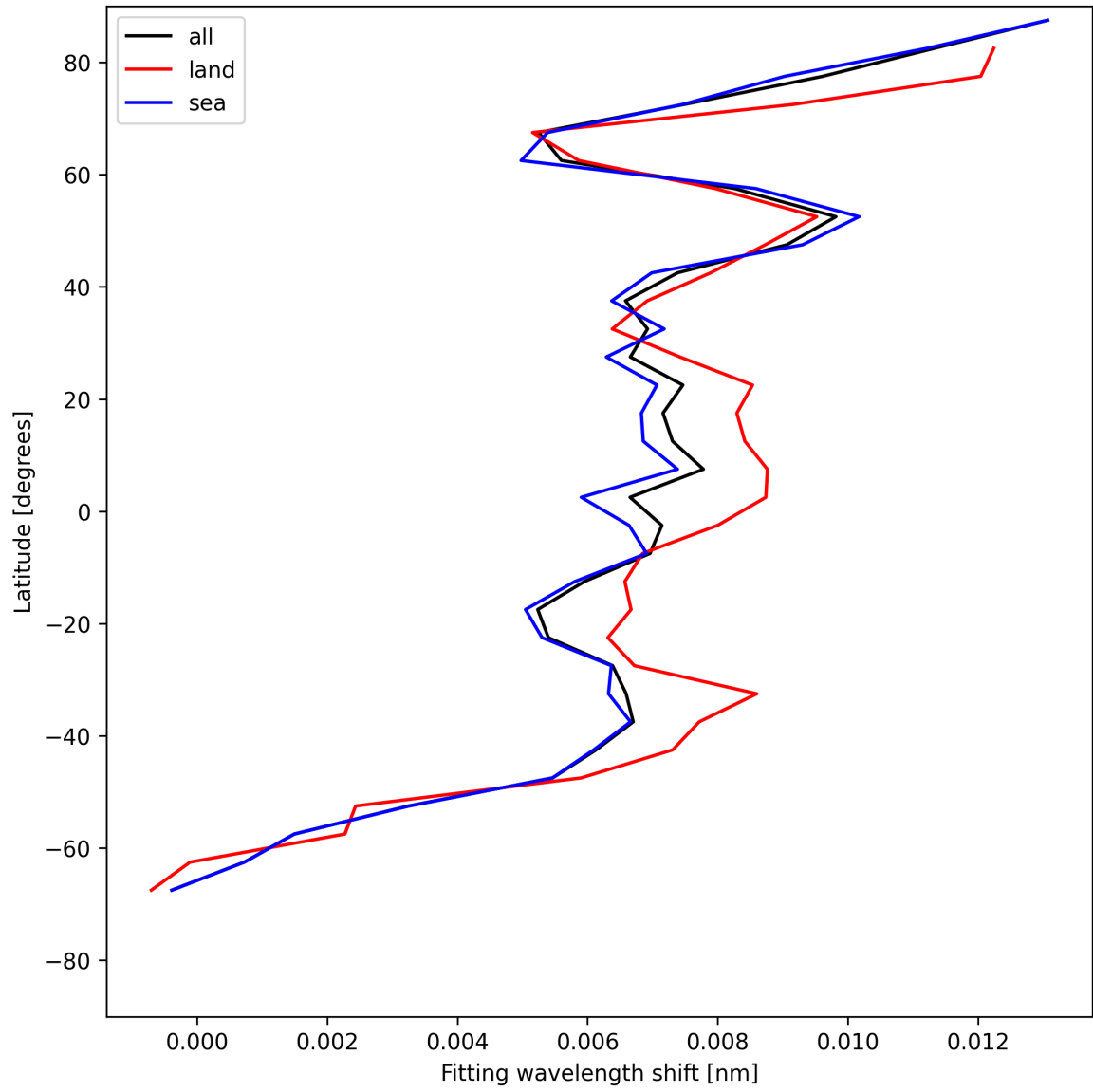
Figure 31: Zonal average of “Fitting wavelength shift” for 2025-07-05 to 2025-07-06.
