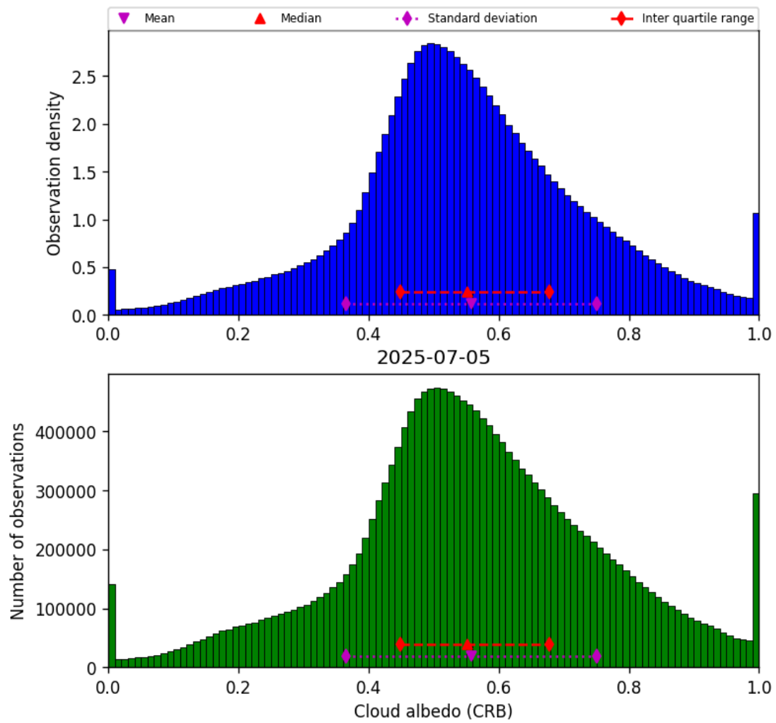
Figure 42: Histogram of “Cloud albedo (CRB)” for 2025-07-05 to 2025-07-06
