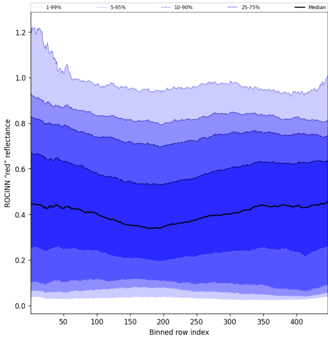
Figure 67: Along track statistics of "ROCINN "red" reflectance" for 2025-07-05 to 2025-07-06
