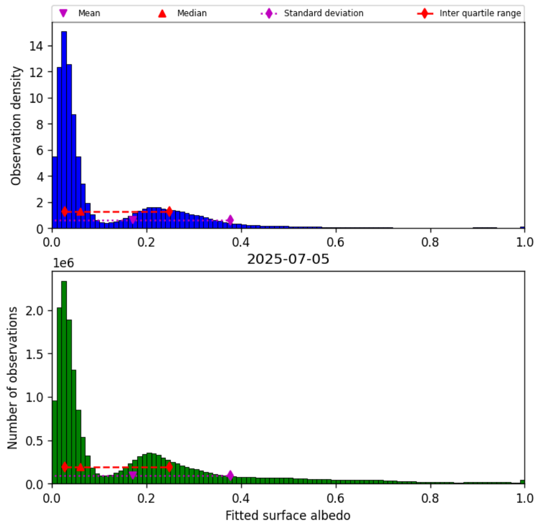
Figure 43: Histogram of “Fitted surface albedo” for 2025-07-05 to 2025-07-06
