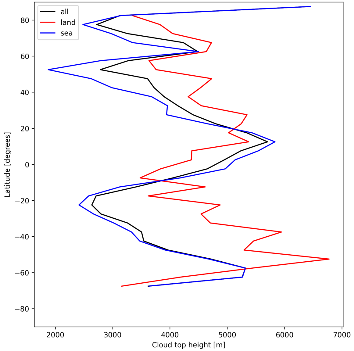
Figure 22: Zonal average of “Cloud top height” for 2025-07-05 to 2025-07-06.
