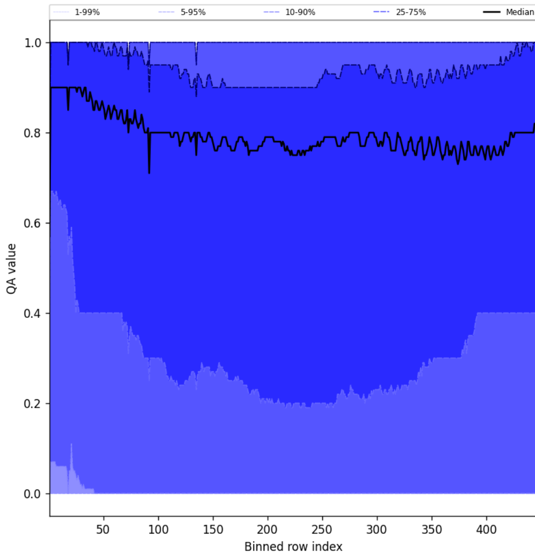
Figure 52: Along track statistics of “QA value” for 2025-07-05 to 2025-07-06
