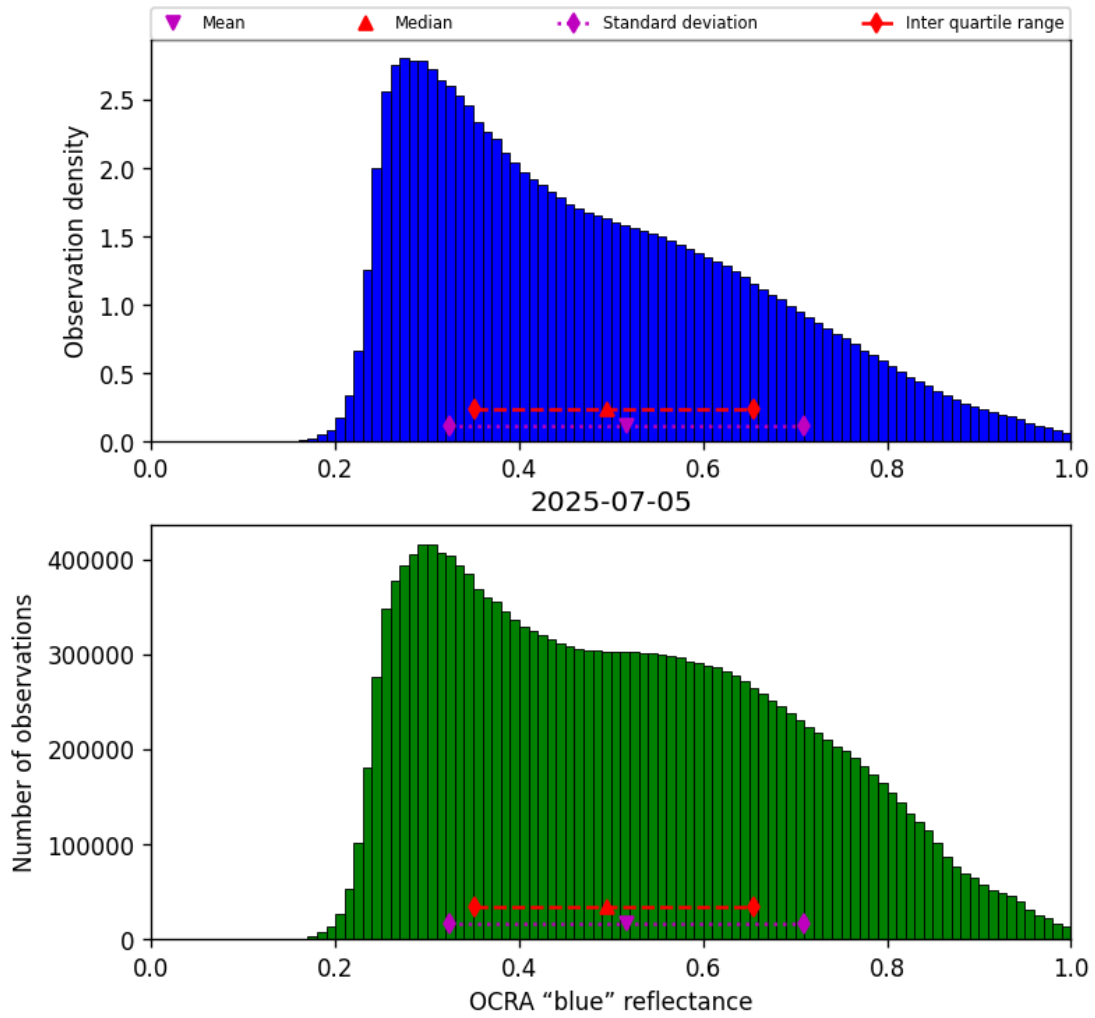
Figure 49: Histogram of “OCRA “blue” reflectance” for 2025-07-05 to 2025-07-06
