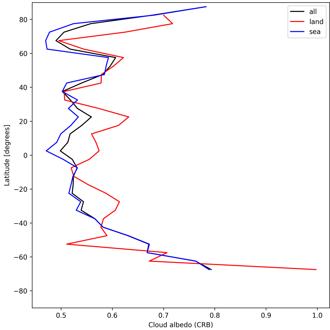
Figure 26: Zonal average of “Cloud albedo (CRB)” for 2025-07-05 to 2025-07-06.
