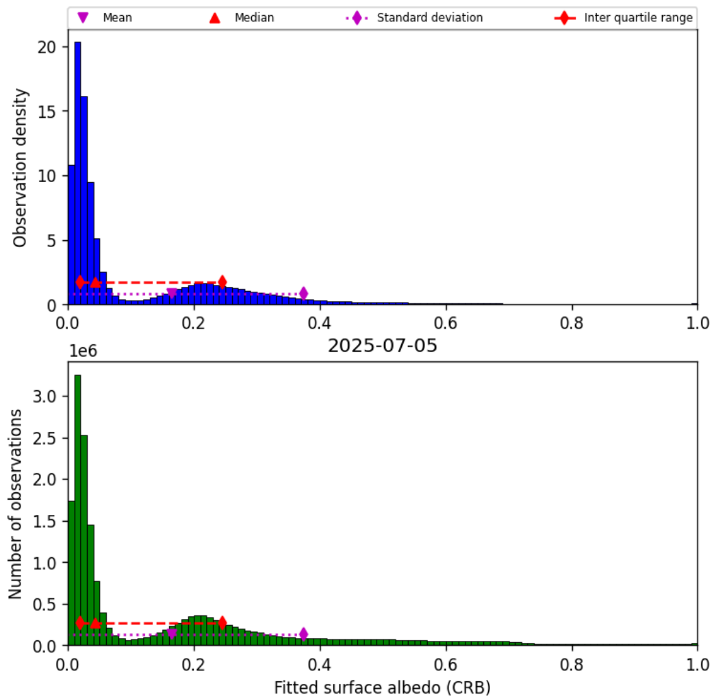
Figure 44: Histogram of “Fitted surface albedo (CRB)” for 2025-07-05 to 2025-07-06
