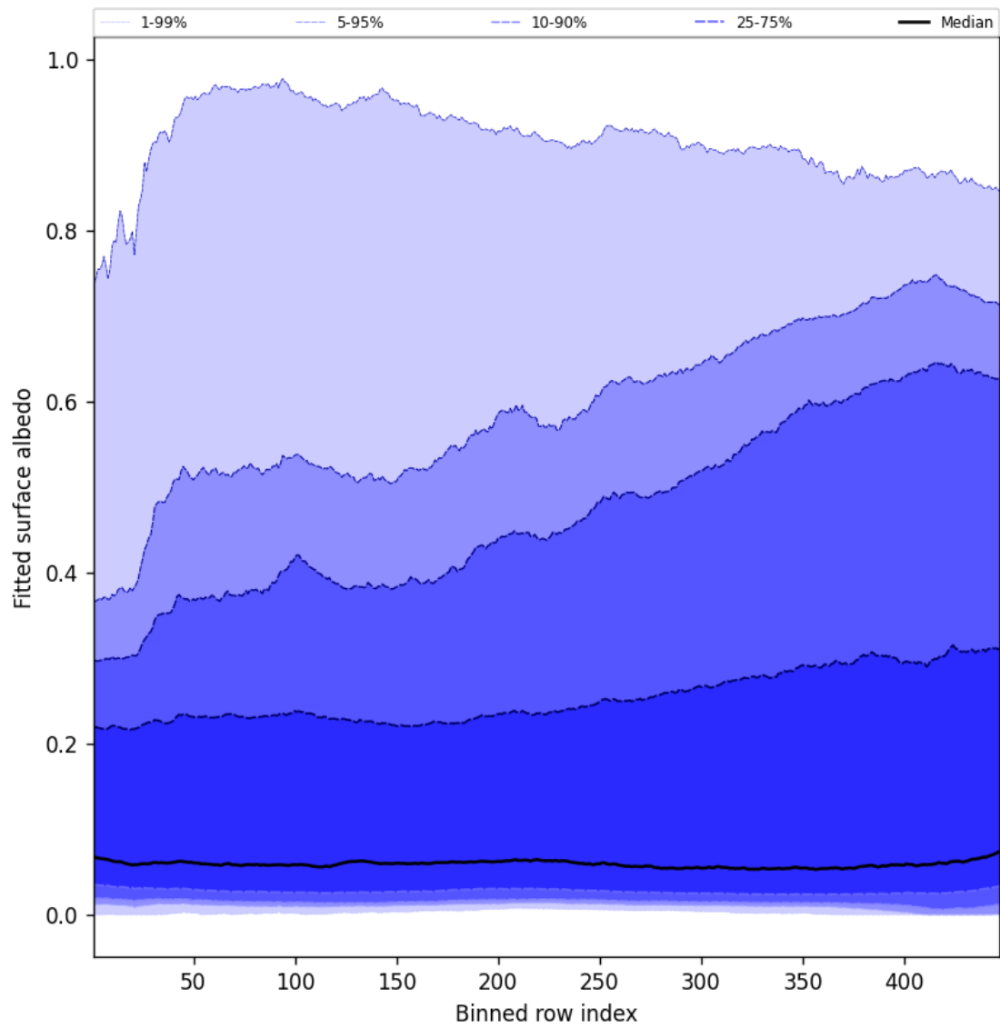
Figure 59: Along track statistics of “Fitted surface albedo” for 2025-07-05 to 2025-07-06
