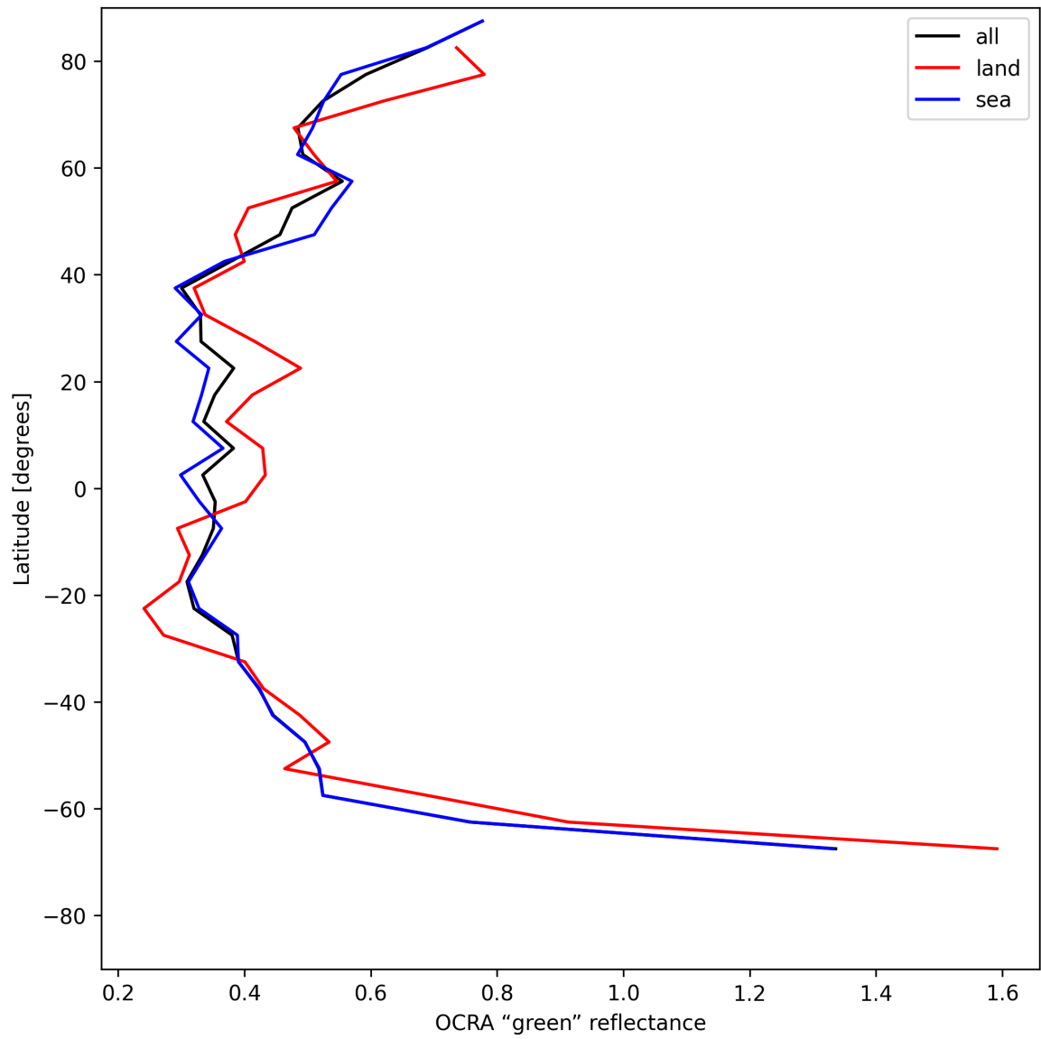
Figure 34: Zonal average of “OCRA “green” reflectance” for 2025-07-05 to 2025-07-06.
