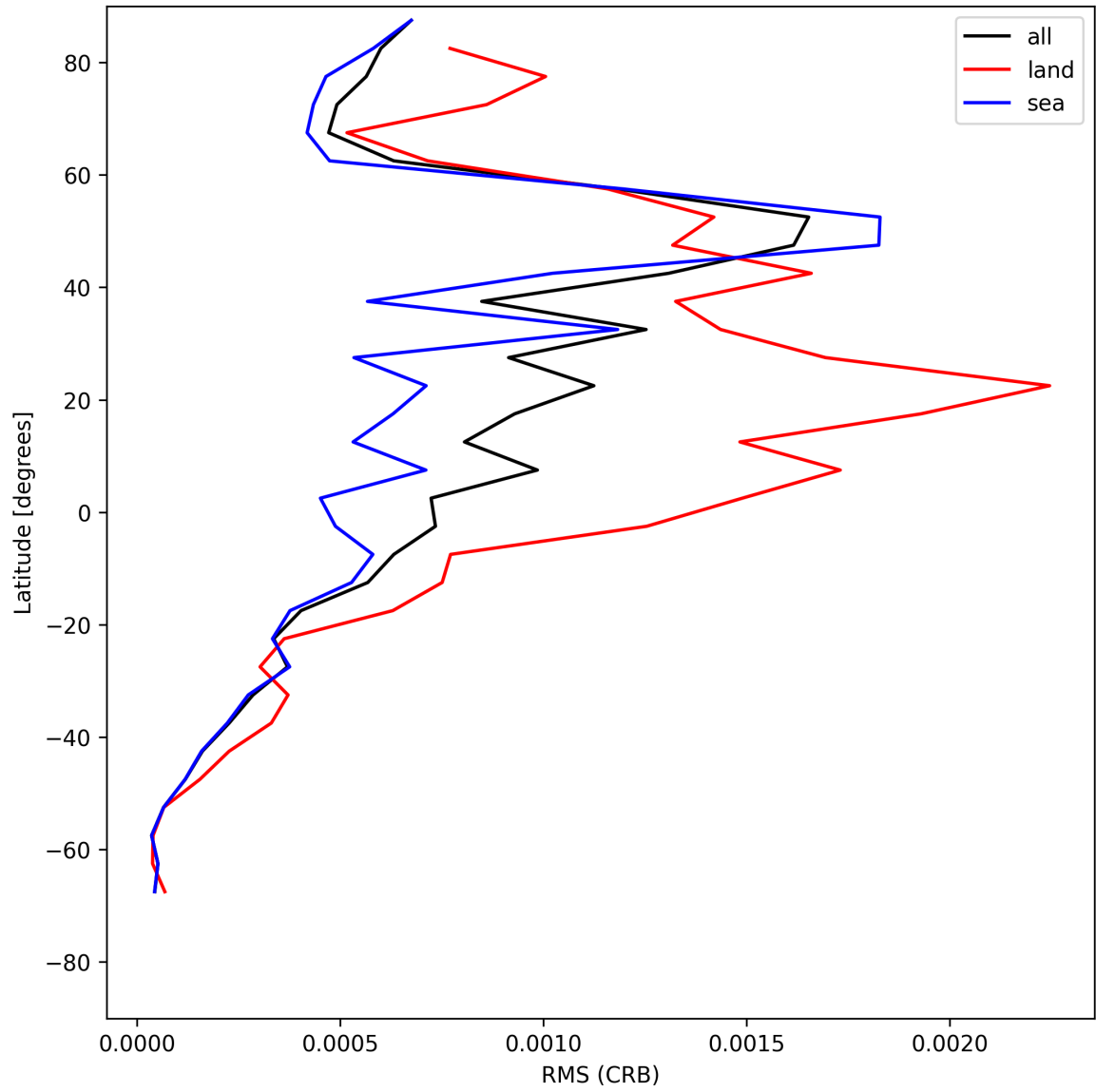
Figure 30: Zonal average of “RMS (CRB)” for 2025-07-05 to 2025-07-06.
