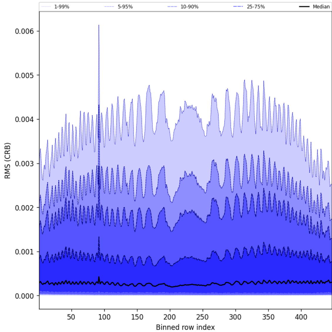
Figure 62: Along track statistics of “RMS (CRB)” for 2025-07-05 to 2025-07-06
