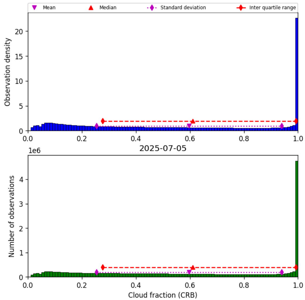
Figure 40: Histogram of “Cloud fraction (CRB)” for 2025-07-05 to 2025-07-06
