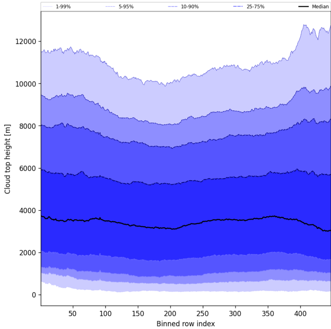
Figure 54: Along track statistics of “Cloud top height” for 2025-07-05 to 2025-07-06
