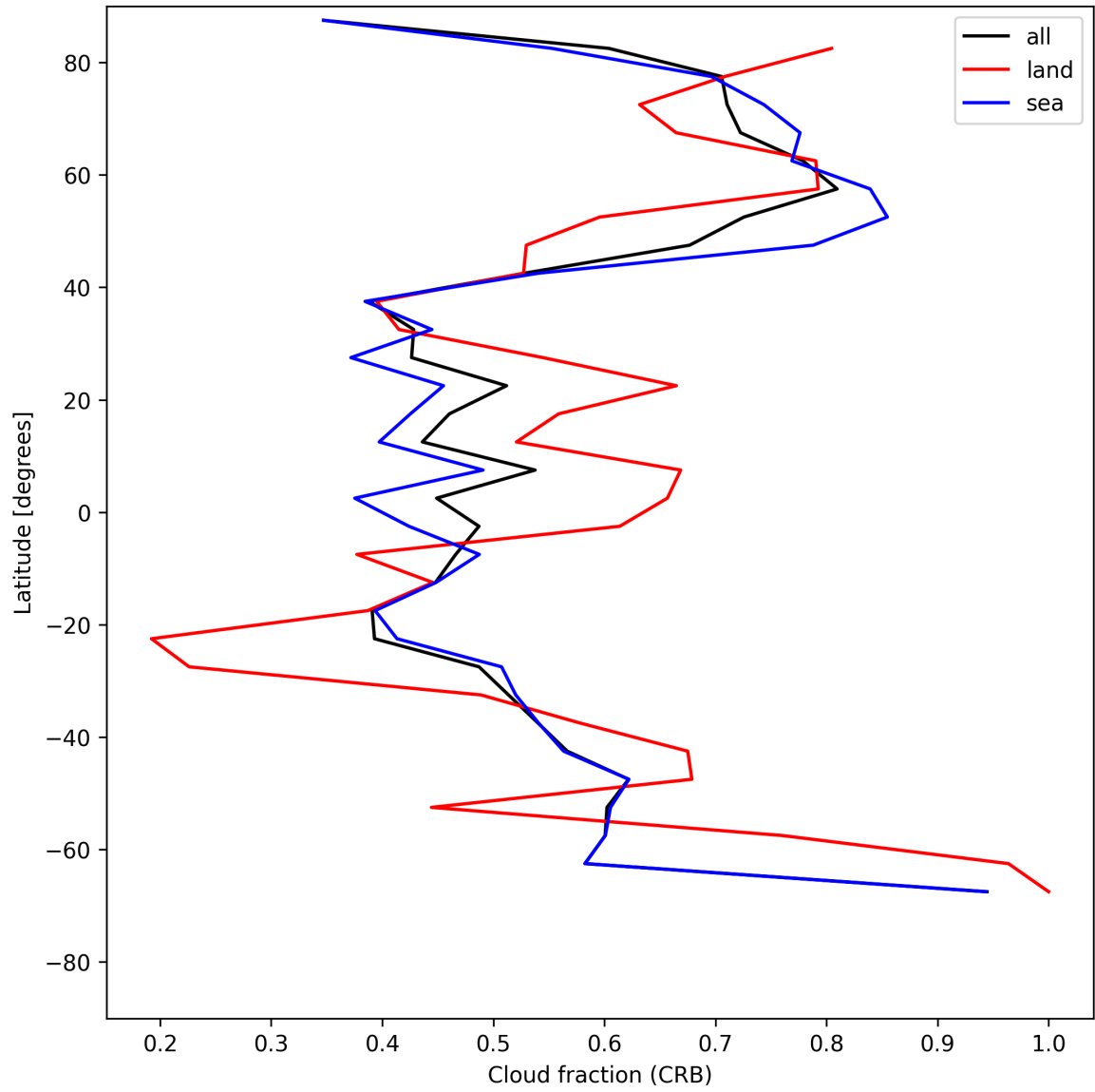
Figure 24: Zonal average of “Cloud fraction (CRB)” for 2025-07-05 to 2025-07-06.
