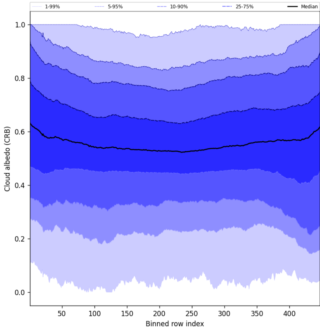
Figure 58: Along track statistics of “Cloud albedo (CRB)” for 2025-07-05 to 2025-07-06
