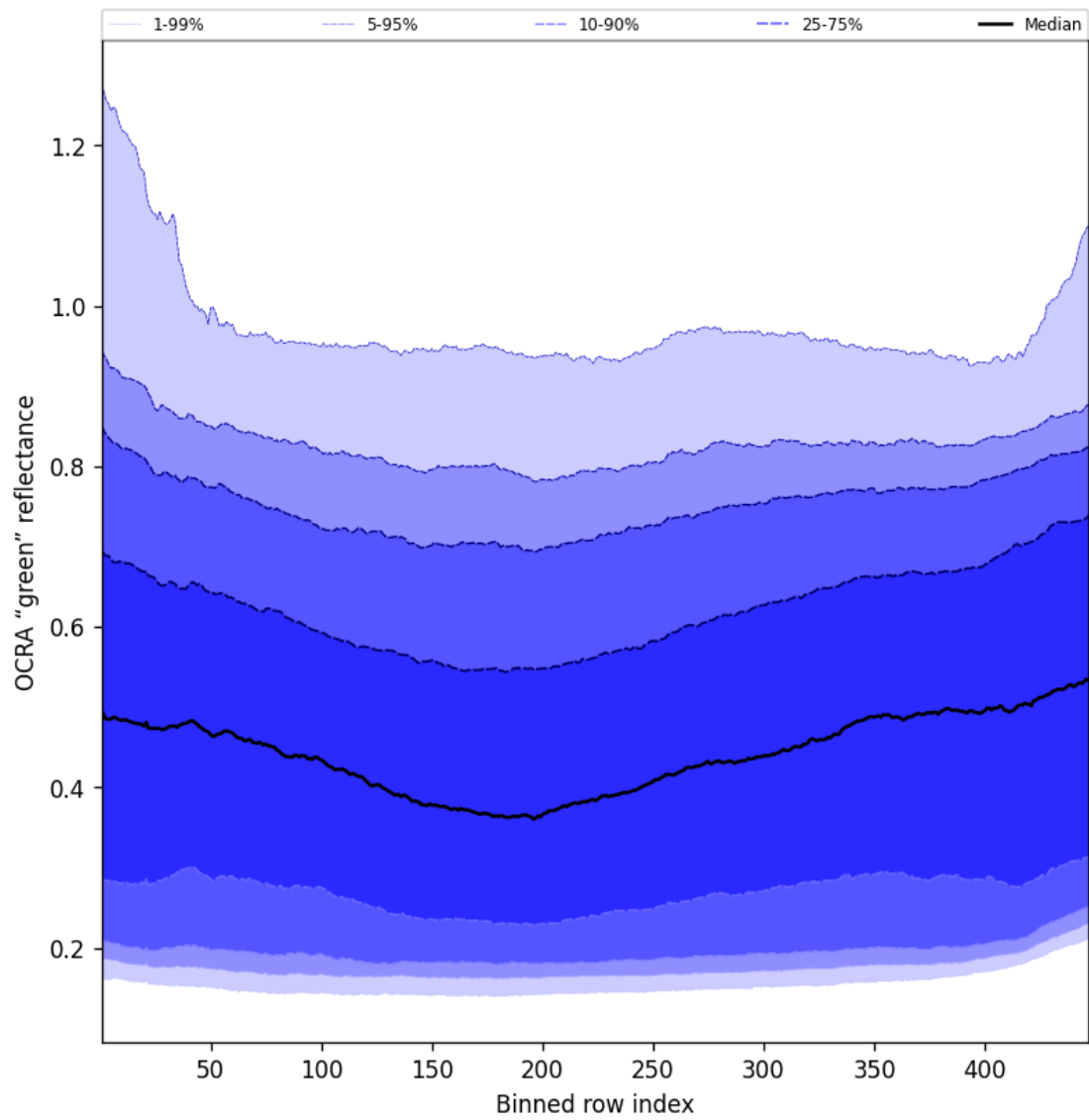
Figure 66: Along track statistics of “OCRA “green” reflectance” for 2025-07-05 to 2025-07-06
