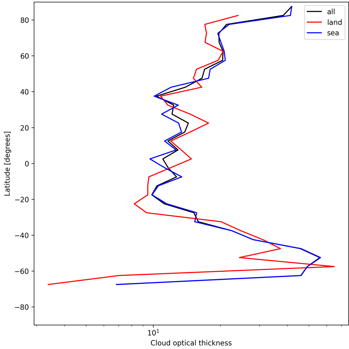
Figure 23: Zonal average of “Cloud optical thickness” for 2025-07-05 to 2025-07-06.
