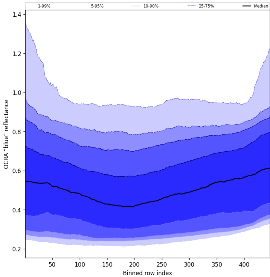
Figure 65: Along track statistics of “OCRA “blue” reflectance” for 2025-07-05 to 2025-07-06
