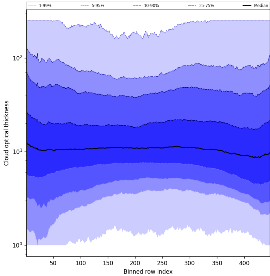
Figure 55: Along track statistics of “Cloud optical thickness” for 2025-07-05 to 2025-07-06
