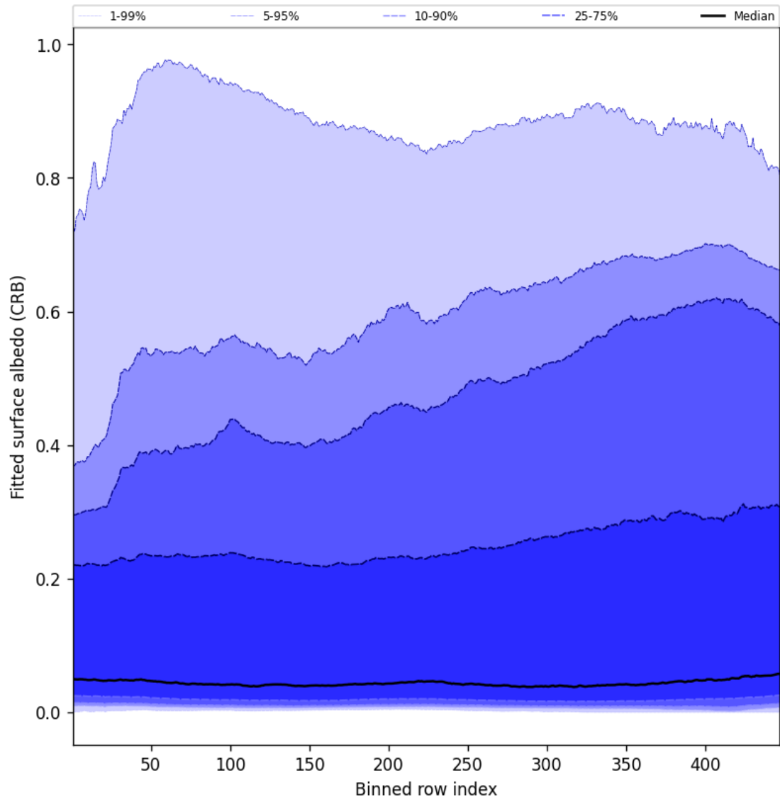
Figure 60: Along track statistics of “Fitted surface albedo (CRB)” for 2025-07-05 to 2025-07-06
