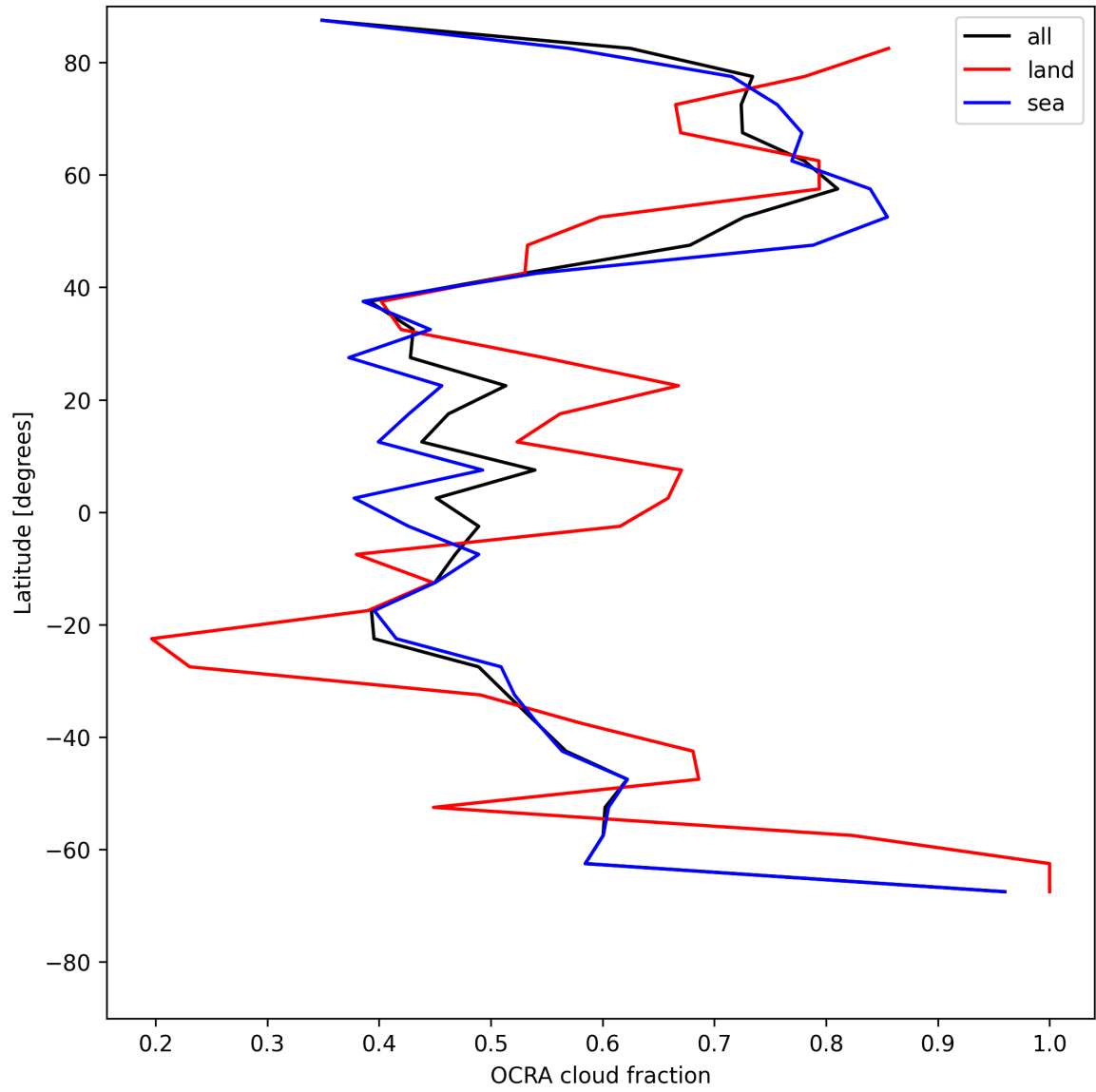
Figure 32: Zonal average of “OCRA cloud fraction” for 2025-07-05 to 2025-07-06.
