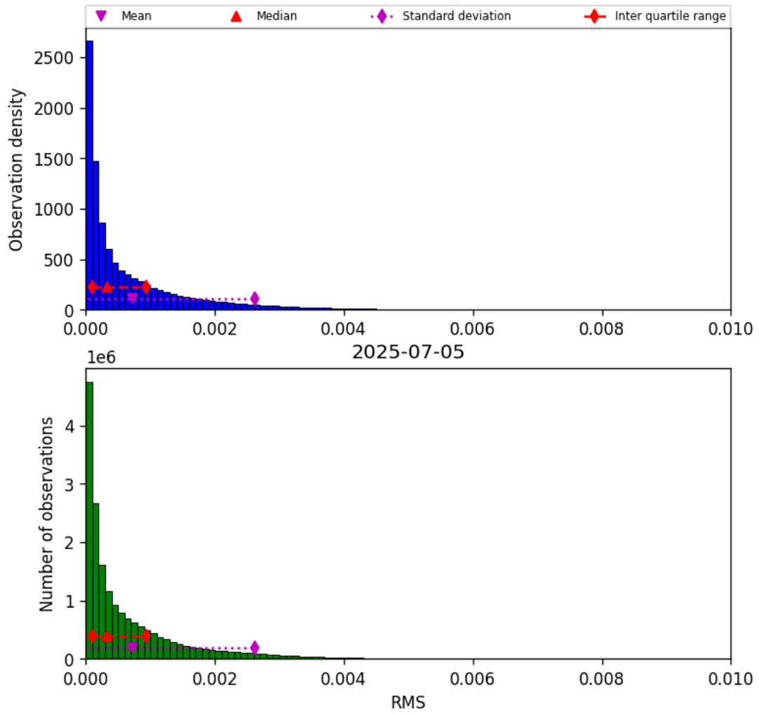
Figure 45: Histogram of “RMS” for 2025-07-05 to 2025-07-06
