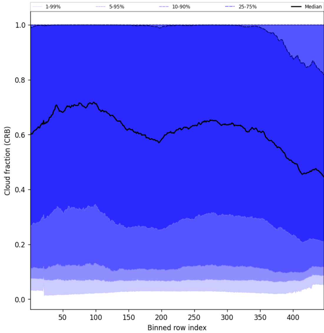
Figure 56: Along track statistics of “Cloud fraction (CRB)” for 2025-07-05 to 2025-07-06
