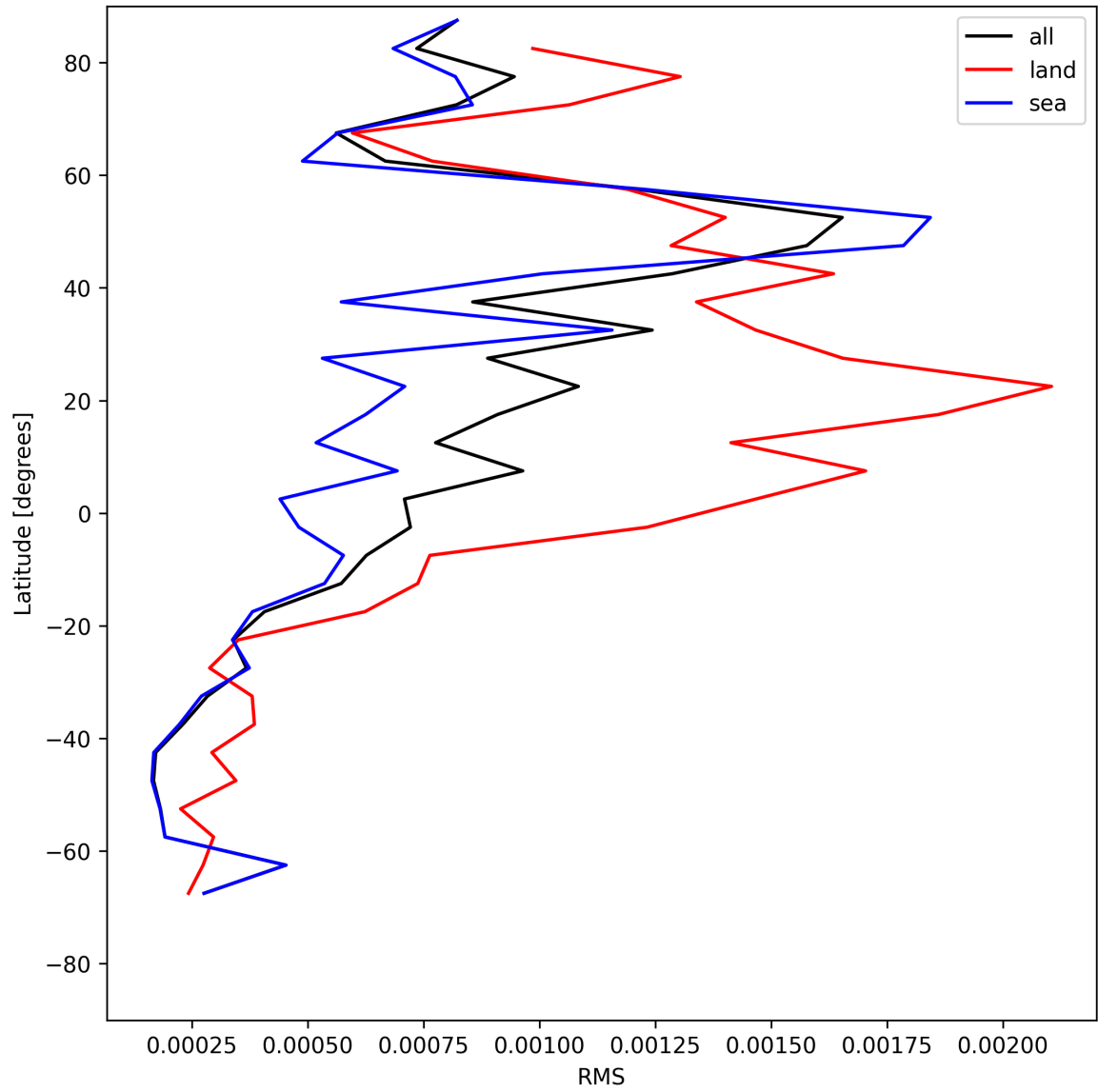
Figure 29: Zonal average of “RMS” for 2025-07-05 to 2025-07-06.
