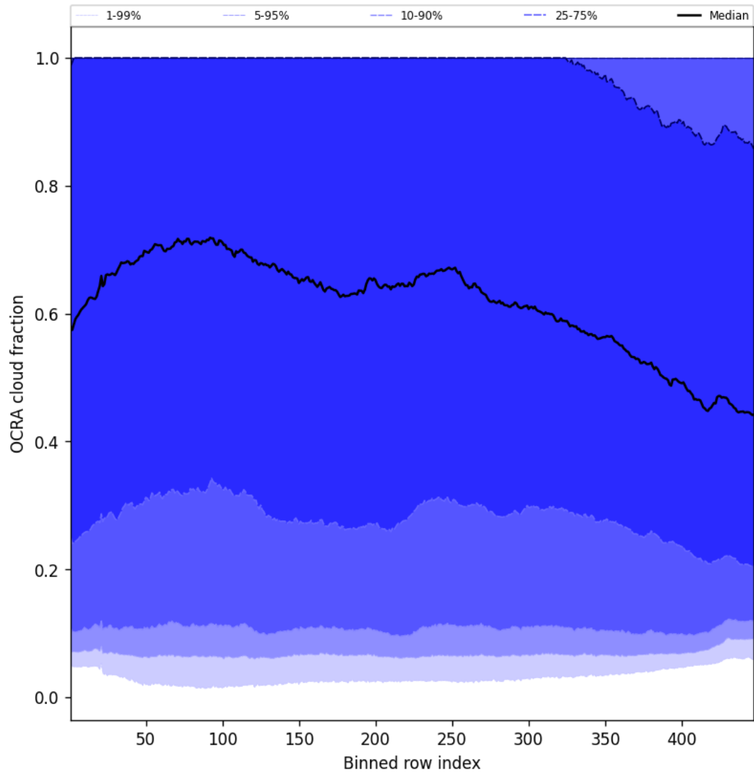
Figure 64: Along track statistics of “OCRA cloud fraction” for 2025-07-06 to 2025-07-06
