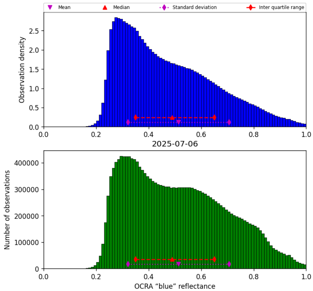
Figure 49: Histogram of “OCRA “blue” reflectance” for 2025-07-06 to 2025-07-06
