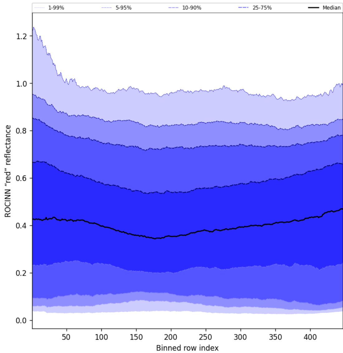
Figure 67: Along track statistics of “ROCINN “red” reflectance” for 2025-07-06 to 2025-07-06
