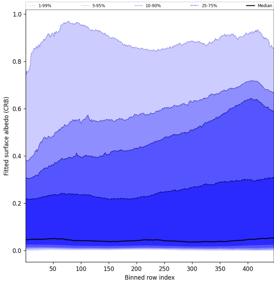
Figure 60: Along track statistics of “Fitted surface albedo (CRB)” for 2025-07-06 to 2025-07-06
