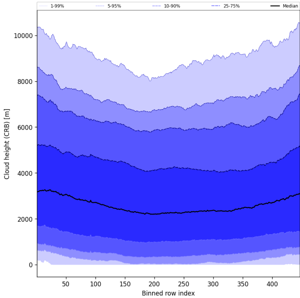
Figure 57: Along track statistics of “Cloud height (CRB)” for 2025-07-06 to 2025-07-06
