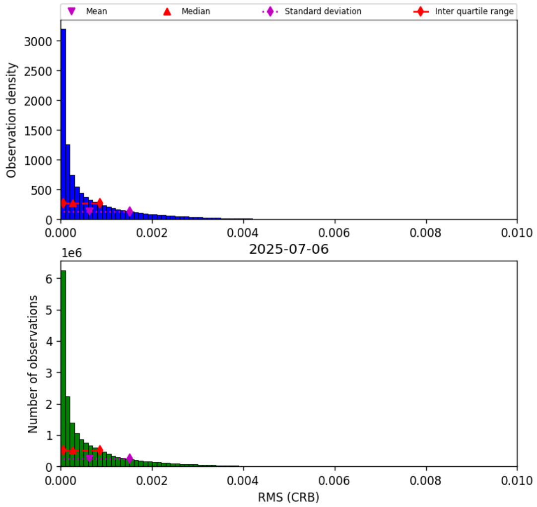
Figure 46: Histogram of “RMS (CRB)” for 2025-07-06 to 2025-07-06
