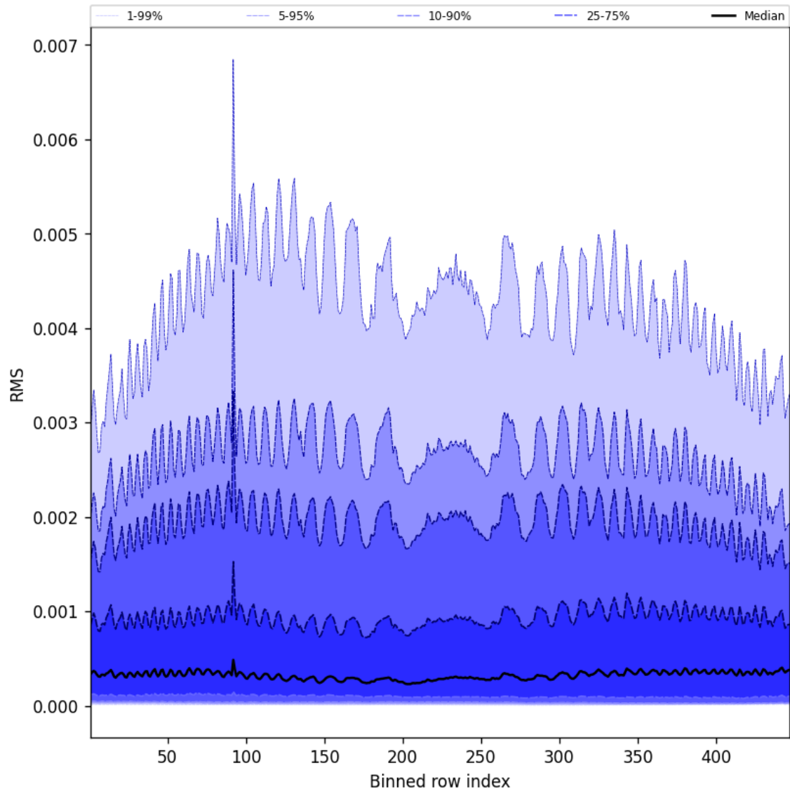
Figure 61: Along track statistics of “RMS” for 2025-07-06 to 2025-07-06
