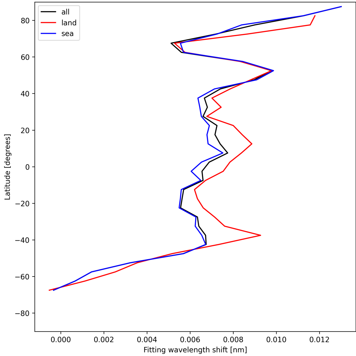
Figure 31: Zonal average of “Fitting wavelength shift” for 2025-07-06 to 2025-07-06.
