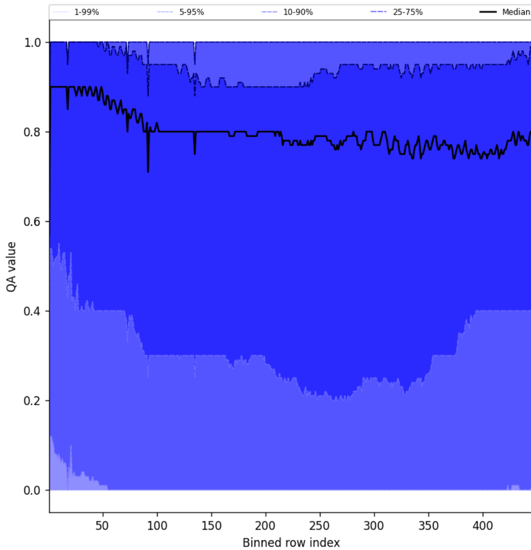
Figure 52: Along track statistics of “QA value” for 2025-07-06 to 2025-07-06
