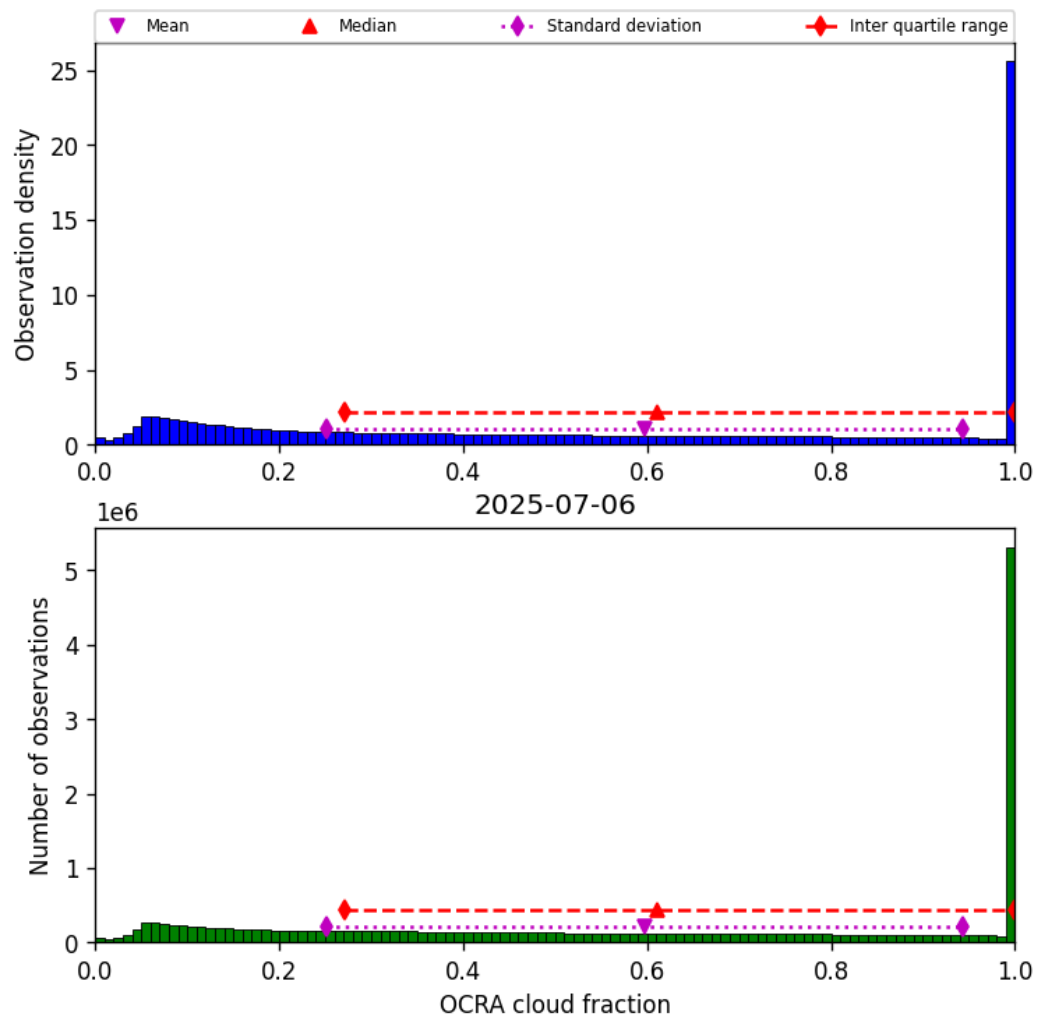
Figure 48: Histogram of “OCRA cloud fraction” for 2025-07-06 to 2025-07-06
