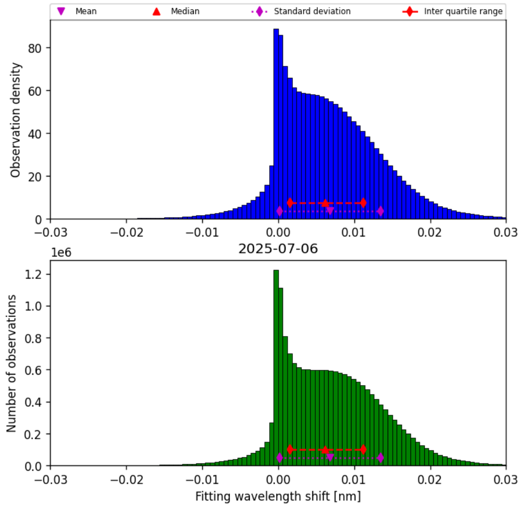
Figure 47: Histogram of “Fitting wavelength shift” for 2025-07-06 to 2025-07-06
