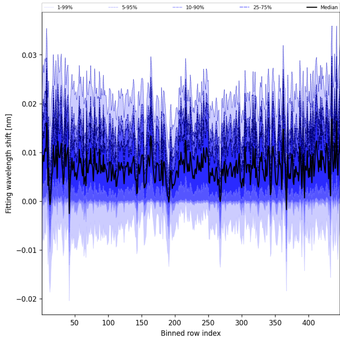
Figure 63: Along track statistics of “Fitting wavelength shift” for 2025-07-06 to 2025-07-06
