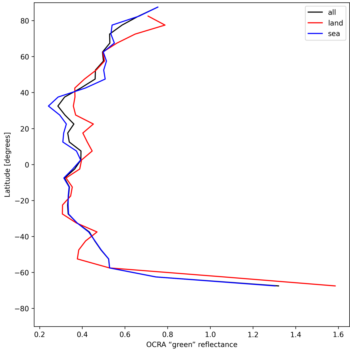
Figure 34: Zonal average of “OCRA “green” reflectance” for 2025-07-08 to 2025-07-09.
