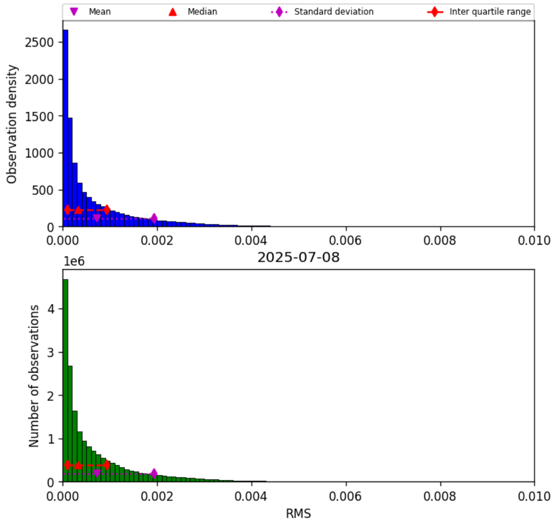
Figure 45: Histogram of “RMS” for 2025-07-08 to 2025-07-09
