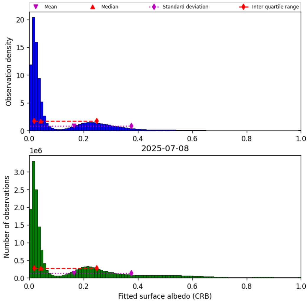
Figure 44: Histogram of “Fitted surface albedo (CRB)” for 2025-07-08 to 2025-07-09
