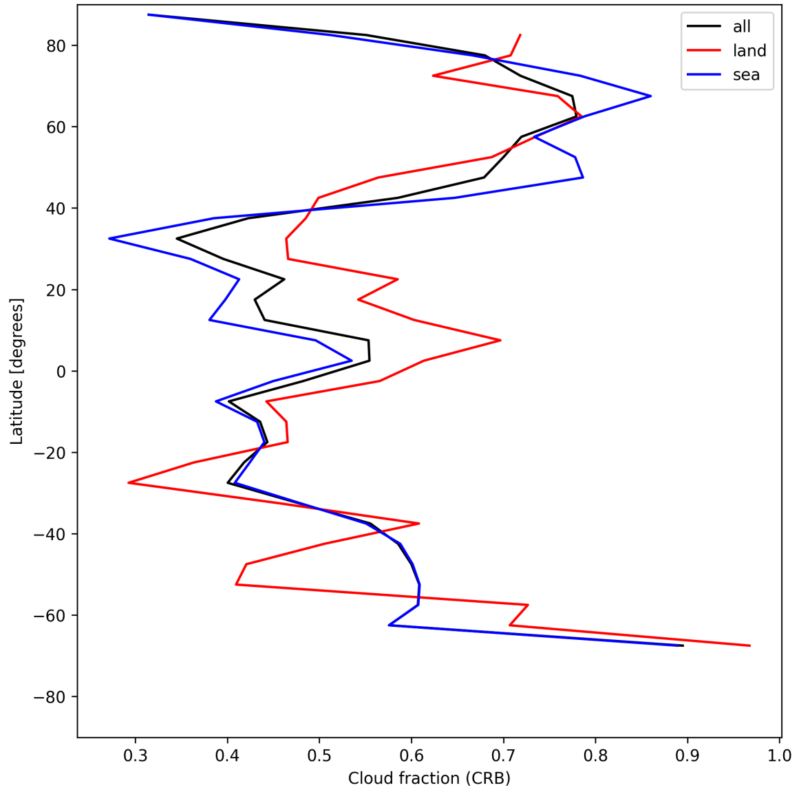
Figure 24: Zonal average of “Cloud fraction (CRB)” for 2025-07-08 to 2025-07-09.
