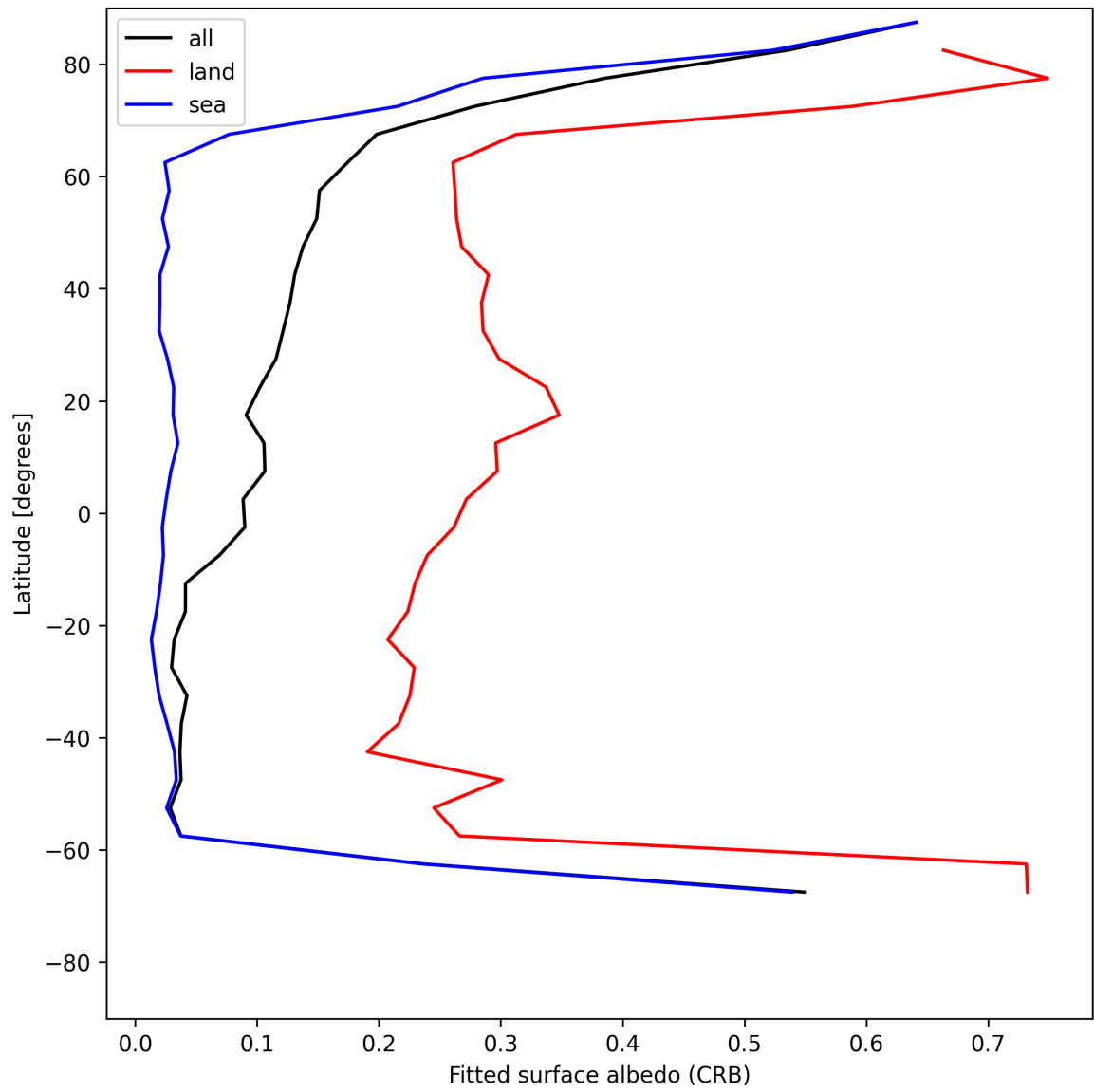
Figure 28: Zonal average of “Fitted surface albedo (CRB)” for 2025-07-08 to 2025-07-09.
