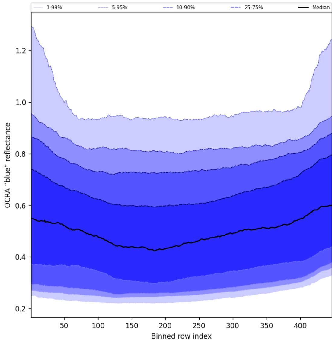
Figure 65: Along track statistics of “OCRA “blue” reflectance” for 2025-07-08 to 2025-07-09
