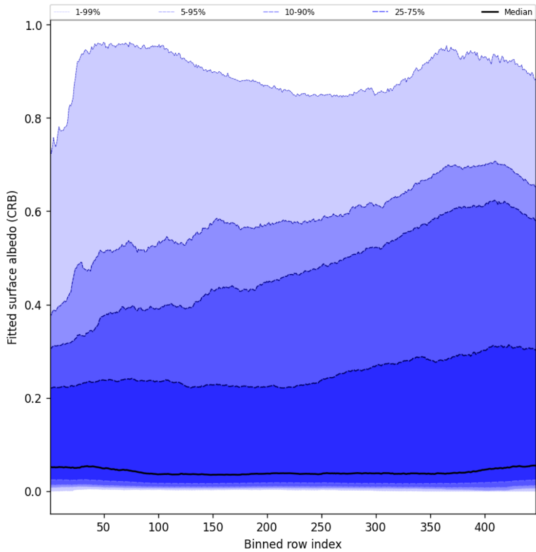
Figure 60: Along track statistics of “Fitted surface albedo (CRB)” for 2025-07-08 to 2025-07-09
