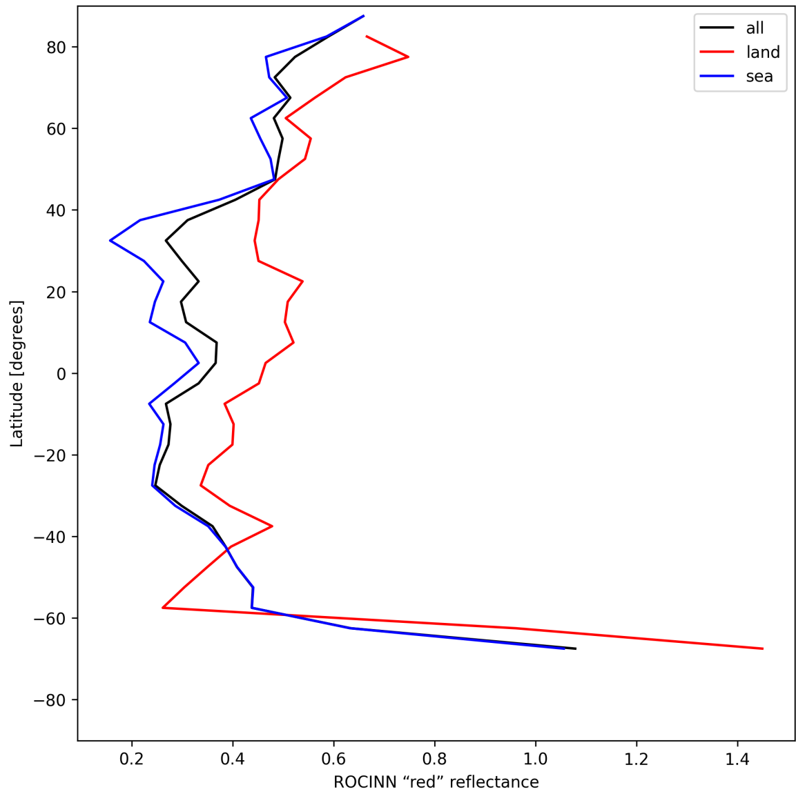
Figure 35: Zonal average of “ROCINN “red” reflectance” for 2025-07-08 to 2025-07-09.
