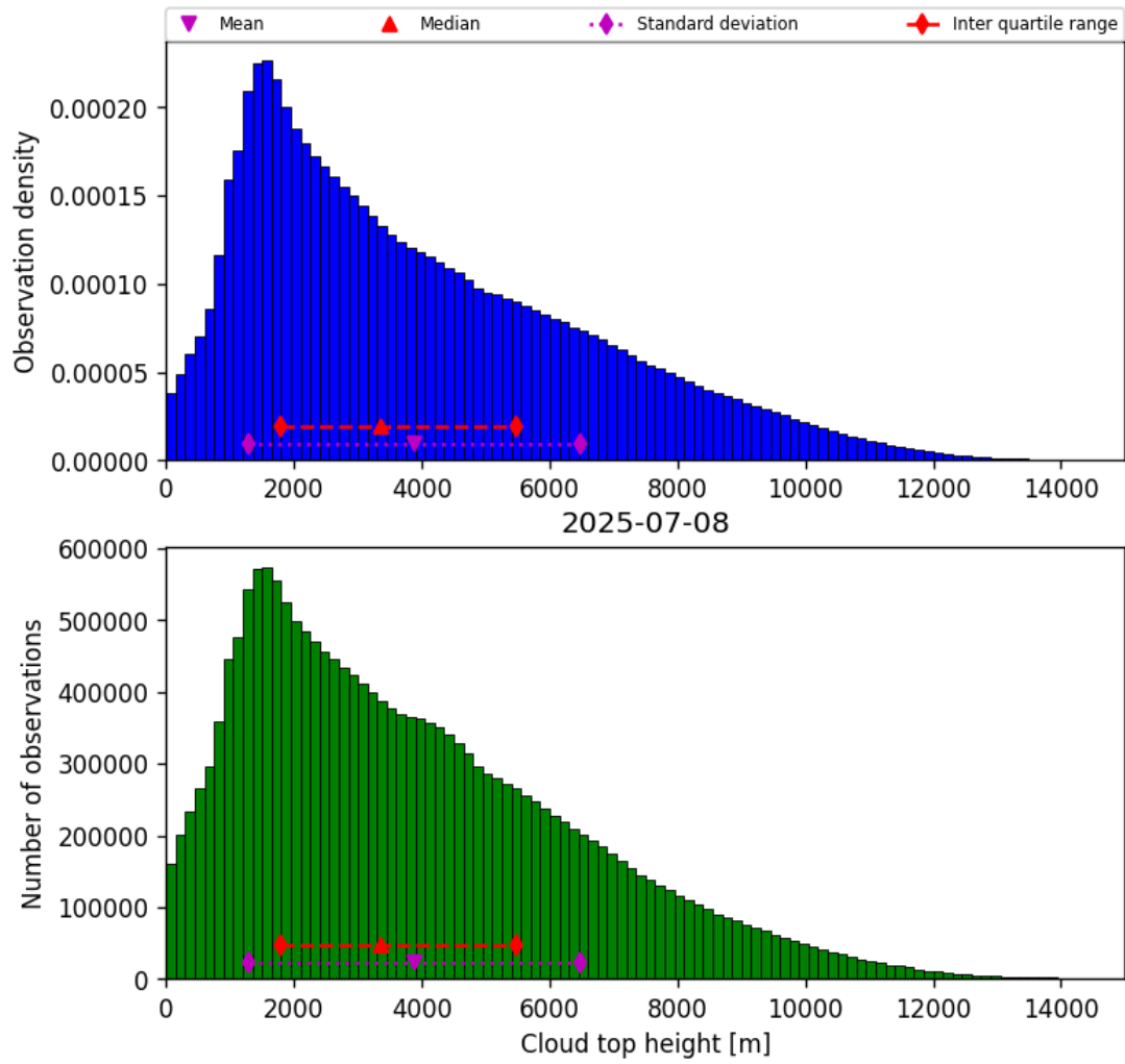
Figure 38: Histogram of “Cloud top height” for 2025-07-08 to 2025-07-09
