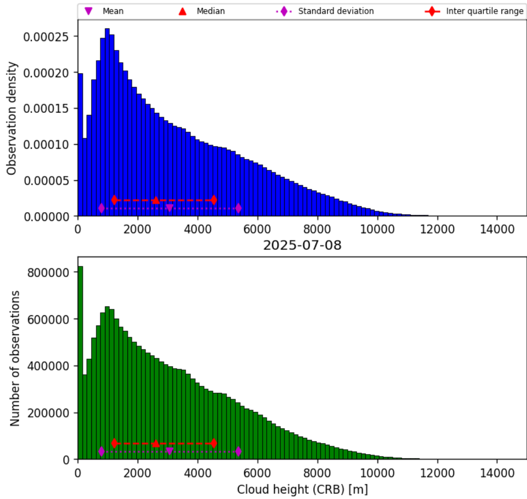
Figure 41: Histogram of “Cloud height (CRB)” for 2025-07-08 to 2025-07-09
