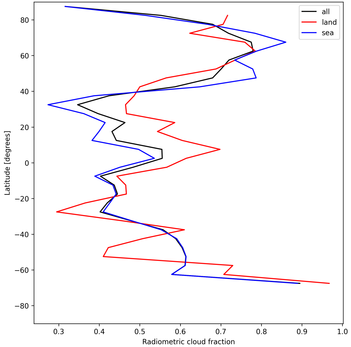
Figure 21: Zonal average of “Radiometric cloud fraction” for 2025-07-08 to 2025-07-09.
