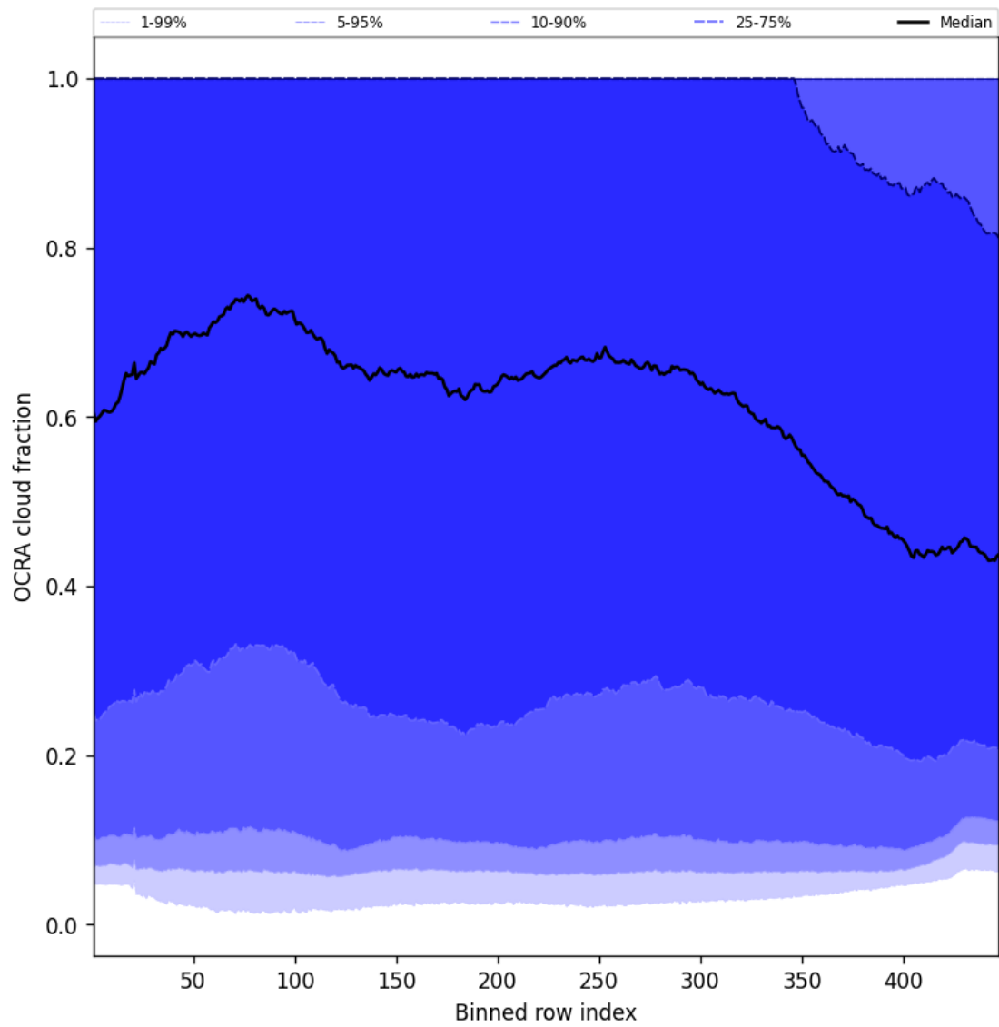
Figure 64: Along track statistics of “OCRA cloud fraction” for 2025-07-08 to 2025-07-09
