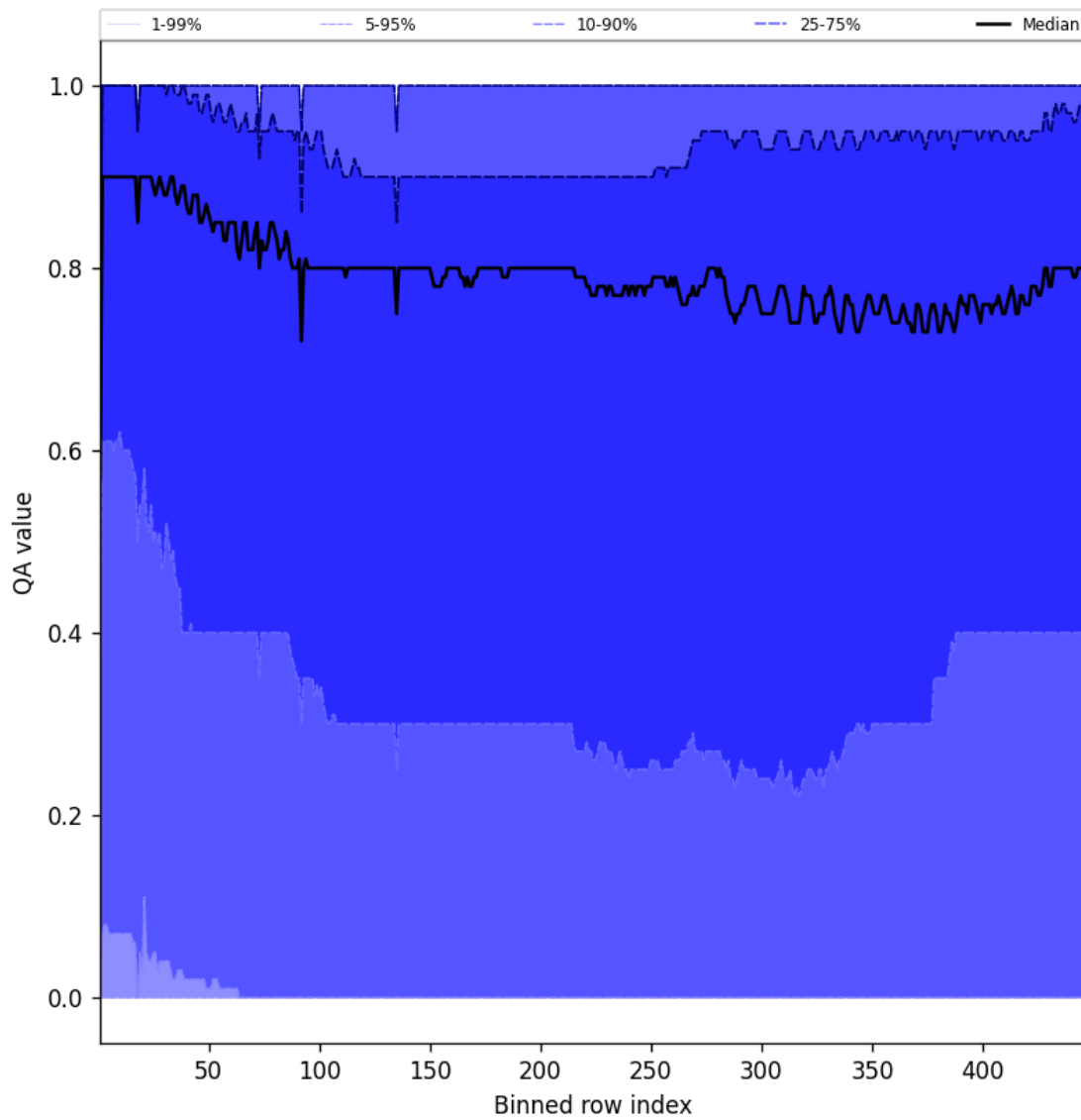
Figure 52: Along track statistics of “QA value” for 2025-07-08 to 2025-07-09
