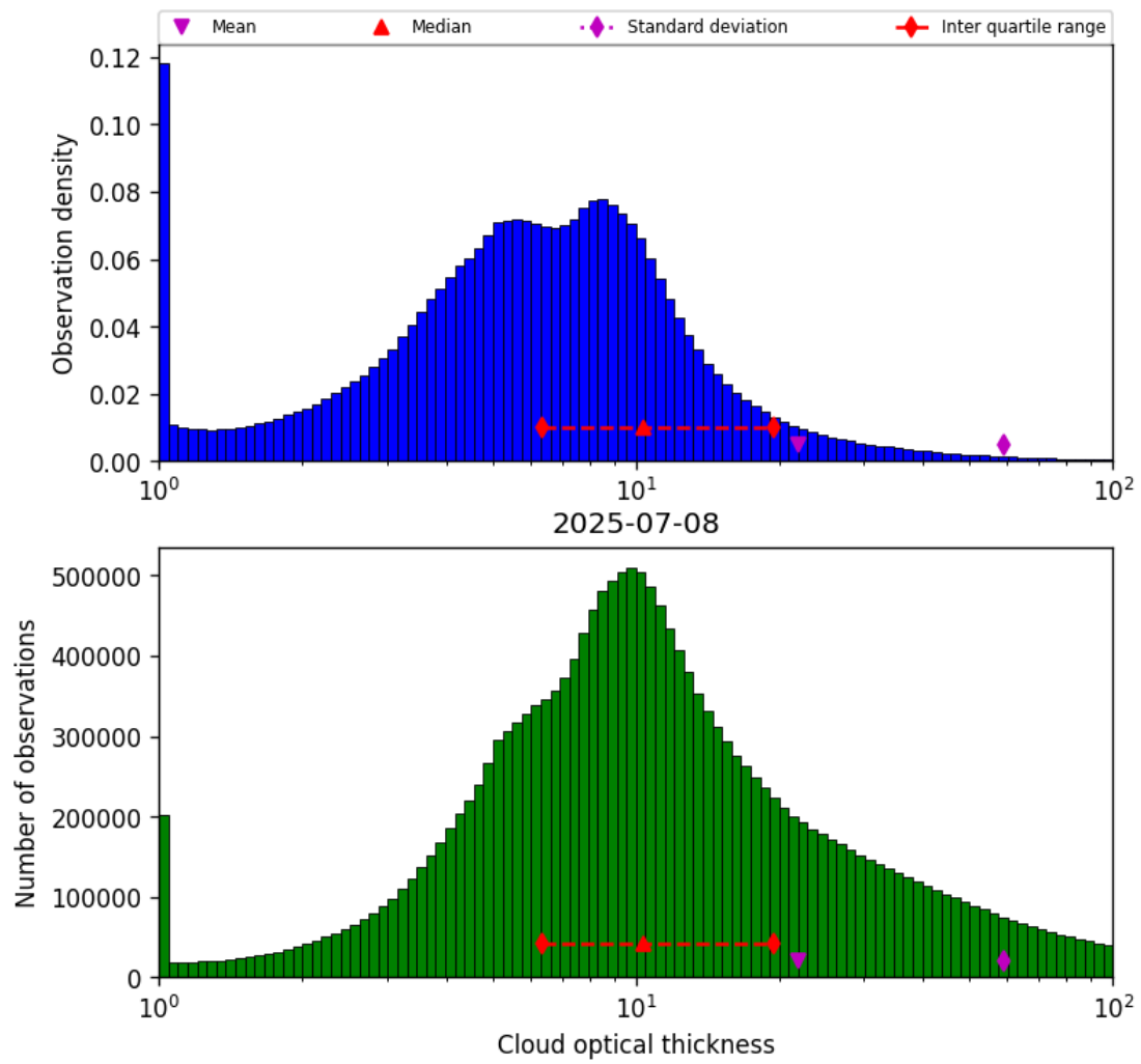
Figure 39: Histogram of “Cloud optical thickness” for 2025-07-08 to 2025-07-09
