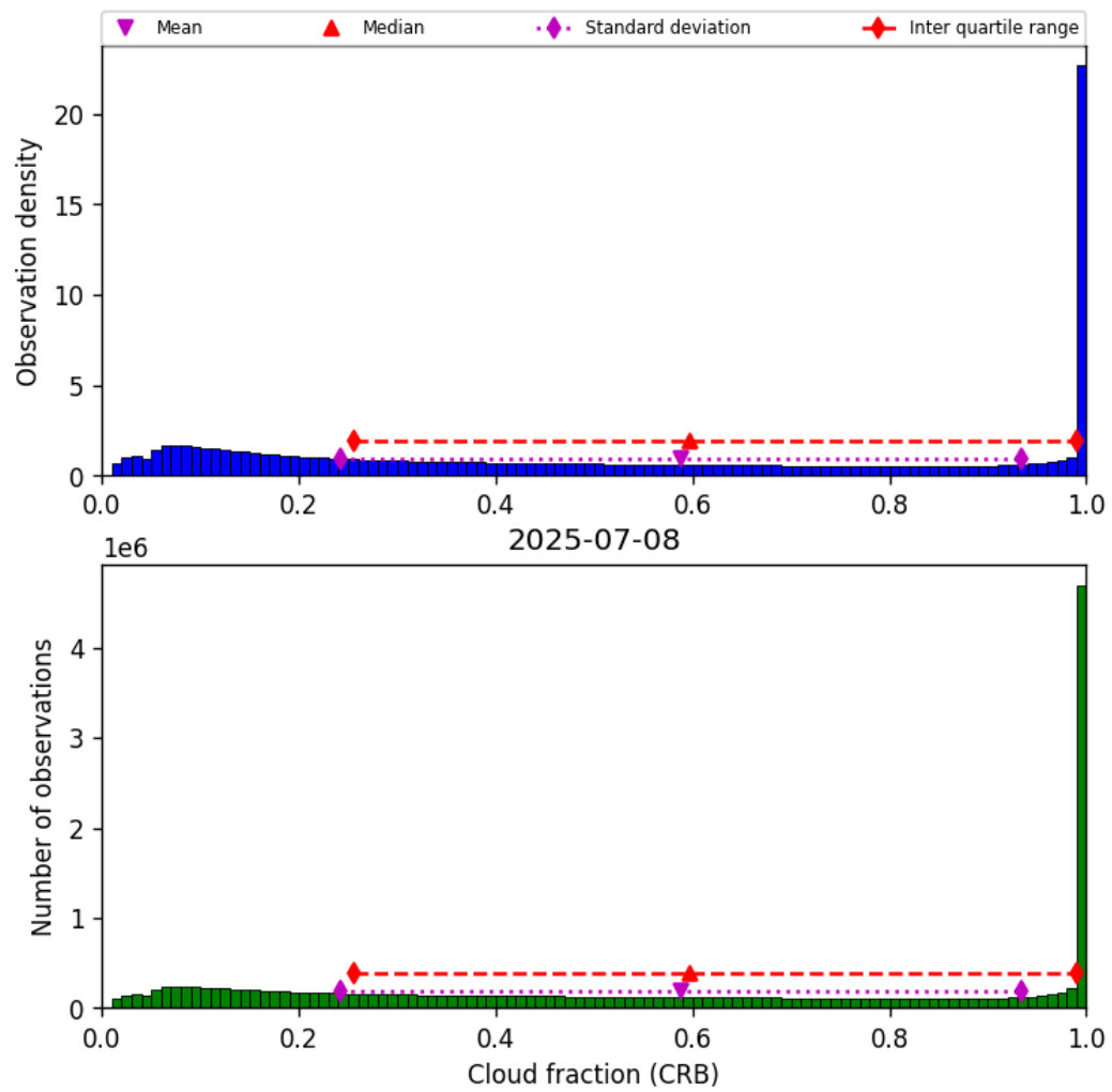
Figure 40: Histogram of “Cloud fraction (CRB)” for 2025-07-08 to 2025-07-09
