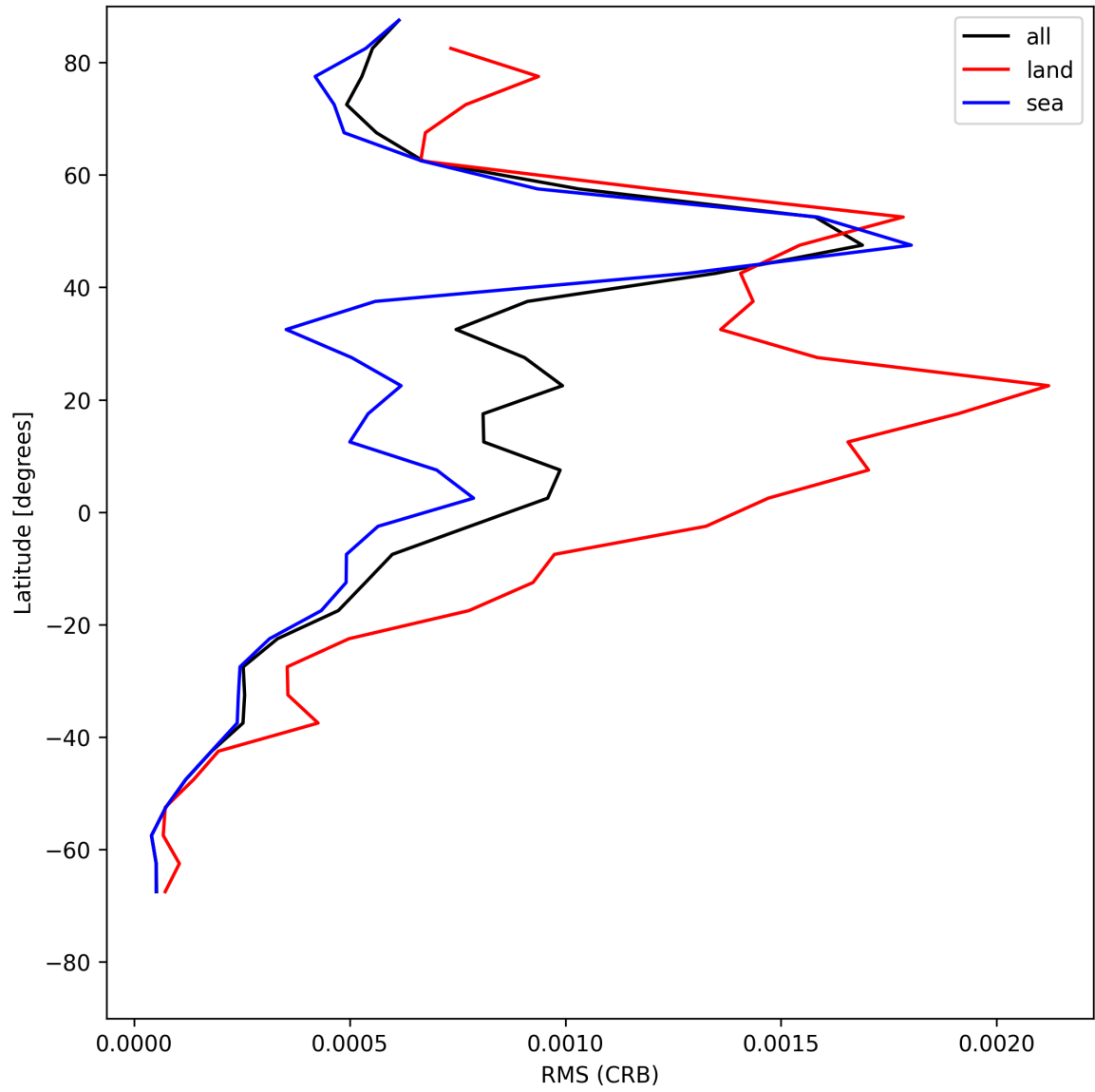
Figure 30: Zonal average of “RMS (CRB)” for 2025-07-08 to 2025-07-09.
