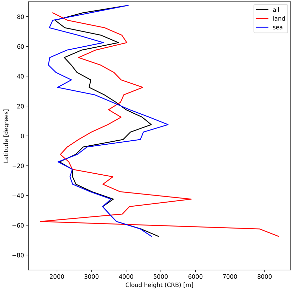
Figure 25: Zonal average of “Cloud height (CRB)” for 2025-07-08 to 2025-07-09.
