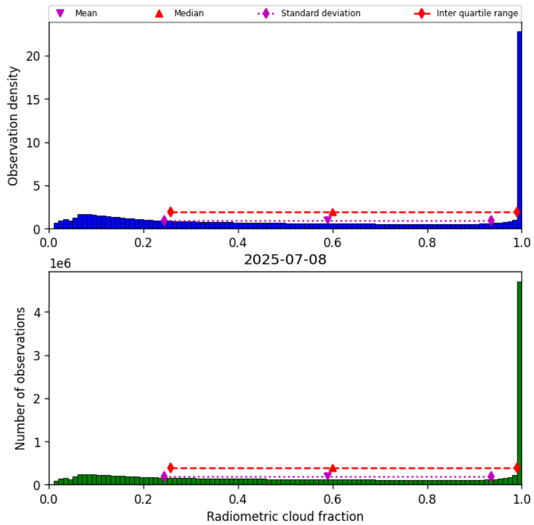
Figure 37: Histogram of “Radiometric cloud fraction” for 2025-07-08 to 2025-07-09
