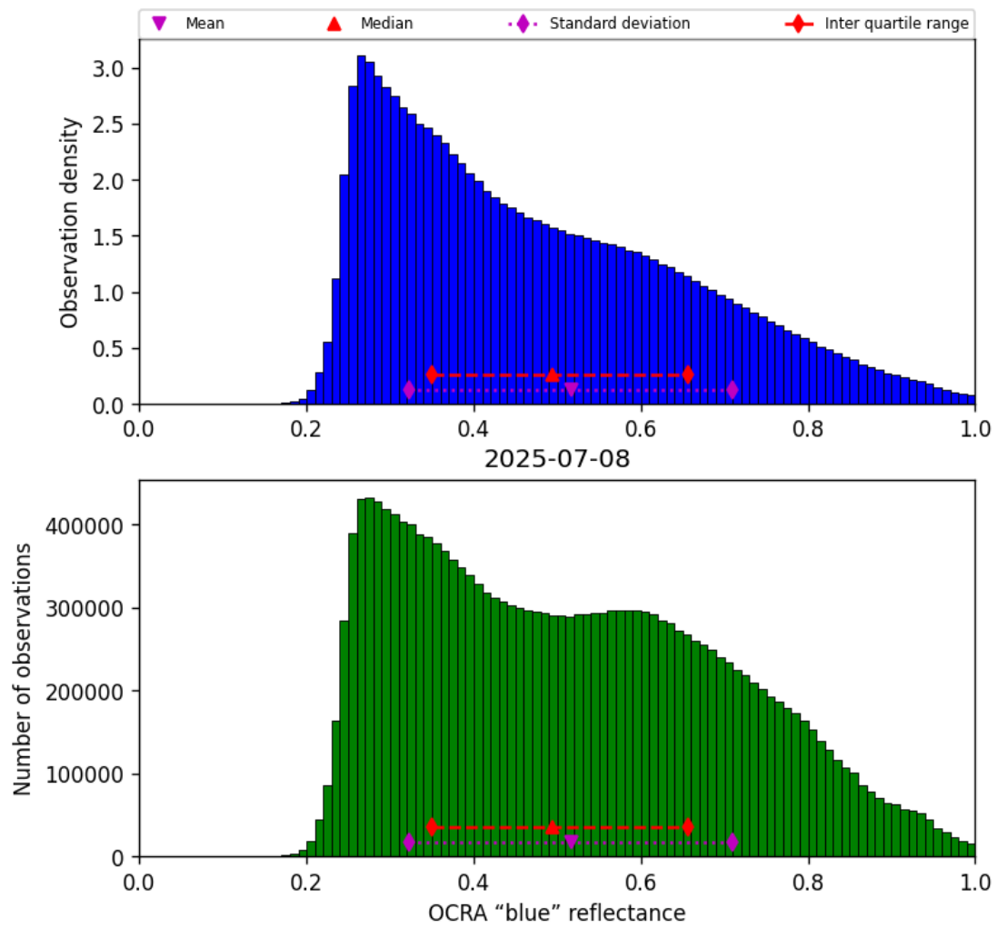
Figure 49: Histogram of “OCRA “blue” reflectance” for 2025-07-08 to 2025-07-09
