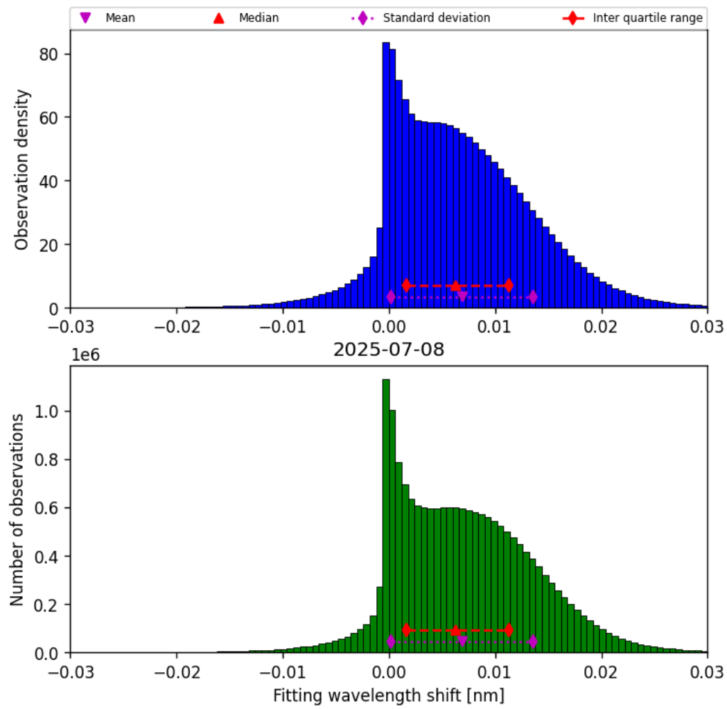
Figure 47: Histogram of “Fitting wavelength shift” for 2025-07-08 to 2025-07-09
