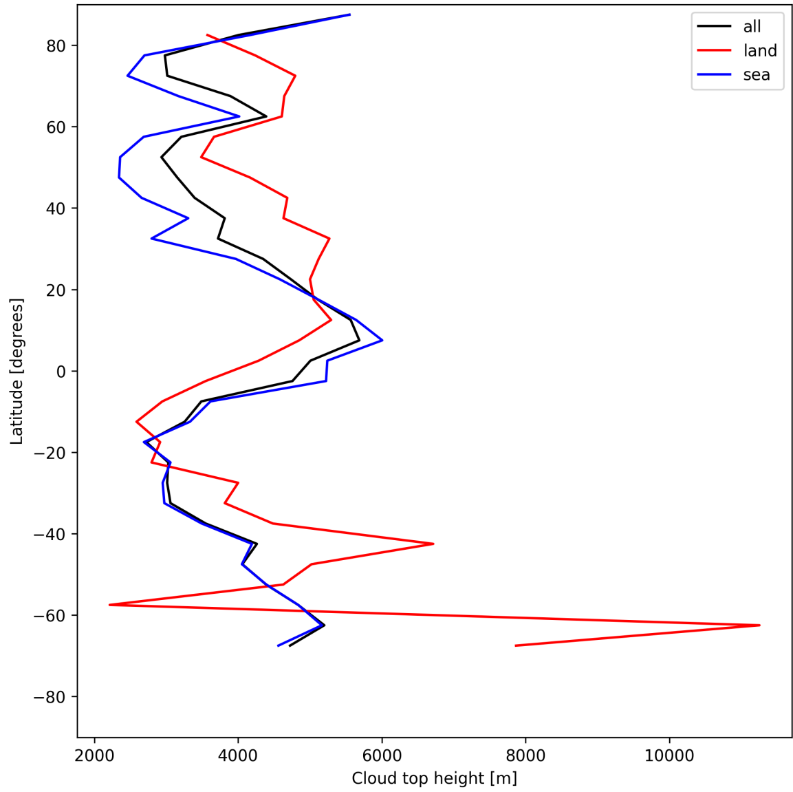
Figure 22: Zonal average of “Cloud top height” for 2025-07-08 to 2025-07-09.
