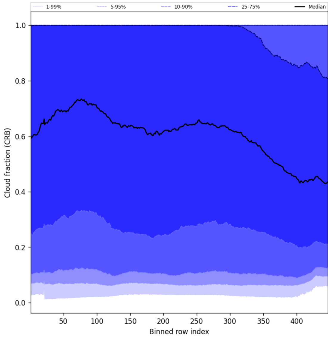
Figure 56: Along track statistics of “Cloud fraction (CRB)” for 2025-07-08 to 2025-07-09
