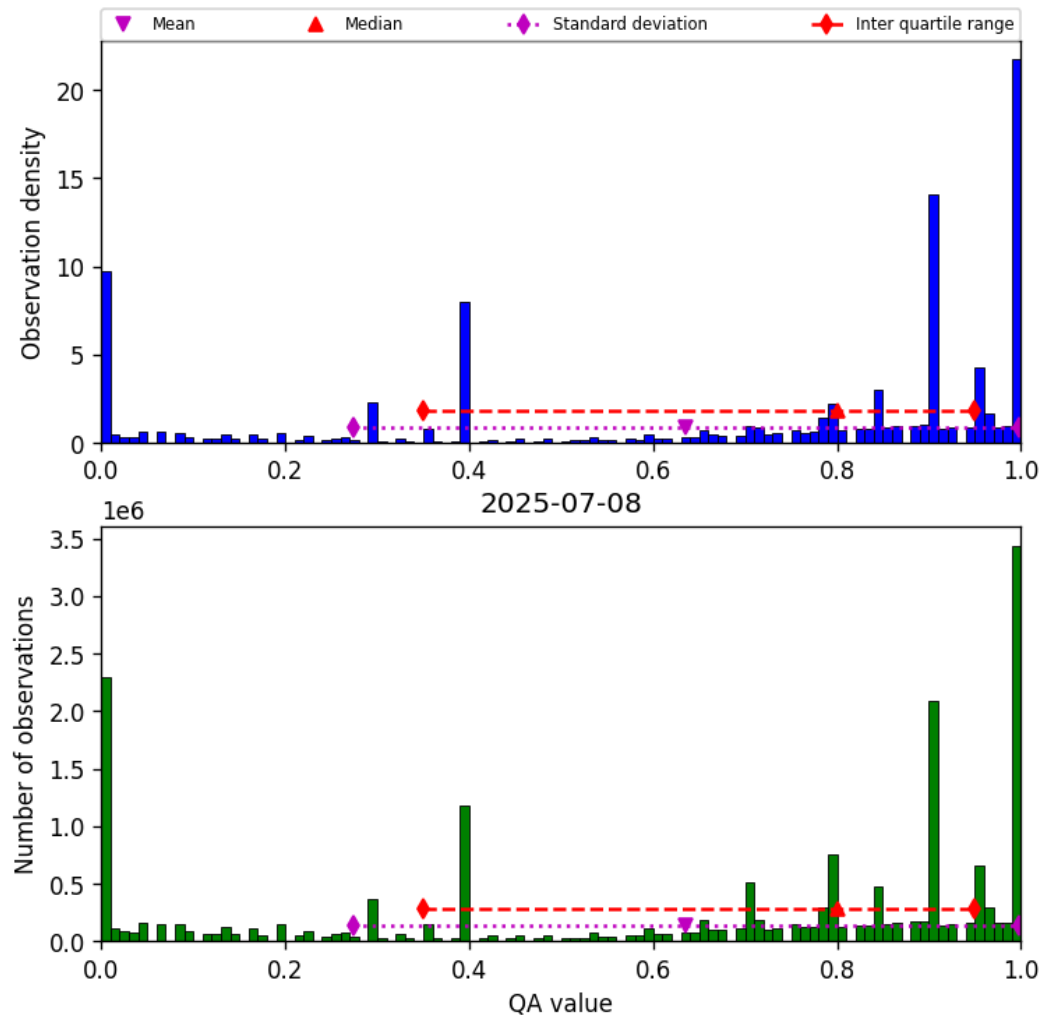
Figure 36: Histogram of “QA value” for 2025-07-08 to 2025-07-09
