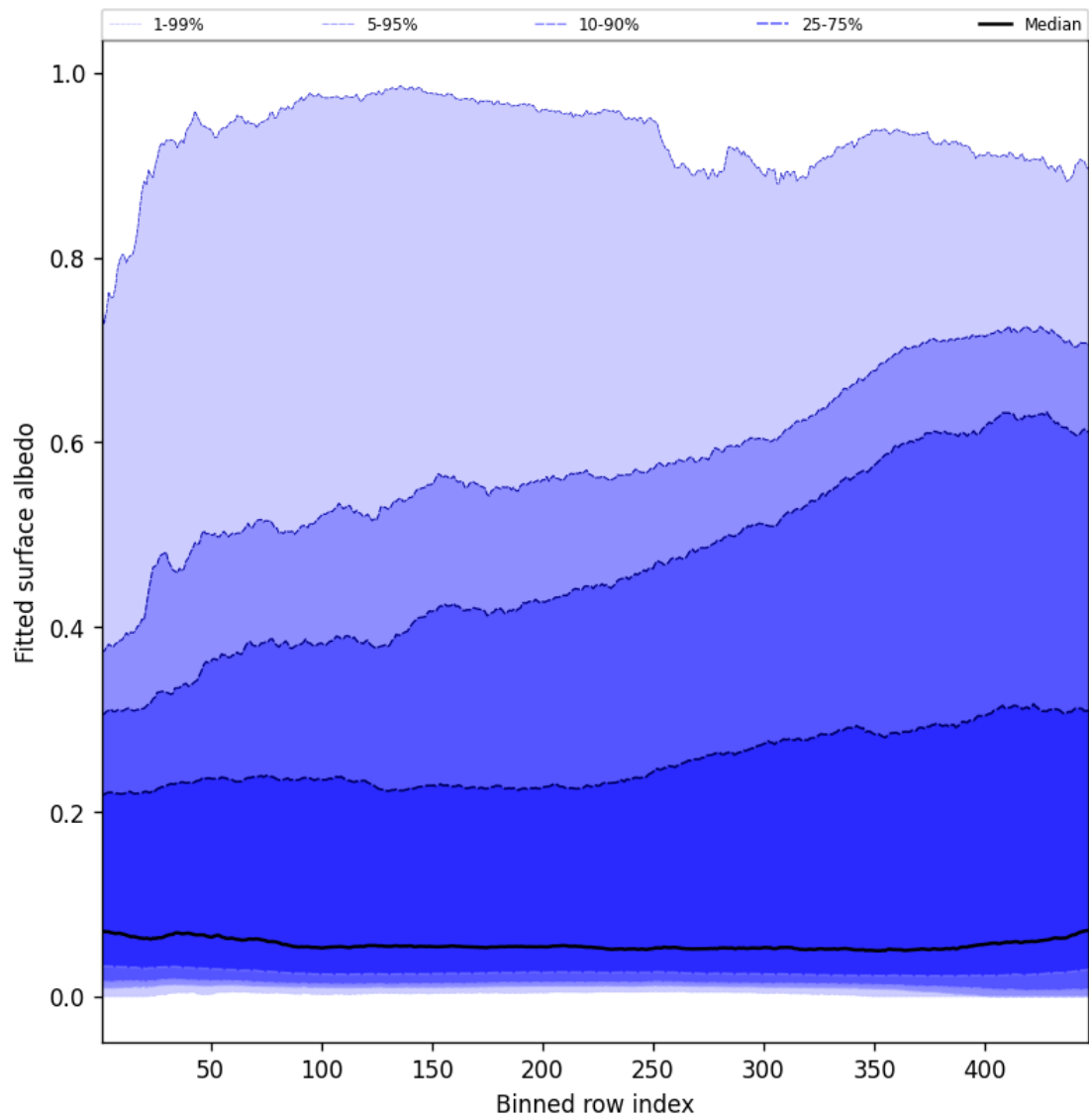
Figure 59: Along track statistics of “Fitted surface albedo” for 2025-07-08 to 2025-07-09
