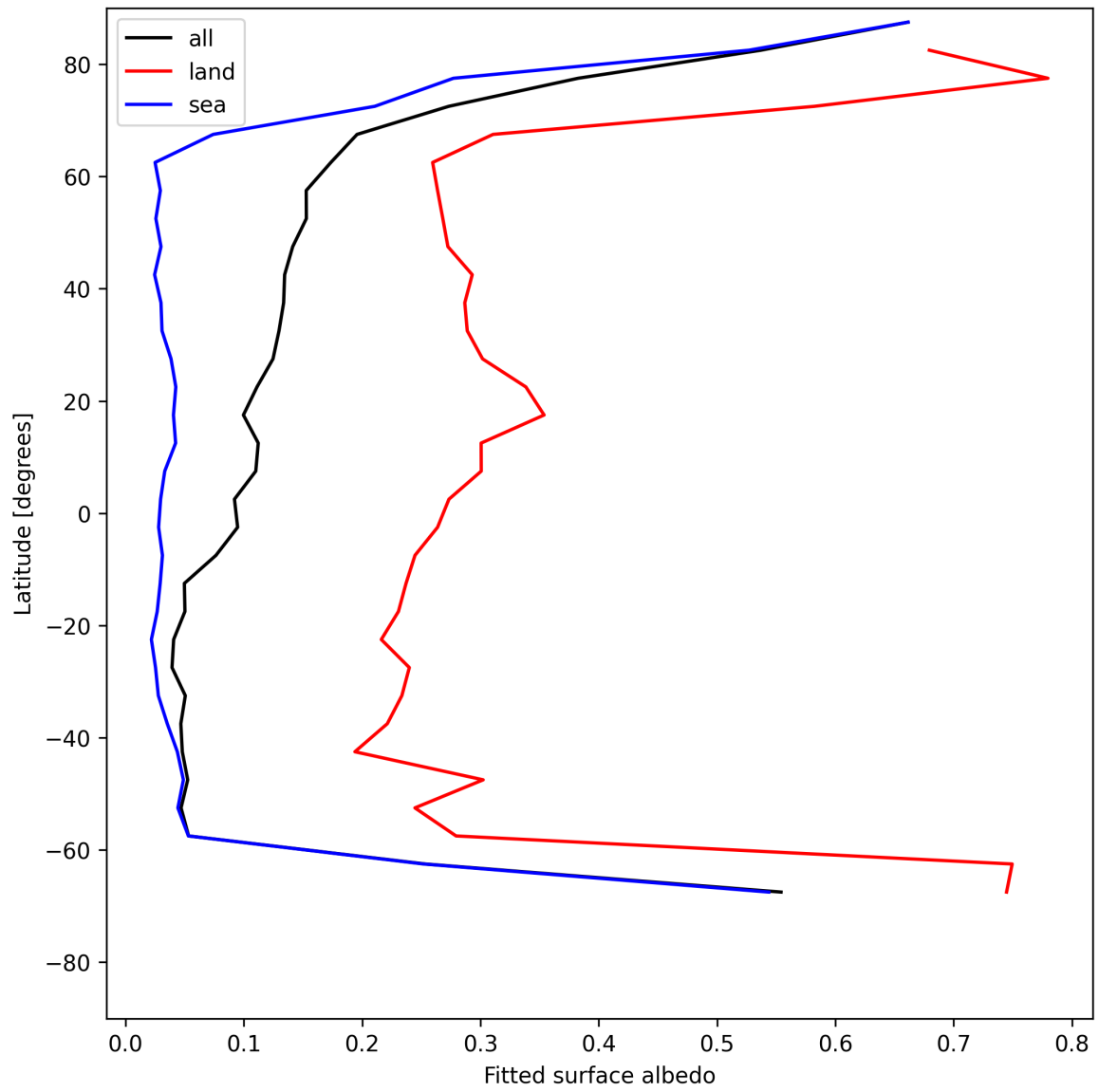
Figure 27: Zonal average of “Fitted surface albedo” for 2025-07-08 to 2025-07-09.
