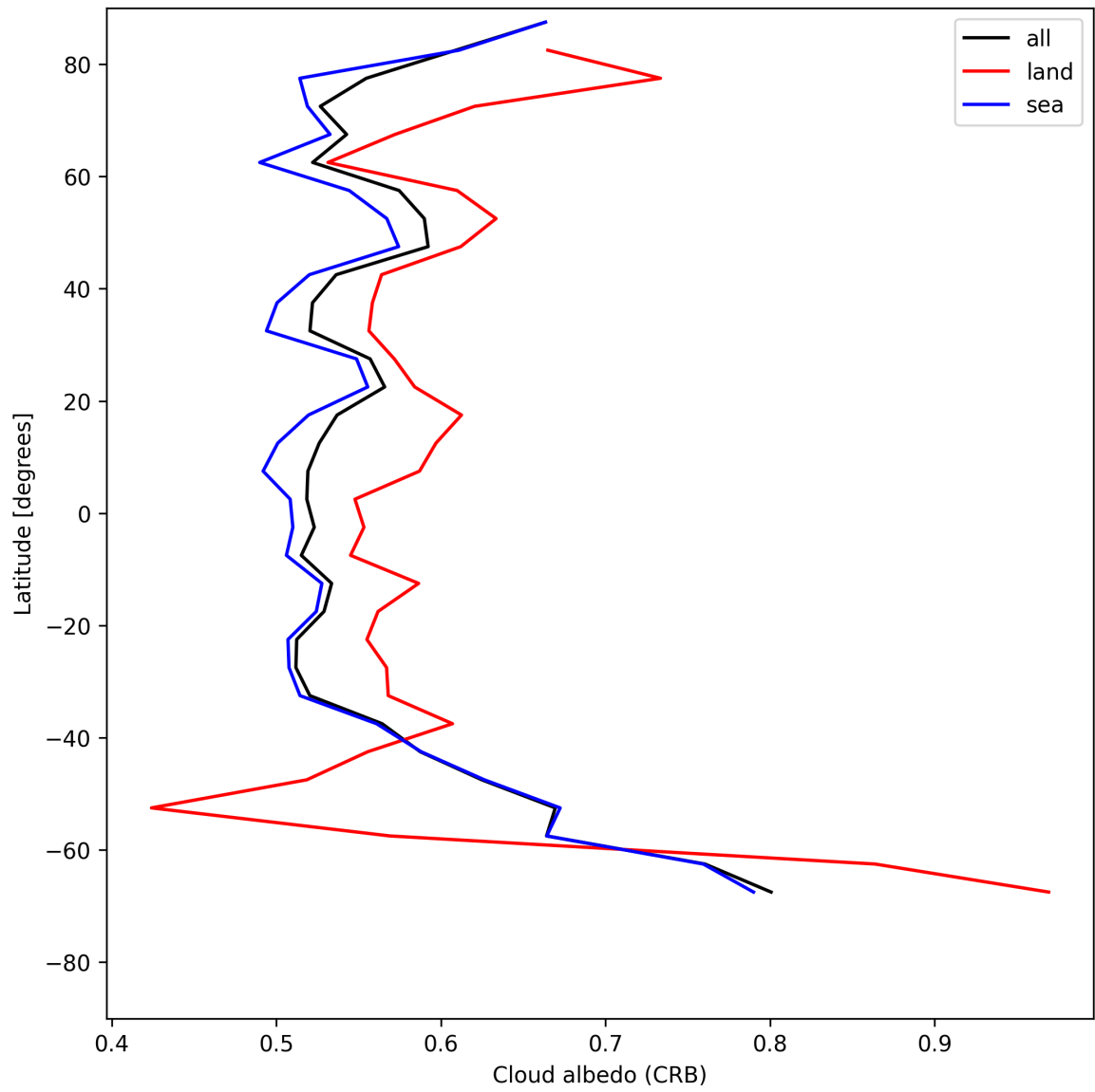
Figure 26: Zonal average of “Cloud albedo (CRB)” for 2025-07-08 to 2025-07-09.
