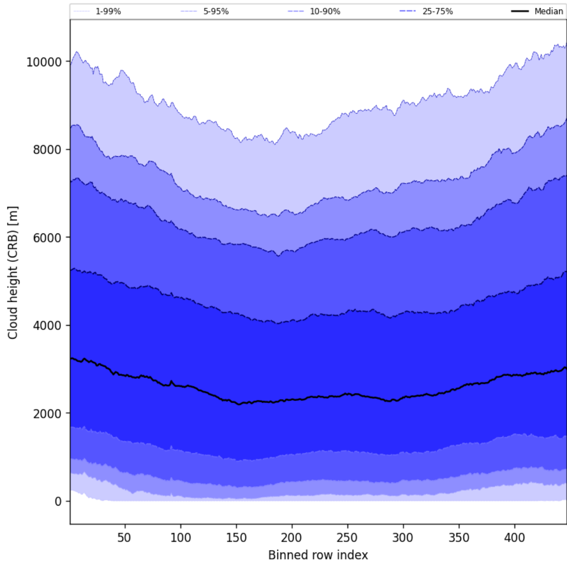
Figure 57: Along track statistics of “Cloud height (CRB)” for 2025-07-08 to 2025-07-09
