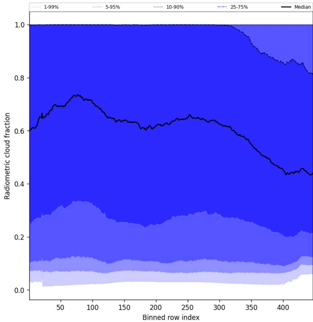
Figure 53: Along track statistics of “Radiometric cloud fraction” for 2025-07-08 to 2025-07-09
