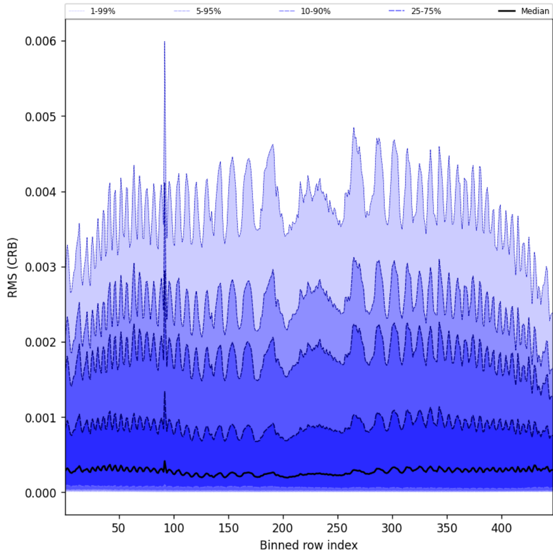
Figure 62: Along track statistics of “RMS (CRB)” for 2025-07-08 to 2025-07-09
