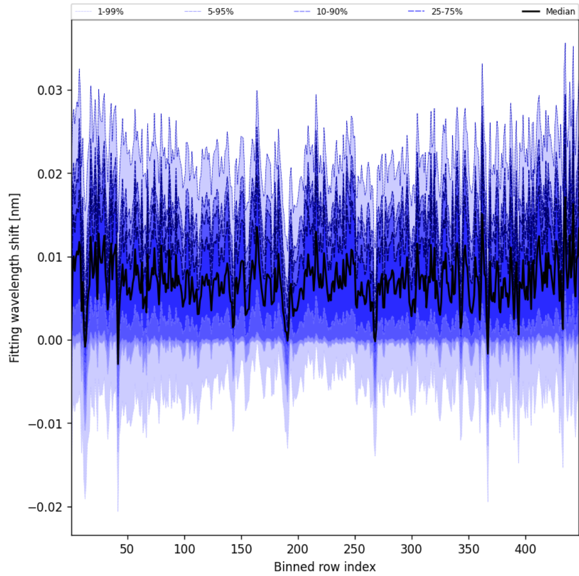
Figure 63: Along track statistics of “Fitting wavelength shift” for 2025-07-08 to 2025-07-09
