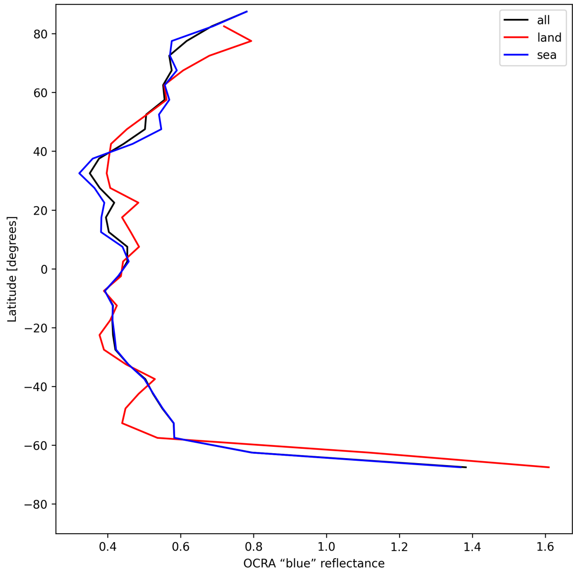
Figure 33: Zonal average of “OCRA “blue” reflectance” for 2025-07-08 to 2025-07-09.
