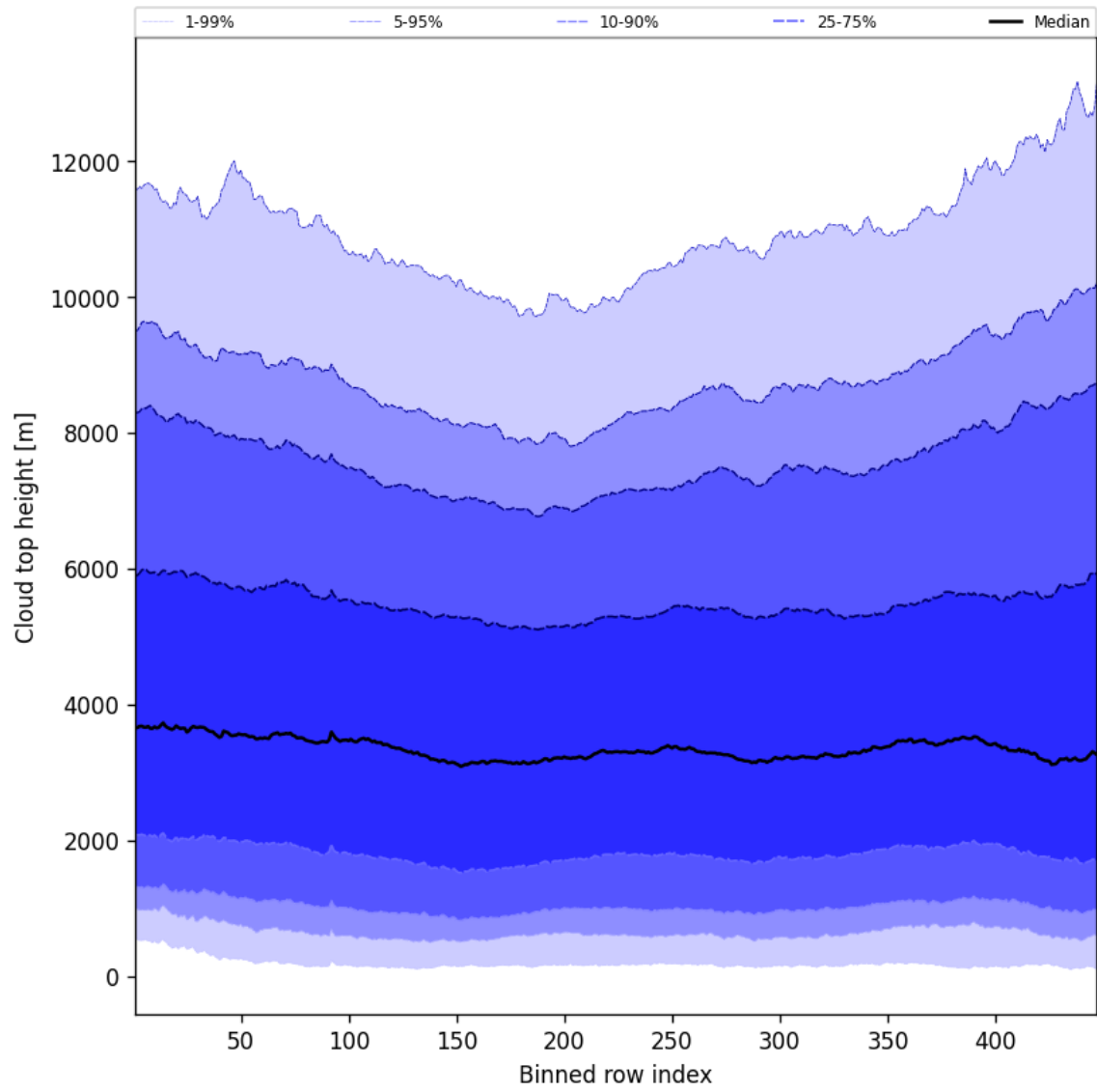
Figure 54: Along track statistics of “Cloud top height” for 2025-07-08 to 2025-07-09
