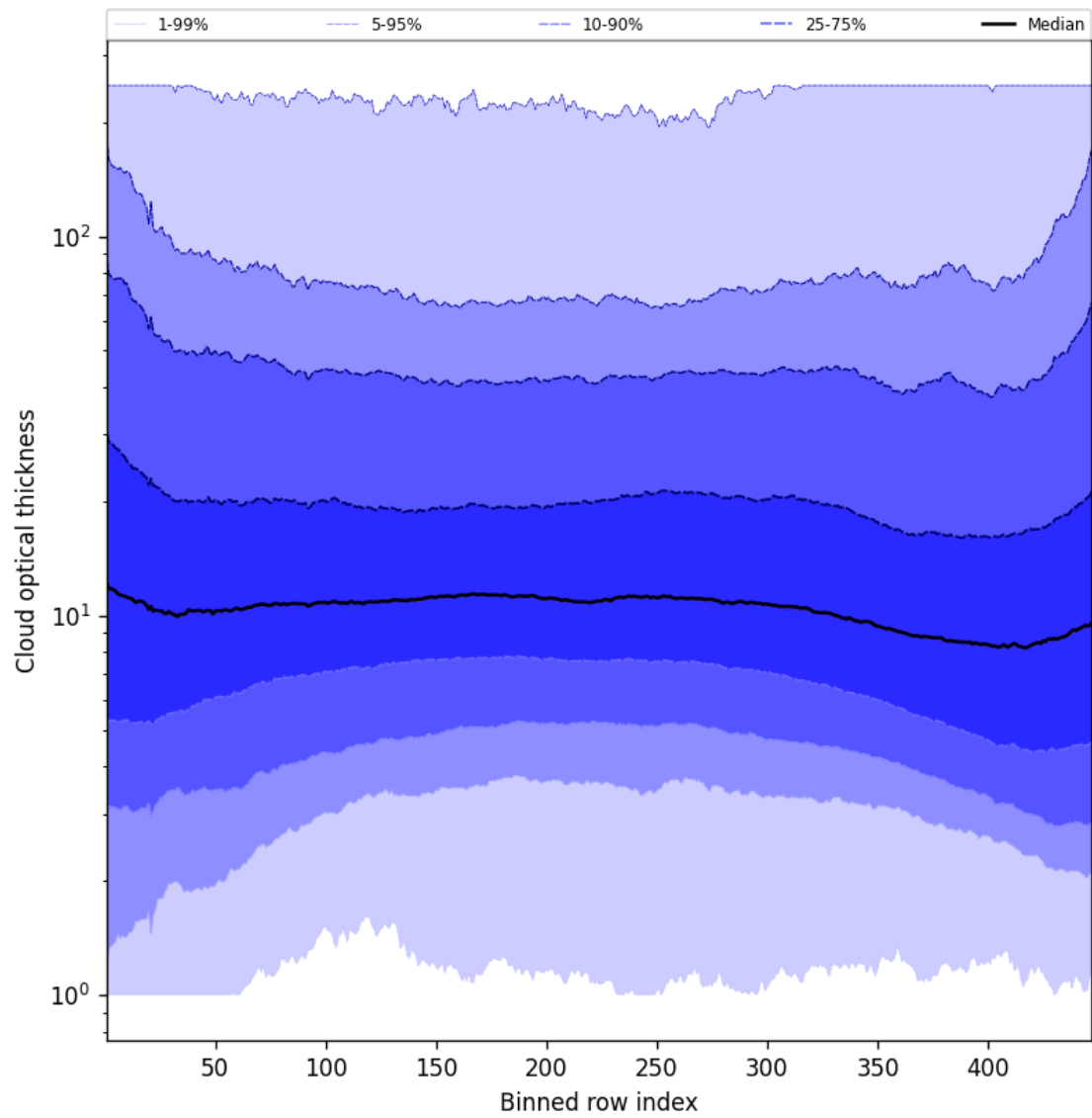
Figure 55: Along track statistics of “Cloud optical thickness” for 2025-07-08 to 2025-07-09
