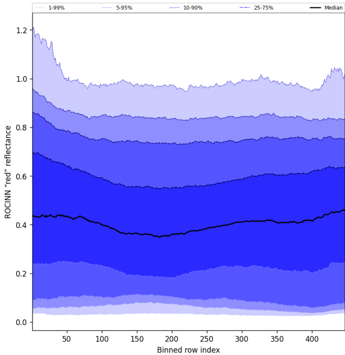
Figure 67: Along track statistics of "ROCINN "red" reflectance" for 2025-07-08 to 2025-07-09
