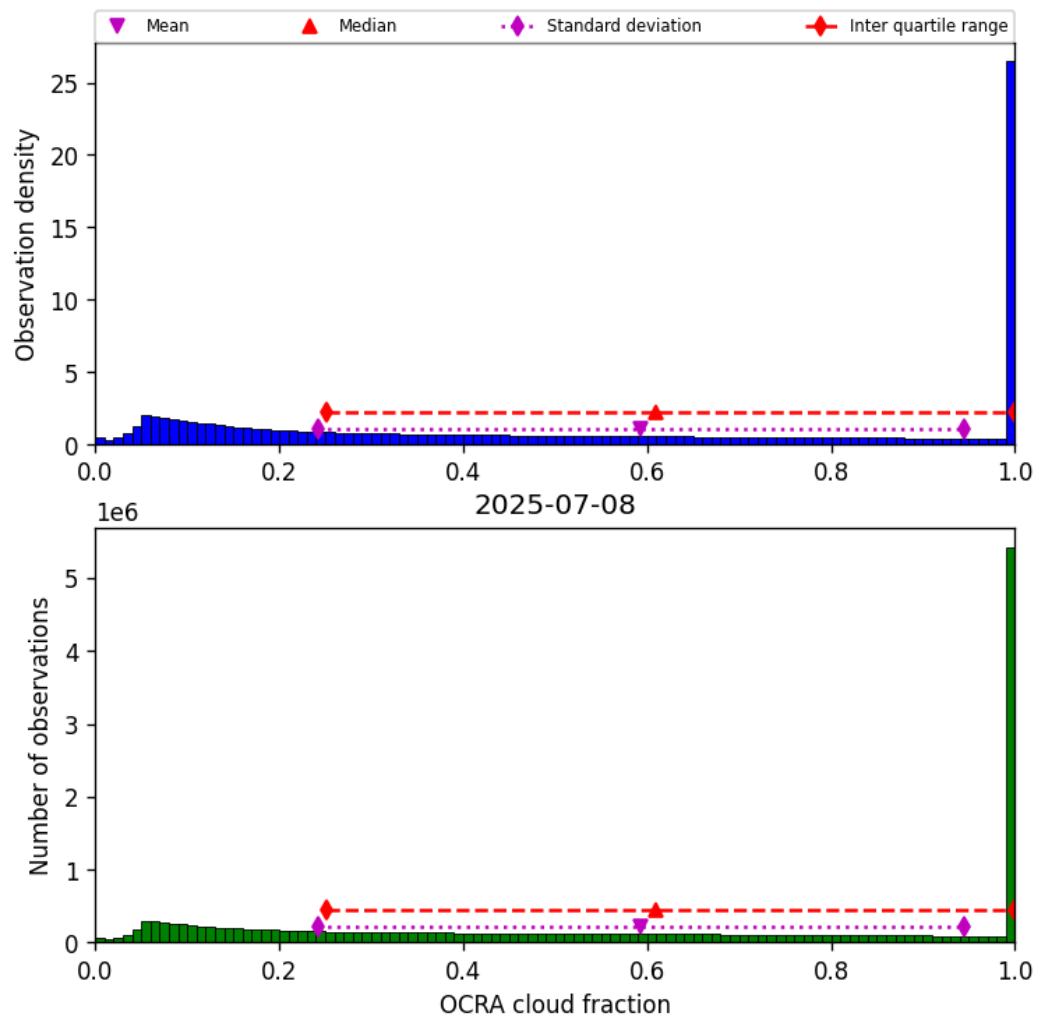
Figure 48: Histogram of “OCRA cloud fraction” for 2025-07-08 to 2025-07-09
