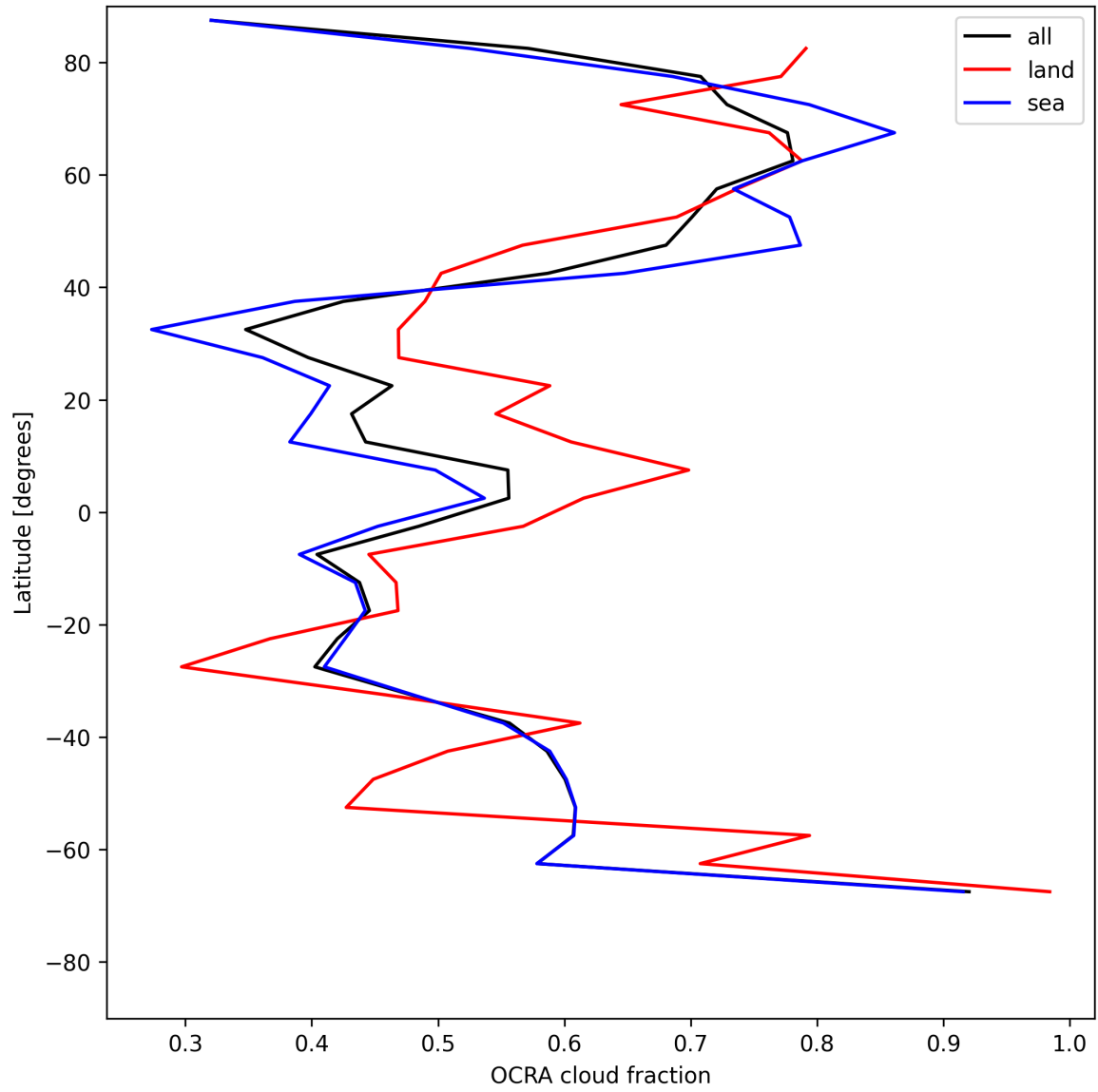
Figure 32: Zonal average of “OCRA cloud fraction” for 2025-07-08 to 2025-07-09.
