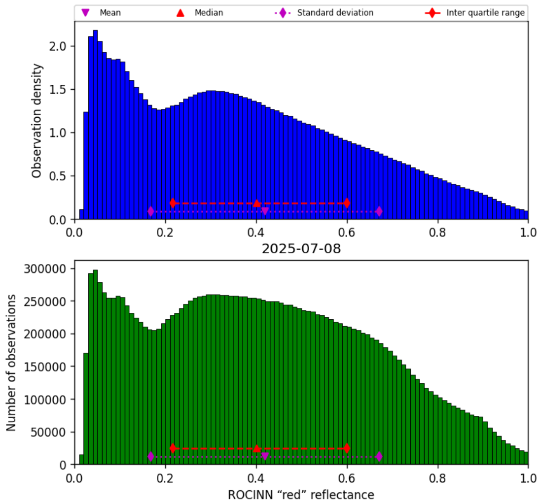
Figure 51: Histogram of “ROCINN “red” reflectance” for 2025-07-08 to 2025-07-09
