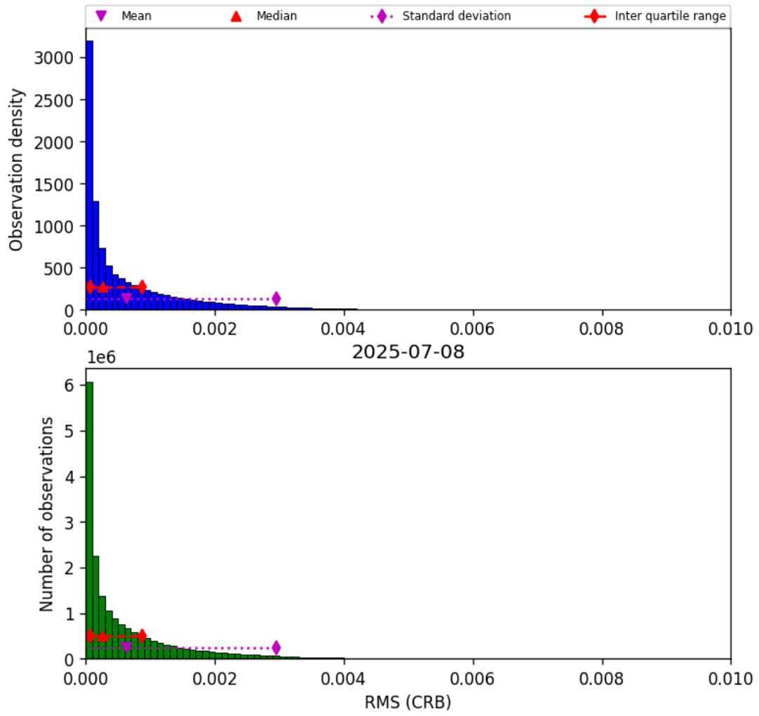
Figure 46: Histogram of “RMS (CRB)” for 2025-07-08 to 2025-07-09
