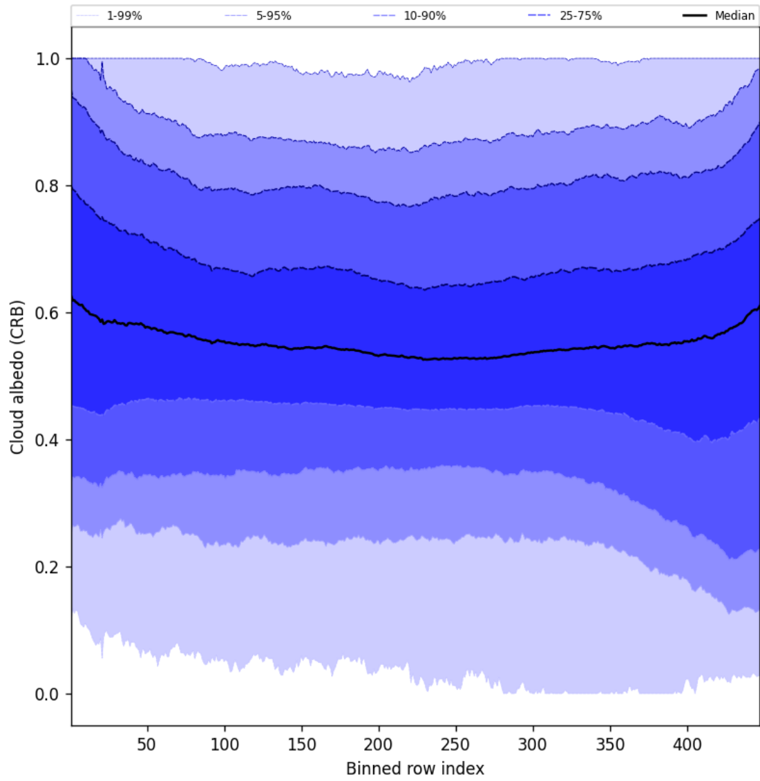
Figure 58: Along track statistics of “Cloud albedo (CRB)” for 2025-07-08 to 2025-07-09
