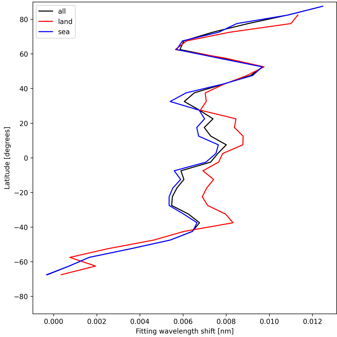
Figure 31: Zonal average of “Fitting wavelength shift” for 2025-07-08 to 2025-07-09.
