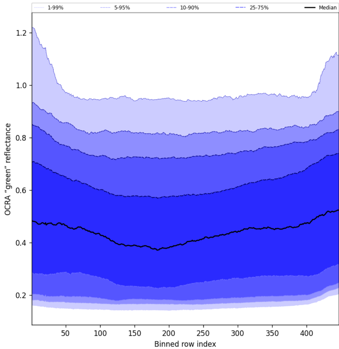
Figure 66: Along track statistics of "OCRA "green" reflectance" for 2025-07-08 to 2025-07-09
