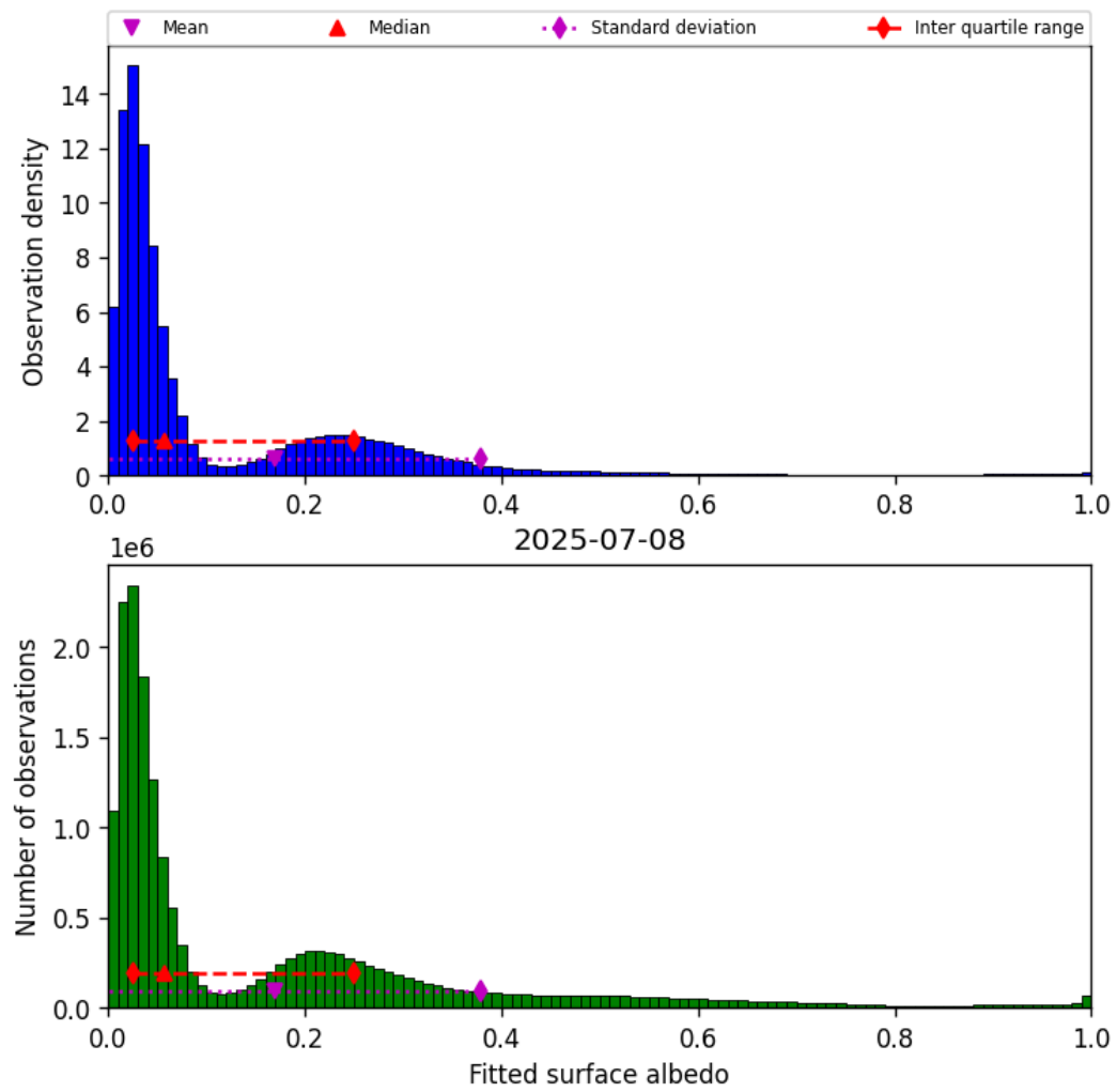
Figure 43: Histogram of “Fitted surface albedo” for 2025-07-08 to 2025-07-09
