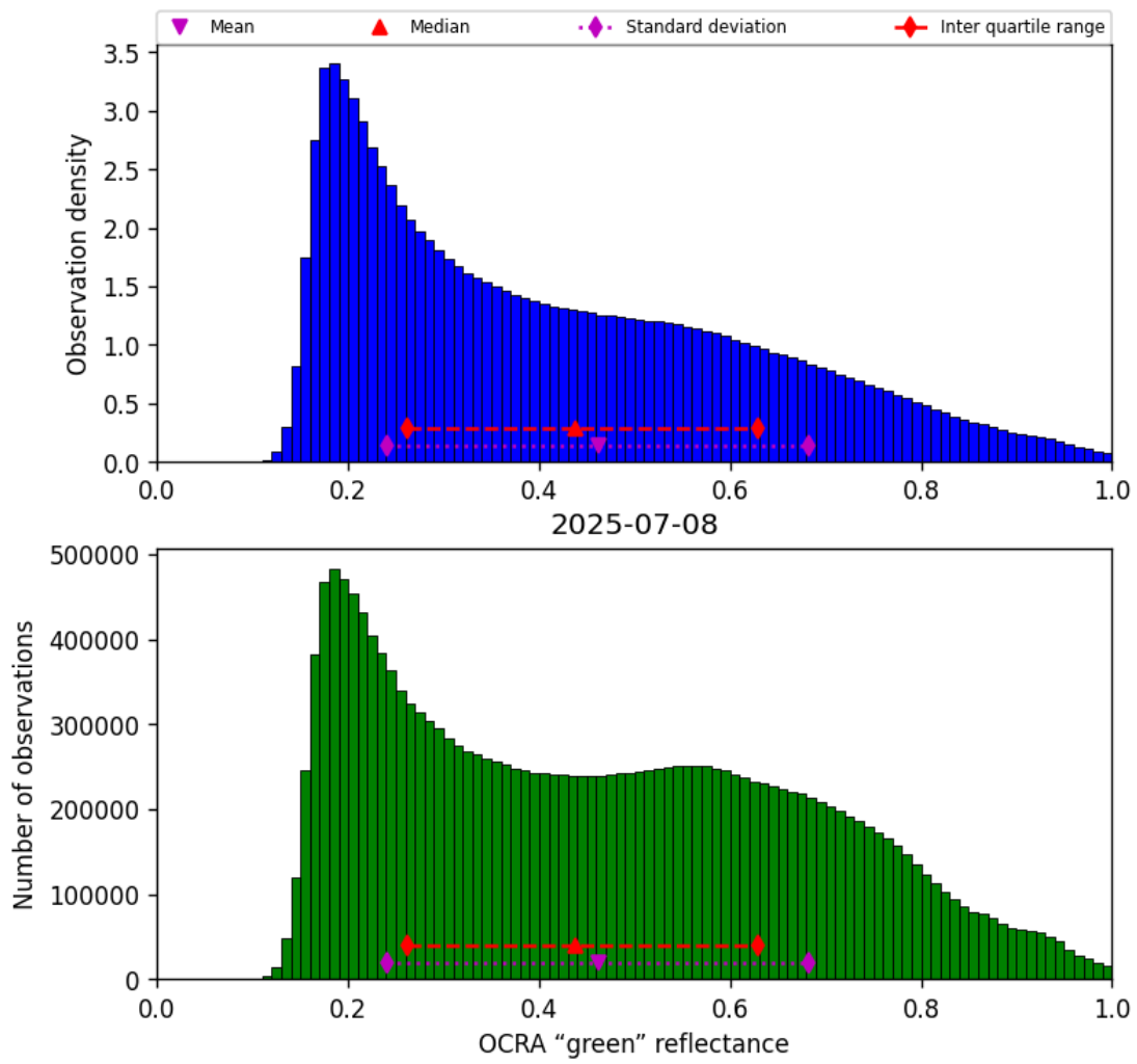
Figure 50: Histogram of “OCRA “green” reflectance” for 2025-07-08 to 2025-07-09
