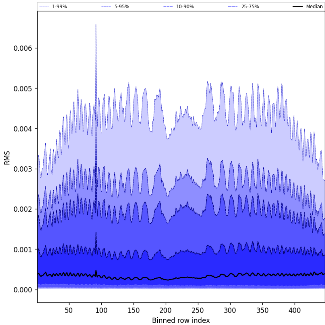
Figure 61: Along track statistics of “RMS” for 2025-07-08 to 2025-07-09
