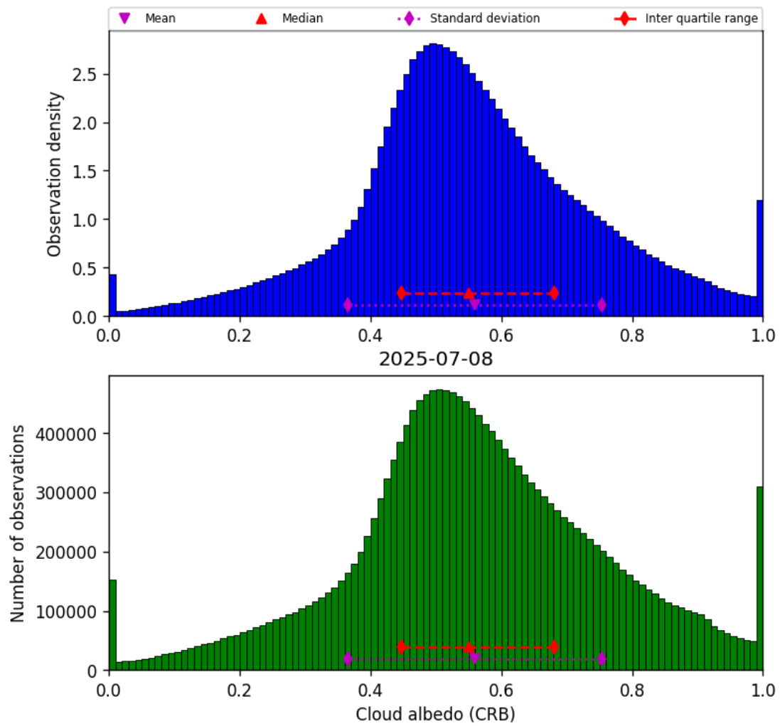
Figure 42: Histogram of “Cloud albedo (CRB)” for 2025-07-08 to 2025-07-09
