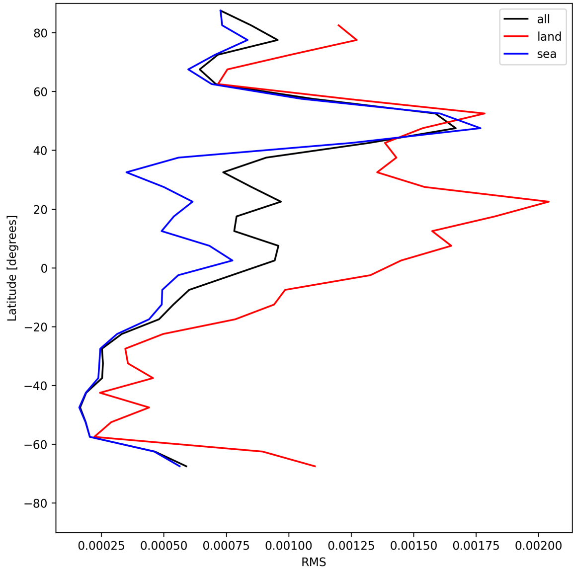
Figure 29: Zonal average of “RMS” for 2025-07-08 to 2025-07-09.
