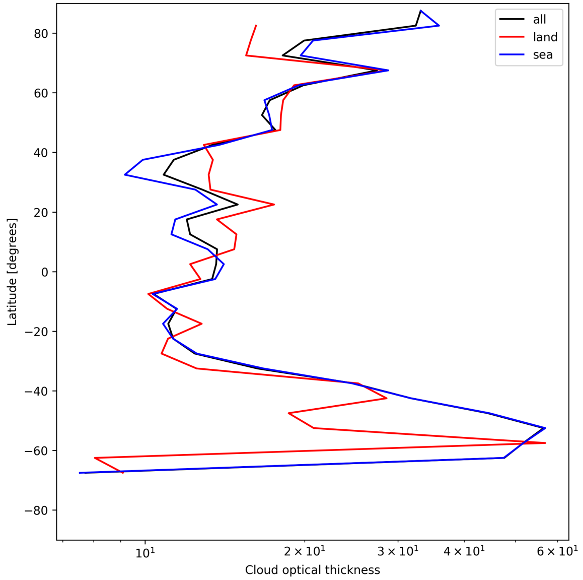
Figure 23: Zonal average of “Cloud optical thickness” for 2025-07-08 to 2025-07-09.
