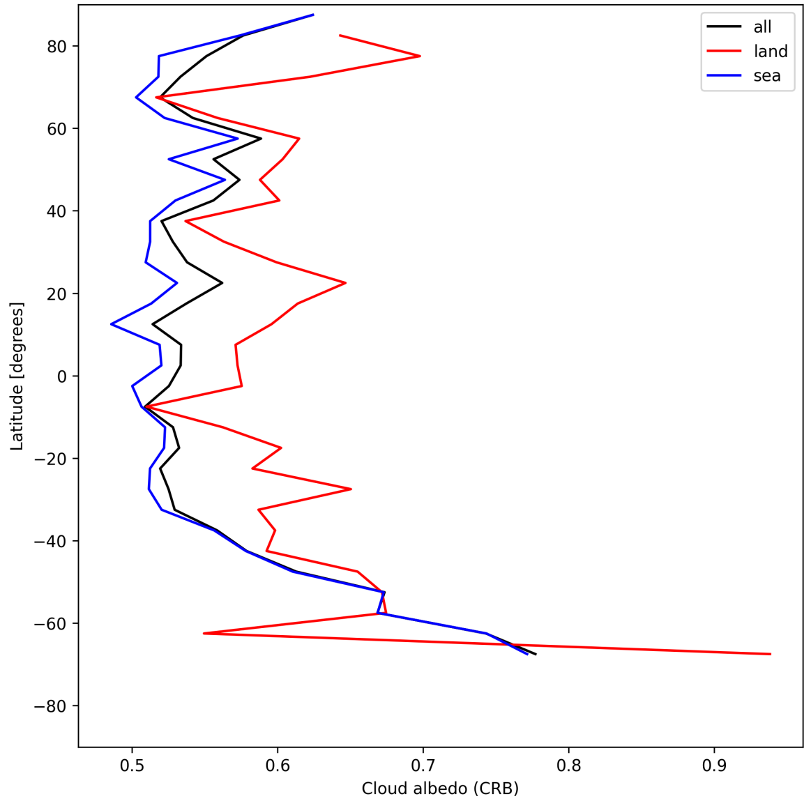
Figure 26: Zonal average of “Cloud albedo (CRB)” for 2025-07-10 to 2025-07-11.
