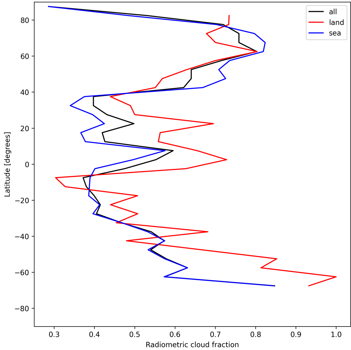
Figure 21: Zonal average of “Radiometric cloud fraction” for 2025-07-10 to 2025-07-11.
