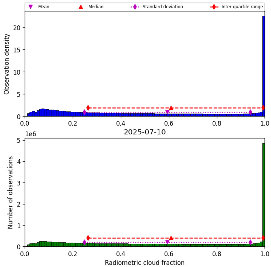
Figure 37: Histogram of “Radiometric cloud fraction” for 2025-07-10 to 2025-07-11
