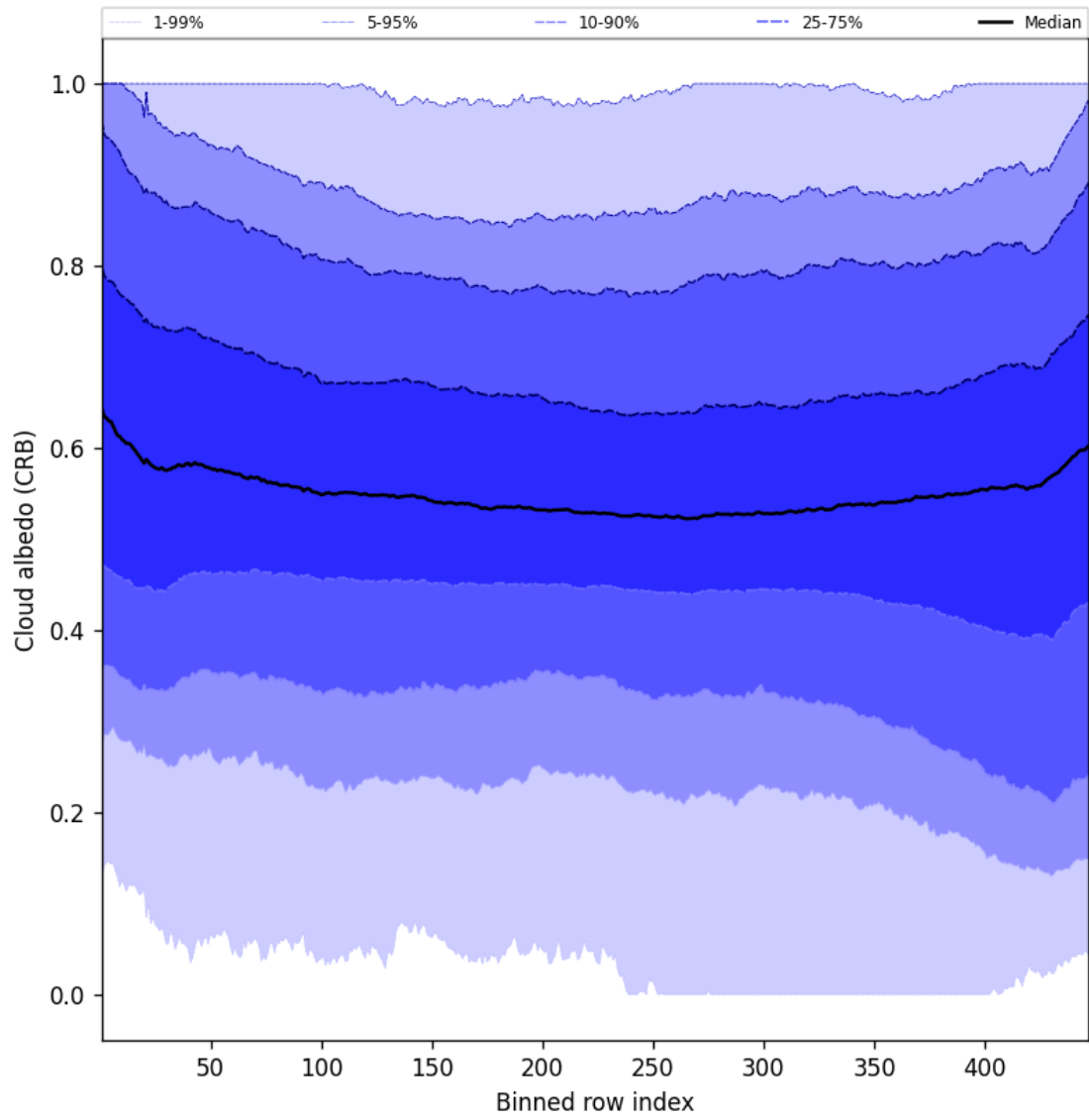
Figure 58: Along track statistics of “Cloud albedo (CRB)” for 2025-07-10 to 2025-07-11
