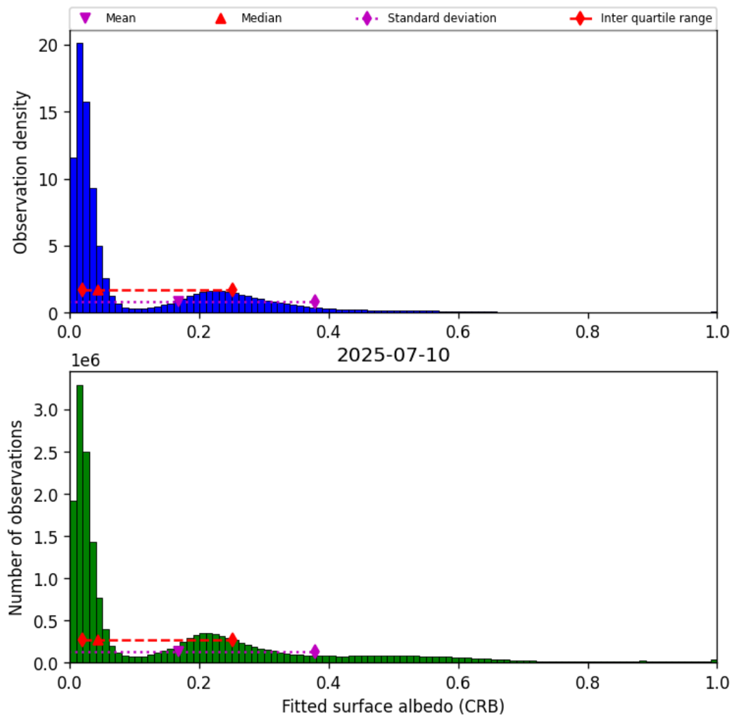
Figure 44: Histogram of “Fitted surface albedo (CRB)” for 2025-07-10 to 2025-07-11
