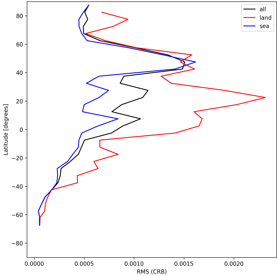
Figure 30: Zonal average of “RMS (CRB)” for 2025-07-10 to 2025-07-11.
