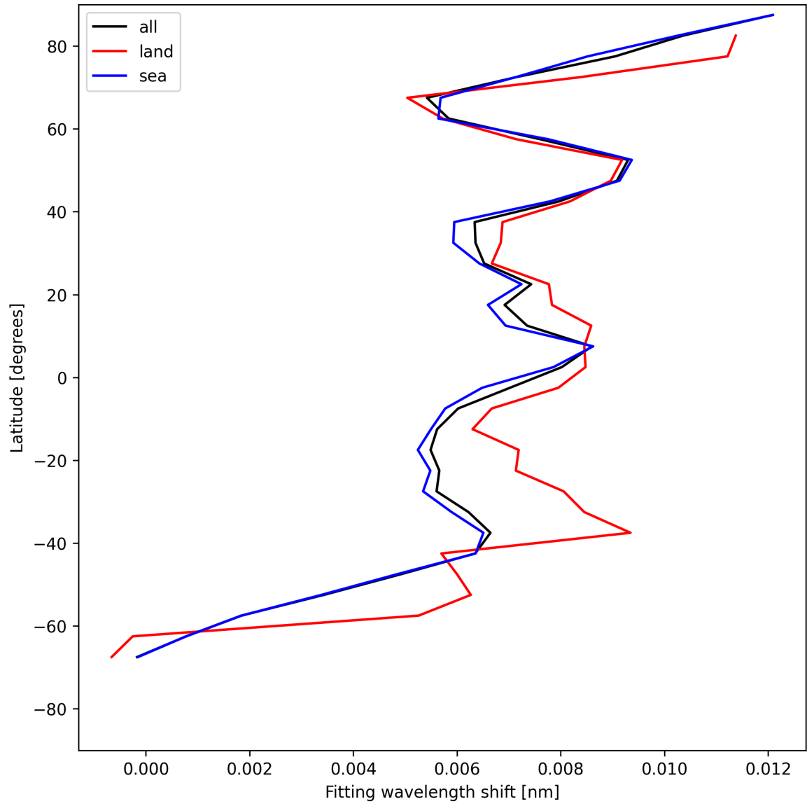
Figure 31: Zonal average of “Fitting wavelength shift” for 2025-07-10 to 2025-07-11.
