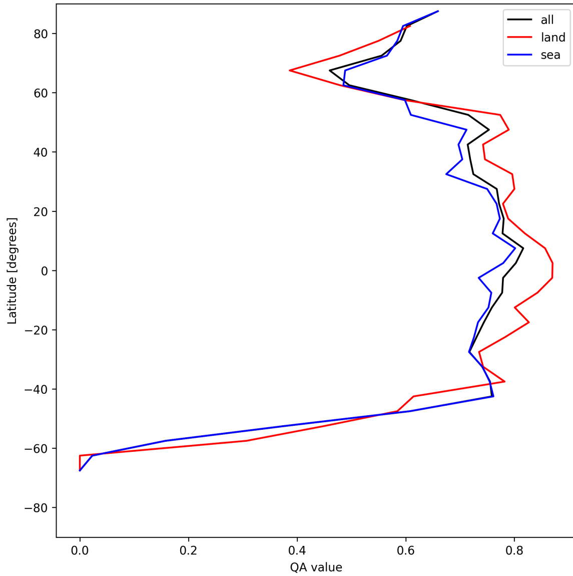
Figure 20: Zonal average of “QA value” for 2025-07-10 to 2025-07-11.
