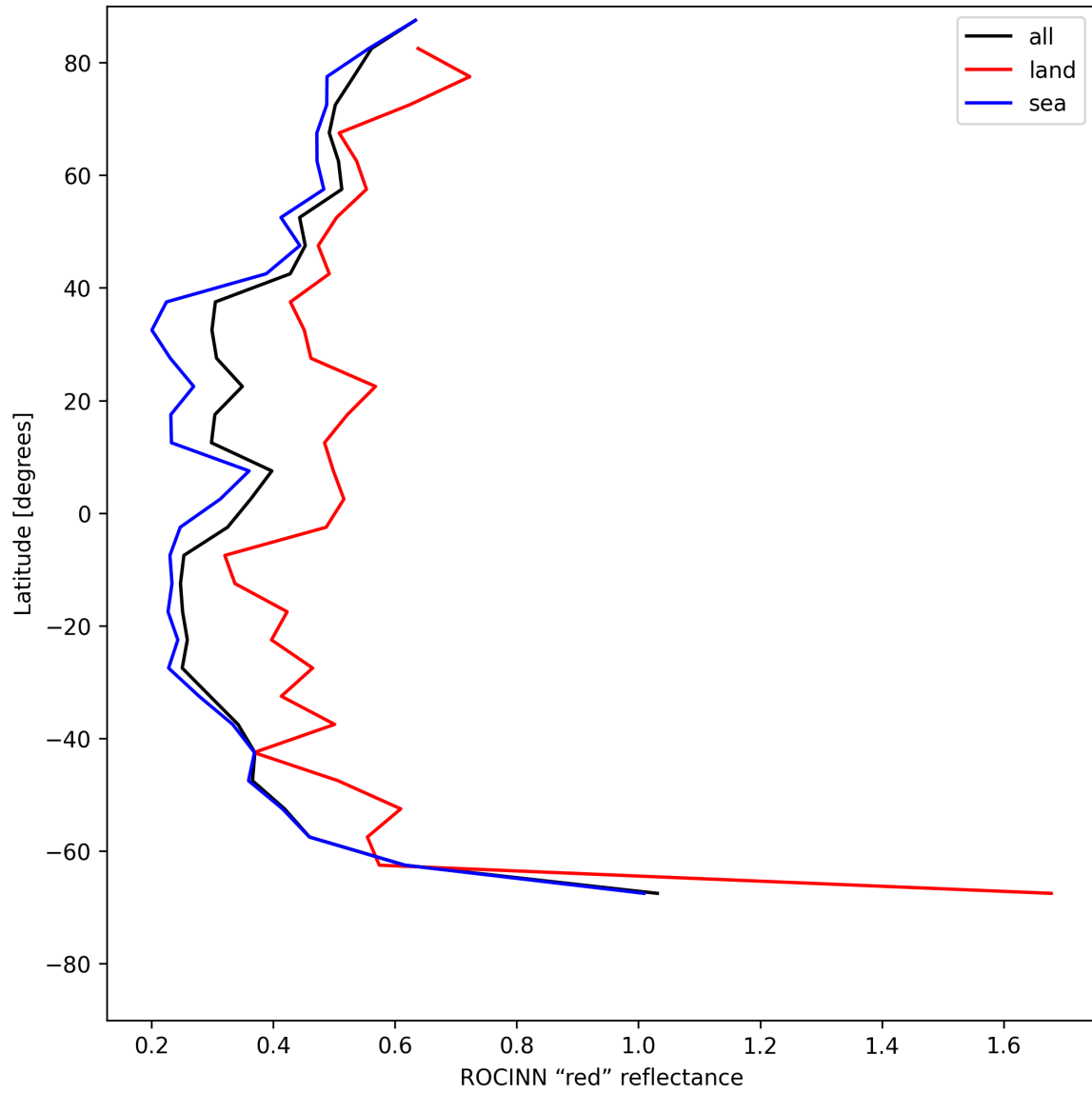
Figure 35: Zonal average of “ROCINN “red” reflectance” for 2025-07-10 to 2025-07-11.
