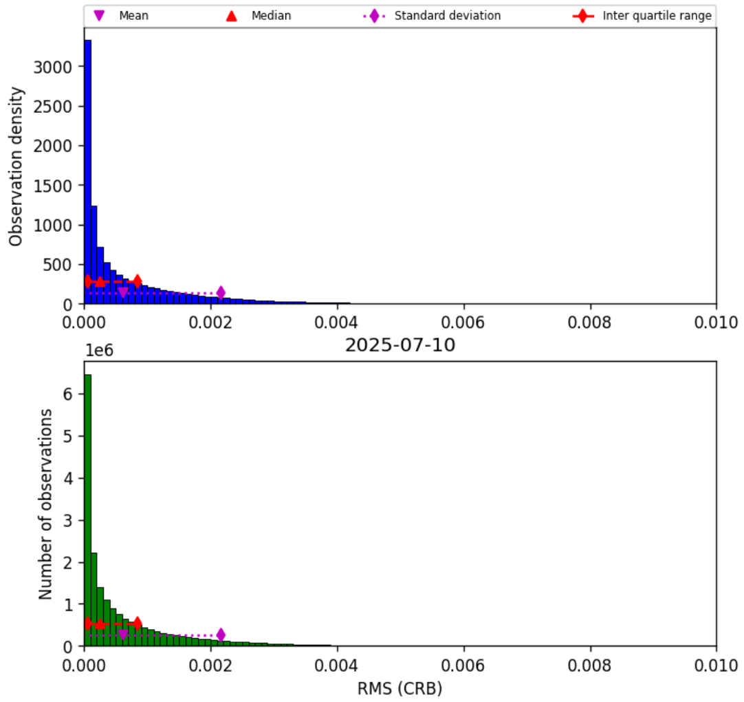
Figure 46: Histogram of “RMS (CRB)” for 2025-07-10 to 2025-07-11
