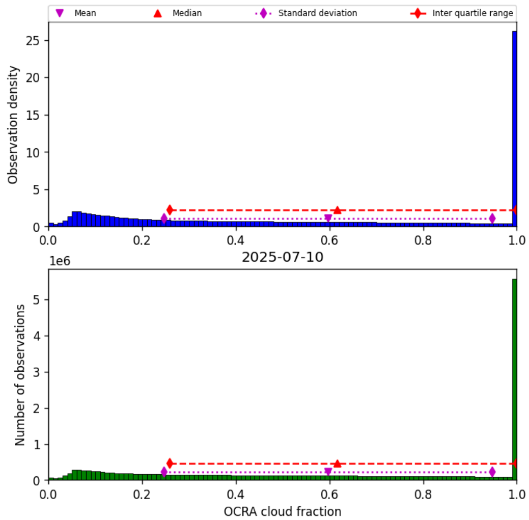
Figure 48: Histogram of “OCRA cloud fraction” for 2025-07-10 to 2025-07-11
