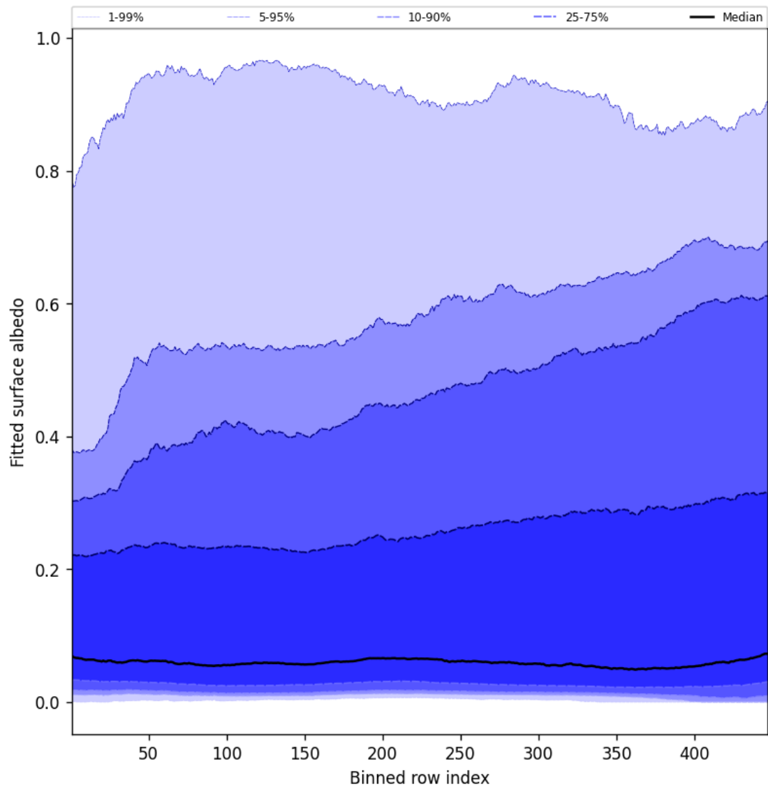
Figure 59: Along track statistics of “Fitted surface albedo” for 2025-07-10 to 2025-07-11
