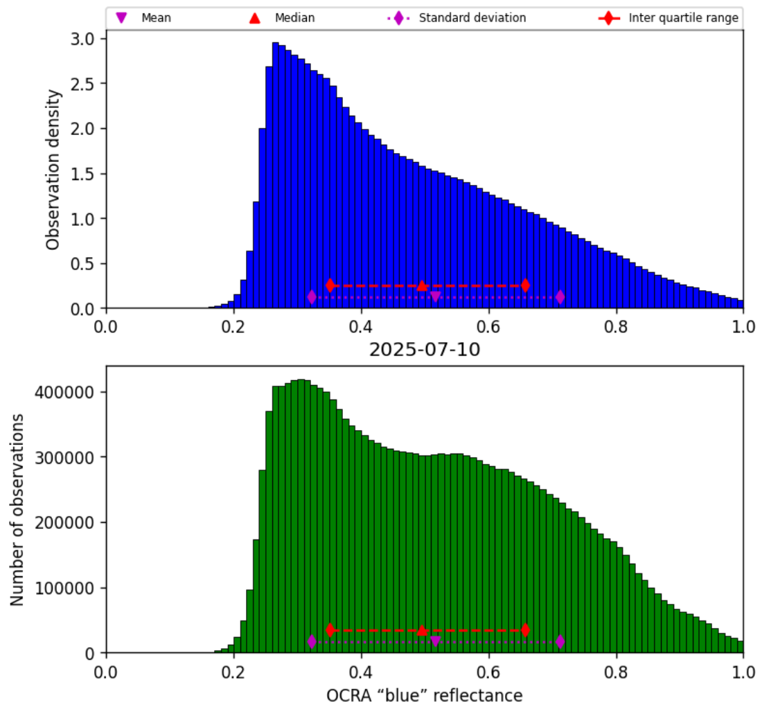
Figure 49: Histogram of “OCRA “blue” reflectance” for 2025-07-10 to 2025-07-11
