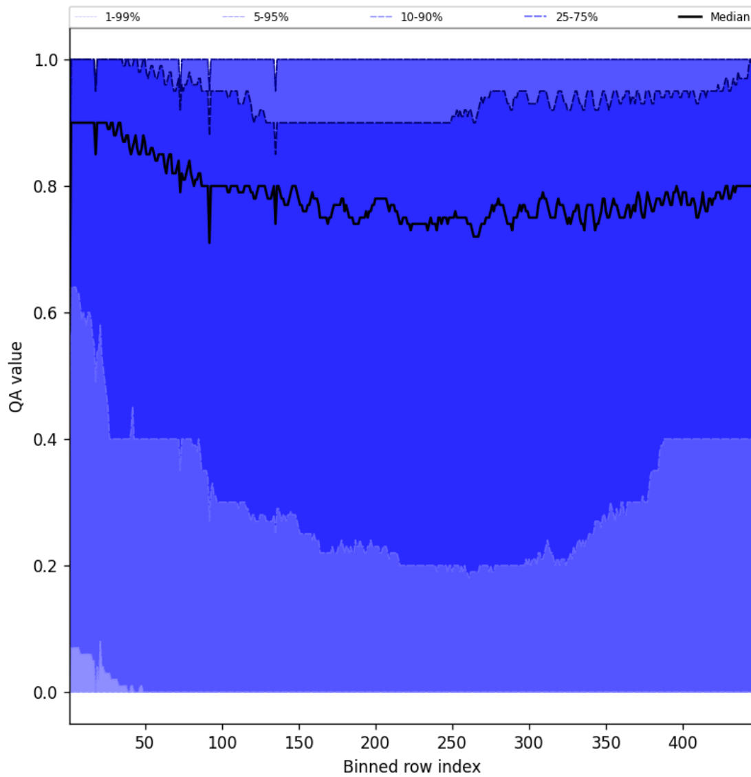
Figure 52: Along track statistics of “QA value” for 2025-07-10 to 2025-07-11
