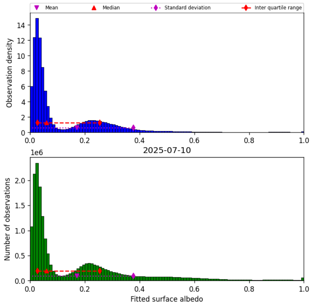
Figure 43: Histogram of “Fitted surface albedo” for 2025-07-10 to 2025-07-11
