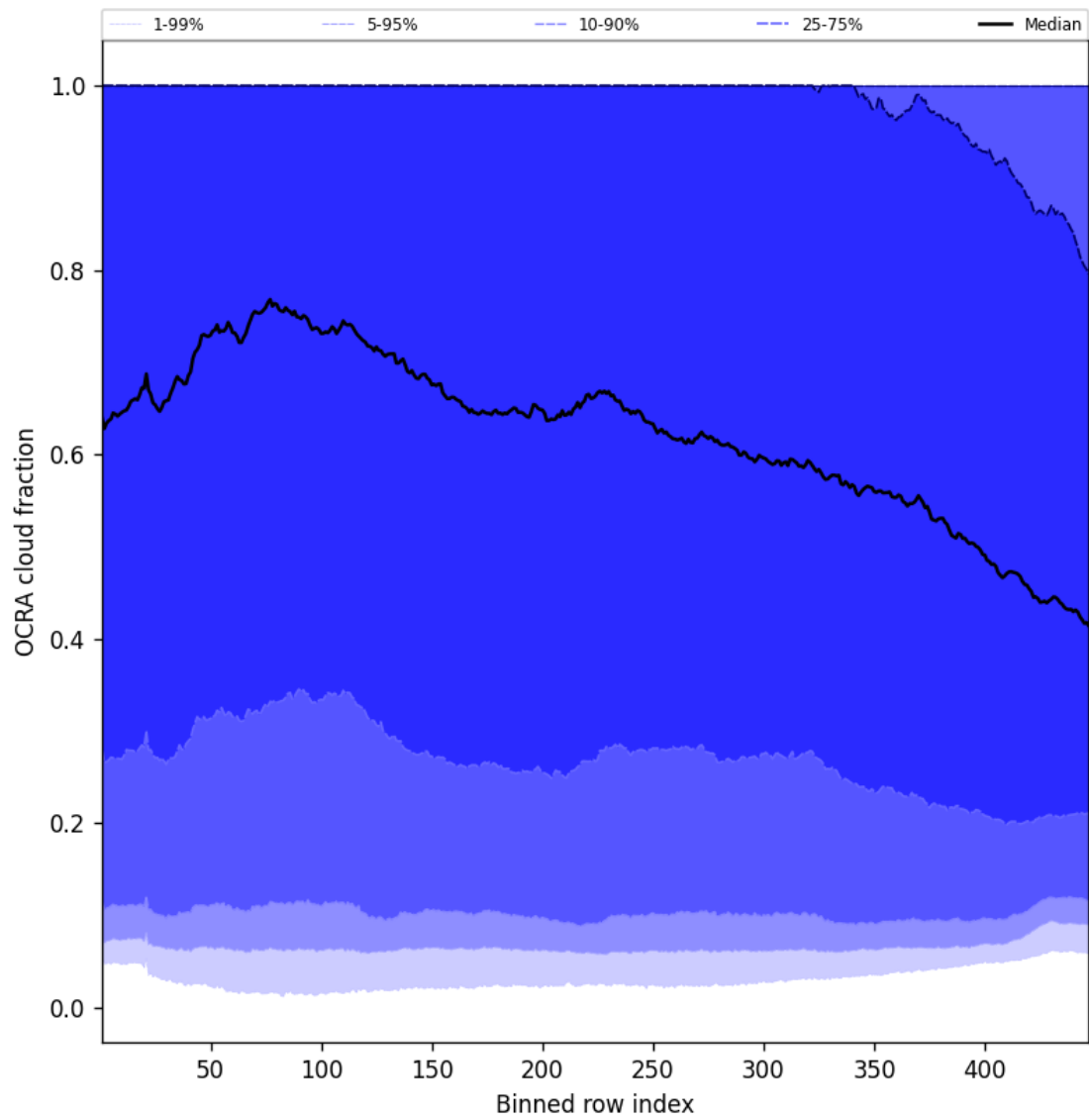
Figure 64: Along track statistics of “OCRA cloud fraction” for 2025-07-10 to 2025-07-11
