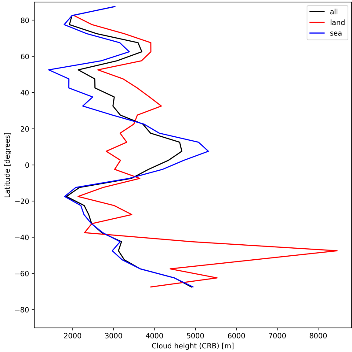
Figure 25: Zonal average of “Cloud height (CRB)” for 2025-07-10 to 2025-07-11.
