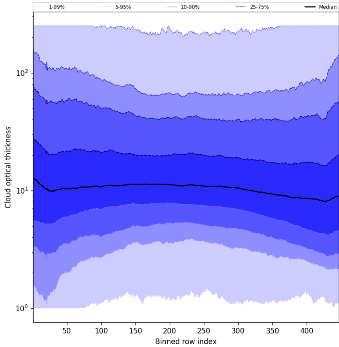
Figure 55: Along track statistics of “Cloud optical thickness” for 2025-07-10 to 2025-07-11
