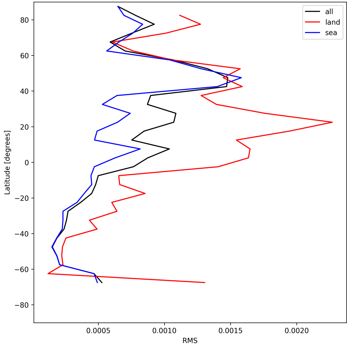
Figure 29: Zonal average of “RMS” for 2025-07-10 to 2025-07-11.
