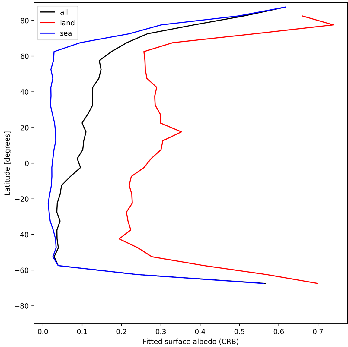
Figure 28: Zonal average of “Fitted surface albedo (CRB)” for 2025-07-10 to 2025-07-11.
