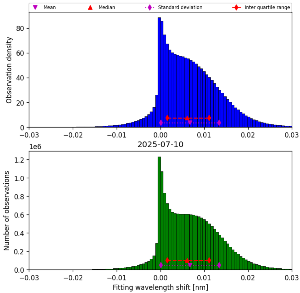
Figure 47: Histogram of “Fitting wavelength shift” for 2025-07-10 to 2025-07-11
