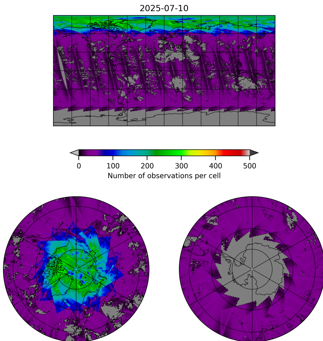
Figure 19: Map of the number of observations for 2025-07-10 to 2025-07-11
