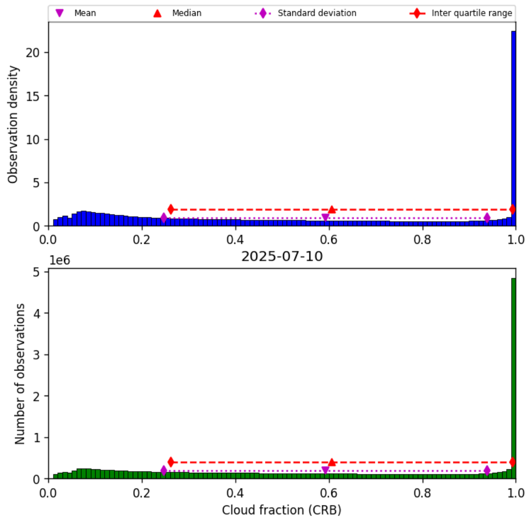
Figure 40: Histogram of “Cloud fraction (CRB)” for 2025-07-10 to 2025-07-11
