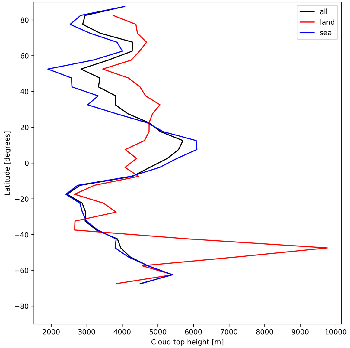
Figure 22: Zonal average of “Cloud top height” for 2025-07-10 to 2025-07-11.
