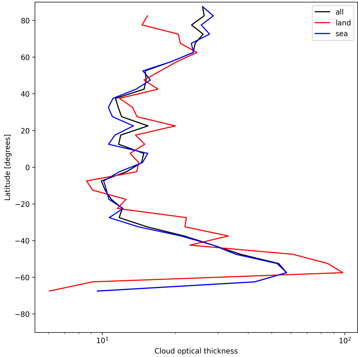
Figure 23: Zonal average of “Cloud optical thickness” for 2025-07-10 to 2025-07-11.
