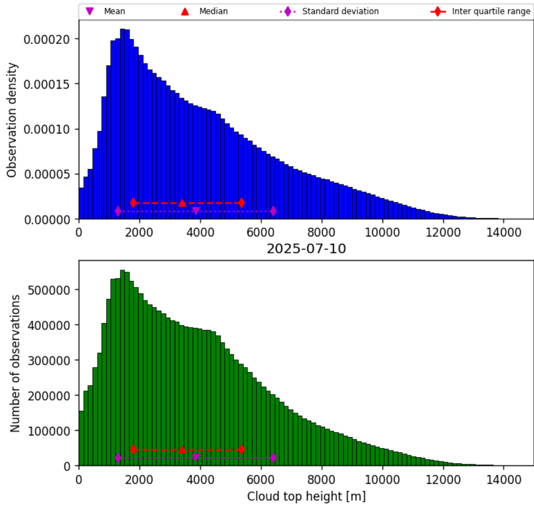
Figure 38: Histogram of “Cloud top height” for 2025-07-10 to 2025-07-11
