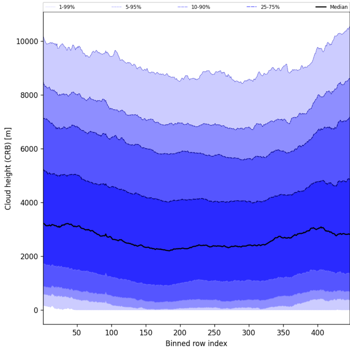
Figure 57: Along track statistics of “Cloud height (CRB)” for 2025-07-10 to 2025-07-11
