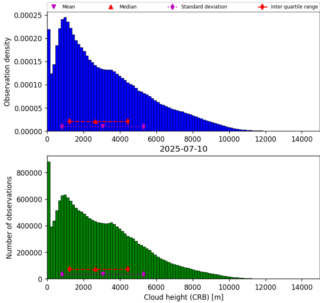
Figure 41: Histogram of “Cloud height (CRB)” for 2025-07-10 to 2025-07-11
