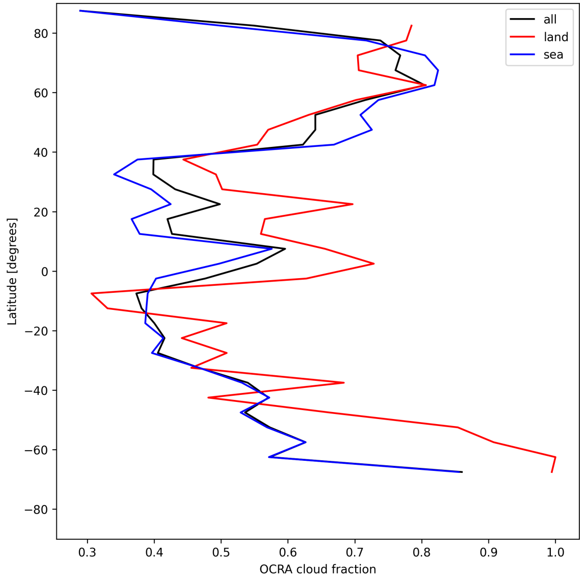
Figure 32: Zonal average of “OCRA cloud fraction” for 2025-07-10 to 2025-07-11.
