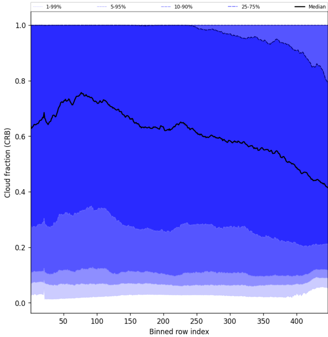
Figure 56: Along track statistics of “Cloud fraction (CRB)” for 2025-07-10 to 2025-07-11
