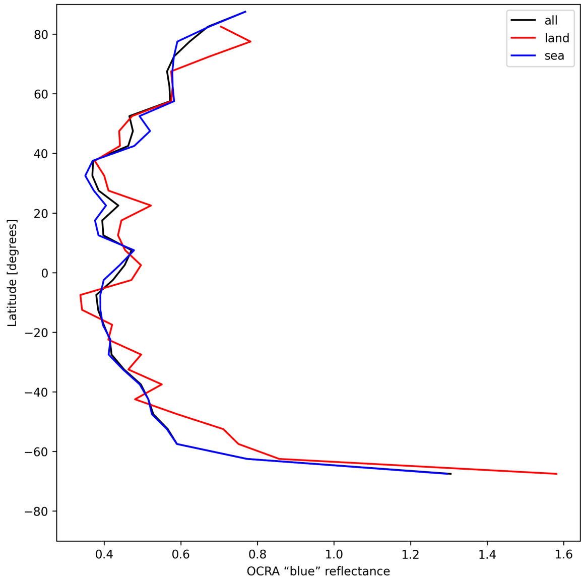
Figure 33: Zonal average of “OCRA “blue” reflectance” for 2025-07-10 to 2025-07-11.
