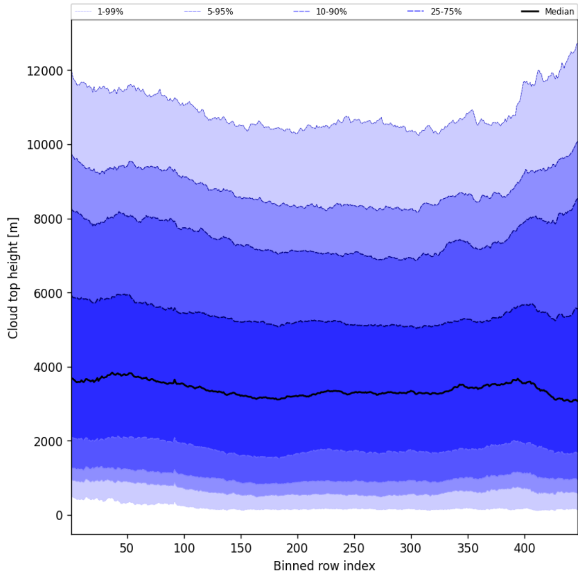
Figure 54: Along track statistics of “Cloud top height” for 2025-07-10 to 2025-07-11
