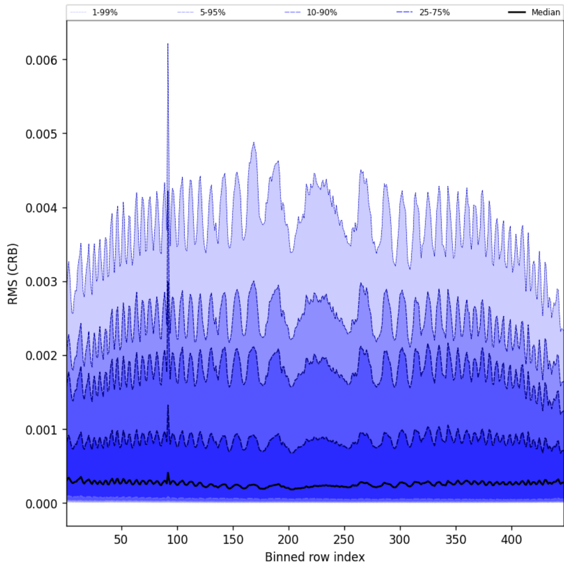
Figure 62: Along track statistics of “RMS (CRB)” for 2025-07-10 to 2025-07-11
