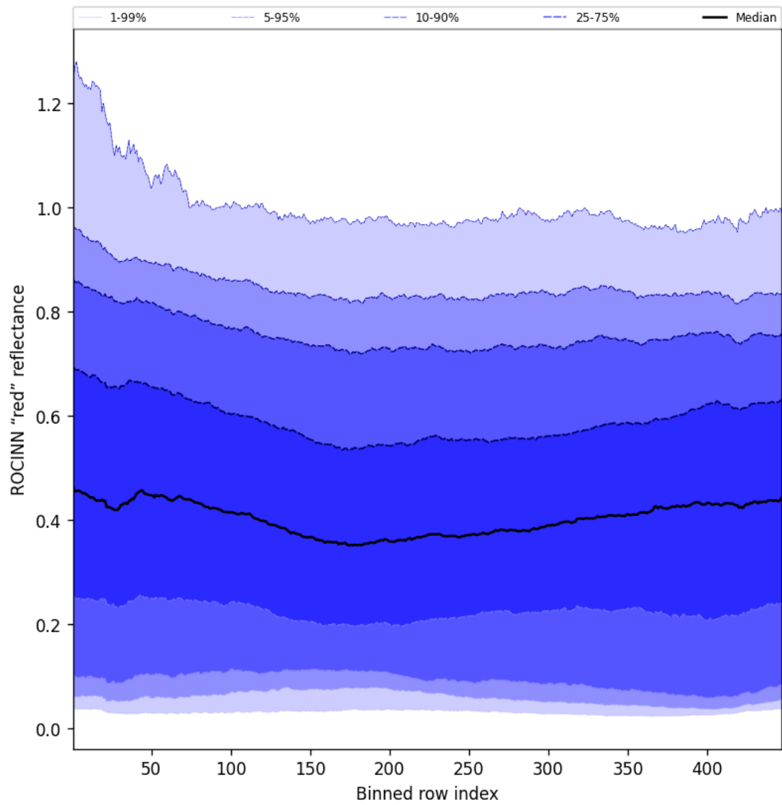
Figure 67: Along track statistics of "ROCINN "red" reflectance" for 2025-07-10 to 2025-07-11
