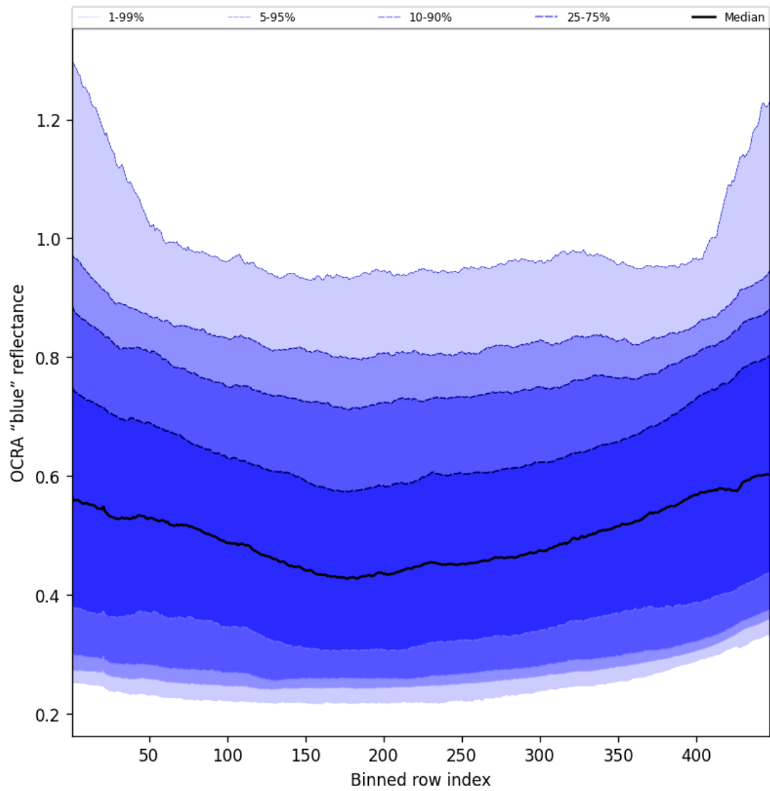
Figure 65: Along track statistics of “OCRA “blue” reflectance” for 2025-07-10 to 2025-07-11
