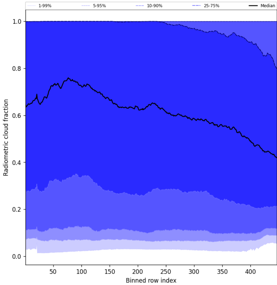
Figure 53: Along track statistics of “Radiometric cloud fraction” for 2025-07-10 to 2025-07-11
