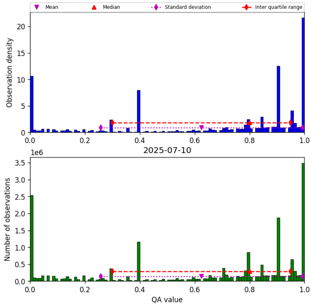
Figure 36: Histogram of “QA value” for 2025-07-10 to 2025-07-11
