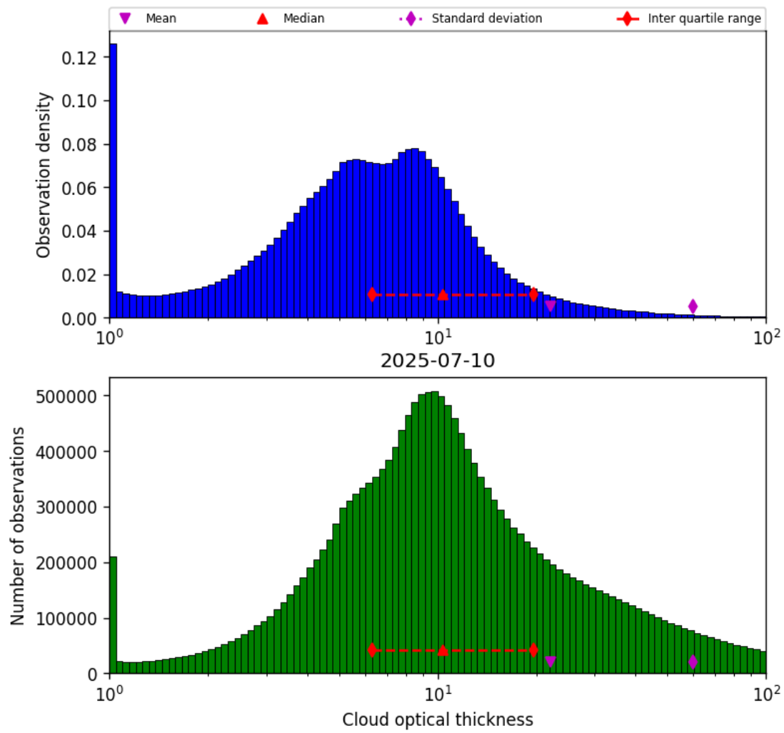
Figure 39: Histogram of “Cloud optical thickness” for 2025-07-10 to 2025-07-11
