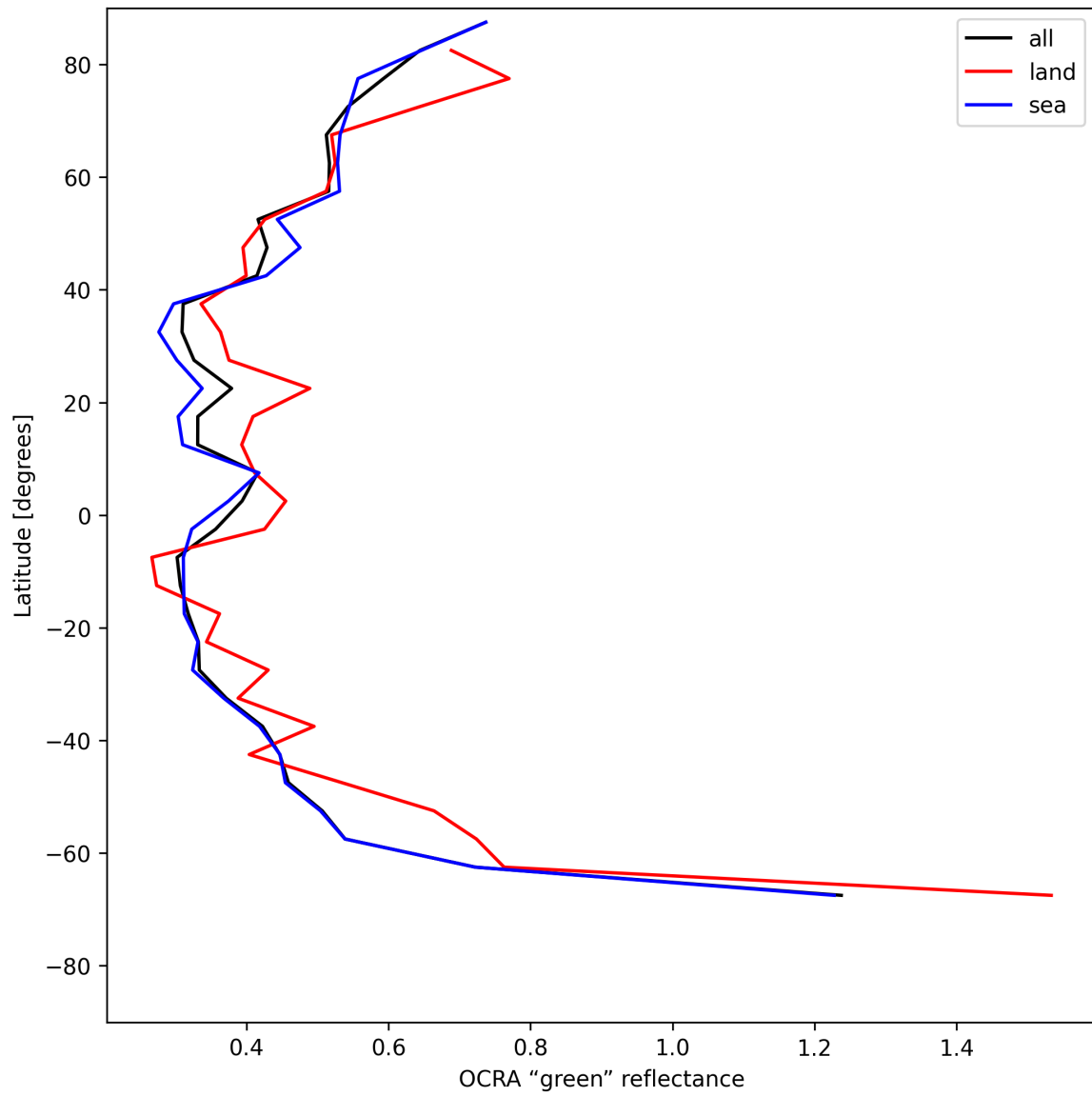
Figure 34: Zonal average of “OCRA “green” reflectance” for 2025-07-10 to 2025-07-11.
