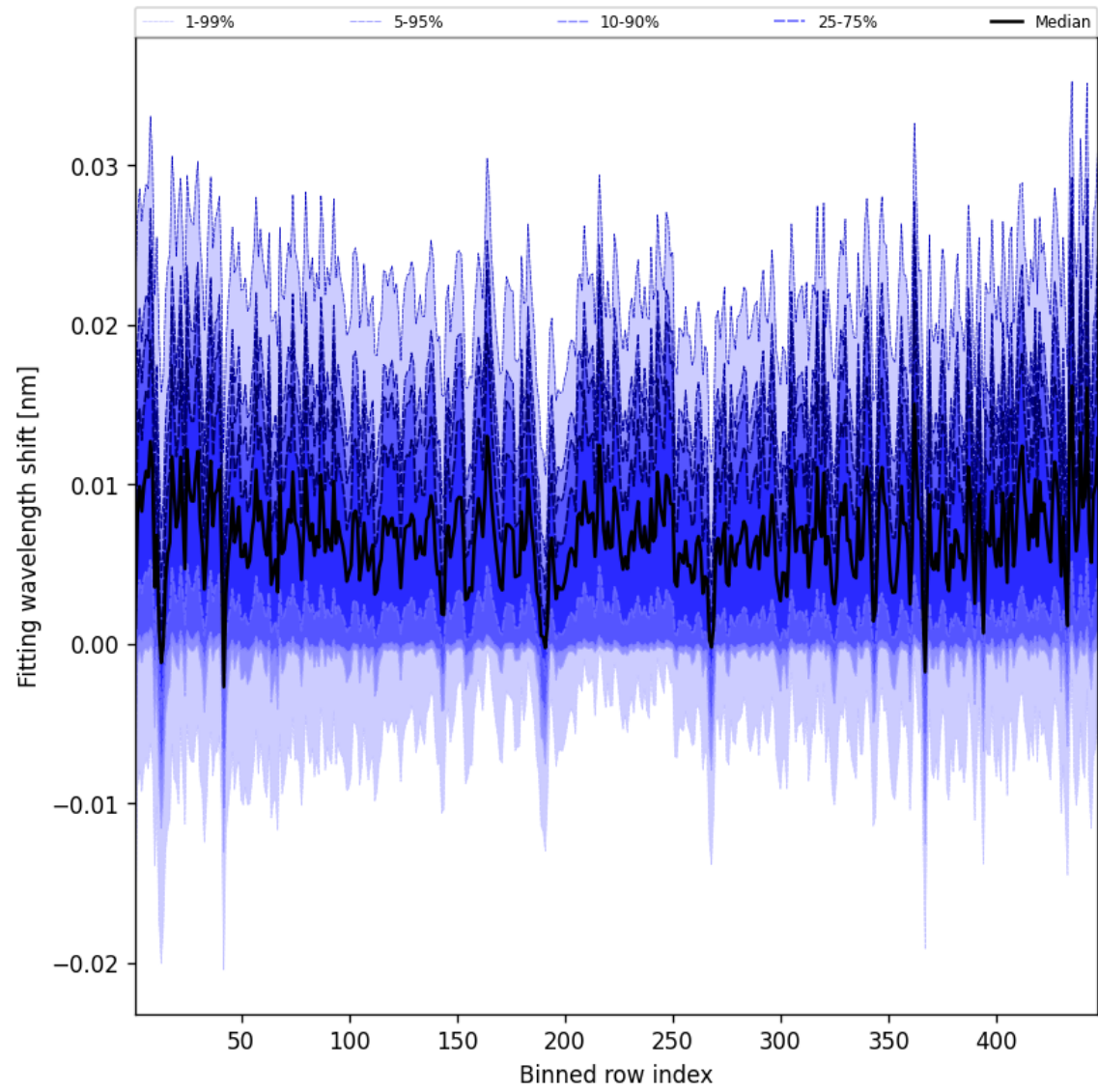
Figure 63: Along track statistics of “Fitting wavelength shift” for 2025-07-10 to 2025-07-11
