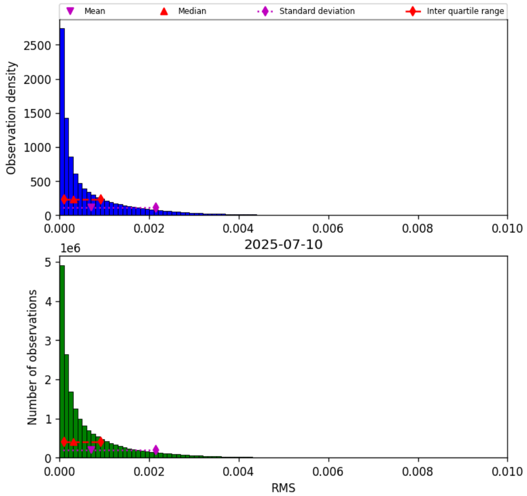
Figure 45: Histogram of “RMS” for 2025-07-10 to 2025-07-11
