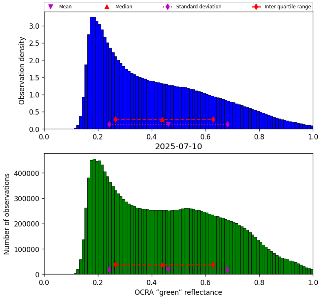
Figure 50: Histogram of “OCRA “green” reflectance” for 2025-07-10 to 2025-07-11
