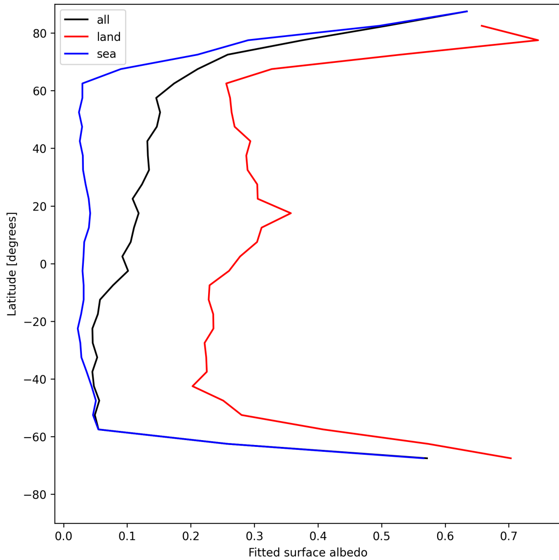
Figure 27: Zonal average of “Fitted surface albedo” for 2025-07-10 to 2025-07-11.
