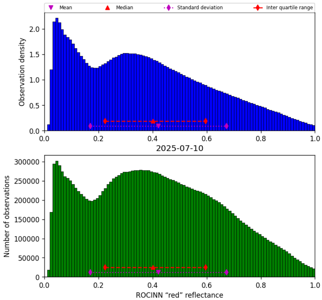
Figure 51: Histogram of “ROCINN “red” reflectance” for 2025-07-10 to 2025-07-11
