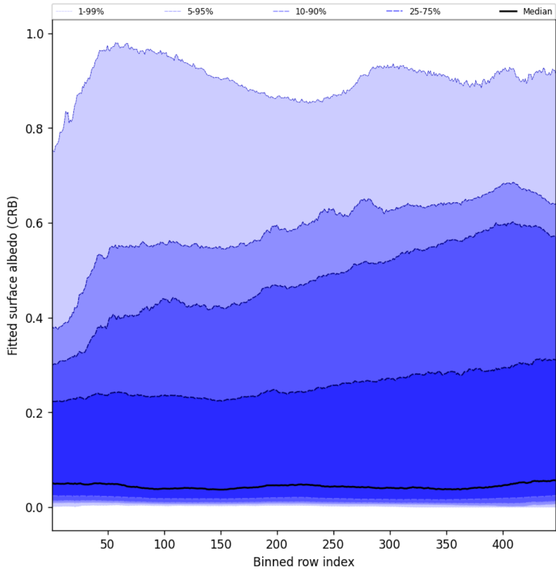
Figure 60: Along track statistics of “Fitted surface albedo (CRB)” for 2025-07-10 to 2025-07-11
