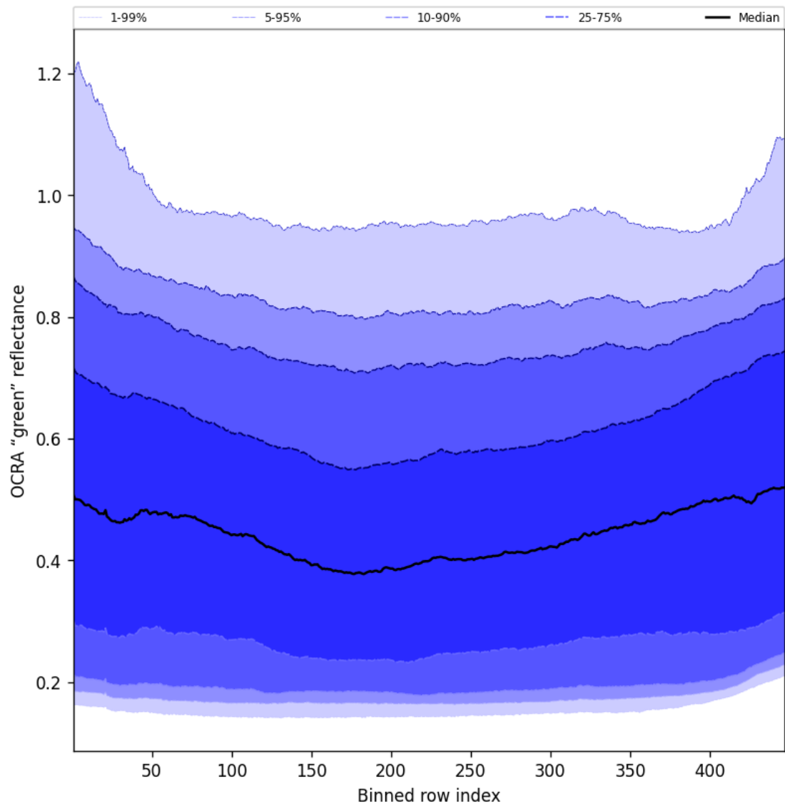
Figure 66: Along track statistics of “OCRA “green” reflectance” for 2025-07-10 to 2025-07-11
