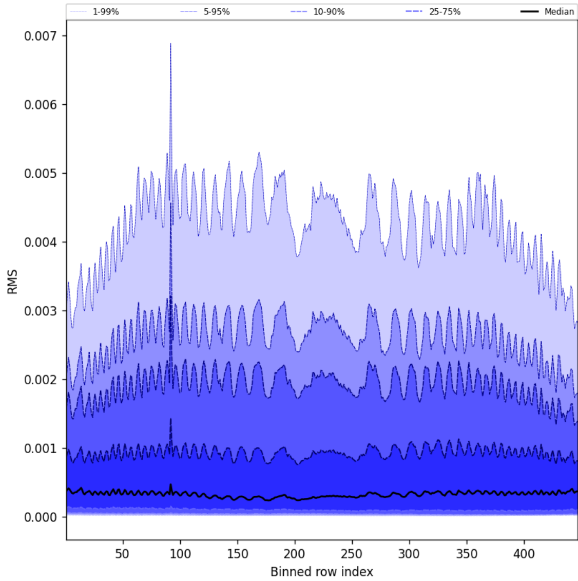
Figure 61: Along track statistics of “RMS” for 2025-07-10 to 2025-07-11
