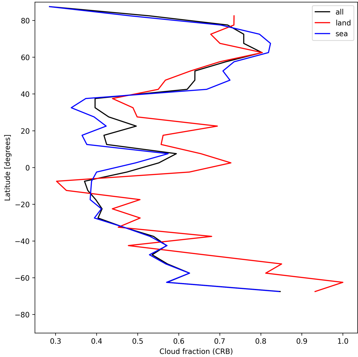
Figure 24: Zonal average of “Cloud fraction (CRB)” for 2025-07-10 to 2025-07-11.
