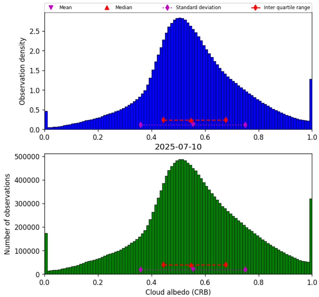
Figure 42: Histogram of “Cloud albedo (CRB)” for 2025-07-10 to 2025-07-11
