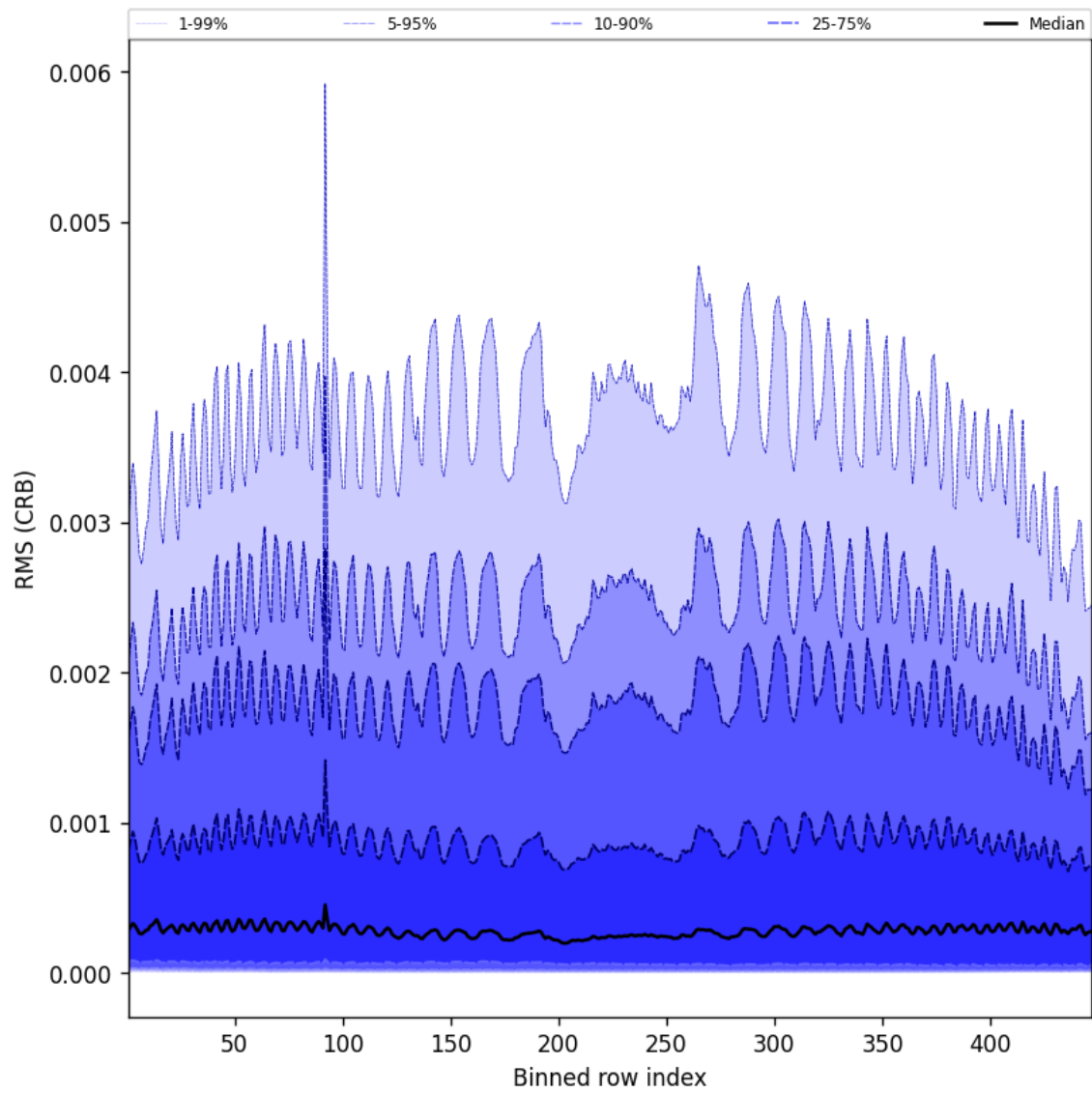
Figure 62: Along track statistics of “RMS (CRB)” for 2025-07-11 to 2025-07-11
