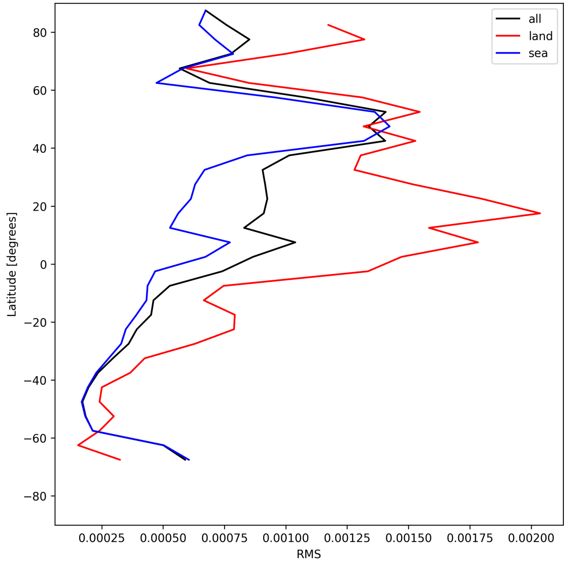
Figure 29: Zonal average of “RMS” for 2025-07-11 to 2025-07-11.
