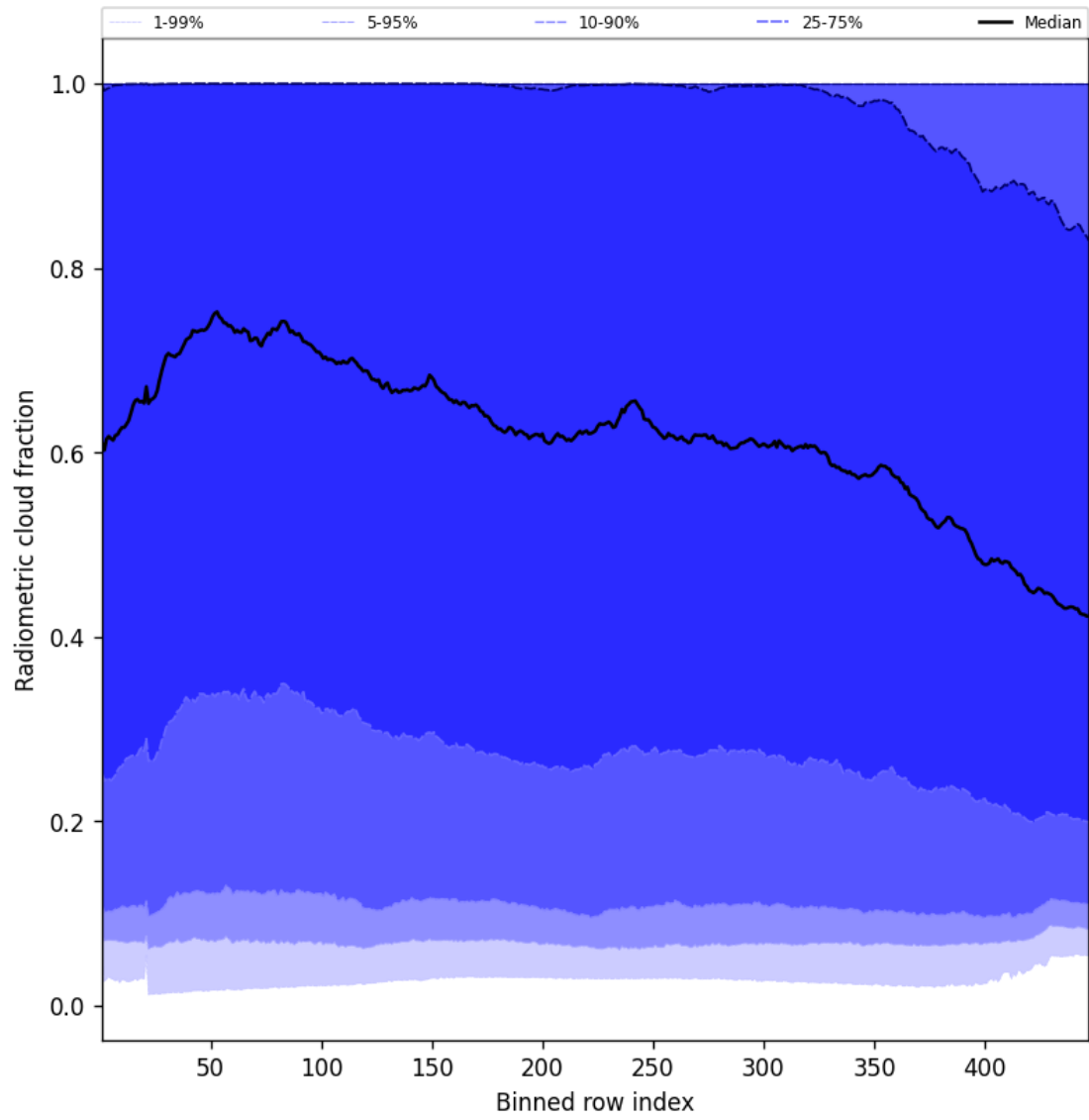
Figure 53: Along track statistics of “Radiometric cloud fraction” for 2025-07-11 to 2025-07-11
