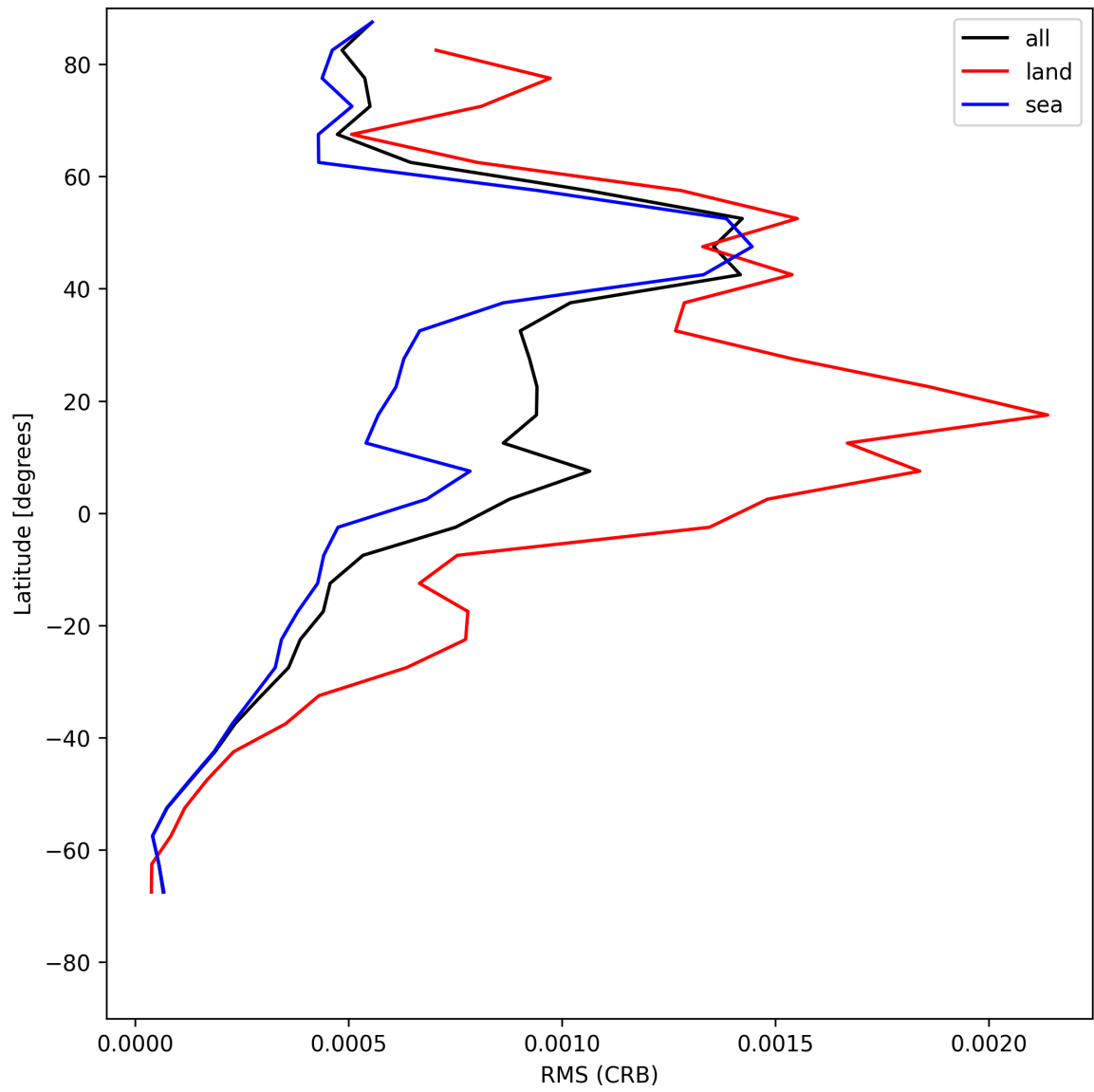
Figure 30: Zonal average of “RMS (CRB)” for 2025-07-11 to 2025-07-11.
