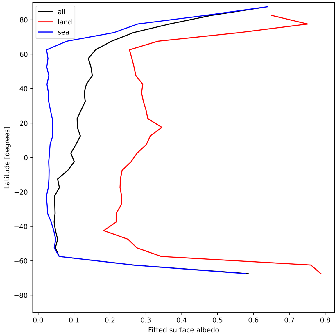
Figure 27: Zonal average of “Fitted surface albedo” for 2025-07-11 to 2025-07-11.
