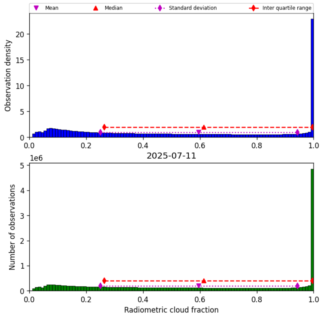
Figure 37: Histogram of “Radiometric cloud fraction” for 2025-07-11 to 2025-07-11
