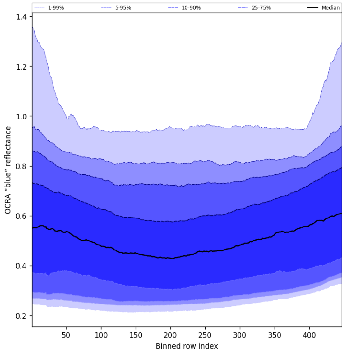
Figure 65: Along track statistics of "OCRA "blue" reflectance" for 2025-07-11 to 2025-07-11
