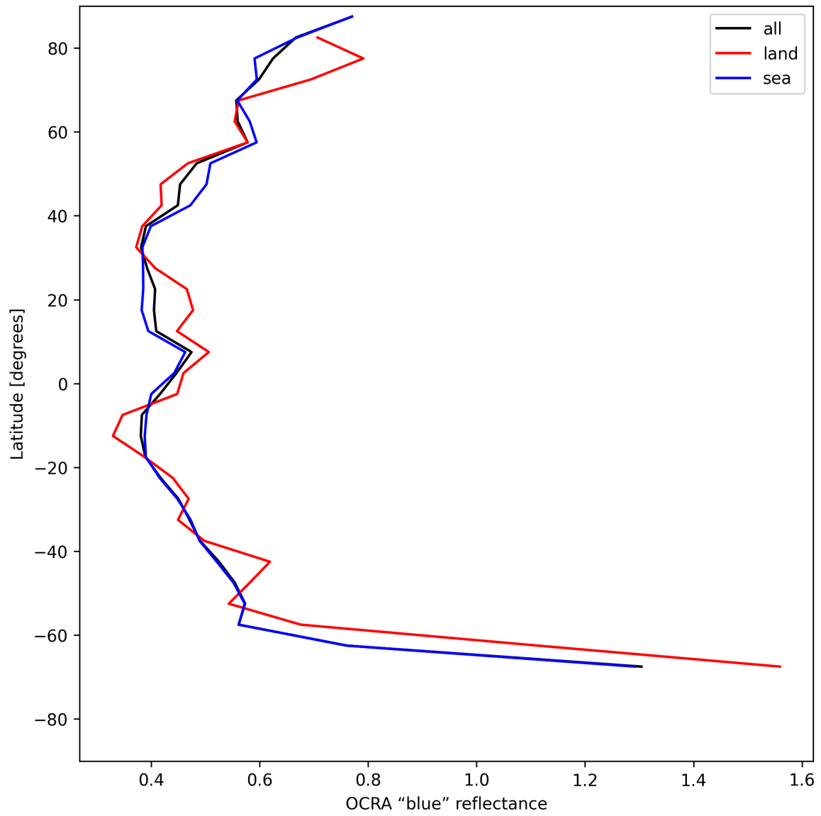
Figure 33: Zonal average of “OCRA “blue” reflectance” for 2025-07-11 to 2025-07-11.
