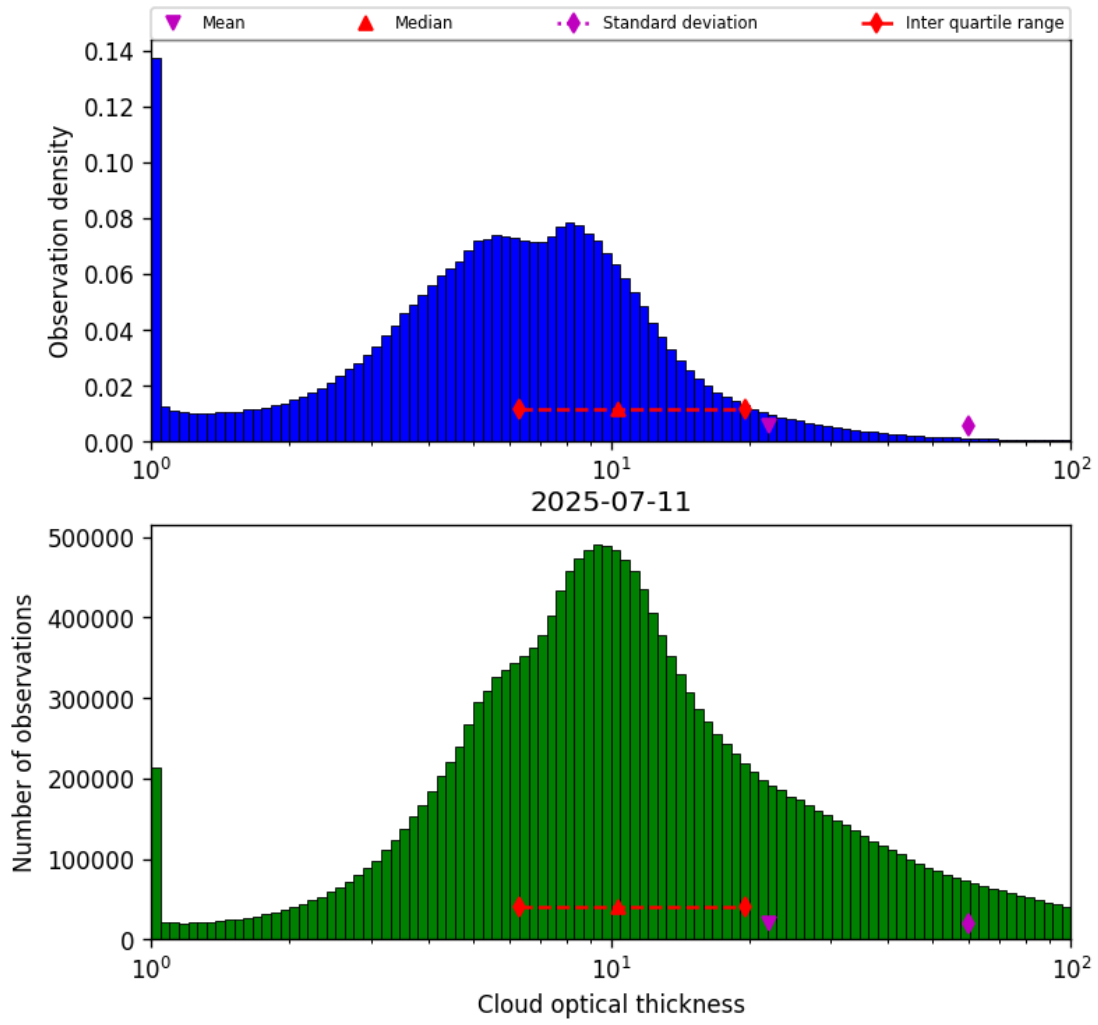
Figure 39: Histogram of “Cloud optical thickness” for 2025-07-11 to 2025-07-11
