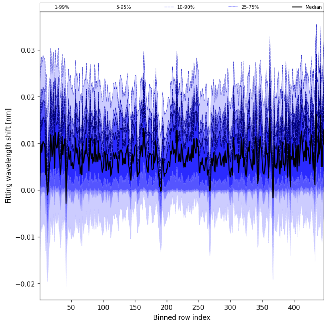
Figure 63: Along track statistics of “Fitting wavelength shift” for 2025-07-11 to 2025-07-11
