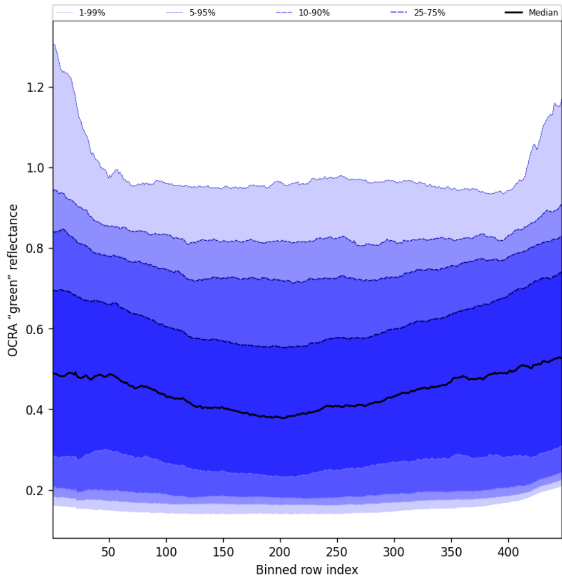
Figure 66: Along track statistics of “OCRA “green” reflectance” for 2025-07-11 to 2025-07-11
