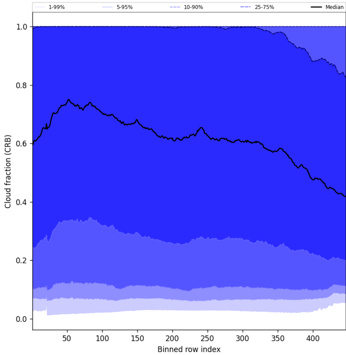
Figure 56: Along track statistics of “Cloud fraction (CRB)” for 2025-07-11 to 2025-07-11
