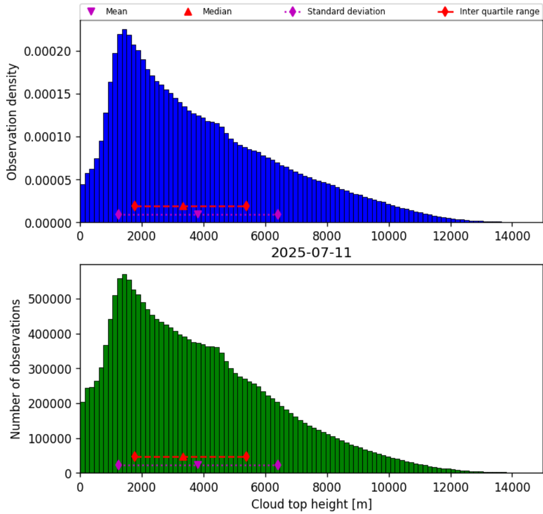
Figure 38: Histogram of “Cloud top height” for 2025-07-11 to 2025-07-11
