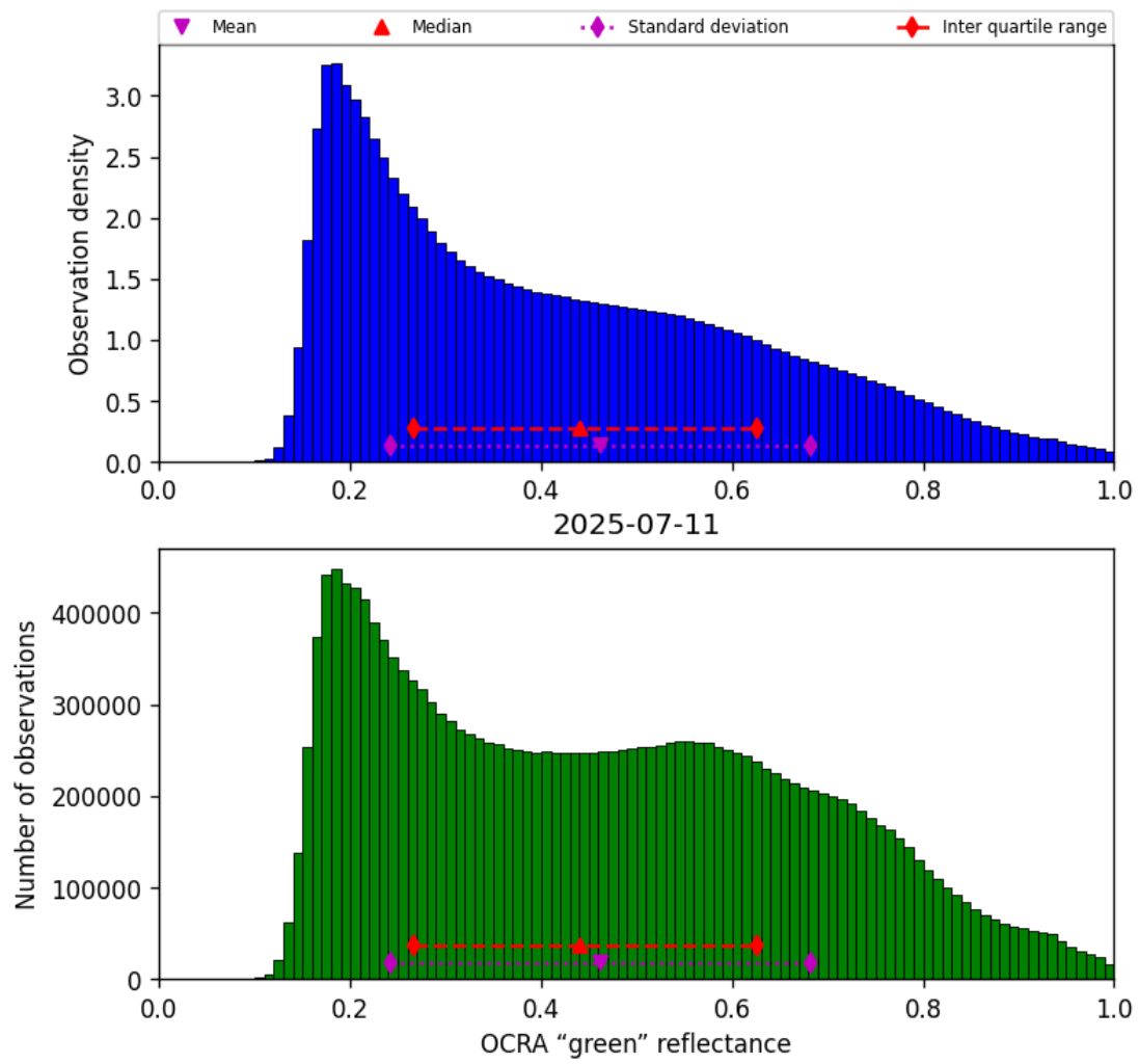
Figure 50: Histogram of “OCRA “green” reflectance” for 2025-07-11 to 2025-07-11
