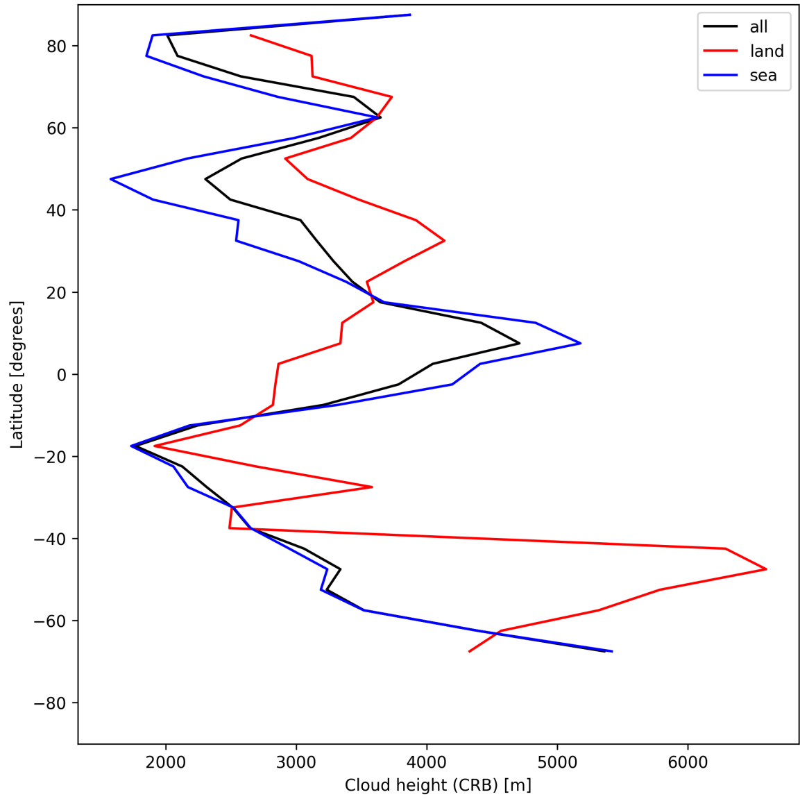
Figure 25: Zonal average of “Cloud height (CRB)” for 2025-07-11 to 2025-07-11.
