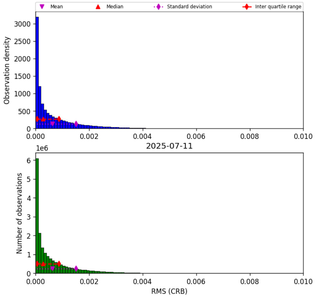
Figure 46: Histogram of “RMS (CRB)” for 2025-07-11 to 2025-07-11
