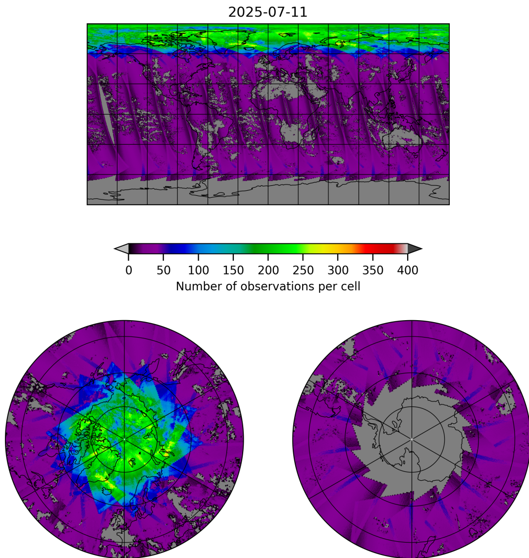
Figure 19: Map of the number of observations for 2025-07-11 to 2025-07-11
