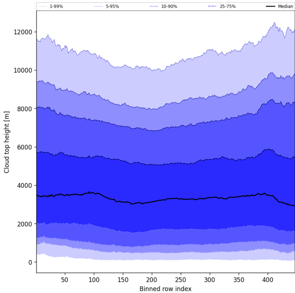
Figure 54: Along track statistics of “Cloud top height” for 2025-07-11 to 2025-07-11
