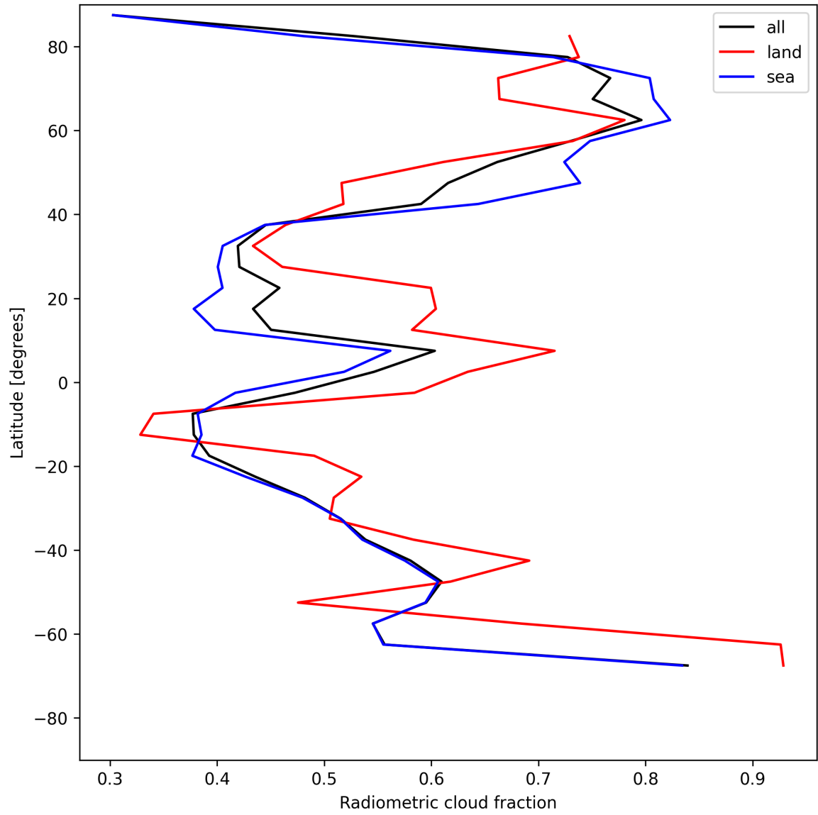
Figure 21: Zonal average of “Radiometric cloud fraction” for 2025-07-11 to 2025-07-11.
