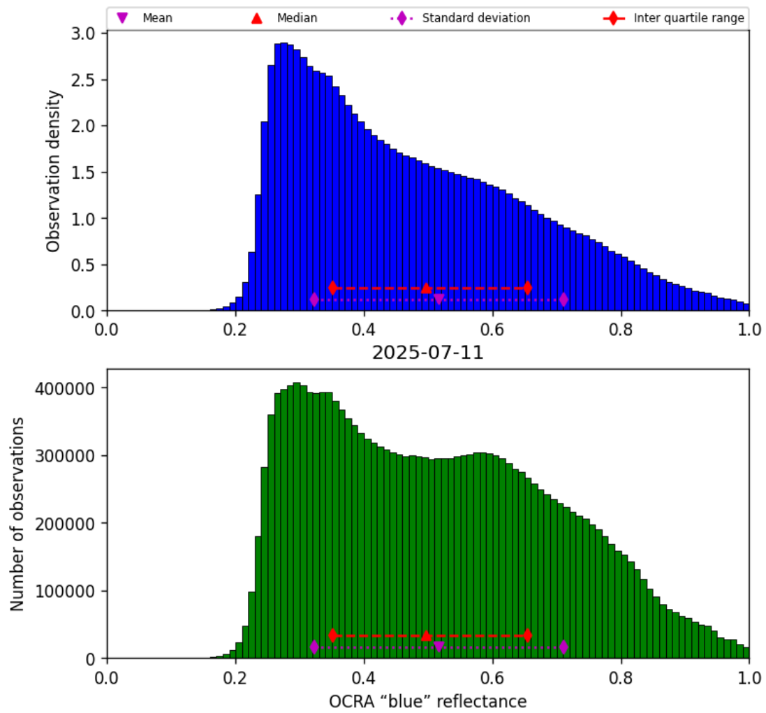
Figure 49: Histogram of “OCRA “blue” reflectance” for 2025-07-11 to 2025-07-11
