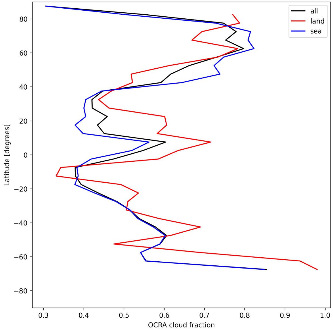
Figure 32: Zonal average of “OCRA cloud fraction” for 2025-07-11 to 2025-07-11.
