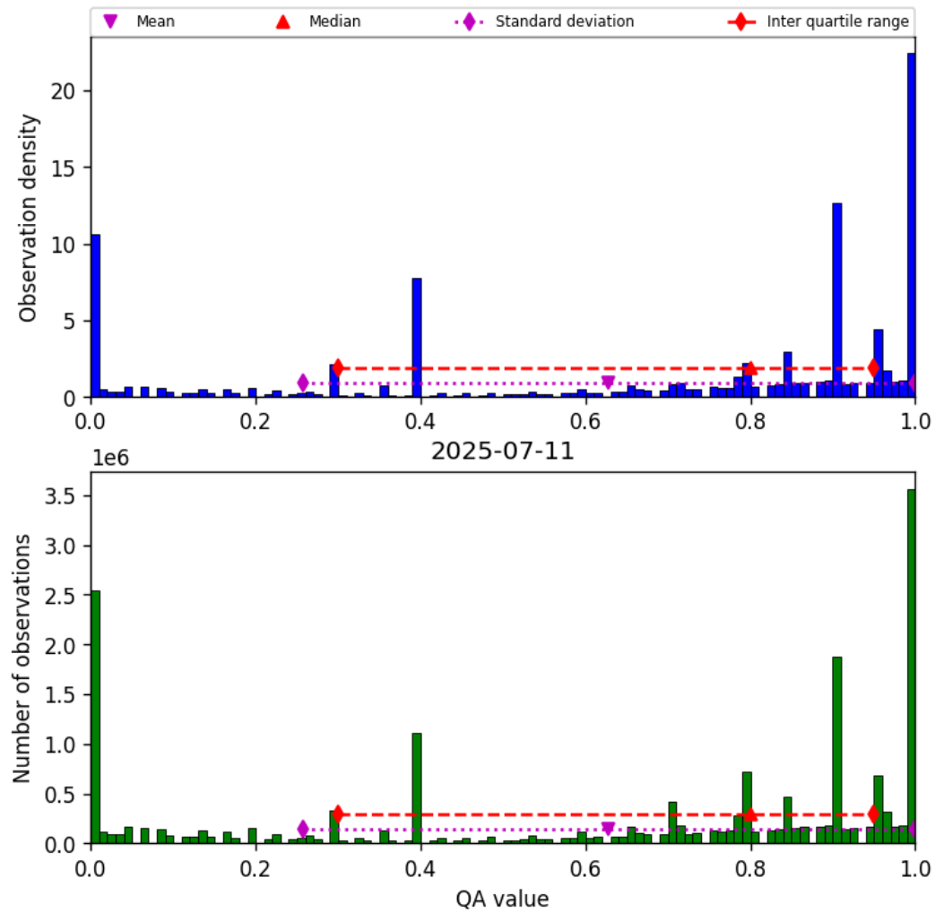
Figure 36: Histogram of “QA value” for 2025-07-11 to 2025-07-11
