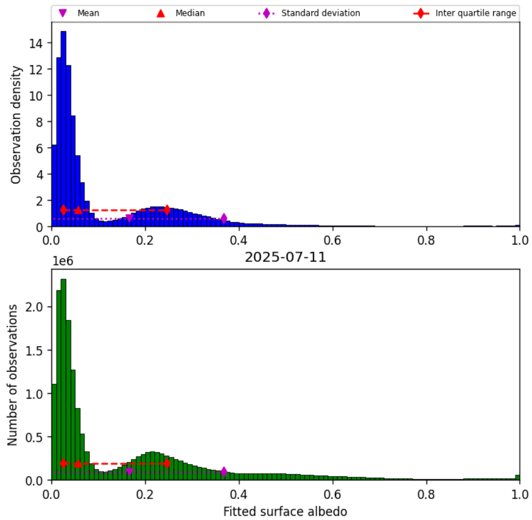
Figure 43: Histogram of “Fitted surface albedo” for 2025-07-11 to 2025-07-11
