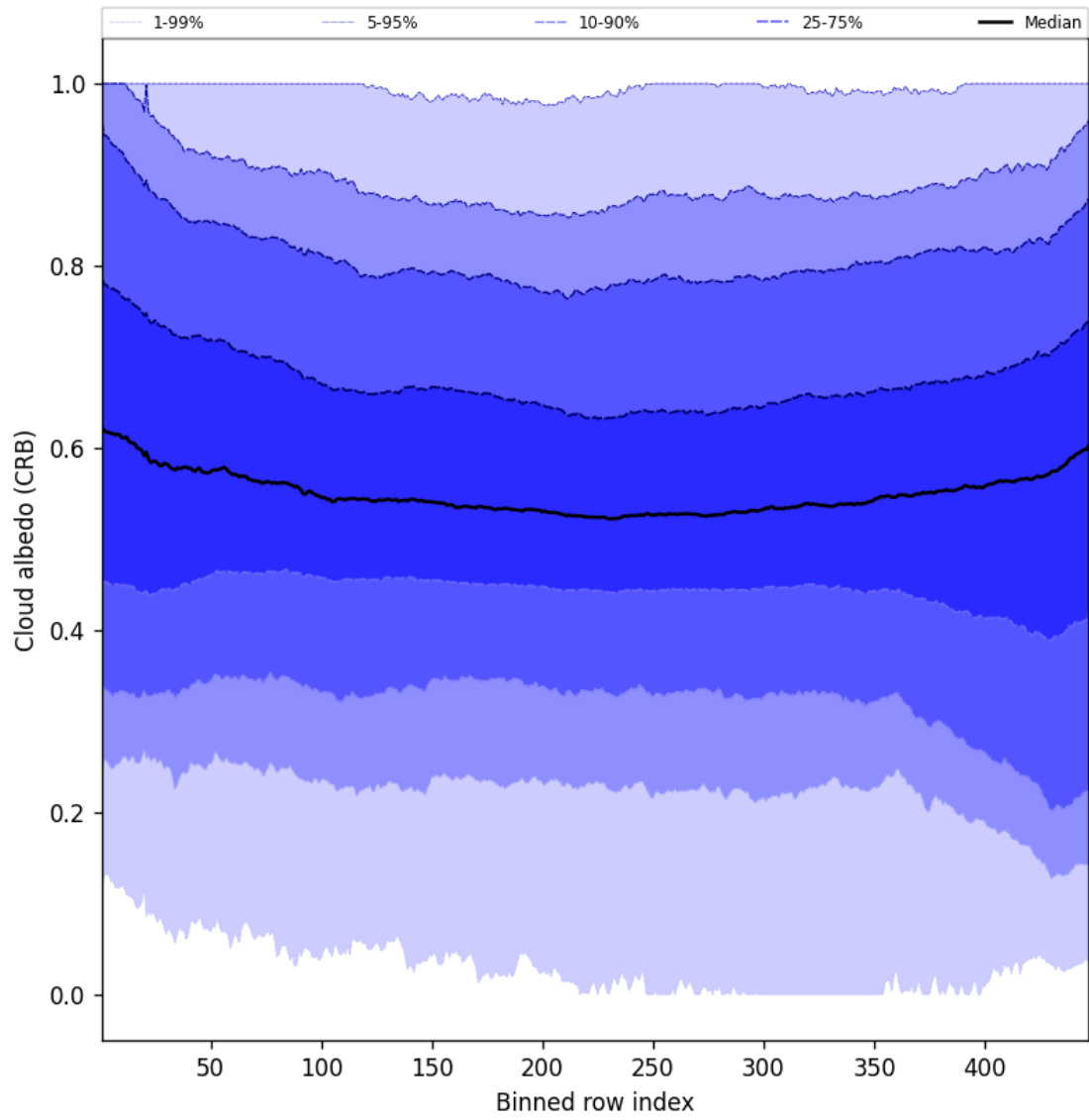
Figure 58: Along track statistics of “Cloud albedo (CRB)” for 2025-07-11 to 2025-07-11
