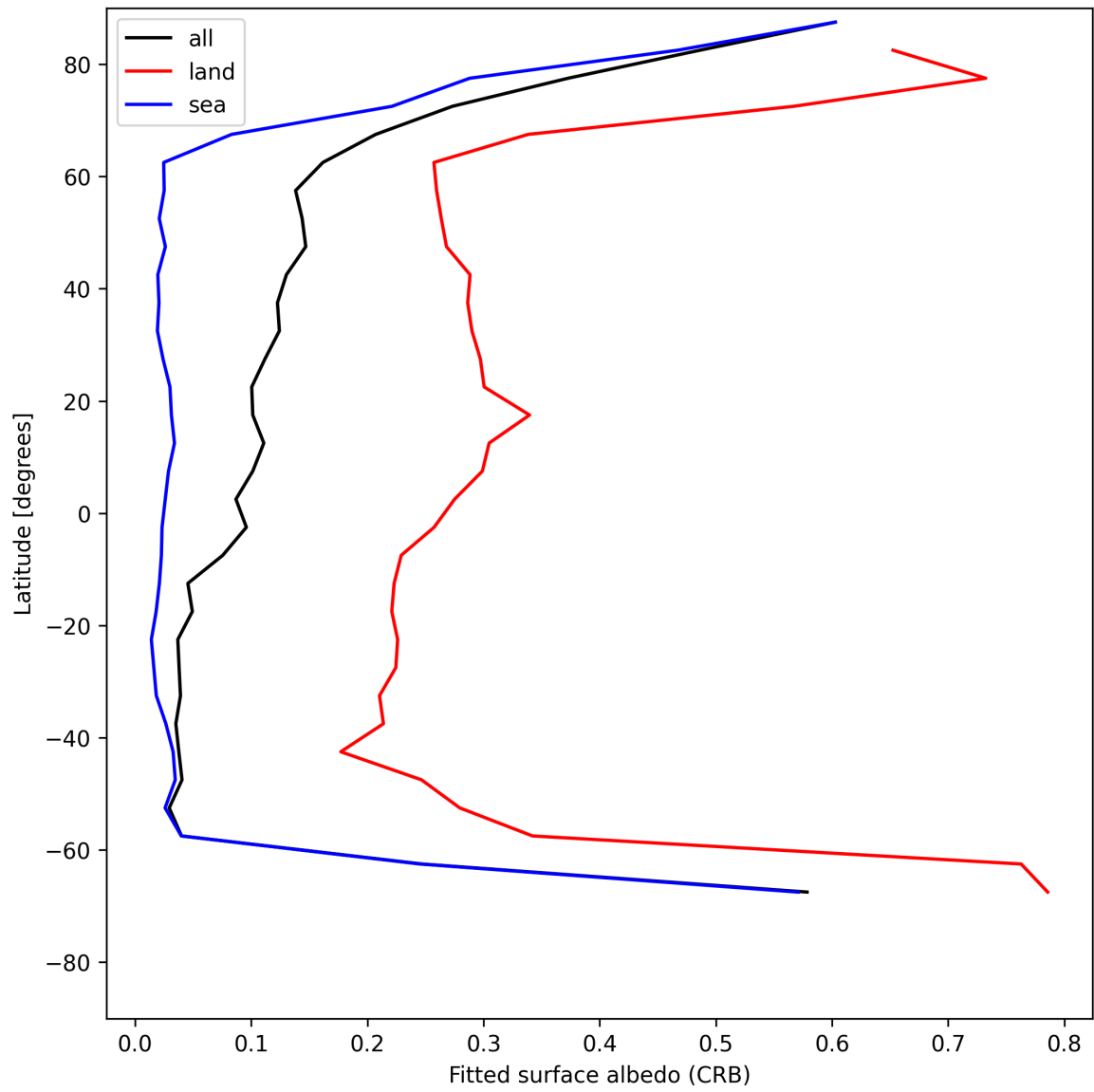
Figure 28: Zonal average of “Fitted surface albedo (CRB)” for 2025-07-11 to 2025-07-11.
