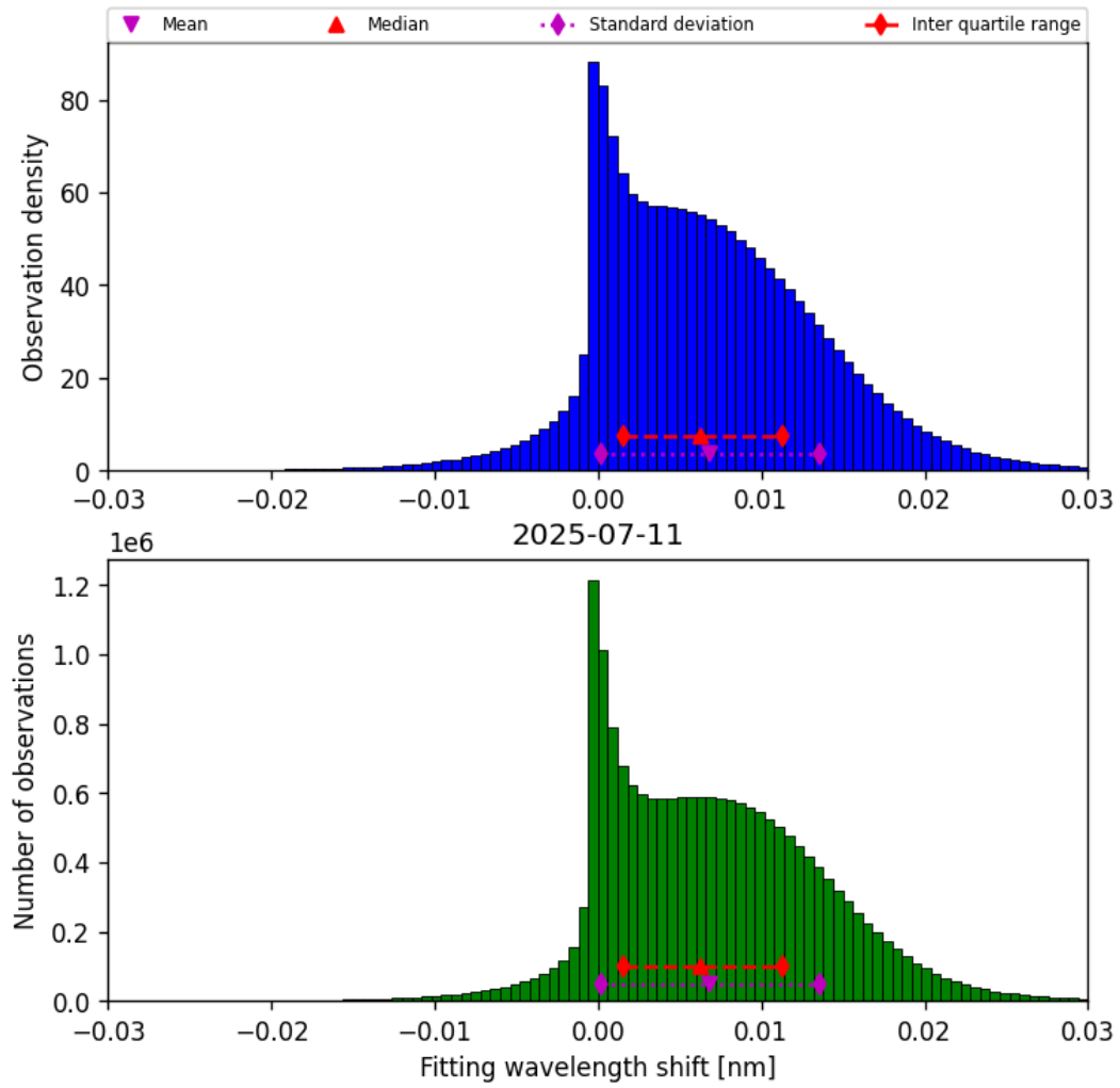
Figure 47: Histogram of “Fitting wavelength shift” for 2025-07-11 to 2025-07-11
