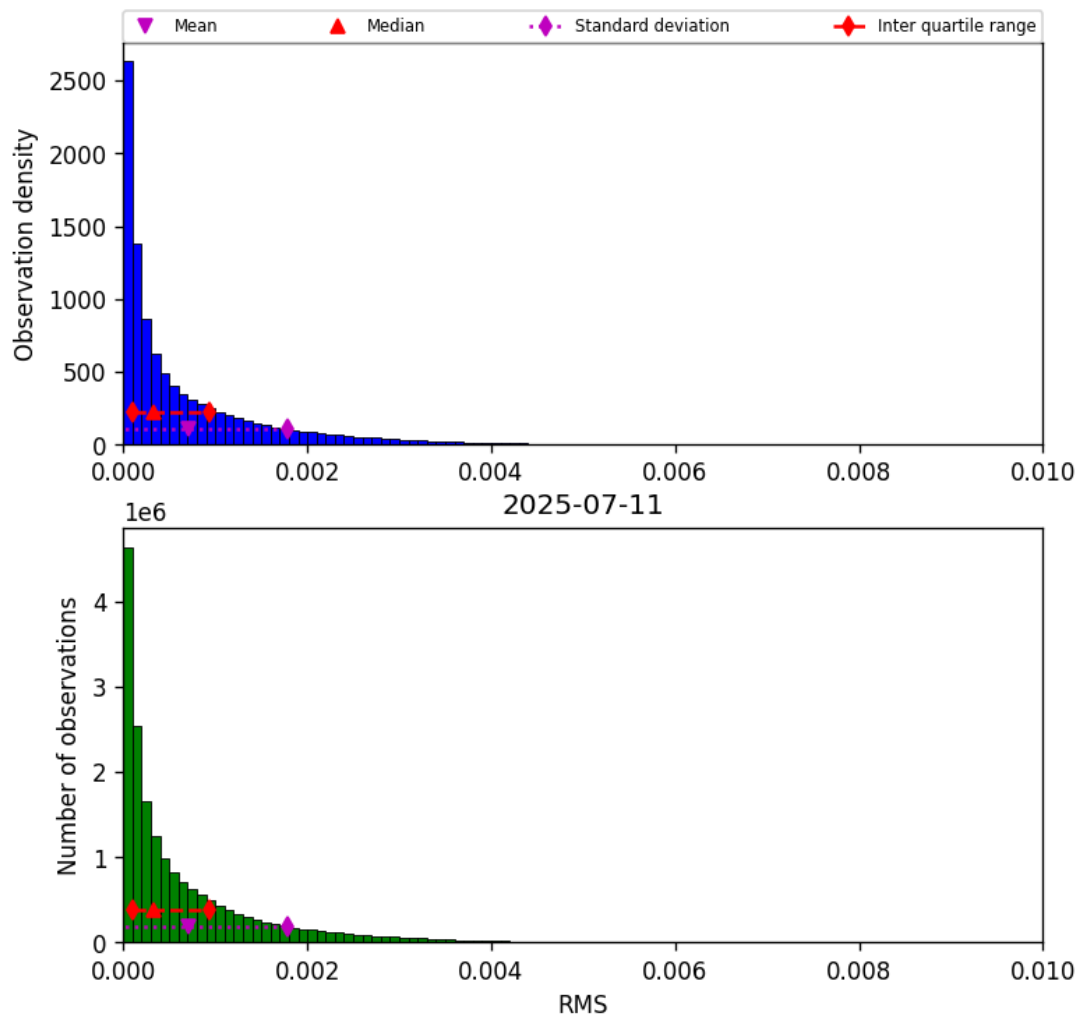
Figure 45: Histogram of “RMS” for 2025-07-11 to 2025-07-11
