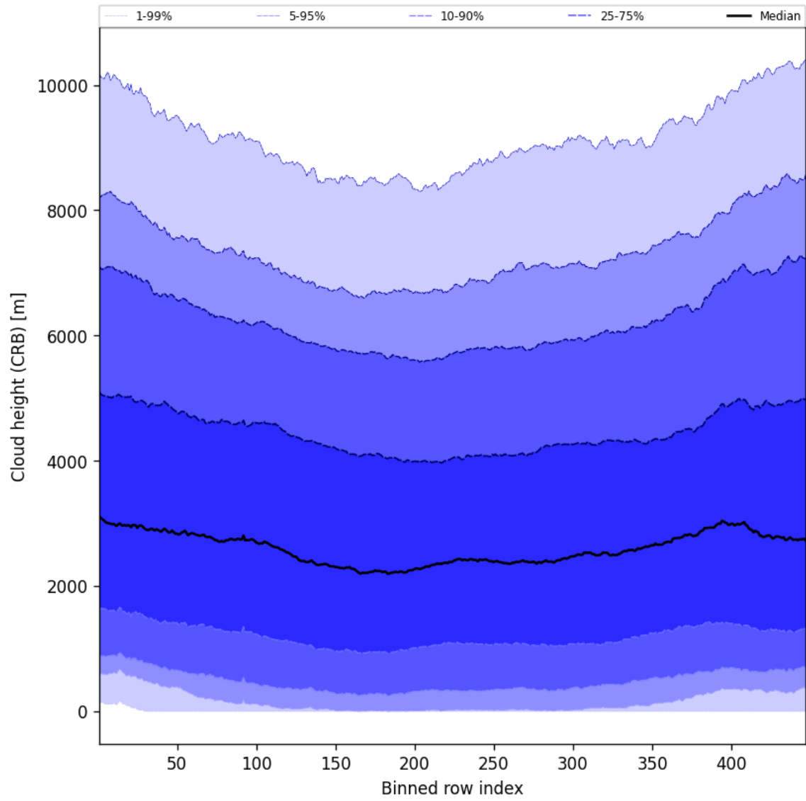
Figure 57: Along track statistics of “Cloud height (CRB)” for 2025-07-11 to 2025-07-11
