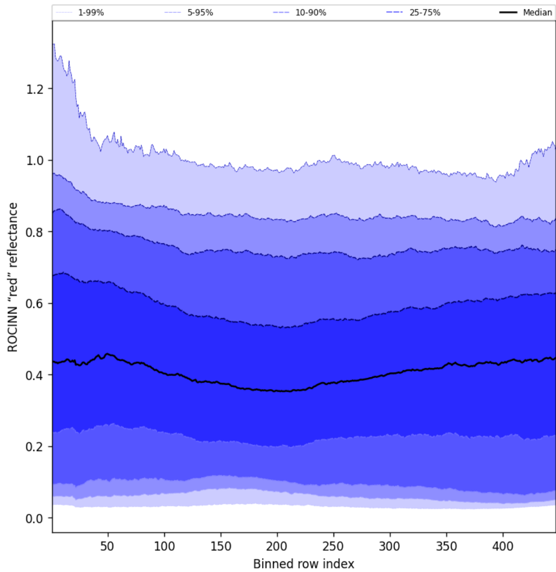
Figure 67: Along track statistics of “ROCINN “red” reflectance” for 2025-07-11 to 2025-07-11
