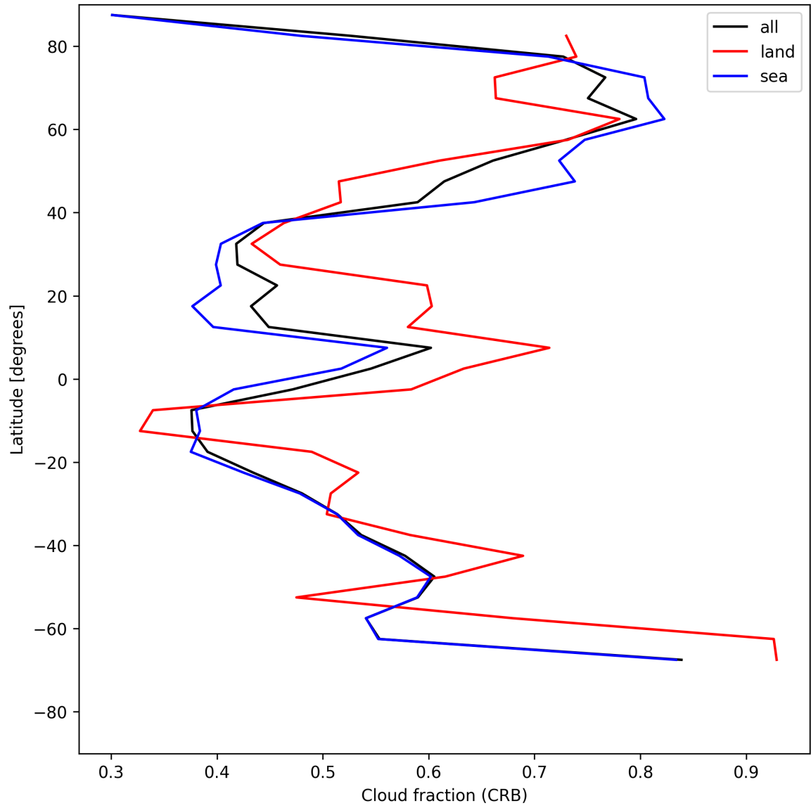
Figure 24: Zonal average of “Cloud fraction (CRB)” for 2025-07-11 to 2025-07-11.
