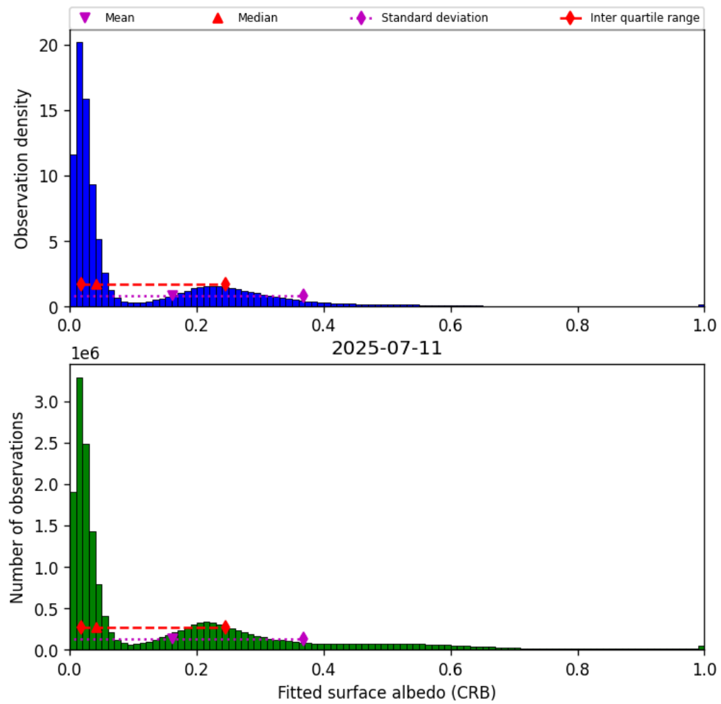
Figure 44: Histogram of “Fitted surface albedo (CRB)” for 2025-07-11 to 2025-07-11
