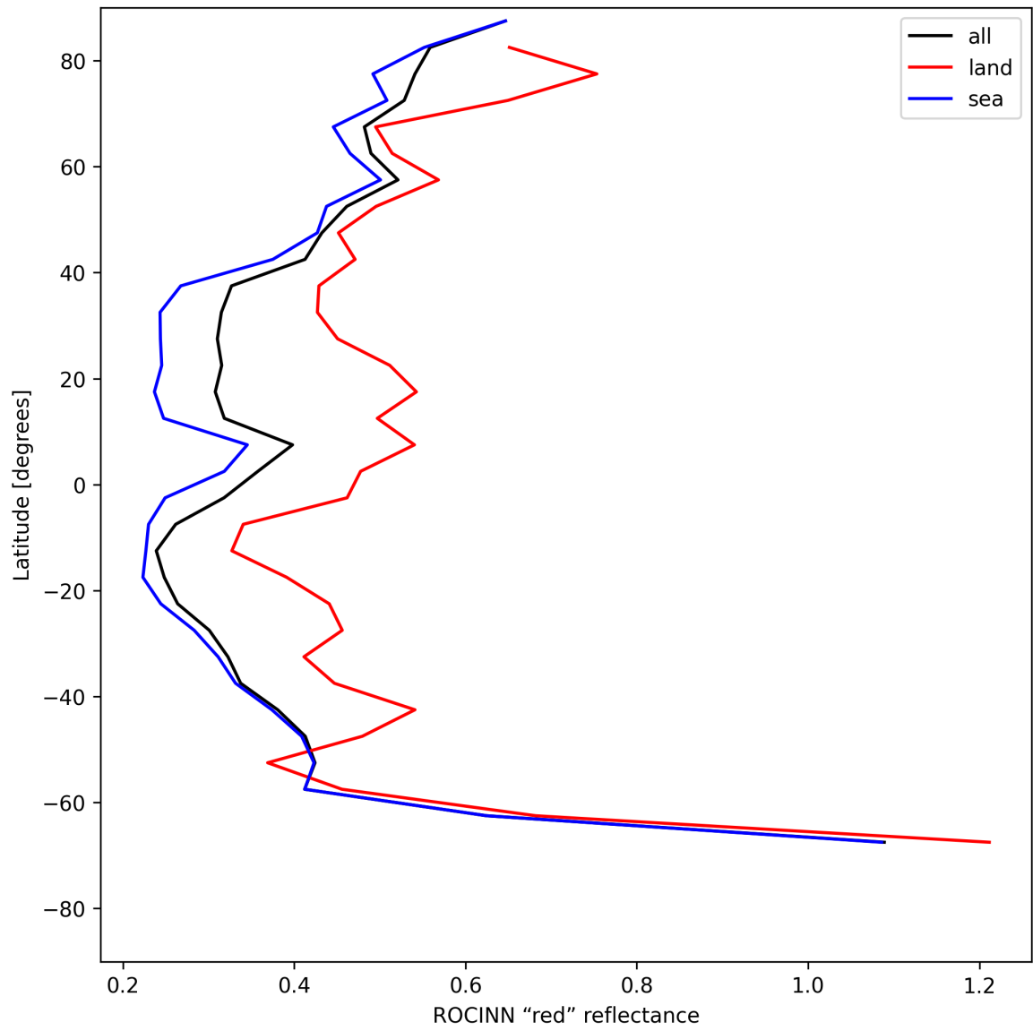
Figure 35: Zonal average of "ROCINN "red" reflectance" for 2025-07-11 to 2025-07-11.
