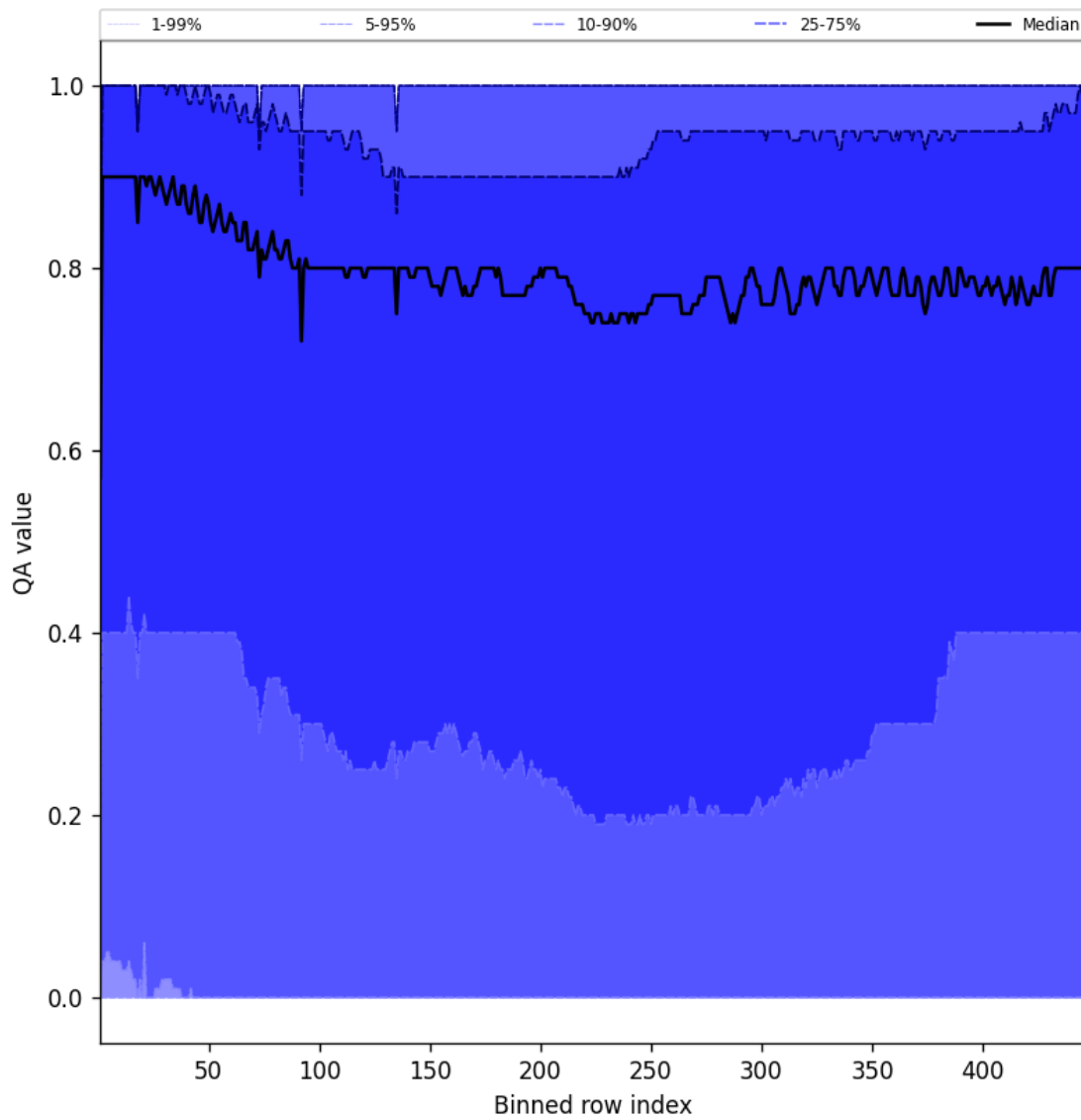
Figure 52: Along track statistics of “QA value” for 2025-07-11 to 2025-07-11
