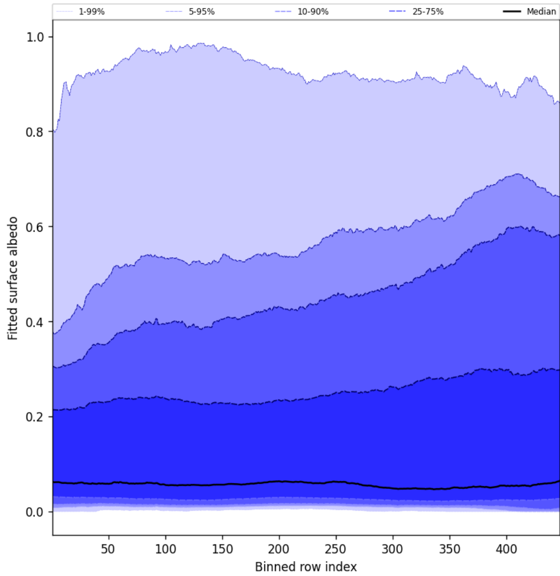
Figure 59: Along track statistics of “Fitted surface albedo” for 2025-07-11 to 2025-07-11
