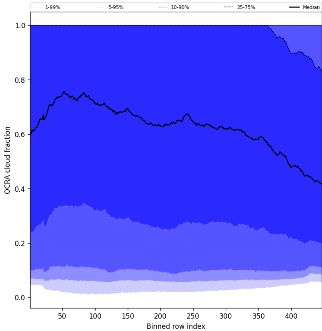
Figure 64: Along track statistics of “OCRA cloud fraction” for 2025-07-11 to 2025-07-11
