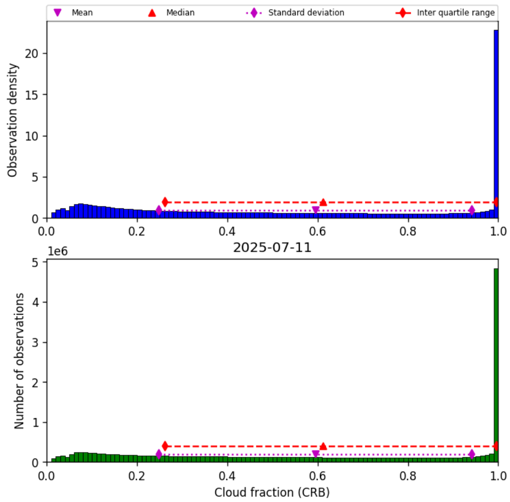
Figure 40: Histogram of “Cloud fraction (CRB)” for 2025-07-11 to 2025-07-11
