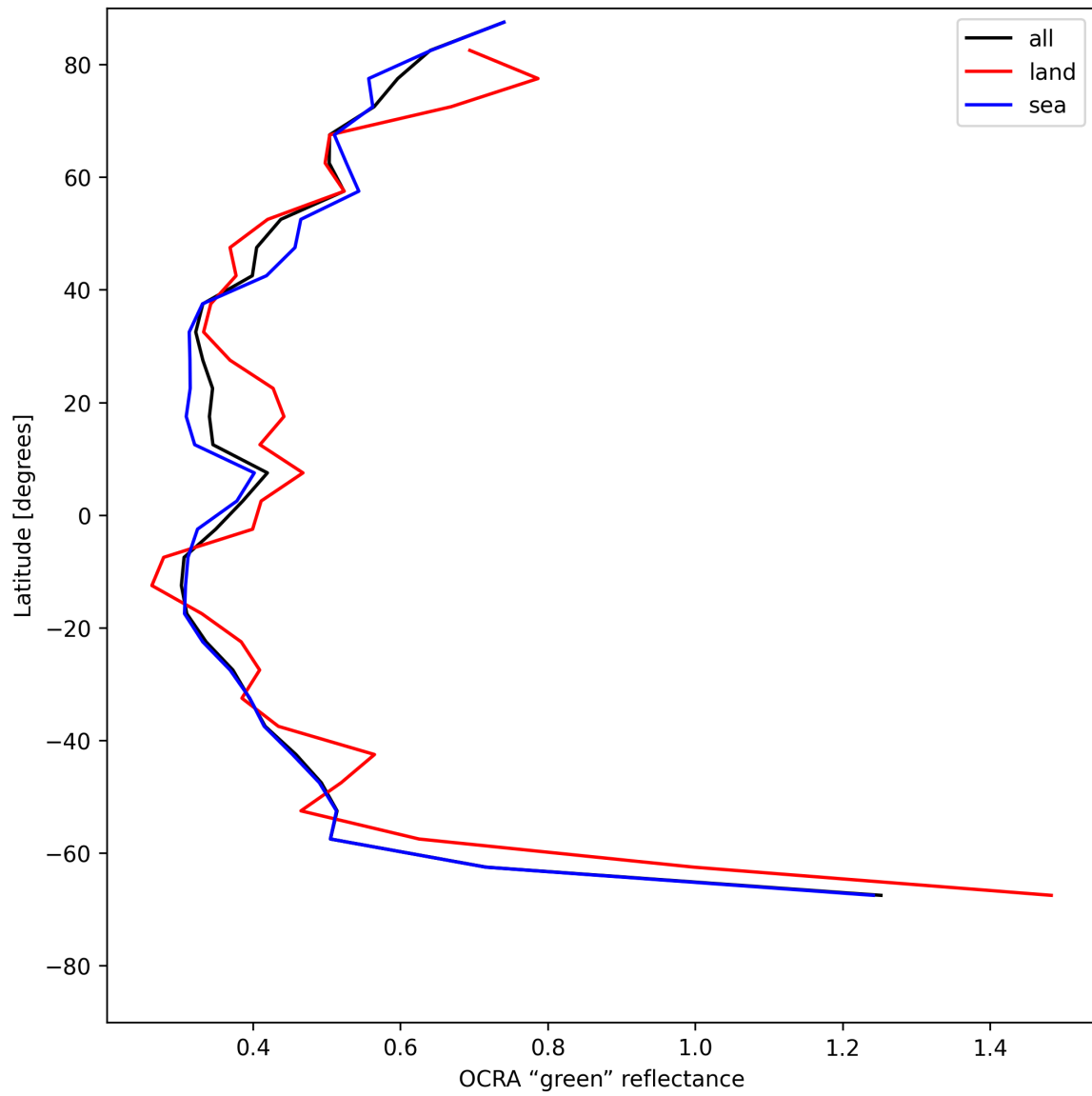
Figure 34: Zonal average of “OCRA “green” reflectance” for 2025-07-11 to 2025-07-11.
