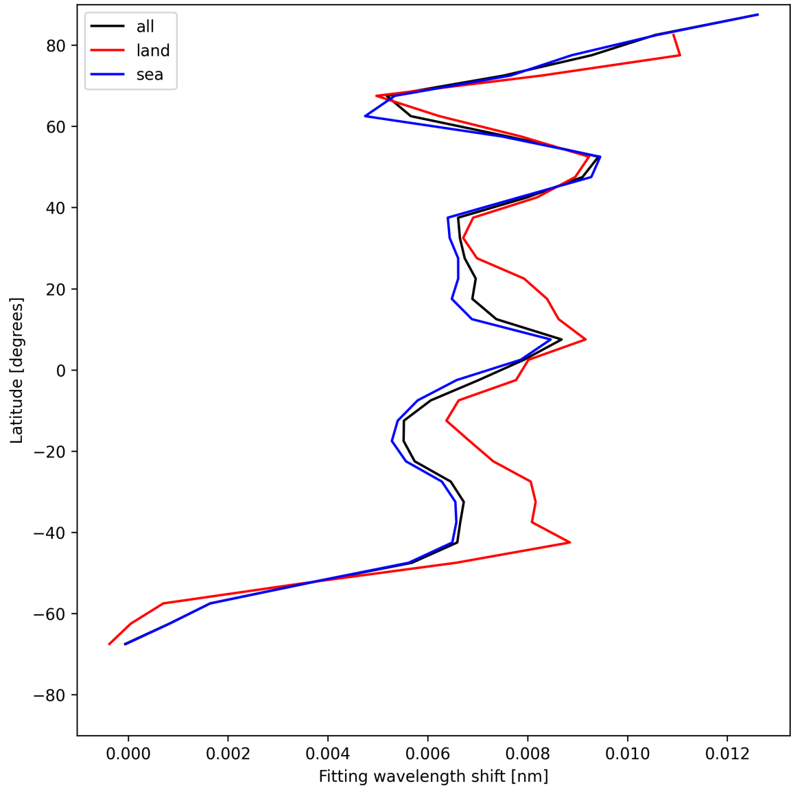
Figure 31: Zonal average of “Fitting wavelength shift” for 2025-07-11 to 2025-07-11.
