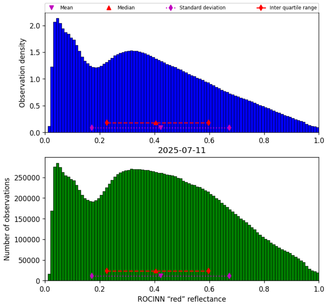
Figure 51: Histogram of “ROCINN “red” reflectance” for 2025-07-11 to 2025-07-11
