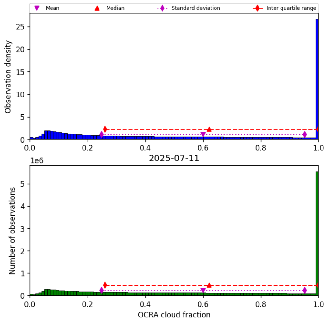
Figure 48: Histogram of “OCRA cloud fraction” for 2025-07-11 to 2025-07-11
