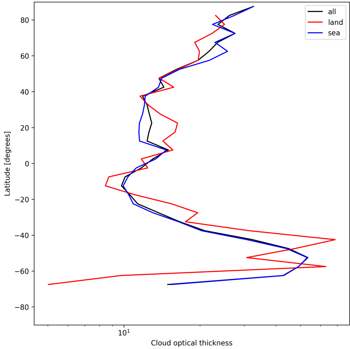
Figure 23: Zonal average of “Cloud optical thickness” for 2025-07-11 to 2025-07-11.
