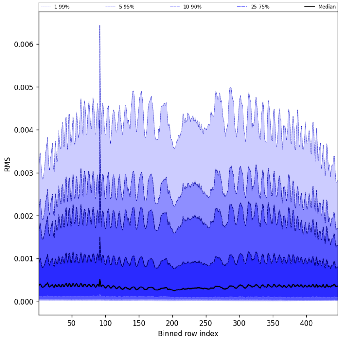
Figure 61: Along track statistics of “RMS” for 2025-07-11 to 2025-07-11
