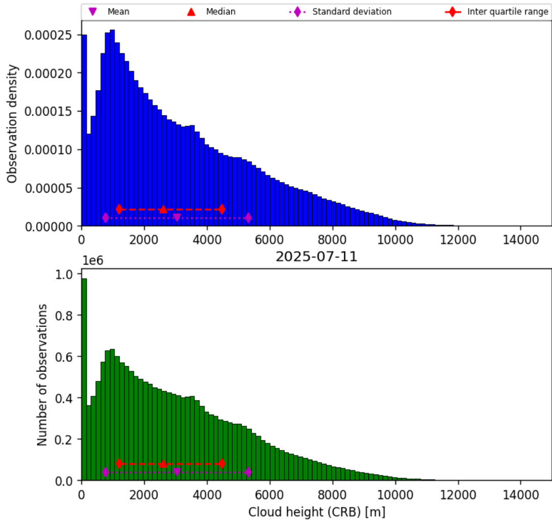
Figure 41: Histogram of “Cloud height (CRB)” for 2025-07-11 to 2025-07-11
