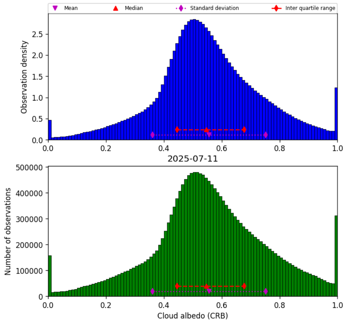
Figure 42: Histogram of “Cloud albedo (CRB)” for 2025-07-11 to 2025-07-11
