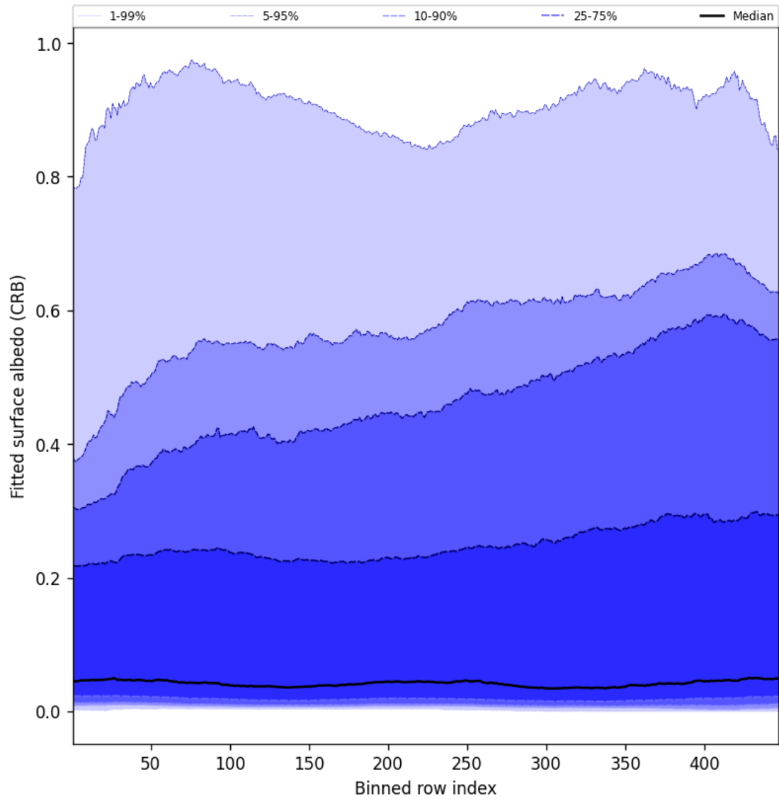
Figure 60: Along track statistics of “Fitted surface albedo (CRB)” for 2025-07-11 to 2025-07-11
