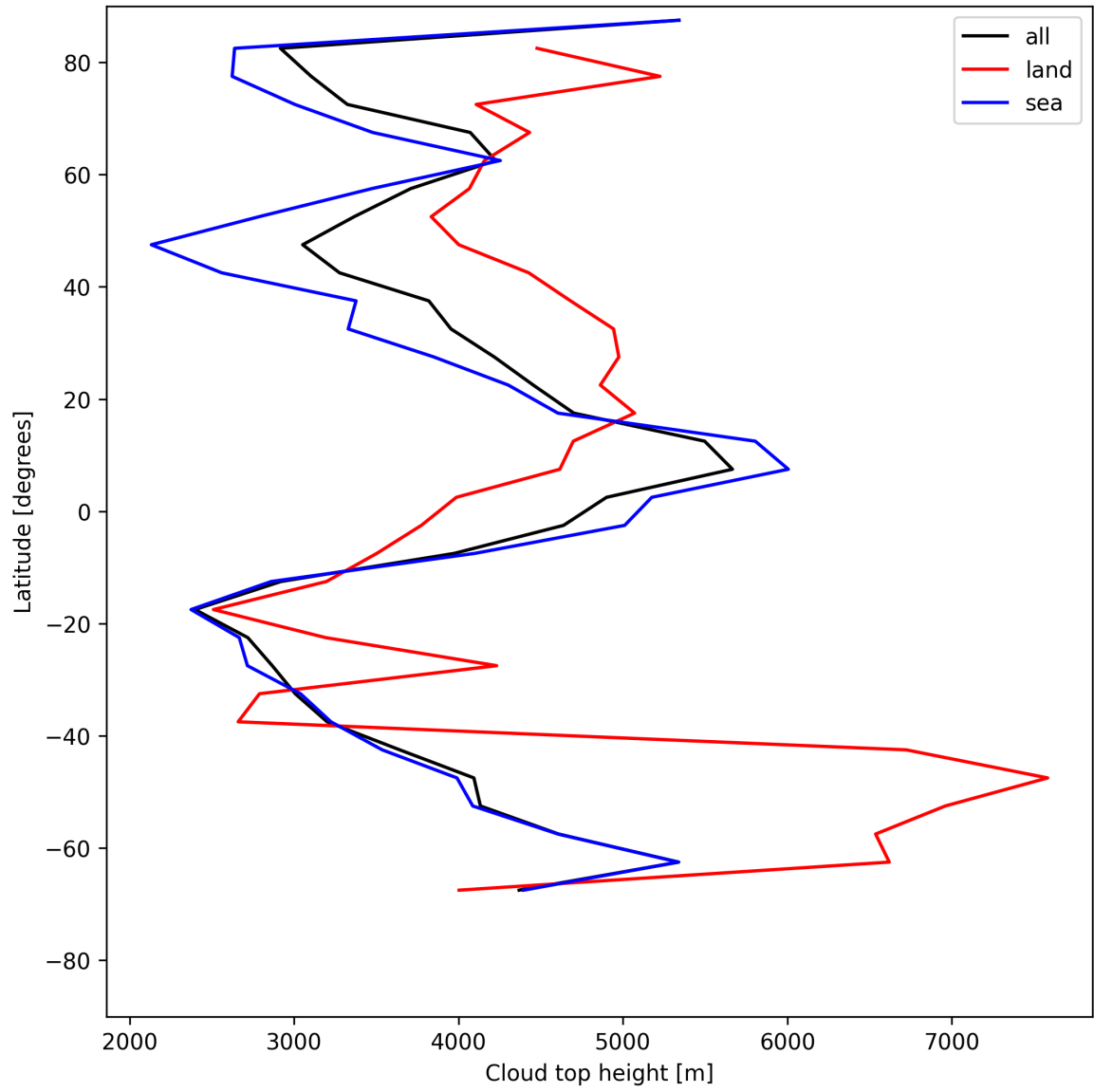
Figure 22: Zonal average of “Cloud top height” for 2025-07-11 to 2025-07-11.
