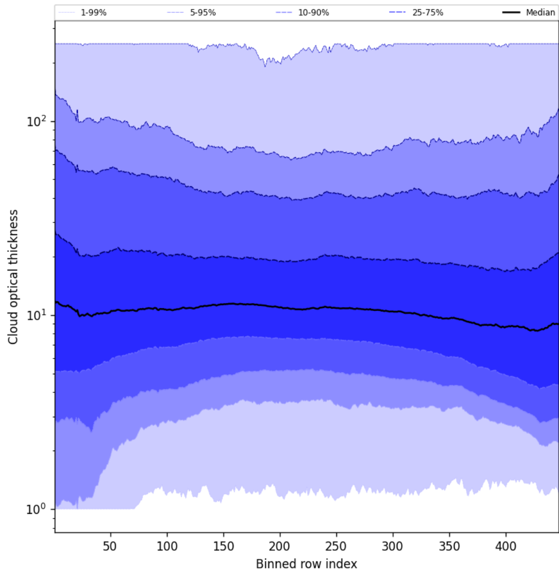
Figure 55: Along track statistics of “Cloud optical thickness” for 2025-07-11 to 2025-07-11
