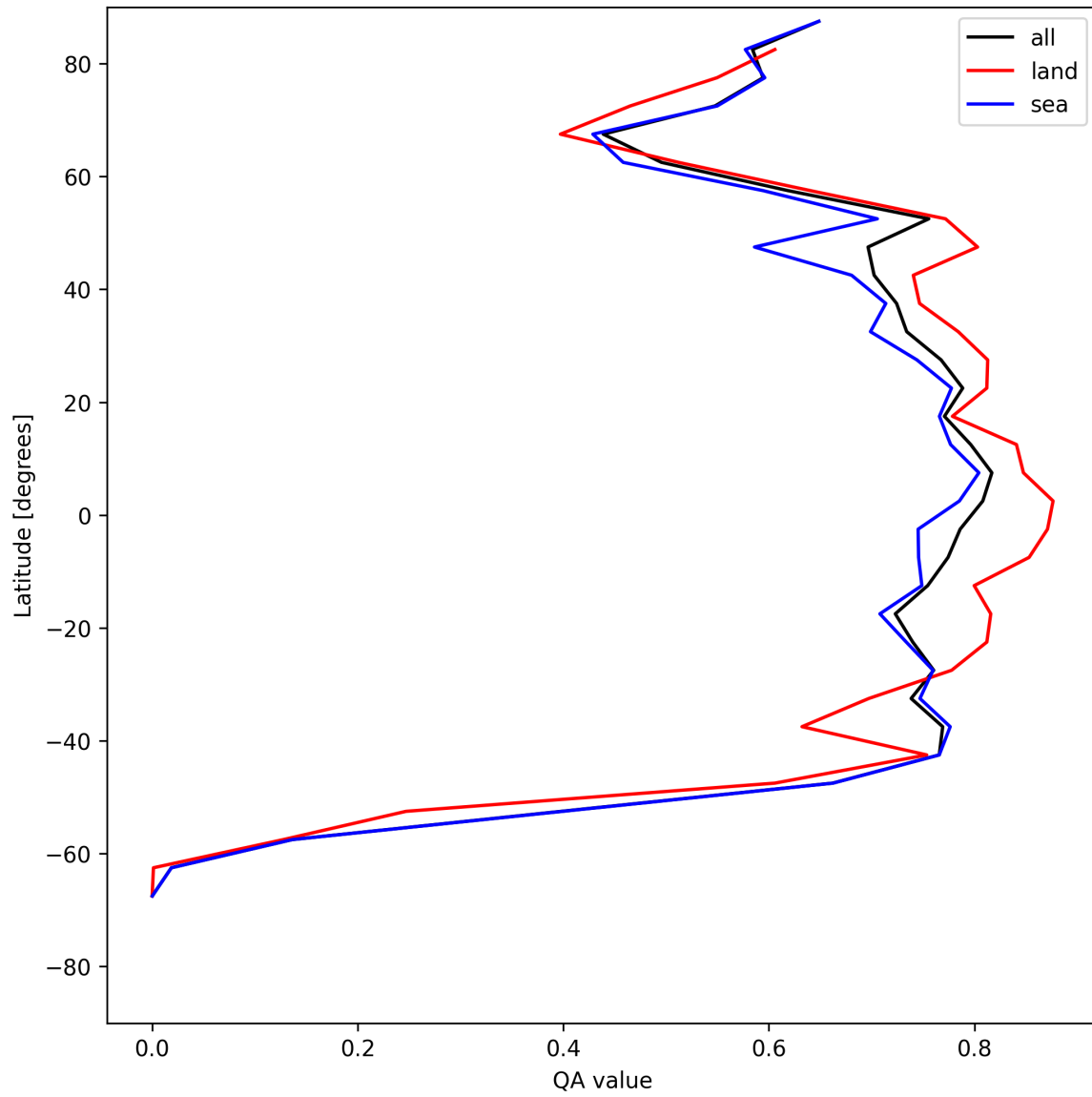
Figure 20: Zonal average of “QA value” for 2025-07-11 to 2025-07-11.
