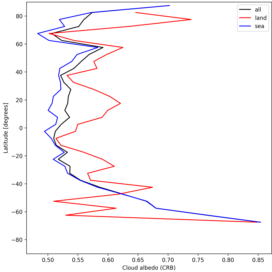
Figure 26: Zonal average of “Cloud albedo (CRB)” for 2025-07-11 to 2025-07-11.
