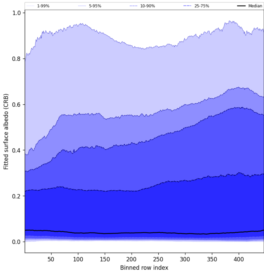
Figure 60: Along track statistics of “Fitted surface albedo (CRB)” for 2025-07-12 to 2025-07-13
