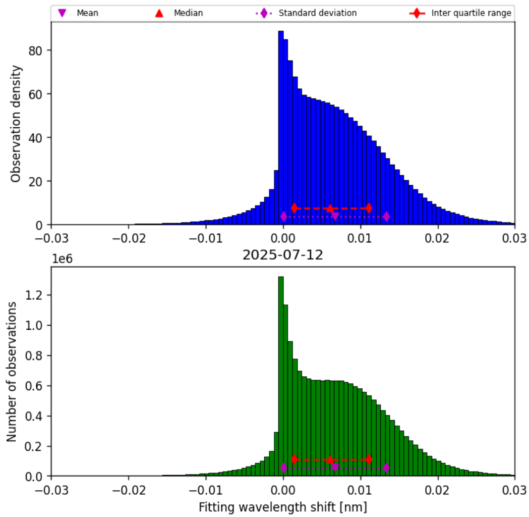
Figure 47: Histogram of “Fitting wavelength shift” for 2025-07-12 to 2025-07-13
