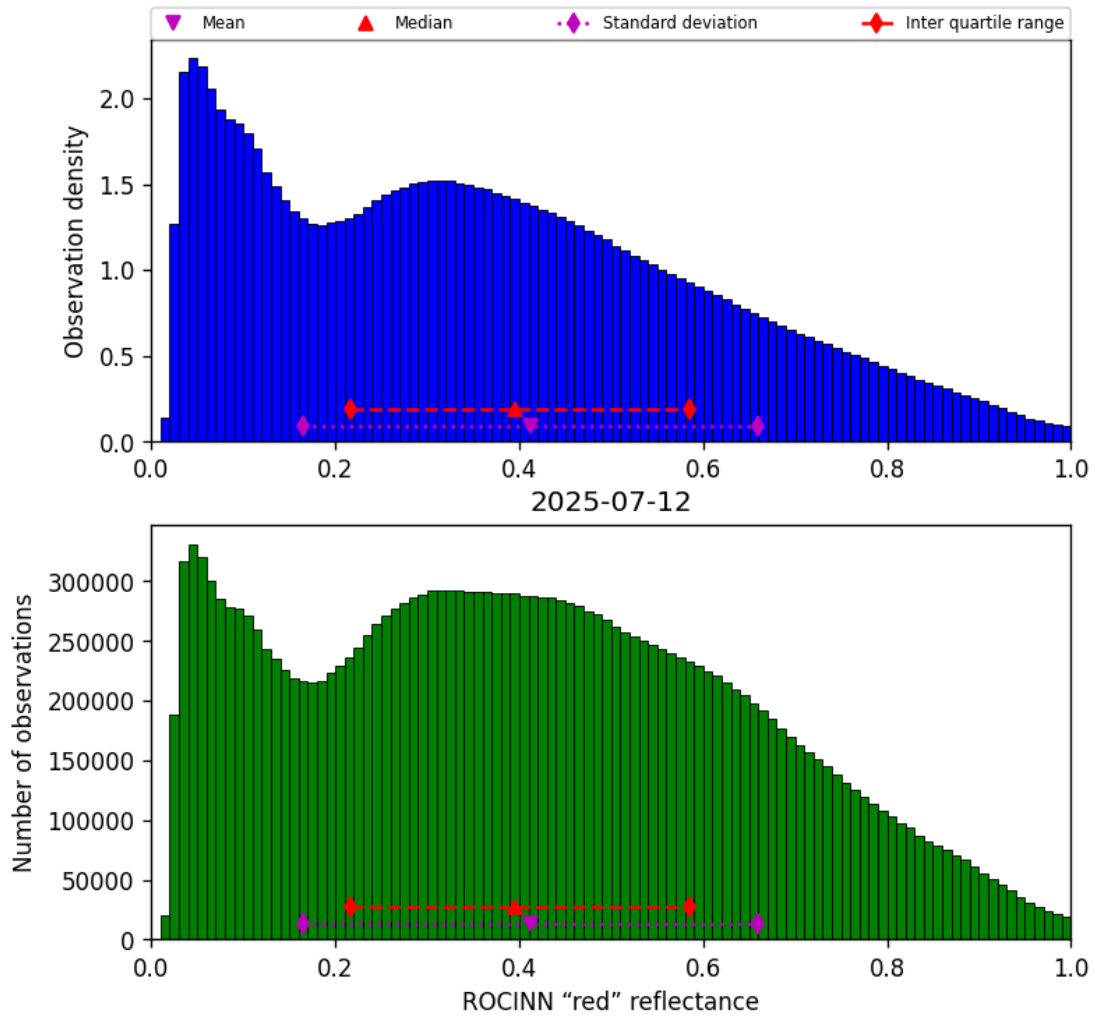
Figure 51: Histogram of “ROCINN “red” reflectance” for 2025-07-12 to 2025-07-13
