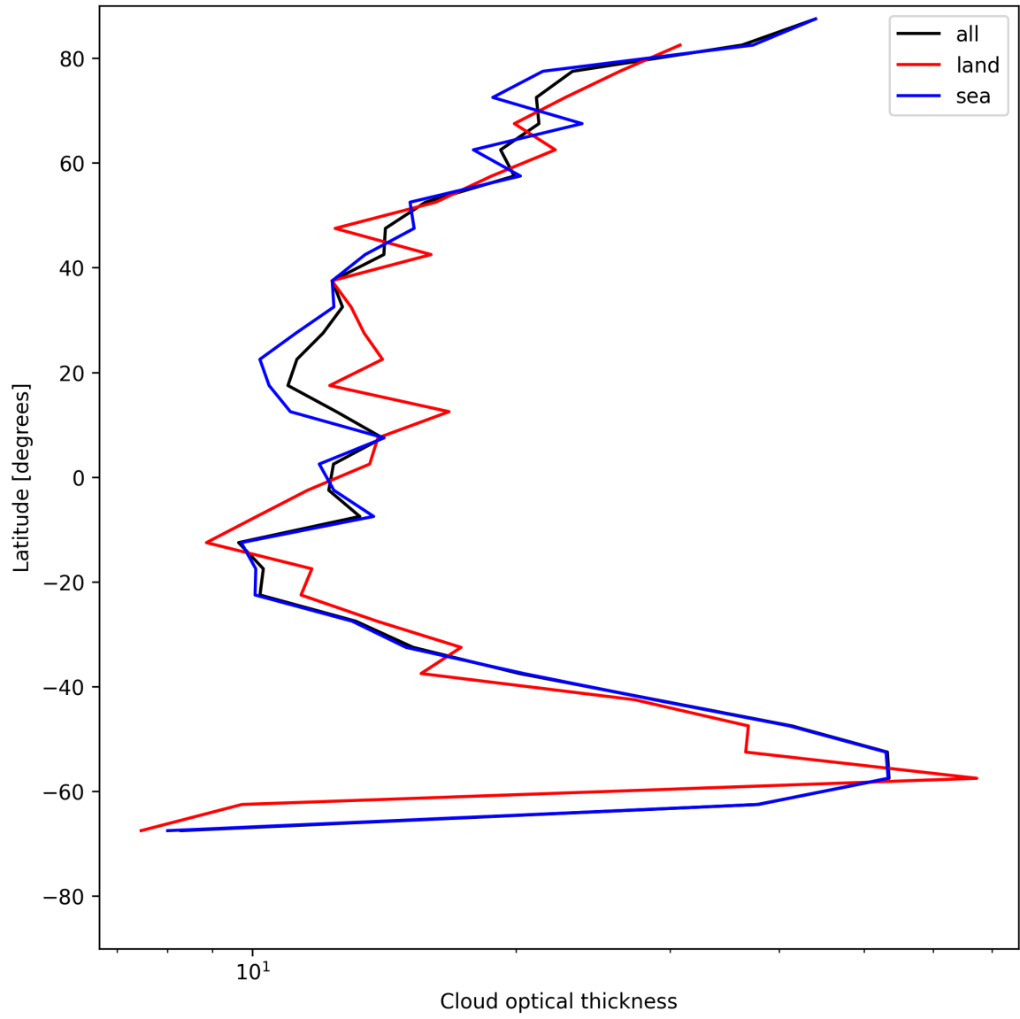
Figure 23: Zonal average of “Cloud optical thickness” for 2025-07-12 to 2025-07-13.
