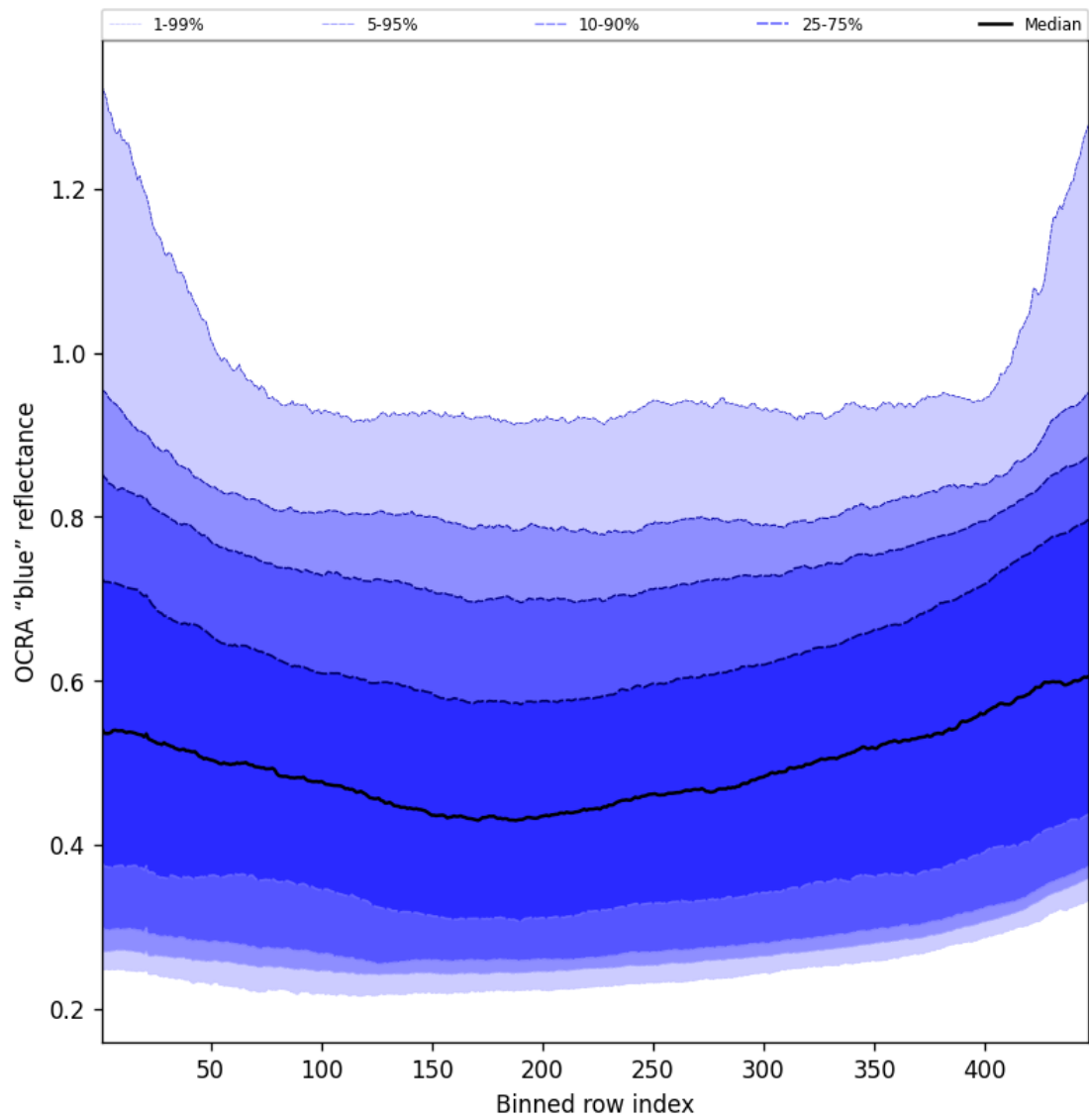
Figure 65: Along track statistics of “OCRA “blue” reflectance” for 2025-07-12 to 2025-07-13
