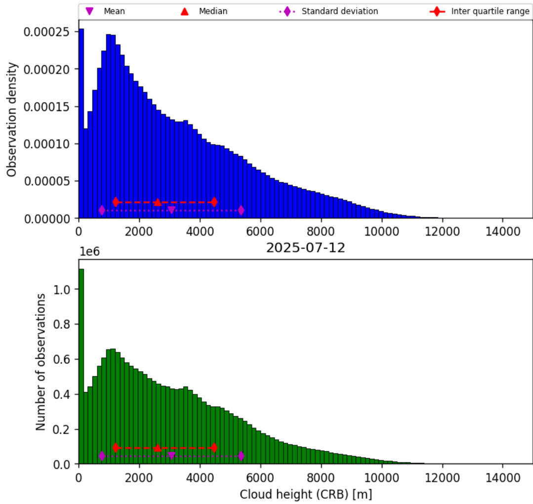
Figure 41: Histogram of “Cloud height (CRB)” for 2025-07-12 to 2025-07-13
