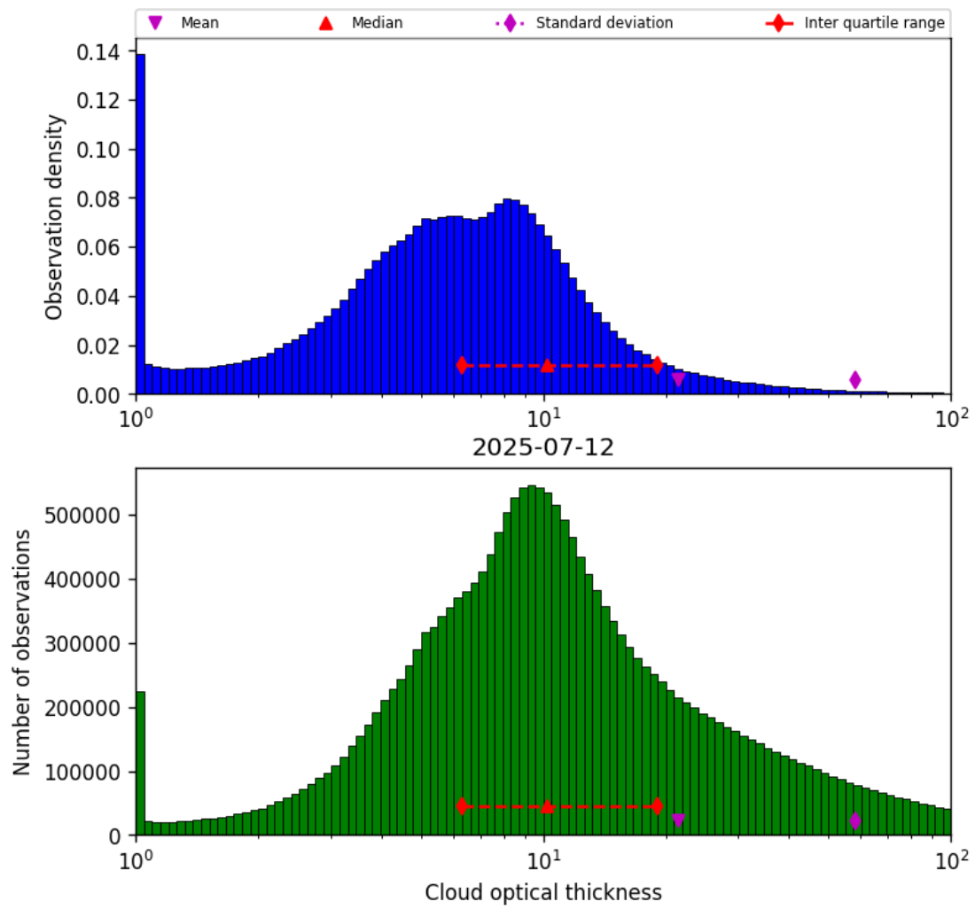
Figure 39: Histogram of “Cloud optical thickness” for 2025-07-12 to 2025-07-13
