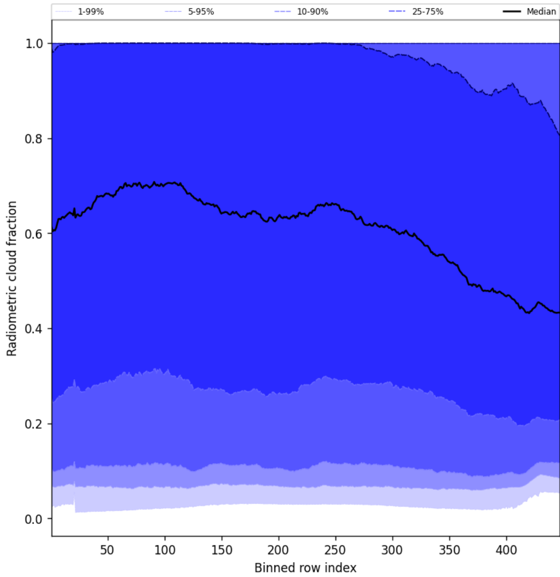
Figure 53: Along track statistics of “Radiometric cloud fraction” for 2025-07-12 to 2025-07-13
