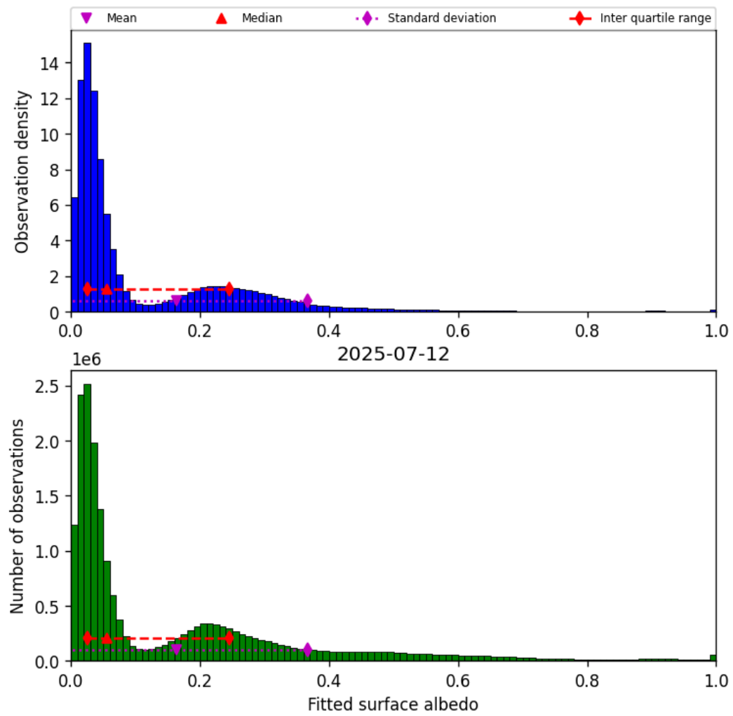
Figure 43: Histogram of “Fitted surface albedo” for 2025-07-12 to 2025-07-13
