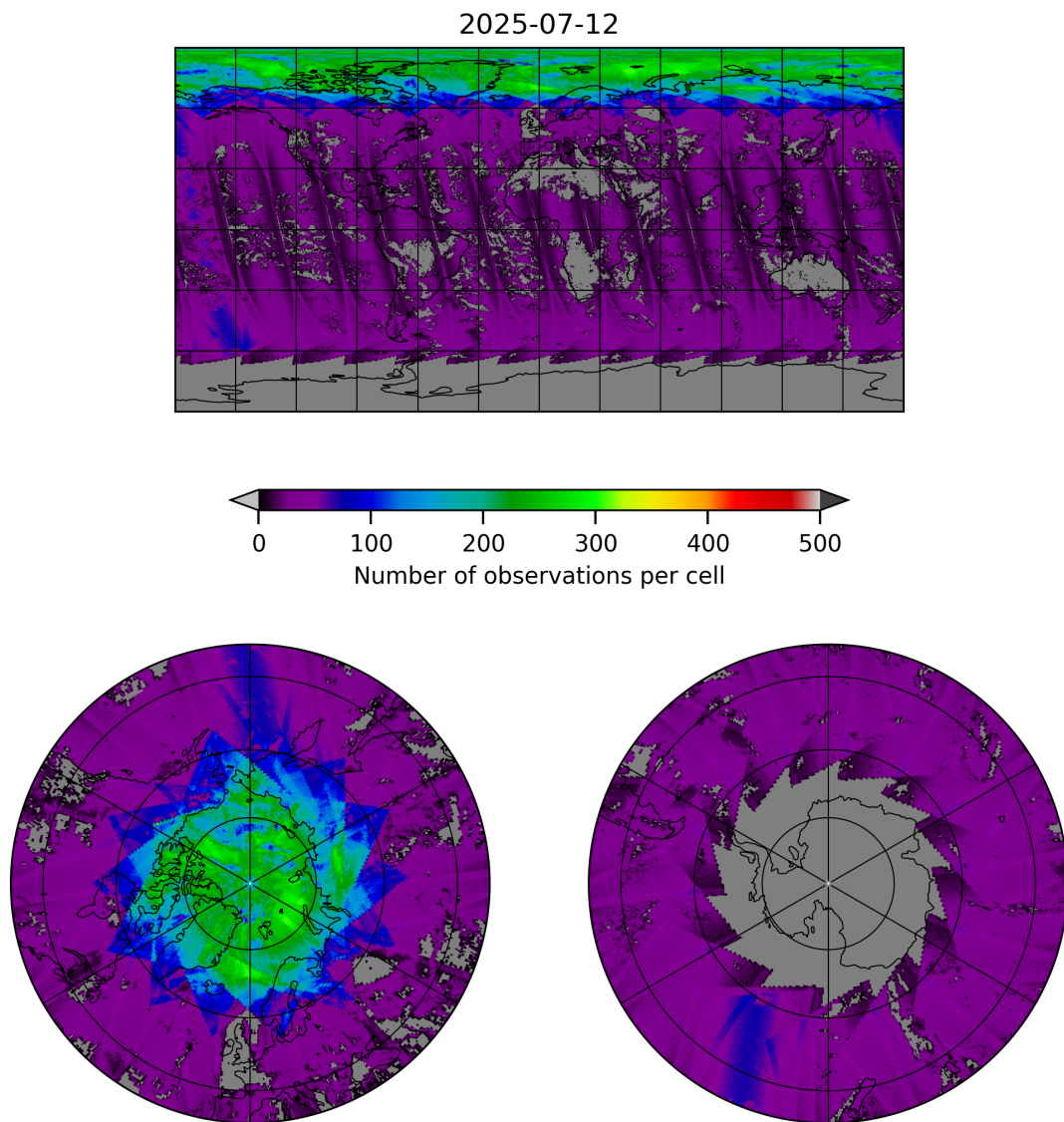
Figure 19: Map of the number of observations for 2025-07-12 to 2025-07-13
