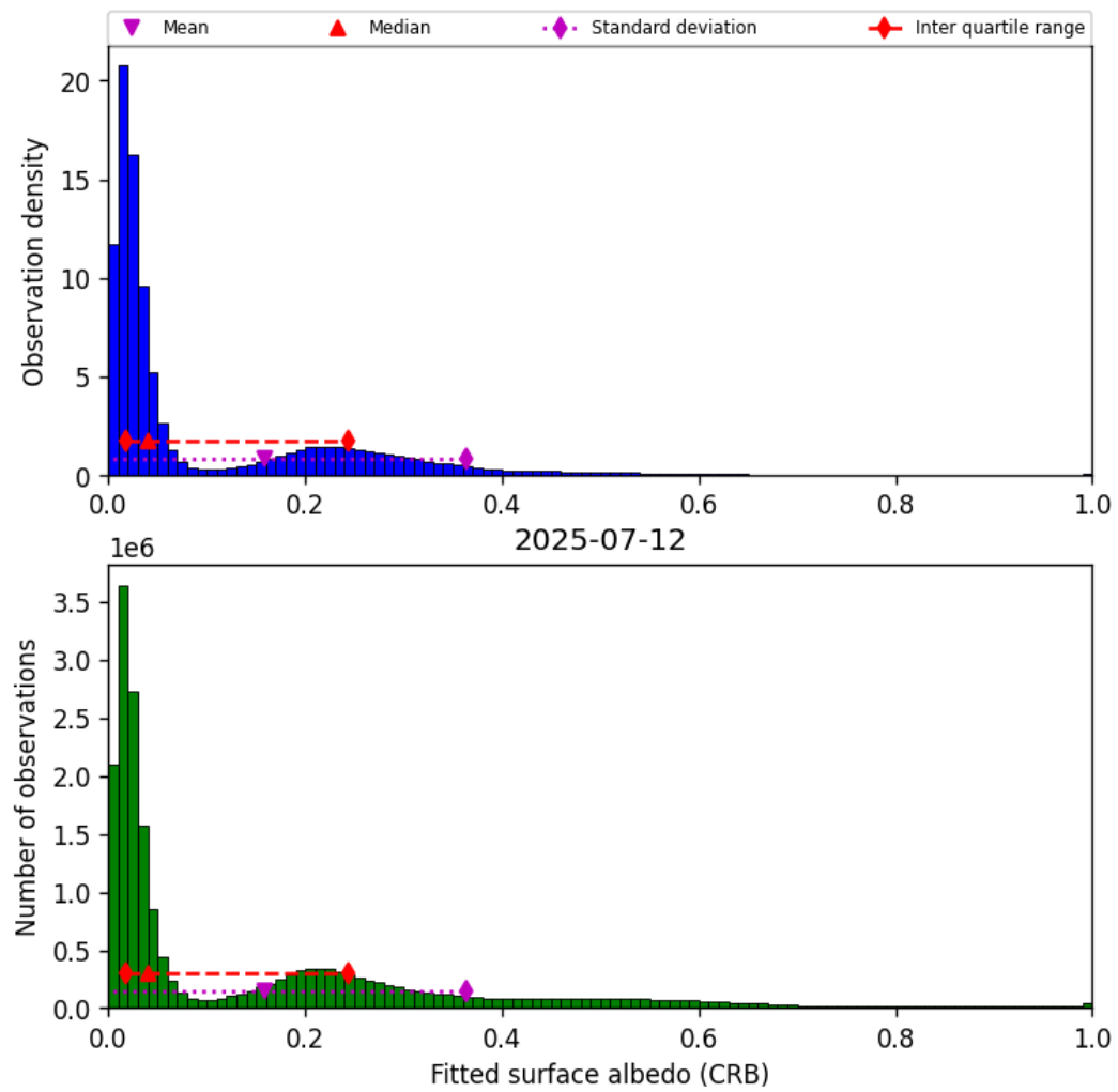
Figure 44: Histogram of “Fitted surface albedo (CRB)” for 2025-07-12 to 2025-07-13
