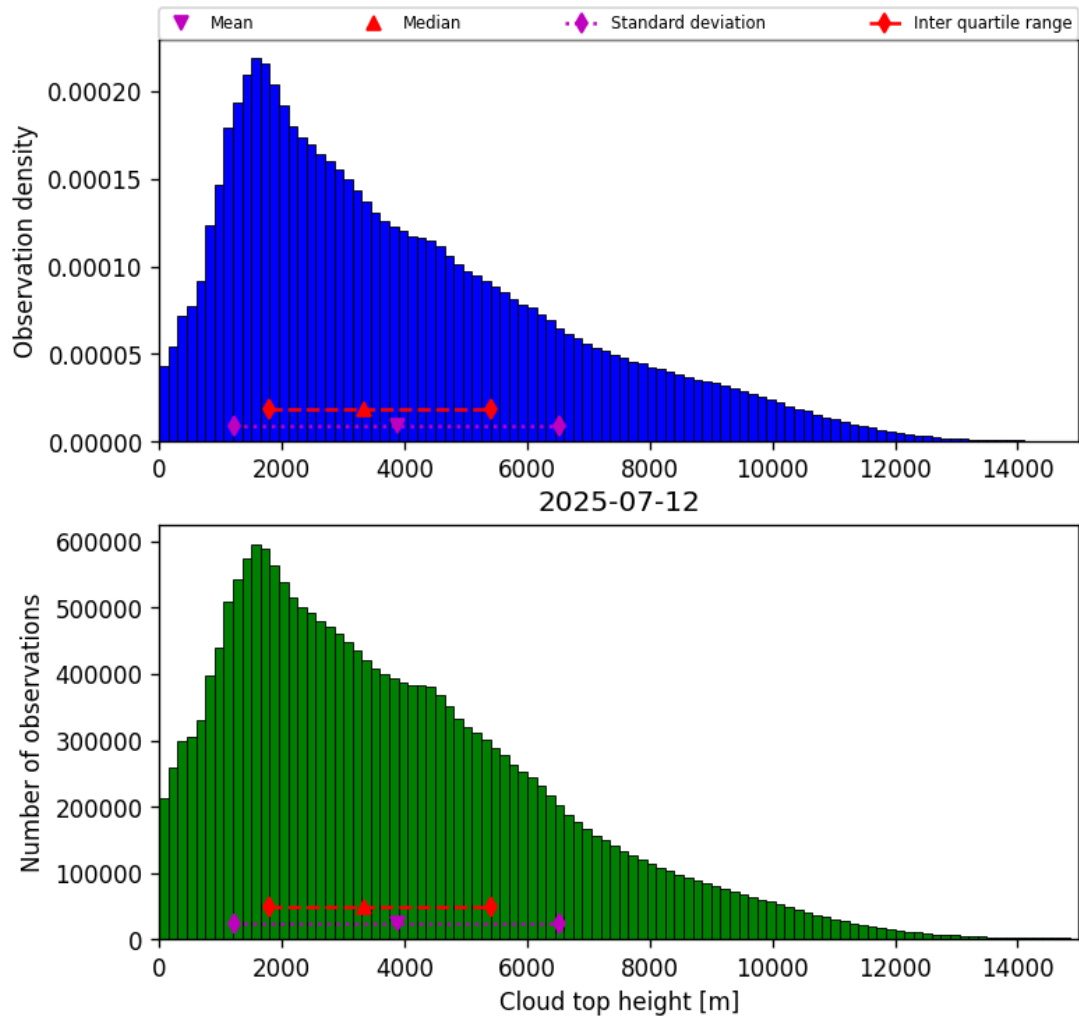
Figure 38: Histogram of “Cloud top height” for 2025-07-12 to 2025-07-13
