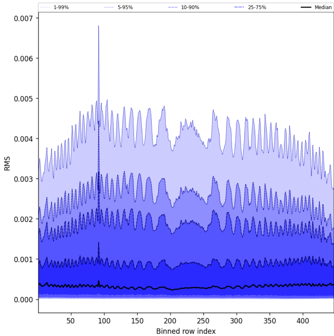
Figure 61: Along track statistics of “RMS” for 2025-07-12 to 2025-07-13
