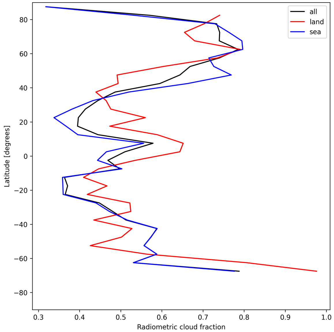
Figure 21: Zonal average of “Radiometric cloud fraction” for 2025-07-12 to 2025-07-13.
