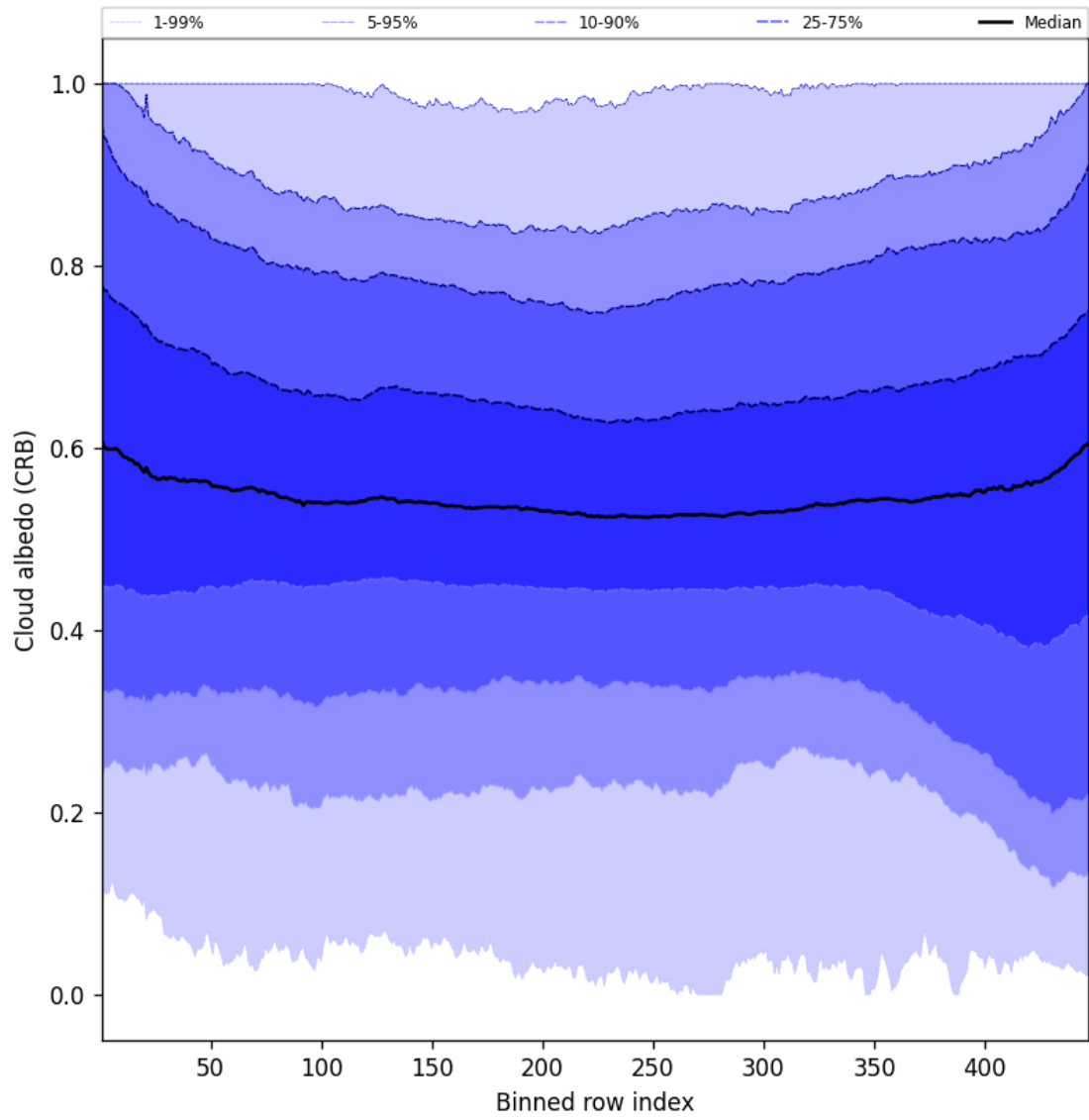
Figure 58: Along track statistics of “Cloud albedo (CRB)” for 2025-07-12 to 2025-07-13
