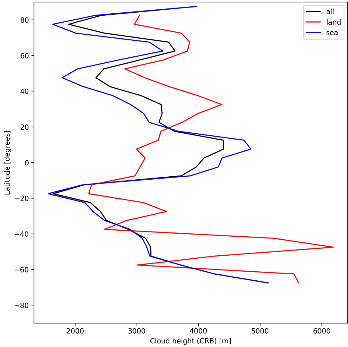
Figure 25: Zonal average of “Cloud height (CRB)” for 2025-07-12 to 2025-07-13.
