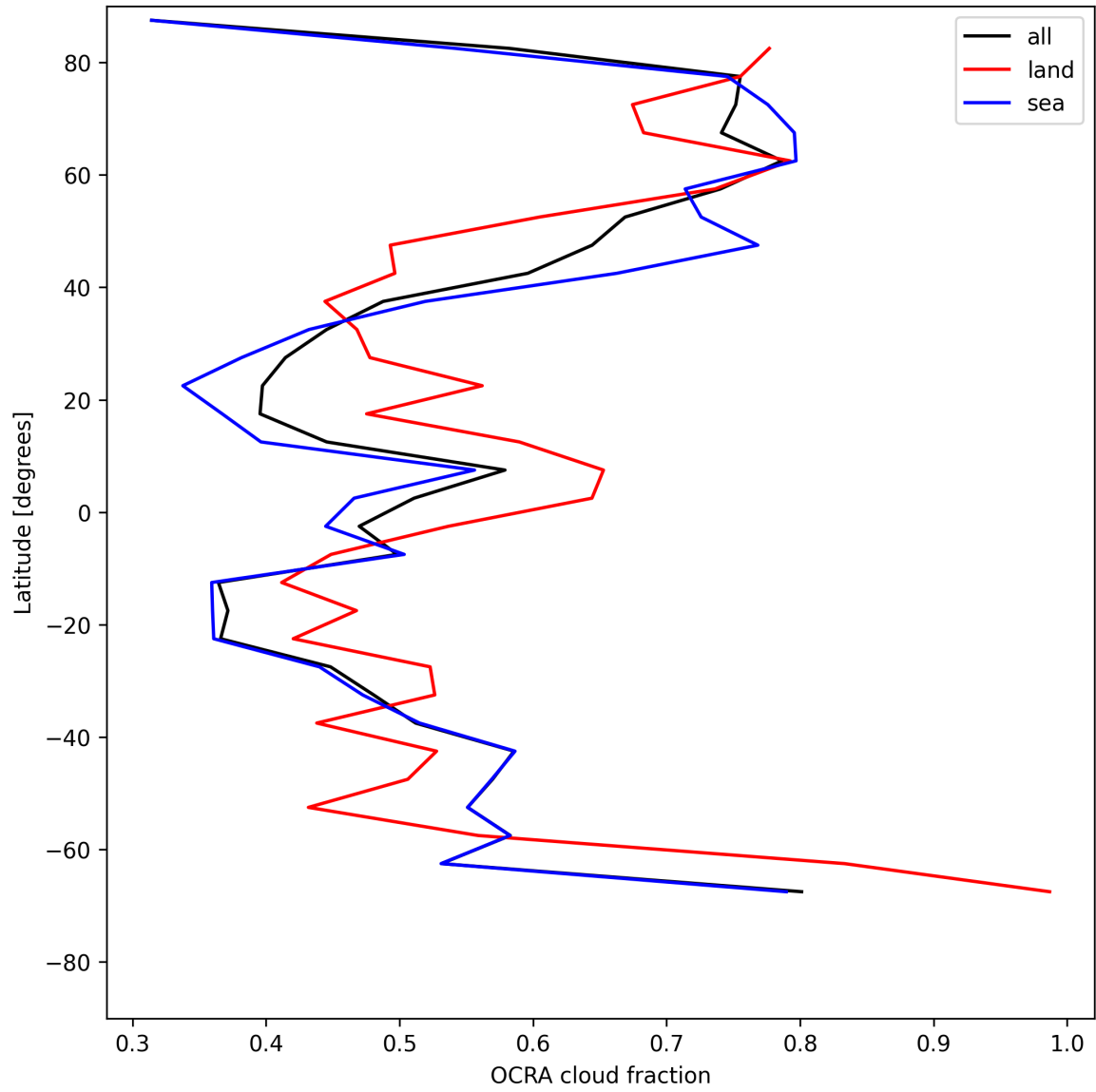
Figure 32: Zonal average of “OCRA cloud fraction” for 2025-07-12 to 2025-07-13.
