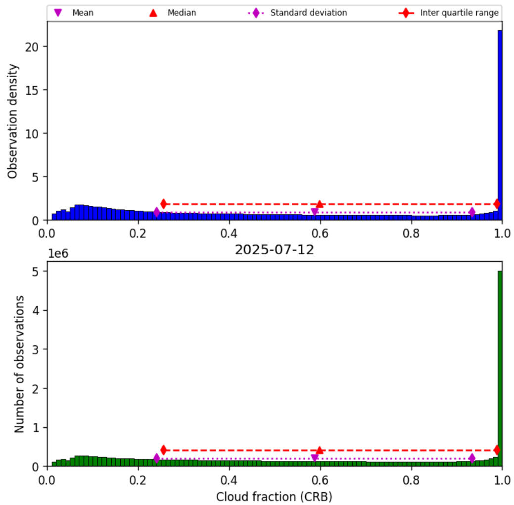
Figure 40: Histogram of “Cloud fraction (CRB)” for 2025-07-12 to 2025-07-13
