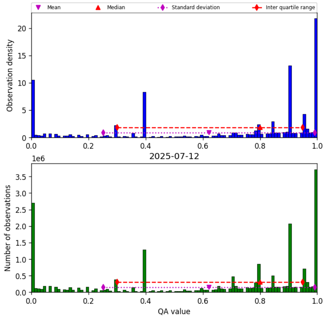
Figure 36: Histogram of “QA value” for 2025-07-12 to 2025-07-13
