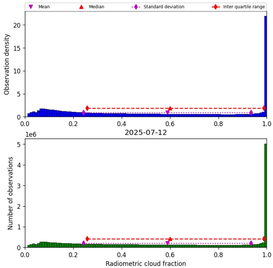
Figure 37: Histogram of “Radiometric cloud fraction” for 2025-07-12 to 2025-07-13
