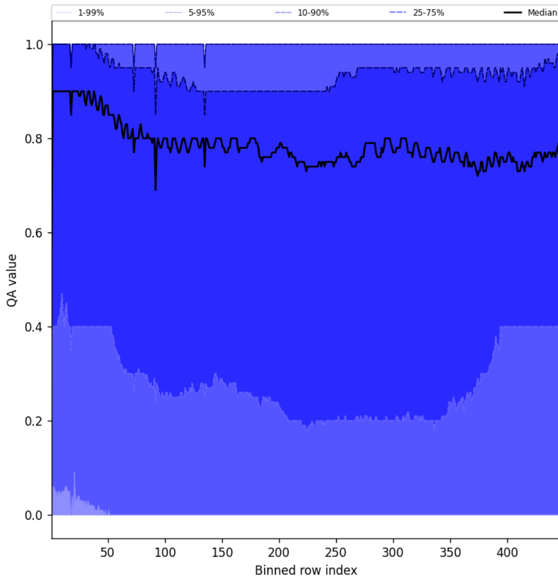
Figure 52: Along track statistics of “QA value” for 2025-07-12 to 2025-07-13
