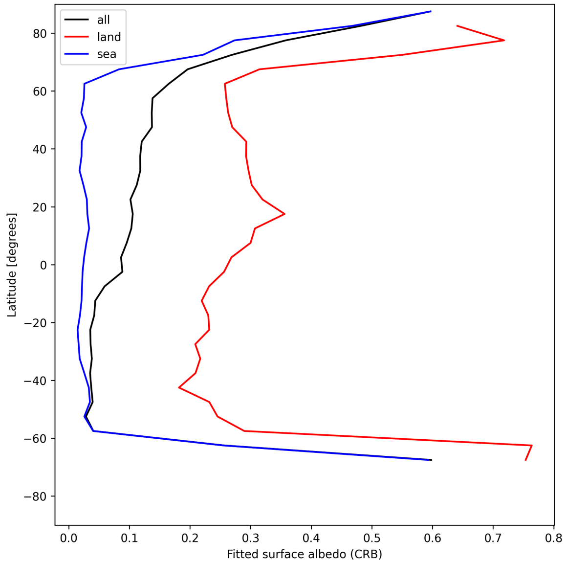
Figure 28: Zonal average of “Fitted surface albedo (CRB)” for 2025-07-12 to 2025-07-13.
