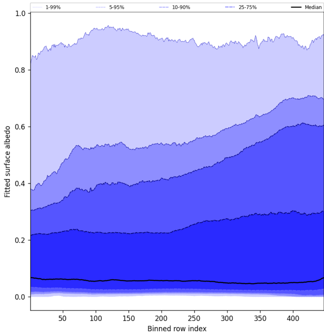
Figure 59: Along track statistics of “Fitted surface albedo” for 2025-07-12 to 2025-07-13
