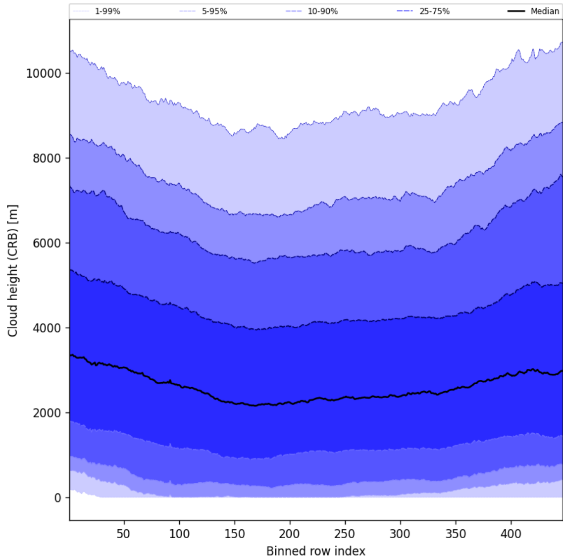
Figure 57: Along track statistics of “Cloud height (CRB)” for 2025-07-12 to 2025-07-13
