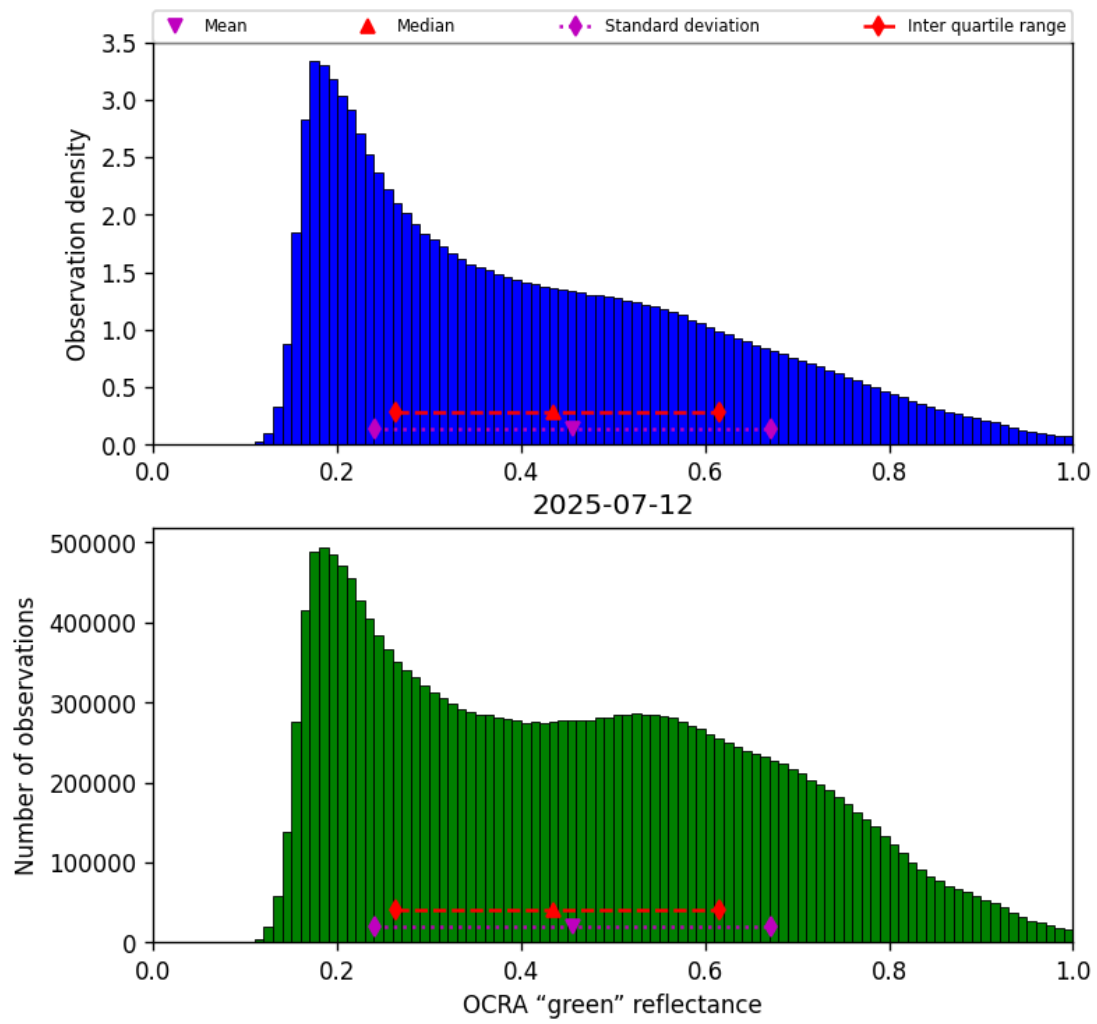
Figure 50: Histogram of “OCRA “green” reflectance” for 2025-07-12 to 2025-07-13
