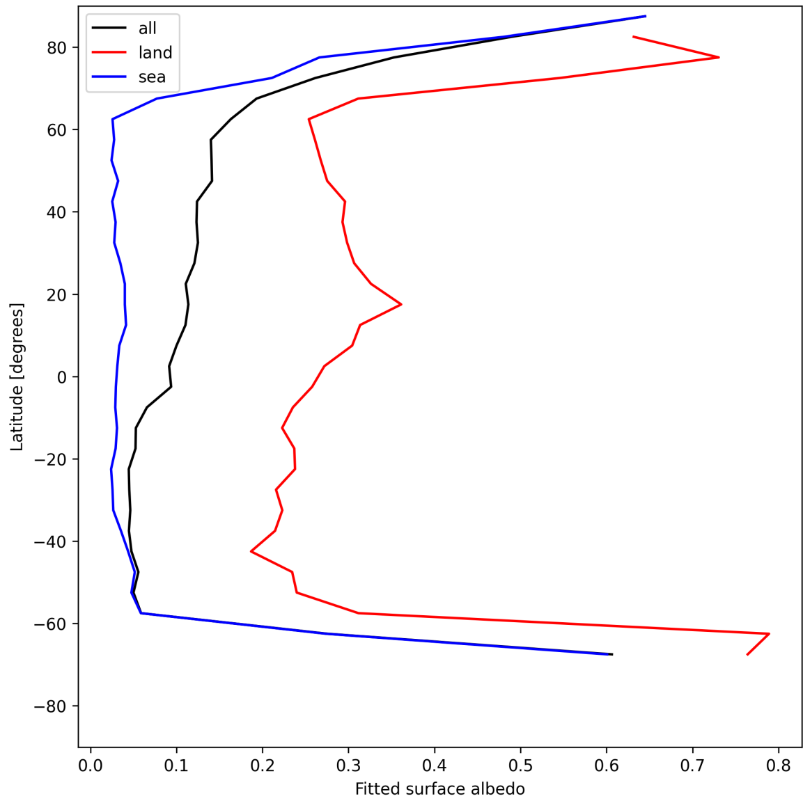
Figure 27: Zonal average of “Fitted surface albedo” for 2025-07-12 to 2025-07-13.
