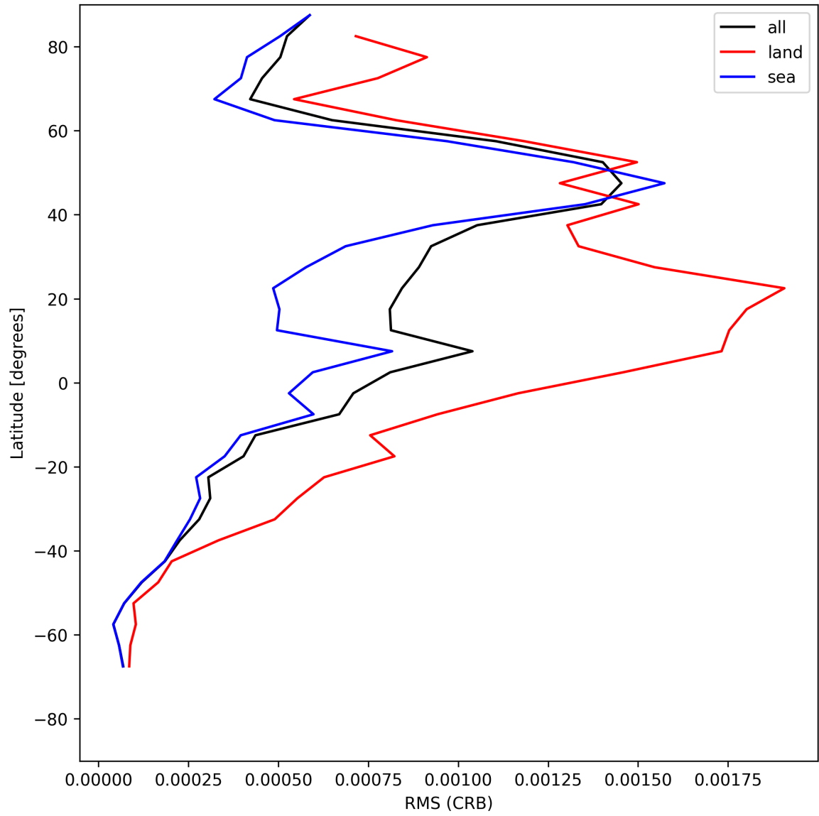
Figure 30: Zonal average of “RMS (CRB)” for 2025-07-12 to 2025-07-13.
