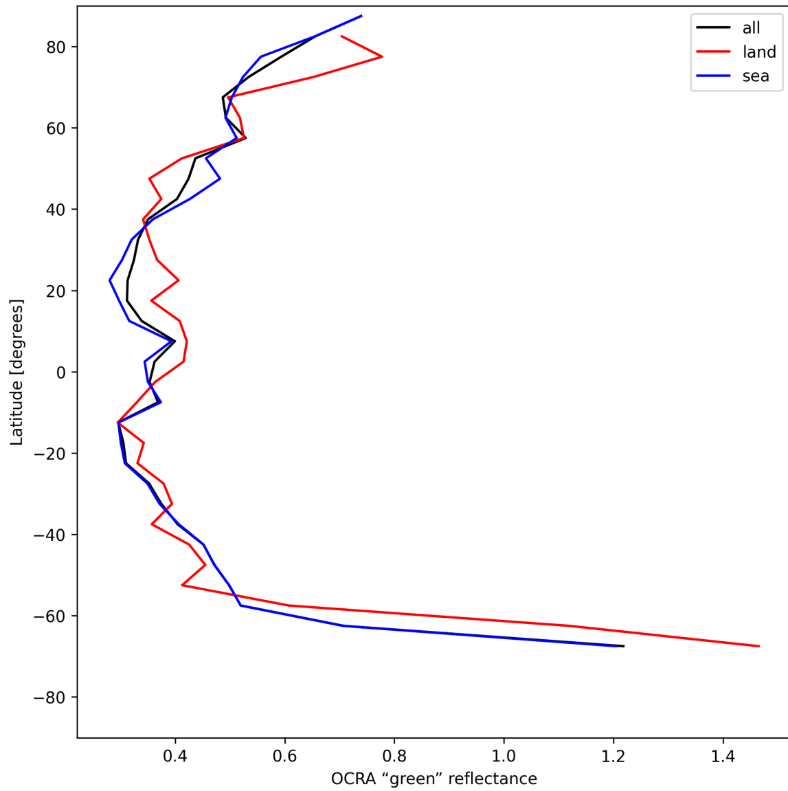
Figure 34: Zonal average of “OCRA “green” reflectance” for 2025-07-12 to 2025-07-13.
