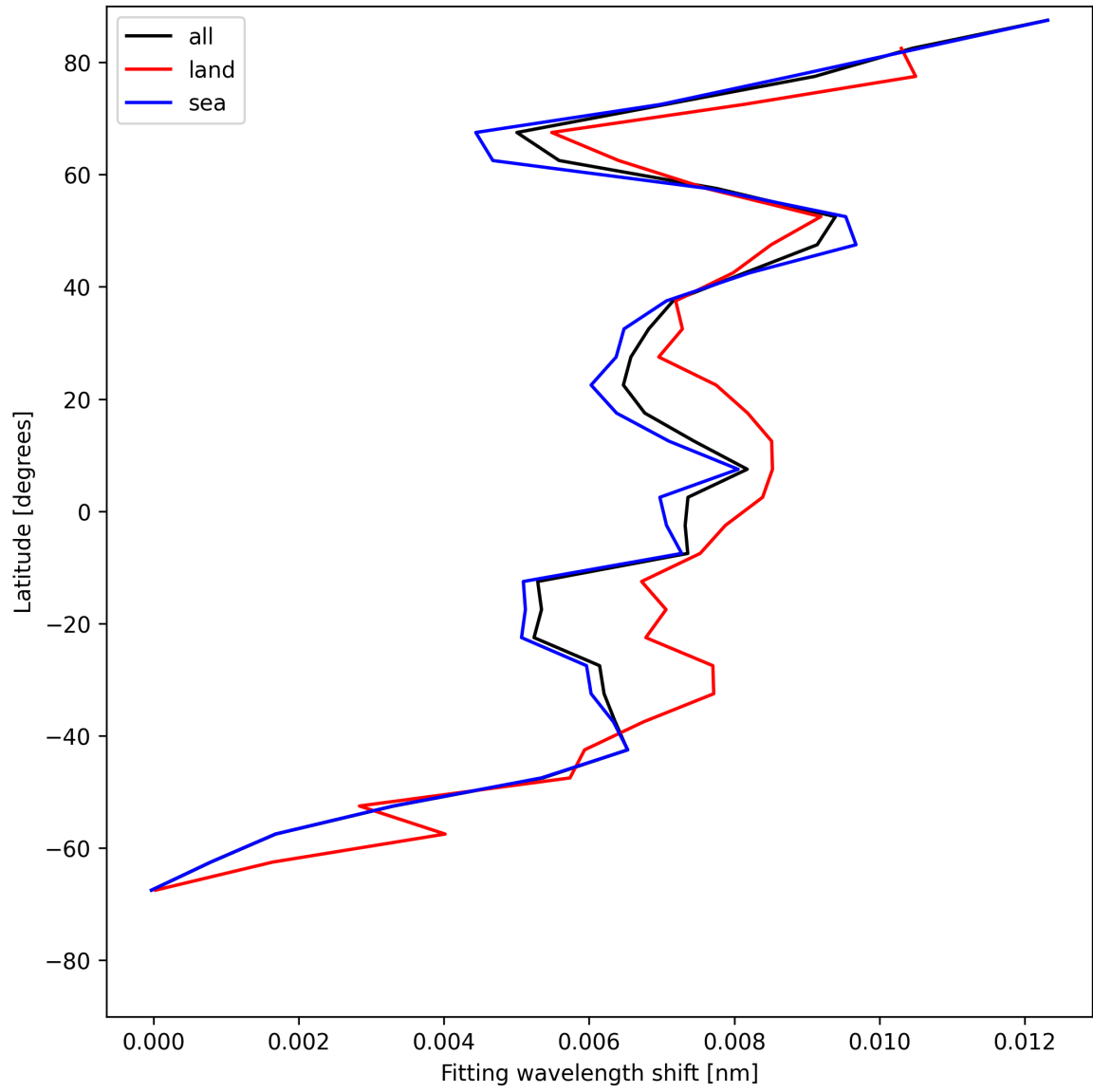
Figure 31: Zonal average of “Fitting wavelength shift” for 2025-07-12 to 2025-07-13.
