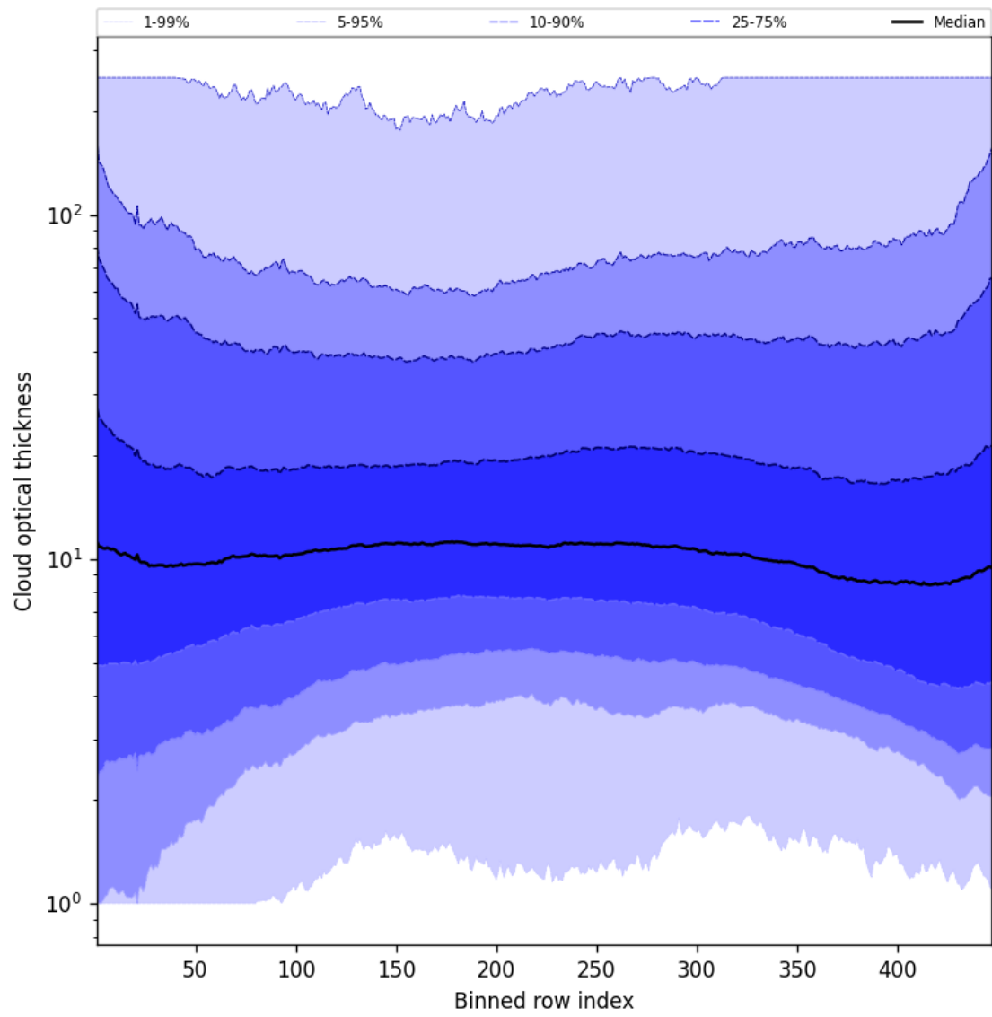
Figure 55: Along track statistics of “Cloud optical thickness” for 2025-07-12 to 2025-07-13
