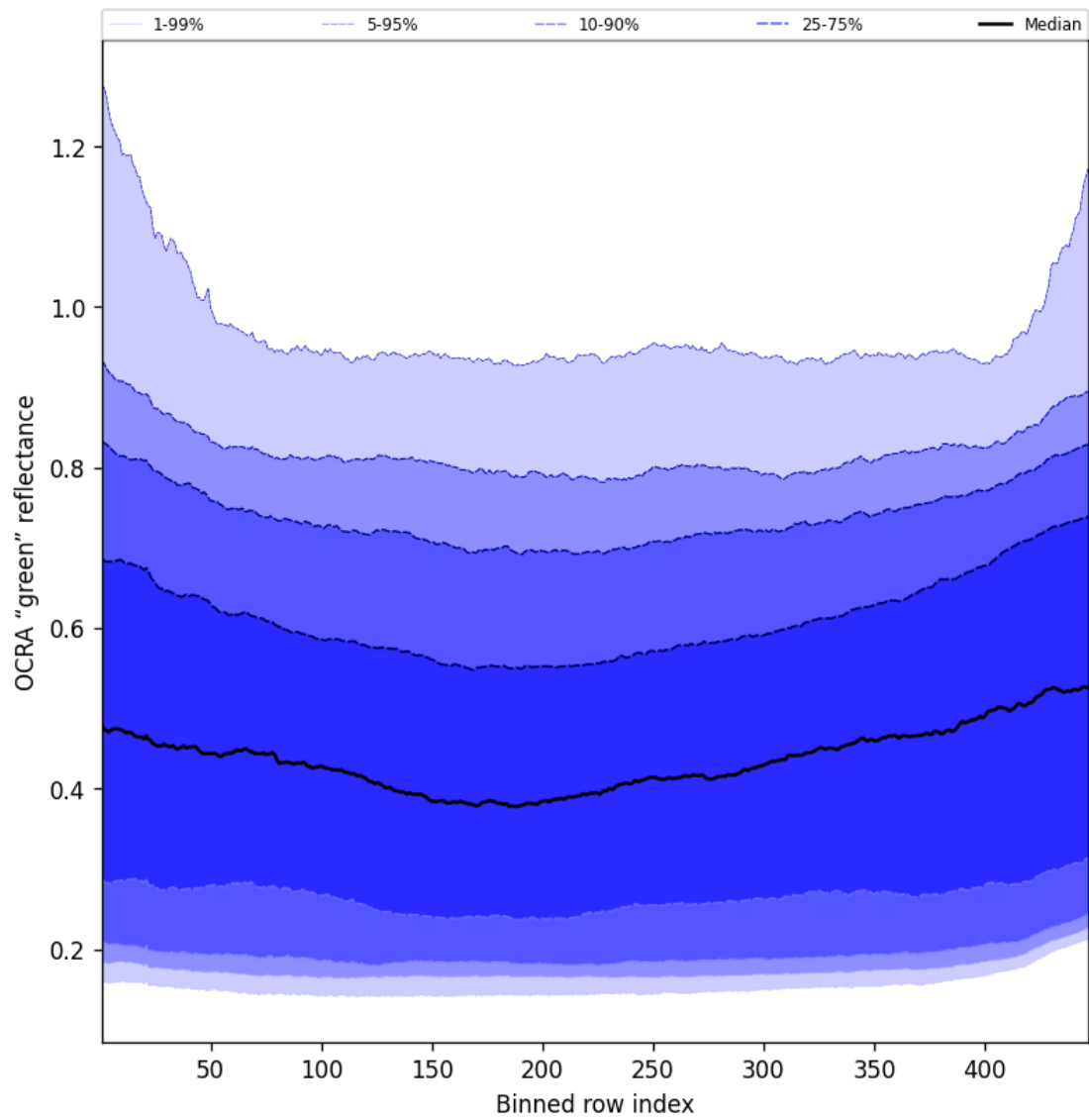
Figure 66: Along track statistics of “OCRA “green” reflectance” for 2025-07-12 to 2025-07-13
