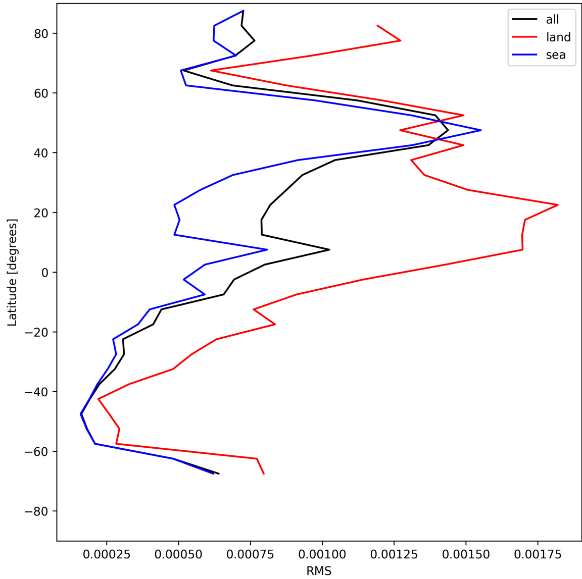
Figure 29: Zonal average of “RMS” for 2025-07-12 to 2025-07-13.
