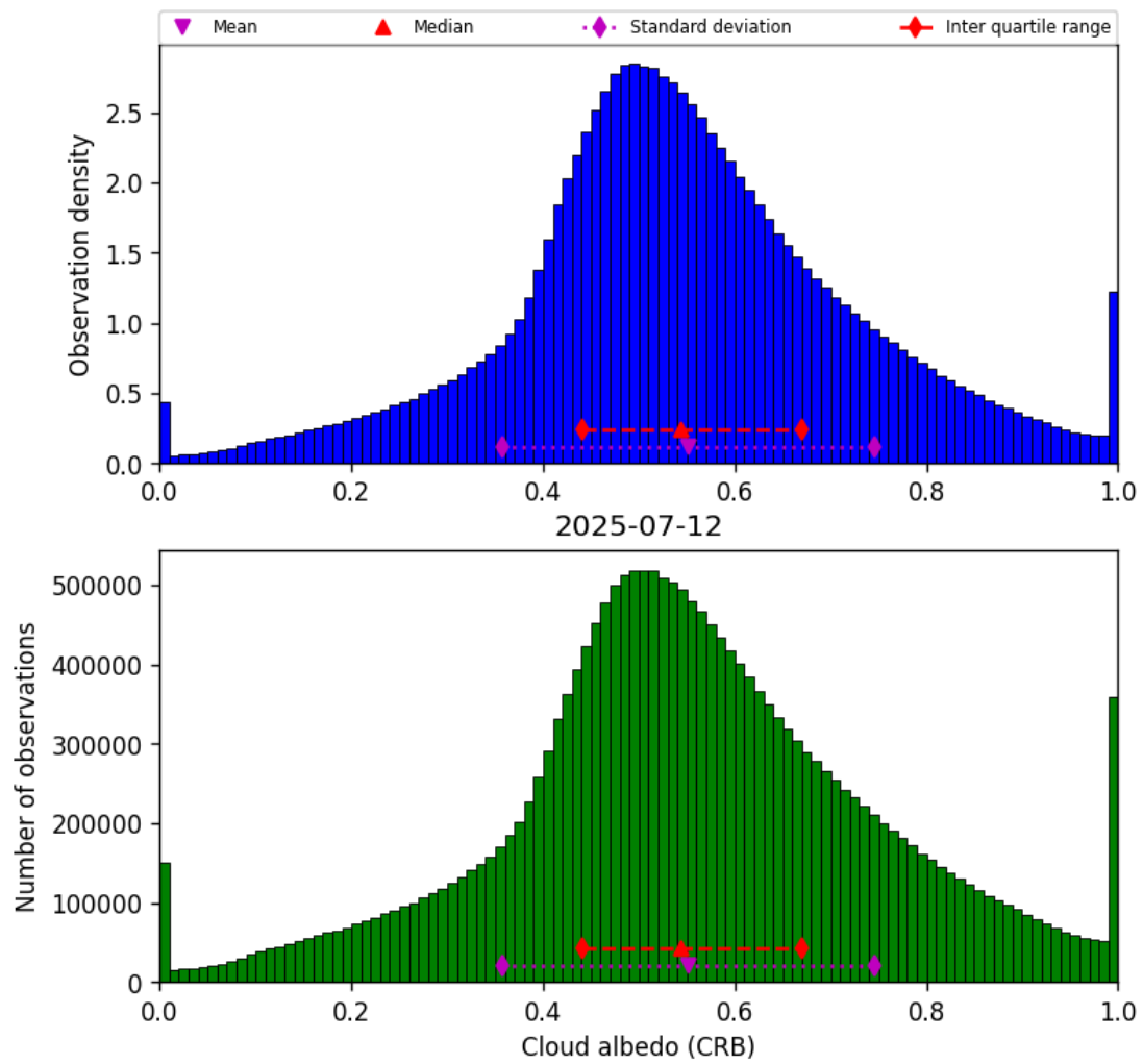
Figure 42: Histogram of “Cloud albedo (CRB)” for 2025-07-12 to 2025-07-13
