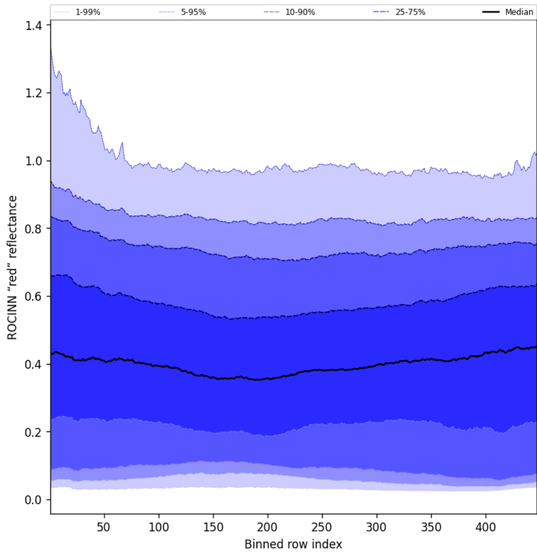
Figure 67: Along track statistics of “ROCINN “red” reflectance” for 2025-07-12 to 2025-07-13
