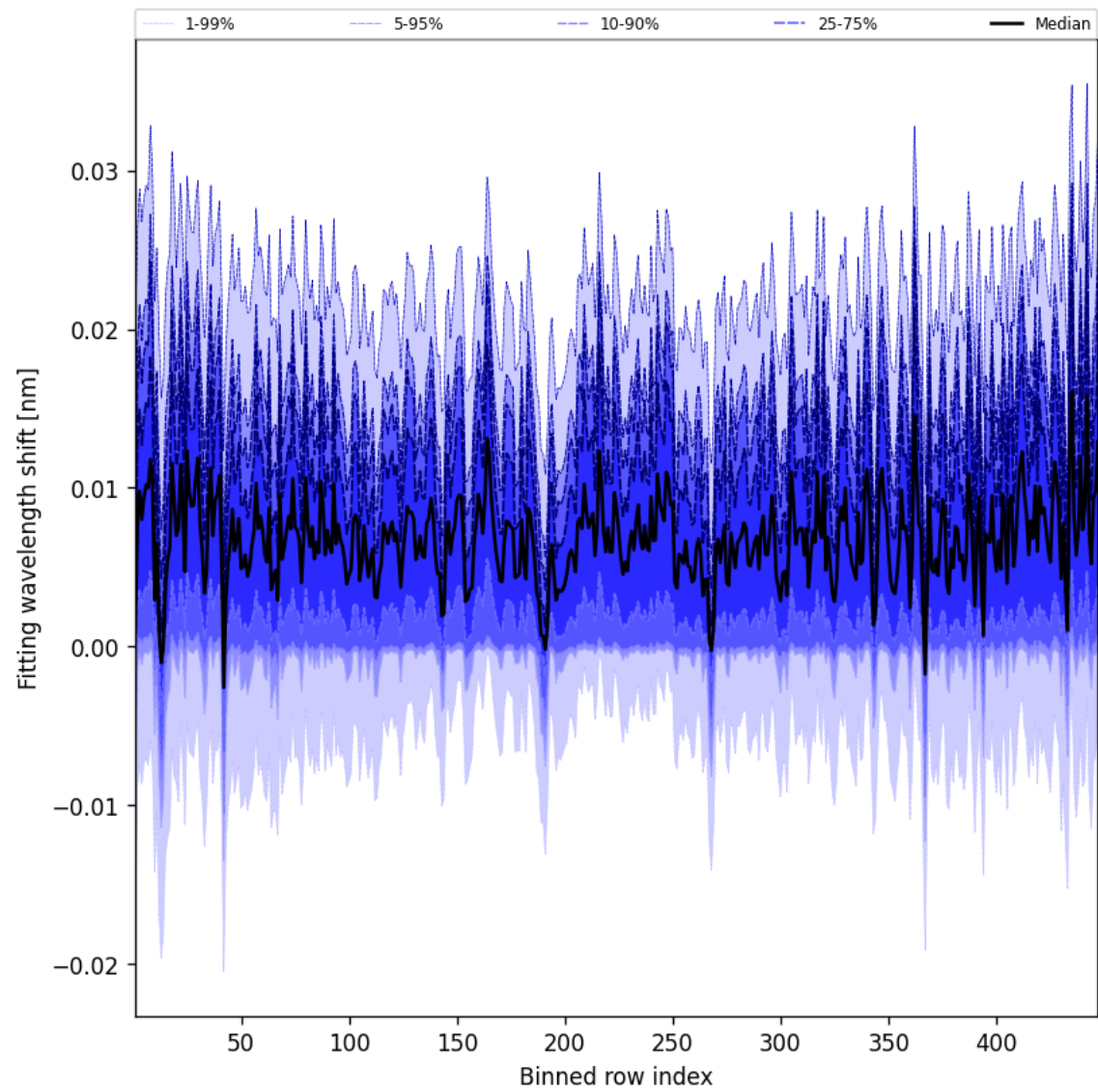
Figure 63: Along track statistics of “Fitting wavelength shift” for 2025-07-12 to 2025-07-13
