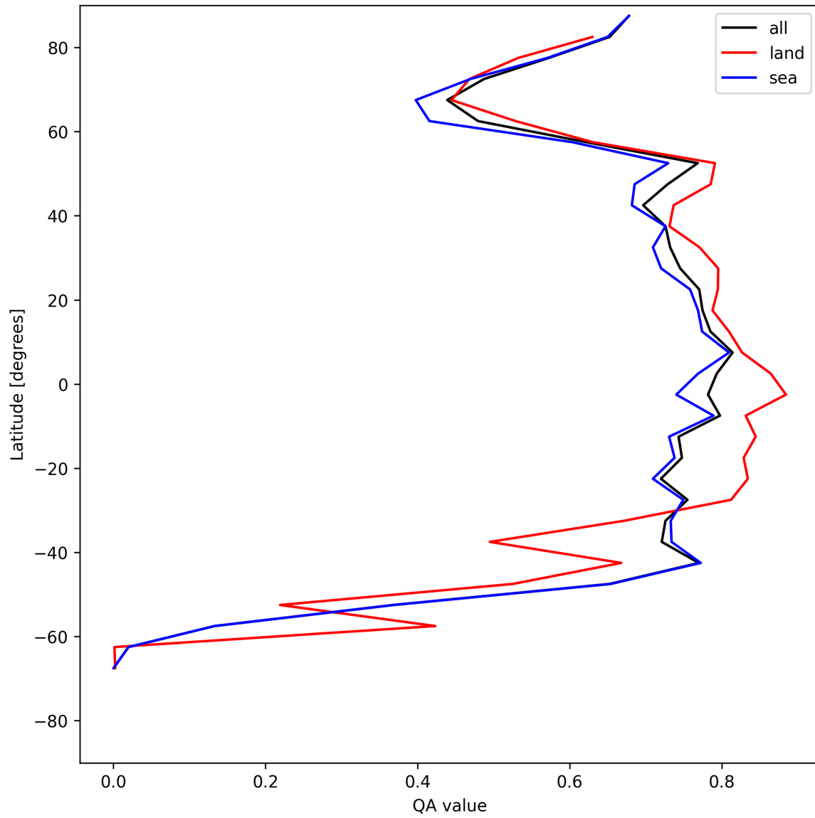
Figure 20: Zonal average of “QA value” for 2025-07-12 to 2025-07-13.
