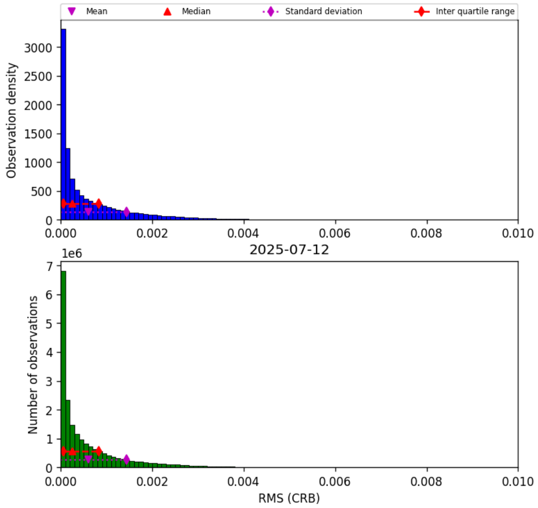
Figure 46: Histogram of "RMS (CRB)" for 2025-07-12 to 2025-07-13
