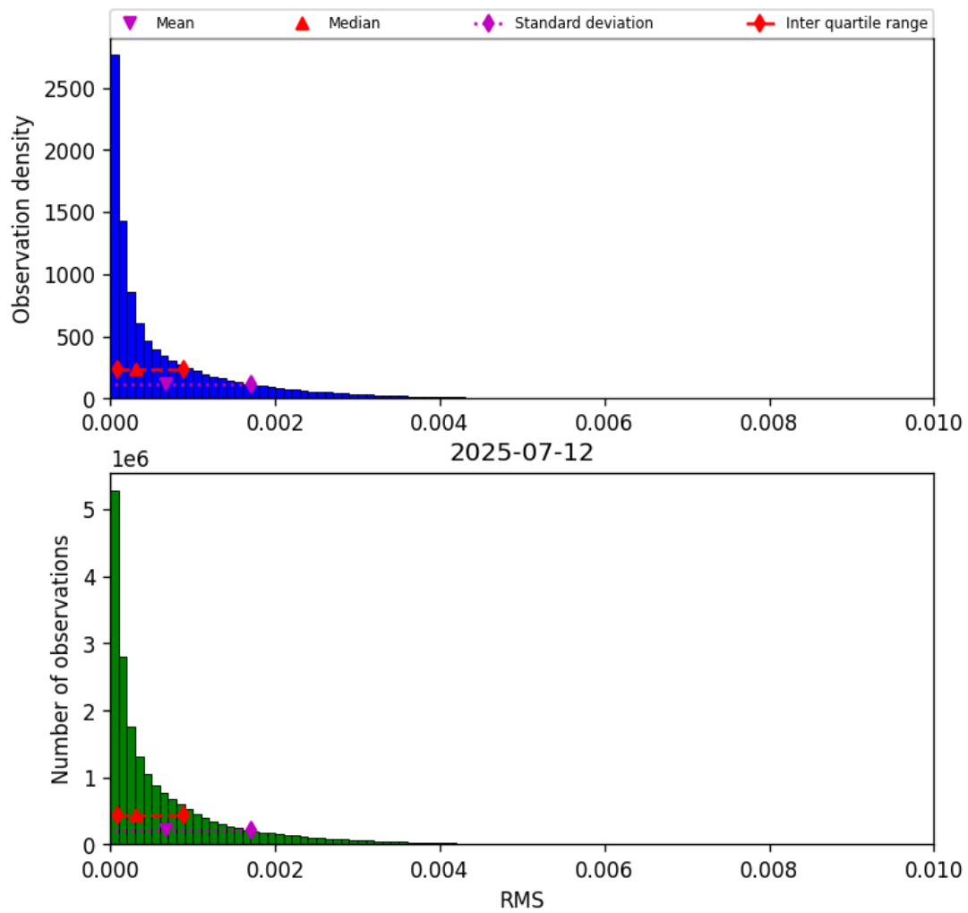
Figure 45: Histogram of “RMS” for 2025-07-12 to 2025-07-13
