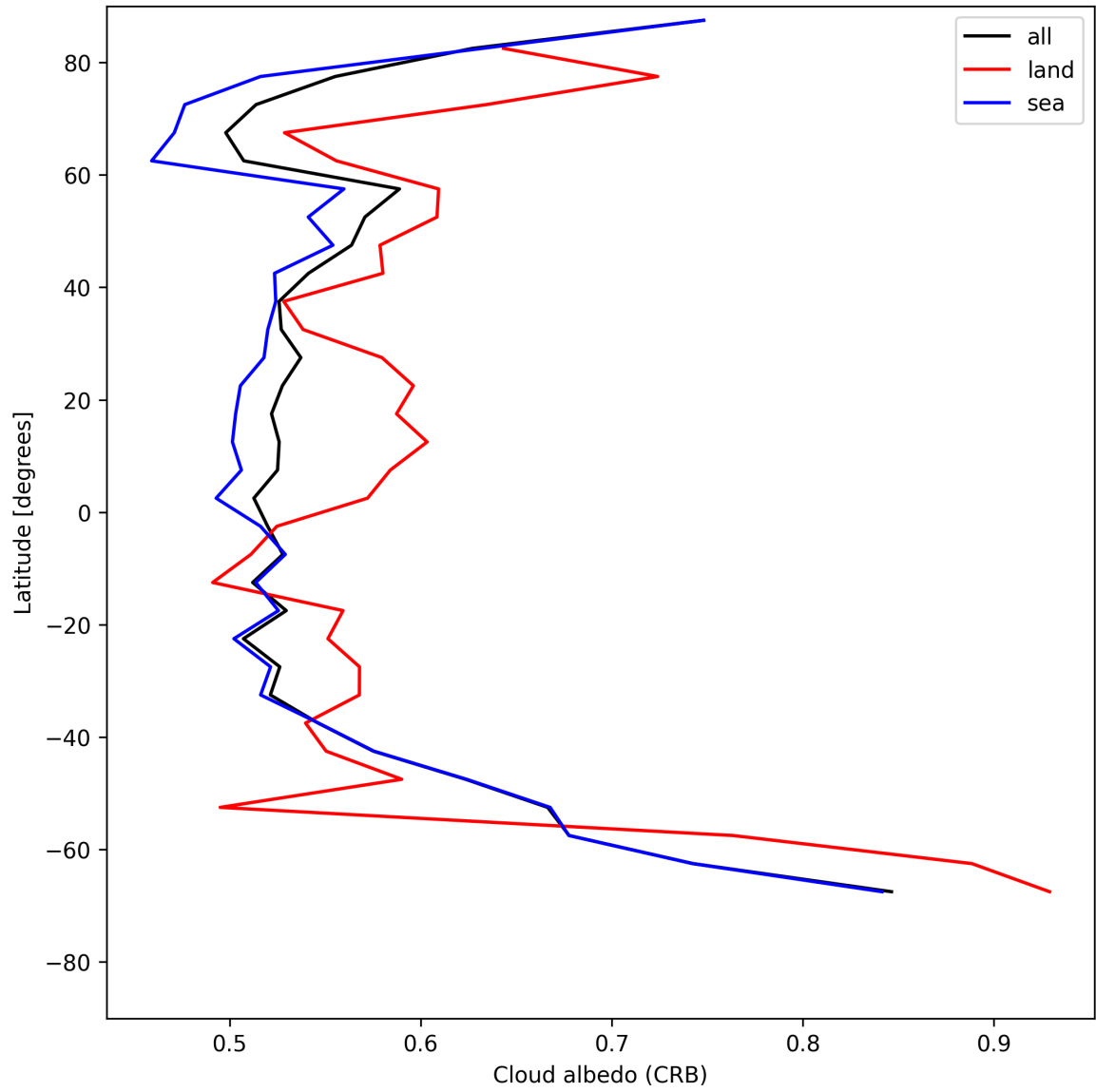
Figure 26: Zonal average of “Cloud albedo (CRB)” for 2025-07-12 to 2025-07-13.
