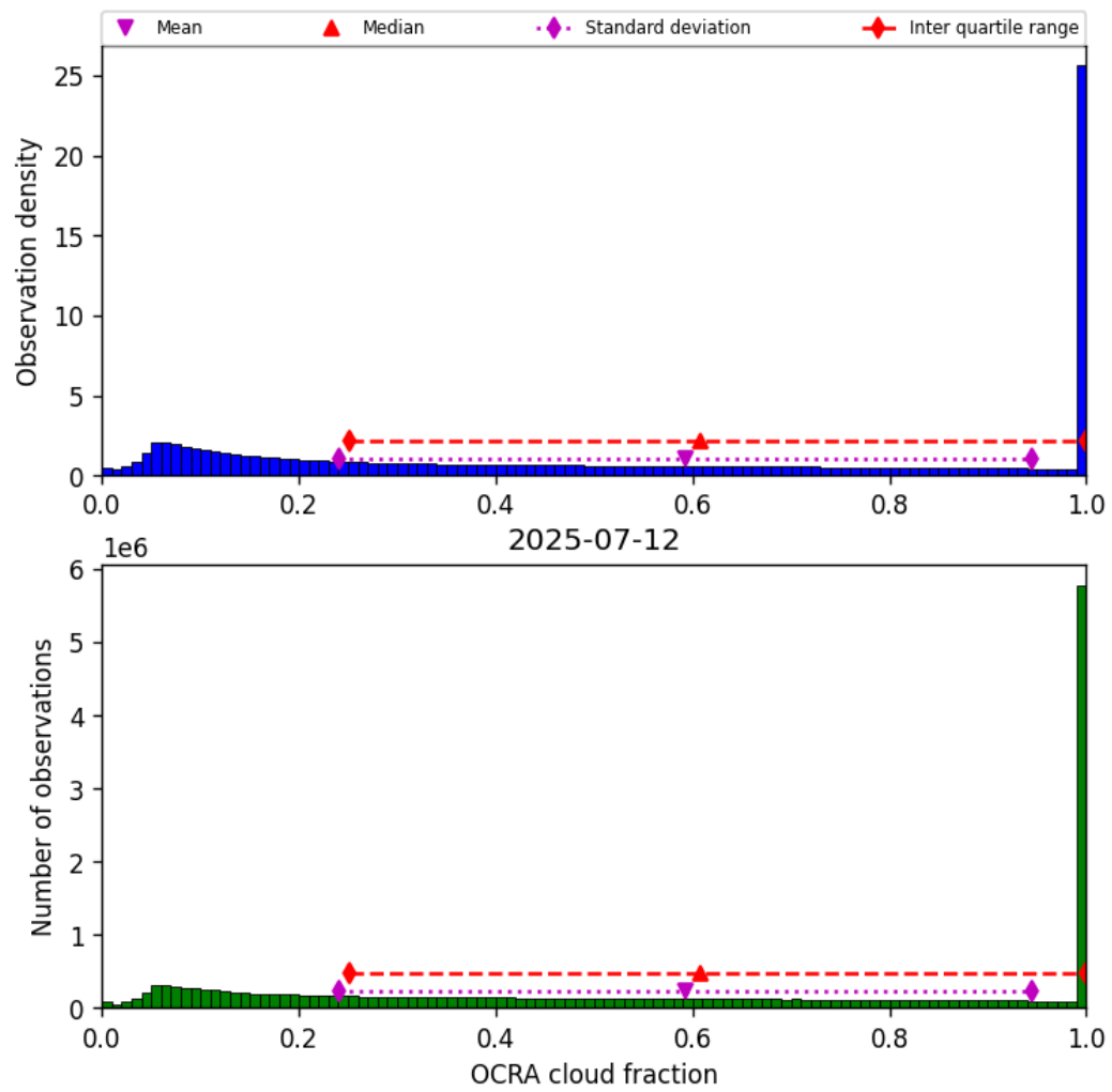
Figure 48: Histogram of “OCRA cloud fraction” for 2025-07-12 to 2025-07-13
