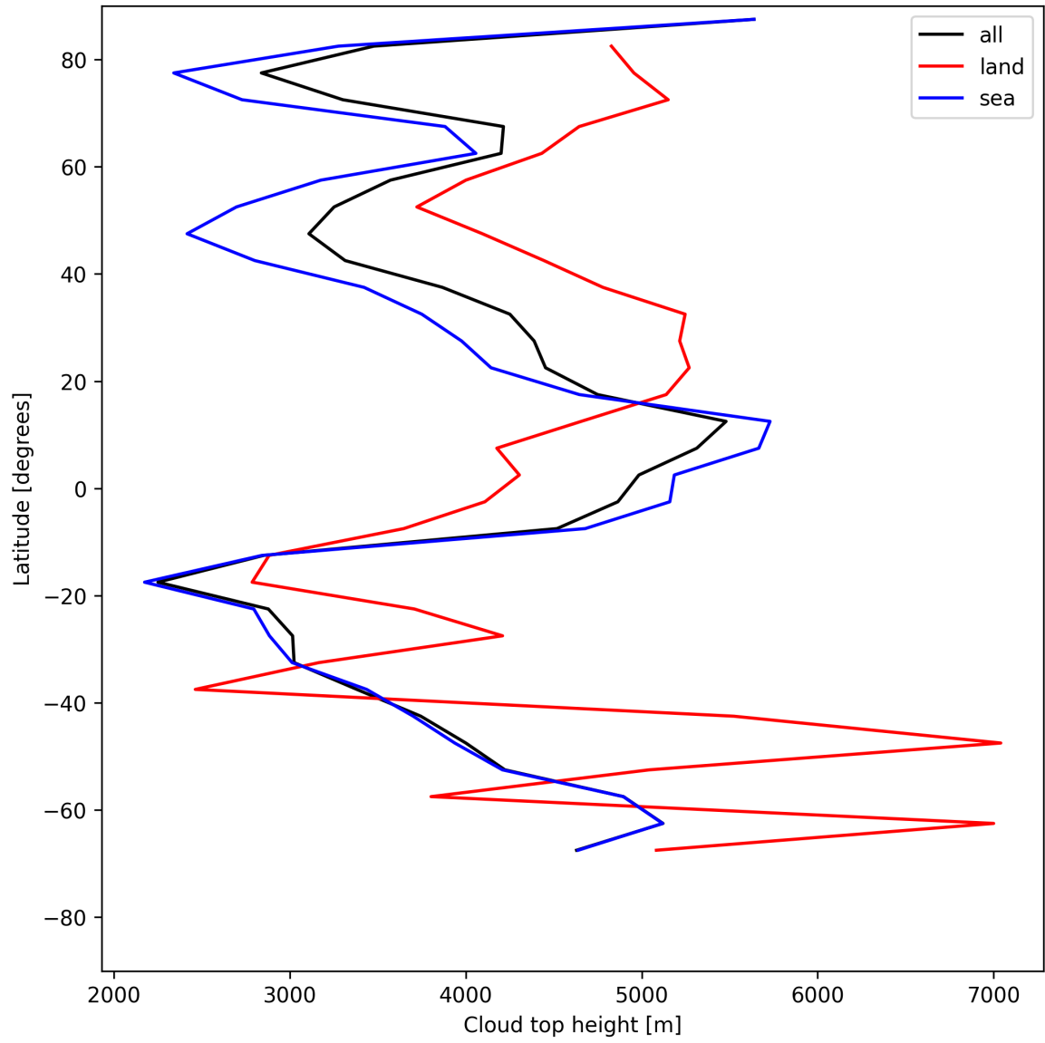
Figure 22: Zonal average of “Cloud top height” for 2025-07-12 to 2025-07-13.
