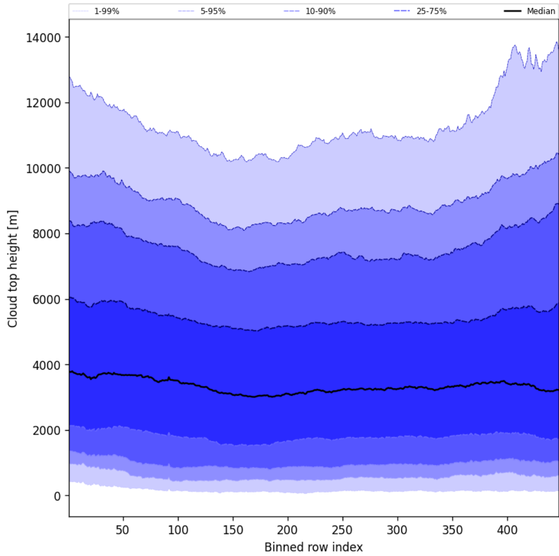
Figure 54: Along track statistics of “Cloud top height” for 2025-07-12 to 2025-07-13
