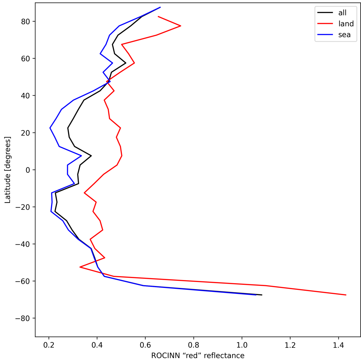
Figure 35: Zonal average of “ROCINN “red” reflectance” for 2025-07-12 to 2025-07-13.
