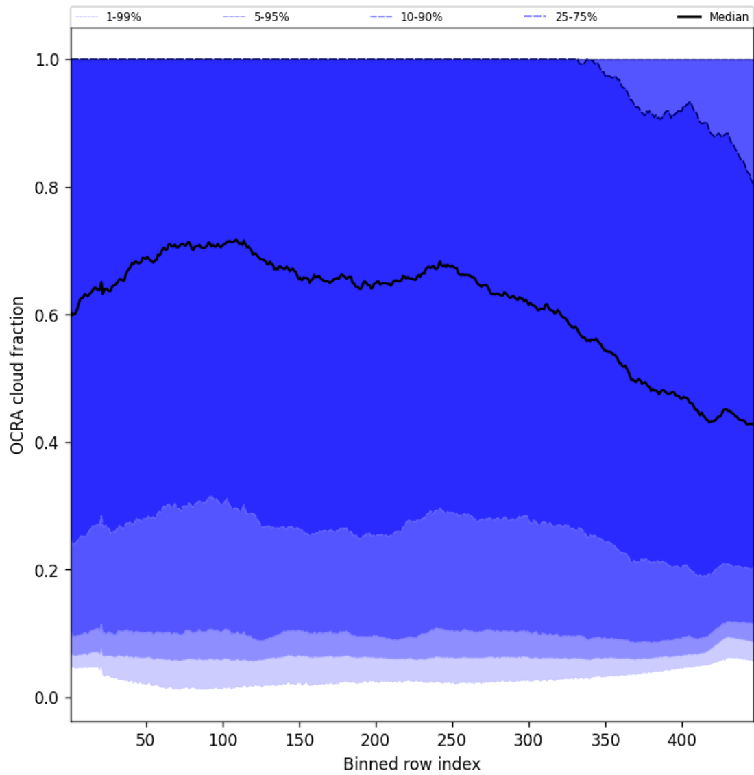
Figure 64: Along track statistics of “OCRA cloud fraction” for 2025-07-12 to 2025-07-13
