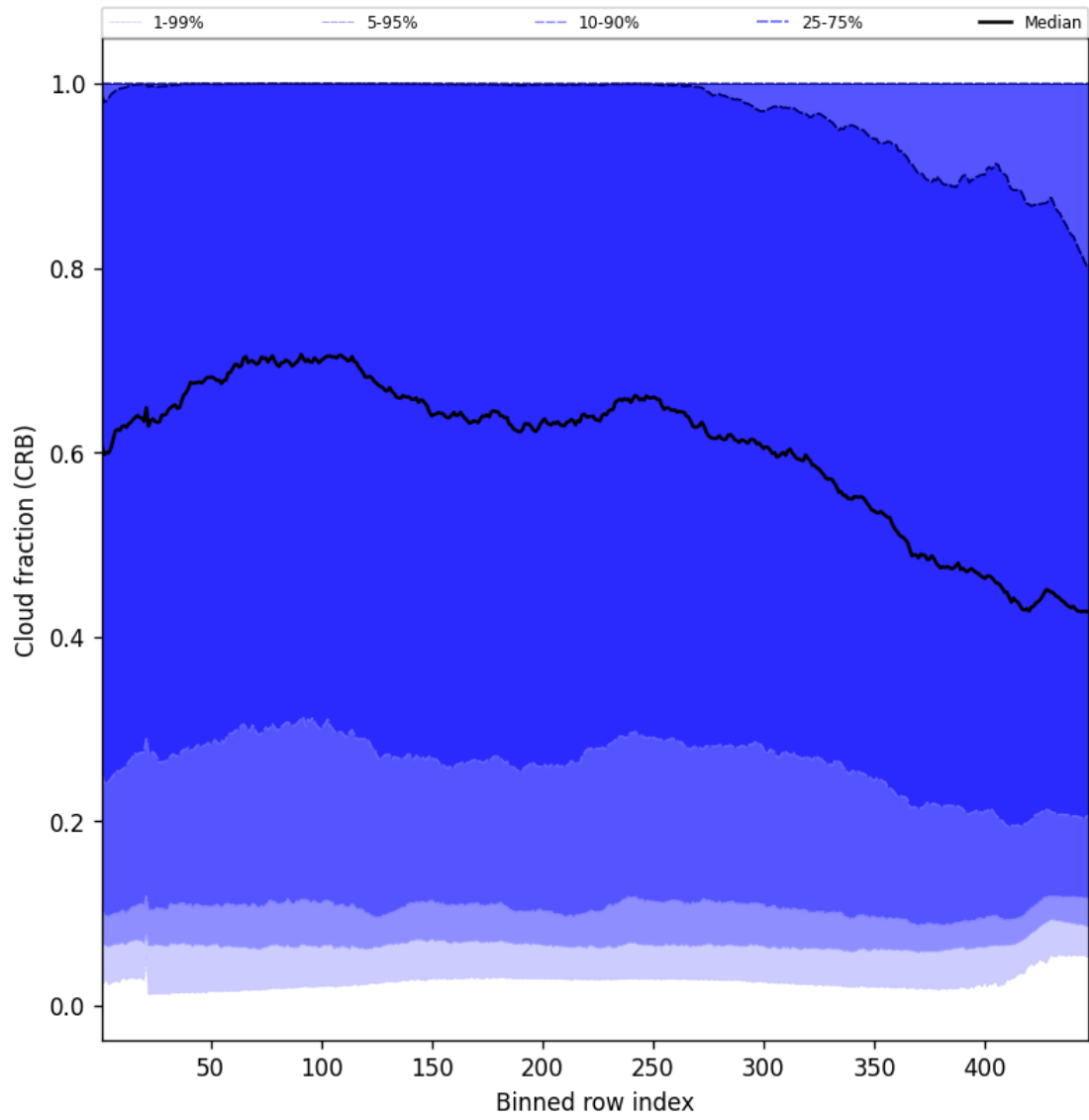
Figure 56: Along track statistics of “Cloud fraction (CRB)” for 2025-07-12 to 2025-07-13
