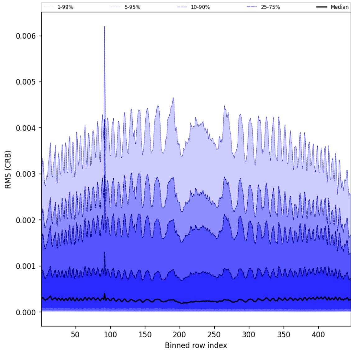
Figure 62: Along track statistics of “RMS (CRB)” for 2025-07-12 to 2025-07-13
