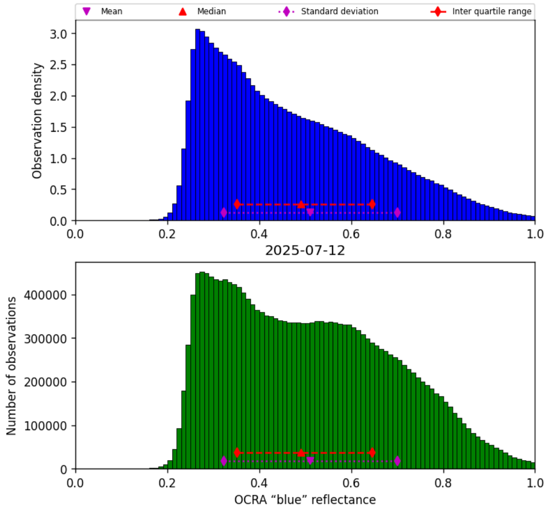
Figure 49: Histogram of “OCRA “blue” reflectance” for 2025-07-12 to 2025-07-13
