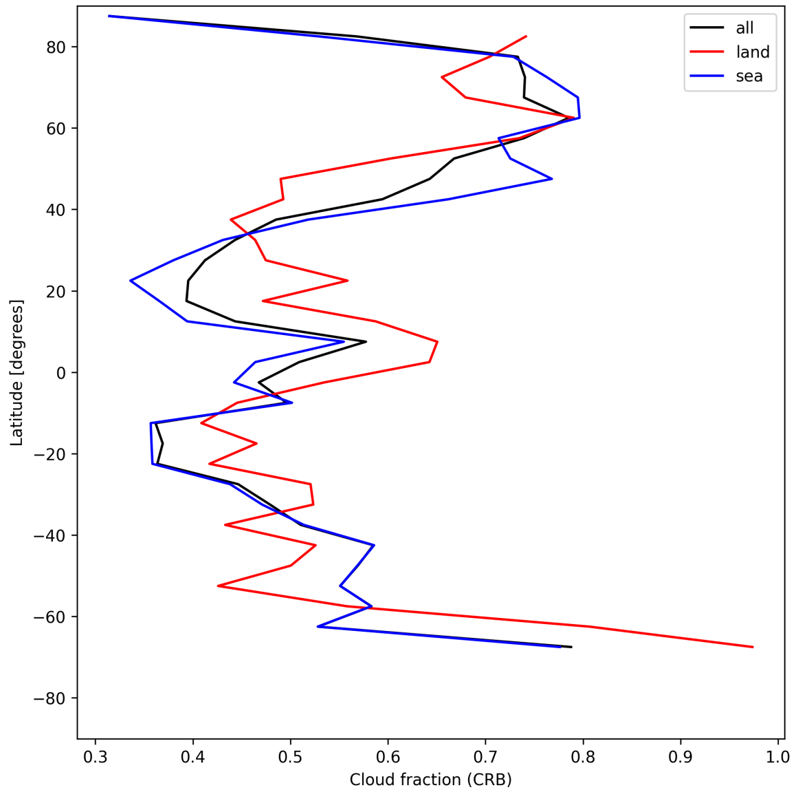
Figure 24: Zonal average of “Cloud fraction (CRB)” for 2025-07-12 to 2025-07-13.
