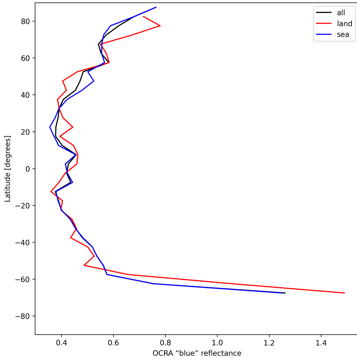
Figure 33: Zonal average of “OCRA “blue” reflectance” for 2025-07-12 to 2025-07-13.
