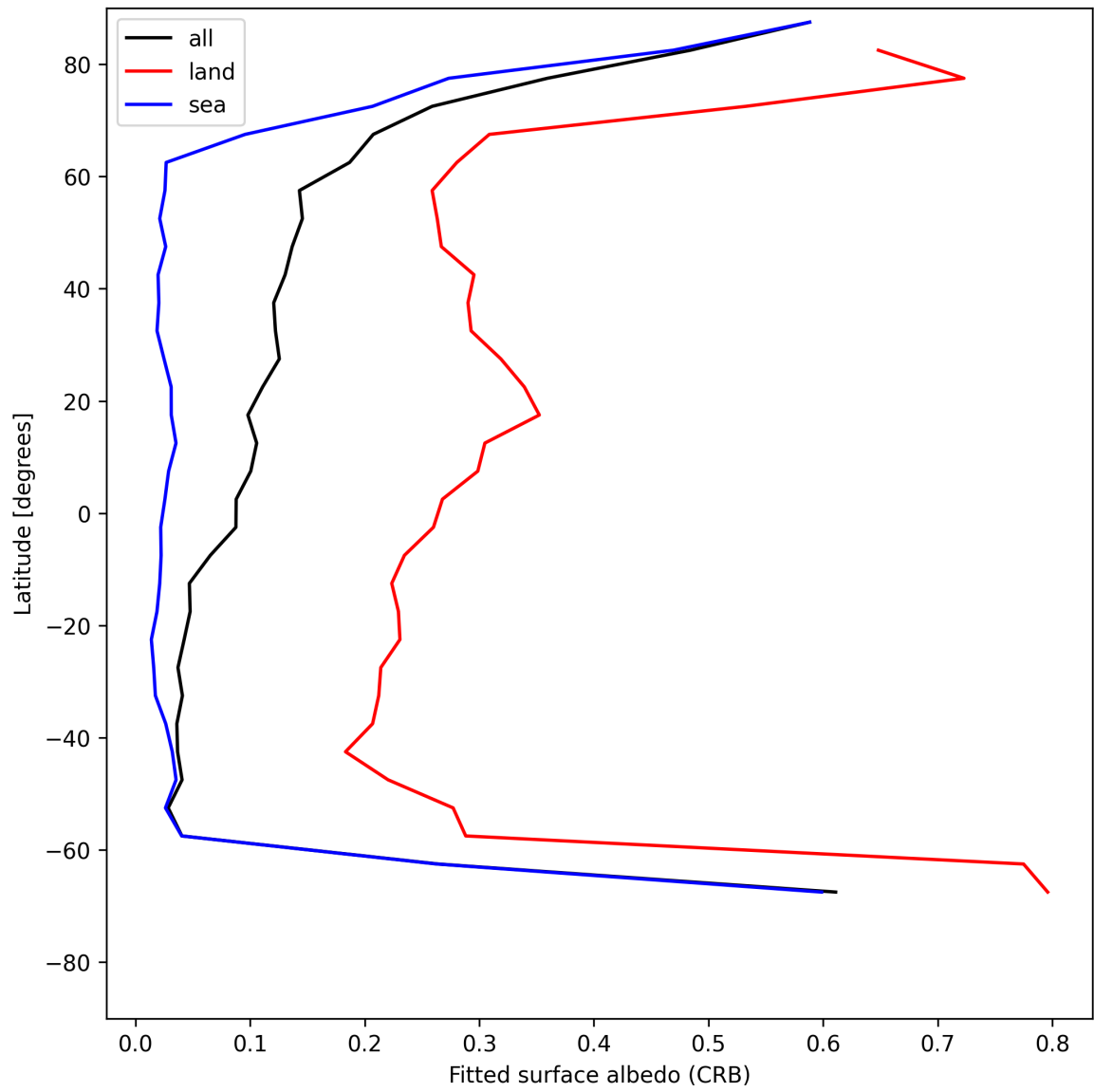
Figure 28: Zonal average of “Fitted surface albedo (CRB)” for 2025-07-13 to 2025-07-14.
