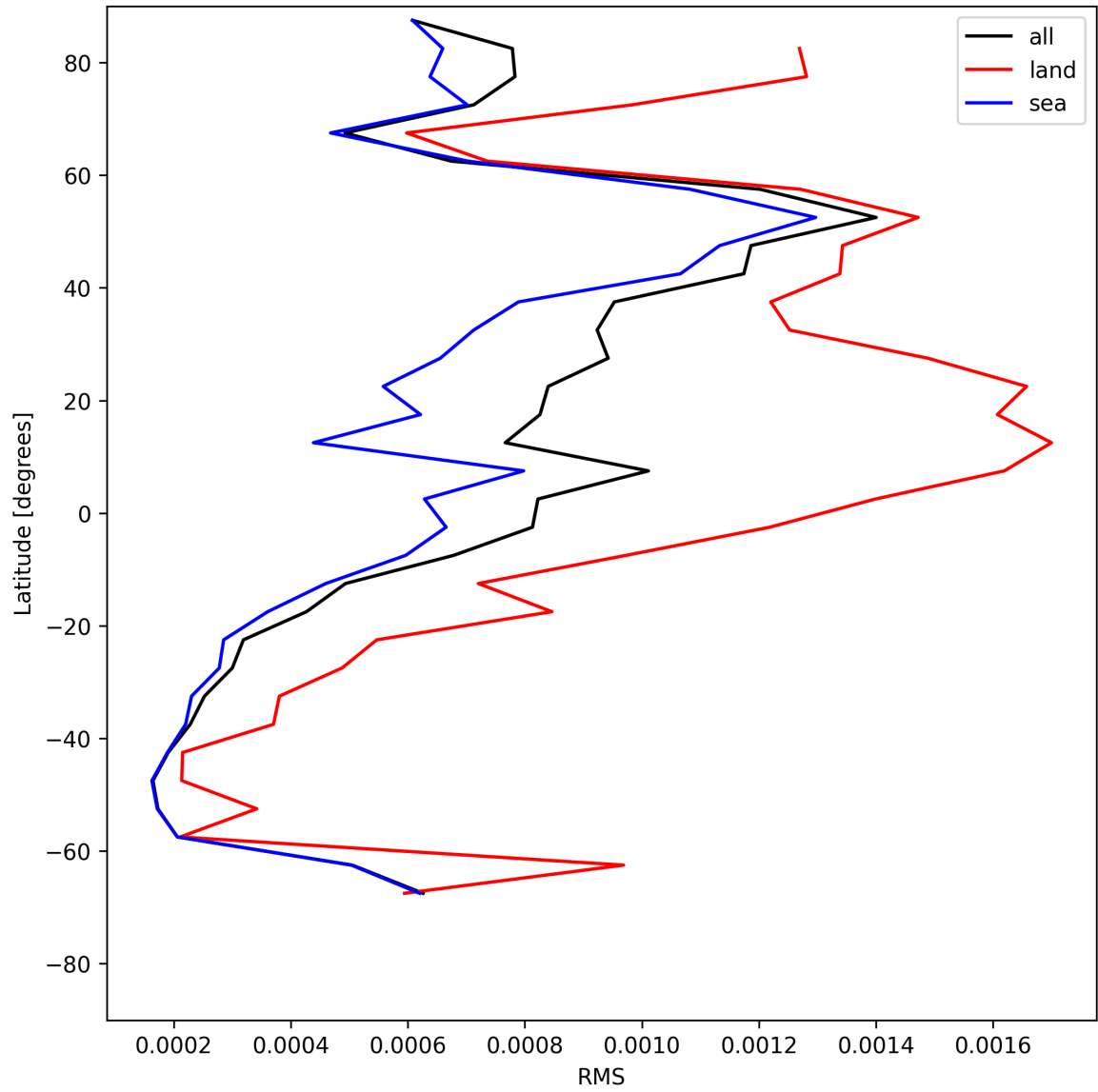
Figure 29: Zonal average of “RMS” for 2025-07-13 to 2025-07-14.
