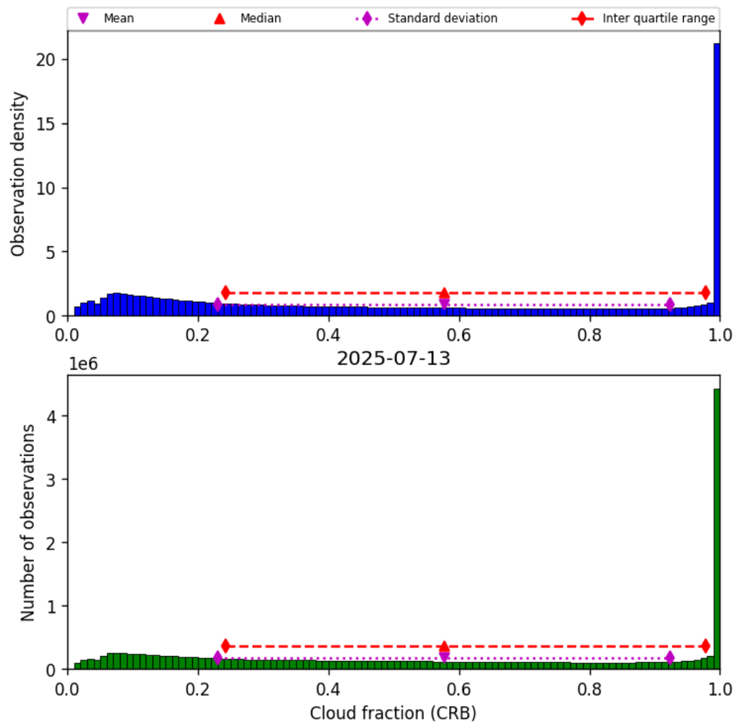
Figure 40: Histogram of “Cloud fraction (CRB)” for 2025-07-13 to 2025-07-14
