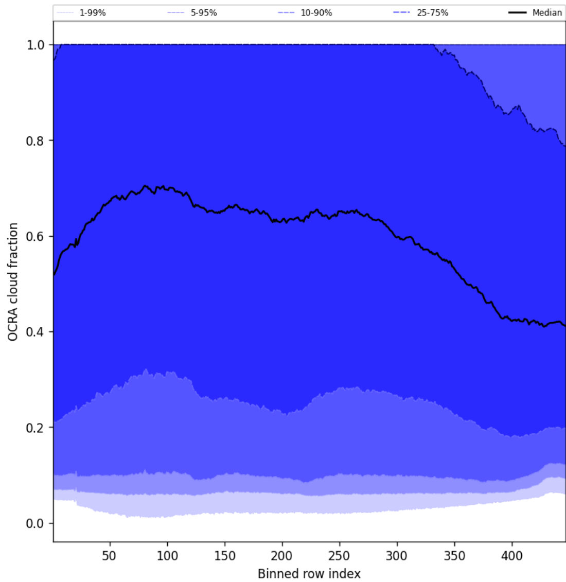
Figure 64: Along track statistics of “OCRA cloud fraction” for 2025-07-13 to 2025-07-14
