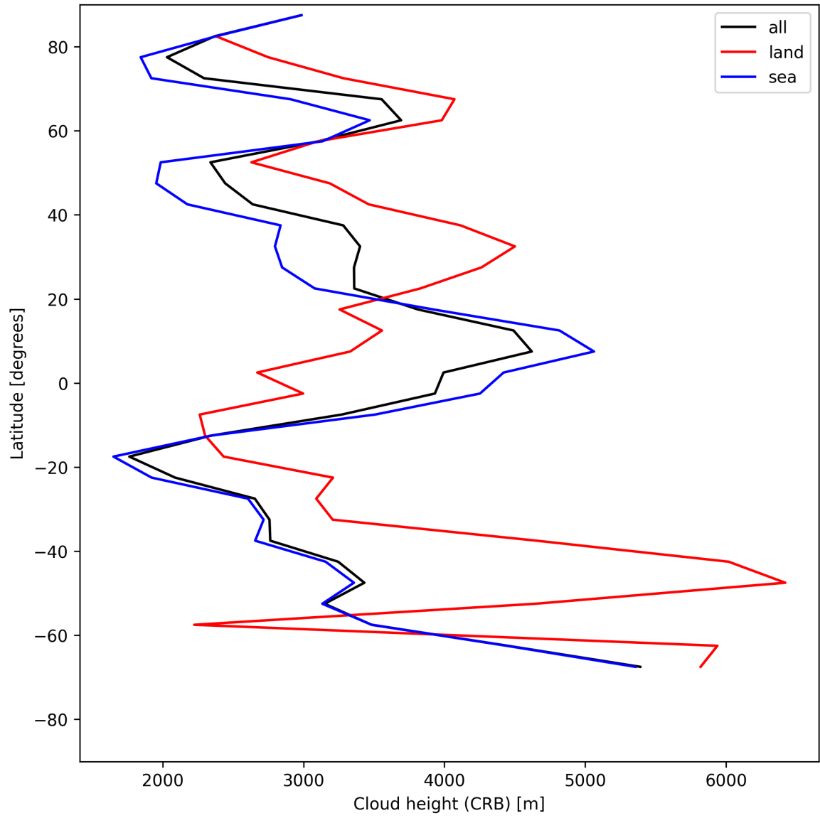
Figure 25: Zonal average of “Cloud height (CRB)” for 2025-07-13 to 2025-07-14.
