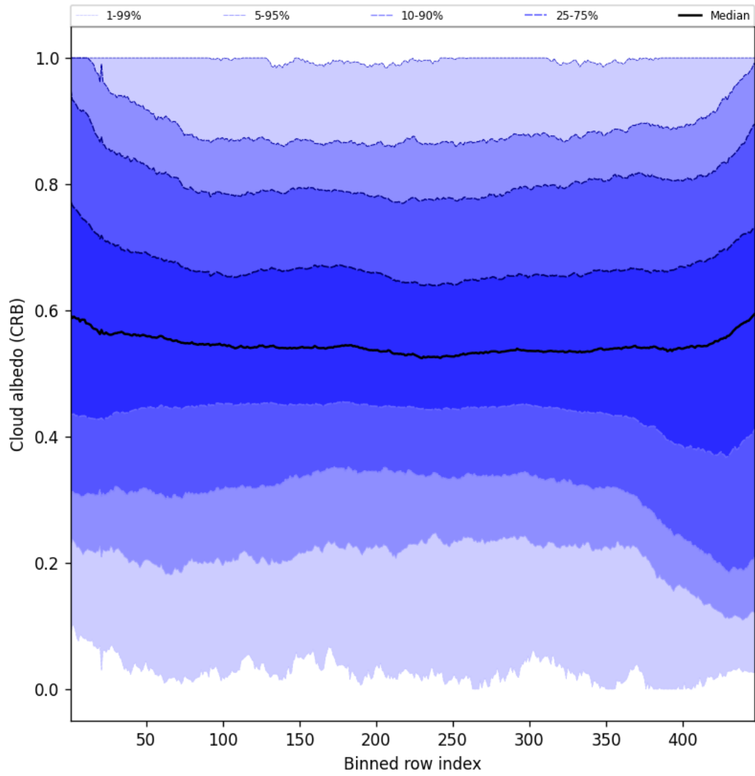
Figure 58: Along track statistics of “Cloud albedo (CRB)” for 2025-07-13 to 2025-07-14
