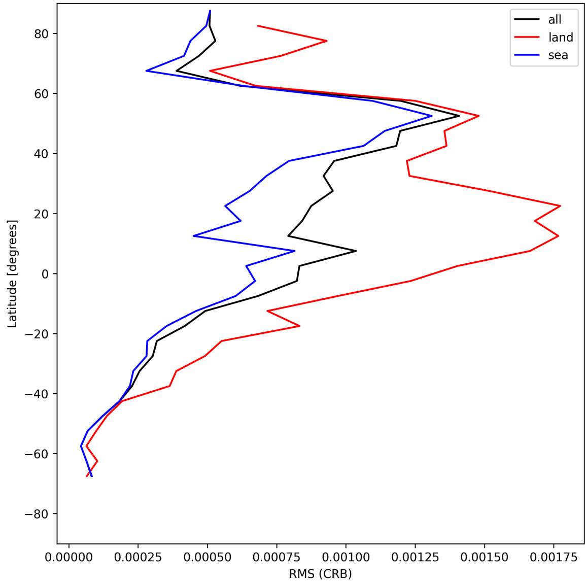
Figure 30: Zonal average of “RMS (CRB)” for 2025-07-13 to 2025-07-14.
