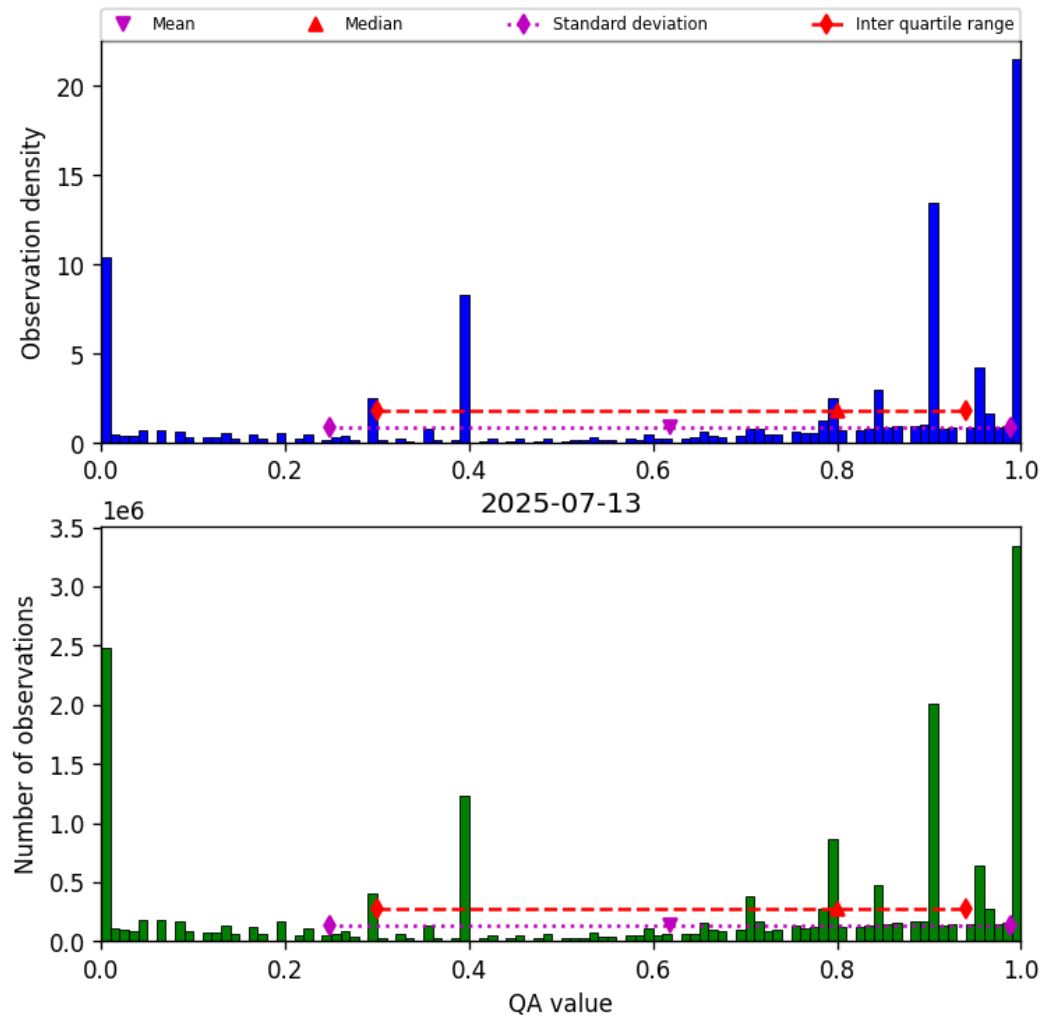
Figure 36: Histogram of “QA value” for 2025-07-13 to 2025-07-14
