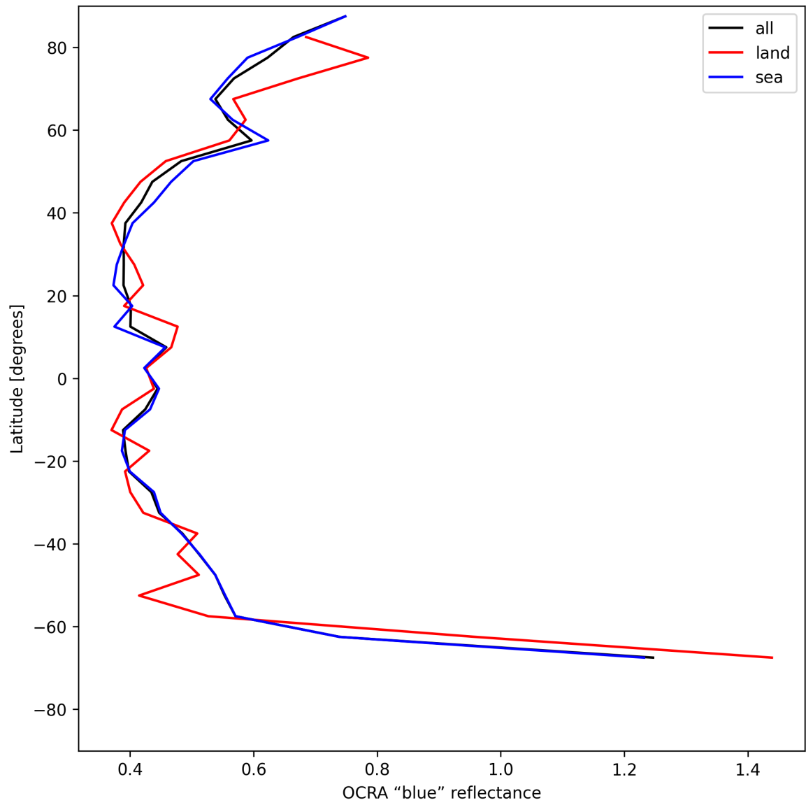
Figure 33: Zonal average of "OCRA "blue" reflectance" for 2025-07-13 to 2025-07-14.
