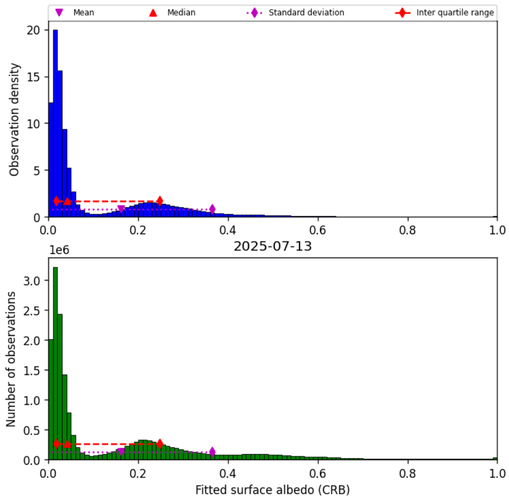
Figure 44: Histogram of “Fitted surface albedo (CRB)” for 2025-07-13 to 2025-07-14
