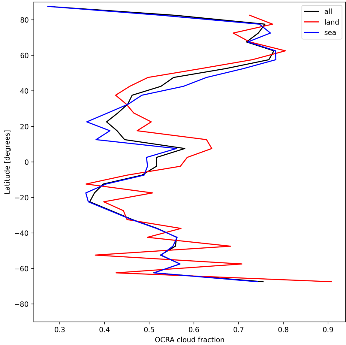
Figure 32: Zonal average of “OCRA cloud fraction” for 2025-07-13 to 2025-07-14.
