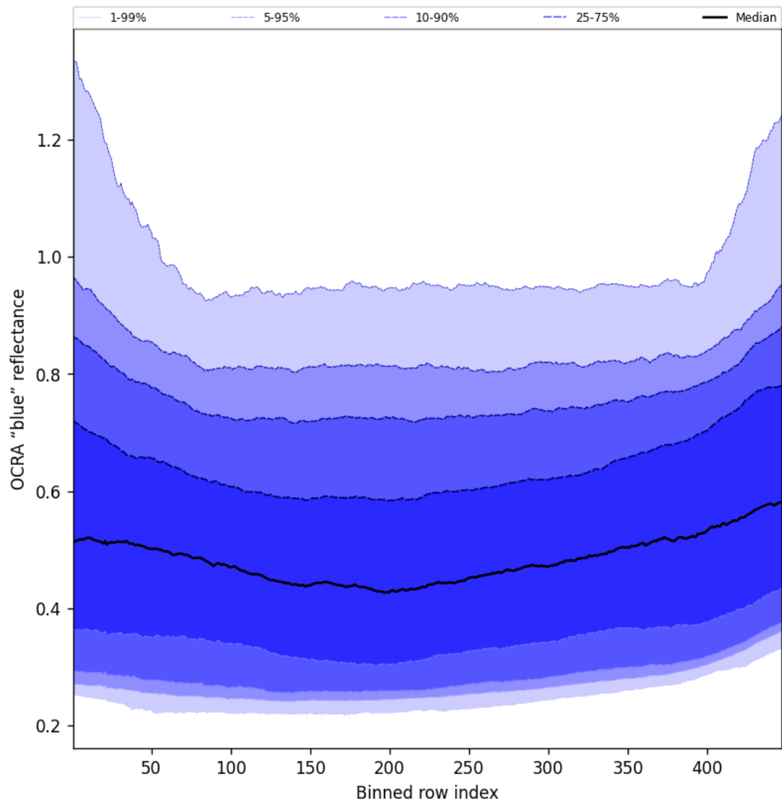
Figure 65: Along track statistics of “OCRA “blue” reflectance” for 2025-07-13 to 2025-07-14
