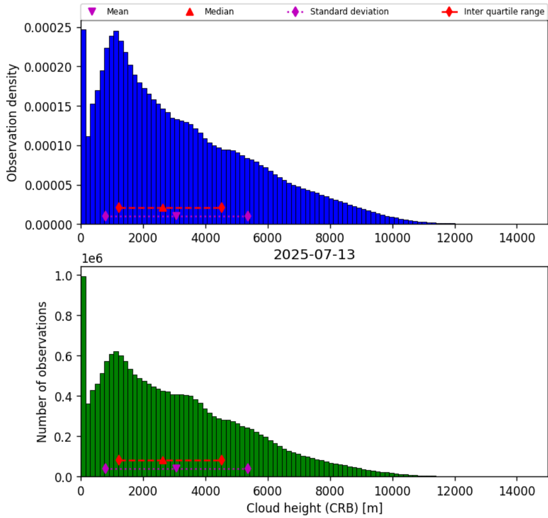
Figure 41: Histogram of “Cloud height (CRB)” for 2025-07-13 to 2025-07-14
