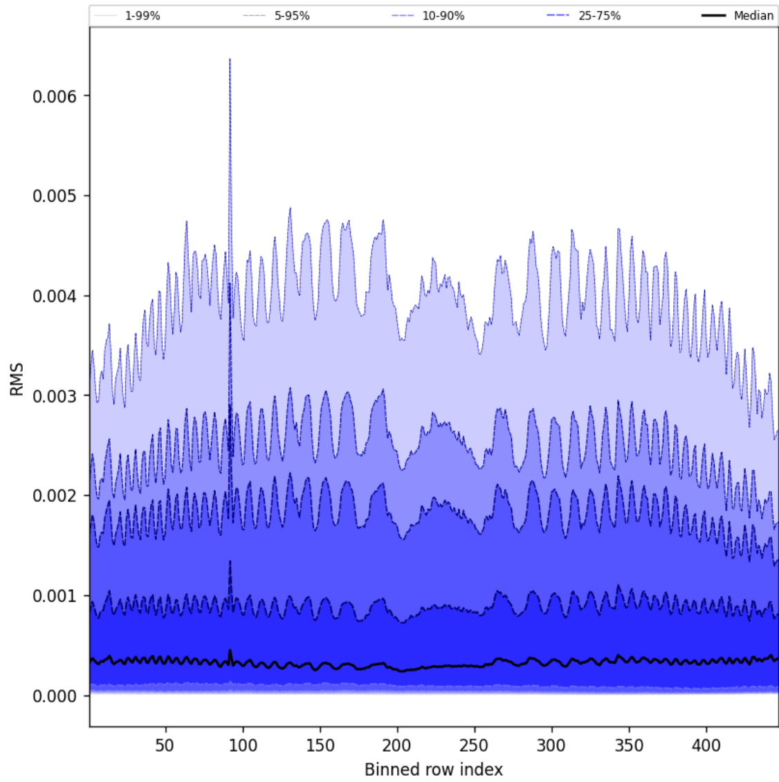
Figure 61: Along track statistics of “RMS” for 2025-07-13 to 2025-07-14
