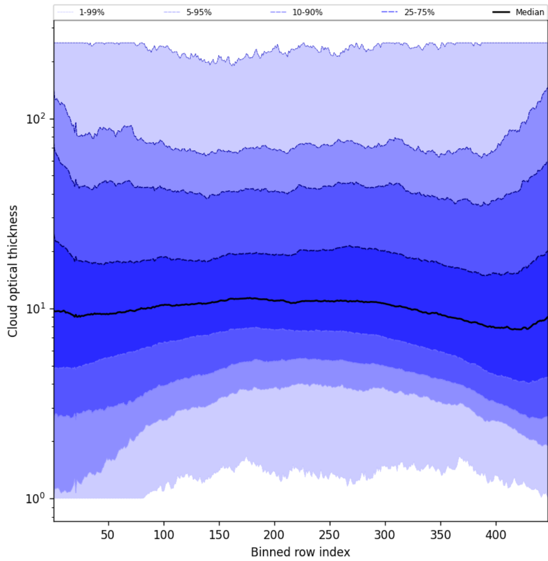
Figure 55: Along track statistics of “Cloud optical thickness” for 2025-07-13 to 2025-07-14
