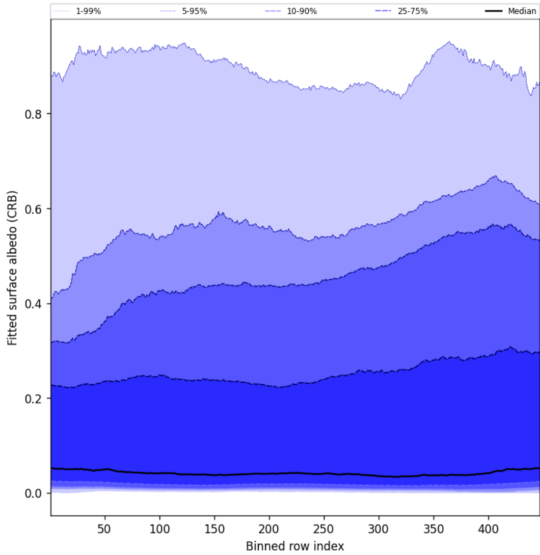
Figure 60: Along track statistics of “Fitted surface albedo (CRB)” for 2025-07-13 to 2025-07-14
