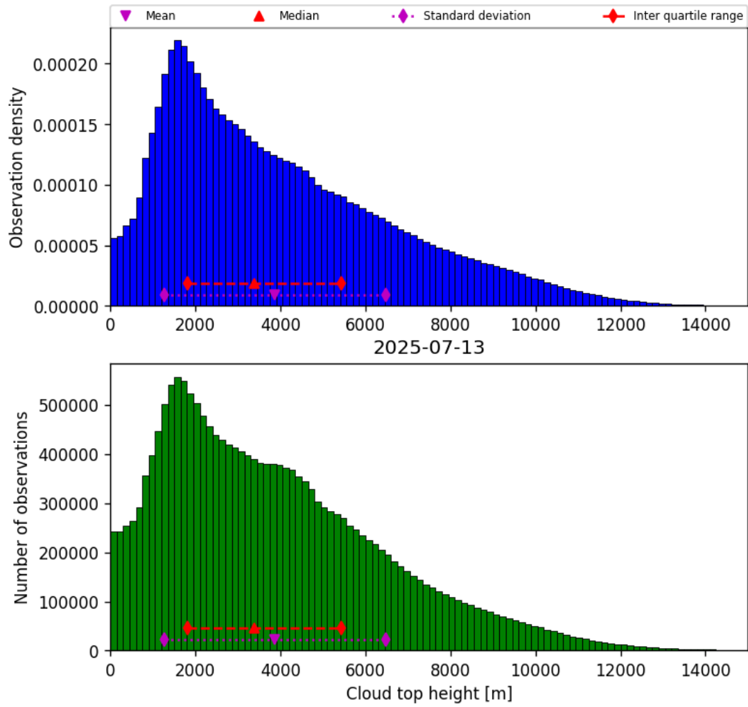
Figure 38: Histogram of “Cloud top height” for 2025-07-13 to 2025-07-14
