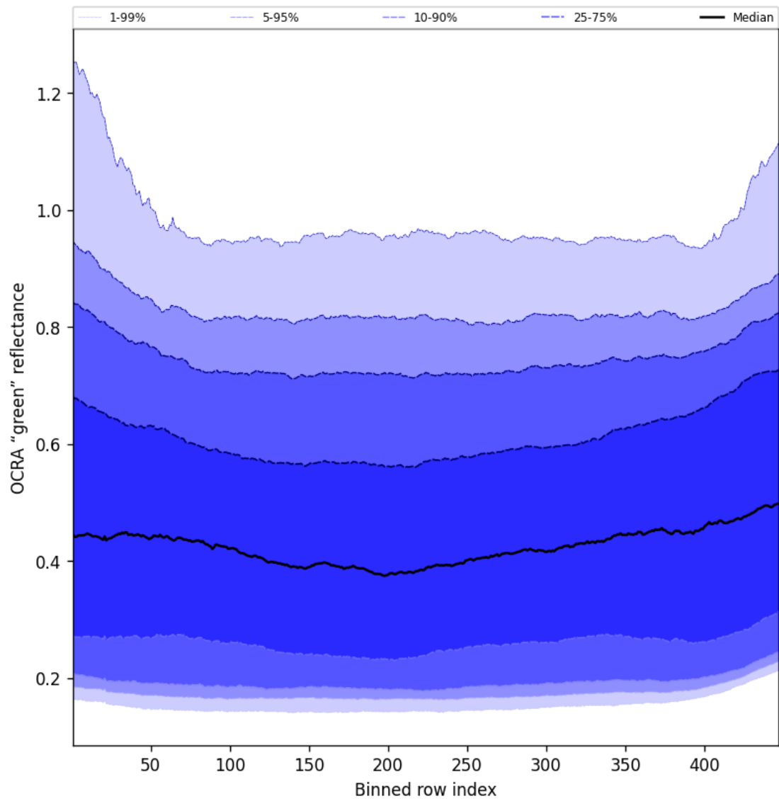
Figure 66: Along track statistics of “OCRA “green” reflectance” for 2025-07-13 to 2025-07-14
