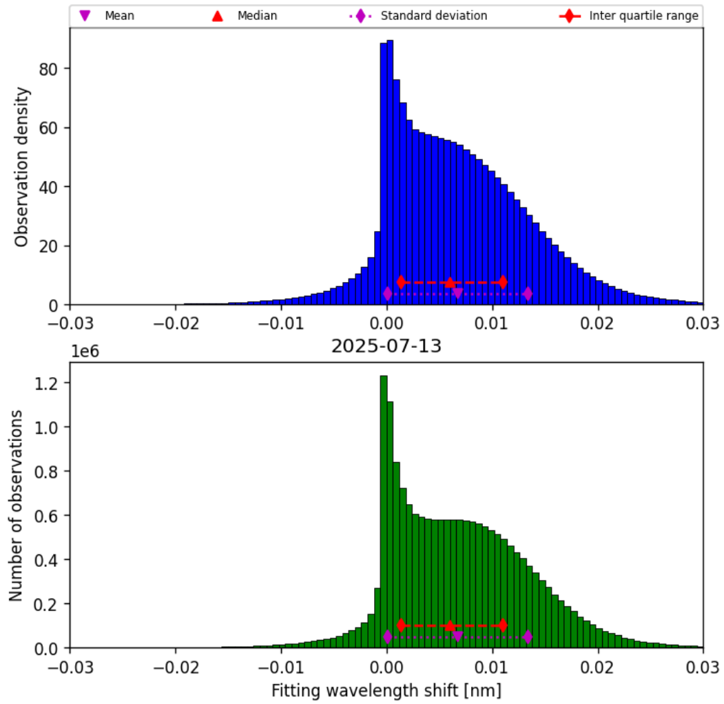
Figure 47: Histogram of “Fitting wavelength shift” for 2025-07-13 to 2025-07-14
