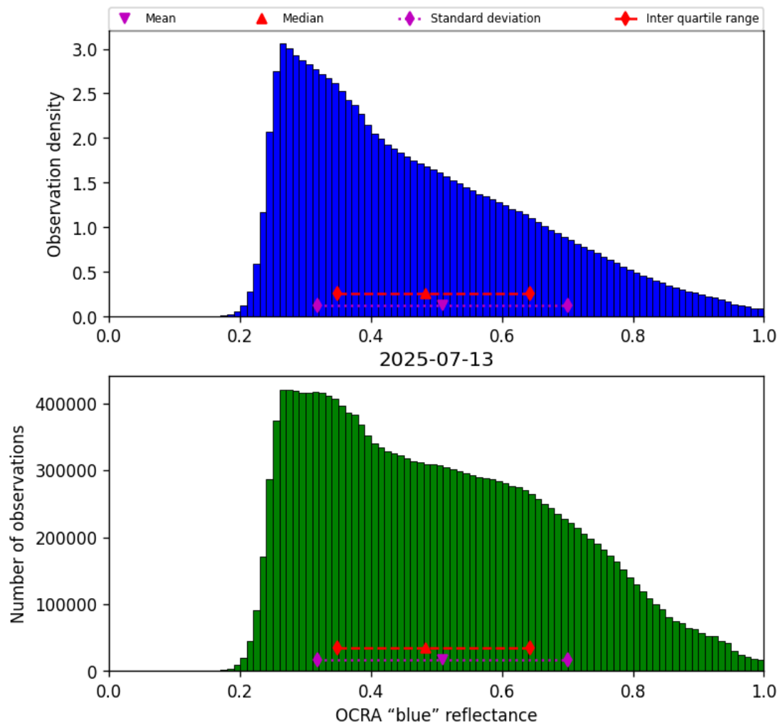
Figure 49: Histogram of “OCRA “blue” reflectance” for 2025-07-13 to 2025-07-14
