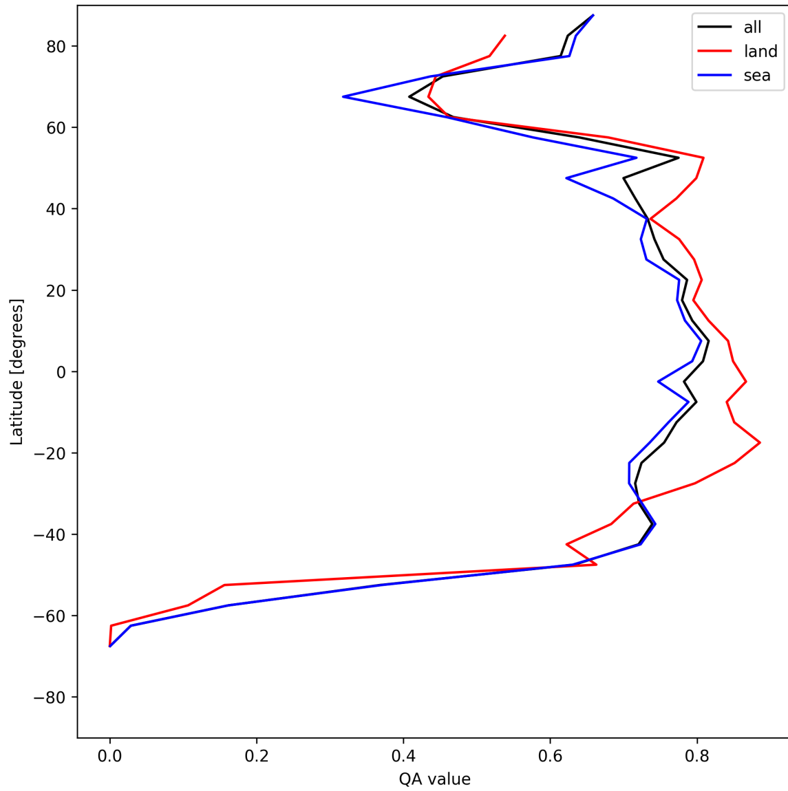
Figure 20: Zonal average of “QA value” for 2025-07-13 to 2025-07-14.
