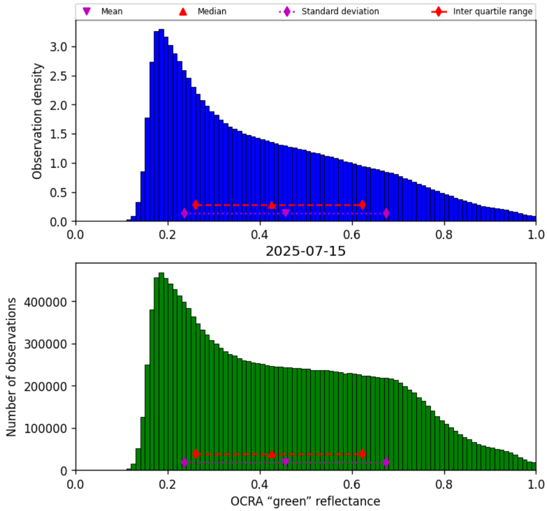
Figure 50: Histogram of “OCRA “green” reflectance” for 2025-07-15 to 2025-07-16
