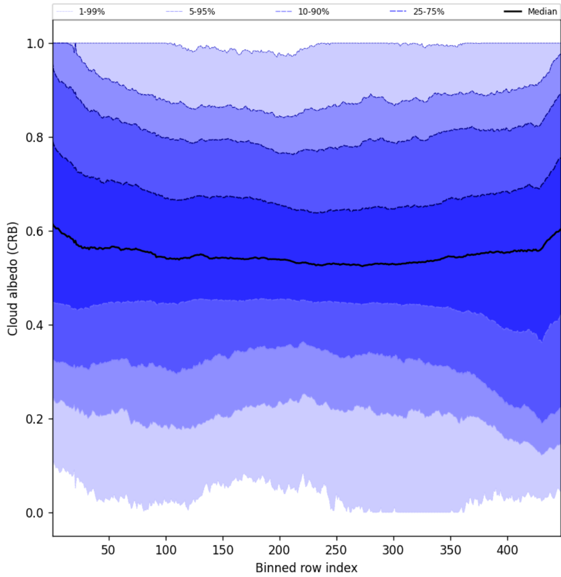
Figure 58: Along track statistics of “Cloud albedo (CRB)” for 2025-07-15 to 2025-07-16
