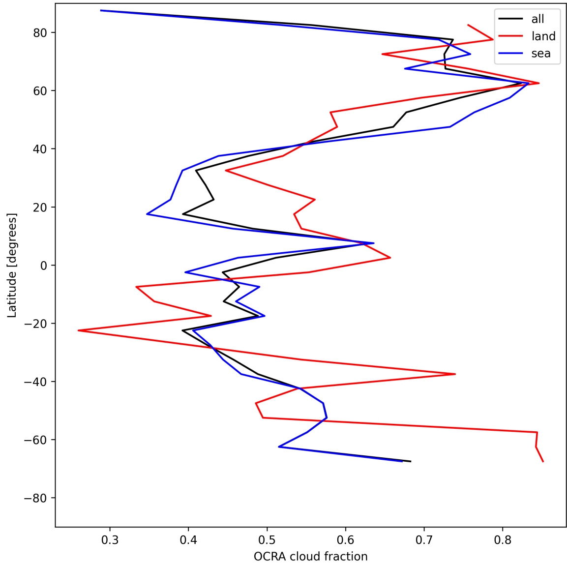
Figure 32: Zonal average of “OCRA cloud fraction” for 2025-07-15 to 2025-07-16.
