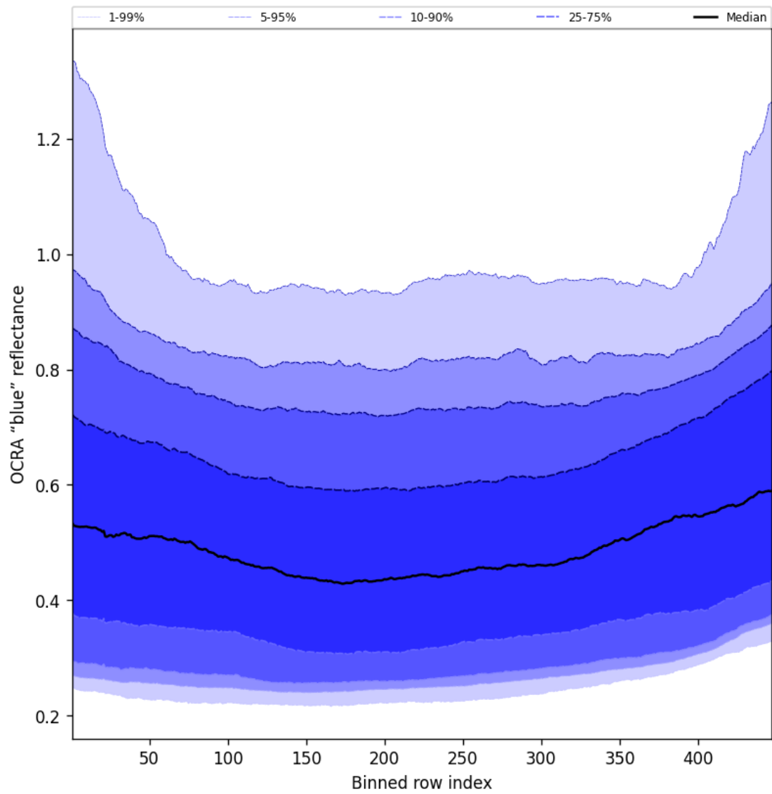
Figure 65: Along track statistics of “OCRA “blue” reflectance” for 2025-07-15 to 2025-07-16
