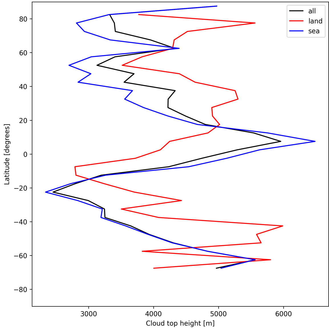
Figure 22: Zonal average of “Cloud top height” for 2025-07-15 to 2025-07-16.
