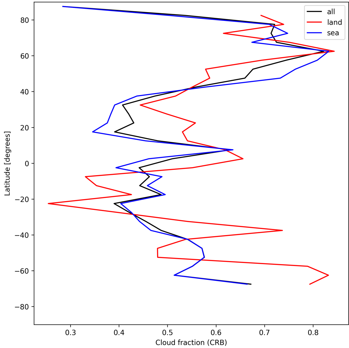
Figure 24: Zonal average of “Cloud fraction (CRB)” for 2025-07-15 to 2025-07-16.
