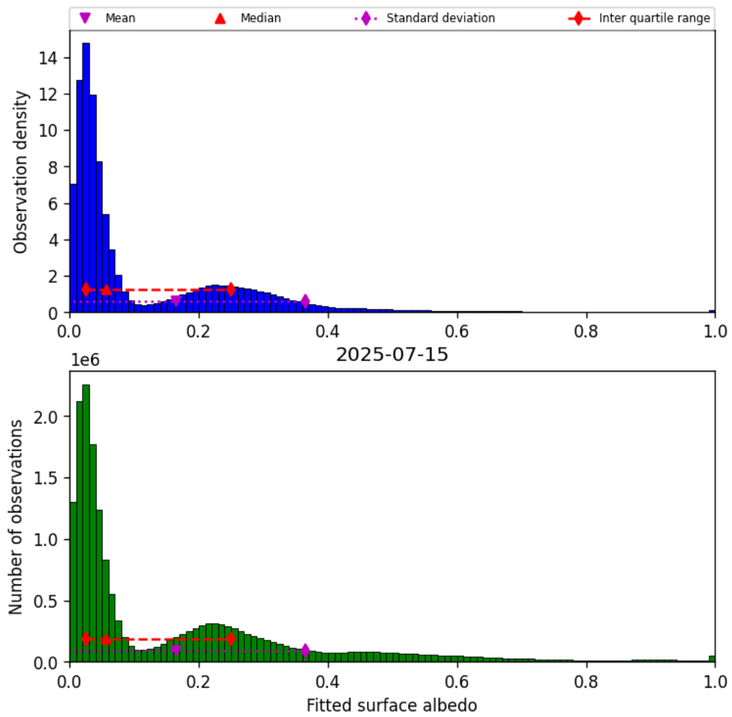
Figure 43: Histogram of “Fitted surface albedo” for 2025-07-15 to 2025-07-16
