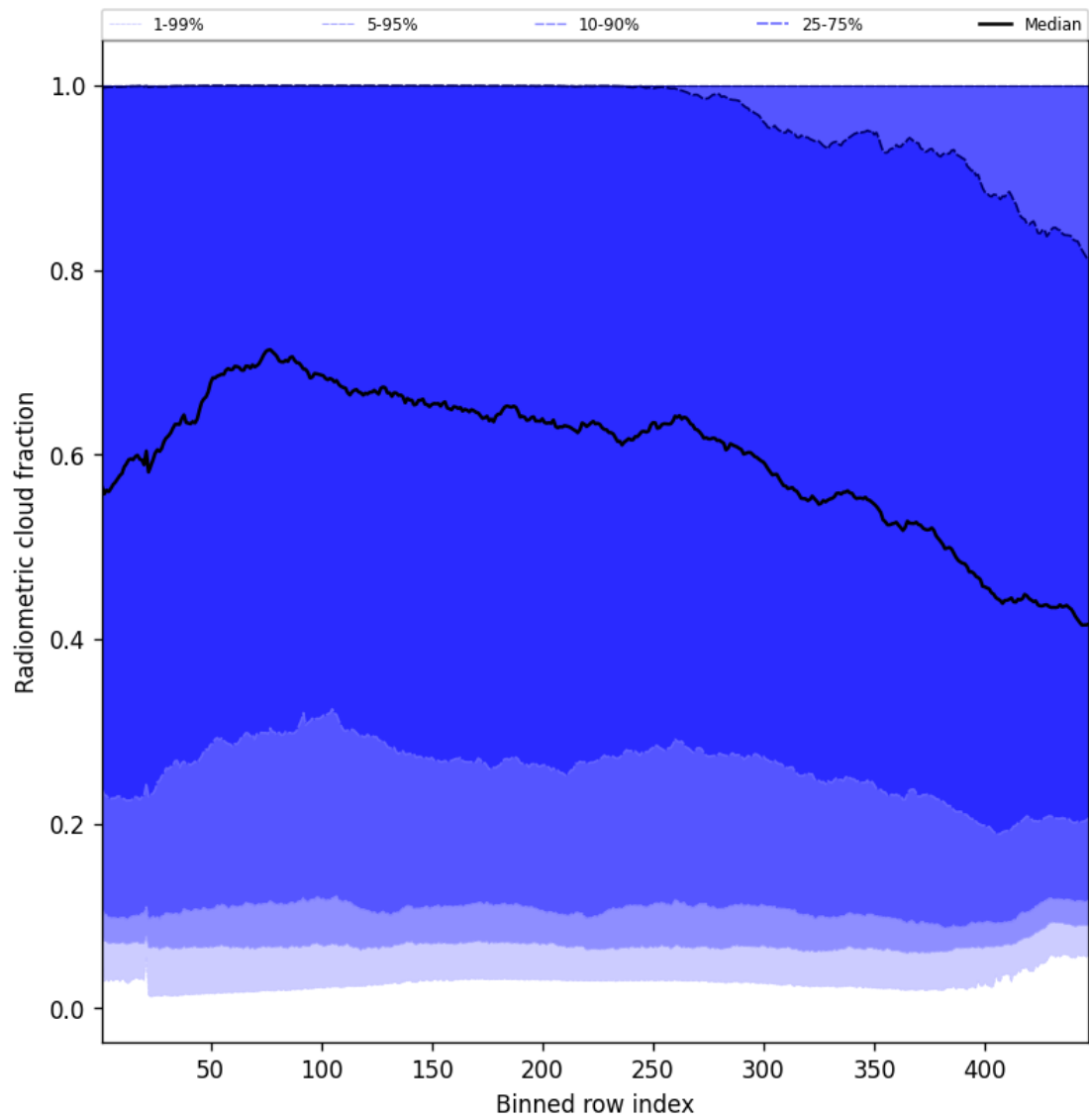
Figure 53: Along track statistics of “Radiometric cloud fraction” for 2025-07-15 to 2025-07-16
