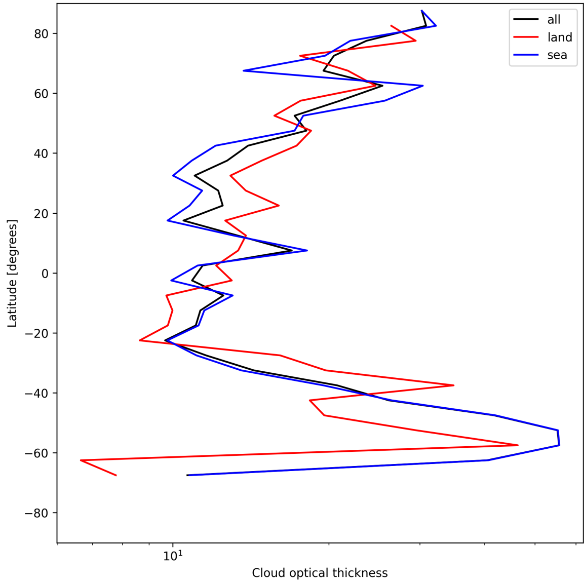
Figure 23: Zonal average of “Cloud optical thickness” for 2025-07-15 to 2025-07-16.
