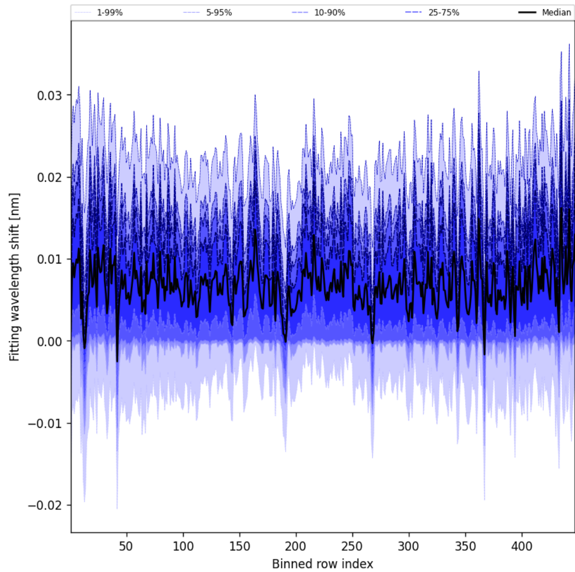
Figure 63: Along track statistics of “Fitting wavelength shift” for 2025-07-15 to 2025-07-16
