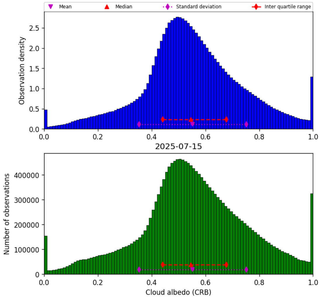
Figure 42: Histogram of “Cloud albedo (CRB)” for 2025-07-15 to 2025-07-16
