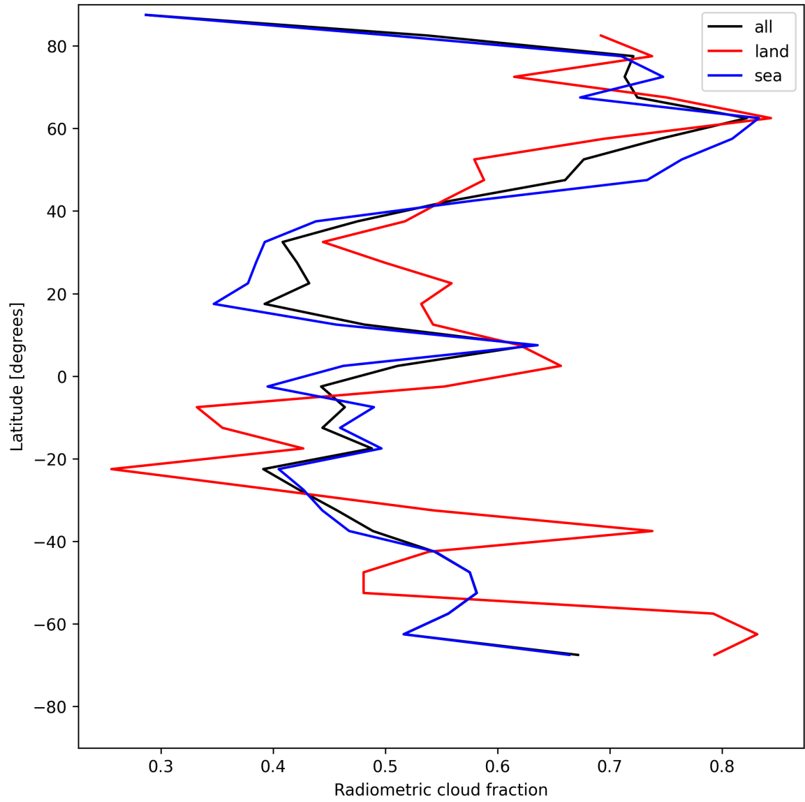
Figure 21: Zonal average of “Radiometric cloud fraction” for 2025-07-15 to 2025-07-16.
