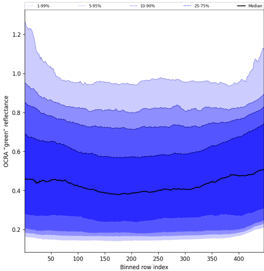
Figure 66: Along track statistics of “OCRA “green” reflectance” for 2025-07-15 to 2025-07-16
