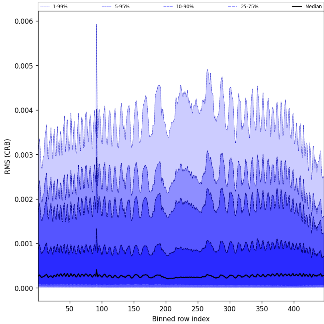
Figure 62: Along track statistics of “RMS (CRB)” for 2025-07-15 to 2025-07-16
