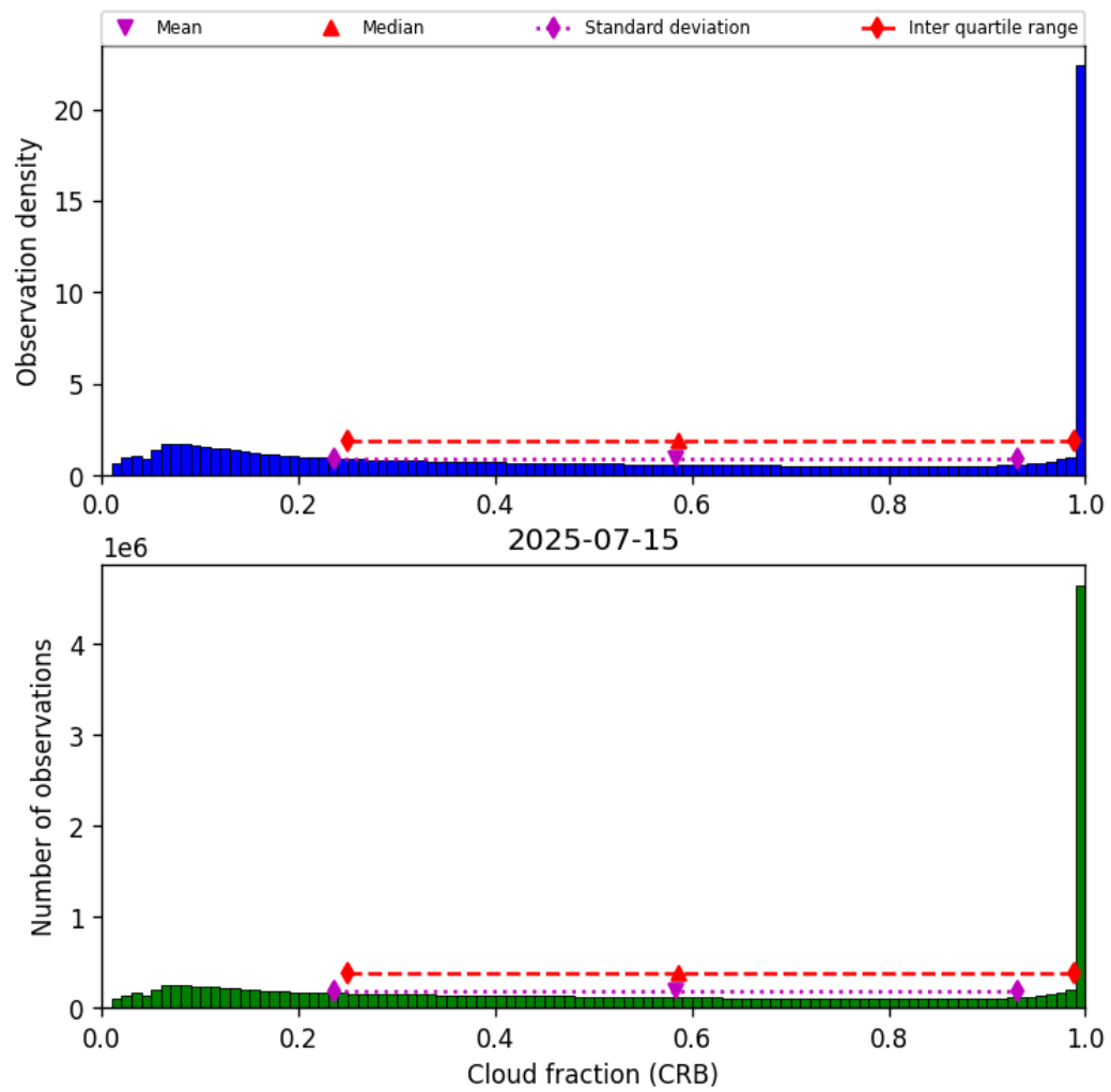
Figure 40: Histogram of “Cloud fraction (CRB)” for 2025-07-15 to 2025-07-16
