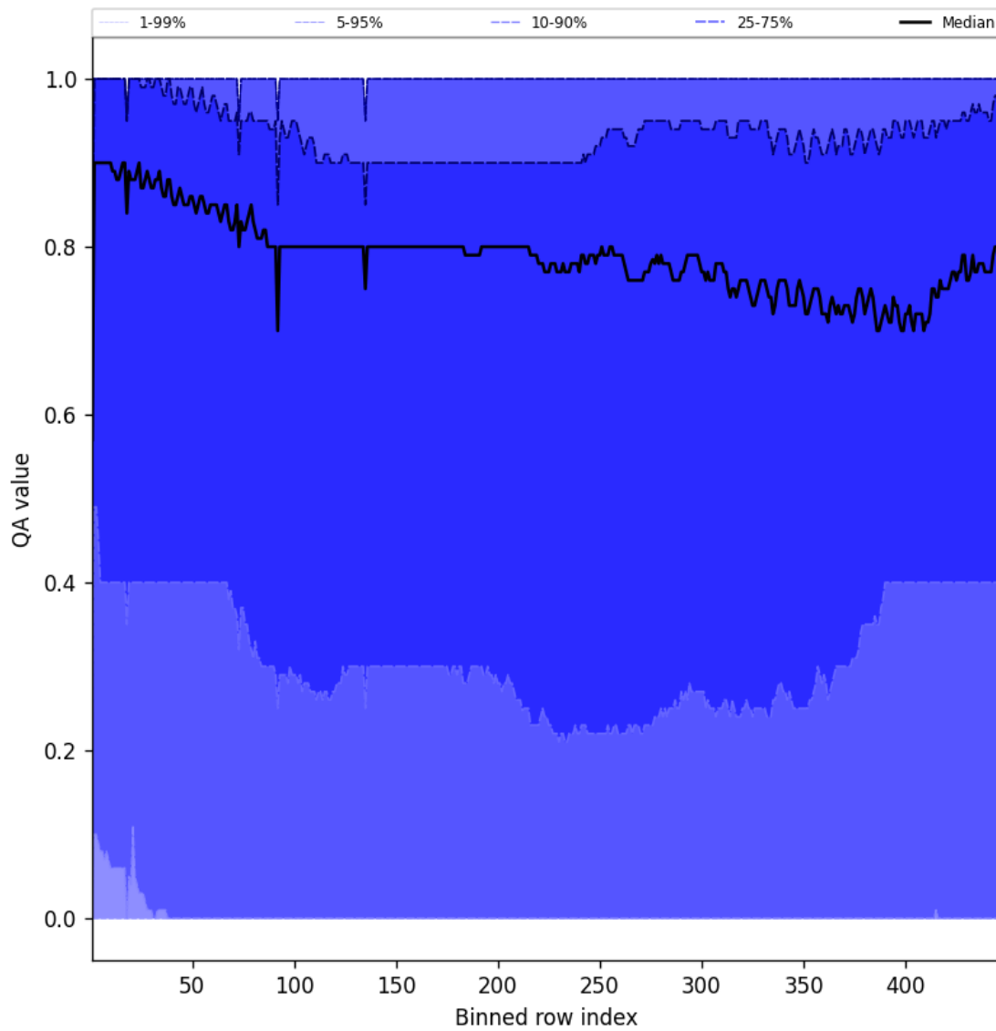
Figure 52: Along track statistics of “QA value” for 2025-07-15 to 2025-07-16
