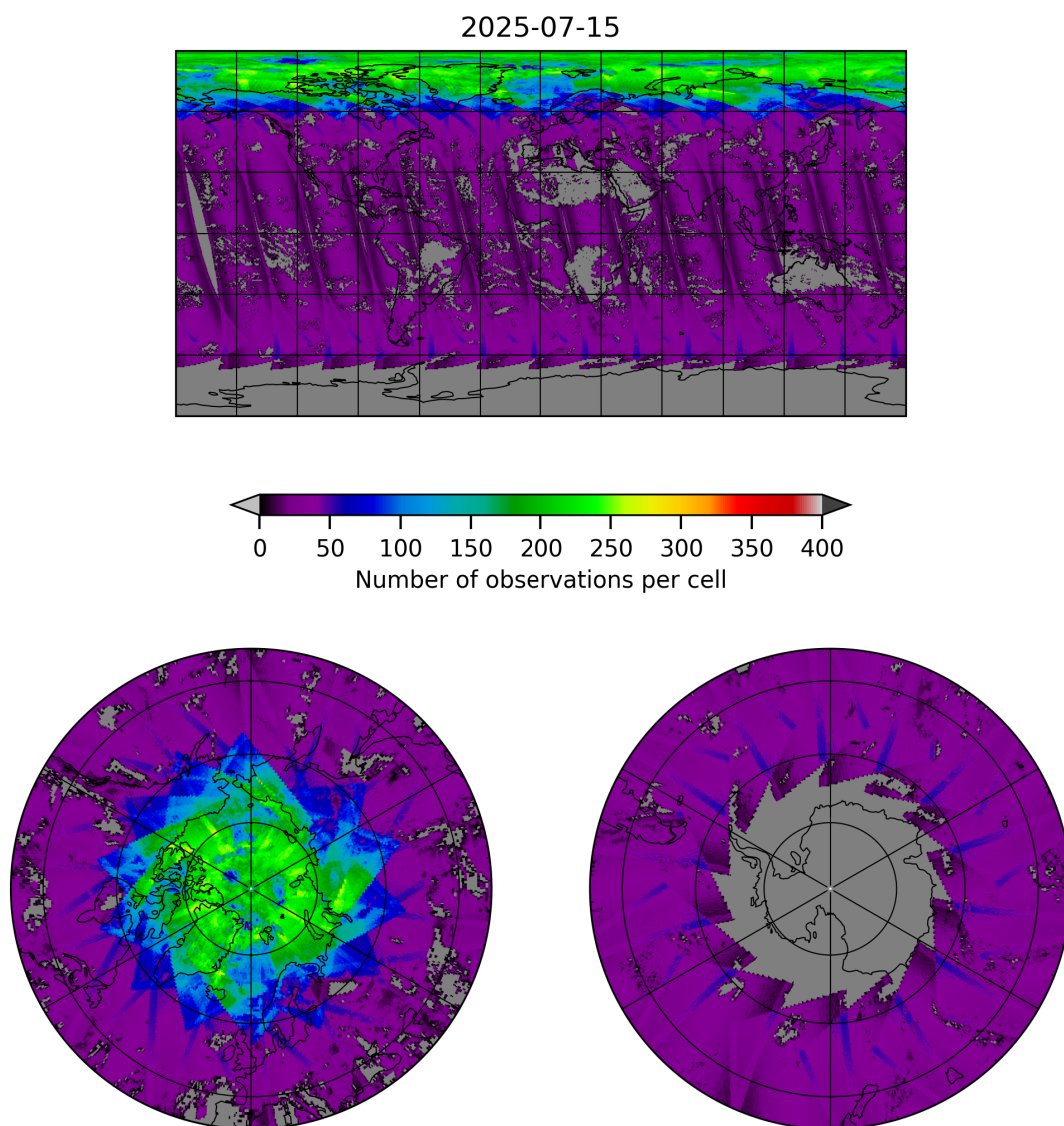
Figure 19: Map of the number of observations for 2025-07-15 to 2025-07-16
