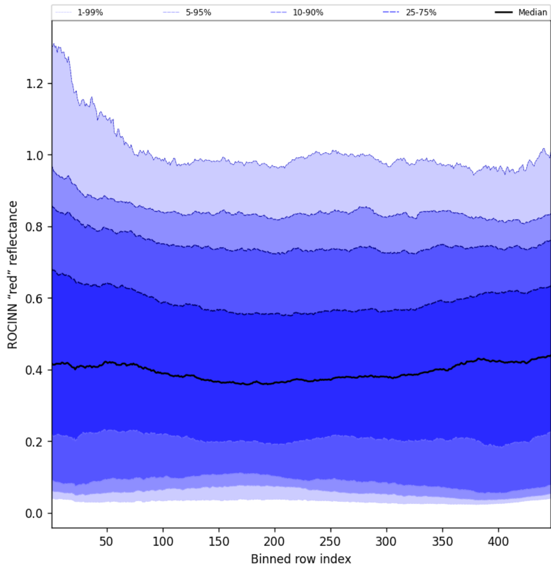
Figure 67: Along track statistics of "ROCINN "red" reflectance" for 2025-07-15 to 2025-07-16
