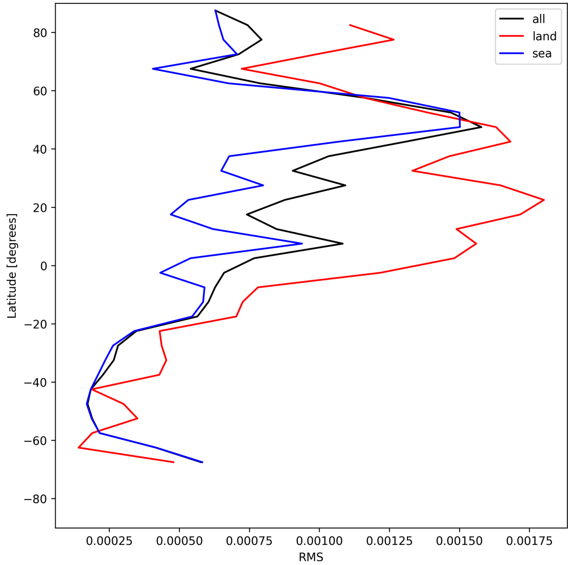
Figure 29: Zonal average of “RMS” for 2025-07-15 to 2025-07-16.
