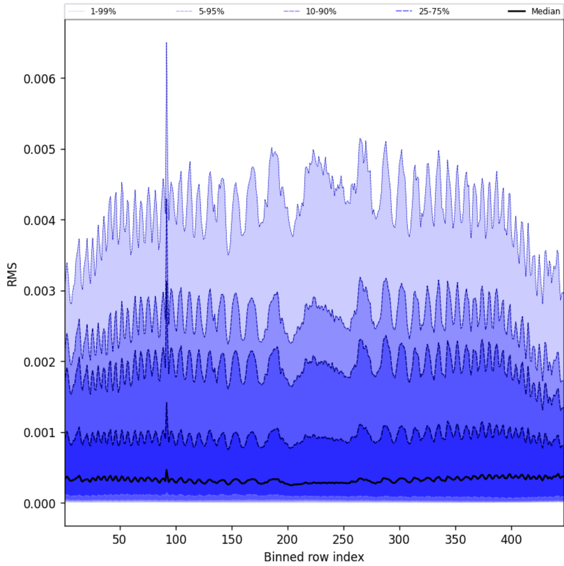
Figure 61: Along track statistics of “RMS” for 2025-07-15 to 2025-07-16
