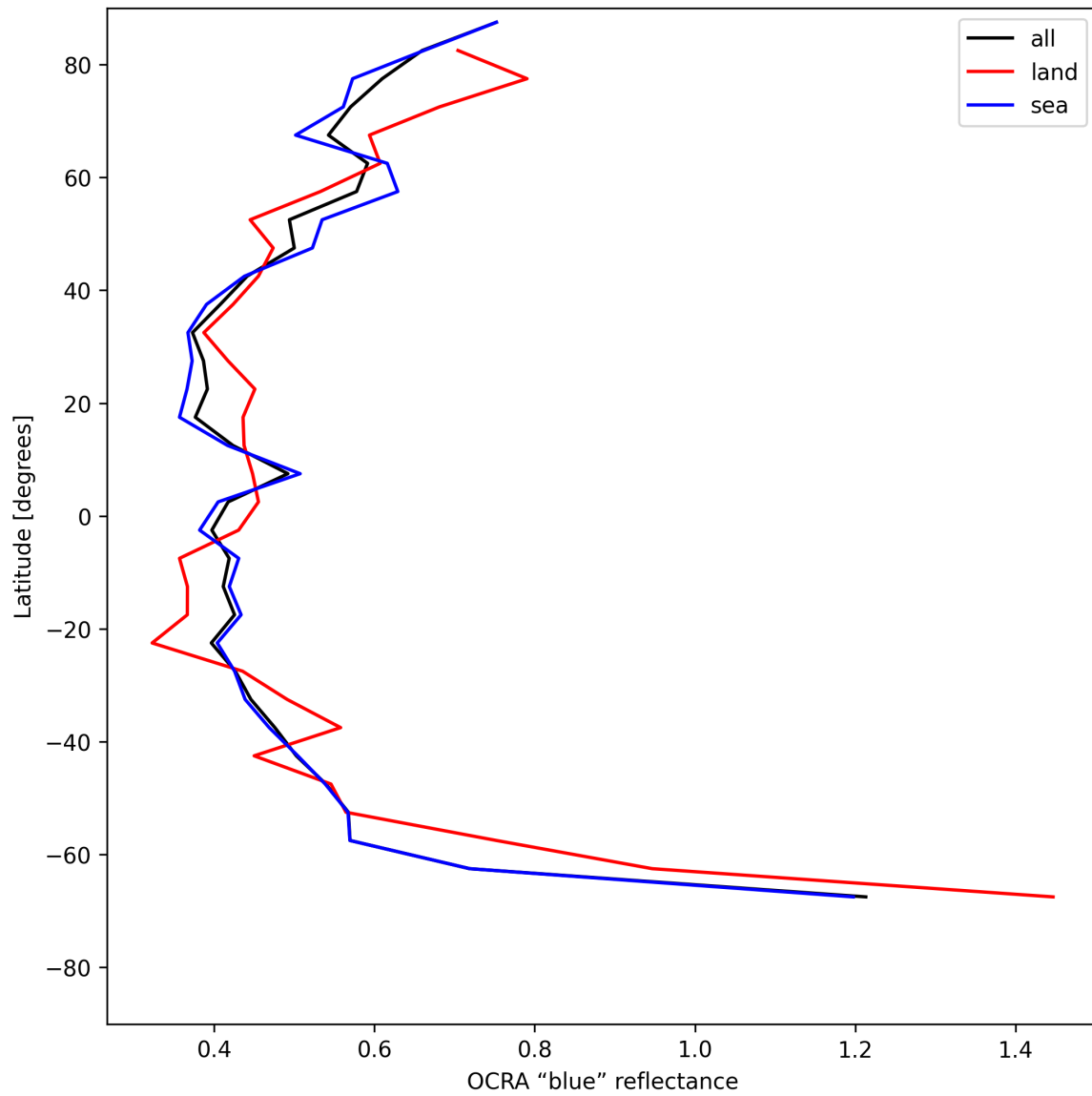
Figure 33: Zonal average of “OCRA “blue” reflectance” for 2025-07-15 to 2025-07-16.
