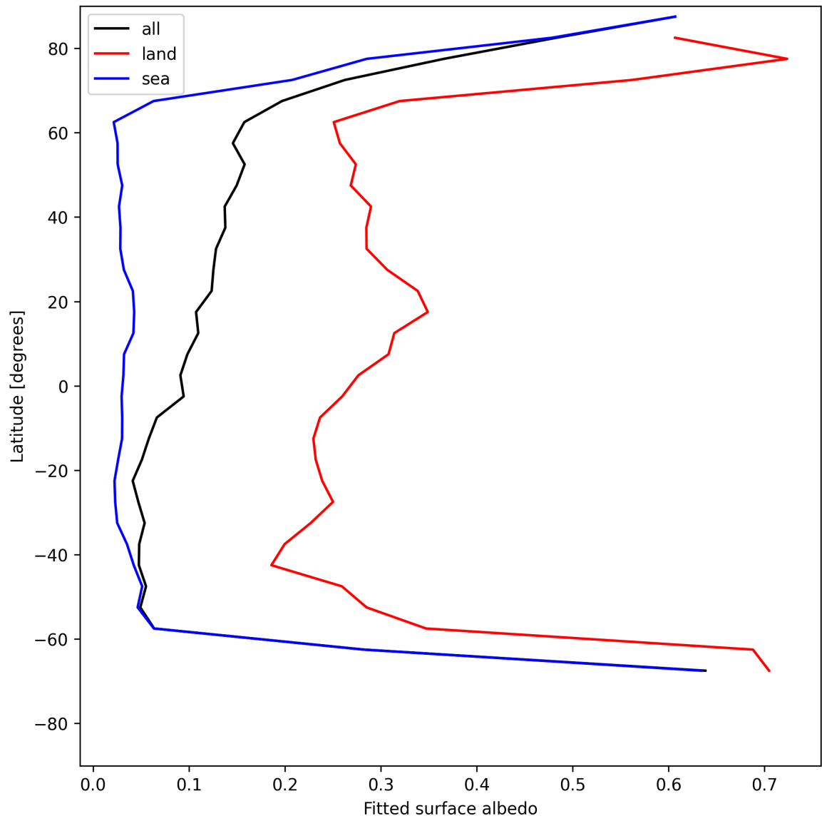
Figure 27: Zonal average of “Fitted surface albedo” for 2025-07-15 to 2025-07-16.
