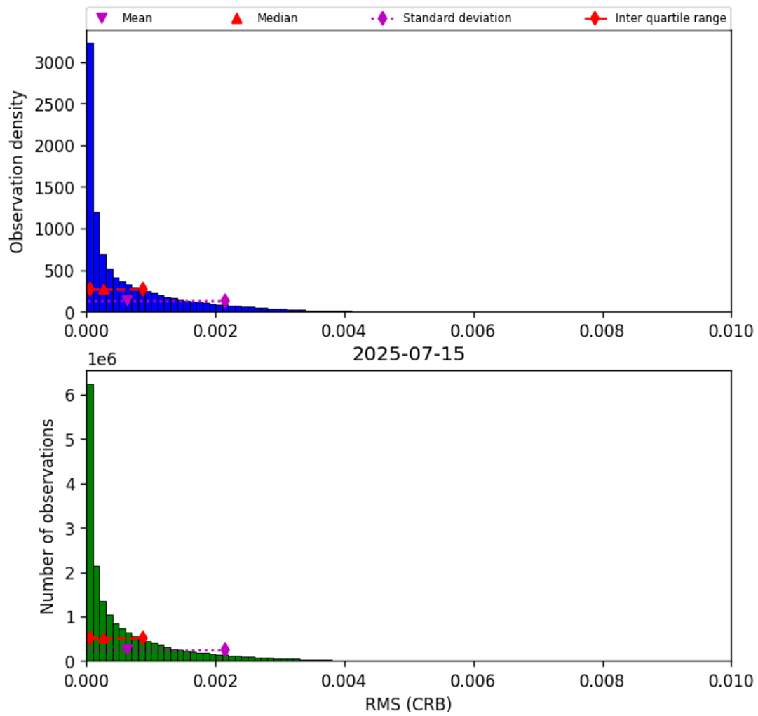
Figure 46: Histogram of “RMS (CRB)” for 2025-07-15 to 2025-07-16
