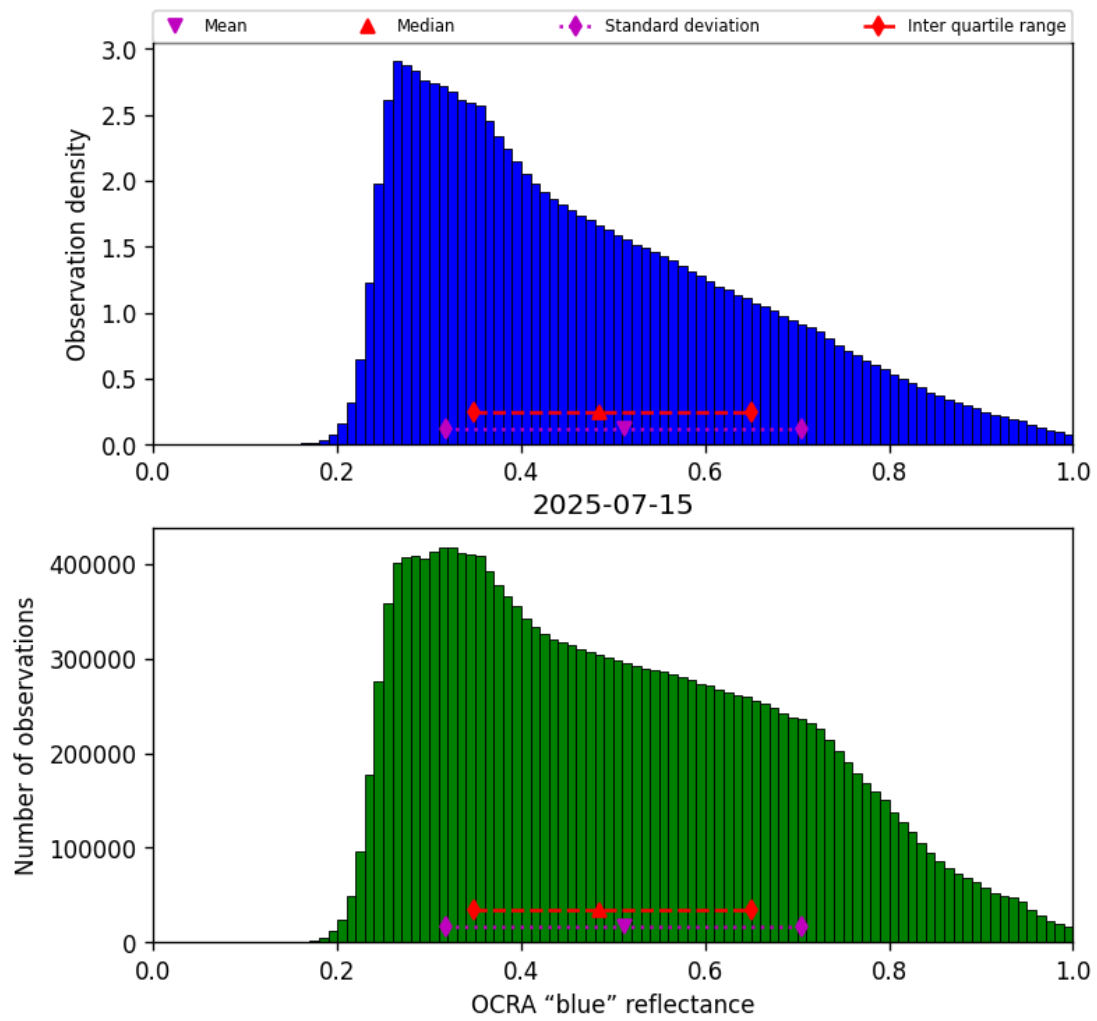
Figure 49: Histogram of “OCRA “blue” reflectance” for 2025-07-15 to 2025-07-16
