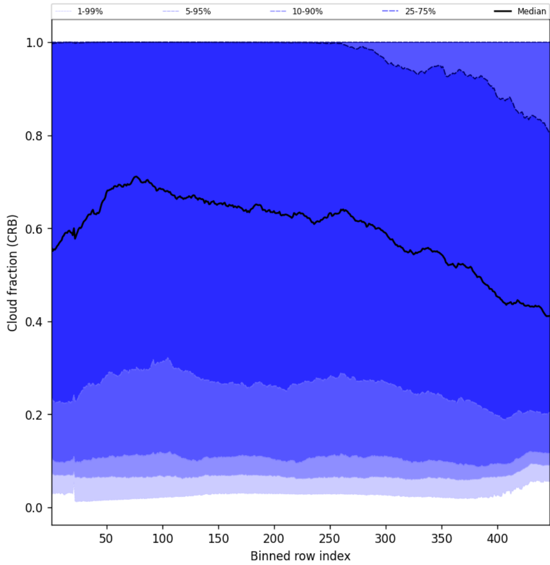
Figure 56: Along track statistics of “Cloud fraction (CRB)” for 2025-07-15 to 2025-07-16
