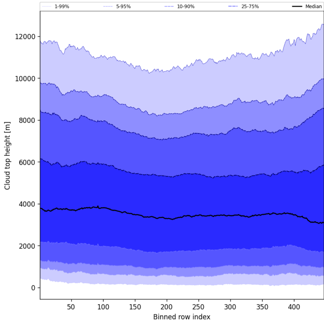
Figure 54: Along track statistics of “Cloud top height” for 2025-07-15 to 2025-07-16
