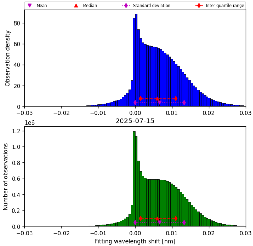
Figure 47: Histogram of “Fitting wavelength shift” for 2025-07-15 to 2025-07-16
