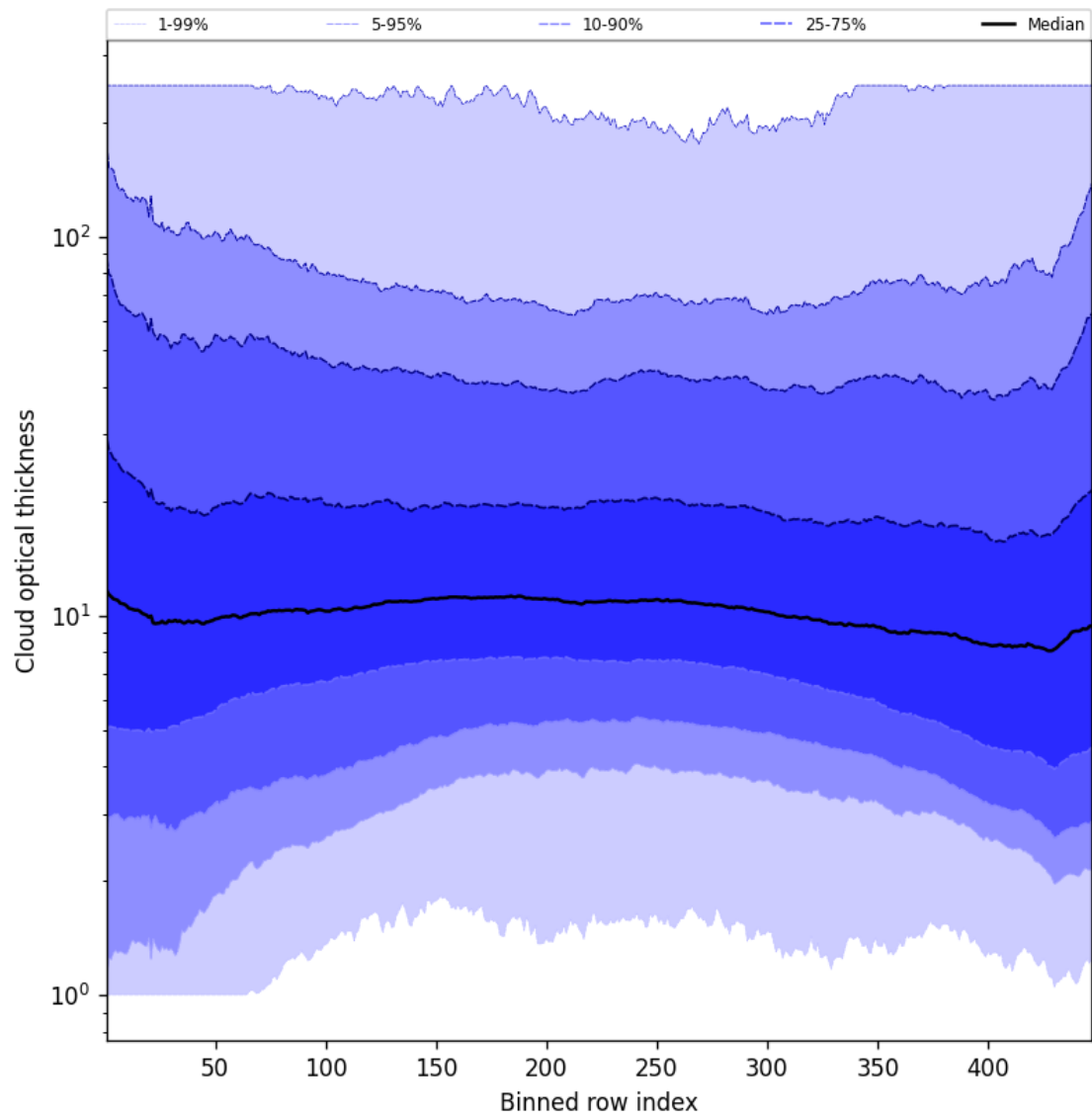
Figure 55: Along track statistics of “Cloud optical thickness” for 2025-07-15 to 2025-07-16
