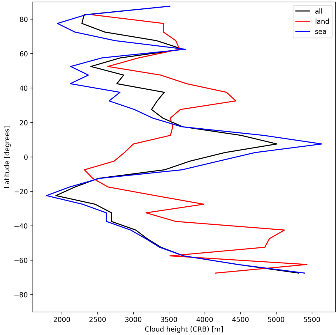
Figure 25: Zonal average of “Cloud height (CRB)” for 2025-07-15 to 2025-07-16.
