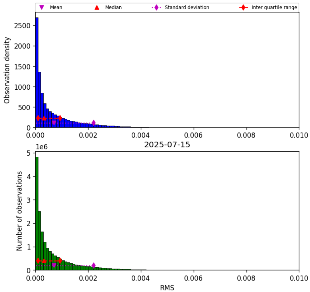
Figure 45: Histogram of “RMS” for 2025-07-15 to 2025-07-16
