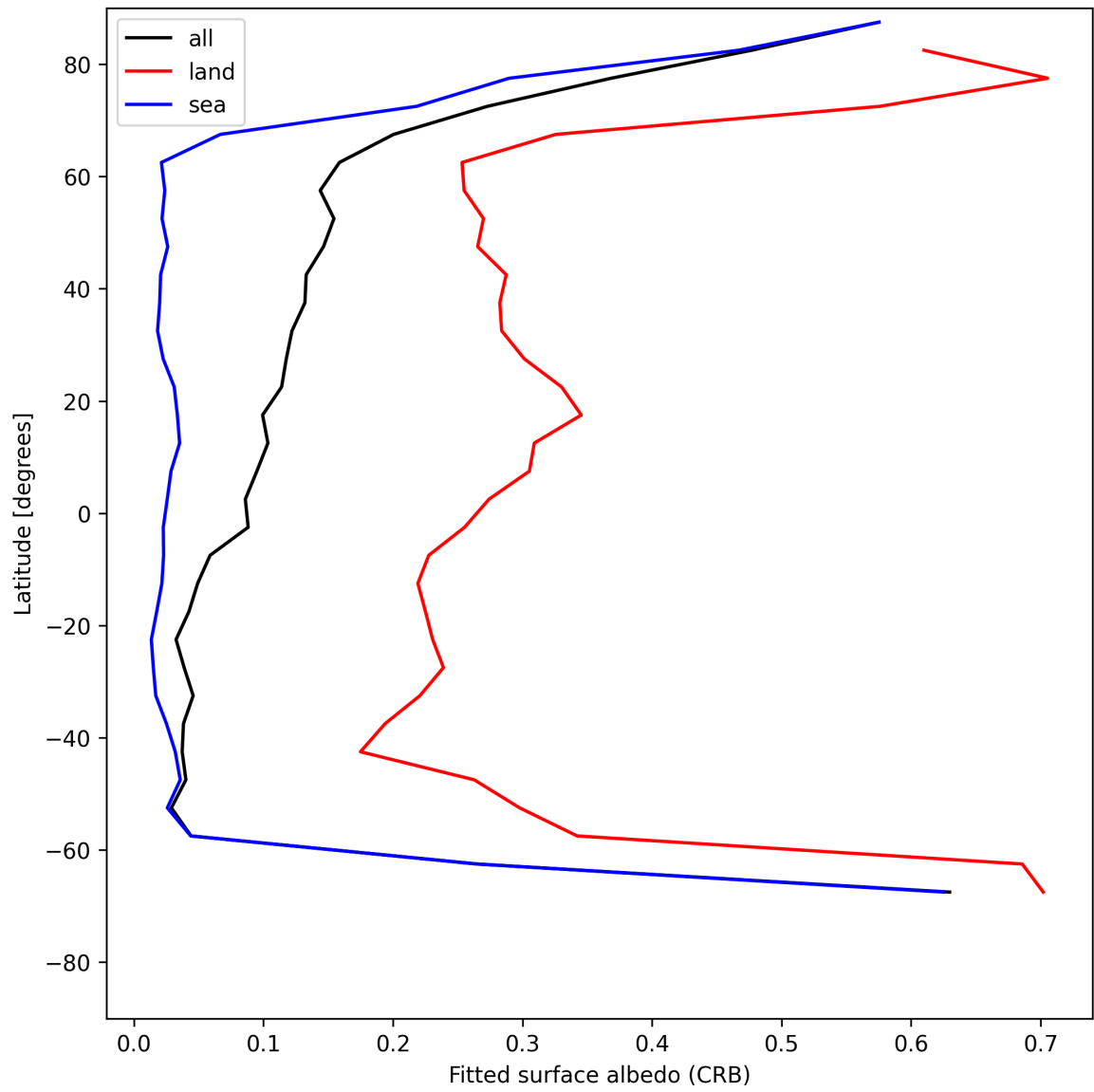
Figure 28: Zonal average of “Fitted surface albedo (CRB)” for 2025-07-15 to 2025-07-16.
