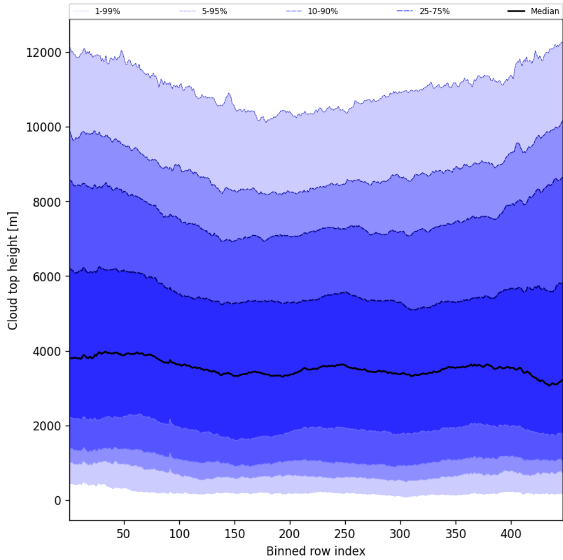
Figure 54: Along track statistics of “Cloud top height” for 2025-07-16 to 2025-07-16
