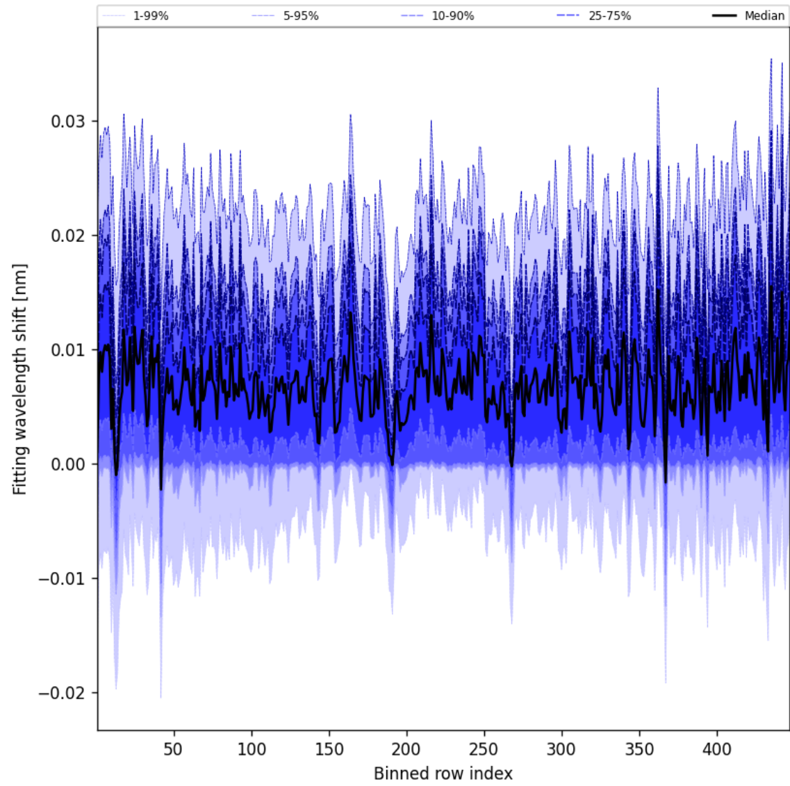
Figure 63: Along track statistics of “Fitting wavelength shift” for 2025-07-16 to 2025-07-16
