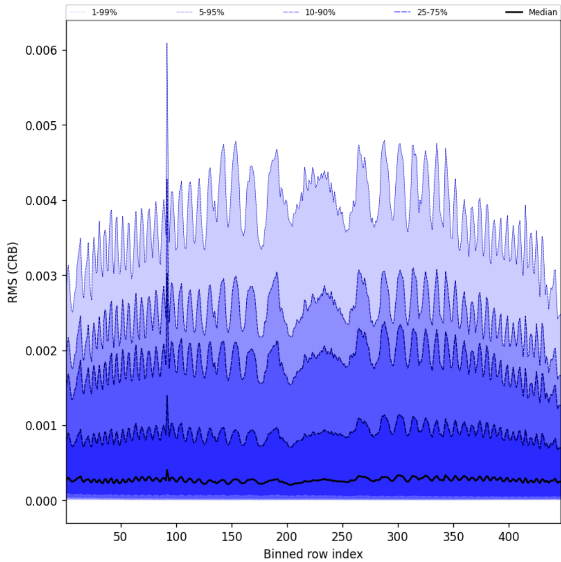
Figure 62: Along track statistics of “RMS (CRB)” for 2025-07-16 to 2025-07-16
