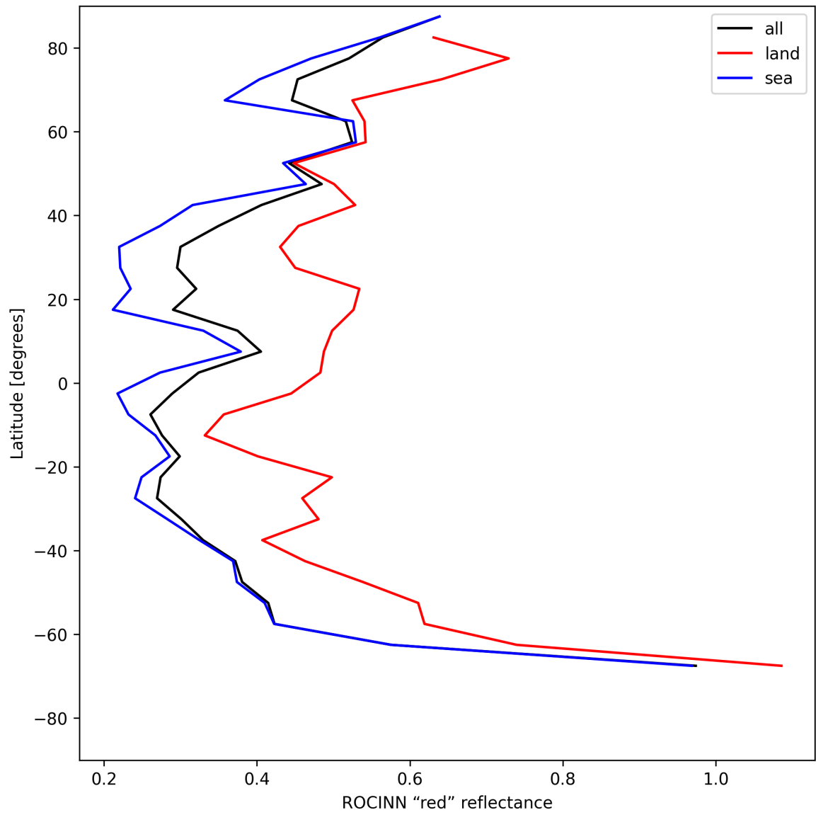
Figure 35: Zonal average of “ROCINN “red” reflectance” for 2025-07-16 to 2025-07-16.
