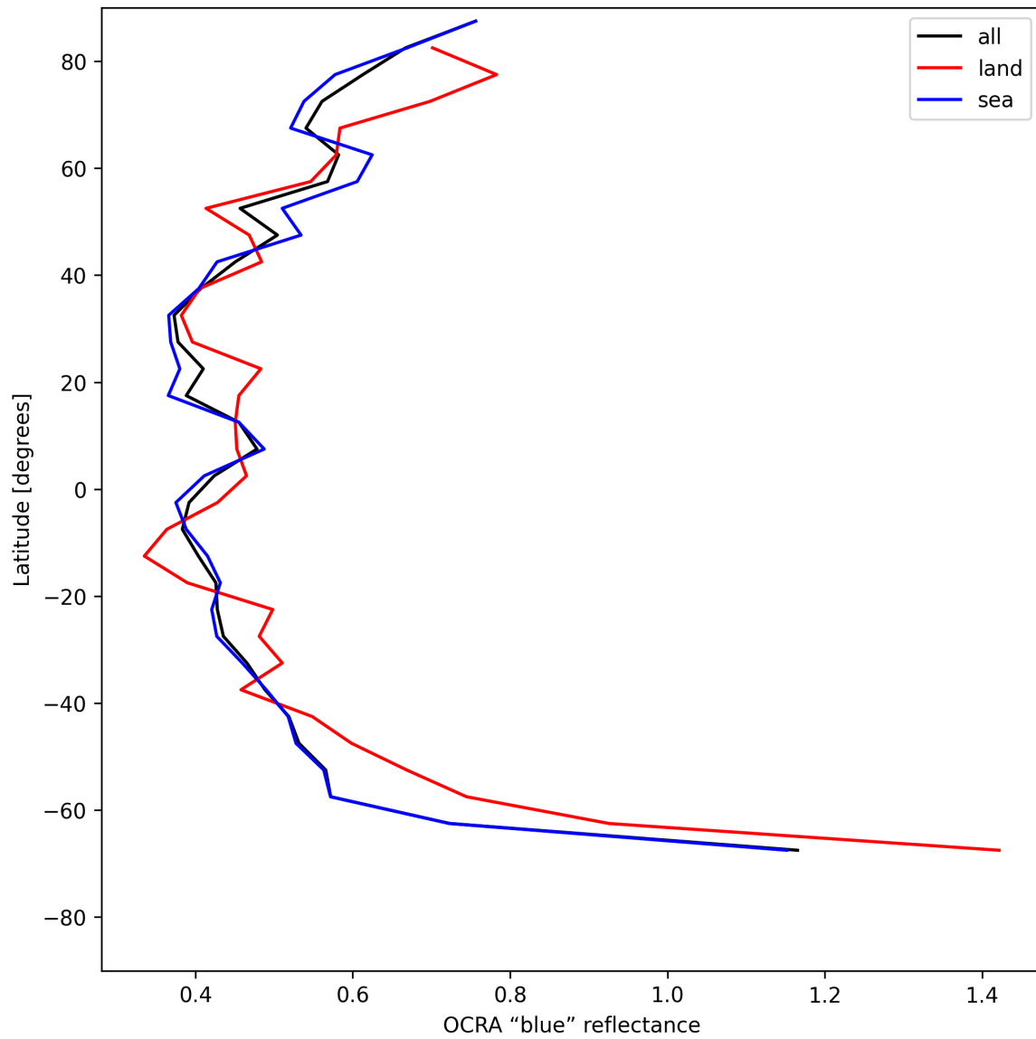
Figure 33: Zonal average of “OCRA “blue” reflectance” for 2025-07-16 to 2025-07-16.
