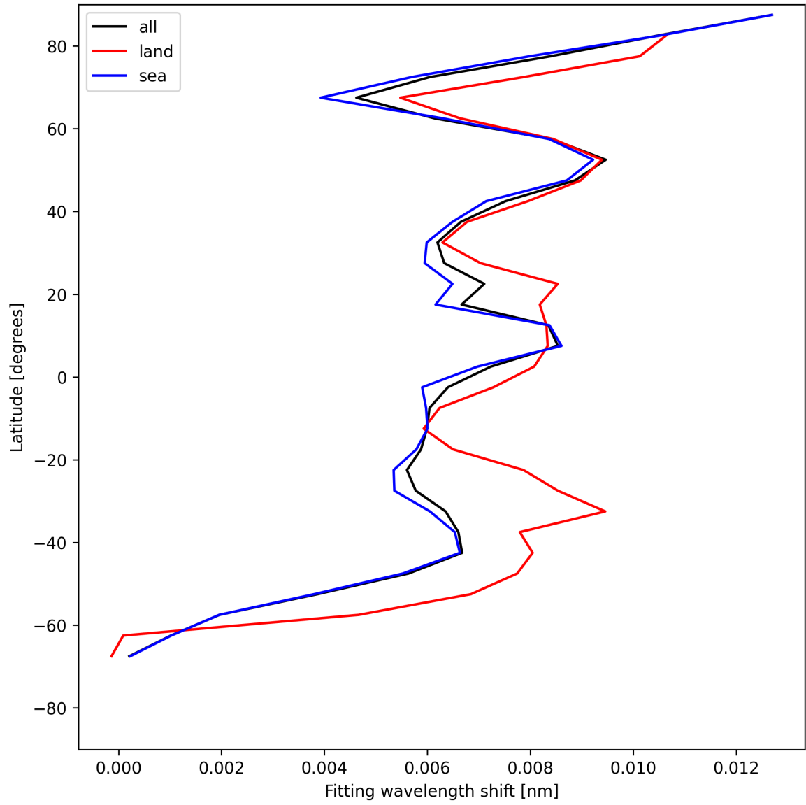
Figure 31: Zonal average of “Fitting wavelength shift” for 2025-07-16 to 2025-07-16.
