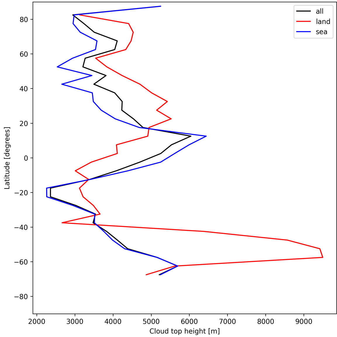
Figure 22: Zonal average of “Cloud top height” for 2025-07-16 to 2025-07-16.
