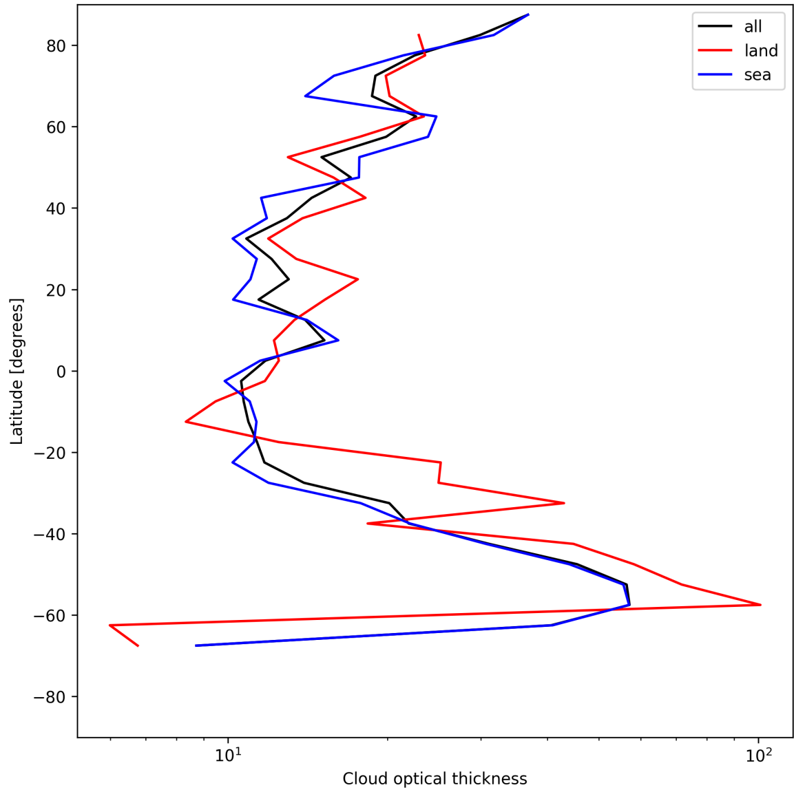
Figure 23: Zonal average of “Cloud optical thickness” for 2025-07-16 to 2025-07-16.
