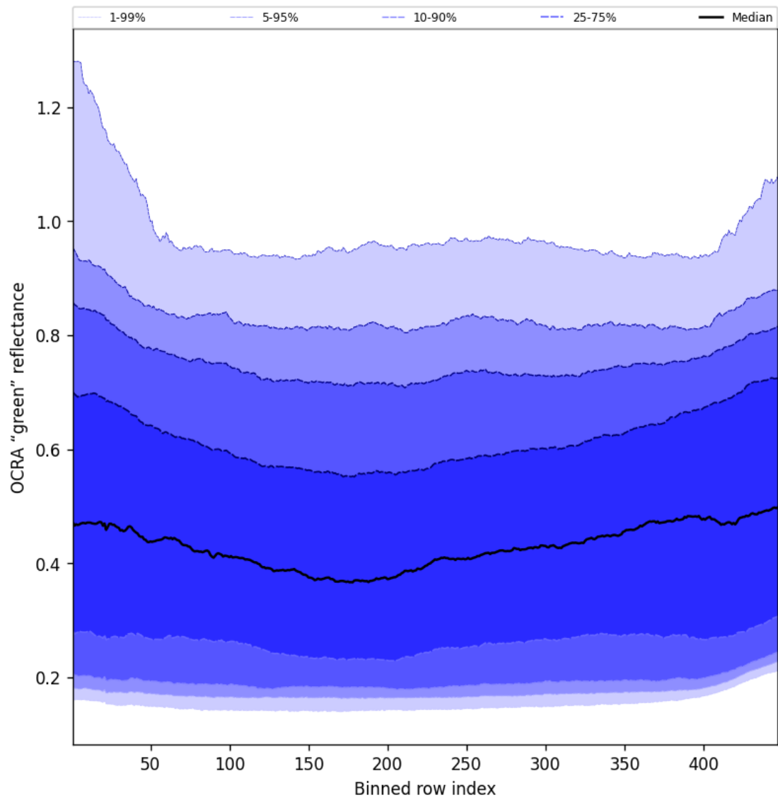
Figure 66: Along track statistics of "OCRA "green" reflectance" for 2025-07-16 to 2025-07-16
