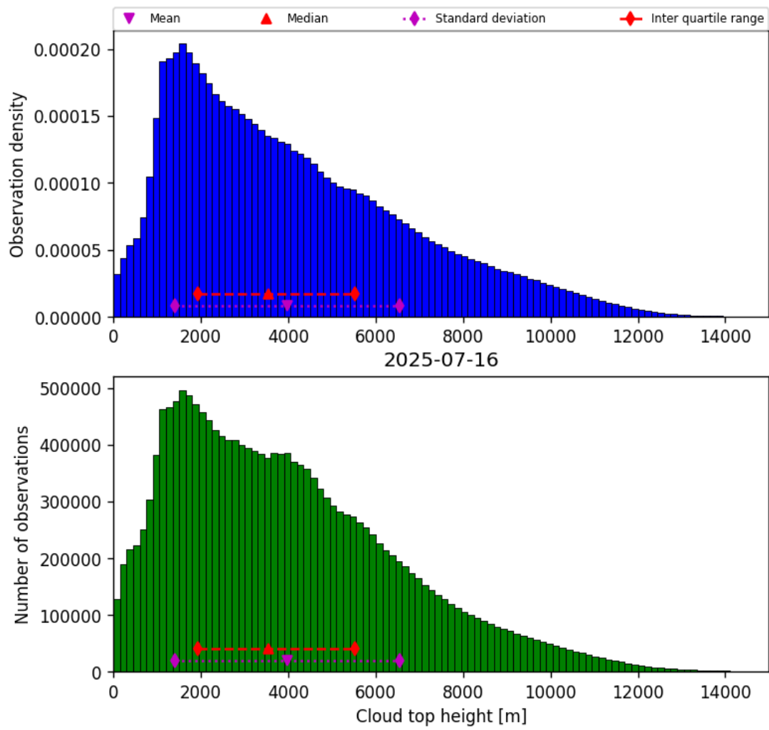
Figure 38: Histogram of “Cloud top height” for 2025-07-16 to 2025-07-16
