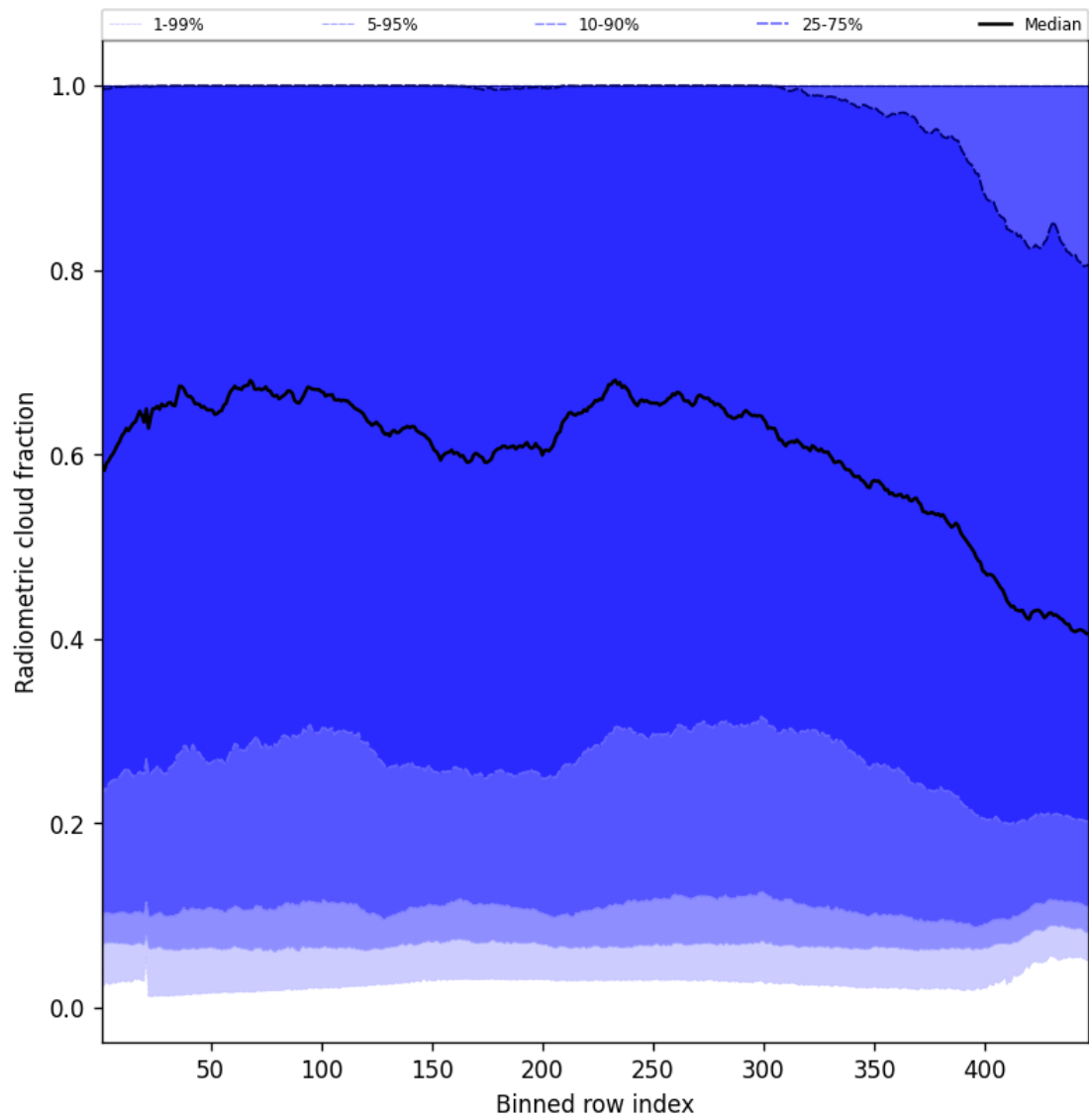
Figure 53: Along track statistics of “Radiometric cloud fraction” for 2025-07-16 to 2025-07-16
