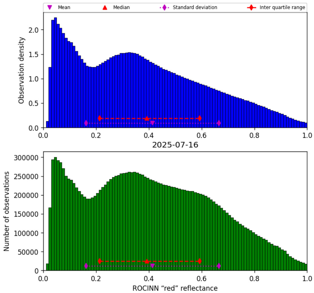
Figure 51: Histogram of “ROCINN “red” reflectance” for 2025-07-16 to 2025-07-16
