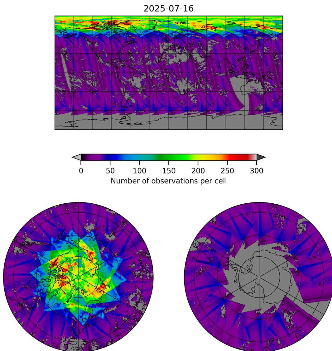
Figure 19: Map of the number of observations for 2025-07-16 to 2025-07-16
