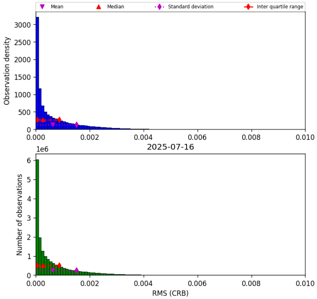
Figure 46: Histogram of “RMS (CRB)” for 2025-07-16 to 2025-07-16
