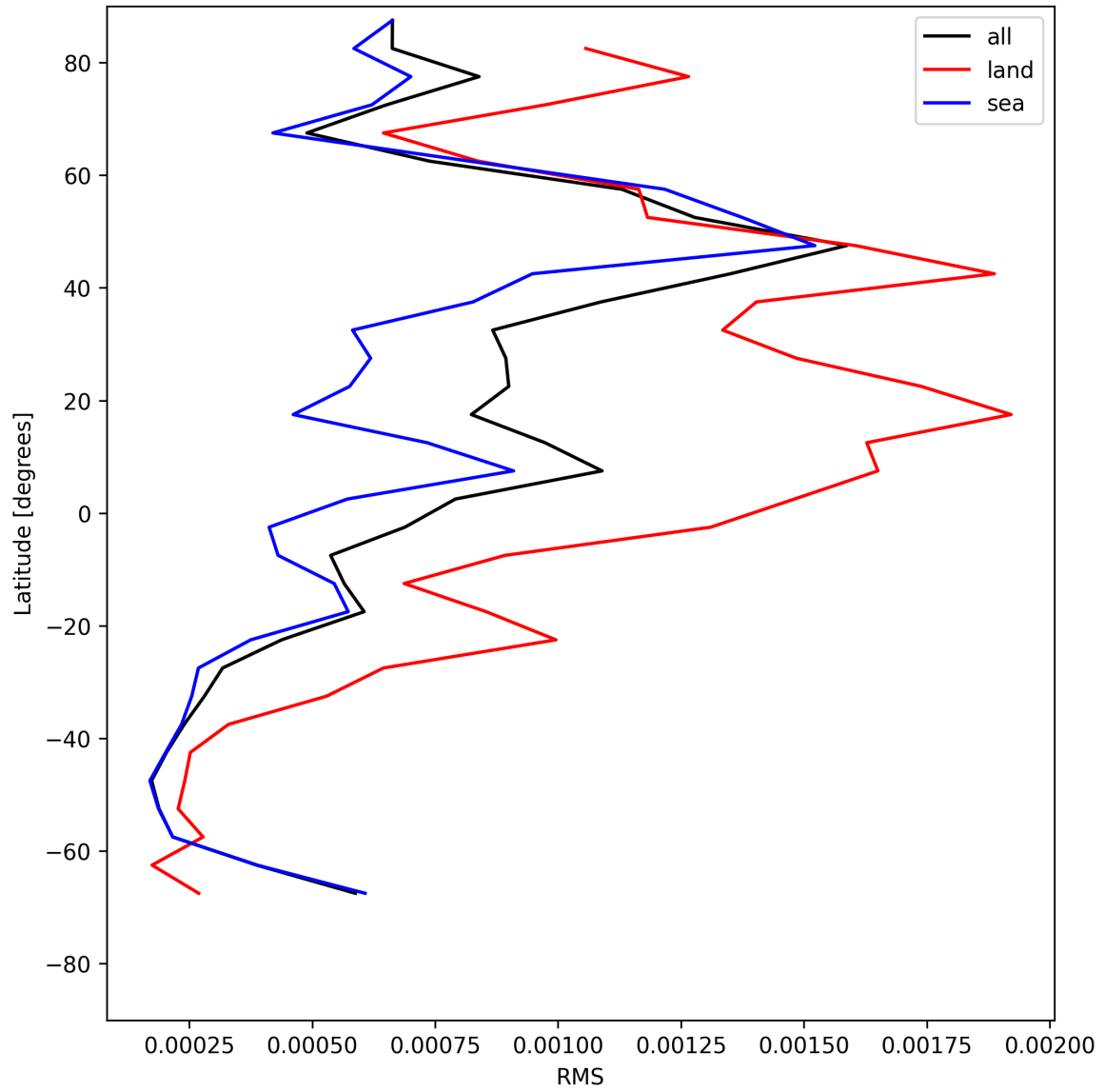
Figure 29: Zonal average of “RMS” for 2025-07-16 to 2025-07-16.
