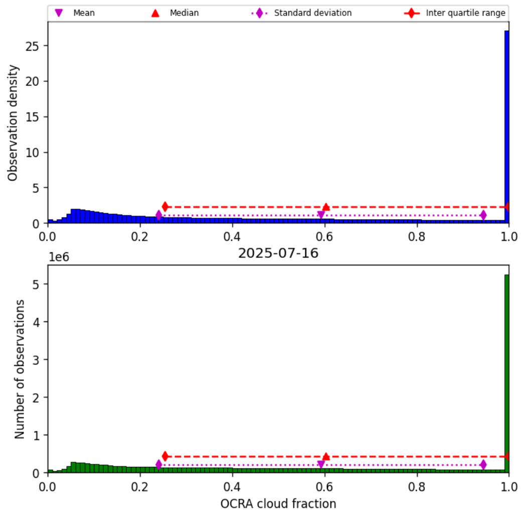
Figure 48: Histogram of “OCRA cloud fraction” for 2025-07-16 to 2025-07-16
