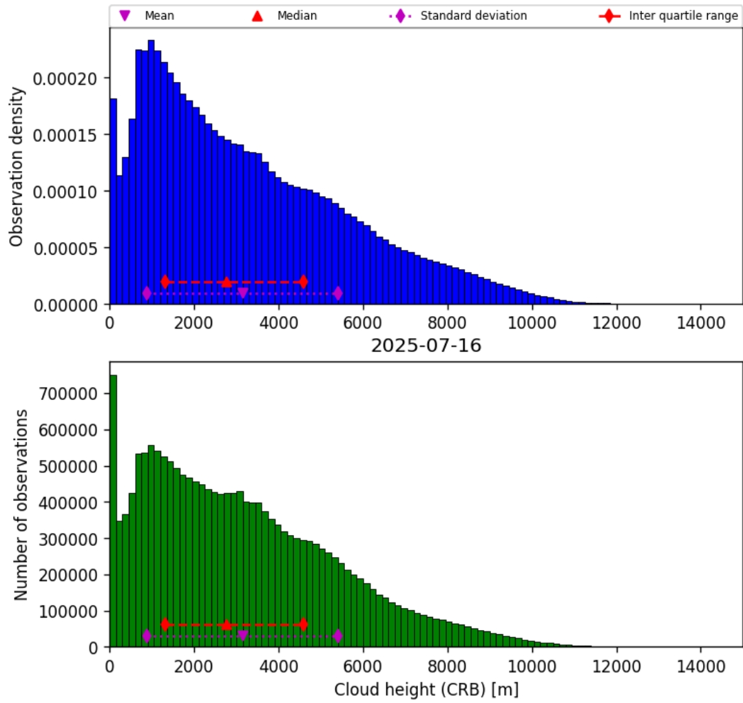
Figure 41: Histogram of “Cloud height (CRB)” for 2025-07-16 to 2025-07-16
