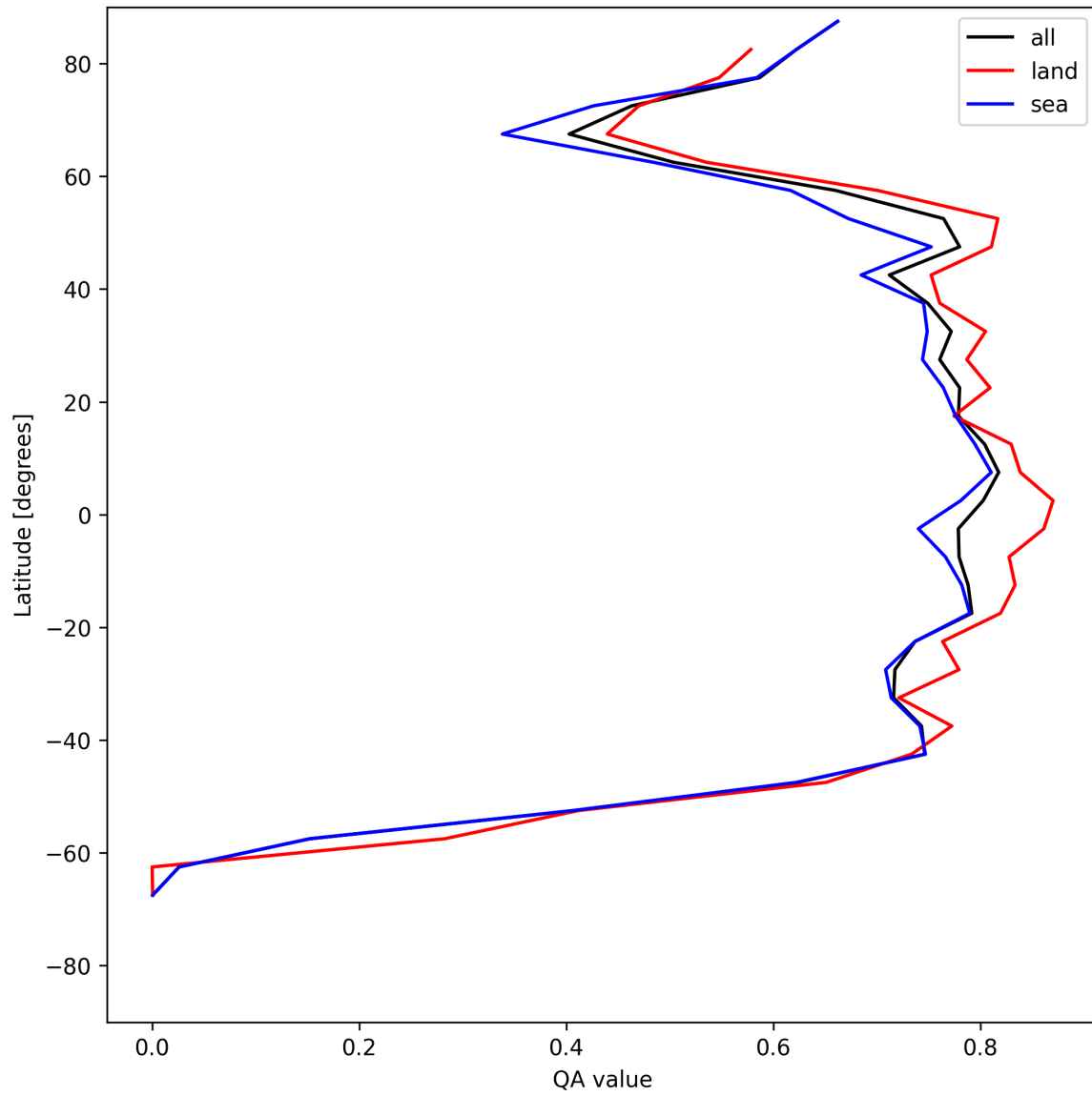
Figure 20: Zonal average of “QA value” for 2025-07-16 to 2025-07-16.
