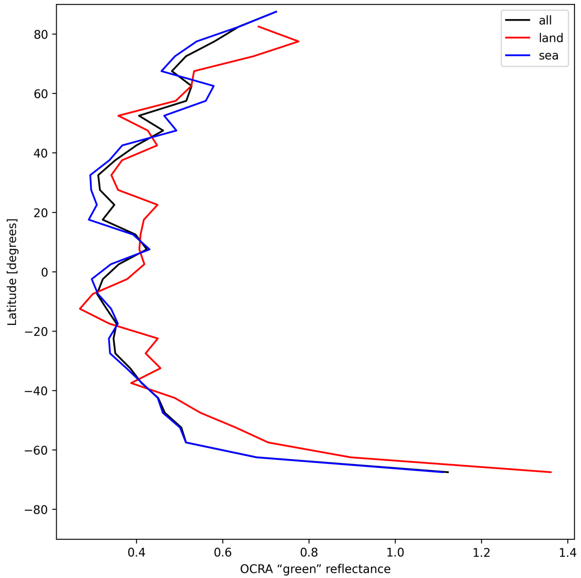
Figure 34: Zonal average of “OCRA “green” reflectance” for 2025-07-16 to 2025-07-16.
