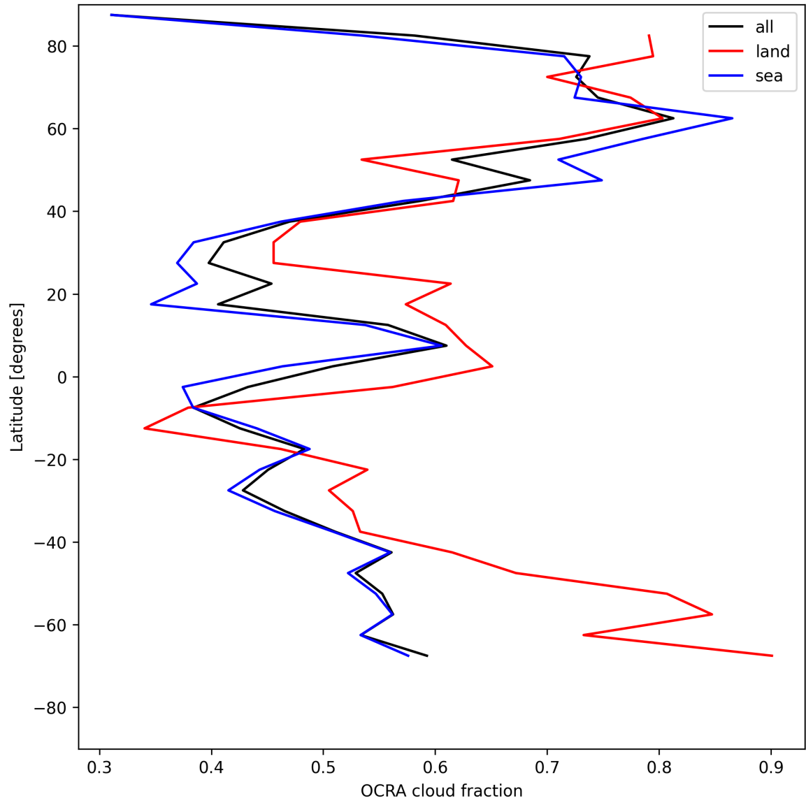
Figure 32: Zonal average of “OCRA cloud fraction” for 2025-07-16 to 2025-07-16.
