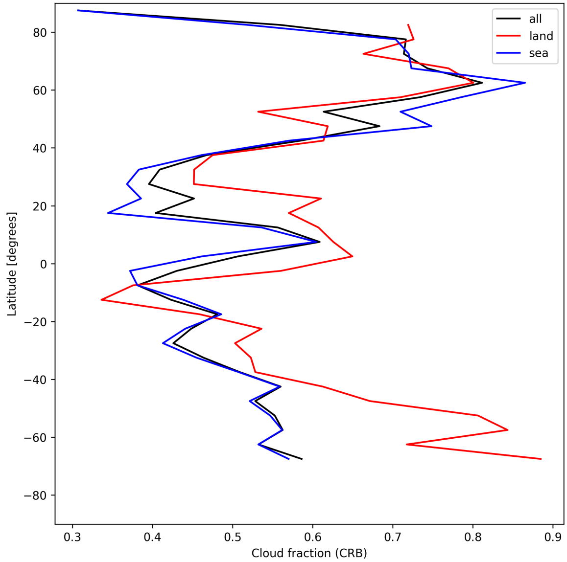
Figure 24: Zonal average of “Cloud fraction (CRB)” for 2025-07-16 to 2025-07-16.
