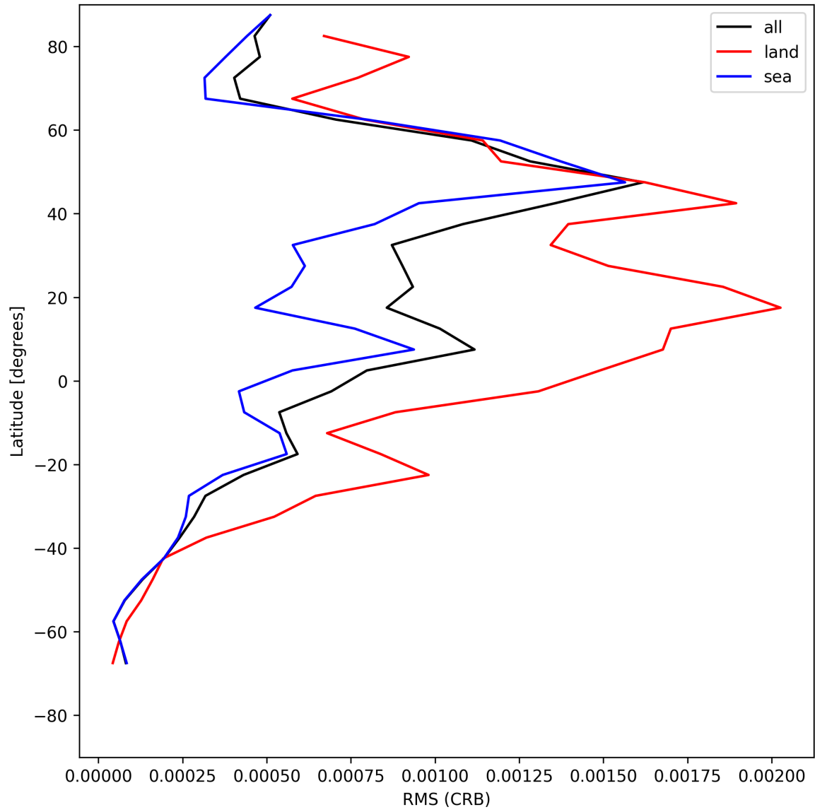
Figure 30: Zonal average of “RMS (CRB)” for 2025-07-16 to 2025-07-16.
