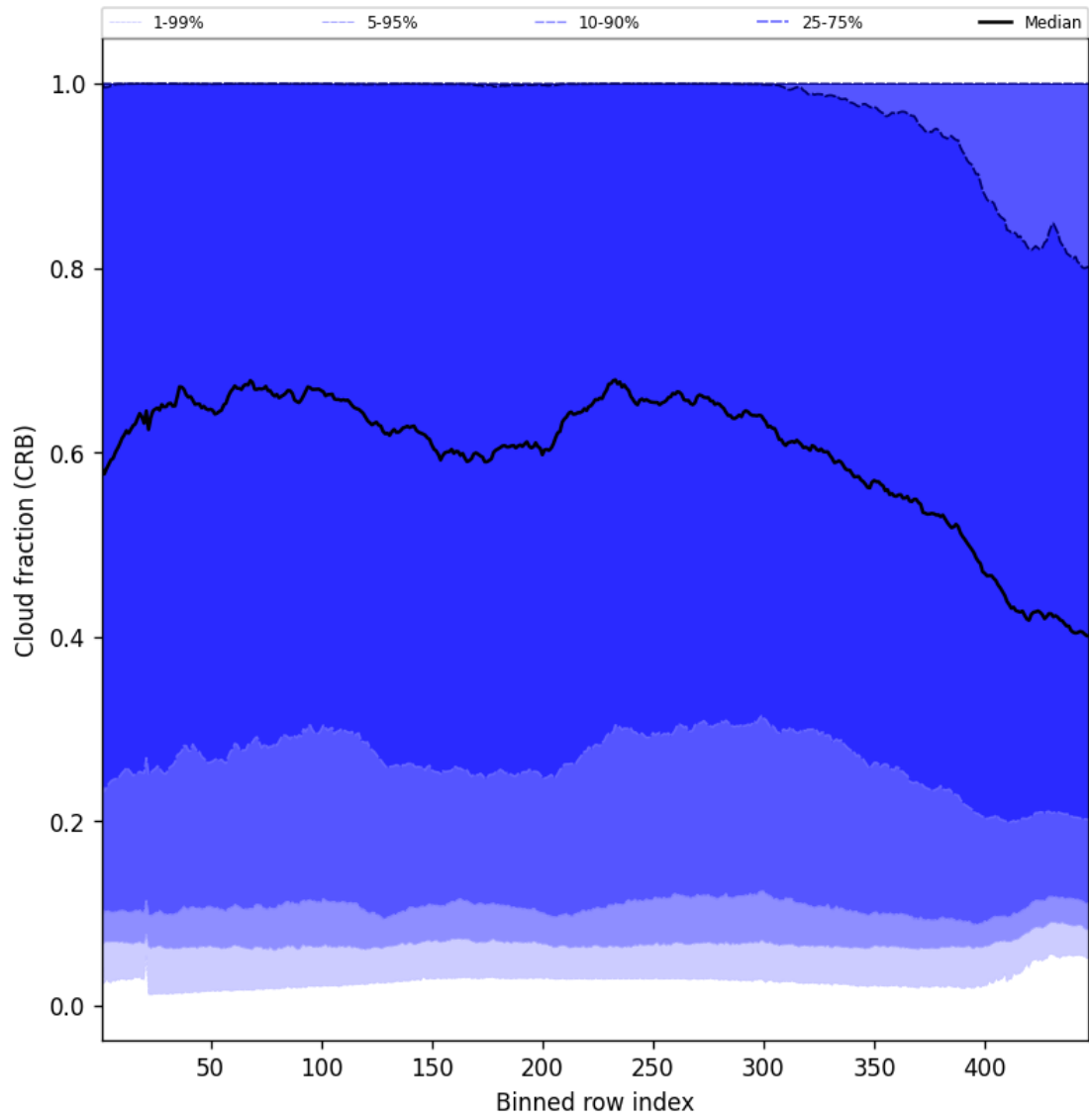
Figure 56: Along track statistics of “Cloud fraction (CRB)” for 2025-07-16 to 2025-07-16
