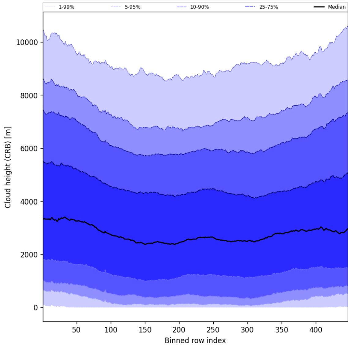
Figure 57: Along track statistics of “Cloud height (CRB)” for 2025-07-16 to 2025-07-16
