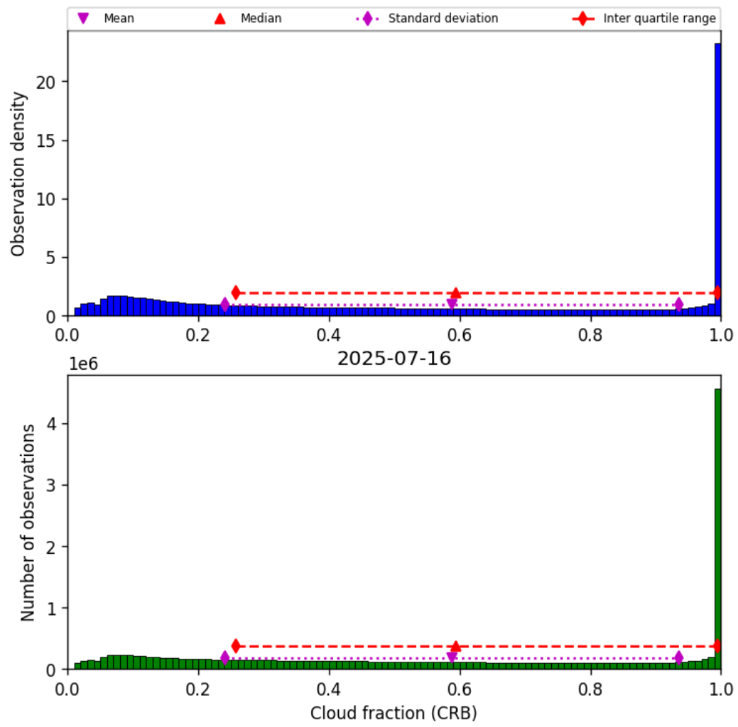
Figure 40: Histogram of “Cloud fraction (CRB)” for 2025-07-16 to 2025-07-16
