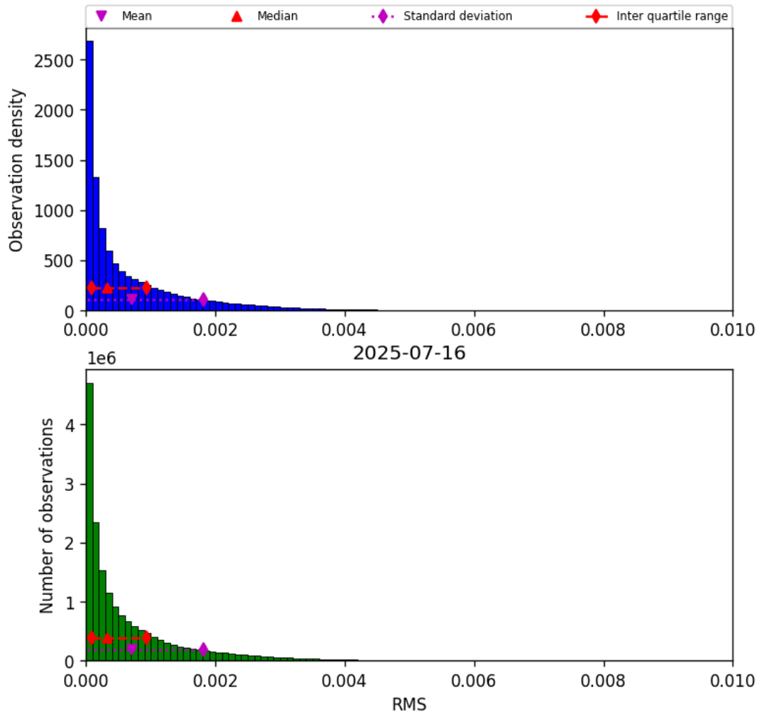
Figure 45: Histogram of “RMS” for 2025-07-16 to 2025-07-16
