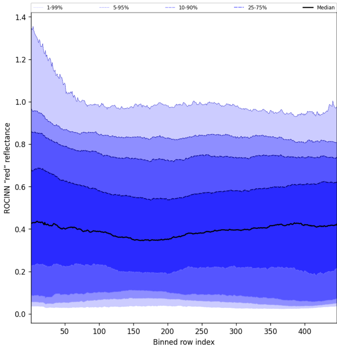
Figure 67: Along track statistics of “ROCINN “red” reflectance” for 2025-07-16 to 2025-07-16
