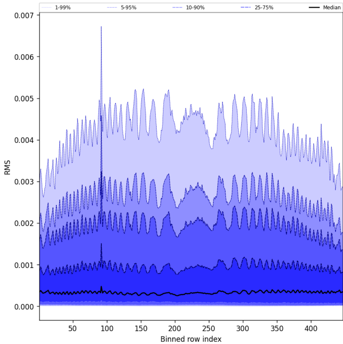
Figure 61: Along track statistics of “RMS” for 2025-07-16 to 2025-07-16
