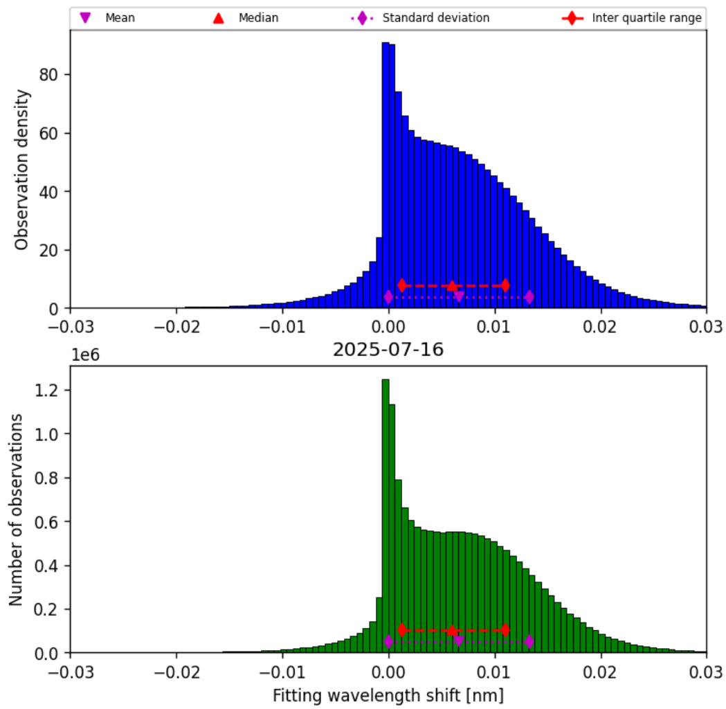
Figure 47: Histogram of “Fitting wavelength shift” for 2025-07-16 to 2025-07-16
