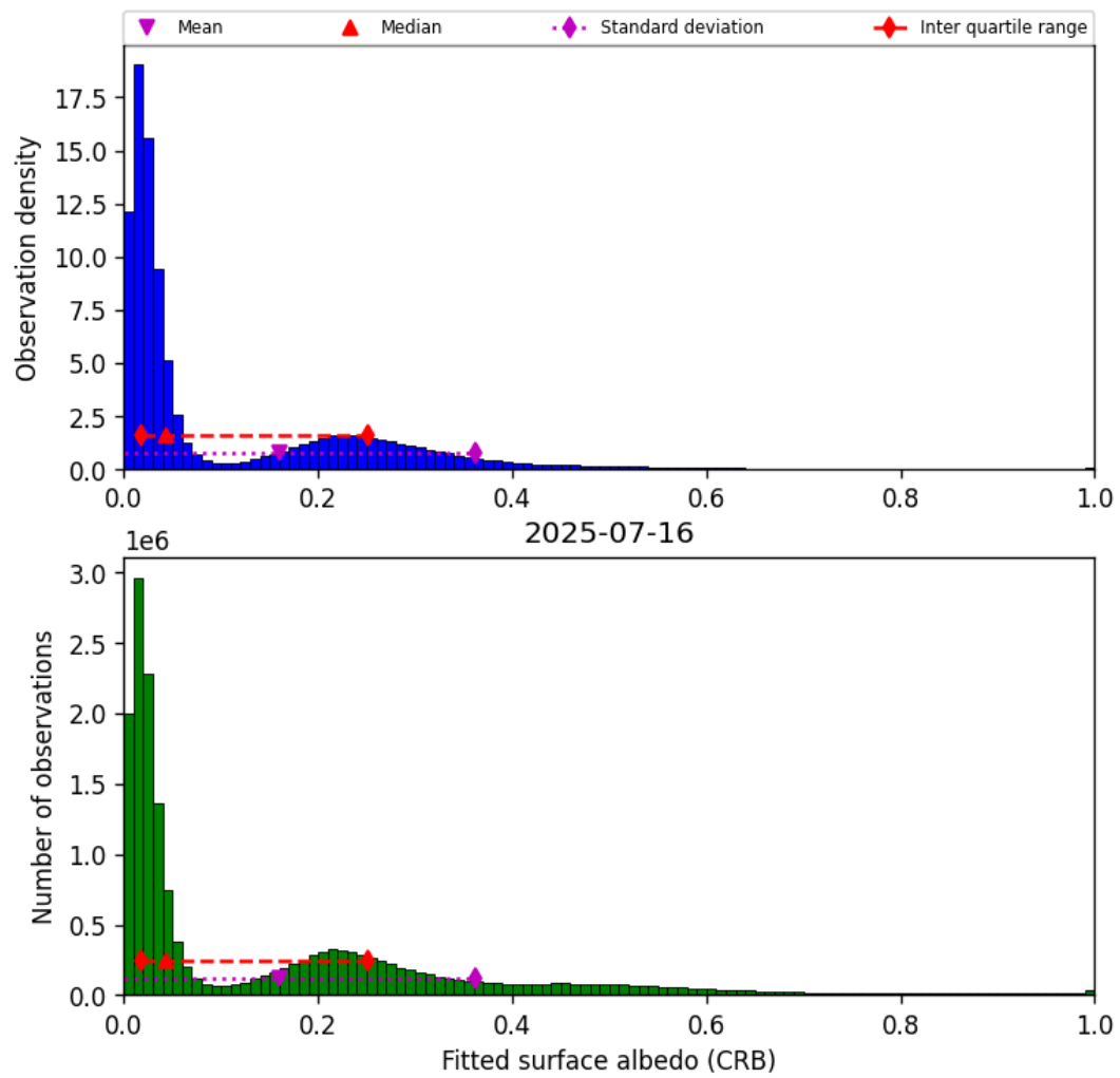
Figure 44: Histogram of “Fitted surface albedo (CRB)” for 2025-07-16 to 2025-07-16
