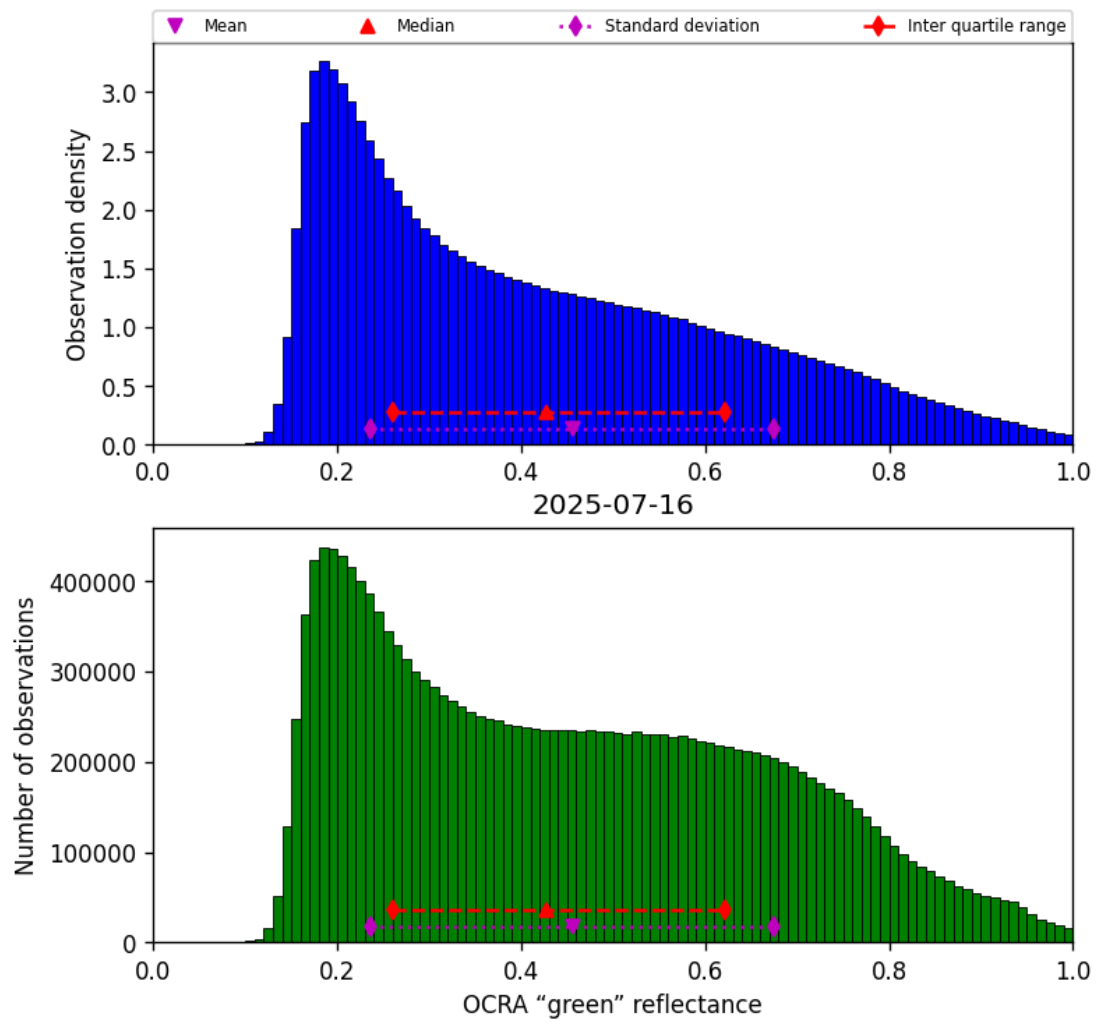
Figure 50: Histogram of “OCRA “green” reflectance” for 2025-07-16 to 2025-07-16
