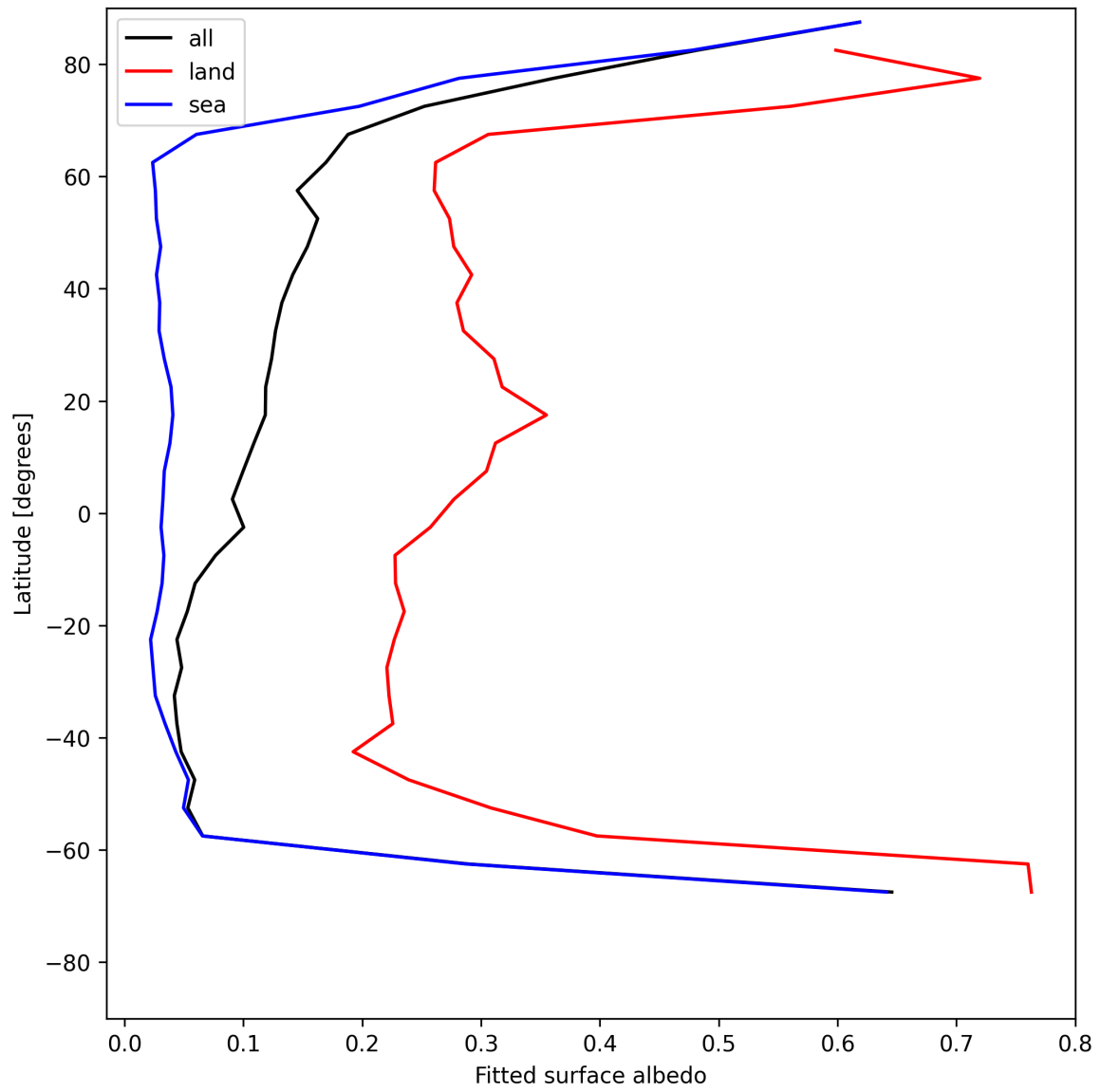
Figure 27: Zonal average of “Fitted surface albedo” for 2025-07-16 to 2025-07-16.
