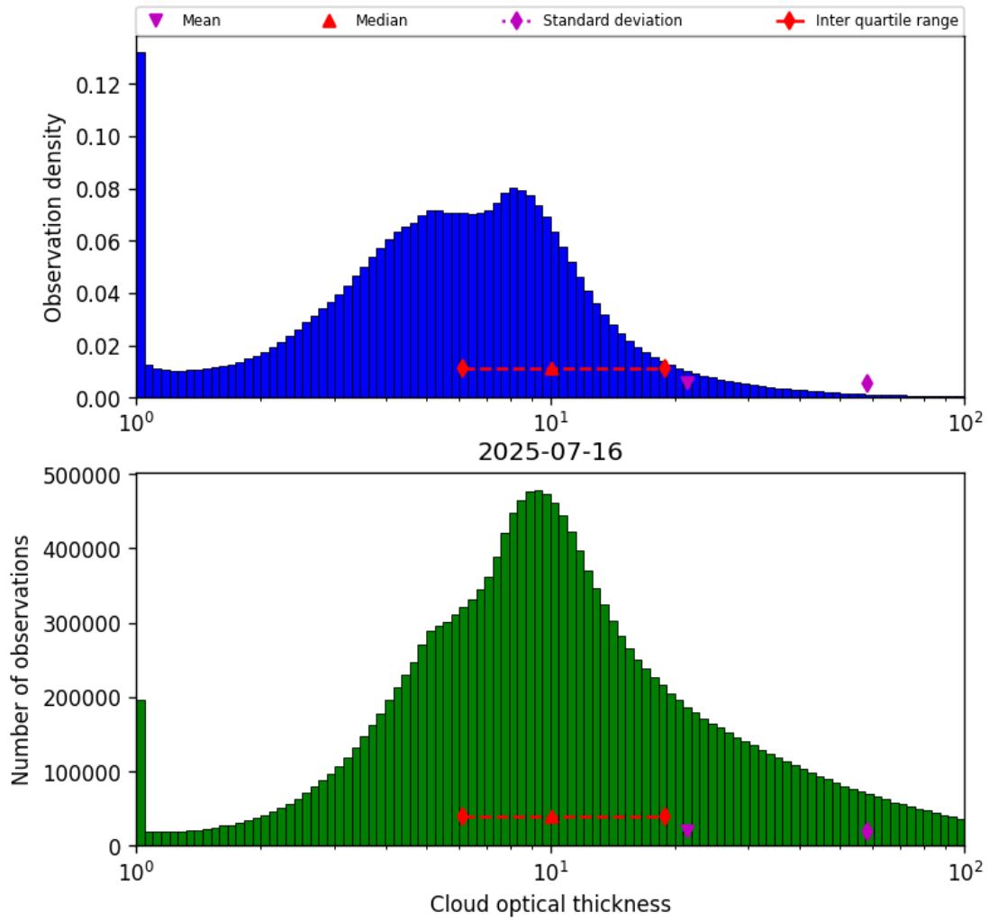
Figure 39: Histogram of “Cloud optical thickness” for 2025-07-16 to 2025-07-16
