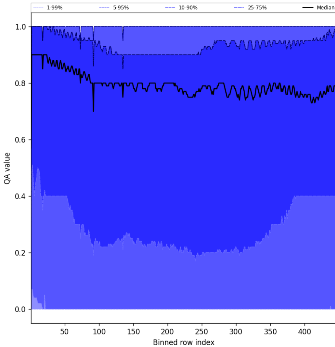
Figure 52: Along track statistics of “QA value” for 2025-07-16 to 2025-07-16
