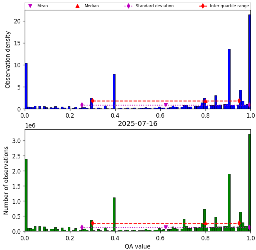
Figure 36: Histogram of “QA value” for 2025-07-16 to 2025-07-16
