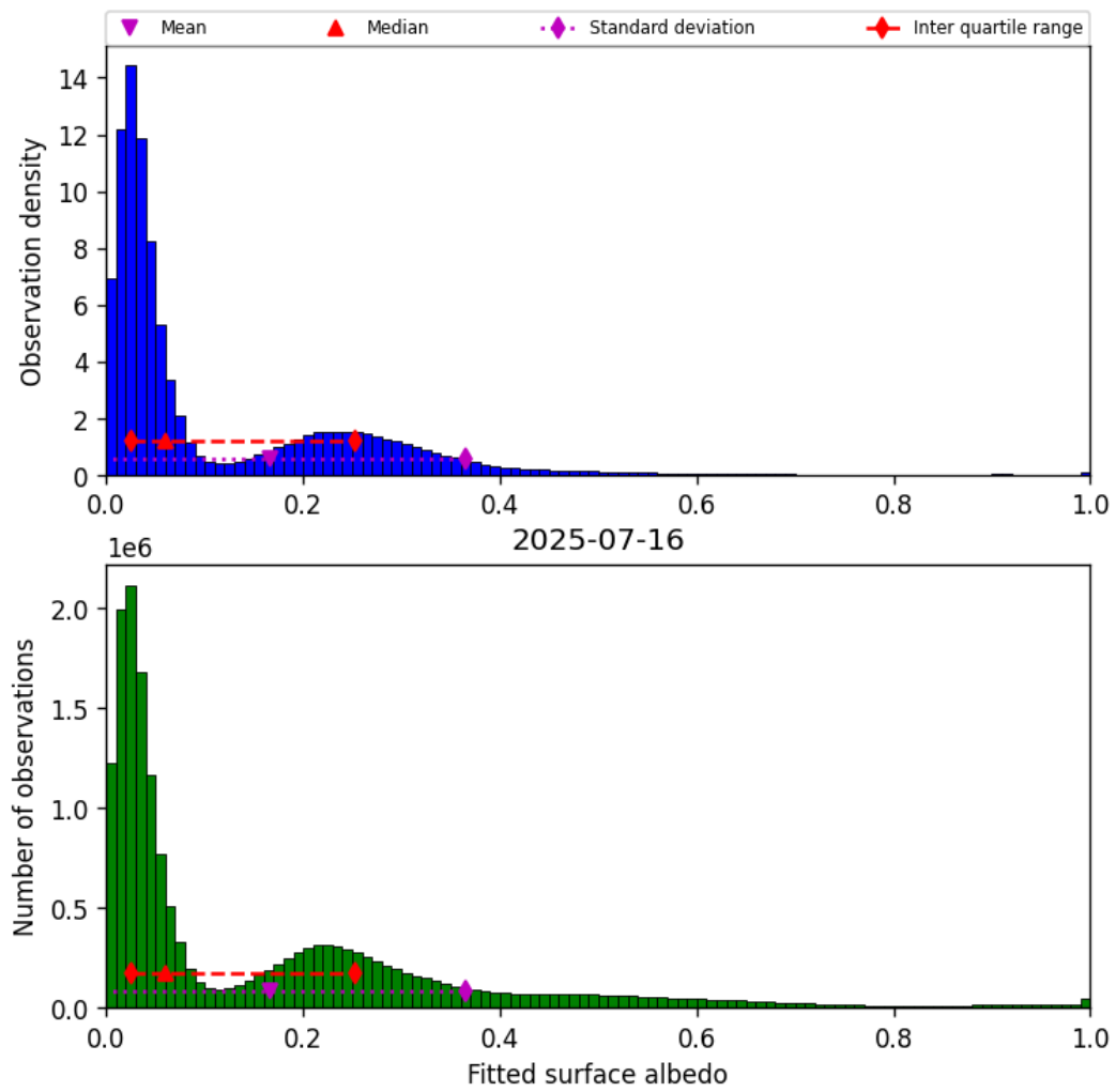
Figure 43: Histogram of “Fitted surface albedo” for 2025-07-16 to 2025-07-16
