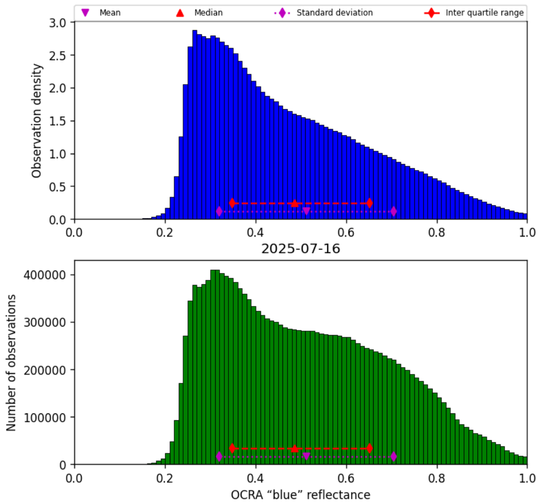
Figure 49: Histogram of “OCRA “blue” reflectance” for 2025-07-16 to 2025-07-16
