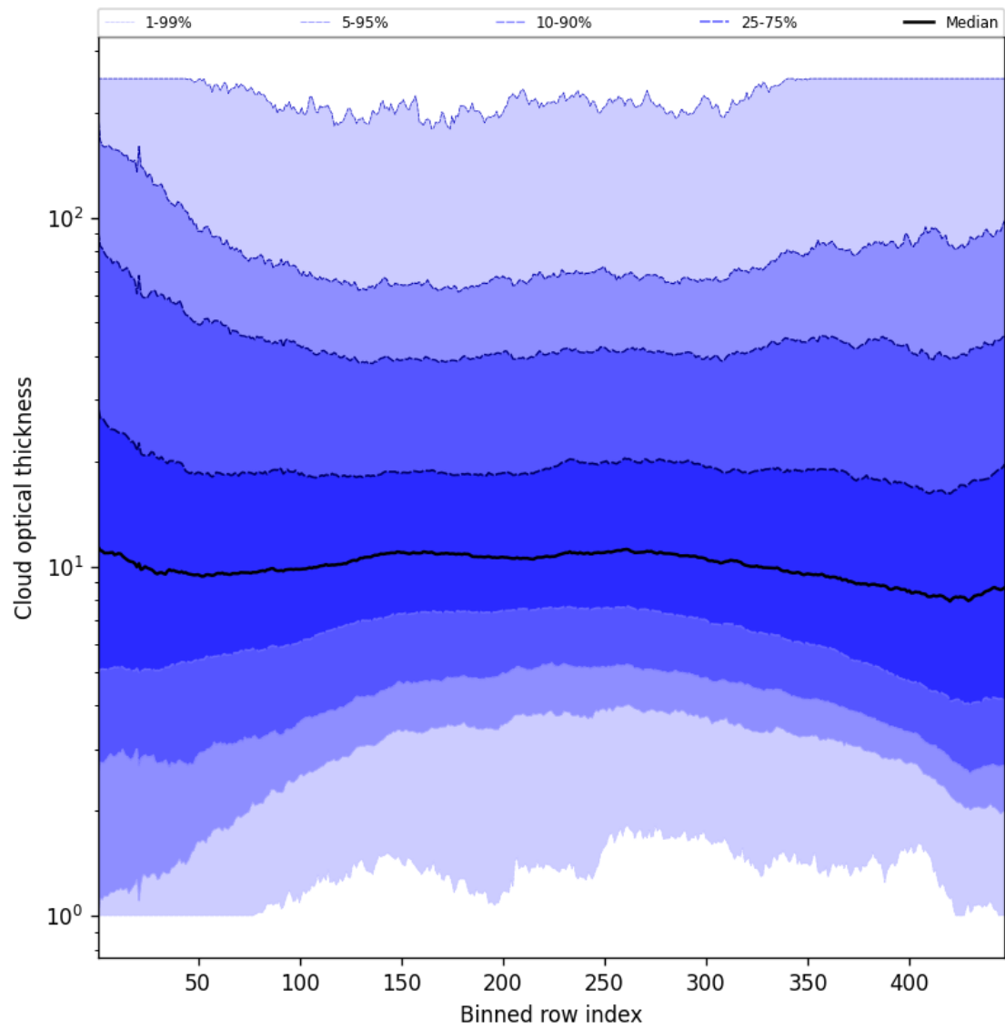
Figure 55: Along track statistics of “Cloud optical thickness” for 2025-07-16 to 2025-07-16
