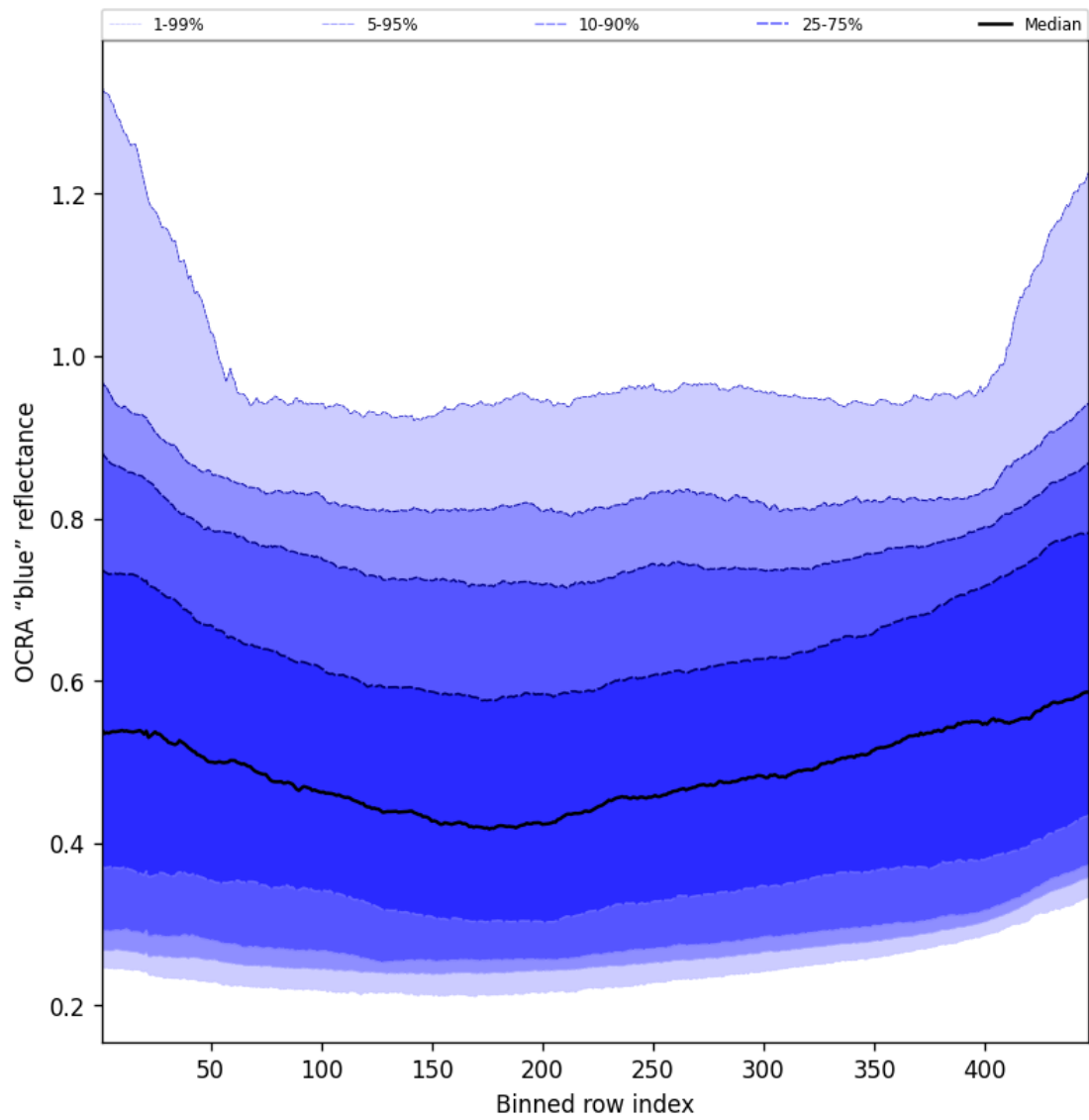
Figure 65: Along track statistics of “OCRA “blue” reflectance” for 2025-07-16 to 2025-07-16
