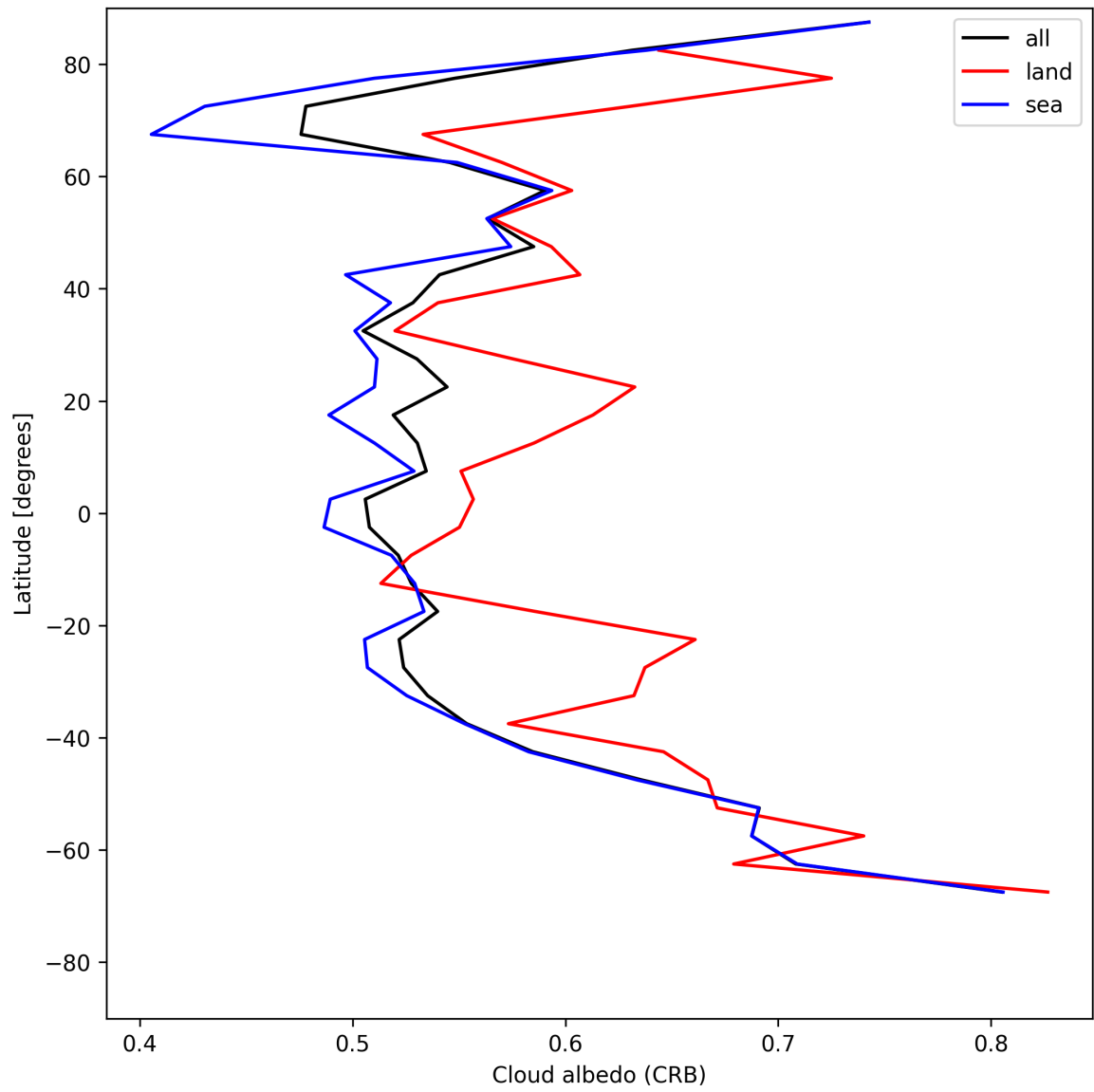
Figure 26: Zonal average of “Cloud albedo (CRB)” for 2025-07-16 to 2025-07-16.
