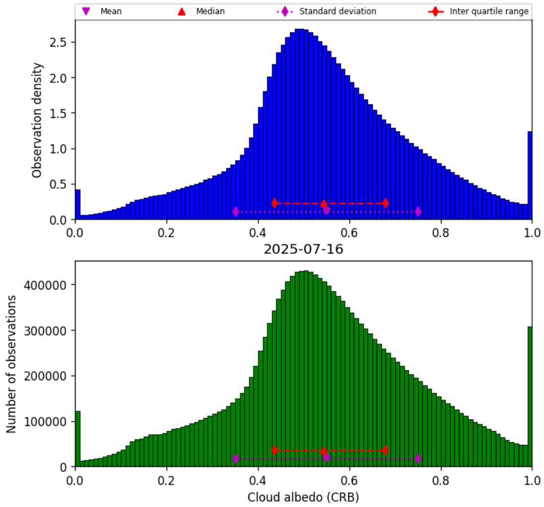
Figure 42: Histogram of “Cloud albedo (CRB)” for 2025-07-16 to 2025-07-16
