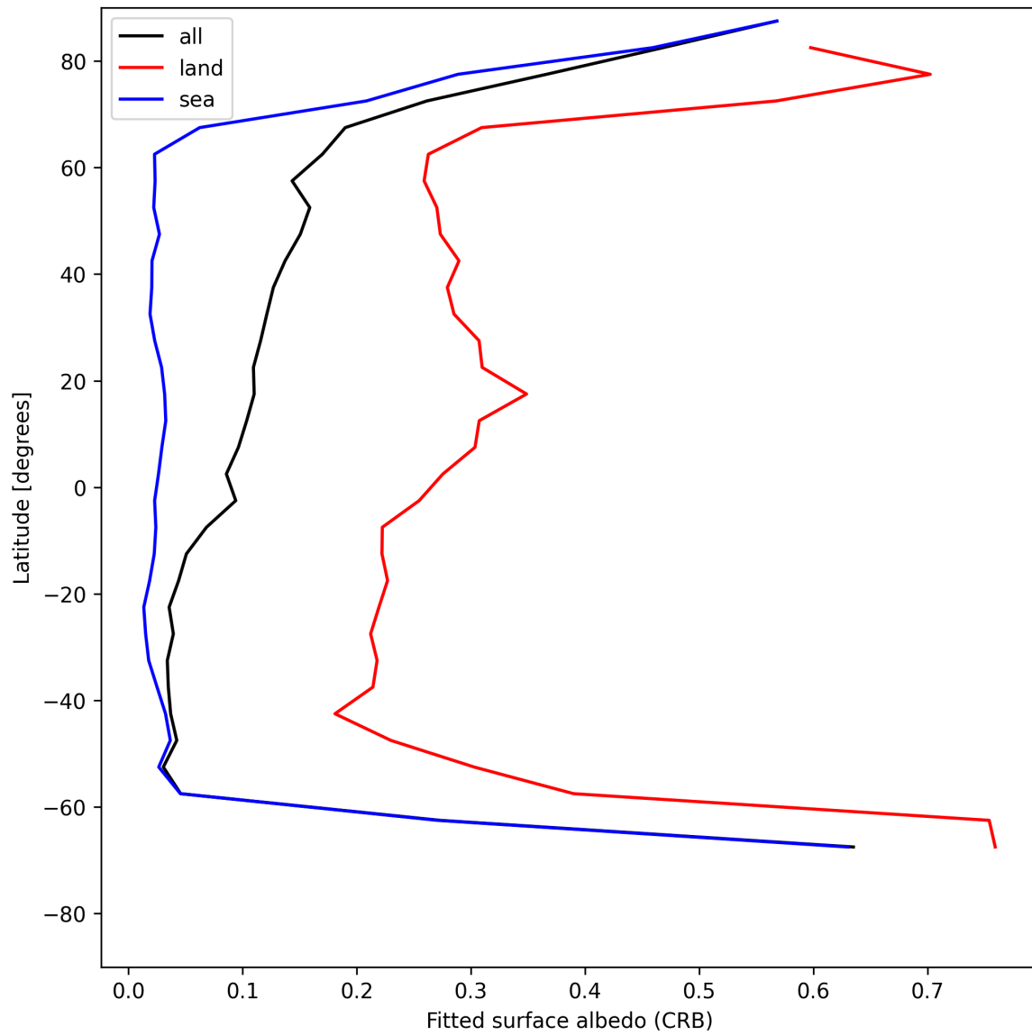
Figure 28: Zonal average of “Fitted surface albedo (CRB)” for 2025-07-16 to 2025-07-16.
