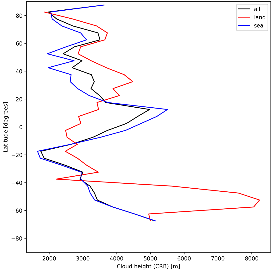
Figure 25: Zonal average of “Cloud height (CRB)” for 2025-07-16 to 2025-07-16.
