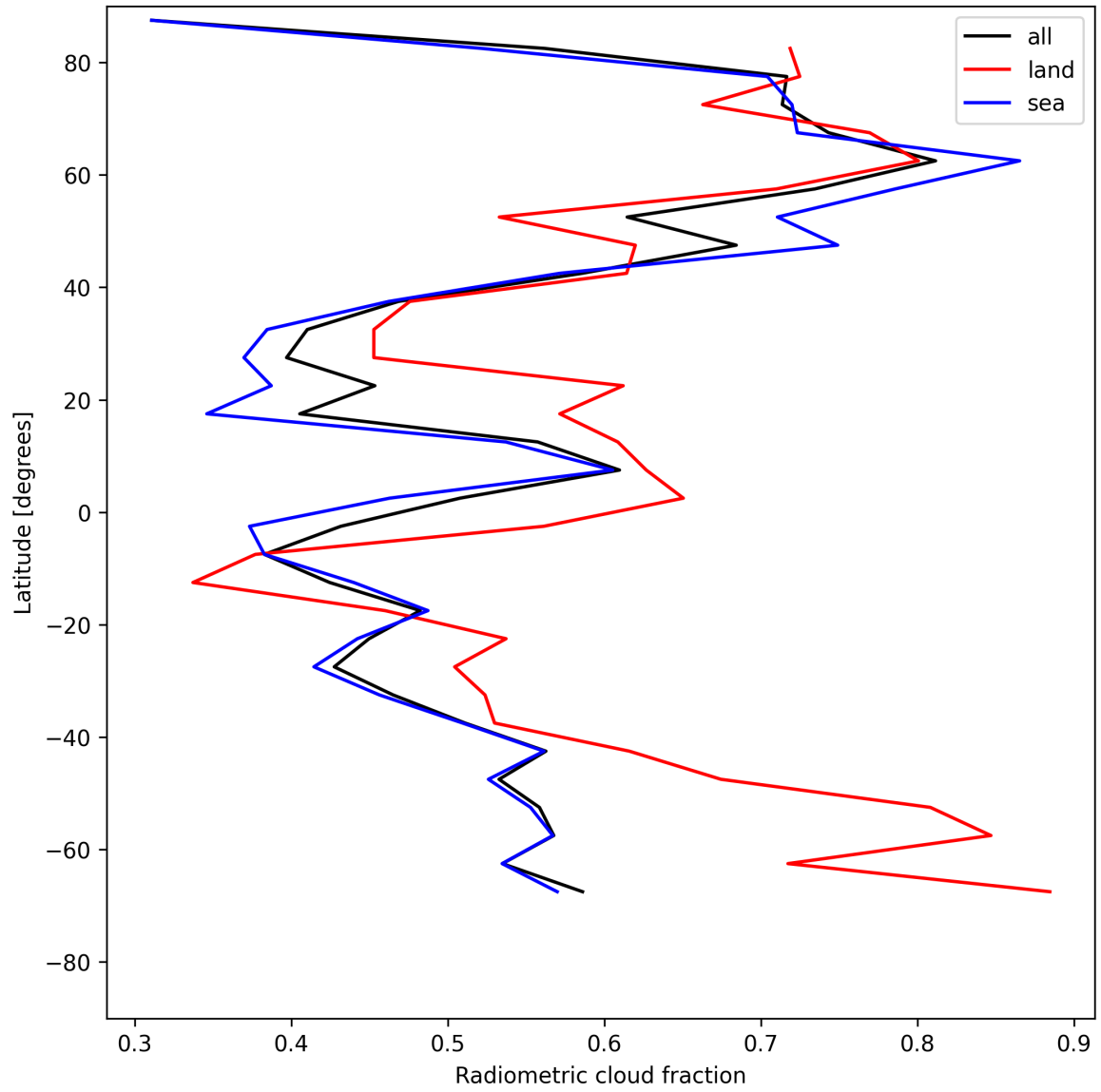
Figure 21: Zonal average of “Radiometric cloud fraction” for 2025-07-16 to 2025-07-16.
