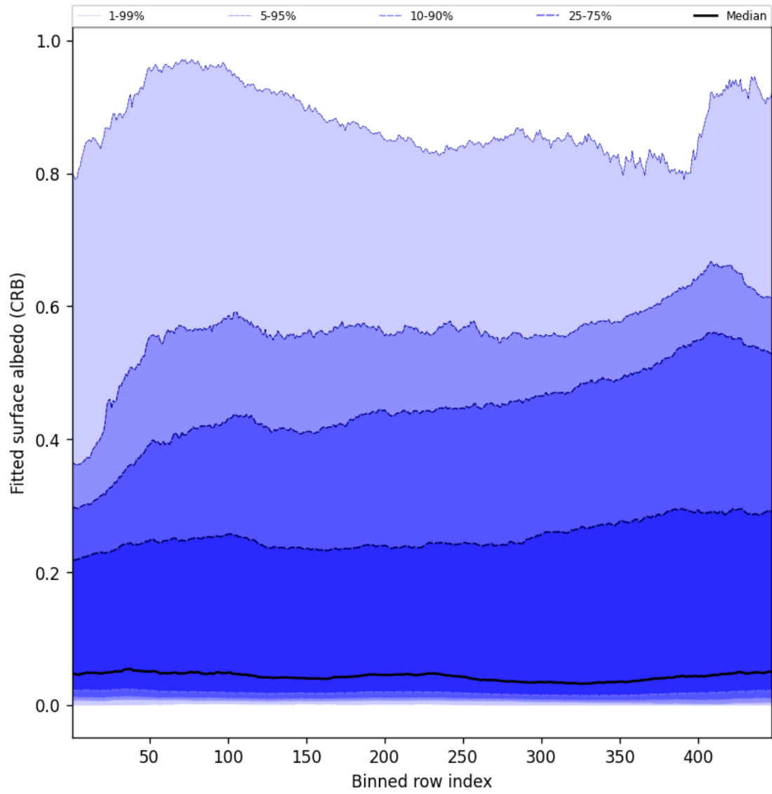
Figure 60: Along track statistics of “Fitted surface albedo (CRB)” for 2025-07-16 to 2025-07-16
