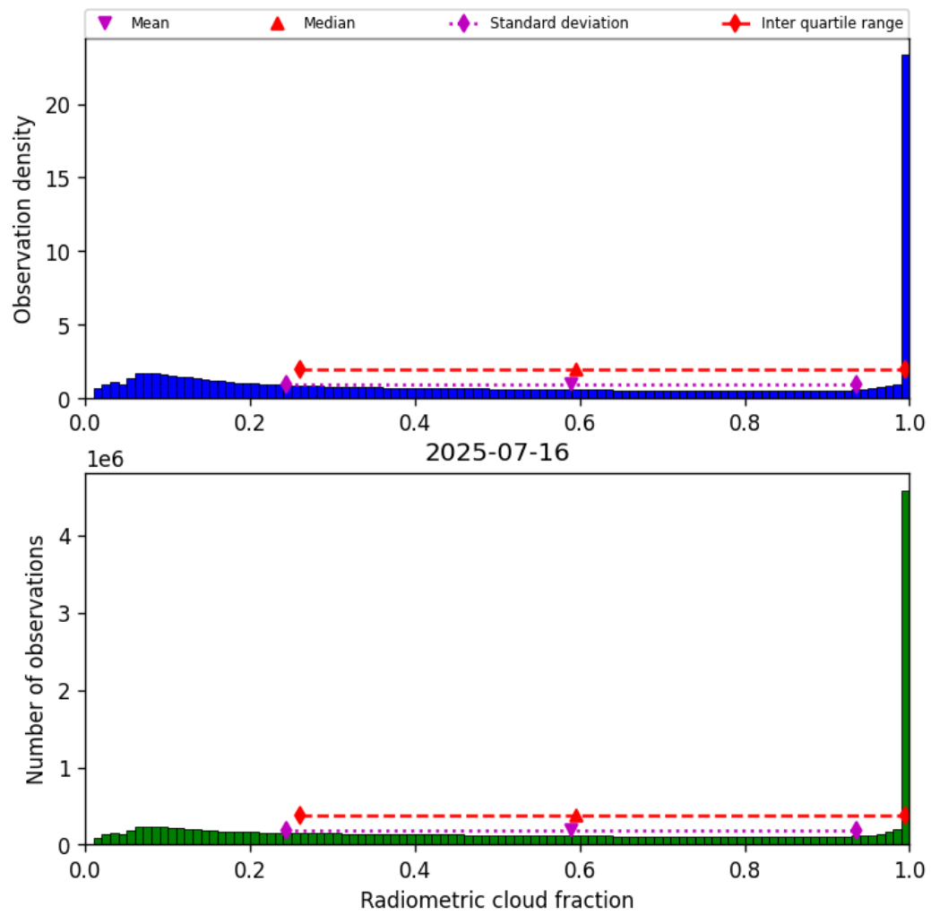
Figure 37: Histogram of “Radiometric cloud fraction” for 2025-07-16 to 2025-07-16
