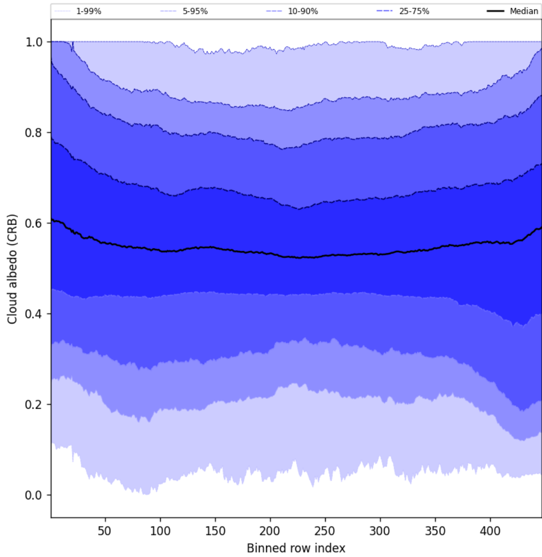
Figure 58: Along track statistics of “Cloud albedo (CRB)” for 2025-07-16 to 2025-07-16
