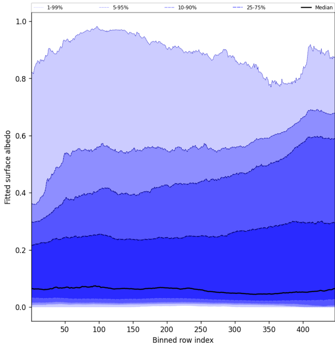
Figure 59: Along track statistics of "Fitted surface albedo" for 2025-07-16 to 2025-07-16
