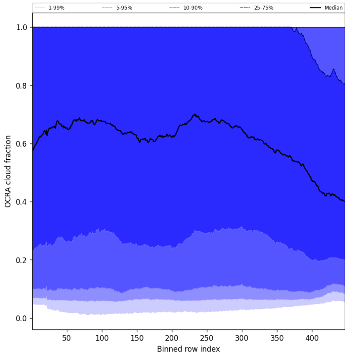
Figure 64: Along track statistics of “OCRA cloud fraction” for 2025-07-16 to 2025-07-16
