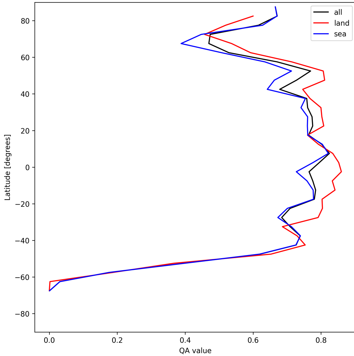
Figure 20: Zonal average of “QA value” for 2025-07-17 to 2025-07-18.
