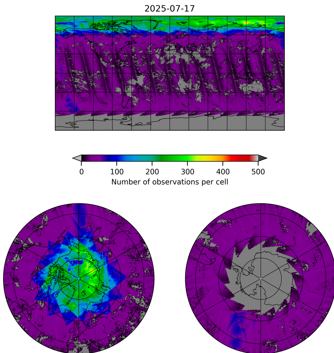
Figure 19: Map of the number of observations for 2025-07-17 to 2025-07-18
