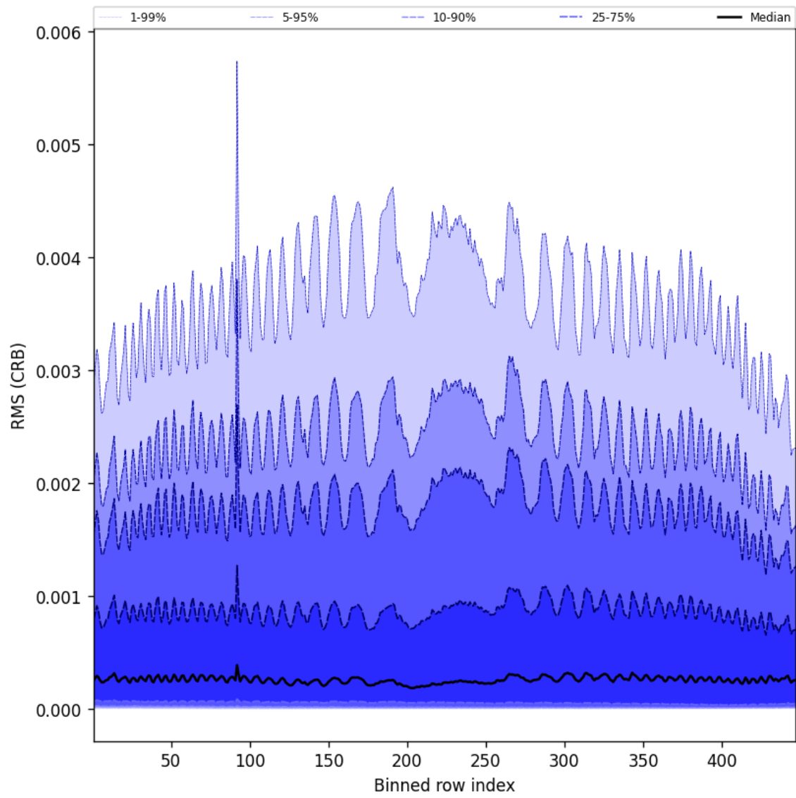
Figure 62: Along track statistics of “RMS (CRB)” for 2025-07-17 to 2025-07-18
