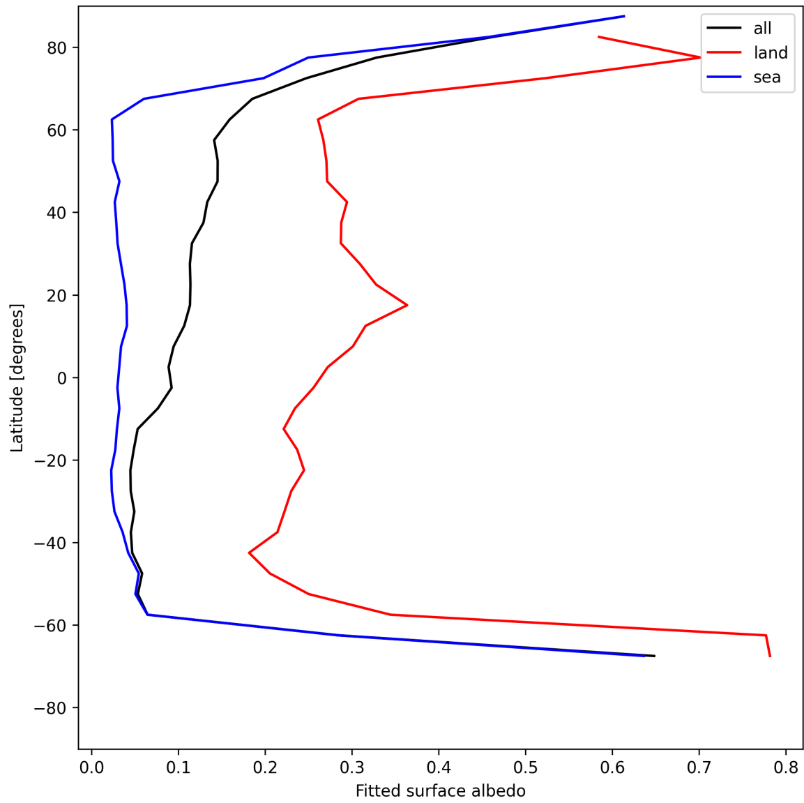
Figure 27: Zonal average of “Fitted surface albedo” for 2025-07-17 to 2025-07-18.
