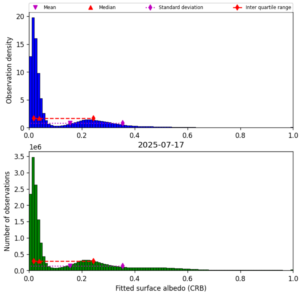
Figure 44: Histogram of “Fitted surface albedo (CRB)” for 2025-07-17 to 2025-07-18
