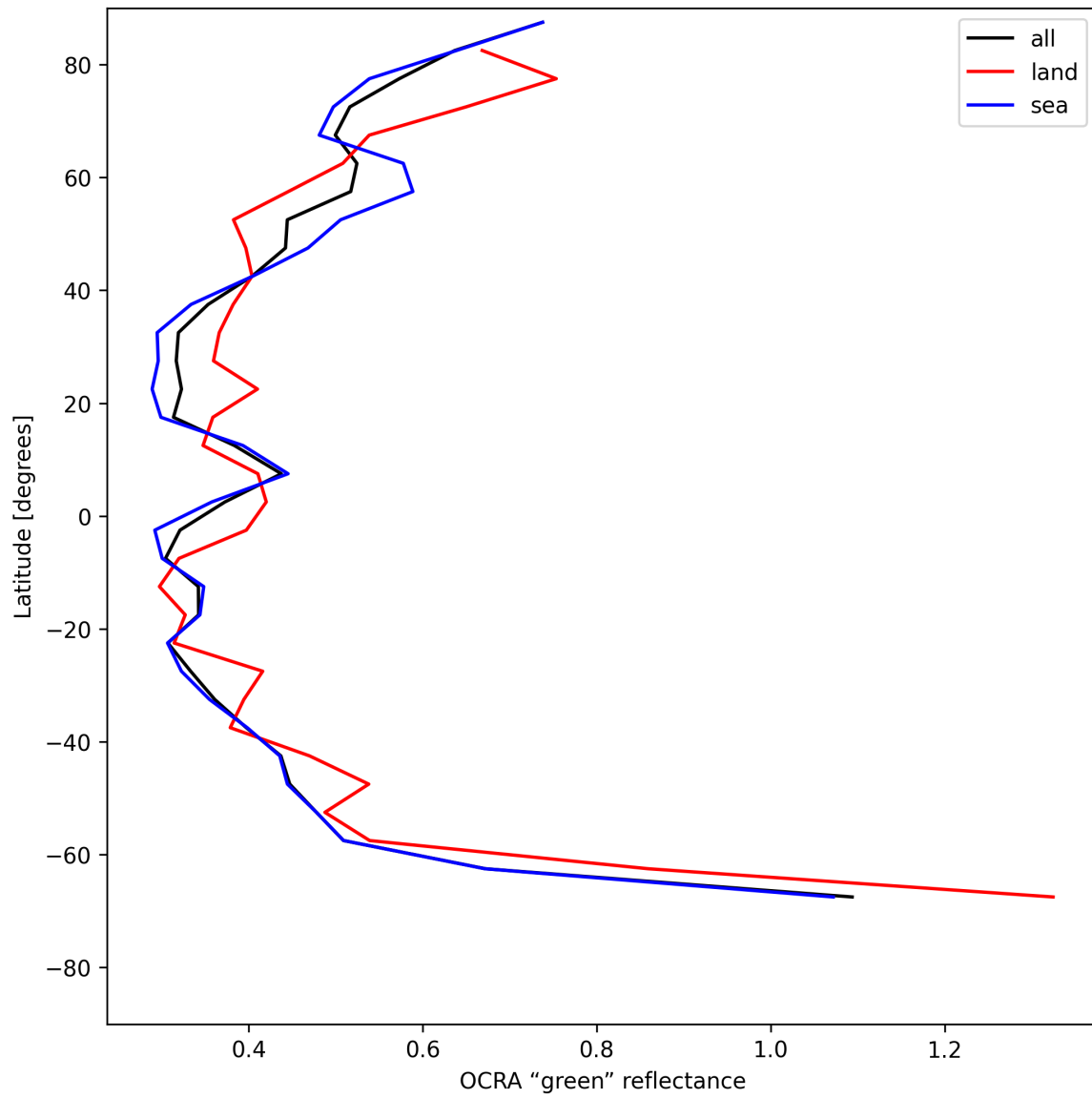
Figure 34: Zonal average of “OCRA “green” reflectance” for 2025-07-17 to 2025-07-18.
