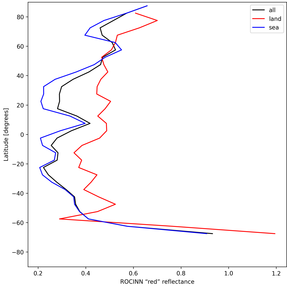
Figure 35: Zonal average of “ROCINN “red” reflectance” for 2025-07-17 to 2025-07-18.
