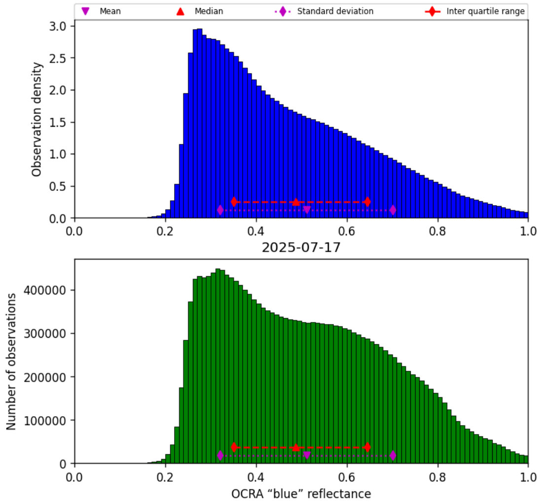
Figure 49: Histogram of “OCRA “blue” reflectance” for 2025-07-17 to 2025-07-18
