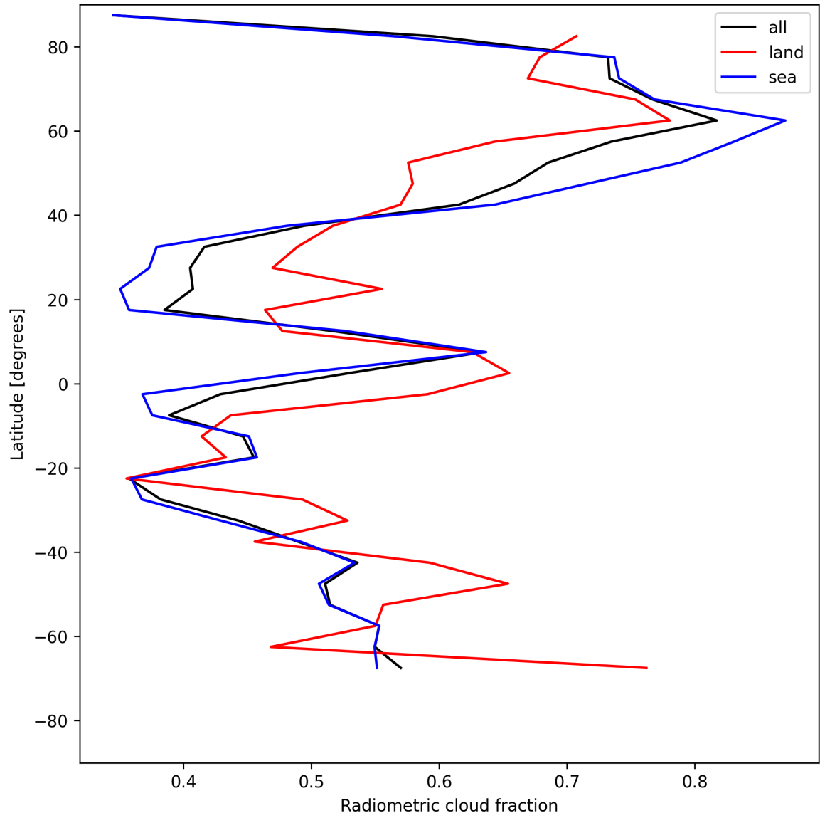
Figure 21: Zonal average of “Radiometric cloud fraction” for 2025-07-17 to 2025-07-18.
