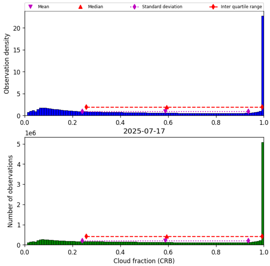
Figure 40: Histogram of “Cloud fraction (CRB)” for 2025-07-17 to 2025-07-18
