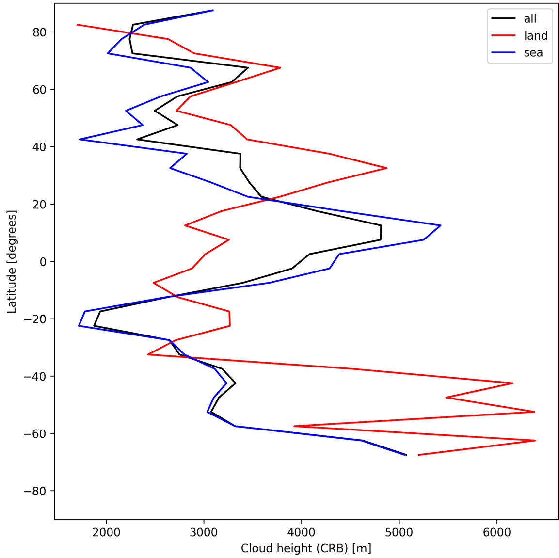
Figure 25: Zonal average of “Cloud height (CRB)” for 2025-07-17 to 2025-07-18.
