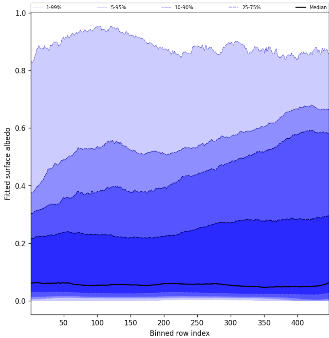
Figure 59: Along track statistics of “Fitted surface albedo” for 2025-07-17 to 2025-07-18
