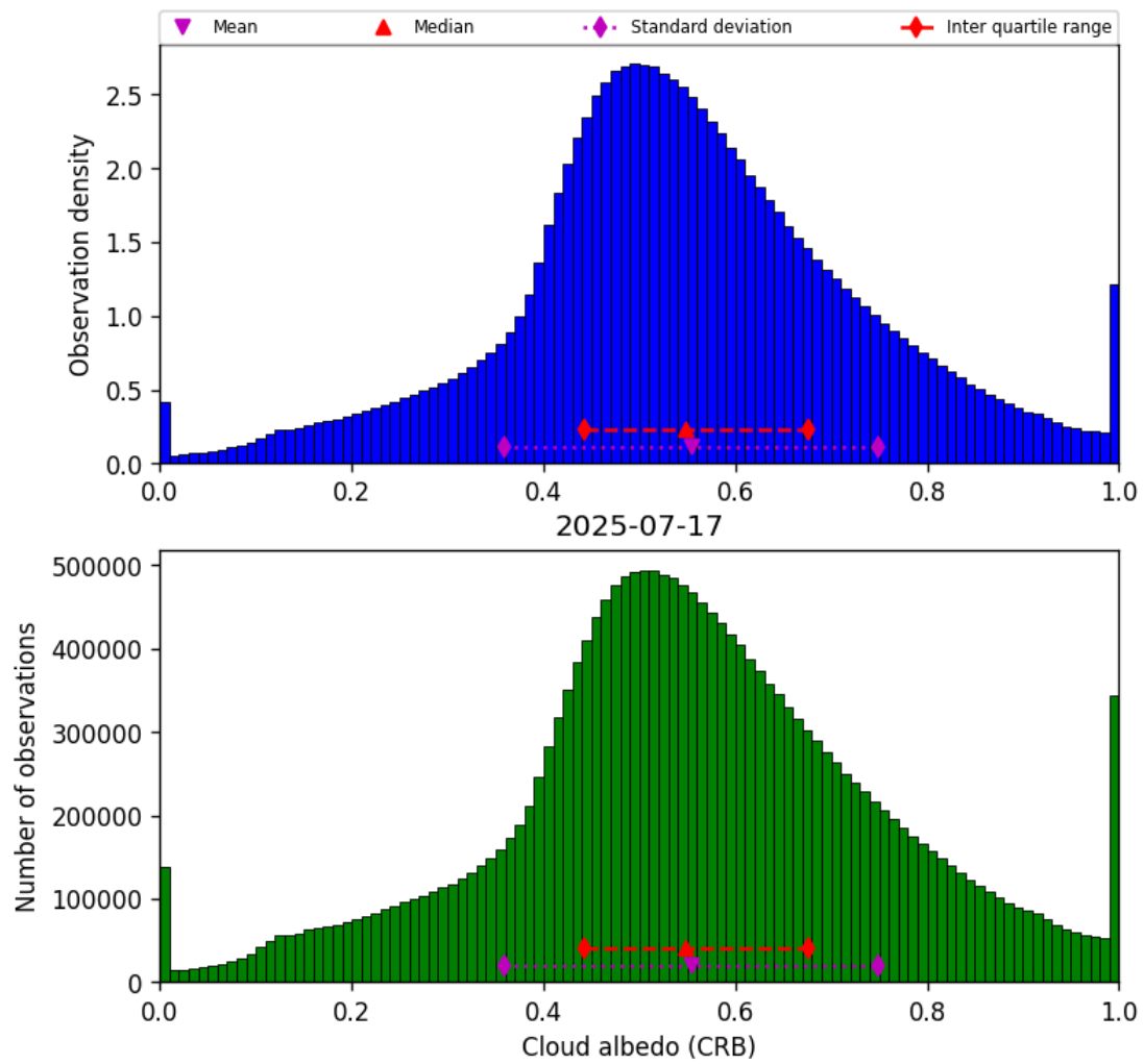
Figure 42: Histogram of “Cloud albedo (CRB)” for 2025-07-17 to 2025-07-18
