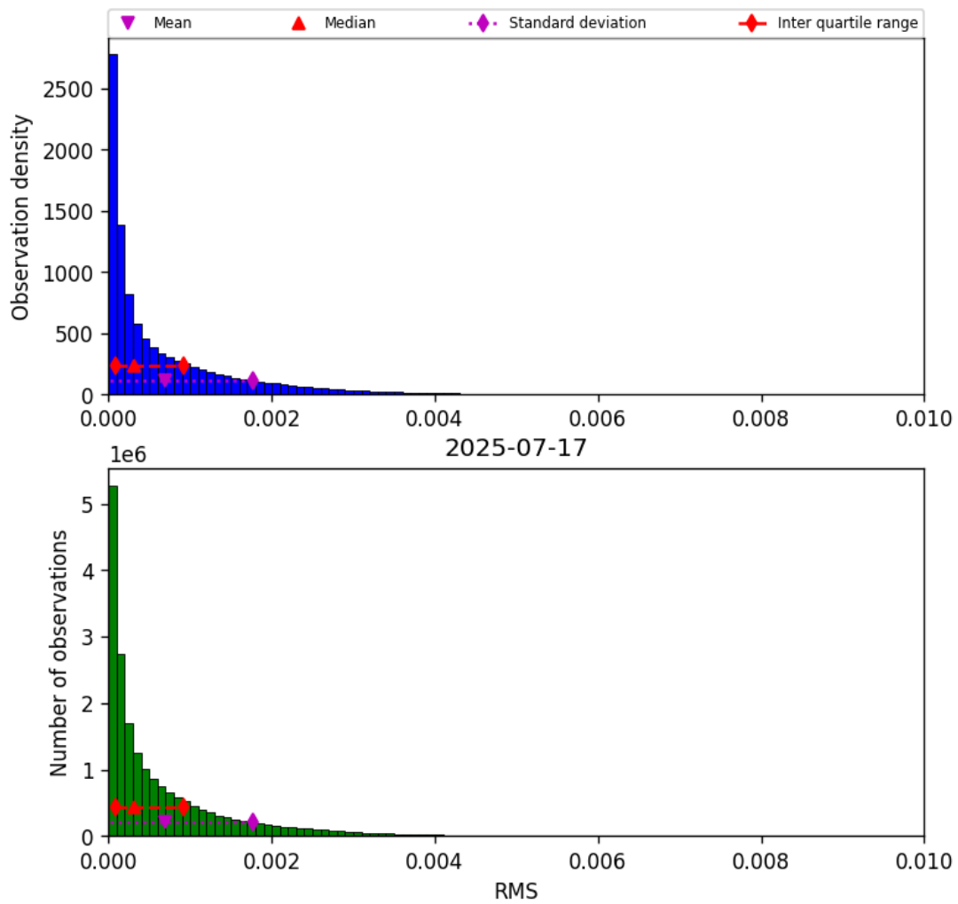
Figure 45: Histogram of “RMS” for 2025-07-17 to 2025-07-18
