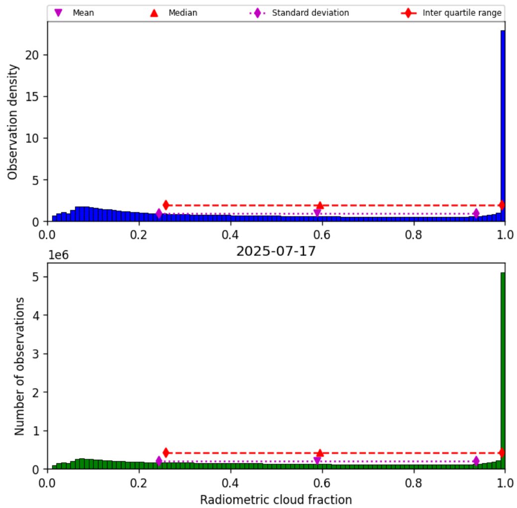
Figure 37: Histogram of “Radiometric cloud fraction” for 2025-07-17 to 2025-07-18
