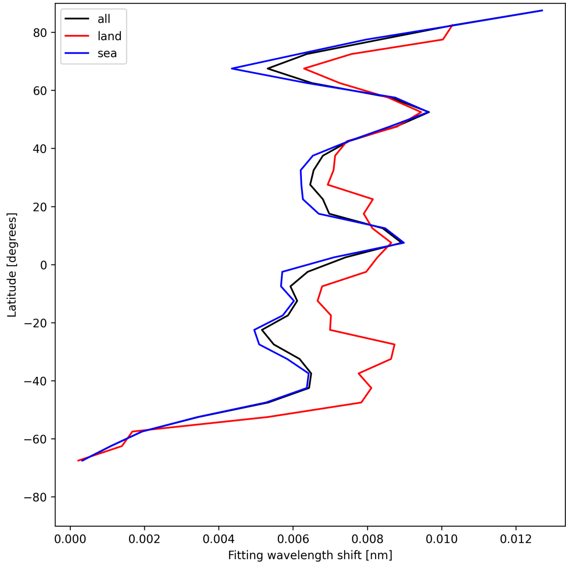
Figure 31: Zonal average of “Fitting wavelength shift” for 2025-07-17 to 2025-07-18.
