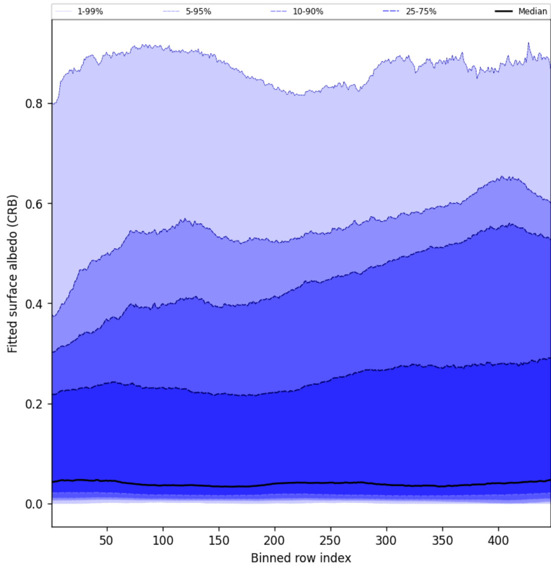
Figure 60: Along track statistics of “Fitted surface albedo (CRB)” for 2025-07-17 to 2025-07-18
