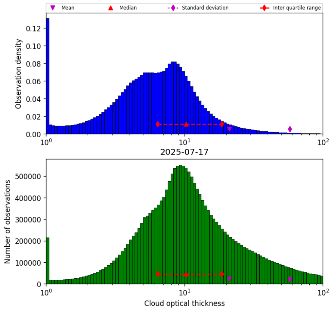
Figure 39: Histogram of “Cloud optical thickness” for 2025-07-17 to 2025-07-18
