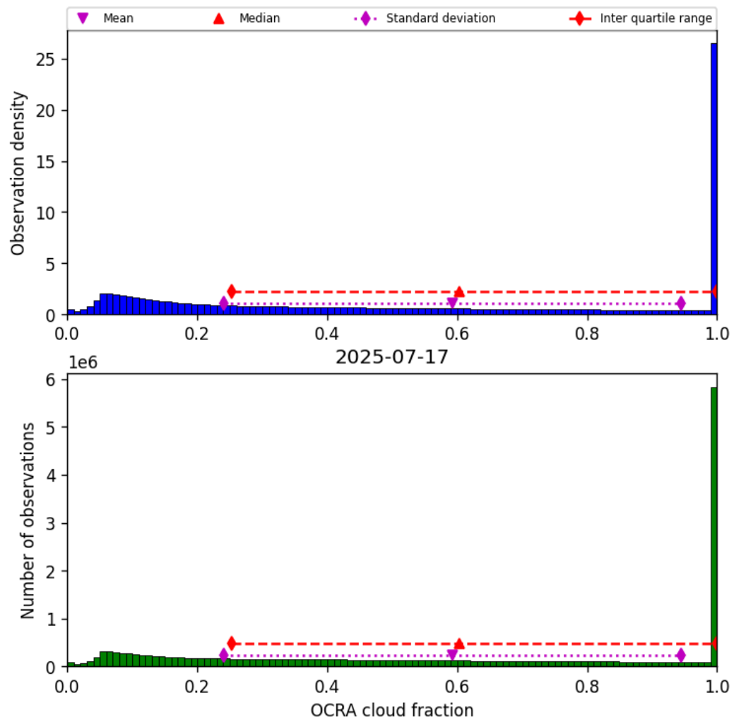
Figure 48: Histogram of “OCRA cloud fraction” for 2025-07-17 to 2025-07-18
