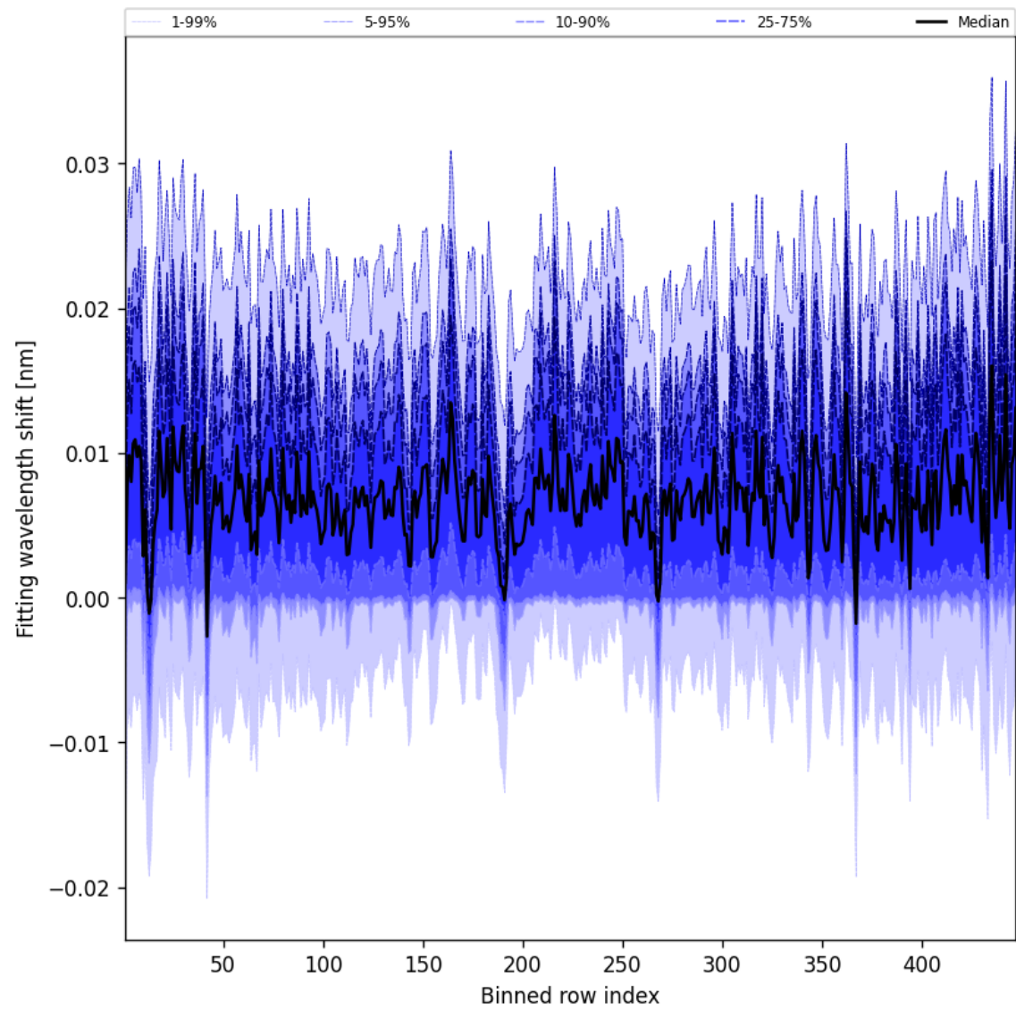
Figure 63: Along track statistics of “Fitting wavelength shift” for 2025-07-17 to 2025-07-18
