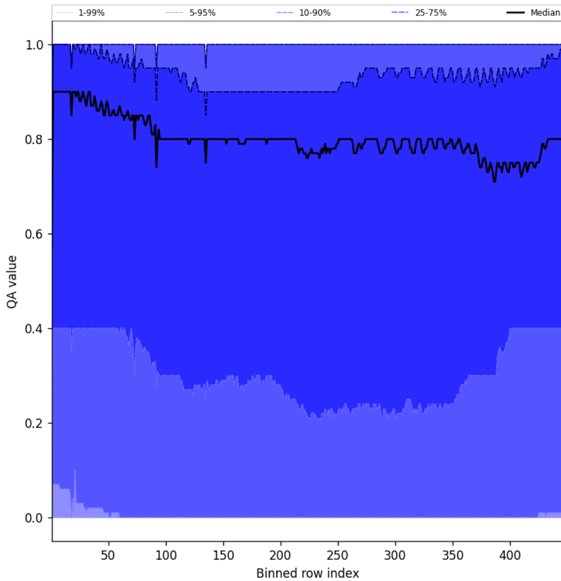
Figure 52: Along track statistics of “QA value” for 2025-07-17 to 2025-07-18
