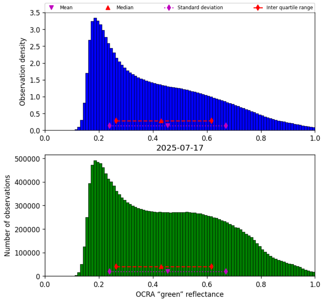
Figure 50: Histogram of “OCRA “green” reflectance” for 2025-07-17 to 2025-07-18
