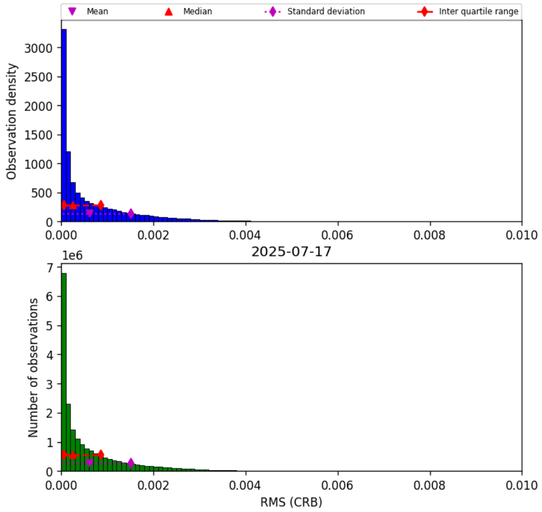
Figure 46: Histogram of “RMS (CRB)” for 2025-07-17 to 2025-07-18
