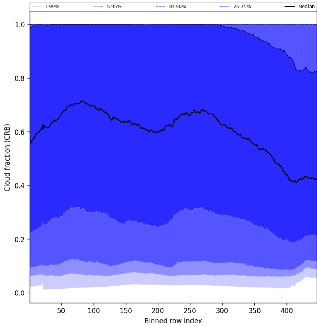
Figure 56: Along track statistics of “Cloud fraction (CRB)” for 2025-07-17 to 2025-07-18
