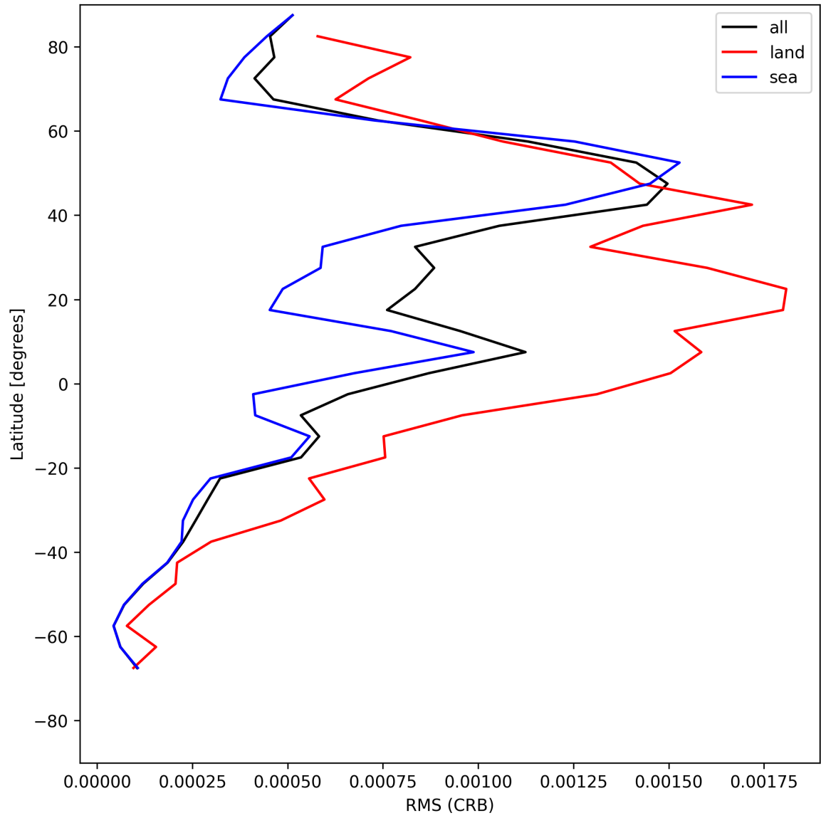
Figure 30: Zonal average of “RMS (CRB)” for 2025-07-17 to 2025-07-18.
