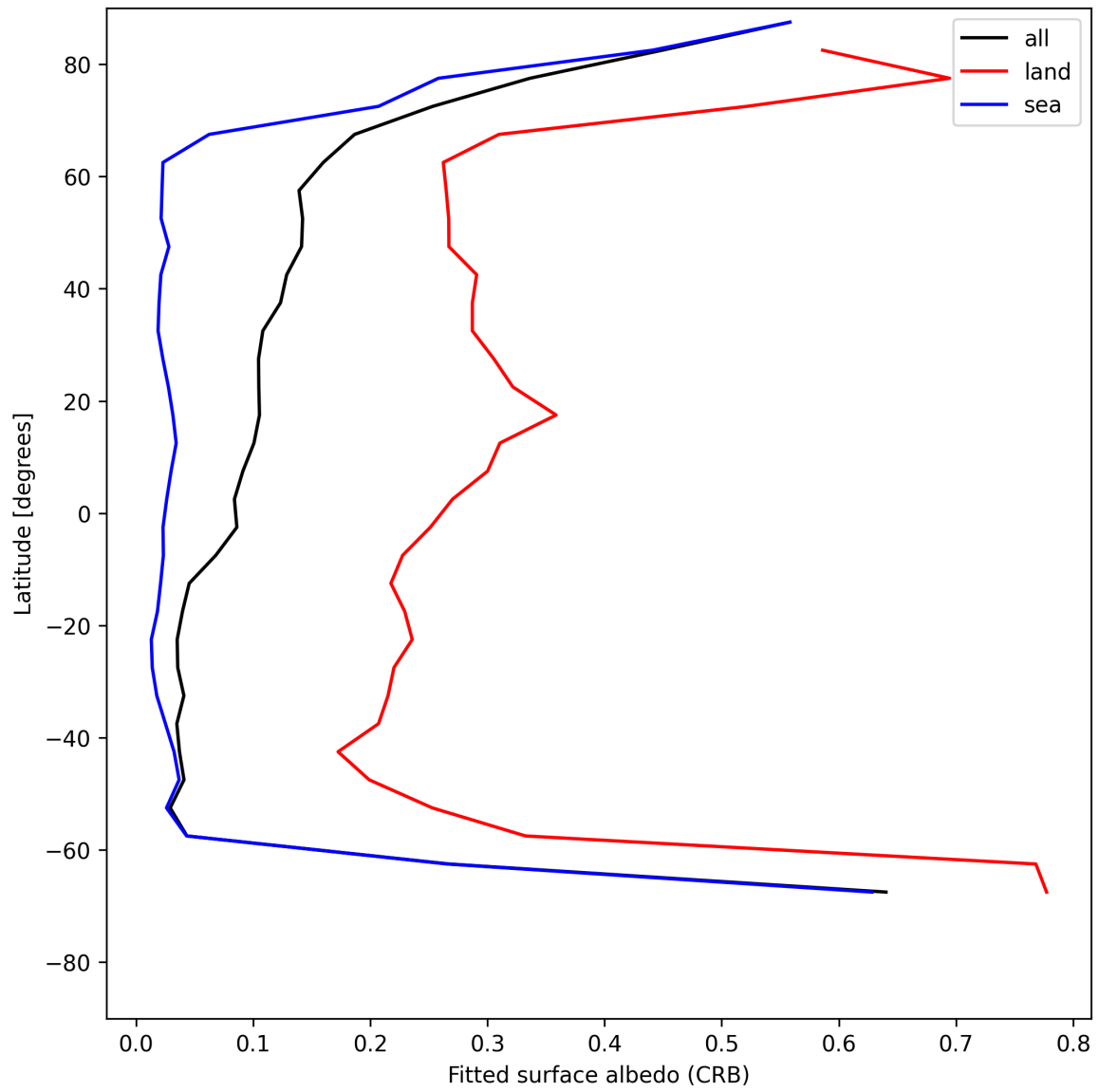
Figure 28: Zonal average of “Fitted surface albedo (CRB)” for 2025-07-17 to 2025-07-18.
