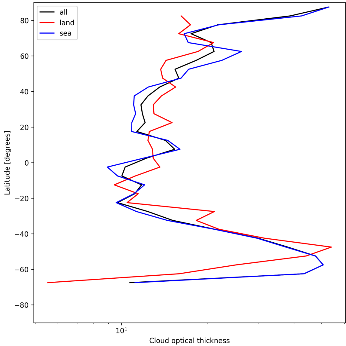
Figure 23: Zonal average of “Cloud optical thickness” for 2025-07-17 to 2025-07-18.
