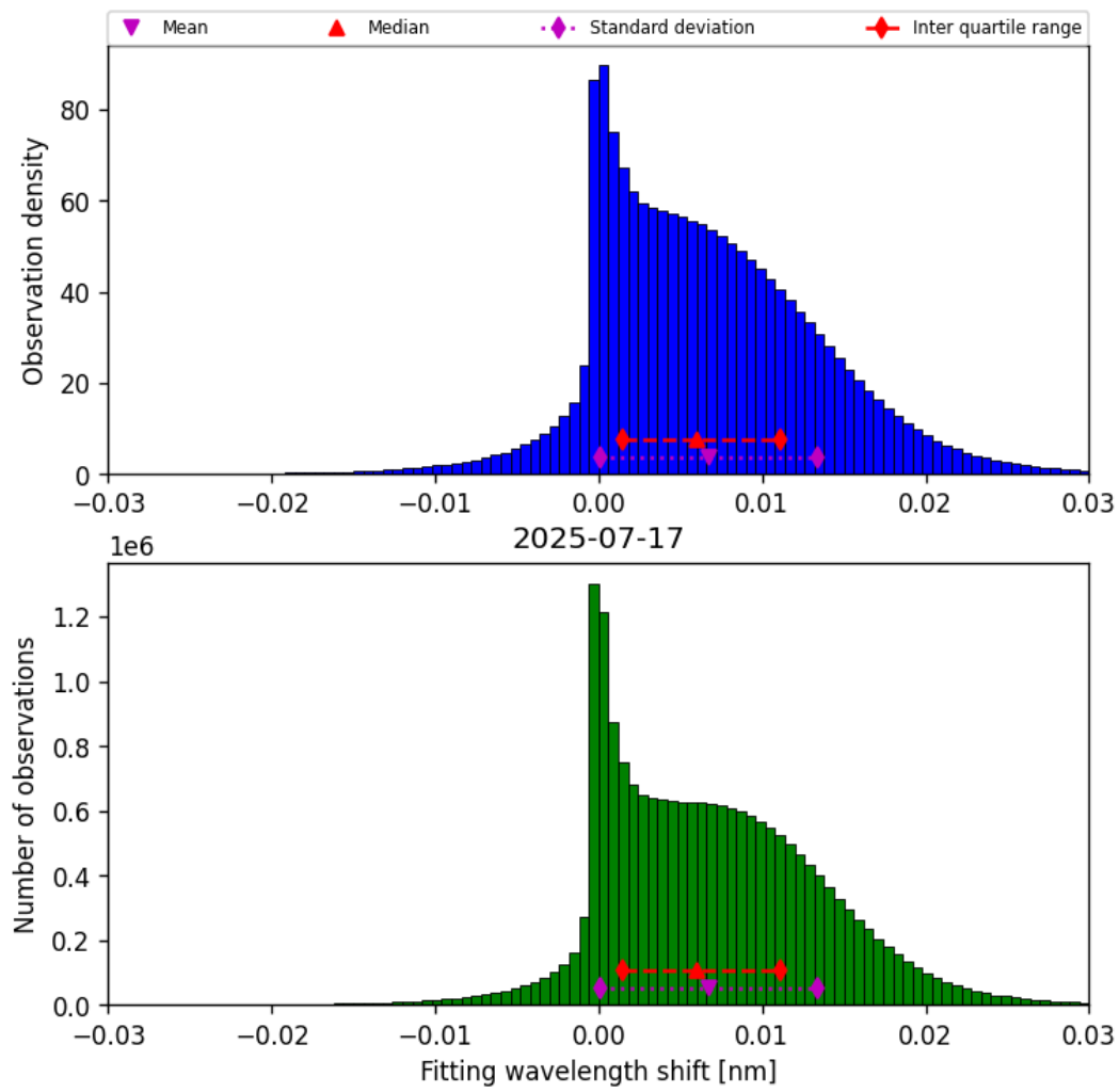
Figure 47: Histogram of “Fitting wavelength shift” for 2025-07-17 to 2025-07-18
