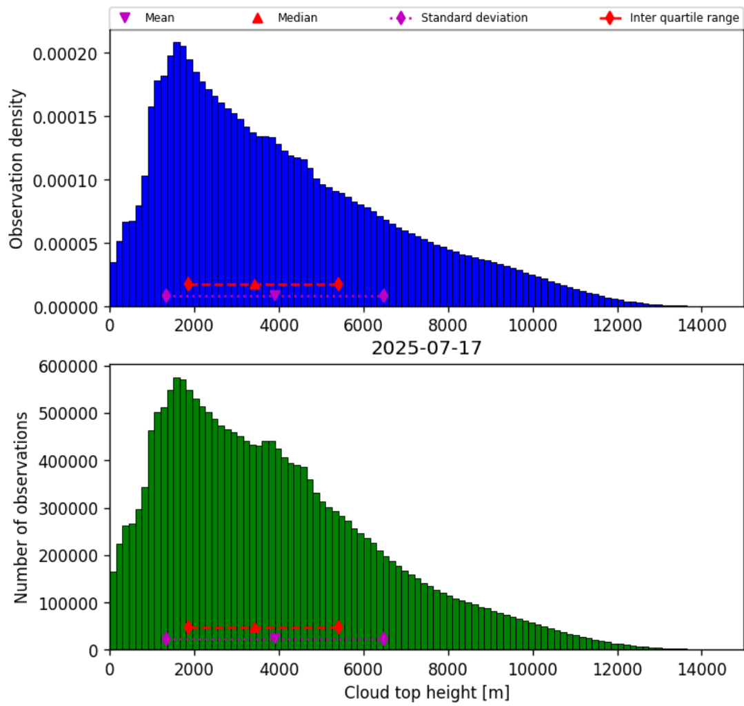
Figure 38: Histogram of “Cloud top height” for 2025-07-17 to 2025-07-18
