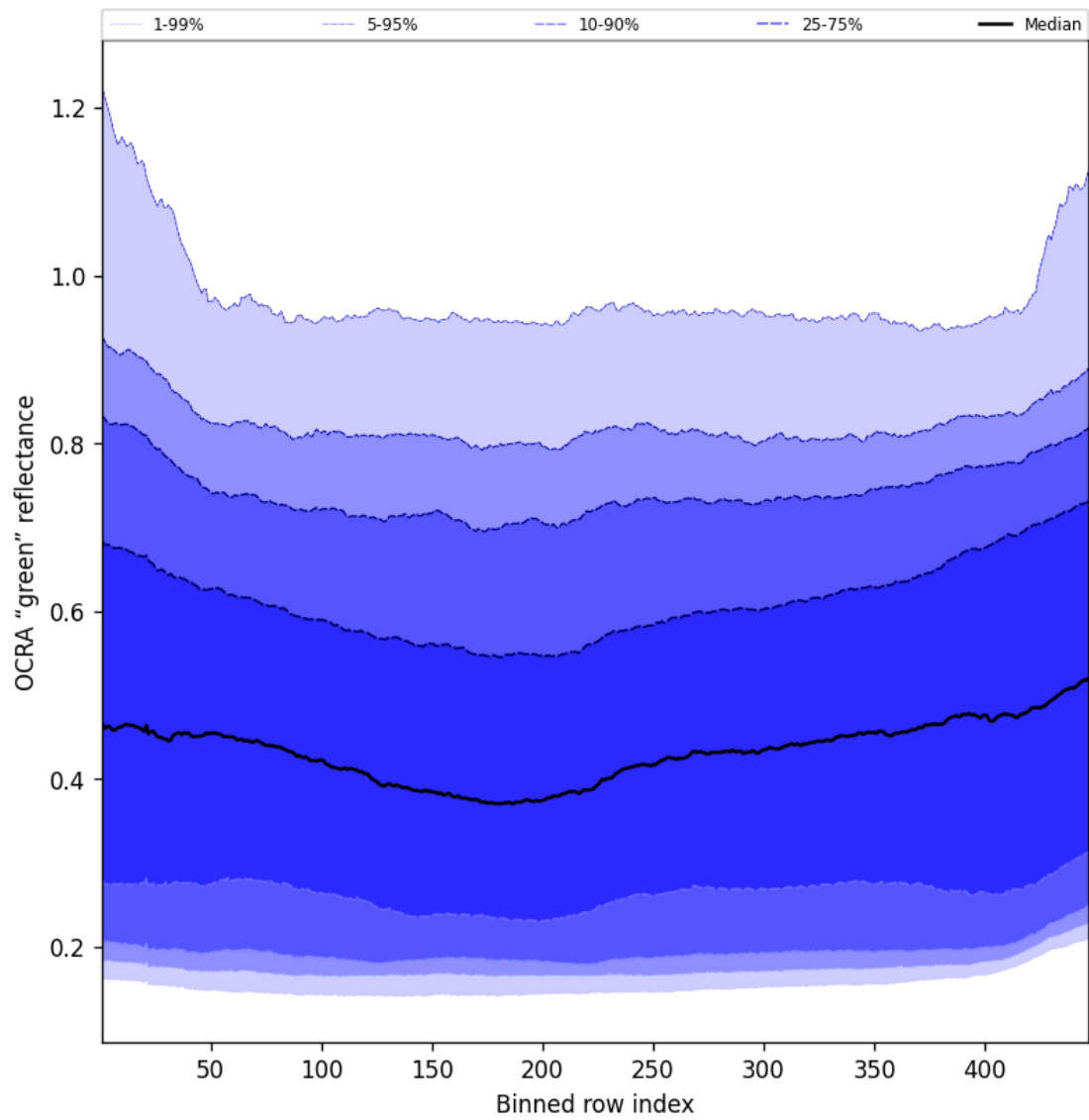
Figure 66: Along track statistics of “OCRA “green” reflectance” for 2025-07-17 to 2025-07-18
