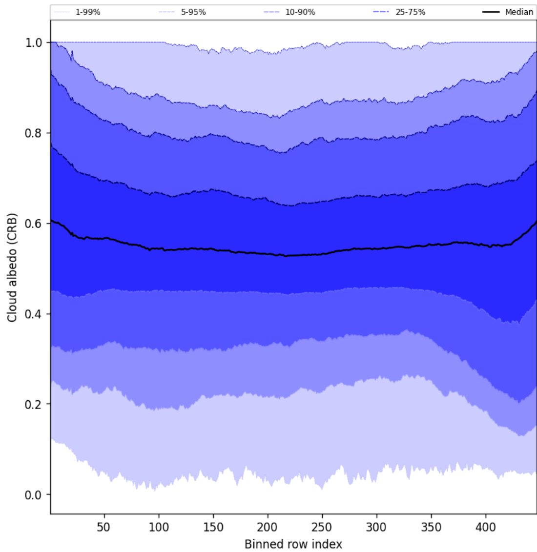
Figure 58: Along track statistics of “Cloud albedo (CRB)” for 2025-07-17 to 2025-07-18
