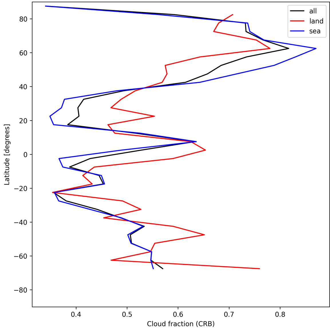
Figure 24: Zonal average of “Cloud fraction (CRB)” for 2025-07-17 to 2025-07-18.
