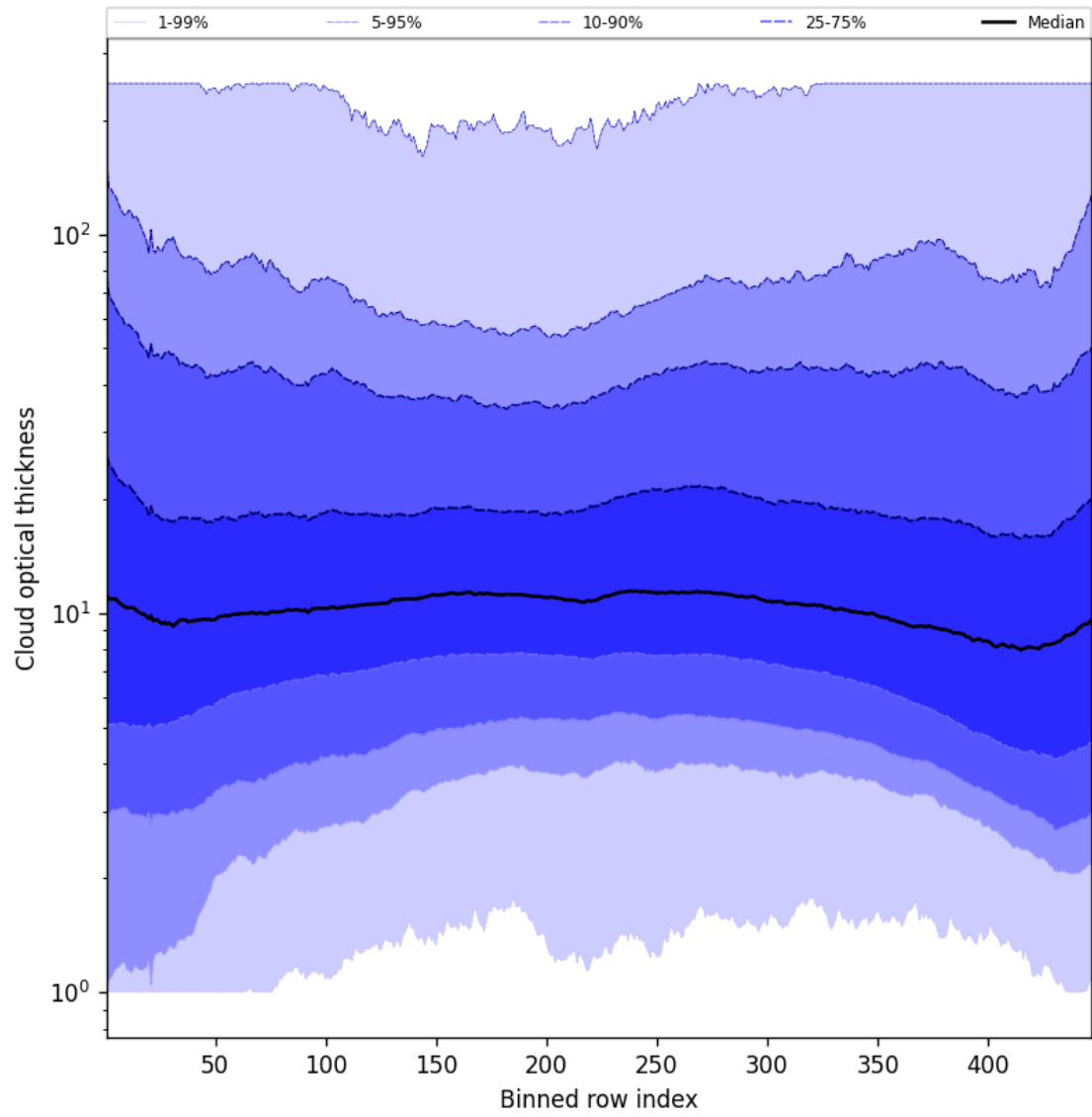
Figure 55: Along track statistics of “Cloud optical thickness” for 2025-07-17 to 2025-07-18
