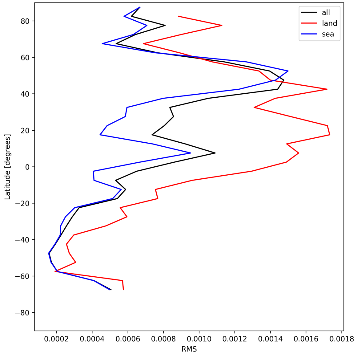
Figure 29: Zonal average of “RMS” for 2025-07-17 to 2025-07-18.
