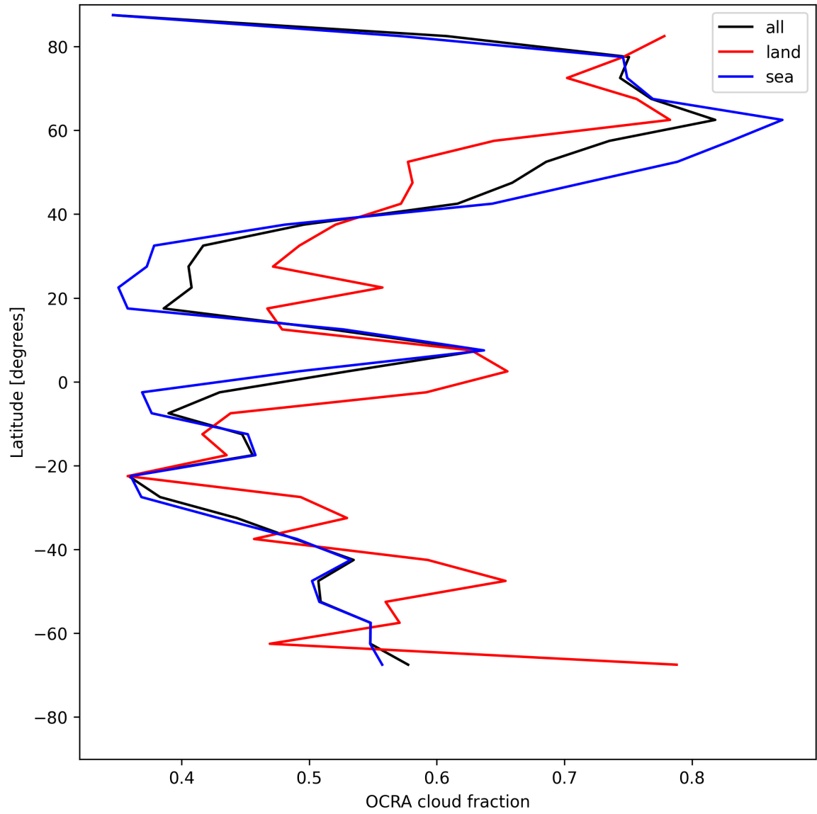
Figure 32: Zonal average of “OCRA cloud fraction” for 2025-07-17 to 2025-07-18.
