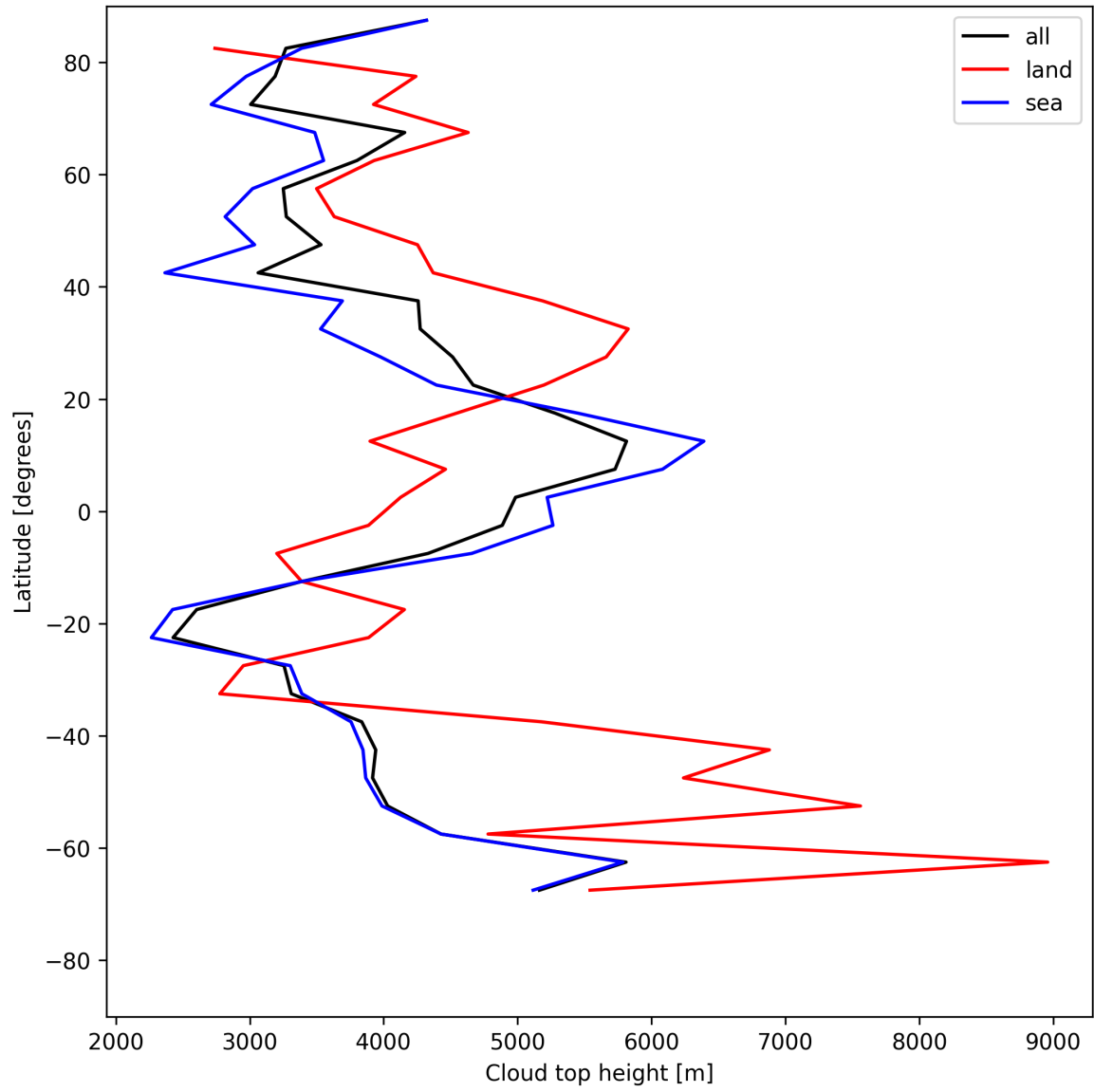
Figure 22: Zonal average of “Cloud top height” for 2025-07-17 to 2025-07-18.
