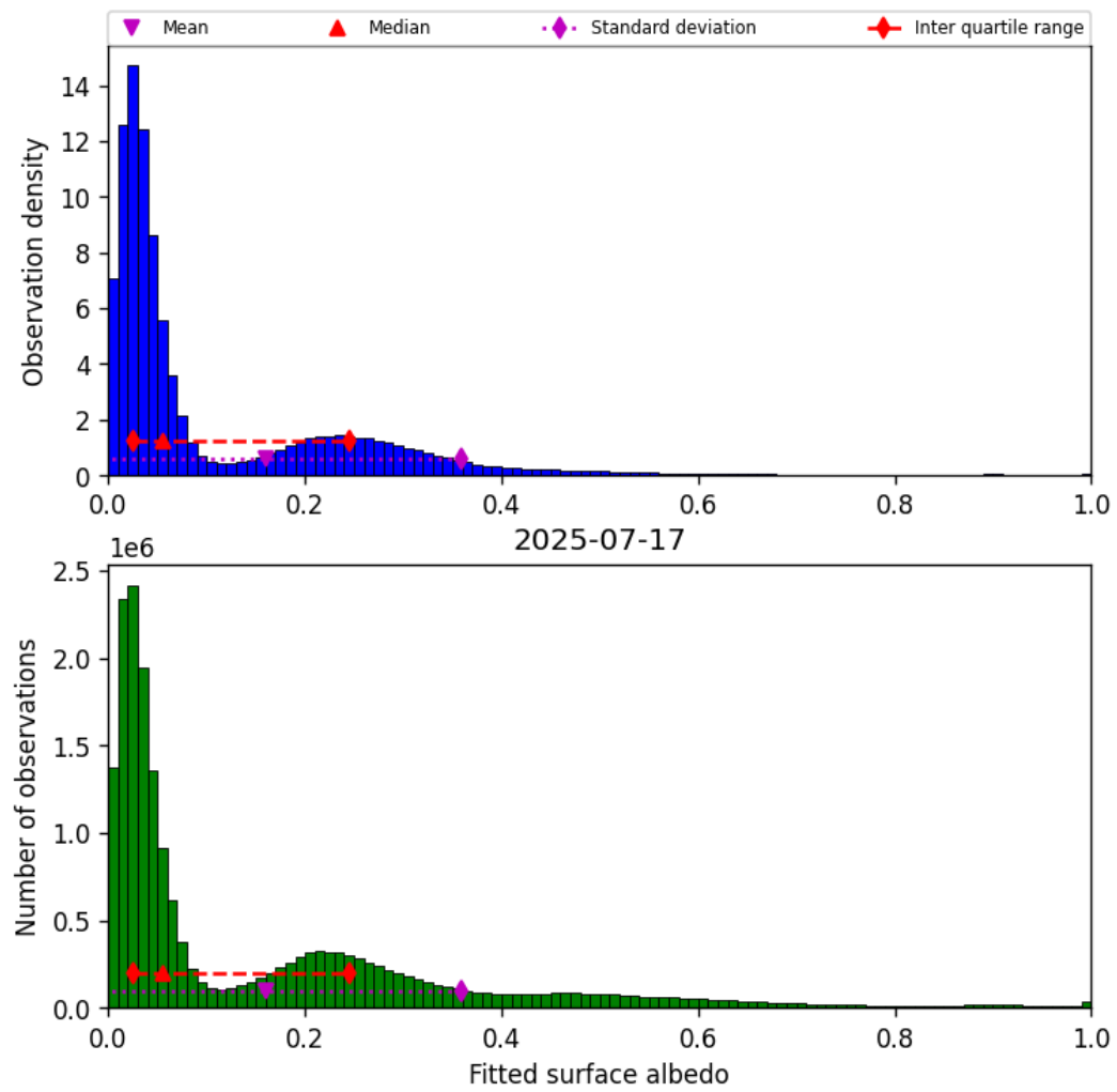
Figure 43: Histogram of “Fitted surface albedo” for 2025-07-17 to 2025-07-18
