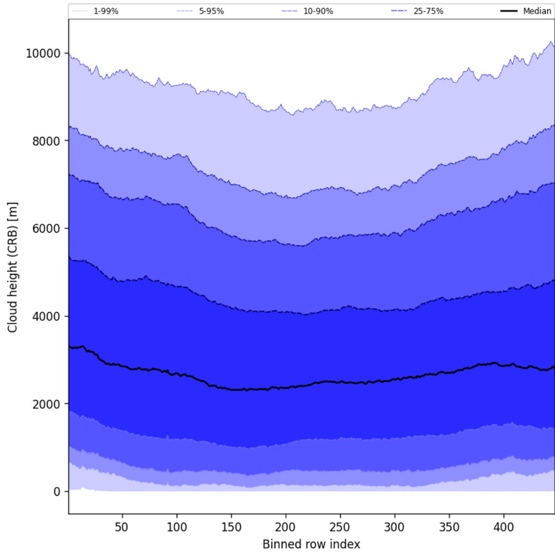
Figure 57: Along track statistics of “Cloud height (CRB)” for 2025-07-17 to 2025-07-18
