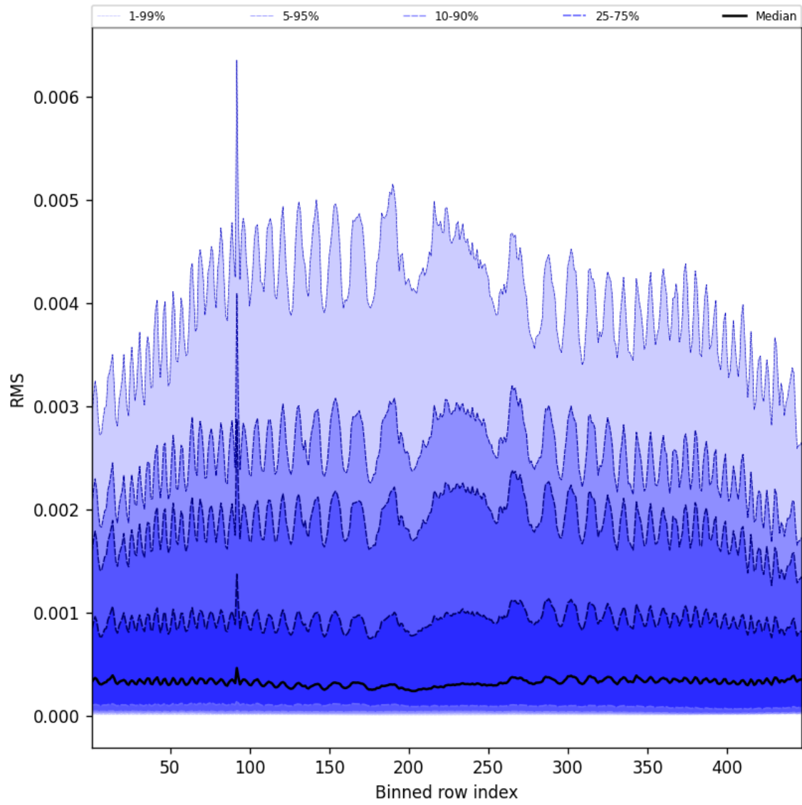
Figure 61: Along track statistics of “RMS” for 2025-07-17 to 2025-07-18
