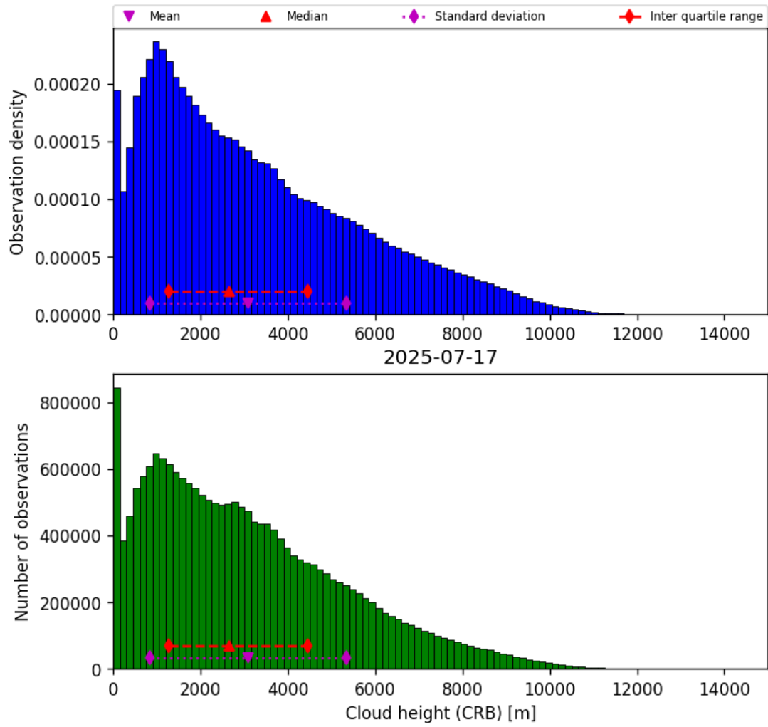
Figure 41: Histogram of “Cloud height (CRB)” for 2025-07-17 to 2025-07-18
