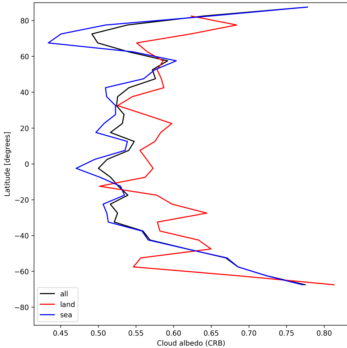
Figure 26: Zonal average of “Cloud albedo (CRB)” for 2025-07-17 to 2025-07-18.
