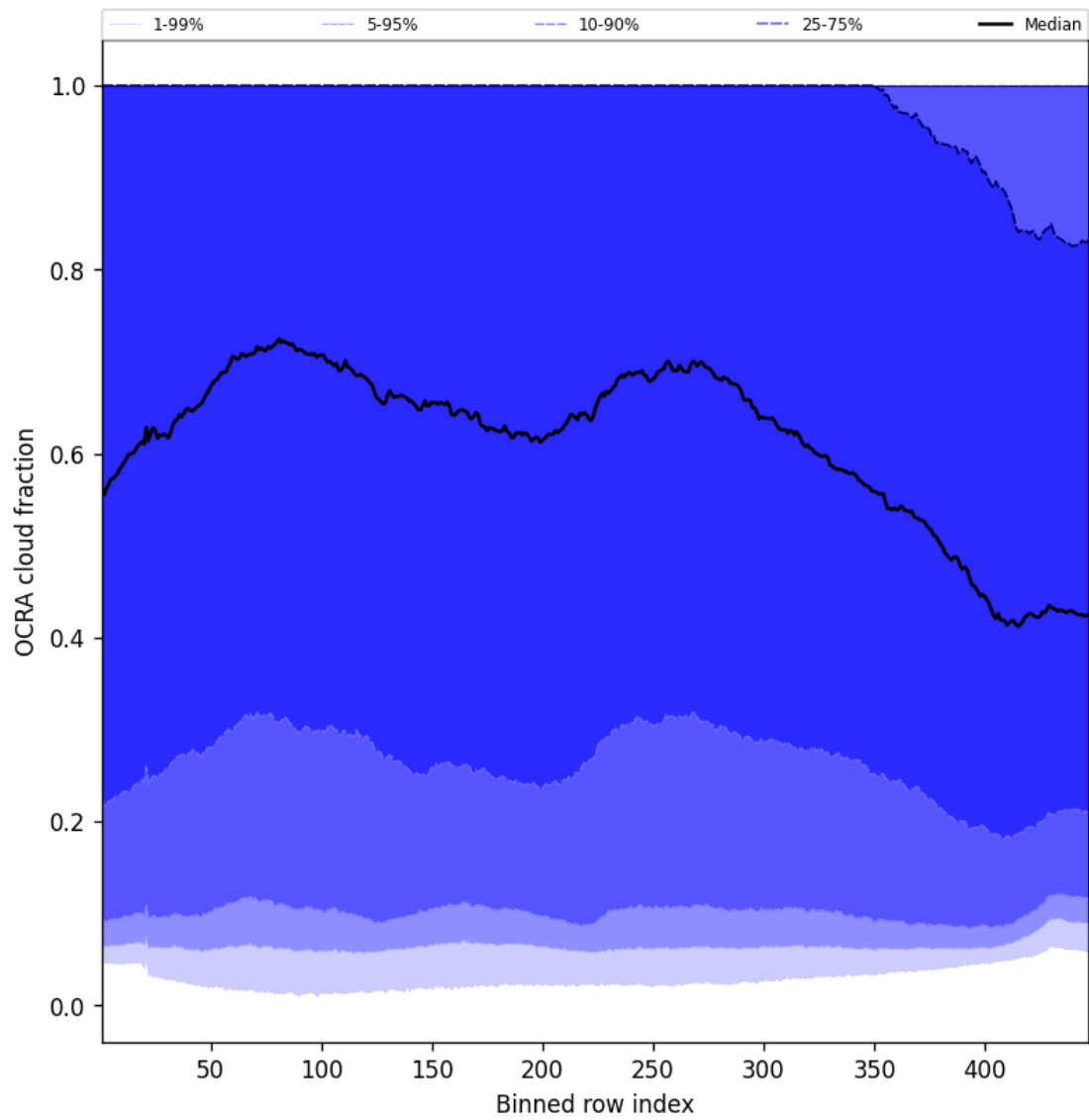
Figure 64: Along track statistics of “OCRA cloud fraction” for 2025-07-17 to 2025-07-18
