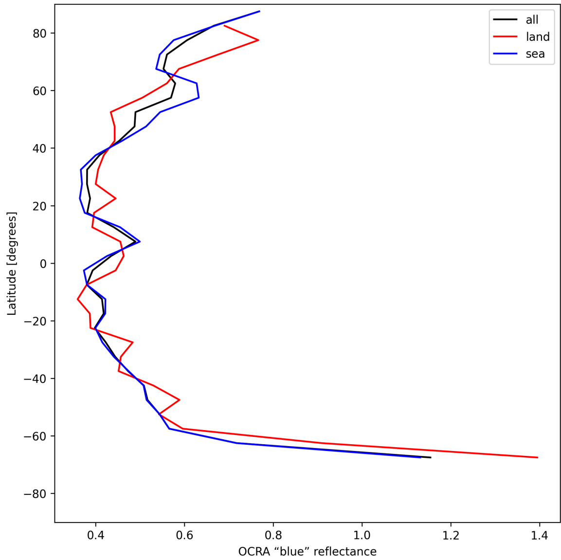
Figure 33: Zonal average of “OCRA “blue” reflectance” for 2025-07-17 to 2025-07-18.
