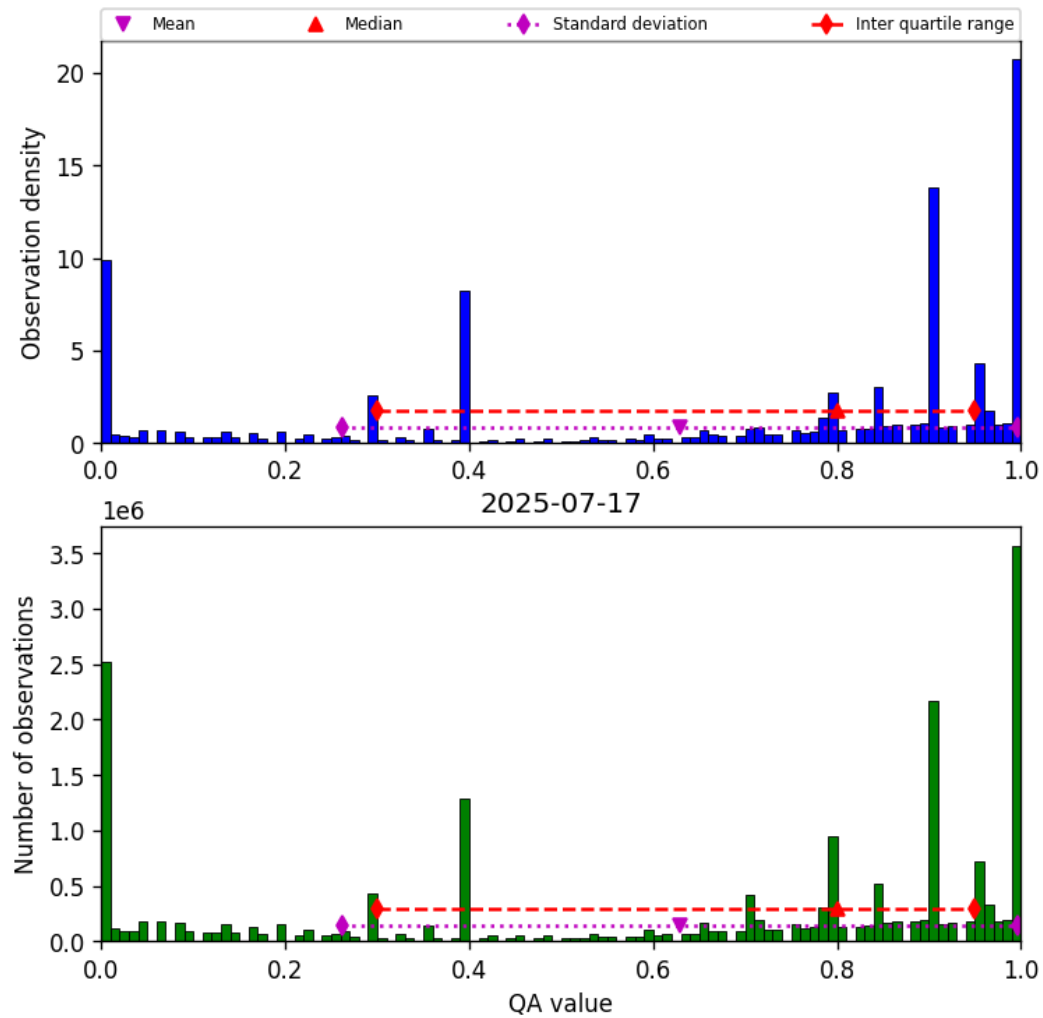
Figure 36: Histogram of “QA value” for 2025-07-17 to 2025-07-18
