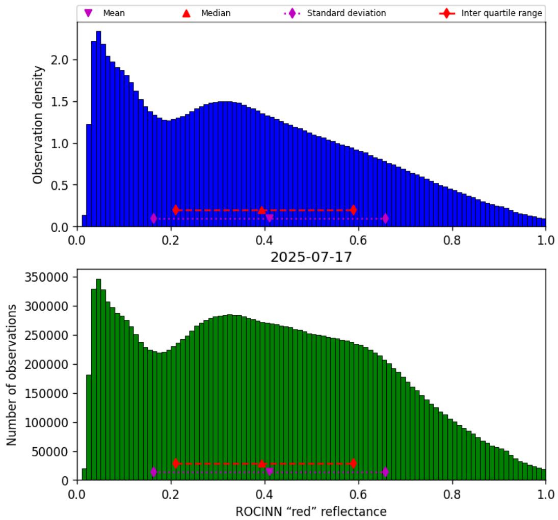
Figure 51: Histogram of “ROCINN “red” reflectance” for 2025-07-17 to 2025-07-18
