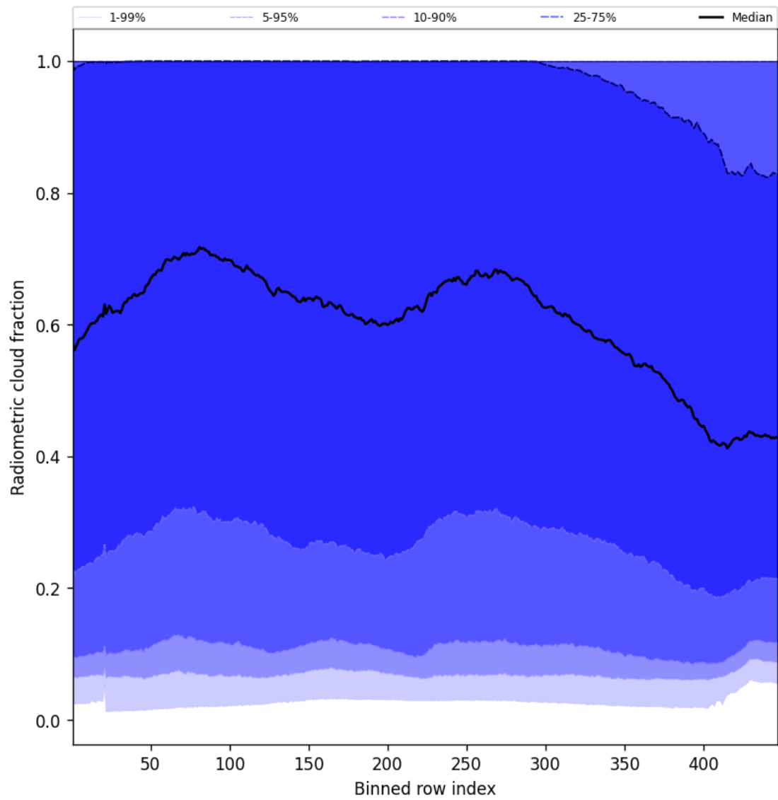
Figure 53: Along track statistics of “Radiometric cloud fraction” for 2025-07-17 to 2025-07-18
