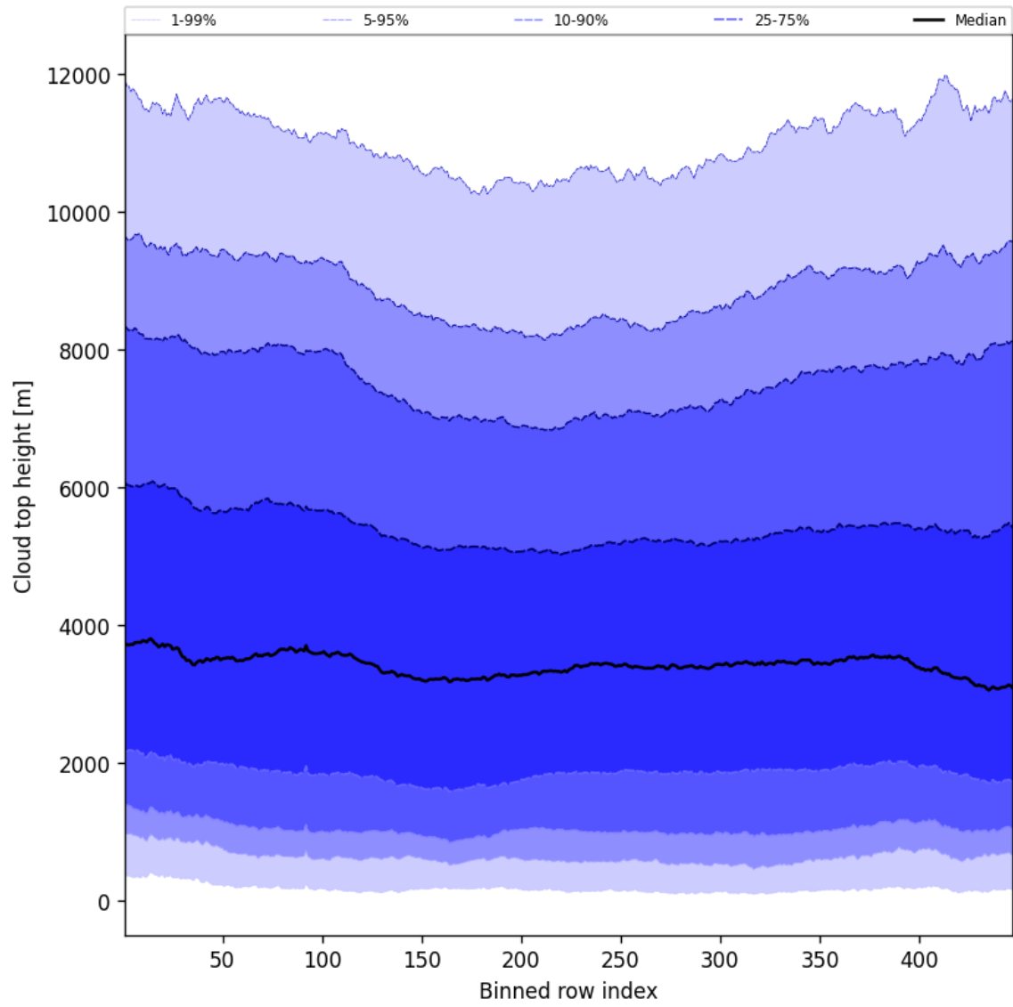
Figure 54: Along track statistics of “Cloud top height” for 2025-07-17 to 2025-07-18
