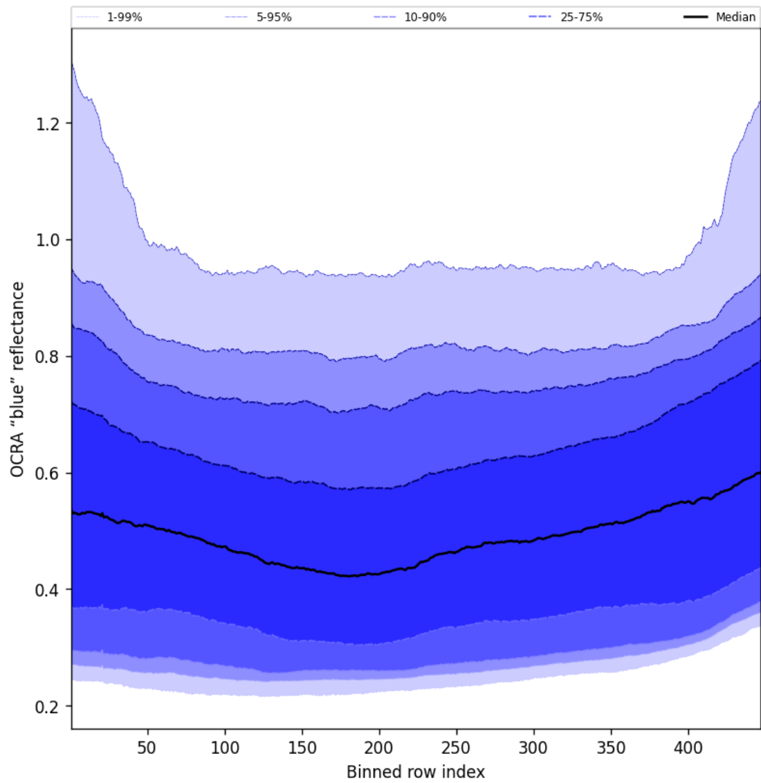
Figure 65: Along track statistics of “OCRA “blue” reflectance” for 2025-07-17 to 2025-07-18
