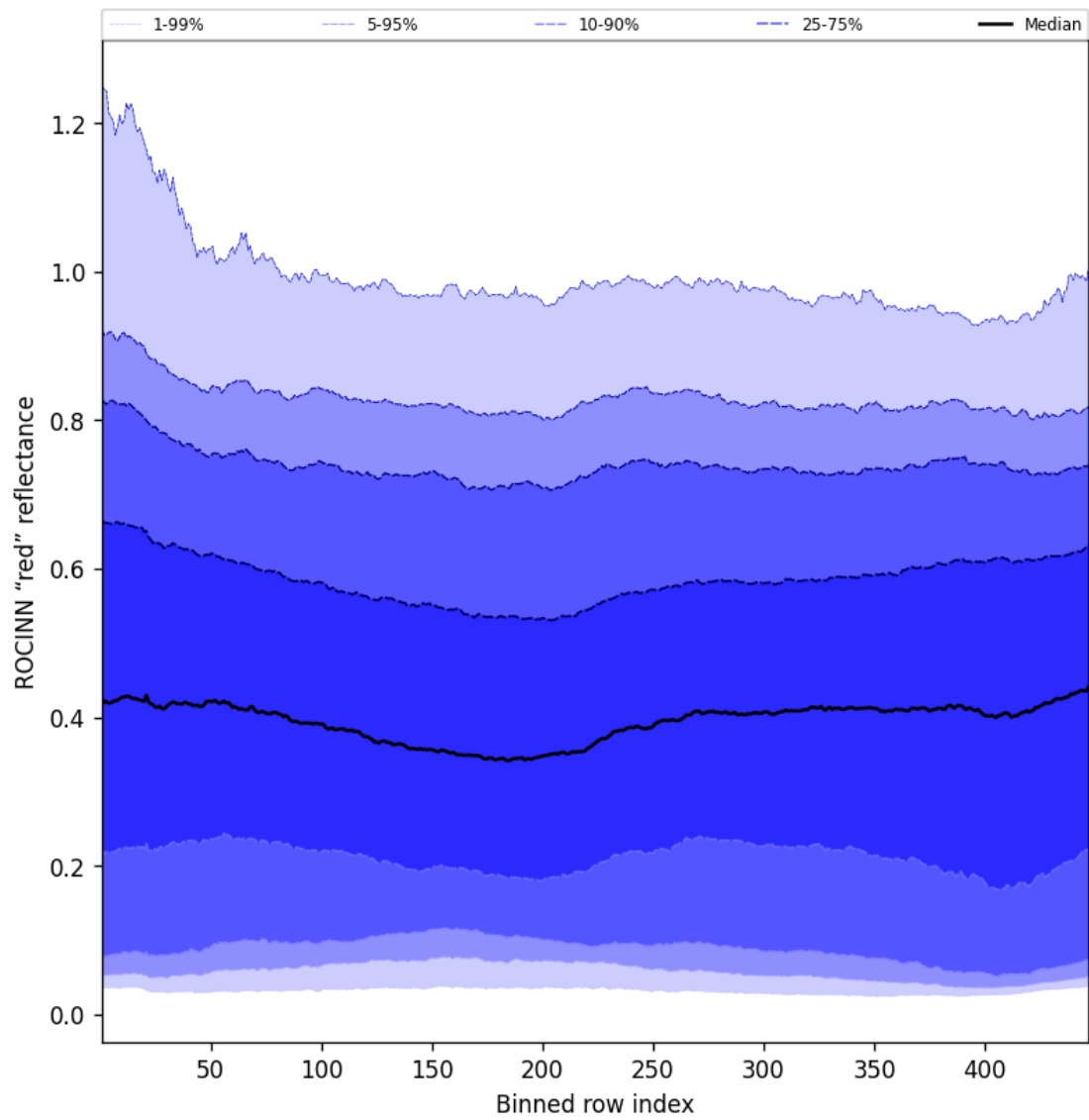
Figure 67: Along track statistics of “ROCINN “red” reflectance” for 2025-07-17 to 2025-07-18
