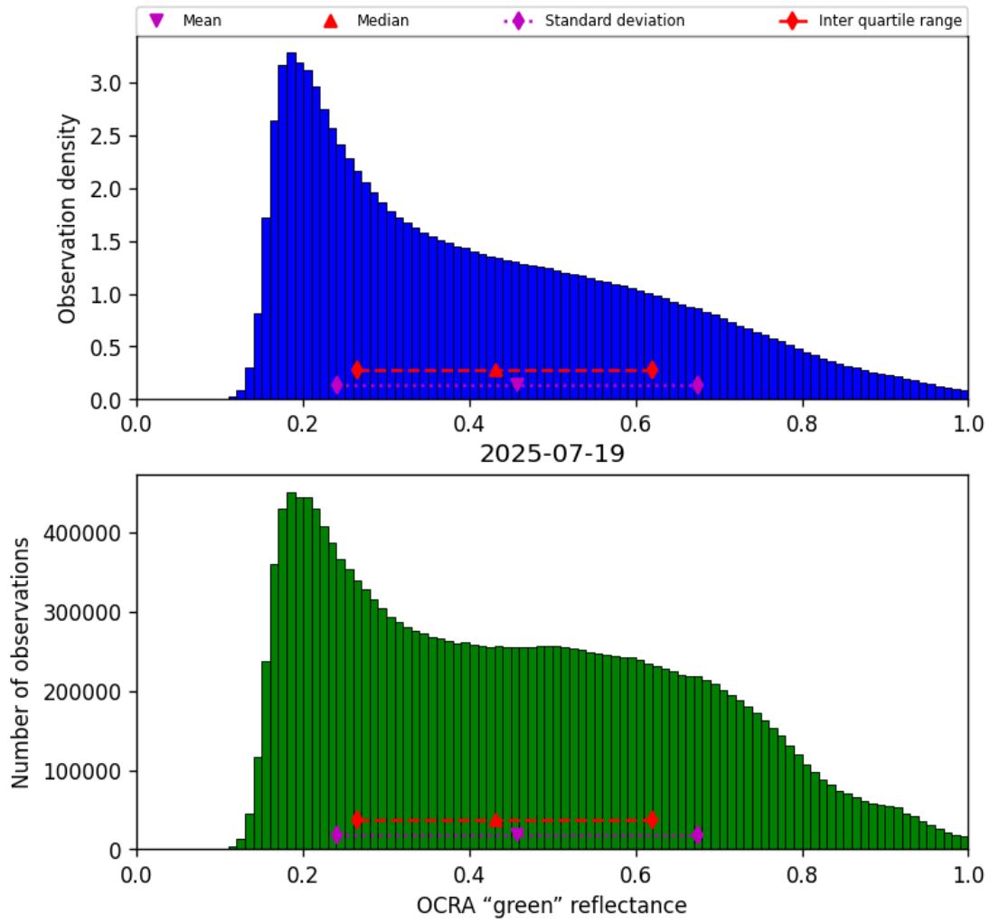
Figure 50: Histogram of “OCRA “green” reflectance” for 2025-07-19 to 2025-07-20
