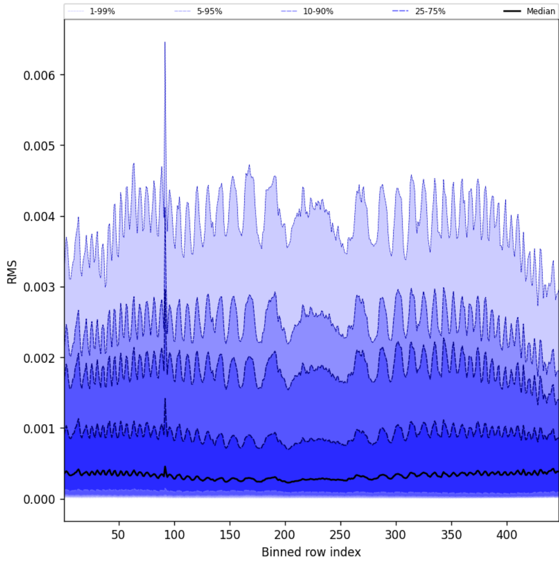
Figure 61: Along track statistics of “RMS” for 2025-07-19 to 2025-07-20
