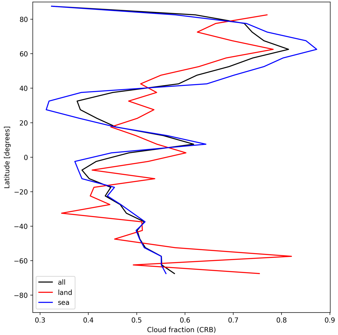
Figure 24: Zonal average of “Cloud fraction (CRB)” for 2025-07-19 to 2025-07-20.
