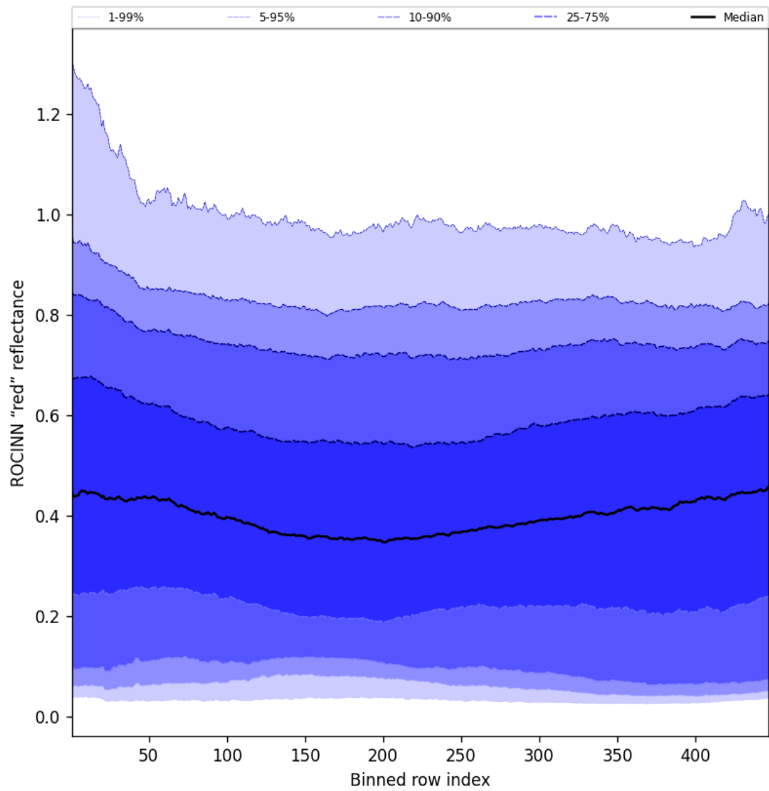
Figure 67: Along track statistics of "ROCINN "red" reflectance" for 2025-07-19 to 2025-07-20
