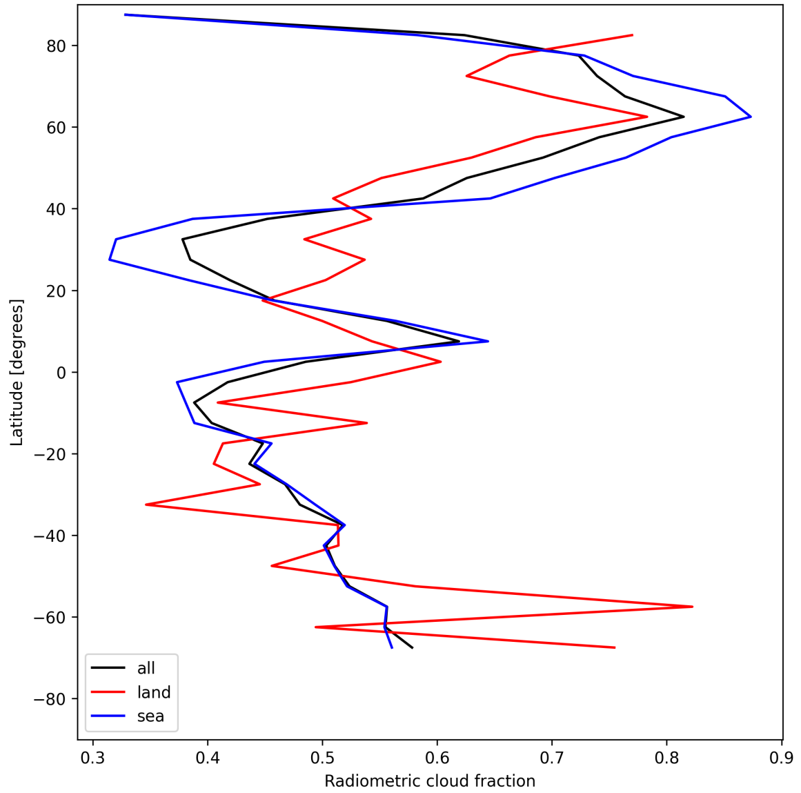
Figure 21: Zonal average of “Radiometric cloud fraction” for 2025-07-19 to 2025-07-20.
