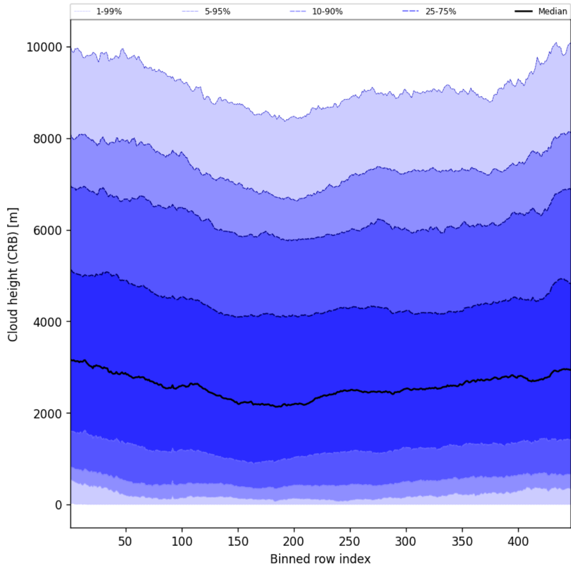
Figure 57: Along track statistics of “Cloud height (CRB)” for 2025-07-19 to 2025-07-20
