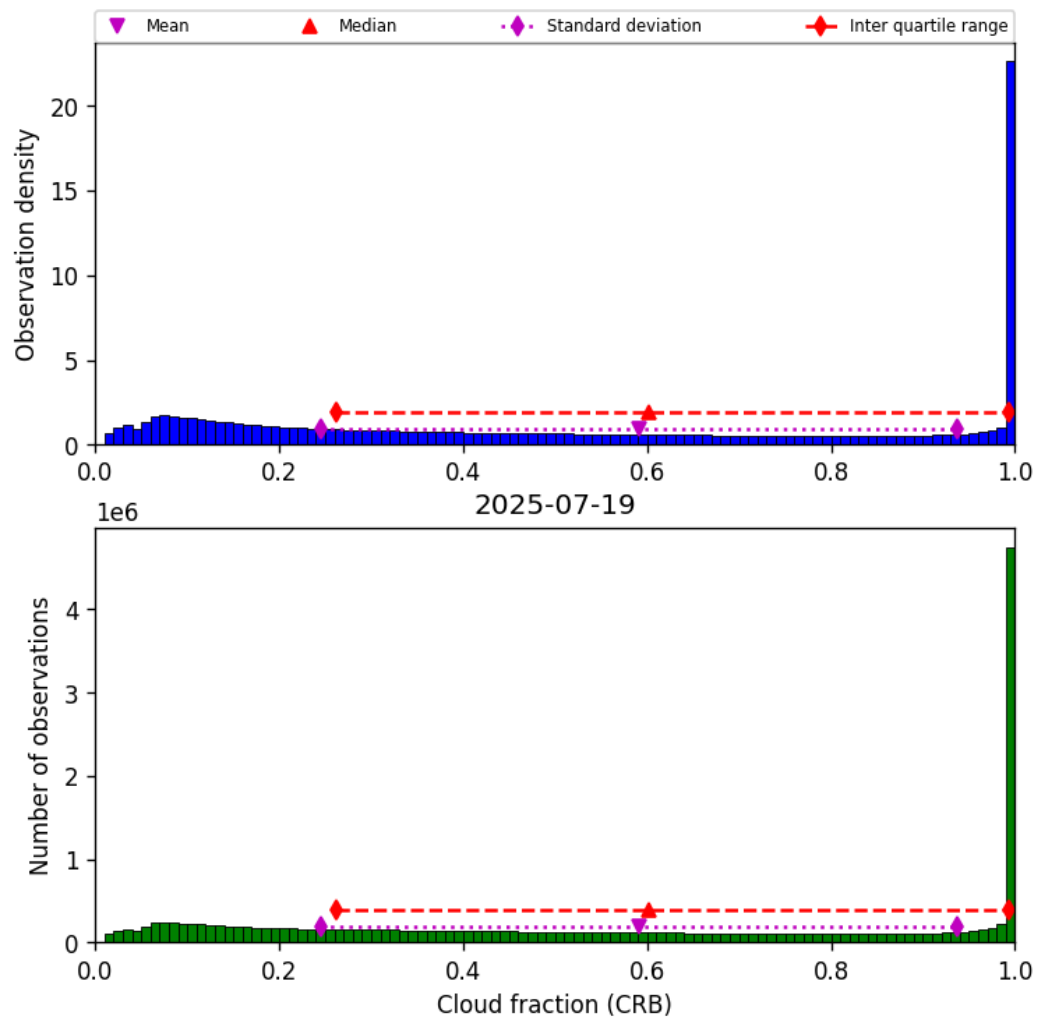
Figure 40: Histogram of “Cloud fraction (CRB)” for 2025-07-19 to 2025-07-20
