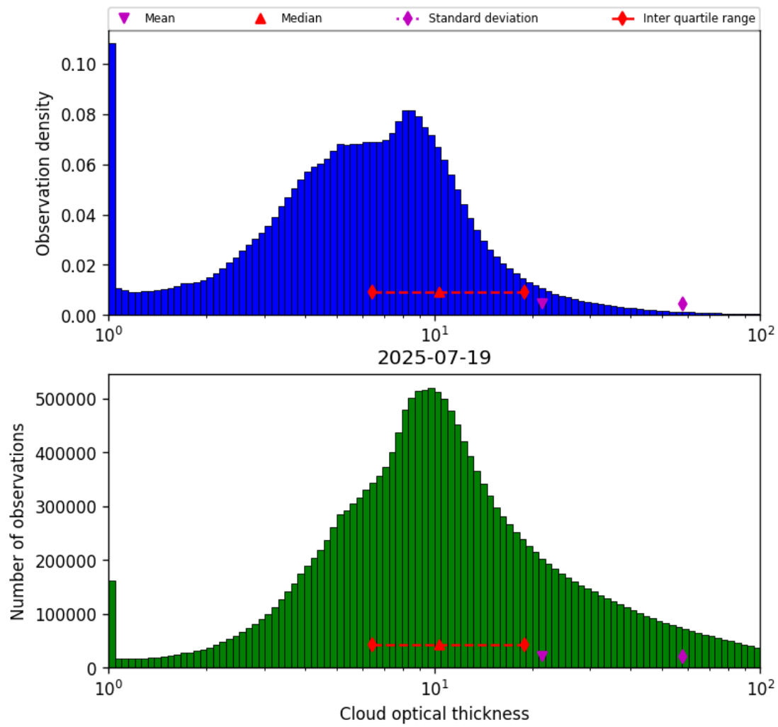
Figure 39: Histogram of “Cloud optical thickness” for 2025-07-19 to 2025-07-20
