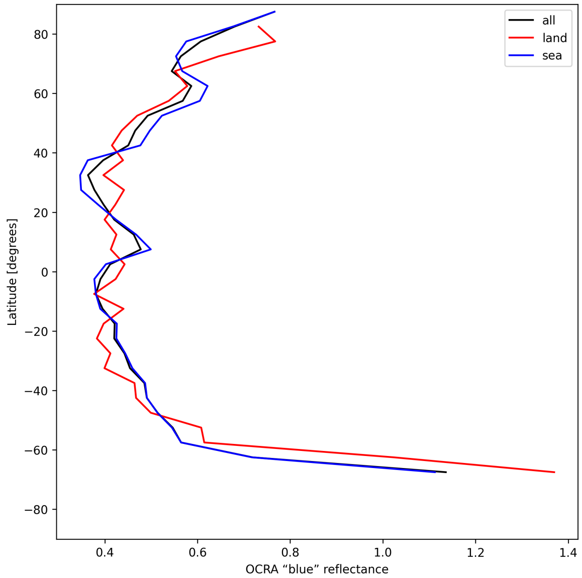
Figure 33: Zonal average of “OCRA “blue” reflectance” for 2025-07-19 to 2025-07-20.
