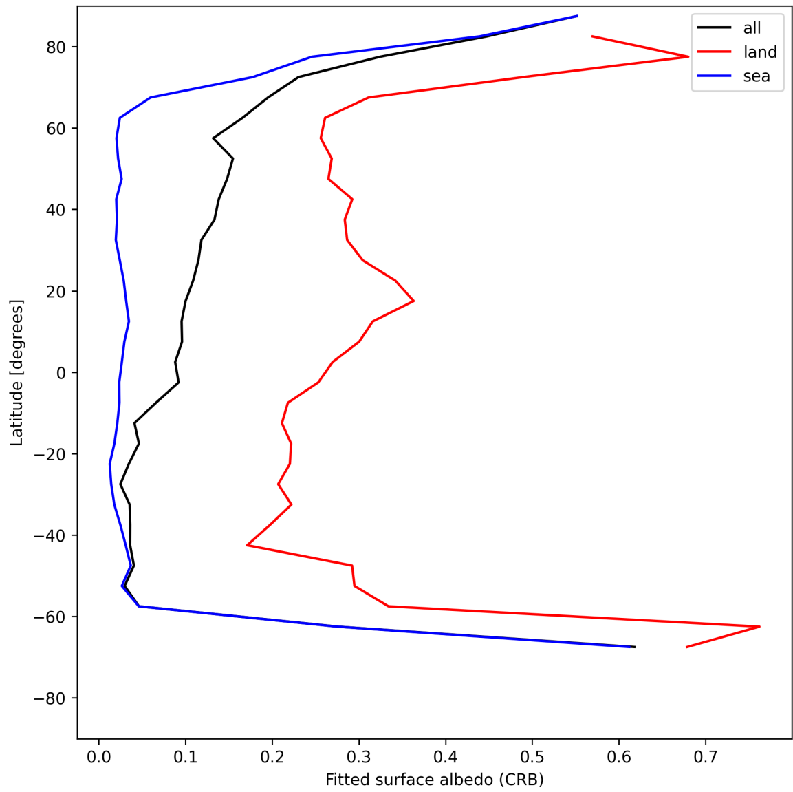
Figure 28: Zonal average of “Fitted surface albedo (CRB)” for 2025-07-19 to 2025-07-20.
