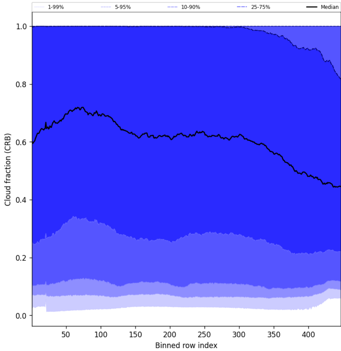
Figure 56: Along track statistics of “Cloud fraction (CRB)” for 2025-07-19 to 2025-07-20
