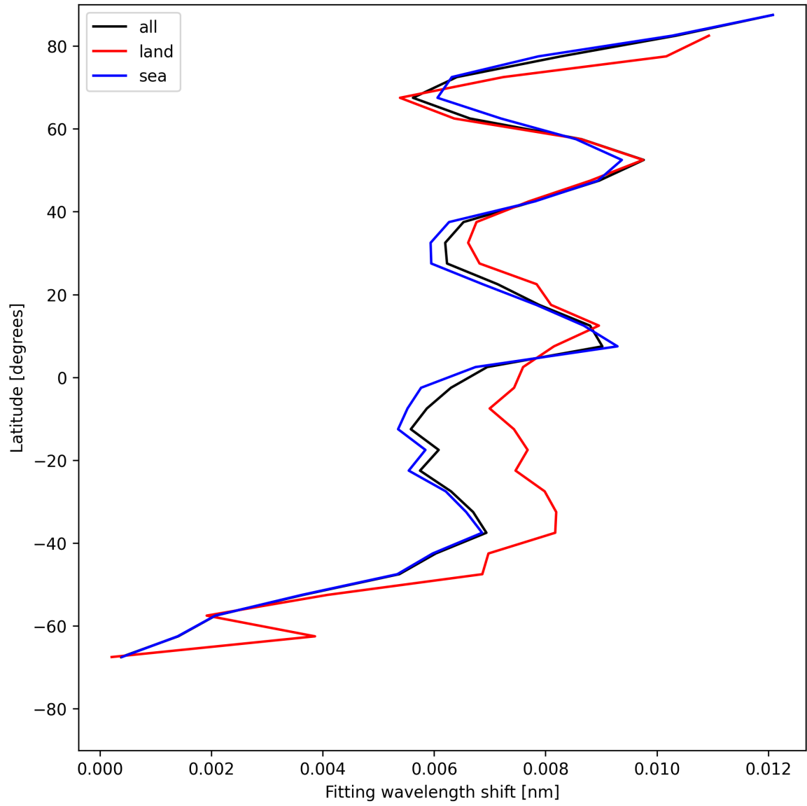
Figure 31: Zonal average of “Fitting wavelength shift” for 2025-07-19 to 2025-07-20.
