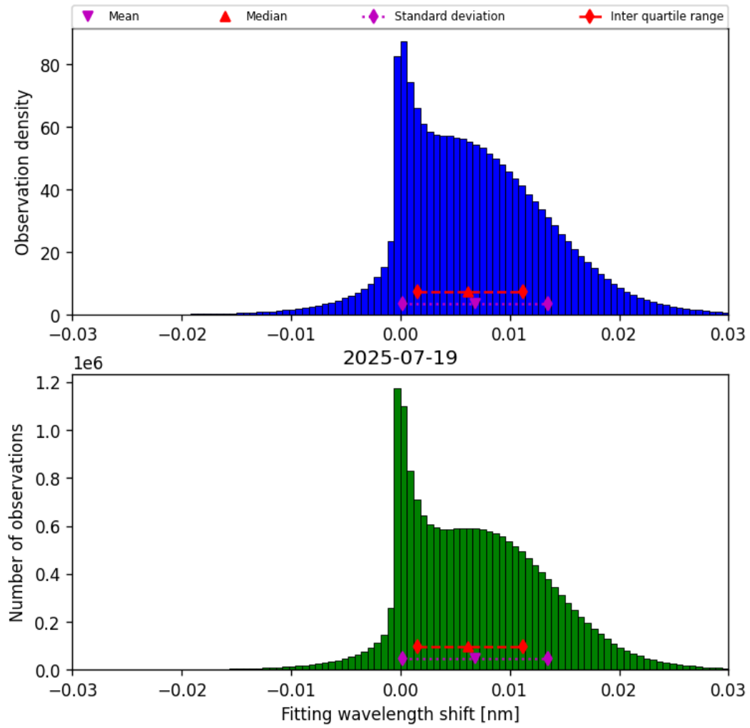
Figure 47: Histogram of “Fitting wavelength shift” for 2025-07-19 to 2025-07-20
