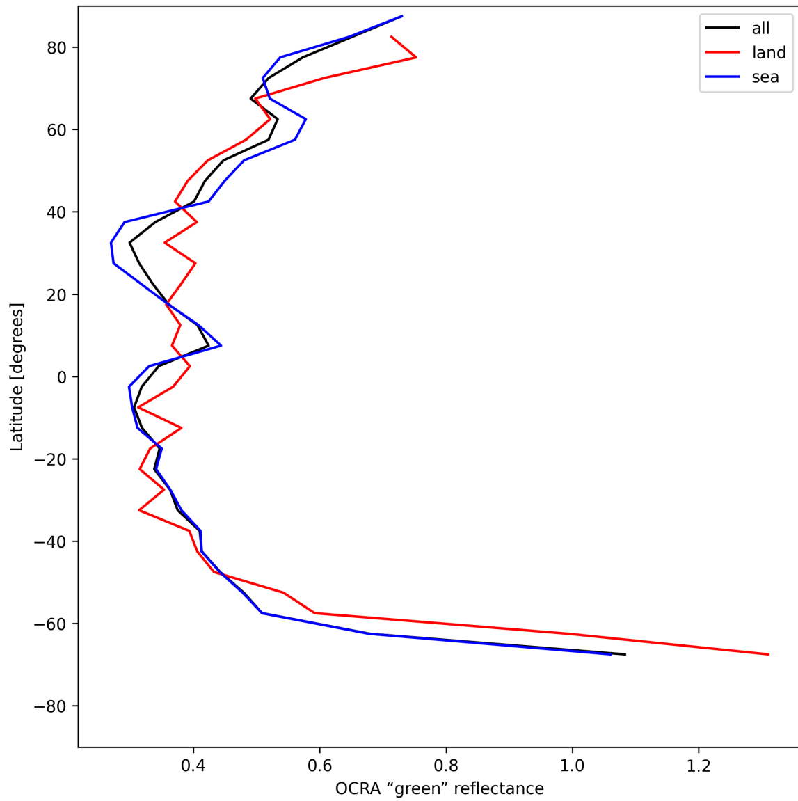
Figure 34: Zonal average of “OCRA “green” reflectance” for 2025-07-19 to 2025-07-20.
