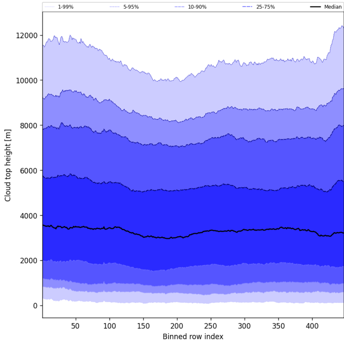
Figure 54: Along track statistics of “Cloud top height” for 2025-07-19 to 2025-07-20
