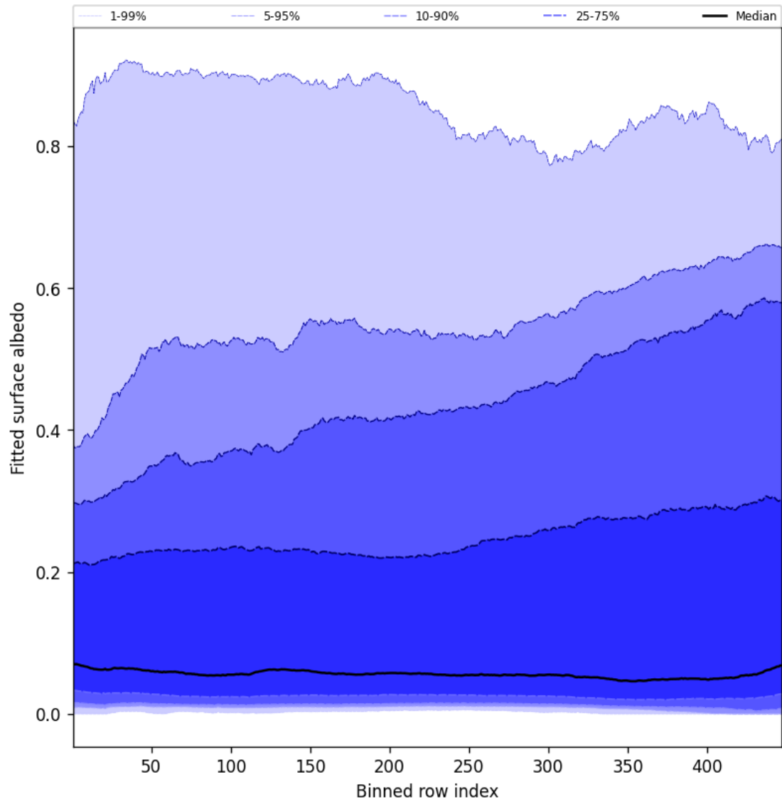
Figure 59: Along track statistics of “Fitted surface albedo” for 2025-07-19 to 2025-07-20
