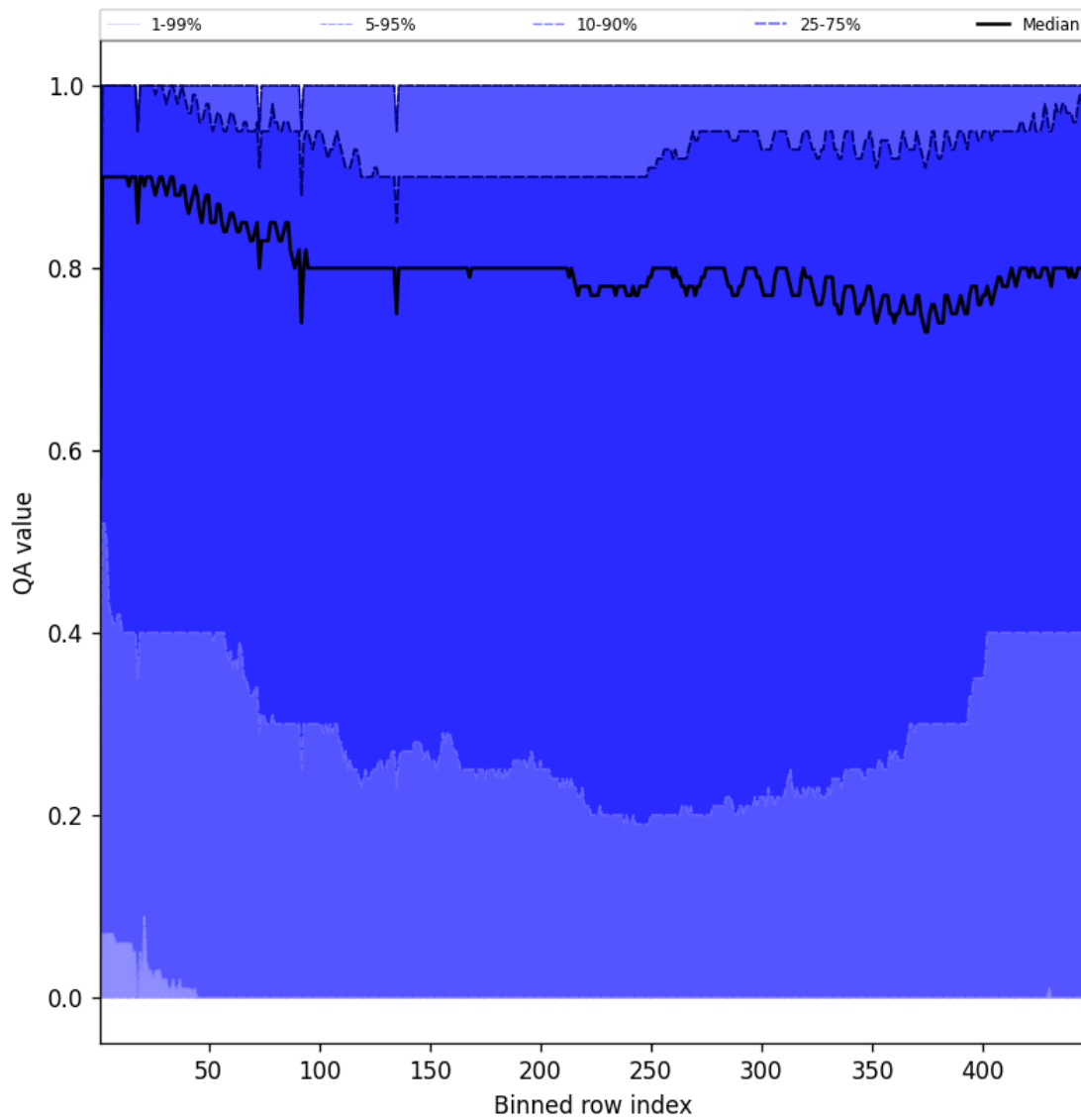
Figure 52: Along track statistics of “QA value” for 2025-07-19 to 2025-07-20
