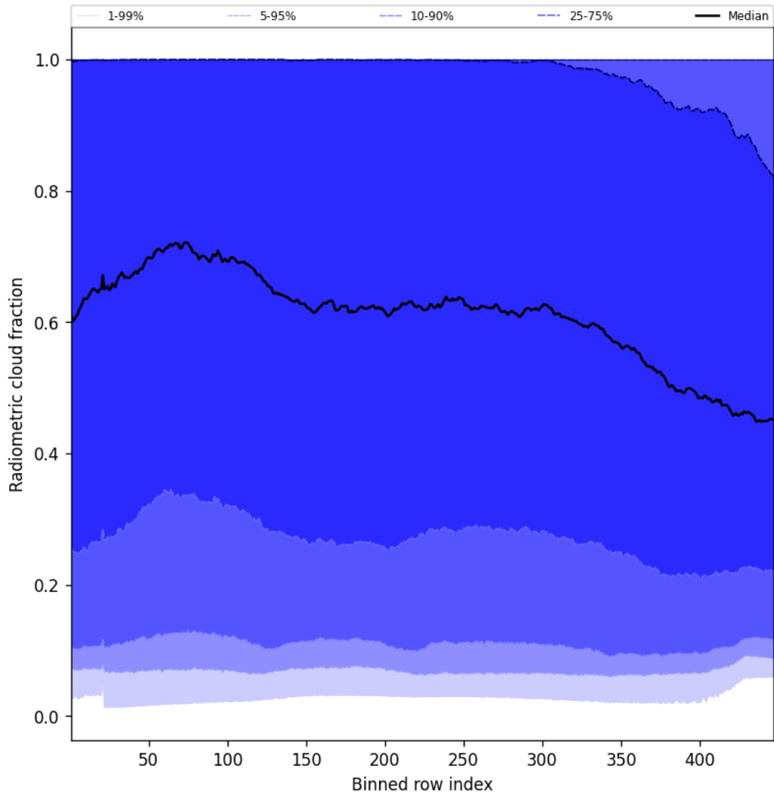
Figure 53: Along track statistics of “Radiometric cloud fraction” for 2025-07-19 to 2025-07-20
