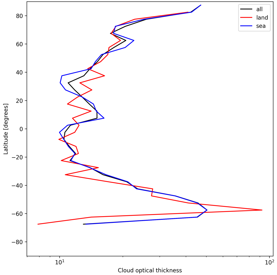
Figure 23: Zonal average of “Cloud optical thickness” for 2025-07-19 to 2025-07-20.
