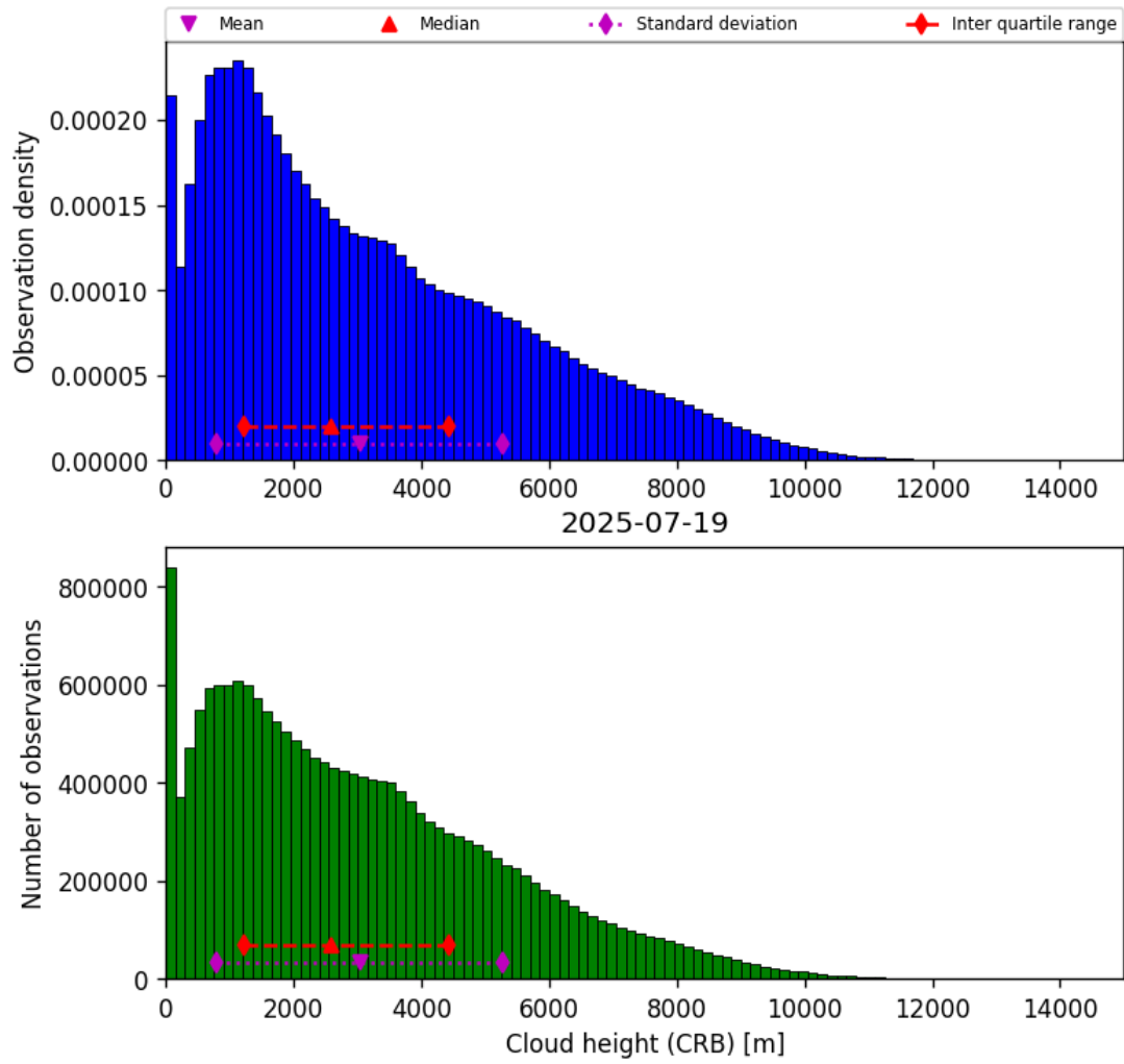
Figure 41: Histogram of “Cloud height (CRB)” for 2025-07-19 to 2025-07-20
