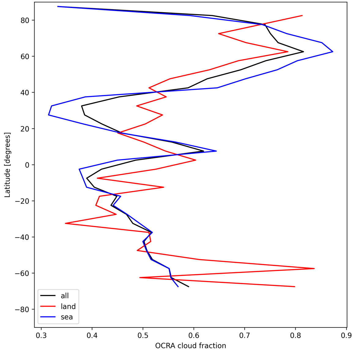
Figure 32: Zonal average of “OCRA cloud fraction” for 2025-07-19 to 2025-07-20.
