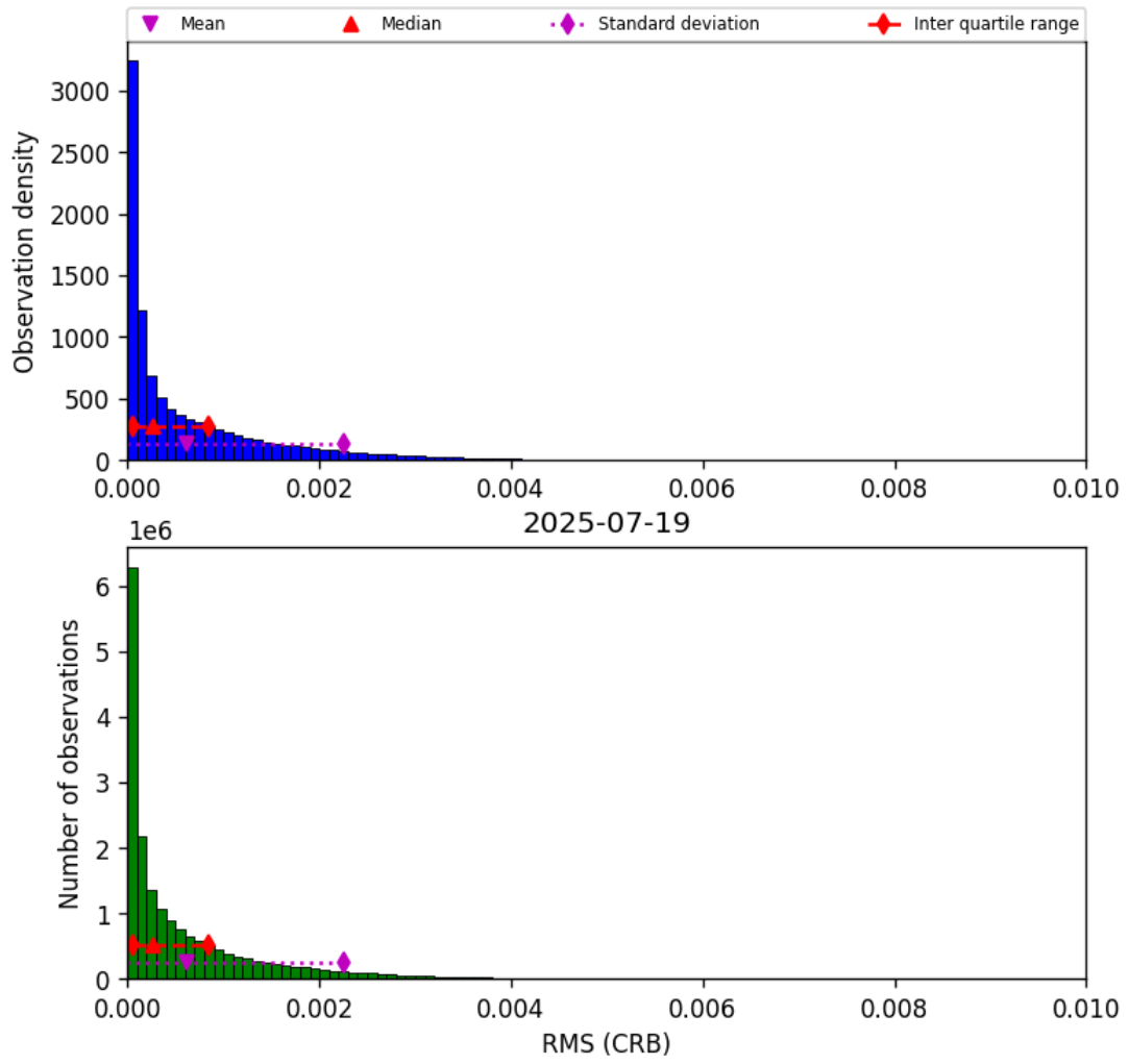
Figure 46: Histogram of “RMS (CRB)” for 2025-07-19 to 2025-07-20
