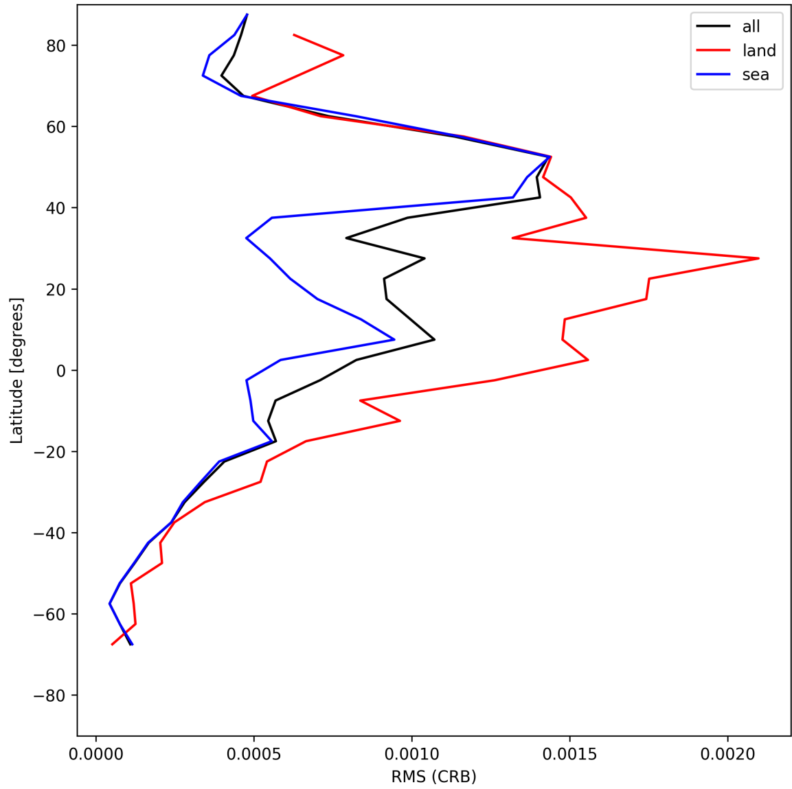
Figure 30: Zonal average of “RMS (CRB)” for 2025-07-19 to 2025-07-20.
