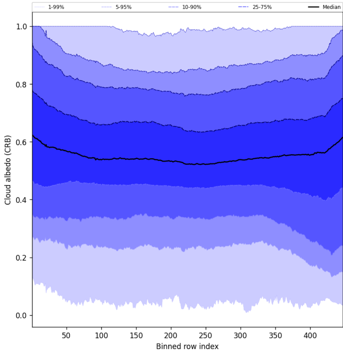
Figure 58: Along track statistics of “Cloud albedo (CRB)” for 2025-07-19 to 2025-07-20
