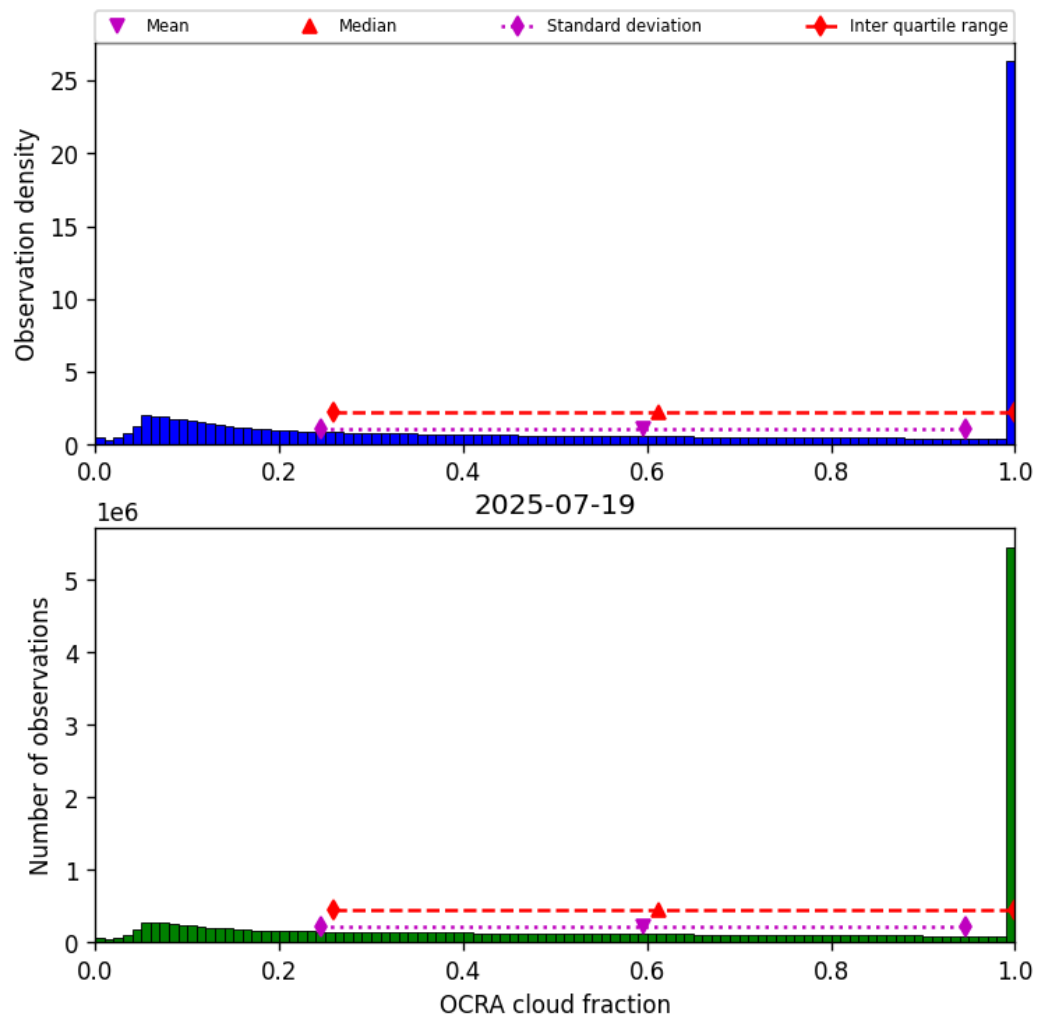
Figure 48: Histogram of “OCRA cloud fraction” for 2025-07-19 to 2025-07-20
