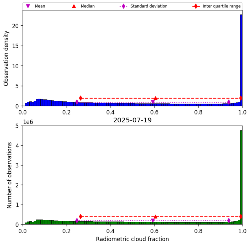
Figure 37: Histogram of “Radiometric cloud fraction” for 2025-07-19 to 2025-07-20
