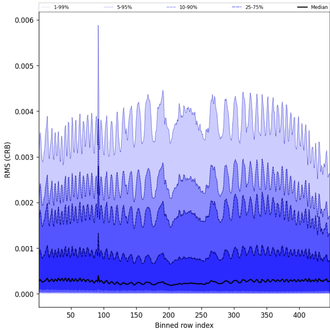
Figure 62: Along track statistics of “RMS (CRB)” for 2025-07-19 to 2025-07-20
