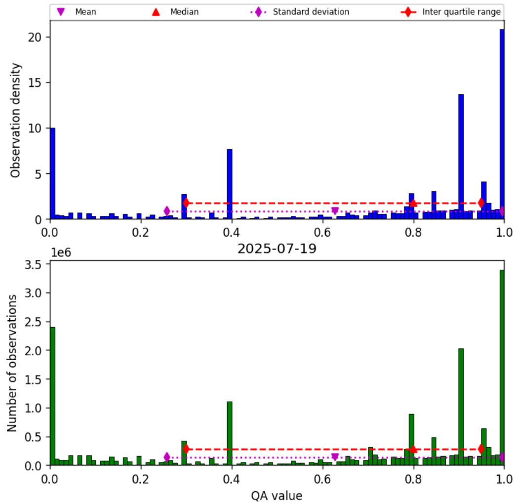
Figure 36: Histogram of “QA value” for 2025-07-19 to 2025-07-20
