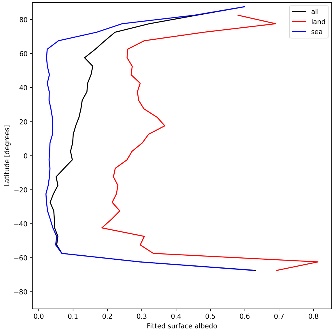
Figure 27: Zonal average of “Fitted surface albedo” for 2025-07-19 to 2025-07-20.
