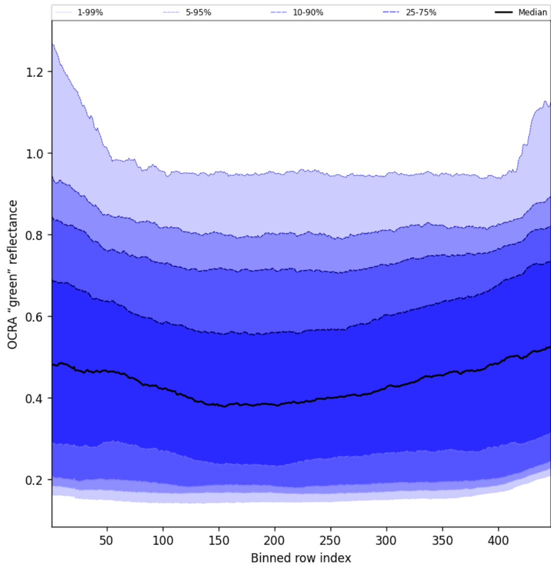
Figure 66: Along track statistics of “OCRA “green” reflectance” for 2025-07-19 to 2025-07-20
