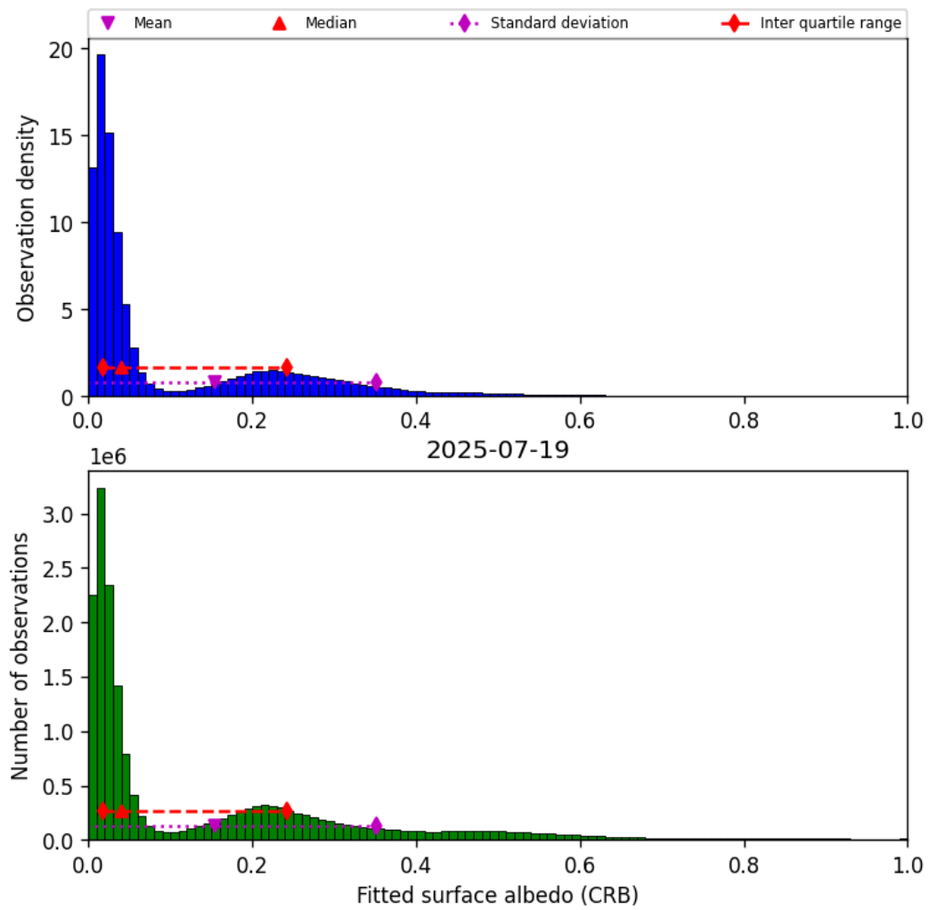
Figure 44: Histogram of “Fitted surface albedo (CRB)” for 2025-07-19 to 2025-07-20
