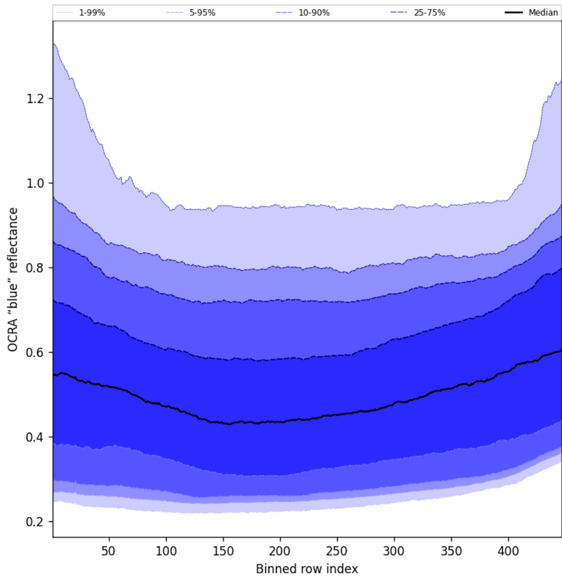
Figure 65: Along track statistics of “OCRA “blue” reflectance” for 2025-07-19 to 2025-07-20
