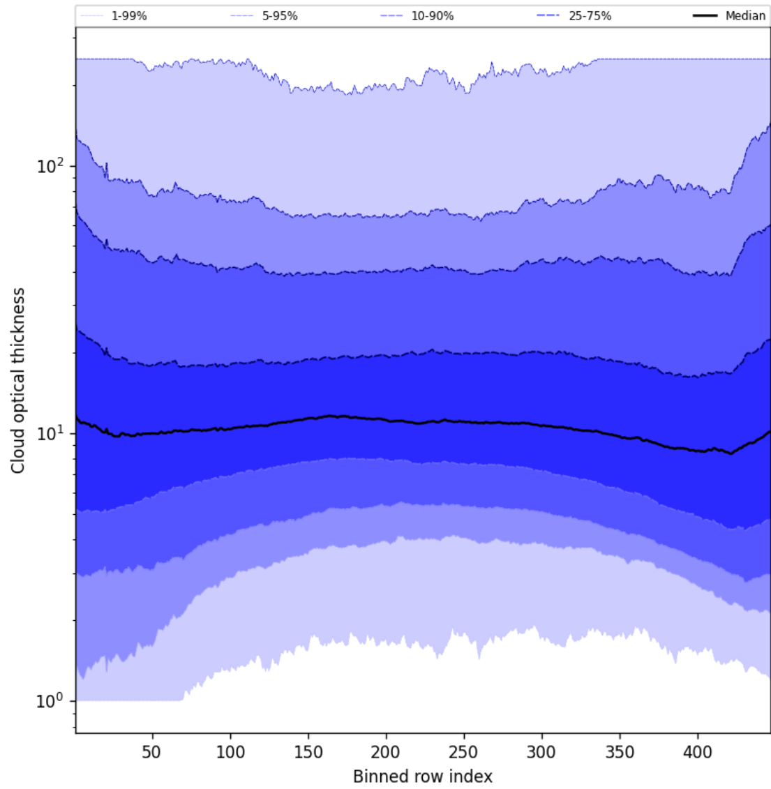
Figure 55: Along track statistics of “Cloud optical thickness” for 2025-07-19 to 2025-07-20
