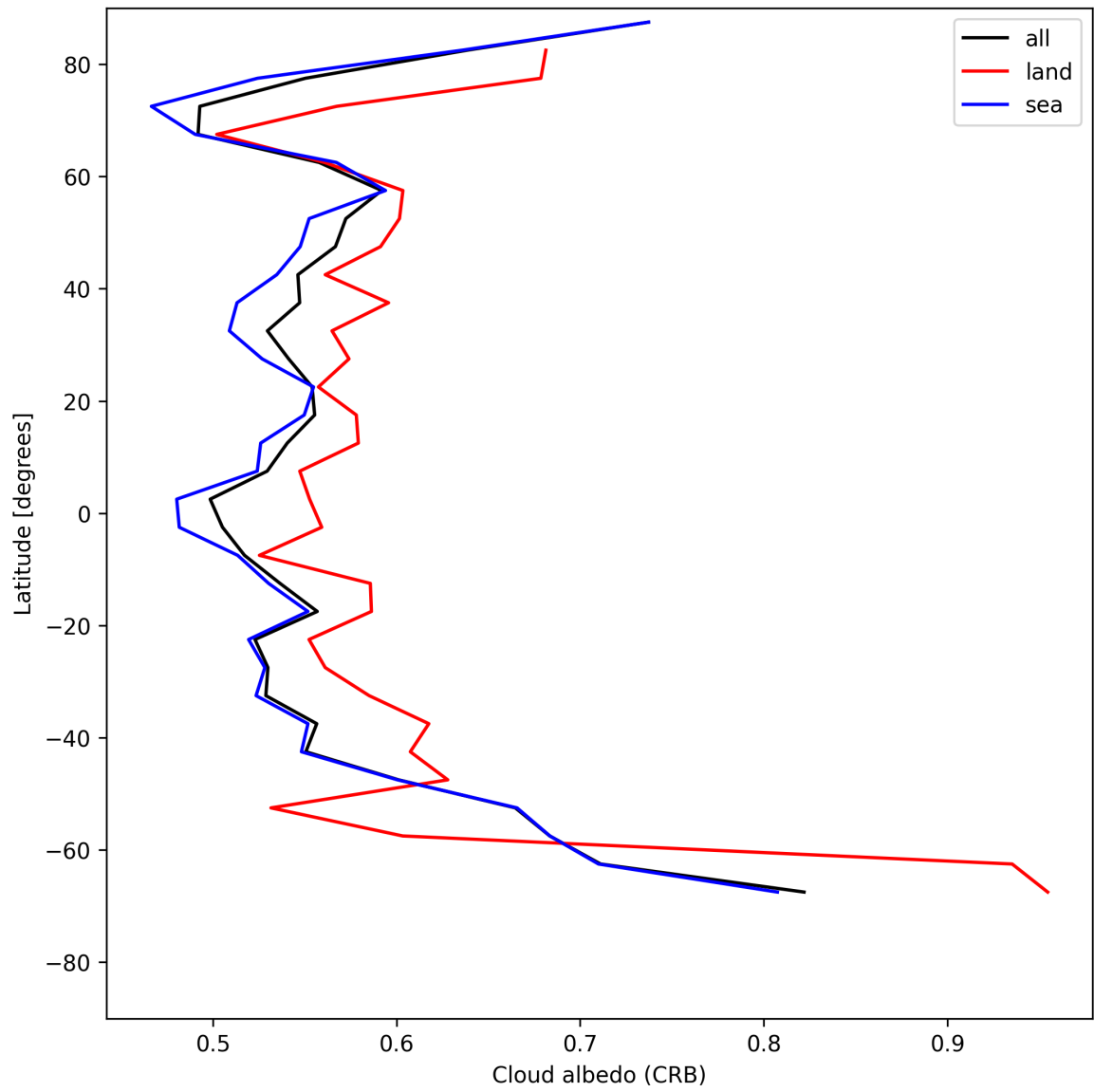
Figure 26: Zonal average of “Cloud albedo (CRB)” for 2025-07-19 to 2025-07-20.
