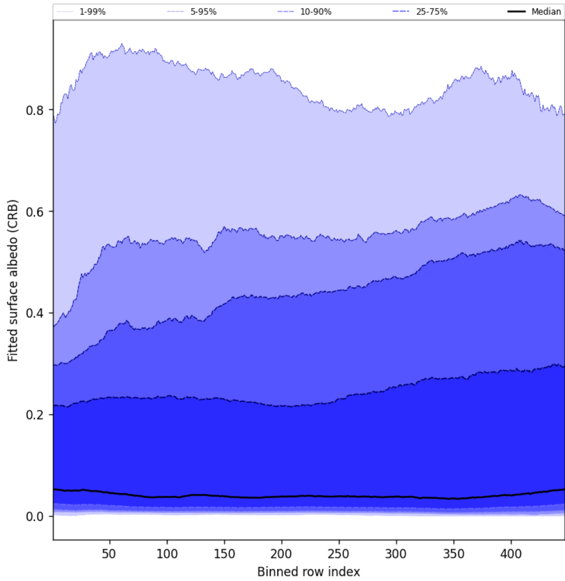
Figure 60: Along track statistics of “Fitted surface albedo (CRB)” for 2025-07-19 to 2025-07-20
