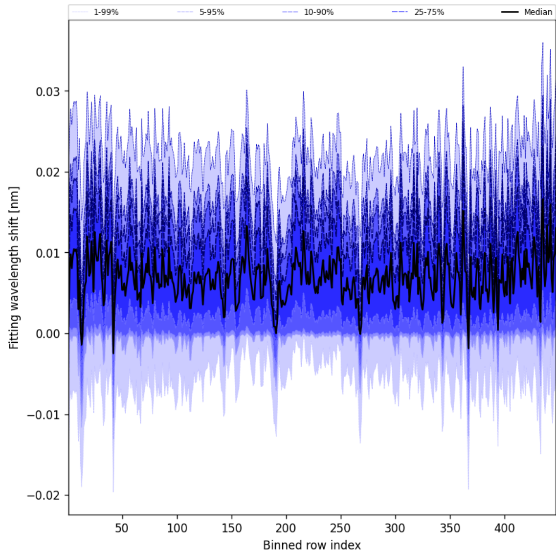
Figure 63: Along track statistics of “Fitting wavelength shift” for 2025-07-19 to 2025-07-20
