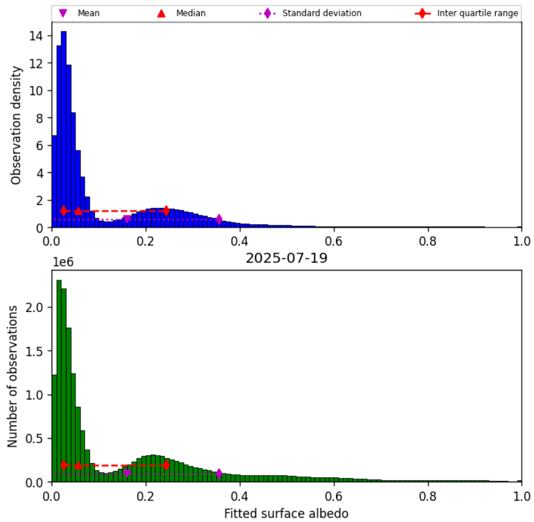
Figure 43: Histogram of “Fitted surface albedo” for 2025-07-19 to 2025-07-20
