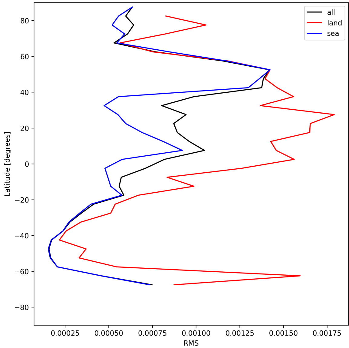
Figure 29: Zonal average of “RMS” for 2025-07-19 to 2025-07-20.
