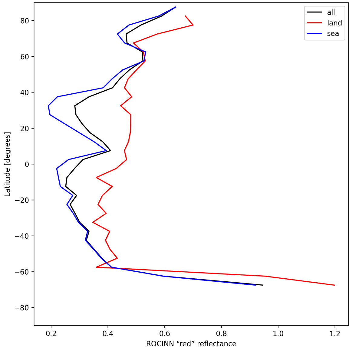
Figure 35: Zonal average of “ROCINN “red” reflectance” for 2025-07-19 to 2025-07-20.
