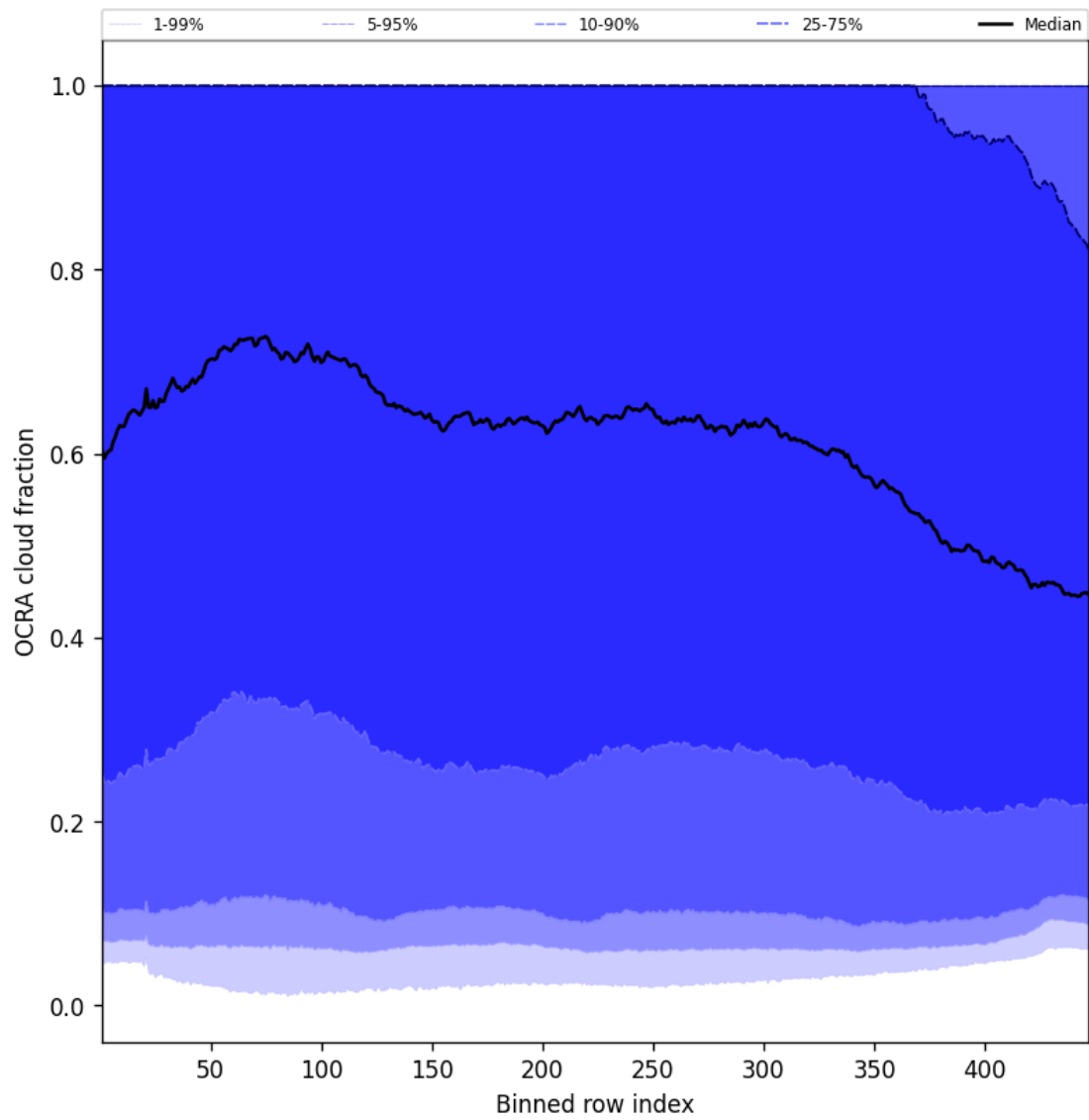
Figure 64: Along track statistics of “OCRA cloud fraction” for 2025-07-19 to 2025-07-20
