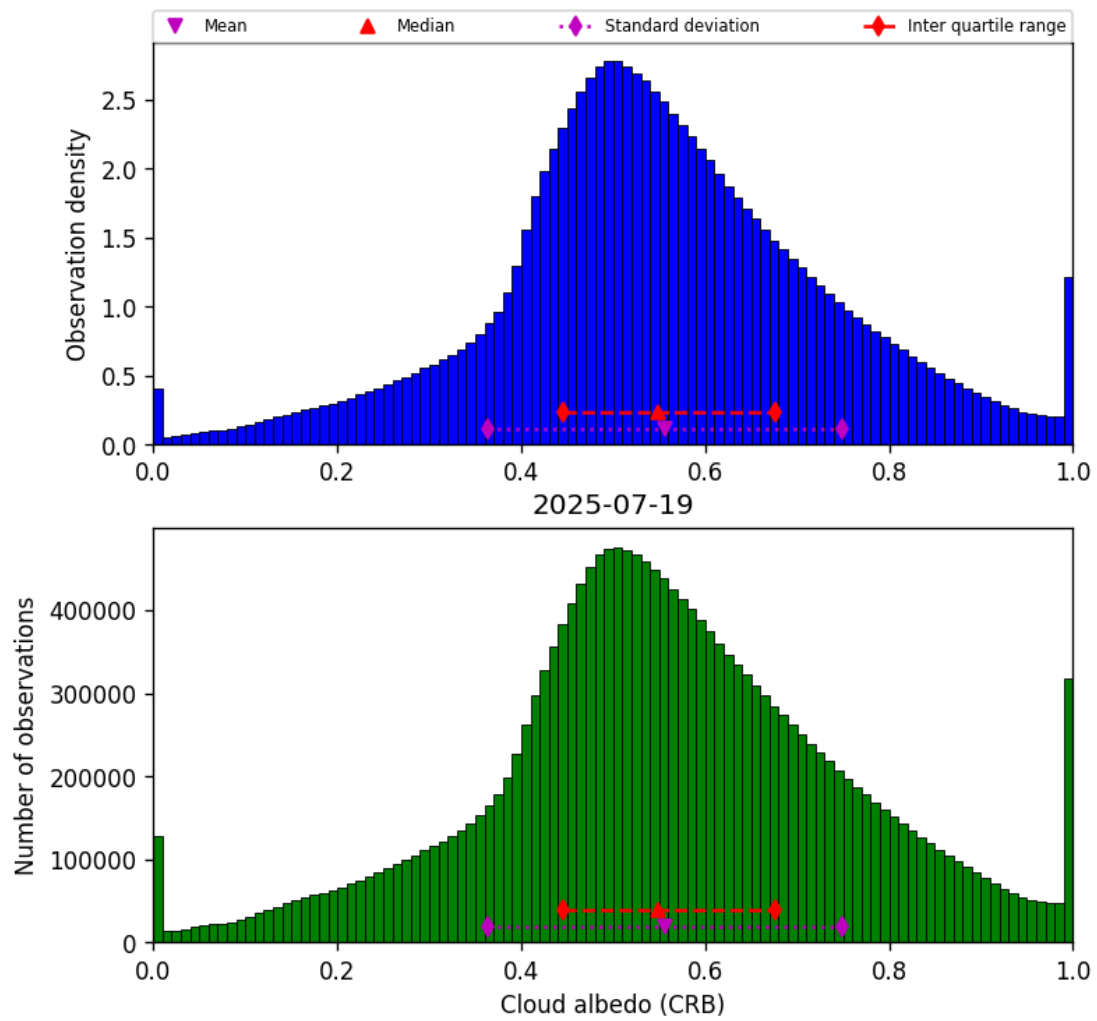
Figure 42: Histogram of “Cloud albedo (CRB)” for 2025-07-19 to 2025-07-20
