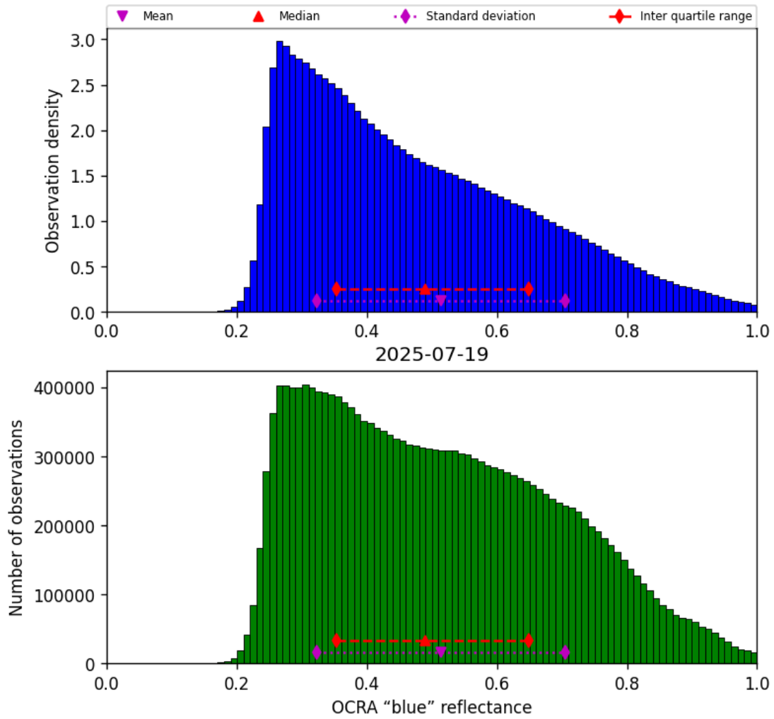
Figure 49: Histogram of “OCRA “blue” reflectance” for 2025-07-19 to 2025-07-20
