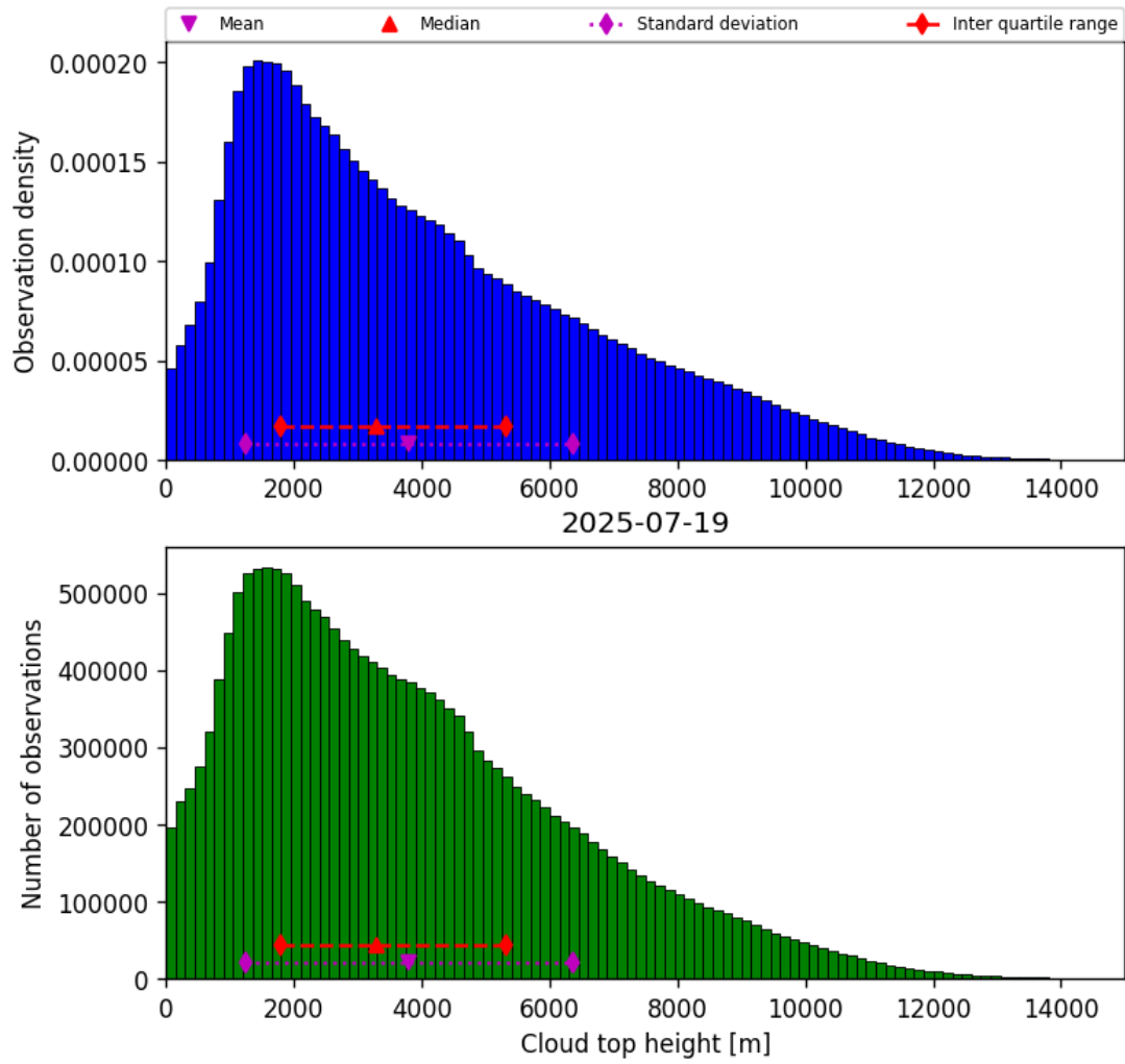
Figure 38: Histogram of “Cloud top height” for 2025-07-19 to 2025-07-20
