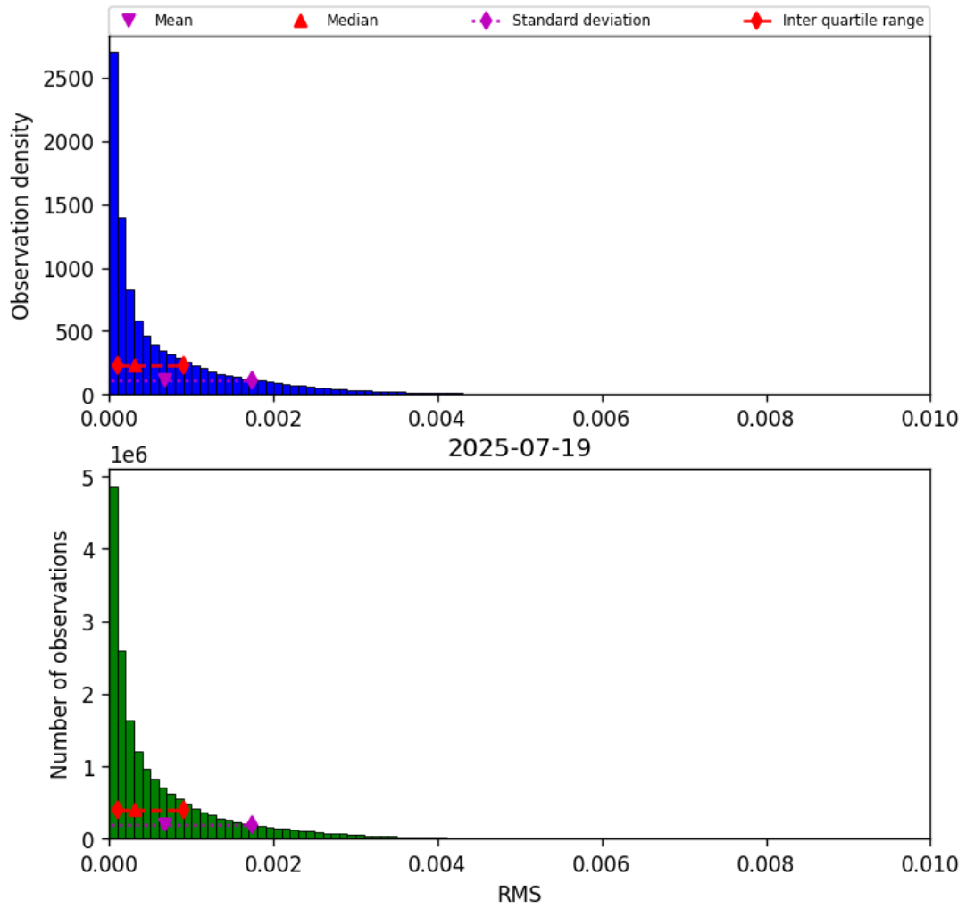
Figure 45: Histogram of “RMS” for 2025-07-19 to 2025-07-20
