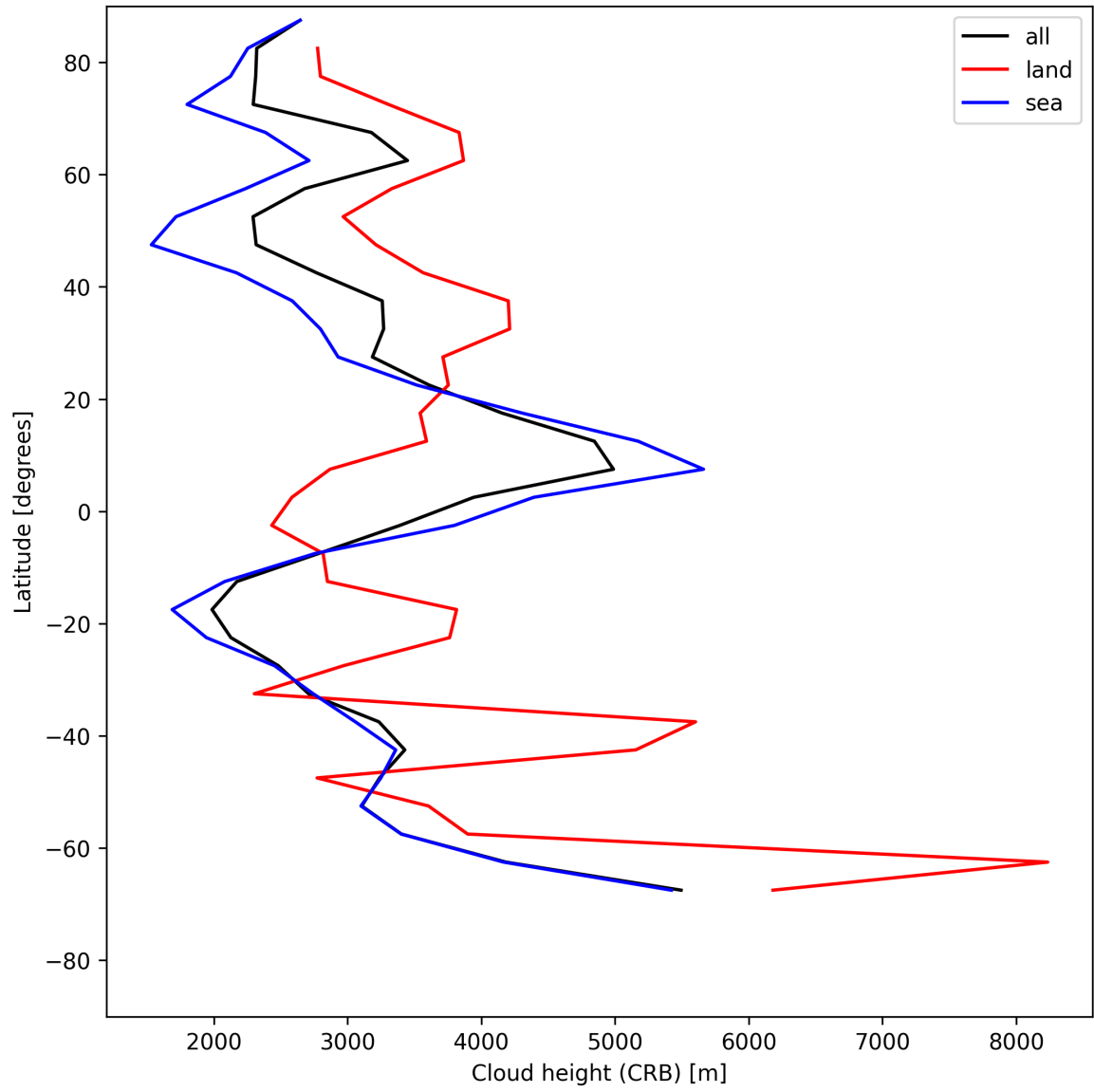
Figure 25: Zonal average of “Cloud height (CRB)” for 2025-07-19 to 2025-07-20.
