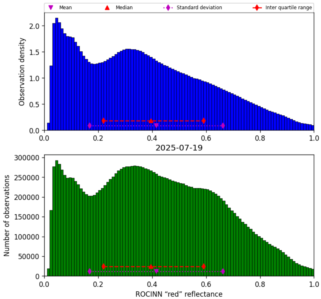
Figure 51: Histogram of “ROCINN “red” reflectance” for 2025-07-19 to 2025-07-20
