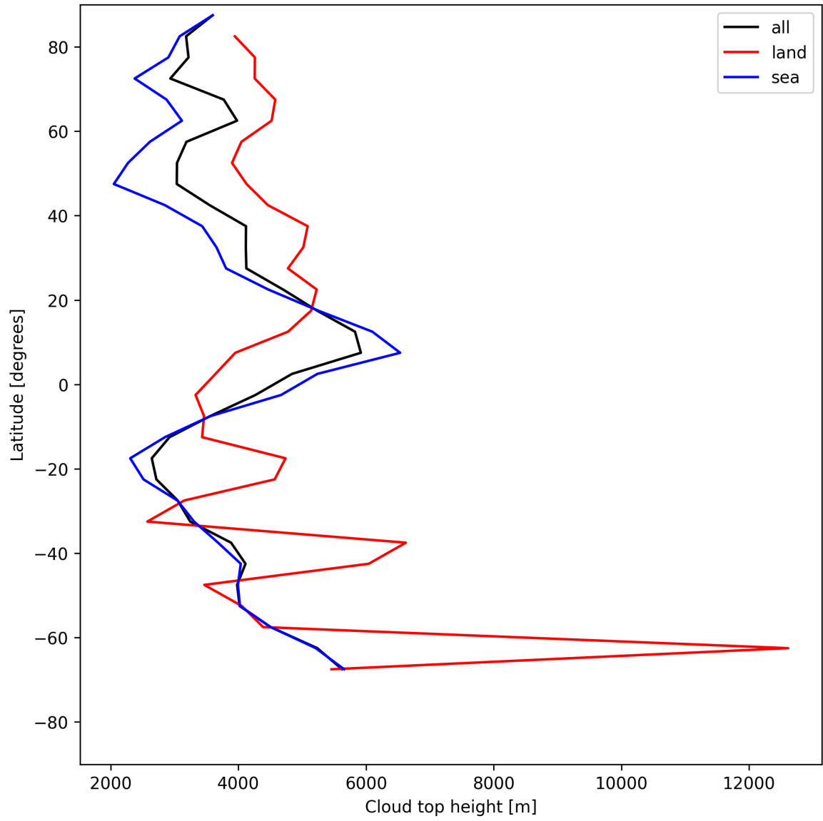
Figure 22: Zonal average of “Cloud top height” for 2025-07-19 to 2025-07-20.
