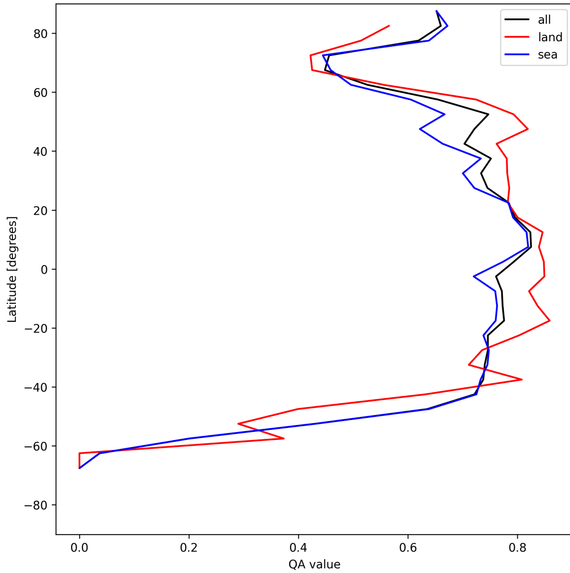
Figure 20: Zonal average of “QA value” for 2025-07-20 to 2025-07-21.
