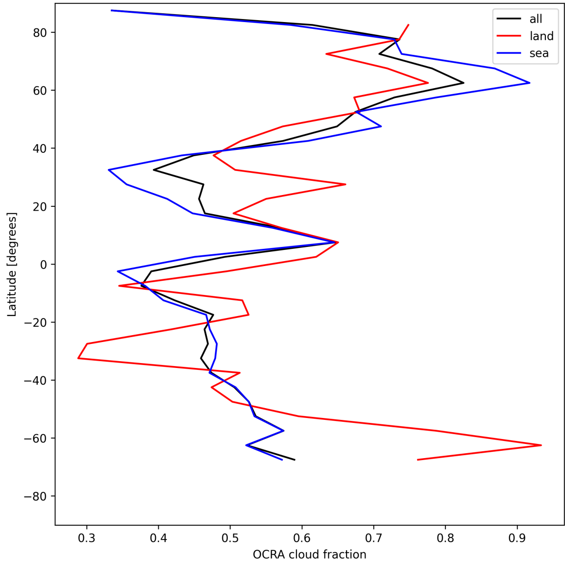
Figure 32: Zonal average of “OCRA cloud fraction” for 2025-07-20 to 2025-07-21.
