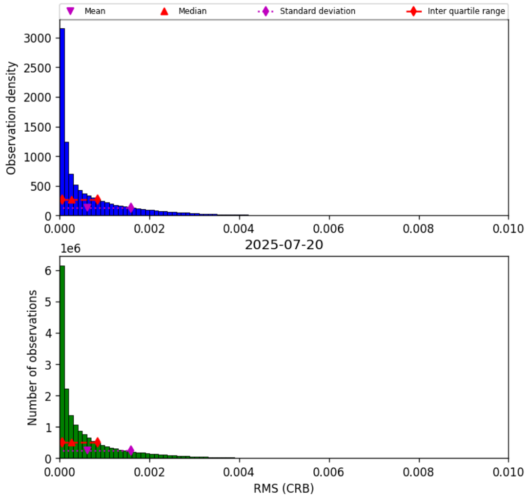
Figure 46: Histogram of “RMS (CRB)” for 2025-07-20 to 2025-07-21
