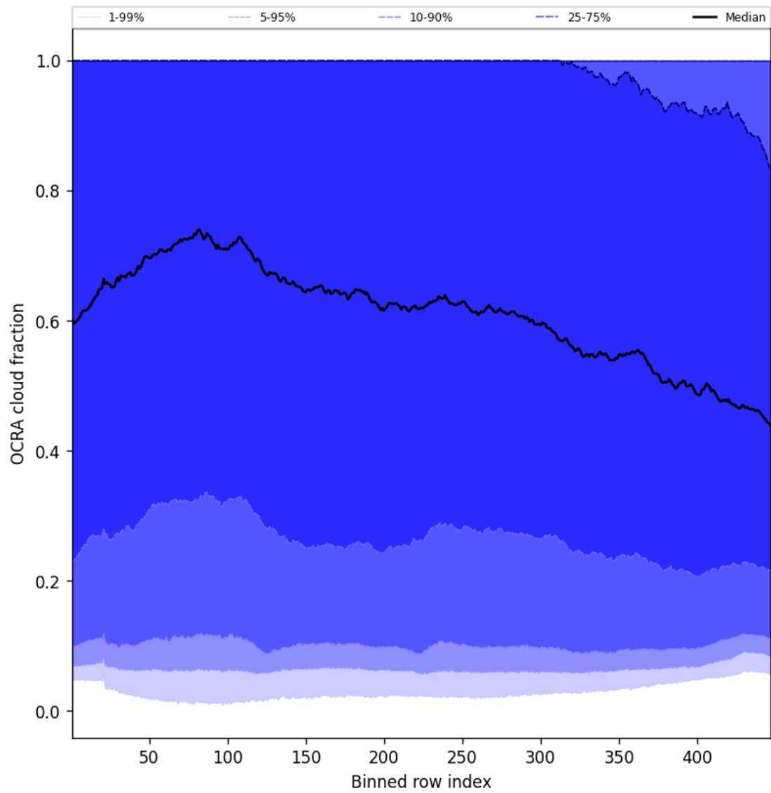
Figure 64: Along track statistics of “OCRA cloud fraction” for 2025-07-20 to 2025-07-21
