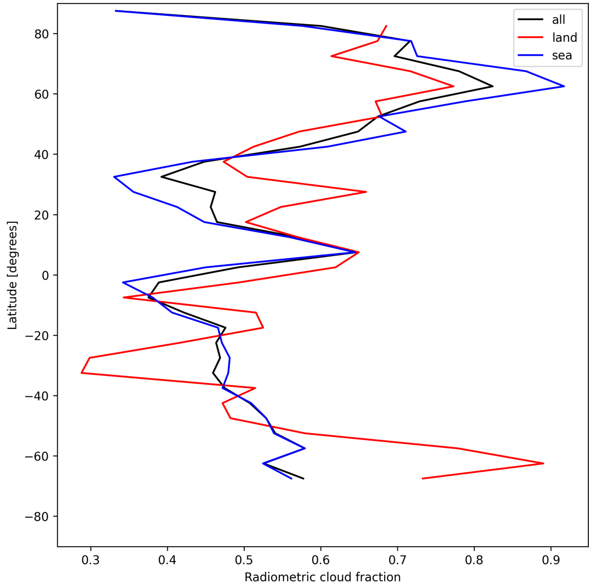
Figure 21: Zonal average of “Radiometric cloud fraction” for 2025-07-20 to 2025-07-21.
