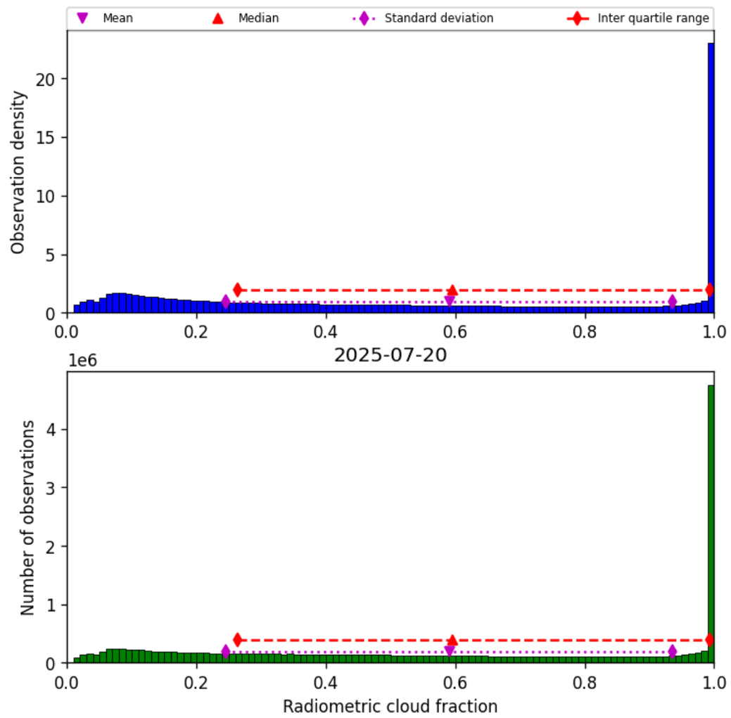
Figure 37: Histogram of “Radiometric cloud fraction” for 2025-07-20 to 2025-07-21
