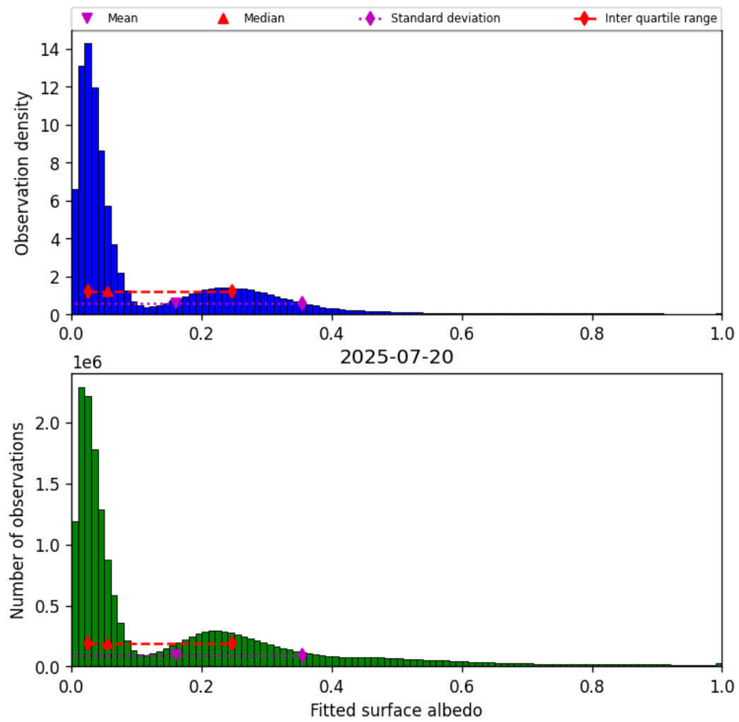
Figure 43: Histogram of “Fitted surface albedo” for 2025-07-20 to 2025-07-21
