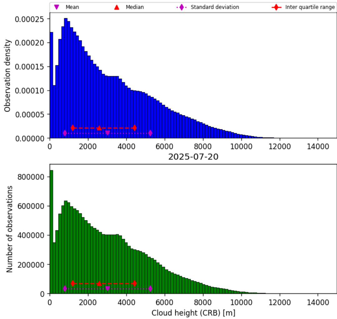
Figure 41: Histogram of “Cloud height (CRB)” for 2025-07-20 to 2025-07-21
