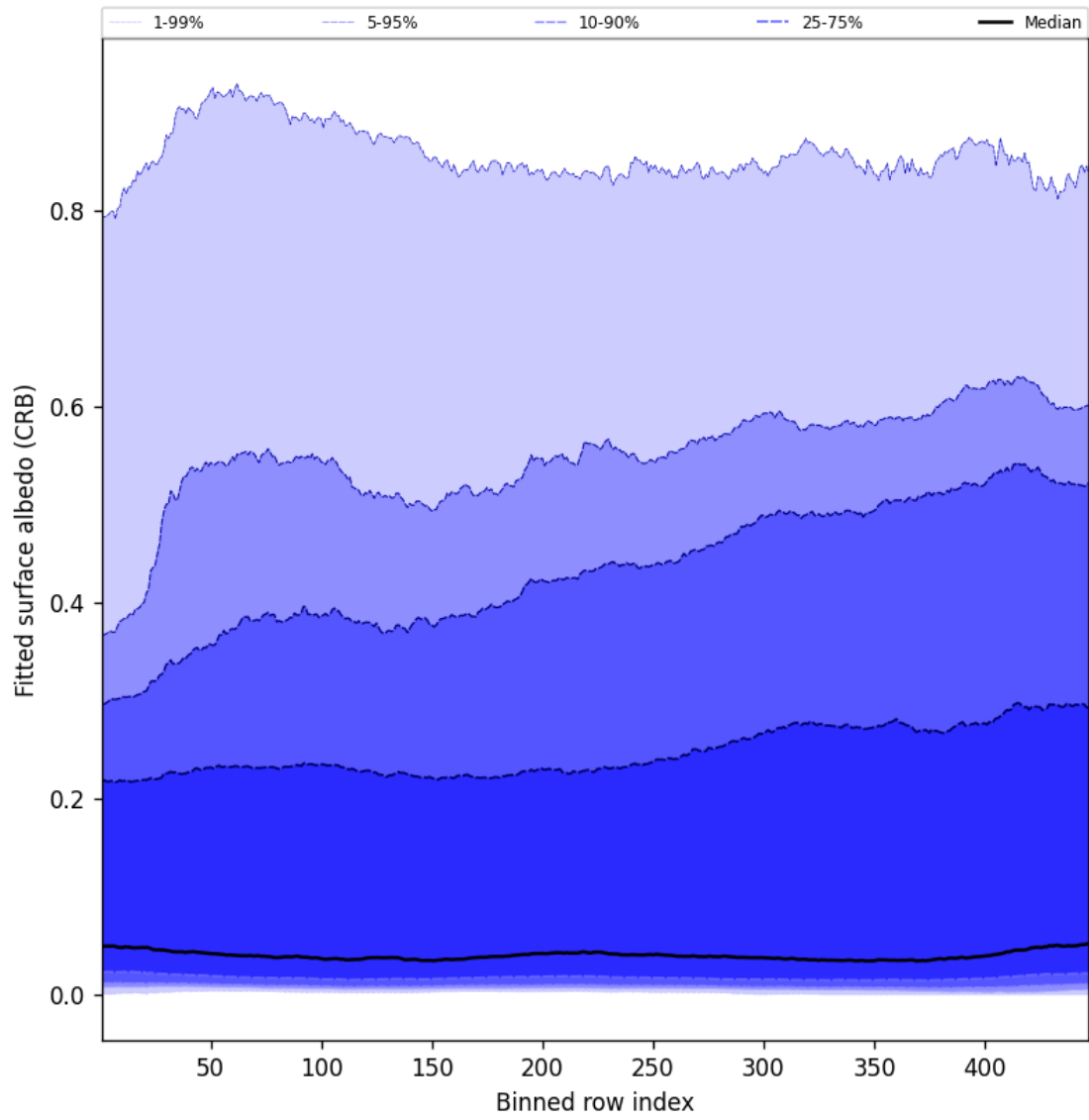
Figure 60: Along track statistics of “Fitted surface albedo (CRB)” for 2025-07-20 to 2025-07-21
