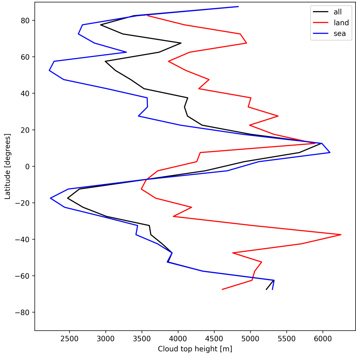
Figure 22: Zonal average of “Cloud top height” for 2025-07-20 to 2025-07-21.
