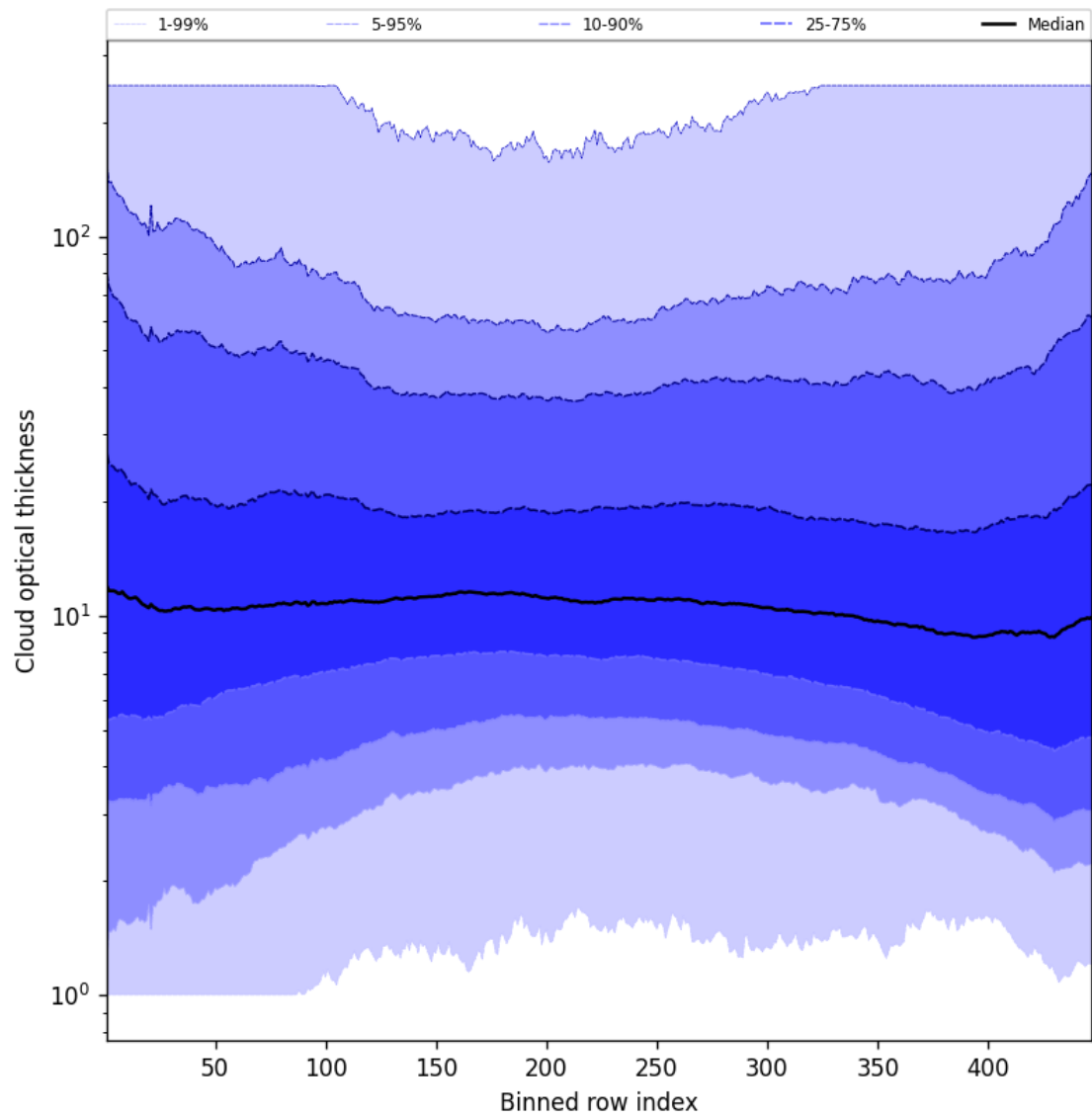
Figure 55: Along track statistics of “Cloud optical thickness” for 2025-07-20 to 2025-07-21
