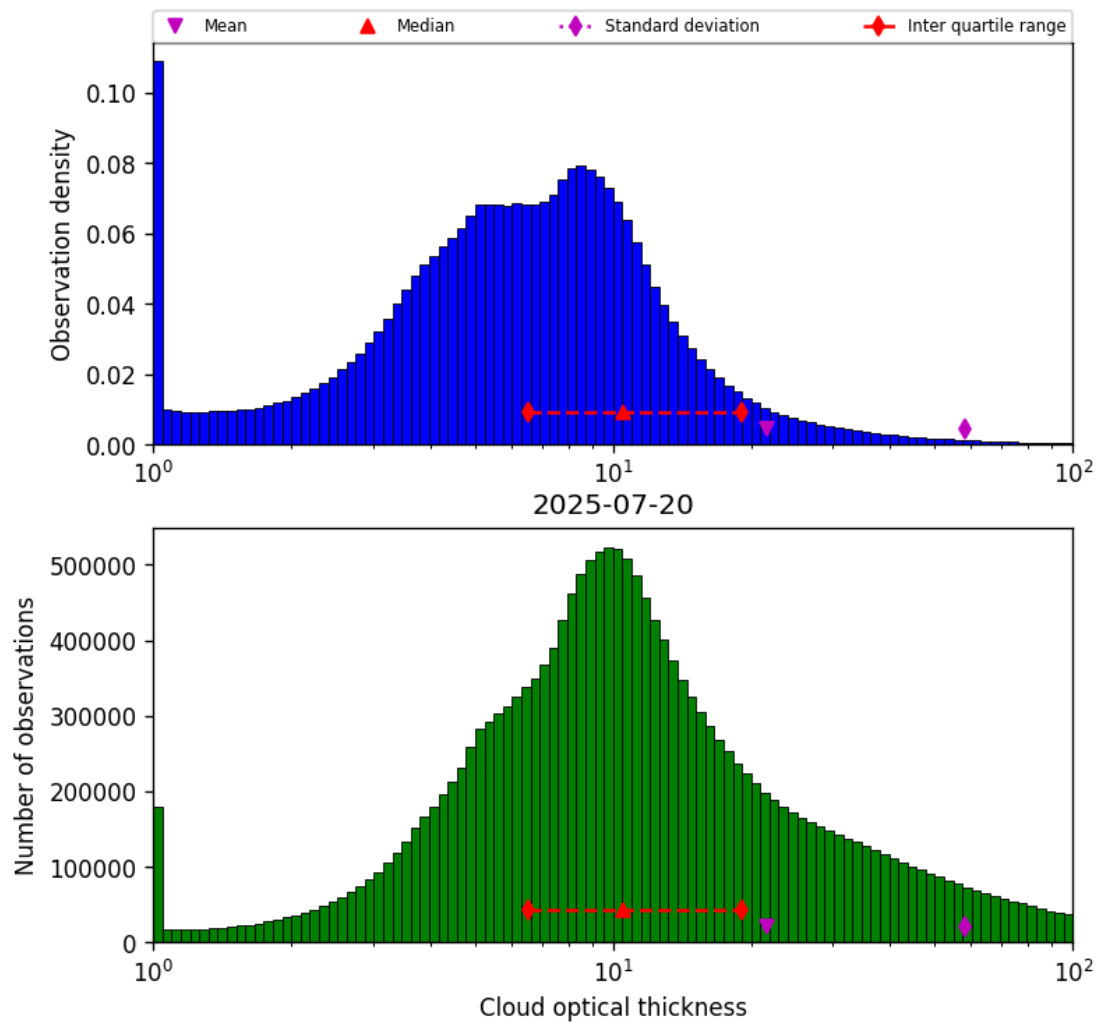
Figure 39: Histogram of “Cloud optical thickness” for 2025-07-20 to 2025-07-21
