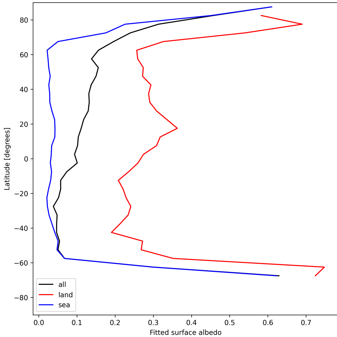
Figure 27: Zonal average of “Fitted surface albedo” for 2025-07-20 to 2025-07-21.
