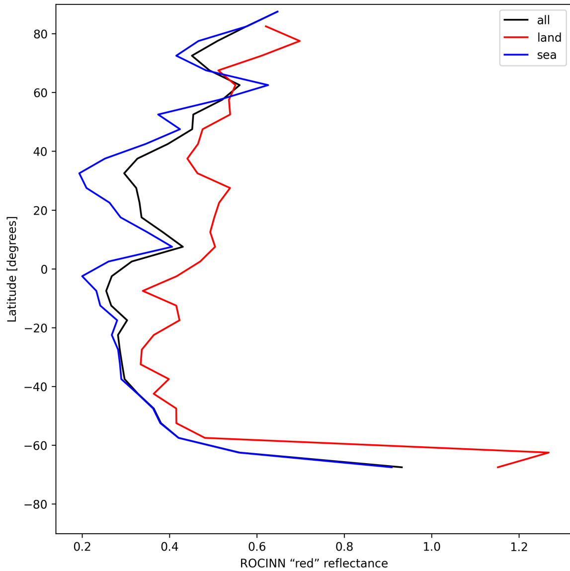
Figure 35: Zonal average of “ROCINN “red” reflectance” for 2025-07-20 to 2025-07-21.
