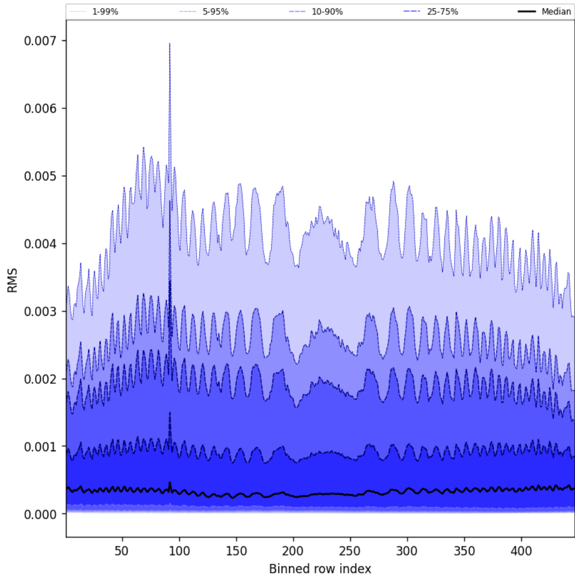
Figure 61: Along track statistics of “RMS” for 2025-07-20 to 2025-07-21
