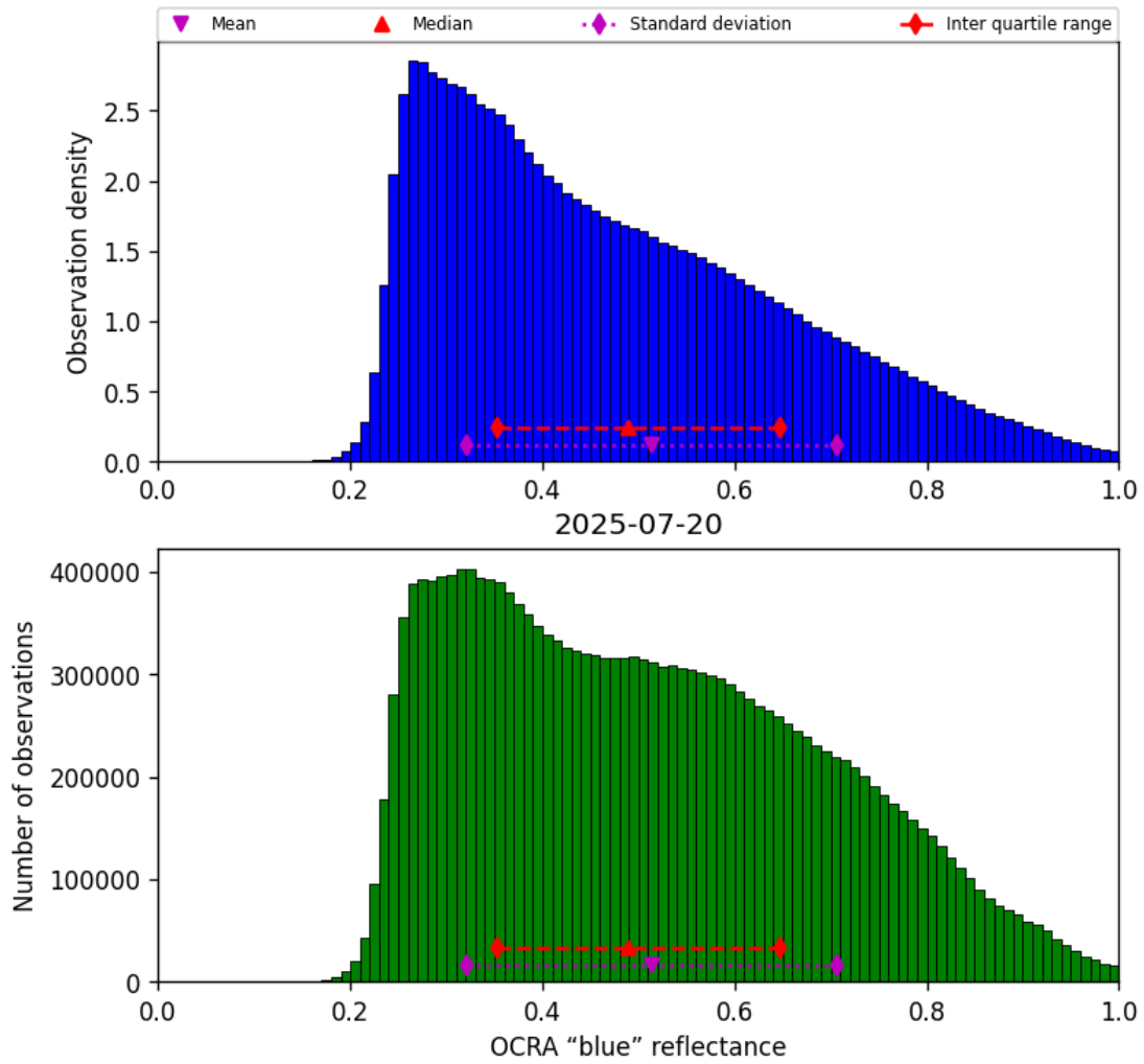
Figure 49: Histogram of “OCRA “blue” reflectance” for 2025-07-20 to 2025-07-21
