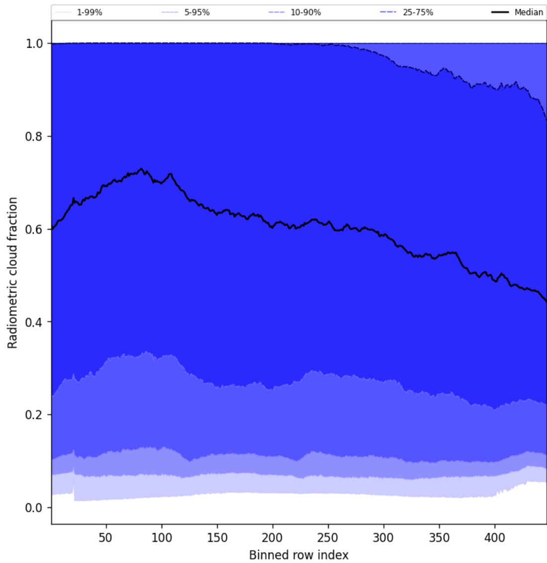
Figure 53: Along track statistics of “Radiometric cloud fraction” for 2025-07-20 to 2025-07-21
