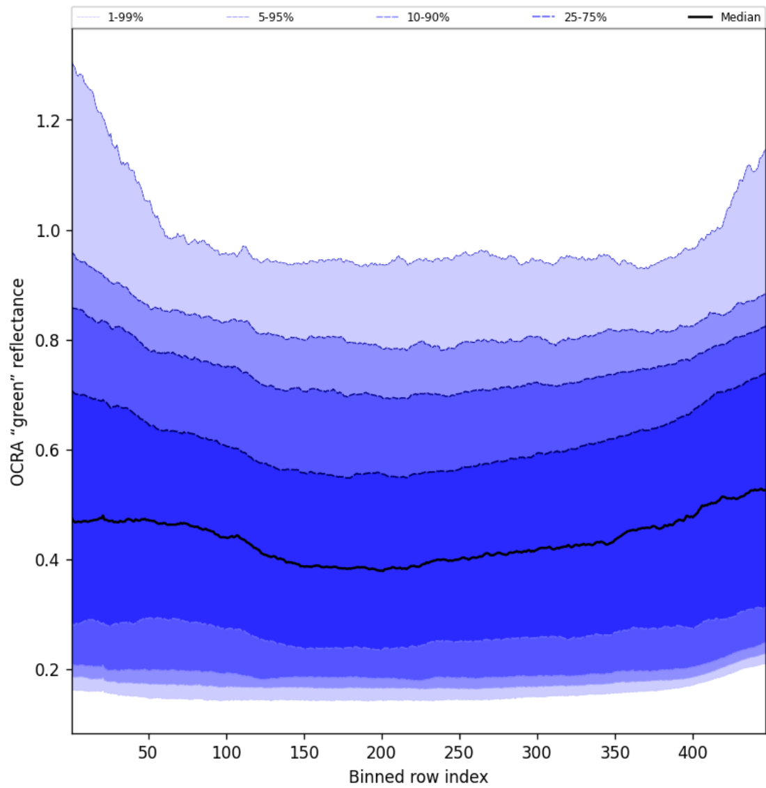
Figure 66: Along track statistics of “OCRA “green” reflectance” for 2025-07-20 to 2025-07-21
