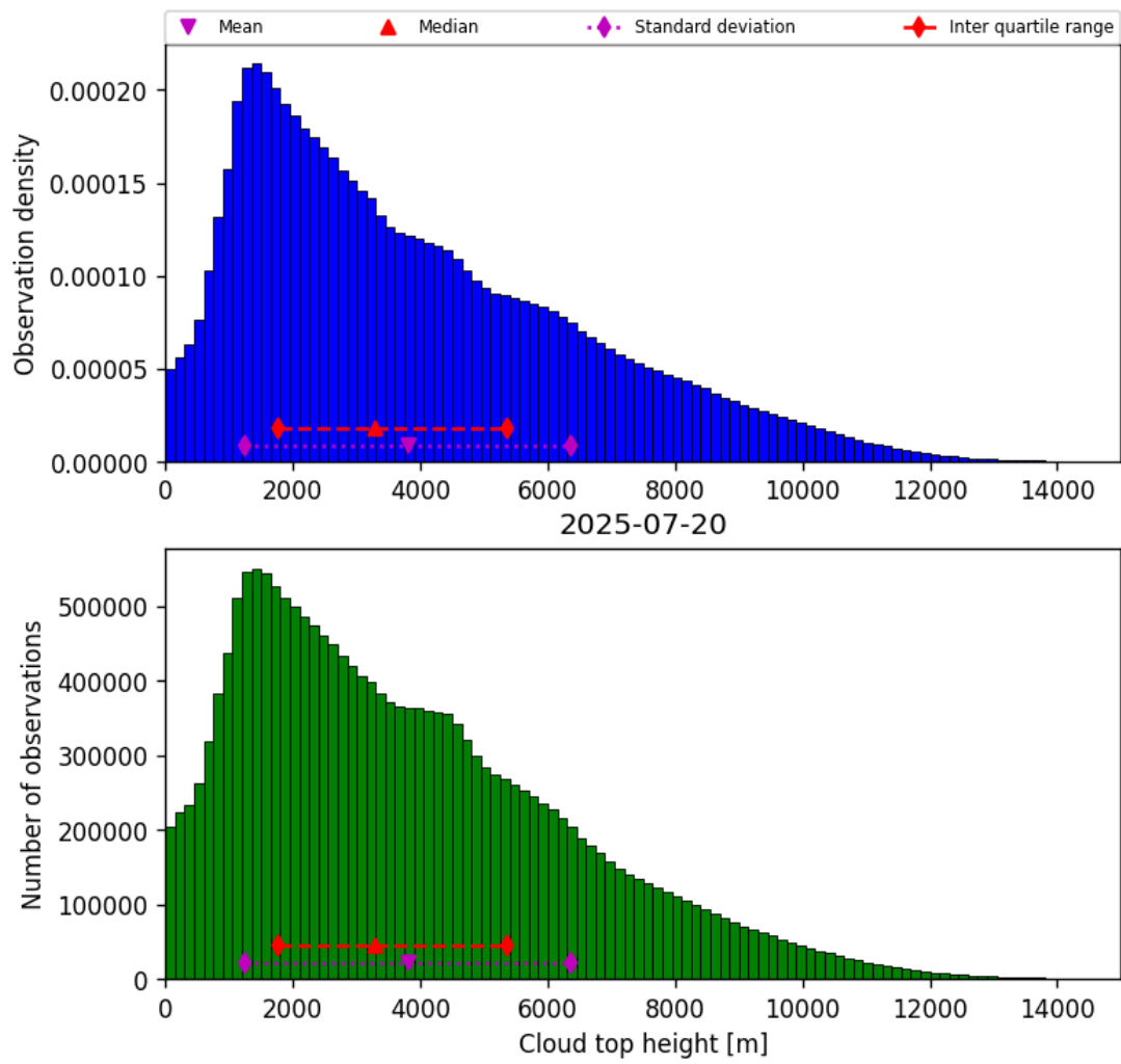
Figure 38: Histogram of “Cloud top height” for 2025-07-20 to 2025-07-21
