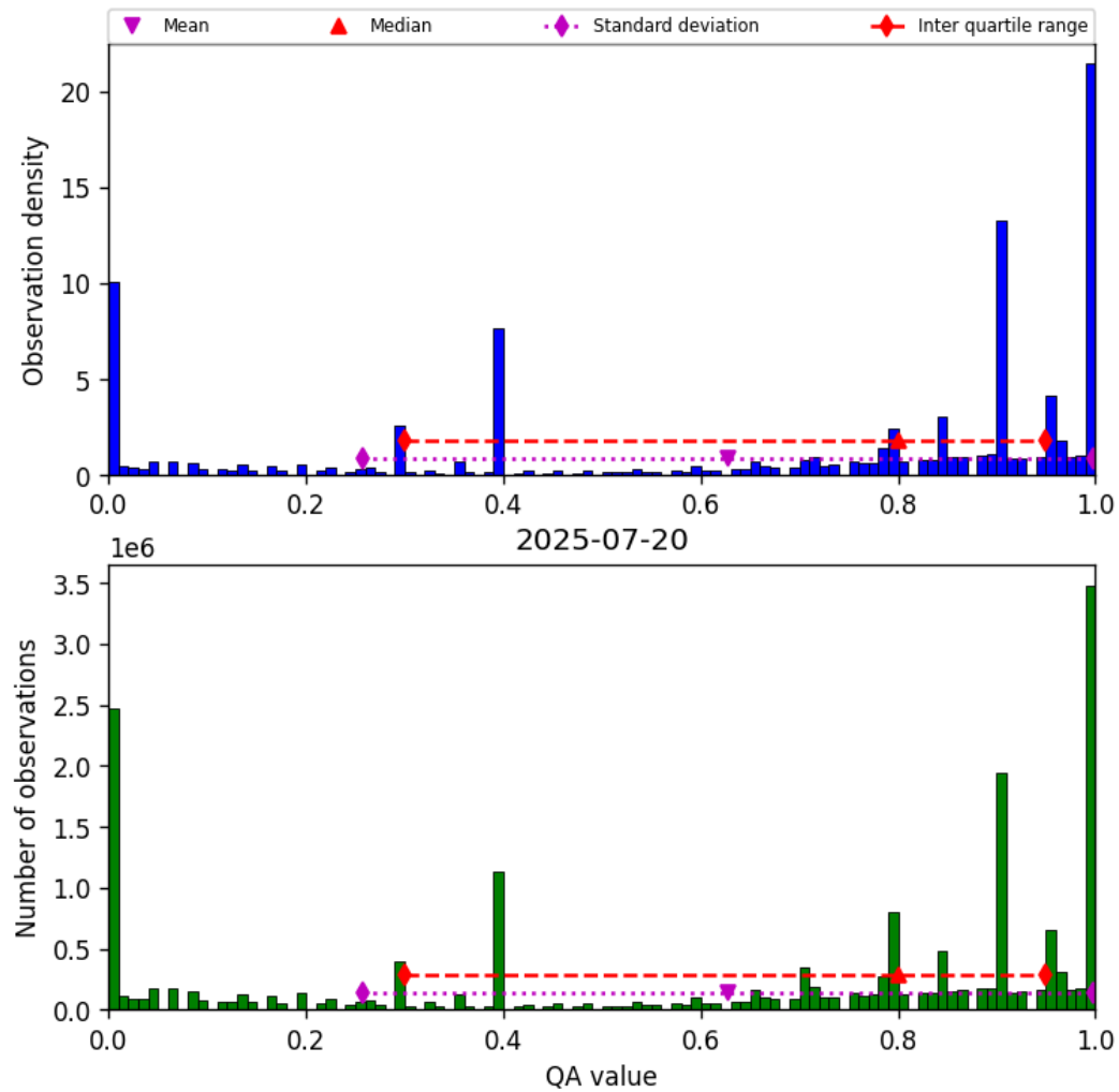
Figure 36: Histogram of “QA value” for 2025-07-20 to 2025-07-21
