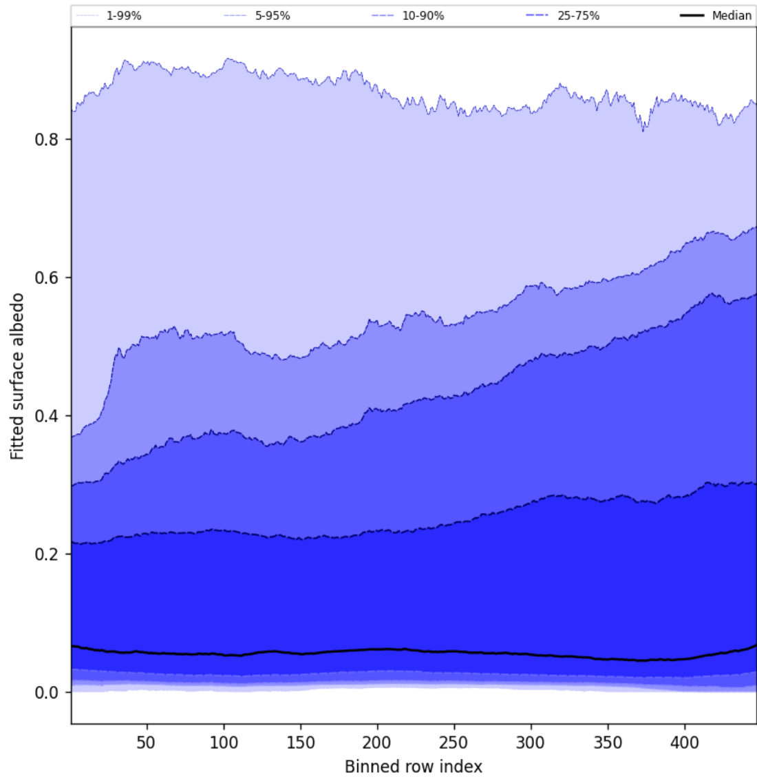
Figure 59: Along track statistics of “Fitted surface albedo” for 2025-07-20 to 2025-07-21
