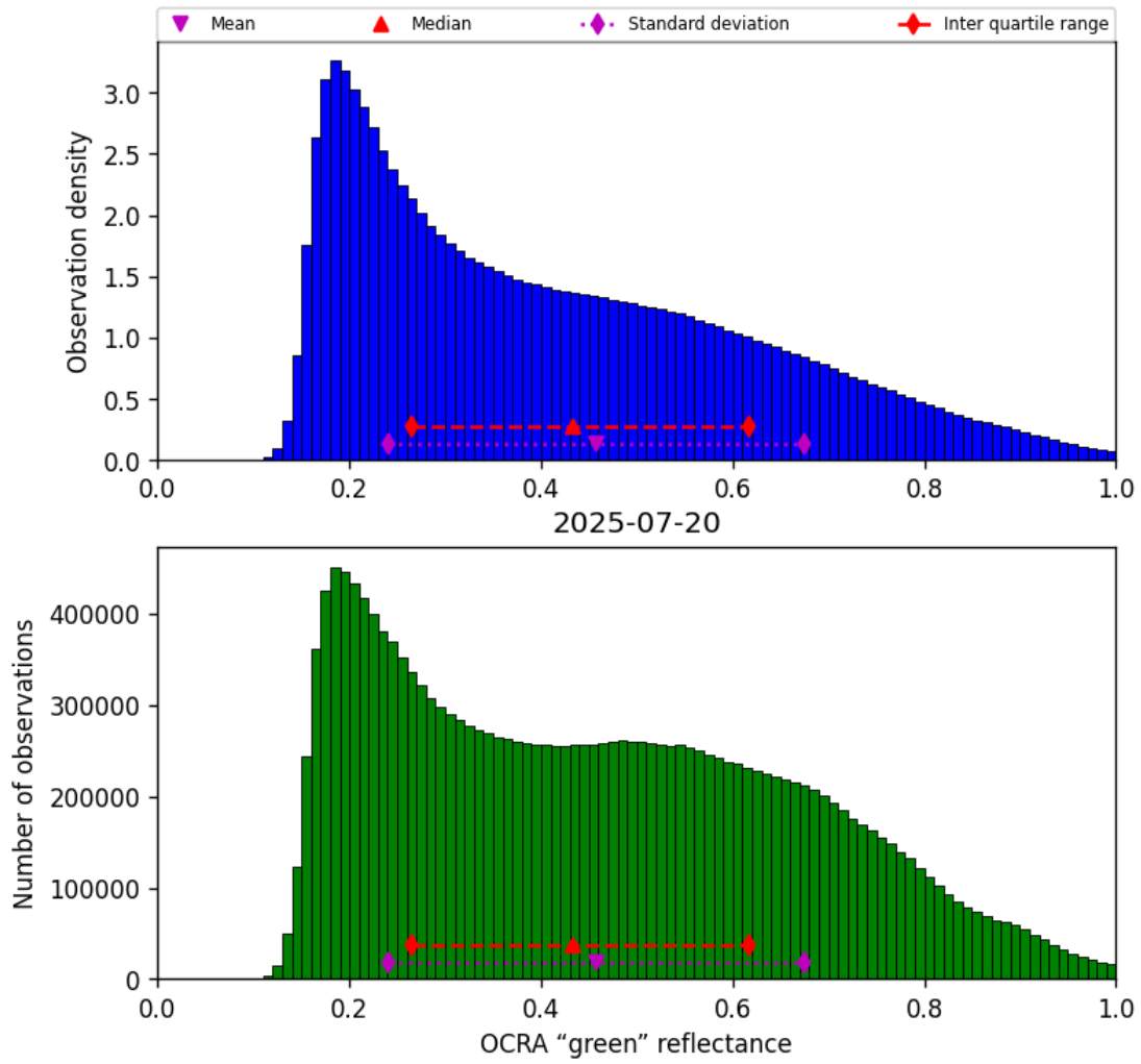
Figure 50: Histogram of “OCRA “green” reflectance” for 2025-07-20 to 2025-07-21
