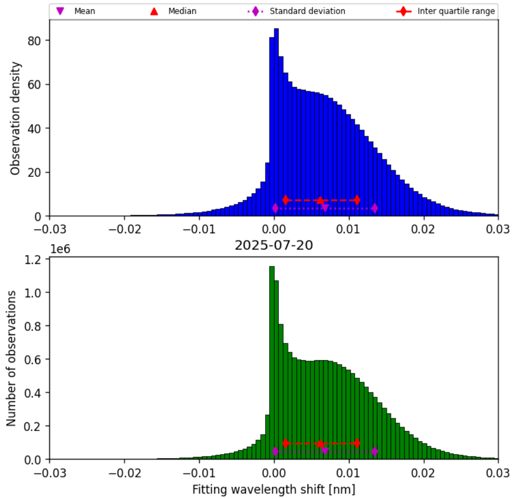
Figure 47: Histogram of “Fitting wavelength shift” for 2025-07-20 to 2025-07-21
