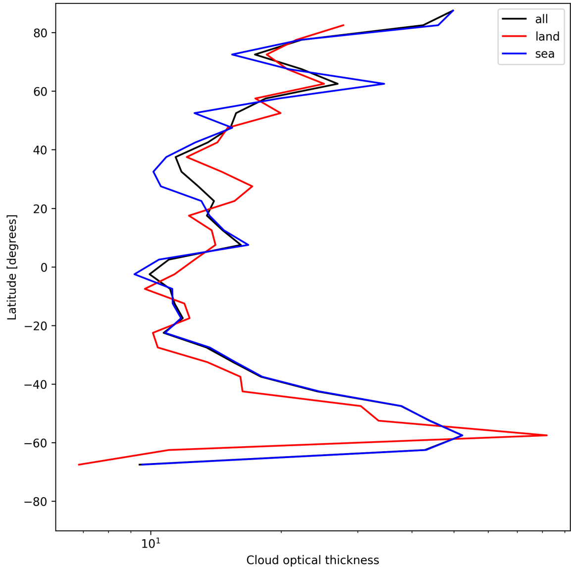
Figure 23: Zonal average of “Cloud optical thickness” for 2025-07-20 to 2025-07-21.
