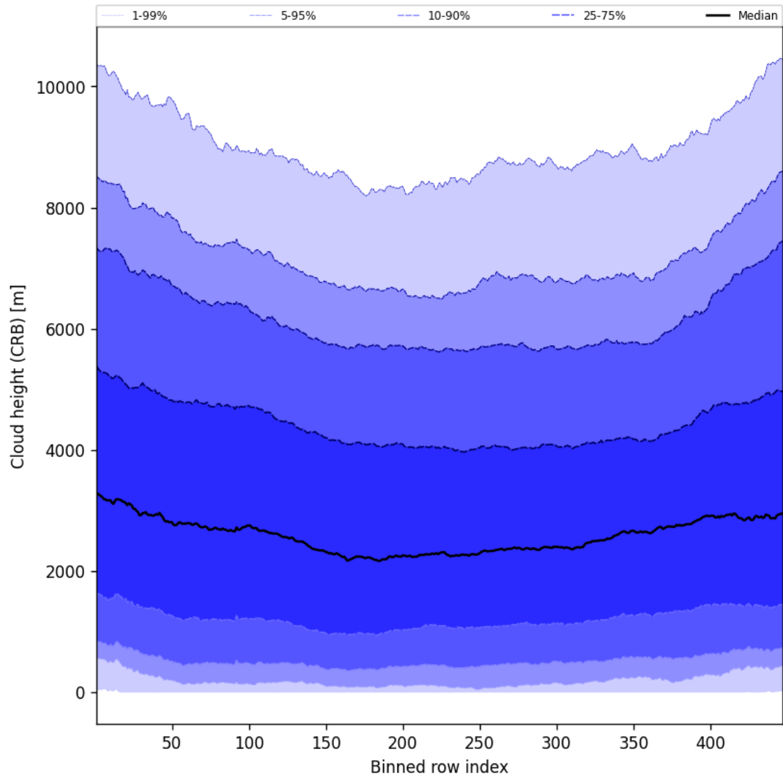
Figure 57: Along track statistics of “Cloud height (CRB)” for 2025-07-20 to 2025-07-21
