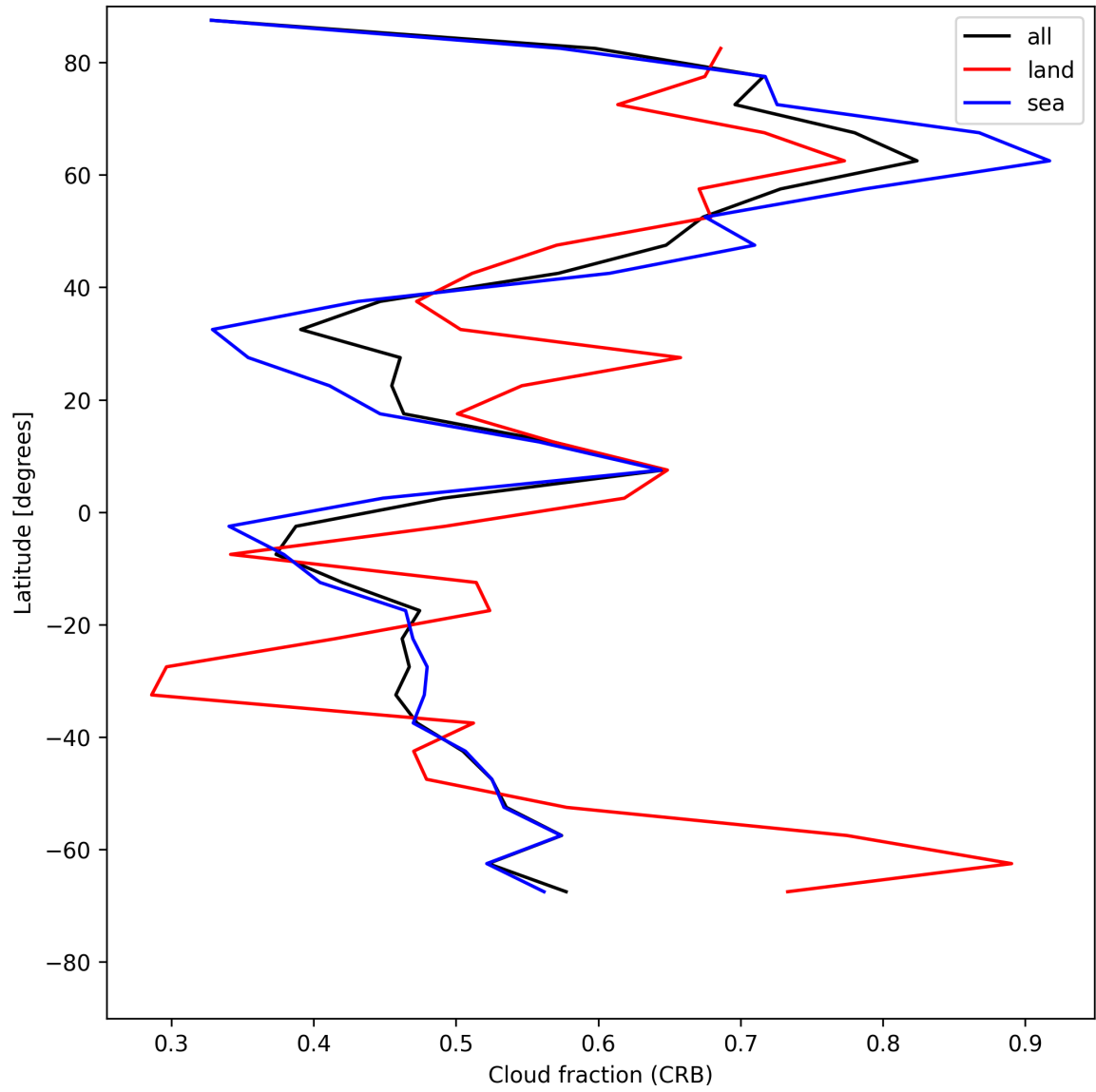
Figure 24: Zonal average of “Cloud fraction (CRB)” for 2025-07-20 to 2025-07-21.
