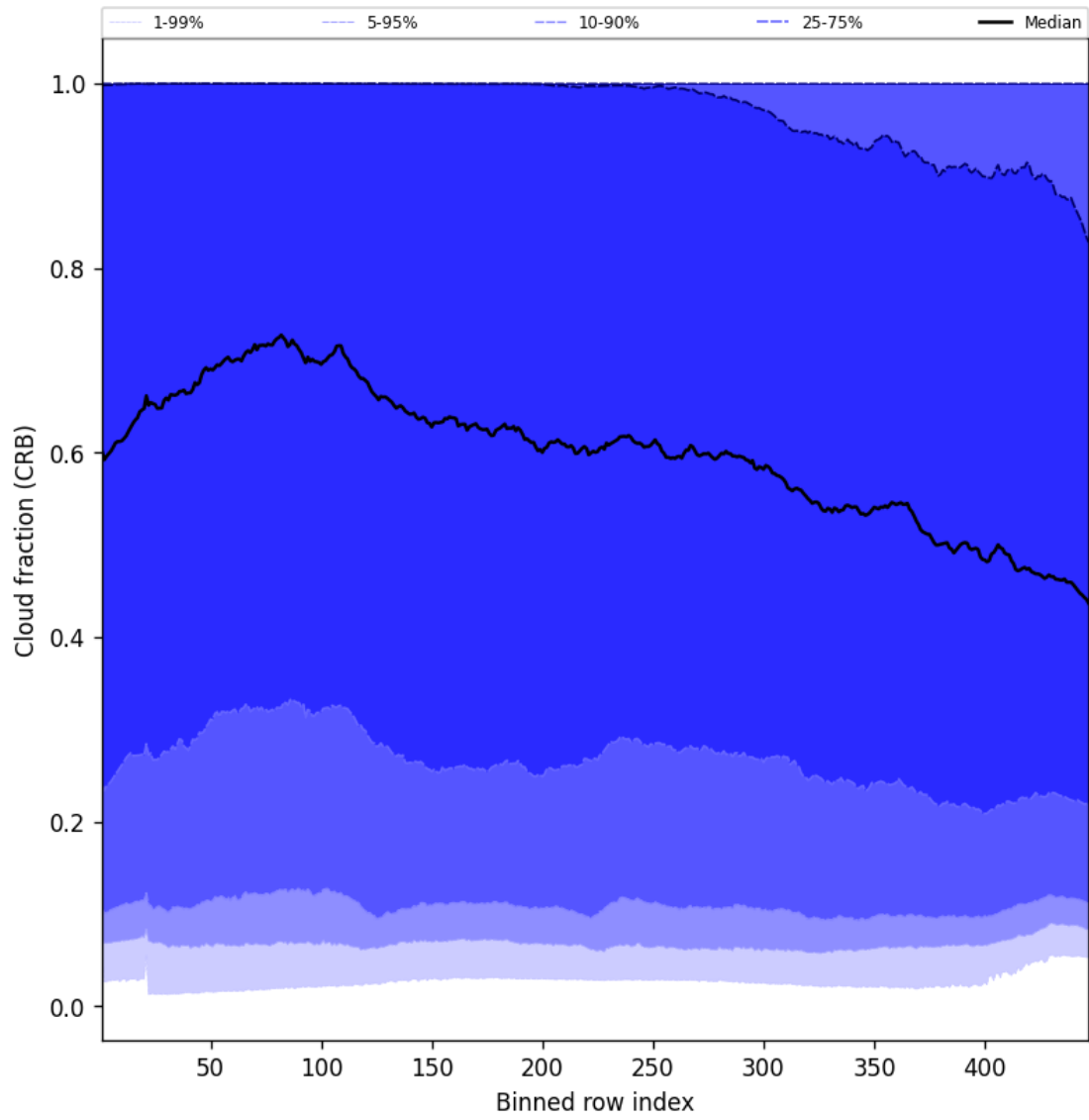
Figure 56: Along track statistics of “Cloud fraction (CRB)” for 2025-07-20 to 2025-07-21
