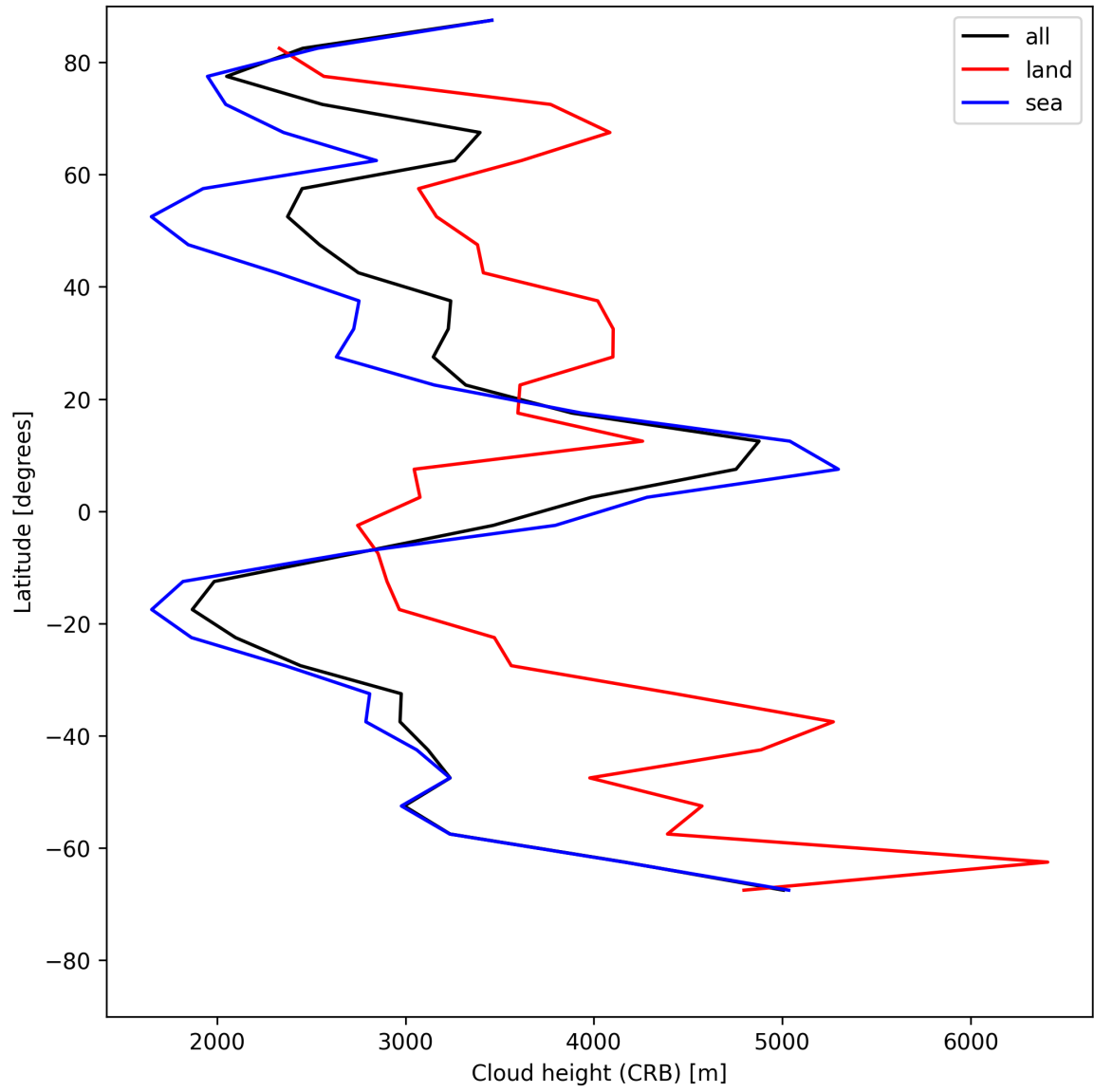
Figure 25: Zonal average of “Cloud height (CRB)” for 2025-07-20 to 2025-07-21.
