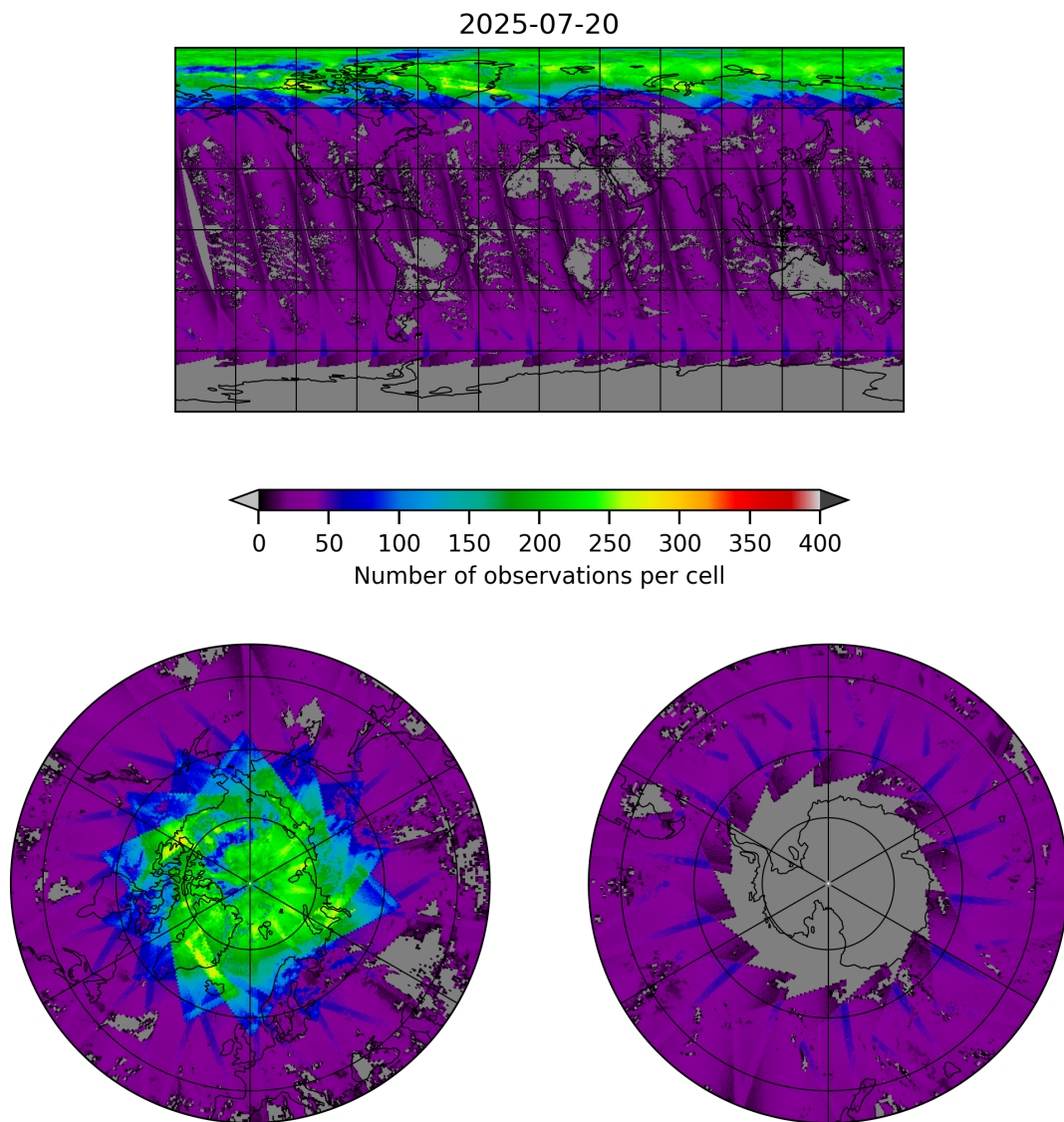
Figure 19: Map of the number of observations for 2025-07-20 to 2025-07-21
