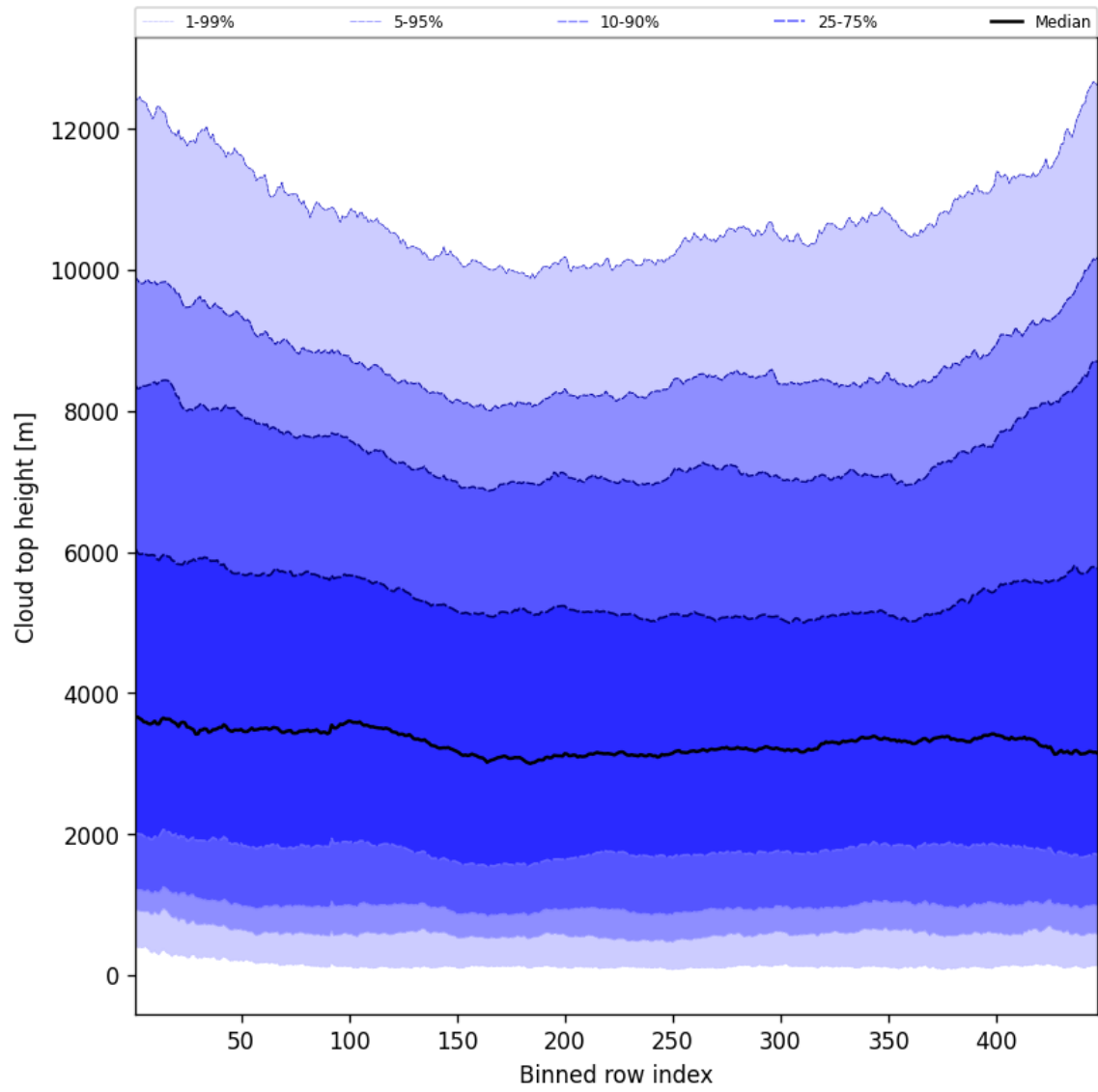
Figure 54: Along track statistics of “Cloud top height” for 2025-07-20 to 2025-07-21
