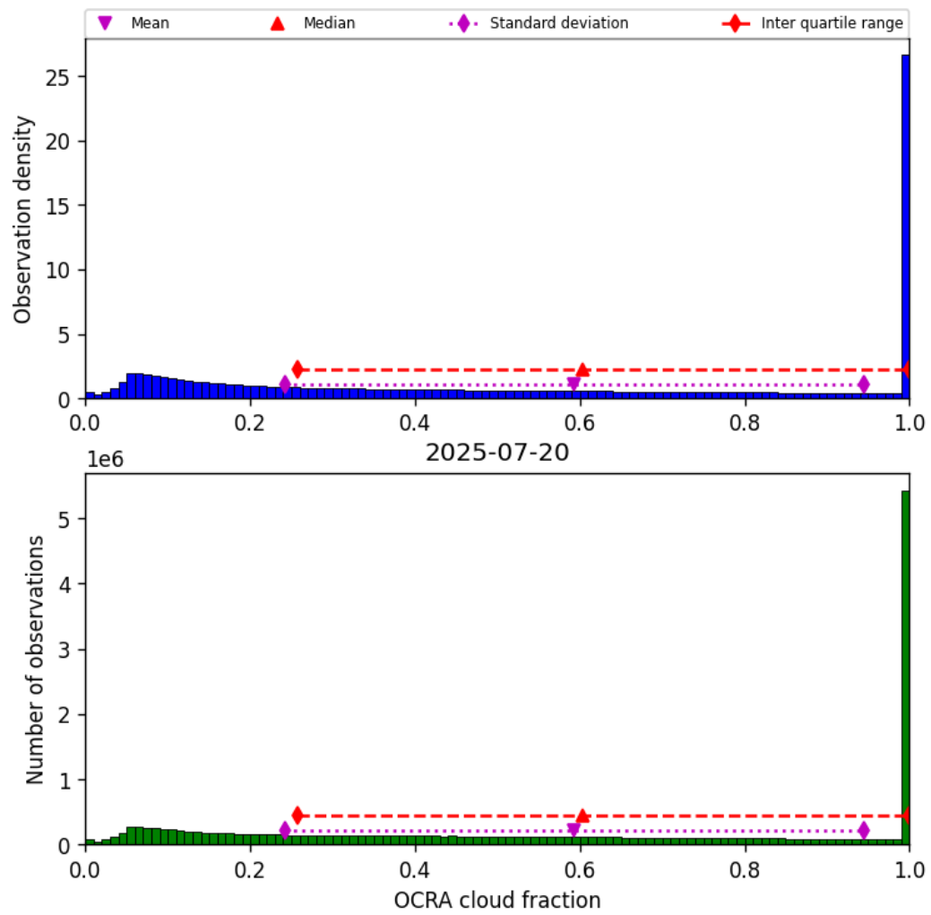
Figure 48: Histogram of “OCRA cloud fraction” for 2025-07-20 to 2025-07-21
