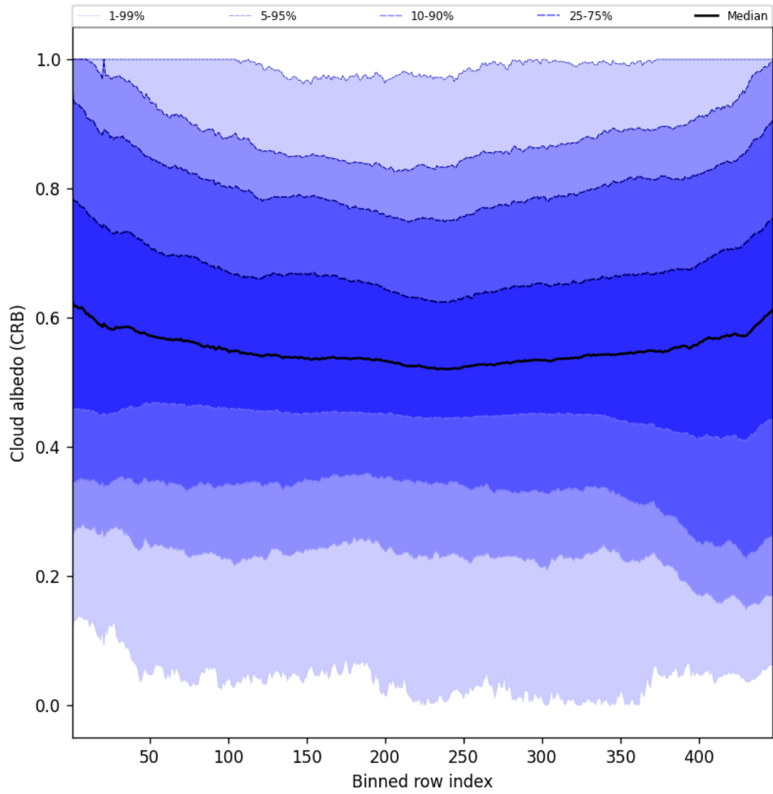
Figure 58: Along track statistics of “Cloud albedo (CRB)” for 2025-07-20 to 2025-07-21
