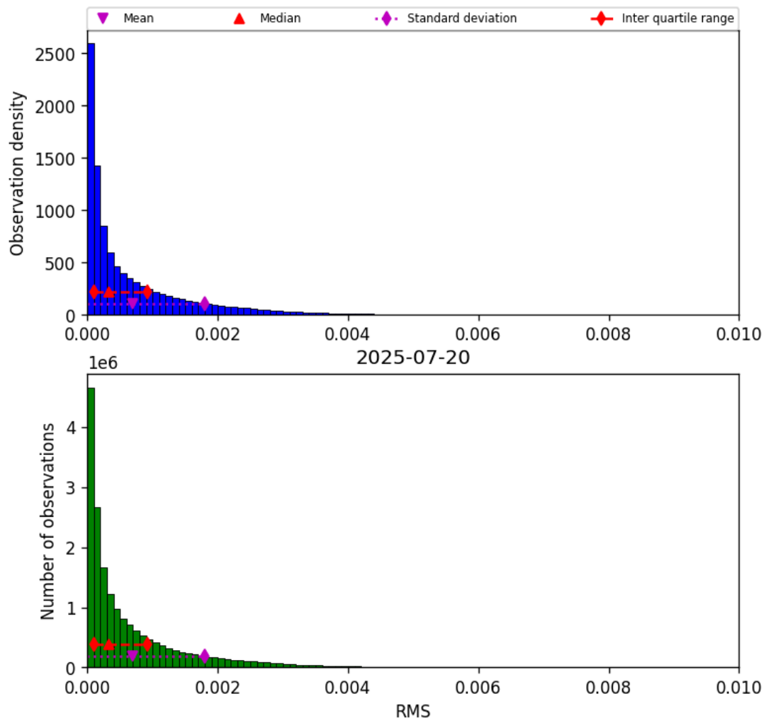
Figure 45: Histogram of “RMS” for 2025-07-20 to 2025-07-21
