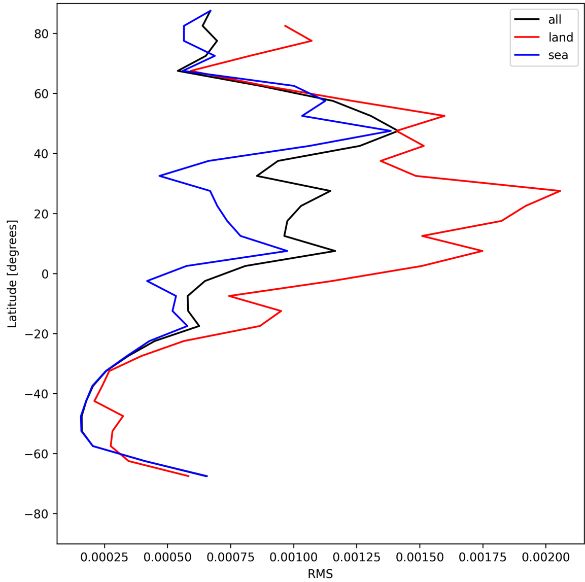
Figure 29: Zonal average of “RMS” for 2025-07-20 to 2025-07-21.
