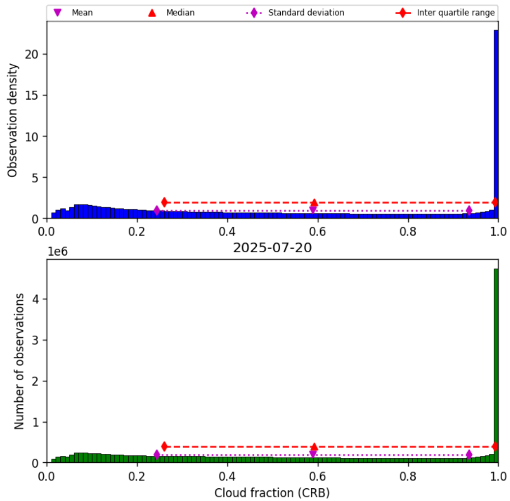
Figure 40: Histogram of “Cloud fraction (CRB)” for 2025-07-20 to 2025-07-21
