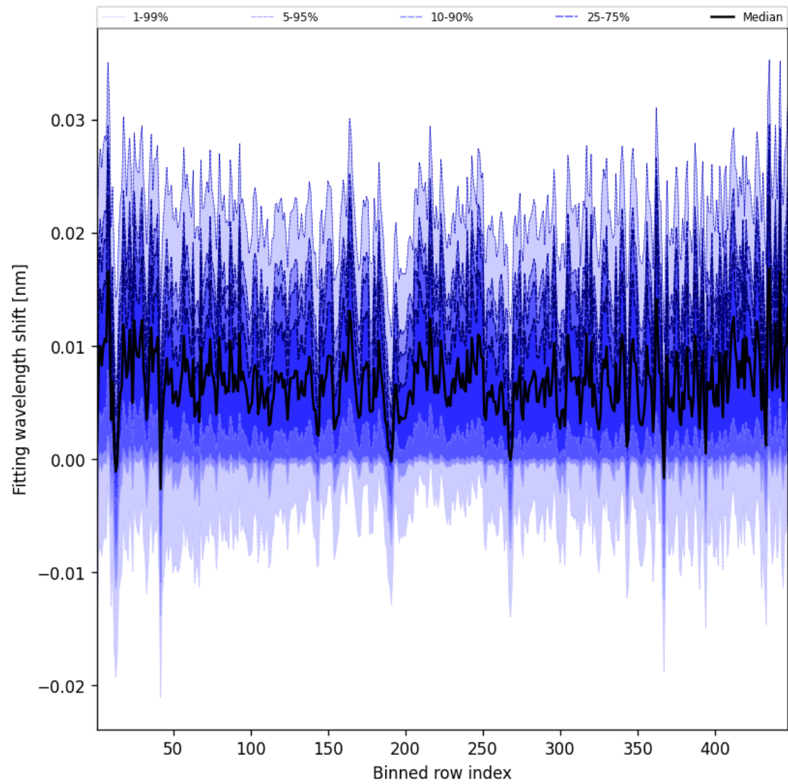
Figure 63: Along track statistics of “Fitting wavelength shift” for 2025-07-20 to 2025-07-21
