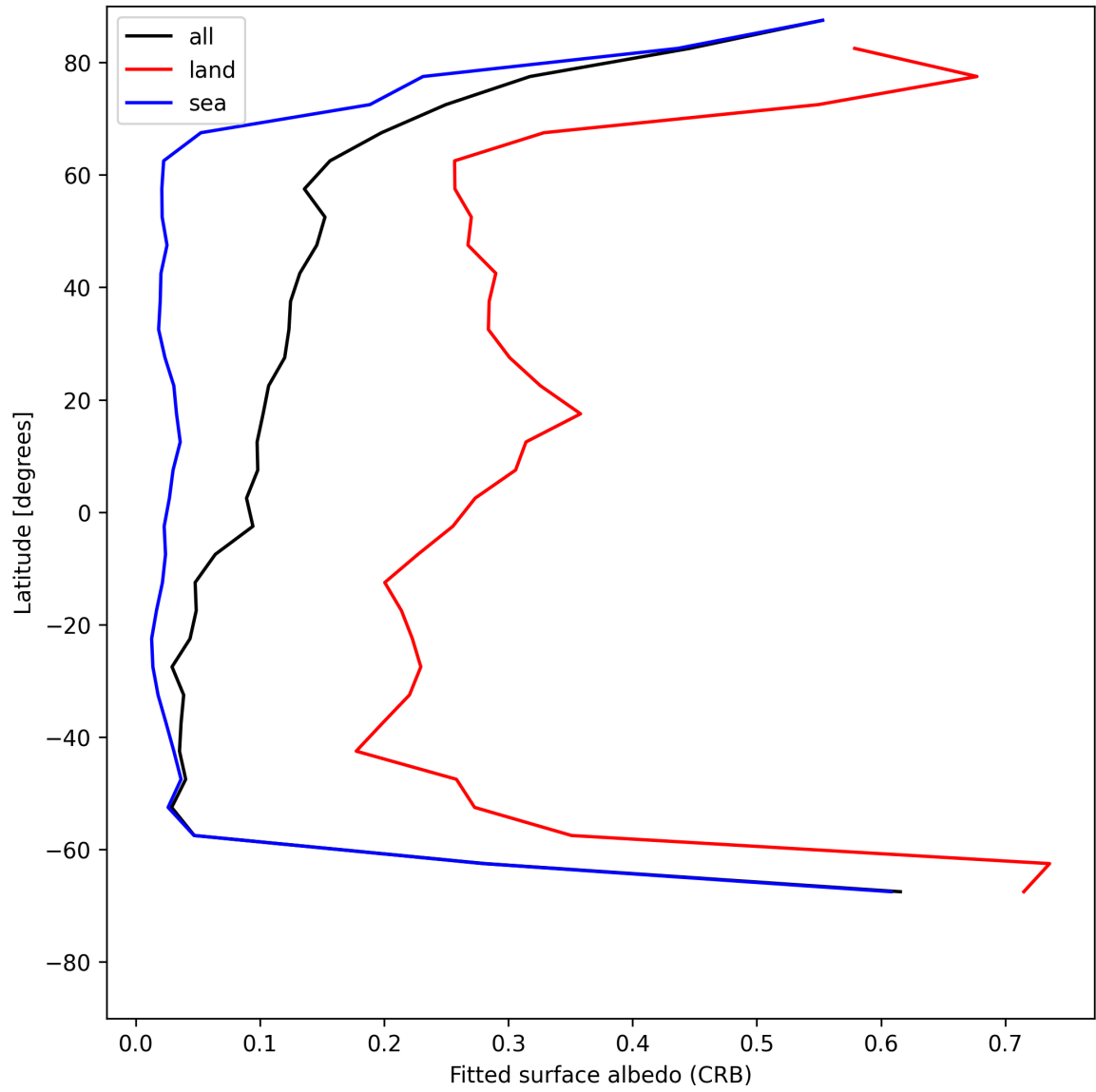
Figure 28: Zonal average of “Fitted surface albedo (CRB)” for 2025-07-20 to 2025-07-21.
