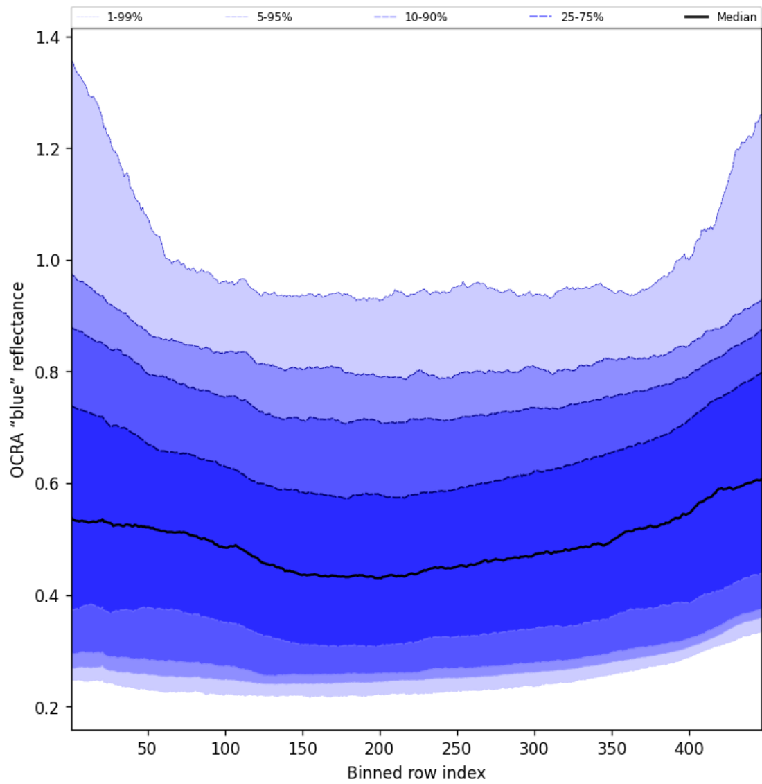
Figure 65: Along track statistics of “OCRA “blue” reflectance” for 2025-07-20 to 2025-07-21
