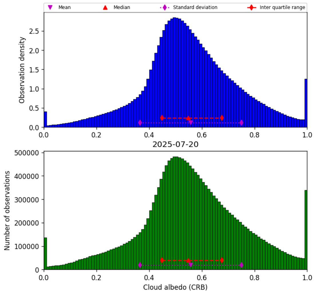
Figure 42: Histogram of “Cloud albedo (CRB)” for 2025-07-20 to 2025-07-21
