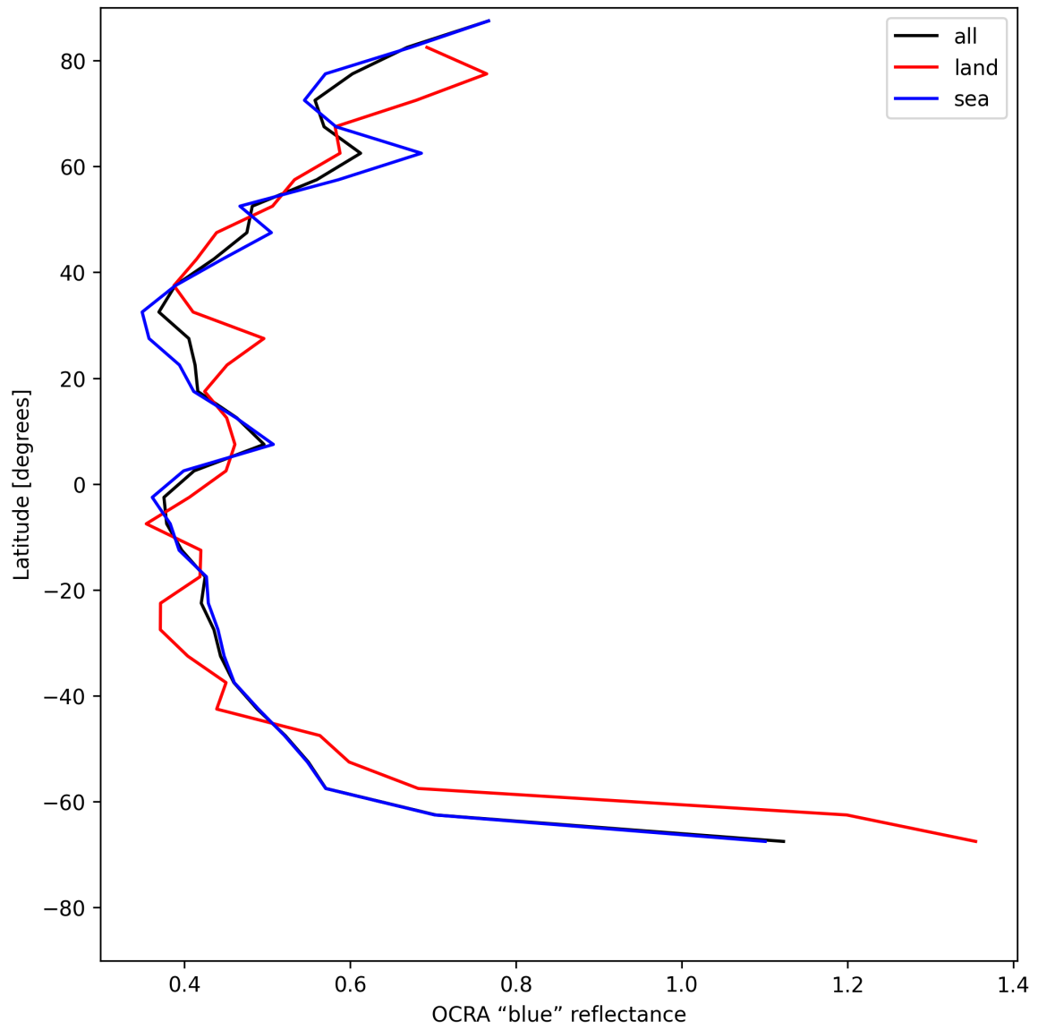
Figure 33: Zonal average of “OCRA “blue” reflectance” for 2025-07-20 to 2025-07-21.
