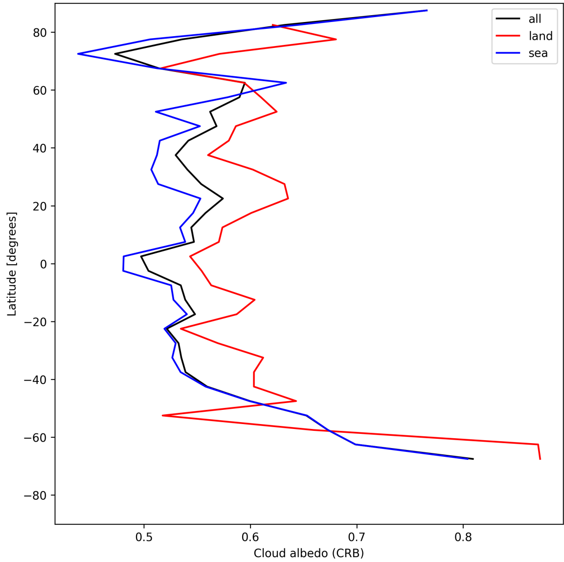
Figure 26: Zonal average of “Cloud albedo (CRB)” for 2025-07-20 to 2025-07-21.
