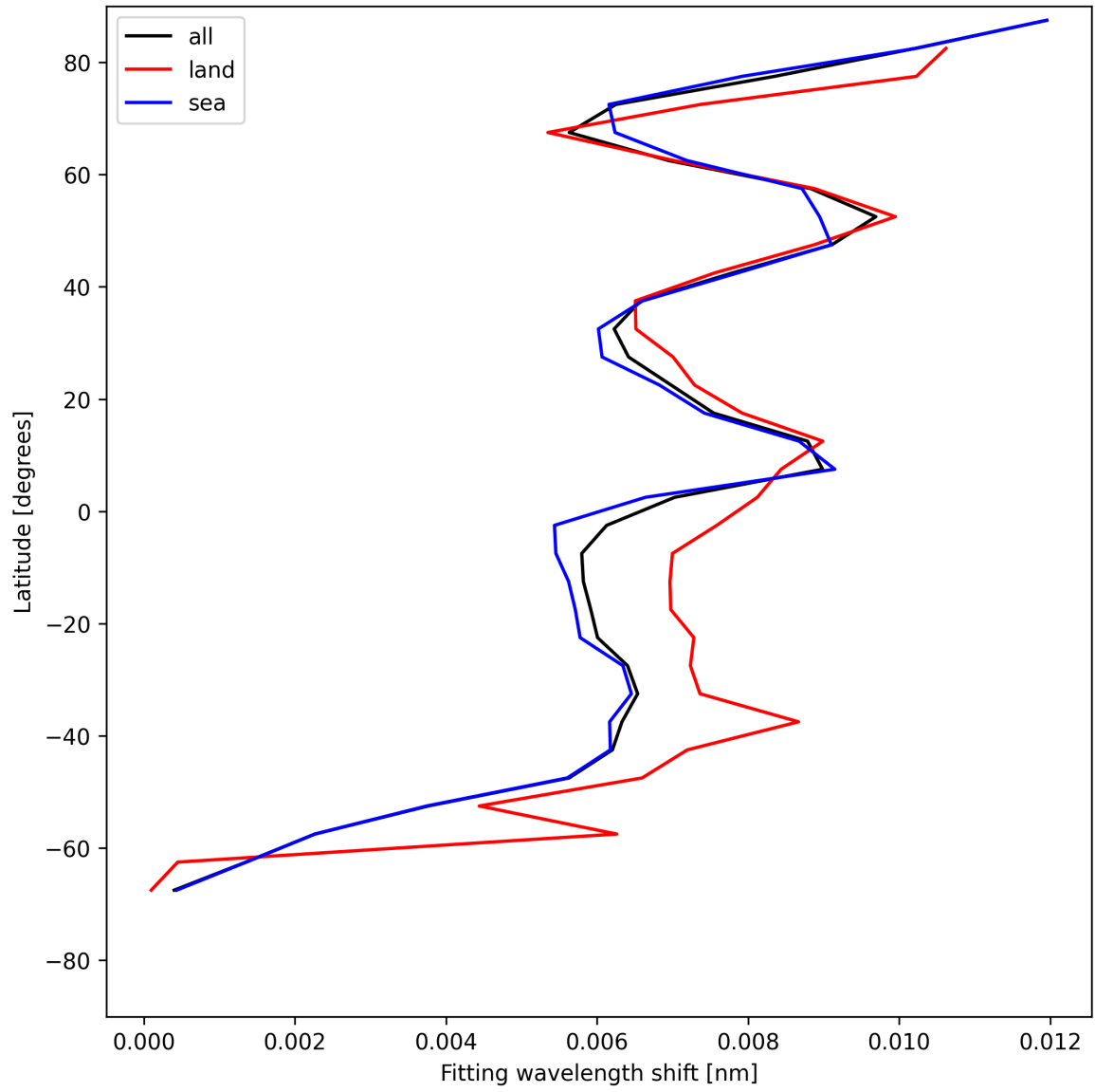
Figure 31: Zonal average of “Fitting wavelength shift” for 2025-07-20 to 2025-07-21.
