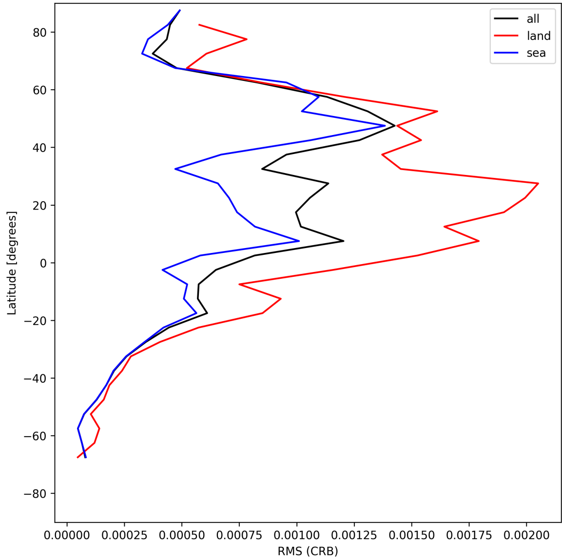
Figure 30: Zonal average of “RMS (CRB)” for 2025-07-20 to 2025-07-21.
