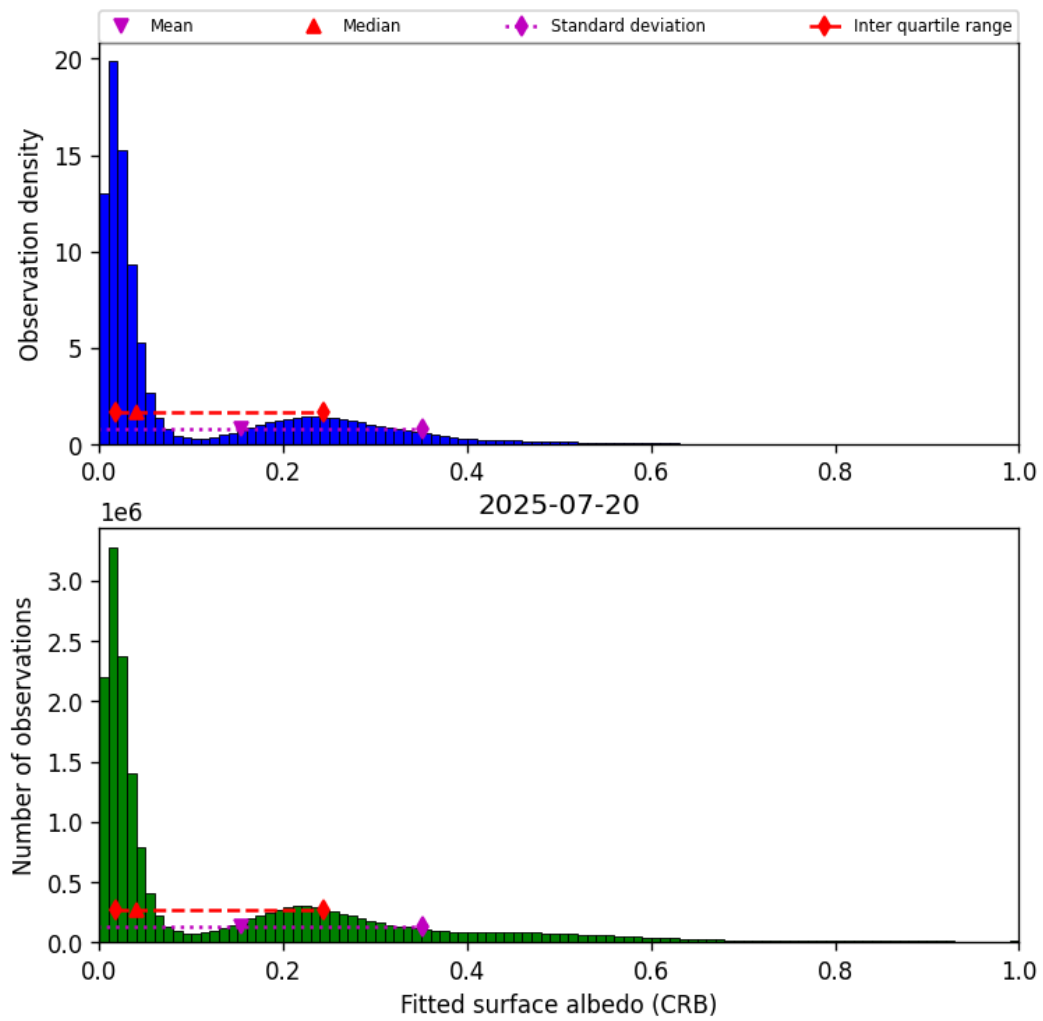
Figure 44: Histogram of “Fitted surface albedo (CRB)” for 2025-07-20 to 2025-07-21
