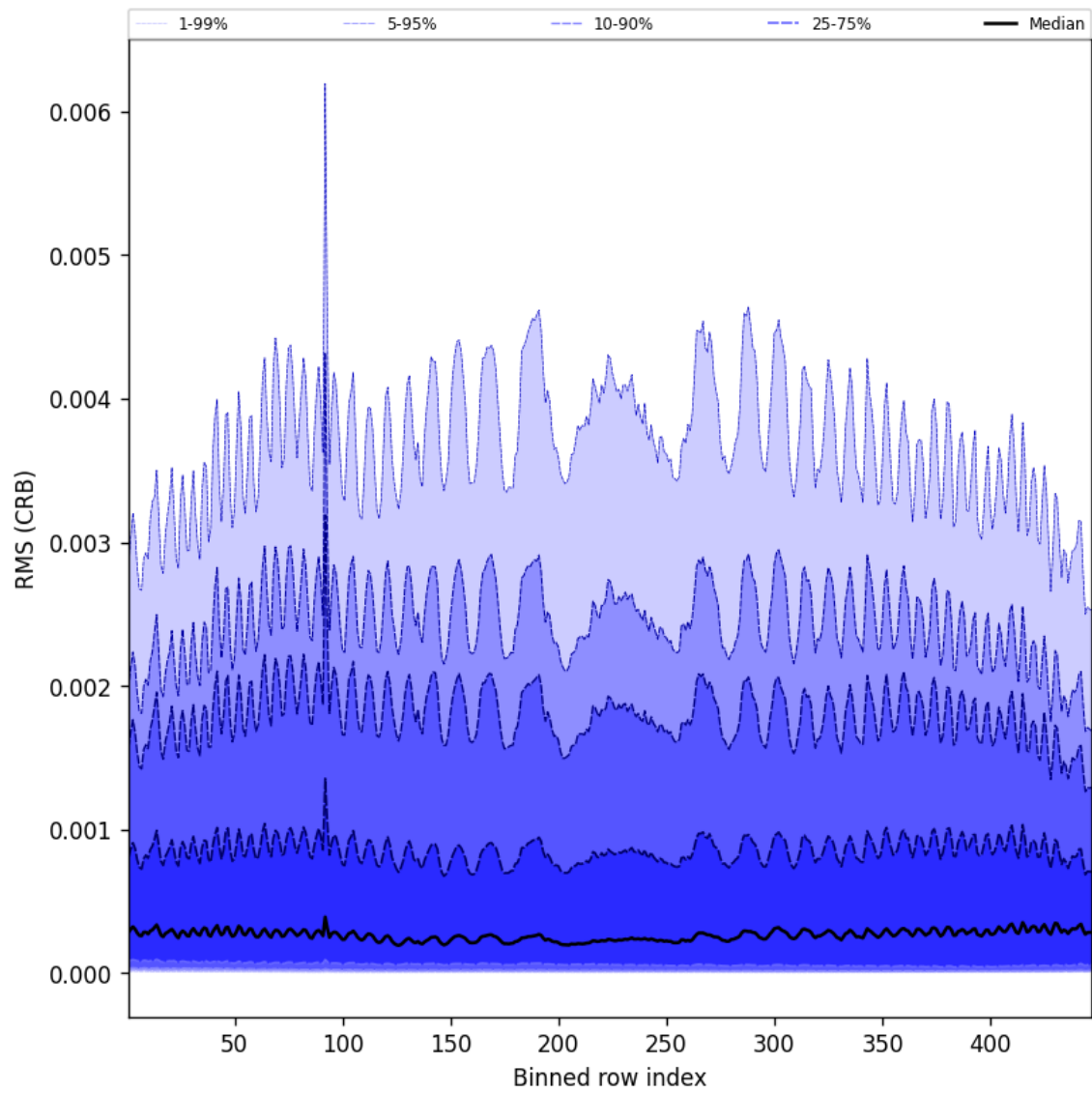
Figure 62: Along track statistics of “RMS (CRB)” for 2025-07-20 to 2025-07-21
