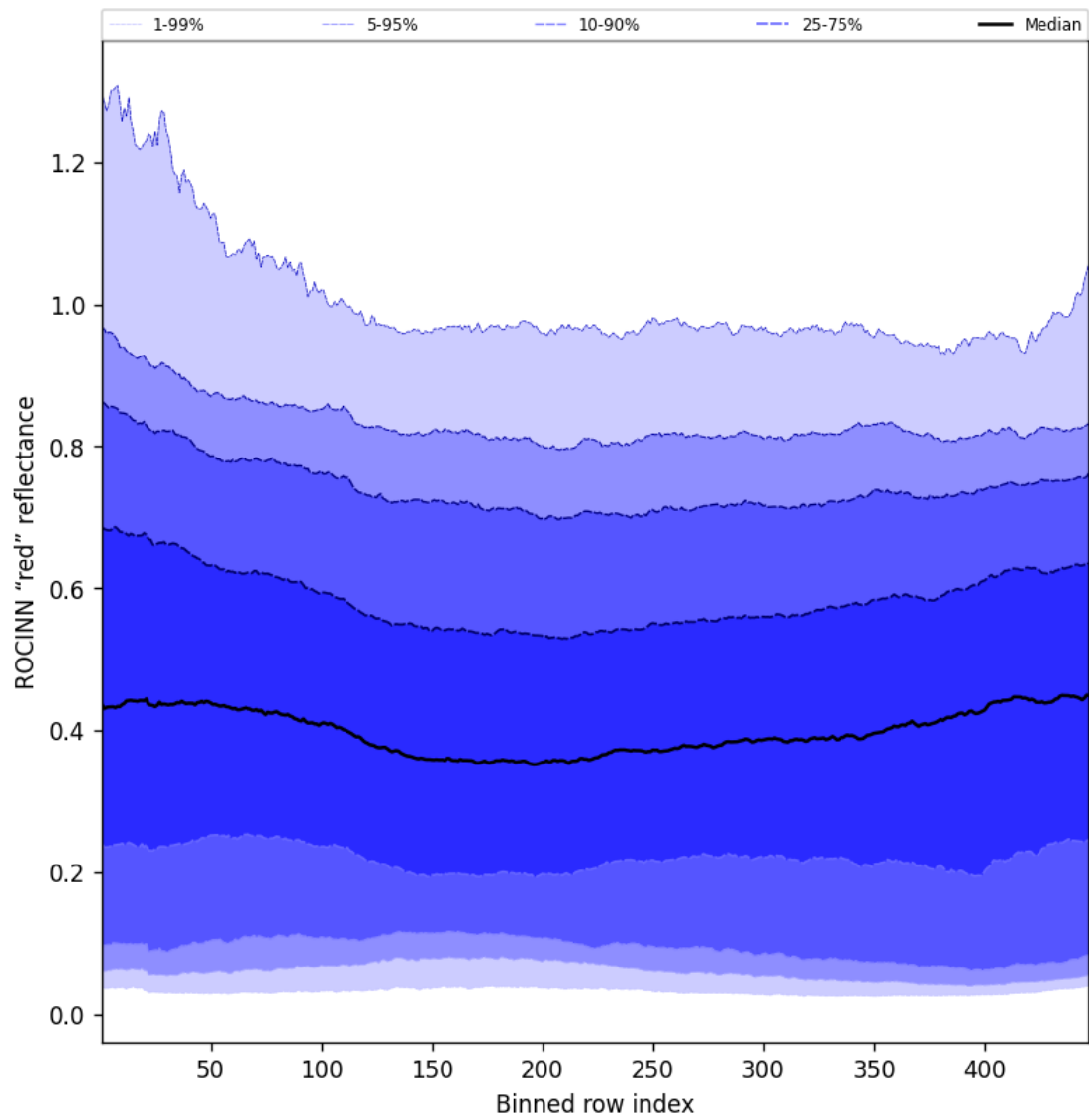
Figure 67: Along track statistics of "ROCINN "red" reflectance" for 2025-07-20 to 2025-07-21
