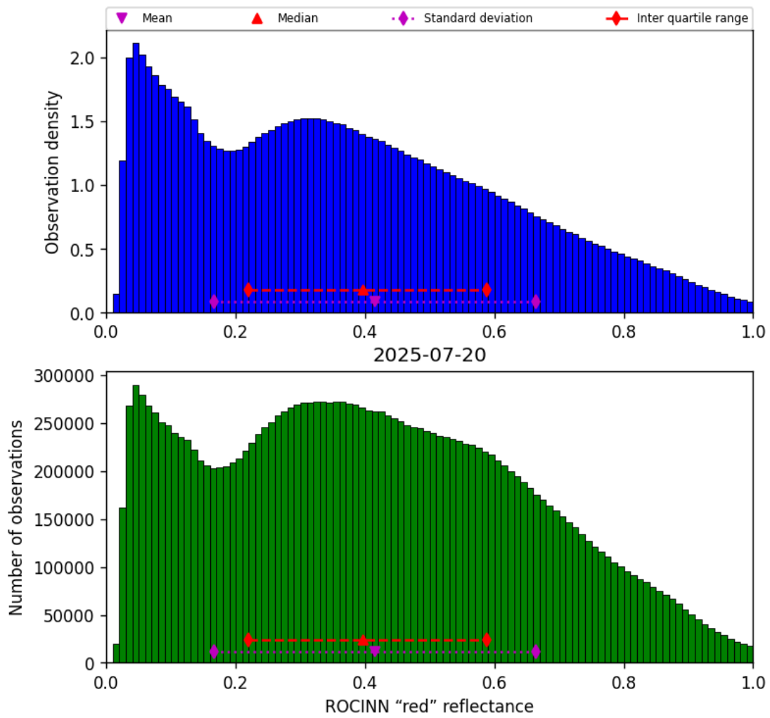
Figure 51: Histogram of “ROCINN “red” reflectance” for 2025-07-20 to 2025-07-21
