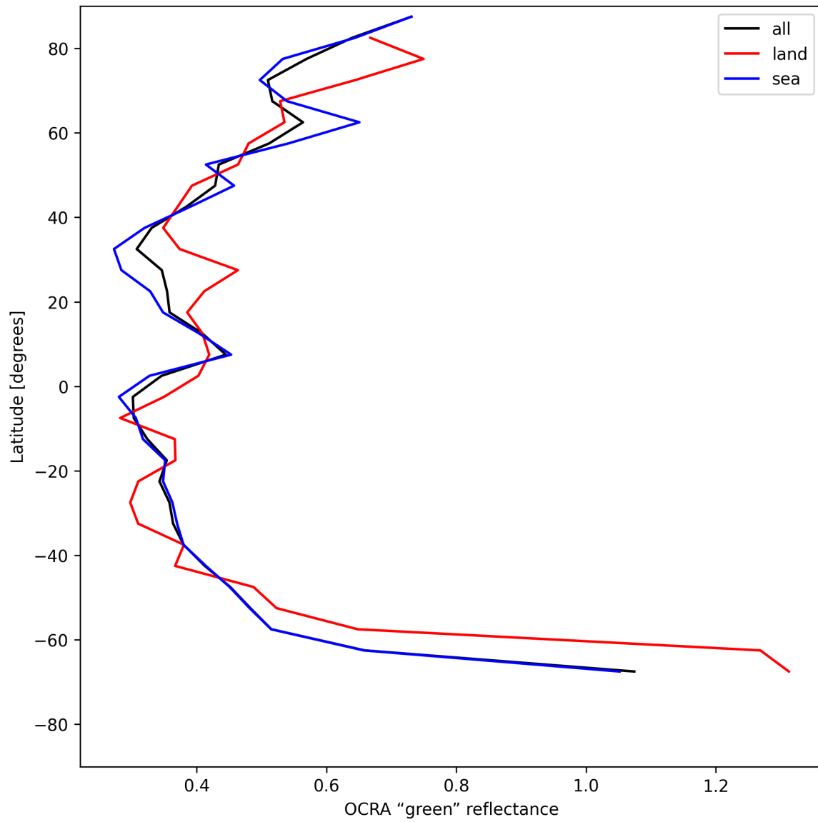
Figure 34: Zonal average of “OCRA “green” reflectance” for 2025-07-20 to 2025-07-21.
