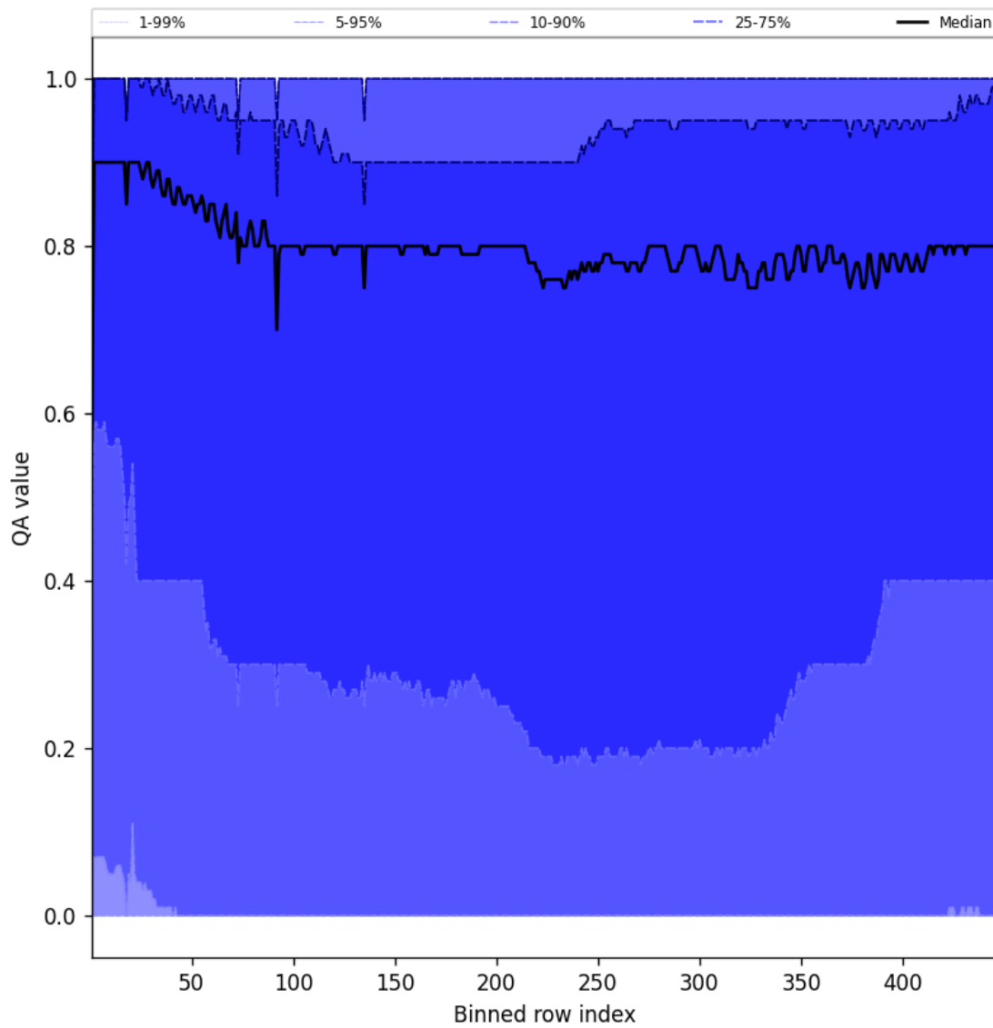
Figure 52: Along track statistics of “QA value” for 2025-07-20 to 2025-07-21
