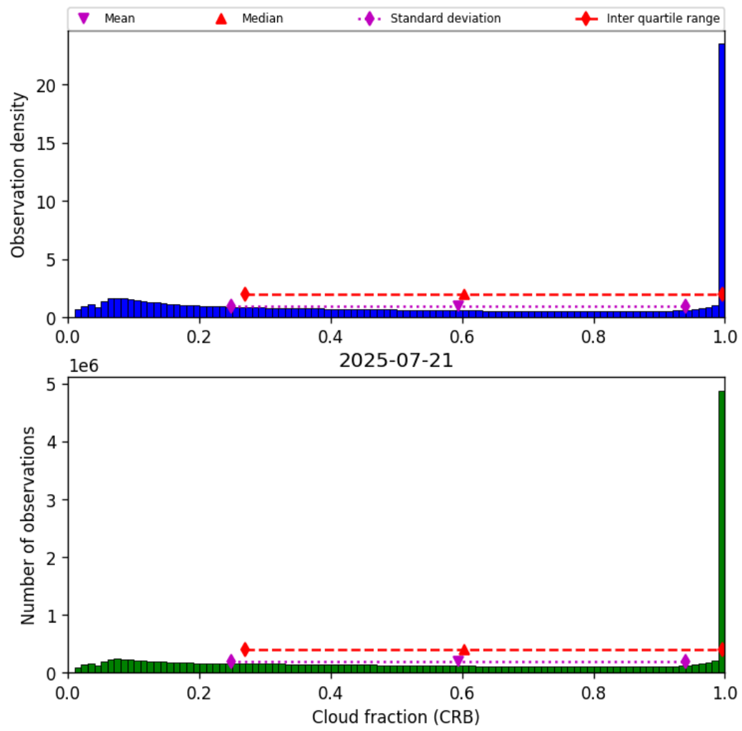
Figure 40: Histogram of “Cloud fraction (CRB)” for 2025-07-21 to 2025-07-22
