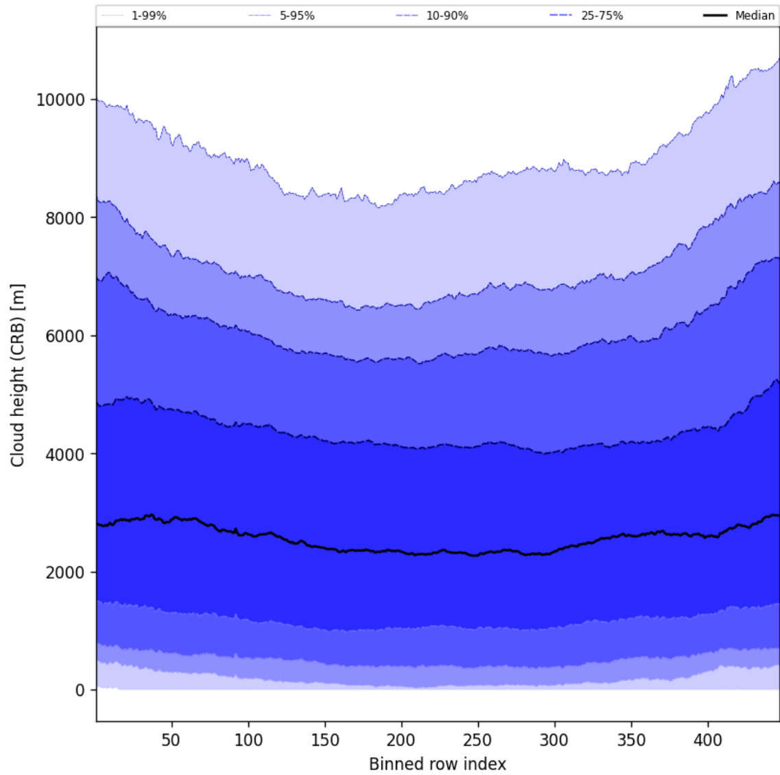
Figure 57: Along track statistics of “Cloud height (CRB)” for 2025-07-21 to 2025-07-22
