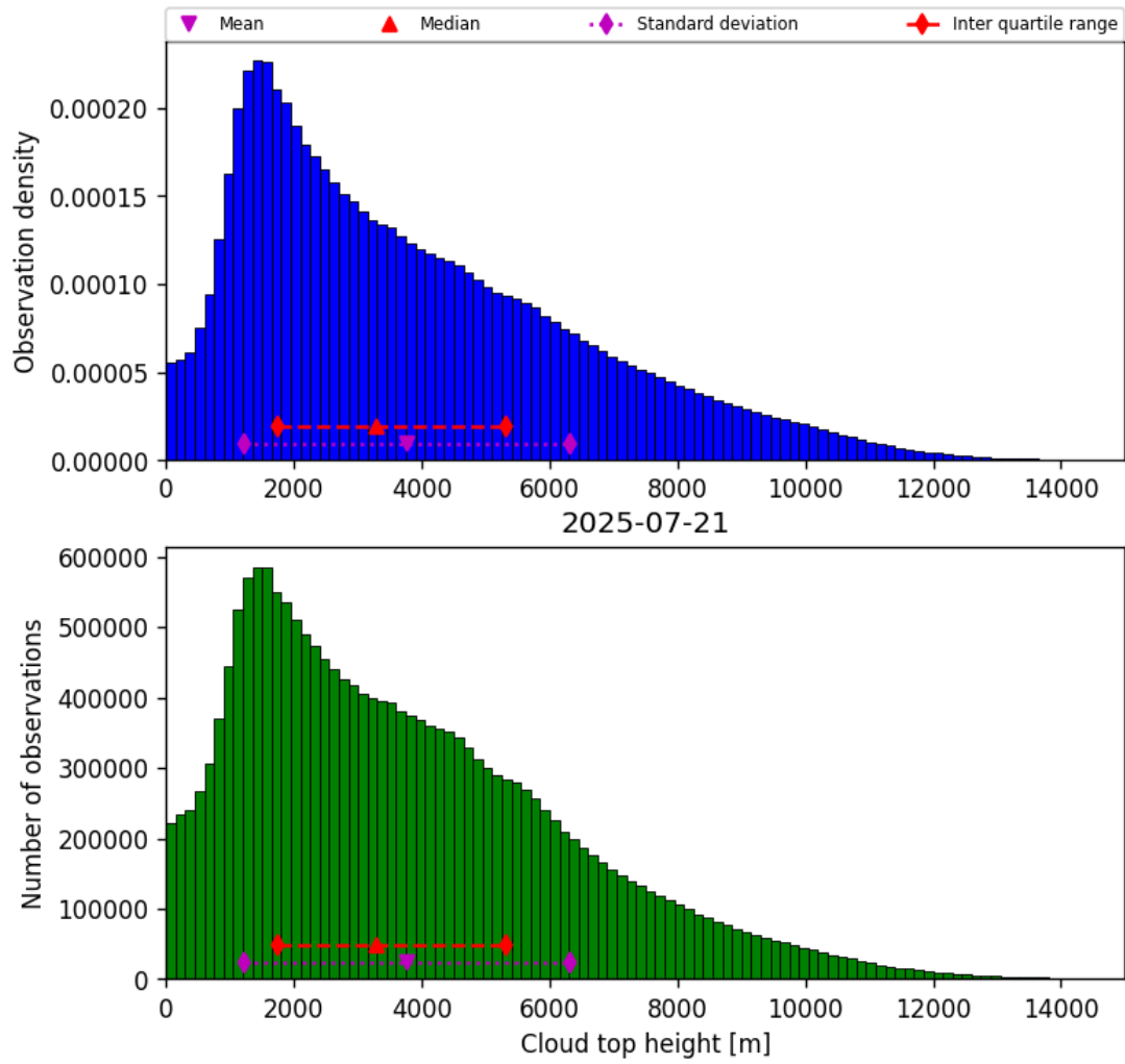
Figure 38: Histogram of “Cloud top height” for 2025-07-21 to 2025-07-22
