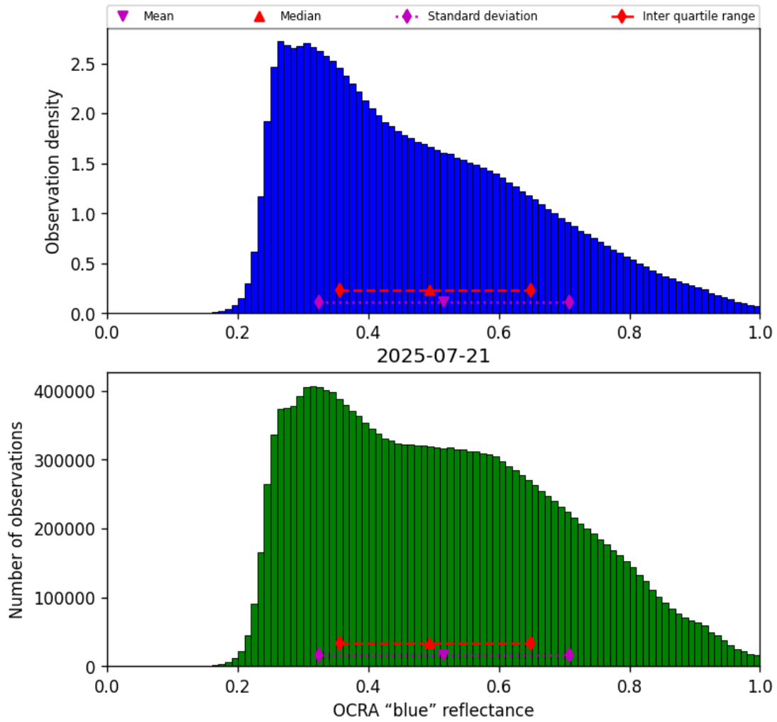
Figure 49: Histogram of “OCRA “blue” reflectance” for 2025-07-21 to 2025-07-22
