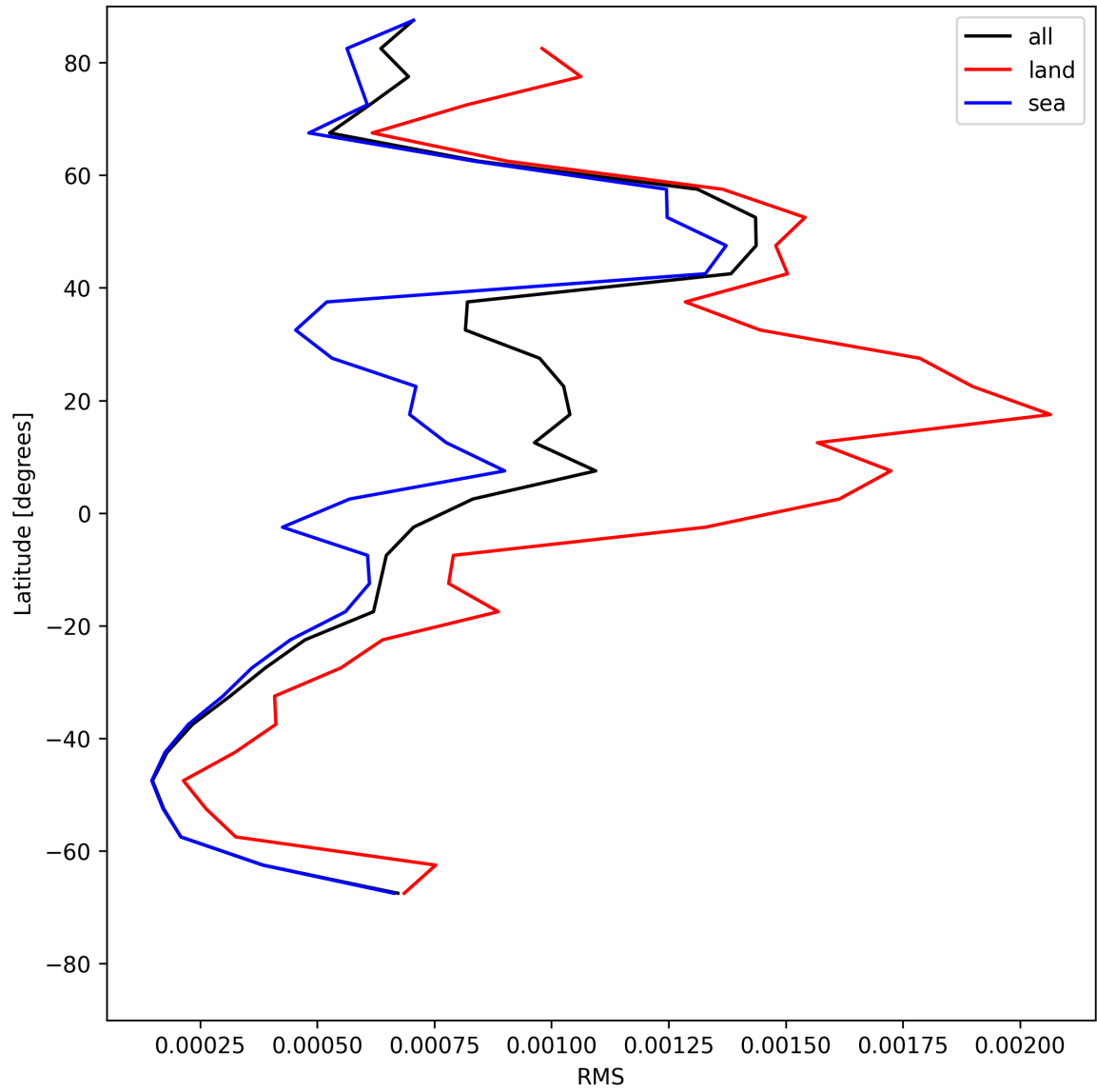
Figure 29: Zonal average of “RMS” for 2025-07-21 to 2025-07-22.
