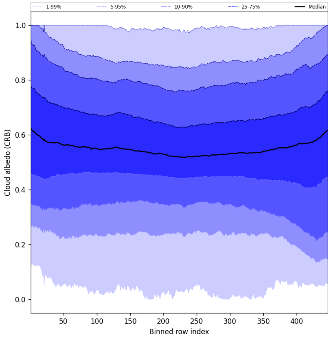
Figure 58: Along track statistics of “Cloud albedo (CRB)” for 2025-07-21 to 2025-07-22
