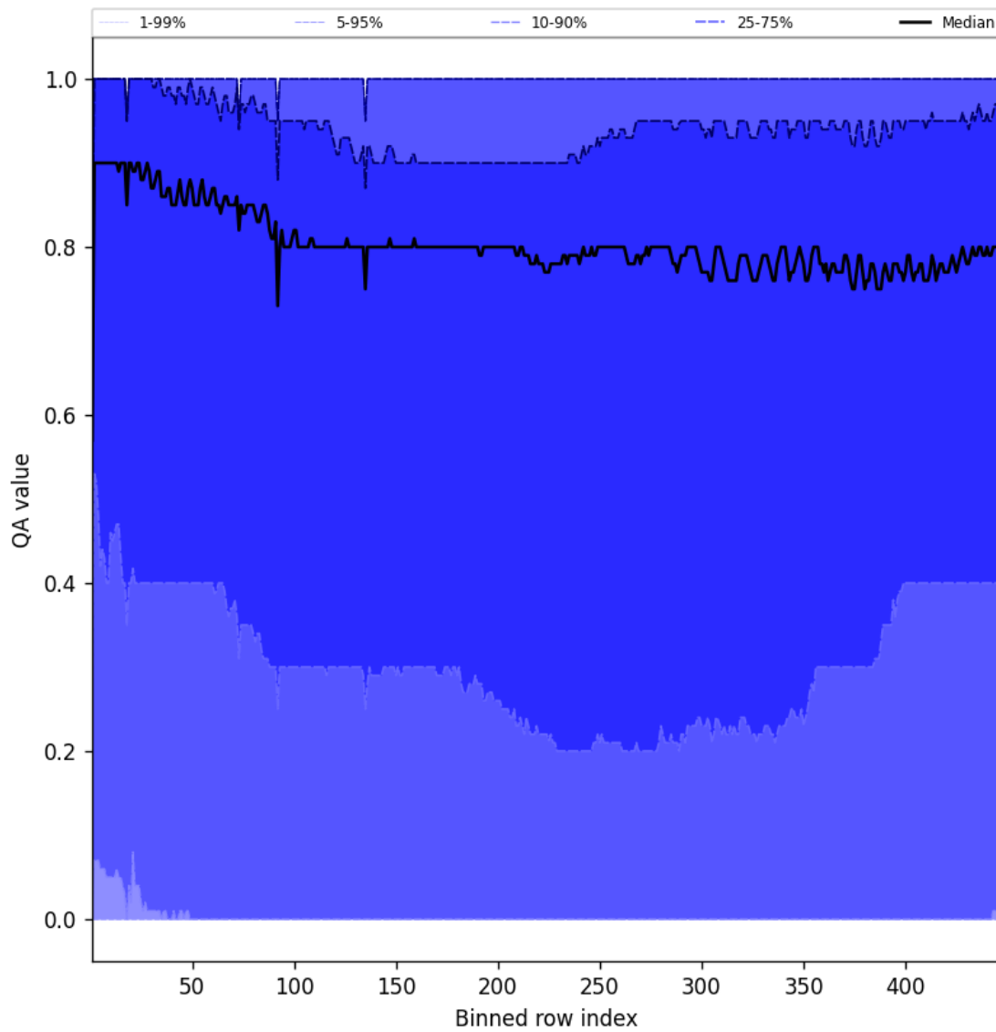
Figure 52: Along track statistics of “QA value” for 2025-07-21 to 2025-07-22
