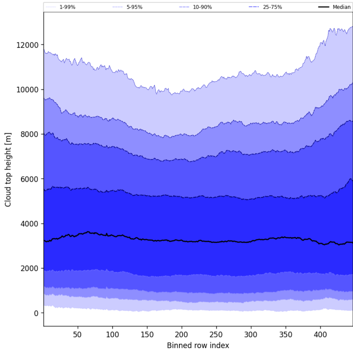
Figure 54: Along track statistics of “Cloud top height” for 2025-07-21 to 2025-07-22
