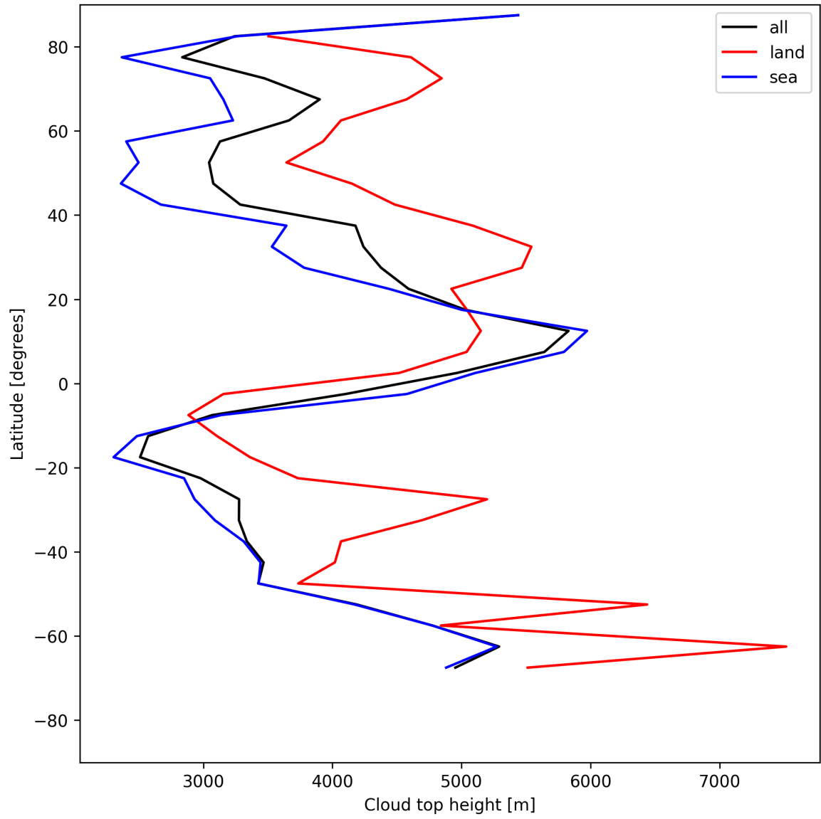
Figure 22: Zonal average of “Cloud top height” for 2025-07-21 to 2025-07-22.
