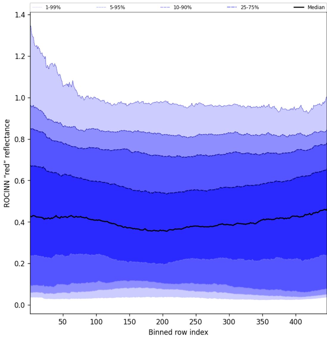
Figure 67: Along track statistics of "ROCINN "red" reflectance" for 2025-07-21 to 2025-07-22
