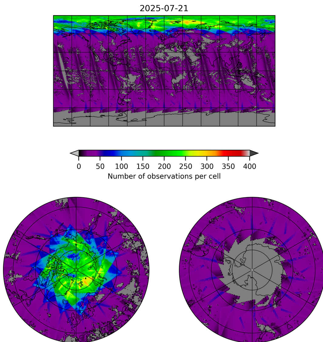
Figure 19: Map of the number of observations for 2025-07-21 to 2025-07-22
