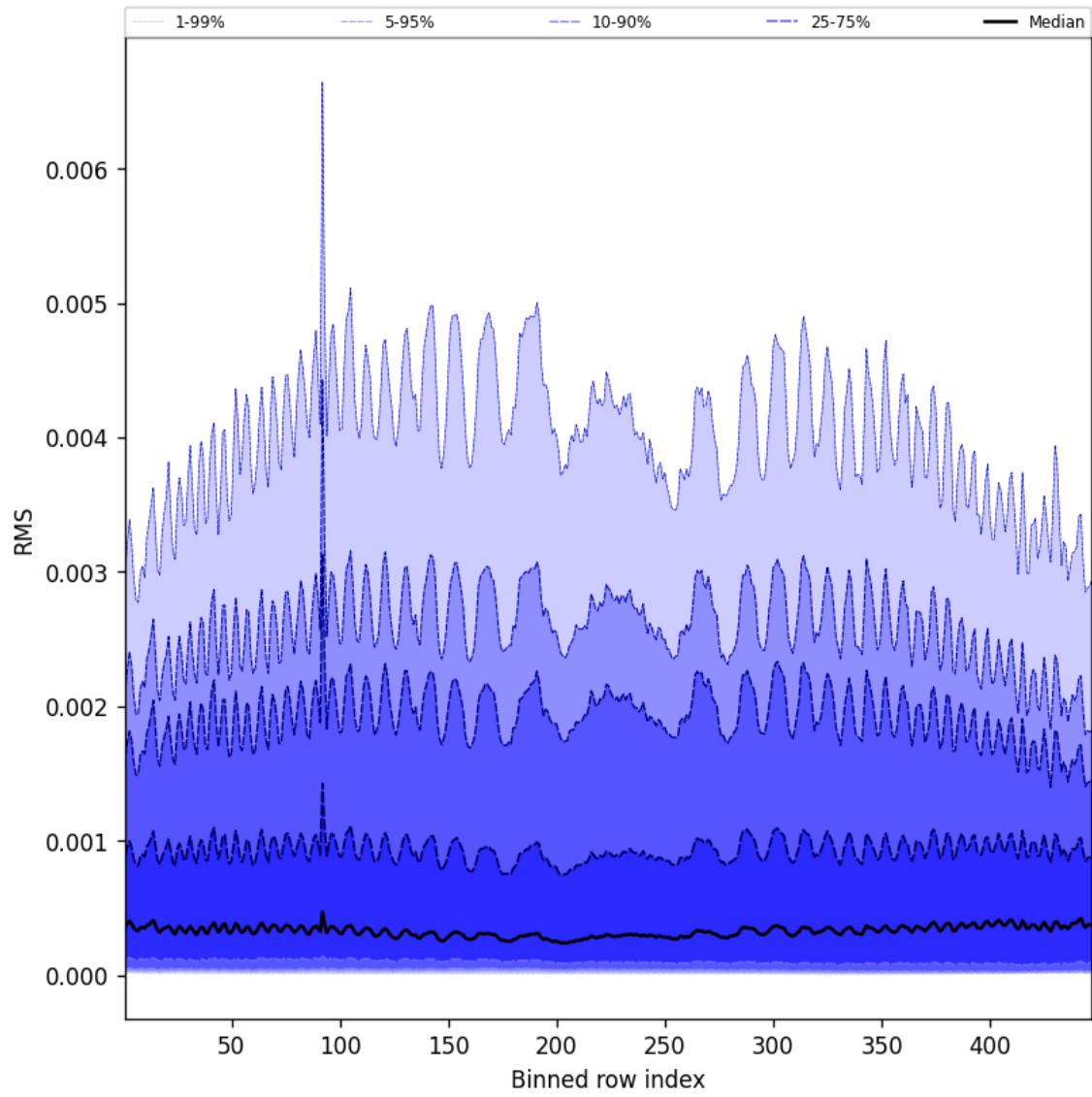
Figure 61: Along track statistics of “RMS” for 2025-07-21 to 2025-07-22
