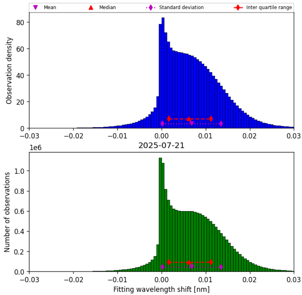
Figure 47: Histogram of “Fitting wavelength shift” for 2025-07-21 to 2025-07-22
