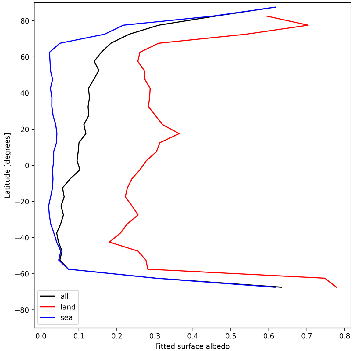
Figure 27: Zonal average of “Fitted surface albedo” for 2025-07-21 to 2025-07-22.
