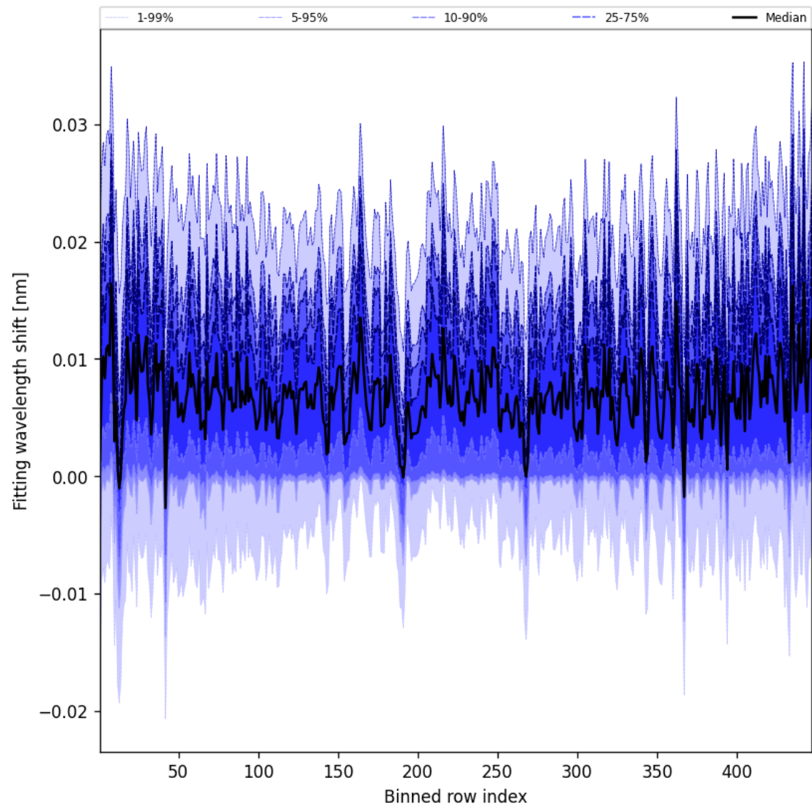
Figure 63: Along track statistics of “Fitting wavelength shift” for 2025-07-21 to 2025-07-22
