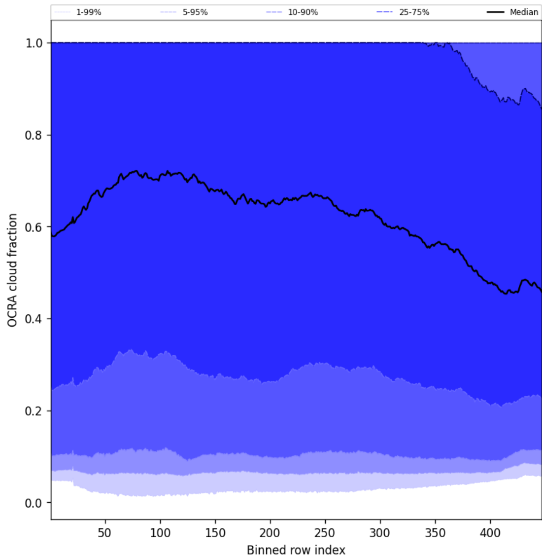
Figure 64: Along track statistics of “OCRA cloud fraction” for 2025-07-21 to 2025-07-22
