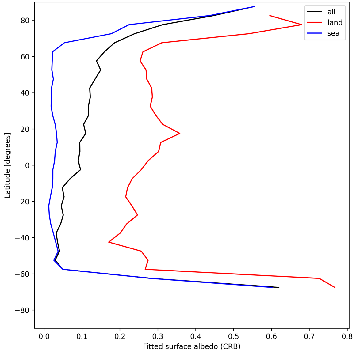
Figure 28: Zonal average of “Fitted surface albedo (CRB)” for 2025-07-21 to 2025-07-22.
