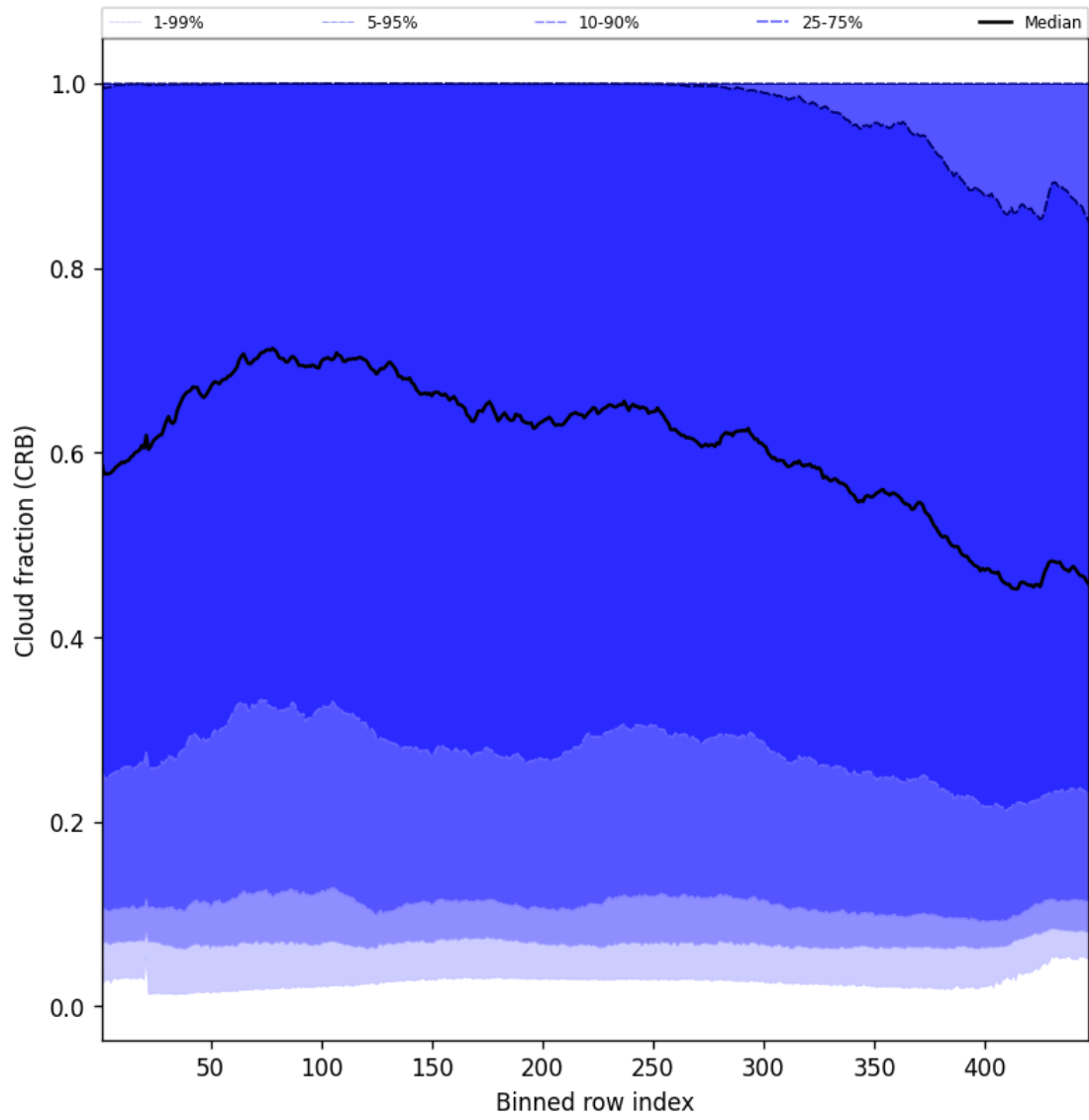
Figure 56: Along track statistics of “Cloud fraction (CRB)” for 2025-07-21 to 2025-07-22
