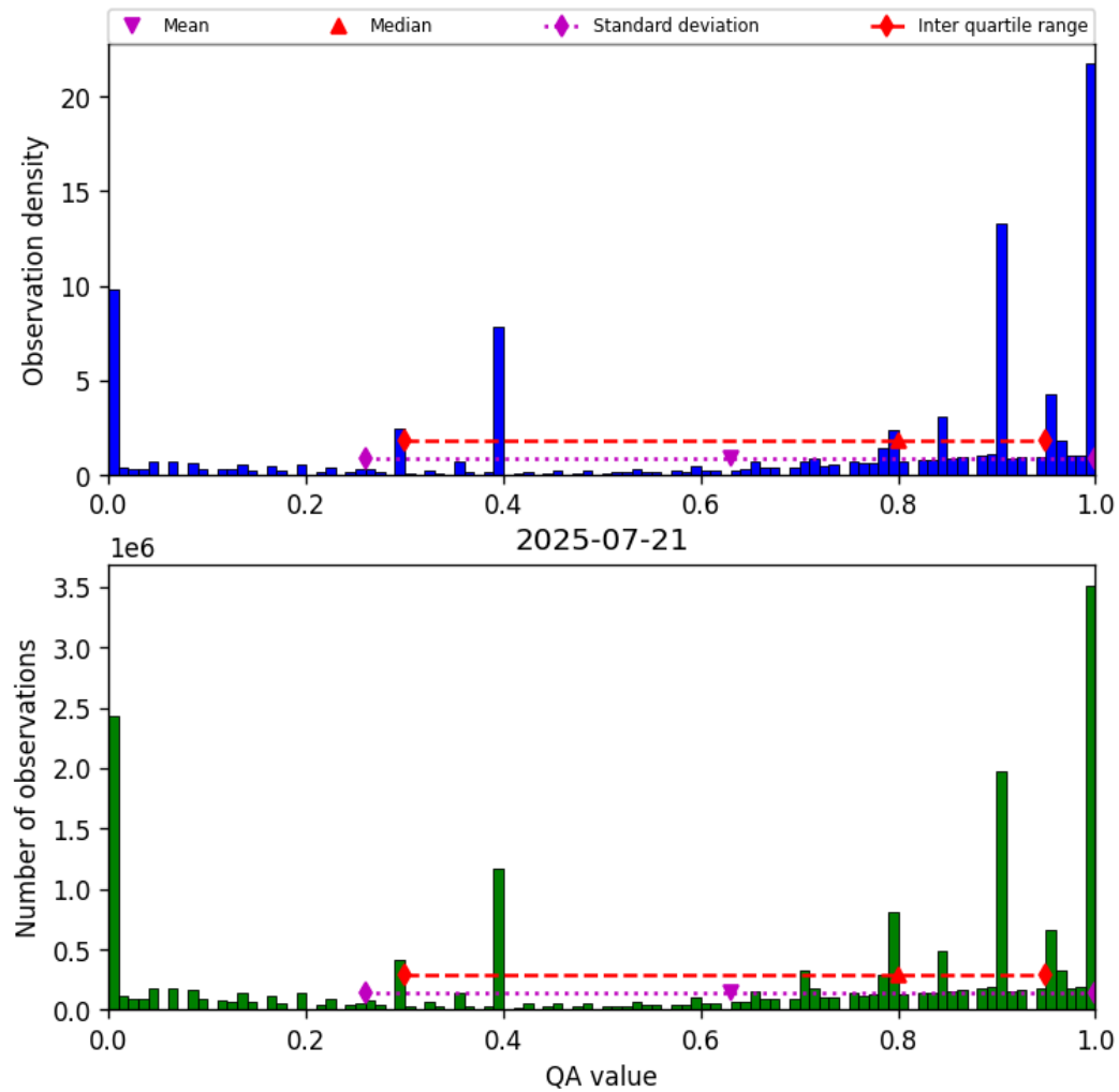
Figure 36: Histogram of “QA value” for 2025-07-21 to 2025-07-22
