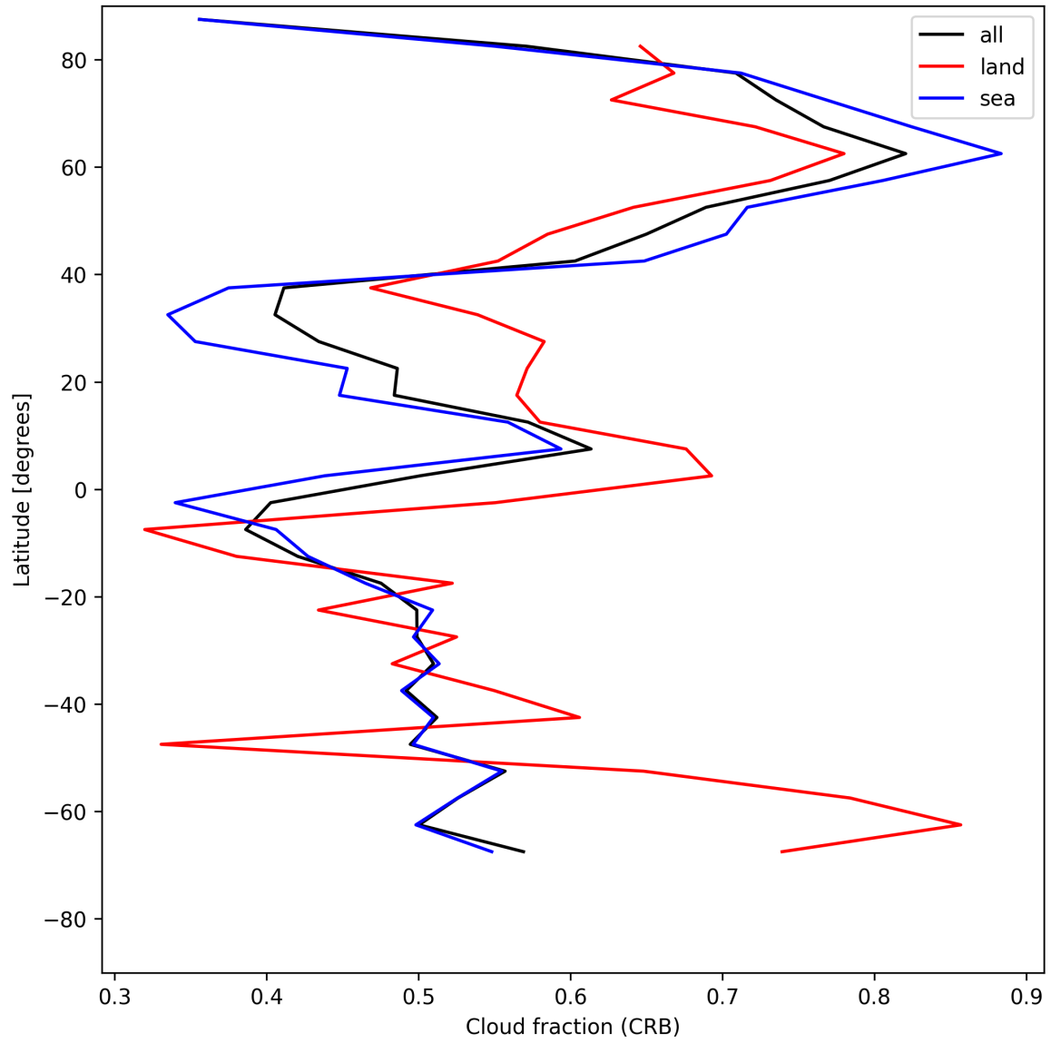
Figure 24: Zonal average of “Cloud fraction (CRB)” for 2025-07-21 to 2025-07-22.
