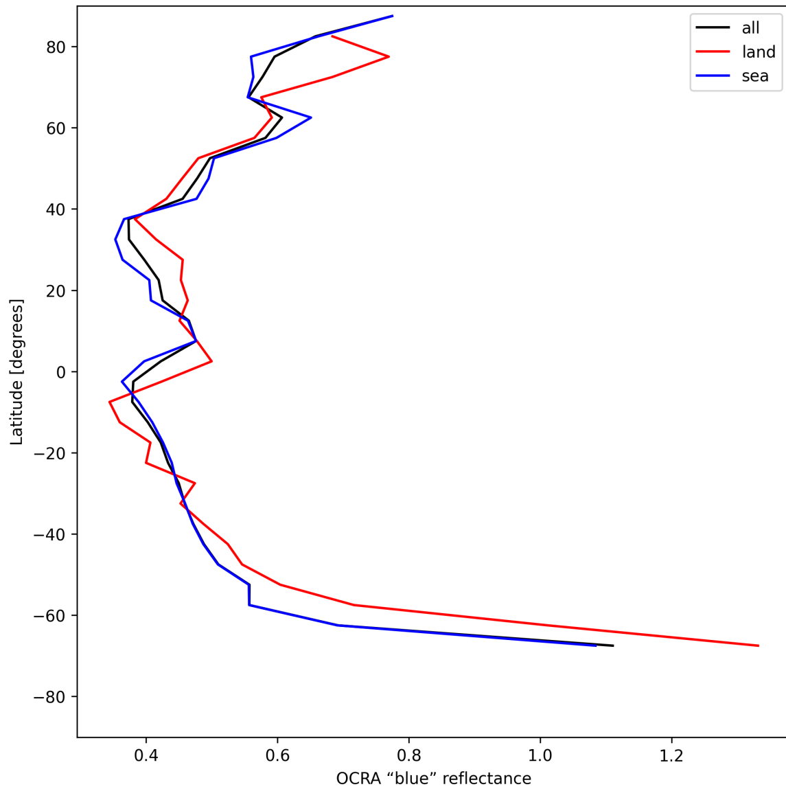
Figure 33: Zonal average of “OCRA “blue” reflectance” for 2025-07-21 to 2025-07-22.
