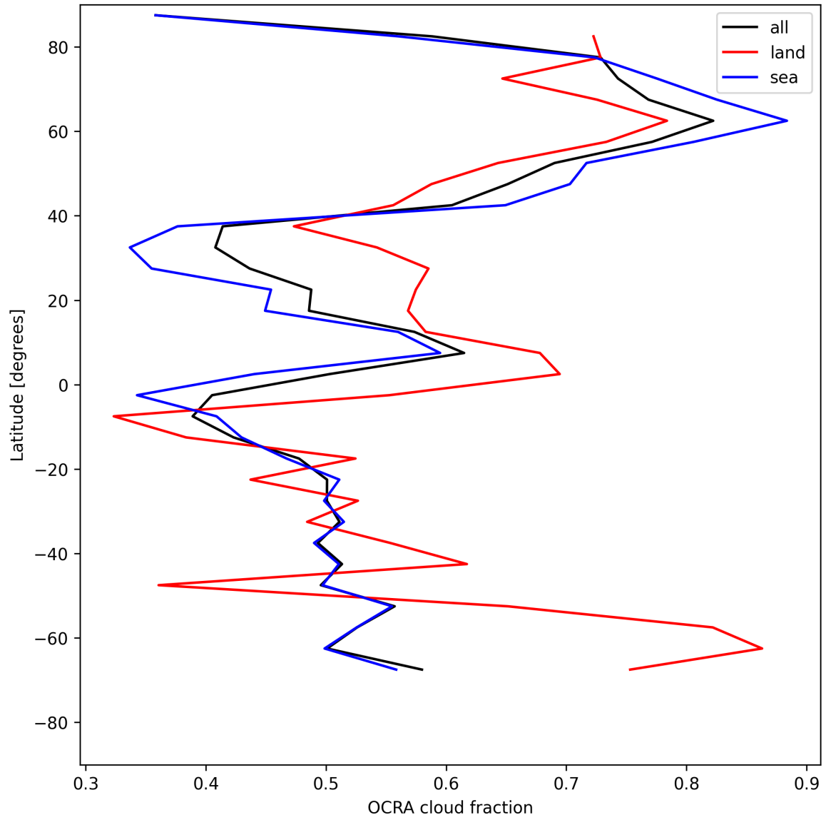
Figure 32: Zonal average of “OCRA cloud fraction” for 2025-07-21 to 2025-07-22.
