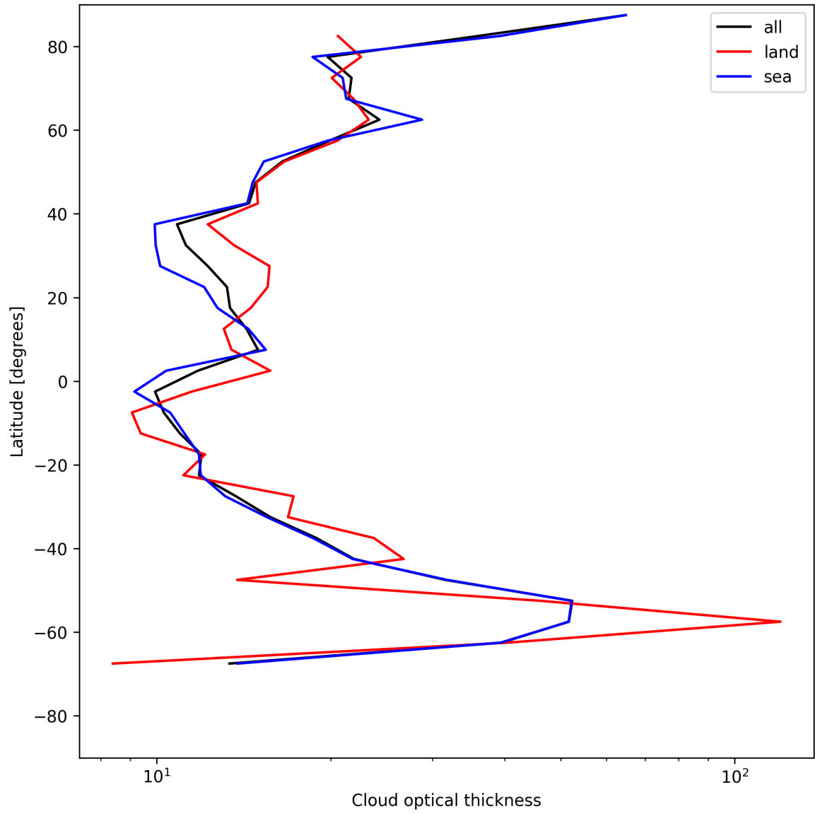
Figure 23: Zonal average of “Cloud optical thickness” for 2025-07-21 to 2025-07-22.
