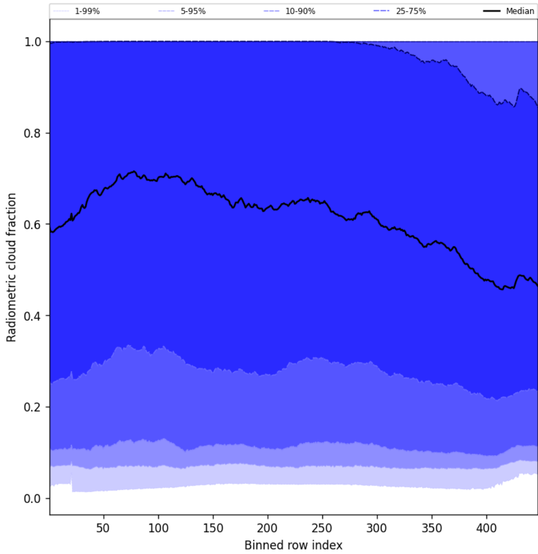
Figure 53: Along track statistics of “Radiometric cloud fraction” for 2025-07-21 to 2025-07-22
