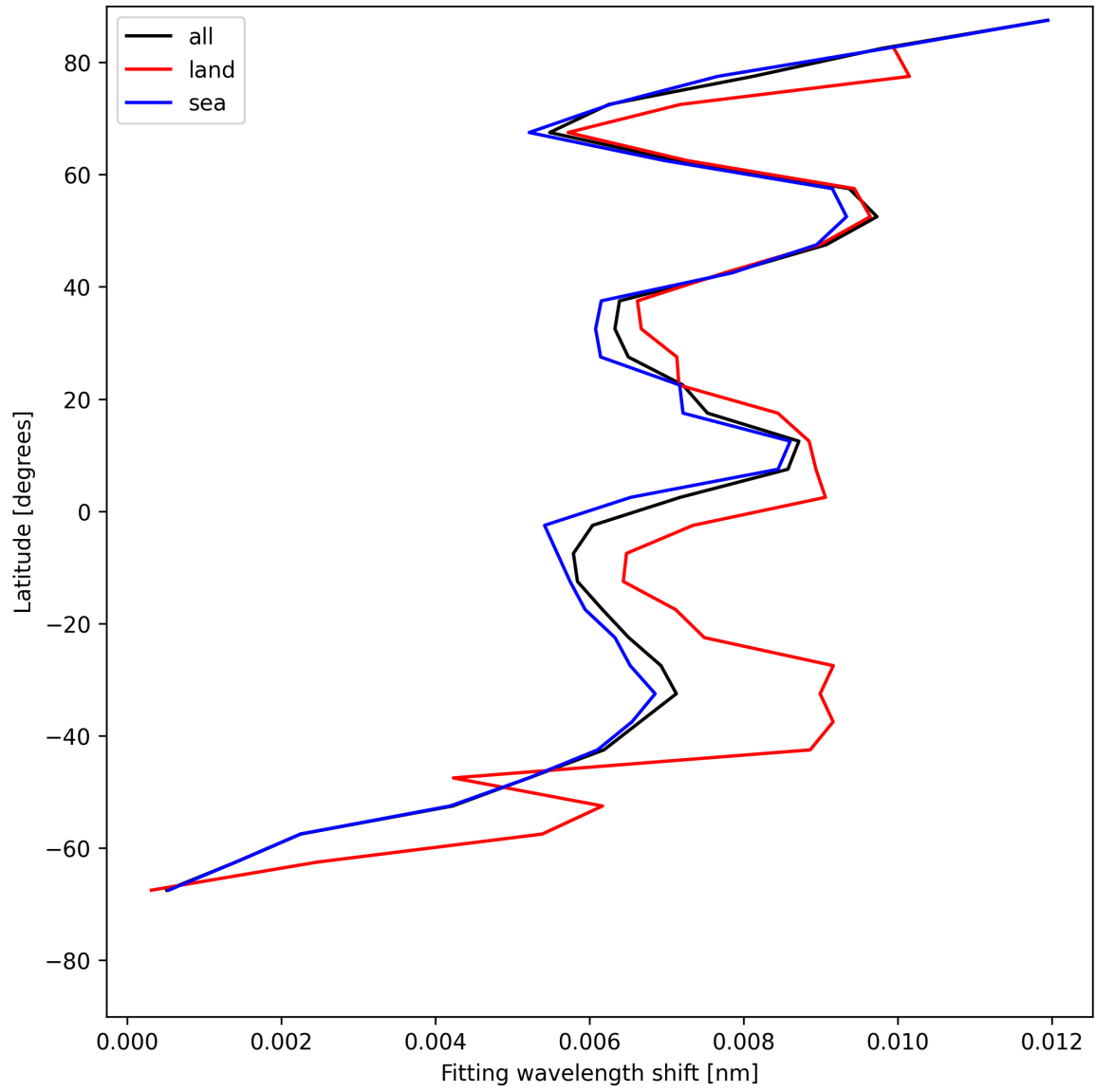
Figure 31: Zonal average of “Fitting wavelength shift” for 2025-07-21 to 2025-07-22.
