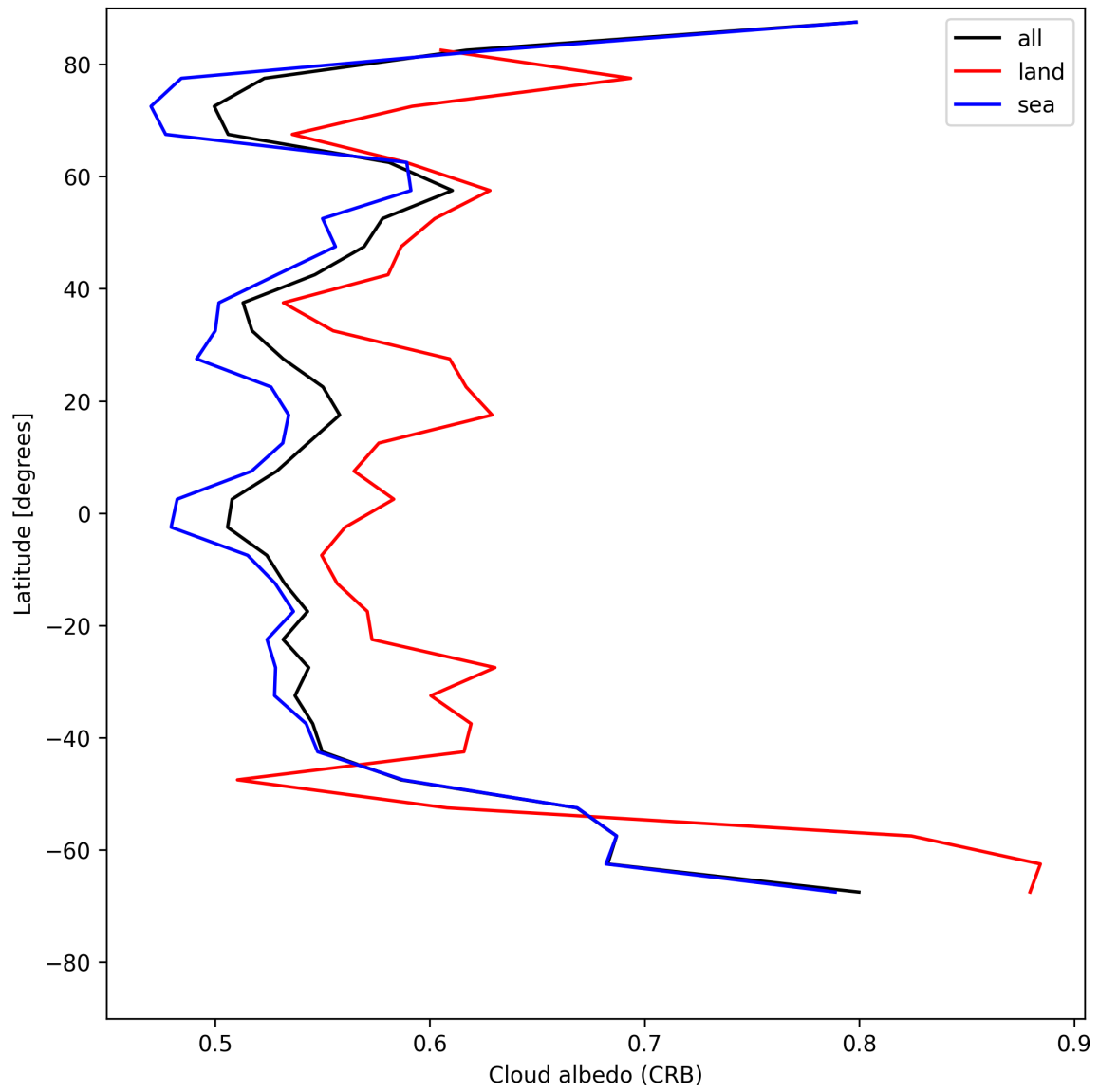
Figure 26: Zonal average of “Cloud albedo (CRB)” for 2025-07-21 to 2025-07-22.
