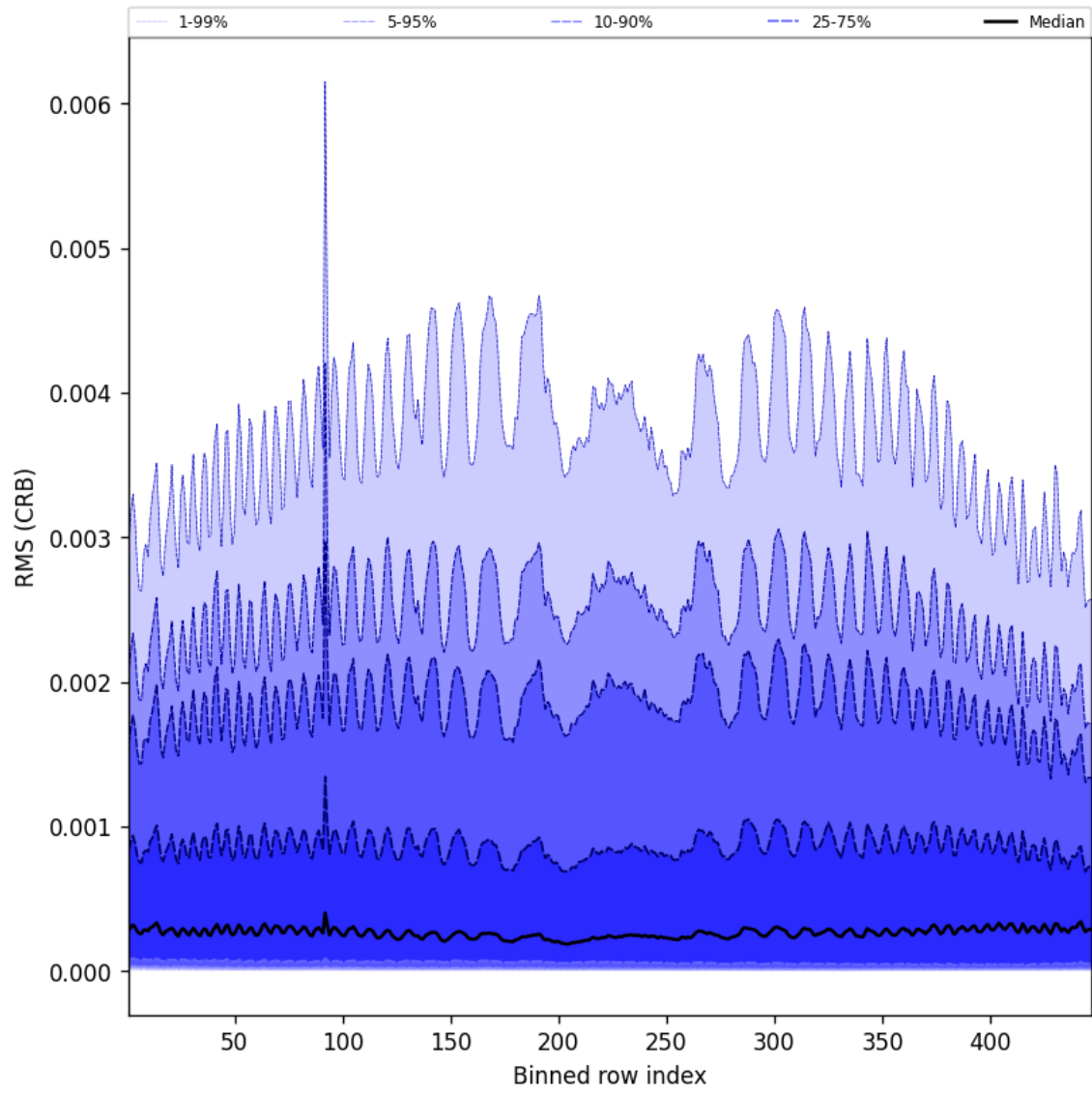
Figure 62: Along track statistics of “RMS (CRB)” for 2025-07-21 to 2025-07-22
