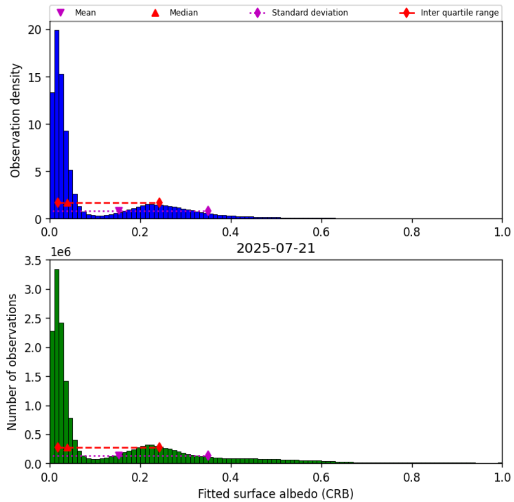
Figure 44: Histogram of “Fitted surface albedo (CRB)” for 2025-07-21 to 2025-07-22
