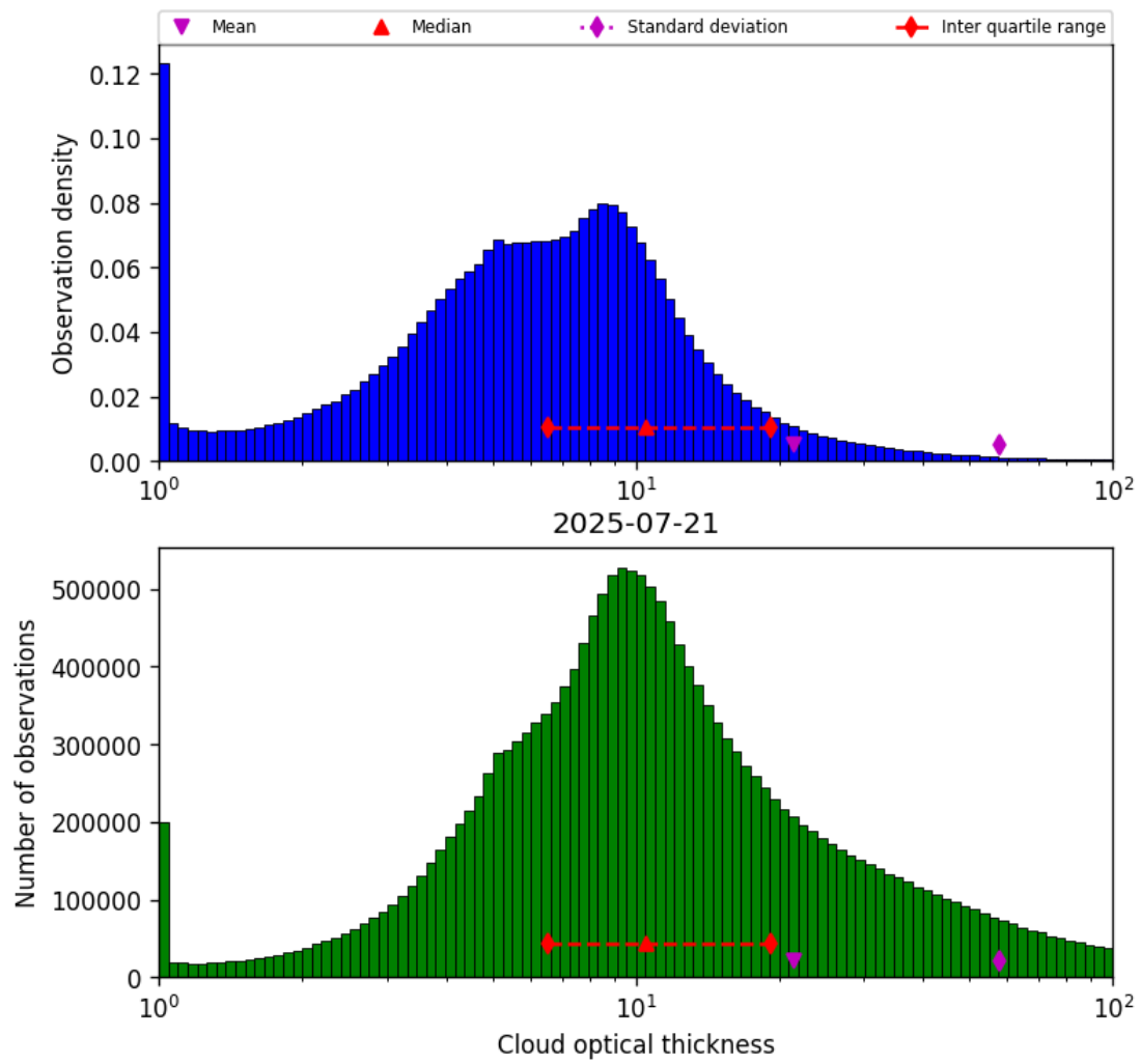
Figure 39: Histogram of “Cloud optical thickness” for 2025-07-21 to 2025-07-22
