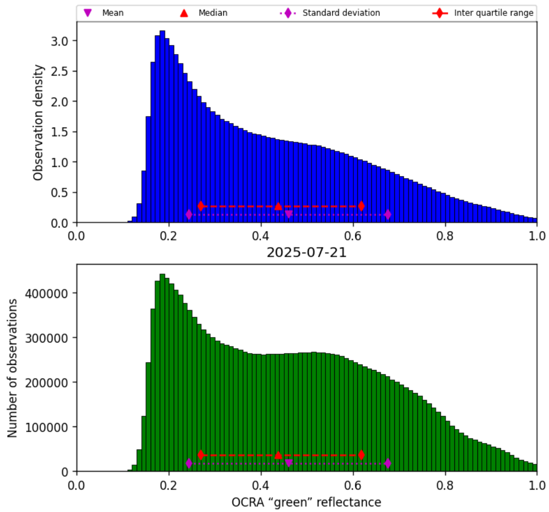
Figure 50: Histogram of “OCRA “green” reflectance” for 2025-07-21 to 2025-07-22
