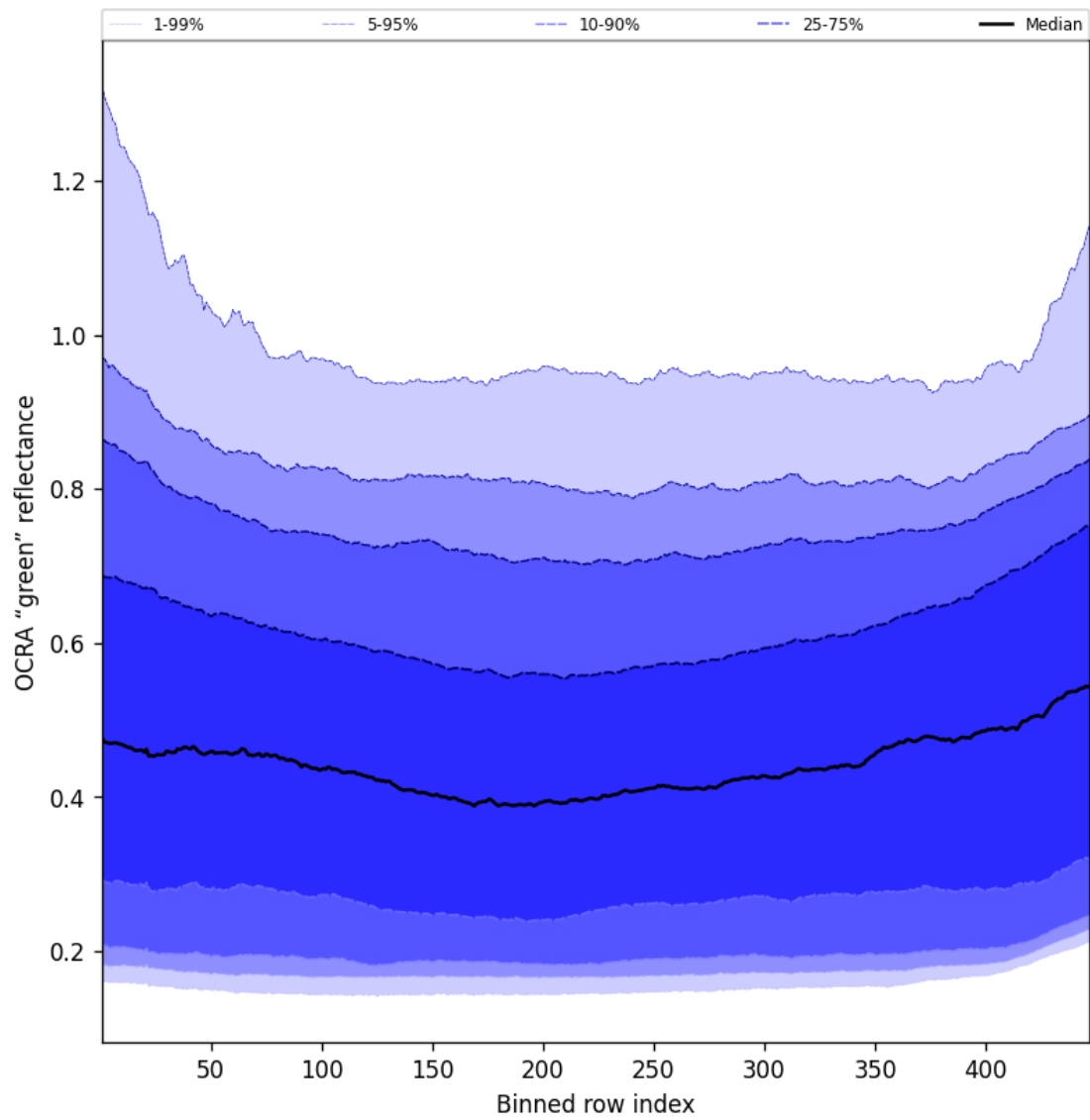
Figure 66: Along track statistics of “OCRA “green” reflectance” for 2025-07-21 to 2025-07-22
