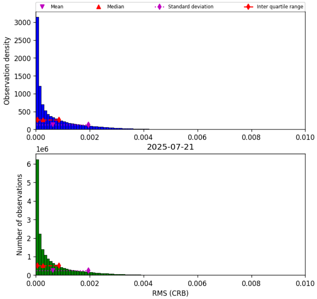
Figure 46: Histogram of “RMS (CRB)” for 2025-07-21 to 2025-07-22
