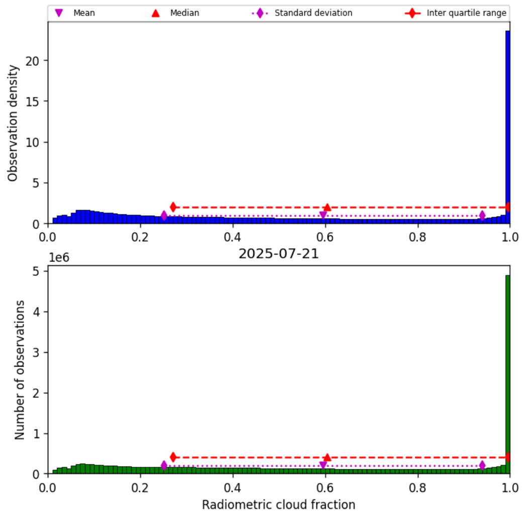
Figure 37: Histogram of “Radiometric cloud fraction” for 2025-07-21 to 2025-07-22
