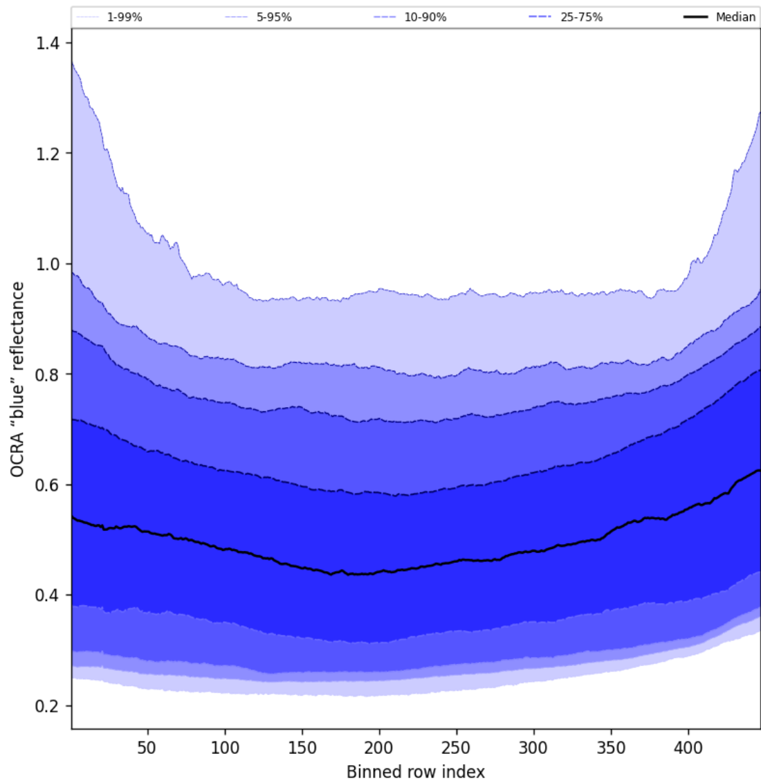
Figure 65: Along track statistics of “OCRA “blue” reflectance” for 2025-07-21 to 2025-07-22
