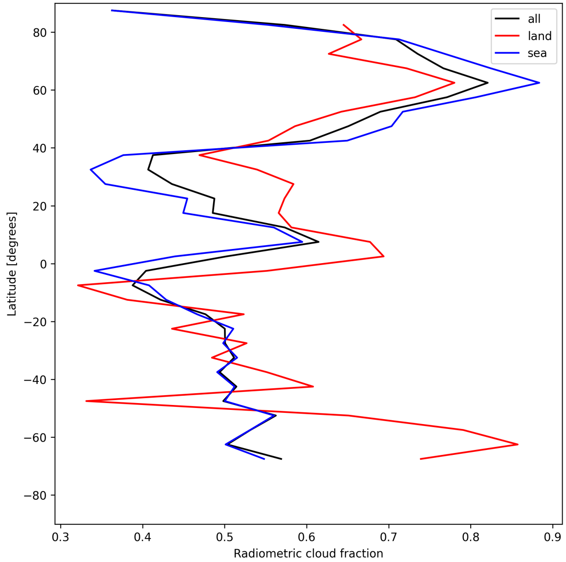
Figure 21: Zonal average of “Radiometric cloud fraction” for 2025-07-21 to 2025-07-22.
