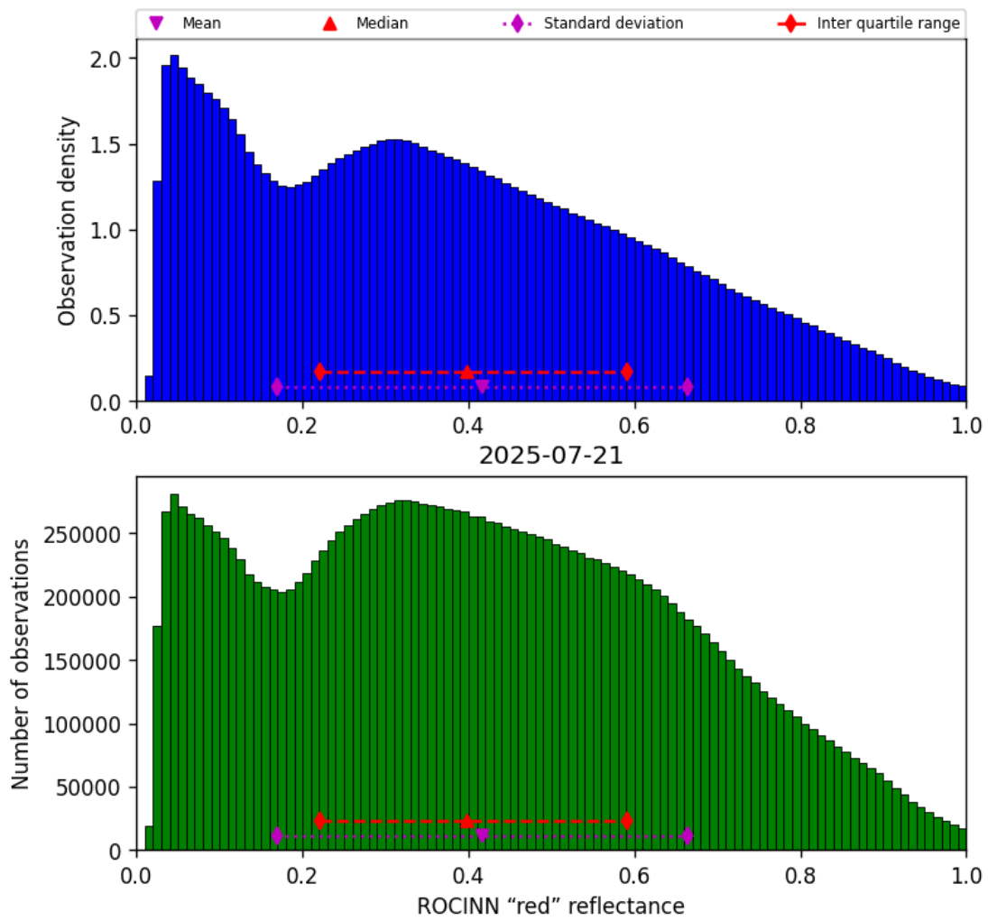
Figure 51: Histogram of “ROCINN “red” reflectance” for 2025-07-21 to 2025-07-22
