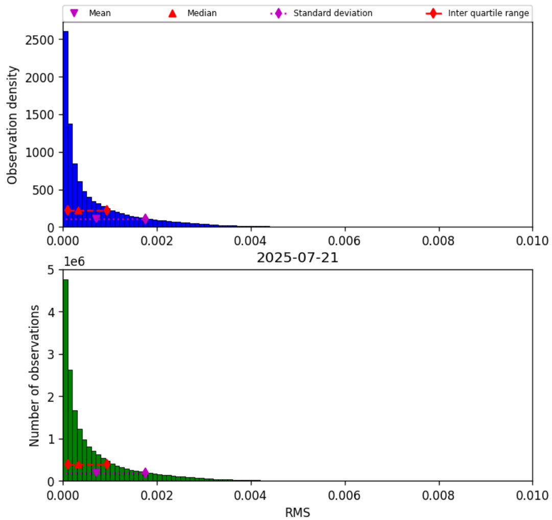
Figure 45: Histogram of “RMS” for 2025-07-21 to 2025-07-22
