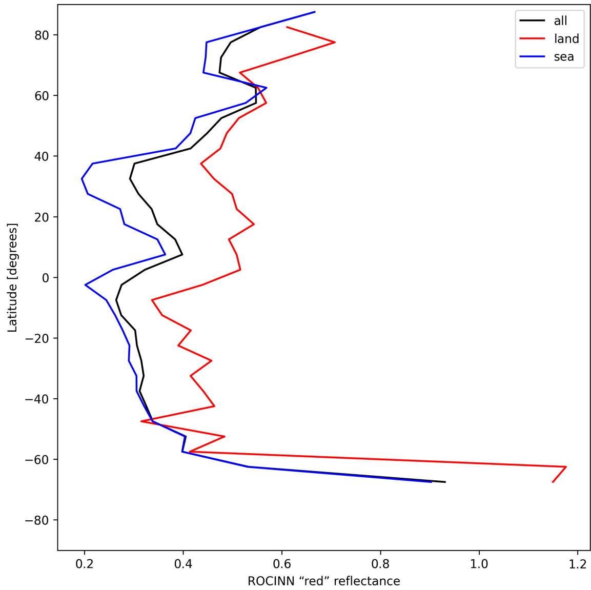
Figure 35: Zonal average of "ROCINN "red" reflectance" for 2025-07-21 to 2025-07-22.
