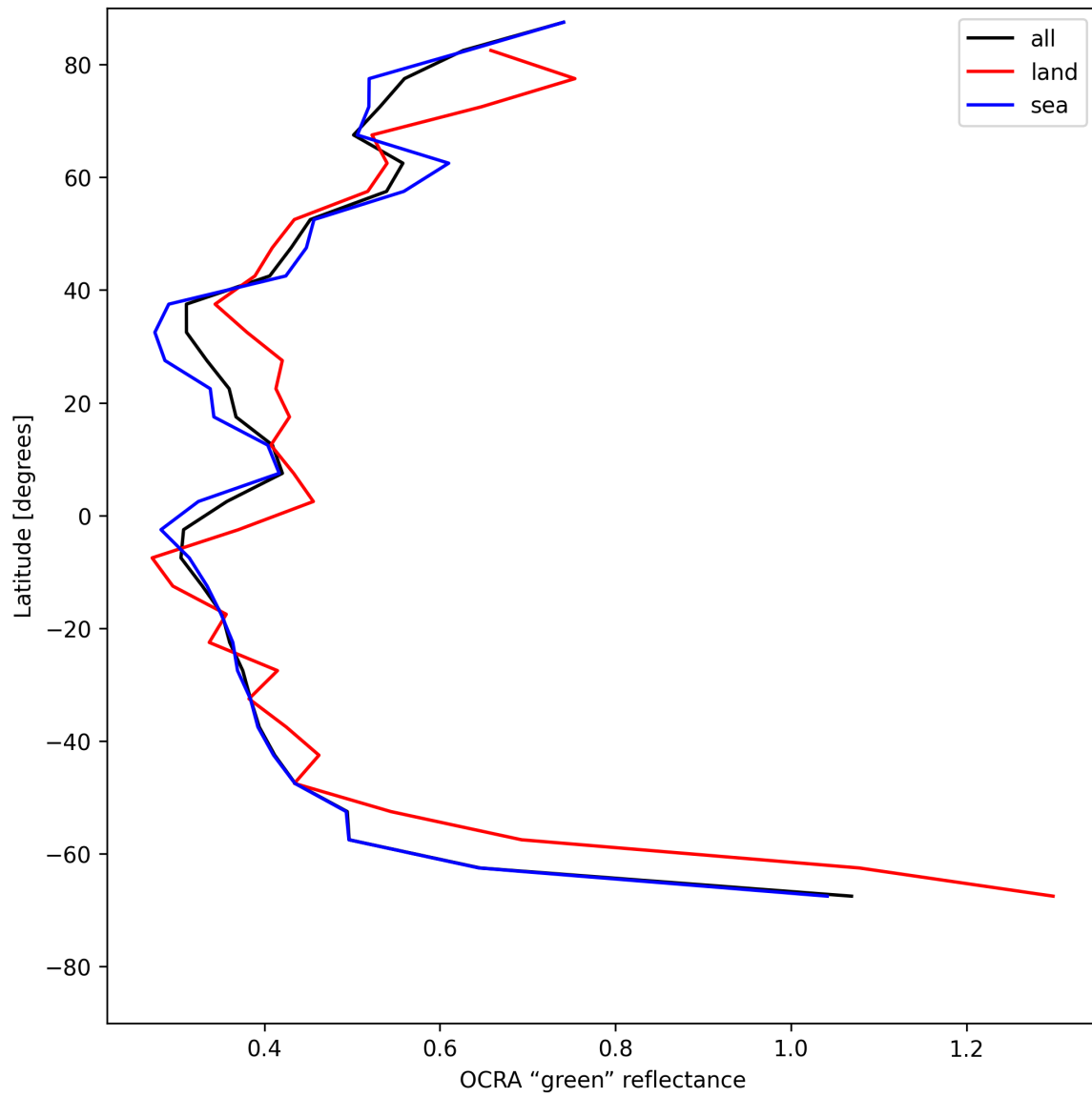
Figure 34: Zonal average of “OCRA “green” reflectance” for 2025-07-21 to 2025-07-22.
