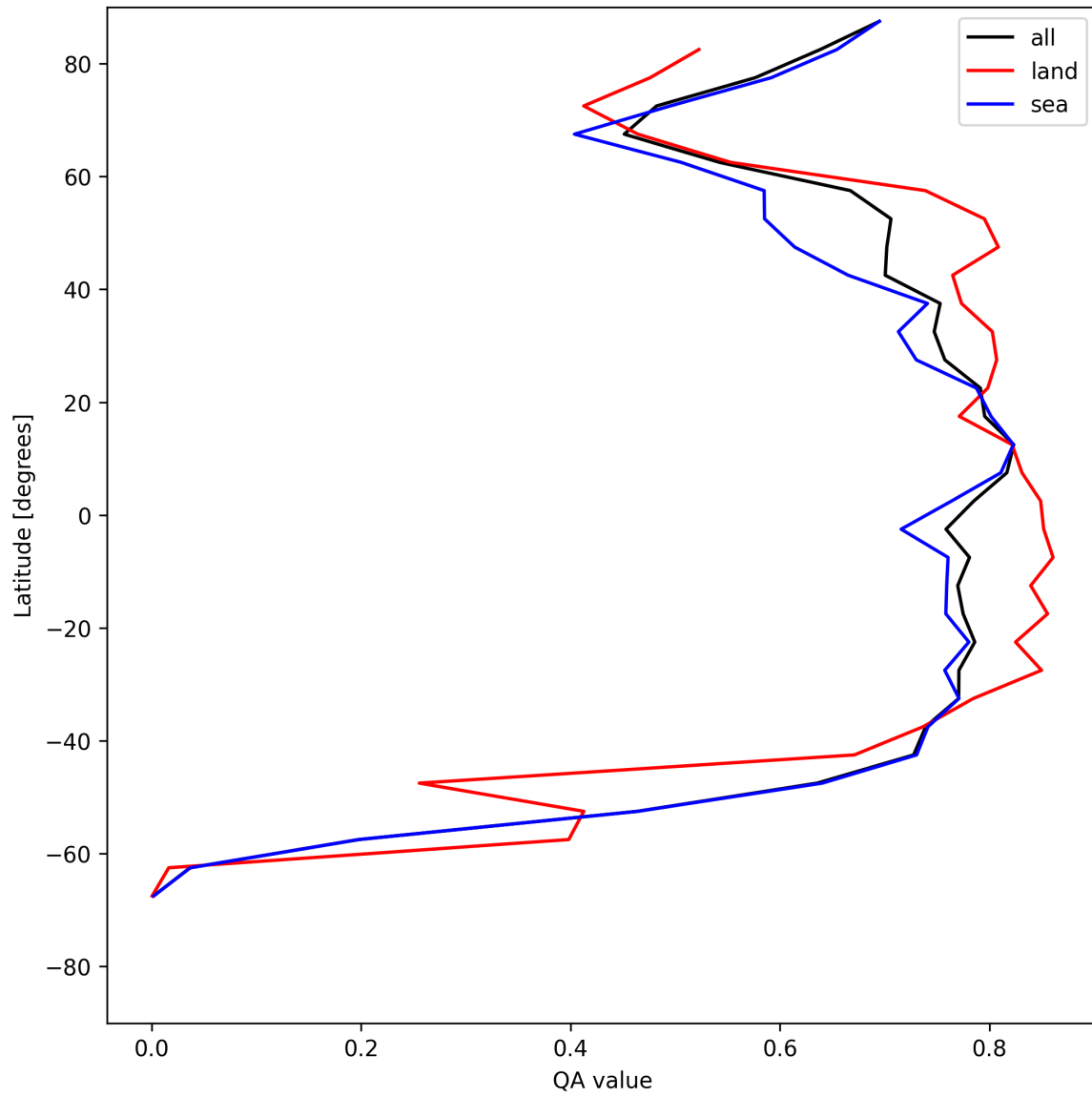
Figure 20: Zonal average of “QA value” for 2025-07-21 to 2025-07-22.
