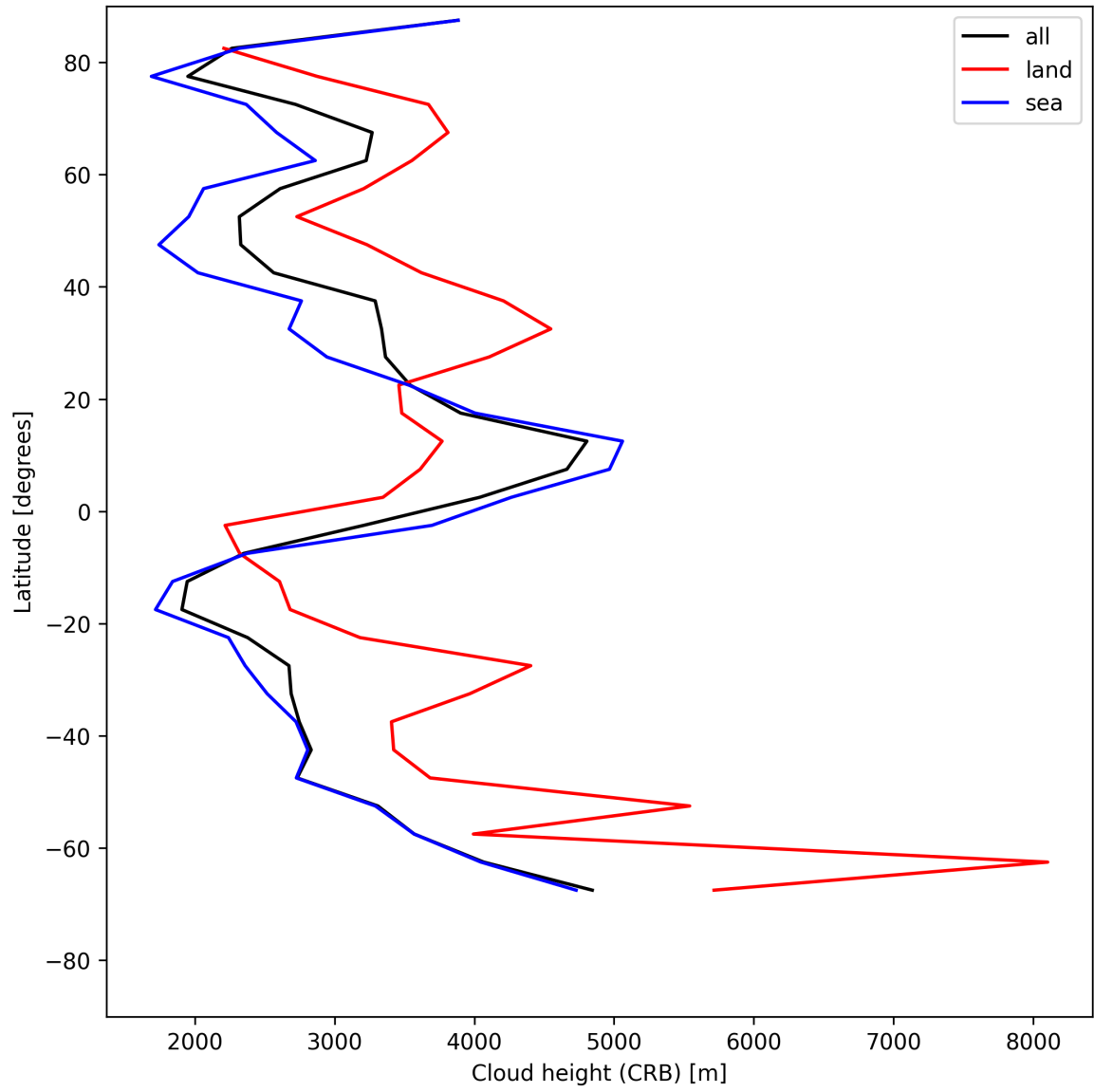
Figure 25: Zonal average of “Cloud height (CRB)” for 2025-07-21 to 2025-07-22.
