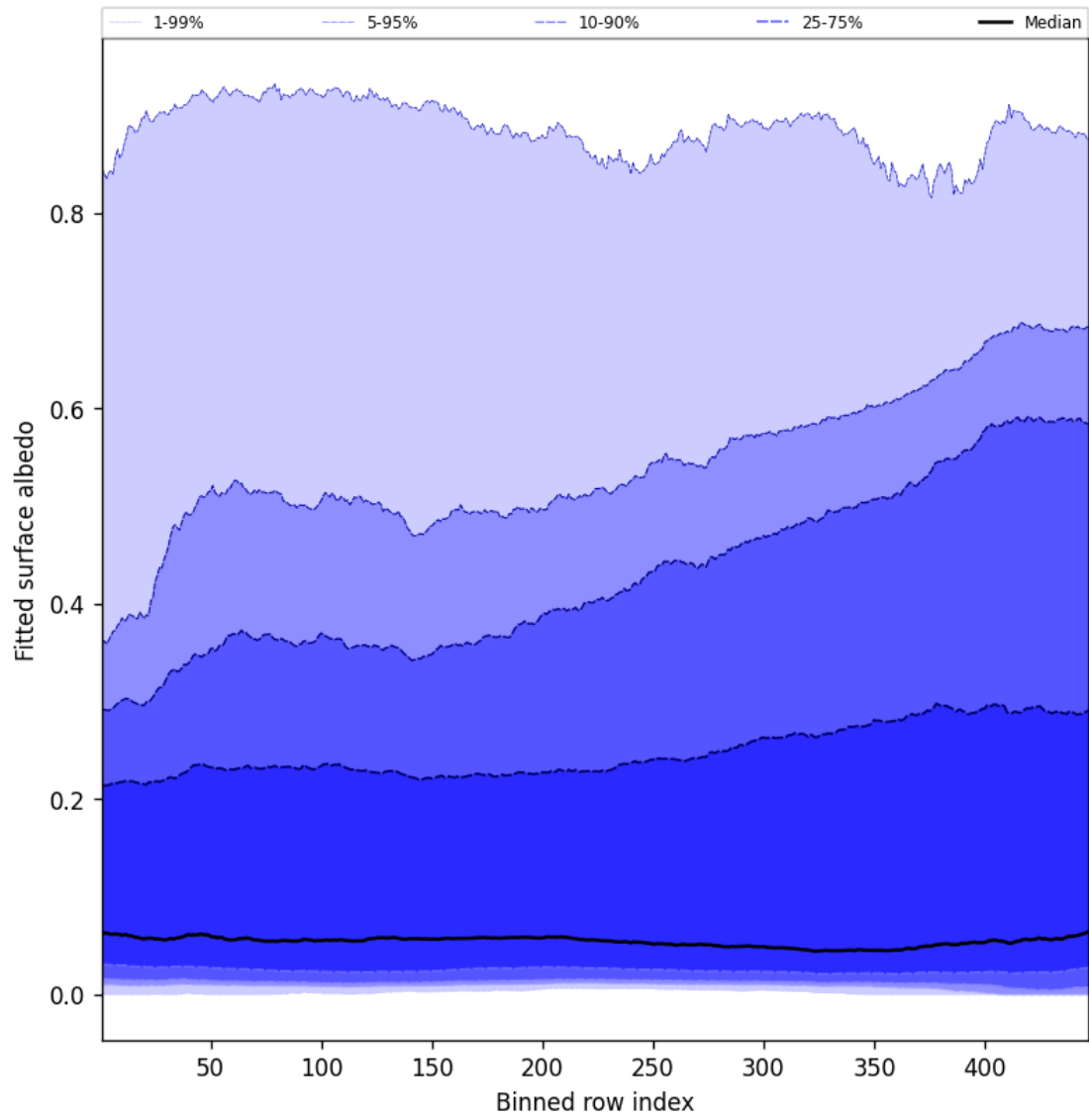
Figure 59: Along track statistics of “Fitted surface albedo” for 2025-07-21 to 2025-07-22
