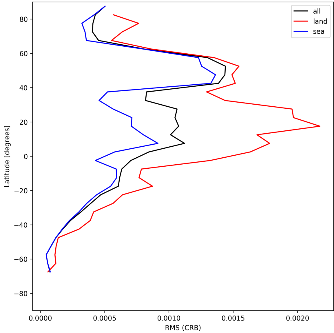
Figure 30: Zonal average of “RMS (CRB)” for 2025-07-21 to 2025-07-22.
