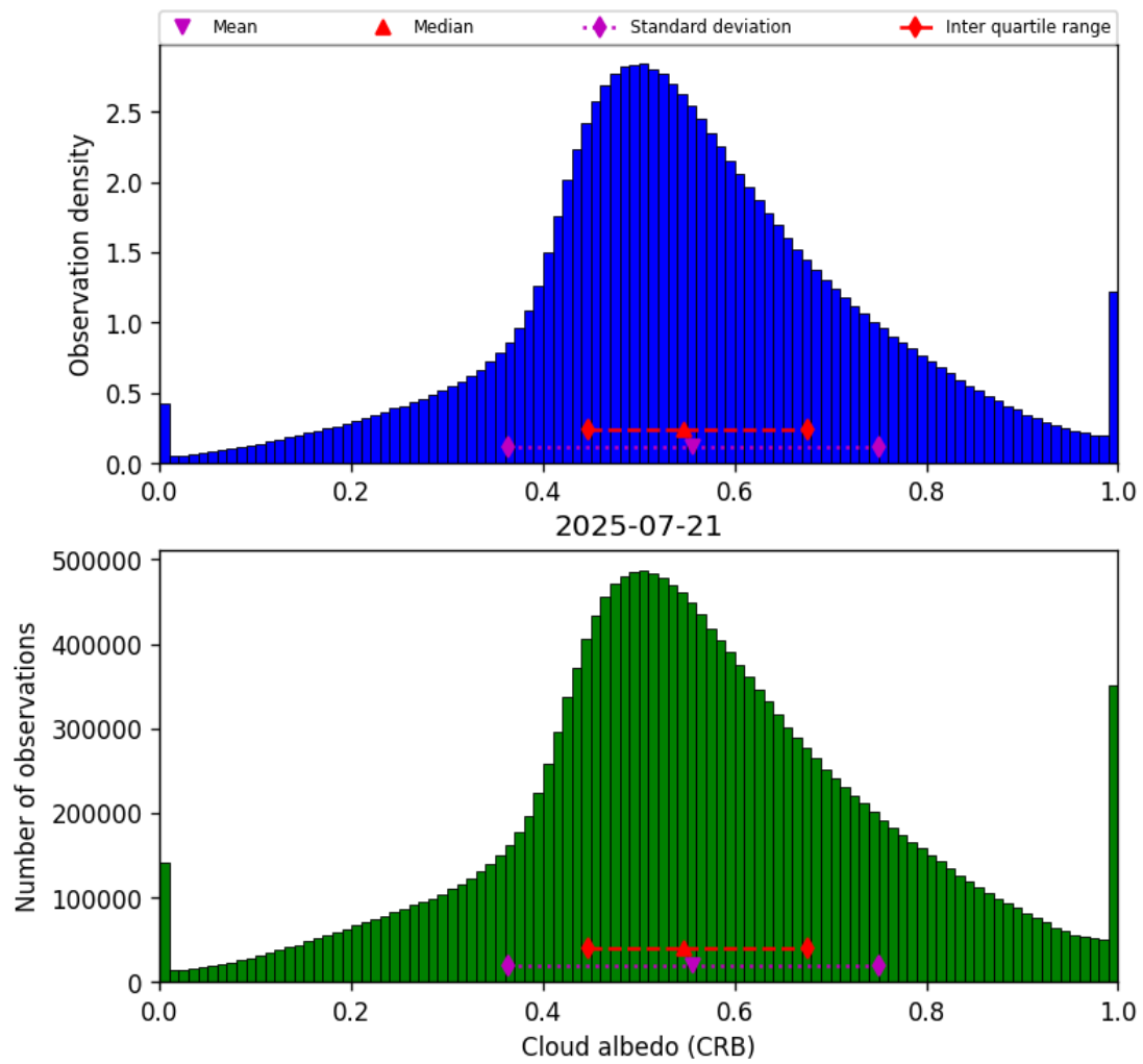
Figure 42: Histogram of “Cloud albedo (CRB)” for 2025-07-21 to 2025-07-22
