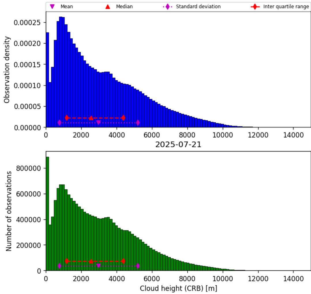
Figure 41: Histogram of “Cloud height (CRB)” for 2025-07-21 to 2025-07-22
