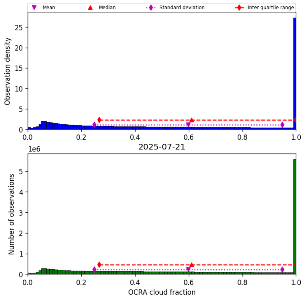
Figure 48: Histogram of “OCRA cloud fraction” for 2025-07-21 to 2025-07-22
