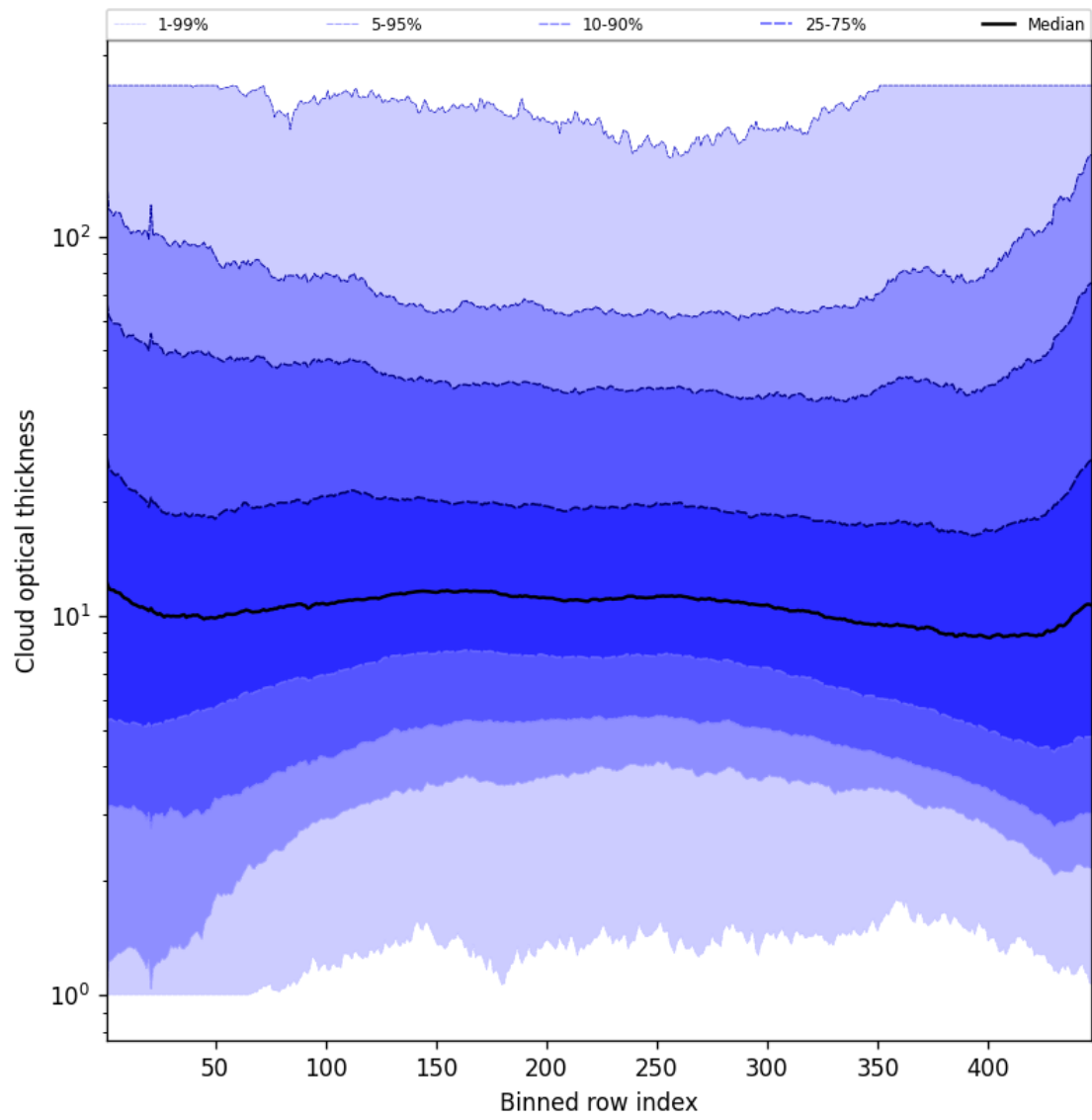
Figure 55: Along track statistics of “Cloud optical thickness” for 2025-07-21 to 2025-07-22
