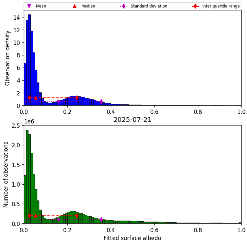
Figure 43: Histogram of “Fitted surface albedo” for 2025-07-21 to 2025-07-22
