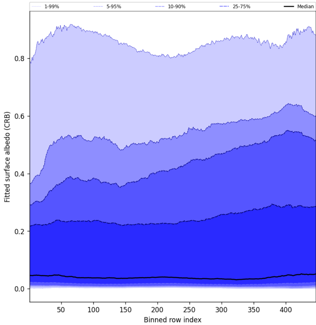
Figure 60: Along track statistics of “Fitted surface albedo (CRB)” for 2025-07-21 to 2025-07-22
