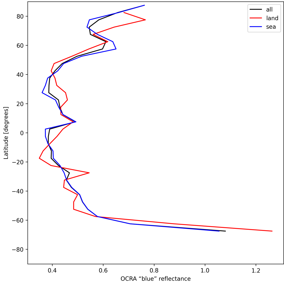
Figure 33: Zonal average of “OCRA “blue” reflectance” for 2025-07-23 to 2025-07-24.
