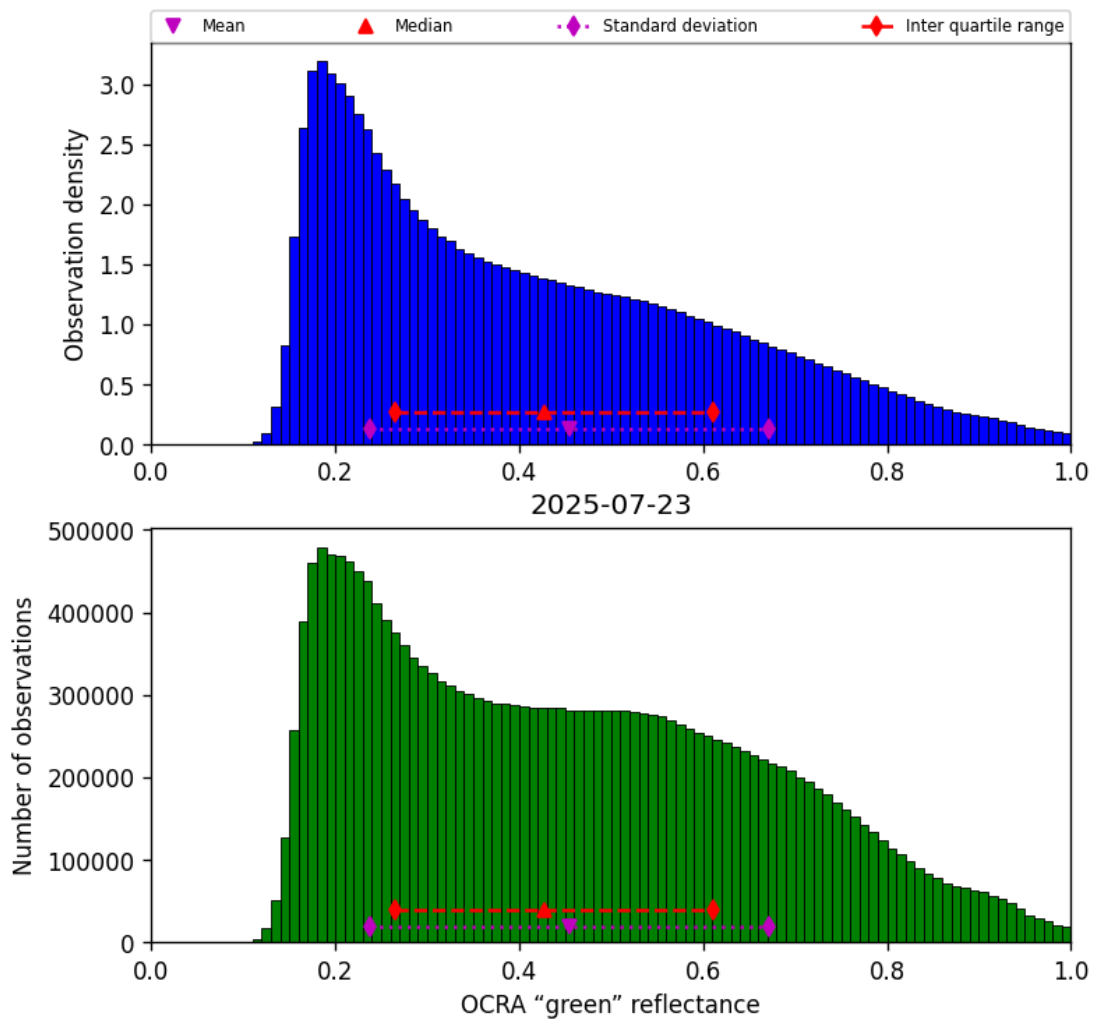
Figure 50: Histogram of “OCRA “green” reflectance” for 2025-07-23 to 2025-07-24
