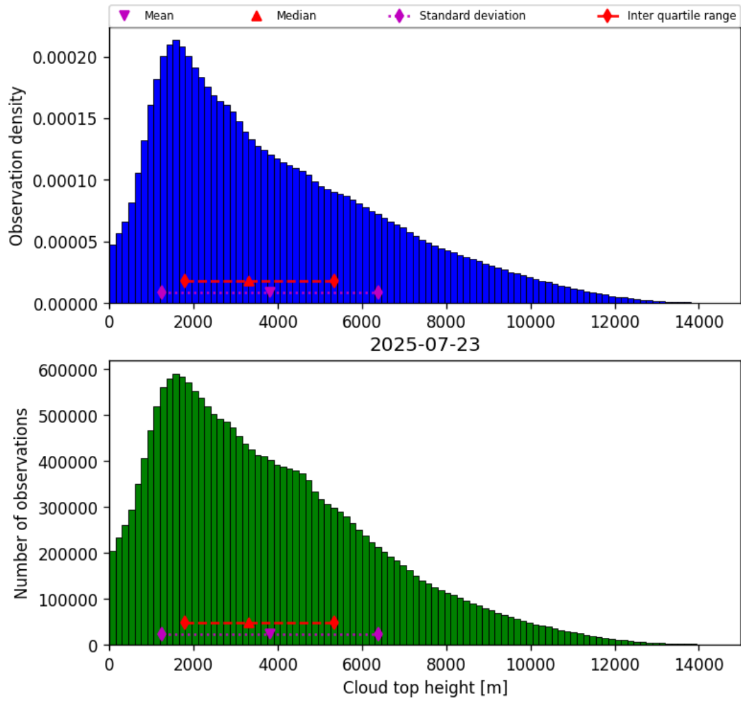
Figure 38: Histogram of “Cloud top height” for 2025-07-23 to 2025-07-24
