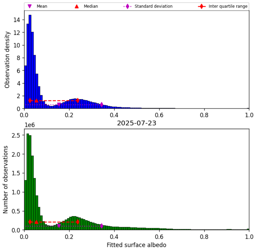
Figure 43: Histogram of “Fitted surface albedo” for 2025-07-23 to 2025-07-24
