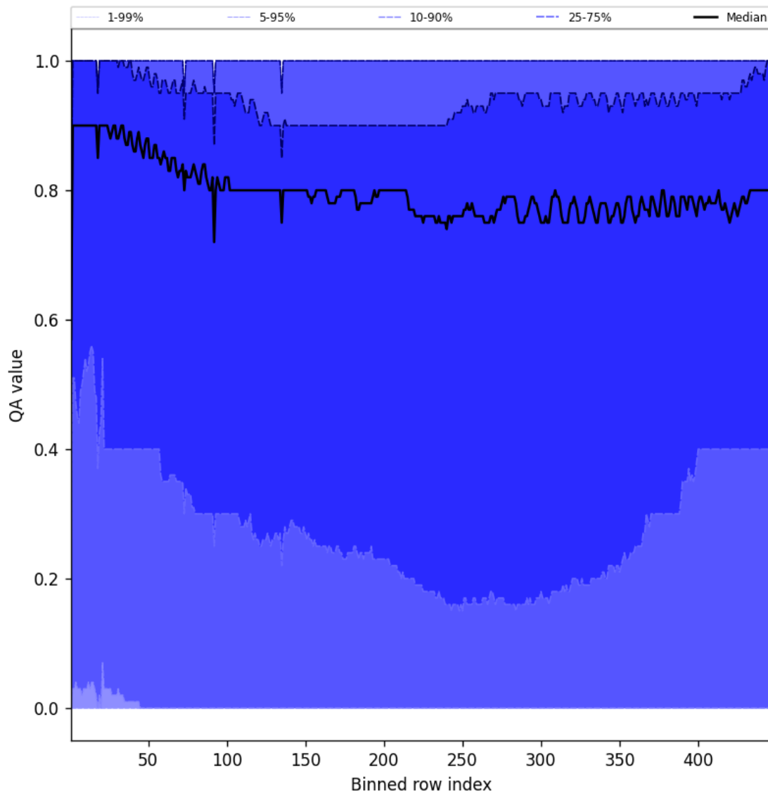
Figure 52: Along track statistics of “QA value” for 2025-07-23 to 2025-07-24
