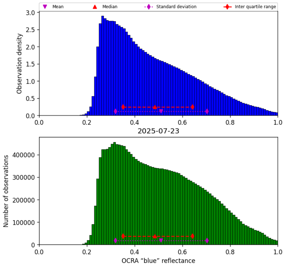
Figure 49: Histogram of “OCRA “blue” reflectance” for 2025-07-23 to 2025-07-24
