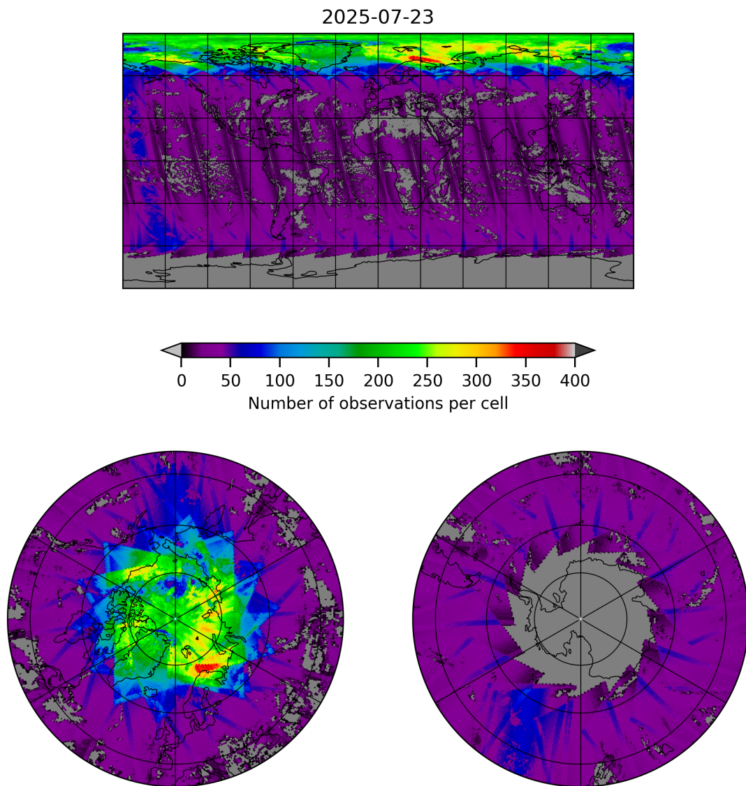
Figure 19: Map of the number of observations for 2025-07-23 to 2025-07-24
