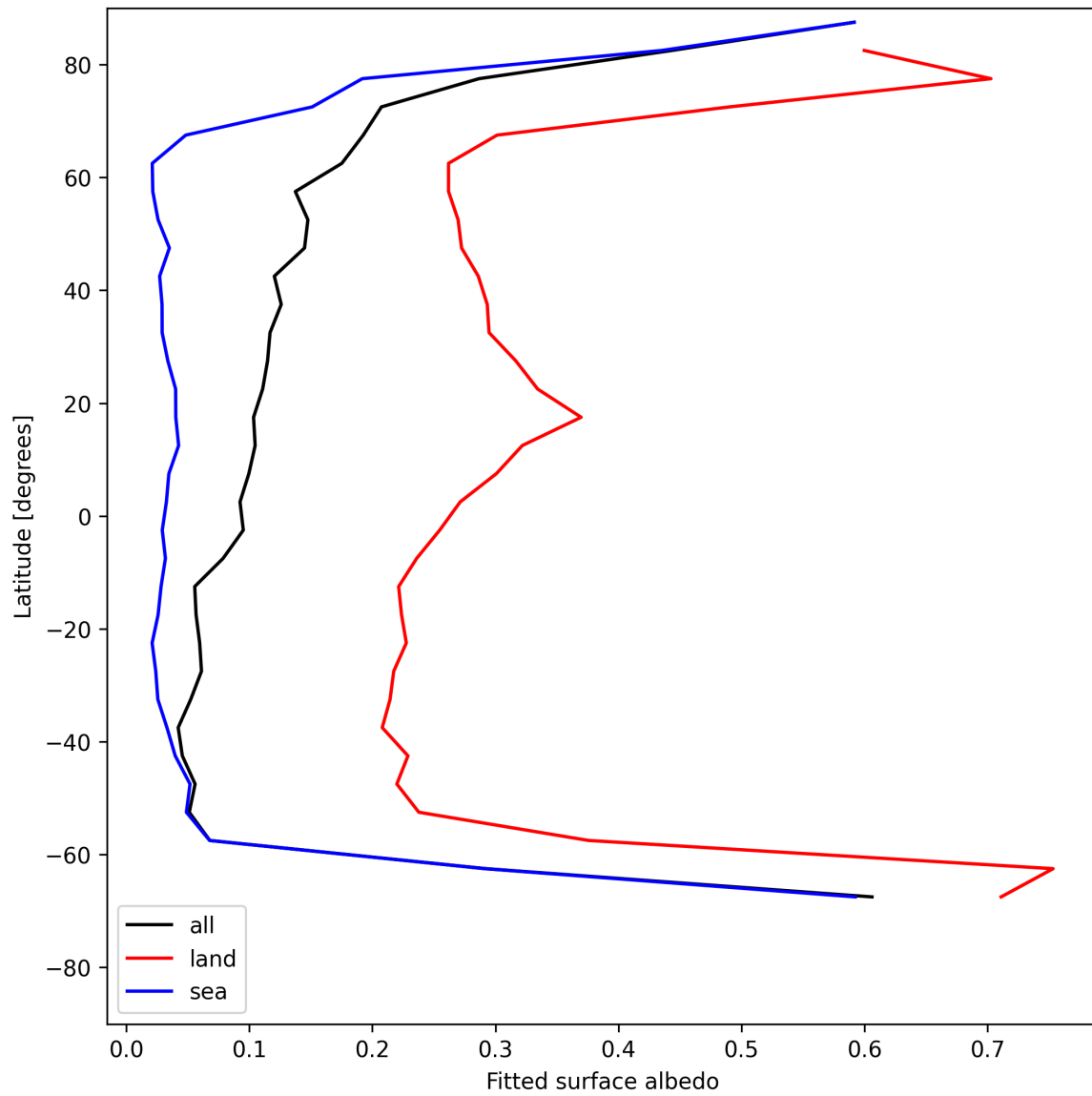
Figure 27: Zonal average of “Fitted surface albedo” for 2025-07-23 to 2025-07-24.
