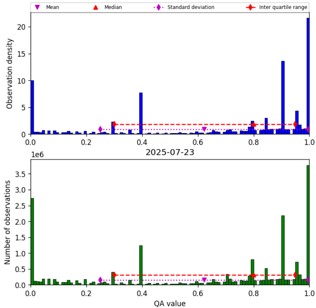
Figure 36: Histogram of “QA value” for 2025-07-23 to 2025-07-24
