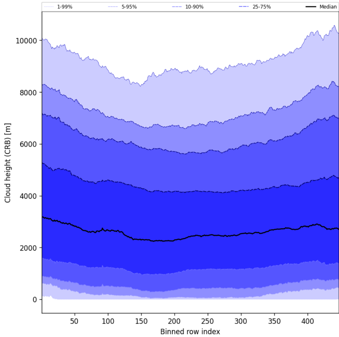
Figure 57: Along track statistics of “Cloud height (CRB)” for 2025-07-23 to 2025-07-24
