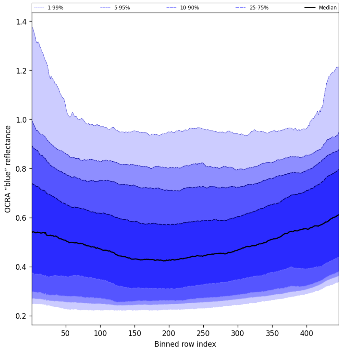
Figure 65: Along track statistics of “OCRA “blue” reflectance” for 2025-07-23 to 2025-07-24
