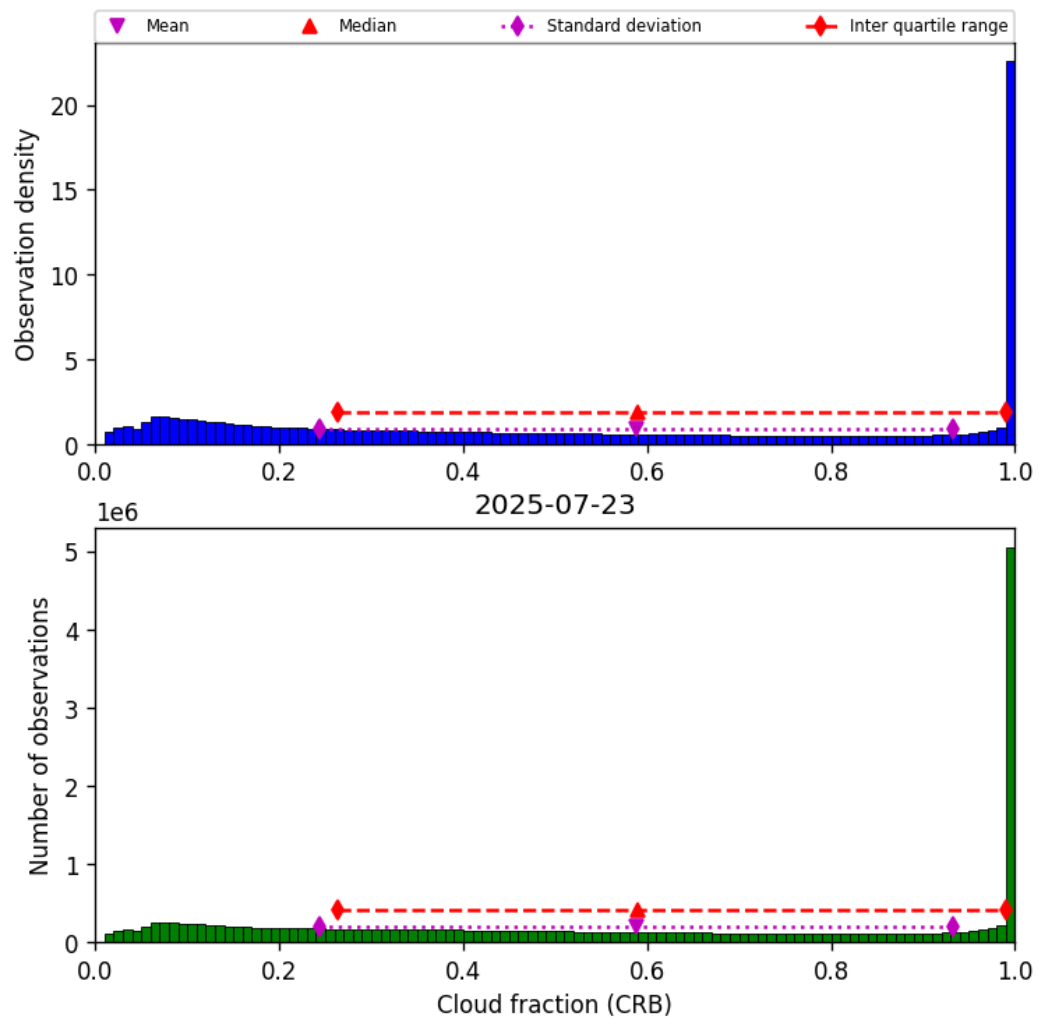
Figure 40: Histogram of “Cloud fraction (CRB)” for 2025-07-23 to 2025-07-24
