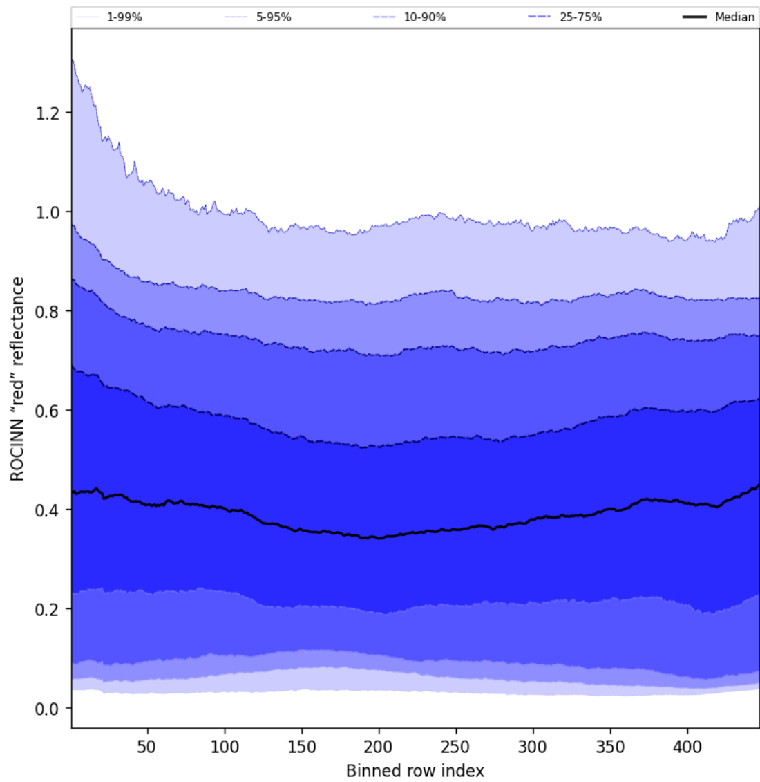
Figure 67: Along track statistics of “ROCINN “red” reflectance” for 2025-07-23 to 2025-07-24
