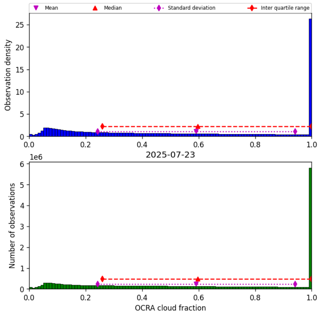
Figure 48: Histogram of “OCRA cloud fraction” for 2025-07-23 to 2025-07-24
