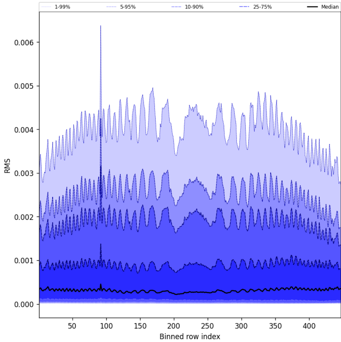
Figure 61: Along track statistics of “RMS” for 2025-07-23 to 2025-07-24
