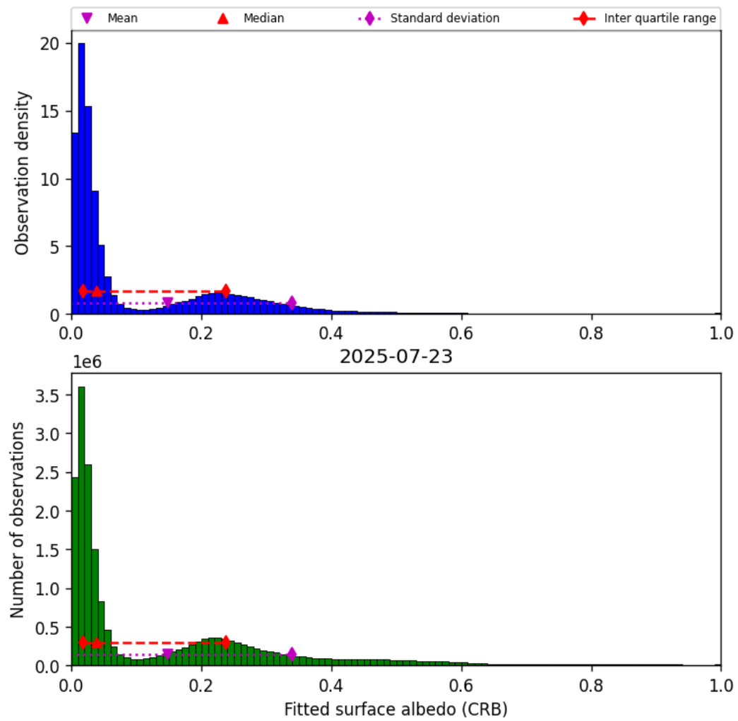
Figure 44: Histogram of “Fitted surface albedo (CRB)” for 2025-07-23 to 2025-07-24
