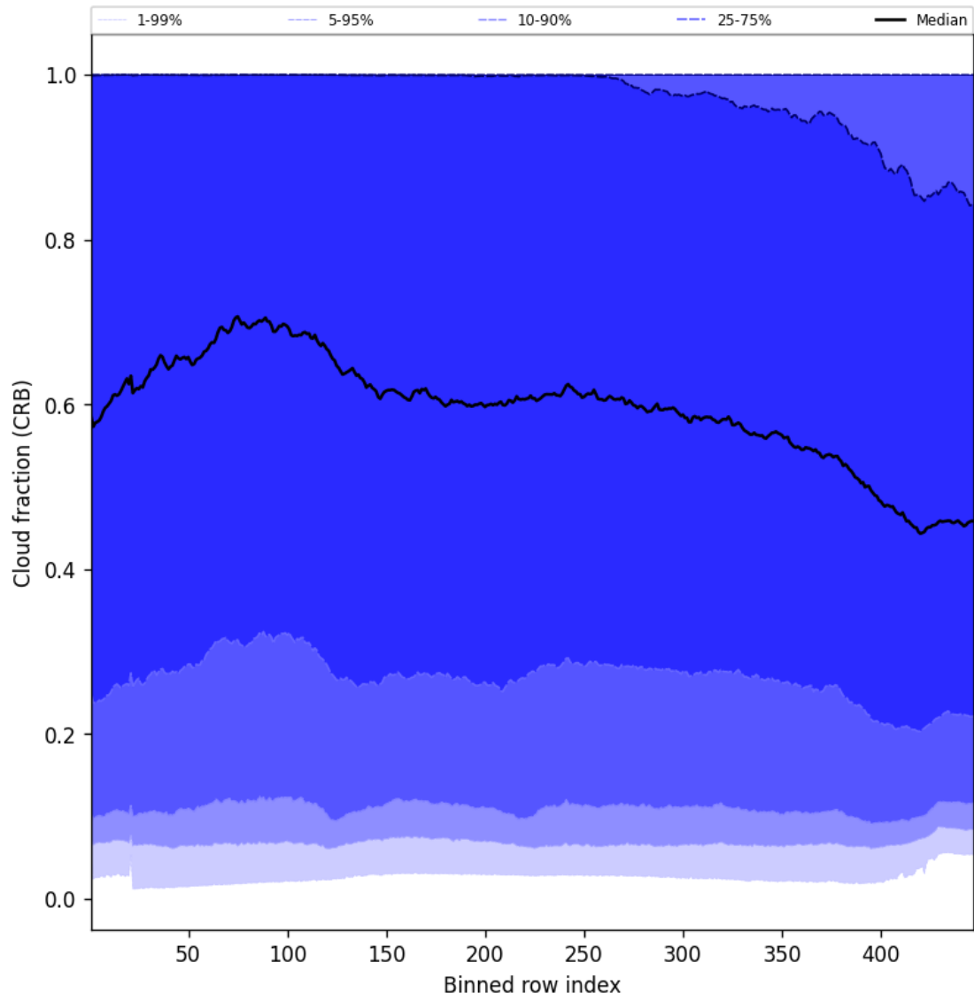
Figure 56: Along track statistics of “Cloud fraction (CRB)” for 2025-07-23 to 2025-07-24
