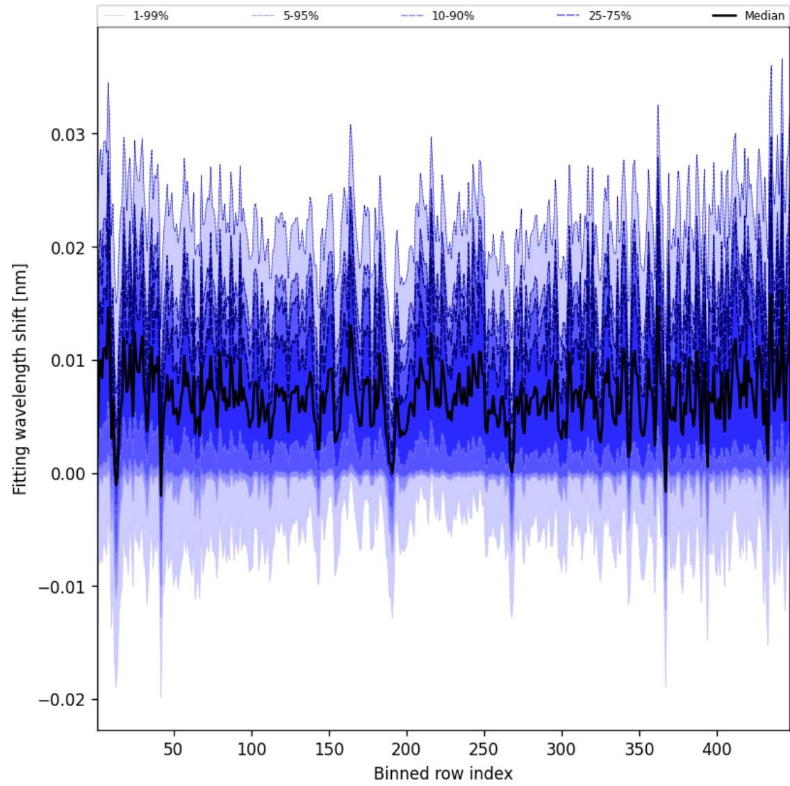
Figure 63: Along track statistics of “Fitting wavelength shift” for 2025-07-23 to 2025-07-24
