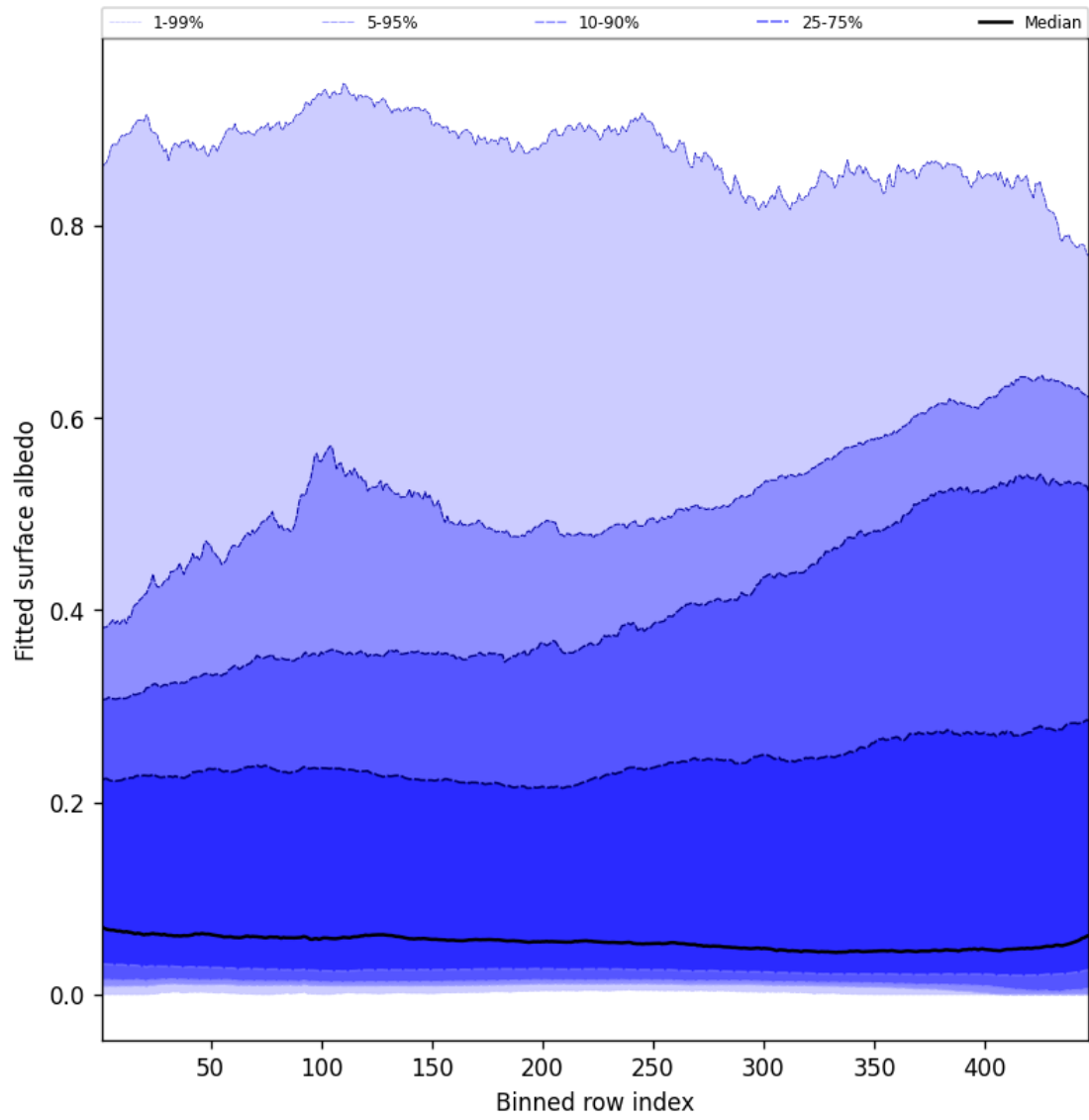
Figure 59: Along track statistics of “Fitted surface albedo” for 2025-07-23 to 2025-07-24
