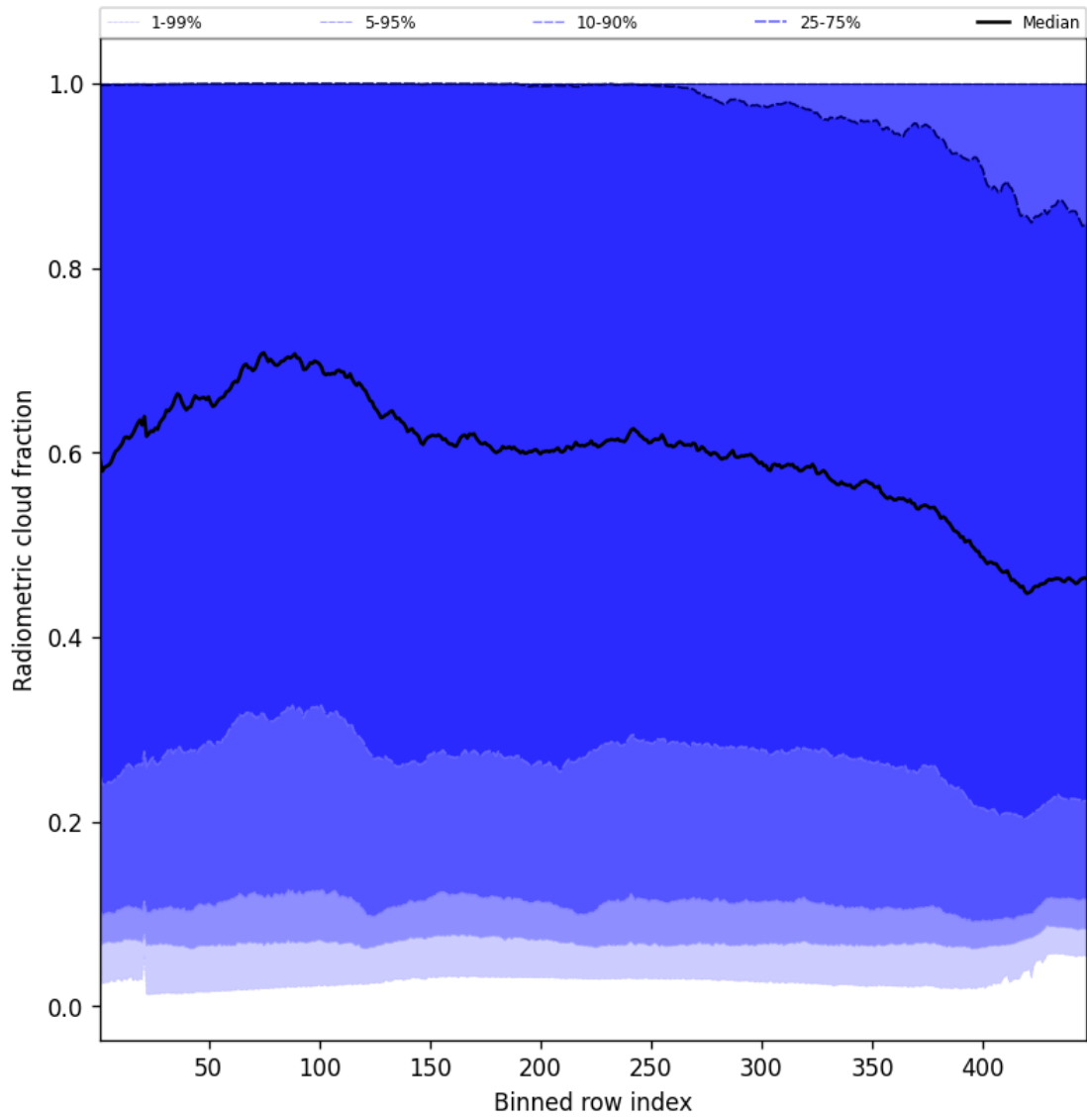
Figure 53: Along track statistics of “Radiometric cloud fraction” for 2025-07-23 to 2025-07-24
