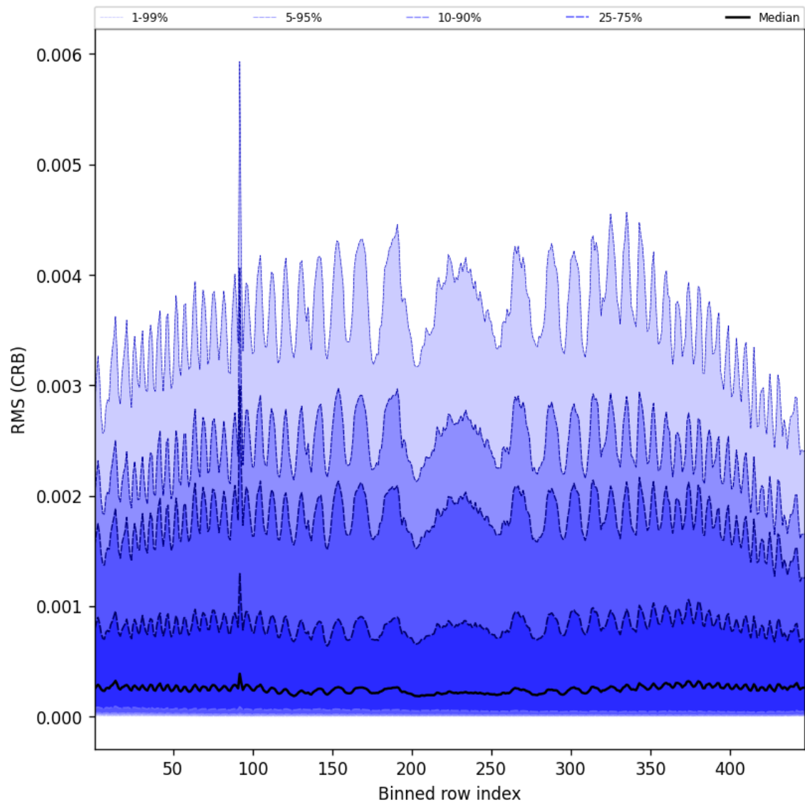
Figure 62: Along track statistics of “RMS (CRB)” for 2025-07-23 to 2025-07-24
