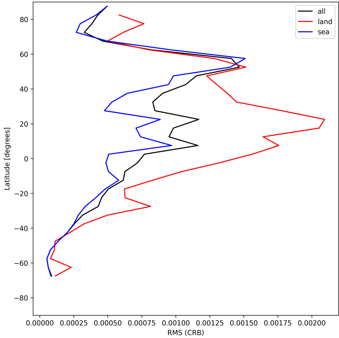
Figure 30: Zonal average of “RMS (CRB)” for 2025-07-23 to 2025-07-24.
