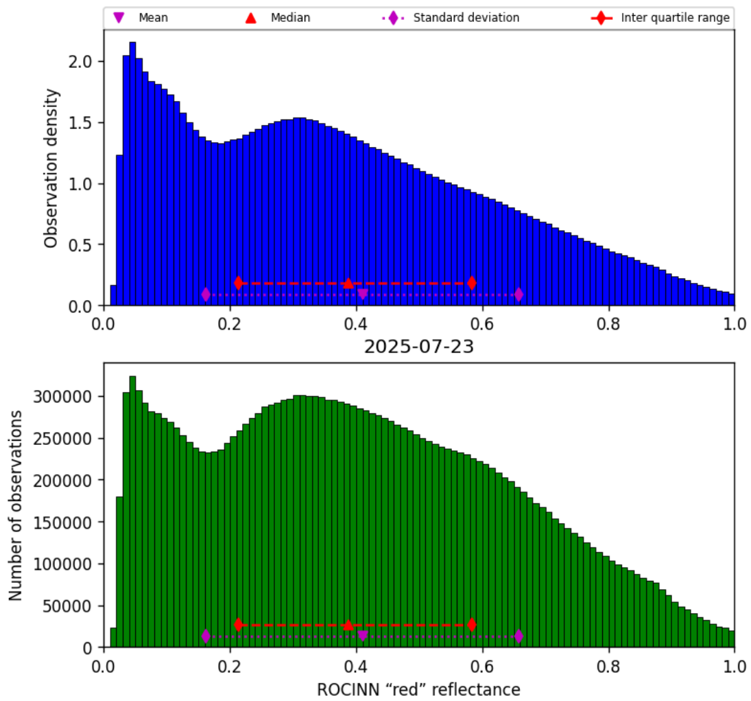
Figure 51: Histogram of “ROCINN “red” reflectance” for 2025-07-23 to 2025-07-24
