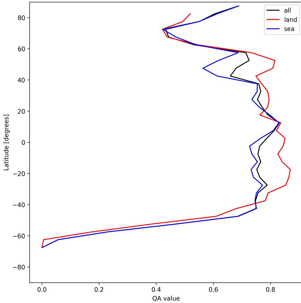
Figure 20: Zonal average of “QA value” for 2025-07-23 to 2025-07-24.
