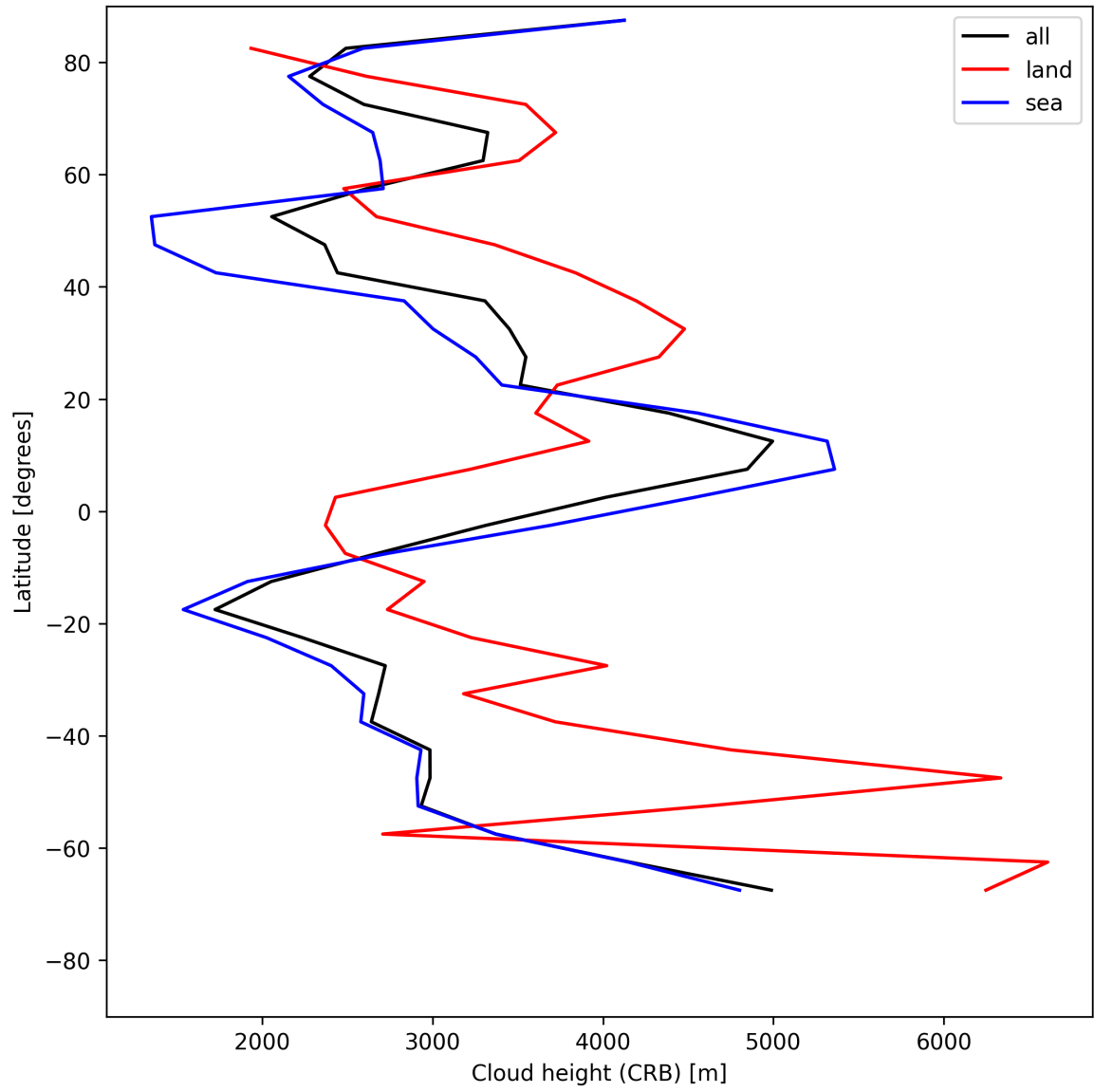
Figure 25: Zonal average of “Cloud height (CRB)” for 2025-07-23 to 2025-07-24.
