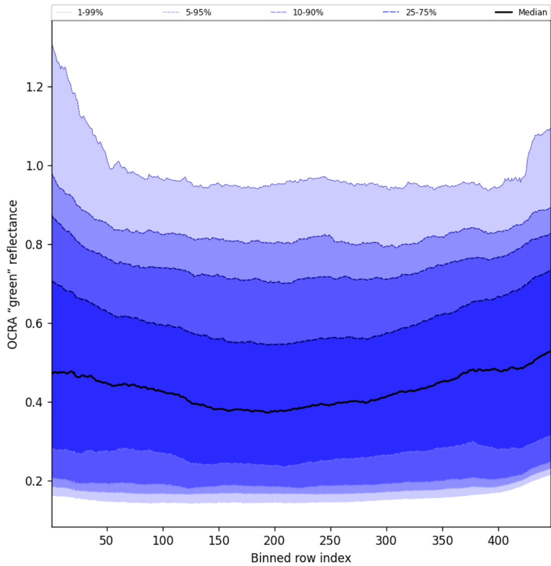
Figure 66: Along track statistics of “OCRA “green” reflectance” for 2025-07-23 to 2025-07-24
