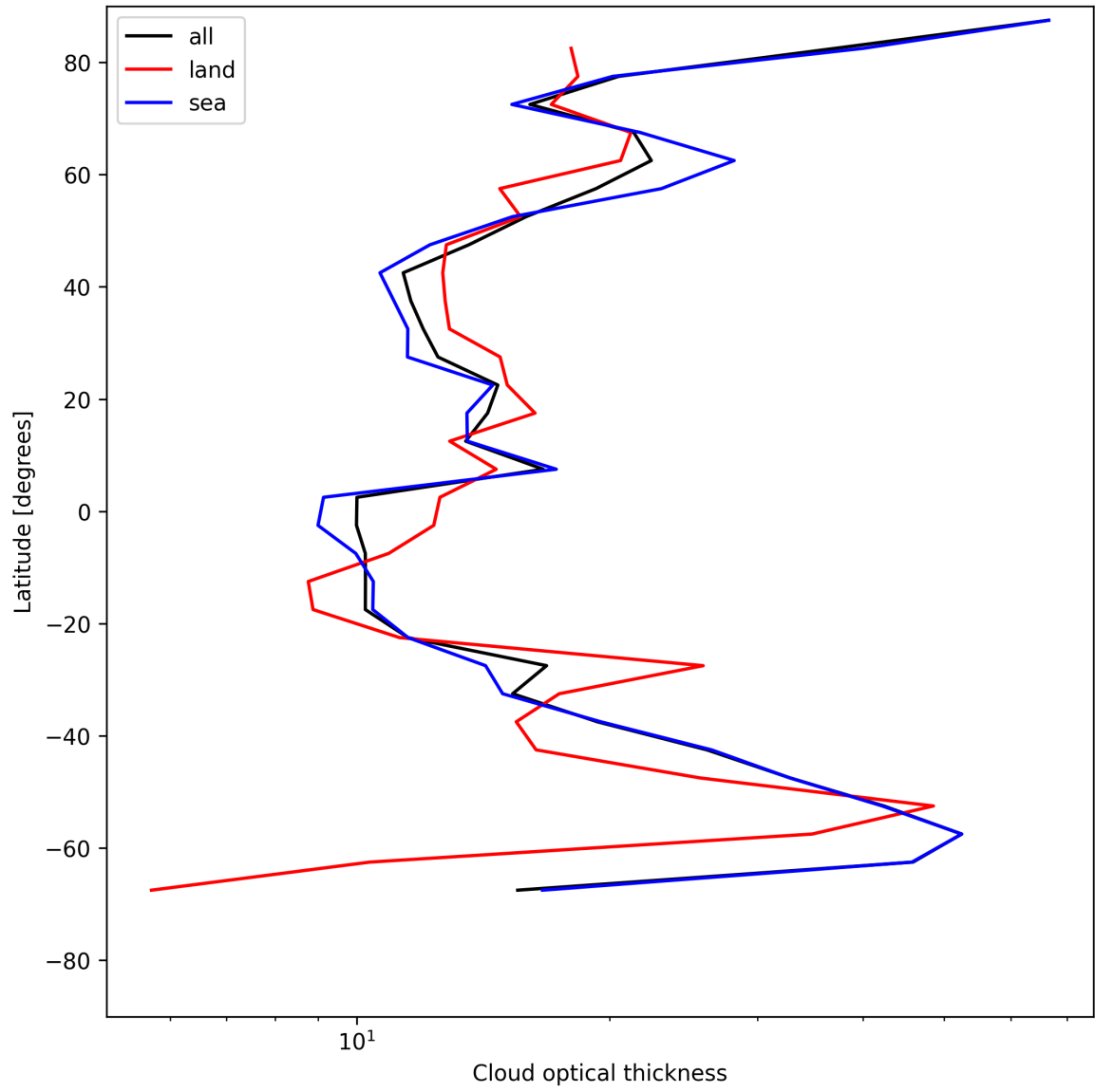
Figure 23: Zonal average of “Cloud optical thickness” for 2025-07-23 to 2025-07-24.
