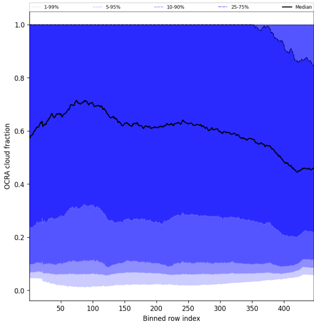
Figure 64: Along track statistics of “OCRA cloud fraction” for 2025-07-23 to 2025-07-24
