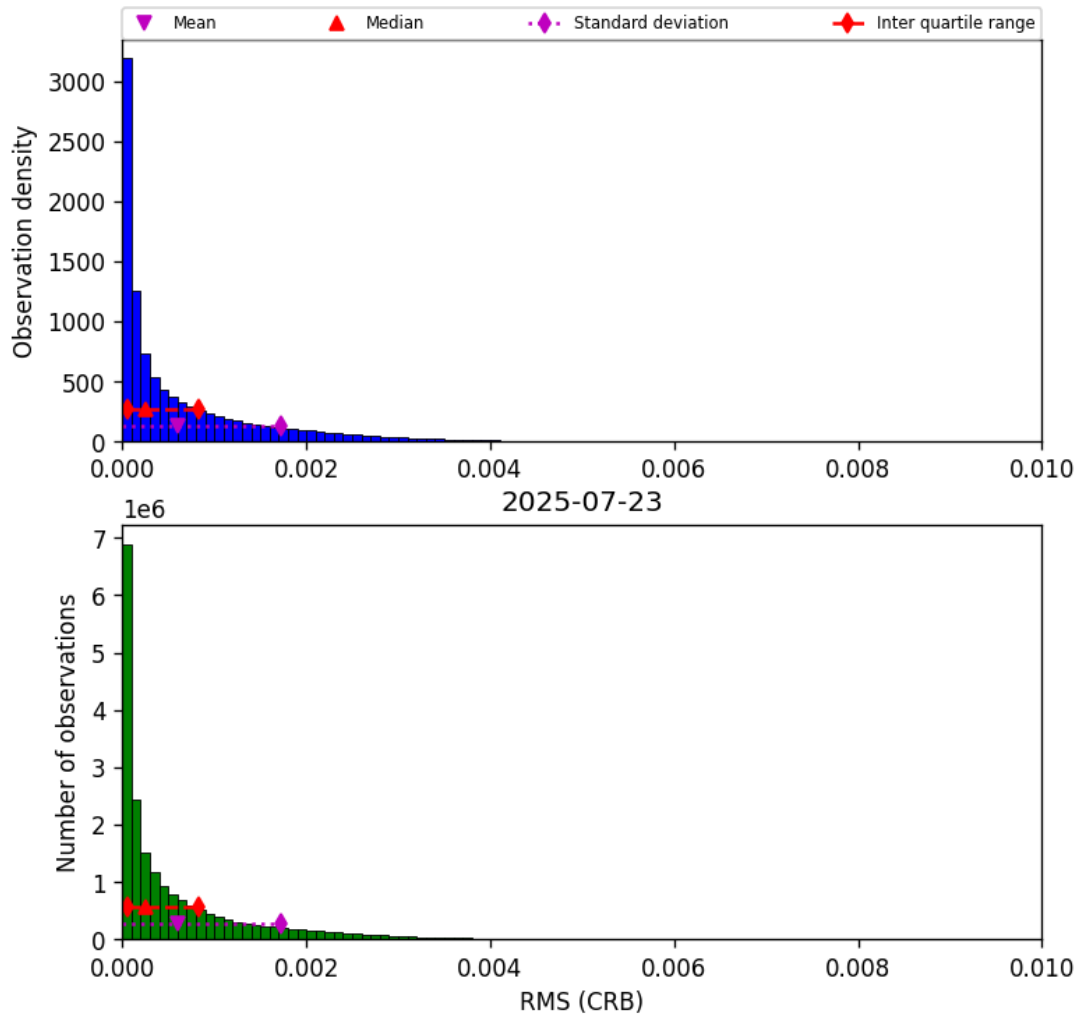
Figure 46: Histogram of “RMS (CRB)” for 2025-07-23 to 2025-07-24
