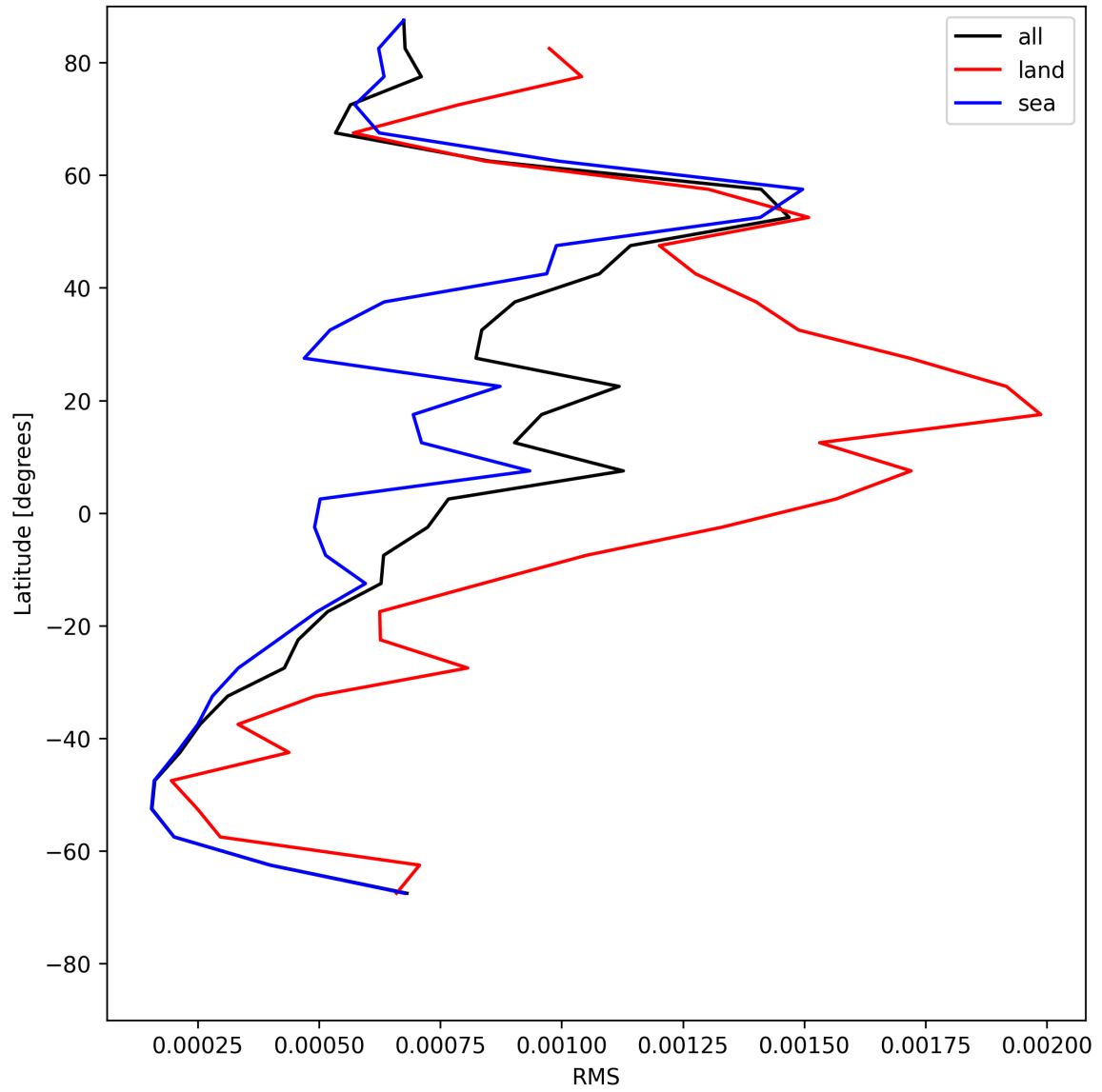
Figure 29: Zonal average of “RMS” for 2025-07-23 to 2025-07-24.
