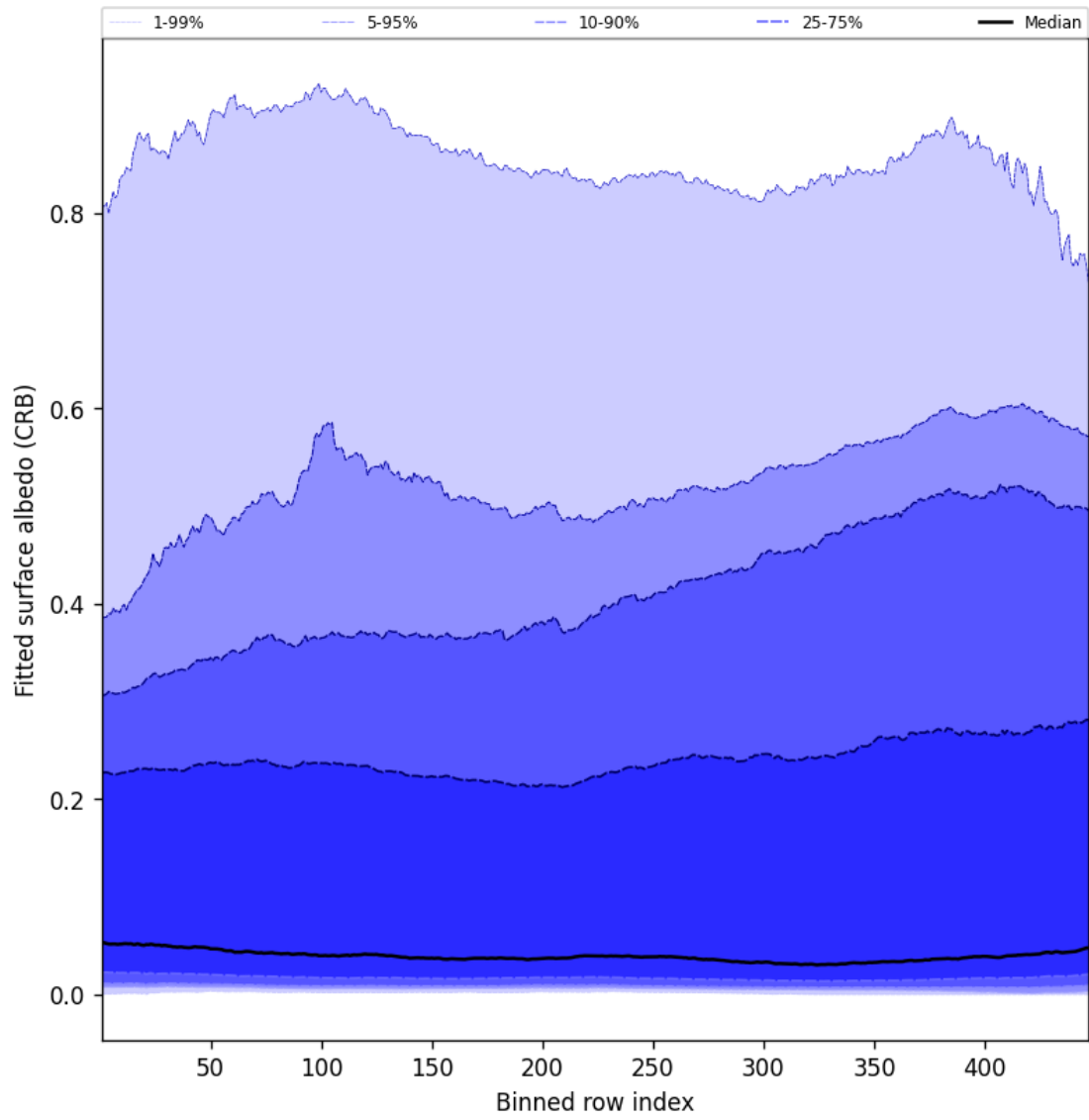
Figure 60: Along track statistics of “Fitted surface albedo (CRB)” for 2025-07-23 to 2025-07-24
