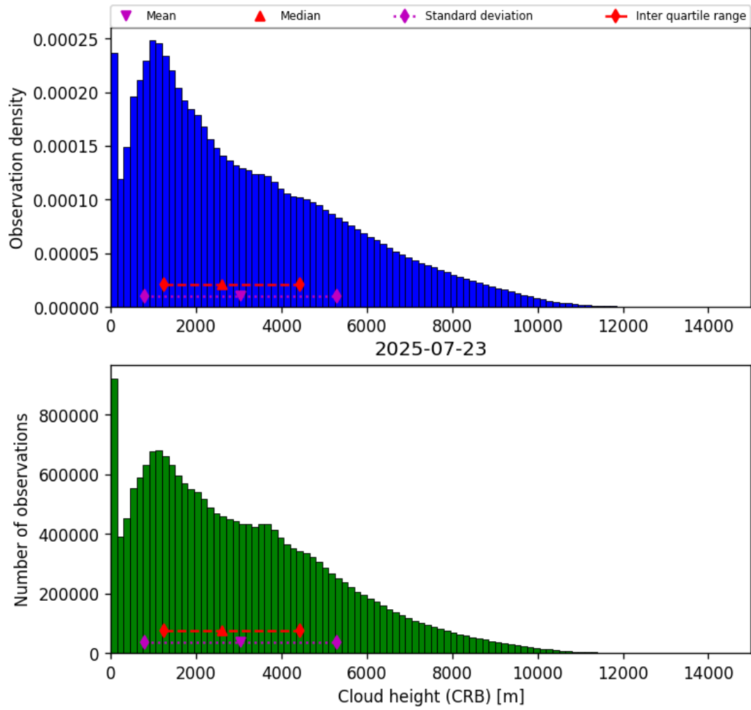
Figure 41: Histogram of “Cloud height (CRB)” for 2025-07-23 to 2025-07-24
