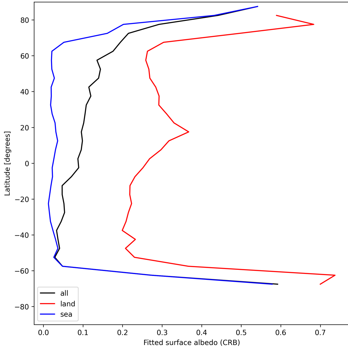
Figure 28: Zonal average of “Fitted surface albedo (CRB)” for 2025-07-23 to 2025-07-24.
