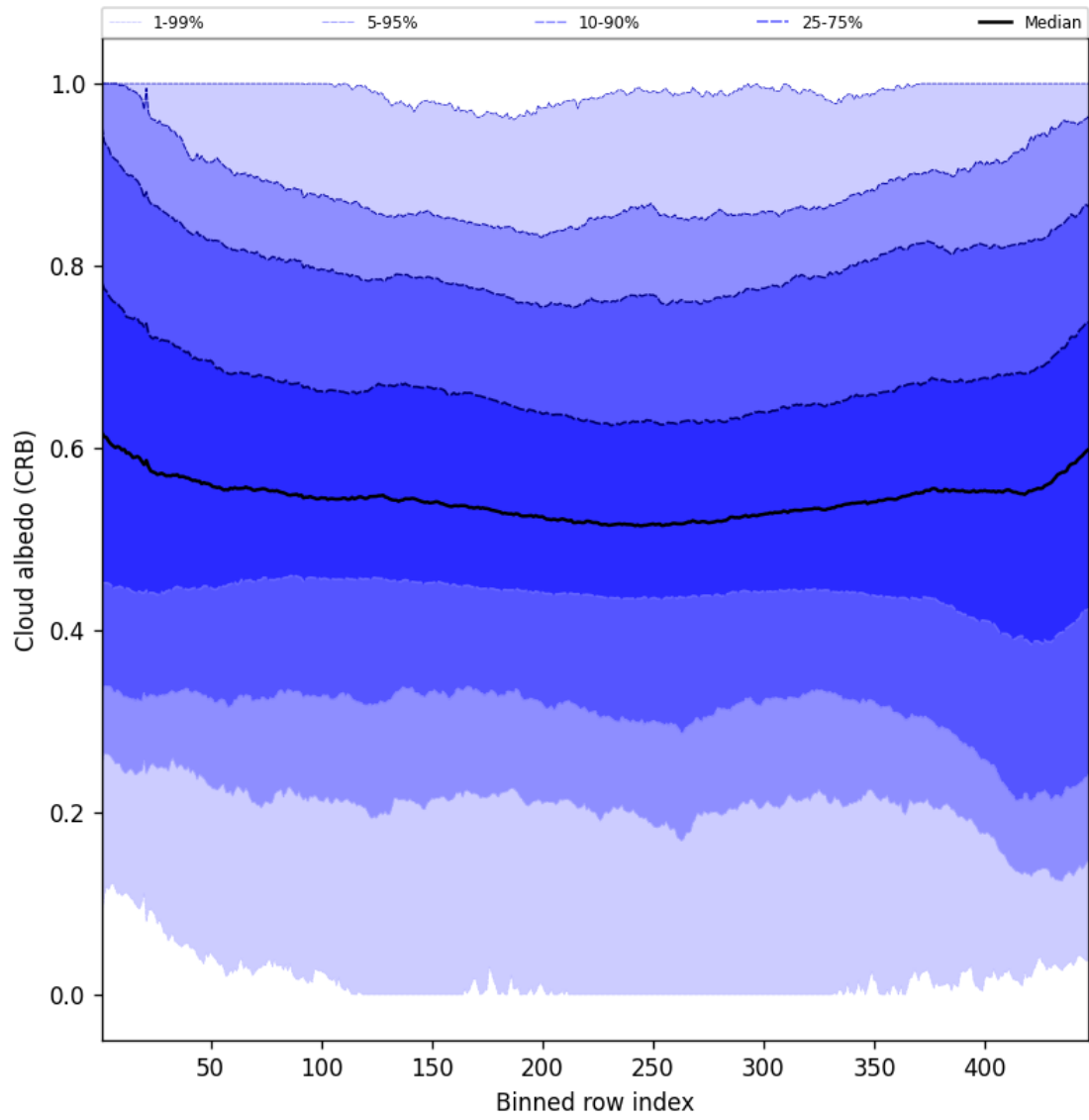
Figure 58: Along track statistics of “Cloud albedo (CRB)” for 2025-07-23 to 2025-07-24
