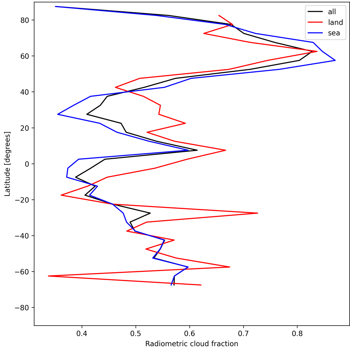
Figure 21: Zonal average of “Radiometric cloud fraction” for 2025-07-23 to 2025-07-24.
