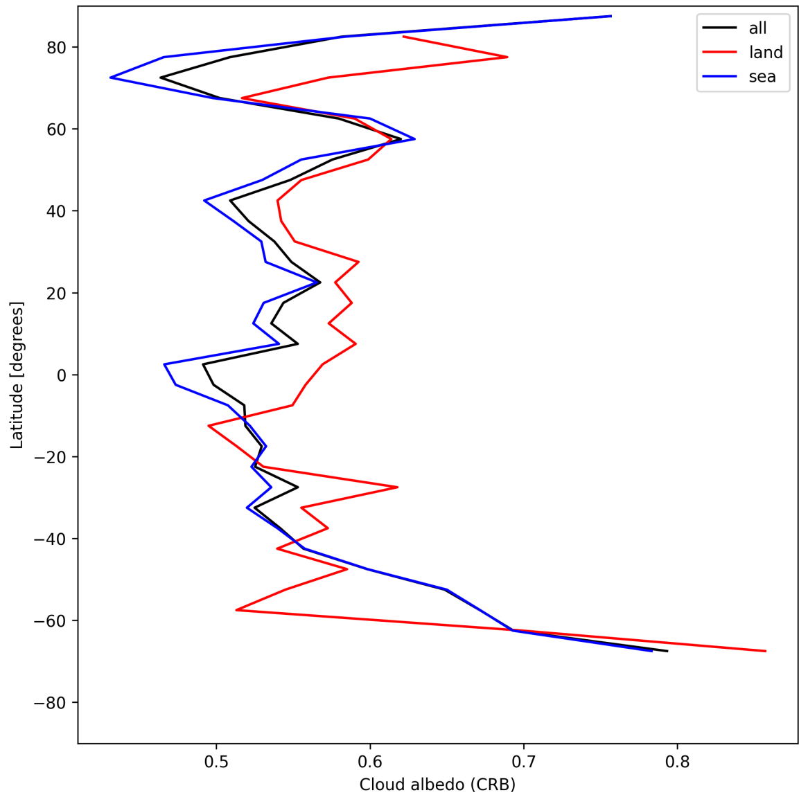
Figure 26: Zonal average of “Cloud albedo (CRB)” for 2025-07-23 to 2025-07-24.
