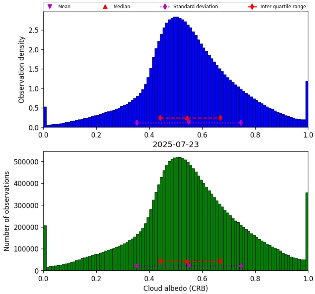
Figure 42: Histogram of “Cloud albedo (CRB)” for 2025-07-23 to 2025-07-24
