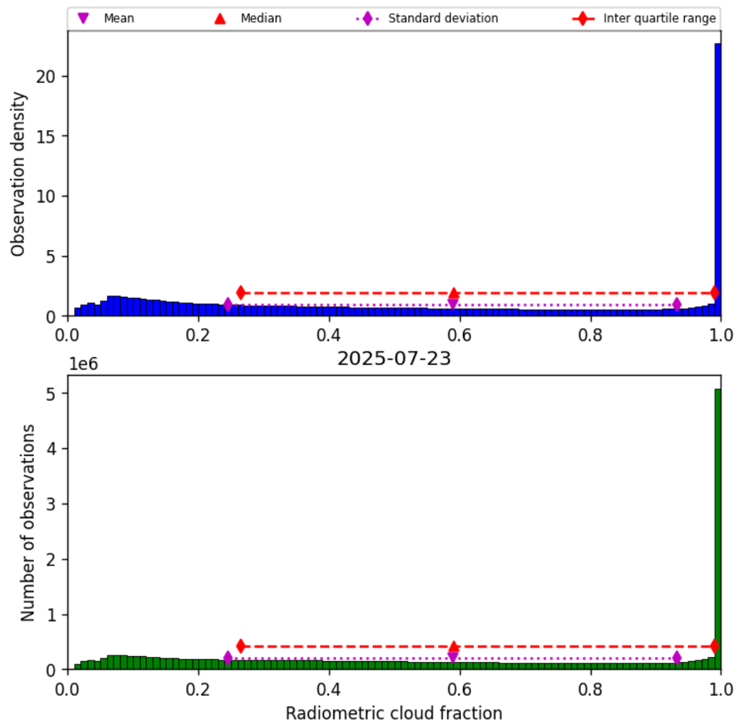
Figure 37: Histogram of “Radiometric cloud fraction” for 2025-07-23 to 2025-07-24
