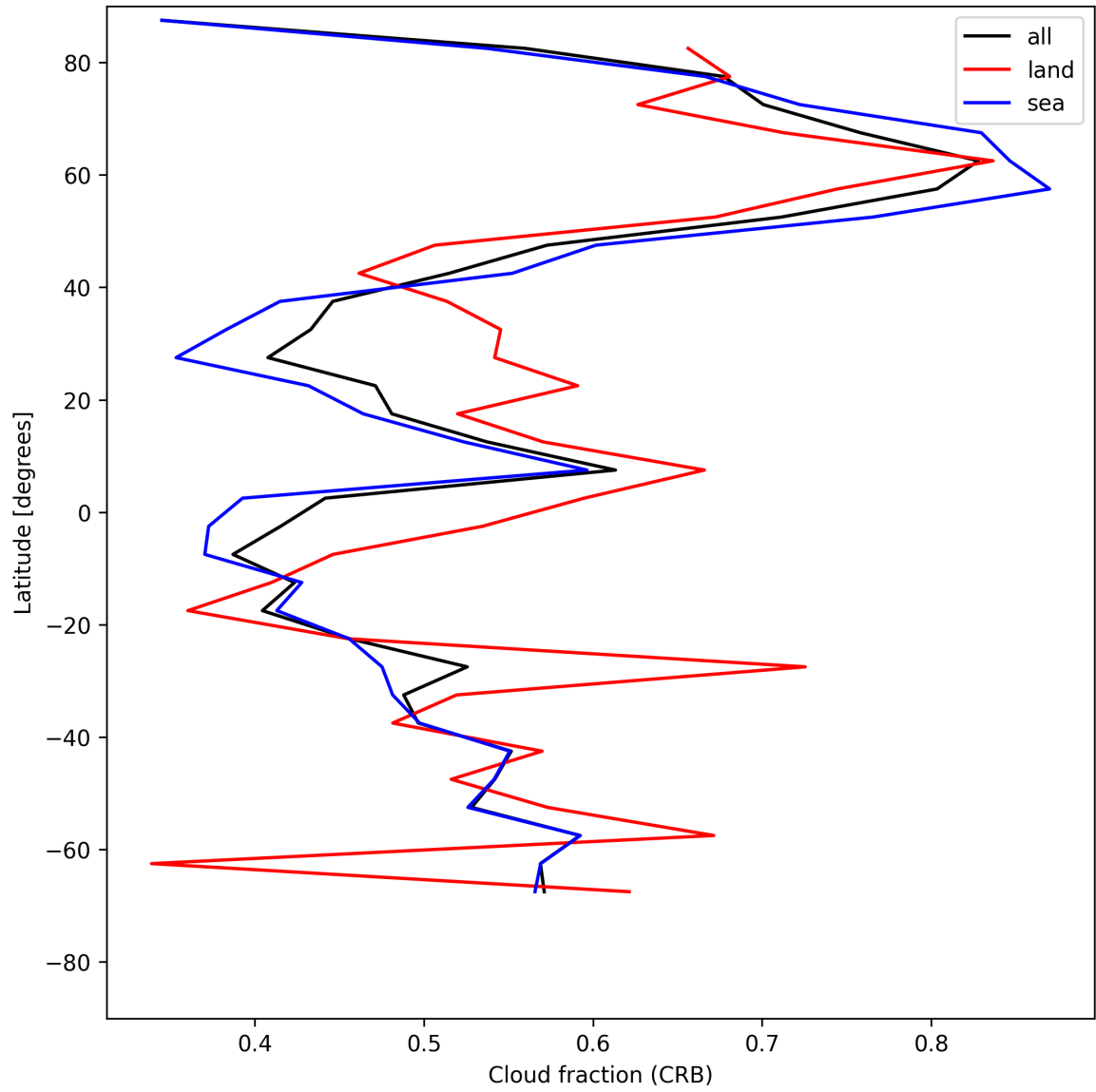
Figure 24: Zonal average of “Cloud fraction (CRB)” for 2025-07-23 to 2025-07-24.
