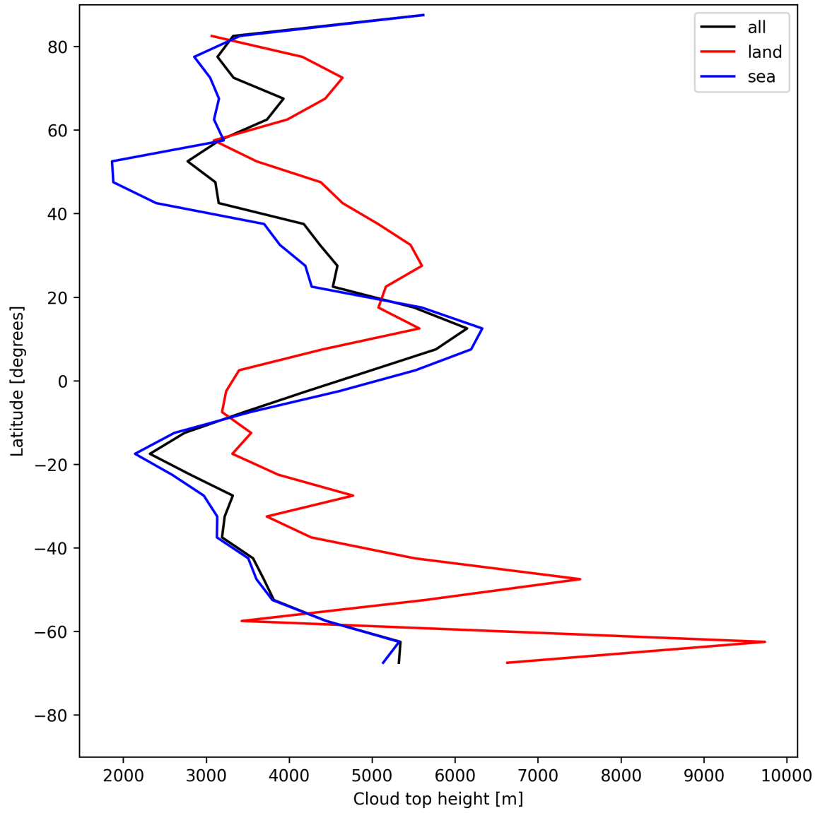
Figure 22: Zonal average of “Cloud top height” for 2025-07-23 to 2025-07-24.
