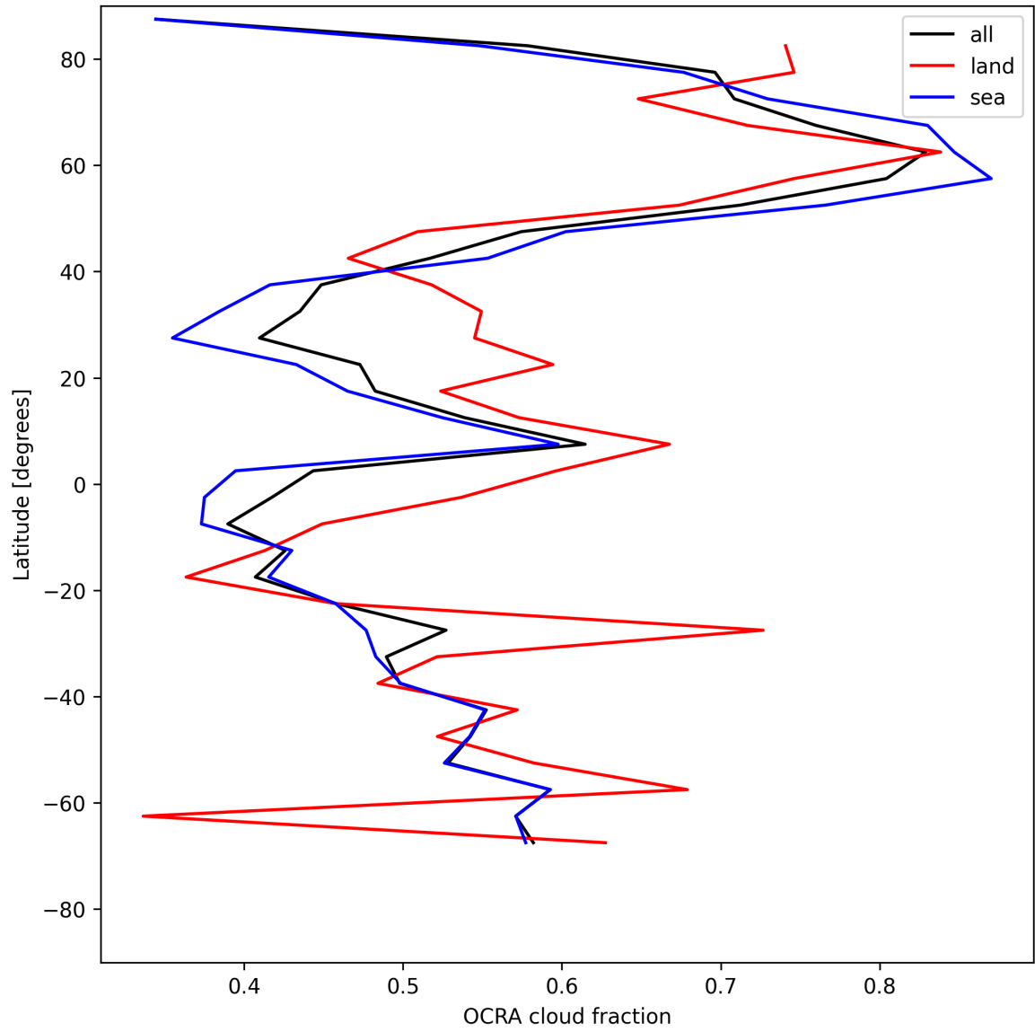
Figure 32: Zonal average of “OCRA cloud fraction” for 2025-07-23 to 2025-07-24.
