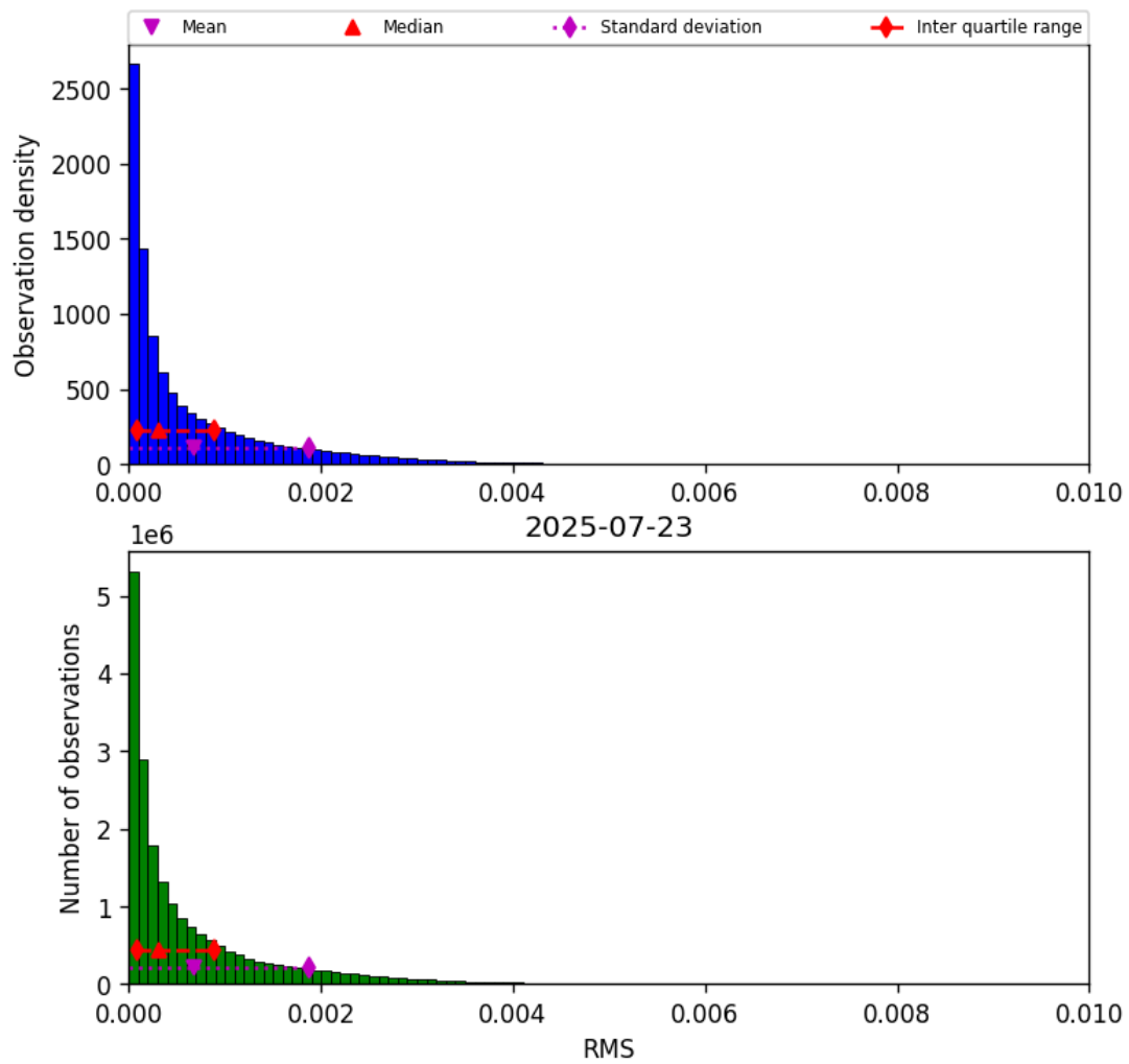
Figure 45: Histogram of “RMS” for 2025-07-23 to 2025-07-24
