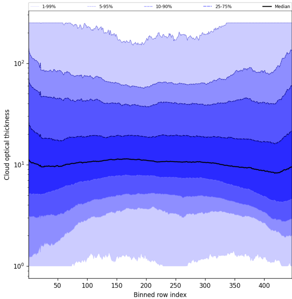
Figure 55: Along track statistics of “Cloud optical thickness” for 2025-07-23 to 2025-07-24
