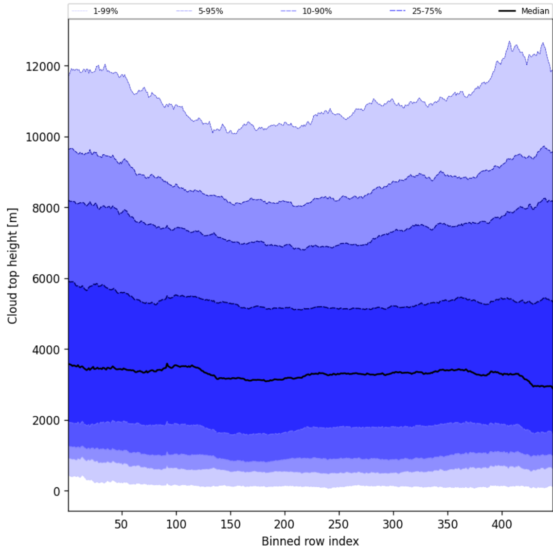
Figure 54: Along track statistics of “Cloud top height” for 2025-07-23 to 2025-07-24
