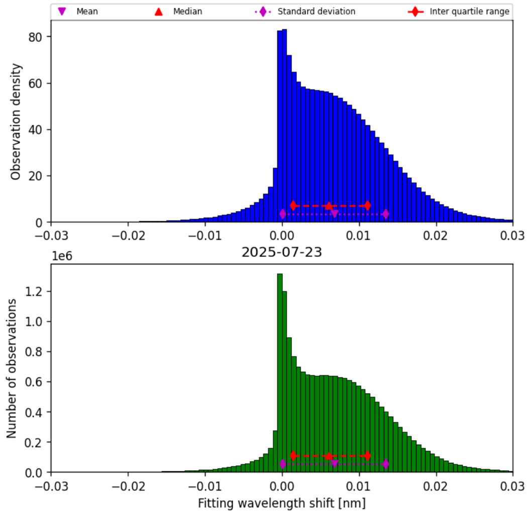
Figure 47: Histogram of “Fitting wavelength shift” for 2025-07-23 to 2025-07-24
