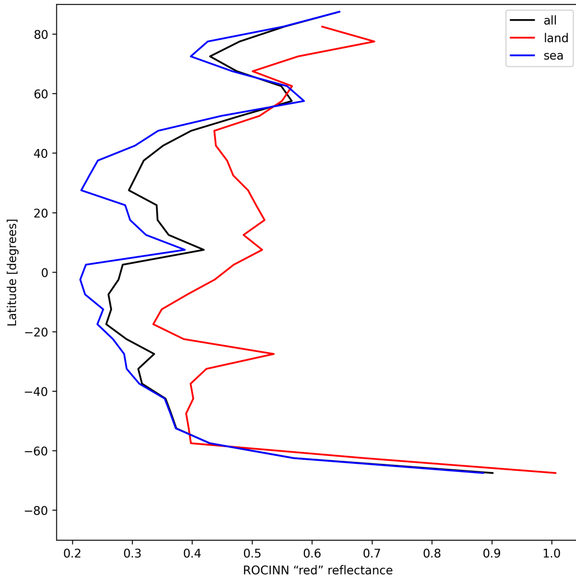
Figure 35: Zonal average of "ROCINN "red" reflectance" for 2025-07-23 to 2025-07-24.
