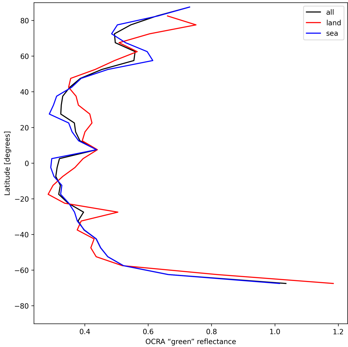
Figure 34: Zonal average of “OCRA “green” reflectance” for 2025-07-23 to 2025-07-24.
