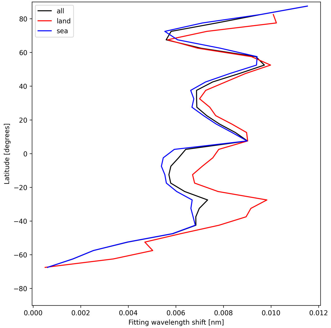
Figure 31: Zonal average of “Fitting wavelength shift” for 2025-07-23 to 2025-07-24.
