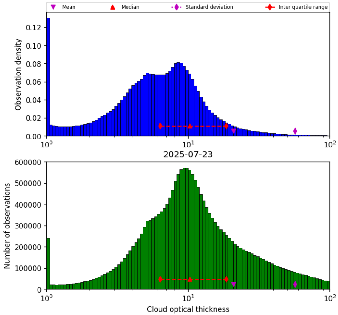
Figure 39: Histogram of “Cloud optical thickness” for 2025-07-23 to 2025-07-24
